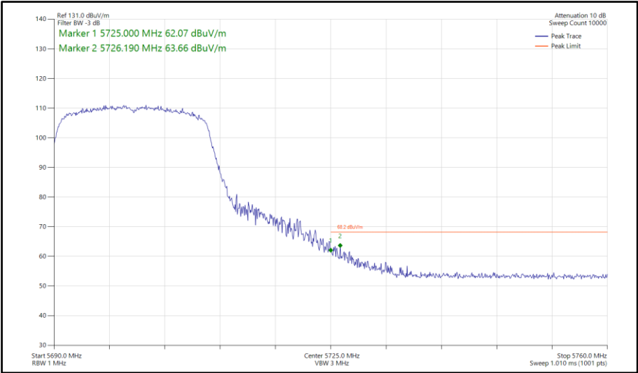
Figure 863 - 802.11ax HE20, SU, TxBF, Core 0-1 - 5700 MHz Band Edge Frequency 5725 MHz
