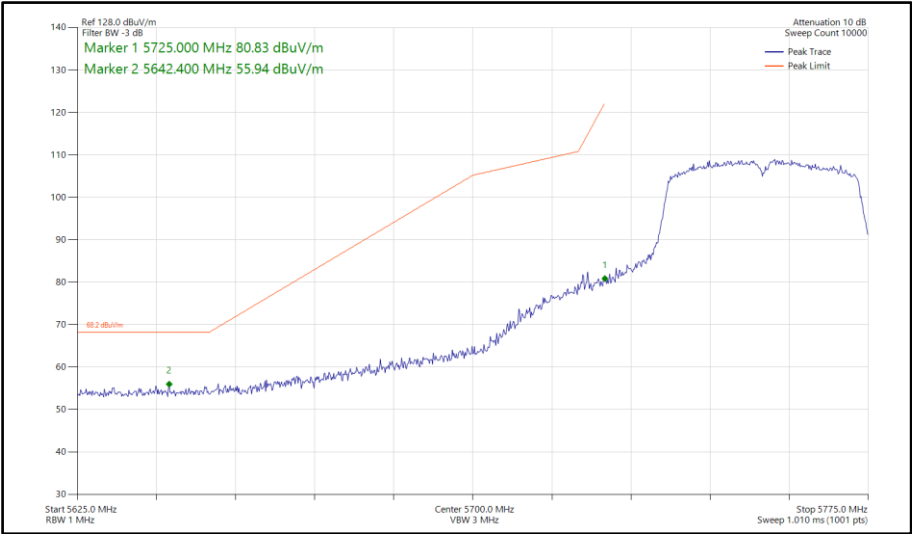
Figure 884 - 802.11n HT40, SISO, Core 0 - 5755 MHz Band Edge Frequency 5725 MHz
