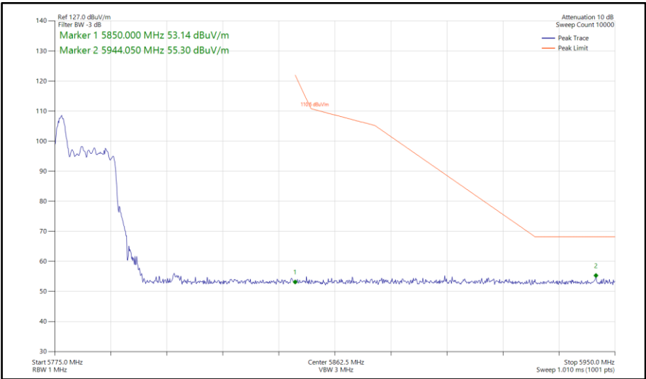
Figure 905 - 802.11ax HE40, RU 26-0, SISO, Core 0 - 5795 MHz Band Edge Frequency 5850 MHz
