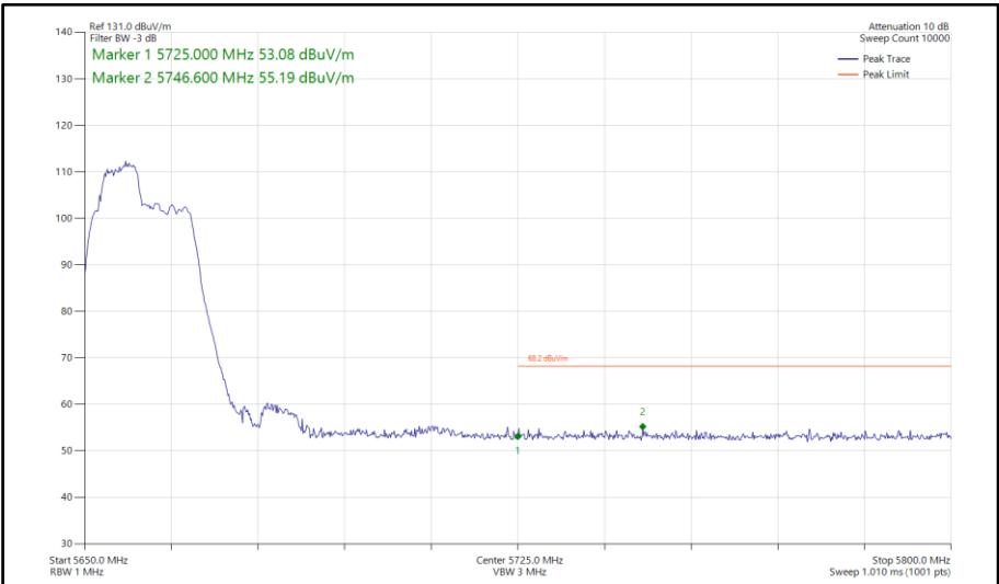
Figure 897 - 802.11be EHT40, RU 52+26-70, SISO, Core 0 - 5670 MHz Band Edge Frequency 5725 MHz
