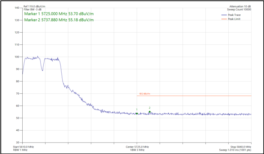
Figure 888 - 802.11a a40, SISO, Core 0 - 5630 MHz Band Edge Frequency 5725 MHz
