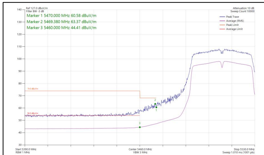
Figure 911 - 802.11n HT40, SISO, Core 1 - 5510 MHz Band Edge Frequency 5470 MHz
