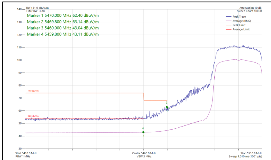
Figure 853 - 802.11ax HE20, SU, TxBF, Core 0-1 - 5500 MHz Band Edge Frequency 5470 MHz
