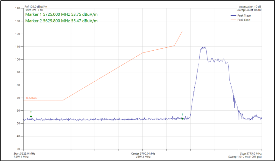
Figure 886 - 802.11ax HE40, RU 52-37, SISO, Core 0 - 5755 MHz Band Edge Frequency 5725 MHz
