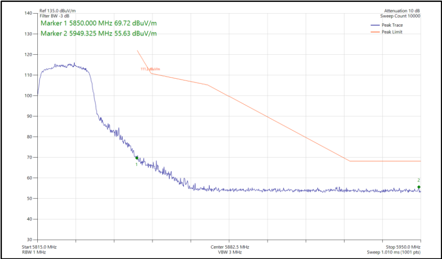
Figure 865 - 802.11ac VHT20, TxBF, Core 0-1 - 5825 MHz Band Edge Frequency 5850 MHz
