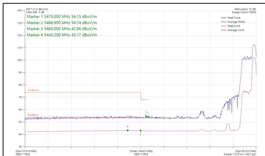
Figure 879 - 802.11ax HE40, RU 52-44, SISO, Core 0 - 5590 MHz Band Edge Frequency 5470 MHz
