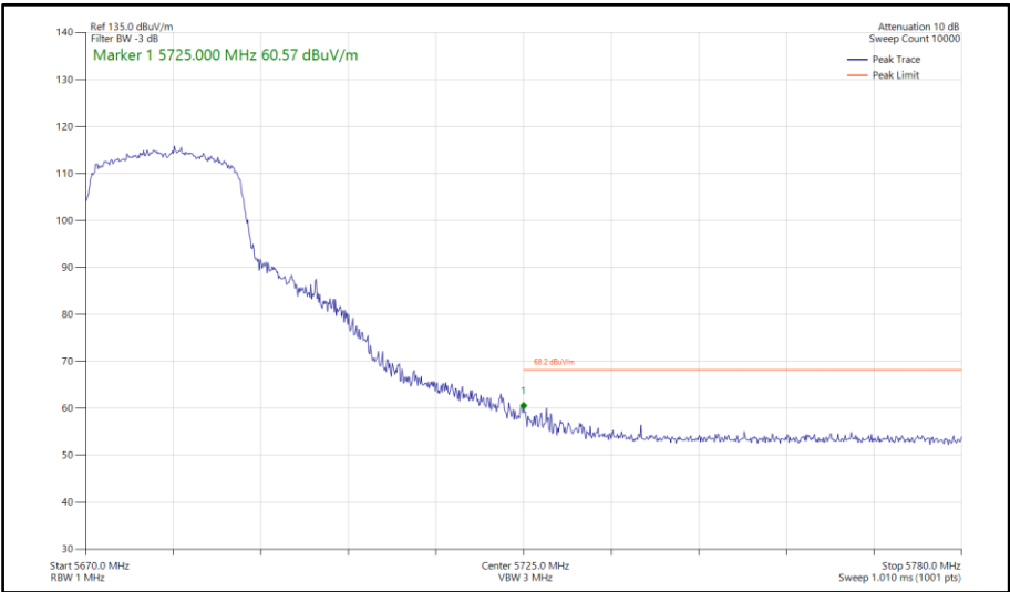
Figure 862 - 802.11ax HE20, SU, TxBF, Core 0-1 - 5680 MHz Band Edge Frequency 5725 MHz
