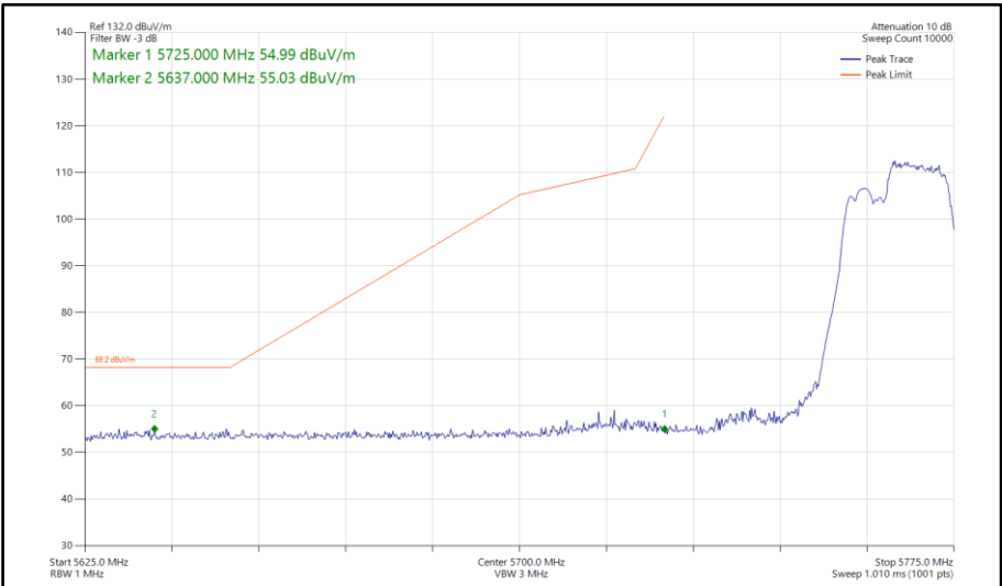
Figure 927 - 802.11be EHT40, RU 106+26-85, SISO, Core 1 - 5755 MHz Band Edge Frequency 5725 MHz
