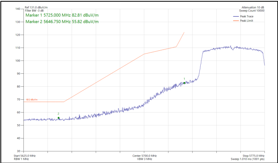
Figure 925 - 802.11ax HE40, SU, SISO, Core 1 - 5755 MHz Band Edge Frequency 5725 MHz
