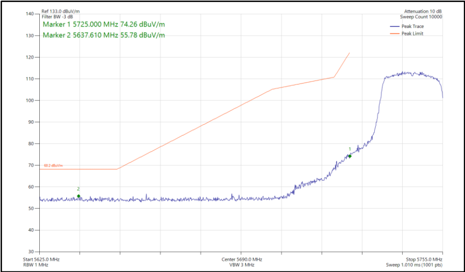
Figure 857 - 802.11ax HE20, SU, TxBF, Core 0-1 - 5745 MHz Band Edge Frequency 5725 MHz
