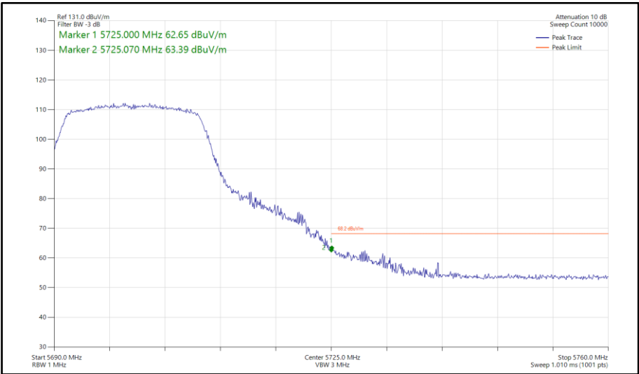
Figure 860 - 802.11ac VHT20, TxBF, Core 0-1 - 5700 MHz Band Edge Frequency 5725 MHz
