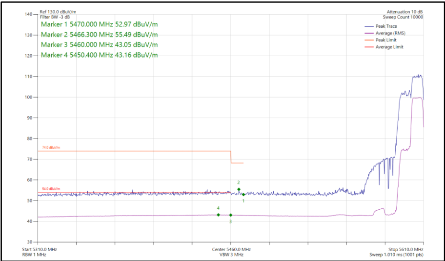
Figure 919 - 802.11ax HE40, RU 106-56, SISO, Core 1 - 5590 MHz Band Edge Frequency 5470 MHz
