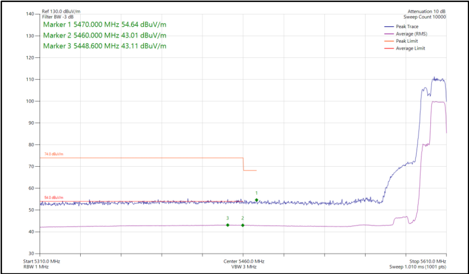
Figure 922 - 802.11be EHT40, RU 106+26-85, SISO, Core 1 - 5590 MHz Band Edge Frequency 5470 MHz
