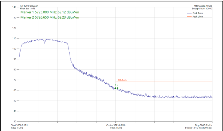
Figure 891 - 802.11n HT40, SISO, Core 0 - 5670 MHz Band Edge Frequency 5725 MHz
