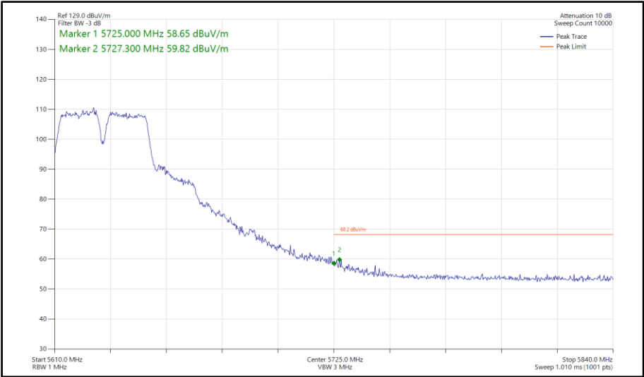
Figure 928 - 802.11a a40, SISO, Core 1 - 5630 MHz Band Edge Frequency 5725 MHz
