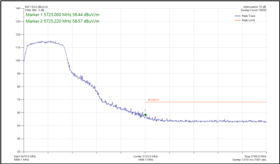
Figure 859 - 802.11ac VHT20, TxBF, Core 0-1 - 5680 MHz Band Edge Frequency 5725 MHz
