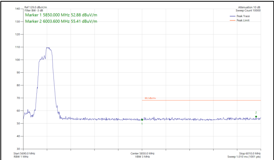
Figure 903 - 802.11ax HE40, RU 106-56, SISO, Core 0 - 5710 MHz Band Edge Frequency 5850 MHz
