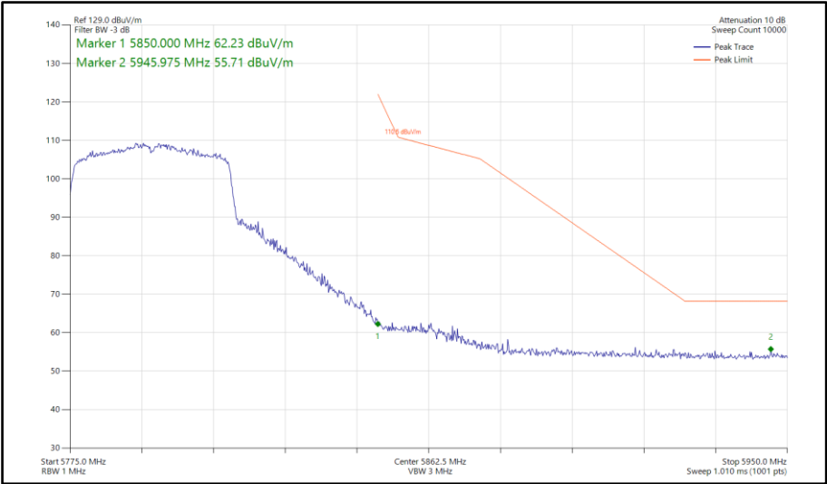
Figure 904 - 802.11ax HE40, SU, SISO, Core 0 - 5795 MHz Band Edge Frequency 5850 MHz
