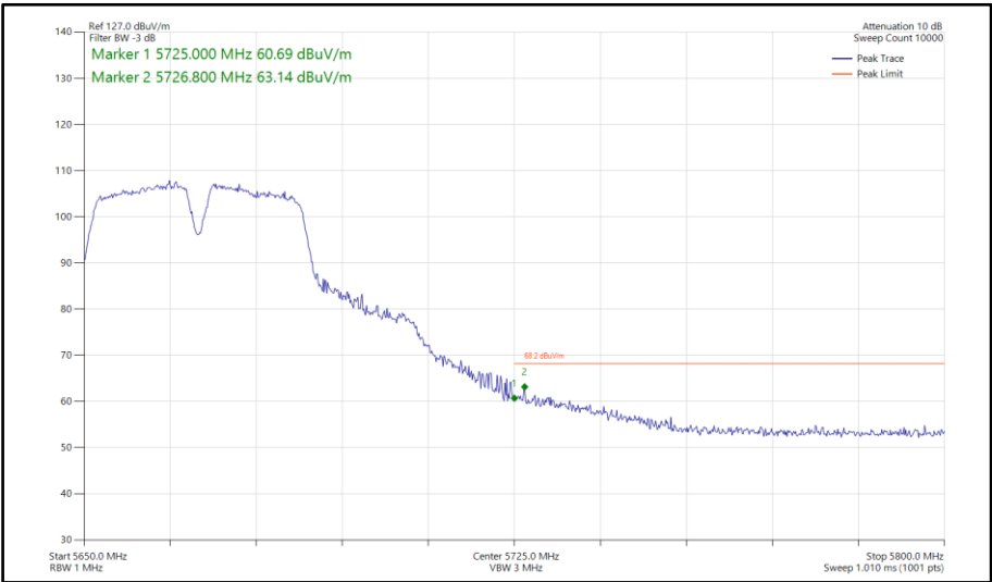
Figure 929 - 802.11a a40, SISO, Core 1 - 5670 MHz Band Edge Frequency 5725 MHz
