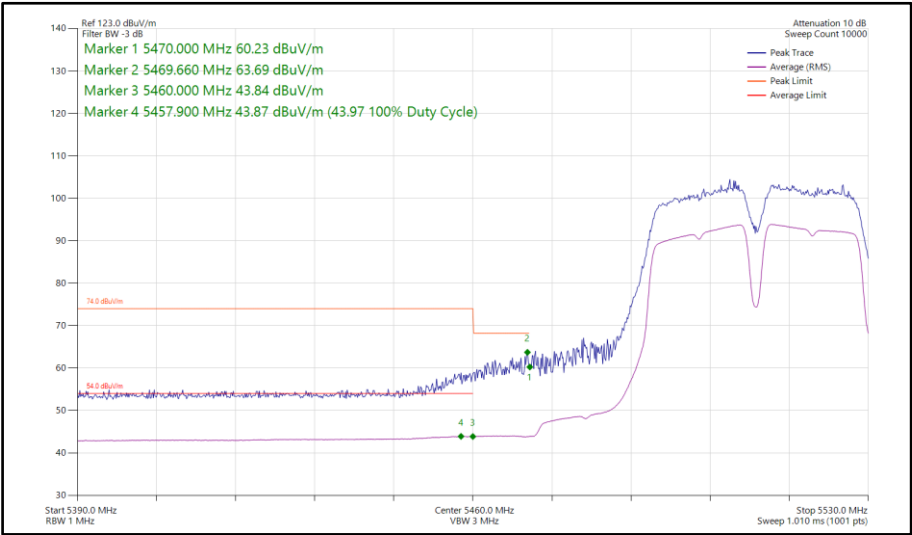
Figure 868 - 802.11a a40, SISO, Core 0 - 5510 MHz Band Edge Frequency 5470 MHz
