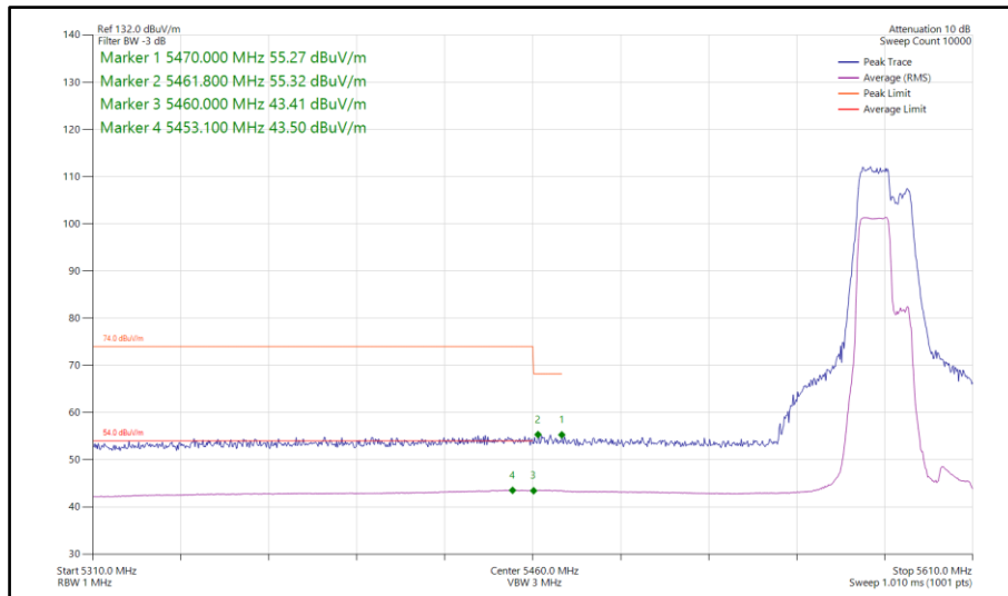
Figure 882 - 802.11be EHT40, RU 106+26-82, SISO, Core 0 - 5590 MHz Band Edge Frequency 5470 MHz
