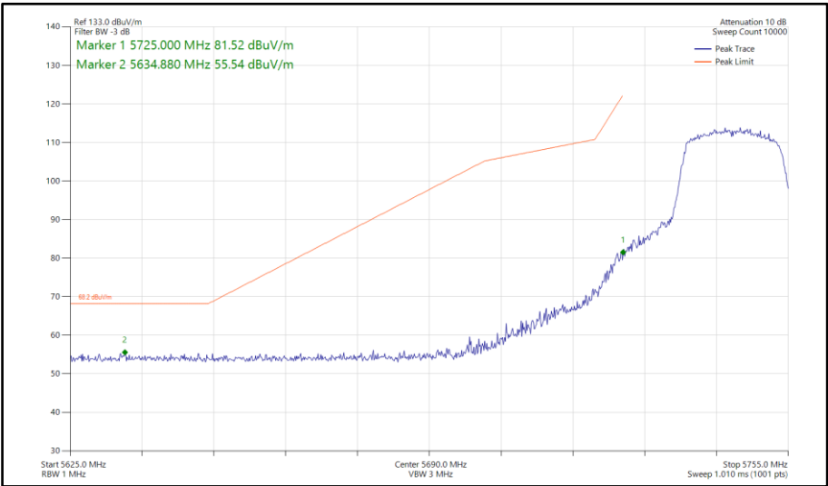
Figure 856 - 802.11ac VHT20, TxBF, Core 0-1 - 5745 MHz Band Edge Frequency 5725 MHz
