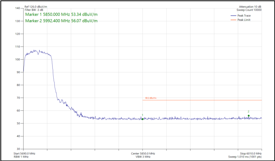
Figure 900 - 802.11n HT40, SISO, Core 0 - 5710 MHz Band Edge Frequency 5850 MHz
