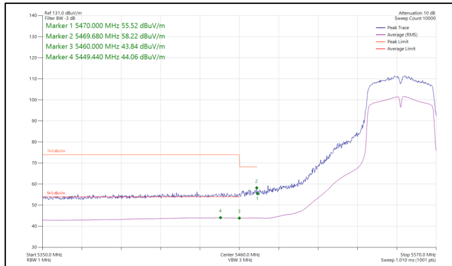
Figure 872 - 802.11n HT40, SISO, Core 0 - 5550 MHz Band Edge Frequency 5470 MHz
