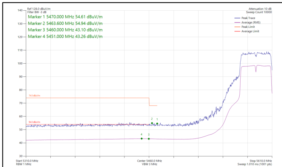
Figure 913 - 802.11n HT40, SISO, Core 1 - 5590 MHz Band Edge Frequency 5470 MHz
