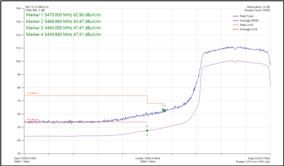
Figure 874 - 802.11ax HE40, SU, SISO, Core 0 - 5510 MHz Band Edge Frequency 5470 MHz
