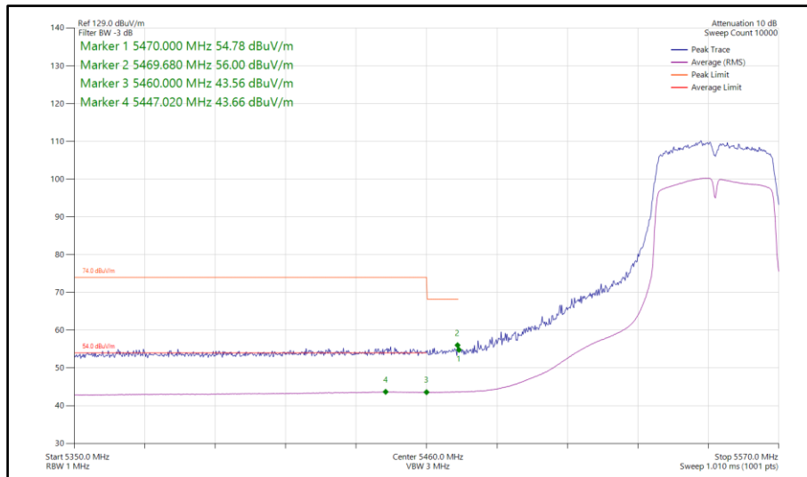
Figure 912 - 802.11n HT40, SISO, Core 1 - 5550 MHz Band Edge Frequency 5470 MHz
