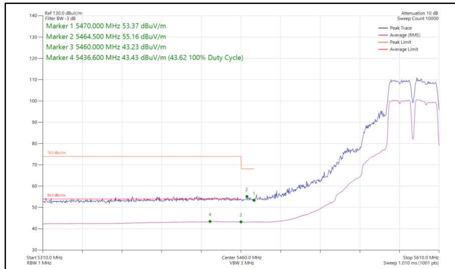
Figure 870 - 802.11a a40, SISO, Core 0 - 5590 MHz Band Edge Frequency 5470 MHz
