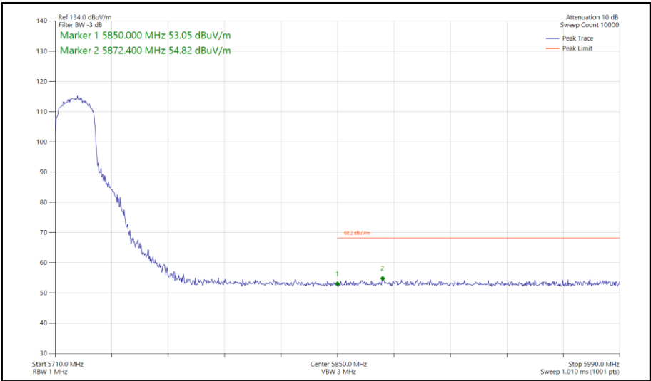
Figure 866 - 802.11ax HE20, SU, TxBF, Core 0-1 - 5720 MHz Band Edge Frequency 5850 MHz
