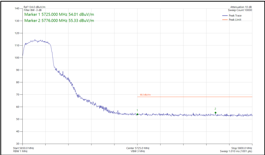
Figure 858 - 802.11ac VHT20, TxBF, Core 0-1 - 5660 MHz Band Edge Frequency 5725 MHz
