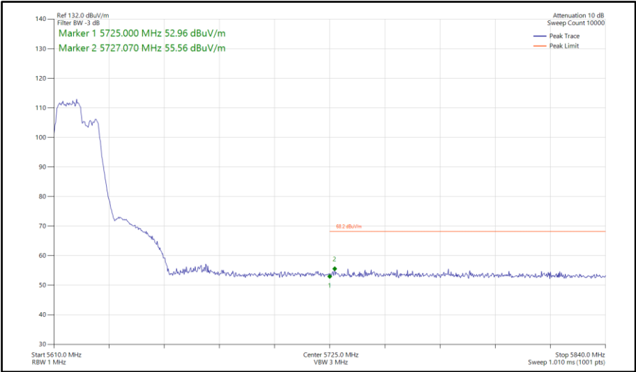
Figure 896 - 802.11be EHT40, RU 106+26-82, SISO, Core 0 - 5630 MHz Band Edge Frequency 5725 MHz
