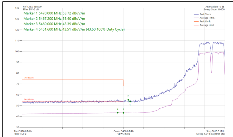
Figure 910 - 802.11a a40, SISO, Core 1 - 5590 MHz Band Edge Frequency 5470 MHz
