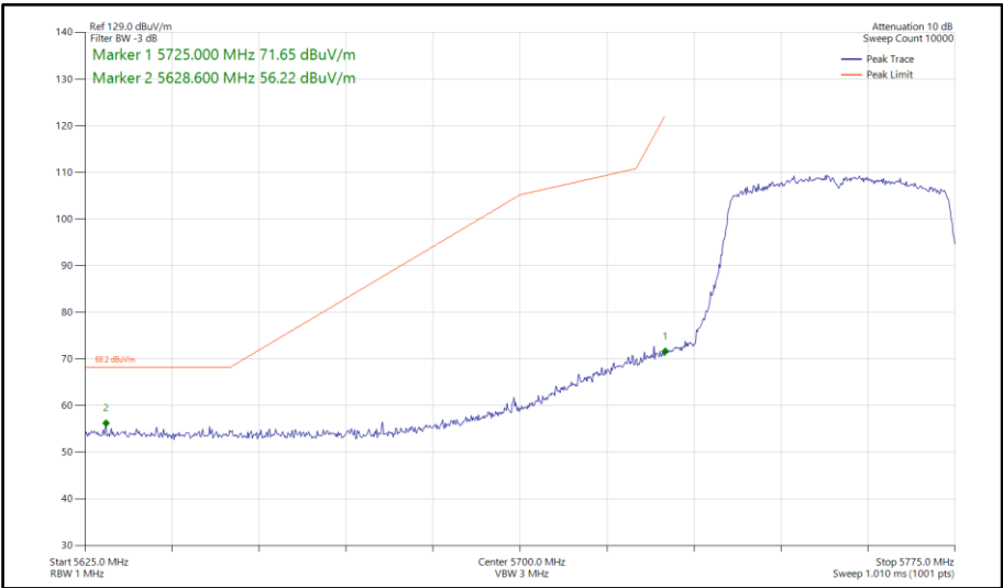
Figure 885 - 802.11ax HE40, SU, SISO, Core 0 - 5755 MHz Band Edge Frequency 5725 MHz
