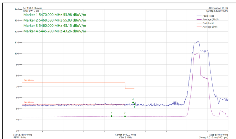
Figure 881 - 802.11be EHT40, RU 52+26-70, SISO, Core 0 - 5550 MHz Band Edge Frequency 5470 MHz
