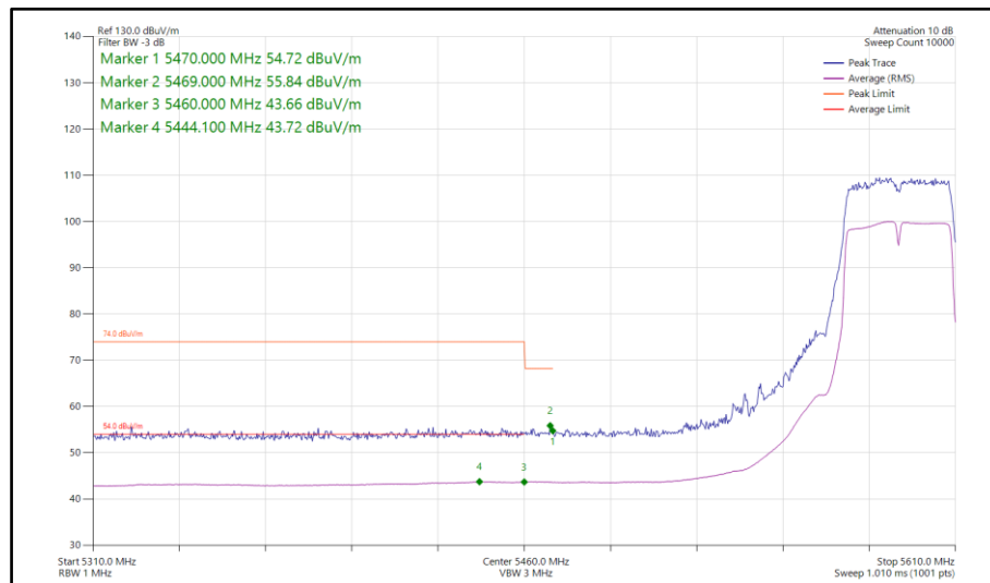
Figure 873 - 802.11n HT40, SISO, Core 0 - 5590 MHz Band Edge Frequency 5470 MHz
