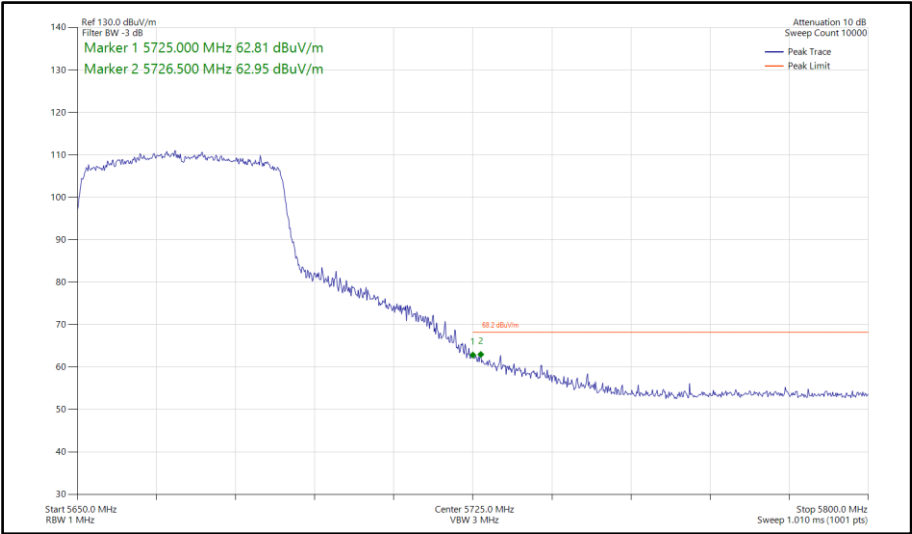
Figure 894 - 802.11ax HE40, SU, SISO, Core 0 - 5670 MHz Band Edge Frequency 5725 MHz
