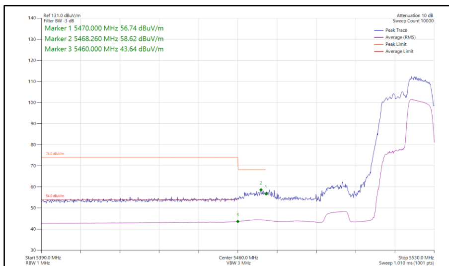
Figure 915 - 802.11ax HE40, RU 106-56, SISO, Core 1 - 5510 MHz Band Edge Frequency 5470 MHz
