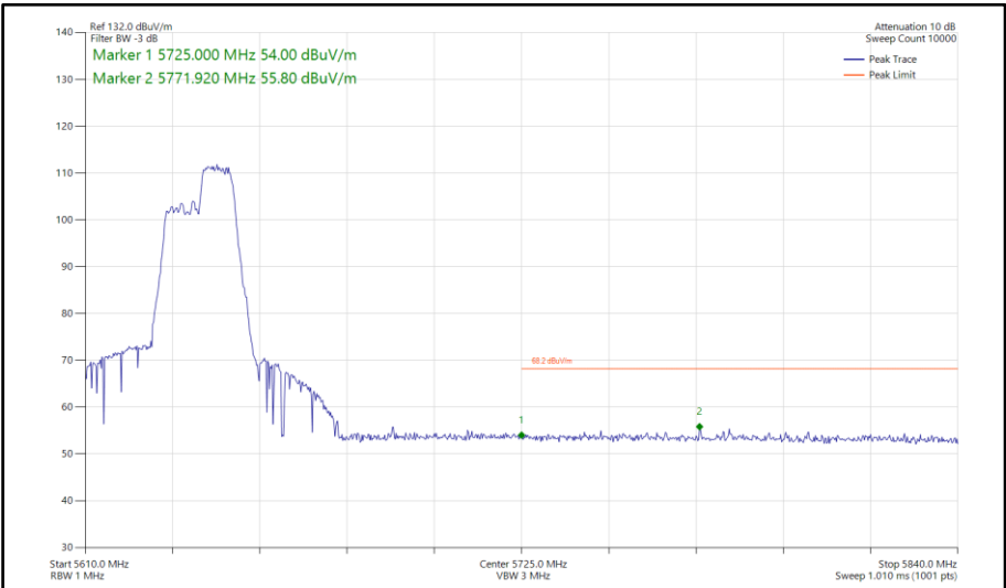
Figure 893 - 802.11ax HE40, RU 106-56, SISO, Core 0 - 5630 MHz Band Edge Frequency 5725 MHz
