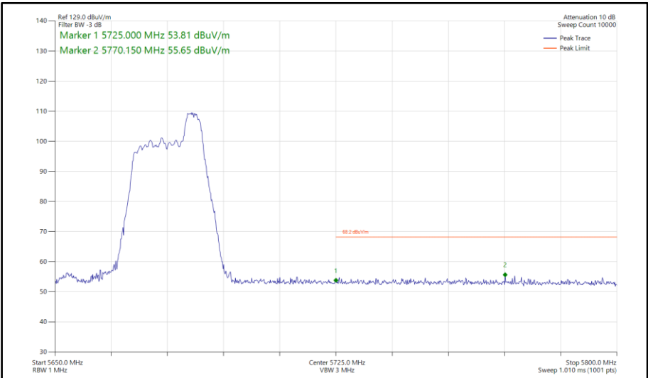
Figure 895 - 802.11ax HE40, RU 52-44, SISO, Core 0 - 5670 MHz Band Edge Frequency 5725 MHz
