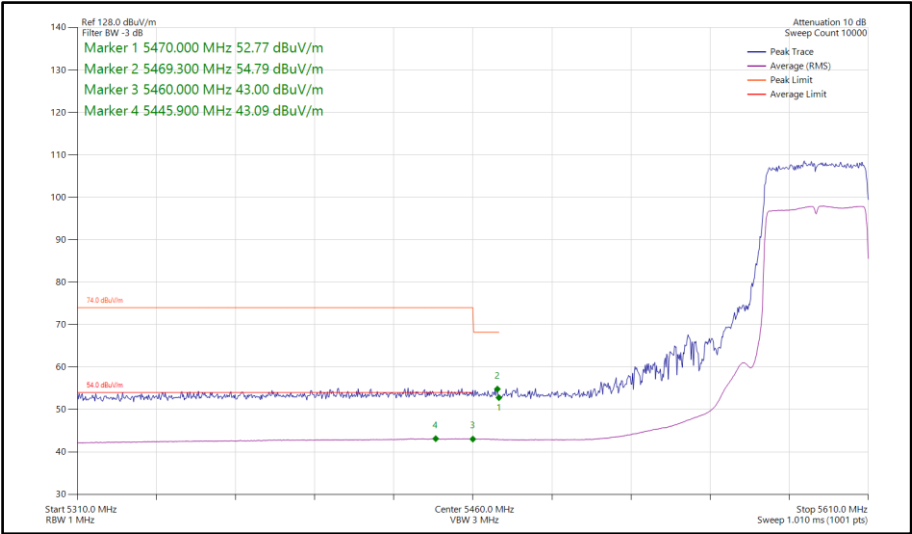
Figure 918 - 802.11ax HE40, SU, SISO, Core 1 - 5590 MHz Band Edge Frequency 5470 MHz
