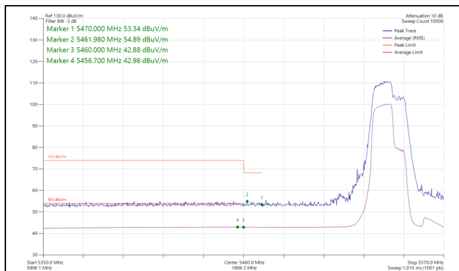
Figure 921 - 802.11be EHT40, RU 106+26-82, SISO, Core 1 - 5550 MHz Band Edge Frequency 5470 MHz
