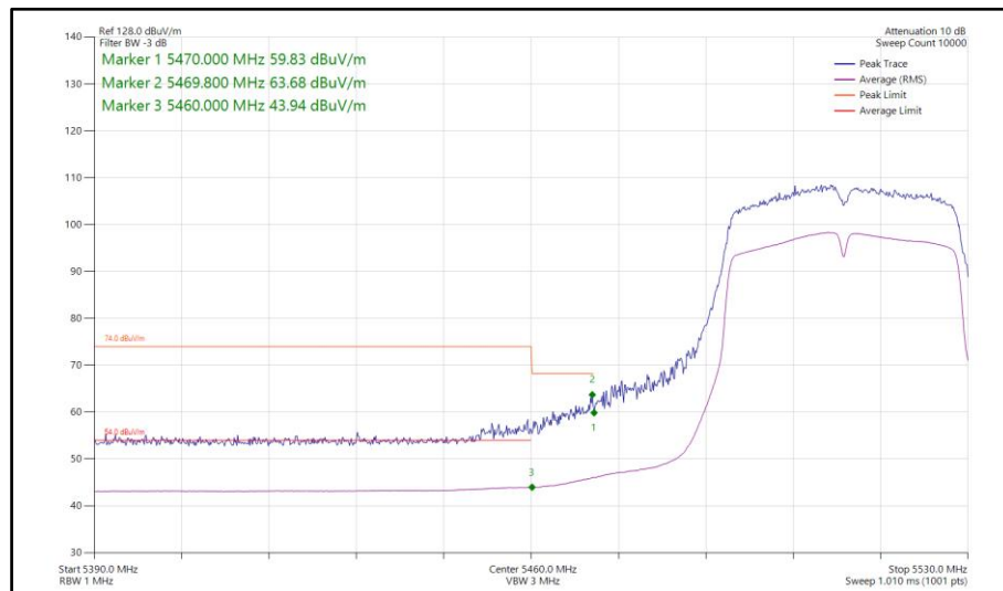
Figure 871 - 802.11n HT40, SISO, Core 0 - 5510 MHz Band Edge Frequency 5470 MHz
