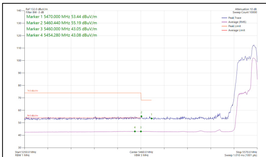
Figure 877 - 802.11ax HE40, RU 52-44, SISO, Core 0 - 5550 MHz Band Edge Frequency 5470 MHz
