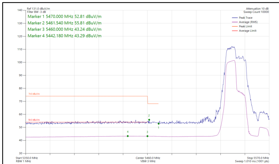
Figure 917 - 802.11ax HE40, RU 106-53, SISO, Core 1 - 5550 MHz Band Edge Frequency 5470 MHz
