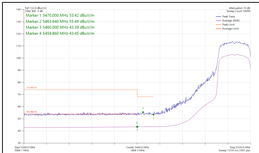
Figure 854 - 802.11ax HE20, SU, TxBF, Core 0-1 - 5520 MHz Band Edge Frequency 5470 MHz
