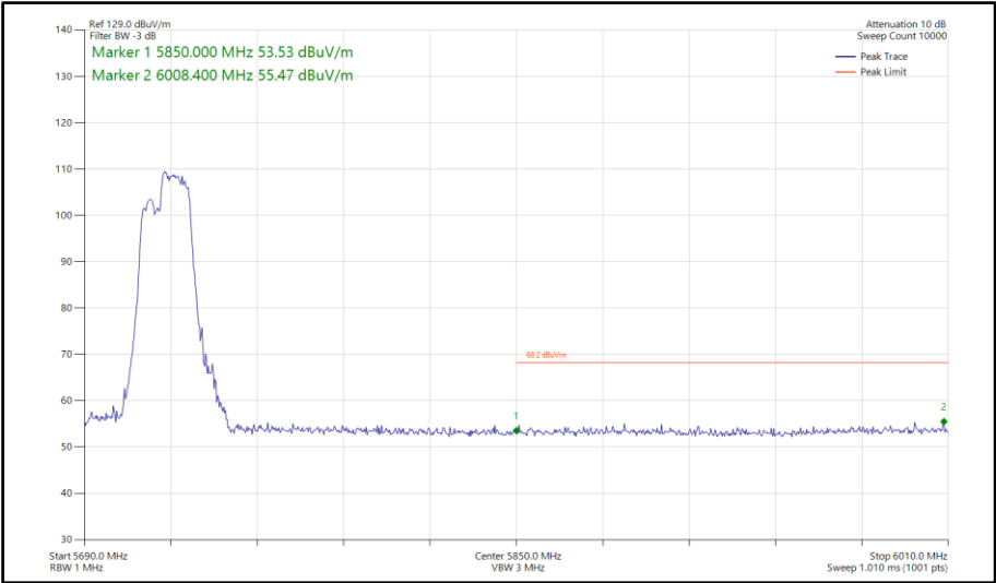
Figure 906 - 802.11be EHT40, RU 106+26-85, SISO, Core 0 - 5710 MHz Band Edge Frequency 5850 MHz
