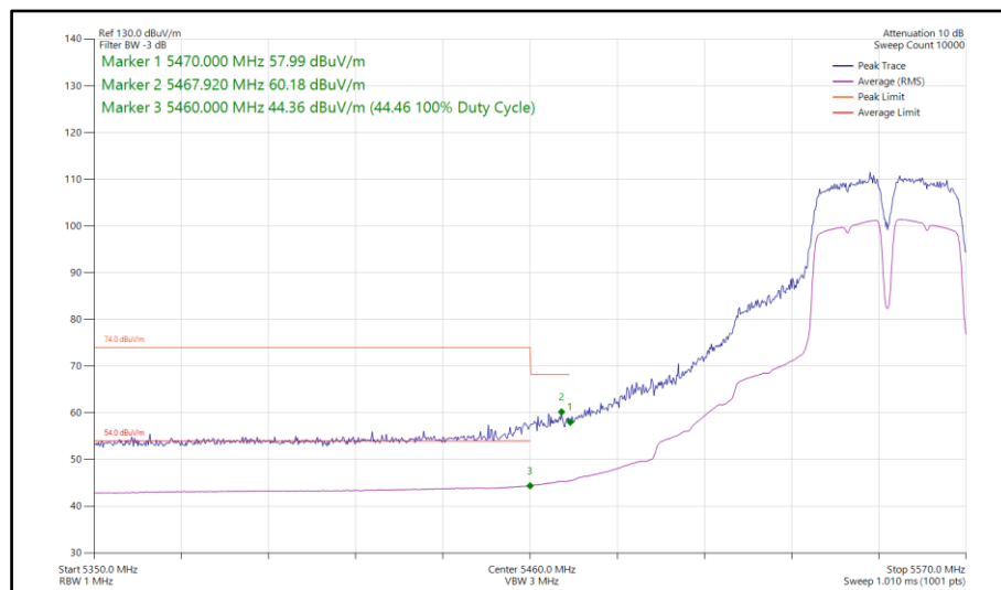
Figure 909 - 802.11a a40, SISO, Core 1 - 5550 MHz Band Edge Frequency 5470 MHz
