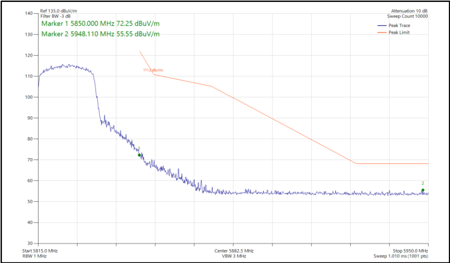
Figure 867 - 802.11ax HE20, SU, TxBF, Core 0-1 - 5825 MHz Band Edge Frequency 5850 MHz
