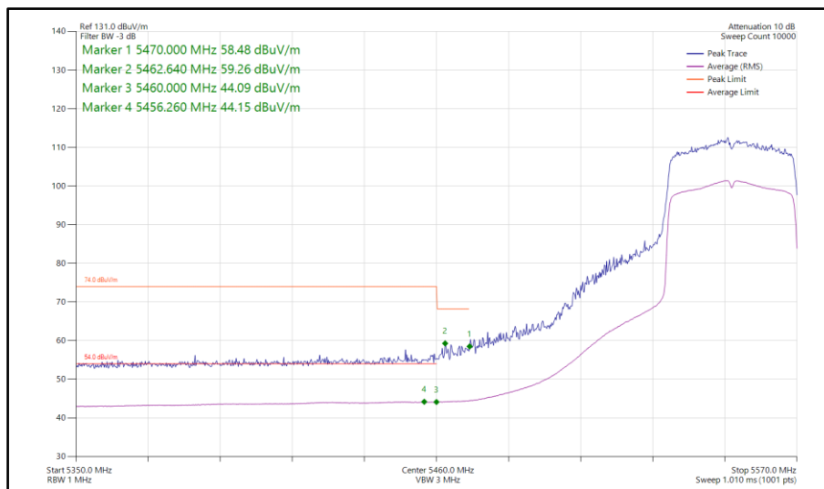
Figure 876 - 802.11ax HE40, SU, SISO, Core 0 - 5550 MHz Band Edge Frequency 5470 MHz
