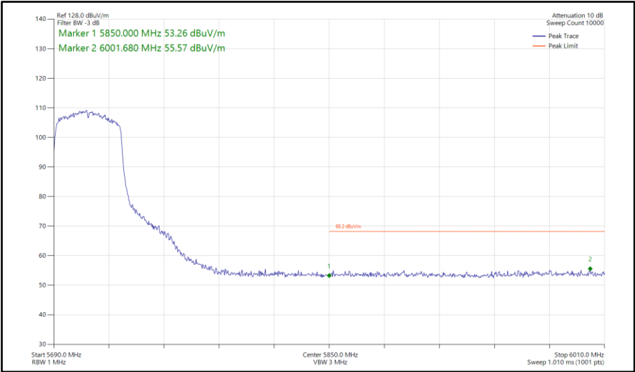
Figure 902 - 802.11ax HE40, SU, SISO, Core 0 - 5710 MHz Band Edge Frequency 5850 MHz
