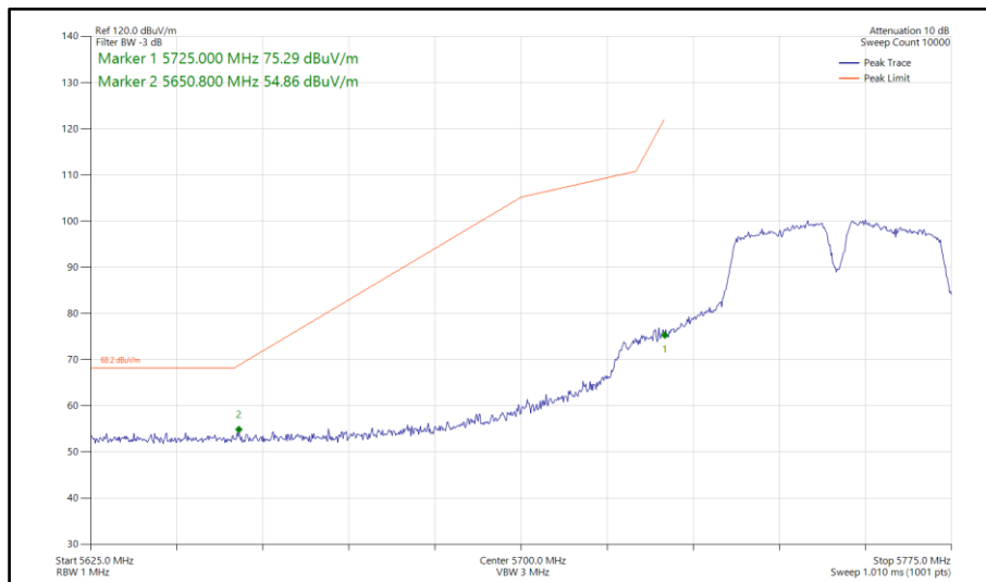
Figure 883 - 802.11a a40, SISO, Core 0 - 5755 MHz Band Edge Frequency 5725 MHz
