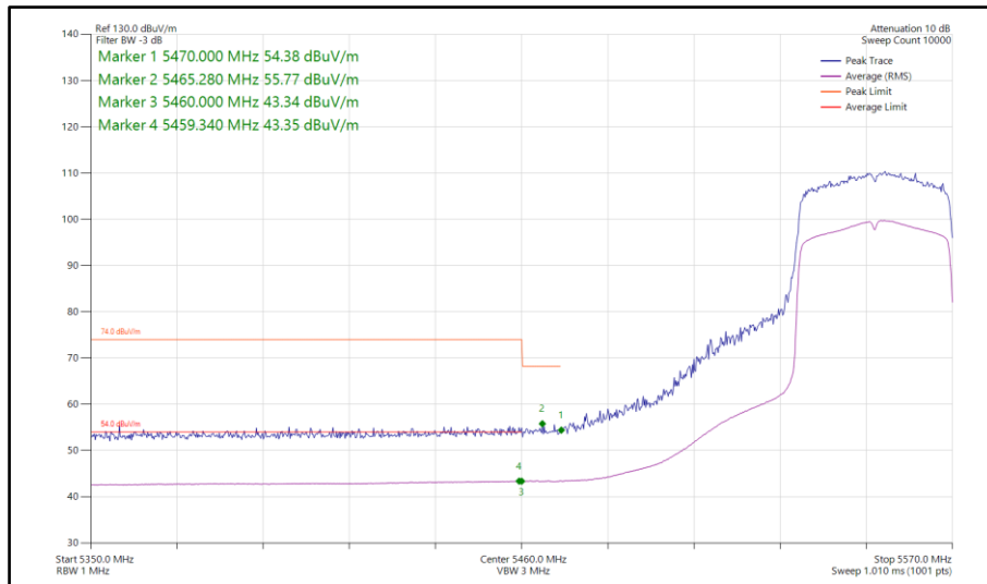
Figure 916 - 802.11ax HE40, SU, SISO, Core 1 - 5550 MHz Band Edge Frequency 5470 MHz
