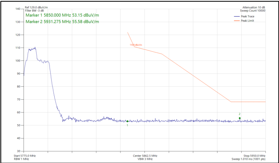
Figure 907 - 802.11be EHT40, RU 52+26-70, SISO, Core 0 - 5795 MHz Band Edge Frequency 5850 MHz
