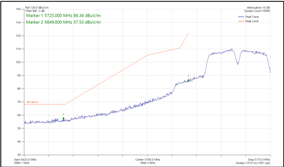
Figure 923 - 802.11a a40, SISO, Core 1 - 5755 MHz Band Edge Frequency 5725 MHz
