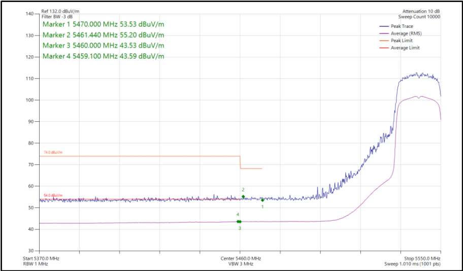
Figure 855 - 802.11ax HE20, SU, TxBF, Core 0-1 - 5540 MHz Band Edge Frequency 5470 MHz
