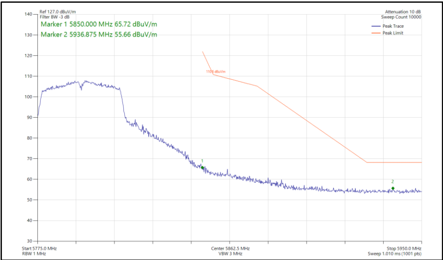
Figure 901 - 802.11n HT40, SISO, Core 0 - 5795 MHz Band Edge Frequency 5850 MHz
