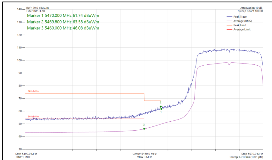
Figure 914 - 802.11ax HE40, SU, SISO, Core 1 - 5510 MHz Band Edge Frequency 5470 MHz
