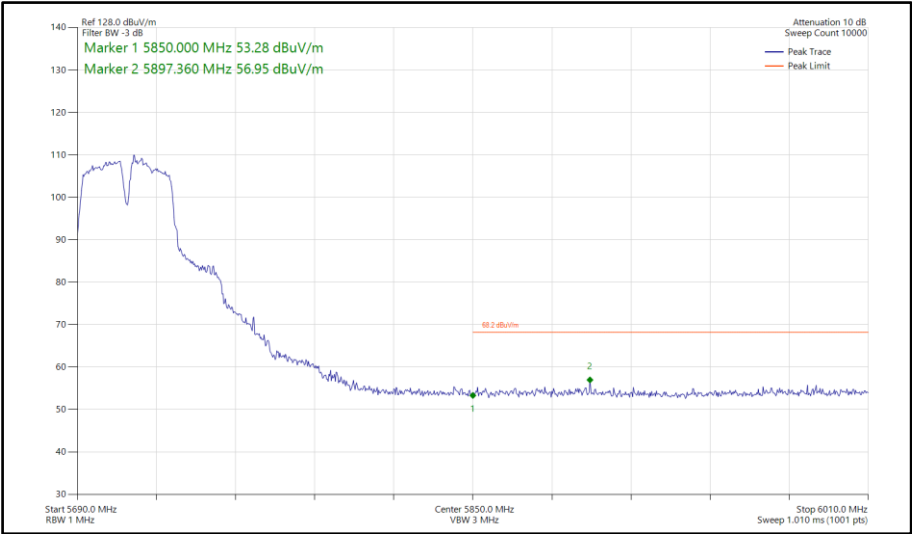
Figure 898 - 802.11a a40, SISO, Core 0 - 5710 MHz Band Edge Frequency 5850 MHz
