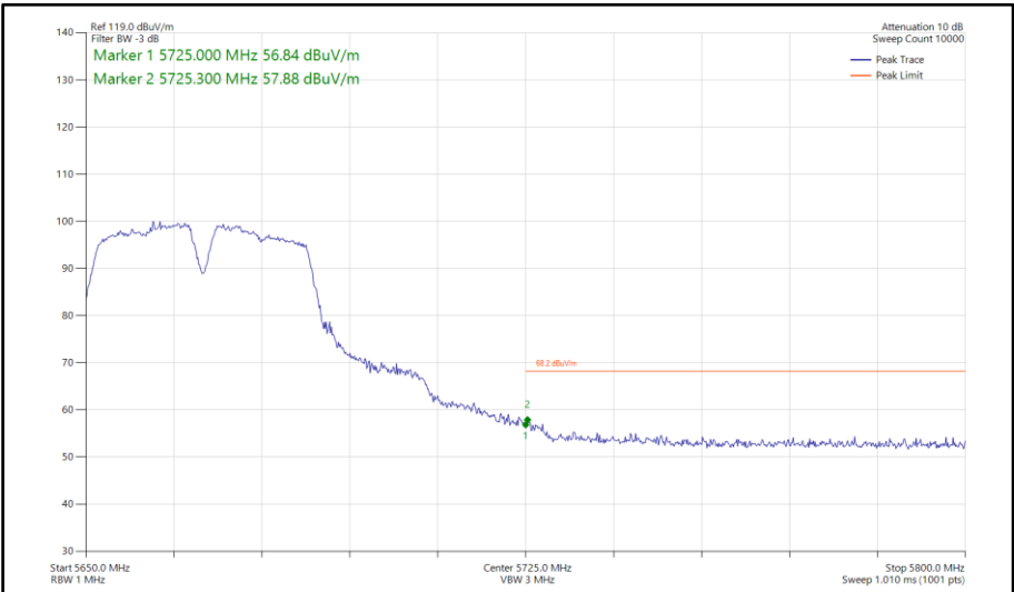
Figure 889 - 802.11a a40, SISO, Core 0 - 5670 MHz Band Edge Frequency 5725 MHz
