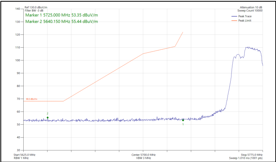
Figure 887 - 802.11be EHT40, RU 106+26-85, SISO, Core 0 - 5755 MHz Band Edge Frequency 5725 MHz
