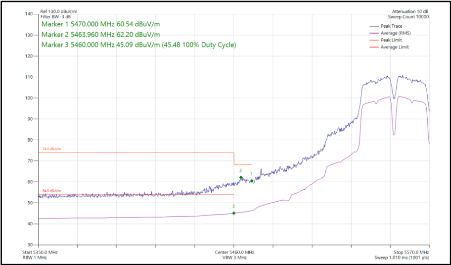
Figure 869 - 802.11a a40, SISO, Core 0 - 5550 MHz Band Edge Frequency 5470 MHz
