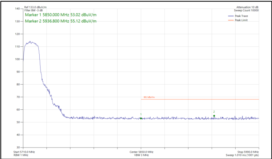
Figure 864 - 802.11ac VHT20, TxBF, Core 0-1 - 5720 MHz Band Edge Frequency 5850 MHz
