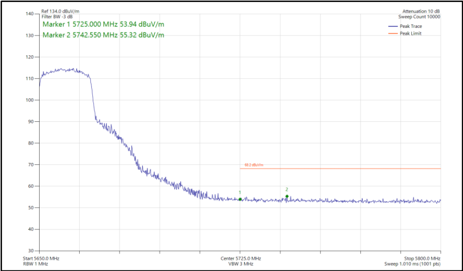
Figure 861 - 802.11ax HE20, SU, TxBF, Core 0-1 - 5660 MHz Band Edge Frequency 5725 MHz
