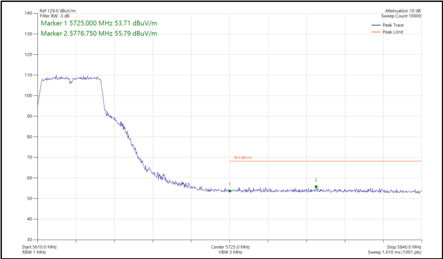
Figure 890 - 802.11n HT40, SISO, Core 0 - 5630 MHz Band Edge Frequency 5725 MHz
