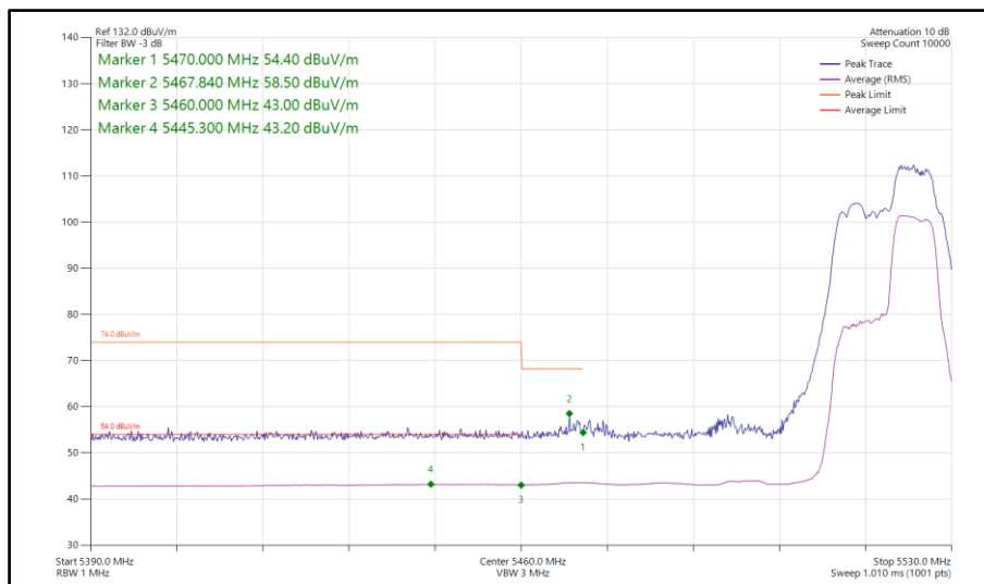
Figure 880 - 802.11be EHT40, RU 52+26-75, SISO, Core 0 - 5510 MHz Band Edge Frequency 5470 MHz
