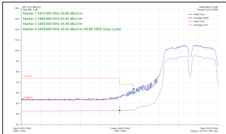
Figure 908 - 802.11a a40, SISO, Core 1 - 5510 MHz Band Edge Frequency 5470 MHz
