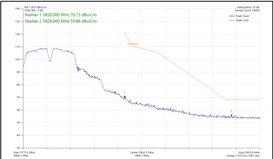
Figure 899 - 802.11a a40, SISO, Core 0 - 5795 MHz Band Edge Frequency 5850 MHz
