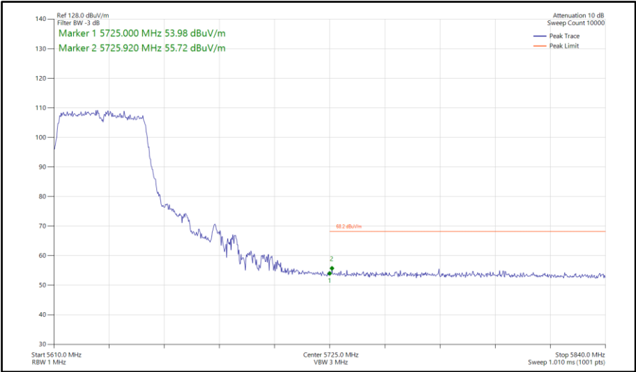
Figure 930 - 802.11n HT40, SISO, Core 1 - 5630 MHz Band Edge Frequency 5725 MHz
