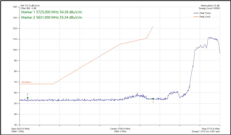
Figure 926 - 802.11ax HE40, RU 106-56, SISO, Core 1 - 5755 MHz Band Edge Frequency 5725 MHz
