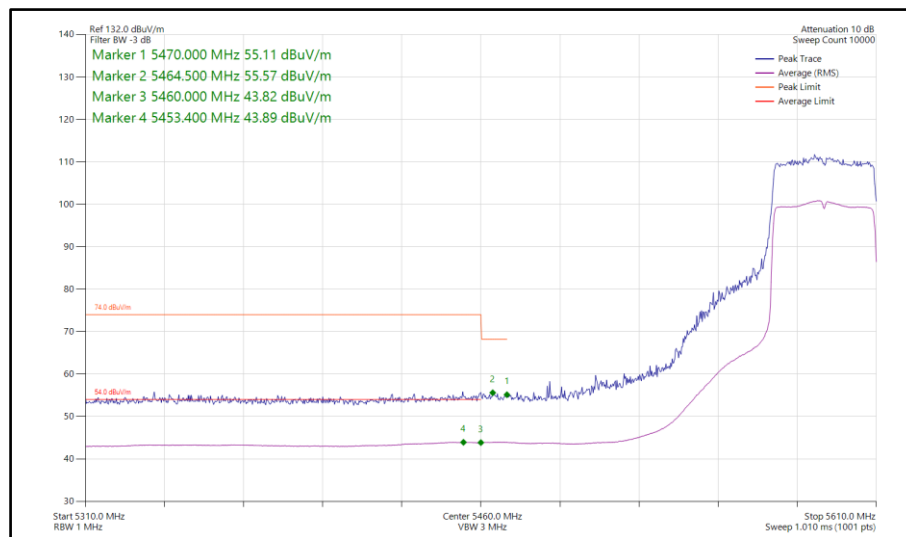
Figure 878 - 802.11ax HE40, SU, SISO, Core 0 - 5590 MHz Band Edge Frequency 5470 MHz
