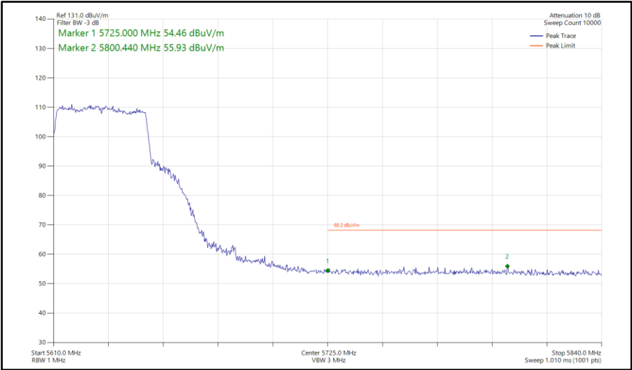
Figure 892 - 802.11ax HE40, SU, SISO, Core 0 - 5630 MHz Band Edge Frequency 5725 MHz
