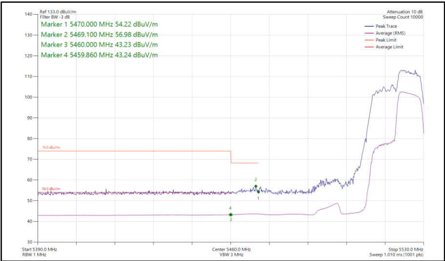
Figure 875 - 802.11ax HE40, RU 106-56, SISO, Core 0 - 5510 MHz Band Edge Frequency 5470 MHz
