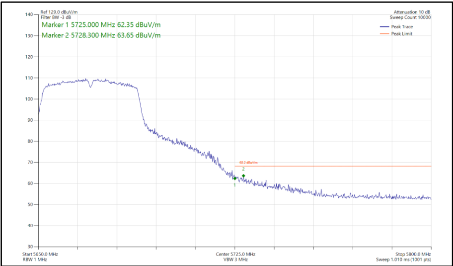
Figure 931 - 802.11n HT40, SISO, Core 1 - 5670 MHz Band Edge Frequency 5725 MHz
