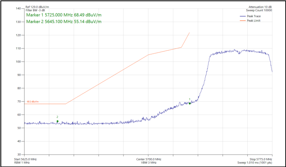
Figure 924 - 802.11n HT40, SISO, Core 1 - 5755 MHz Band Edge Frequency 5725 MHz
