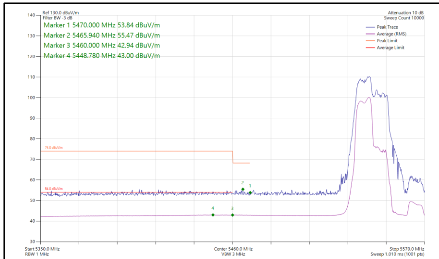
Figure 994 - 802.11ax HE40, RU 106-53, SDM, Core 0-1 - 5550 MHz Band Edge Frequency 5470 MHz
