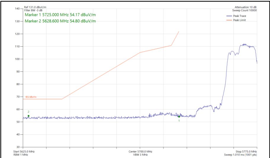
Figure 967 - 802.11be EHT40, RU 106+26-85, CDD, Core 0-1 - 5755 MHz Band Edge Frequency 5725 MHz
