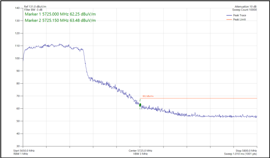
Figure 974 - 802.11ax HE40, SU, CDD, Core 0-1 - 5670 MHz Band Edge Frequency 5725 MHz
