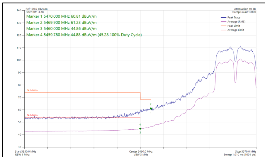
Figure 949 - 802.11a a40, CDD, Core 0-1 - 5550 MHz Band Edge Frequency 5470 MHz
