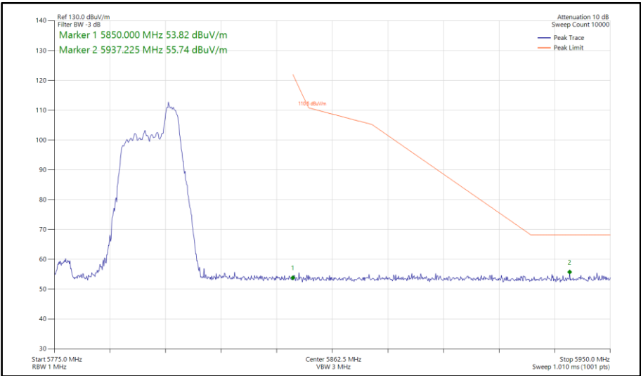
Figure 945 - 802.11ax HE40, RU 52-44, SISO, Core 1 - 5795 MHz Band Edge Frequency 5850 MHz
