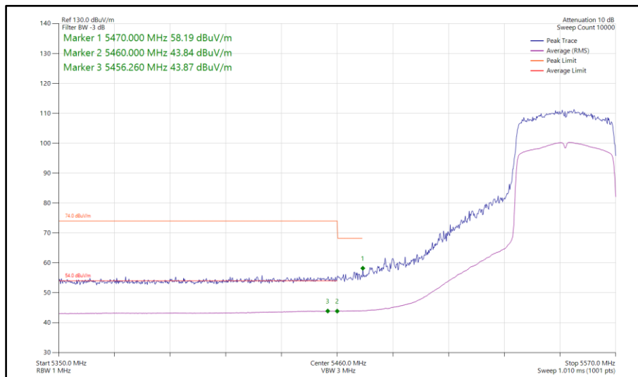
Figure 993 - 802.11ax HE40, SU, SDM, Core 0-1 - 5550 MHz Band Edge Frequency 5470 MHz
