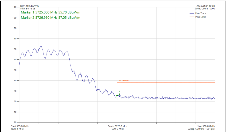
Figure 969 - 802.11a a40, CDD, Core 0-1 - 5670 MHz Band Edge Frequency 5725 MHz
