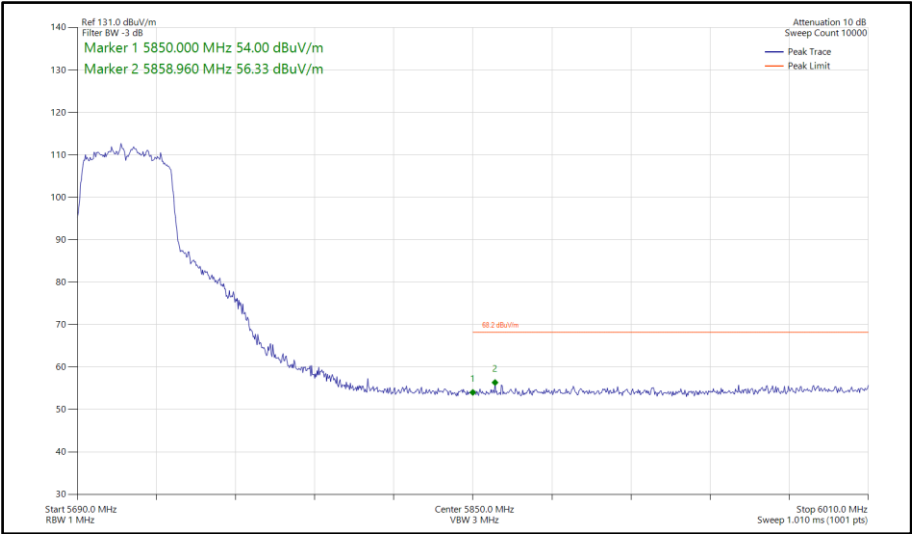
Figure 980 - 802.11n HT40, CDD, Core 0-1 - 5710 MHz Band Edge Frequency 5850 MHz
