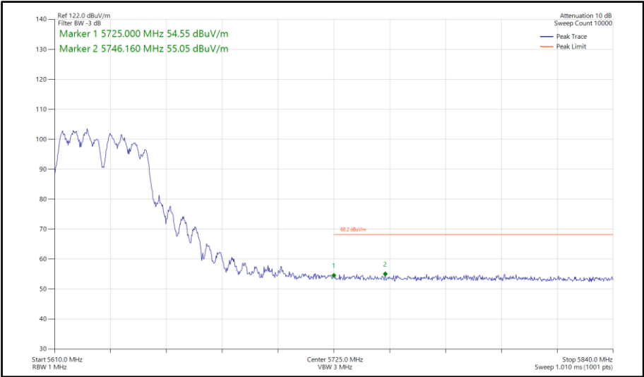
Figure 968 - 802.11a a40, CDD, Core 0-1 - 5630 MHz Band Edge Frequency 5725 MHz
