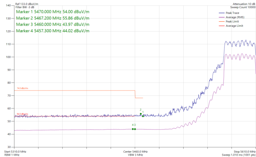
Figure 958 - 802.11ax HE40, SU, CDD, Core 0-1 - 5590 MHz Band Edge Frequency 5470 MHz
