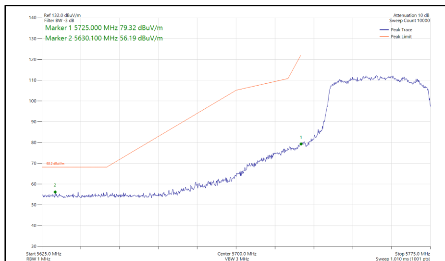
Figure 965 - 802.11ax HE40, SU, CDD, Core 0-1 - 5755 MHz Band Edge Frequency 5725 MHz
