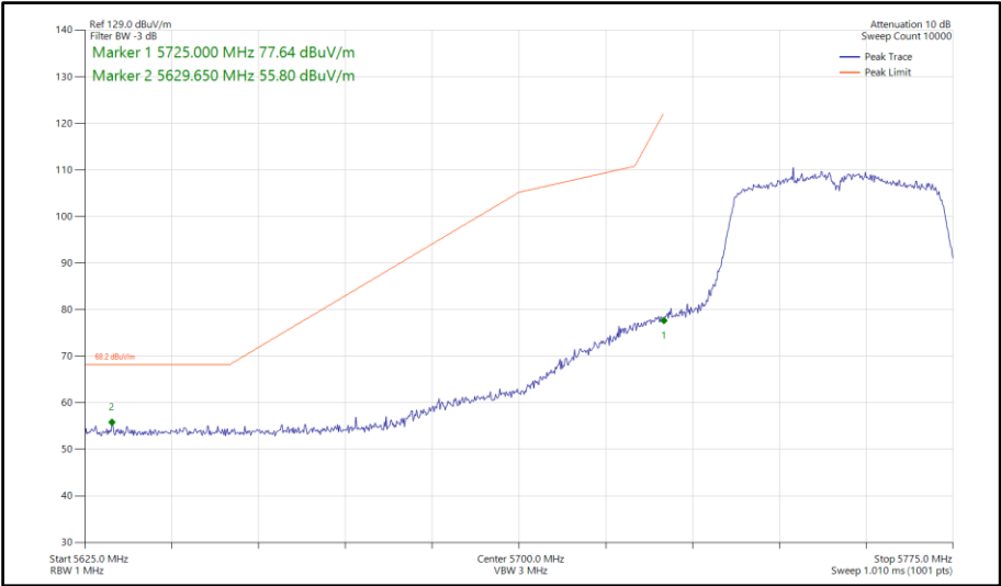
Figure 1000 - 802.11n HT40, SDM, Core 0-1 - 5755 MHz Band Edge Frequency 5725 MHz
