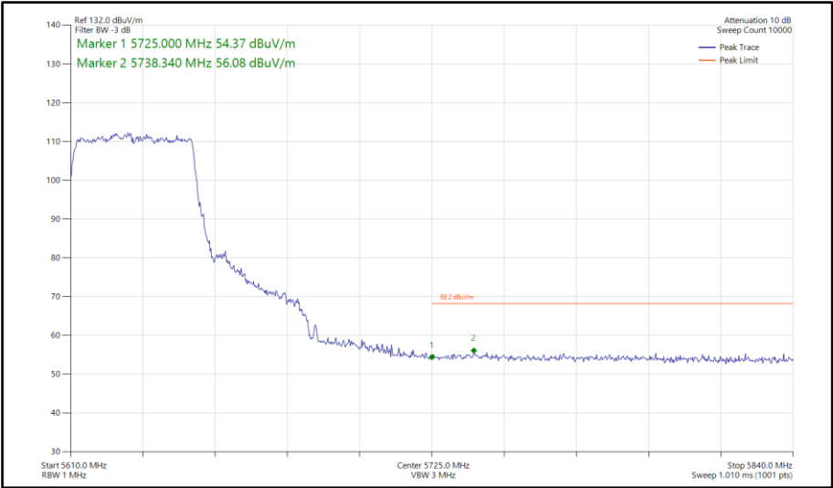
Figure 972 - 802.11ax HE40, SU, CDD, Core 0-1 - 5630 MHz Band Edge Frequency 5725 MHz
