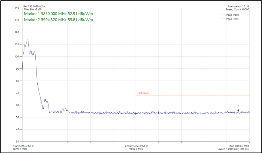
Figure 986 - 802.11be EHT40, RU 52+26-70, CDD, Core 0-1 - 5710 MHz Band Edge Frequency 5850 MHz
