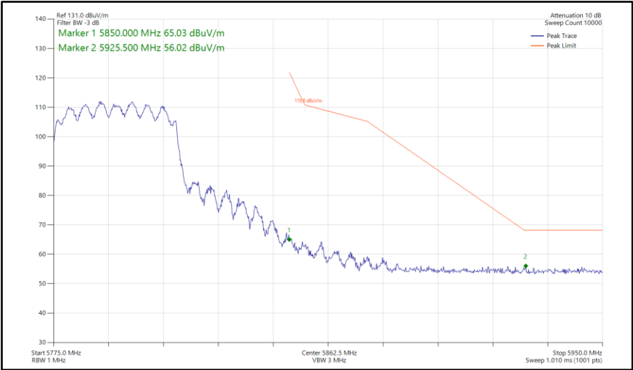
Figure 984 - 802.11ax HE40, SU, CDD, Core 0-1 - 5795 MHz Band Edge Frequency 5850 MHz
