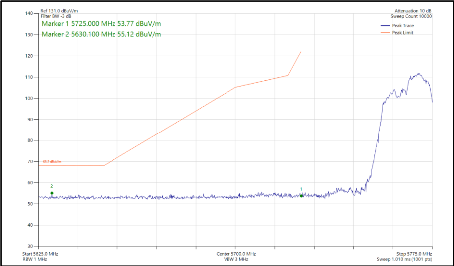
Figure 1002 - 802.11ax HE40, RU 106-56, SDM, Core 0-1 - 5755 MHz Band Edge Frequency 5725 MHz
