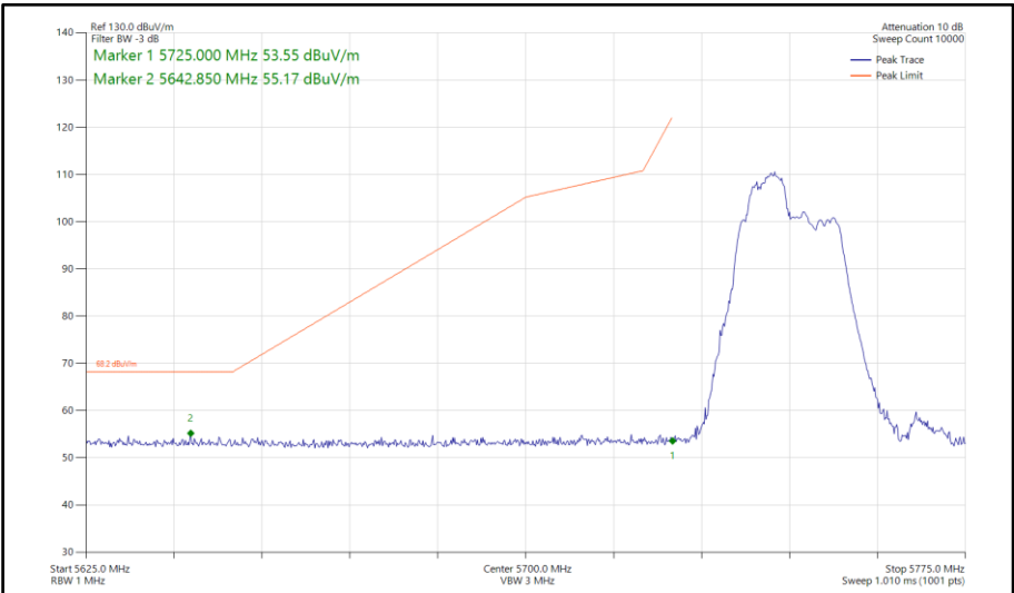
Figure 1003 - 802.11be EHT40, RU 52+26-70, SDM, Core 0-1 - 5755 MHz Band Edge Frequency 5725 MHz
