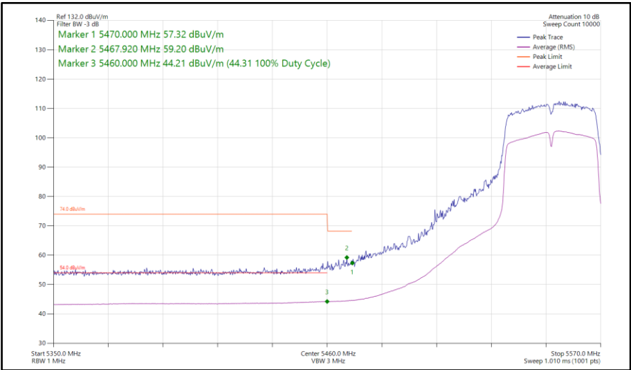
Figure 989 - 802.11n HT40, SDM, Core 0-1 - 5550 MHz Band Edge Frequency 5470 MHz
