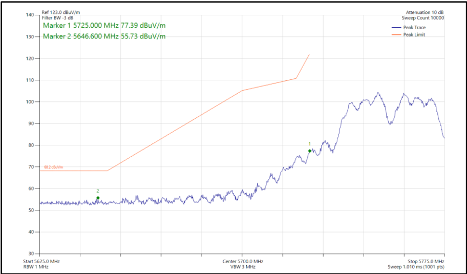
Figure 963 - 802.11a a40, CDD, Core 0-1 - 5755 MHz Band Edge Frequency 5725 MHz
