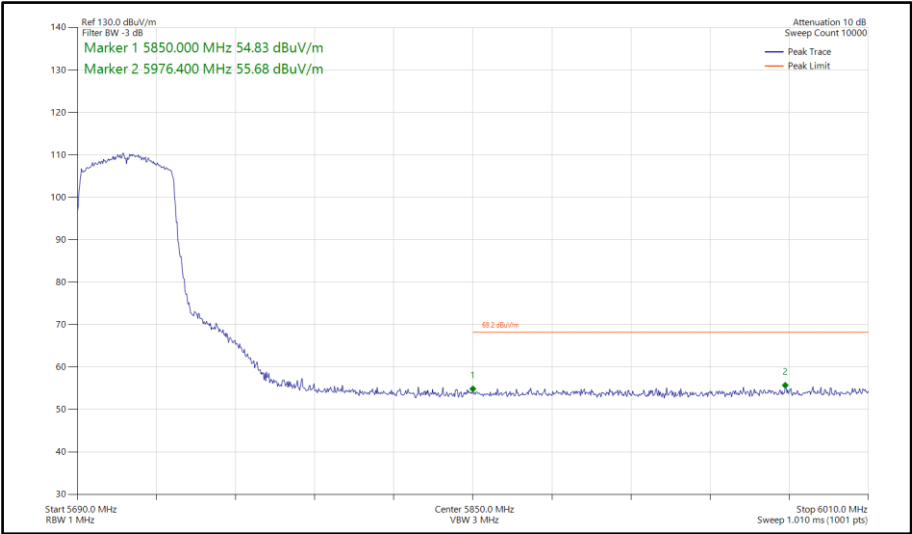
Figure 942 - 802.11ax HE40, SU, SISO, Core 1 - 5710 MHz Band Edge Frequency 5850 MHz
