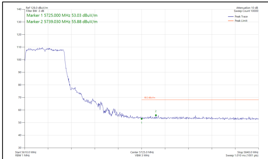
Figure 932 - 802.11ax HE40, SU, SISO, Core 1 - 5630 MHz Band Edge Frequency 5725 MHz
