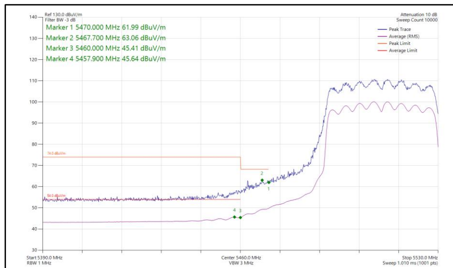
Figure 954 - 802.11ax HE40, SU, CDD, Core 0-1 - 5510 MHz Band Edge Frequency 5470 MHz
