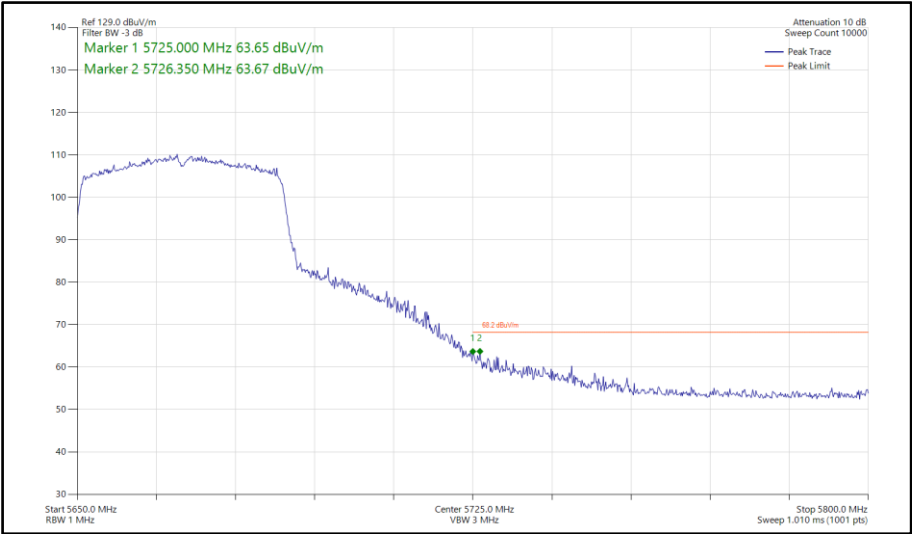
Figure 934 - 802.11ax HE40, SU, SISO, Core 1 - 5670 MHz Band Edge Frequency 5725 MHz
