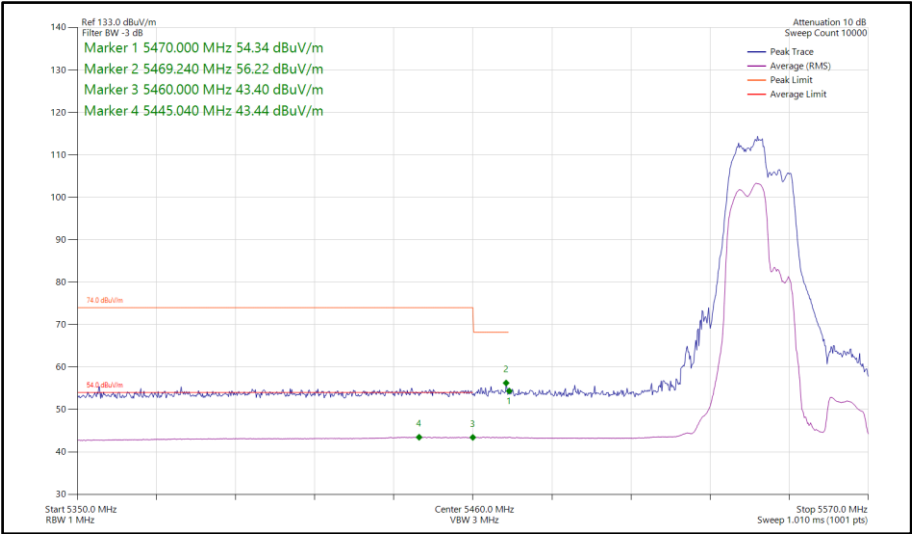
Figure 998 - 802.11be EHT40, RU 106+26-82, SDM, Core 0-1 - 5550 MHz Band Edge Frequency 5470 MHz
