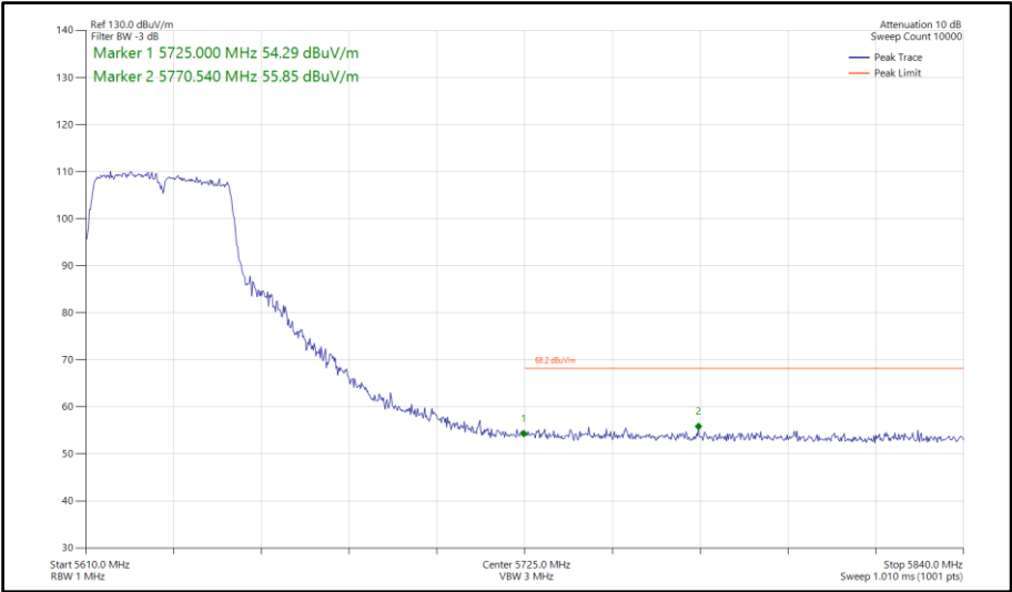
Figure 1004 - 802.11n HT40, SDM, Core 0-1 - 5630 MHz Band Edge Frequency 5725 MHz
