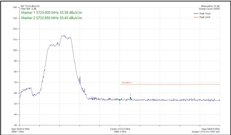
Figure 975 - 802.11ax HE40, RU 106-56, CDD, Core 0-1 - 5670 MHz Band Edge Frequency 5725 MHz
