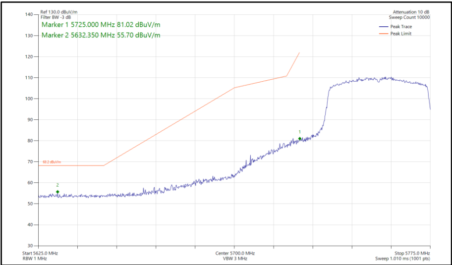
Figure 1001 - 802.11ax HE40, SU, SDM, Core 0-1 - 5755 MHz Band Edge Frequency 5725 MHz
