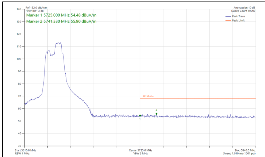
Figure 976 - 802.11be EHT40, RU 52+26-75, CDD, Core 0-1 - 5630 MHz Band Edge Frequency 5725 MHz
