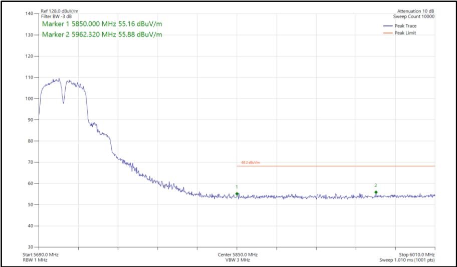
Figure 938 - 802.11a a40, SISO, Core 1 - 5710 MHz Band Edge Frequency 5850 MHz
