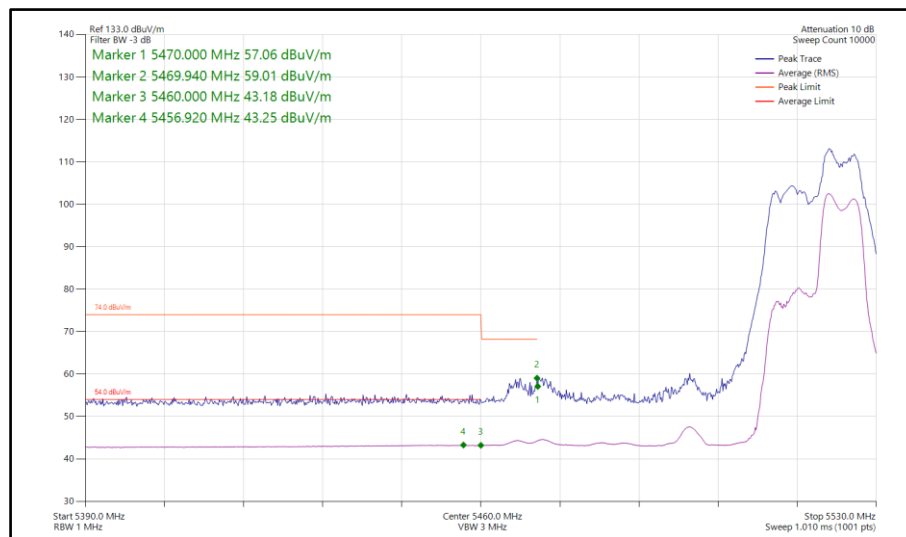
Figure 960 - 802.11be EHT40, RU 52+26-75, CDD, Core 0-1 - 5510 MHz Band Edge Frequency 5470 MHz
