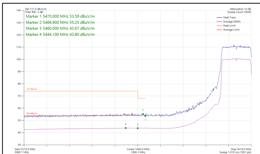
Figure 995 - 802.11ax HE40, SU, SDM, Core 0-1 - 5590 MHz Band Edge Frequency 5470 MHz
