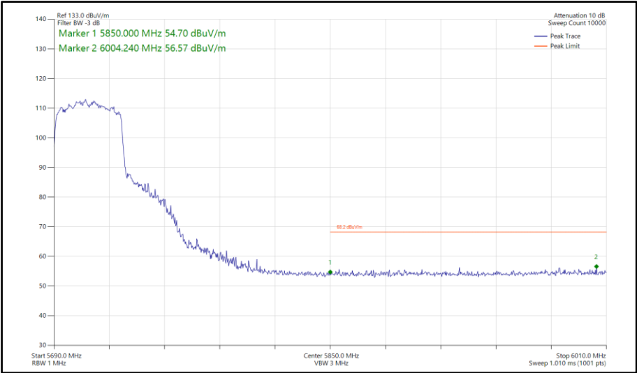
Figure 982 - 802.11ax HE40, SU, CDD, Core 0-1 - 5710 MHz Band Edge Frequency 5850 MHz
