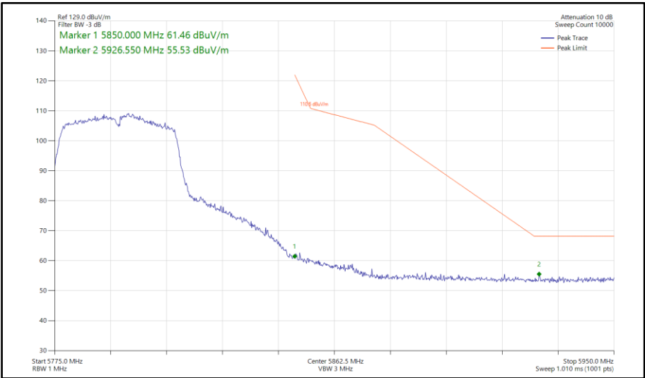
Figure 1013 - 802.11n HT40, SDM, Core 0-1 - 5795 MHz Band Edge Frequency 5850 MHz
