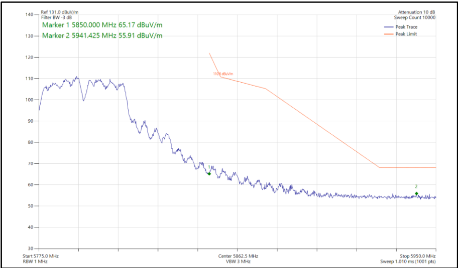
Figure 979 - 802.11a a40, CDD, Core 0-1 - 5795 MHz Band Edge Frequency 5850 MHz
