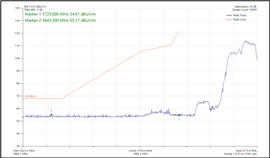
Figure 966 - 802.11ax HE40, RU 106-56, CDD, Core 0-1 - 5755 MHz Band Edge Frequency 5725 MHz
