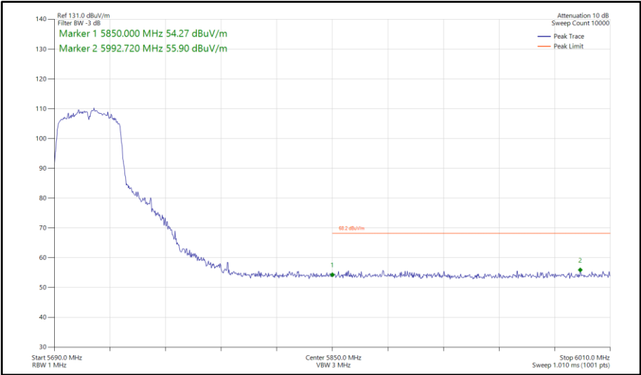
Figure 1012 - 802.11n HT40, SDM, Core 0-1 - 5710 MHz Band Edge Frequency 5850 MHz
