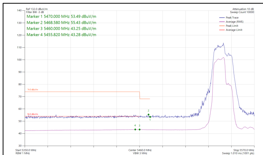
Figure 961 - 802.11be EHT40, RU 106+26-82, CDD, Core 0-1 - 5550 MHz Band Edge Frequency 5470 MHz
