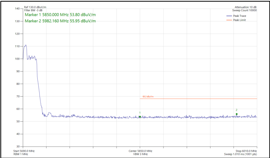
Figure 943 - 802.11ax HE40, RU 52-37, SISO, Core 1 - 5710 MHz Band Edge Frequency 5850 MHz
