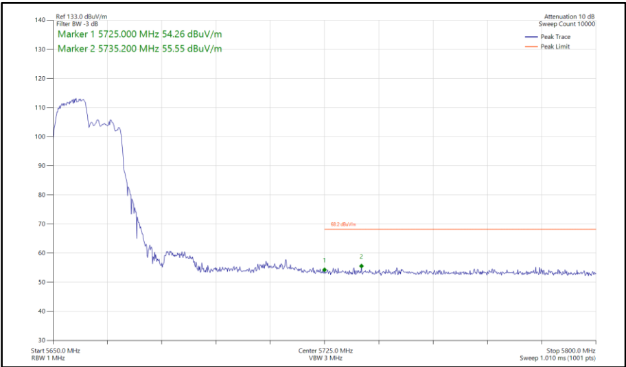
Figure 935 - 802.11ax HE40, RU 106-53, SISO, Core 1 - 5670 MHz Band Edge Frequency 5725 MHz
