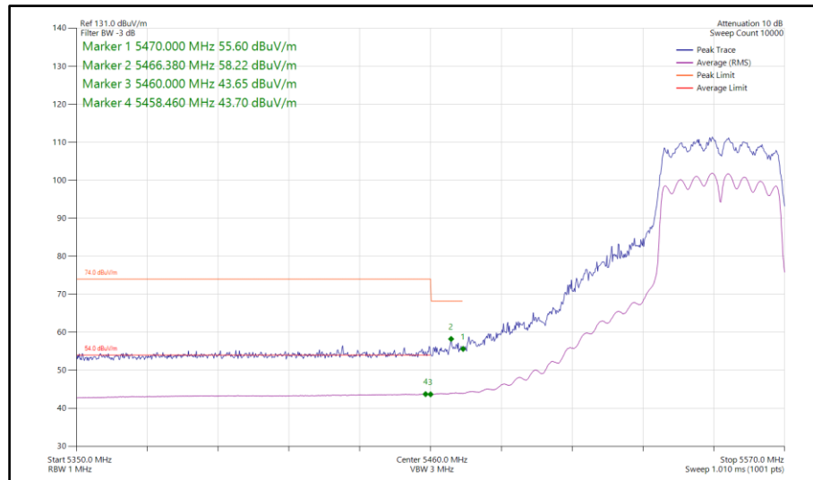
Figure 952 - 802.11n HT40, CDD, Core 0-1 - 5550 MHz Band Edge Frequency 5470 MHz
