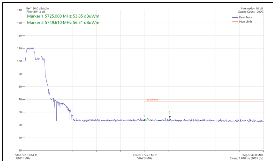
Figure 933 - 802.11ax HE40, RU 106-53, SISO, Core 1 - 5630 MHz Band Edge Frequency 5725 MHz
