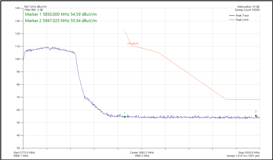
Figure 944 - 802.11ax HE40, SU, SISO, Core 1 - 5795 MHz Band Edge Frequency 5850 MHz
