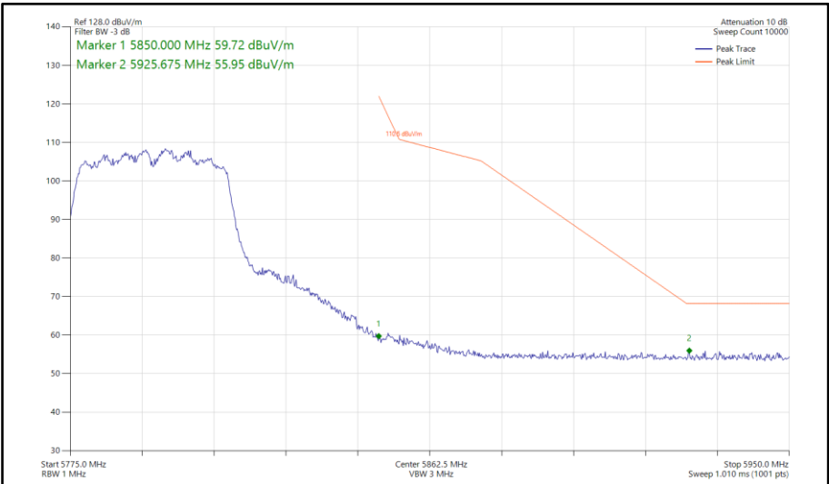
Figure 981 - 802.11n HT40, CDD, Core 0-1 - 5795 MHz Band Edge Frequency 5850 MHz
