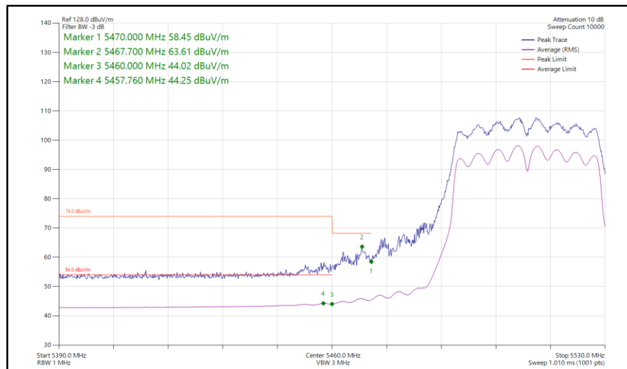
Figure 951 - 802.11n HT40, CDD, Core 0-1 - 5510 MHz Band Edge Frequency 5470 MHz
