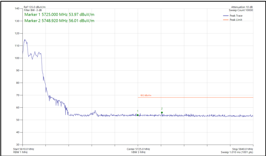
Figure 973 - 802.11ax HE40, RU 52-37, CDD, Core 0-1 - 5630 MHz Band Edge Frequency 5725 MHz
