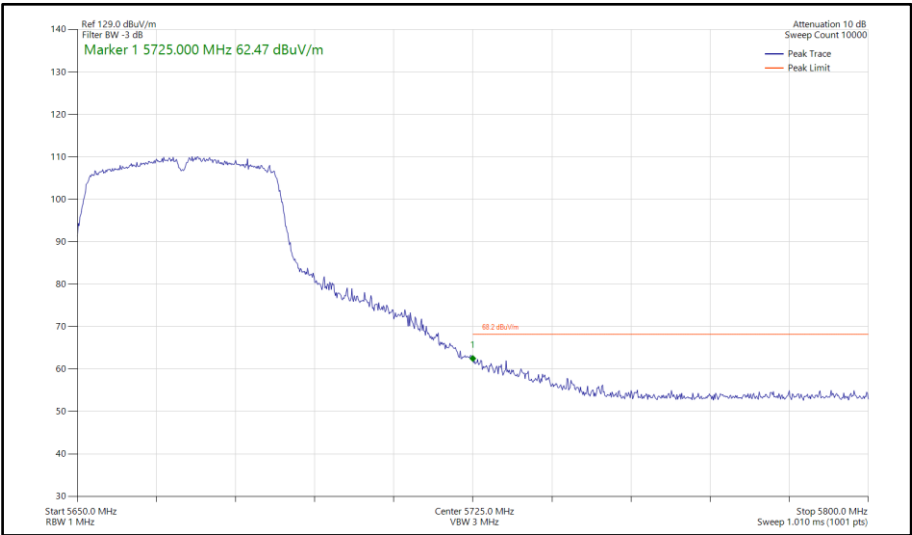
Figure 1005 - 802.11n HT40, SDM, Core 0-1 - 5670 MHz Band Edge Frequency 5725 MHz
