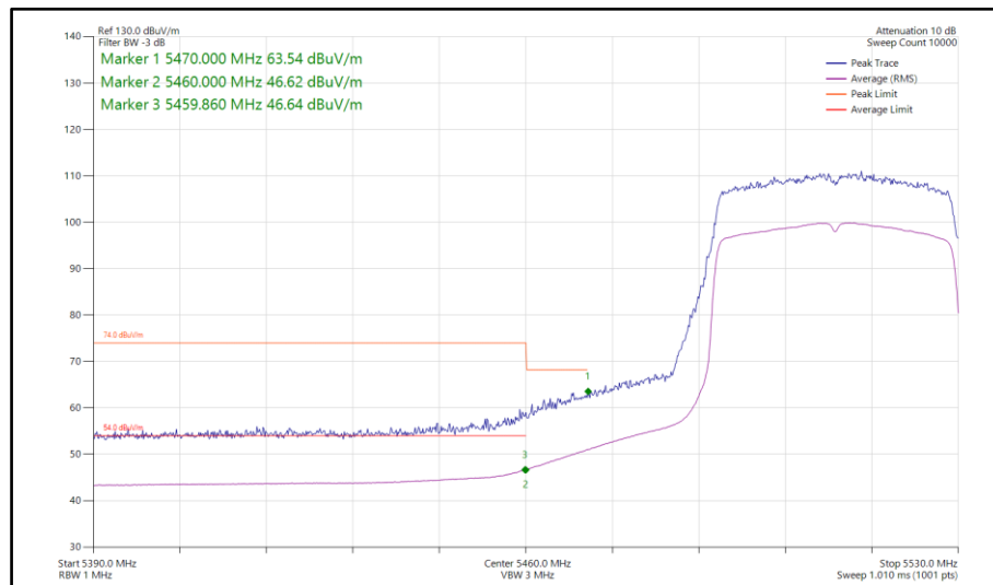
Figure 991 - 802.11ax HE40, SU, SDM, Core 0-1 - 5510 MHz Band Edge Frequency 5470 MHz
