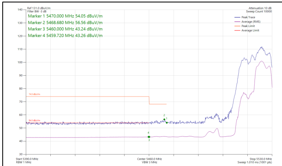
Figure 992 - 802.11ax HE40, RU 106-56, SDM, Core 0-1 - 5510 MHz Band Edge Frequency 5470 MHz
