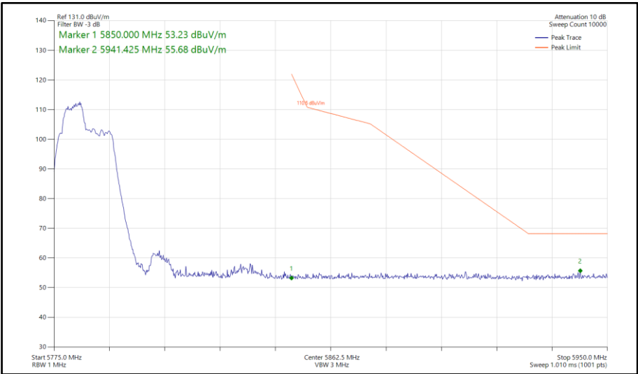
Figure 947 - 802.11be EHT40, RU 52+26-70, SISO, Core 1 - 5795 MHz Band Edge Frequency 5850 MHz
