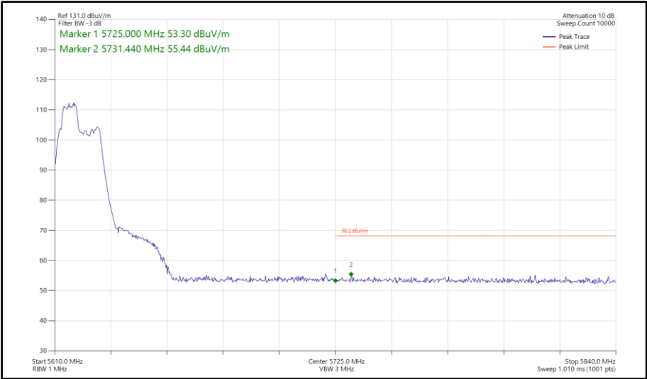
Figure 936 - 802.11be EHT40, RU 52+26-70, SISO, Core 1 - 5630 MHz Band Edge Frequency 5725 MHz
