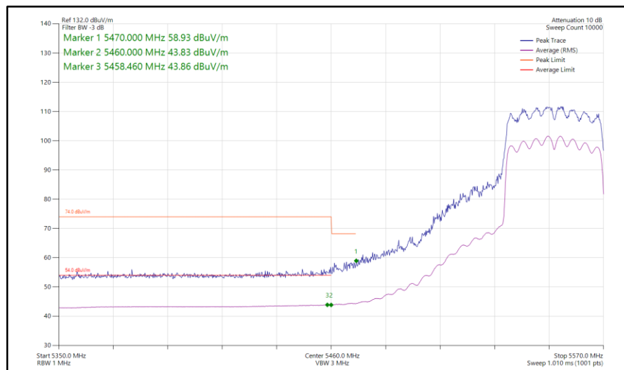
Figure 956 - 802.11ax HE40, SU, CDD, Core 0-1 - 5550 MHz Band Edge Frequency 5470 MHz
