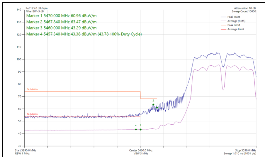
Figure 948 - 802.11a a40, CDD, Core 0-1 - 5510 MHz Band Edge Frequency 5470 MHz
