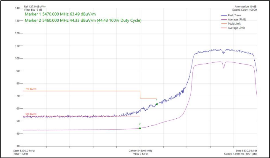
Figure 988 - 802.11n HT40, SDM, Core 0-1 - 5510 MHz Band Edge Frequency 5470 MHz
