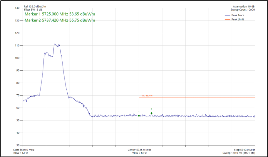
Figure 1010 - 802.11be EHT40, RU 52+26-75, SDM, Core 0-1 - 5630 MHz Band Edge Frequency 5725 MHz
