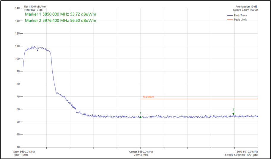
Figure 940 - 802.11n HT40, SISO, Core 1 - 5710 MHz Band Edge Frequency 5850 MHz
