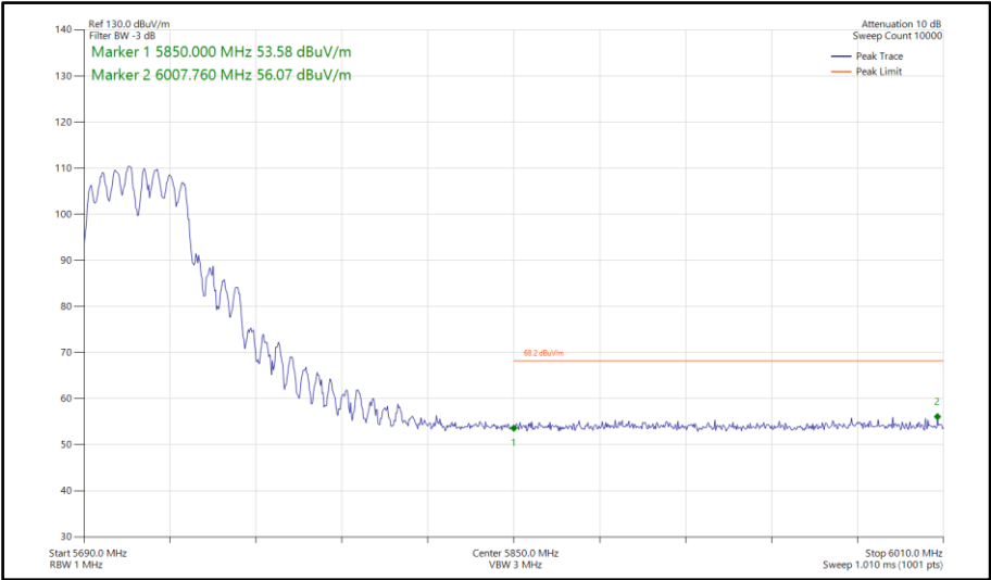
Figure 978 - 802.11a a40, CDD, Core 0-1 - 5710 MHz Band Edge Frequency 5850 MHz
