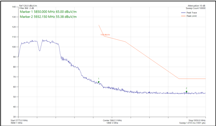
Figure 939 - 802.11a a40, SISO, Core 1 - 5795 MHz Band Edge Frequency 5850 MHz
