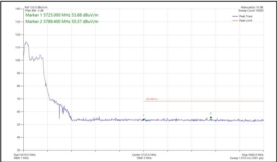
Figure 1007 - 802.11ax HE40, RU 52-37, SDM, Core 0-1 - 5630 MHz Band Edge Frequency 5725 MHz
