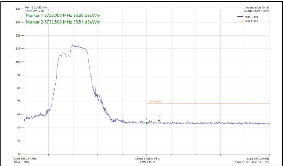
Figure 937 - 802.11be EHT40, RU 106+26-85, SISO, Core 1 - 5670 MHz Band Edge Frequency 5725 MHz
