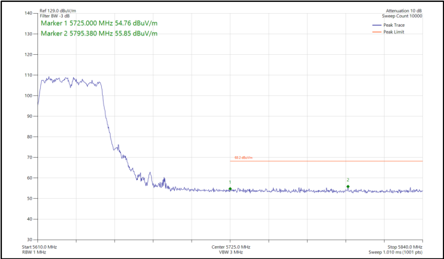
Figure 970 - 802.11n HT40, CDD, Core 0-1 - 5630 MHz Band Edge Frequency 5725 MHz
