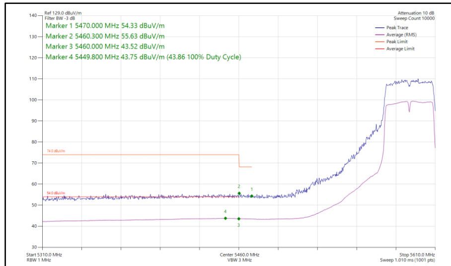
Figure 990 - 802.11n HT40, SDM, Core 0-1 - 5590 MHz Band Edge Frequency 5470 MHz
