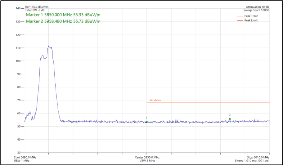
Figure 946 - 802.11be EHT40, RU 52+26-75, SISO, Core 1 - 5710 MHz Band Edge Frequency 5850 MHz
