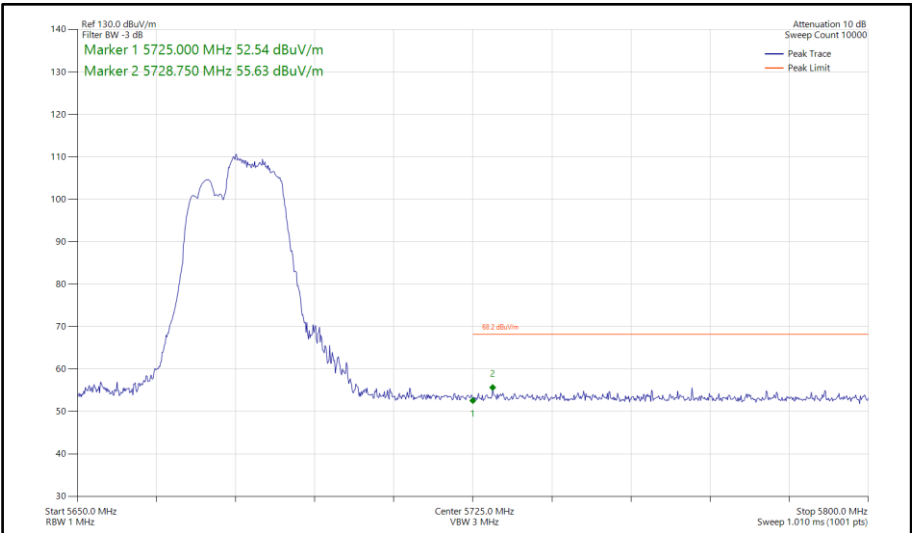
Figure 1011 - 802.11be EHT40, RU 106+26-85, SDM, Core 0-1 - 5670 MHz Band Edge Frequency 5725 MHz
