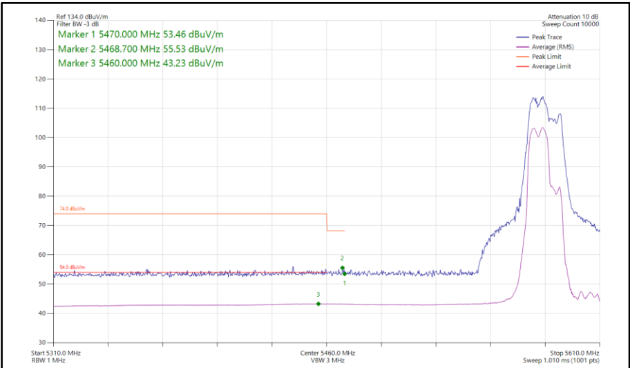
Figure 999 - 802.11be EHT40, RU 106+26-82, SDM, Core 0-1 - 5590 MHz Band Edge Frequency 5470 MHz
