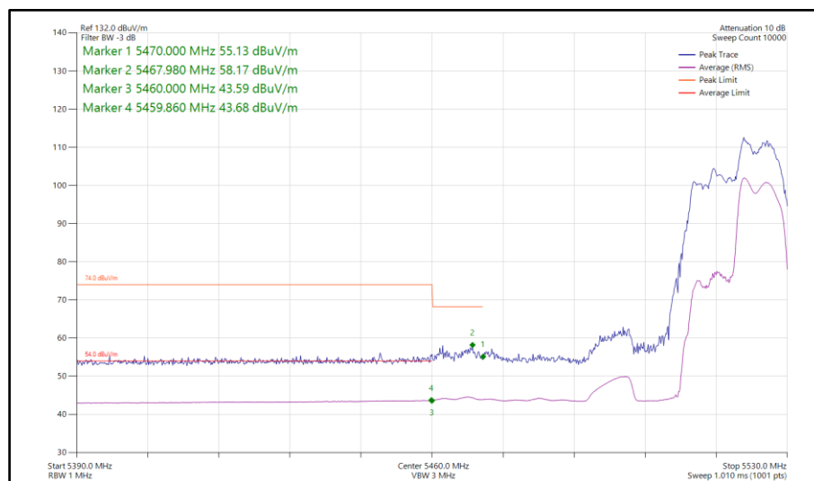
Figure 955 - 802.11ax HE40, RU 106-56, CDD, Core 0-1 - 5510 MHz Band Edge Frequency 5470 MHz
