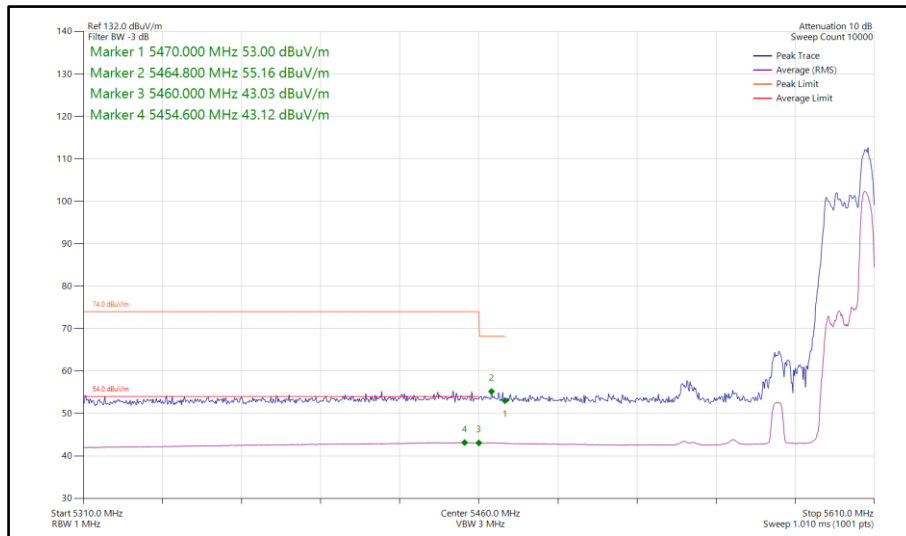
Figure 996 - 802.11ax HE40, RU 52-44, SDM, Core 0-1 - 5590 MHz Band Edge Frequency 5470 MHz
