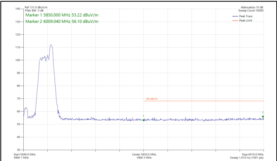
Figure 983 - 802.11ax HE40, RU 52-44, CDD, Core 0-1 - 5710 MHz Band Edge Frequency 5850 MHz
