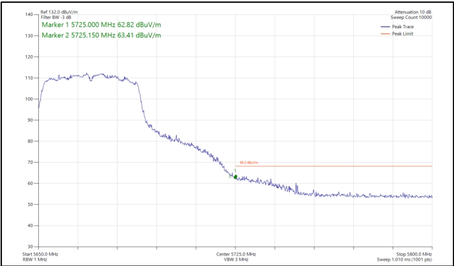
Figure 971 - 802.11n HT40, CDD, Core 0-1 - 5670 MHz Band Edge Frequency 5725 MHz
