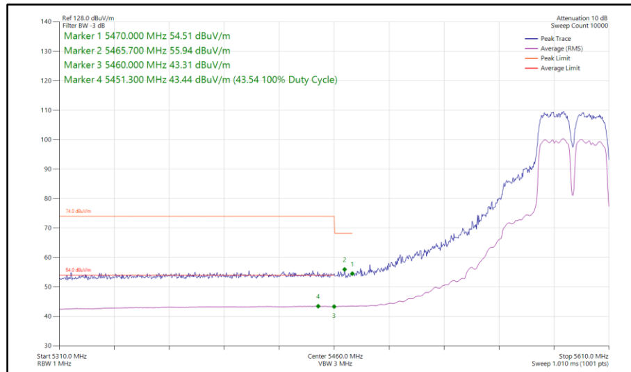
Figure 950 - 802.11a a40, CDD, Core 0-1 - 5590 MHz Band Edge Frequency 5470 MHz
