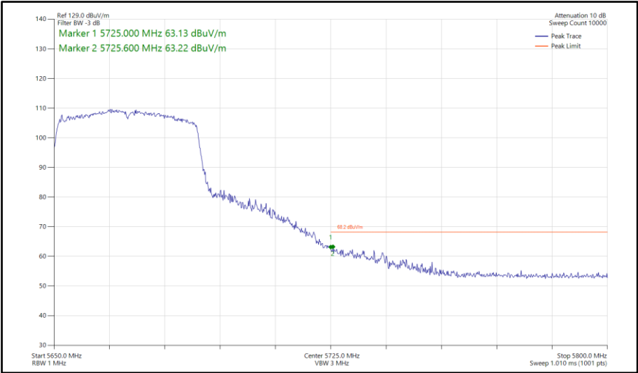
Figure 1008 - 802.11ax HE40, SU, SDM, Core 0-1 - 5670 MHz Band Edge Frequency 5725 MHz
