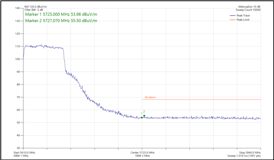
Figure 1006 - 802.11ax HE40, SU, SDM, Core 0-1 - 5630 MHz Band Edge Frequency 5725 MHz
