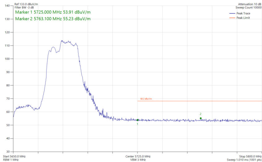
Figure 977 - 802.11be EHT40, RU 106+26-85, CDD, Core 0-1 - 5670 MHz Band Edge Frequency 5725 MHz
