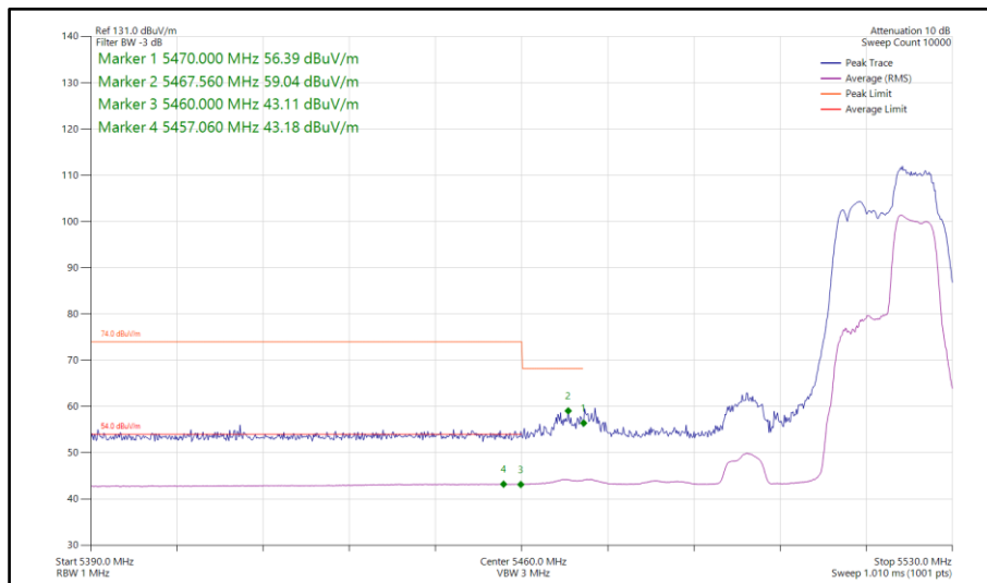
Figure 997 - 802.11be EHT40, RU 52+26-75, SDM, Core 0-1 - 5510 MHz Band Edge Frequency 5470 MHz
