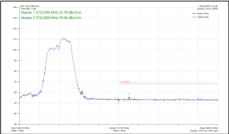
Figure 1009 - 802.11ax HE40, RU 106-56, SDM, Core 0-1 - 5670 MHz Band Edge Frequency 5725 MHz
