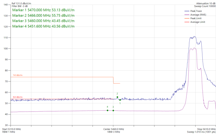
Figure 962 - 802.11be EHT40, RU 106+26-82, CDD, Core 0-1 - 5590 MHz Band Edge Frequency 5470 MHz
