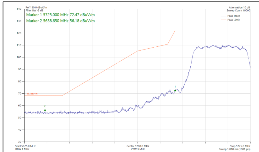
Figure 964 - 802.11n HT40, CDD, Core 0-1 - 5755 MHz Band Edge Frequency 5725 MHz
