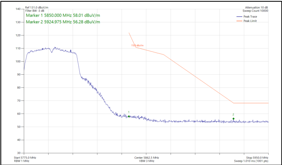
Figure 941 - 802.11n HT40, SISO, Core 1 - 5795 MHz Band Edge Frequency 5850 MHz
