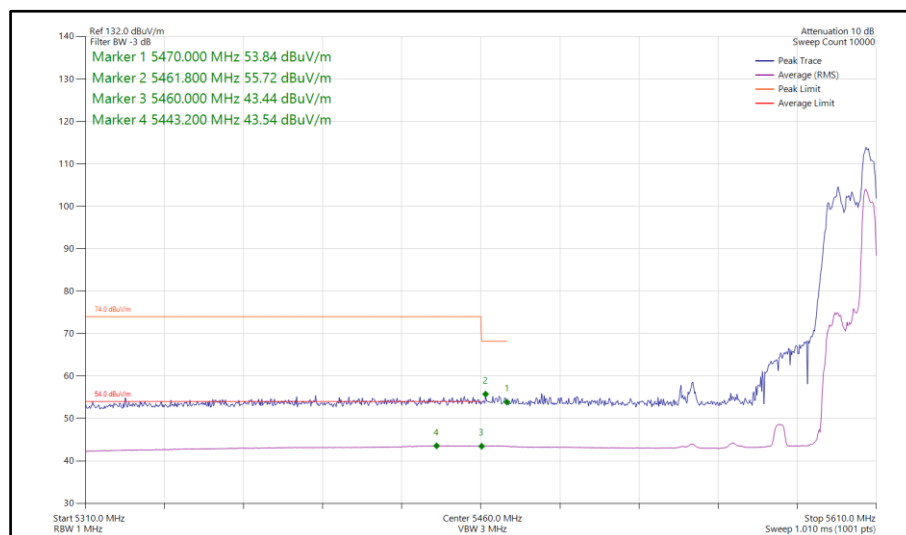
Figure 959 - 802.11ax HE40, RU 52-44, CDD, Core 0-1 - 5590 MHz Band Edge Frequency 5470 MHz
