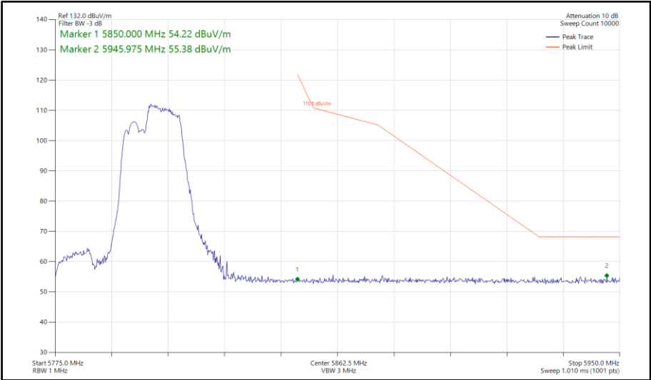
Figure 987 - 802.11be EHT40, RU 106+26-85, CDD, Core 0-1 - 5795 MHz Band Edge Frequency 5850 MHz
