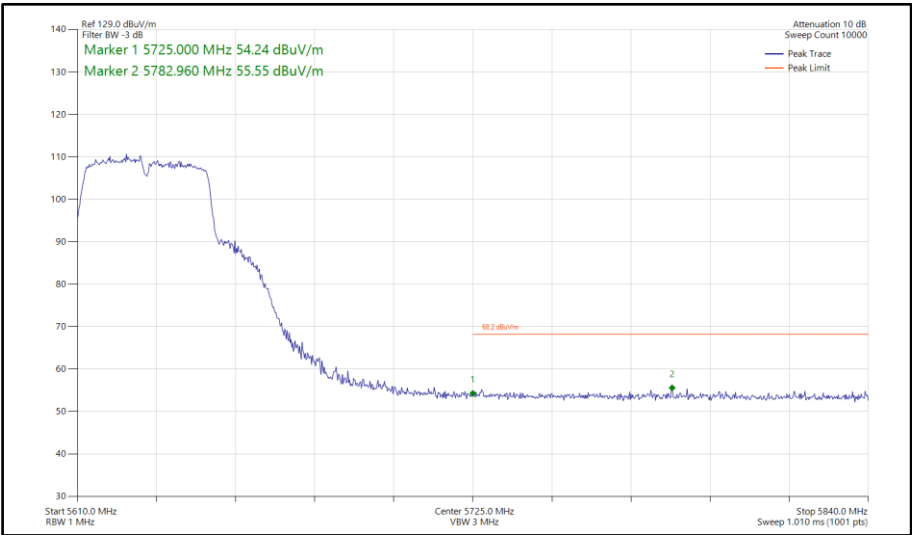
Figure 1028 - 802.11ac VHT40, TxBF, Core 0-1 - 5630 MHz Band Edge Frequency 5725 MHz
