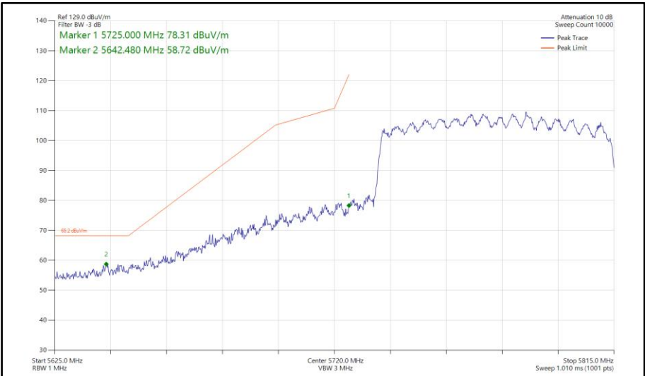
Figure 1093 - 802.11ax HE80, SU, CDD, Core 0-1 - 5775 MHz Band Edge Frequency 5725 MHz
