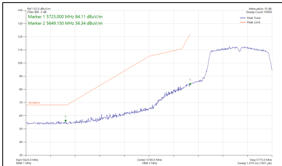
Figure 1026 - 802.11ac VHT40, TxBF, Core 0-1 - 5755 MHz Band Edge Frequency 5725 MHz
