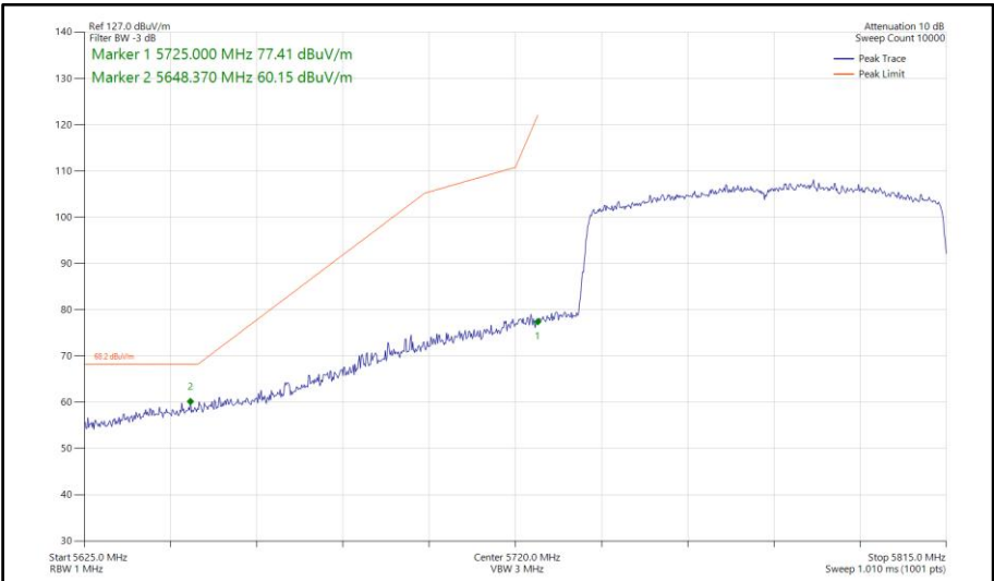
Figure 1043 - 802.11ax HE80, SU, SISO, Core 0 - 5775 MHz Band Edge Frequency 5725 MHz
