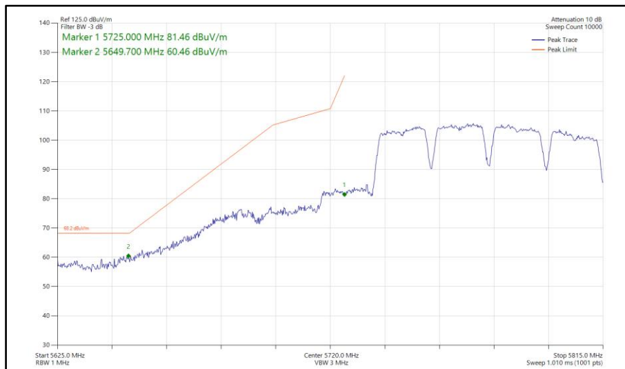
Figure 1041 - 802.11a a80, SISO, Core 0 - 5775 MHz Band Edge Frequency 5725 MHz
