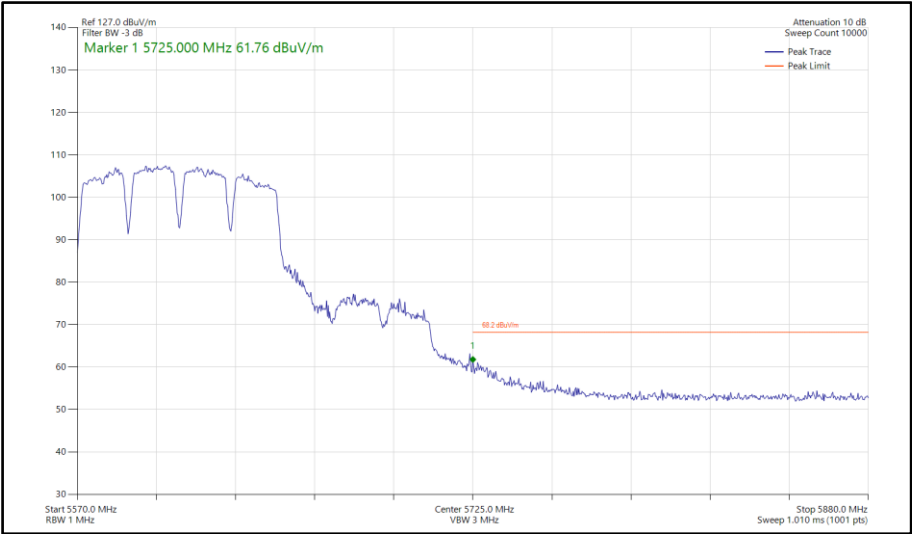
Figure 1071 - 802.11a a80, SISO, Core 1 - 5610 MHz Band Edge Frequency 5725 MHz
