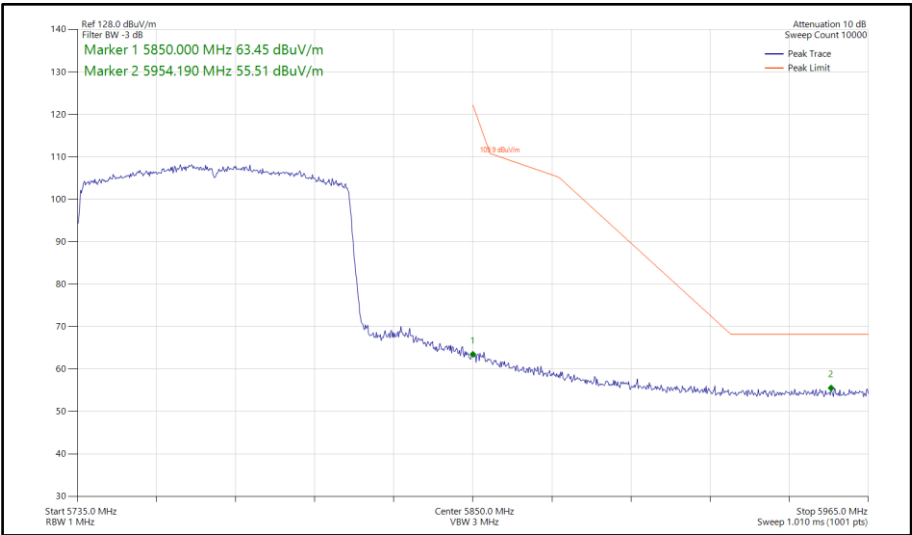
Figure 1082 - 802.11ax HE80, SU, SISO, Core 1 - 5775 MHz Band Edge Frequency 5850 MHz
