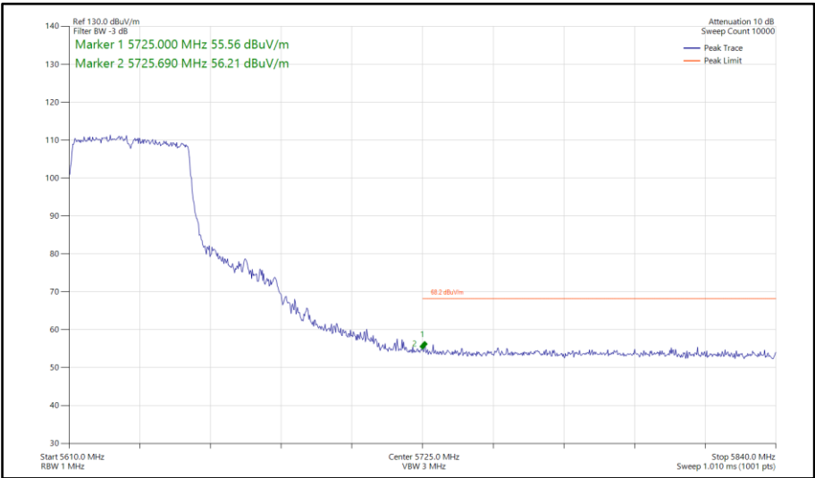
Figure 1030 - 802.11ax HE40, SU, TxBF, Core 0-1 - 5630 MHz Band Edge Frequency 5725 MHz
