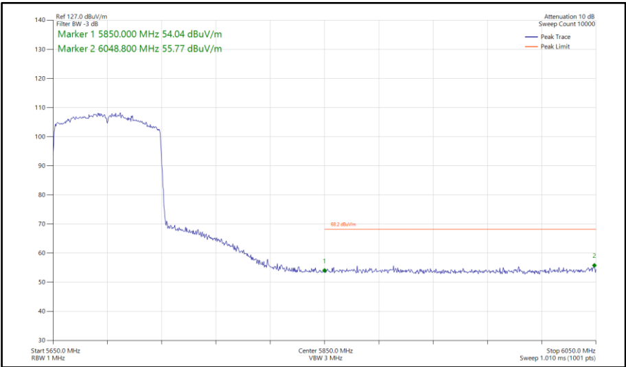
Figure 1055 - 802.11ax HE80, SU, SISO, Core 0 - 5690 MHz Band Edge Frequency 5850 MHz
