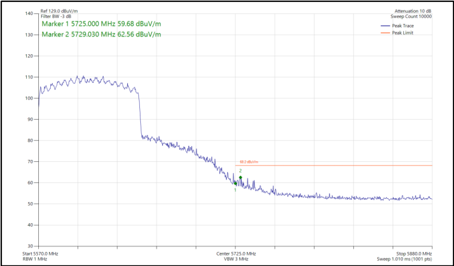
Figure 1098 - 802.11ax HE80, SU, CDD, Core 0-1 - 5610 MHz Band Edge Frequency 5725 MHz
