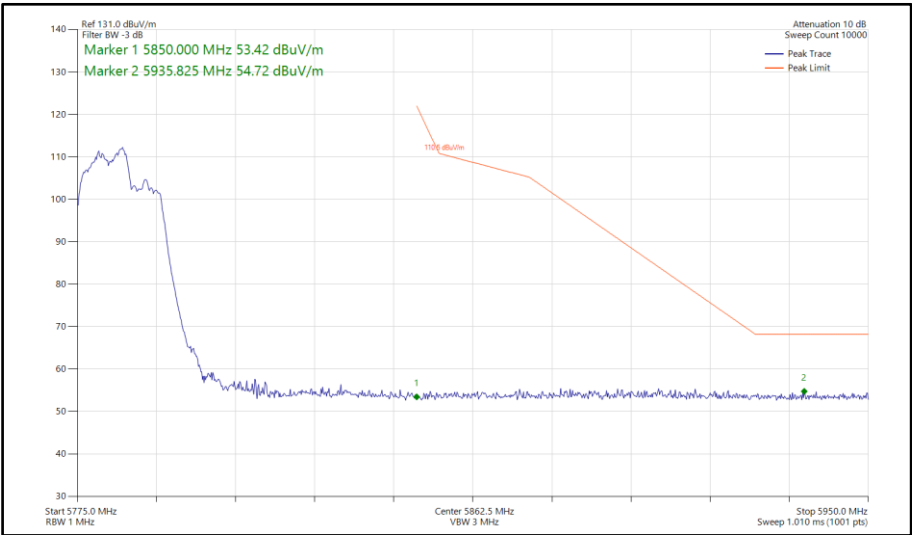
Figure 1019 - 802.11be EHT40, RU 106+26-82, SDM, Core 0-1 - 5795 MHz Band Edge Frequency 5850 MHz
