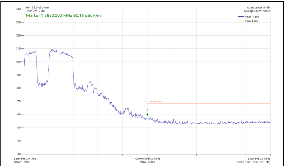
Figure 1084 - 802.11be EHT80, RU 484+242-91, SISO, Core 1 - 5690 MHz Band Edge Frequency 5850 MHz
