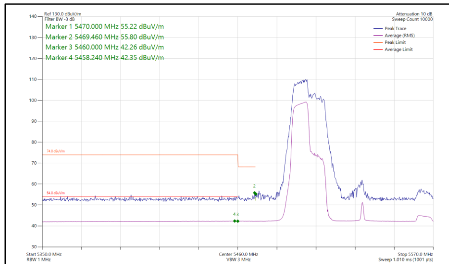
Figure 1064 - 802.11ax HE80, RU 106-53, SISO, Core 1 - 5530 MHz Band Edge Frequency 5470 MHz
