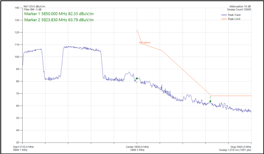
Figure 1060 - 802.11be EHT80, RU 484+242-91, SISO, Core 0 - 5775 MHz Band Edge Frequency 5850 MHz
