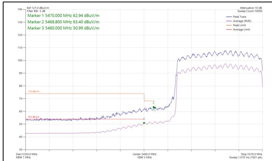
Figure 1088 - 802.11ax HE80, SU, CDD, Core 0-1 - 5530 MHz Band Edge Frequency 5470 MHz
