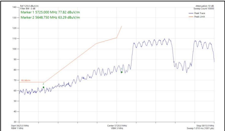
Figure 1095 - 802.11be EHT80, RU 484+242-92, CDD, Core 0-1 - 5775 MHz Band Edge Frequency 5725 MHz
