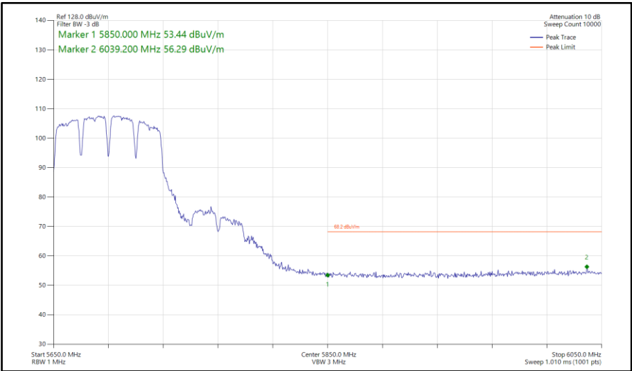
Figure 1076 - 802.11a a80, SISO, Core 1 - 5690 MHz Band Edge Frequency 5850 MHz
