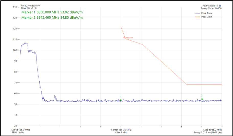
Figure 1058 - 802.11ax HE80, RU 106-53, SISO, Core 0 - 5775 MHz Band Edge Frequency 5850 MHz
