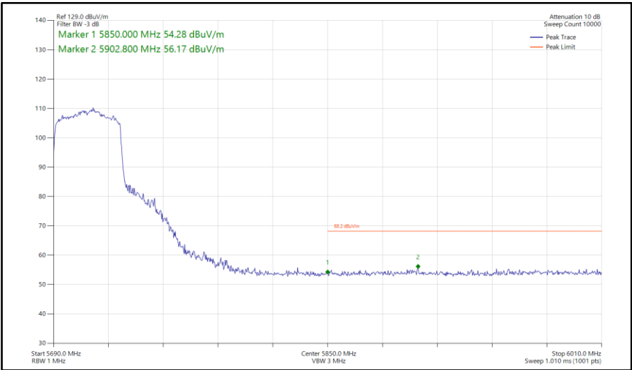
Figure 1034 - 802.11ax HE40, SU, TxBF, Core 0-1 - 5710 MHz Band Edge Frequency 5850 MHz
