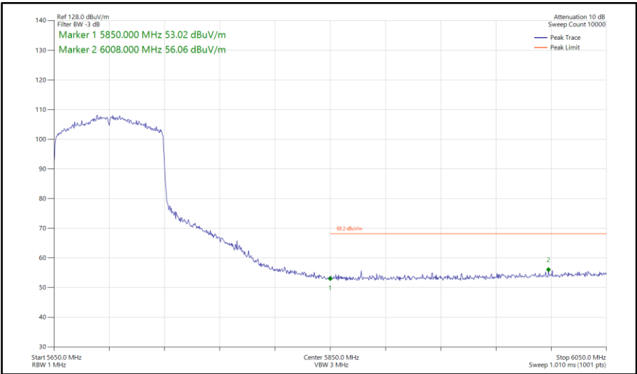
Figure 1080 - 802.11ax HE80, SU, SISO, Core 1 - 5690 MHz Band Edge Frequency 5850 MHz
