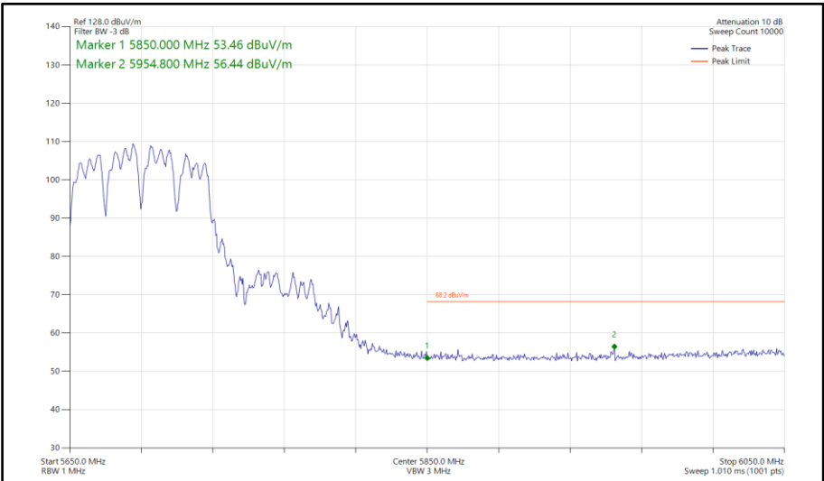
Figure 1101 - 802.11a a80, CDD, Core 0-1 - 5690 MHz Band Edge Frequency 5850 MHz
