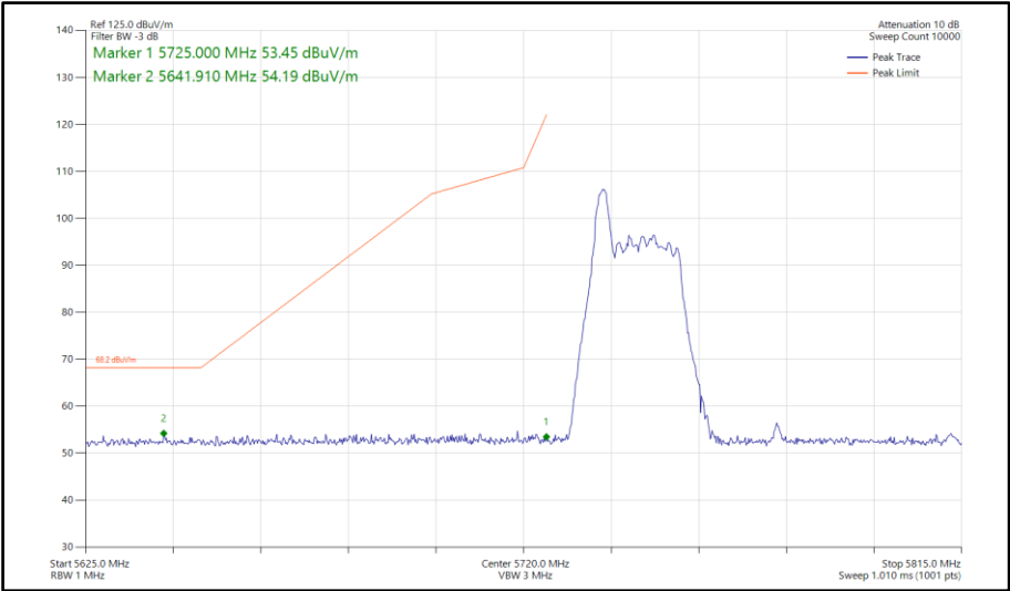
Figure 1069 - 802.11ax HE80, RU 26-0, SISO, Core 1 - 5775 MHz Band Edge Frequency 5725 MHz
