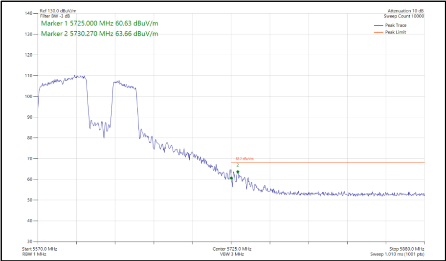
Figure 1075 - 802.11be EHT80, RU 484+242-92, SISO, Core 1 - 5610 MHz Band Edge Frequency 5725 MHz
