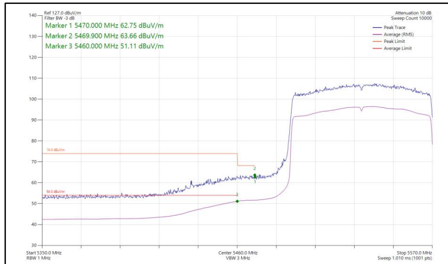
Figure 1063 - 802.11ax HE80, SU, SISO, Core 1 - 5530 MHz Band Edge Frequency 5470 MHz
