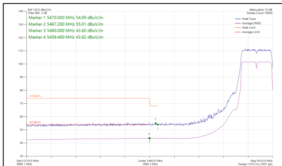
Figure 1022 - 802.11ac VHT40, TxBF, Core 0-1 - 5590 MHz Band Edge Frequency 5470 MHz
