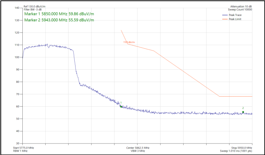
Figure 1035 - 802.11ax HE40, SU, TxBF, Core 0-1 - 5795 MHz Band Edge Frequency 5850 MHz
