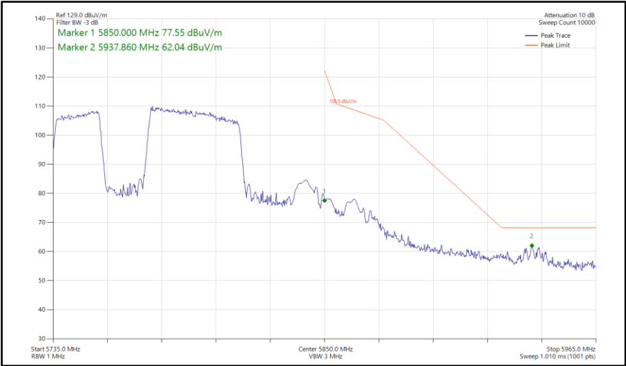
Figure 1085 - 802.11be EHT80, RU 484+242-91, SISO, Core 1 - 5775 MHz Band Edge Frequency 5850 MHz
