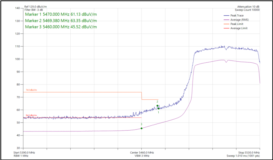
Figure 1023 - 802.11ax HE40, SU, TxBF, Core 0-1 - 5510 MHz Band Edge Frequency 5470 MHz
