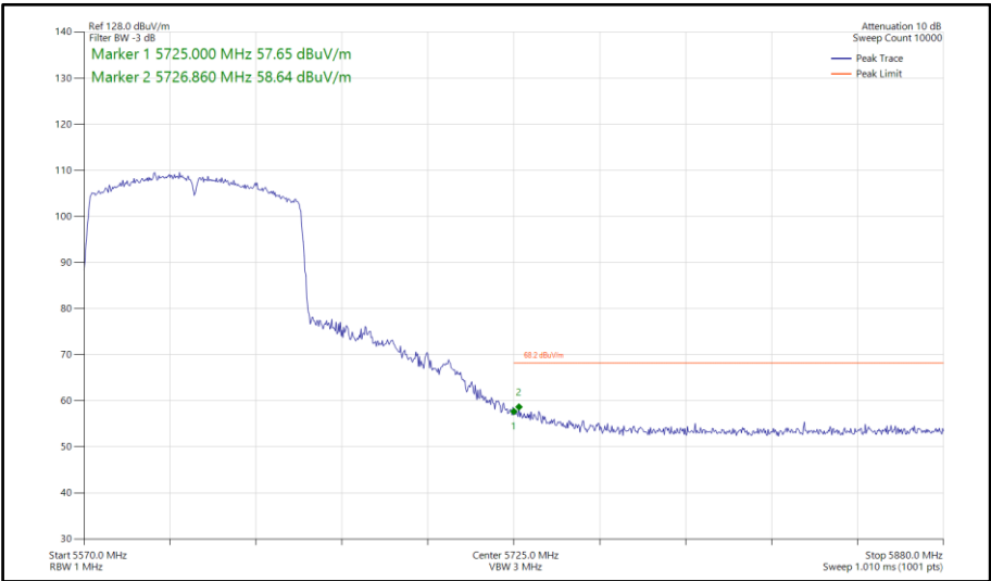
Figure 1047 - 802.11ac VHT80, SISO, Core 0 - 5610 MHz Band Edge Frequency 5725 MHz
