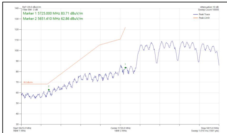
Figure 1091 - 802.11a a80, CDD, Core 0-1 - 5775 MHz Band Edge Frequency 5725 MHz
