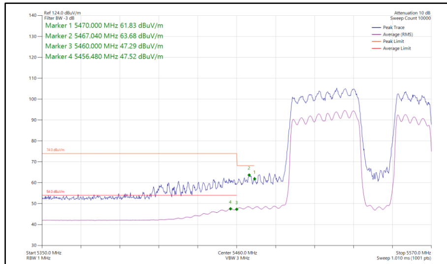
Figure 1090 - 802.11be EHT80, RU 484+242-92, CDD, Core 0-1 - 5530 MHz Band Edge Frequency 5470 MHz
