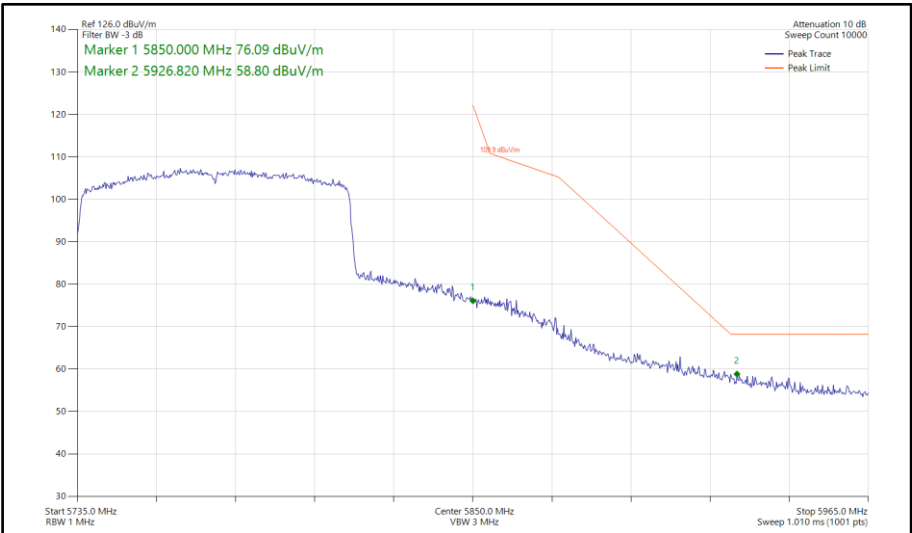
Figure 1057 - 802.11ax HE80, SU, SISO, Core 0 - 5775 MHz Band Edge Frequency 5850 MHz
