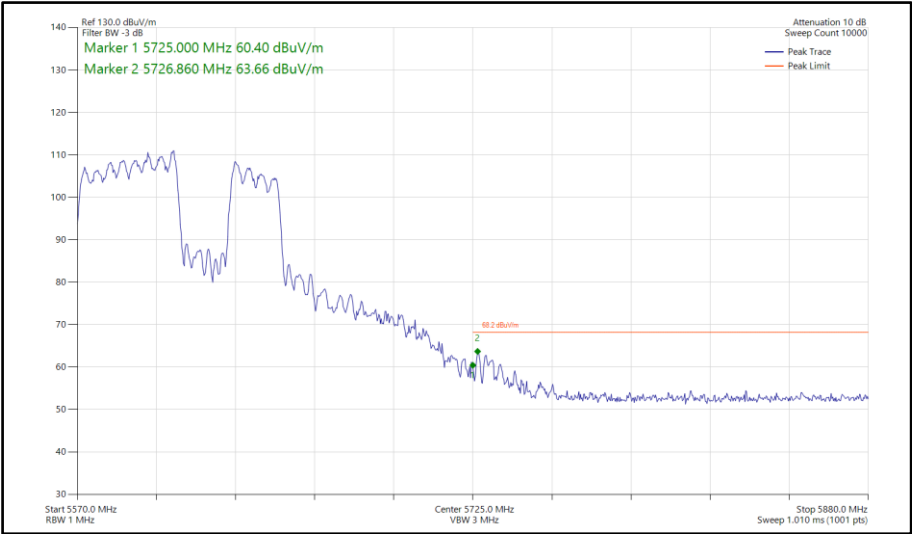
Figure 1100 - 802.11be EHT80, RU 484+242-92, CDD, Core 0-1 - 5610 MHz Band Edge Frequency 5725 MHz
