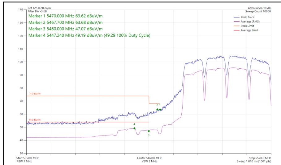
Figure 1061 - 802.11a a80, SISO, Core 1 - 5530 MHz Band Edge Frequency 5470 MHz
