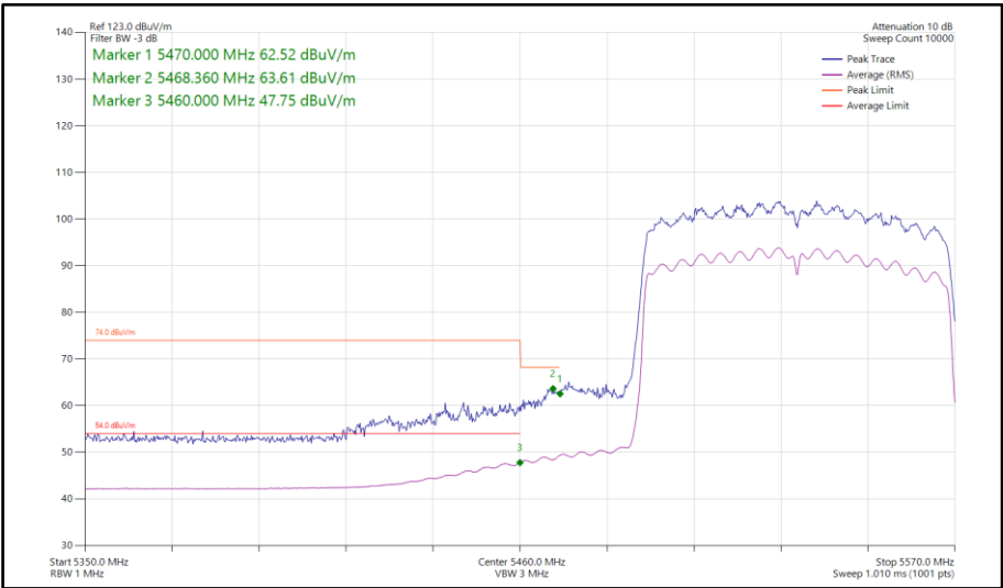
Figure 1087 - 802.11ac VHT80, CDD, Core 0-1 - 5530 MHz Band Edge Frequency 5470 MHz
