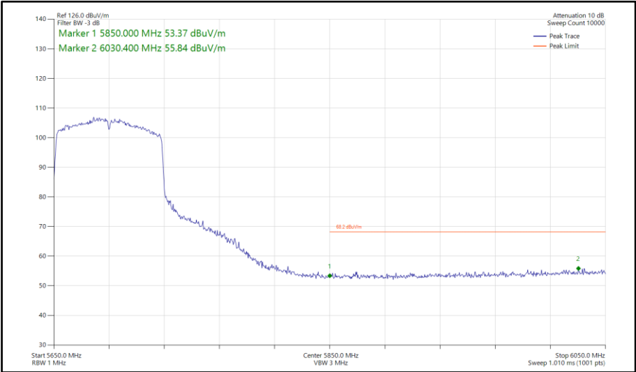
Figure 1078 - 802.11ac VHT80, SISO, Core 1 - 5690 MHz Band Edge Frequency 5850 MHz
