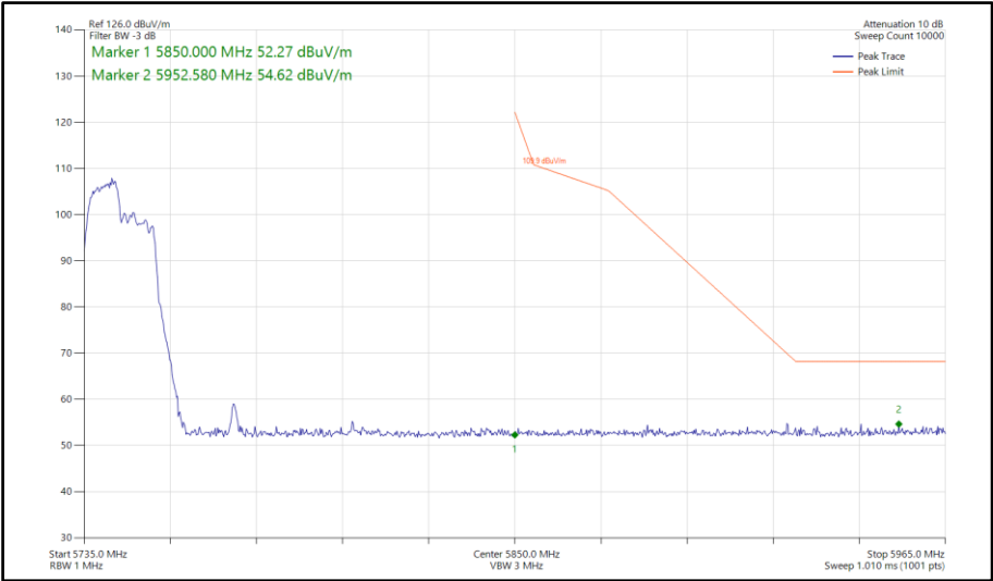
Figure 1083 - 802.11ax HE80, RU 106-53, SISO, Core 1 - 5775 MHz Band Edge Frequency 5850 MHz
