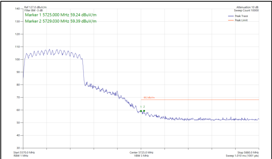
Figure 1097 - 802.11ac VHT80, CDD, Core 0-1 - 5610 MHz Band Edge Frequency 5725 MHz
