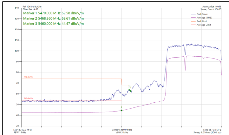
Figure 1065 - 802.11be EHT80, RU 484+242-90, SISO, Core 1 - 5530 MHz Band Edge Frequency 5470 MHz
