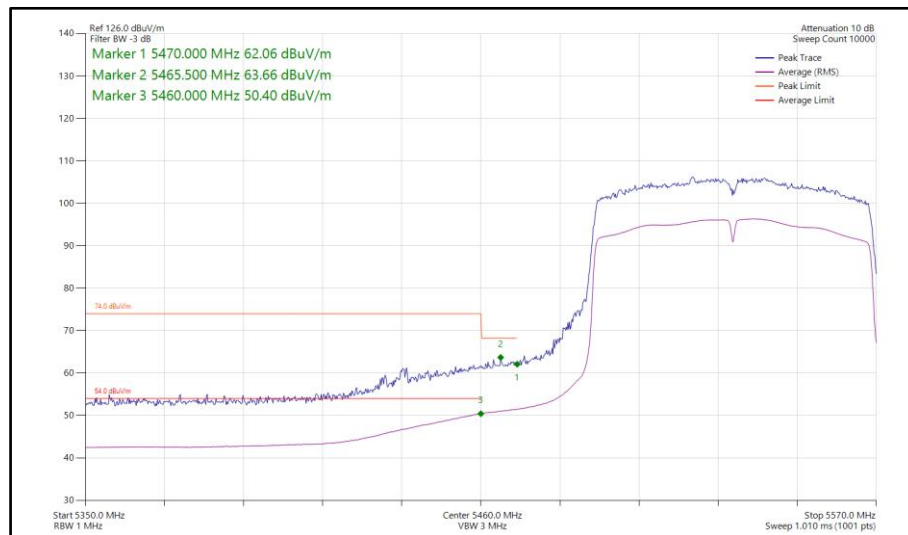
Figure 1062 - 802.11ac VHT80, SISO, Core 1 - 5530 MHz Band Edge Frequency 5470 MHz
