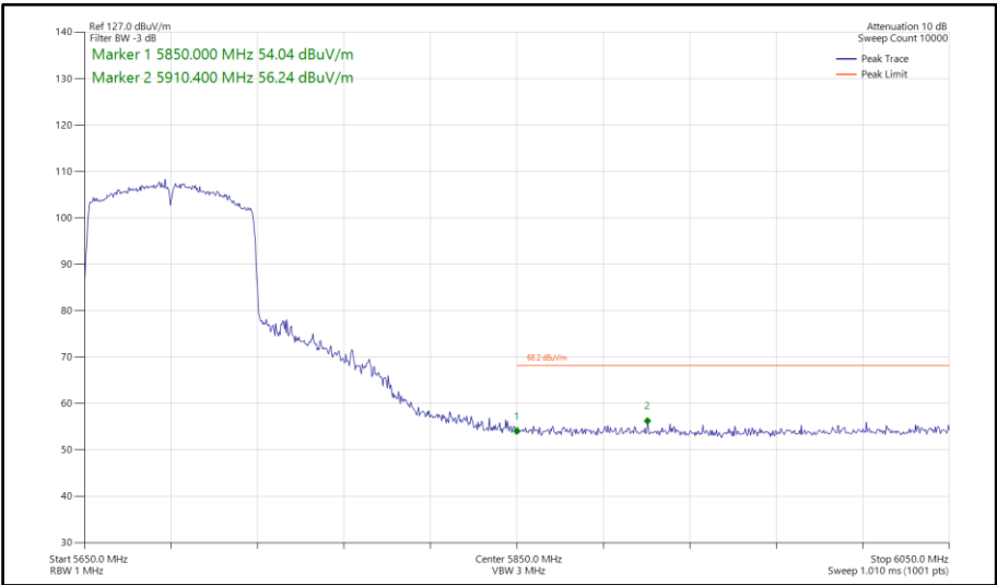
Figure 1053 - 802.11ac VHT80, SISO, Core 0 - 5690 MHz Band Edge Frequency 5850 MHz
