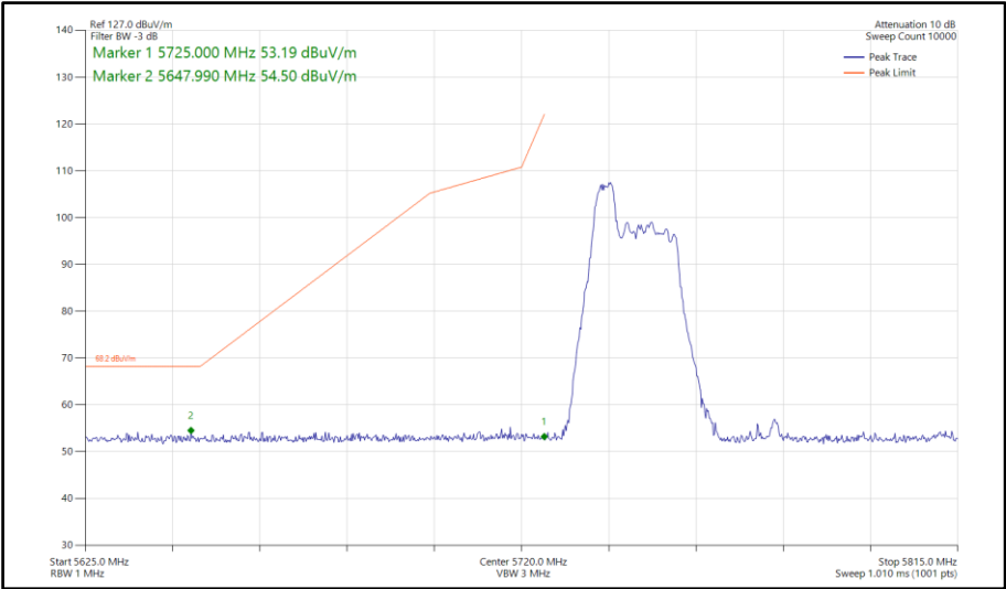
Figure 1044 - 802.11ax HE80, RU 52-37, SISO, Core 0 - 5775 MHz Band Edge Frequency 5725 MHz
