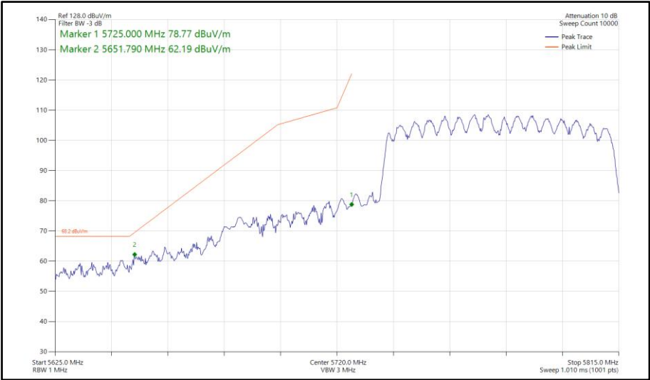
Figure 1092 - 802.11ac VHT80, CDD, Core 0-1 - 5775 MHz Band Edge Frequency 5725 MHz
