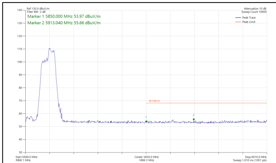
Figure 1015 - 802.11ax HE40, RU 106-56, SDM, Core 0-1 - 5710 MHz Band Edge Frequency 5850 MHz
