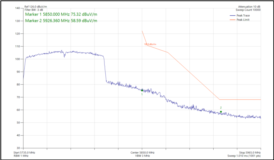
Figure 1054 - 802.11ac VHT80, SISO, Core 0 - 5775 MHz Band Edge Frequency 5850 MHz
