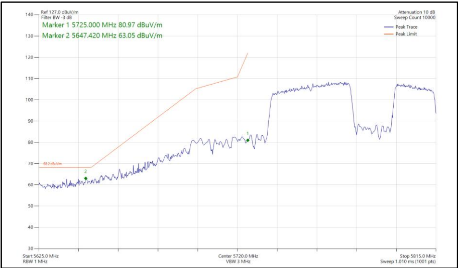
Figure 1045 - 802.11be EHT80, RU 484+242-92, SISO, Core 0 - 5775 MHz Band Edge Frequency 5725 MHz
