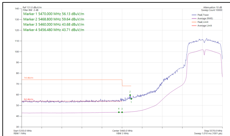
Figure 1021 - 802.11ac VHT40, TxBF, Core 0-1 - 5550 MHz Band Edge Frequency 5470 MHz
