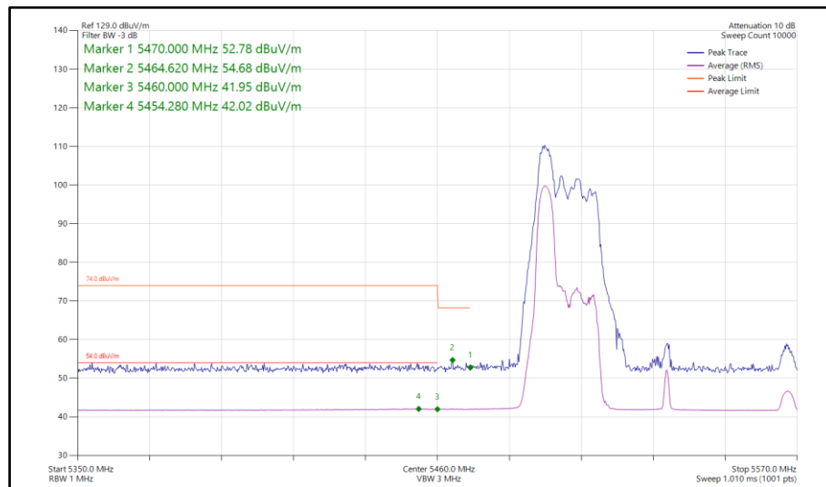
Figure 1089 - 802.11ax HE80, RU 52-37, CDD, Core 0-1 - 5530 MHz Band Edge Frequency 5470 MHz
