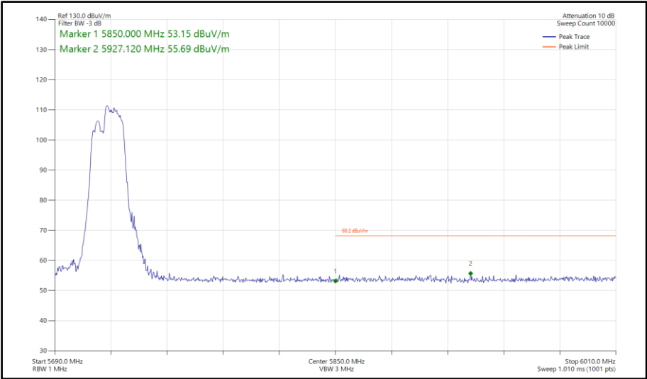
Figure 1018 - 802.11be EHT40, RU 106+26-85, SDM, Core 0-1 - 5710 MHz Band Edge Frequency 5850 MHz
