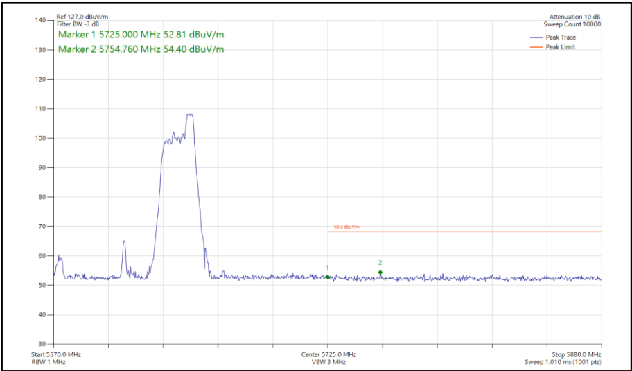
Figure 1099 - 802.11ax HE80, RU 52-52, CDD, Core 0-1 - 5610 MHz Band Edge Frequency 5725 MHz
