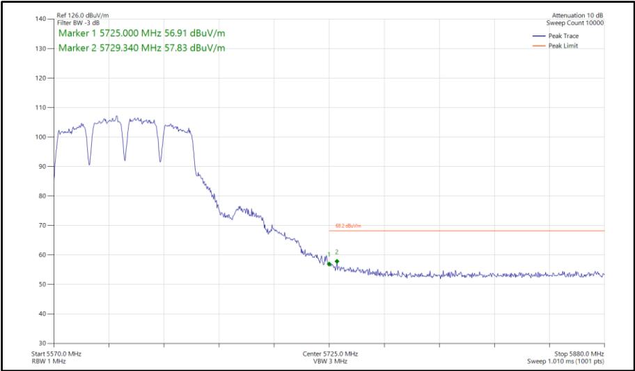
Figure 1046 - 802.11a a80, SISO, Core 0 - 5610 MHz Band Edge Frequency 5725 MHz
