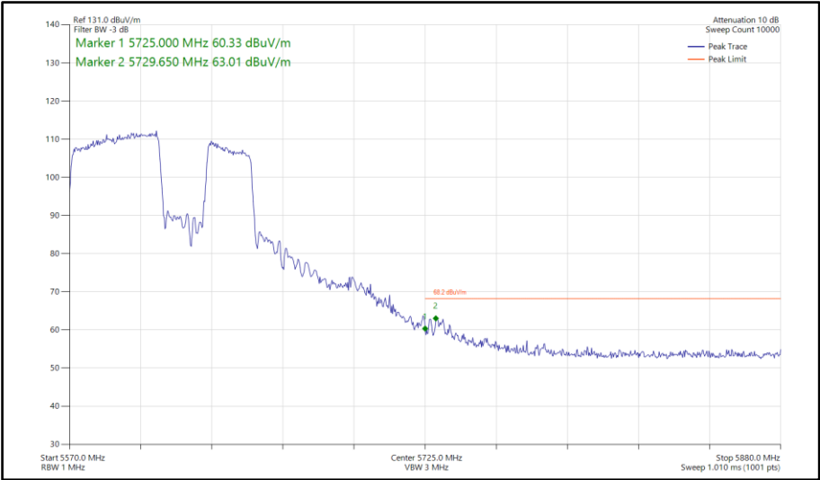
Figure 1050 - 802.11be EHT80, RU 484+242-92, SISO, Core 0 - 5610 MHz Band Edge Frequency 5725 MHz
