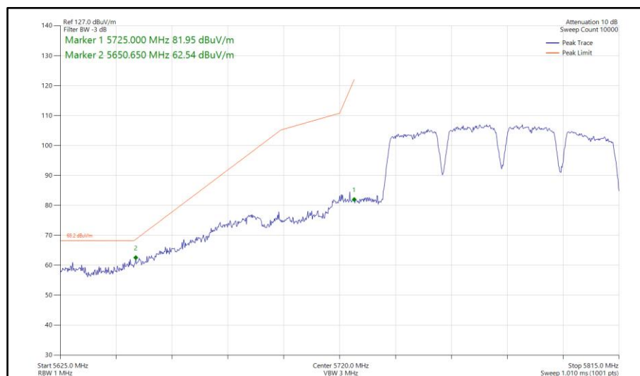
Figure 1066 - 802.11a a80, SISO, Core 1 - 5775 MHz Band Edge Frequency 5725 MHz
