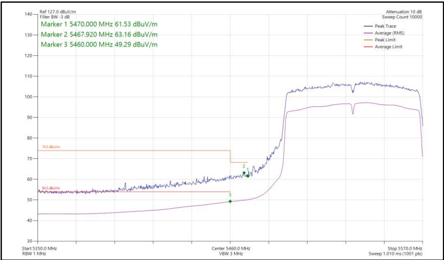
Figure 1037 - 802.11ac VHT80, SISO, Core 0 - 5530 MHz Band Edge Frequency 5470 MHz
