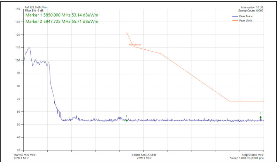
Figure 1017 - 802.11ax HE40, RU 52-37, SDM, Core 0-1 - 5795 MHz Band Edge Frequency 5850 MHz
