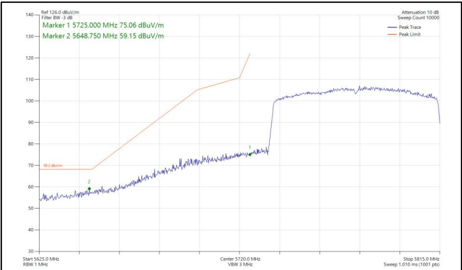
Figure 1068 - 802.11ax HE80, SU, SISO, Core 1 - 5775 MHz Band Edge Frequency 5725 MHz
