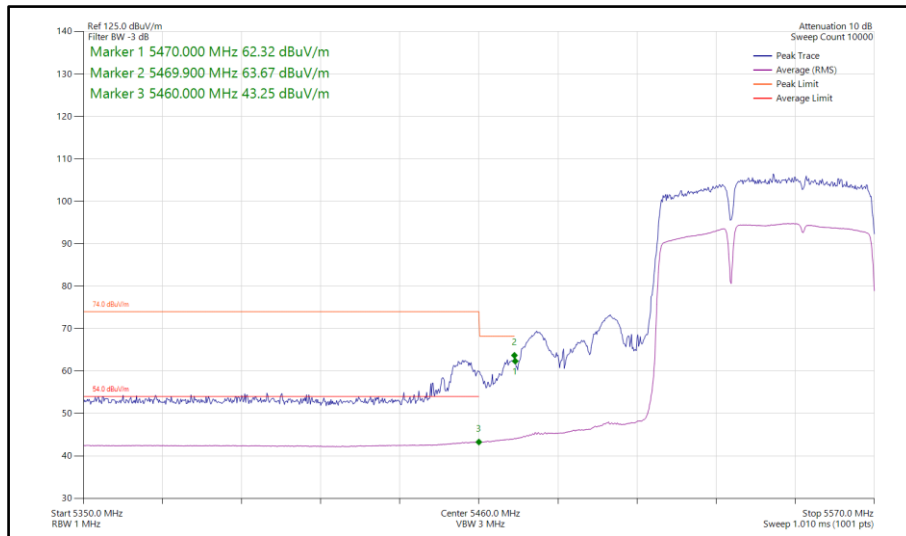
Figure 1040 - 802.11be EHT80, RU 484+242-90, SISO, Core 0 - 5530 MHz Band Edge Frequency 5470 MHz
