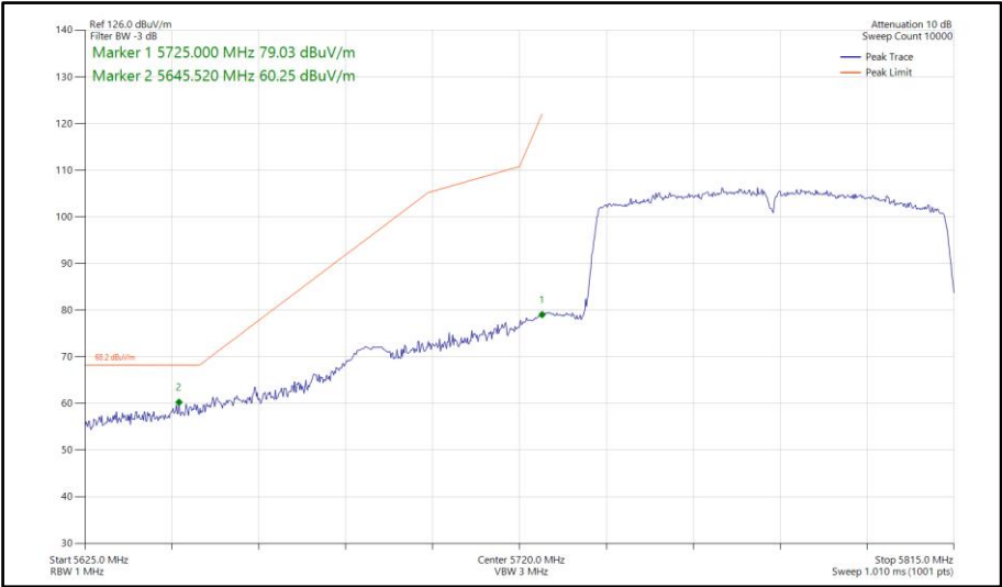
Figure 1067 - 802.11ac VHT80, SISO, Core 1 - 5775 MHz Band Edge Frequency 5725 MHz
