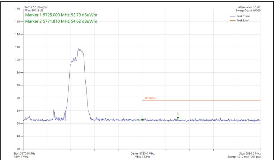
Figure 1074 - 802.11ax HE80, RU 106-60, SISO, Core 1 - 5610 MHz Band Edge Frequency 5725 MHz
