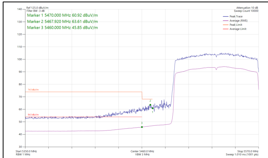
Figure 1038 - 802.11ax HE80, SU, SISO, Core 0 - 5530 MHz Band Edge Frequency 5470 MHz
