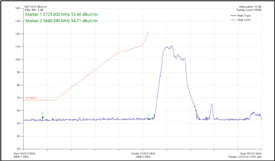
Figure 1094 - 802.11ax HE80, RU 106-53, CDD, Core 0-1 - 5775 MHz Band Edge Frequency 5725 MHz
