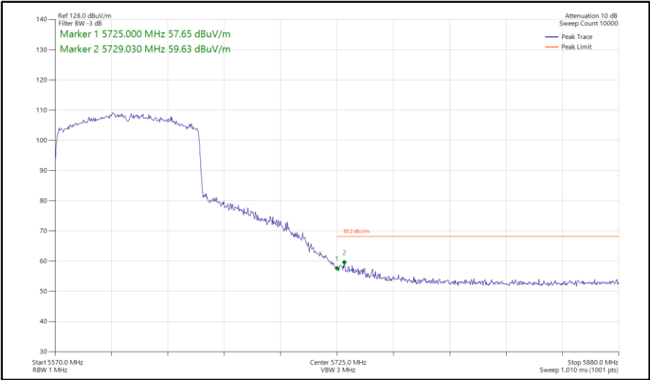
Figure 1073 - 802.11ax HE80, SU, SISO, Core 1 - 5610 MHz Band Edge Frequency 5725 MHz
