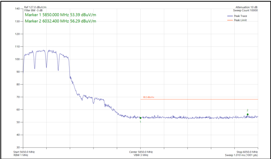
Figure 1051 - 802.11a a80, SISO, Core 0 - 5690 MHz Band Edge Frequency 5850 MHz
