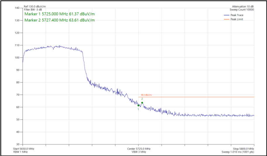
Figure 1031 - 802.11ax HE40, SU, TxBF, Core 0-1 - 5670 MHz Band Edge Frequency 5725 MHz
