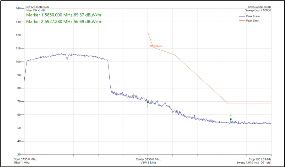
Figure 1079 - 802.11ac VHT80, SISO, Core 1 - 5775 MHz Band Edge Frequency 5850 MHz
