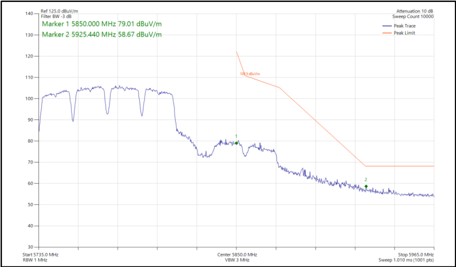
Figure 1052 - 802.11a a80, SISO, Core 0 - 5775 MHz Band Edge Frequency 5850 MHz
