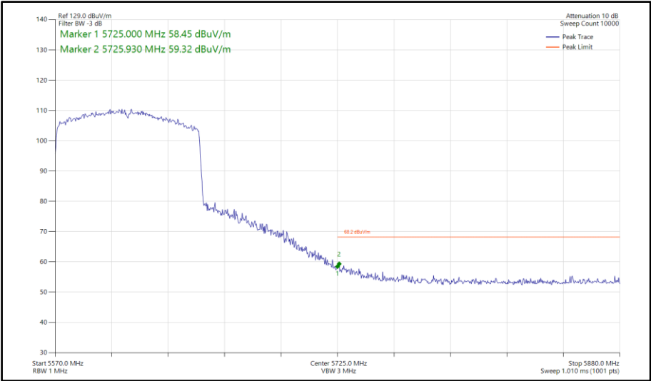
Figure 1048 - 802.11ax HE80, SU, SISO, Core 0 - 5610 MHz Band Edge Frequency 5725 MHz
