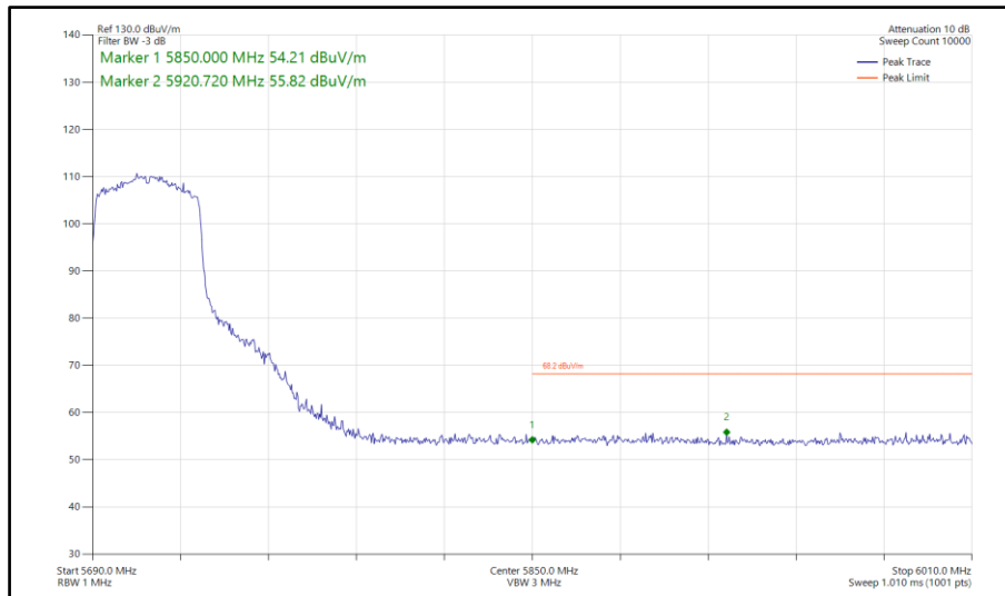
Figure 1014 - 802.11ax HE40, SU, SDM, Core 0-1 - 5710 MHz Band Edge Frequency 5850 MHz
