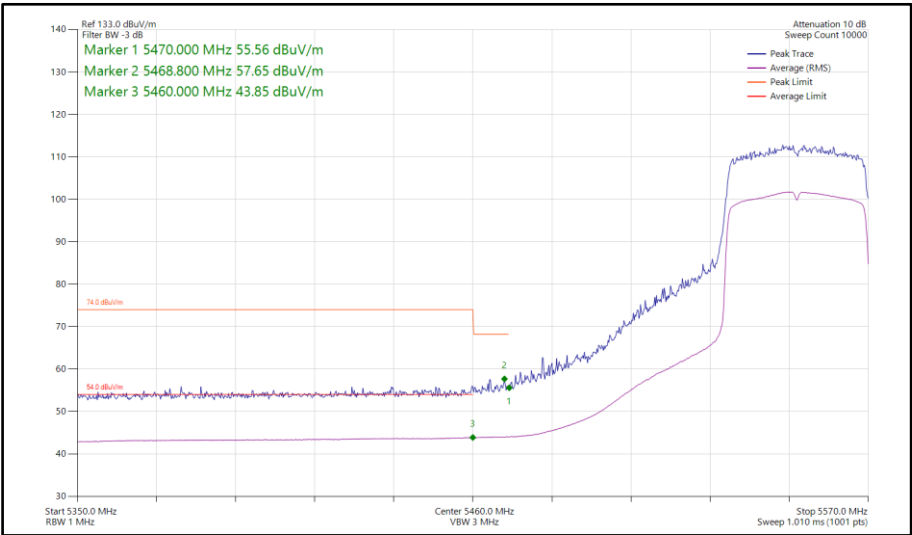
Figure 1024 - 802.11ax HE40, SU, TxBF, Core 0-1 - 5550 MHz Band Edge Frequency 5470 MHz
