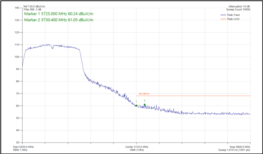
Figure 1029 - 802.11ac VHT40, TxBF, Core 0-1 - 5670 MHz Band Edge Frequency 5725 MHz
