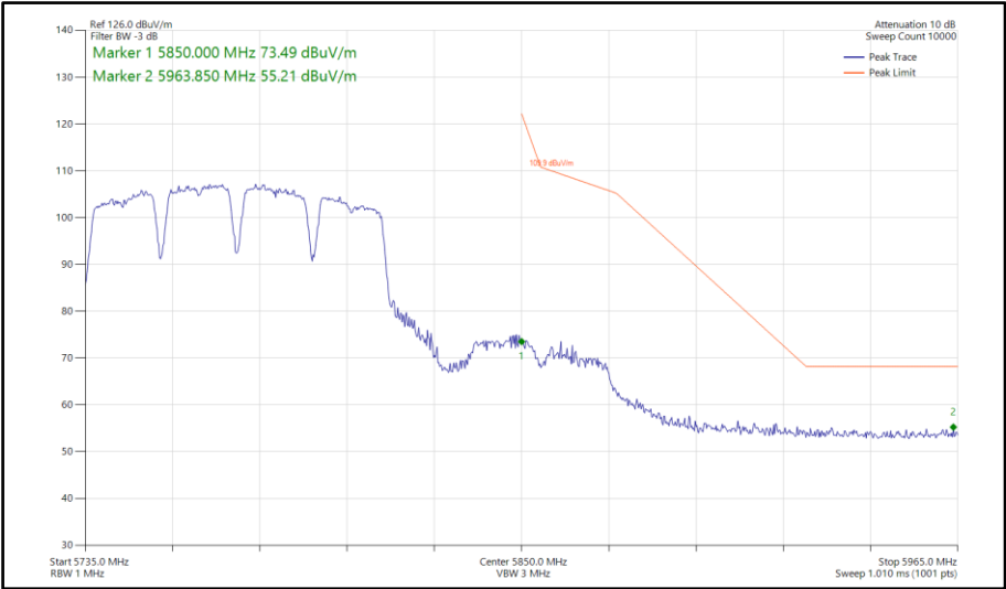
Figure 1077 - 802.11a a80, SISO, Core 1 - 5775 MHz Band Edge Frequency 5850 MHz
