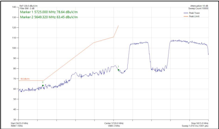
Figure 1070 - 802.11be EHT80, RU 484+242-91, SISO, Core 1 - 5775 MHz Band Edge Frequency 5725 MHz
