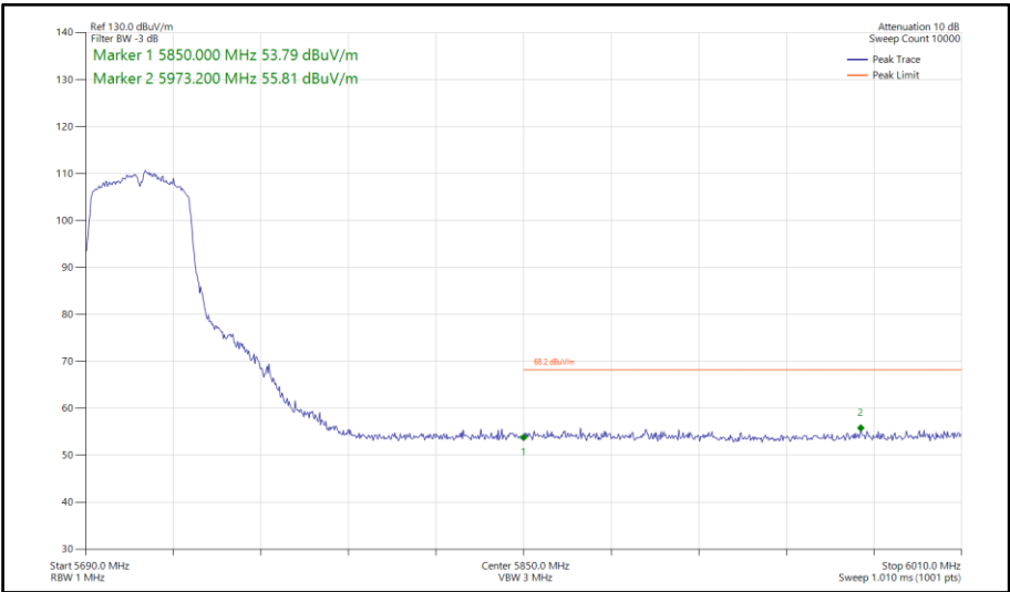
Figure 1032 - 802.11ac VHT40, TxBF, Core 0-1 - 5710 MHz Band Edge Frequency 5850 MHz
