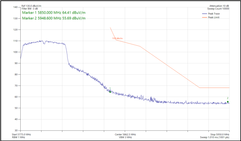
Figure 1033 - 802.11ac VHT40, TxBF, Core 0-1 - 5795 MHz Band Edge Frequency 5850 MHz
