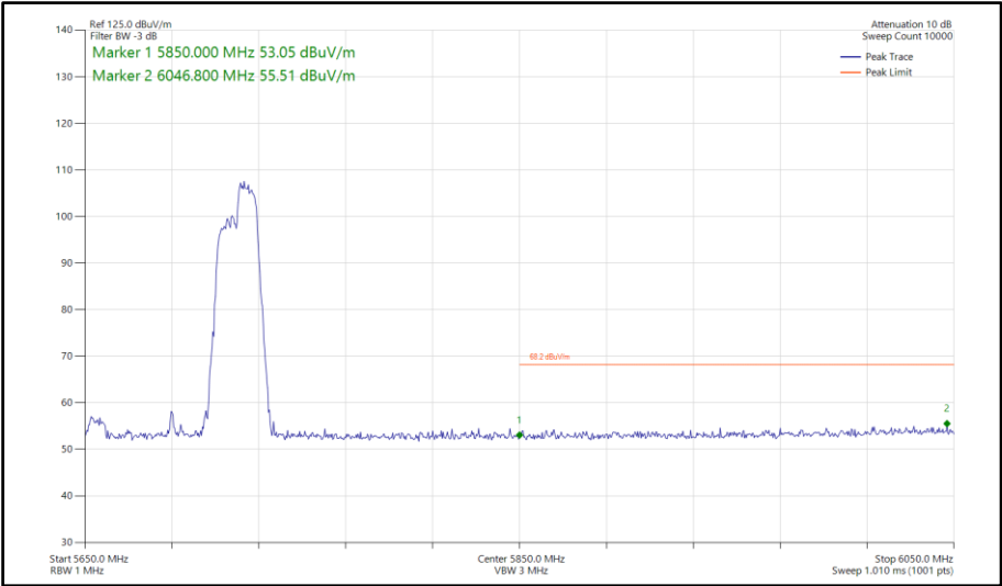
Figure 1056 - 802.11ax HE80, RU 106-60, SISO, Core 0 - 5690 MHz Band Edge Frequency 5850 MHz
