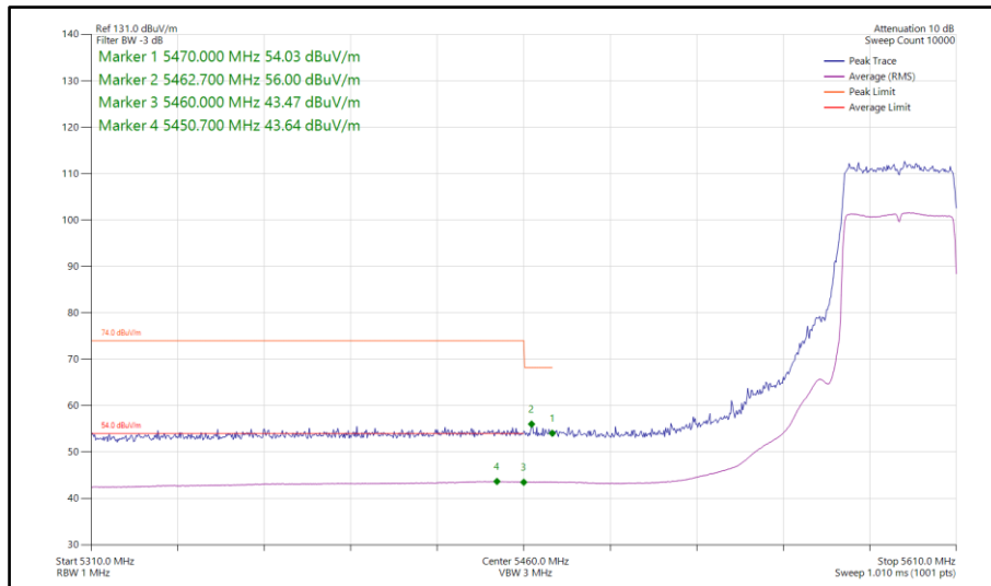
Figure 1025 - 802.11ax HE40, SU, TxBF, Core 0-1 - 5590 MHz Band Edge Frequency 5470 MHz
