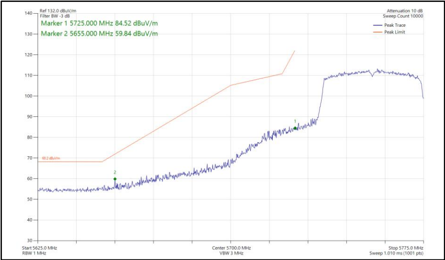
Figure 1027 - 802.11ax HE40, SU, TxBF, Core 0-1 - 5755 MHz Band Edge Frequency 5725 MHz
