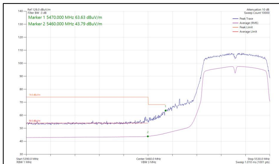
Figure 1020 - 802.11ac VHT40, TxBF, Core 0-1 - 5510 MHz Band Edge Frequency 5470 MHz
