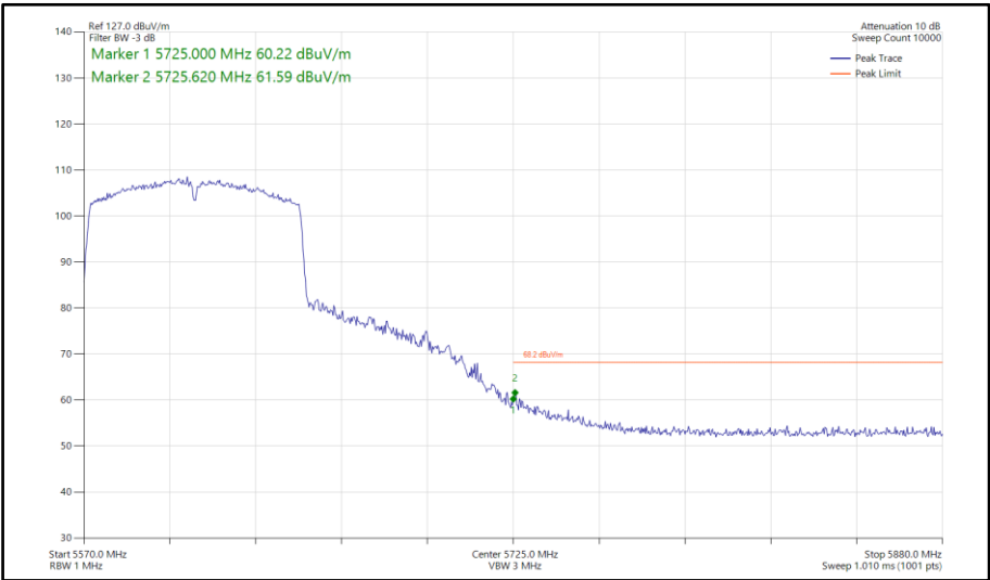
Figure 1072 - 802.11ac VHT80, SISO, Core 1 - 5610 MHz Band Edge Frequency 5725 MHz
