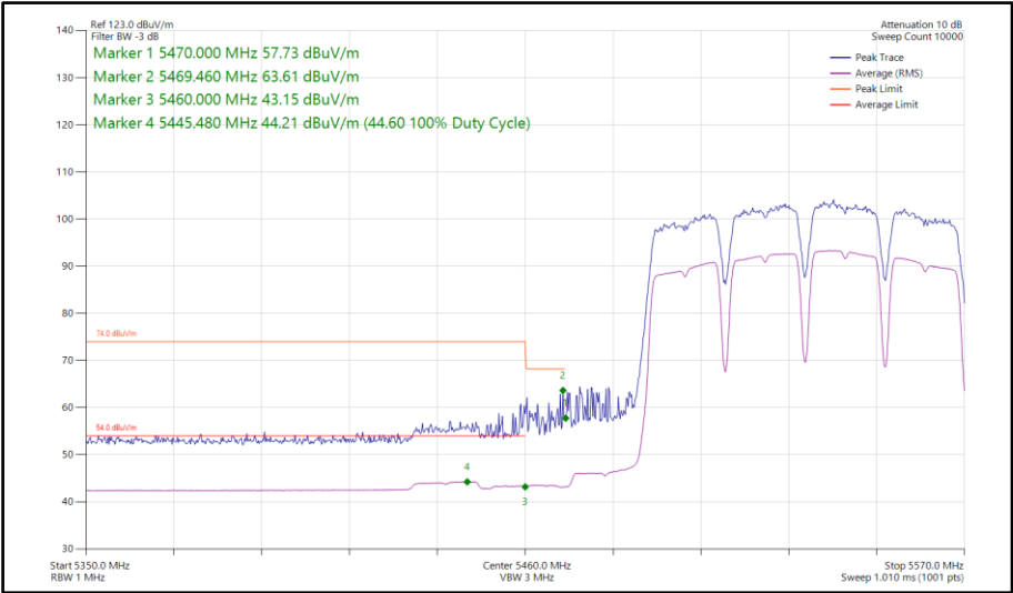
Figure 1036 - 802.11a a80, SISO, Core 0 - 5530 MHz Band Edge Frequency 5470 MHz
