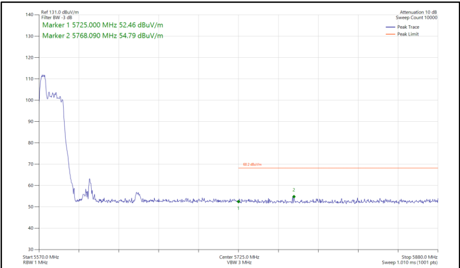
Figure 1049 - 802.11ax HE80, RU 52-37, SISO, Core 0 - 5610 MHz Band Edge Frequency 5725 MHz
