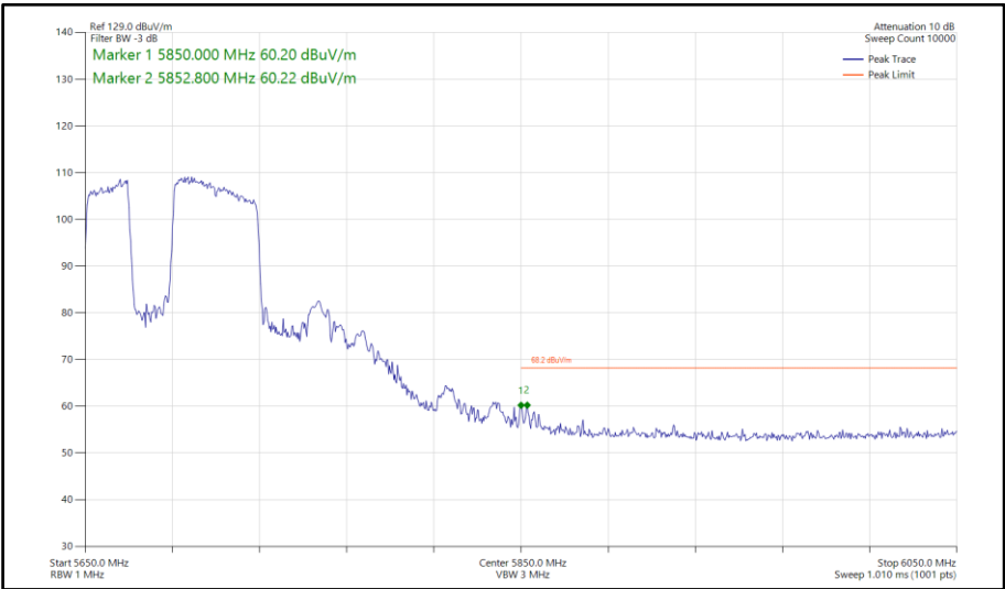
Figure 1059 - 802.11be EHT80, RU 484+242-91, SISO, Core 0 - 5690 MHz Band Edge Frequency 5850 MHz
