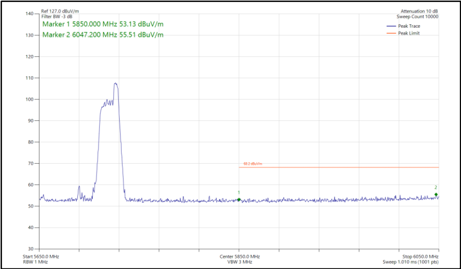
Figure 1081 - 802.11ax HE80, RU 52-52, SISO, Core 1 - 5690 MHz Band Edge Frequency 5850 MHz
