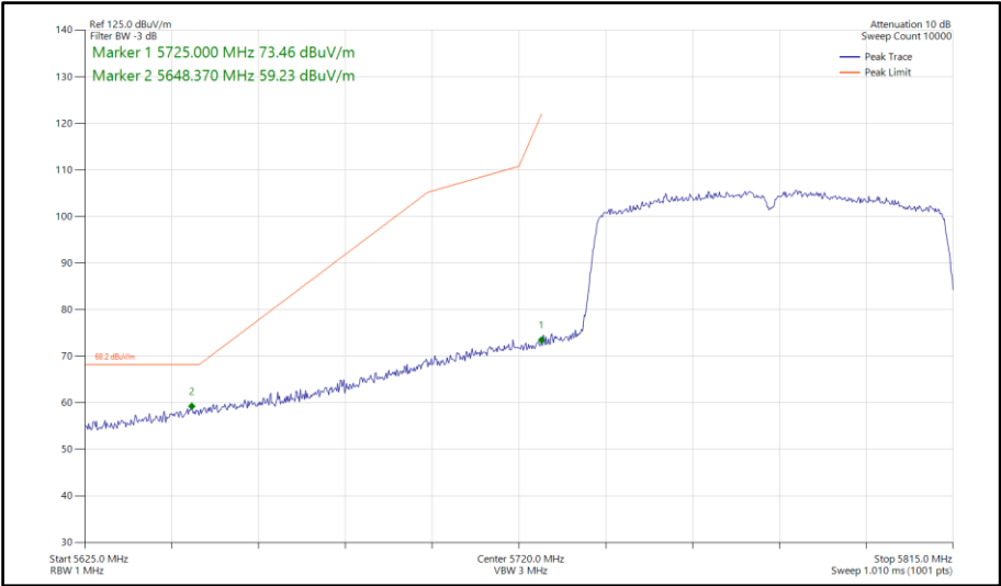
Figure 1042 - 802.11ac VHT80, SISO, Core 0 - 5775 MHz Band Edge Frequency 5725 MHz
