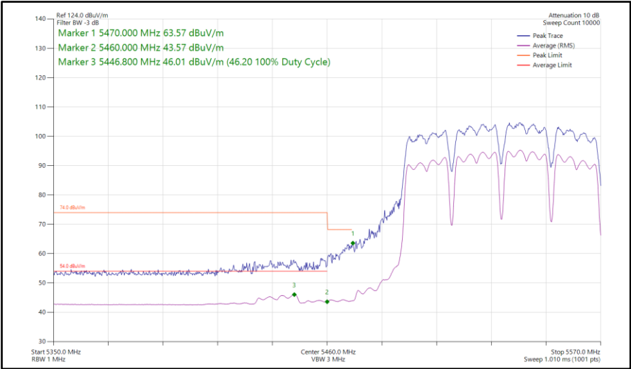
Figure 1086 - 802.11a a80, CDD, Core 0-1 - 5530 MHz Band Edge Frequency 5470 MHz
