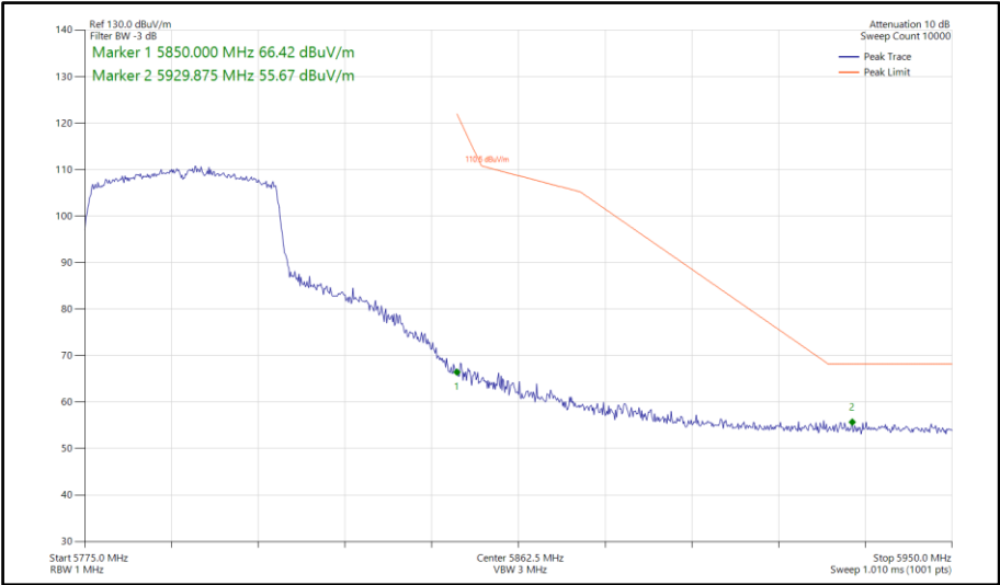
Figure 1016 - 802.11ax HE40, SU, SDM, Core 0-1 - 5795 MHz Band Edge Frequency 5850 MHz
