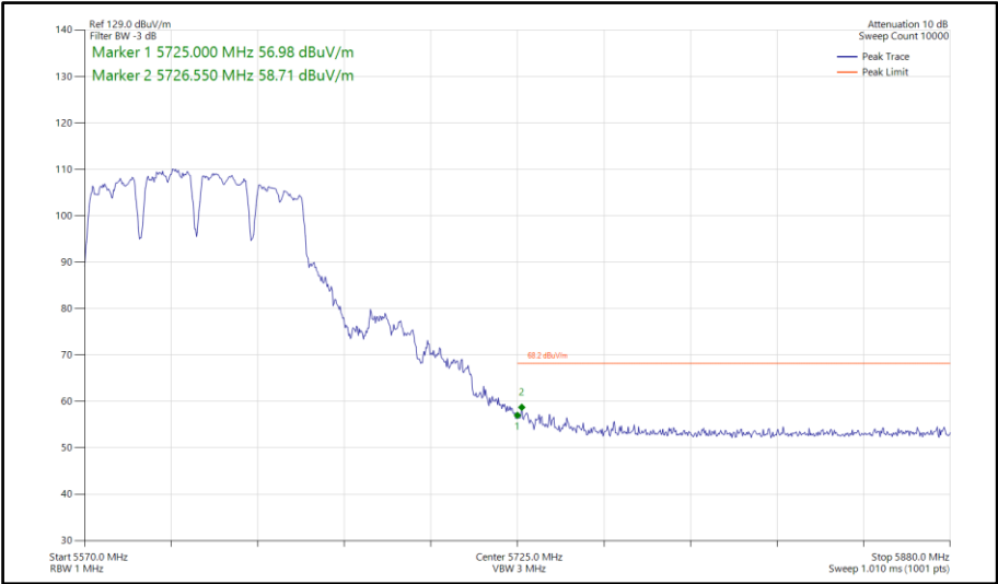
Figure 1096 - 802.11a a80, CDD, Core 0-1 - 5610 MHz Band Edge Frequency 5725 MHz
