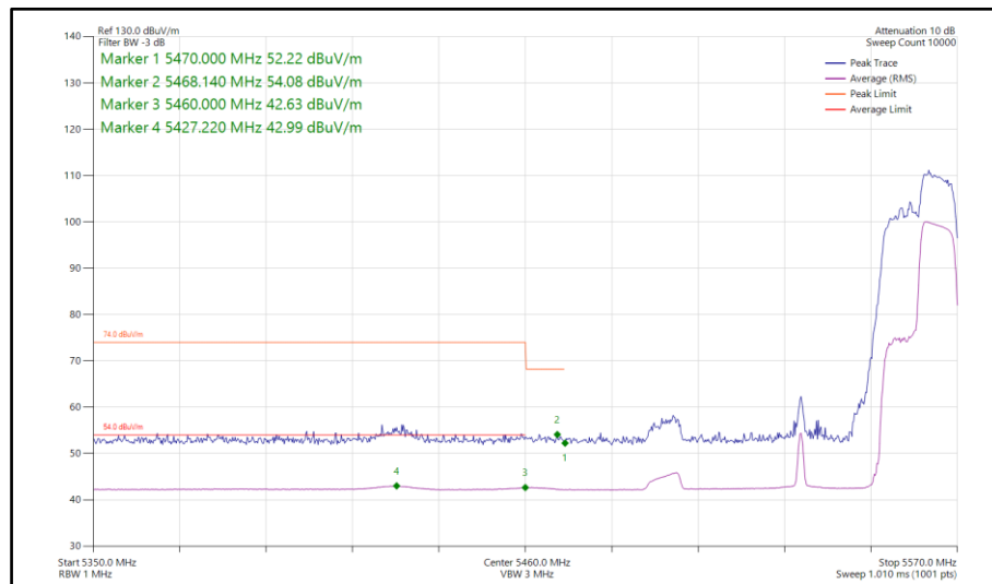
Figure 1039 - 802.11ax HE80, RU 106-60, SISO, Core 0 - 5530 MHz Band Edge Frequency 5470 MHz
