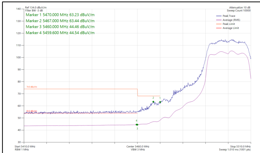
Figure 87 - 802.11n HT20, CDD, Core 0-1 - 5500 MHz Band Edge Frequency 5460 MHz
