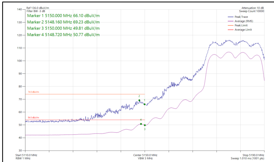
Figure 67 - 802.11n HT20, CDD, Core 0-1 - 5180 MHz Band Edge Frequency 5150 MHz
