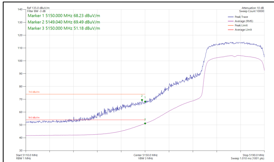
Figure 99 - 802.11ax HE20, SU, SDM, Core 0-1 - 5180 MHz Band Edge Frequency 5150 MHz
