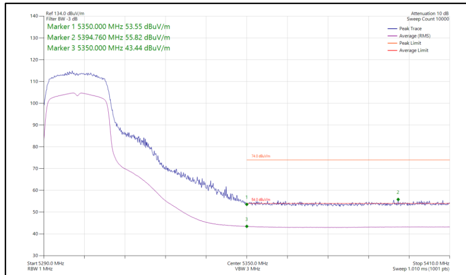
Figure 105 - 802.11n HT20, SDM, Core 0-1 - 5300 MHz Band Edge Frequency 5350 MHz
