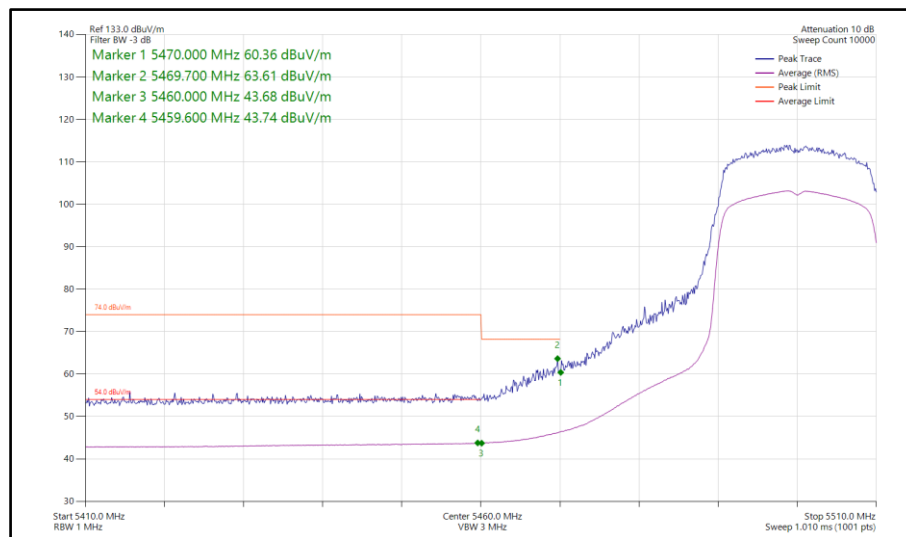
Figure 115 - 802.11ax HE20, SU, SDM, Core 0-1 - 5500 MHz Band Edge Frequency 5460 MHz
