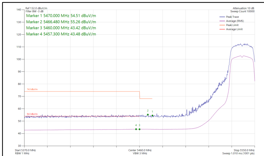
Figure 132 - 802.11ac VHT20, TxBF, Core 0-1 - 5540 MHz Band Edge Frequency 5460 MHz
