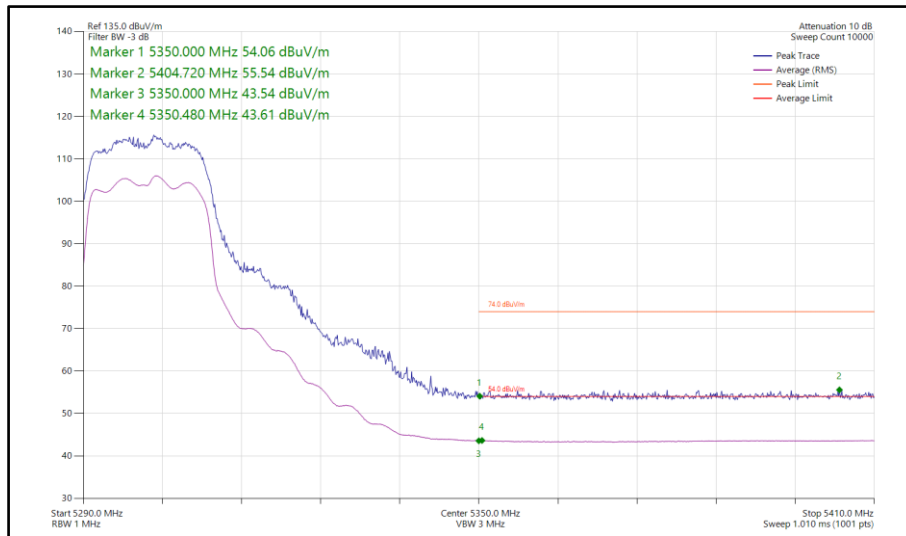
Figure 77 - 802.11n HT20, CDD, Core 0-1 - 5300 MHz Band Edge Frequency 5350 MHz
