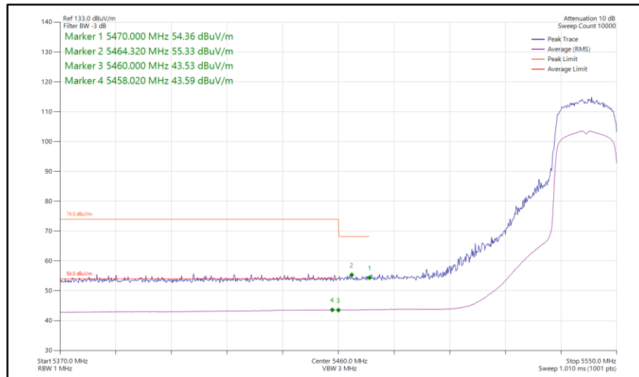
Figure 119 - 802.11ax HE20, SU, SDM, Core 0-1 - 5540 MHz Band Edge Frequency 5460 MHz
