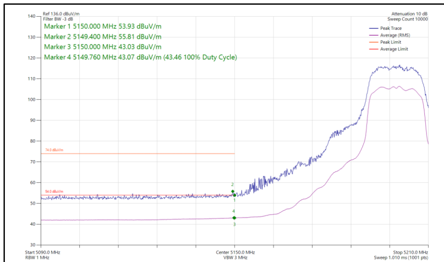
Figure 66 - 802.11a, CDD, Core 0-1 - 5200 MHz Band Edge Frequency 5150 MHz
