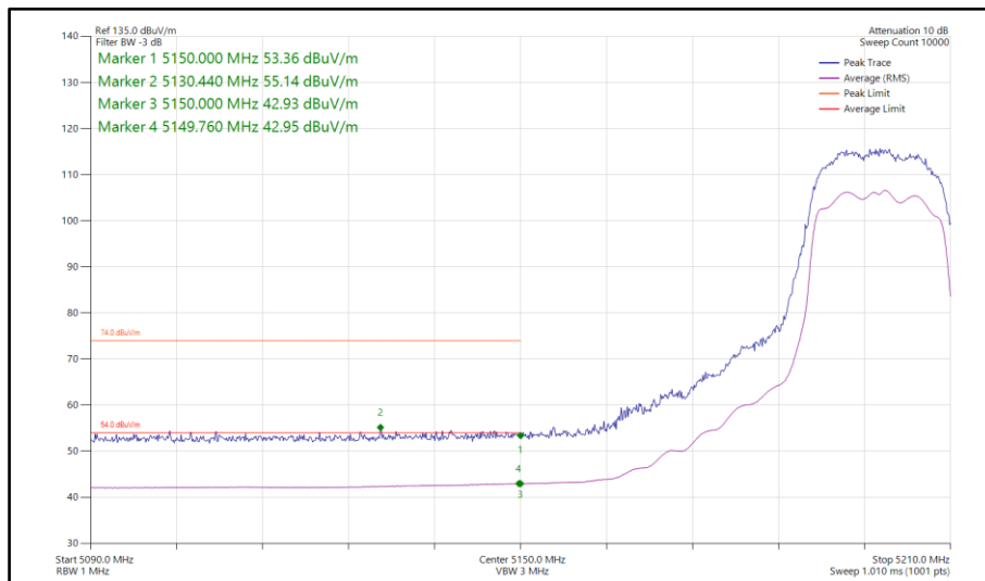
Figure 68 - 802.11n HT20, CDD, Core 0-1 - 5200 MHz Band Edge Frequency 5150 MHz
