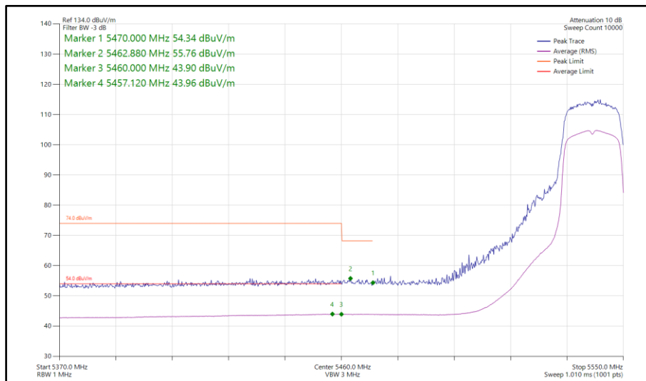
Figure 114 - 802.11n HT20, SDM, Core 0-1 - 5540 MHz Band Edge Frequency 5460 MHz
