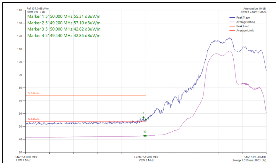
Figure 70 - 802.11ax HE20, RU 106-53, CDD, Core 0-1 - 5180 MHz Band Edge Frequency 5150 MHz
