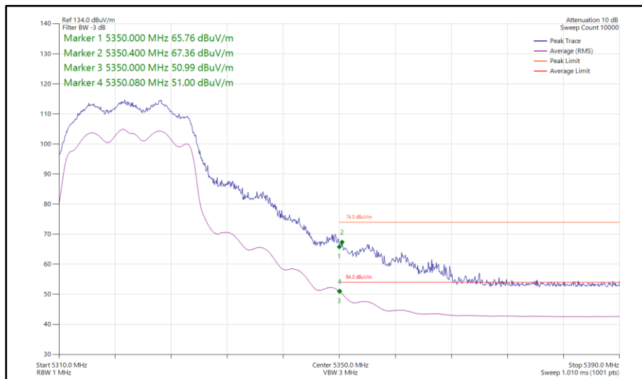
Figure 78 - 802.11n HT20, CDD, Core 0-1 - 5320 MHz Band Edge Frequency 5350 MHz
