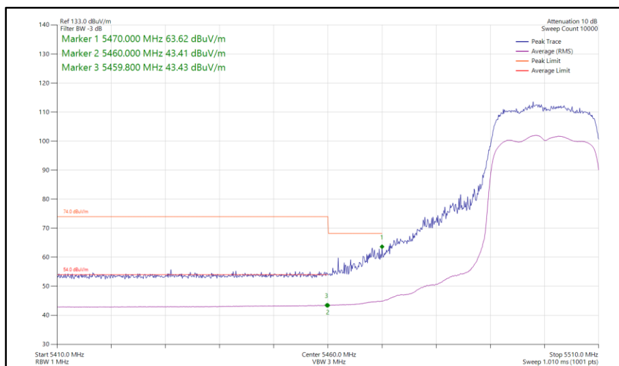
Figure 90 - 802.11ax HE20, SU, CDD, Core 0-1 - 5500 MHz Band Edge Frequency 5460 MHz
