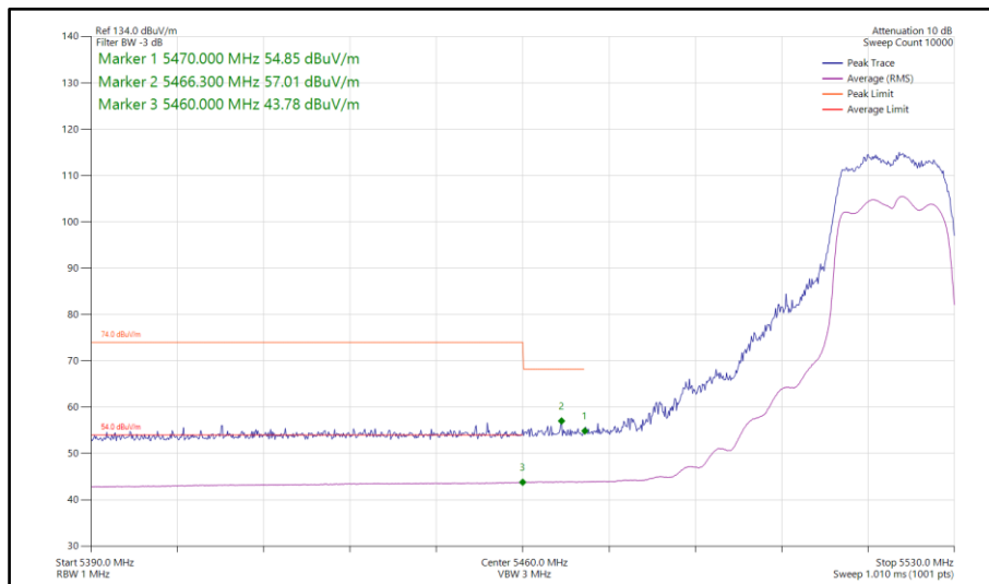
Figure 88 - 802.11n HT20, CDD, Core 0-1 - 5520 MHz Band Edge Frequency 5460 MHz
