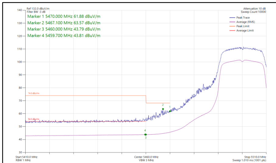
Figure 130 - 802.11ac VHT20, TxBF, Core 0-1 - 5500 MHz Band Edge Frequency 5460 MHz
