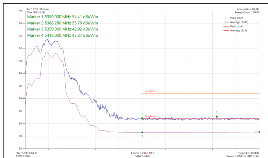
Figure 82 - 802.11be EHT20, RU 106+26-83, CDD, Core 0-1 - 5300 MHz Band Edge Frequency 5350 MHz
