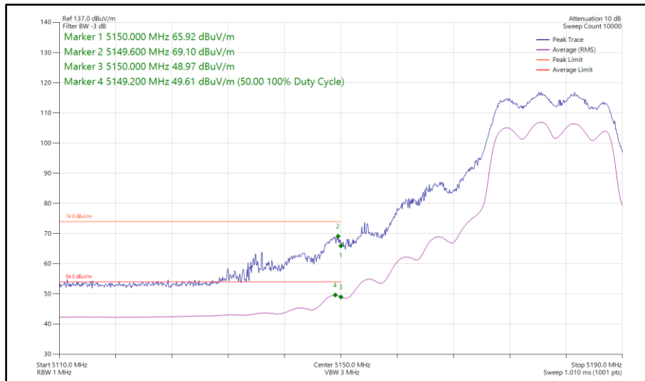
Figure 65 - 802.11a, CDD, Core 0-1 - 5180 MHz Band Edge Frequency 5150 MHz
