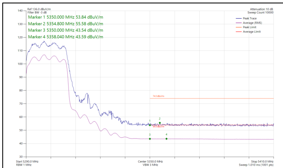
Figure 79 - 802.11ax HE20, SU, CDD, Core 0-1 - 5300 MHz Band Edge Frequency 5350 MHz
