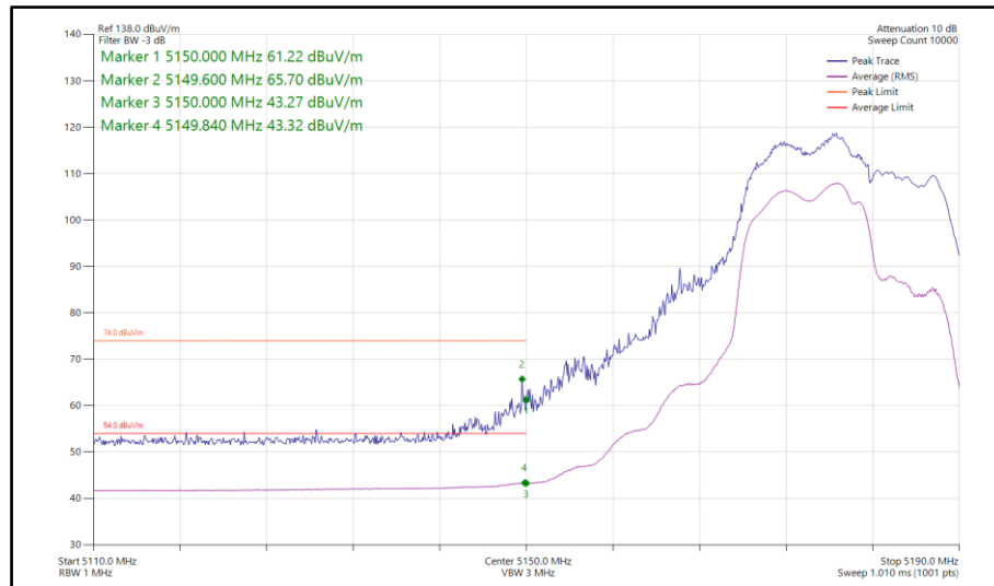
Figure 73 - 802.11be EHT20, RU 106+26-82, CDD, Core 0-1 - 5180 MHz Band Edge Frequency 5150 MHz
