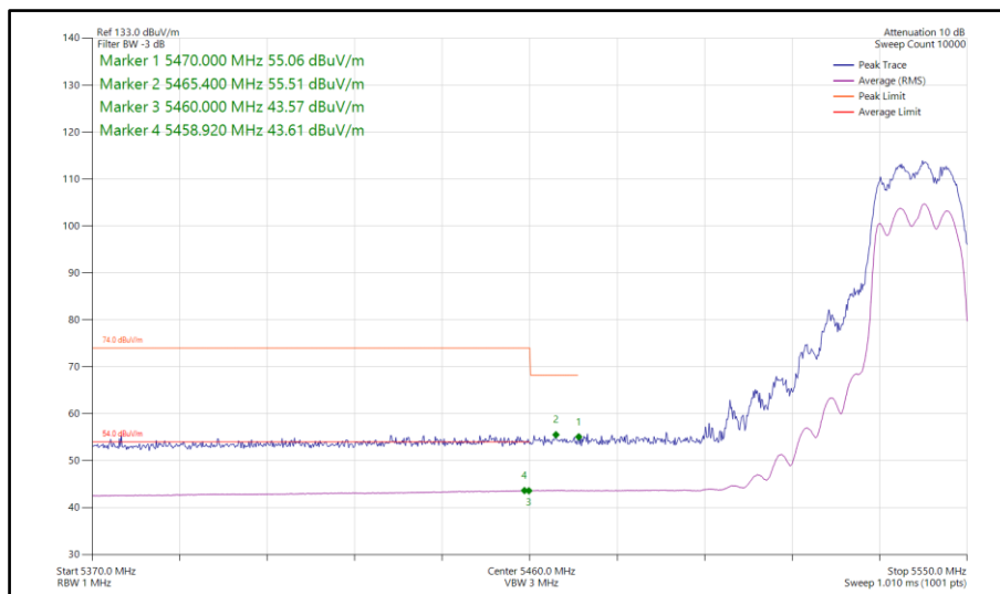
Figure 89 - 802.11n HT20, CDD, Core 0-1 - 5540 MHz Band Edge Frequency 5460 MHz
