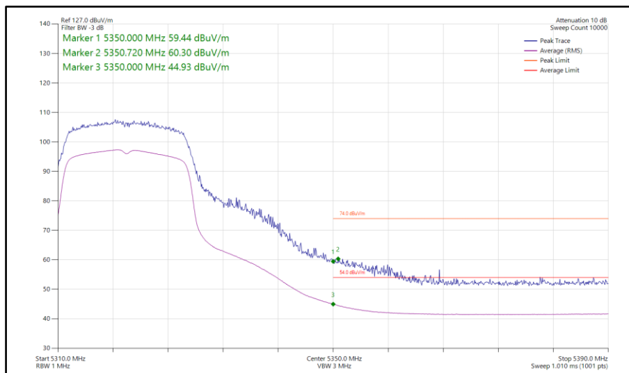
Figure 127 - 802.11ac VHT20, TxBF, Core 0-1 - 5320 MHz Band Edge Frequency 5350 MHz
