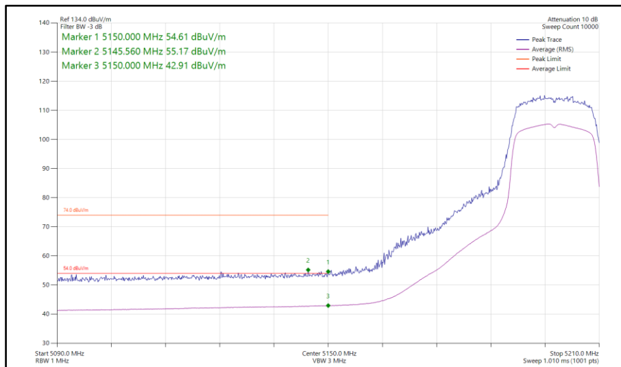
Figure 98 - 802.11n HT20, SDM, Core 0-1 - 5200 MHz Band Edge Frequency 5150 MHz
