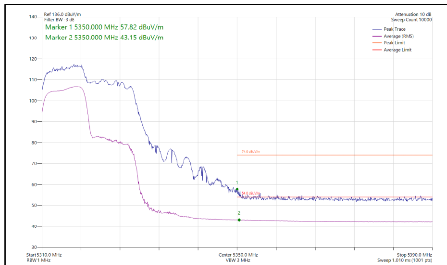
Figure 81 - 802.11ax HE20, RU 106-53, CDD, Core 0-1 - 5320 MHz Band Edge Frequency 5350 MHz
