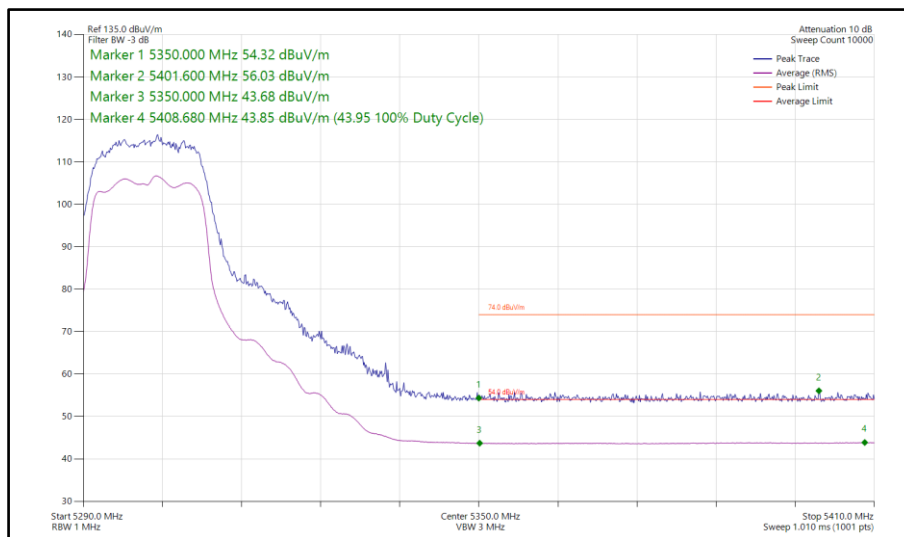
Figure 75 - 802.11a, CDD, Core 0-1 - 5300 MHz Band Edge Frequency 5350 MHz
