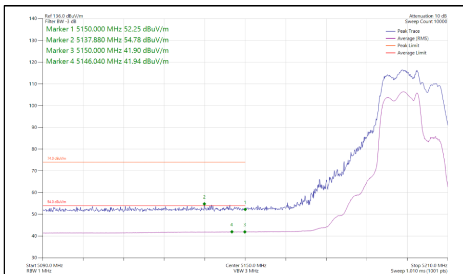
Figure 104 - 802.11be EHT20, RU 106+26-82, SDM, Core 0-1 - 5200 MHz Band Edge Frequency 5150 MHz
