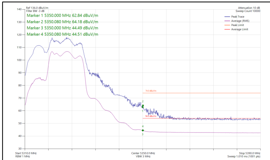
Figure 83 - 802.11be EHT20, RU 106+26-83, CDD, Core 0-1 - 5320 MHz Band Edge Frequency 5350 MHz
