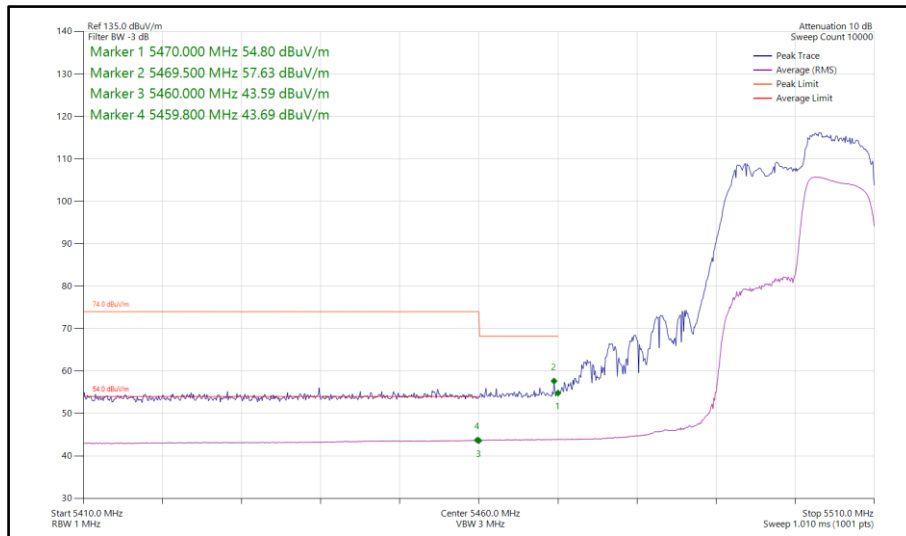
Figure 91 - 802.11ax HE20, RU 106-54, CDD, Core 0-1 - 5500 MHz Band Edge Frequency 5460 MHz
