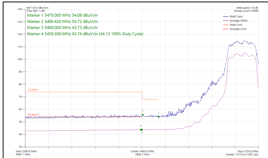
Figure 85 - 802.11a, CDD, Core 0-1 - 5520 MHz Band Edge Frequency 5460 MHz
