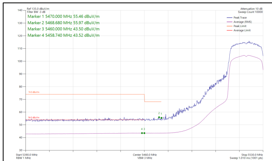
Figure 117 - 802.11ax HE20, SU, SDM, Core 0-1 - 5520 MHz Band Edge Frequency 5460 MHz
