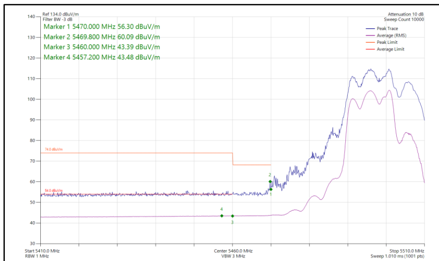
Figure 95 - 802.11be EHT20, RU 106+26-82, CDD, Core 0-1 - 5500 MHz Band Edge Frequency 5460 MHz
