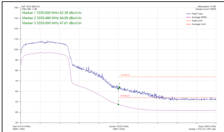
Figure 129 - 802.11ax HE20, SU, TxBF, Core 0-1 - 5320 MHz Band Edge Frequency 5350 MHz
