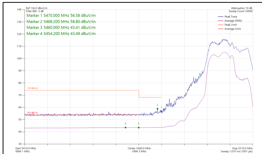
Figure 120 - 802.11be EHT20, RU 106+26-82, SDM, Core 0-1 - 5500 MHz Band Edge Frequency 5460 MHz
