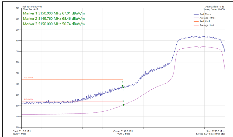
Figure 97 - 802.11n HT20, SDM, Core 0-1 - 5180 MHz Band Edge Frequency 5150 MHz
