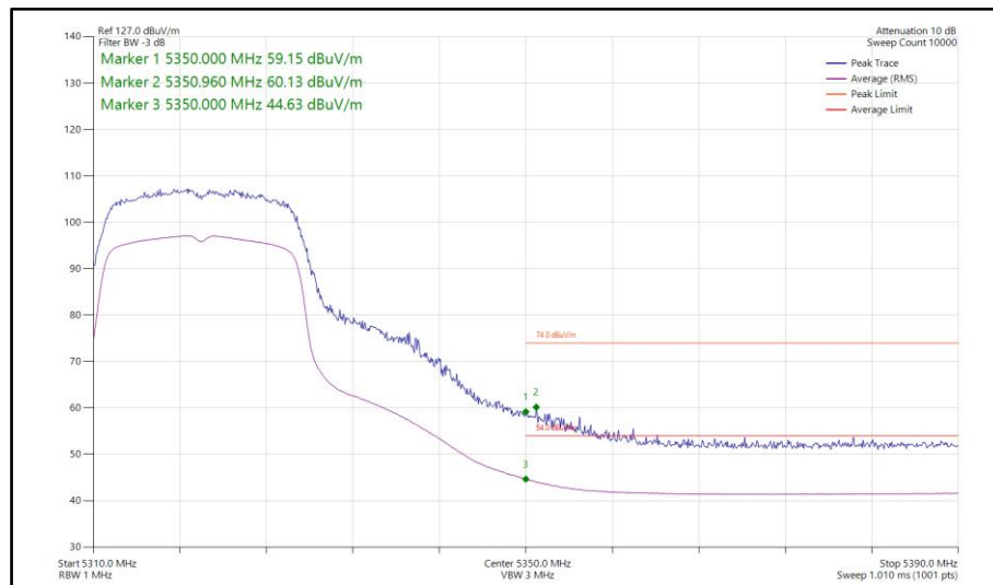
Figure 106 - 802.11n HT20, SDM, Core 0-1 - 5320 MHz Band Edge Frequency 5350 MHz
