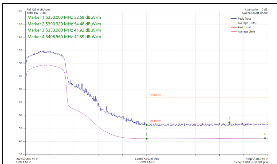
Figure 128 - 802.11ax HE20, SU, TxBF, Core 0-1 - 5300 MHz Band Edge Frequency 5350 MHz
