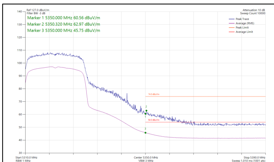
Figure 108 - 802.11ax HE20, SU, SDM, Core 0-1 - 5320 MHz Band Edge Frequency 5350 MHz
