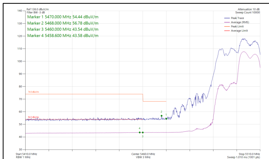
Figure 116 - 802.11ax HE20, RU 106-54, SDM, Core 0-1 - 5500 MHz Band Edge Frequency 5460 MHz
