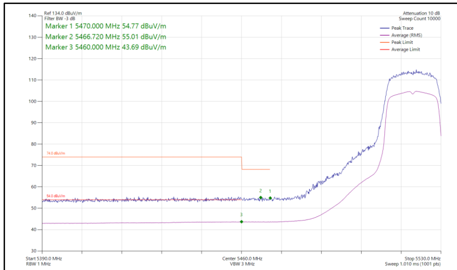
Figure 113 - 802.11n HT20, SDM, Core 0-1 - 5520 MHz Band Edge Frequency 5460 MHz
