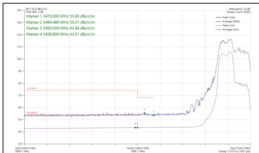
Figure 118 - 802.11ax HE20, RU 106-53, SDM, Core 0-1 - 5520 MHz Band Edge Frequency 5460 MHz
