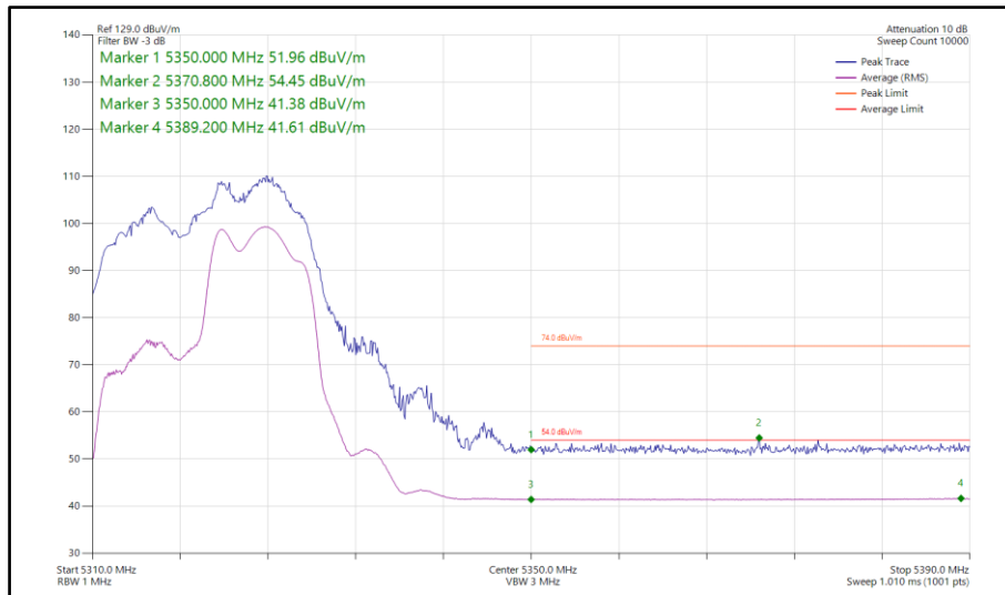
Figure 109 - 802.11ax HE20, RU 106-54, SDM, Core 0-1 - 5320 MHz Band Edge Frequency 5350 MHz
