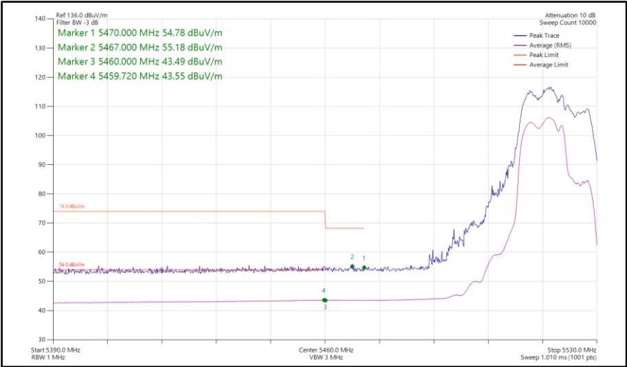
Figure 121 - 802.11be EHT20, RU 106+26-82, SDM, Core 0-1 - 5520 MHz Band Edge Frequency 5460 MHz
