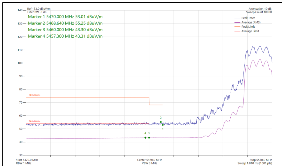
Figure 94 - 802.11ax HE20, SU, CDD, Core 0-1 - 5540 MHz Band Edge Frequency 5460 MHz
