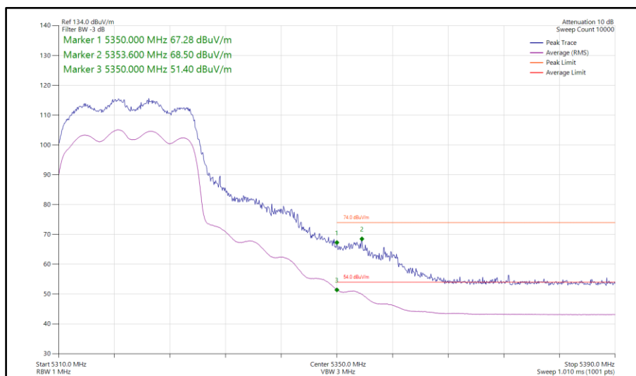
Figure 80 - 802.11ax HE20, SU, CDD, Core 0-1 - 5320 MHz Band Edge Frequency 5350 MHz
