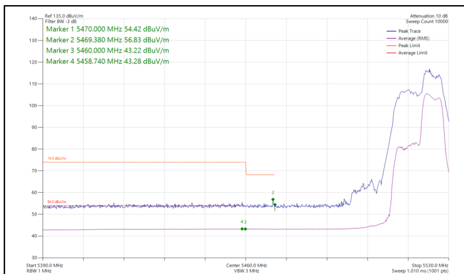
Figure 96 - 802.11be EHT20, RU 52+26-72 CDD, Core 0-1 - 5520 MHz Band Edge Frequency 5460 MHz
