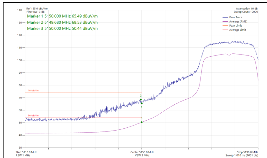
Figure 122 - 802.11ac VHT20, TxBF, Core 0-1 - 5180 MHz Band Edge Frequency 5150 MHz
