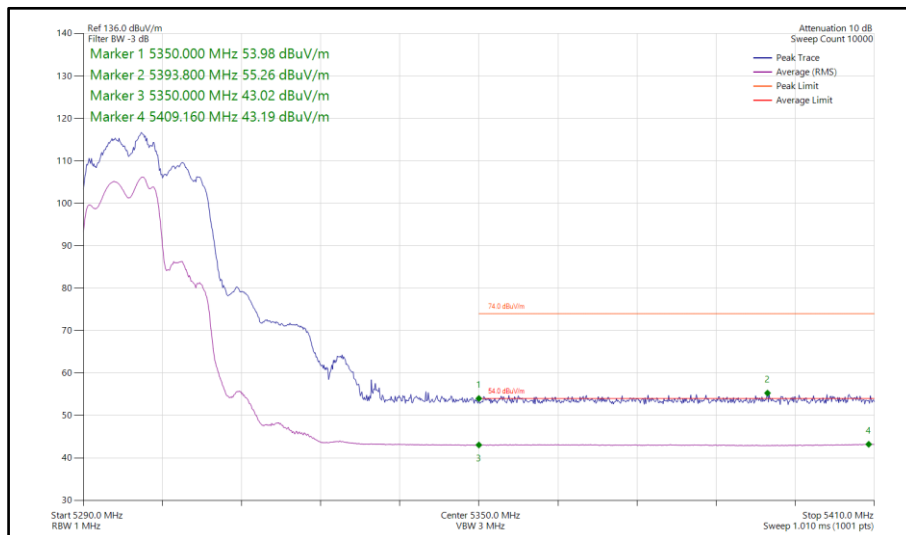
Figure 110 - 802.11be EHT20, RU 106+26-82, SDM, Core 0-1 - 5300 MHz Band Edge Frequency 5350 MHz
