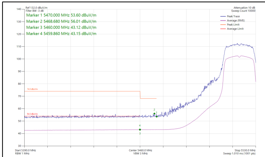
Figure 131 - 802.11ac VHT20, TxBF, Core 0-1 - 5520 MHz Band Edge Frequency 5460 MHz
