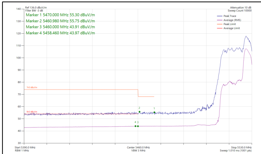
Figure 93 - 802.11ax HE20, RU 52-40, CDD, Core 0-1 - 5520 MHz Band Edge Frequency 5460 MHz
