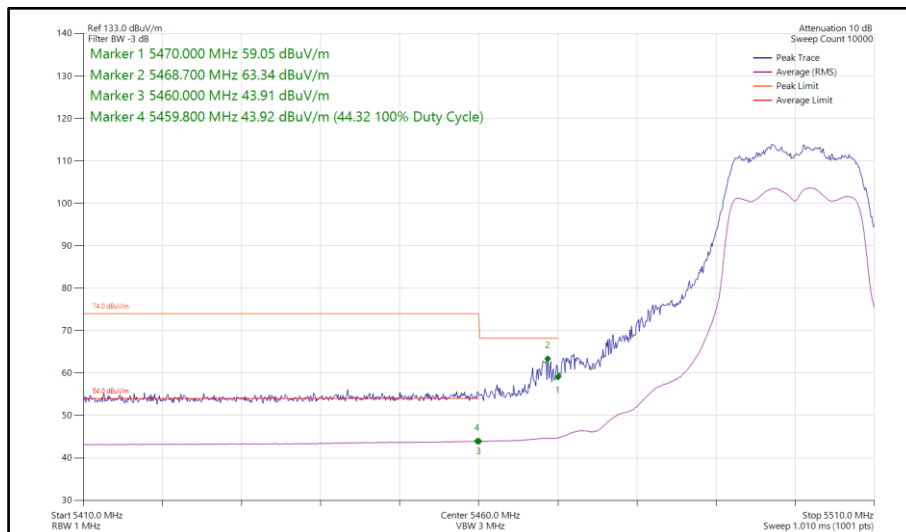
Figure 84 - 802.11a, CDD, Core 0-1 - 5500 MHz Band Edge Frequency 5460 MHz
