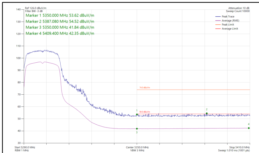
Figure 126 - 802.11ac VHT20, TxBF, Core 0-1 - 5300 MHz Band Edge Frequency 5350 MHz
