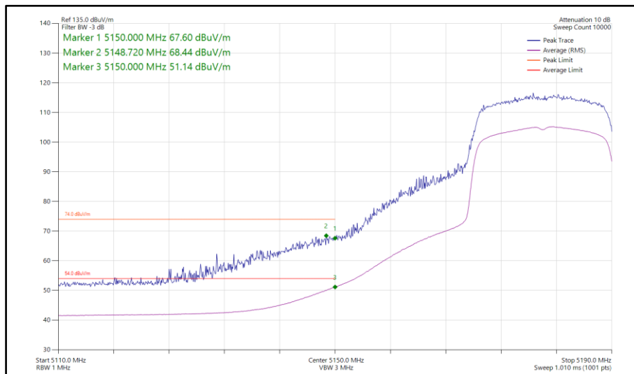
Figure 124 - 802.11ax HE20, SU, TxBF, Core 0-1 - 5180 MHz Band Edge Frequency 5150 MHz
