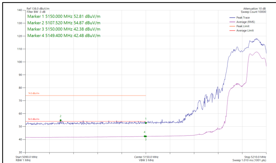
Figure 72 - 802.11ax HE20, RU 106-54, CDD, Core 0-1 - 5200 MHz Band Edge Frequency 5150 MHz
