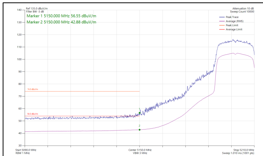
Figure 101 - 802.11ax HE20, SU, SDM, Core 0-1 - 5200 MHz Band Edge Frequency 5150 MHz
