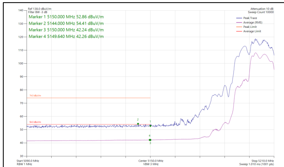
Figure 74 - 802.11be EHT20, RU 106+26-83, CDD, Core 0-1 - 5200 MHz Band Edge Frequency 5150 MHz
