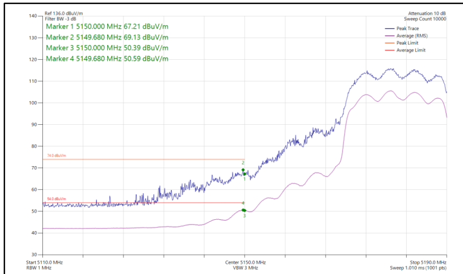
Figure 69 - 802.11ax HE20, SU, CDD, Core 0-1 - 5180 MHz Band Edge Frequency 5150 MHz
