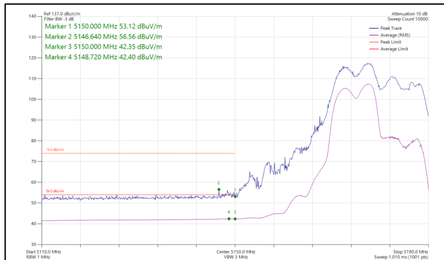
Figure 100 - 802.11ax HE20, RU 106-53, SDM, Core 0-1 - 5180 MHz Band Edge Frequency 5150 MHz
