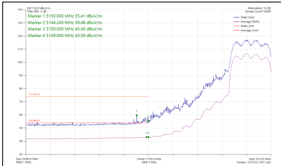
Figure 71 - 802.11ax HE20, SU, CDD, Core 0-1 - 5200 MHz Band Edge Frequency 5150 MHz
