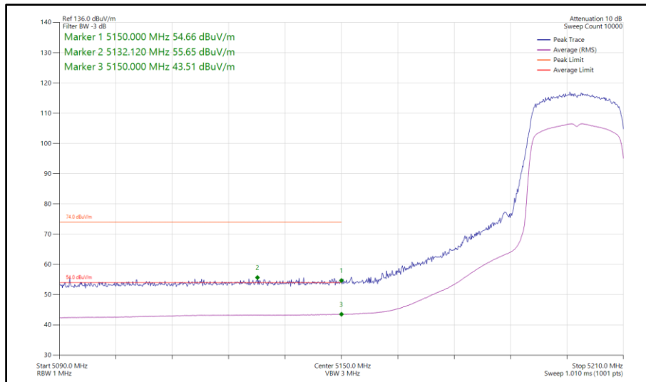
Figure 125 - 802.11ax HE20, SU, TxBF, Core 0-1 - 5200 MHz Band Edge Frequency 5150 MHz
