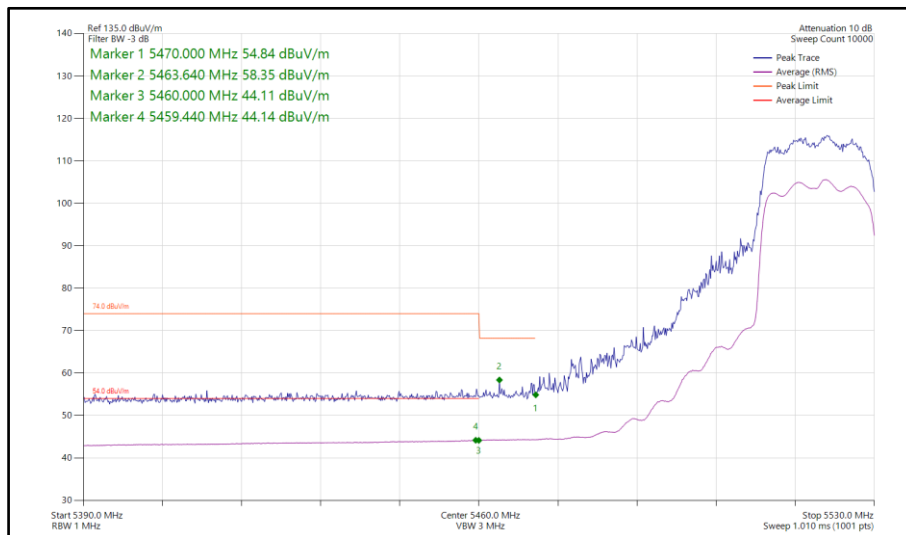
Figure 92 - 802.11ax HE20, SU, CDD, Core 0-1 - 5520 MHz Band Edge Frequency 5460 MHz
