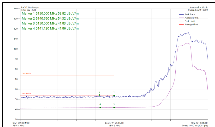
Figure 102 - 802.11ax HE20, RU 106-53, SDM, Core 0-1 - 5200 MHz Band Edge Frequency 5150 MHz
