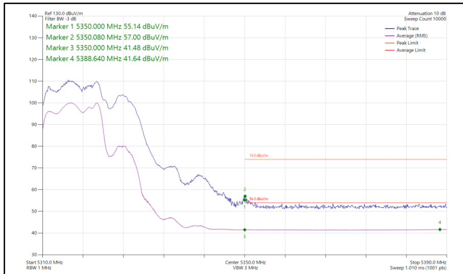
Figure 111 - 802.11be EHT20, RU 106+26-82, SDM, Core 0-1 - 5320 MHz Band Edge Frequency 5350 MHz
