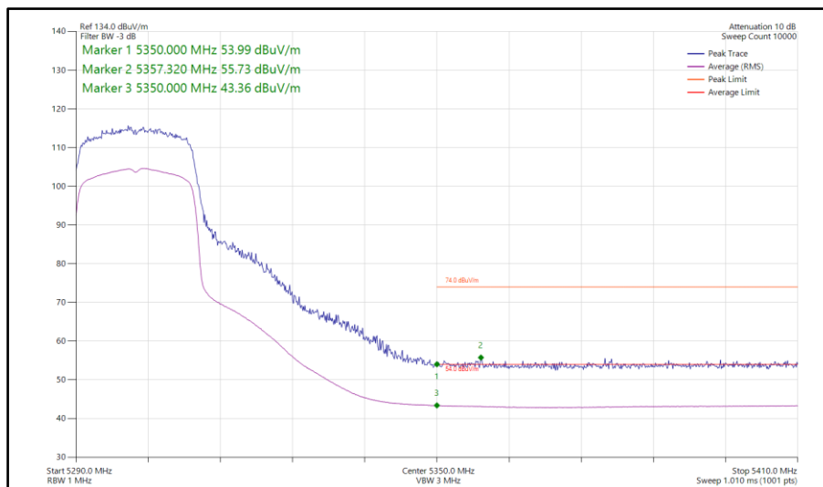
Figure 107 - 802.11ax HE20, SU, SDM, Core 0-1 - 5300 MHz Band Edge Frequency 5350 MHz
