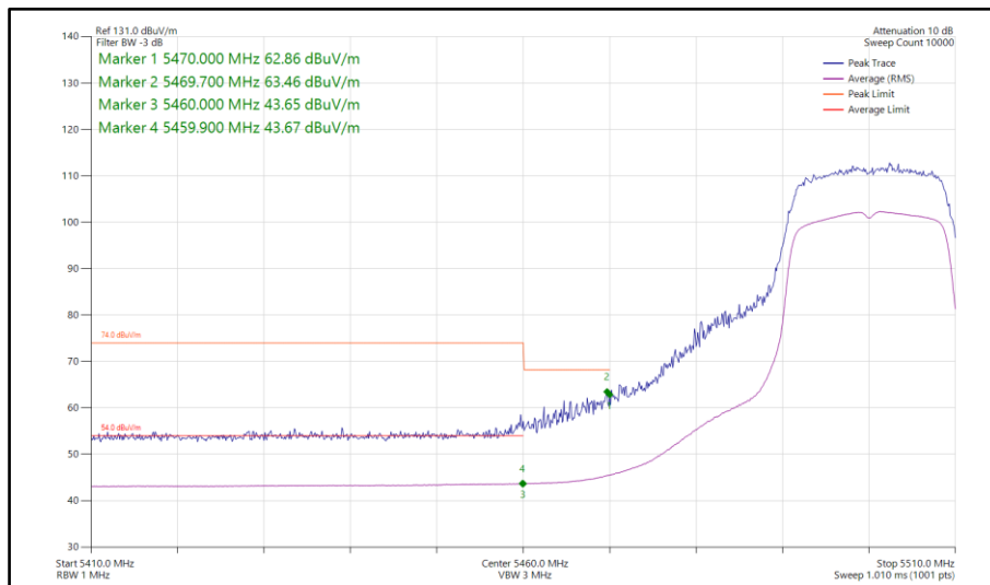
Figure 112 - 802.11n HT20, SDM, Core 0-1 - 5500 MHz Band Edge Frequency 5460 MHz
