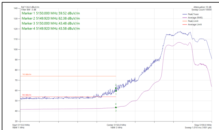
Figure 103 - 802.11be EHT20, RU 106+26-82, SDM, Core 0-1 - 5180 MHz Band Edge Frequency 5150 MHz
