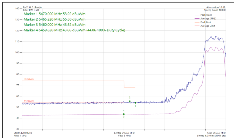
Figure 86 - 802.11a, CDD, Core 0-1 - 5540 MHz Band Edge Frequency 5460 MHz
