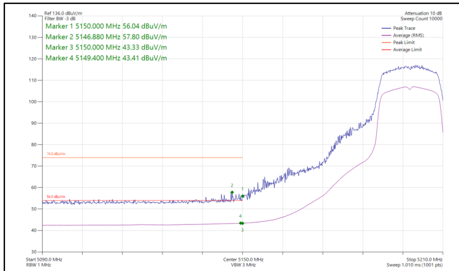
Figure 123 - 802.11ac VHT20, TxBF, Core 0-1 - 5200 MHz Band Edge Frequency 5150 MHz
