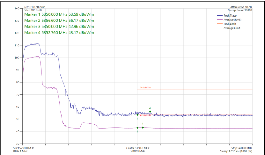
Figure 188 - 802.11ax HE40, RU 106-53, SISO, Core 1 - 5310 MHz Band Edge Frequency 5350 MHz
