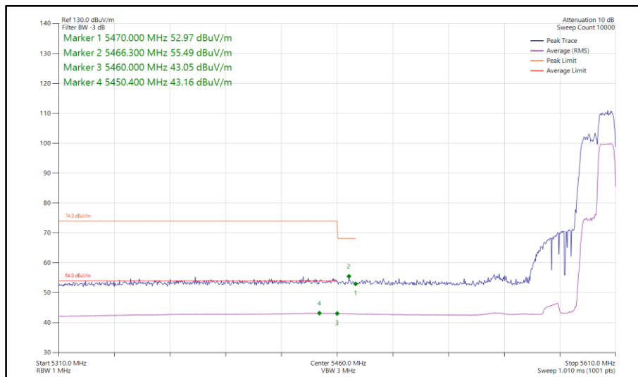
Figure 202 - 802.11ax HE40, RU 106-56, SISO, Core 1 - 5590 MHz Band Edge Frequency 5460 MHz
