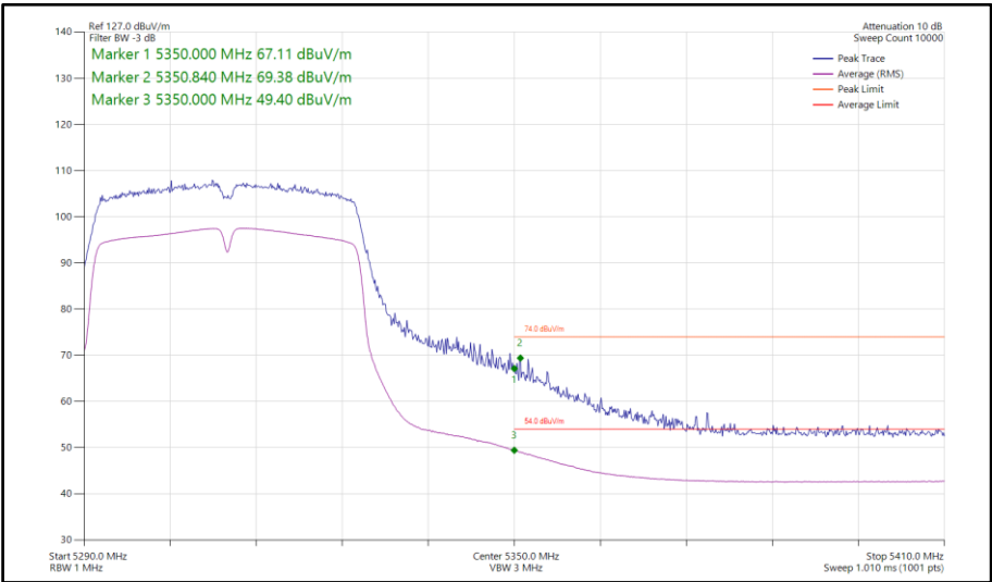
Figure 184 - 802.11n HT40, SISO, Core 1 - 5310 MHz Band Edge Frequency 5350 MHz
