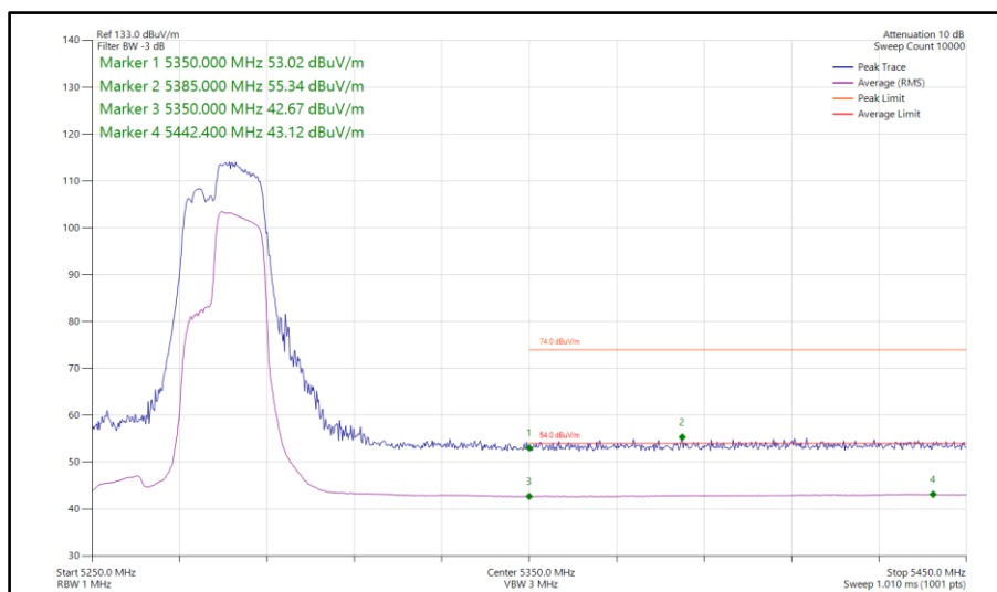
Figure 154 - 802.11be EHT40, RU 106+26-85, SISO, Core 0 - 5270 MHz Band Edge Frequency 5350 MHz
