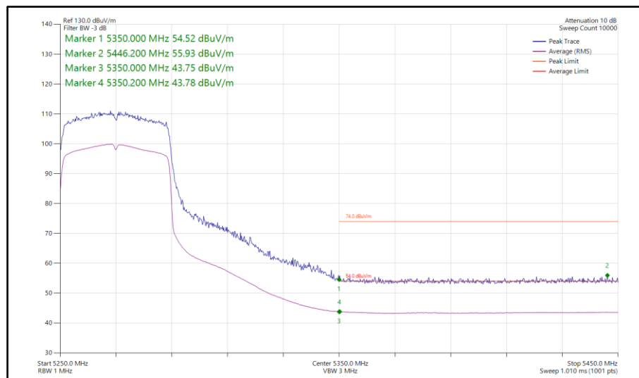
Figure 185 - 802.11ax HE40, SU, SISO, Core 1 - 5270 MHz Band Edge Frequency 5350 MHz
