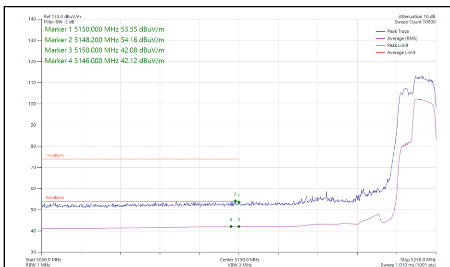
Figure 145 - 802.11be EHT40, RU 106+26-85, SISO, Core 0 - 5230 MHz Band Edge Frequency 5150 MHz
