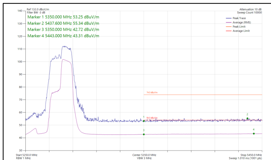
Figure 186 - 802.11ax HE40, RU 106-56, SISO, Core 1 - 5270 MHz Band Edge Frequency 5350 MHz
