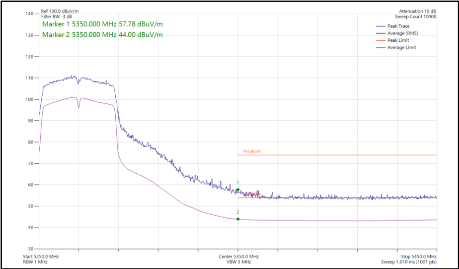
Figure 183 - 802.11n HT40, SISO, Core 1 - 5270 MHz Band Edge Frequency 5350 MHz
