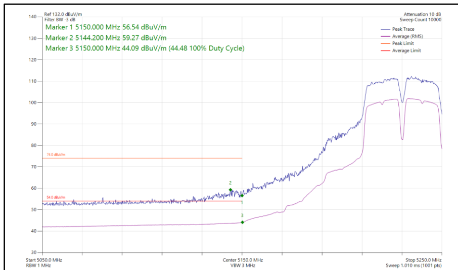
Figure 137 - 802.11a a40, SISO, Core 0 - 5230 MHz Band Edge Frequency 5150 MHz
