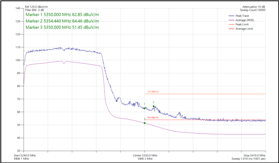
Figure 187 - 802.11ax HE40, SU, SISO, Core 1 - 5310 MHz Band Edge Frequency 5350 MHz
