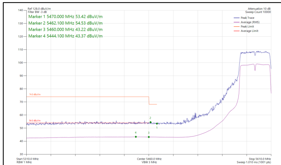
Figure 196 - 802.11n HT40, SISO, Core 1 - 5590 MHz Band Edge Frequency 5460 MHz
