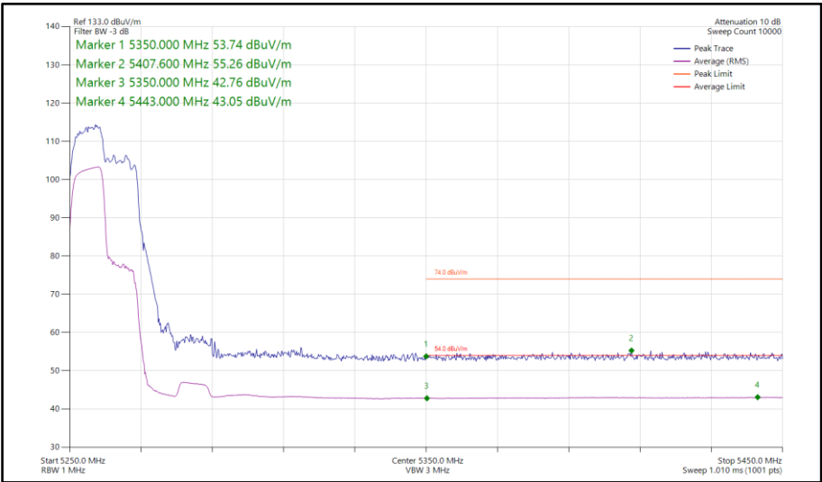
Figure 151 - 802.11ax HE40, RU 106-53, SISO, Core 0 - 5270 MHz Band Edge Frequency 5350 MHz
