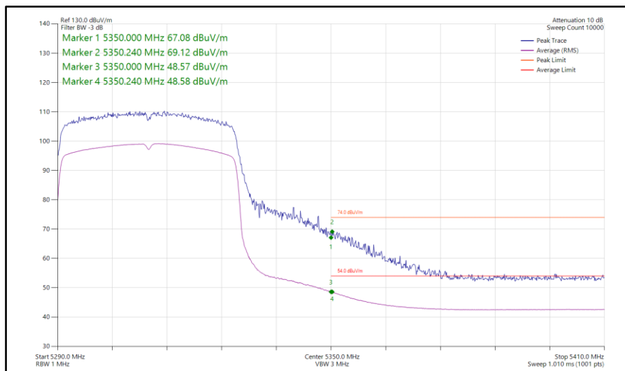
Figure 152 - 802.11ax HE40, SU, SISO, Core 0 - 5310 MHz Band Edge Frequency 5350 MHz
