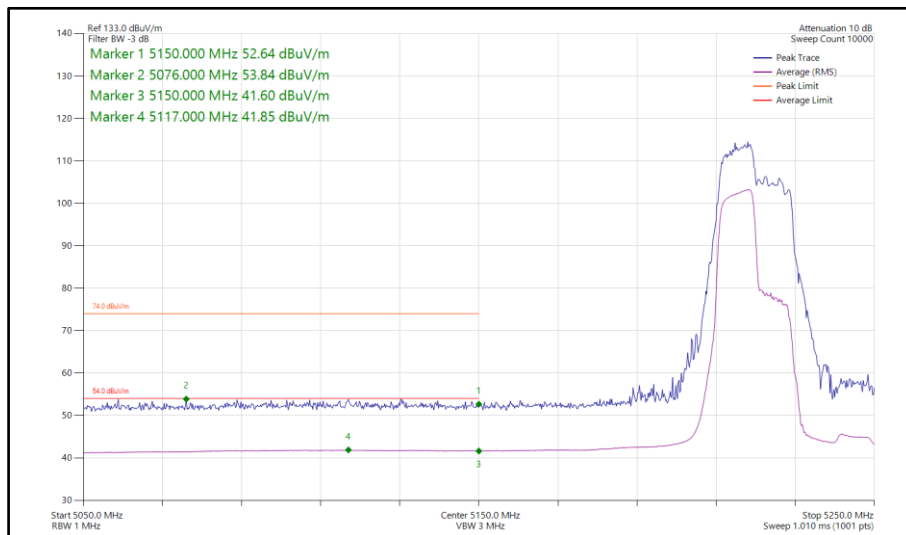
Figure 143 - 802.11ax HE40, RU 106-53, SISO, Core 0 - 5230 MHz Band Edge Frequency 5150 MHz
