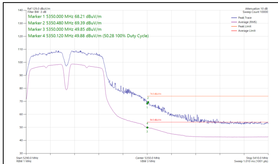
Figure 147 - 802.11a a40, SISO, Core 0 - 5310 MHz Band Edge Frequency 5350 MHz
