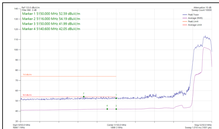
Figure 178 - 802.11ax HE40, RU 106-56, SISO, Core 1 - 5230 MHz Band Edge Frequency 5150 MHz
