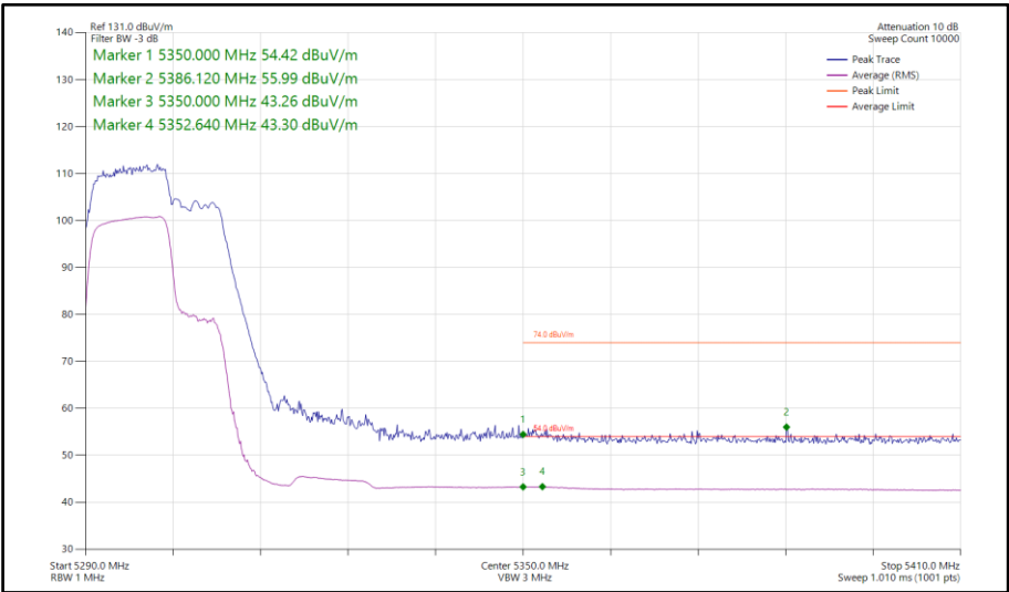
Figure 190 - 802.11be EHT40, RU 106+26-82, SISO, Core 1 - 5310 MHz Band Edge Frequency 5350 MHz
