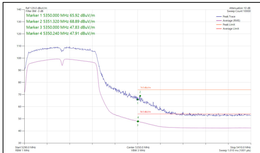
Figure 149 - 802.11n HT40, SISO, Core 0 - 5310 MHz Band Edge Frequency 5350 MHz
