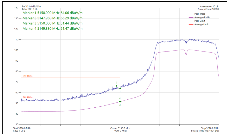
Figure 173 - 802.11n HT40, SISO, Core 1 - 5190 MHz Band Edge Frequency 5150 MHz
