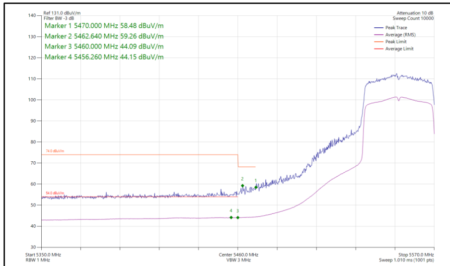
Figure 164 - 802.11ax HE40, SU, SISO, Core 0 - 5550 MHz Band Edge Frequency 5460 MHz
