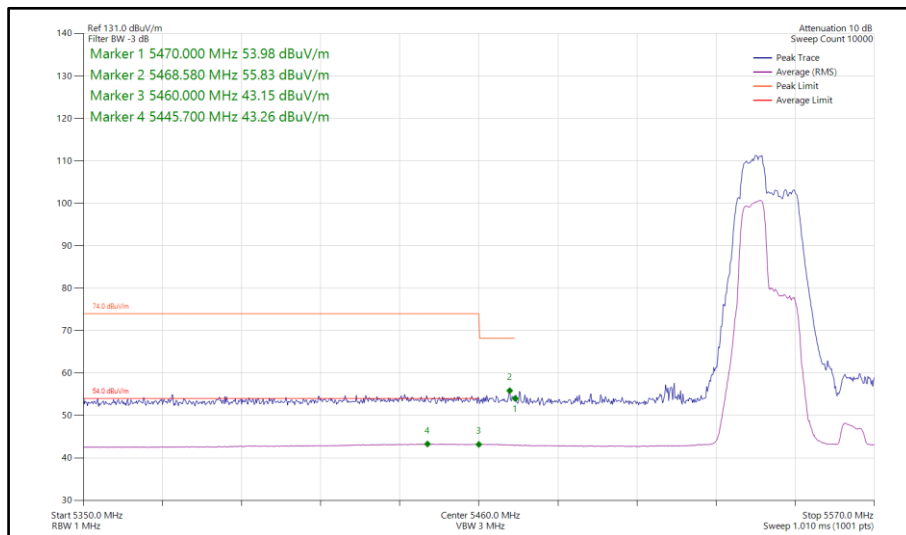
Figure 169 - 802.11be EHT40, RU 52+26-70, SISO, Core 0 - 5550 MHz Band Edge Frequency 5460 MHz
