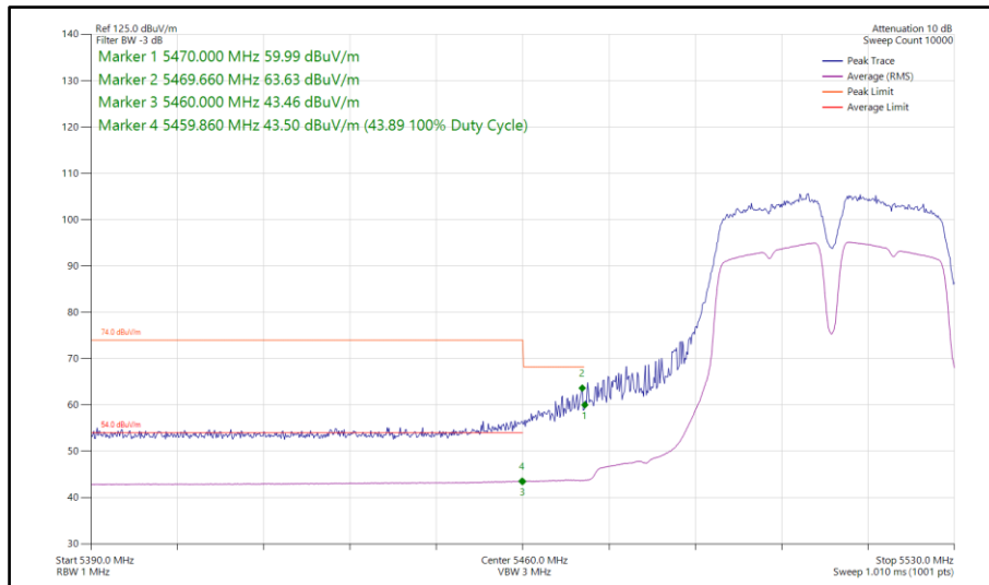
Figure 191 - 802.11a a40, SISO, Core 1 - 5510 MHz Band Edge Frequency 5460 MHz
