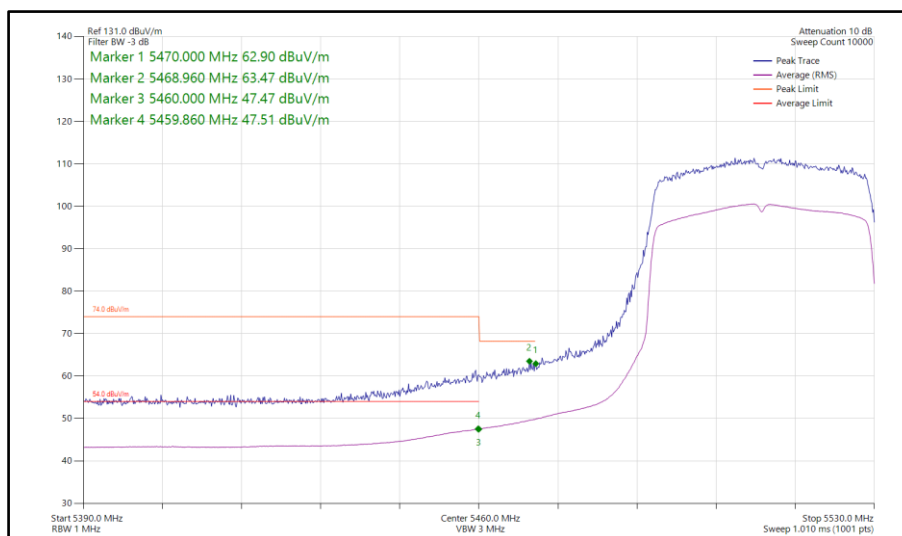
Figure 162 - 802.11ax HE40, SU, SISO, Core 0 - 5510 MHz Band Edge Frequency 5460 MHz
