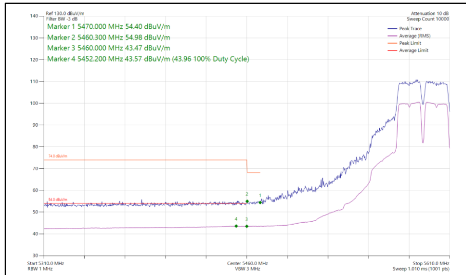
Figure 158 - 802.11a a40, SISO, Core 0 - 5590 MHz Band Edge Frequency 5460 MHz
