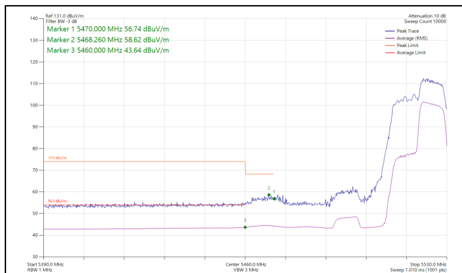
Figure 198 - 802.11ax HE40, RU 106-56, SISO, Core 1 - 5510 MHz Band Edge Frequency 5460 MHz
