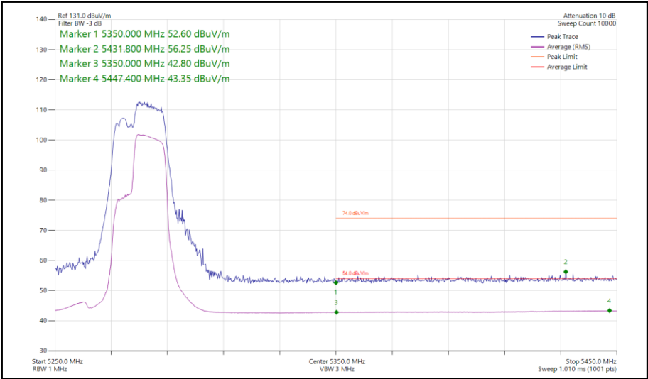
Figure 189 - 802.11be EHT40, RU 106+26-85, SISO, Core 1 - 5270 MHz Band Edge Frequency 5350 MHz
