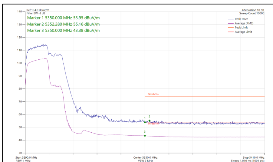
Figure 155 - 802.11be EHT40, RU 106+26-82, SISO, Core 0 - 5310 MHz Band Edge Frequency 5350 MHz
