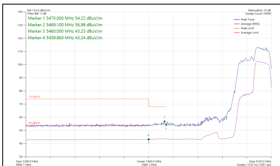
Figure 163 - 802.11ax HE40, RU 106-56, SISO, Core 0 - 5510 MHz Band Edge Frequency 5460 MHz
