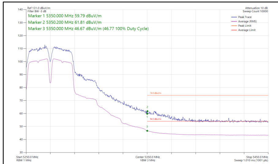
Figure 146 - 802.11a a40, SISO, Core 0 - 5270 MHz Band Edge Frequency 5350 MHz
