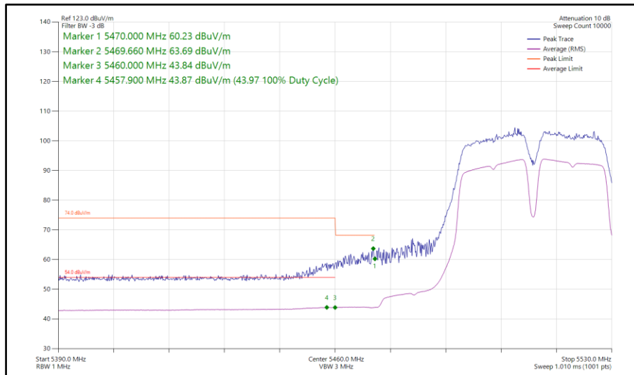
Figure 156 - 802.11a a40, SISO, Core 0 - 5510 MHz Band Edge Frequency 5460 MHz
