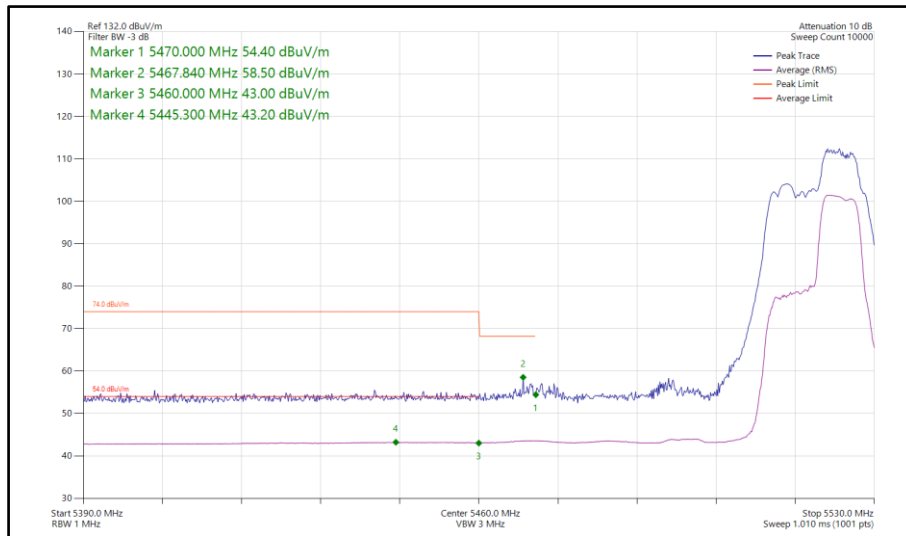
Figure 168 - 802.11be EHT40, RU 52+26-75, SISO, Core 0 - 5510 MHz Band Edge Frequency 5460 MHz
