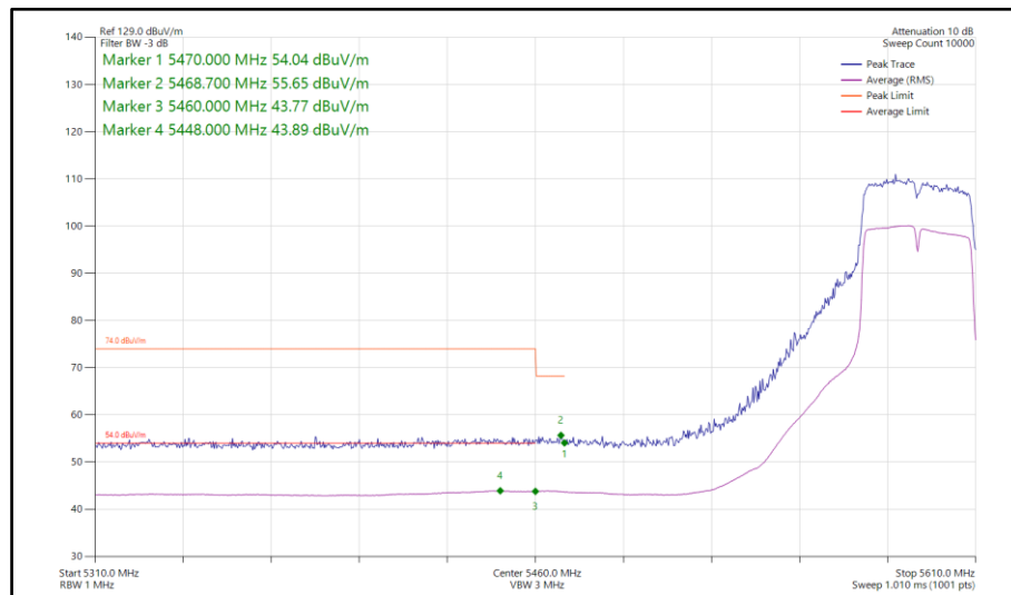
Figure 161 - 802.11n HT40, SISO, Core 0 - 5590 MHz Band Edge Frequency 5460 MHz
