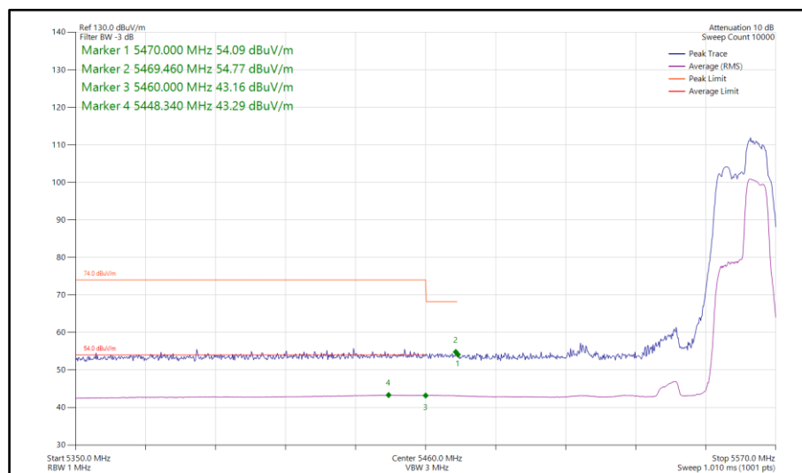
Figure 204 - 802.11be EHT40, RU 52+26-75, SISO, Core 1 - 5550 MHz Band Edge Frequency 5460 MHz
