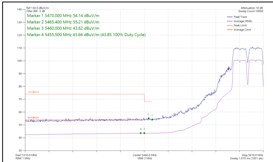
Figure 193 - 802.11a a40, SISO, Core 1 - 5590 MHz Band Edge Frequency 5460 MHz
