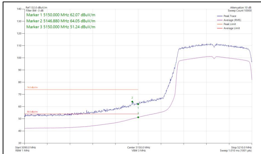
Figure 175 - 802.11ax HE40, SU, SISO, Core 1 - 5190 MHz Band Edge Frequency 5150 MHz
