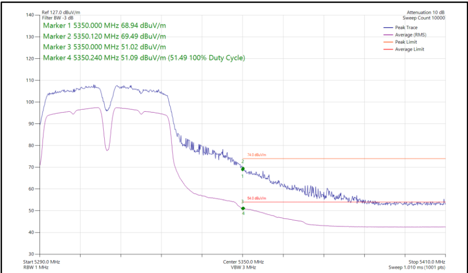
Figure 182 - 802.11a a40, SISO, Core 1 - 5310 MHz Band Edge Frequency 5350 MHz
