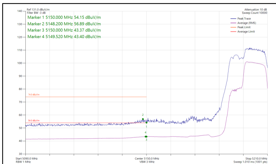
Figure 144 - 802.11be EHT40, RU 106+26-85, SISO, Core 0 - 5190 MHz Band Edge Frequency 5150 MHz
