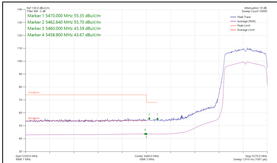
Figure 199 - 802.11ax HE40, SU, SISO, Core 1 - 5550 MHz Band Edge Frequency 5460 MHz
