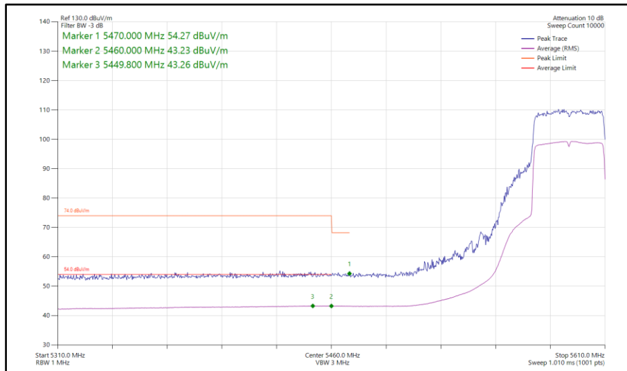
Figure 201 - 802.11ax HE40, SU, SISO, Core 1 - 5590 MHz Band Edge Frequency 5460 MHz
