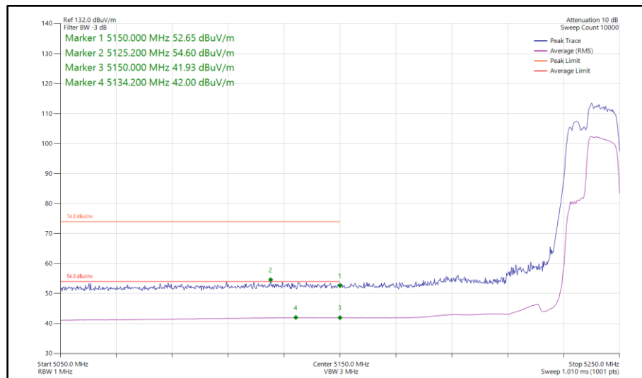
Figure 180 - 802.11be EHT40, RU 106+26-85, SISO, Core 1 - 5230 MHz Band Edge Frequency 5150 MHz
