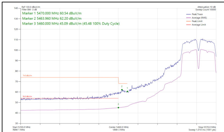
Figure 157 - 802.11a a40, SISO, Core 0 - 5550 MHz Band Edge Frequency 5460 MHz
