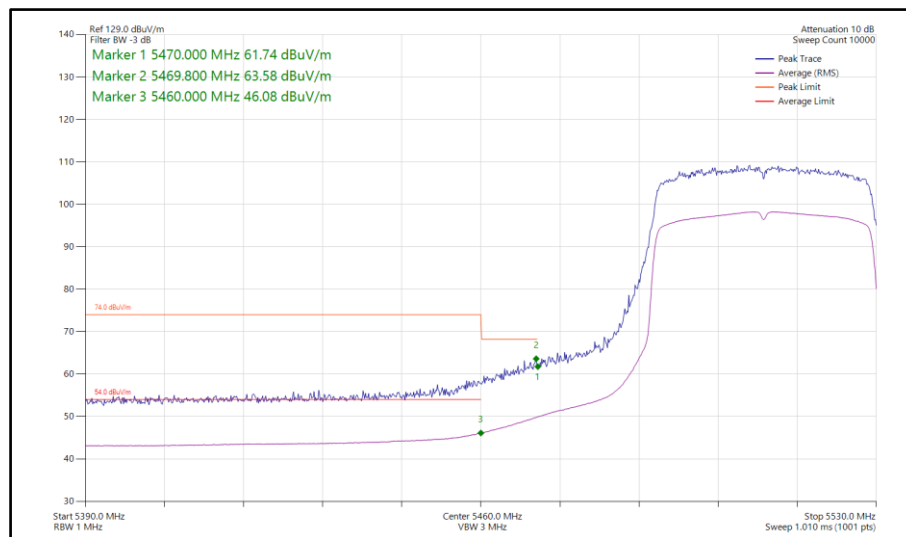
Figure 197 - 802.11ax HE40, SU, SISO, Core 1 - 5510 MHz Band Edge Frequency 5460 MHz
