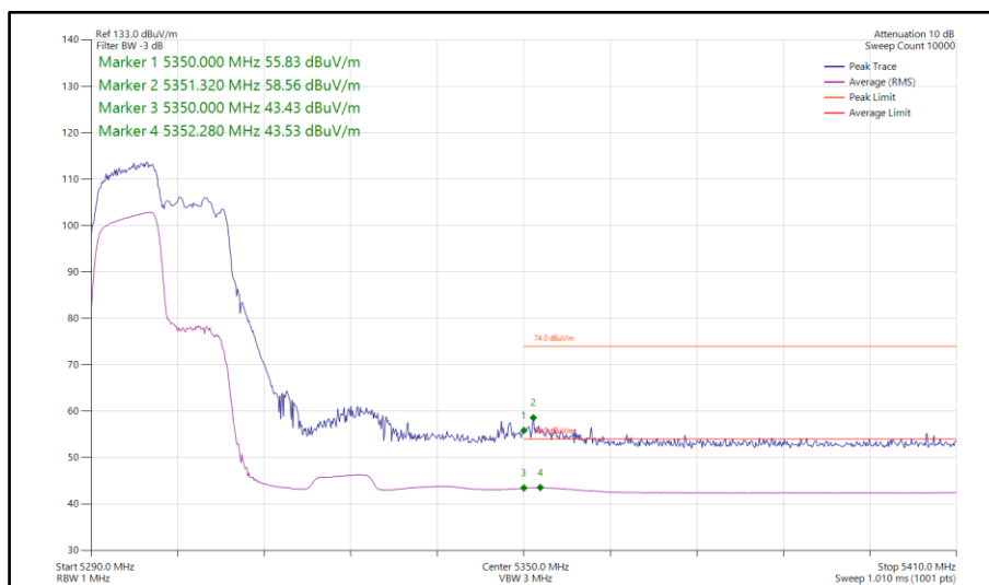
Figure 153 - 802.11ax HE40, RU 106-53, SISO, Core 0 - 5310 MHz Band Edge Frequency 5350 MHz
