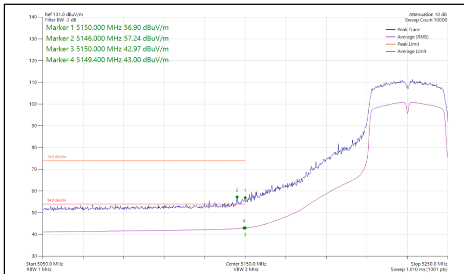
Figure 174 - 802.11n HT40, SISO, Core 1 - 5230 MHz Band Edge Frequency 5150 MHz
