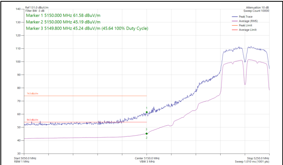
Figure 172 - 802.11a a40, SISO, Core 1 - 5230 MHz Band Edge Frequency 5150 MHz
