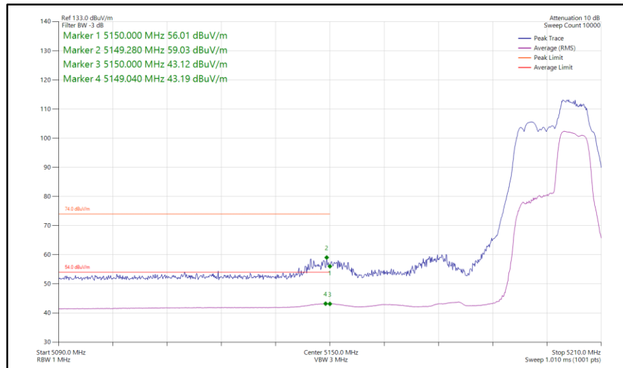
Figure 179 - 802.11be EHT40, RU 52+26-75, SISO, Core 1 - 5190 MHz Band Edge Frequency 5150 MHz
