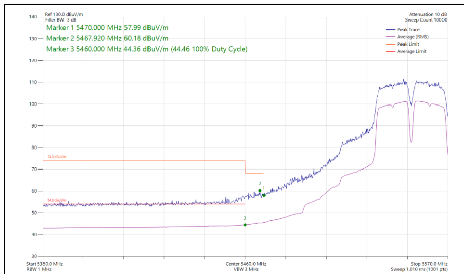
Figure 192 - 802.11a a40, SISO, Core 1 - 5550 MHz Band Edge Frequency 5460 MHz
