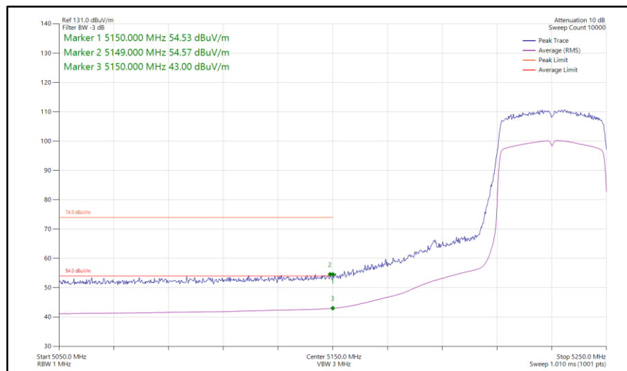
Figure 177 - 802.11ax HE40, SU, SISO, Core 1 - 5230 MHz Band Edge Frequency 5150 MHz
