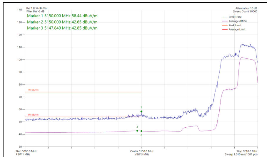
Figure 176 - 802.11ax HE40, RU 106-56, SISO, Core 1 - 5190 MHz Band Edge Frequency 5150 MHz
