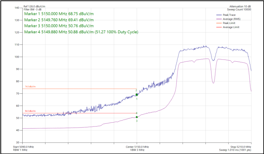
Figure 171 - 802.11a a40, SISO, Core 1 - 5190 MHz Band Edge Frequency 5150 MHz
