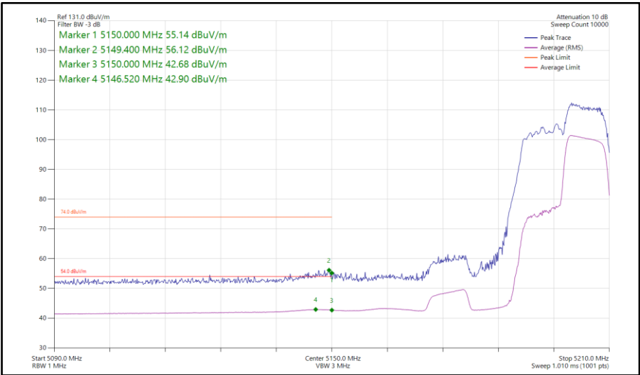
Figure 141 - 802.11ax HE40, RU 106-56, SISO, Core 0 - 5190 MHz Band Edge Frequency 5150 MHz
