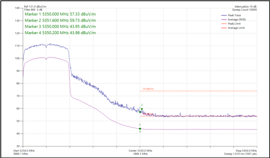
Figure 150 - 802.11ax HE40, SU, SISO, Core 0 - 5270 MHz Band Edge Frequency 5350 MHz
