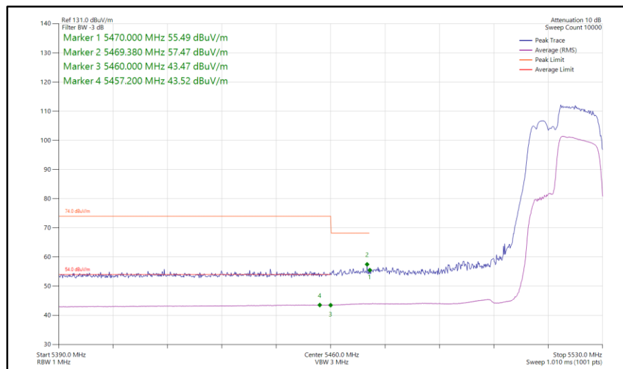
Figure 203 - 802.11be EHT40, RU 106+26-85, SISO, Core 1 - 5510 MHz Band Edge Frequency 5460 MHz
