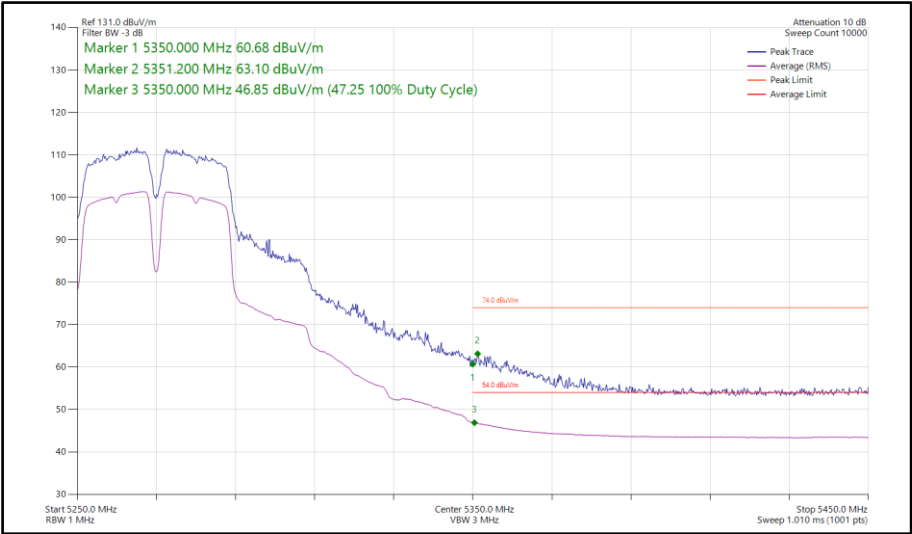
Figure 181 - 802.11a a40, SISO, Core 1 - 5270 MHz Band Edge Frequency 5350 MHz
