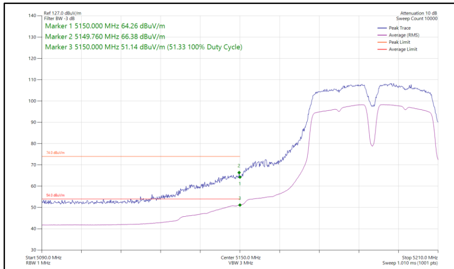
Figure 136 - 802.11a a40, SISO, Core 0 - 5190 MHz Band Edge Frequency 5150 MHz
