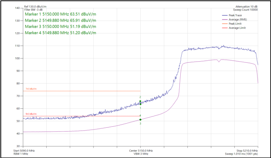
Figure 140 - 802.11ax HE40, SU, SISO, Core 0 - 5190 MHz Band Edge Frequency 5150 MHz
