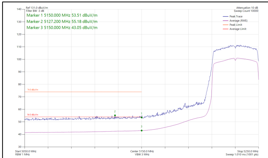
Figure 142 - 802.11ax HE40, SU, SISO, Core 0 - 5230 MHz Band Edge Frequency 5150 MHz
