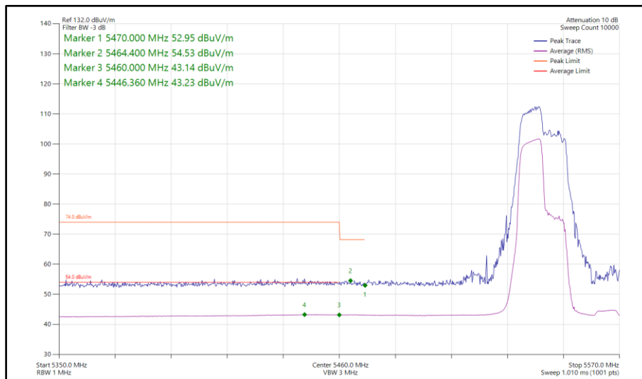
Figure 165 - 802.11ax HE40, RU 106-53, SISO, Core 0 - 5550 MHz Band Edge Frequency 5460 MHz
