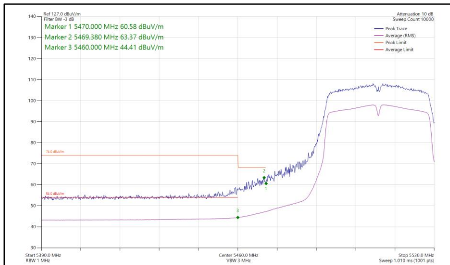
Figure 194 - 802.11n HT40, SISO, Core 1 - 5510 MHz Band Edge Frequency 5460 MHz
