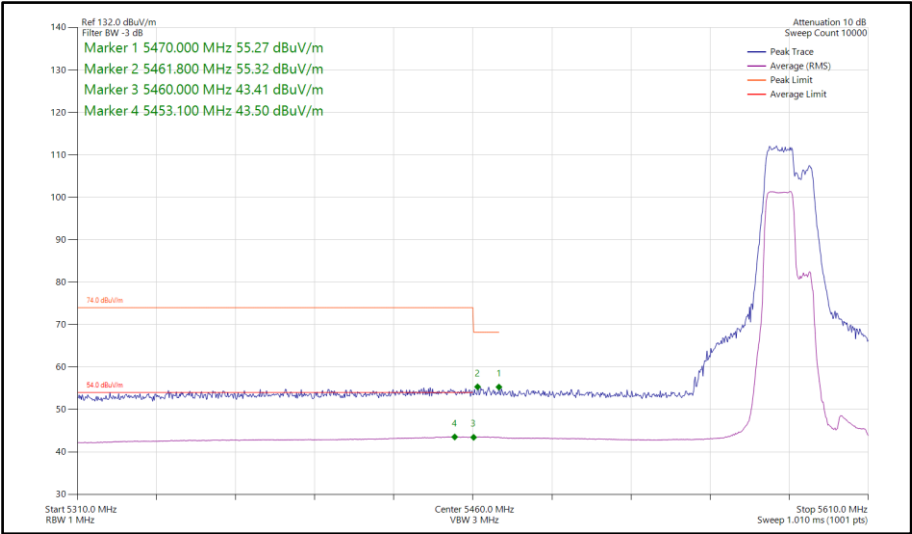
Figure 170 - 802.11be EHT40, RU 106+26-82 SISO, Core 0 - 5590 MHz Band Edge Frequency 5460 MHz
