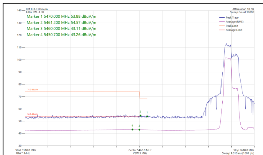
Figure 167 - 802.11ax HE40, RU 106-53, SISO, Core 0 - 5590 MHz Band Edge Frequency 5460 MHz
