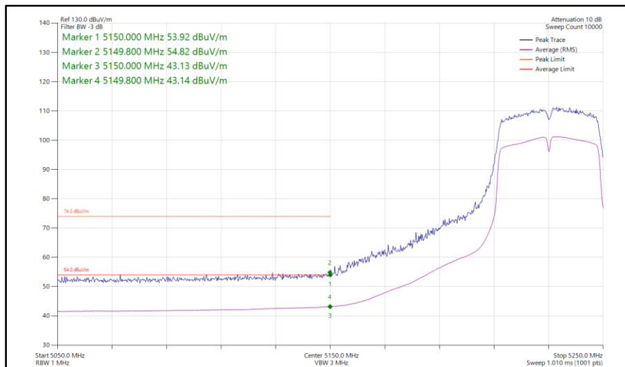
Figure 139 - 802.11n HT40, SISO, Core 0 - 5230 MHz Band Edge Frequency 5150 MHz
