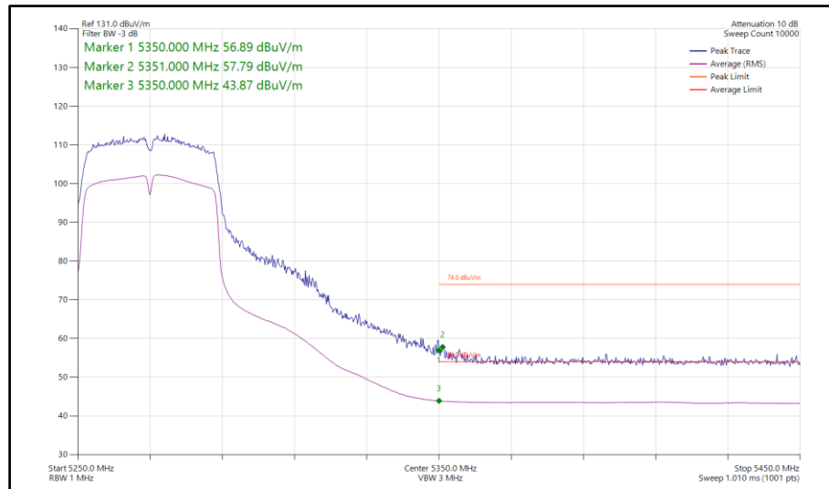
Figure 148 - 802.11n HT40, SISO, Core 0 - 5270 MHz Band Edge Frequency 5350 MHz
