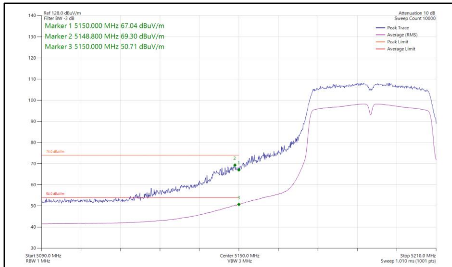
Figure 138 - 802.11n HT40, SISO, Core 0 - 5190 MHz Band Edge Frequency 5150 MHz
