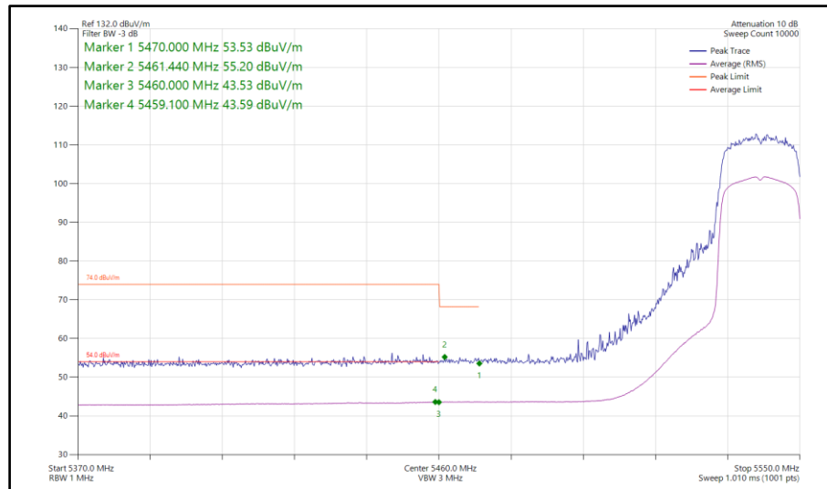
Figure 135 - 802.11ax HE20, SU, TxBF, Core 0-1 - 5540 MHz Band Edge Frequency 5460 MHz
