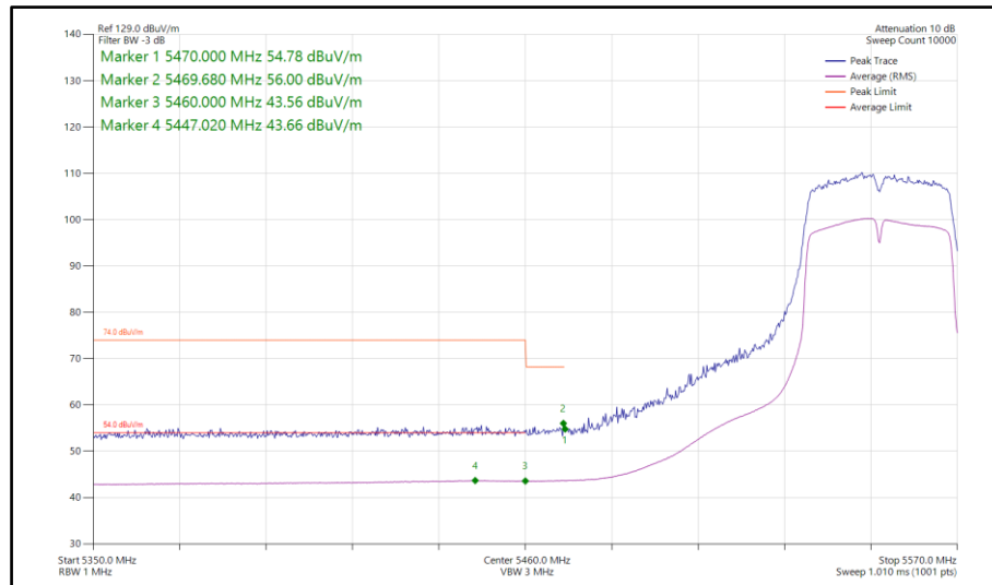
Figure 195 - 802.11n HT40, SISO, Core 1 - 5550 MHz Band Edge Frequency 5460 MHz
