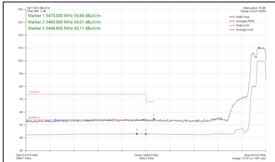
Figure 205 - 802.11be EHT40, RU 106+26-85, SISO, Core 1 - 5590 MHz Band Edge Frequency 5460 MHz
