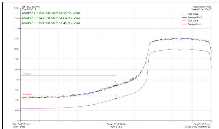
Figure 271 - 802.11ax HE40, SU, TxBF, Core 0-1 - 5190 MHz Band Edge Frequency 5150 MHz
