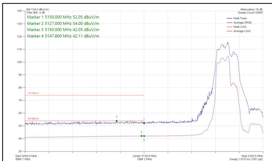
Figure 248 - 802.11be EHT40, RU 106+26-82, SDM, Core 0-1 - 5230 MHz Band Edge Frequency 5150 MHz
