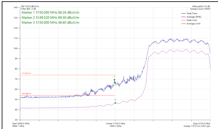
Figure 210 - 802.11ax HE40, SU, CDD, Core 0-1 - 5190 MHz Band Edge Frequency 5150 MHz
