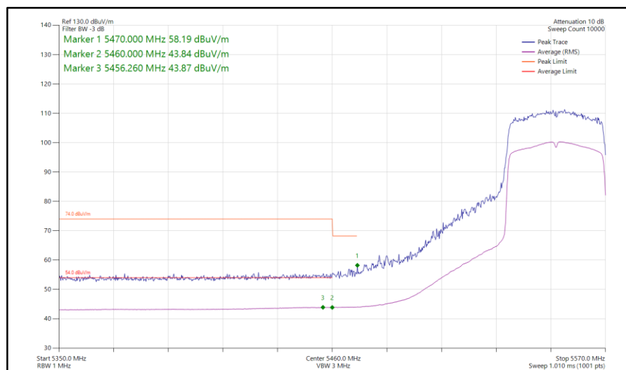
Figure 262 - 802.11ax HE40, SU, SDM, Core 0-1 - 5550 MHz Band Edge Frequency 5460 MHz
