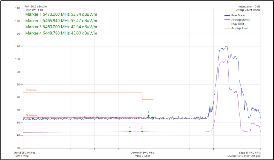
Figure 263 - 802.11ax HE40, RU 106-53, SDM, Core 0-1 - 5550 MHz Band Edge Frequency 5460 MHz
