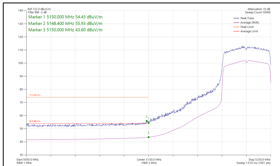
Figure 245 - 802.11ax HE40, SU, SDM, Core 0-1 - 5230 MHz Band Edge Frequency 5150 MHz
