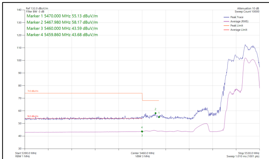
Figure 233 - 802.11ax HE40, RU 106-56, CDD, Core 0-1 - 5510 MHz Band Edge Frequency 5460 MHz
