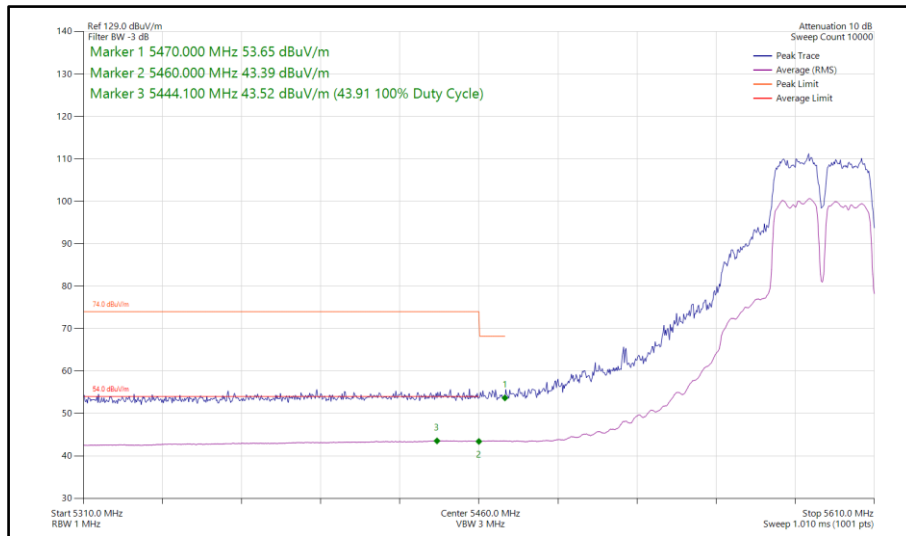
Figure 228 - 802.11a a40, CDD, Core 0-1 - 5590 MHz Band Edge Frequency 5460 MHz
