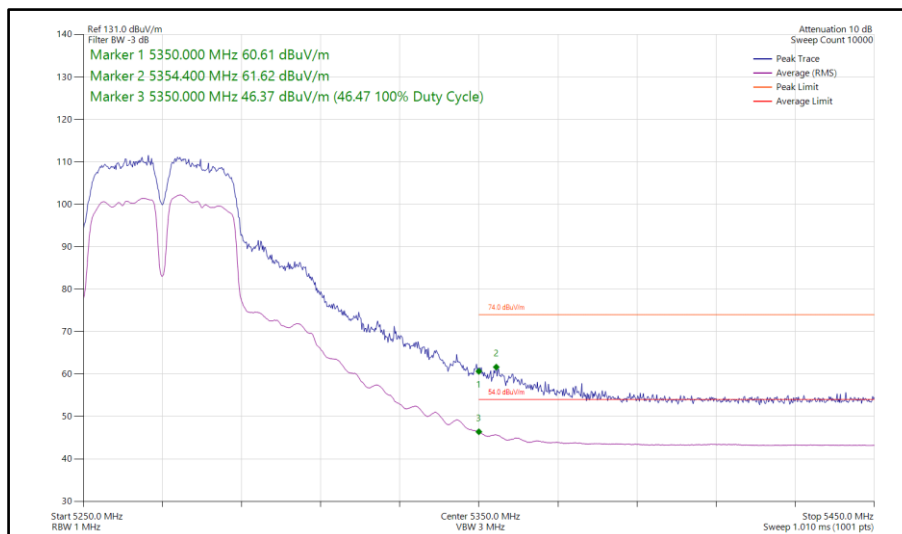
Figure 216 - 802.11a a40, CDD, Core 0-1 - 5270 MHz Band Edge Frequency 5350 MHz
