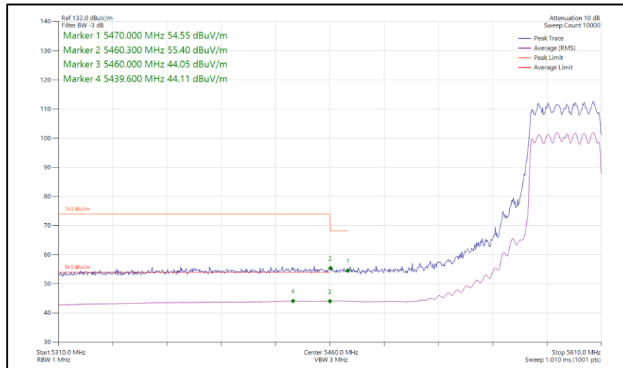
Figure 236 - 802.11ax HE40, SU, CDD, Core 0-1 - 5590 MHz Band Edge Frequency 5460 MHz
