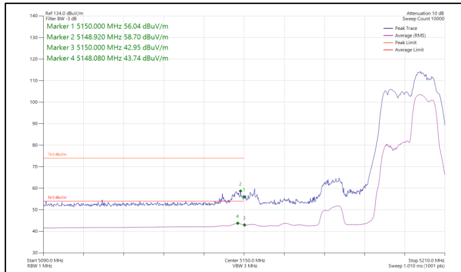
Figure 214 - 802.11be EHT40, RU 52+26-75, CDD, Core 0-1 - 5190 MHz Band Edge Frequency 5150 MHz
