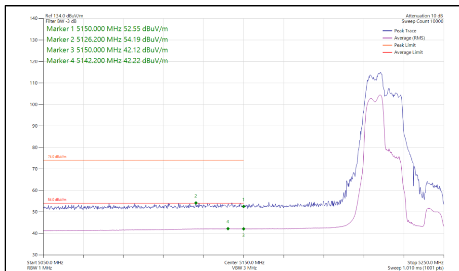
Figure 246 - 802.11ax HE40, RU 106-53, SDM, Core 0-1 - 5230 MHz Band Edge Frequency 5150 MHz
