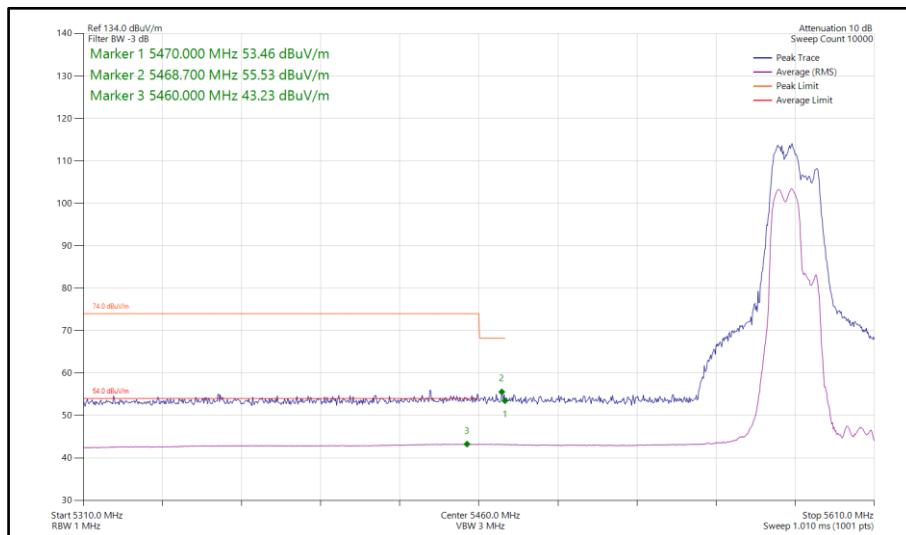
Figure 268 - 802.11be EHT40, RU 106+26-82, SDM, Core 0-1 - 5590 MHz Band Edge Frequency 5460 MHz
