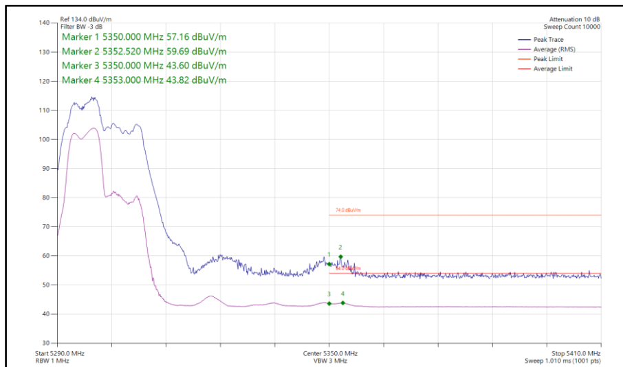
Figure 256 - 802.11be EHT40, RU 52+26-70, SDM, Core 0-1 - 5310 MHz Band Edge Frequency 5350 MHz
