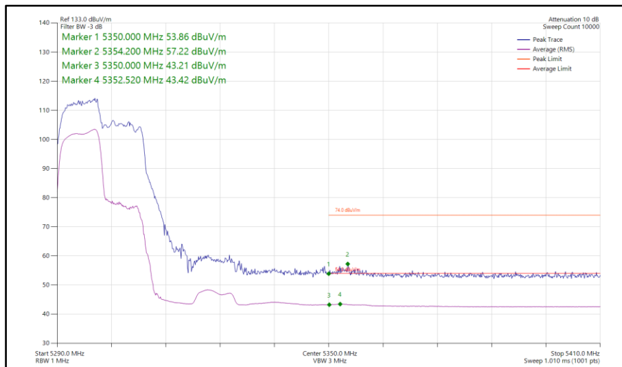
Figure 254 - 802.11ax HE40, RU 106-53, SDM, Core 0-1 - 5310 MHz Band Edge Frequency 5350 MHz
