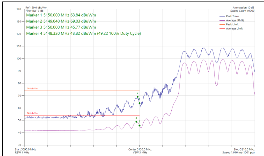
Figure 206 - 802.11a a40, CDD, Core 0-1 - 5190 MHz Band Edge Frequency 5150 MHz
