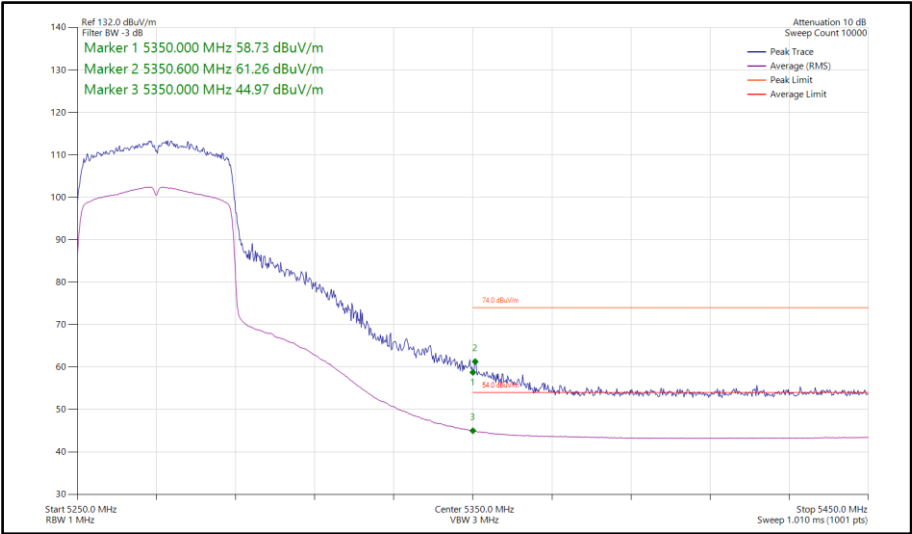
Figure 251 - 802.11ax HE40, SU, SDM, Core 0-1 - 5270 MHz Band Edge Frequency 5350 MHz
