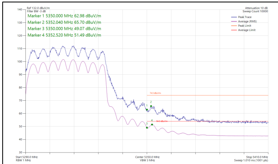
Figure 222 - 802.11ax HE40, SU, CDD, Core 0-1 - 5310 MHz Band Edge Frequency 5350 MHz
