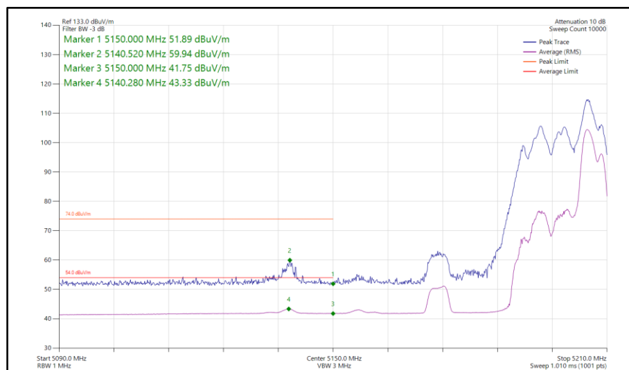
Figure 244 - 802.11ax HE40, RU 52-44, SDM, Core 0-1 - 5190 MHz Band Edge Frequency 5150 MHz
