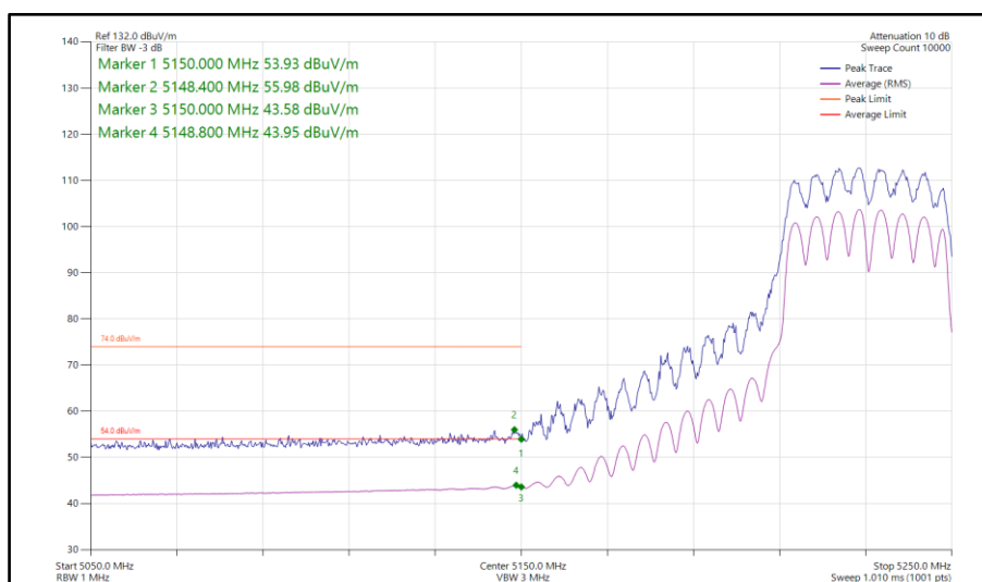
Figure 209 - 802.11n HT40, CDD, Core 0-1 - 5230 MHz Band Edge Frequency 5150 MHz
