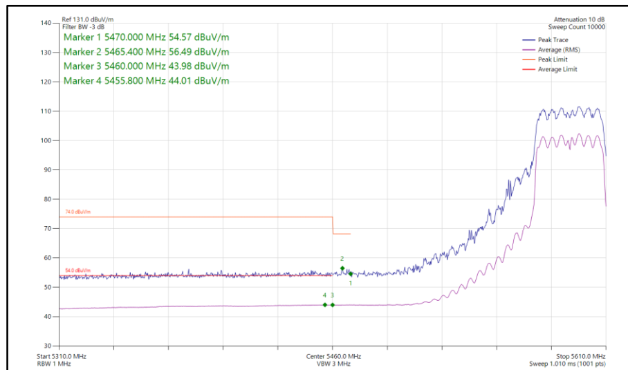
Figure 231 - 802.11n HT40, CDD, Core 0-1 - 5590 MHz Band Edge Frequency 5460 MHz
