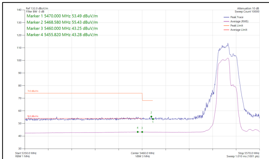
Figure 239 - 802.11be EHT40, RU 106+26-82, CDD, Core 0-1 - 5550 MHz Band Edge Frequency 5460 MHz
