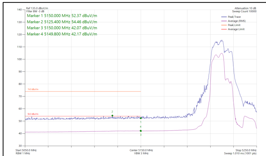
Figure 215 - 802.11be EHT40, CDD, RU 106+26-82, Core 0-1 - 5230 MHz Band Edge Frequency 5150 MHz
