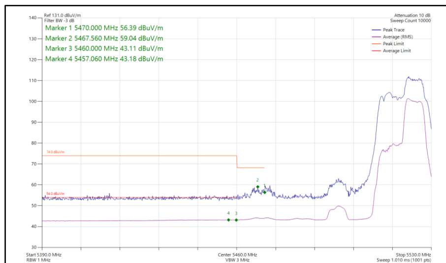
Figure 266 - 802.11be EHT40, RU 52+26-75, SDM, Core 0-1 - 5510 MHz Band Edge Frequency 5460 MHz
