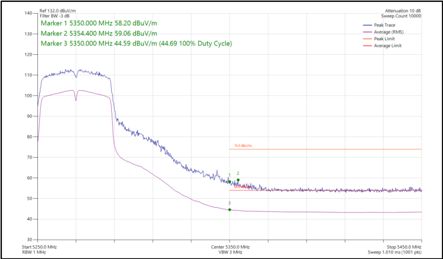
Figure 249 - 802.11n HT40, SDM, Core 0-1 - 5270 MHz Band Edge Frequency 5350 MHz
