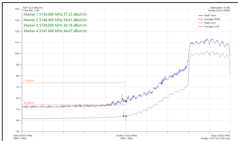
Figure 212 - 802.11ax HE40, SU, CDD, Core 0-1 - 5230 MHz Band Edge Frequency 5150 MHz
