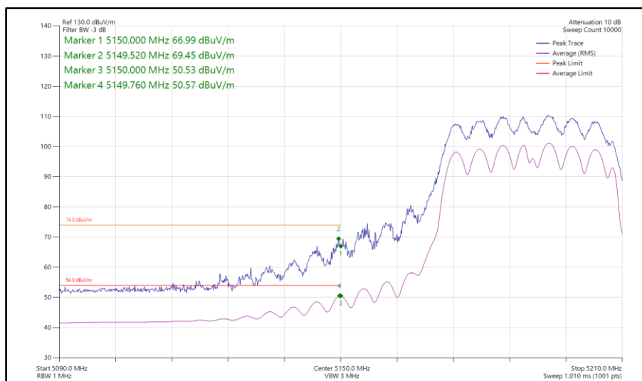
Figure 208 - 802.11n HT40, CDD, Core 0-1 - 5190 MHz Band Edge Frequency 5150 MHz
