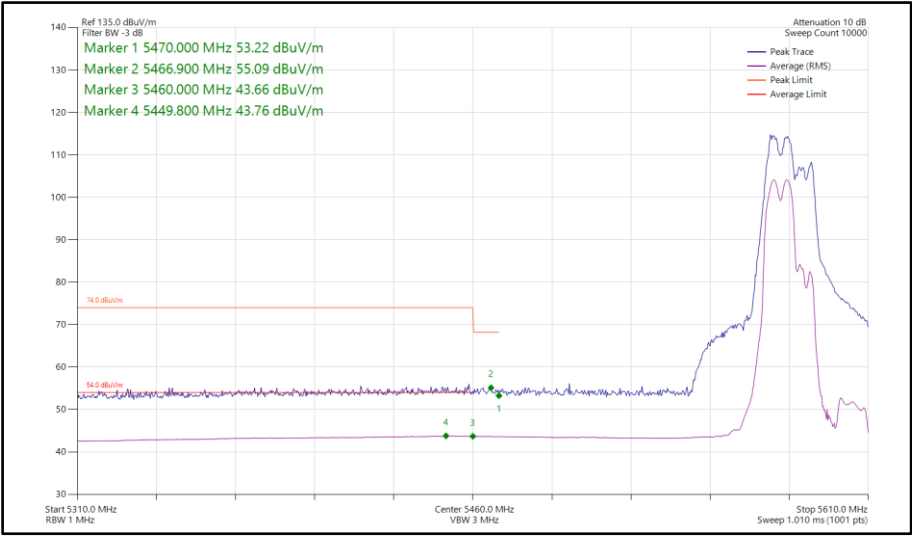
Figure 240 - 802.11be EHT40, RU 106+26-82, CDD, Core 0-1 - 5590 MHz Band Edge Frequency 5460 MHz
