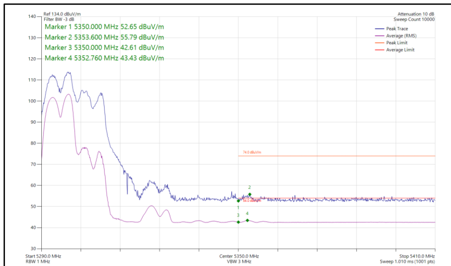
Figure 223 - 802.11ax HE40, RU 106-53, CDD, Core 0-1 - 5310 MHz Band Edge Frequency 5350 MHz
