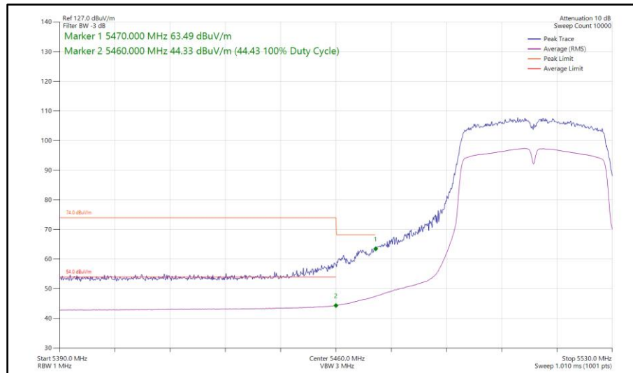
Figure 257 - 802.11n HT40, SDM, Core 0-1 - 5510 MHz Band Edge Frequency 5460 MHz
