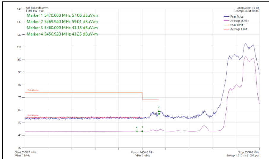
Figure 238 - 802.11be EHT40, RU 52+26-75, CDD, Core 0-1 - 5510 MHz Band Edge Frequency 5460 MHz
