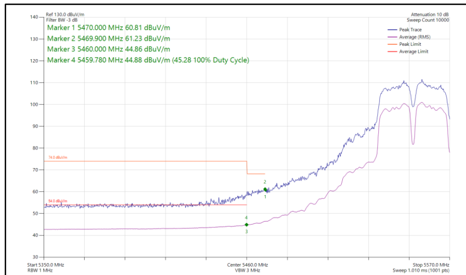
Figure 227 - 802.11a a40, CDD, Core 0-1 - 5550 MHz Band Edge Frequency 5460 MHz
