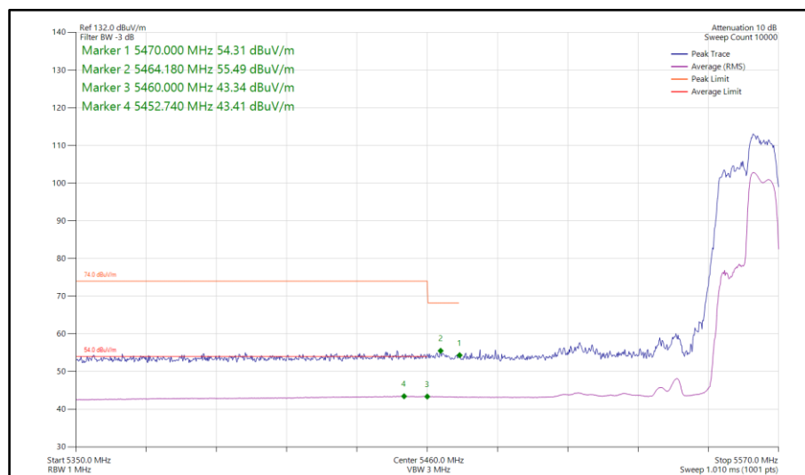
Figure 235 - 802.11ax HE40, RU 106-56, CDD, Core 0-1 - 5550 MHz Band Edge Frequency 5460 MHz
