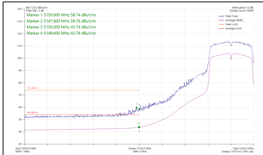
Figure 270 - 802.11ac VHT40, TxBF, Core 0-1 - 5230 MHz Band Edge Frequency 5150 MHz
