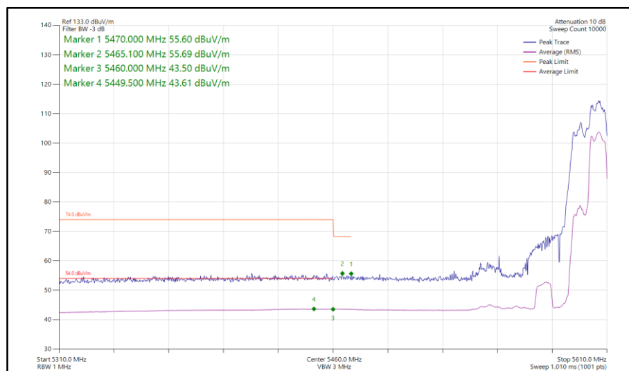
Figure 237 - 802.11ax HE40, RU 106-56, CDD, Core 0-1 - 5590 MHz Band Edge Frequency 5460 MHz
