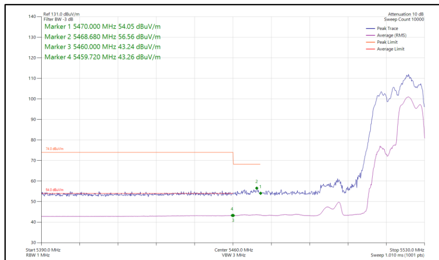
Figure 261 - 802.11ax HE40, RU 106-56, SDM, Core 0-1 - 5510 MHz Band Edge Frequency 5460 MHz
