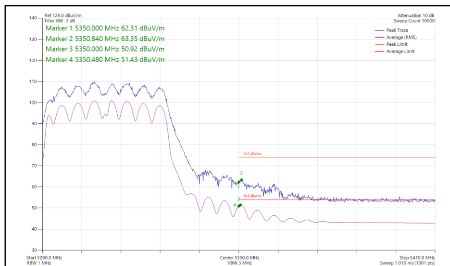
Figure 219 - 802.11n HT40, CDD, Core 0-1 - 5310 MHz Band Edge Frequency 5350 MHz
