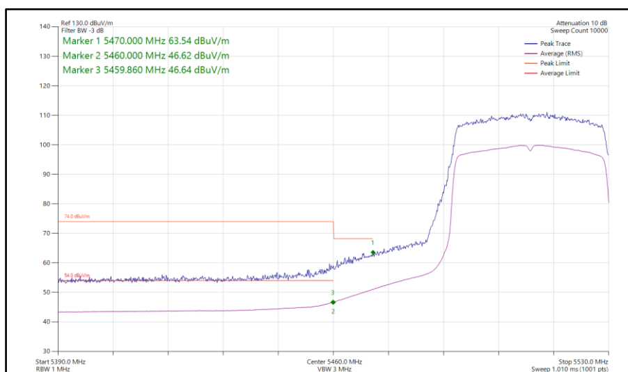
Figure 260 - 802.11ax HE40, SU, SDM, Core 0-1 - 5510 MHz Band Edge Frequency 5460 MHz
