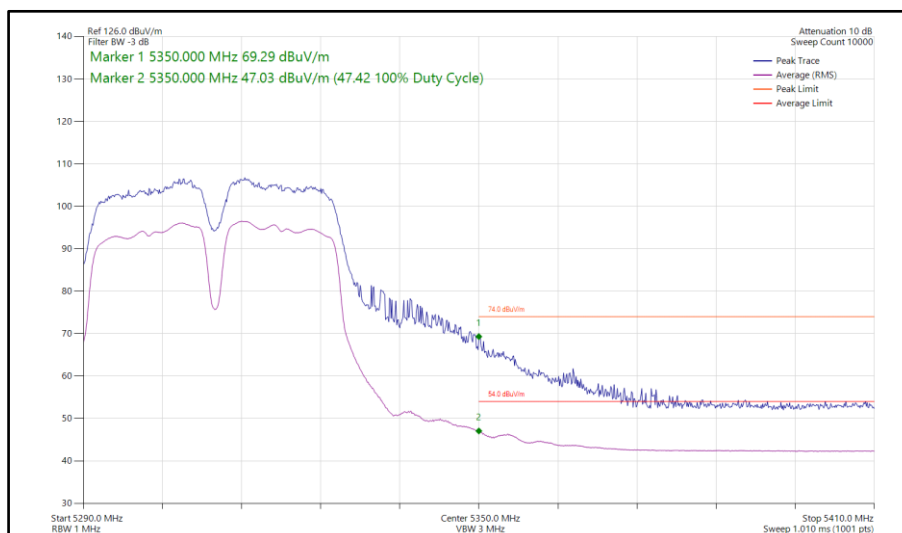
Figure 217 - 802.11a a40, CDD, Core 0-1 - 5310 MHz Band Edge Frequency 5350 MHz
