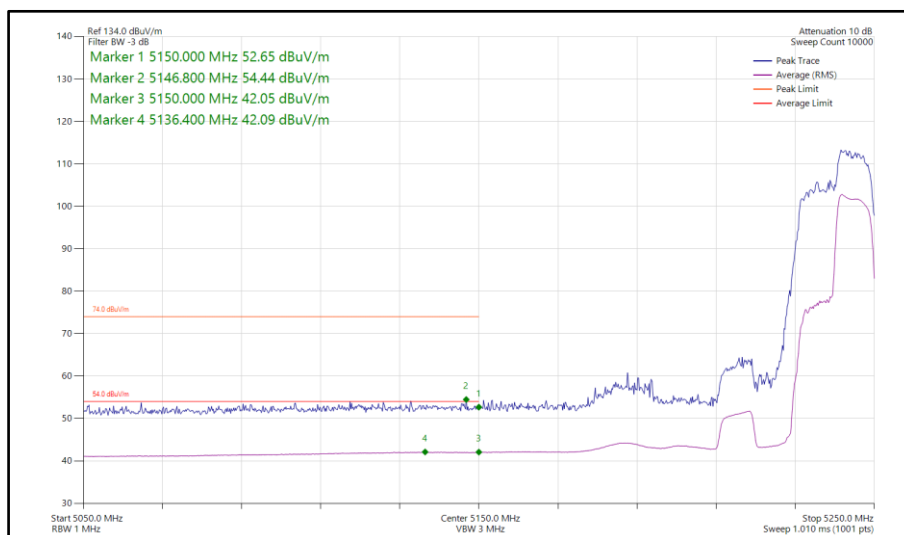
Figure 213 - 802.11ax HE40, RU 106-56, CDD, Core 0-1 - 5230 MHz Band Edge Frequency 5150 MHz
