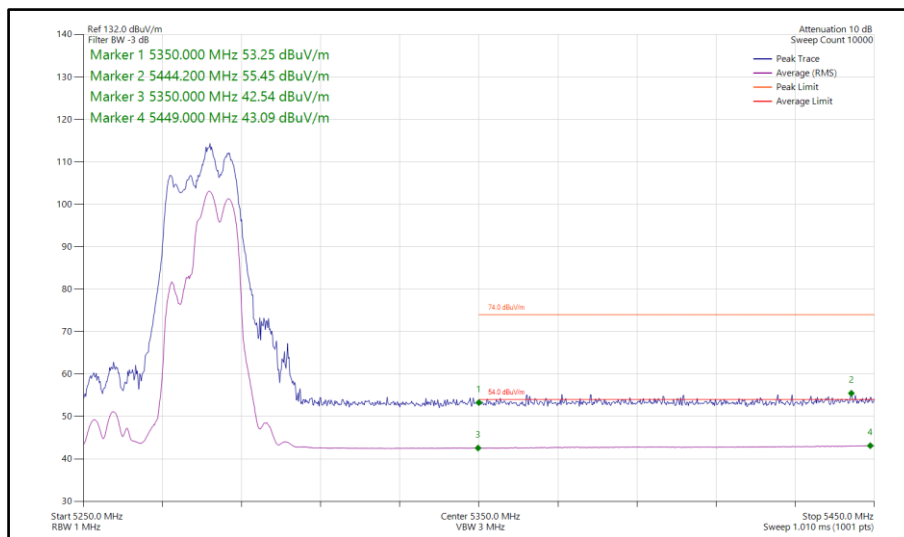
Figure 224 - 802.11be EHT40, RU 106+26-85, CDD, Core 0-1 - 5270 MHz Band Edge Frequency 5350 MHz
