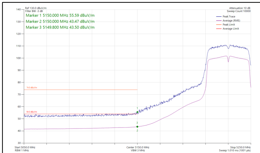
Figure 242 - 802.11n HT40, SDM, Core 0-1 - 5230 MHz Band Edge Frequency 5150 MHz
