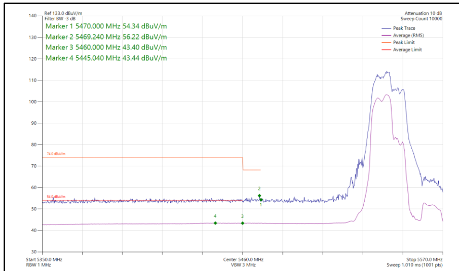
Figure 267 - 802.11be EHT40, RU 106+26-82, SDM, Core 0-1 - 5550 MHz Band Edge Frequency 5460 MHz
