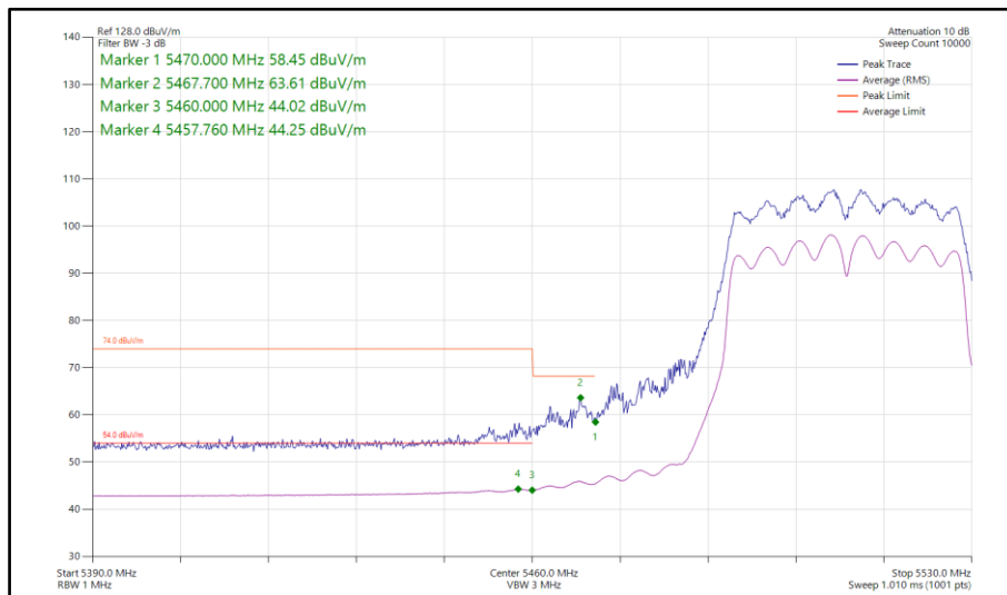
Figure 229 - 802.11n HT40, CDD, Core 0-1 - 5510 MHz Band Edge Frequency 5460 MHz
