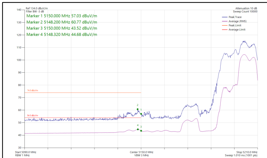
Figure 211 - 802.11ax HE40, RU 106-56, CDD, Core 0-1 - 5190 MHz Band Edge Frequency 5150 MHz
