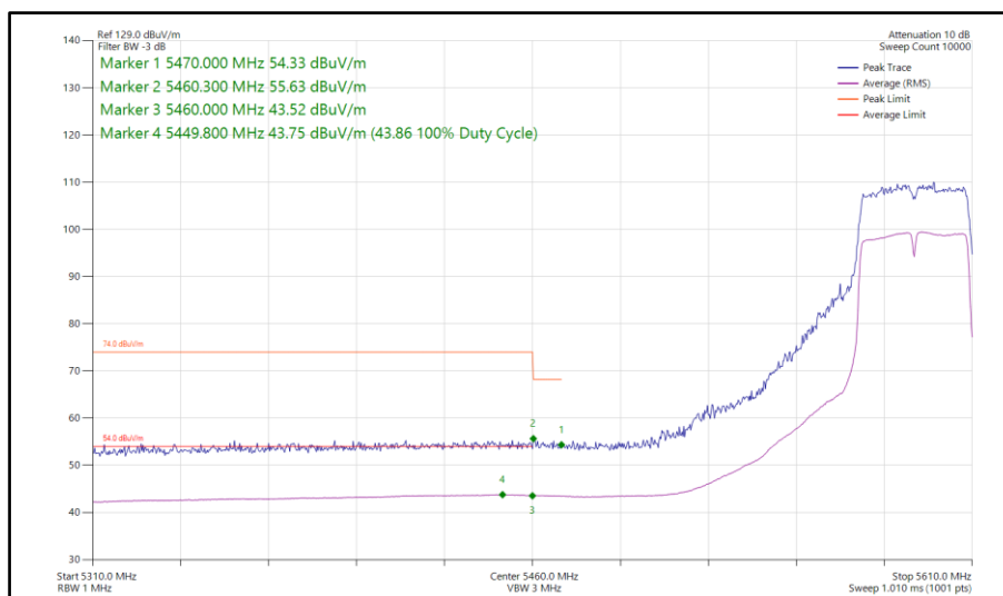
Figure 259 - 802.11n HT40, SDM, Core 0-1 - 5590 MHz Band Edge Frequency 5460 MHz
