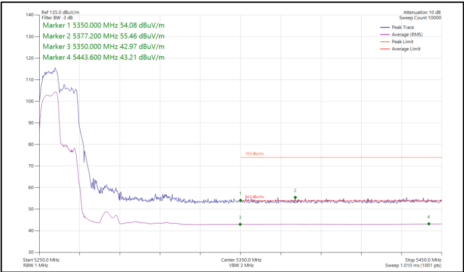
Figure 252 - 802.11ax HE40, RU 106-53, SDM, Core 0-1 - 5270 MHz Band Edge Frequency 5350 MHz
