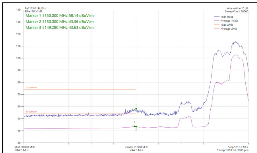
Figure 247 - 802.11be EHT40, RU 52+26-75, SDM, Core 0-1 - 5190 MHz Band Edge Frequency 5150 MHz
