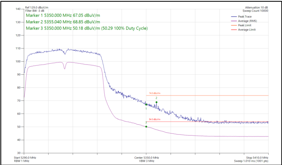
Figure 250 - 802.11n HT40, SDM, Core 0-1 - 5310 MHz Band Edge Frequency 5350 MHz
