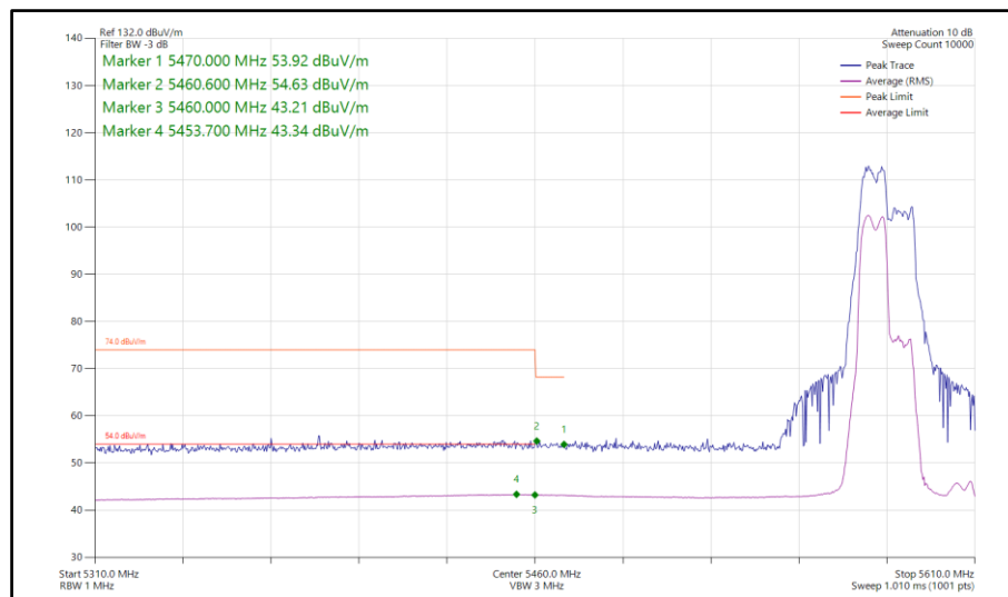
Figure 265 - 802.11ax HE40, RU 106-53, SDM, Core 0-1 - 5590 MHz Band Edge Frequency 5460 MHz
