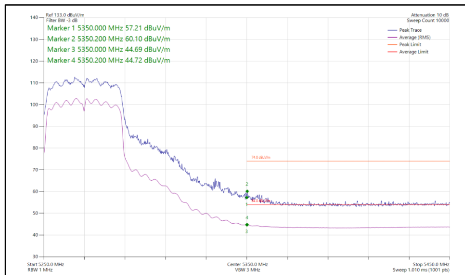
Figure 218 - 802.11n HT40, CDD, Core 0-1 - 5270 MHz Band Edge Frequency 5350 MHz
