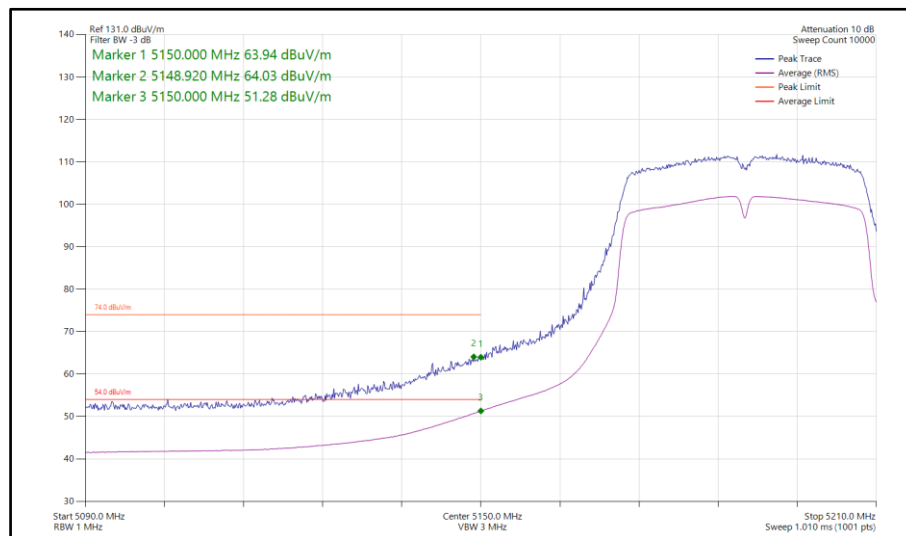
Figure 269 - 802.11ac VHT40, TxBF, Core 0-1 - 5190 MHz Band Edge Frequency 5150 MHz
