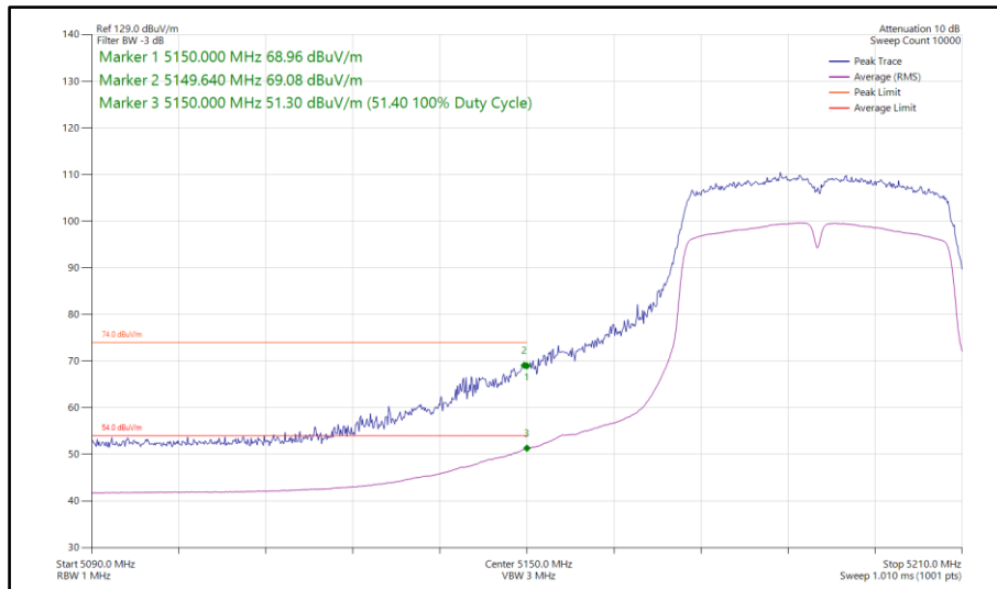
Figure 241 - 802.11n HT40, SDM, Core 0-1 - 5190 MHz Band Edge Frequency 5150 MHz
