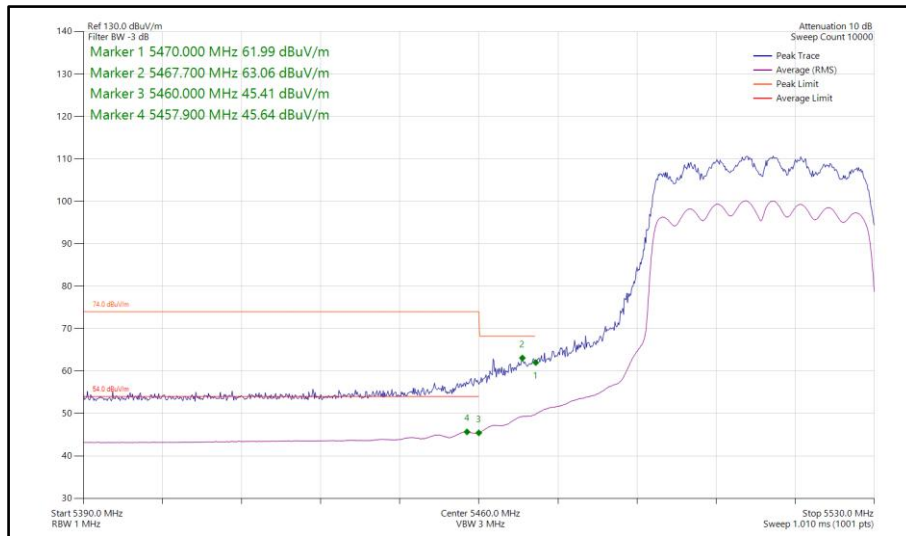
Figure 232 - 802.11ax HE40, SU, CDD, Core 0-1 - 5510 MHz Band Edge Frequency 5460 MHz
