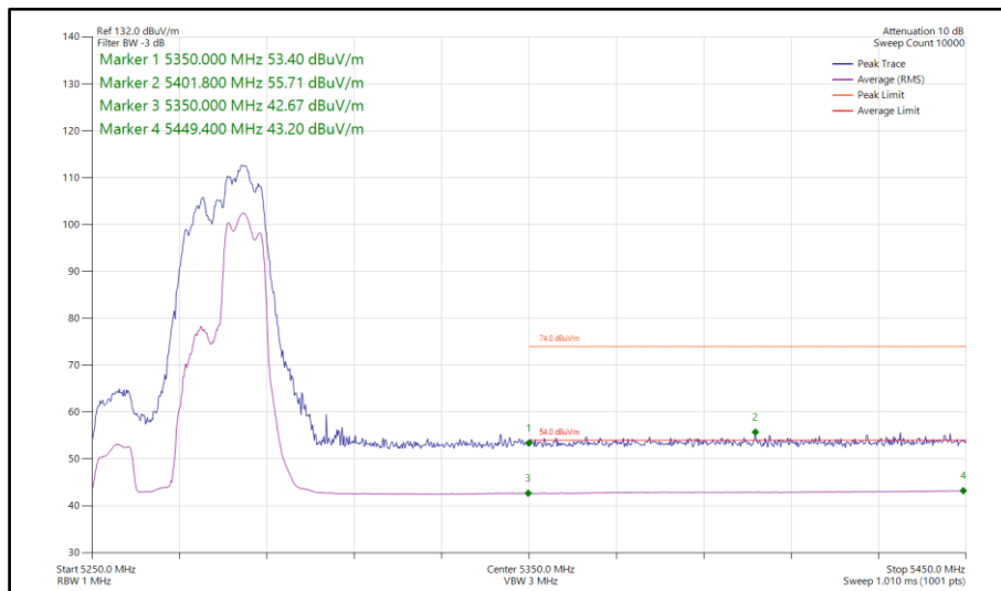
Figure 221 - 802.11ax HE40, RU 106-56, CDD, Core 0-1 - 5270 MHz Band Edge Frequency 5350 MHz
