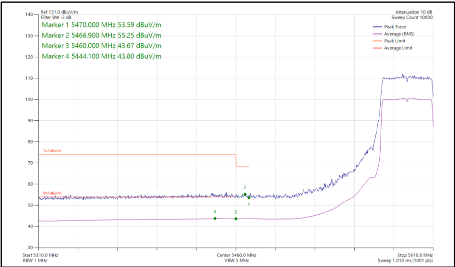
Figure 264 - 802.11ax HE40, SU, SDM, Core 0-1 - 5590 MHz Band Edge Frequency 5460 MHz
