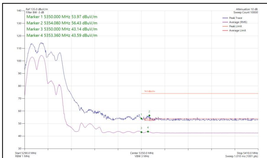
Figure 225 - 802.11be EHT40, RU 106+26-82, CDD, Core 0-1 - 5310 MHz Band Edge Frequency 5350 MHz
