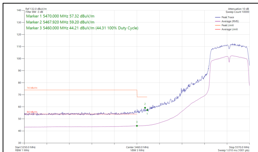
Figure 258 - 802.11n HT40, SDM, Core 0-1 - 5550 MHz Band Edge Frequency 5460 MHz
