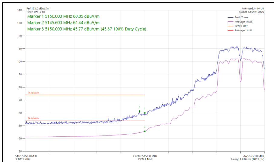
Figure 207 - 802.11a a40, CDD, Core 0-1 - 5230 MHz Band Edge Frequency 5150 MHz
