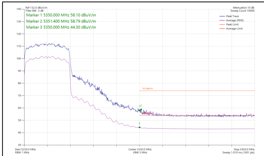
Figure 220 - 802.11ax HE40, SU, CDD, Core 0-1 - 5270 MHz Band Edge Frequency 5350 MHz
