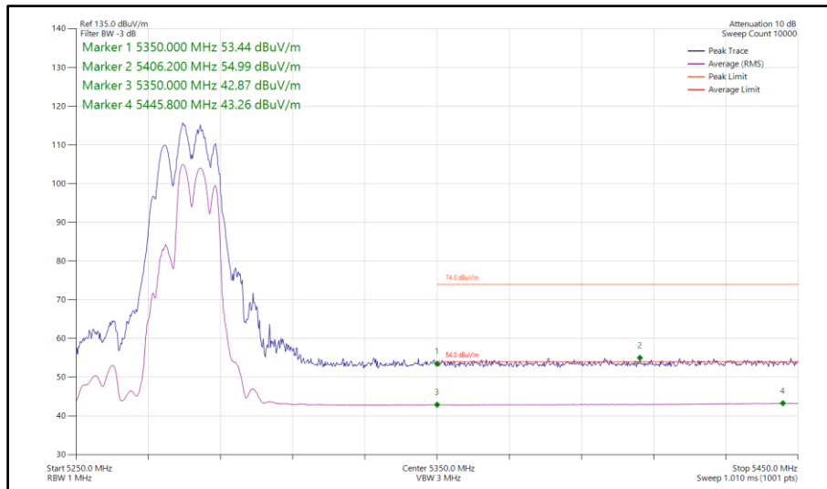
Figure 255 - 802.11be EHT40, RU 106+26-85, SDM, Core 0-1 - 5270 MHz Band Edge Frequency 5350 MHz
