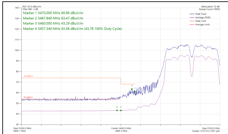
Figure 226 - 802.11a a40, CDD, Core 0-1 - 5510 MHz Band Edge Frequency 5460 MHz
