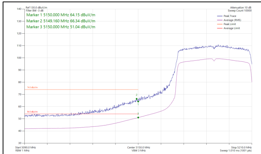
Figure 243 - 802.11ax HE40, SU, SDM, Core 0-1 - 5190 MHz Band Edge Frequency 5150 MHz
