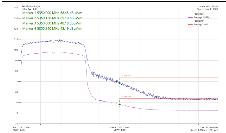
Figure 253 - 802.11ax HE40, SU, SDM, Core 0-1 - 5310 MHz Band Edge Frequency 5350 MHz
