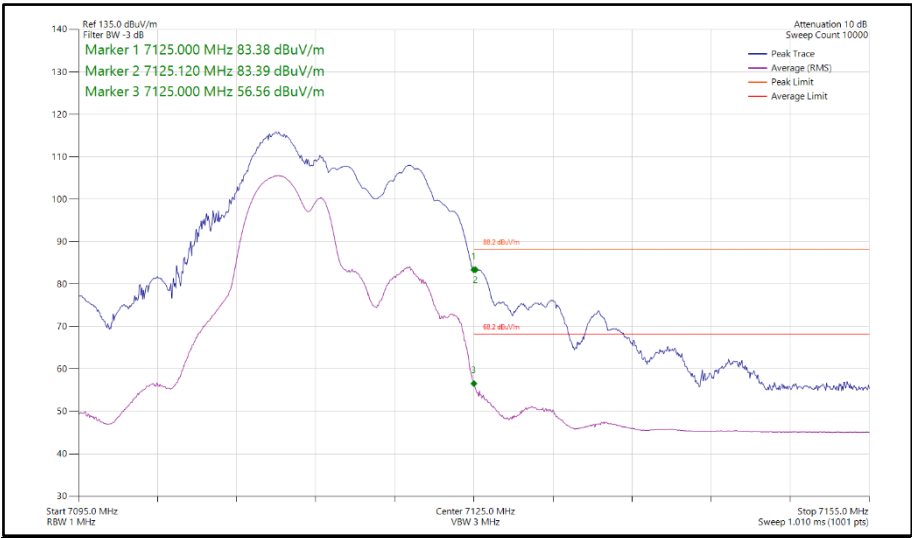
Figure 424 - 802.11be EHT20 RU 52+26-70, CDD, Core 0-1 - 7115 MHz Band Edge Frequency 7125 MHz
