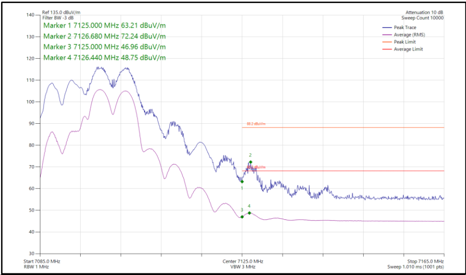
Figure 432 - 802.11be EHT20 106+26-83, SDM, Core 0-1 - 7095 MHz Band Edge Frequency 7125 MHz
