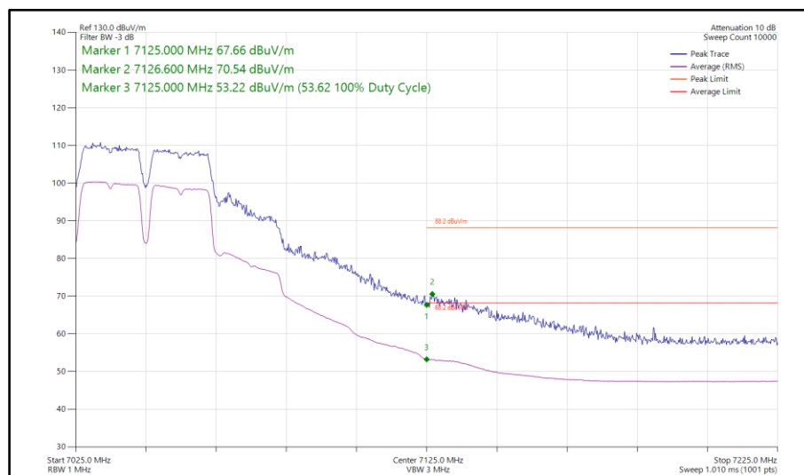
Figure 441 - 802.11a 40, SISO, Core 0 - 7045 MHz Band Edge Frequency 7125 MHz
