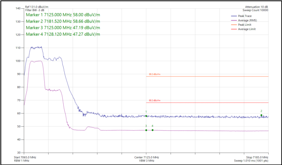
Figure 446 - 802.11be EHT40 RU 52+26-70, SISO, Core 0 - 7085 MHz Band Edge Frequency 7125 MHz
