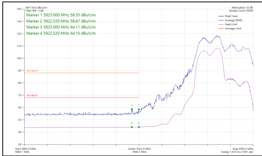
Figure 426 - 802.11ax HE20, RU 106-53, SDM, Core 0-1 - 5955 MHz Band Edge Frequency 5925 MHz
