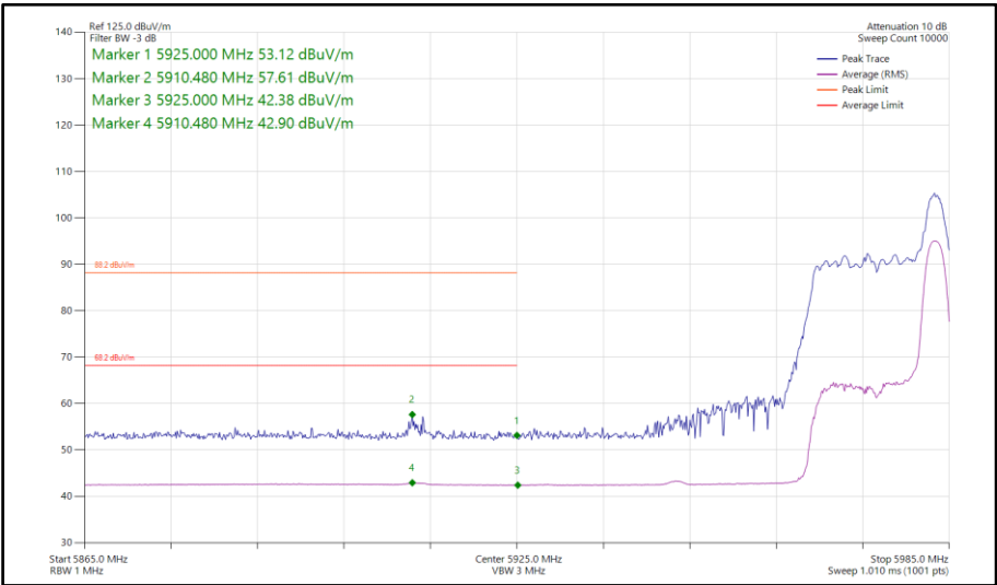
Figure 449 - 802.11ax HE40, RU 26-17, SISO, Core 1 - 5965 MHz Band Edge Frequency 5925 MHz
