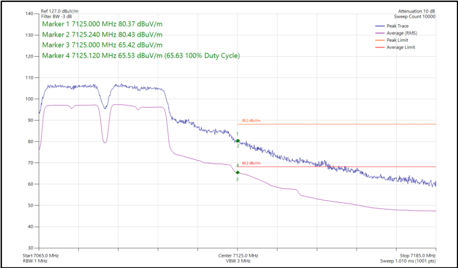
Figure 442 - 802.11a 40, SISO, Core 0 - 7085 MHz Band Edge Frequency 7125 MHz
