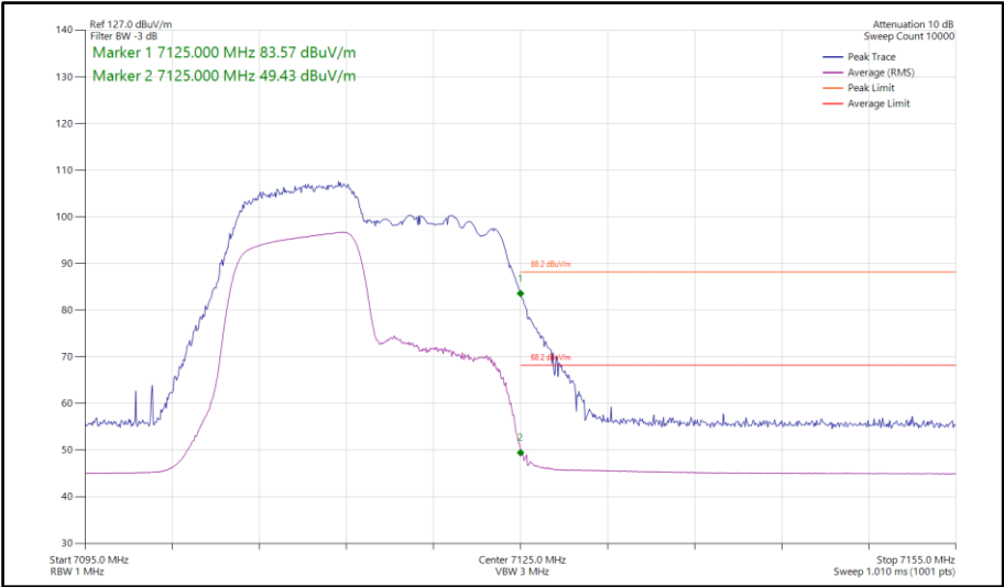
Figure 410 - 802.11ax HE20, RU 106-53, SISO, Core 1 - 7115 MHz Band Edge Frequency 7125 MHz
