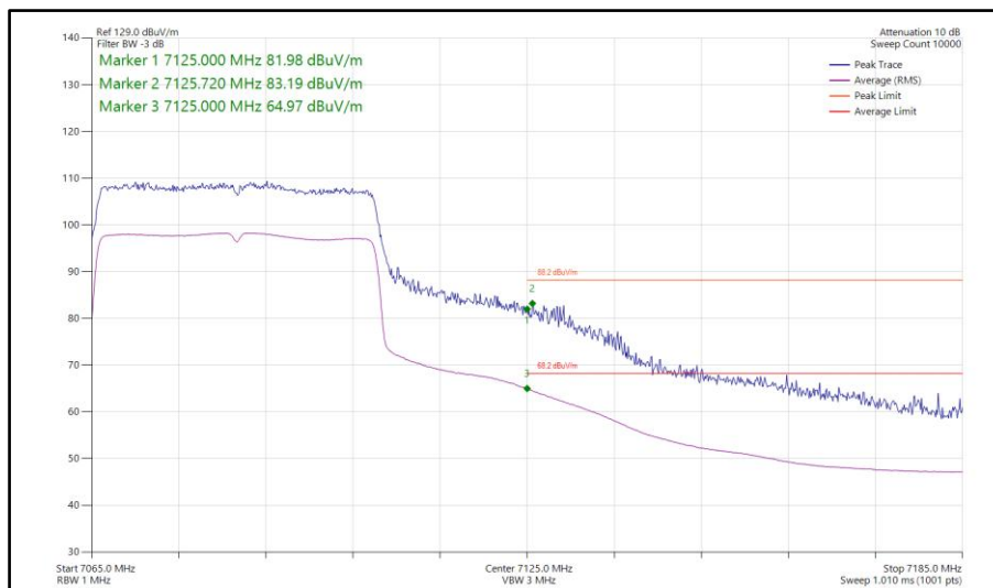
Figure 444 - 802.11ax HE40, SU, SISO, Core 0 - 7085 MHz Band Edge Frequency 7125 MHz
