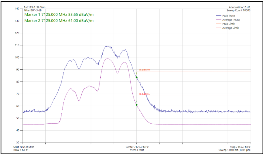
Figure 433 - 802.11be EHT20 RU 52+26-72, SDM, Core 0-1 - 7115 MHz Band Edge Frequency 7125 MHz
