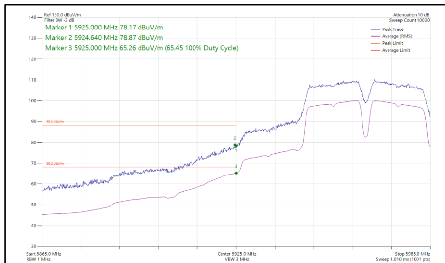
Figure 437 - 802.11a 40, SISO, Core 0 - 5965 MHz Band Edge Frequency 5925 MHz
