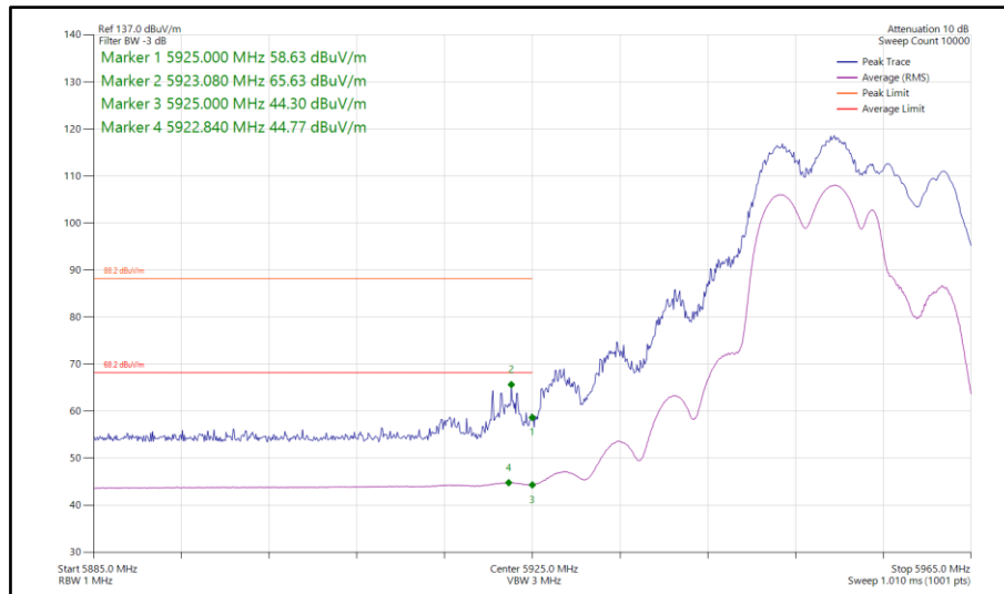
Figure 416 - 802.11be EHT20, CDD, Core 0-1 - 5955 MHz Band Edge Frequency 5925 MHz
