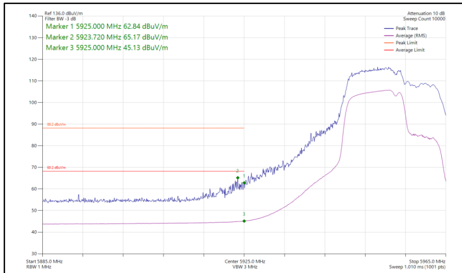
Figure 392 - 802.11be EHT20 RU 106+26-82, SISO, Core 0 - 5955 MHz Band Edge Frequency 5925 MHz
