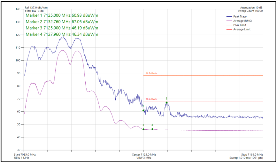
Figure 429 - 802.11ax HE20, RU 106-54, SDM, Core 0-1 - 7095 MHz Band Edge Frequency 7125 MHz
