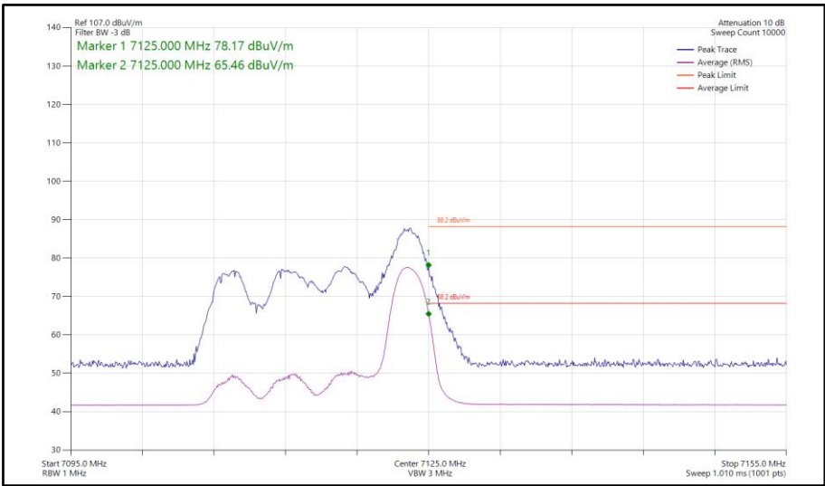
Figure 431 - 802.11ax HE20, RU 26-8, SDM, Core 0-1 - 7115 MHz Band Edge Frequency 7125 MHz
