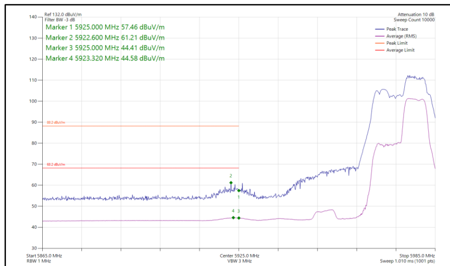
Figure 440 - 802.11be EHT40 RU 52+26-75, SISO, Core 0 - 5965 MHz Band Edge Frequency 5925 MHz
