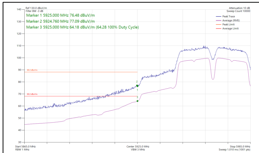
Figure 447 - 802.11a 40, SISO, Core 1 - 5965 MHz Band Edge Frequency 5925 MHz
