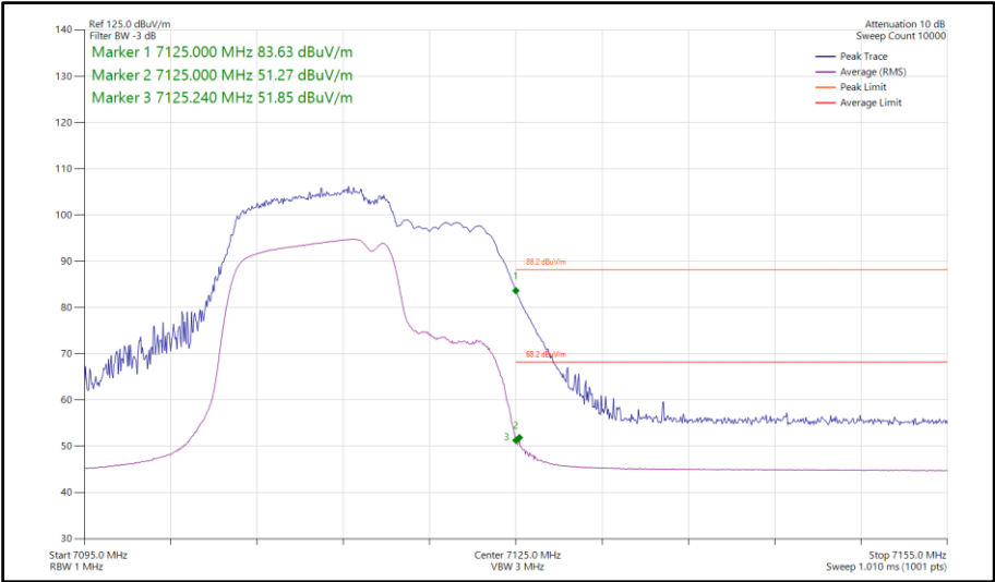
Figure 400 - 802.11be EHT20 RU 106+26-82, SISO, Core 0 - 7115 MHz Band Edge Frequency 7125 MHz
