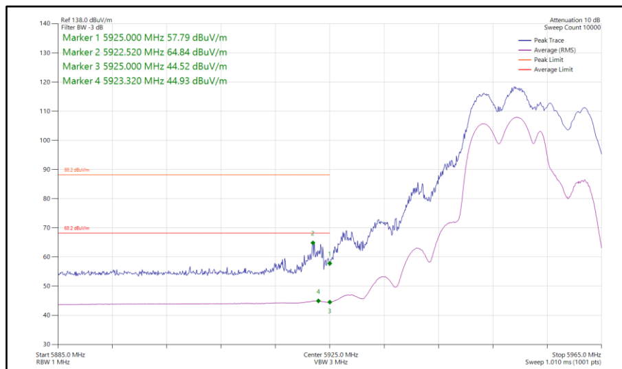
Figure 427 - 802.11be EHT20, SDM, Core 0-1 - 5955 MHz Band Edge Frequency 5925 MHz
