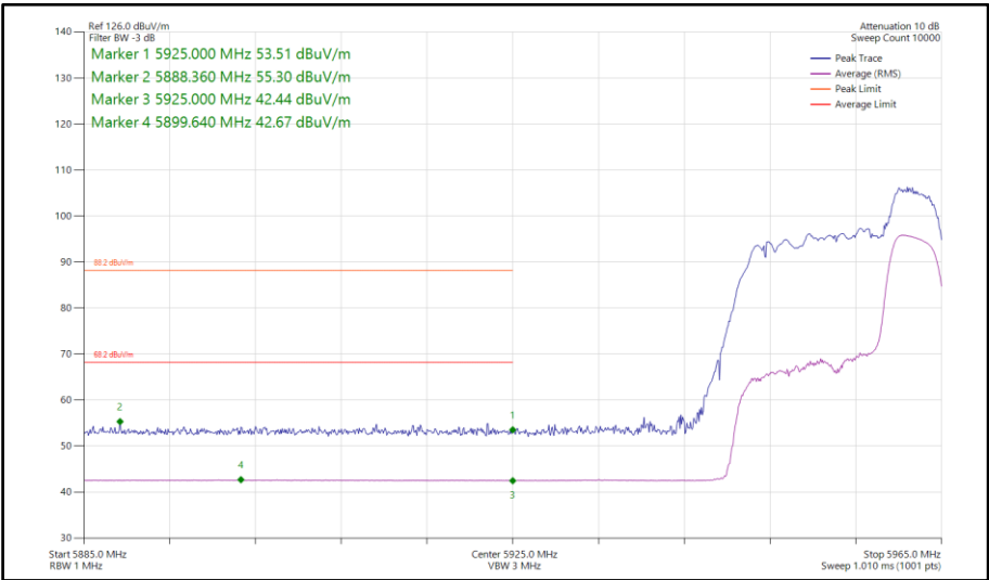
Figure 403 - 802.11ax HE20, RU 52-40, SISO, Core 1 - 5955 MHz Band Edge Frequency 5925 MHz
