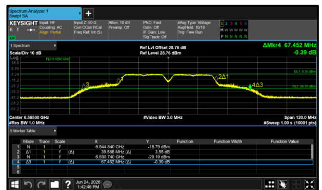
Figure 276 - 802.11a40 LPI Maximum 99% OBW
