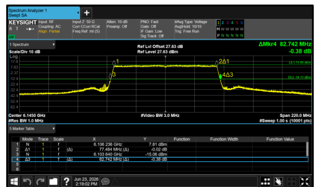
Figure 254 - 802.11ax HE80 SU SP Maximum 99% OBW
