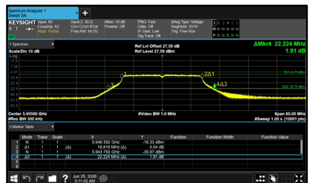
Figure 270 - 802.11a20 LPI Maximum 99% OBW
