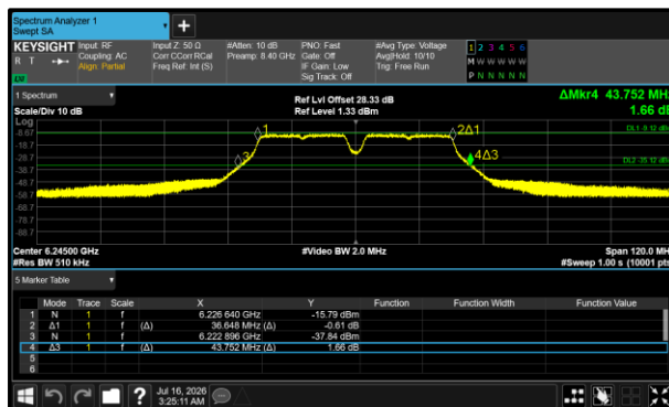
Figure 223 - 802.11a40 VLP Minimum 26 dB EBW
