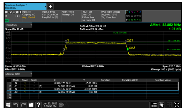
Figure 262 - 802.11ax HE80 SU VLP Maximum 99% OBW
