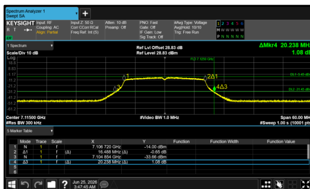
Figure 269 - 802.11a20 LPI Minimum 99% OBW
