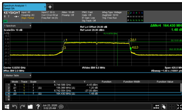
Figure 215 - 802.11ax HE160 SU VLP Minimum 26 dB EBW
