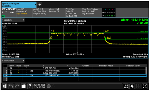
Figure 240 - 802.11a160 LPI Maximum 26 dB EBW
