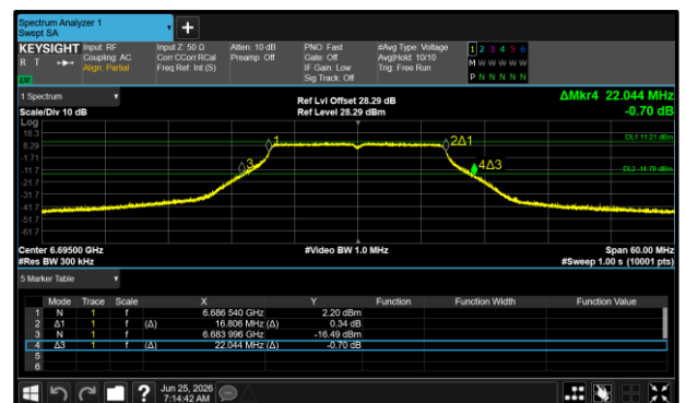
Figure 266 - 802.11a20 SP Maximum 99% OBW
