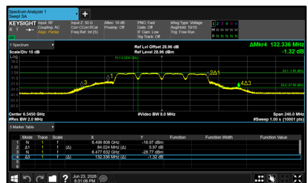
Figure 282 - 802.11a80 VLP Maximum 99% OBW
