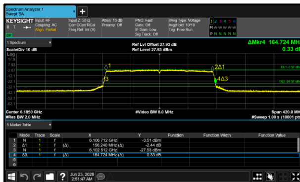
Figure 263 - 802.11ax HE160 SU VLP Minimum 99% OBW
