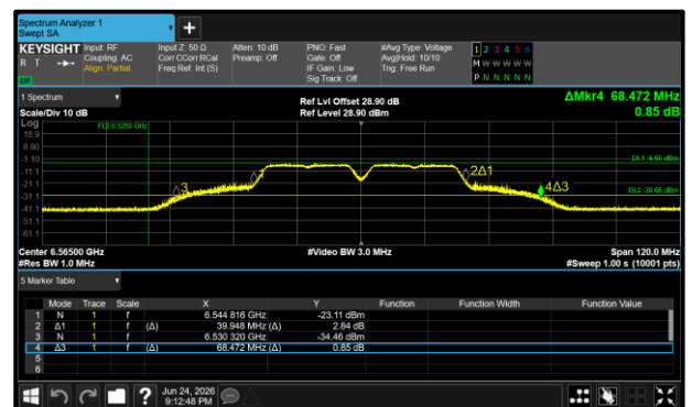
Figure 272 - 802.11a40 VLP Maximum 99% OBW
