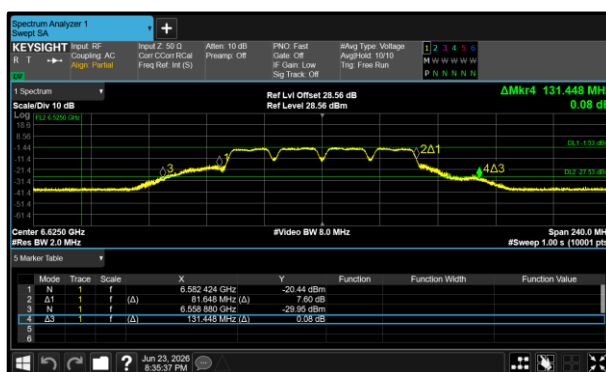
Figure 281 - 802.11a80 VLP Minimum 99% OBW
