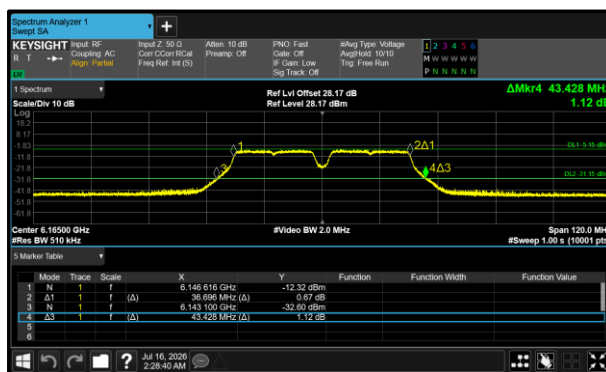
Figure 227 - 802.11a40 LPI Minimum 26 dB EBW
