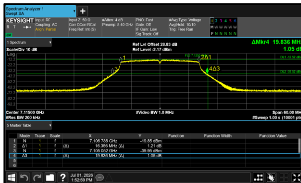
Figure 267 - 802.11a20 VLP Minimum 99% OBW
