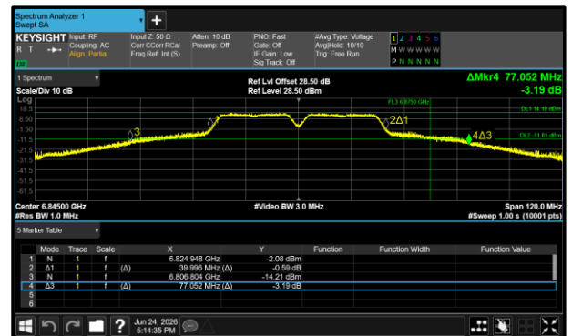
Figure 226 - 802.11a40 SP Maximum 26 dB EBW
