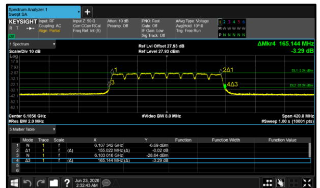
Figure 236 - 802.11a160 VLP Maximum 26 dB EBW
