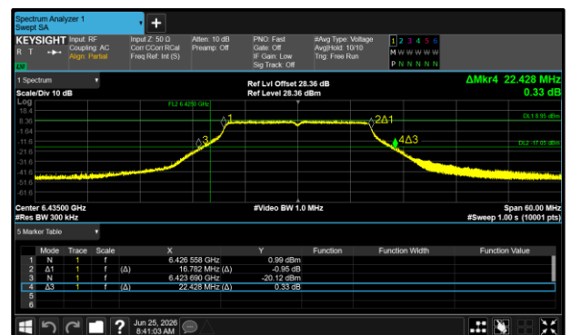
Figure 218 - 802.11a20 SP Maximum 26 dB EBW
