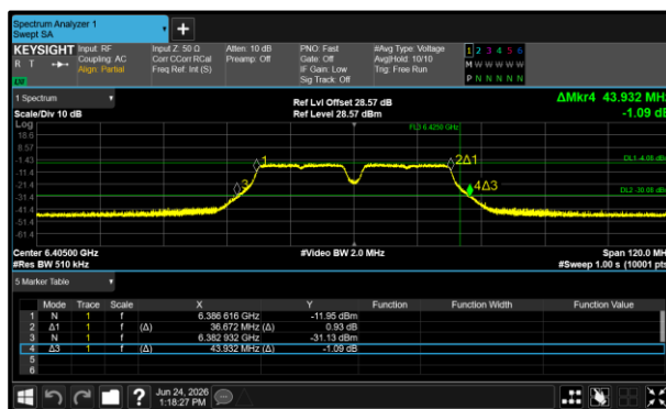
Figure 275 - 802.11a40 LPI Minimum 99% OBW
