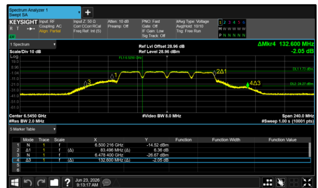
Figure 280 - 802.11a80 LPI Maximum 99% OBW
