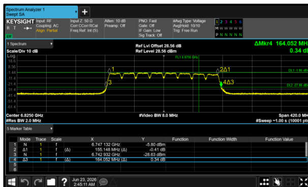
Figure 235 - 802.11a160 VLP Minimum 26 dB EBW
