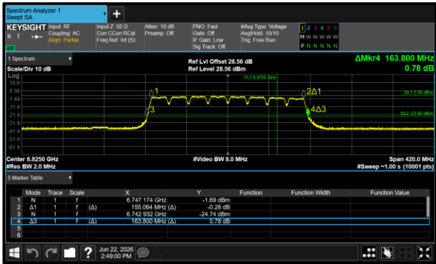
Figure 239 - 802.11a160 LPI Minimum 26 dB EBW
