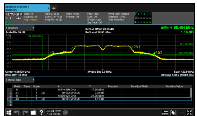
Figure 228 - 802.11a40 LPI Maximum 26 dB EBW
