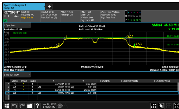
Figure 273 - 802.11a40 SP Minimum 99% OBW
