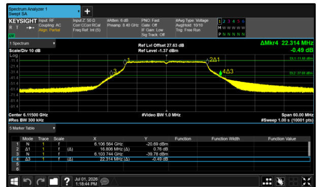
Figure 268 - 802.11a20 VLP Maximum 99% OBW
