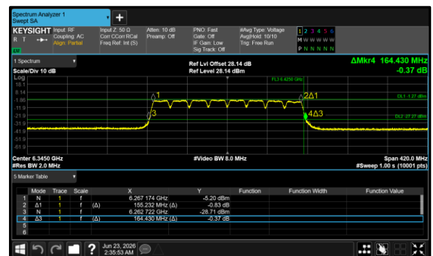
Figure 284 - 802.11a160 VLP Maximum 99% OBW
