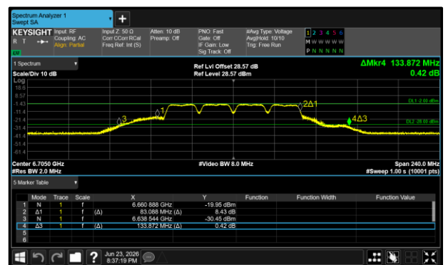
Figure 234 - 802.11a80 VLP Maximum 26 dB EBW
