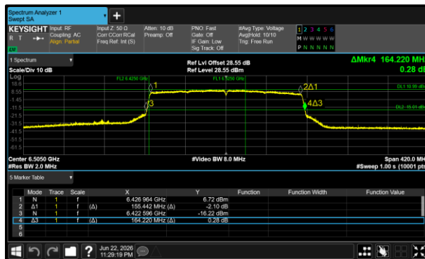
Figure 255 - 802.11ax HE160 SU SP Minimum 99% OBW
