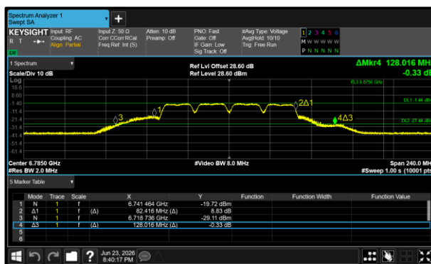
Figure 233 - 802.11a80 VLP Minimum 26 dB EBW
