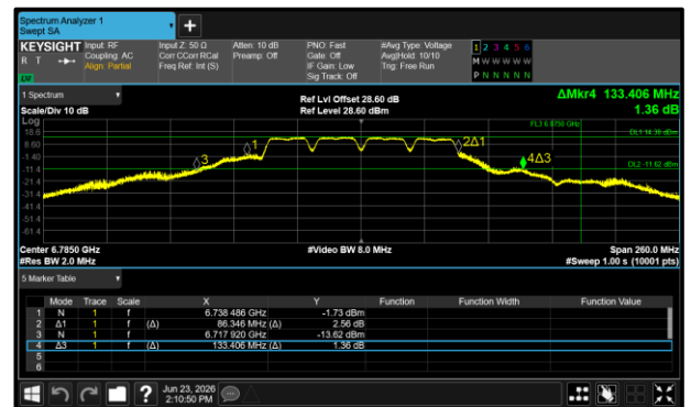
Figure 278 - 802.11a80 SP Maximum 99% OBW
