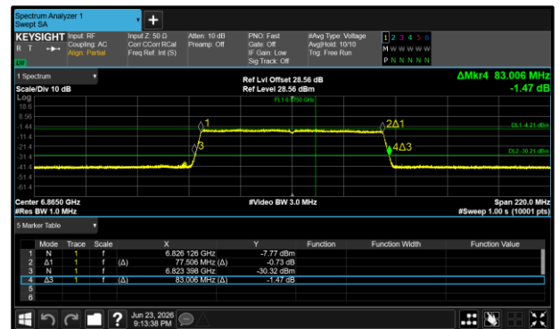
Figure 214 - 802.11ax HE80 SU VLP Maximum 26 dB EBW
