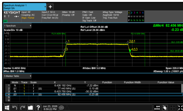
Figure 261 - 802.11ax HE80 SU VLP Minimum 99% OBW
