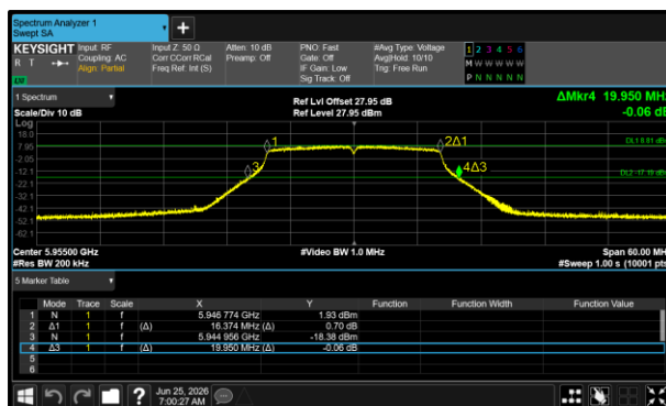
Figure 265 - 802.11a20 SP Minimum 99% OBW
