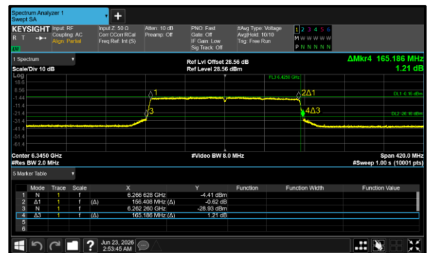
Figure 264 - 802.11ax HE160 SU VLP Maximum 99% OBW
