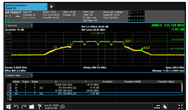
Figure 232 - 802.11a80 LPI Maximum 26 dB EBW
