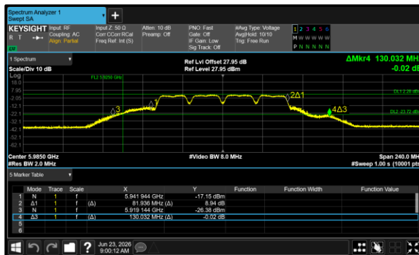
Figure 231 - 802.11a80 LPI Minimum 26 dB EBW
