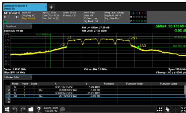
Figure 277 - 802.11a80 SP Minimum 99% OBW
