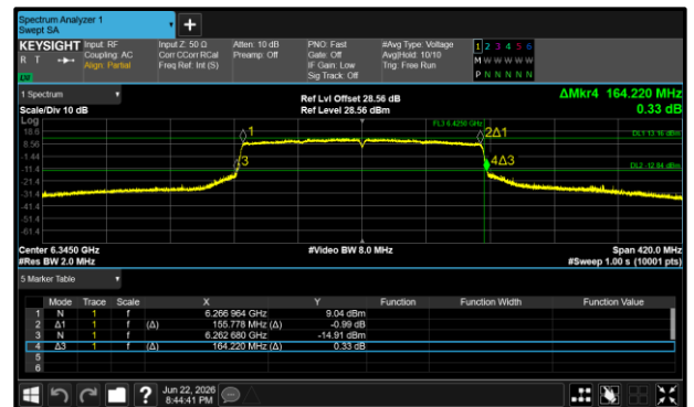
Figure 256 - 802.11ax HE160 SU SP Maximum 99% OBW
