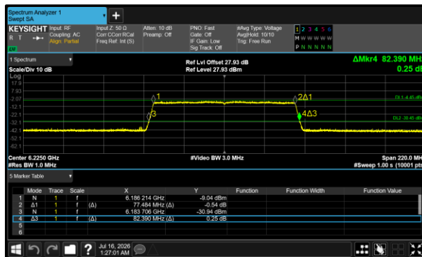
Figure 213 - 802.11ax HE80 SU VLP Minimum 26 dB EBW
