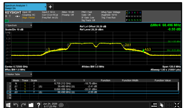
Figure 224 - 802.11a40 VLP Maximum 26 dB EBW
