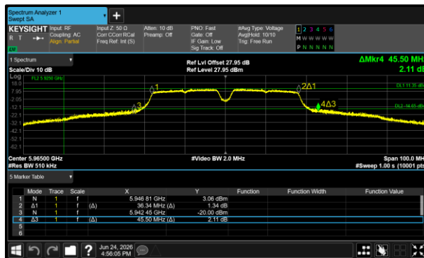
Figure 225 - 802.11a40 SP Minimum 26 dB EBW
