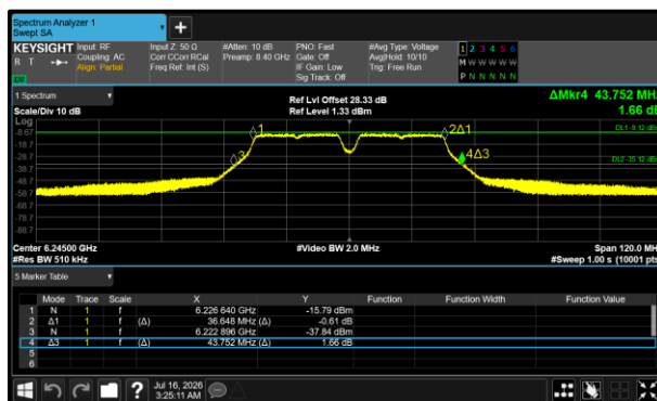
Figure 271 - 802.11a40 VLP Minimum 99% OBW
