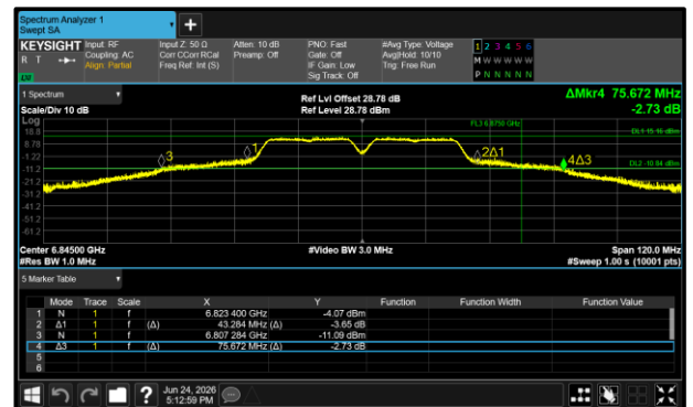
Figure 274 - 802.11a40 SP Maximum 99% OBW
