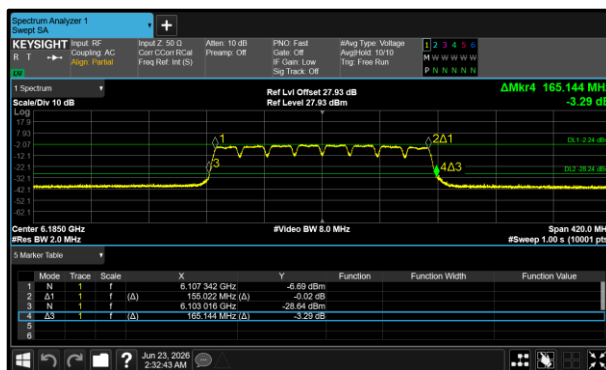
Figure 283 - 802.11a160 VLP Minimum 99% OBW
