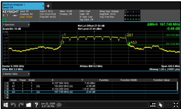
Figure 238 - 802.11a160 SP Maximum 26 dB EBW
