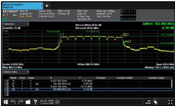
Figure 237 - 802.11a160 SP Minimum 26 dB EBW
