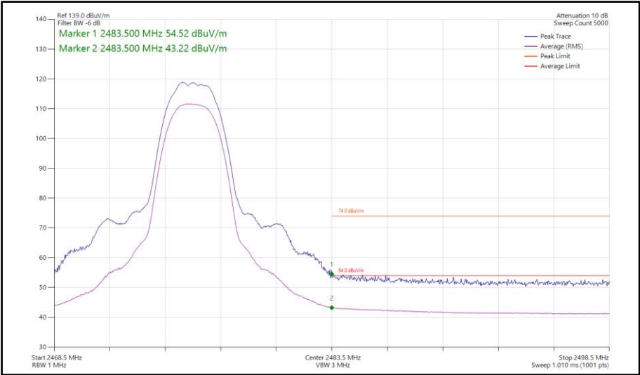
Figure 141 - Bluetooth HDT6, SISO, Core 1 - 2476 MHz Band Edge Frequency 2483.5 MHz
