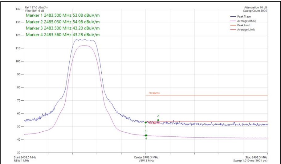
Figure 142 - Bluetooth HDRPS2, SISO, Core 1 - 2476 MHz Band Edge Frequency 2483.5 MHz
