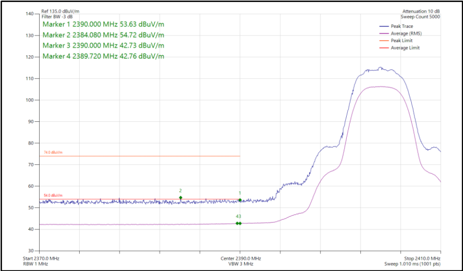
Figure 107 - Bluetooth HDRPM12, SISO, Core 0 - 2404 MHz Band Edge Frequency 2390 MHz
