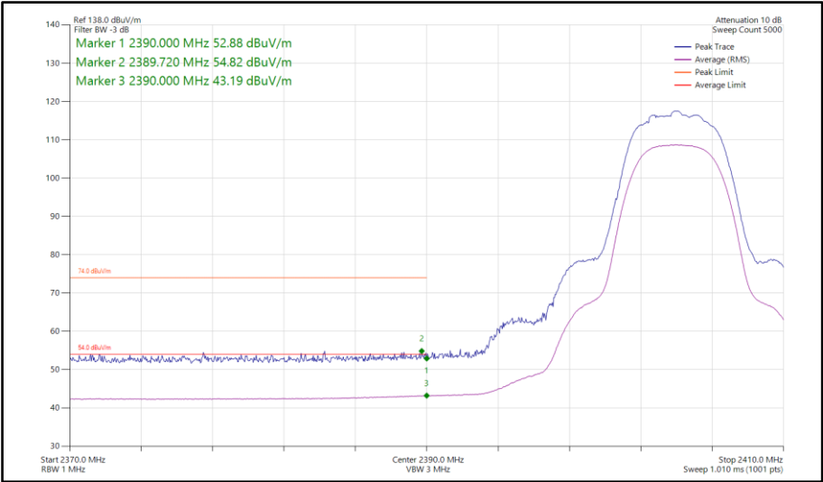
Figure 155 - Bluetooth HDRPM12, MIMO, Core 0-1 - 2404 MHz Band Edge Frequency 2390 MHz
