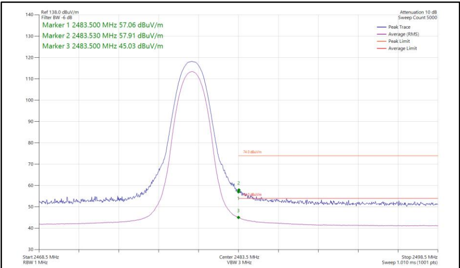
Figure 158 - Bluetooth 3DH5, MIMO, Core 0-1 - 2480 MHz Band Edge Frequency 2483.5 MHz
