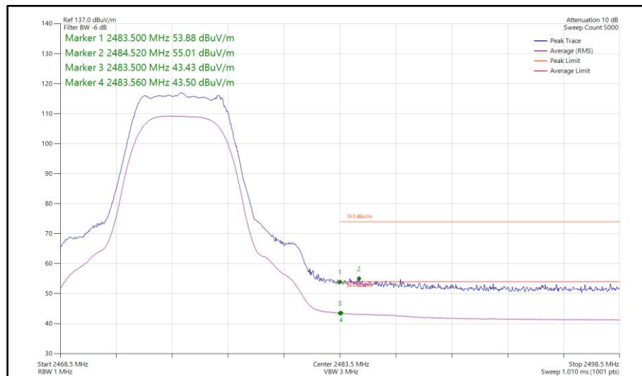
Figure 144 - Bluetooth XHDRPM8, SISO, Core 1 - 2475 MHz Band Edge Frequency 2483.5 MHz
