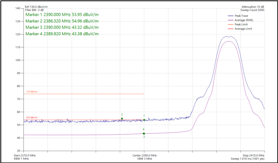
Figure 127 - Bluetooth HDT3, SISO, Core 1 - 2404 MHz Band Edge Frequency 2390 MHz
