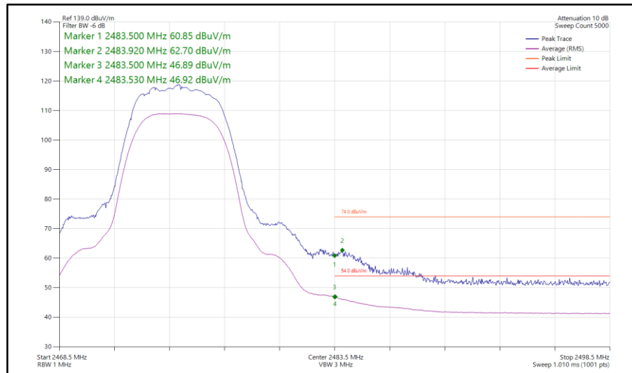
Figure 143 - Bluetooth HDRPM12, SISO, Core 1 - 2475 MHz Band Edge Frequency 2483.5 MHz
