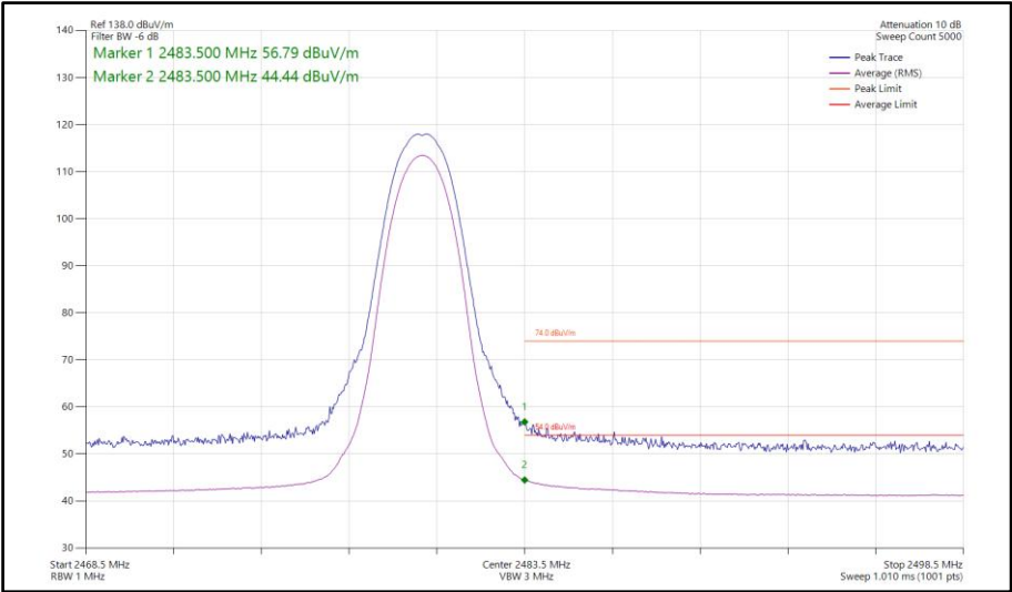
Figure 157 - Bluetooth 2DH5, MIMO, Core 0-1 - 2480 MHz Band Edge Frequency 2483.5 MHz
