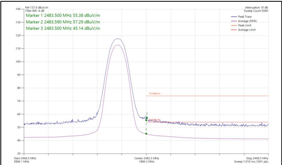
Figure 134 - Bluetooth 3DH5, SISO, Core 1 - 2480 MHz Band Edge Frequency 2483.5 MHz
