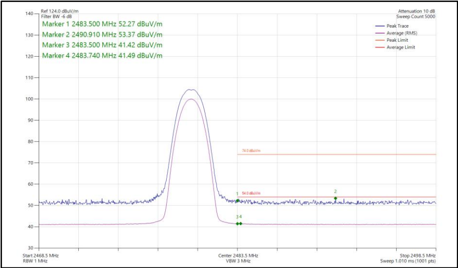
Figure 85 - Bluetooth 2DH5, MIMO, Core 0-1 - 2480 MHz Band Edge Frequency 2483.5 MHz
