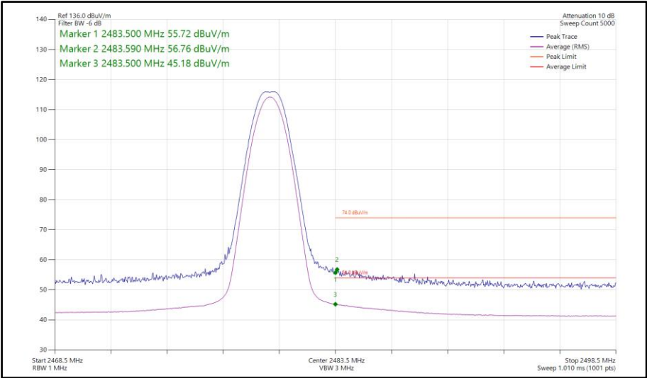
Figure 137 - Bluetooth LE1M, SISO, Core 1 - 2480 MHz Band Edge Frequency 2483.5 MHz
