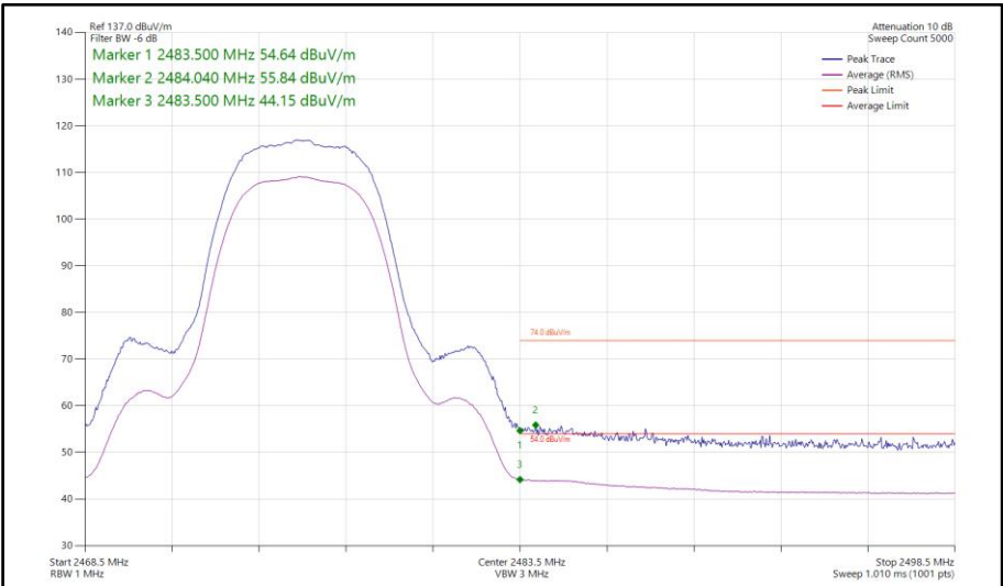
Figure 136 - Bluetooth HDR8, SISO, Core 1 - 2476 MHz Band Edge Frequency 2483.5 MHz
