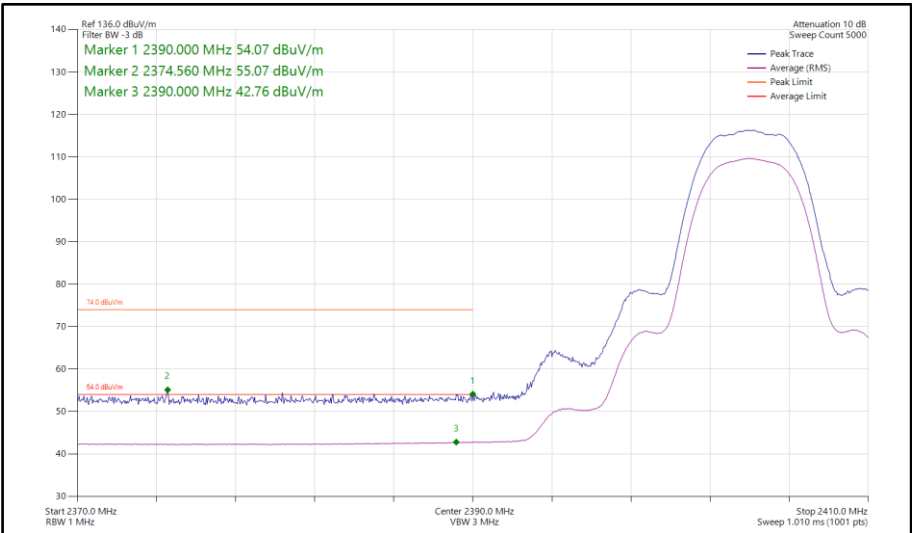
Figure 148 - Bluetooth HDR8, MIMO, Core 0-1 - 2404 MHz Band Edge Frequency 2390 MHz
