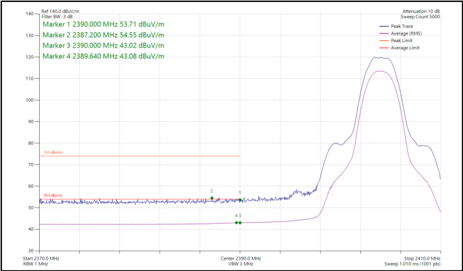
Figure 105 - Bluetooth HDT6, SISO, Core 0 - 2404 MHz Band Edge Frequency 2390 MHz
