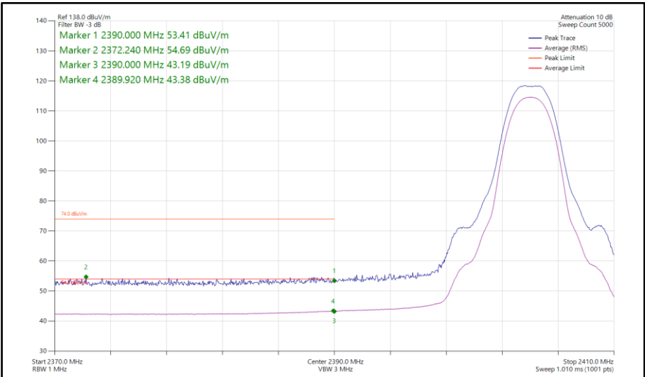
Figure 128 - Bluetooth HDT4, SISO, Core 1 - 2404 MHz Band Edge Frequency 2390 MHz
