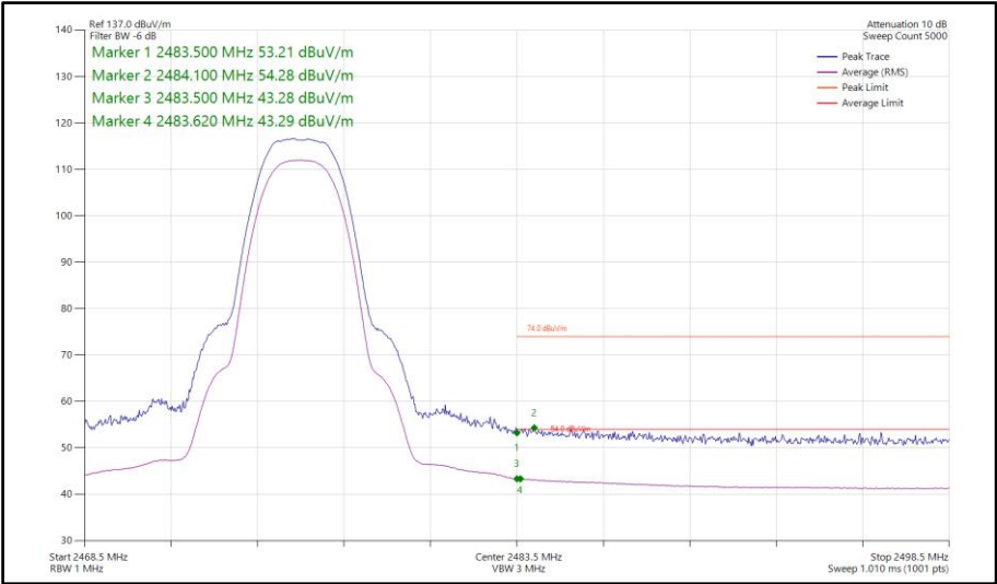
Figure 139 - Bluetooth HDT3, SISO, Core 1 - 2476 MHz Band Edge Frequency 2483.5 MHz
