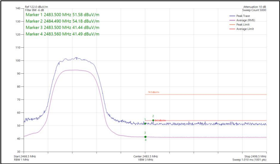
Figure 95 - Bluetooth HDRPM12, MIMO, Core 0-1 - 2475 MHz Band Edge Frequency 2483.5 MHz
