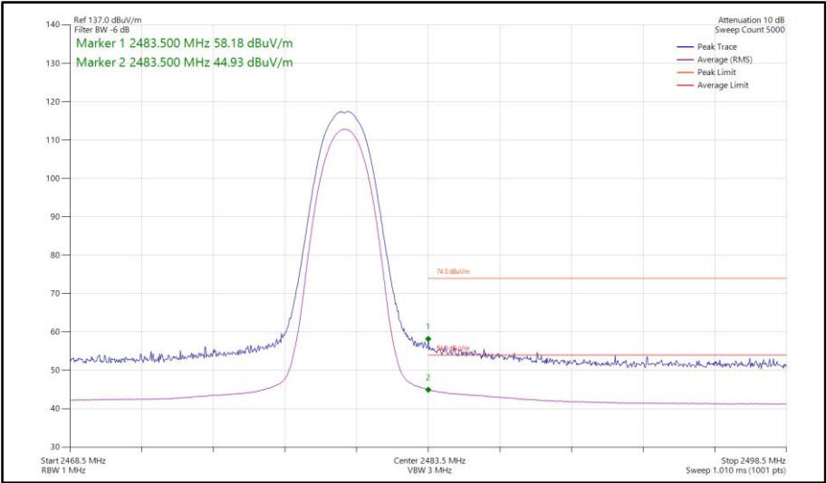
Figure 133 - Bluetooth 2DH5, SISO, Core 1 - 2480 MHz Band Edge Frequency 2483.5 MHz
