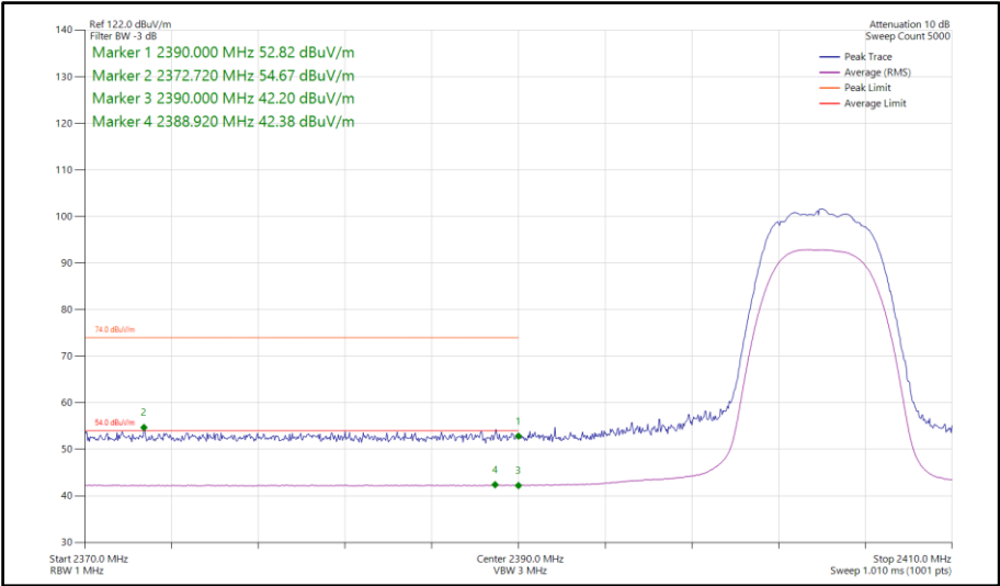
Figure 83 - Bluetooth HDRPM12, MIMO, Core 0-1 - 2404 MHz Band Edge Frequency 2390 MHz
