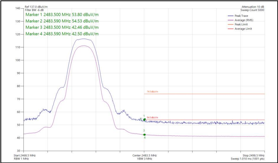
Figure 159 - Bluetooth HDR4, MIMO, Core 0-1 - 2476 MHz Band Edge Frequency 2483.5 MHz
