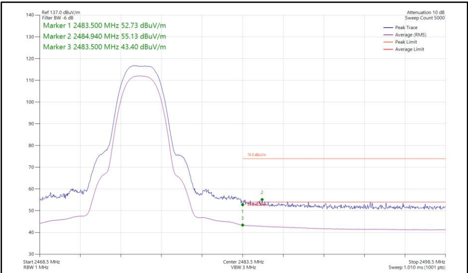
Figure 140 - Bluetooth HDT4, SISO, Core 1 - 2476 MHz Band Edge Frequency 2483.5 MHz
