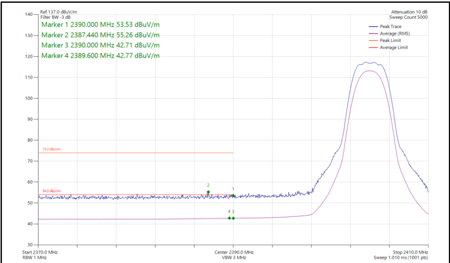
Figure 154 - Bluetooth HDRPS2, MIMO, Core 0-1 - 2404 MHz Band Edge Frequency 2390 MHz
