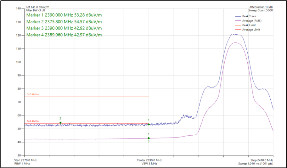
Figure 153 - Bluetooth HDT6, MIMO, Core 0-1 - 2404 MHz Band Edge Frequency 2390 MHz
