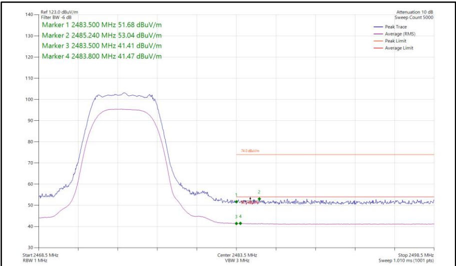
Figure 96 - Bluetooth XHDRPM8, MIMO, Core 0-1 - 2475 MHz Band Edge Frequency 2483.5 MHz
