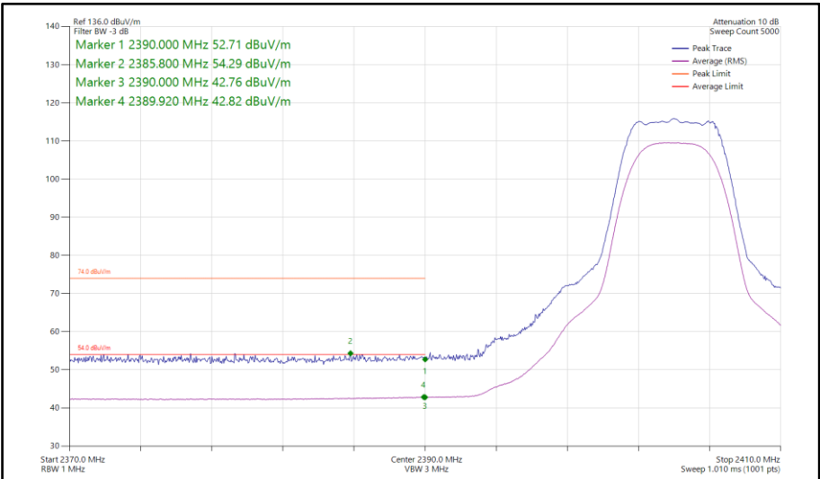
Figure 156 - Bluetooth XHDRPM8, MIMO, Core 0-1 - 2404 MHz Band Edge Frequency 2390 MHz
