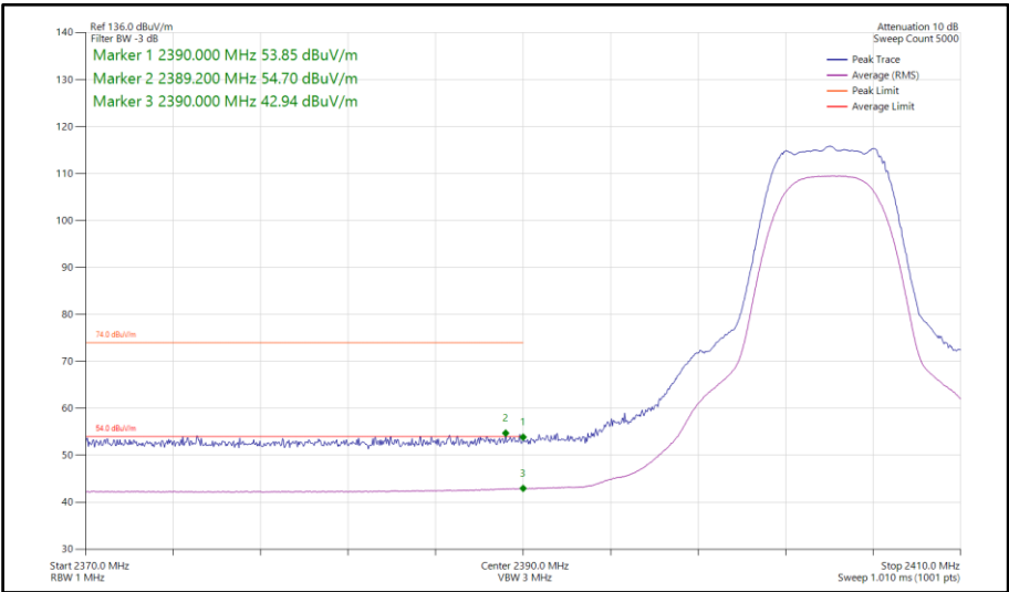
Figure 132 - Bluetooth XHDRPM8, SISO, Core 1 - 2404 MHz Band Edge Frequency 2390 MHz
