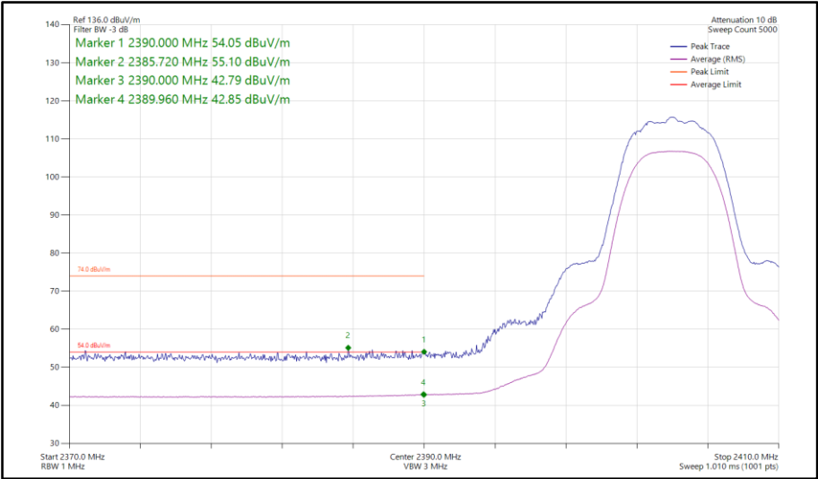
Figure 131 - Bluetooth HDRPM12, SISO, Core 1 - 2404 MHz Band Edge Frequency 2390 MHz
