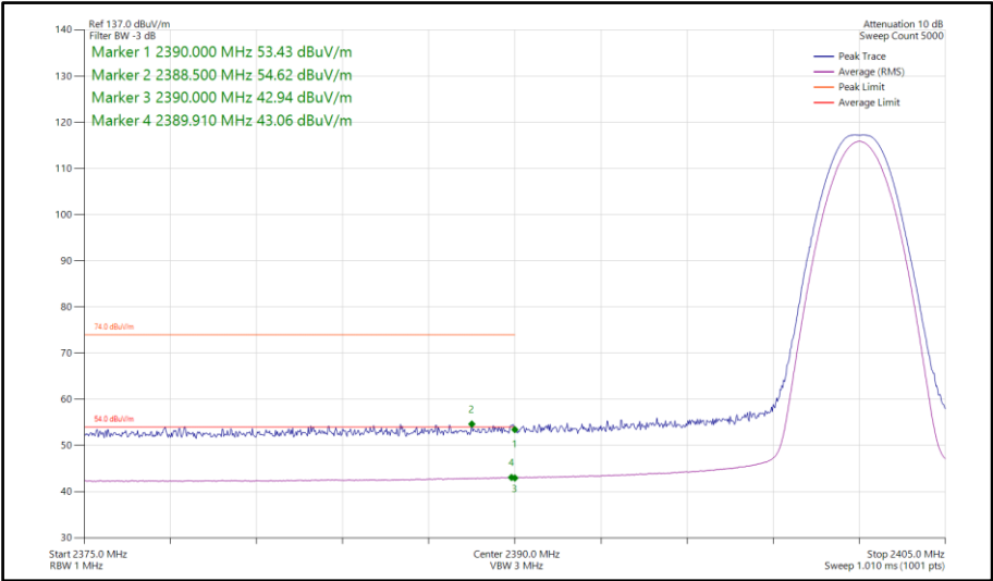
Figure 149 - Bluetooth LE1M, MIMO, Core 0-1 - 2402 MHz Band Edge Frequency 2390 MHz
