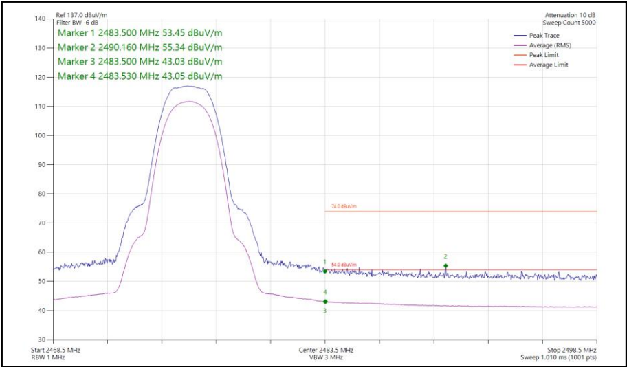
Figure 135 - Bluetooth HDR4, SISO, Core 1 - 2476 MHz Band Edge Frequency 2483.5 MHz
