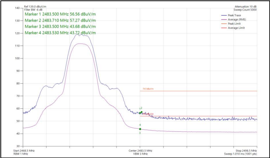
Figure 117 - Bluetooth HDT6, SISO, Core 0 - 2476 MHz Band Edge Frequency 2483.5 MHz
