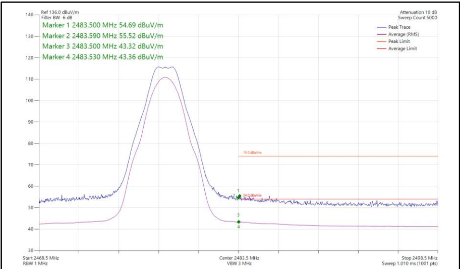
Figure 138 - Bluetooth LE2M, SISO, Core 1 - 2478 MHz Band Edge Frequency 2483.5 MHz
