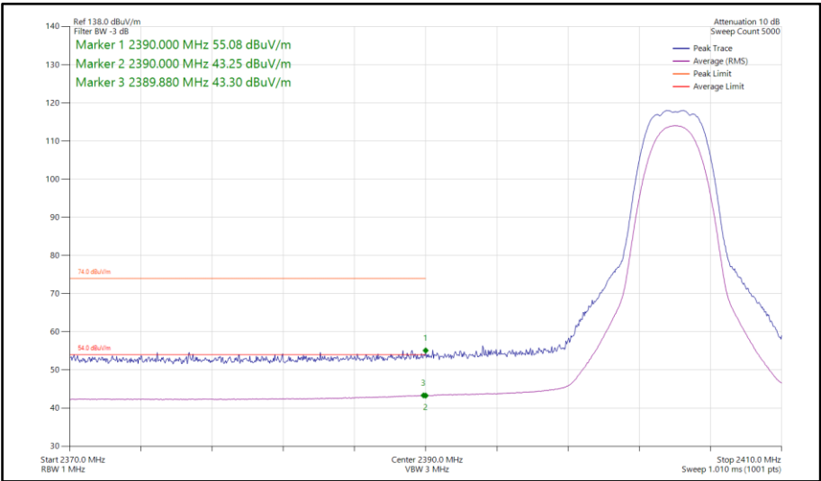
Figure 130 - Bluetooth HDRPS2, SISO, Core 1 - 2404 MHz Band Edge Frequency 2390 MHz
