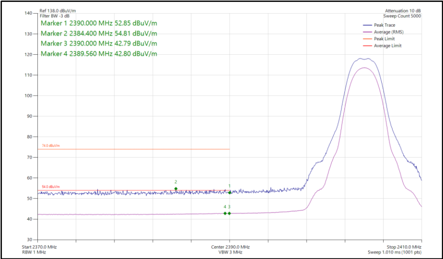
Figure 147 - Bluetooth HDR4, MIMO, Core 0-1 - 2404 MHz Band Edge Frequency 2390 MHz
