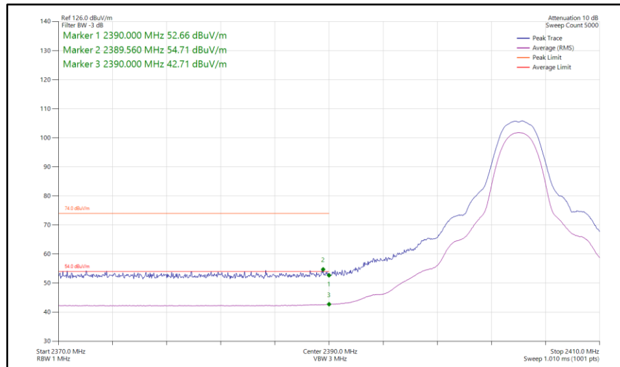
Figure 79 - Bluetooth HDT3, MIMO, Core 0-1 - 2404 MHz Band Edge Frequency 2390 MHz
