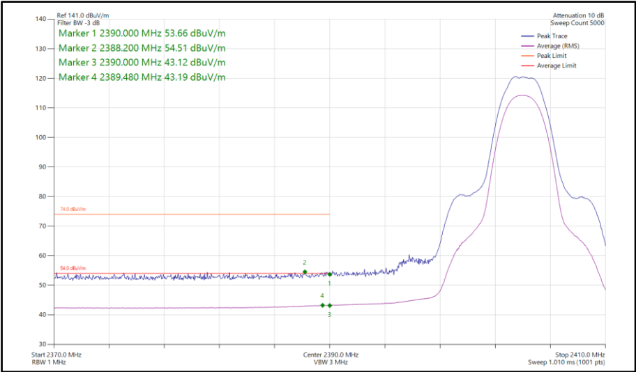
Figure 129 - Bluetooth HDT6, SISO, Core 1 - 2404 MHz Band Edge Frequency 2390 MHz
