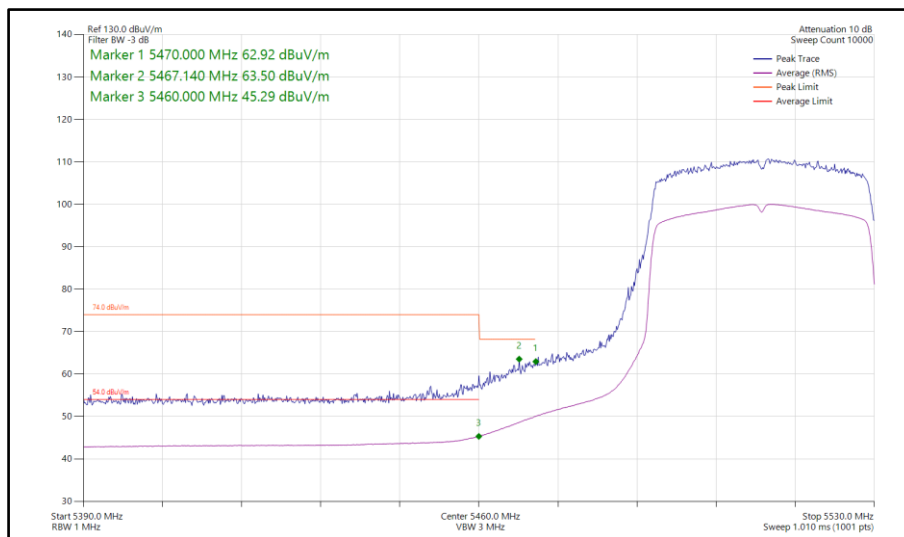
Figure 725 - 802.11ax HE40, SU, SISO, Core 1 - 5510 MHz Band Edge Frequency 5470 MHz
