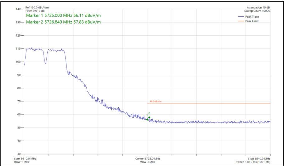
Figure 706 - 802.11a a40, SISO, Core 0 - 5630 MHz Band Edge Frequency 5725 MHz
