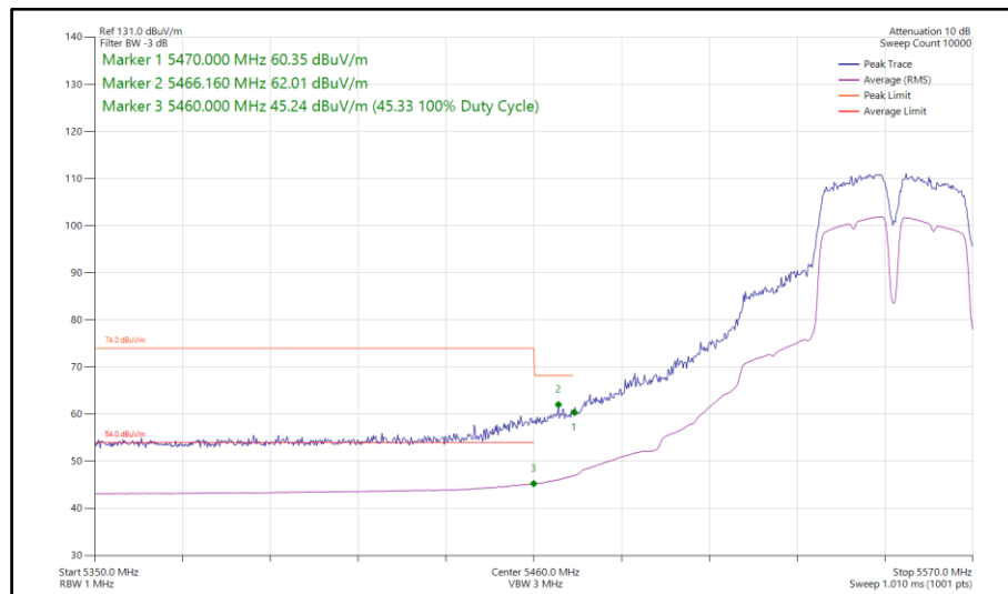
Figure 694 - 802.11a a40, SISO, Core 0 - 5550 MHz Band Edge Frequency 5470 MHz
