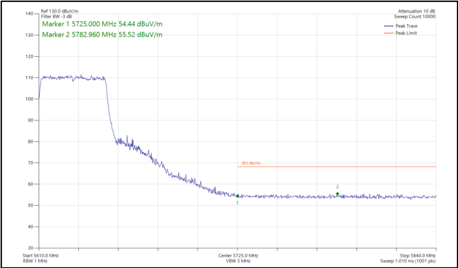
Figure 709 - 802.11ax HE40, SU, SISO, Core 0 - 5630 MHz Band Edge Frequency 5725 MHz
