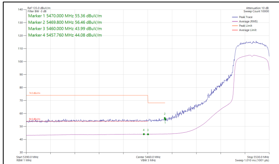
Figure 661 - 802.11ax HE20, SU, SDM, Core 0-1 - 5520 MHz Band Edge Frequency 5470 MHz
