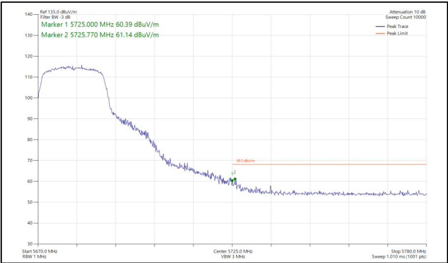
Figure 686 - 802.11ac VHT20, TxBF, Core 0-1 - 5680 MHz Band Edge Frequency 5725 MHz
