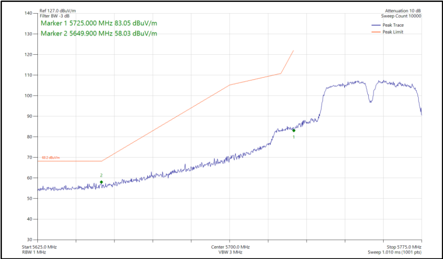
Figure 701 - 802.11a a40, SISO, Core 0 - 5755 MHz Band Edge Frequency 5725 MHz
