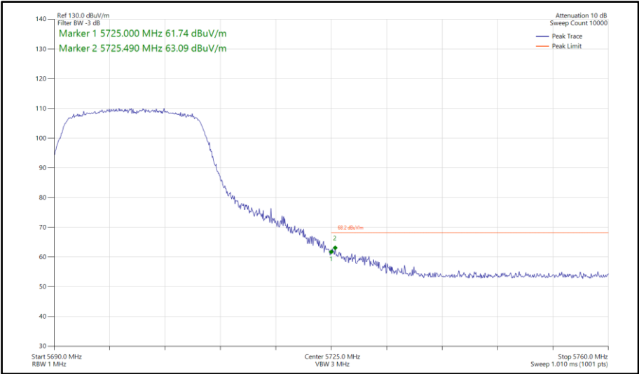
Figure 687 - 802.11ac VHT20, TxBF, Core 0-1 - 5700 MHz Band Edge Frequency 5725 MHz
