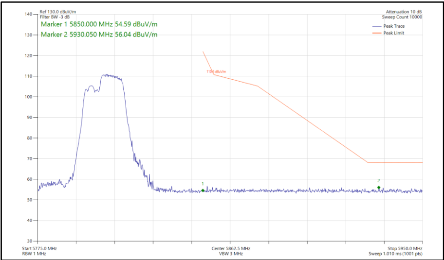
Figure 722 - 802.11be EHT40, RU 106+26-85, SISO, Core 0 - 5795 MHz Band Edge Frequency 5850 MHz
