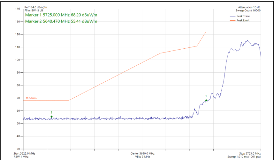
Figure 666 - 802.11be EHT20, RU 106+26-83, SDM, Core 0-1 - 5745 MHz Band Edge Frequency 5725 MHz
