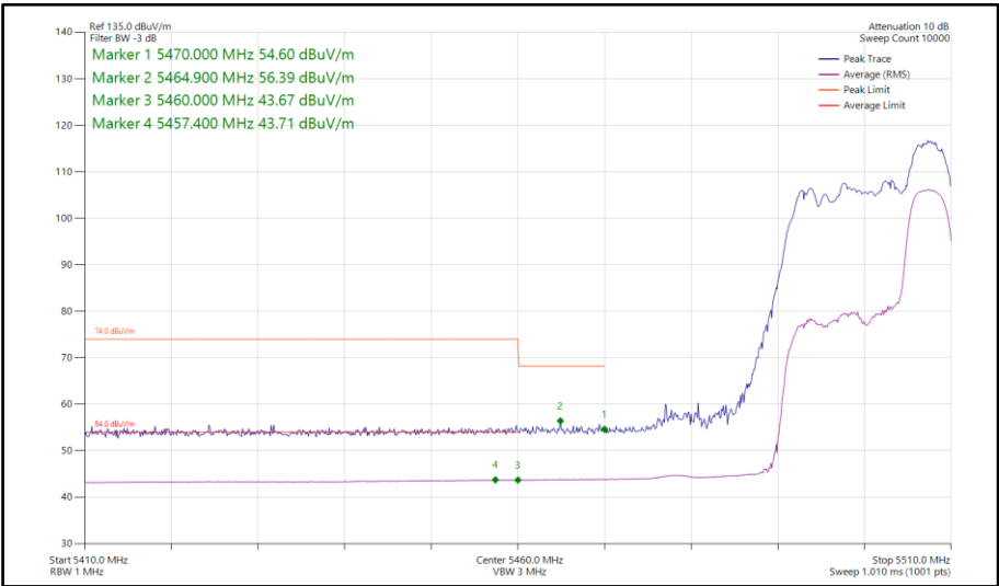
Figure 660 - 802.11ax HE20, RU 52-40, SDM, Core 0-1 - 5500 MHz Band Edge Frequency 5470 MHz
