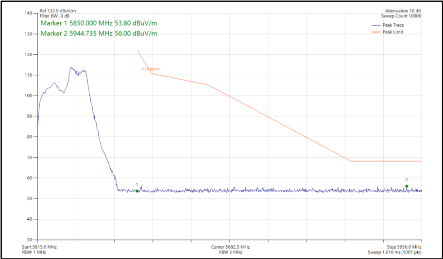
Figure 656 - 802.11be EHT20, RU 52+26-72, CDD, Core 0-1 - 5825 MHz Band Edge Frequency 5850 MHz
