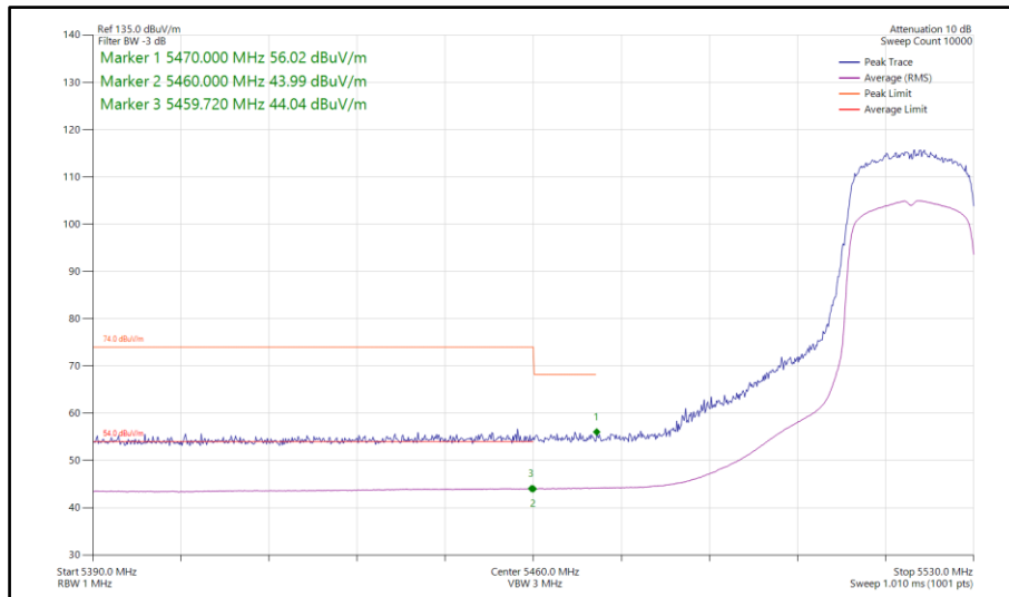
Figure 683 - 802.11ax HE20, SU, TxBF, Core 0-1 - 5520 MHz Band Edge Frequency 5470 MHz
