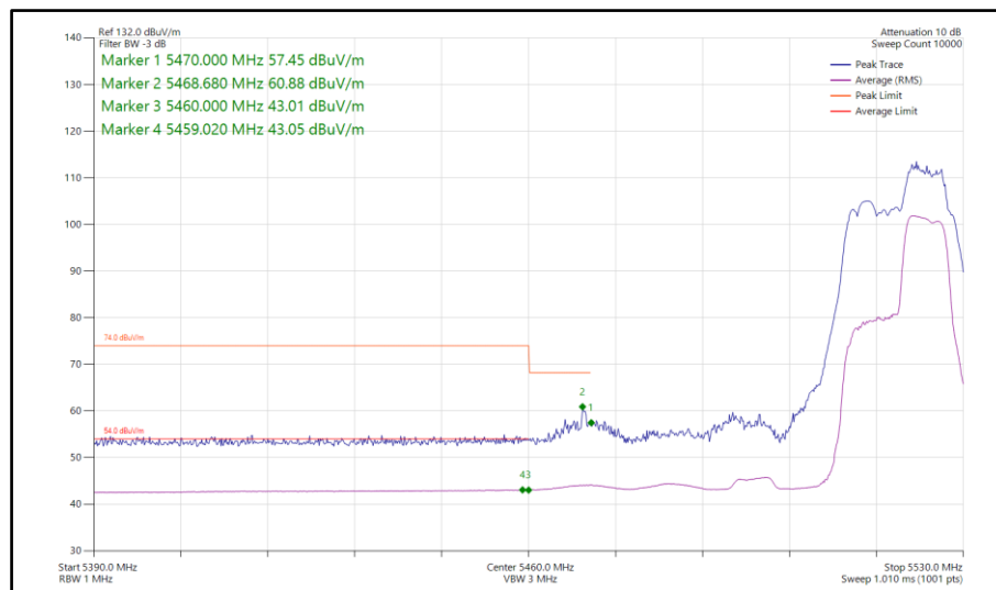
Figure 727 - 802.11be EHT40, RU 52+26-75, SISO, Core 1 - 5510 MHz Band Edge Frequency 5470 MHz
