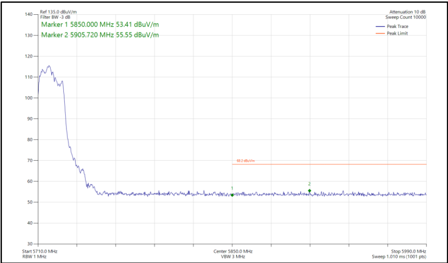
Figure 678 - 802.11be EHT20, RU 106+26-82, SDM, Core 0-1 - 5720 MHz Band Edge Frequency 5850 MHz
