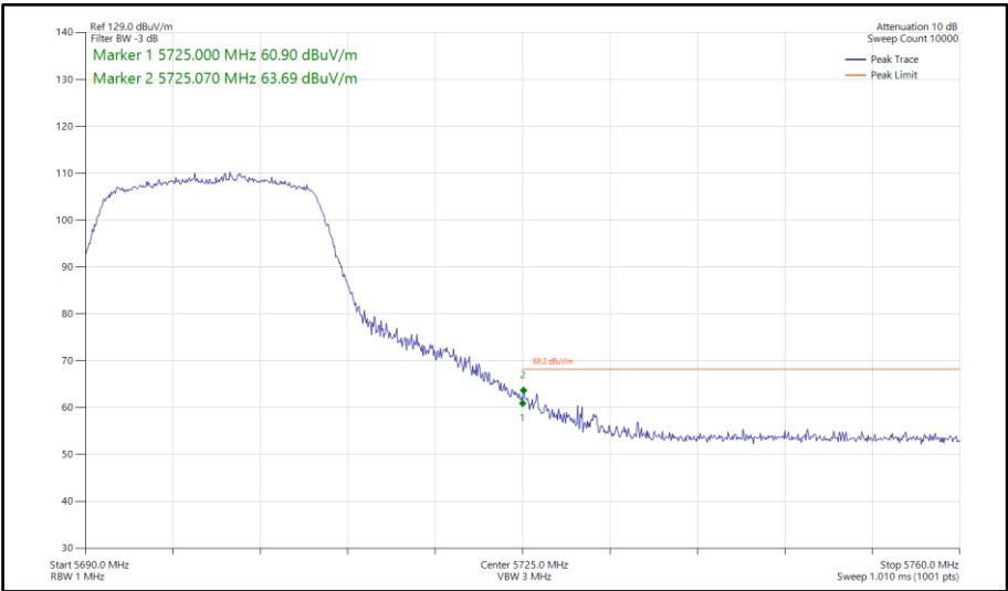
Figure 668 - 802.11n HT20, SDM, Core 0-1 - 5700 MHz Band Edge Frequency 5725 MHz
