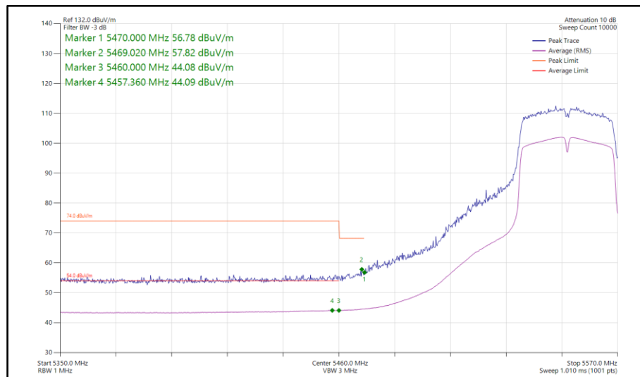
Figure 696 - 802.11n HT40, SISO, Core 0 - 5550 MHz Band Edge Frequency 5470 MHz
