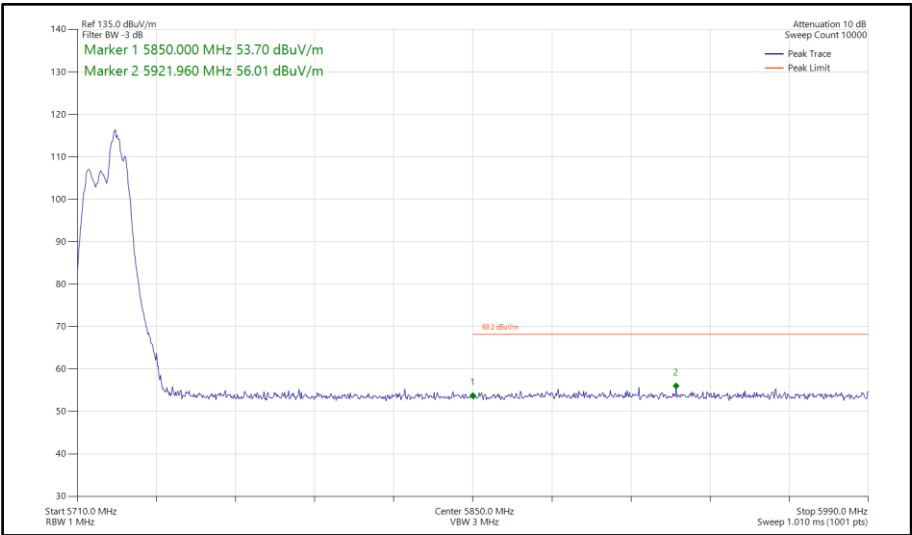
Figure 655 - 802.11be EHT20, RU 52+26-72, CDD, Core 0-1 - 5720 MHz Band Edge Frequency 5850 MHz
