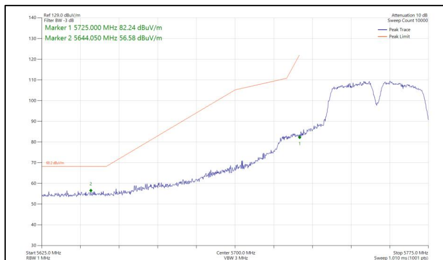
Figure 728 - 802.11a a40, SISO, Core 1 - 5755 MHz Band Edge Frequency 5725 MHz
