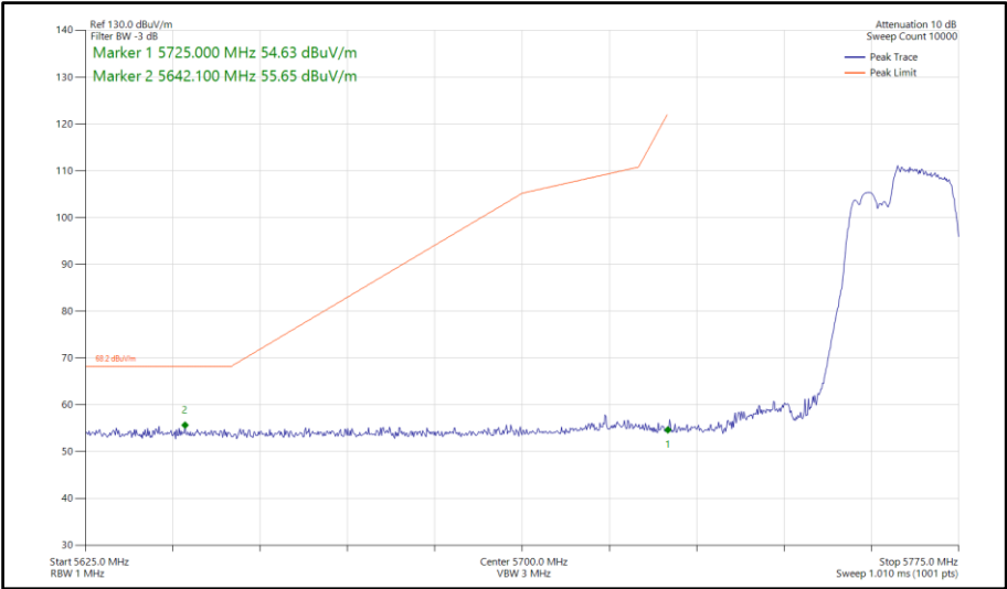
Figure 705 - 802.11be EHT40, RU 106+26-85, SISO, Core 0 - 5755 MHz Band Edge Frequency 5725 MHz
