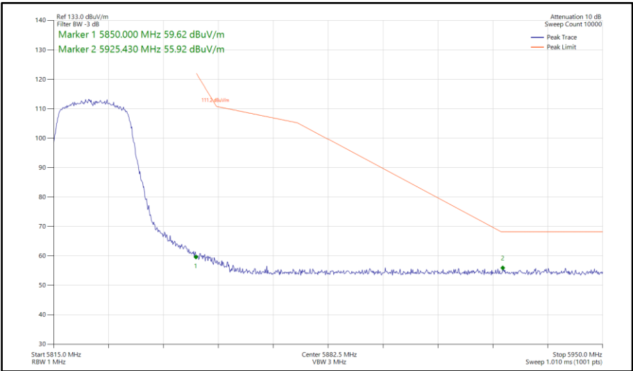
Figure 690 - 802.11ac VHT20, TxBF, Core 0-1 - 5825 MHz Band Edge Frequency 5850 MHz
