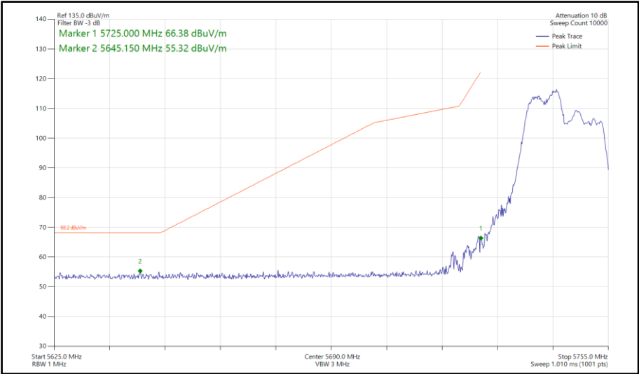
Figure 665 - 802.11ax HE20, RU 106-53, SDM, Core 0-1 - 5745 MHz Band Edge Frequency 5725 MHz
