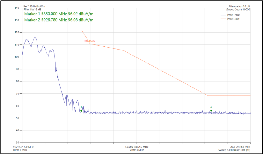
Figure 654 - 802.11ax HE20, RU 106-53, CDD, Core 0-1 - 5825 MHz Band Edge Frequency 5850 MHz
