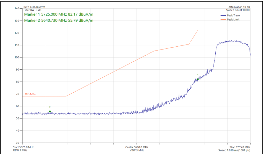
Figure 664 - 802.11ax HE20, SU, SDM, Core 0-1 - 5745 MHz Band Edge Frequency 5725 MHz
