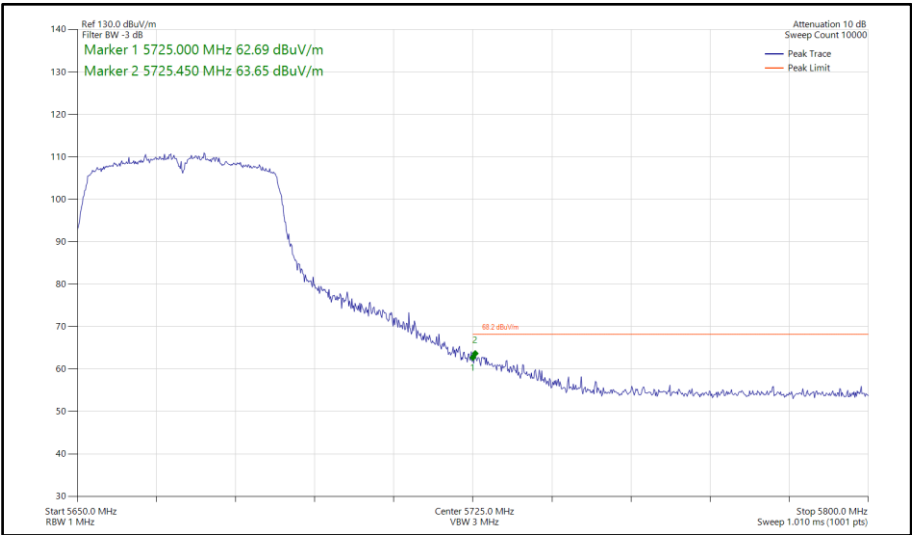
Figure 708 - 802.11n HT40, SISO, Core 0 - 5670 MHz Band Edge Frequency 5725 MHz
