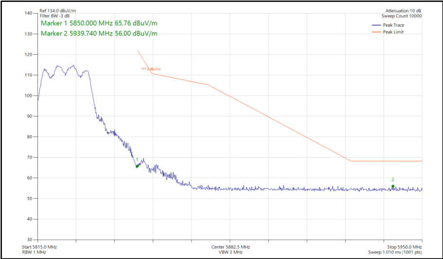
Figure 648 - 802.11a, CDD, Core 0-1 - 5825 MHz Band Edge Frequency 5850 MHz
