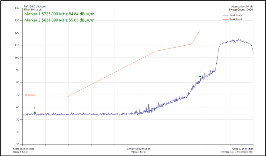
Figure 685 - 802.11ax HE20, SU, TxBF, Core 0-1 - 5745 MHz Band Edge Frequency 5725 MHz
