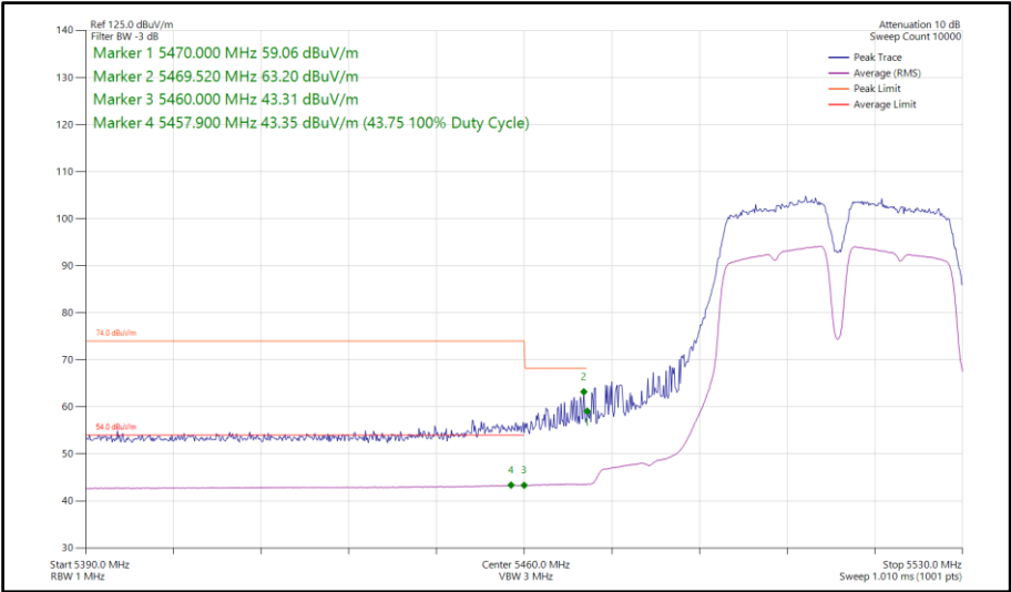
Figure 723 - 802.11a a40, SISO, Core 1 - 5510 MHz Band Edge Frequency 5470 MHz
