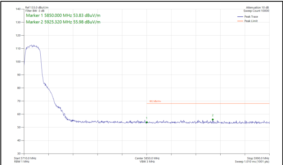
Figure 672 - 802.11n HT20, SDM, Core 0-1 - 5720 MHz Band Edge Frequency 5850 MHz
