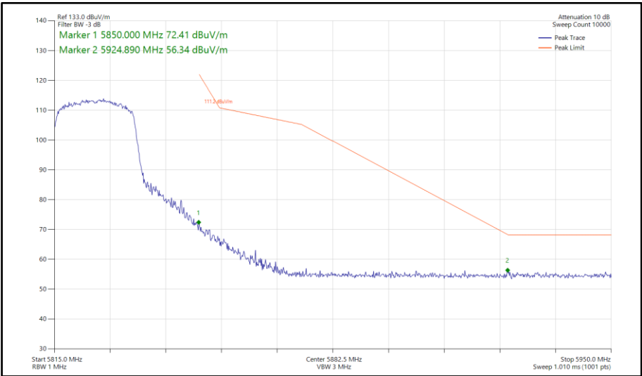
Figure 676 - 802.11ax HE20, SU, SDM, Core 0-1 - 5825 MHz Band Edge Frequency 5850 MHz
