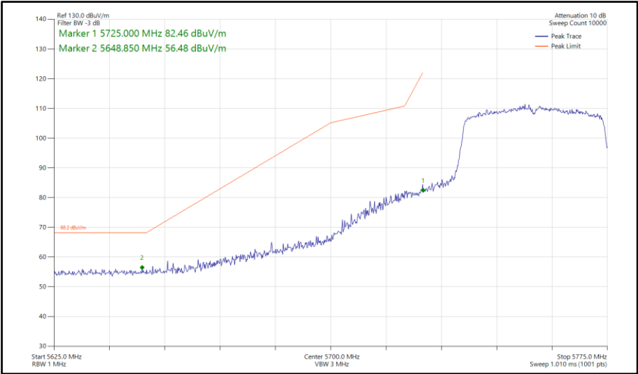
Figure 703 - 802.11ax HE40, SU, SISO, Core 0 - 5755 MHz Band Edge Frequency 5725 MHz
