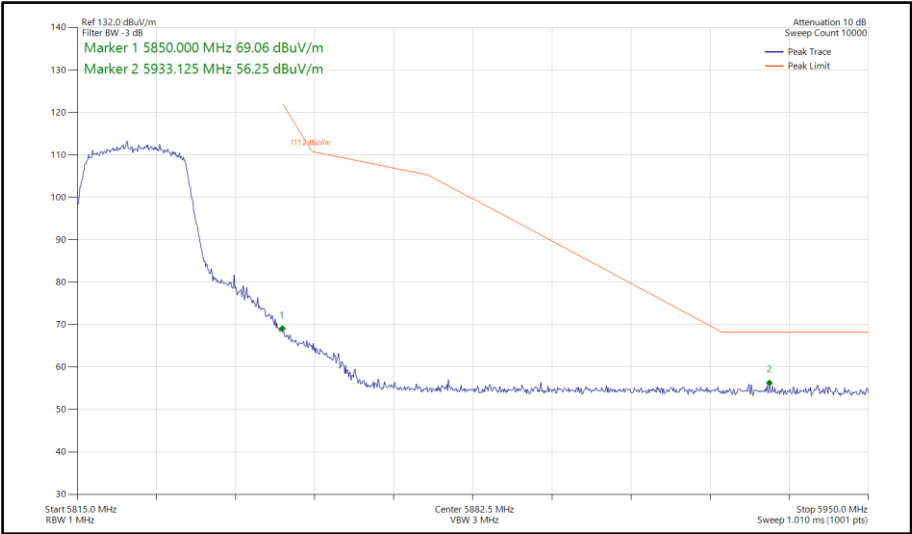
Figure 673 - 802.11n HT20, SDM, Core 0-1 - 5825 MHz Band Edge Frequency 5850 MHz
