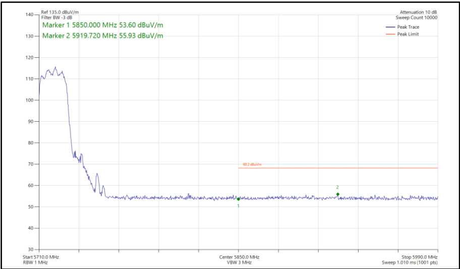
Figure 651 - 802.11ax HE20, SU, CDD, Core 0-1 - 5720 MHz Band Edge Frequency 5850 MHz
