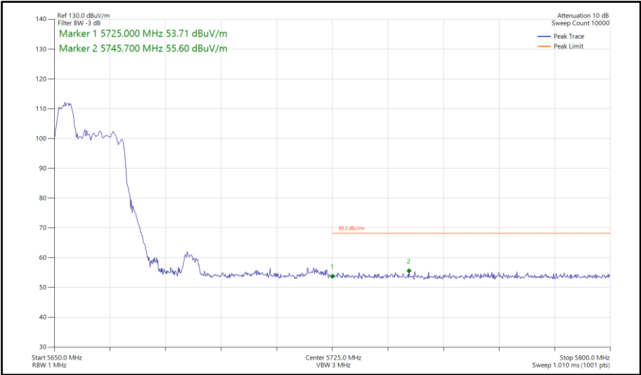
Figure 711 - 802.11ax HE40, RU 52-37, SISO, Core 0 - 5670 MHz Band Edge Frequency 5725 MHz
