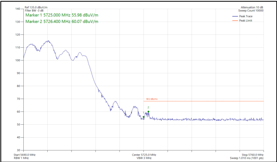
Figure 670 - 802.11ax HE20, RU 106-53, SDM, Core 0-1 - 5700 MHz Band Edge Frequency 5725 MHz
