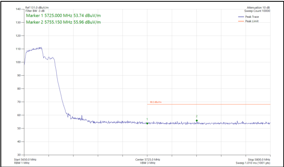
Figure 712 - 802.11be EHT40, RU 106+26-82, SISO, Core 0 - 5670 MHz Band Edge Frequency 5725 MHz
