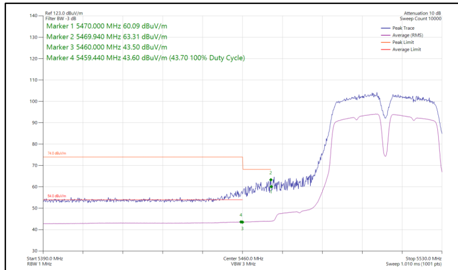
Figure 693 - 802.11a a40, SISO, Core 0 - 5510 MHz Band Edge Frequency 5470 MHz
