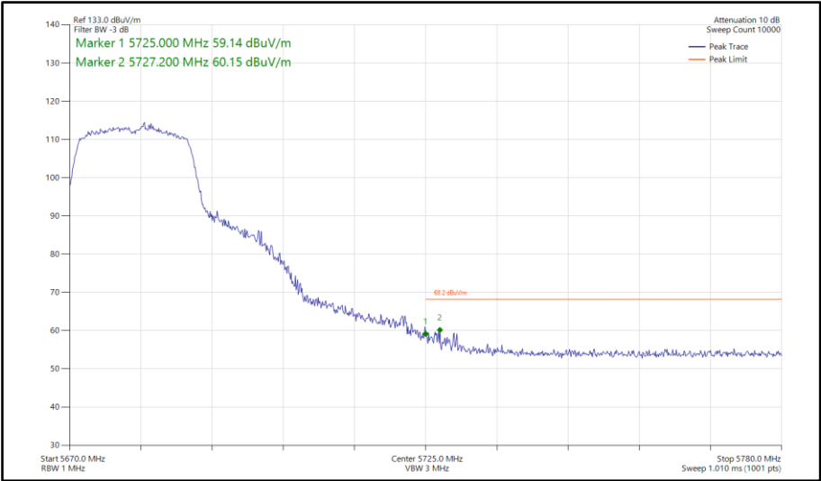
Figure 667 - 802.11n HT20, SDM, Core 0-1 - 5680 MHz Band Edge Frequency 5725 MHz
