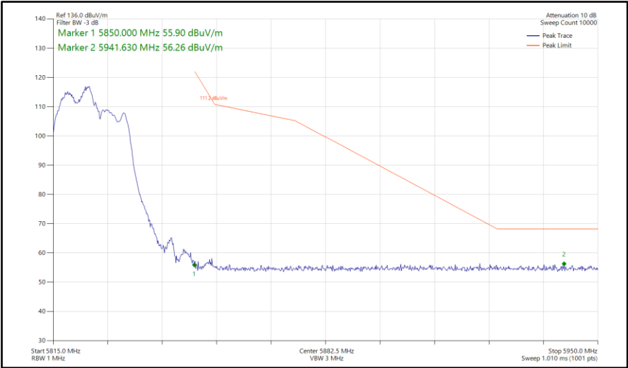
Figure 679 - 802.11be EHT20, RU 106+26-82, SDM, Core 0-1 - 5825 MHz Band Edge Frequency 5850 MHz
