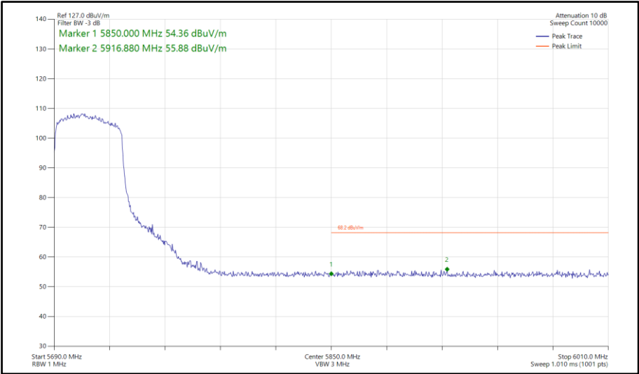
Figure 717 - 802.11ax HE40, SU, SISO, Core 0 - 5710 MHz Band Edge Frequency 5850 MHz
