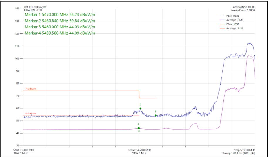
Figure 698 - 802.11ax HE40, RU 52-44, SISO, Core 0 - 5510 MHz Band Edge Frequency 5470 MHz
