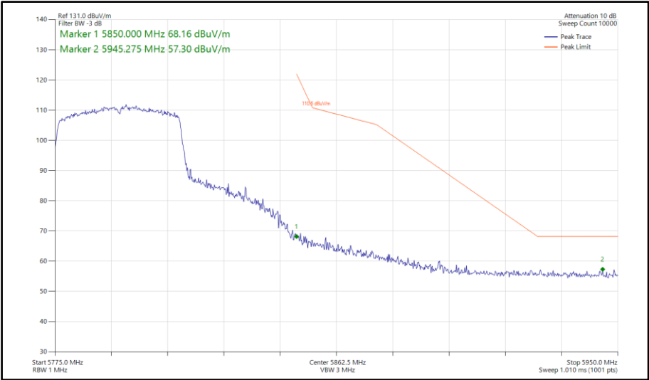
Figure 719 - 802.11ax HE40, SU, SISO, Core 0 - 5795 MHz Band Edge Frequency 5850 MHz
