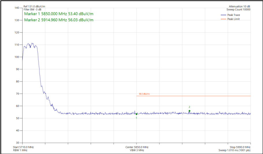
Figure 649 - 802.11n HT20, CDD, Core 0-1 - 5720 MHz Band Edge Frequency 5850 MHz
