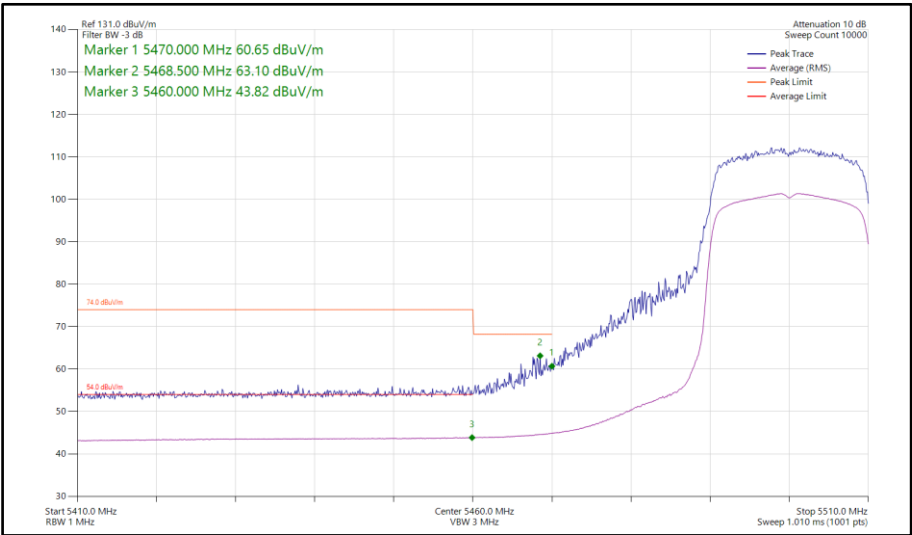
Figure 682 - 802.11ax HE20, SU, TxBF, Core 0-1 - 5500 MHz Band Edge Frequency 5470 MHz
