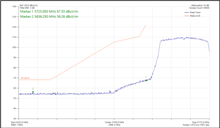
Figure 730 - 802.11ax HE40, SU, SISO, Core 1 - 5755 MHz Band Edge Frequency 5725 MHz
