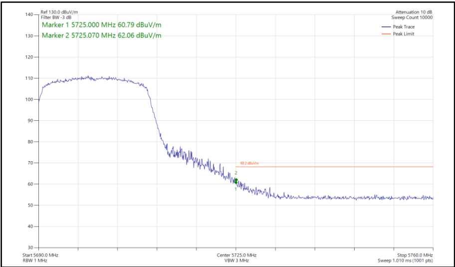
Figure 688 - 802.11ax HE20, SU, TxBF, Core 0-1 - 5700 MHz Band Edge Frequency 5725 MHz
