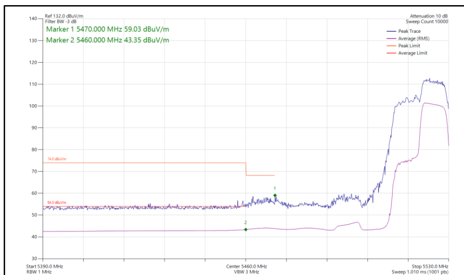
Figure 726 - 802.11ax HE40, RU 106-56, SISO, Core 1 - 5510 MHz Band Edge Frequency 5470 MHz
