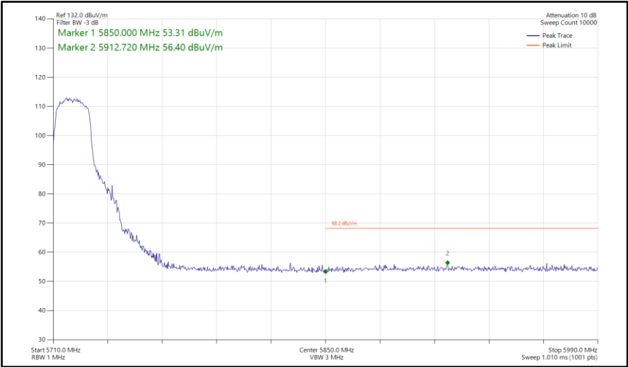
Figure 689 - 802.11ac VHT20, TxBF, Core 0-1 - 5720 MHz Band Edge Frequency 5850 MHz
