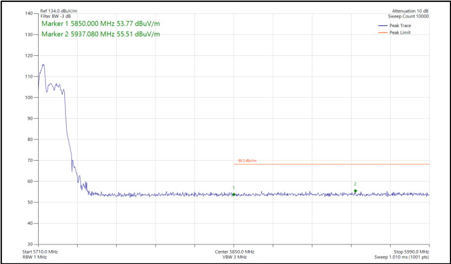
Figure 675 - 802.11ax HE20, RU 52-37, SDM, Core 0-1 - 5720 MHz Band Edge Frequency 5850 MHz
