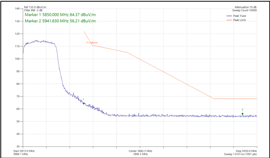
Figure 692 - 802.11ax HE20, SU, TxBF, Core 0-1 - 5825 MHz Band Edge Frequency 5850 MHz
