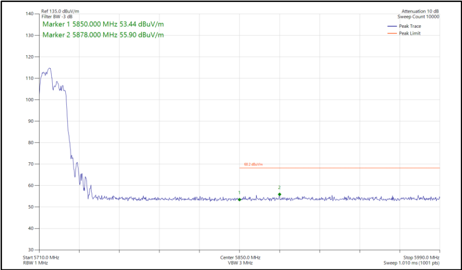
Figure 652 - 802.11ax HE20, RU 106-53, CDD, Core 0-1 - 5720 MHz Band Edge Frequency 5850 MHz
