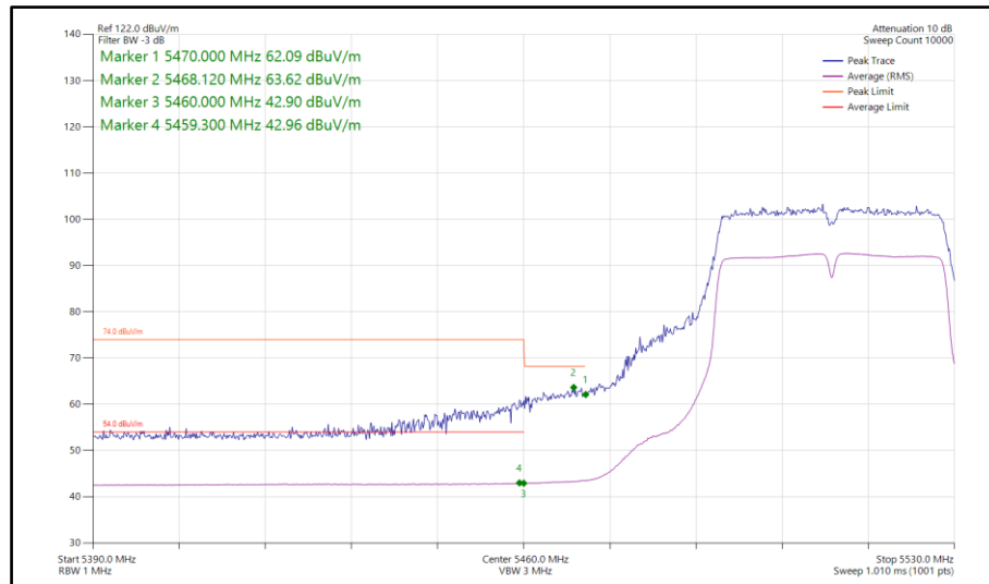
Figure 695 - 802.11n HT40, SISO, Core 0 - 5510 MHz Band Edge Frequency 5470 MHz
