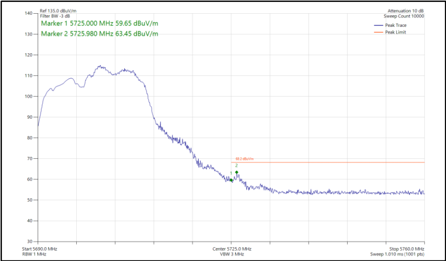
Figure 671 - 802.11be EHT20, RU 106+26-83, SDM, Core 0-1 - 5700 MHz Band Edge Frequency 5725 MHz
