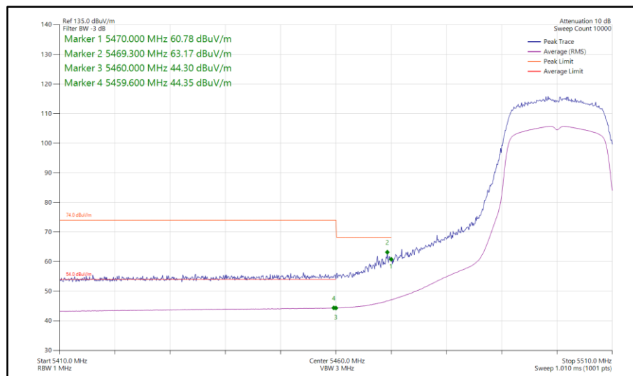
Figure 680 - 802.11ac VHT20, TxBF, Core 0-1 - 5500 MHz Band Edge Frequency 5470 MHz
