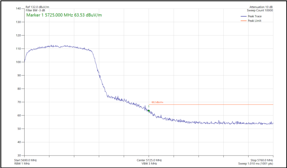
Figure 669 - 802.11ax HE20, SU, SDM, Core 0-1 - 5700 MHz Band Edge Frequency 5725 MHz
