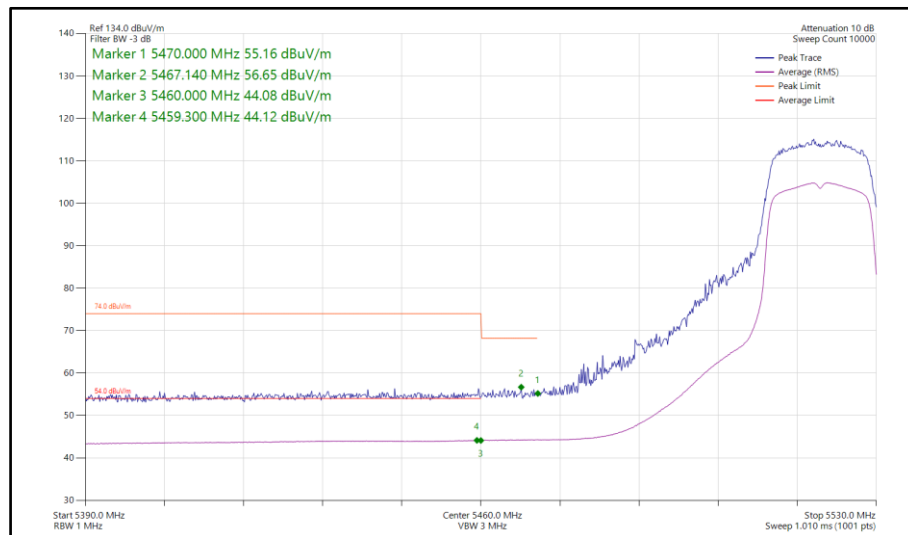
Figure 658 - 802.11n HT20, SDM, Core 0-1 - 5520 MHz Band Edge Frequency 5470 MHz
