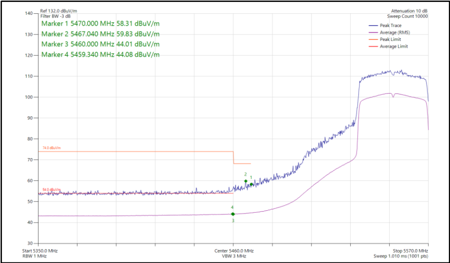
Figure 699 - 802.11ax HE40, SU, SISO, Core 0 - 5550 MHz Band Edge Frequency 5470 MHz
