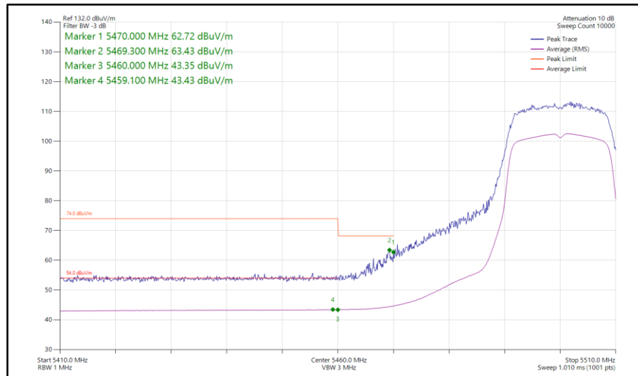
Figure 657 - 802.11n HT20, SDM, Core 0-1 - 5500 MHz Band Edge Frequency 5470 MHz
