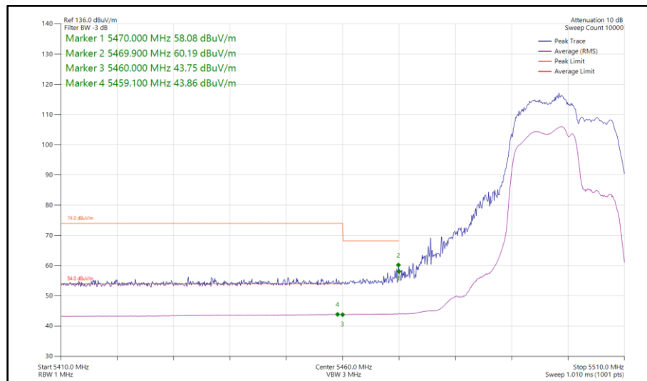
Figure 662 - 802.11be EHT20, RU 106+26-82, SDM, Core 0-1 - 5500 MHz Band Edge Frequency 5470 MHz
