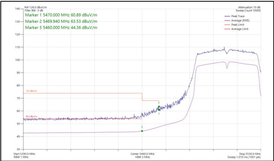
Figure 724 - 802.11n HT40, SISO, Core 1 - 5510 MHz Band Edge Frequency 5470 MHz
