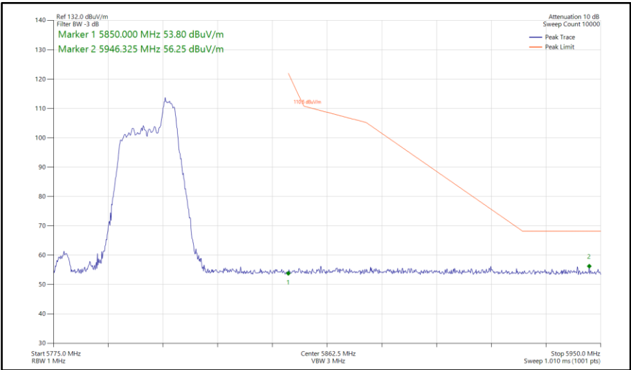
Figure 720 - 802.11ax HE40, RU 52-44, SISO, Core 0 - 5795 MHz Band Edge Frequency 5850 MHz
