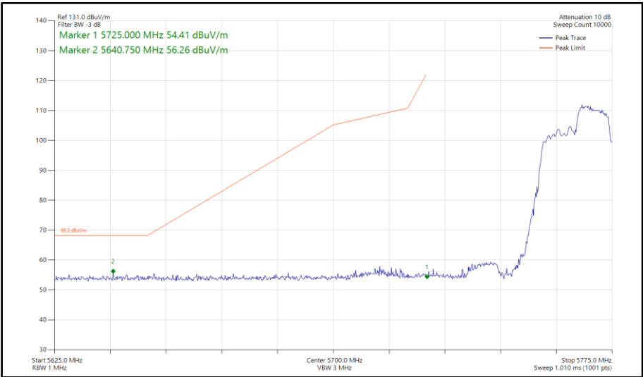
Figure 704 - 802.11ax HE40, RU 106-56, SISO, Core 0 - 5755 MHz Band Edge Frequency 5725 MHz
