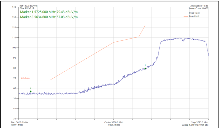
Figure 702 - 802.11n HT40, SISO, Core 0 - 5755 MHz Band Edge Frequency 5725 MHz
