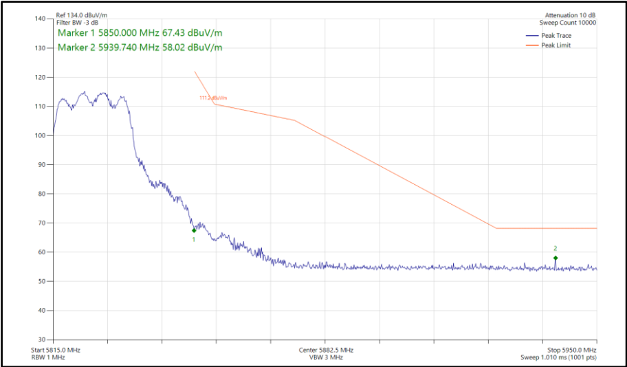
Figure 650 - 802.11n HT20, CDD, Core 0-1 - 5825 MHz Band Edge Frequency 5850 MHz
