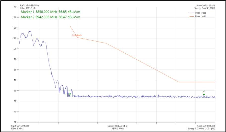
Figure 677 - 802.11ax HE20, RU 106-53, SDM, Core 0-1 - 5825 MHz Band Edge Frequency 5850 MHz
