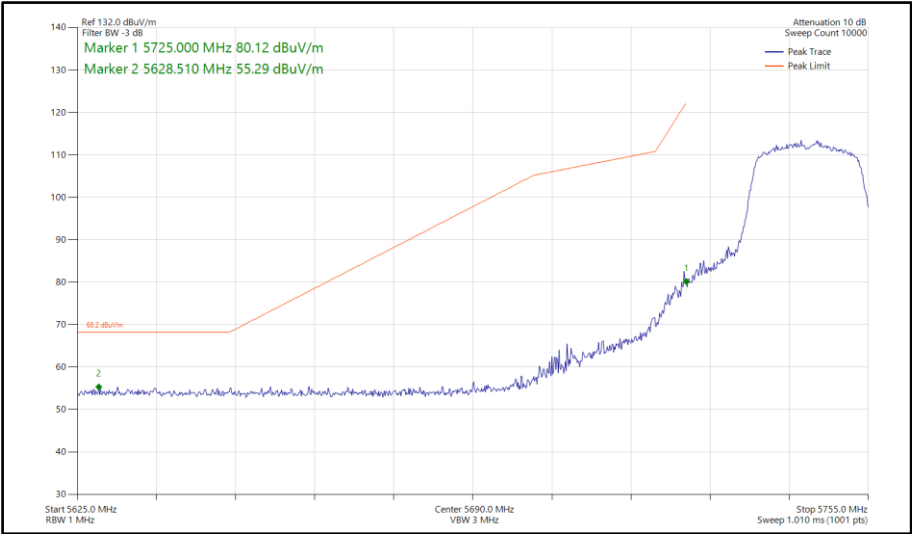
Figure 663 - 802.11n HT20, SDM, Core 0-1 - 5745 MHz Band Edge Frequency 5725 MHz
