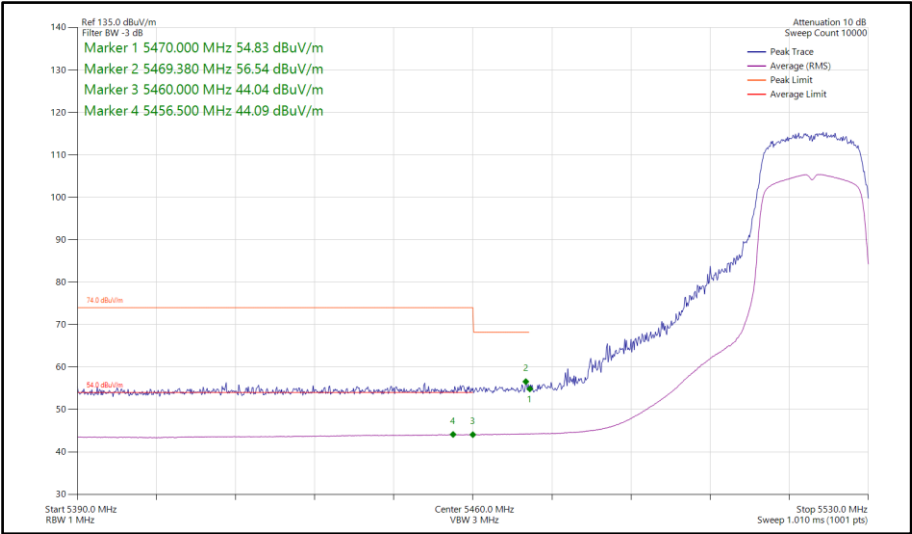
Figure 681 - 802.11ac VHT20, TxBF, Core 0-1 - 5520 MHz Band Edge Frequency 5470 MHz
