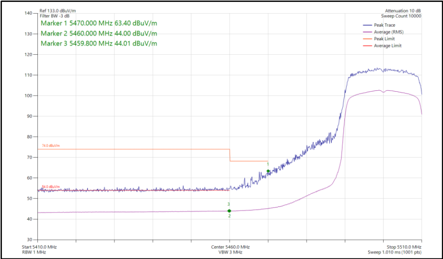
Figure 659 - 802.11ax HE20, SU, SDM, Core 0-1 - 5500 MHz Band Edge Frequency 5470 MHz
