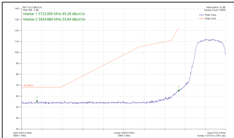
Figure 684 - 802.11ac VHT20, TxBF, Core 0-1 - 5745 MHz Band Edge Frequency 5725 MHz
