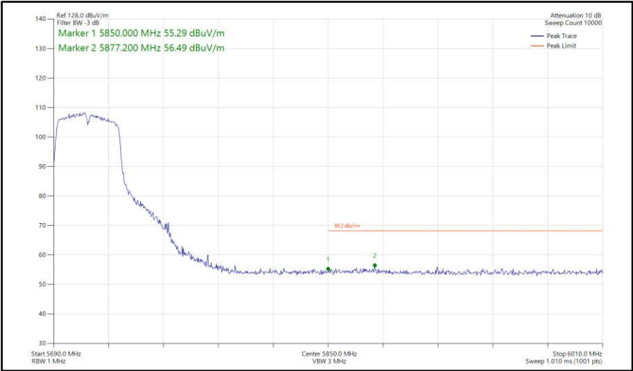
Figure 715 - 802.11n HT40, SISO, Core 0 - 5710 MHz Band Edge Frequency 5850 MHz
