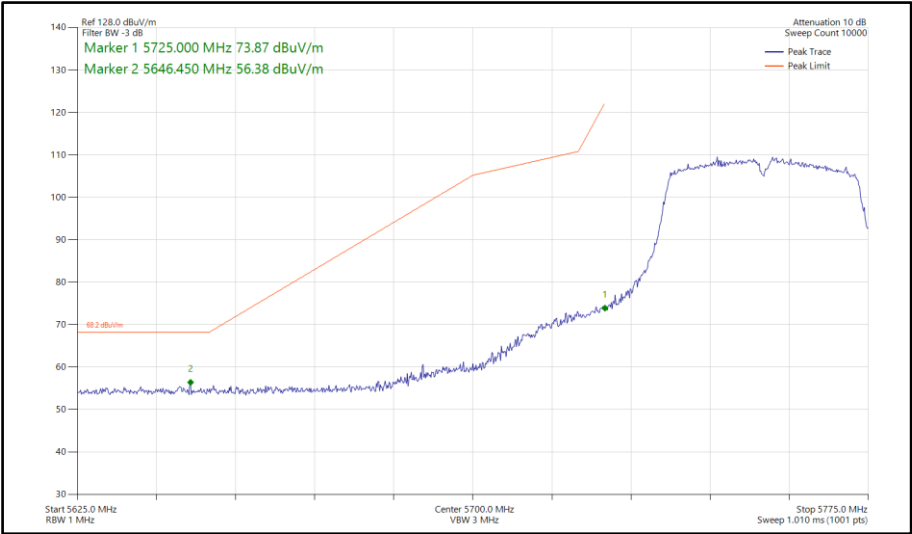
Figure 729 - 802.11n HT40, SISO, Core 1 - 5755 MHz Band Edge Frequency 5725 MHz
