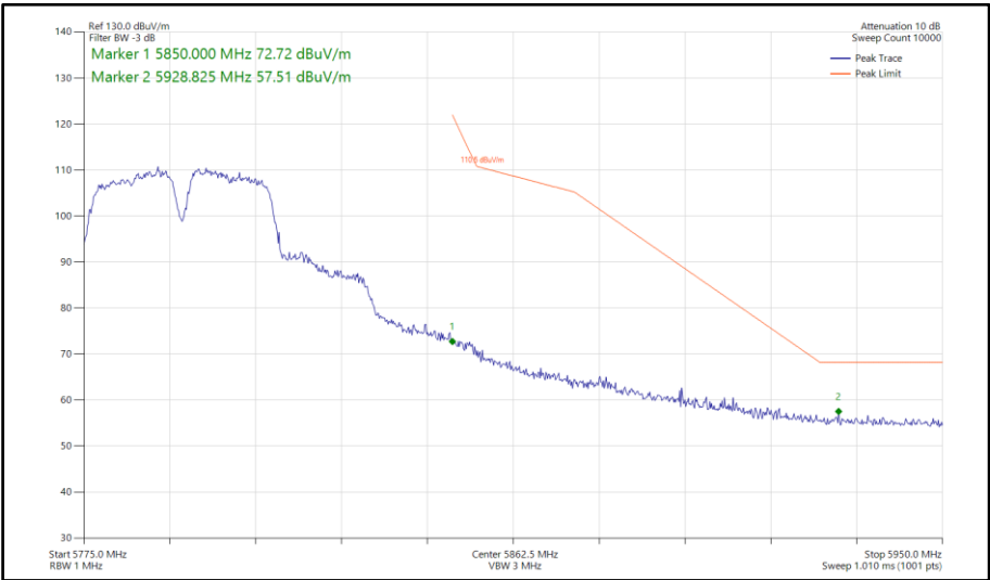
Figure 714 - 802.11a a40, SISO, Core 0 - 5795 MHz Band Edge Frequency 5850 MHz
