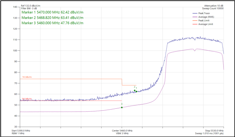
Figure 697 - 802.11ax HE40, SU, SISO, Core 0 - 5510 MHz Band Edge Frequency 5470 MHz
