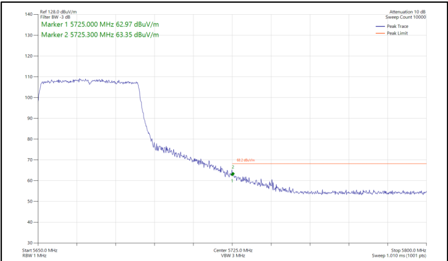
Figure 710 - 802.11ax HE40, SU, SISO, Core 0 - 5670 MHz Band Edge Frequency 5725 MHz
