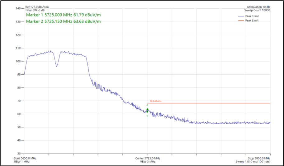
Figure 707 - 802.11a a40, SISO, Core 0 - 5670 MHz Band Edge Frequency 5725 MHz
