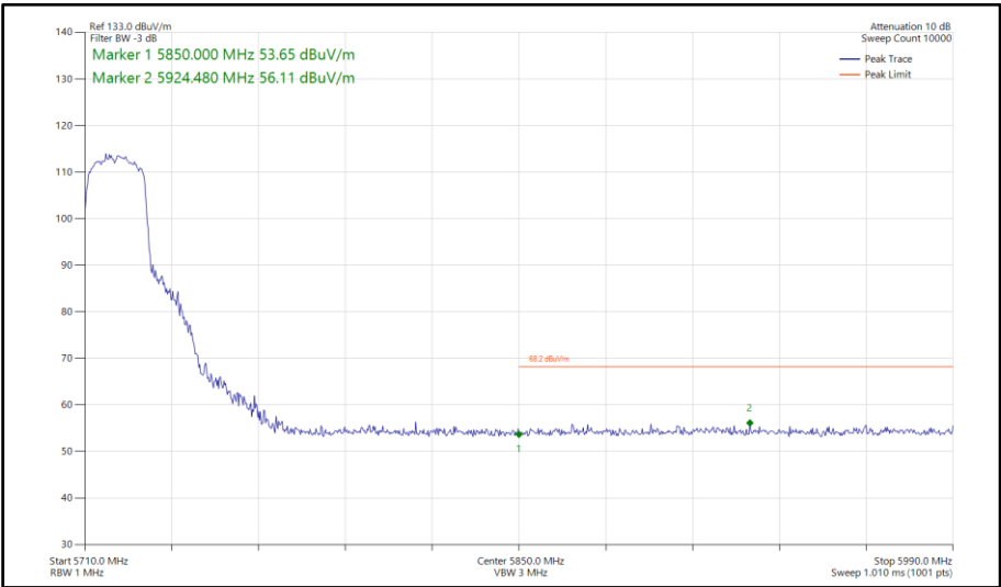
Figure 674 - 802.11ax HE20, SU, SDM, Core 0-1 - 5720 MHz Band Edge Frequency 5850 MHz
