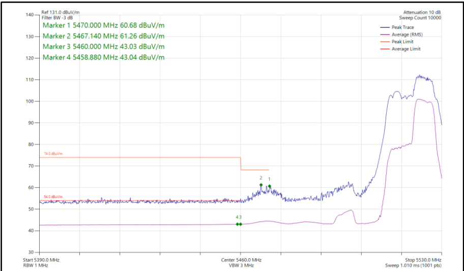
Figure 700 - 802.11be EHT40, RU 52+26-75, SISO, Core 0 - 5510 MHz Band Edge Frequency 5470 MHz
