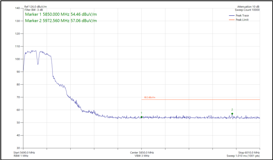
Figure 713 - 802.11a a40, SISO, Core 0 - 5710 MHz Band Edge Frequency 5850 MHz
