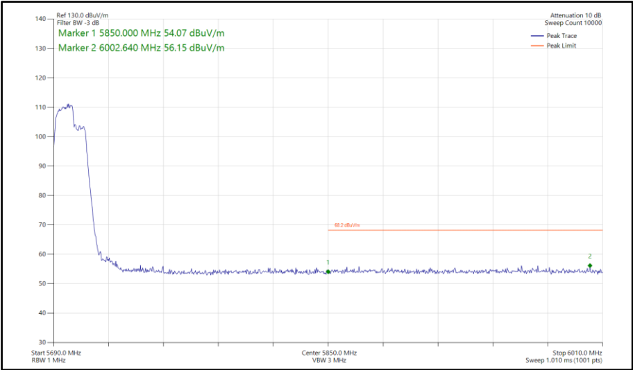
Figure 721 - 802.11be EHT40, RU 106+26-82, SISO, Core 0 - 5710 MHz Band Edge Frequency 5850 MHz
