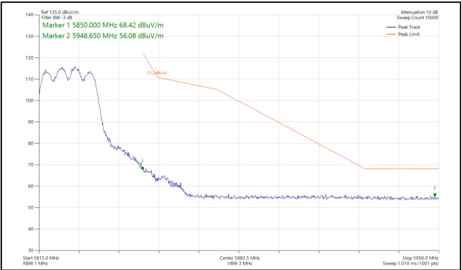
Figure 653 - 802.11ax HE20, SU, CDD, Core 0-1 - 5825 MHz Band Edge Frequency 5850 MHz
