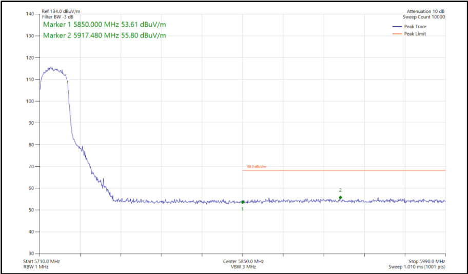
Figure 691 - 802.11ax HE20, SU, TxBF, Core 0-1 - 5720 MHz Band Edge Frequency 5850 MHz
