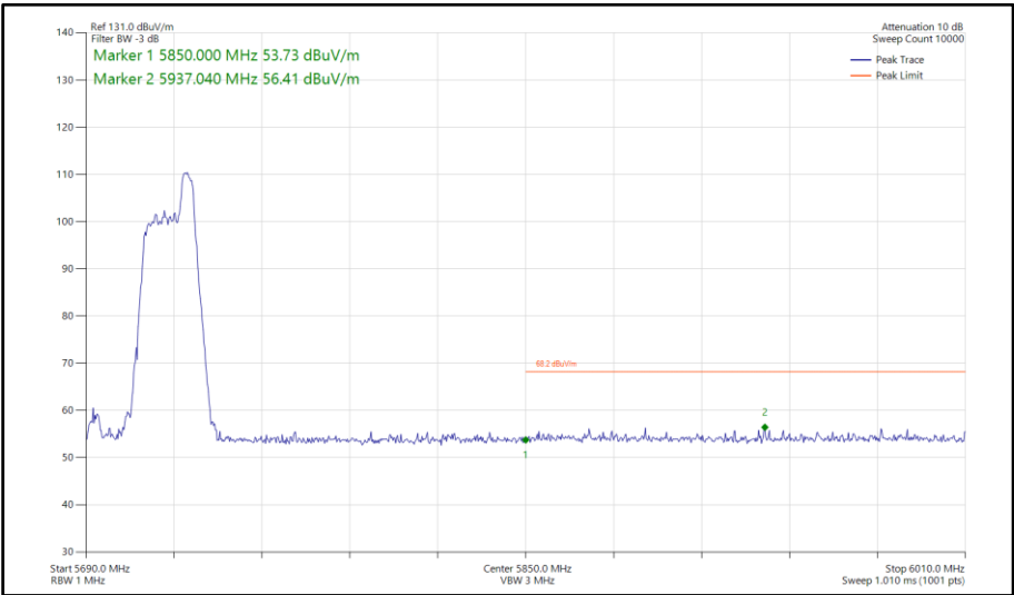
Figure 718 - 802.11ax HE40, RU 52-44, SISO, Core 0 - 5710 MHz Band Edge Frequency 5850 MHz
