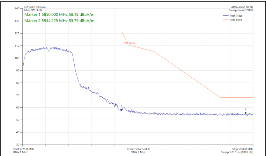
Figure 716 - 802.11n HT40, SISO, Core 0 - 5795 MHz Band Edge Frequency 5850 MHz
