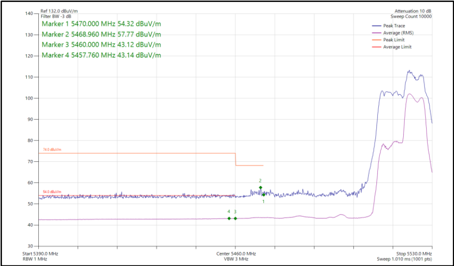
Figure 779 - 802.11be EHT40, RU 52+26-75, SDM, Core 0-1 - 5510 MHz Band Edge Frequency 5470 MHz
