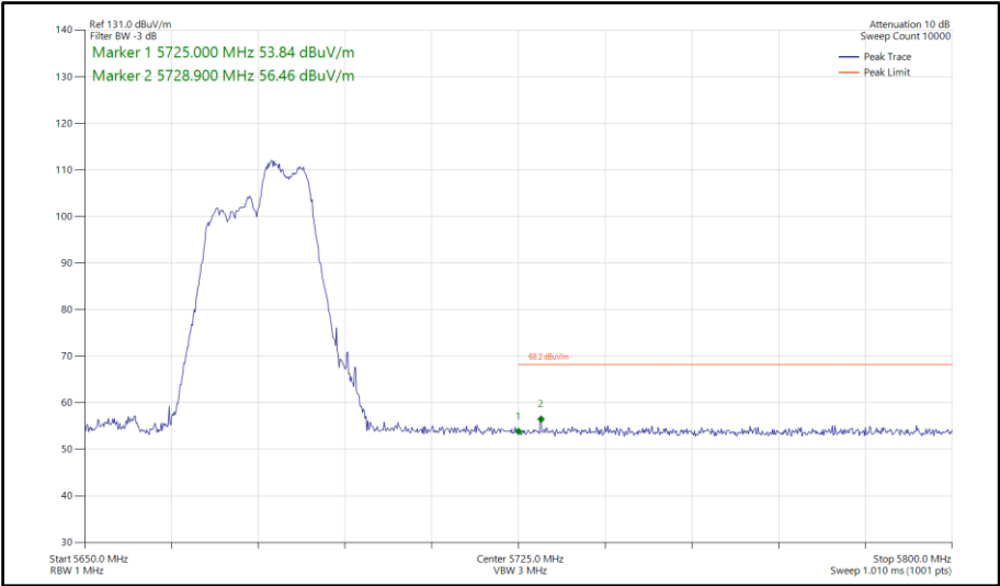
Figure 763 - 802.11ax HE40, RU 106-56, CDD, Core 0-1 - 5670 MHz Band Edge Frequency 5725 MHz
