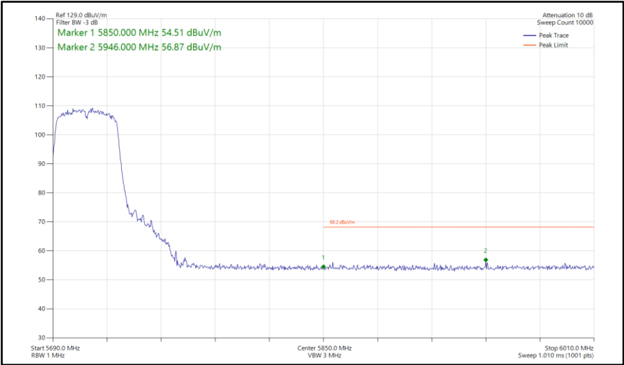
Figure 803 - 802.11ac VHT40, TxBF, Core 0-1 - 5710 MHz Band Edge Frequency 5850 MHz
