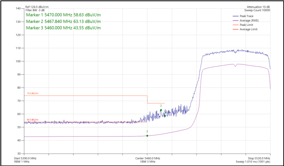
Figure 797 - 802.11ax HE40, SU, TxBF, Core 0-1 - 5510 MHz Band Edge Frequency 5470 MHz
