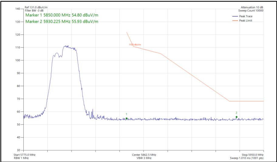
Figure 748 - 802.11be EHT40, RU 106+26-85, SISO, Core 1 - 5795 MHz Band Edge Frequency 5850 MHz
