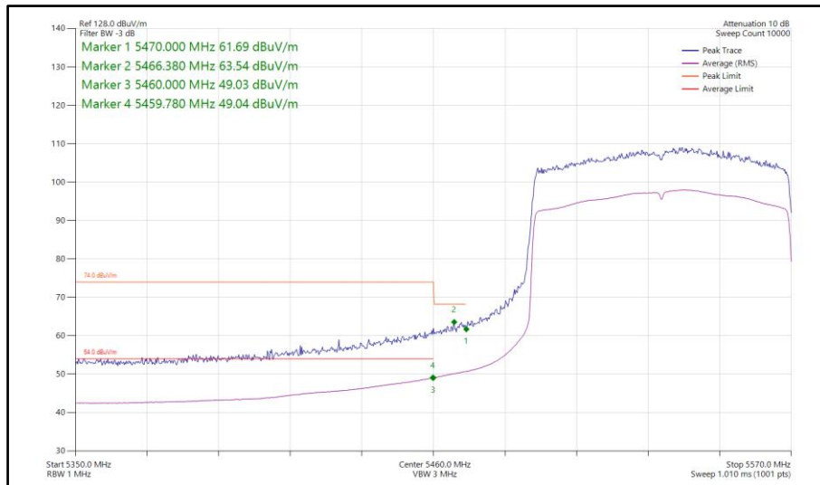
Figure 809 - 802.11ax HE80, SU, SISO, Core 0 - 5530 MHz Band Edge Frequency 5470 MHz
