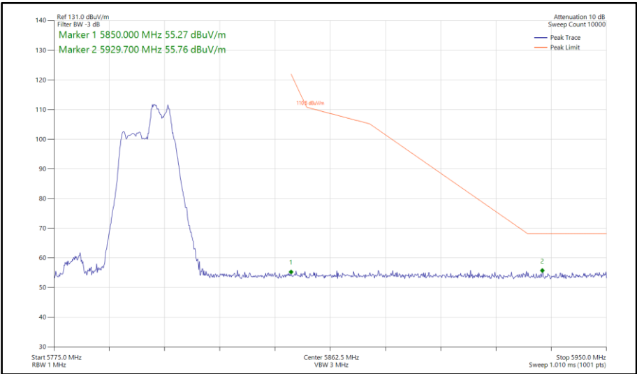
Figure 774 - 802.11be EHT40, RU 52+26-75, CDD, Core 0-1 - 5795 MHz Band Edge Frequency 5850 MHz
