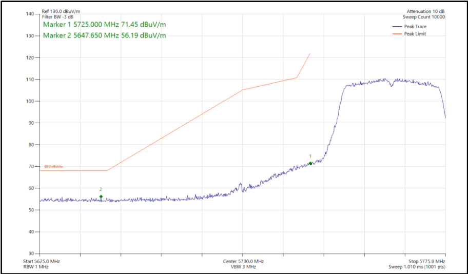
Figure 799 - 802.11ac VHT40, TxBF, Core 0-1 - 5755 MHz Band Edge Frequency 5725 MHz
