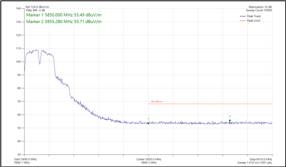
Figure 739 - 802.11a a40, SISO, Core 1 - 5710 MHz Band Edge Frequency 5850 MHz
