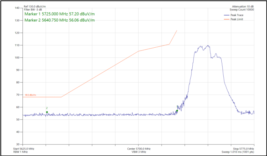
Figure 783 - 802.11be EHT40, RU 106+26-82, SDM, Core 0-1 - 5755 MHz Band Edge Frequency 5725 MHz
