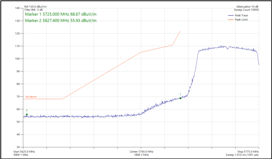
Figure 781 - 802.11ax HE40, SU, SDM, Core 0-1 - 5755 MHz Band Edge Frequency 5725 MHz
