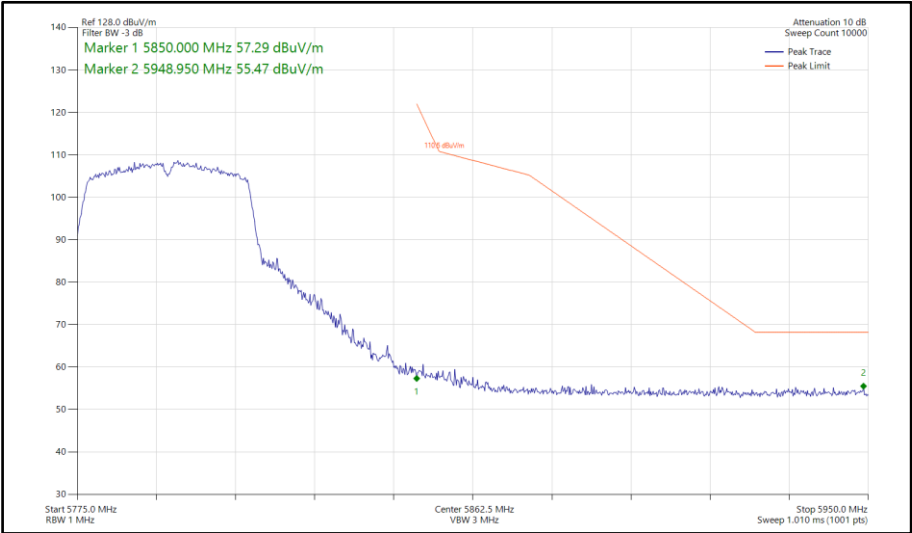
Figure 742 - 802.11n HT40, SISO, Core 1 - 5795 MHz Band Edge Frequency 5850 MHz
