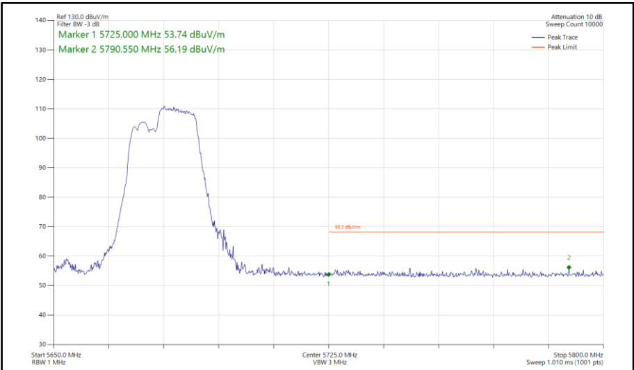
Figure 738 - 802.11be EHT40, RU 106+26-85, SISO, Core 1 - 5670 MHz Band Edge Frequency 5725 MHz
