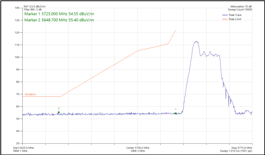
Figure 757 - 802.11ax HE40, RU 52-37, CDD, Core 0-1 - 5755 MHz Band Edge Frequency 5725 MHz
