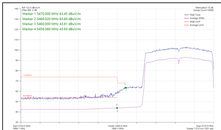
Figure 808 - 802.11ac VHT80, SISO, Core 0 - 5530 MHz Band Edge Frequency 5470 MHz
