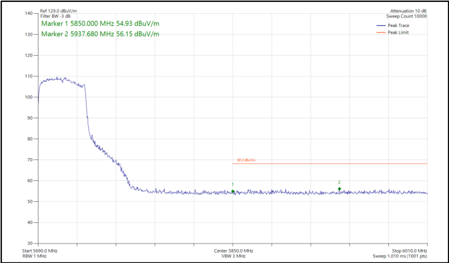
Figure 805 - 802.11ax HE40, SU, TxBF, Core 0-1 - 5710 MHz Band Edge Frequency 5850 MHz
