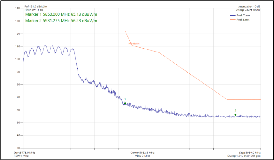
Figure 771 - 802.11ax HE40, SU, CDD, Core 0-1 - 5795 MHz Band Edge Frequency 5850 MHz
