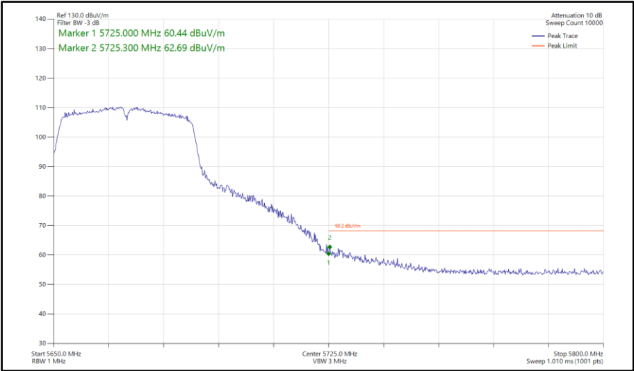
Figure 801 - 802.11ac VHT40, TxBF, Core 0-1 - 5670 MHz Band Edge Frequency 5725 MHz
