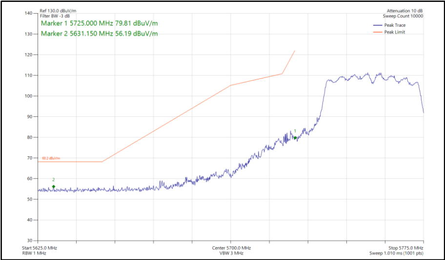
Figure 755 - 802.11n HT40, CDD, Core 0-1 - 5755 MHz Band Edge Frequency 5725 MHz
