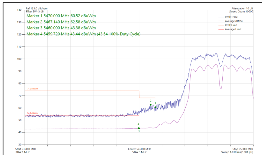
Figure 749 - 802.11a a40, CDD, Core 0-1 - 5510 MHz Band Edge Frequency 5470 MHz
