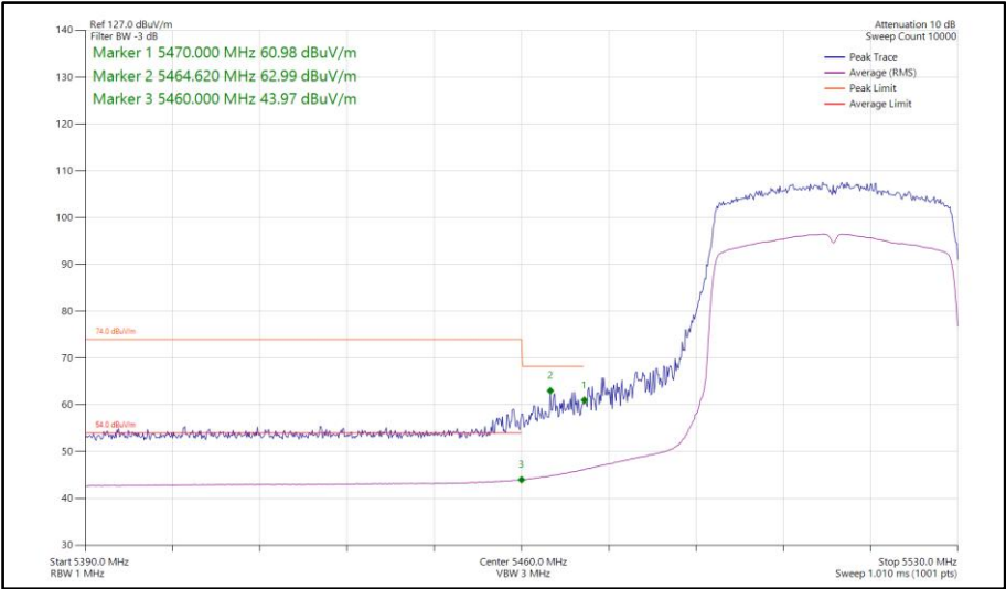
Figure 777 - 802.11ax HE40, SU, SDM, Core 0-1 - 5510 MHz Band Edge Frequency 5470 MHz
