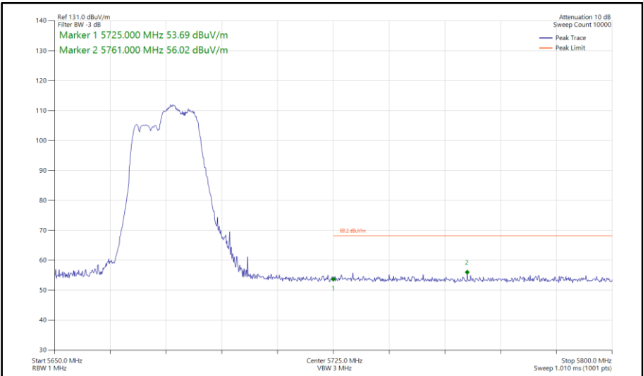
Figure 764 - 802.11be EHT40, RU 106+26-85, CDD, Core 0-1 - 5670 MHz Band Edge Frequency 5725 MHz
