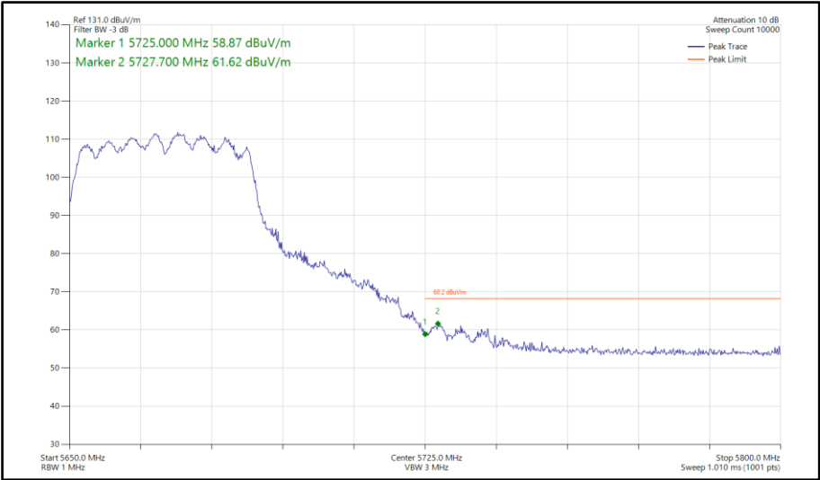
Figure 761 - 802.11n HT40, CDD, Core 0-1 - 5670 MHz Band Edge Frequency 5725 MHz
