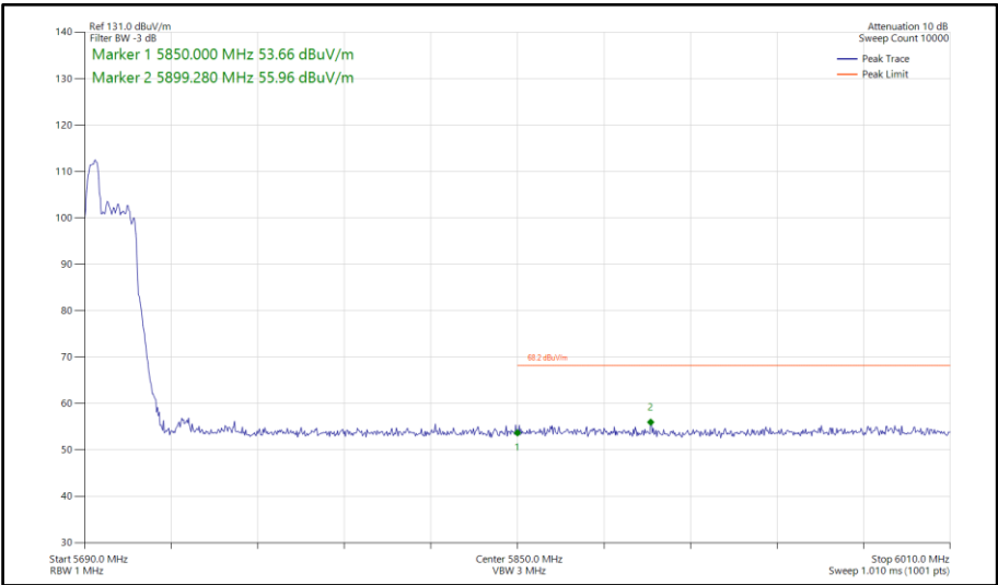
Figure 744 - 802.11ax HE40, RU 52-37, SISO, Core 1 - 5710 MHz Band Edge Frequency 5850 MHz
