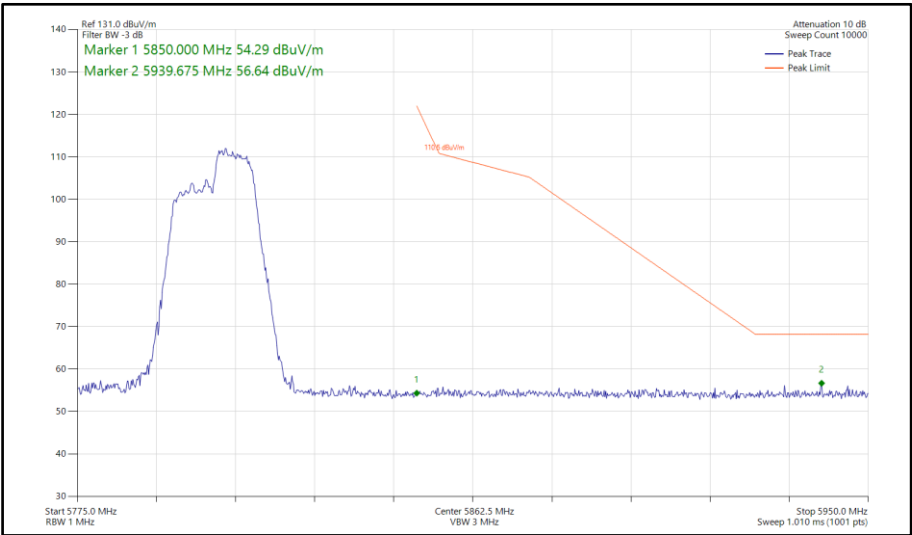
Figure 746 - 802.11ax HE40, RU 106-56, SISO, Core 1 - 5795 MHz Band Edge Frequency 5850 MHz
