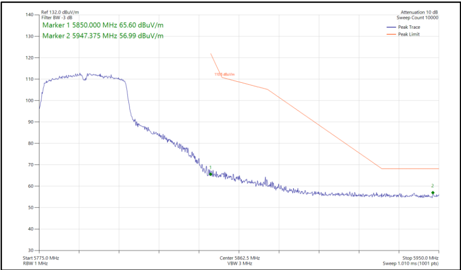
Figure 804 - 802.11ac VHT40, TxBF, Core 0-1 - 5795 MHz Band Edge Frequency 5850 MHz
