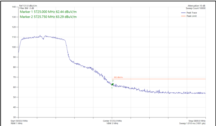
Figure 784 - 802.11n HT40, SDM, Core 0-1 - 5670 MHz Band Edge Frequency 5725 MHz
