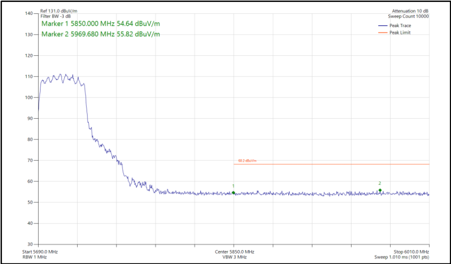
Figure 767 - 802.11n HT40, CDD, Core 0-1 - 5710 MHz Band Edge Frequency 5850 MHz
