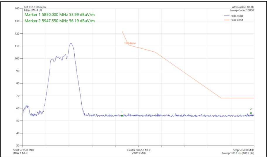
Figure 772 - 802.11ax HE40, RU 52-44, CDD, Core 0-1 - 5795 MHz Band Edge Frequency 5850 MHz
