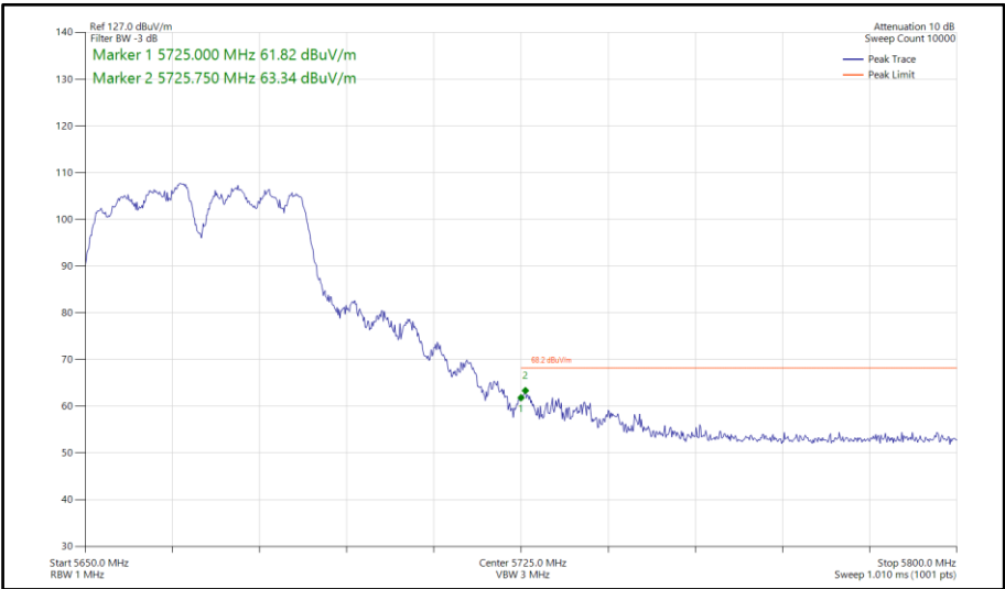
Figure 760 - 802.11a a40, CDD, Core 0-1 - 5670 MHz Band Edge Frequency 5725 MHz
