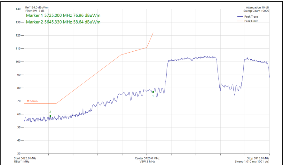
Figure 816 - 802.11be EHT80, RU 484+242-92, SISO, Core 0 - 5775 MHz Band Edge Frequency 5725 MHz
