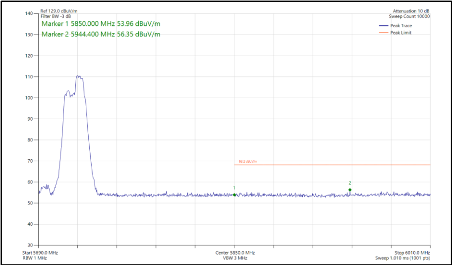
Figure 747 - 802.11be EHT40, RU 52+26-75, SISO, Core 1 - 5710 MHz Band Edge Frequency 5850 MHz
