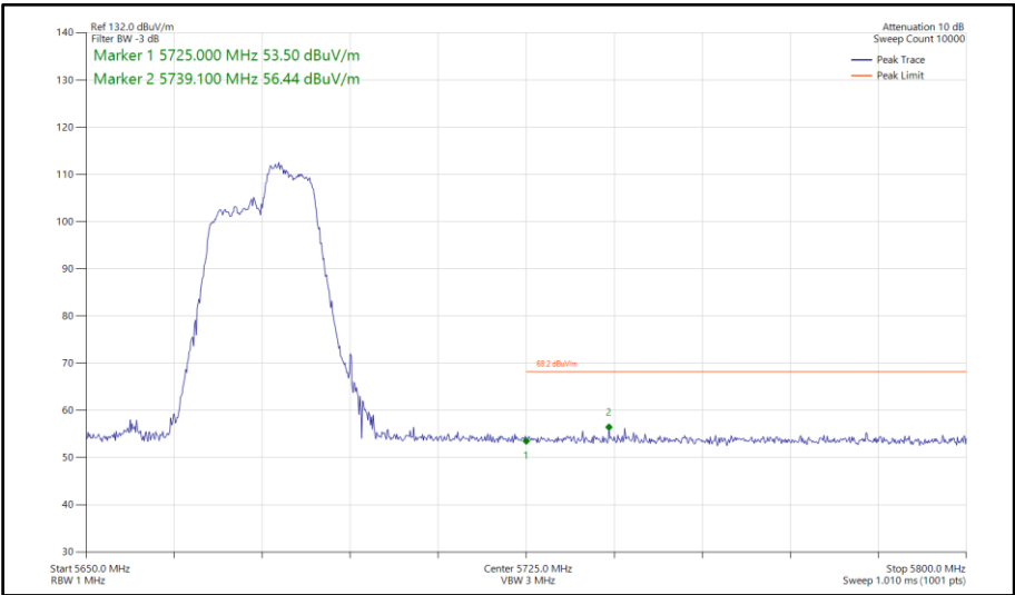
Figure 786 - 802.11ax HE40, RU 106-56, SDM, Core 0-1 - 5670 MHz Band Edge Frequency 5725 MHz
