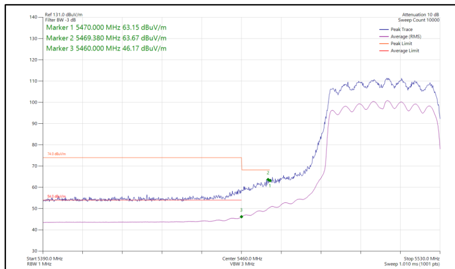
Figure 751 - 802.11ax HE40, SU, CDD, Core 0-1 - 5510 MHz Band Edge Frequency 5470 MHz
