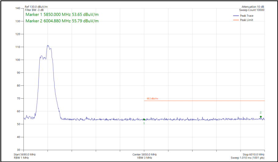
Figure 773 - 802.11be EHT40, RU 52+26-75, CDD, Core 0-1 - 5710 MHz Band Edge Frequency 5850 MHz
