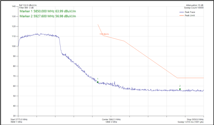
Figure 806 - 802.11ax HE40, SU, TxBF, Core 0-1 - 5795 MHz Band Edge Frequency 5850 MHz
