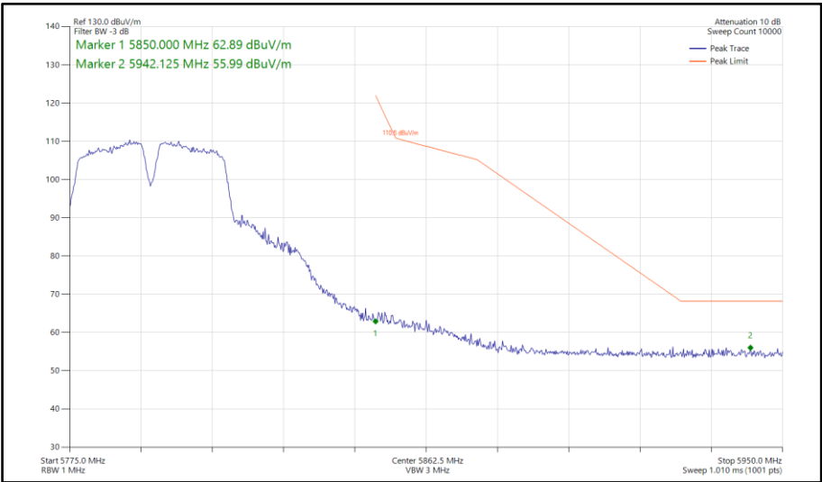
Figure 740 - 802.11a a40, SISO, Core 1 - 5795 MHz Band Edge Frequency 5850 MHz
