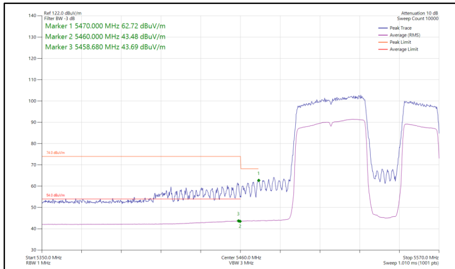
Figure 811 - 802.11be EHT80, RU 484+242-92, SISO, Core 0 - 5530 MHz Band Edge Frequency 5470 MHz
