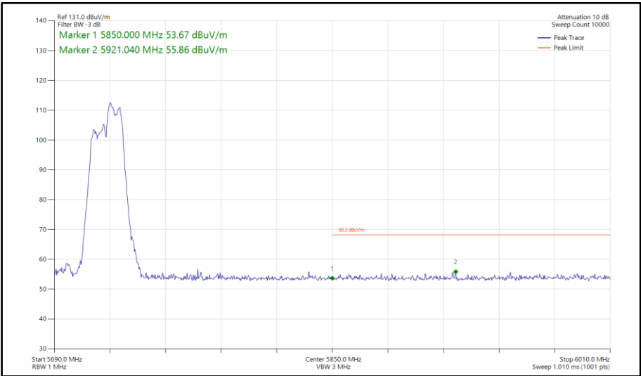
Figure 770 - 802.11ax HE40, RU 106-56, CDD, Core 0-1 - 5710 MHz Band Edge Frequency 5850 MHz
