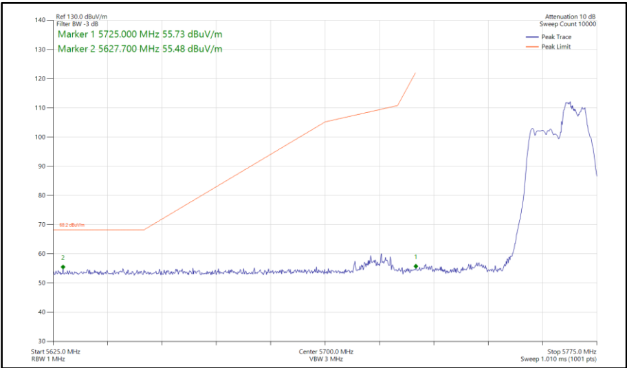
Figure 758 - 802.11be EHT40, RU 52+26-75, CDD, Core 0-1 - 5755 MHz Band Edge Frequency 5725 MHz
