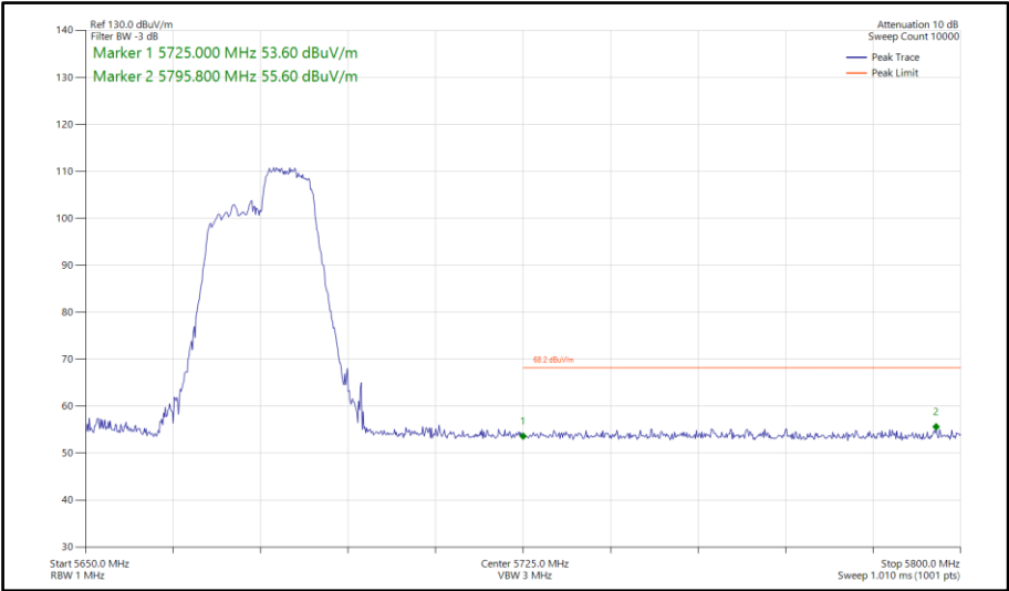
Figure 737 - 802.11ax HE40, RU 106-56, SISO, Core 1 - 5670 MHz Band Edge Frequency 5725 MHz
