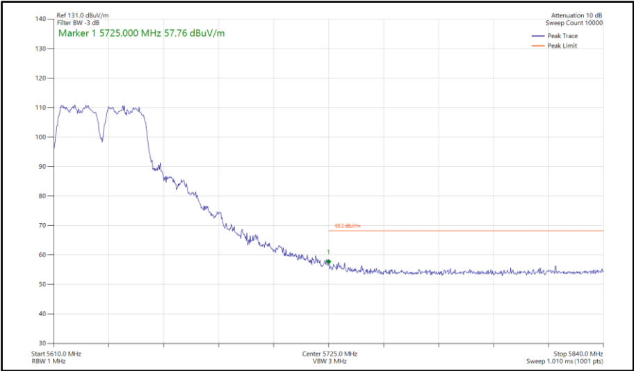
Figure 759 - 802.11a a40, CDD, Core 0-1 - 5630 MHz Band Edge Frequency 5725 MHz
