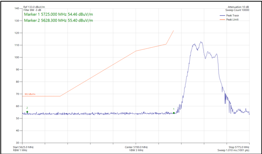
Figure 782 - 802.11ax HE40, RU 106-53, SDM, Core 0-1 - 5755 MHz Band Edge Frequency 5725 MHz
