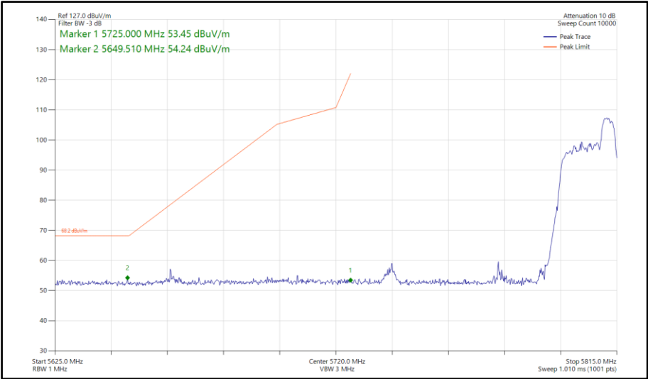
Figure 815 - 802.11ax HE80, RU 52-52, SISO, Core 0 - 5775 MHz Band Edge Frequency 5725 MHz
