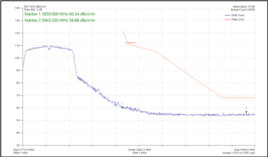
Figure 789 - 802.11n HT40, SDM, Core 0-1 - 5795 MHz Band Edge Frequency 5850 MHz
