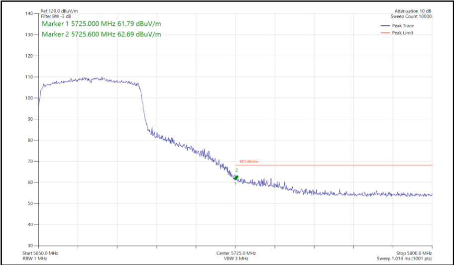
Figure 736 - 802.11ax HE40, SU, SISO, Core 1 - 5670 MHz Band Edge Frequency 5725 MHz
