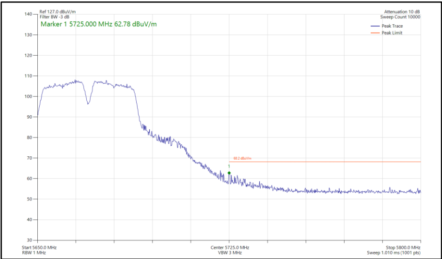
Figure 734 - 802.11a a40, SISO, Core 1 - 5670 MHz Band Edge Frequency 5725 MHz
