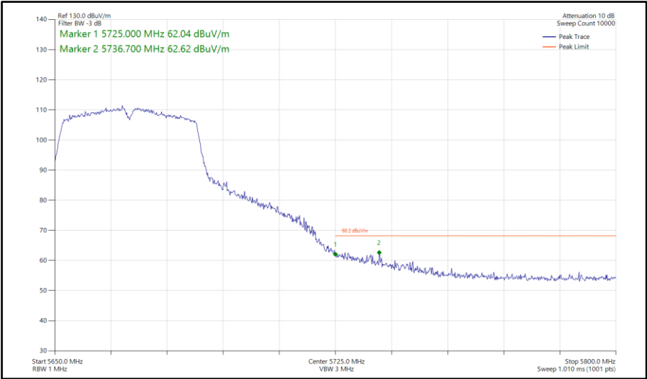
Figure 735 - 802.11n HT40, SISO, Core 1 - 5670 MHz Band Edge Frequency 5725 MHz
