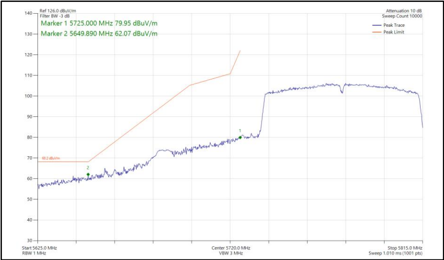
Figure 813 - 802.11ac VHT80, SISO, Core 0 - 5775 MHz Band Edge Frequency 5725 MHz
