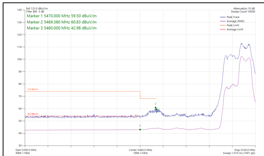
Figure 753 - 802.11be EHT40, RU 52+26-75, CDD, Core 0-1 - 5510 MHz Band Edge Frequency 5470 MHz
