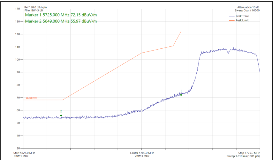
Figure 780 - 802.11n HT40, SDM, Core 0-1 - 5755 MHz Band Edge Frequency 5725 MHz
