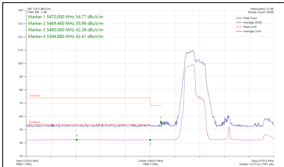
Figure 810 - 802.11ax HE80, RU 106-53, SISO, Core 0 - 5530 MHz Band Edge Frequency 5470 MHz
