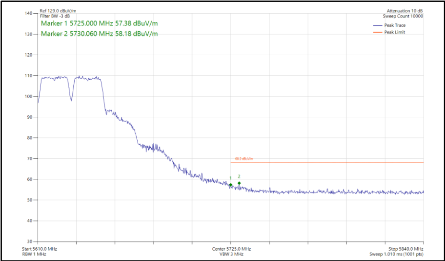
Figure 733 - 802.11a a40, SISO, Core 1 - 5630 MHz Band Edge Frequency 5725 MHz
