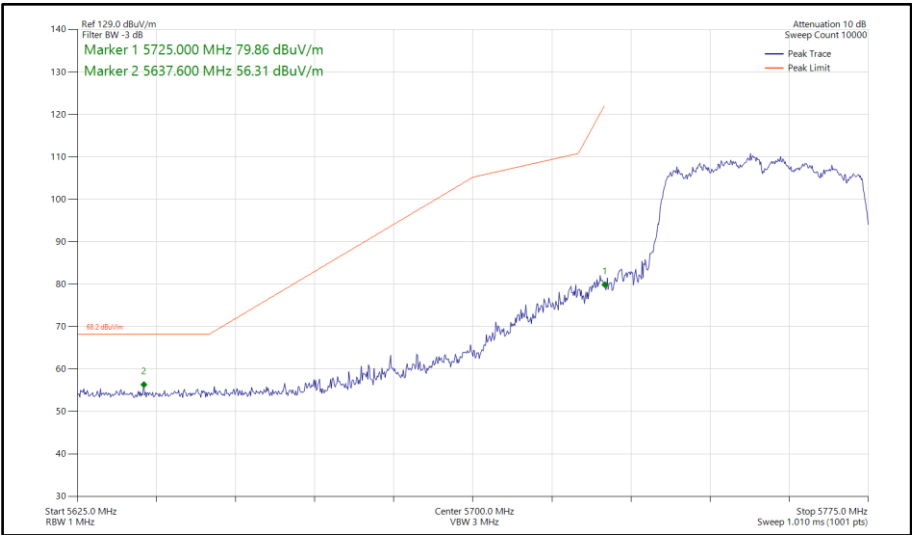
Figure 756 - 802.11ax HE40, SU, CDD, Core 0-1 - 5755 MHz Band Edge Frequency 5725 MHz
