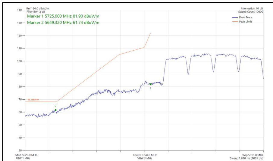
Figure 812 - 802.11a a80, SISO, Core 0 - 5775 MHz Band Edge Frequency 5725 MHz
