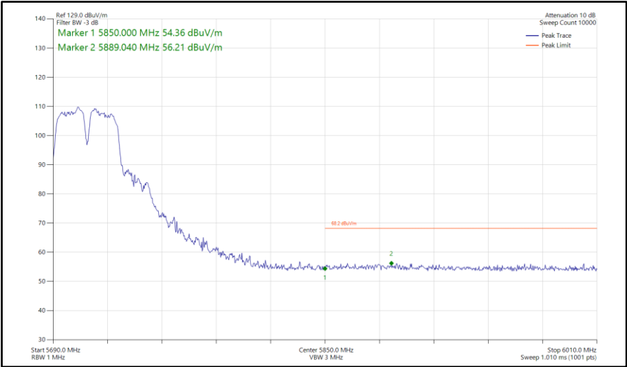
Figure 765 - 802.11a a40, CDD, Core 0-1 - 5710 MHz Band Edge Frequency 5850 MHz
