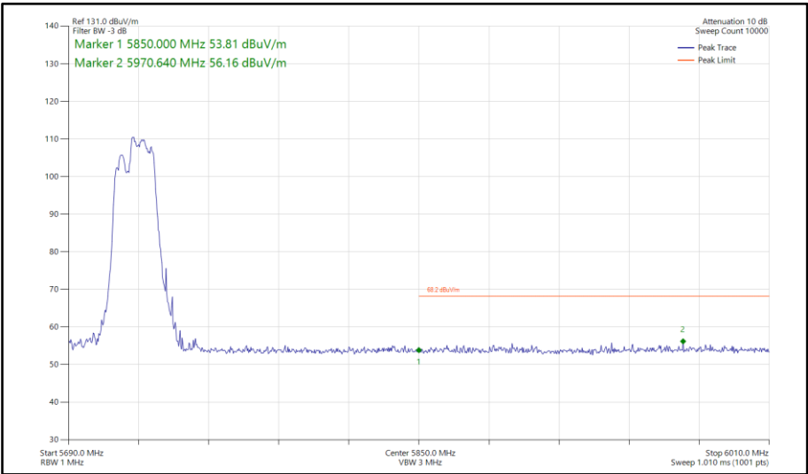
Figure 794 - 802.11be EHT40, RU 106+26-85, SDM, Core 0-1 - 5710 MHz Band Edge Frequency 5850 MHz
