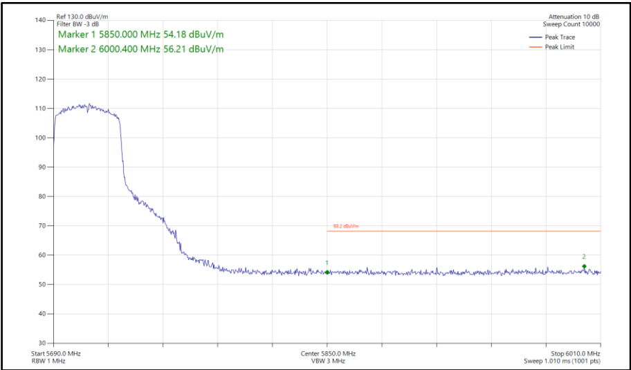
Figure 790 - 802.11ax HE40, SU, SDM, Core 0-1 - 5710 MHz Band Edge Frequency 5850 MHz
