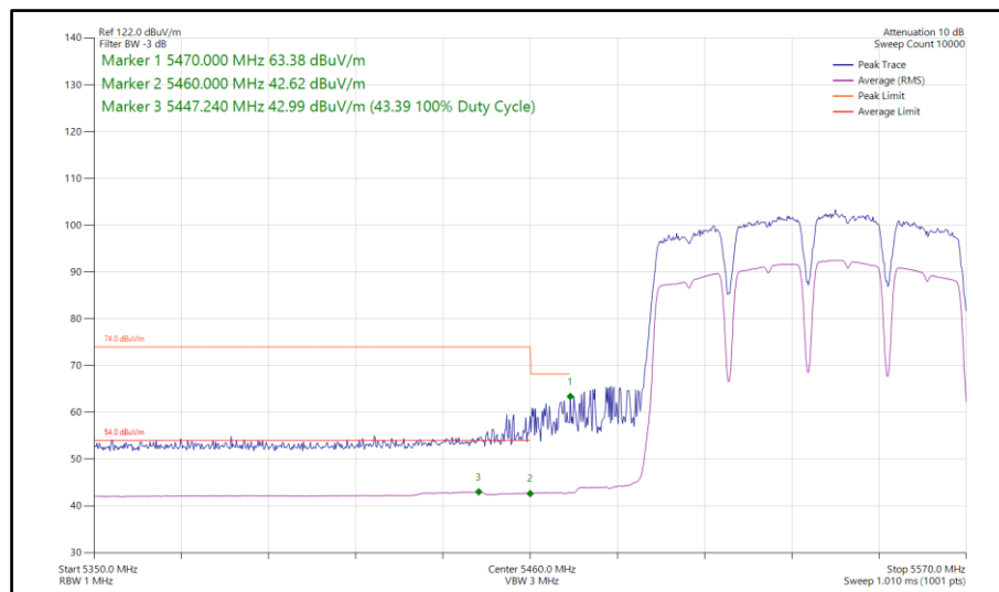
Figure 807 - 802.11a a80, SISO, Core 0 - 5530 MHz Band Edge Frequency 5470 MHz
