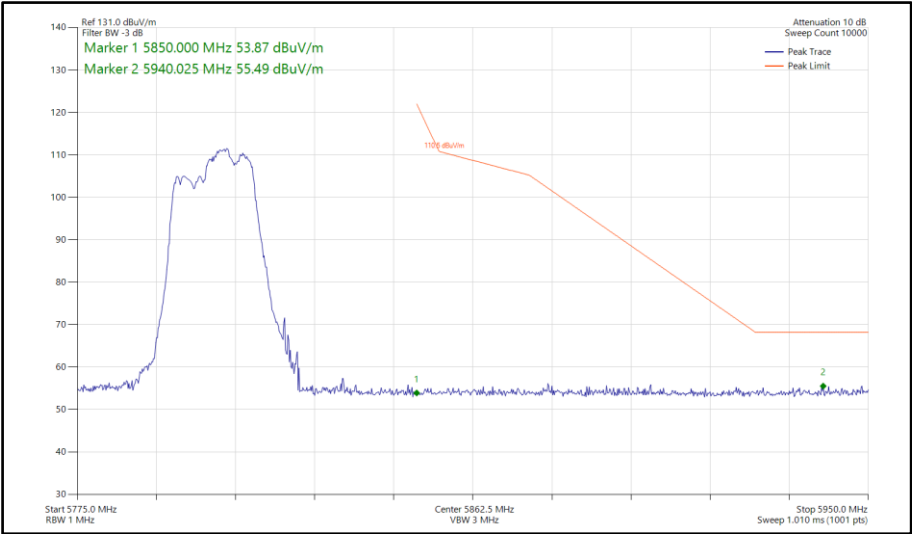
Figure 795 - 802.11be EHT40, RU 106+26-85, SDM, Core 0-1 - 5795 MHz Band Edge Frequency 5850 MHz
