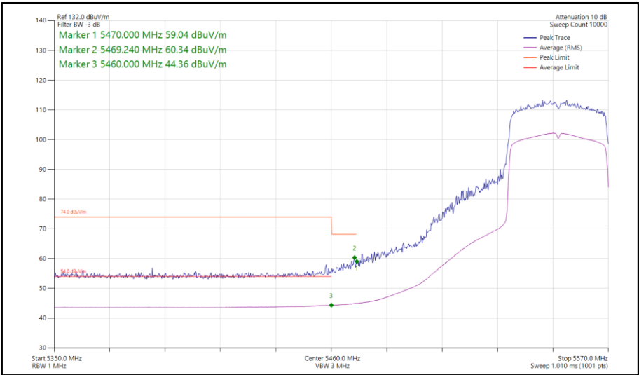
Figure 798 - 802.11ax HE40, SU, TxBF, Core 0-1 - 5550 MHz Band Edge Frequency 5470 MHz
