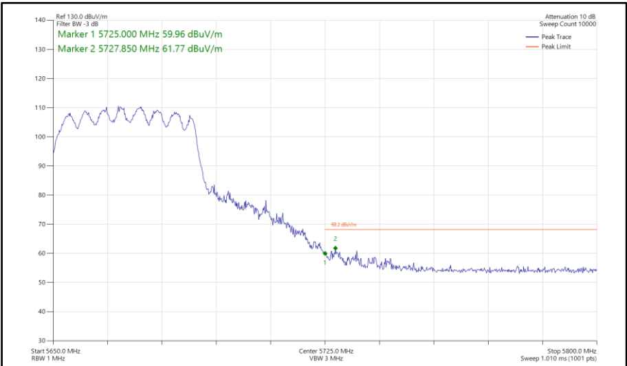
Figure 762 - 802.11ax HE40, SU, CDD, Core 0-1 - 5670 MHz Band Edge Frequency 5725 MHz
