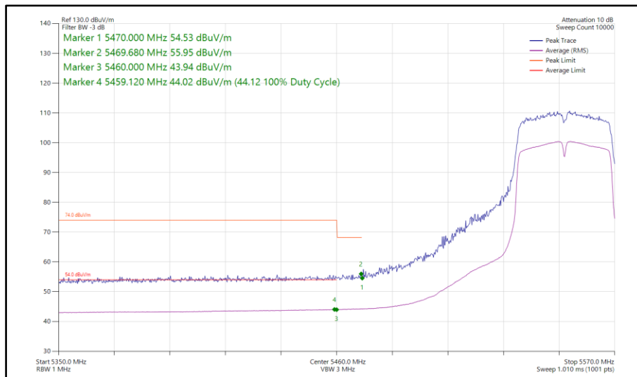
Figure 776 - 802.11n HT40, SDM, Core 0-1 - 5550 MHz Band Edge Frequency 5470 MHz
