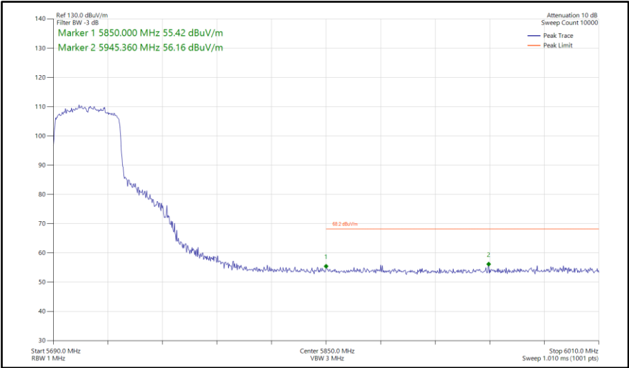
Figure 743 - 802.11ax HE40, SU, SISO, Core 1 - 5710 MHz Band Edge Frequency 5850 MHz
