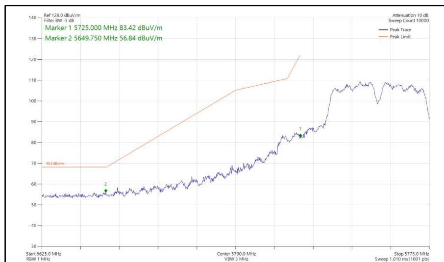
Figure 754 - 802.11a a40, CDD, Core 0-1 - 5755 MHz Band Edge Frequency 5725 MHz
