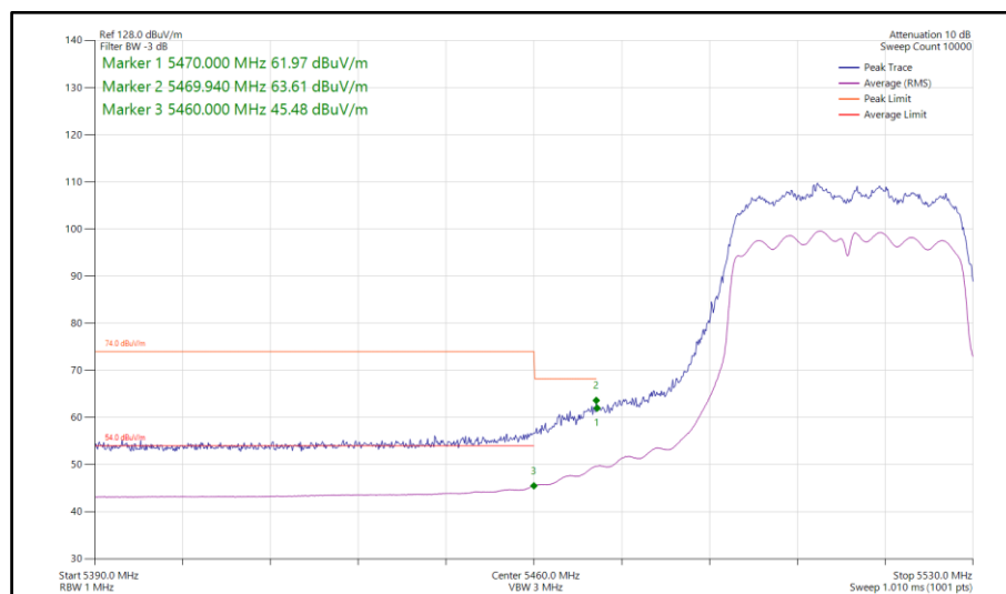
Figure 750 - 802.11n HT40, CDD, Core 0-1 - 5510 MHz Band Edge Frequency 5470 MHz
