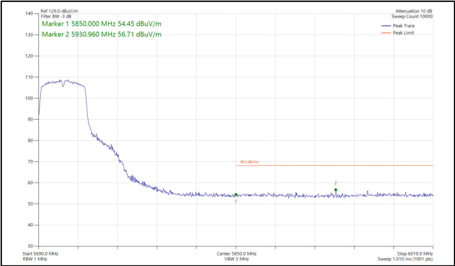
Figure 741 - 802.11n HT40, SISO, Core 1 - 5710 MHz Band Edge Frequency 5850 MHz
