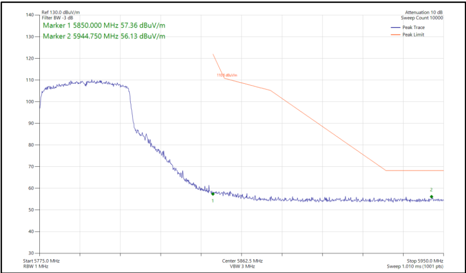
Figure 792 - 802.11ax HE40, SU, SDM, Core 0-1 - 5795 MHz Band Edge Frequency 5850 MHz
