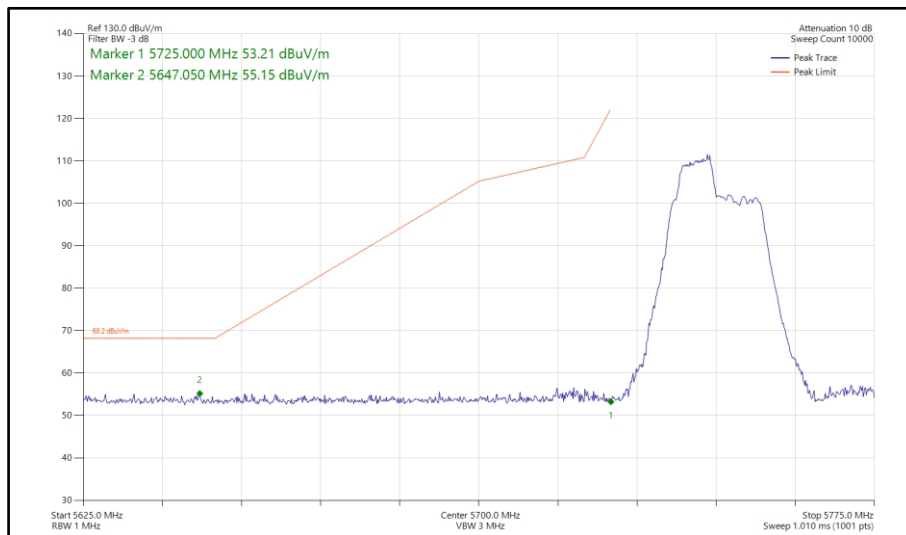
Figure 732 - 802.11be EHT40, RU 52+26-70, SISO, Core 1 - 5755 MHz Band Edge Frequency 5725 MHz
