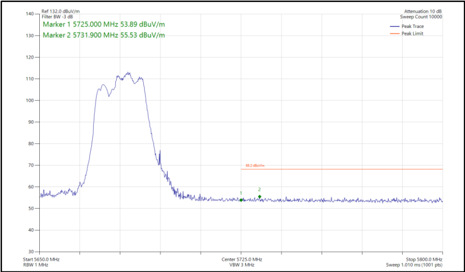
Figure 787 - 802.11be EHT40, RU 106+26-85, SDM, Core 0-1 - 5670 MHz Band Edge Frequency 5725 MHz
