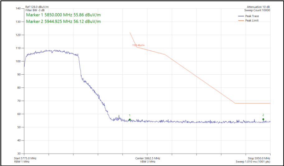
Figure 745 - 802.11ax HE40, SU, SISO, Core 1 - 5795 MHz Band Edge Frequency 5850 MHz
