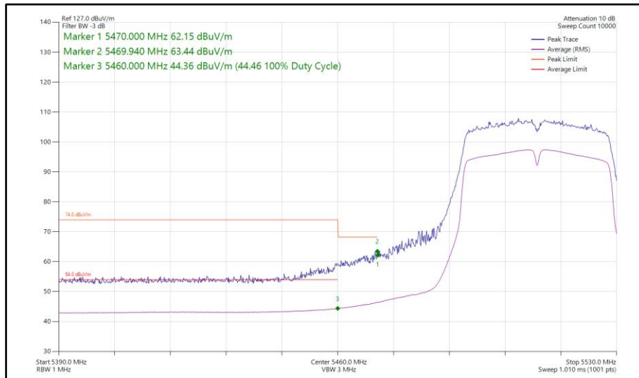
Figure 775 - 802.11n HT40, SDM, Core 0-1 - 5510 MHz Band Edge Frequency 5470 MHz
