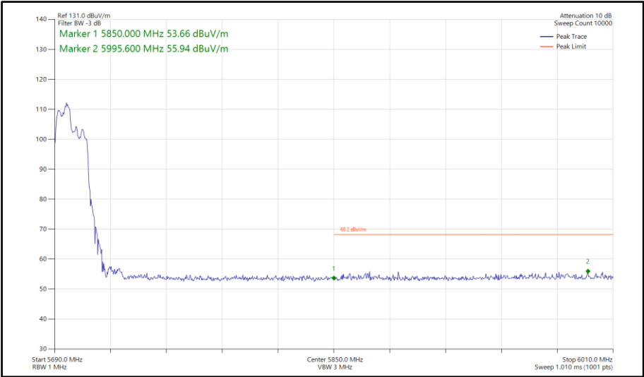
Figure 791 - 802.11ax HE40, RU 106-53, SDM, Core 0-1 - 5710 MHz Band Edge Frequency 5850 MHz
