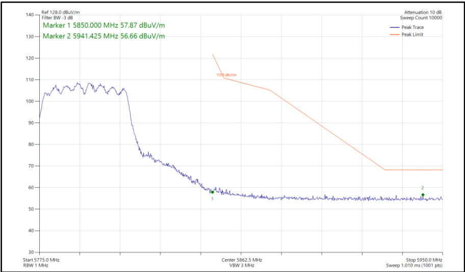
Figure 768 - 802.11n HT40, CDD, Core 0-1 - 5795 MHz Band Edge Frequency 5850 MHz
