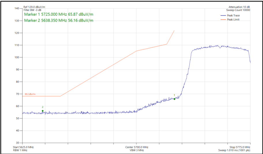
Figure 800 - 802.11ax HE40, SU, TxBF, Core 0-1 - 5755 MHz Band Edge Frequency 5725 MHz
