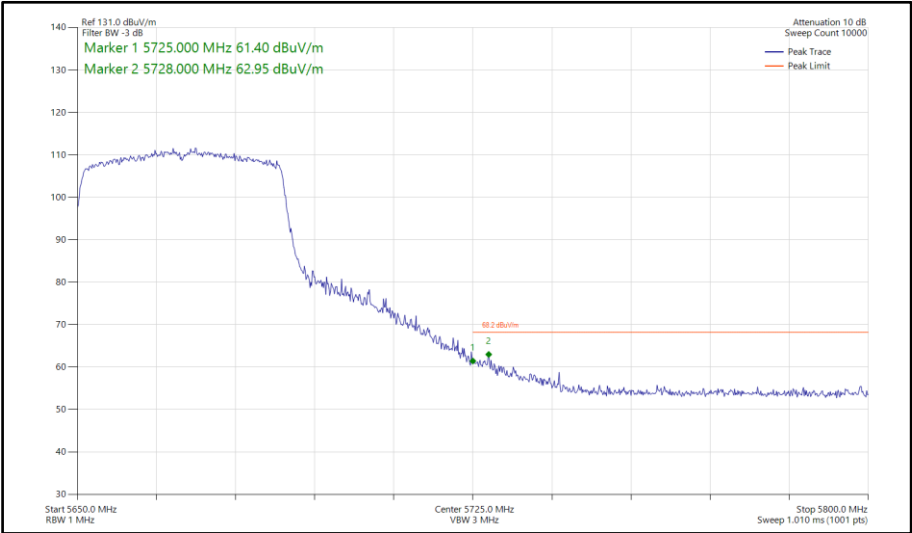
Figure 802 - 802.11ax HE40, SU, TxBF, Core 0-1 - 5670 MHz Band Edge Frequency 5725 MHz
