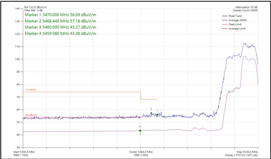
Figure 778 - 802.11ax HE40, RU 106-56, SDM, Core 0-1 - 5510 MHz Band Edge Frequency 5470 MHz
