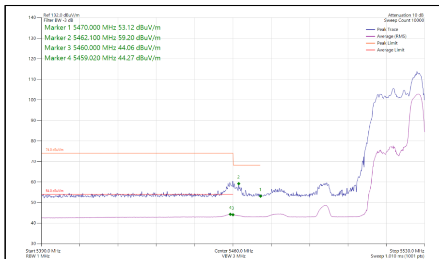
Figure 752 - 802.11ax HE40, RU 52-44, CDD, Core 0-1 - 5510 MHz Band Edge Frequency 5470 MHz
