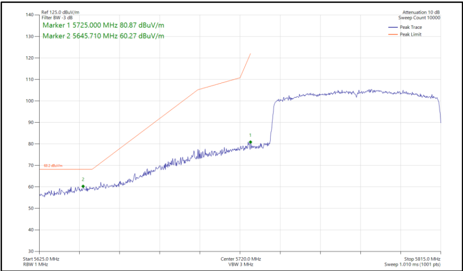
Figure 814 - 802.11ax HE80, SU, SISO, Core 0 - 5775 MHz Band Edge Frequency 5725 MHz
