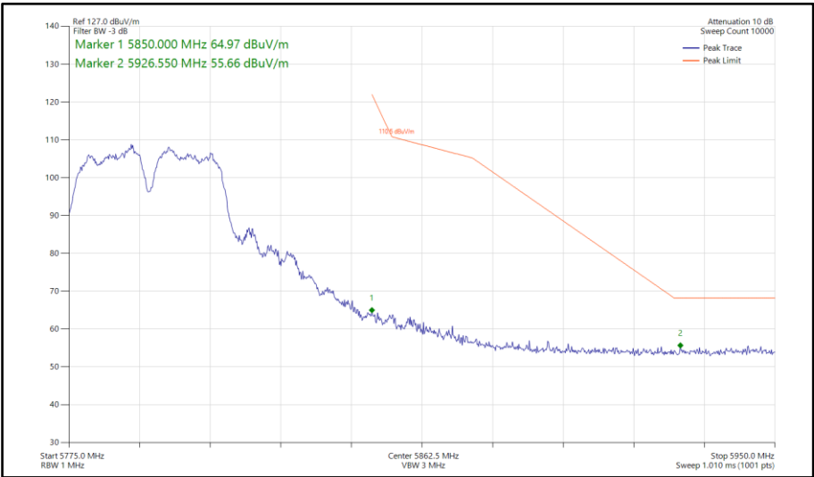
Figure 766 - 802.11a a40, CDD, Core 0-1 - 5795 MHz Band Edge Frequency 5850 MHz
