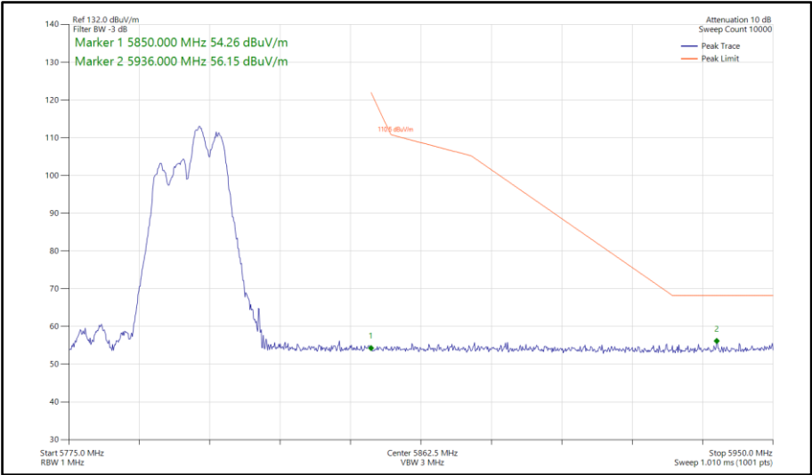
Figure 793 - 802.11ax HE40, RU 106-56, SDM, Core 0-1 - 5795 MHz Band Edge Frequency 5850 MHz
