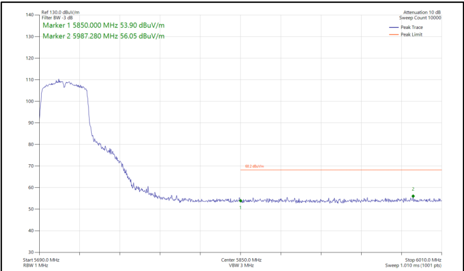
Figure 788 - 802.11n HT40, SDM, Core 0-1 - 5710 MHz Band Edge Frequency 5850 MHz
