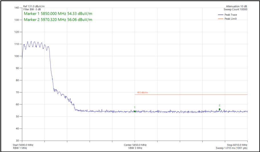
Figure 769 - 802.11ax HE40, SU, CDD, Core 0-1 - 5710 MHz Band Edge Frequency 5850 MHz
