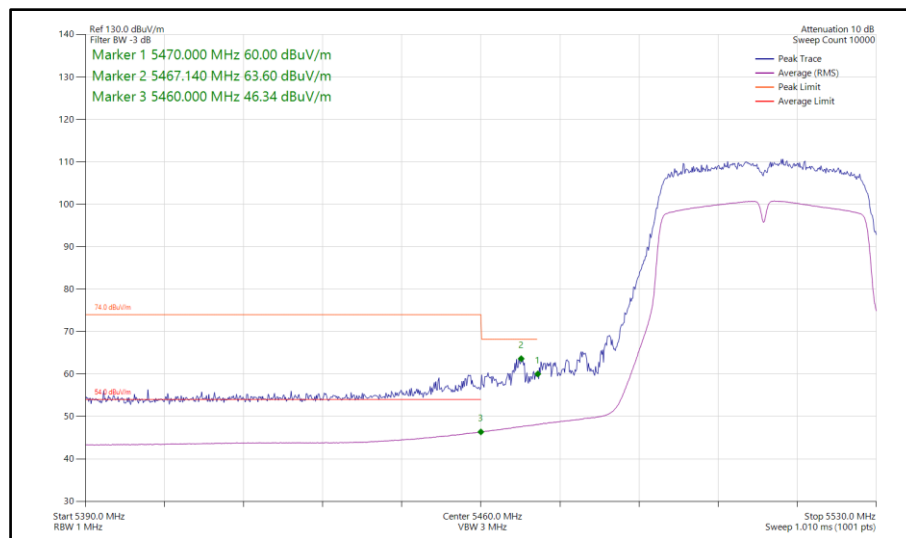
Figure 796 - 802.11ac VHT40, TxBF, Core 0-1 - 5510 MHz Band Edge Frequency 5470 MHz
