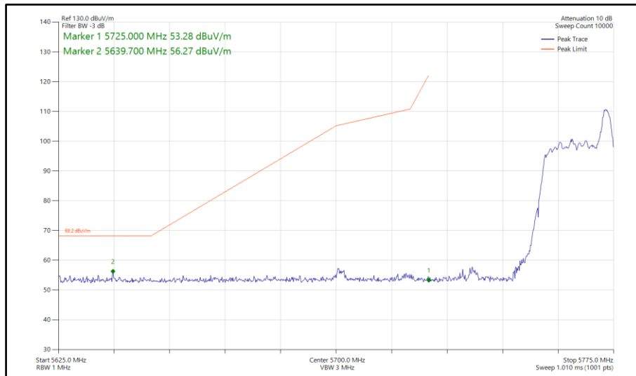
Figure 731 - 802.11ax HE40, RU 26-17, SISO, Core 1 - 5755 MHz Band Edge Frequency 5725 MHz
