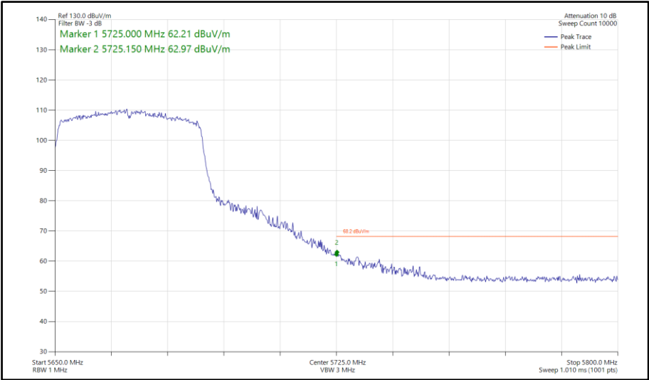
Figure 785 - 802.11ax HE40, SU, SDM, Core 0-1 - 5670 MHz Band Edge Frequency 5725 MHz
