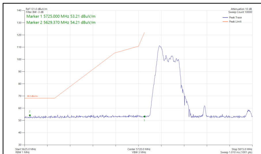
Figure 888 - 802.11ax HE80, RU 52-37, SDM, Core 0-1 - 5775 MHz Band Edge Frequency 5725 MHz
