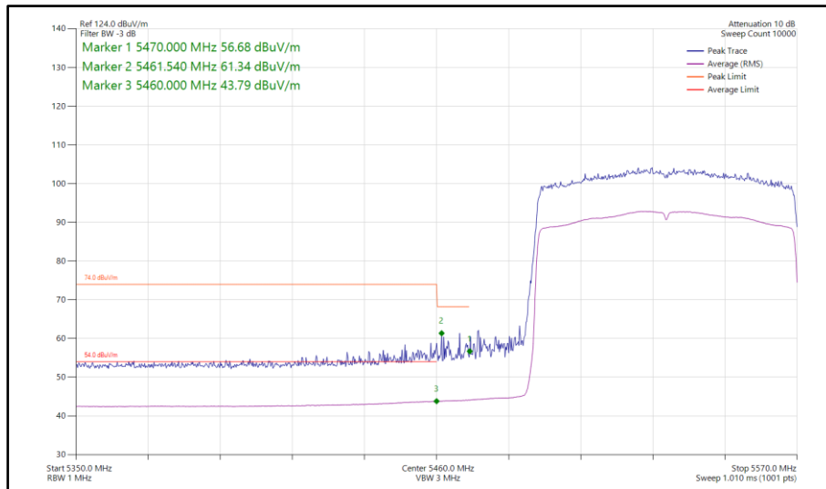
Figure 903 - 802.11ax HE80, SU, TxBF, Core 0-1 - 5530 MHz Band Edge Frequency 5470 MHz
