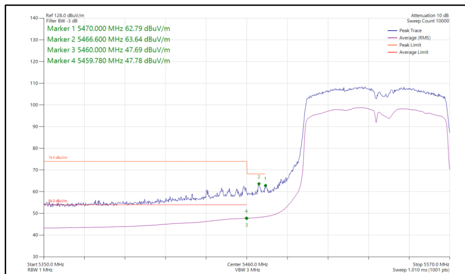
Figure 902 - 802.11ac VHT80, TxBF, Core 0-1 - 5530 MHz Band Edge Frequency 5470 MHz
