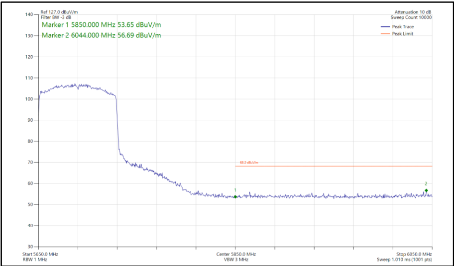
Figure 826 - 802.11ax HE80, SU, SISO, Core 0 - 5690 MHz Band Edge Frequency 5850 MHz
