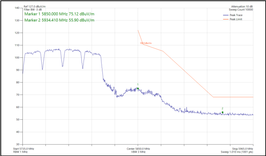
Figure 848 - 802.11a a80, SISO, Core 1 - 5775 MHz Band Edge Frequency 5850 MHz
