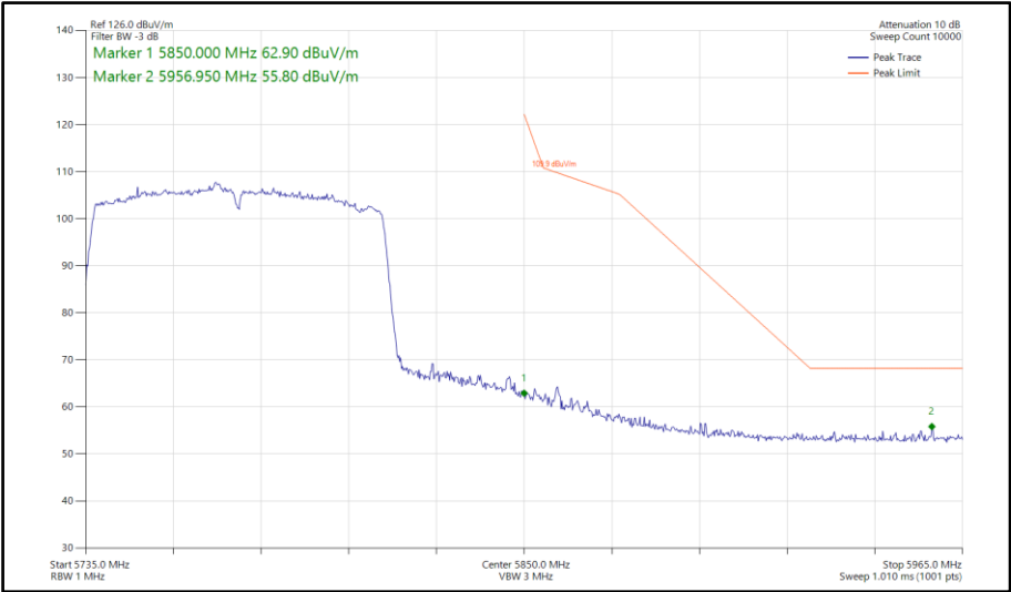
Figure 895 - 802.11ac VHT80, SDM, Core 0-1 - 5775 MHz Band Edge Frequency 5850 MHz
