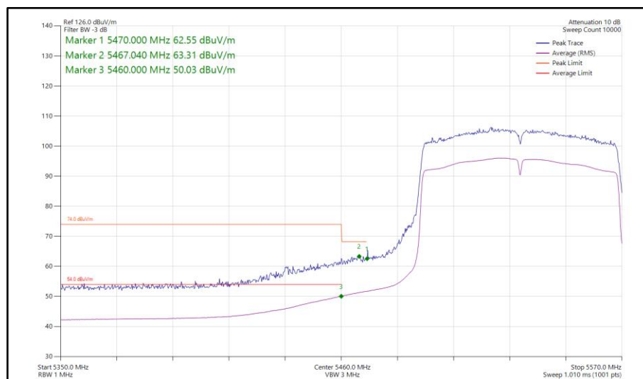
Figure 833 - 802.11ac VHT80, SISO, Core 1 - 5530 MHz Band Edge Frequency 5470 MHz
