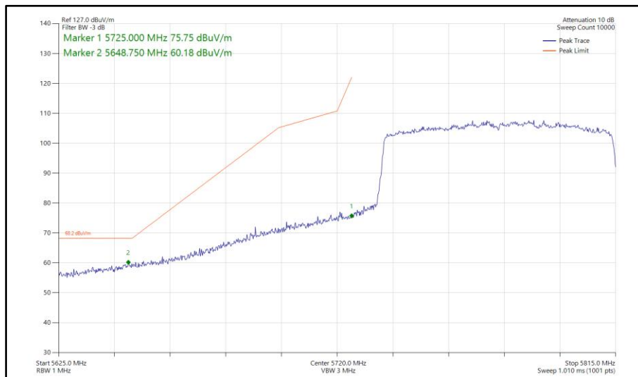
Figure 864 - 802.11ax HE80, SU, CDD, Core 0-1 - 5775 MHz Band Edge Frequency 5725 MHz
