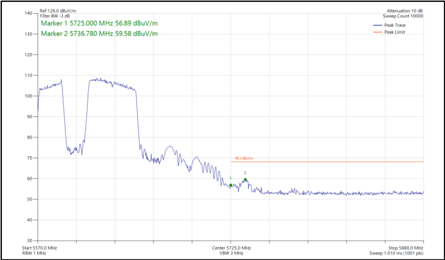
Figure 821 - 802.11be EHT80, RU 484+242-91, SISO, Core 0 - 5610 MHz Band Edge Frequency 5725 MHz
