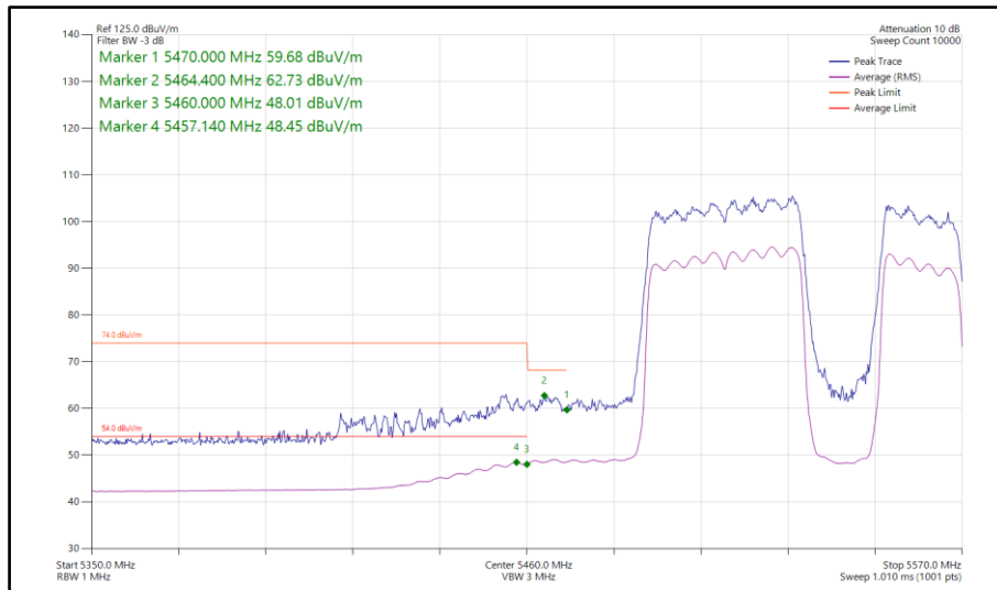
Figure 861 - 802.11be EHT80, RU 484+242-92, CDD, Core 0-1 - 5530 MHz Band Edge Frequency 5470 MHz
