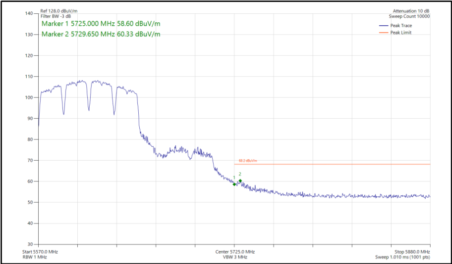
Figure 842 - 802.11a a80, SISO, Core 1 - 5610 MHz Band Edge Frequency 5725 MHz
