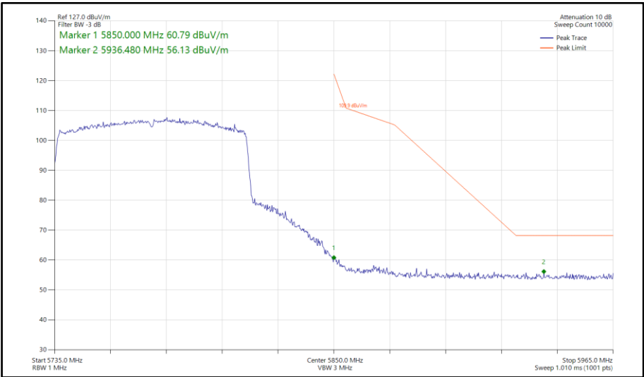
Figure 853 - 802.11ax HE80, SU, SISO, Core 1 - 5775 MHz Band Edge Frequency 5850 MHz
