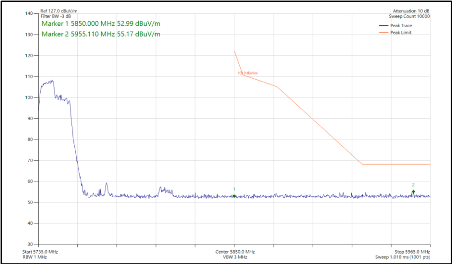
Figure 854 - 802.11ax HE80, RU 106-53, SISO, Core 1 - 5775 MHz Band Edge Frequency 5850 MHz
