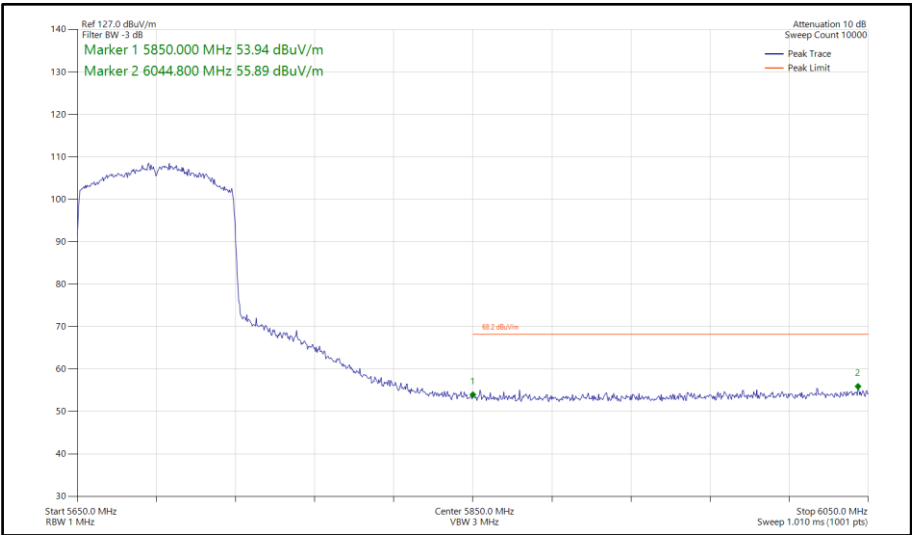
Figure 851 - 802.11ax HE80, SU, SISO, Core 1 - 5690 MHz Band Edge Frequency 5850 MHz
