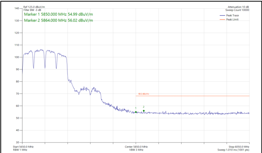
Figure 822 - 802.11a a80, SISO, Core 0 - 5690 MHz Band Edge Frequency 5850 MHz
