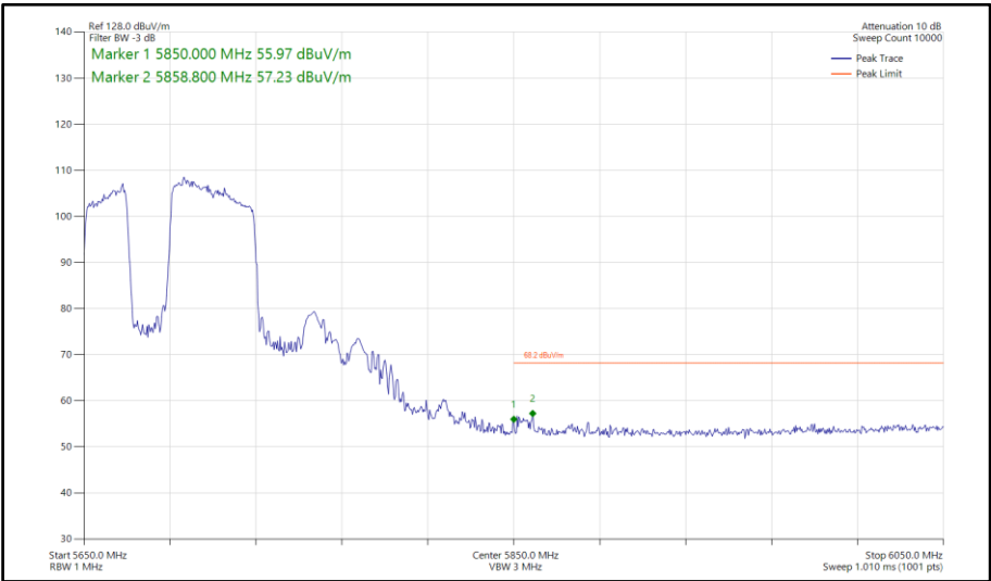
Figure 855 - 802.11be EHT80, RU 484+242-91, SISO, Core 1 - 5690 MHz Band Edge Frequency 5850 MHz
