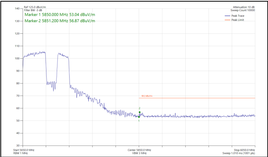
Figure 830 - 802.11be EHT80, RU 484+242-92, SISO, Core 0 - 5690 MHz Band Edge Frequency 5850 MHz
