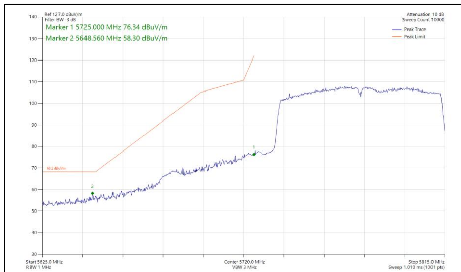
Figure 904 - 802.11ac VHT80, TxBF, Core 0-1 - 5775 MHz Band Edge Frequency 5725 MHz
