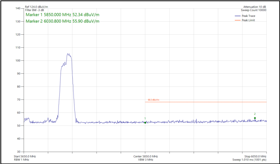
Figure 827 - 802.11ax HE80, RU 106-60, SISO, Core 0 - 5690 MHz Band Edge Frequency 5850 MHz
