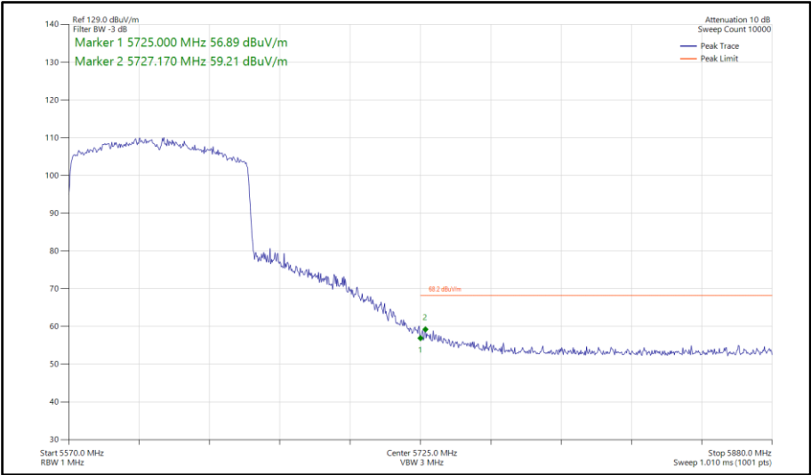
Figure 869 - 802.11ax HE80, SU, CDD, Core 0-1 - 5610 MHz Band Edge Frequency 5725 MHz
