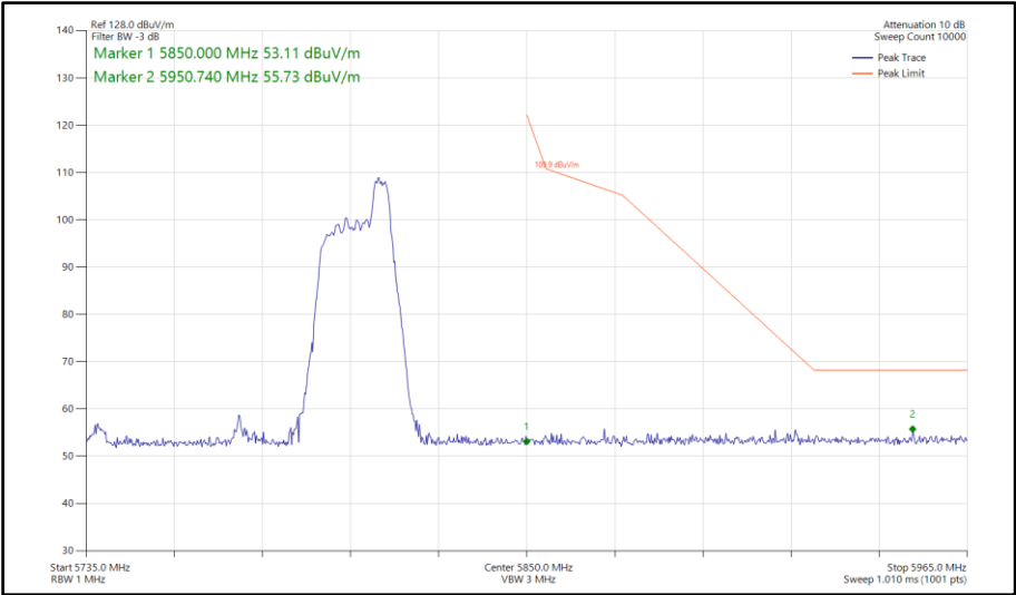
Figure 829 - 802.11ax HE80, RU 52-52, SISO, Core 0 - 5775 MHz Band Edge Frequency 5850 MHz
