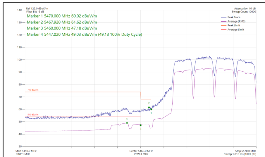
Figure 832 - 802.11a a80, SISO, Core 1 - 5530 MHz Band Edge Frequency 5470 MHz
