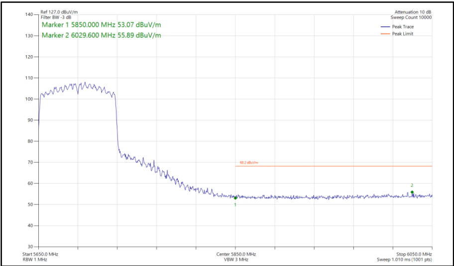
Figure 874 - 802.11ac VHT80, CDD, Core 0-1 - 5690 MHz Band Edge Frequency 5850 MHz
