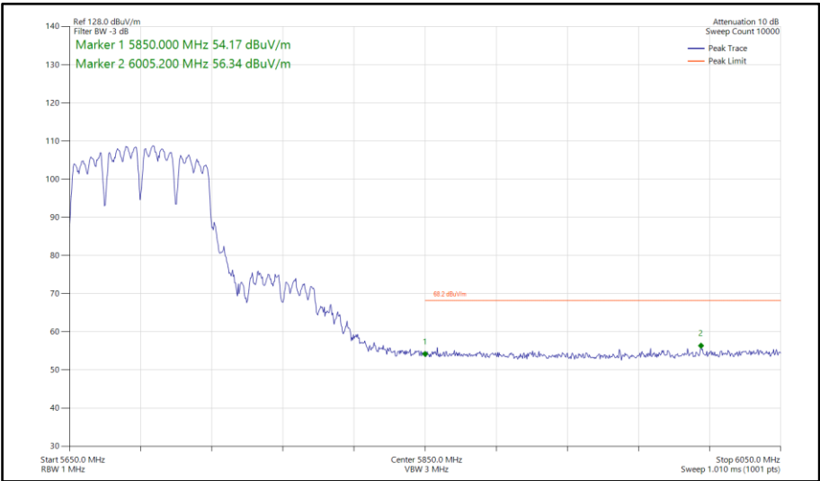
Figure 872 - 802.11a a80, CDD, Core 0-1 - 5690 MHz Band Edge Frequency 5850 MHz
