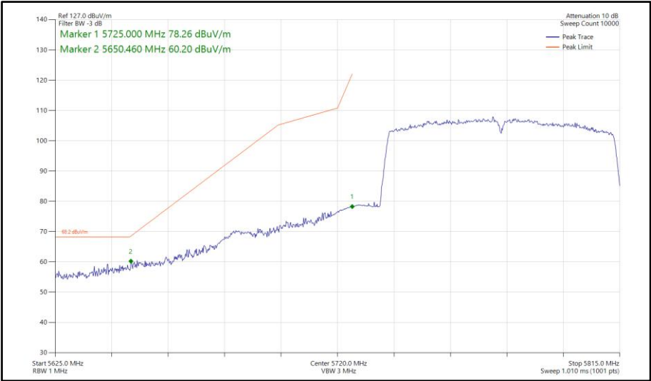
Figure 838 - 802.11ac VHT80, SISO, Core 1 - 5775 MHz Band Edge Frequency 5725 MHz
