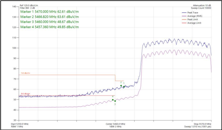
Figure 859 - 802.11ax HE80, SU, CDD, Core 0-1 - 5530 MHz Band Edge Frequency 5470 MHz
