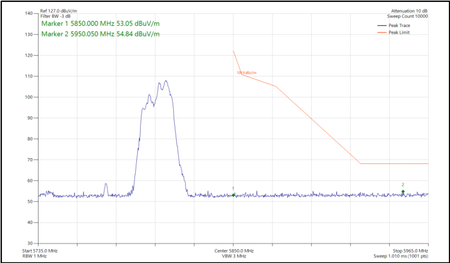
Figure 899 - 802.11ax HE80, RU 106-60, SDM, Core 0-1 - 5775 MHz Band Edge Frequency 5850 MHz
