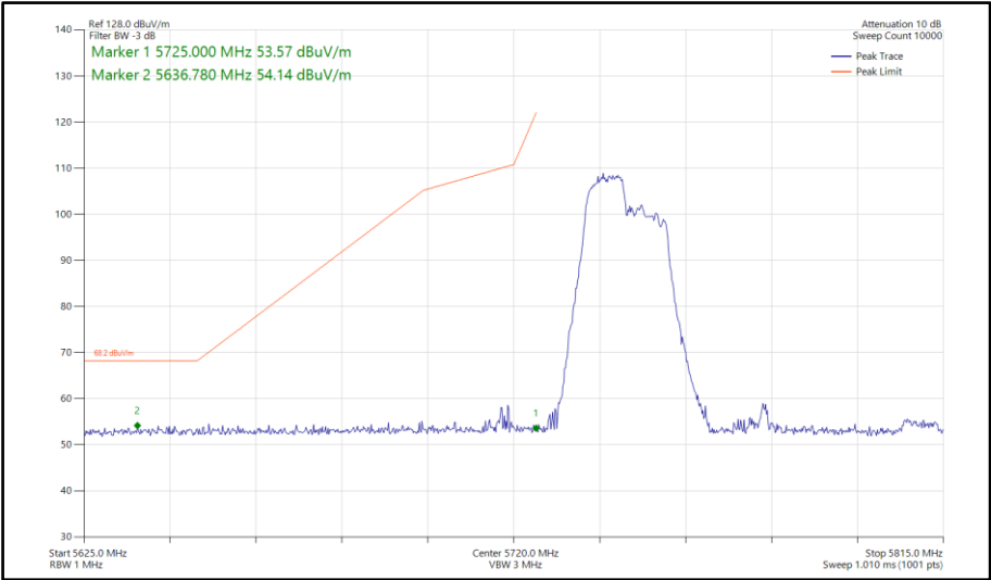
Figure 840 - 802.11ax HE80, RU 106-53, SISO, Core 1 - 5775 MHz Band Edge Frequency 5725 MHz
