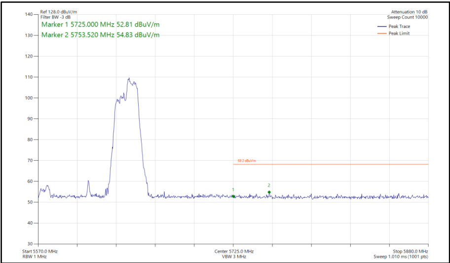
Figure 892 - 802.11ax HE80, RU 106-60, SDM, Core 0-1 - 5610 MHz Band Edge Frequency 5725 MHz
