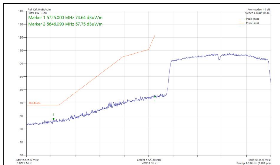
Figure 886 - 802.11ac VHT80, SDM, Core 0-1 - 5775 MHz Band Edge Frequency 5725 MHz
