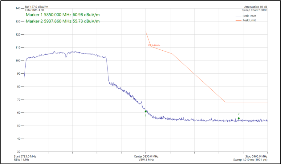
Figure 850 - 802.11ac VHT80, SISO, Core 1 - 5775 MHz Band Edge Frequency 5850 MHz
