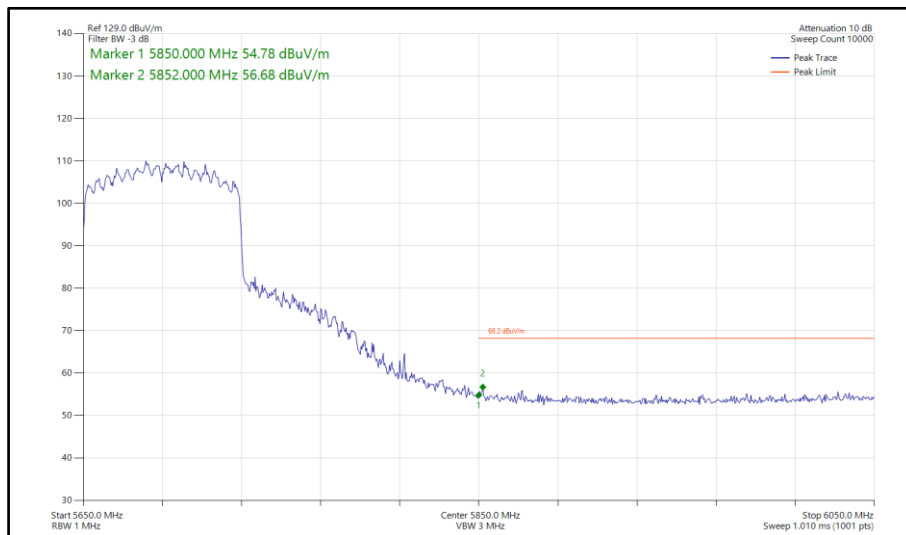
Figure 876 - 802.11ax HE80, SU, CDD, Core 0-1 - 5690 MHz Band Edge Frequency 5850 MHz
