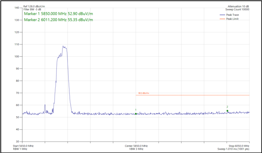
Figure 852 - 802.11ax HE80, RU 106-60, SISO, Core 1 - 5690 MHz Band Edge Frequency 5850 MHz
