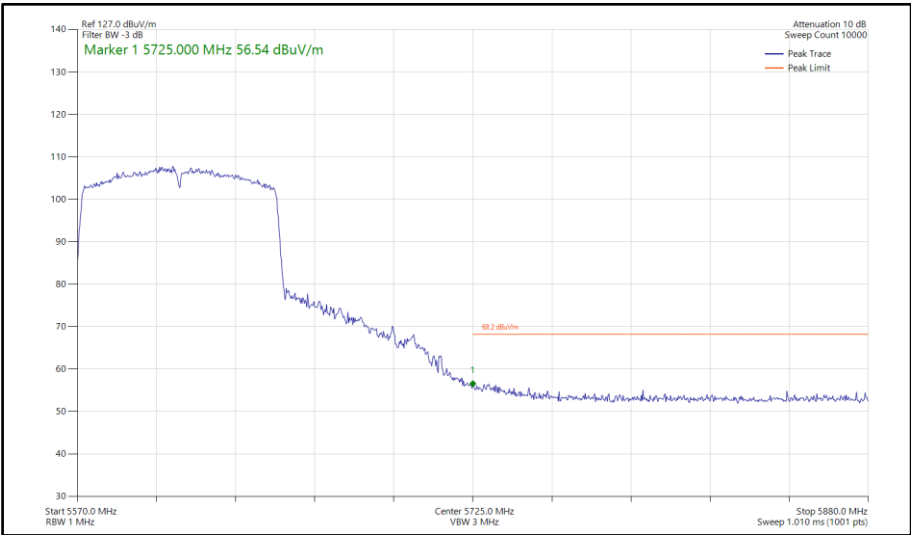
Figure 818 - 802.11ac VHT80, SISO, Core 0 - 5610 MHz Band Edge Frequency 5725 MHz
