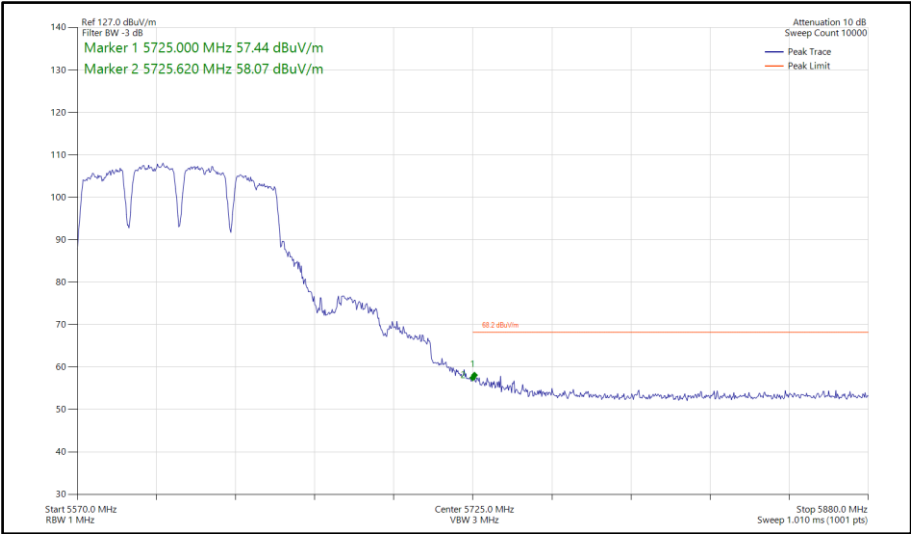
Figure 817 - 802.11a a80, SISO, Core 0 - 5610 MHz Band Edge Frequency 5725 MHz
