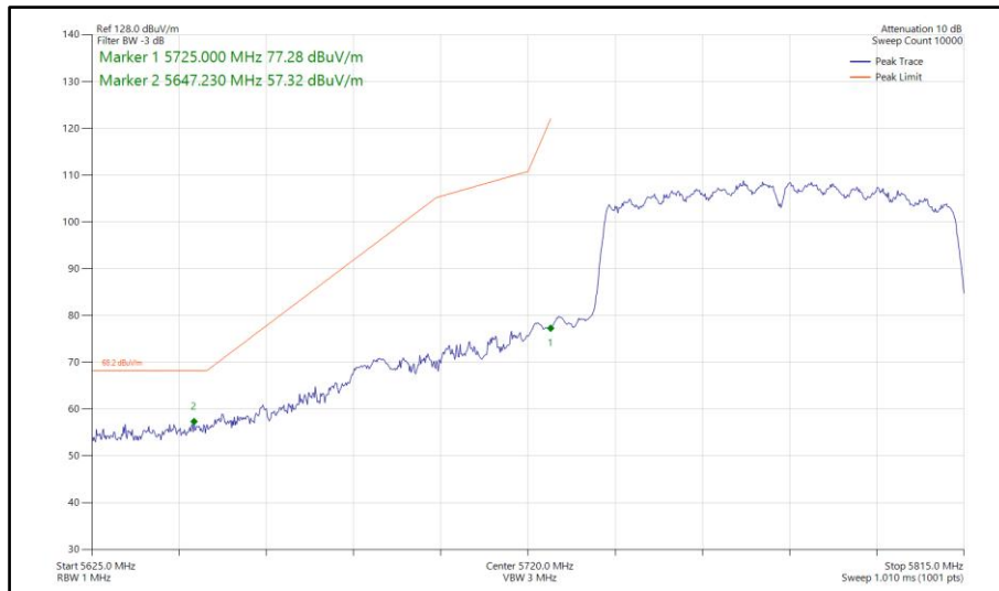
Figure 863 - 802.11ac VHT80, CDD, Core 0-1 - 5775 MHz Band Edge Frequency 5725 MHz
