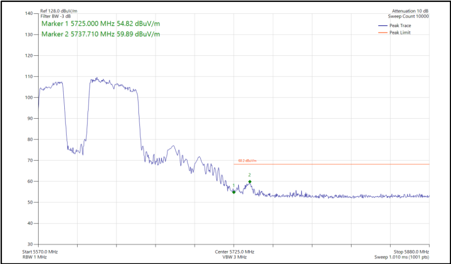
Figure 871 - 802.11be EHT80, RU 484+242-91, CDD, Core 0-1 - 5610 MHz Band Edge Frequency 5725 MHz
