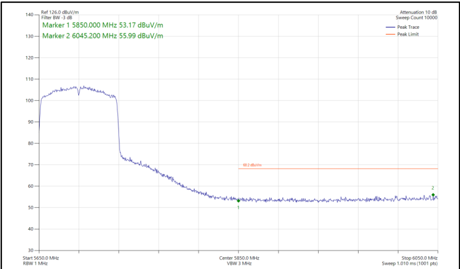
Figure 849 - 802.11ac VHT80, SISO, Core 1 - 5690 MHz Band Edge Frequency 5850 MHz
