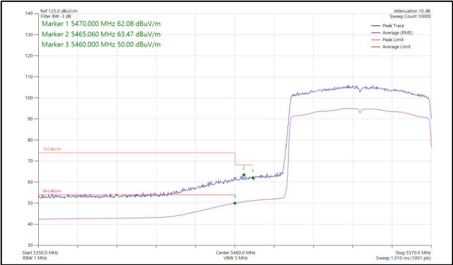
Figure 834 - 802.11ax HE80, SU, SISO, Core 1 - 5530 MHz Band Edge Frequency 5470 MHz
