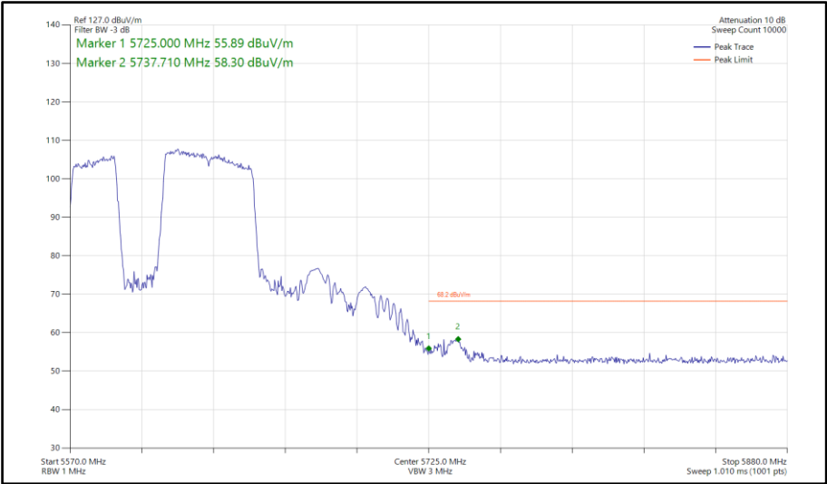
Figure 846 - 802.11be EHT80, RU 484+242-91, SISO, Core 1 - 5610 MHz Band Edge Frequency 5725 MHz
