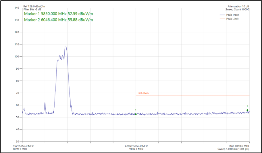
Figure 897 - 802.11ax HE80, RU 52-52, SDM, Core 0-1 - 5690 MHz Band Edge Frequency 5850 MHz
