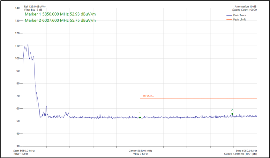
Figure 877 - 802.11ax HE80, RU 106-53, CDD, Core 0-1 - 5690 MHz Band Edge Frequency 5850 MHz
