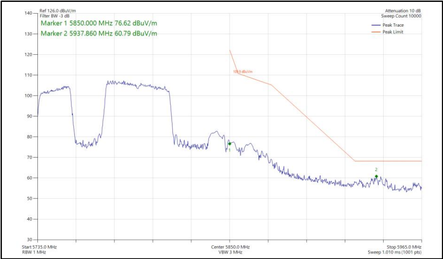
Figure 831 - 802.11be EHT80, RU 484+242-91, SISO, Core 0 - 5775 MHz Band Edge Frequency 5850 MHz
