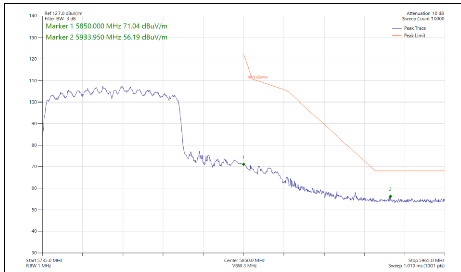
Figure 875 - 802.11ac VHT80, CDD, Core 0-1 - 5775 MHz Band Edge Frequency 5850 MHz
