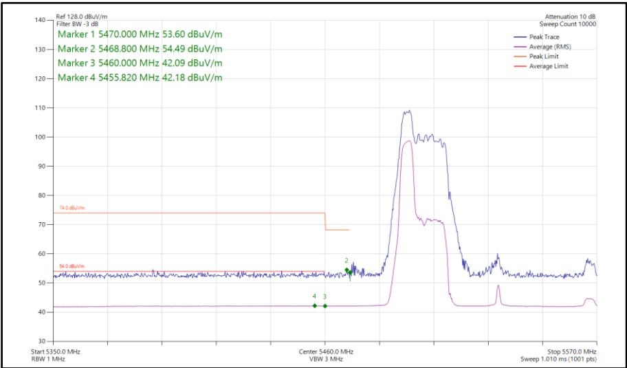
Figure 835 - 802.11ax HE80, RU 52-37, SISO, Core 1 - 5530 MHz Band Edge Frequency 5470 MHz
