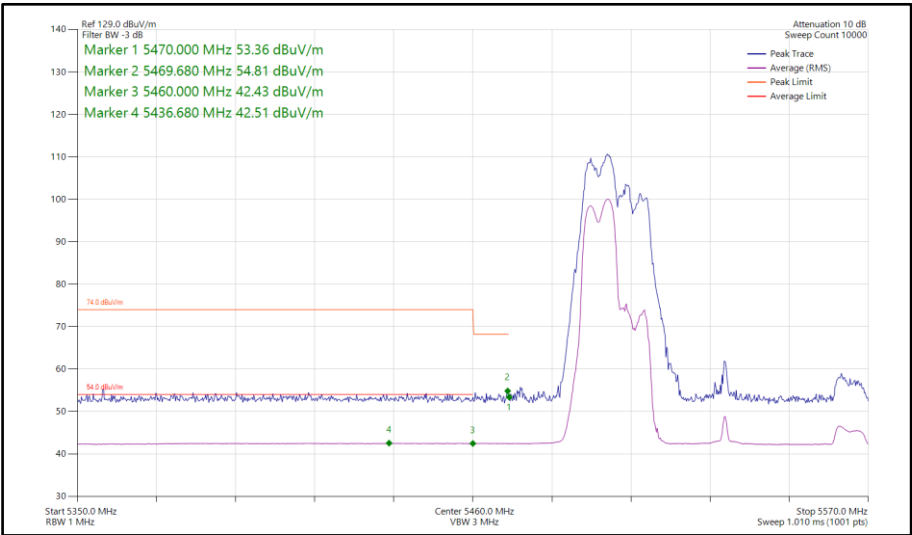
Figure 860 - 802.11ax HE80, RU 106-53, CDD, Core 0-1 - 5530 MHz Band Edge Frequency 5470 MHz
