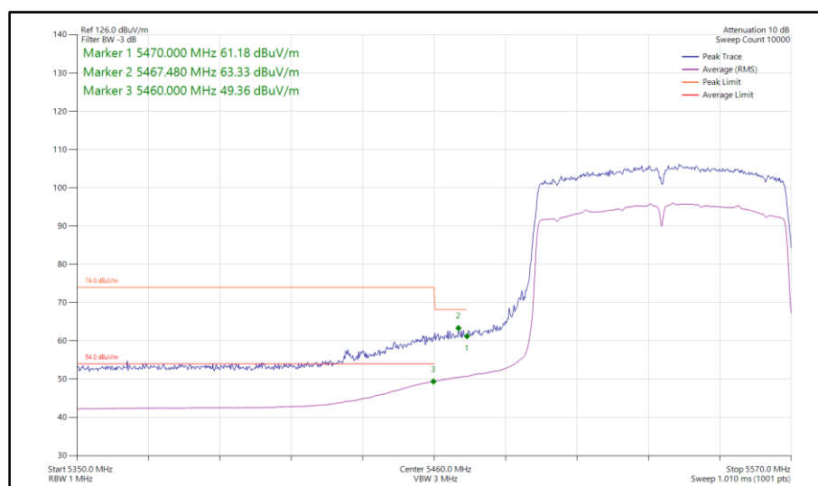
Figure 882 - 802.11ac VHT80, SDM, Core 0-1 - 5530 MHz Band Edge Frequency 5470 MHz
