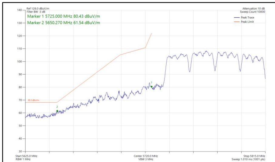
Figure 862 - 802.11a a80, CDD, Core 0-1 - 5775 MHz Band Edge Frequency 5725 MHz
