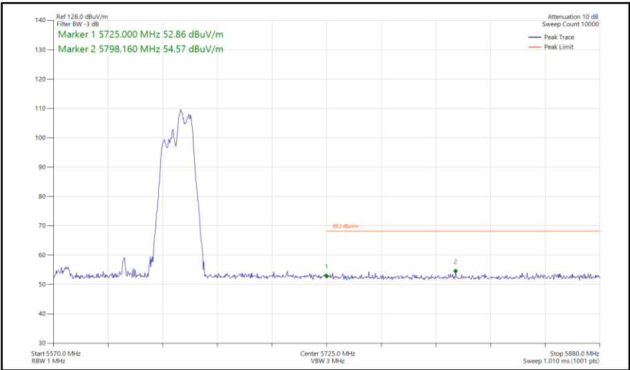
Figure 870 - 802.11ax HE80, RU 106-60, CDD, Core 0-1 - 5610 MHz Band Edge Frequency 5725 MHz
