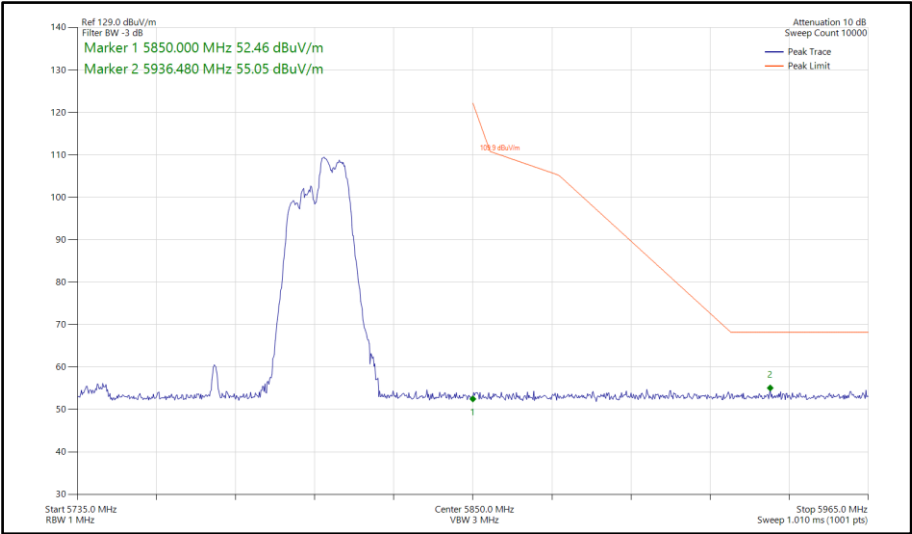
Figure 879 - 802.11ax HE80, RU 106-60, CDD, Core 0-1 - 5775 MHz Band Edge Frequency 5850 MHz
