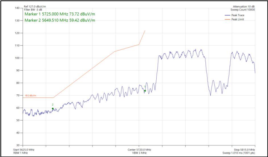
Figure 889 - 802.11be EHT80, RU 484+242-92, SDM, Core 0-1 - 5775 MHz Band Edge Frequency 5725 MHz
