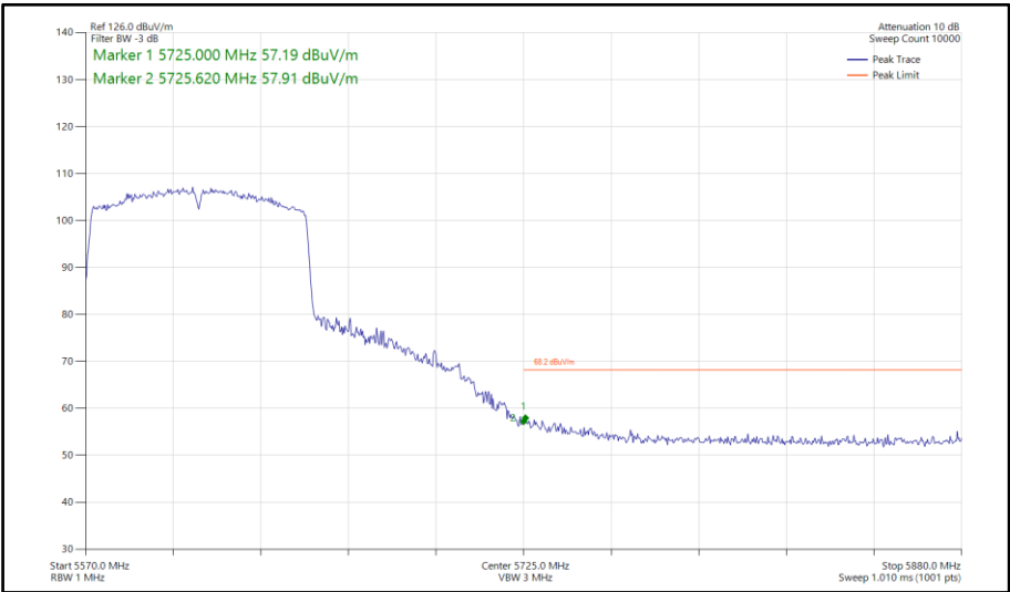
Figure 843 - 802.11ac VHT80, SISO, Core 1 - 5610 MHz Band Edge Frequency 5725 MHz
