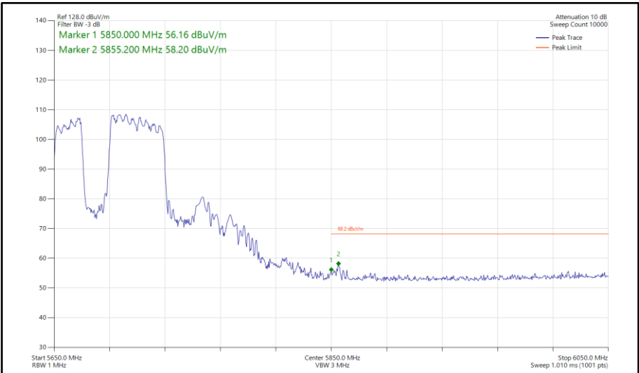
Figure 880 - 802.11be EHT80, RU 484+242-91, CDD, Core 0-1 - 5690 MHz Band Edge Frequency 5850 MHz
