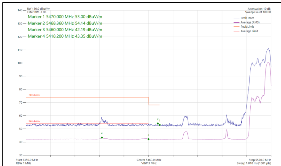
Figure 884 - 802.11ax HE80, RU 52-52, SDM, Core 0-1 - 5530 MHz Band Edge Frequency 5470 MHz
