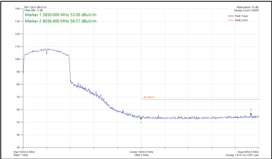
Figure 894 - 802.11ac VHT80, SDM, Core 0-1 - 5690 MHz Band Edge Frequency 5850 MHz
