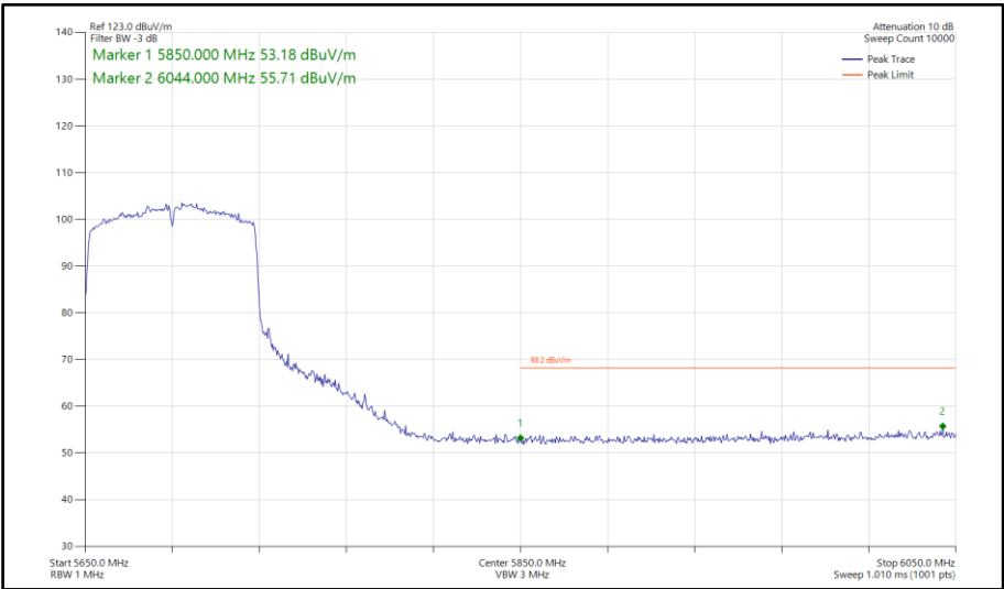
Figure 824 - 802.11ac VHT80, SISO, Core 0 - 5690 MHz Band Edge Frequency 5850 MHz
