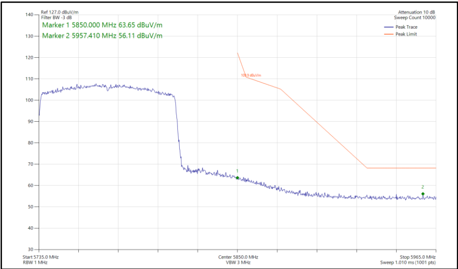
Figure 898 - 802.11ax HE80, SU, SDM, Core 0-1 - 5775 MHz Band Edge Frequency 5850 MHz
