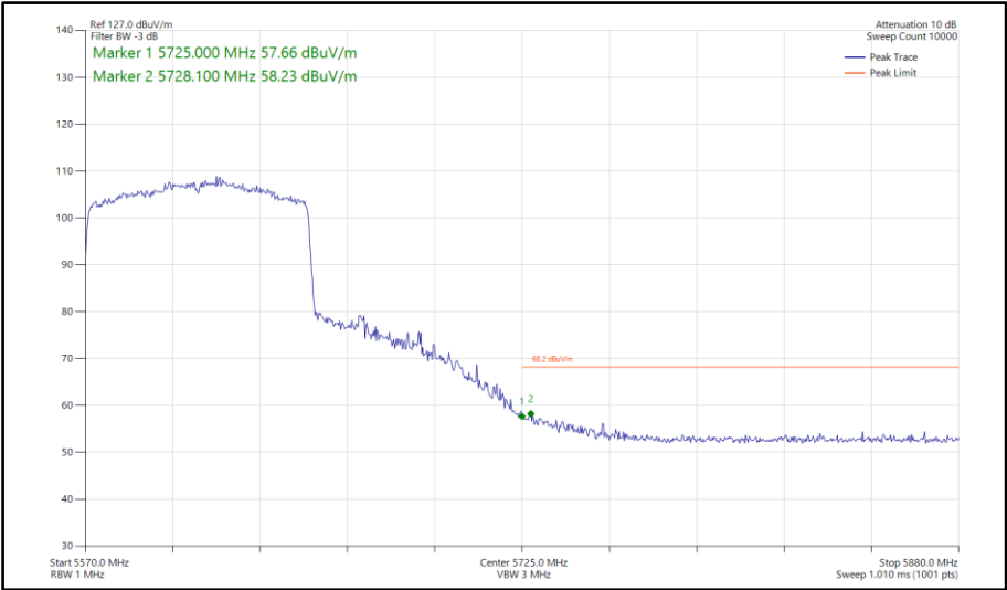
Figure 891 - 802.11ax HE80, SU, SDM, Core 0-1 - 5610 MHz Band Edge Frequency 5725 MHz
