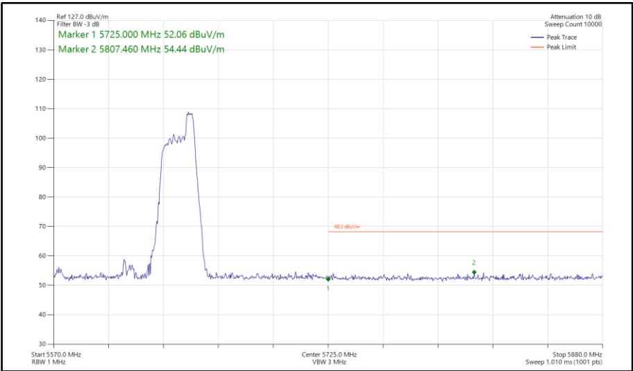
Figure 820 - 802.11ax HE80, RU 52-52, SISO, Core 0 - 5610 MHz Band Edge Frequency 5725 MHz
