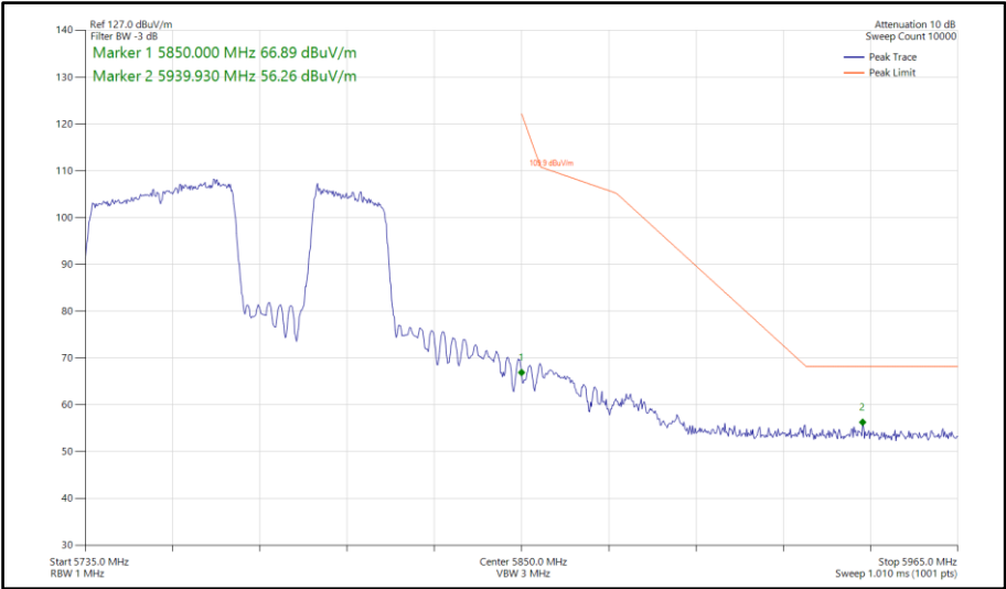
Figure 856 - 802.11be EHT80, RU 484+242-92, SISO, Core 1 - 5775 MHz Band Edge Frequency 5850 MHz
