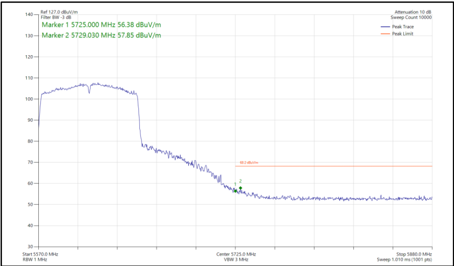
Figure 890 - 802.11ac VHT80, SDM, Core 0-1 - 5610 MHz Band Edge Frequency 5725 MHz
