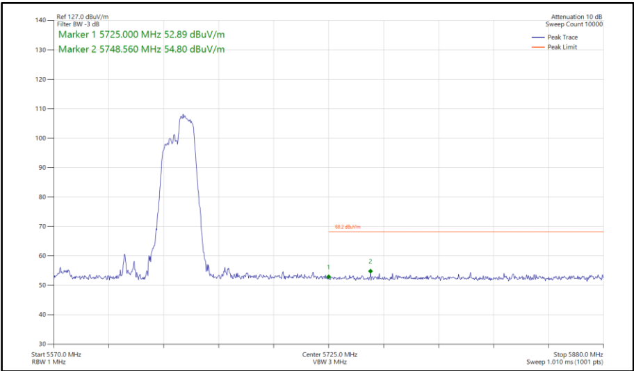
Figure 845 - 802.11ax HE80, RU 106-60, SISO, Core 1 - 5610 MHz Band Edge Frequency 5725 MHz
