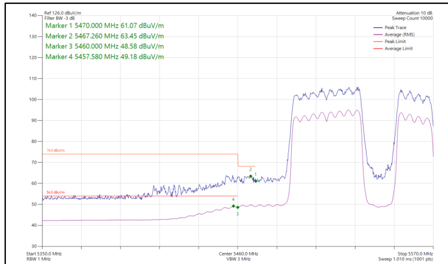
Figure 885 - 802.11be EHT80, RU 484+242-92, SDM, Core 0-1 - 5530 MHz Band Edge Frequency 5470 MHz
