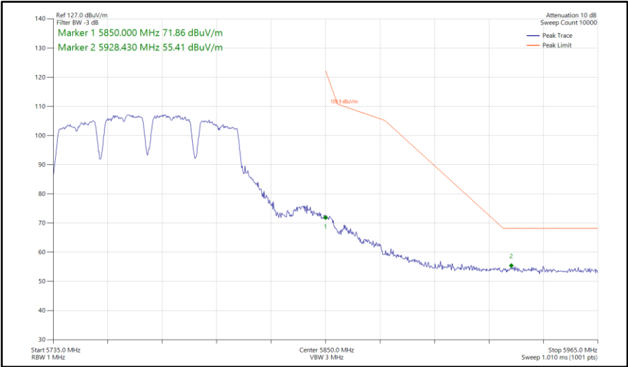
Figure 873 - 802.11a a80, CDD, Core 0-1 - 5775 MHz Band Edge Frequency 5850 MHz
