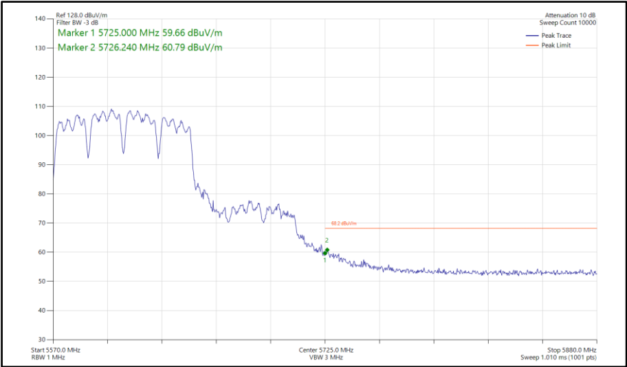
Figure 867 - 802.11a a80, CDD, Core 0-1 - 5610 MHz Band Edge Frequency 5725 MHz
