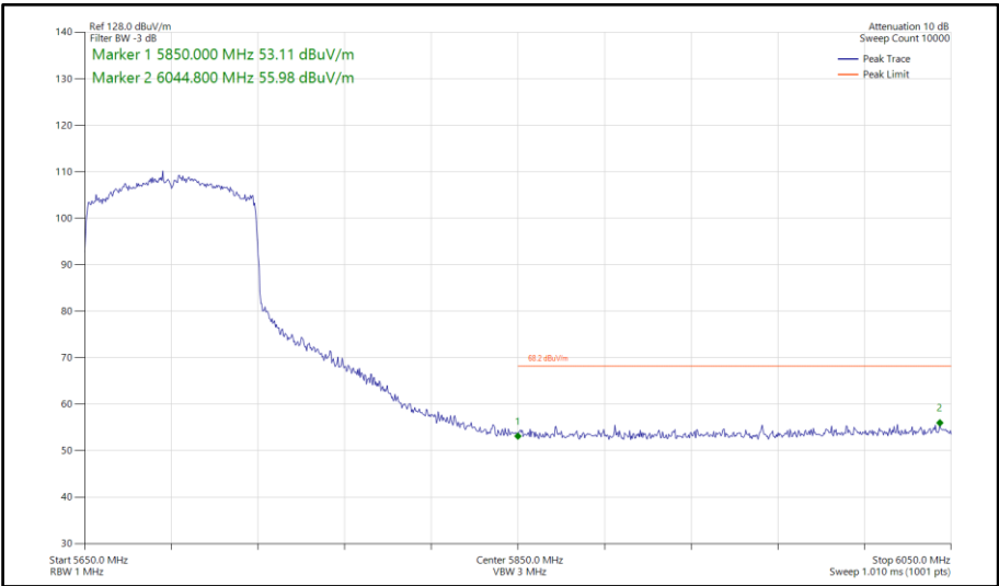
Figure 896 - 802.11ax HE80, SU, SDM, Core 0-1 - 5690 MHz Band Edge Frequency 5850 MHz
