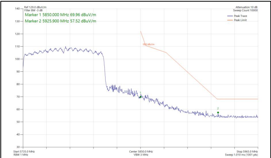
Figure 878 - 802.11ax HE80, SU, CDD, Core 0-1 - 5775 MHz Band Edge Frequency 5850 MHz
