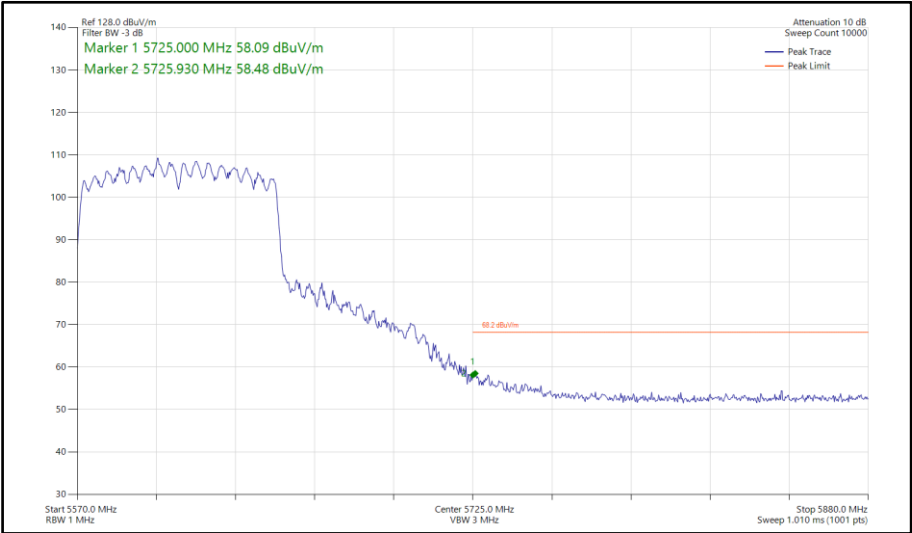
Figure 868 - 802.11ac VHT80, CDD, Core 0-1 - 5610 MHz Band Edge Frequency 5725 MHz
