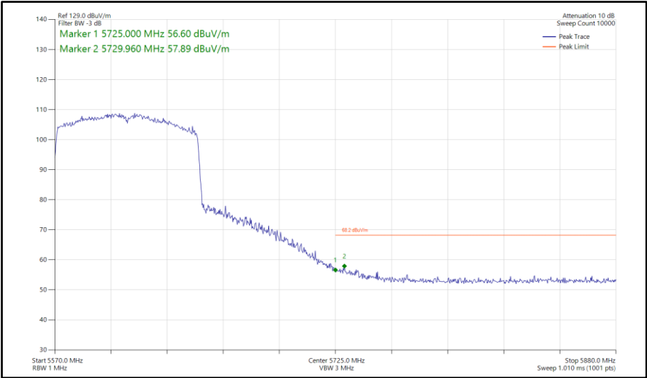
Figure 819 - 802.11ax HE80, SU, SISO, Core 0 - 5610 MHz Band Edge Frequency 5725 MHz
