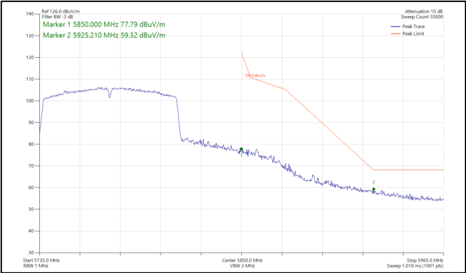
Figure 825 - 802.11ac VHT80, SISO, Core 0 - 5775 MHz Band Edge Frequency 5850 MHz
