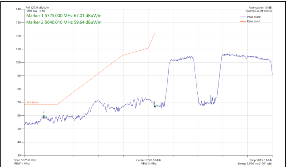
Figure 841 - 802.11be EHT80, RU 484+242-91, SISO, Core 1 - 5775 MHz Band Edge Frequency 5725 MHz
