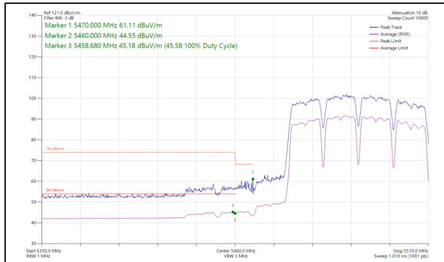
Figure 857 - 802.11a a80, CDD, Core 0-1 - 5530 MHz Band Edge Frequency 5470 MHz
