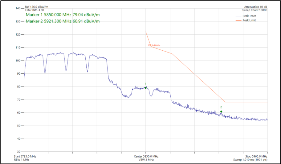
Figure 823 - 802.11a a80, SISO, Core 0 - 5775 MHz Band Edge Frequency 5850 MHz
