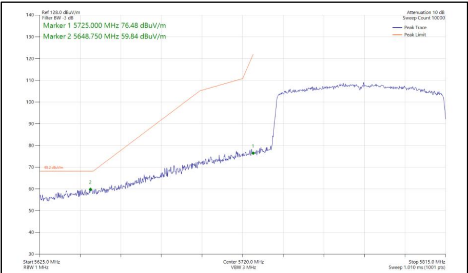
Figure 839 - 802.11ax HE80, SU, SISO, Core 1 - 5775 MHz Band Edge Frequency 5725 MHz
