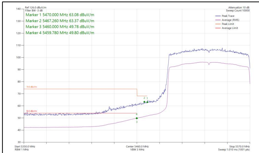
Figure 883 - 802.11ax HE80, SU, SDM, Core 0-1 - 5530 MHz Band Edge Frequency 5470 MHz
