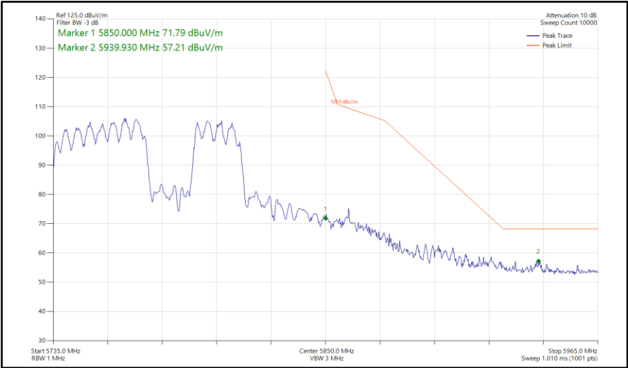
Figure 901 - 802.11be EHT80, RU 484+242-92, SDM, Core 0-1 - 5775 MHz Band Edge Frequency 5850 MHz
