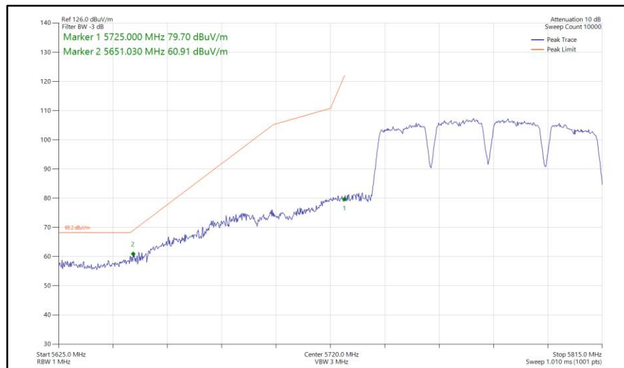
Figure 837 - 802.11a a80, SISO, Core 1 - 5775 MHz Band Edge Frequency 5725 MHz
