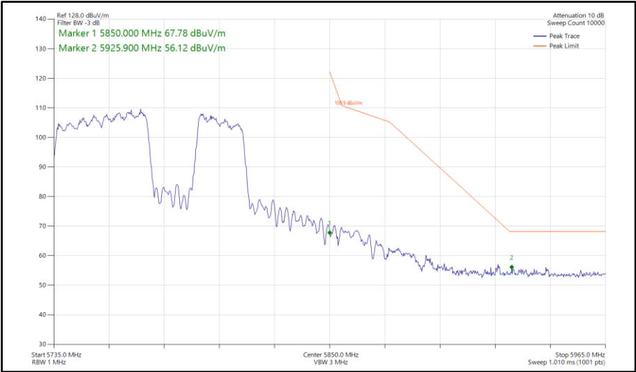
Figure 881 - 802.11be EHT80, RU 484+242-92, CDD, Core 0-1 - 5775 MHz Band Edge Frequency 5850 MHz
