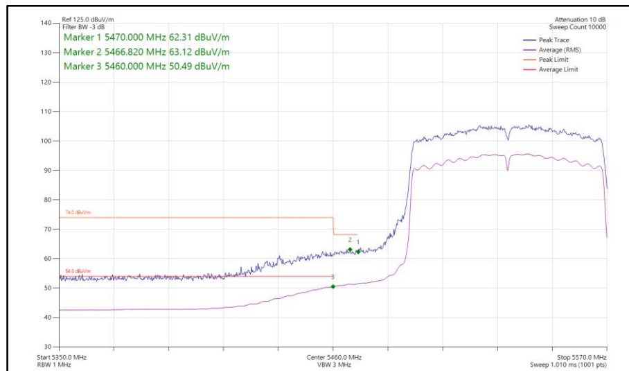
Figure 858 - 802.11ac VHT80, CDD, Core 0-1 - 5530 MHz Band Edge Frequency 5470 MHz
