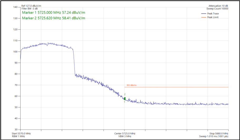
Figure 844 - 802.11ax HE80, SU, SISO, Core 1 - 5610 MHz Band Edge Frequency 5725 MHz
