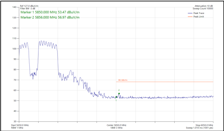
Figure 900 - 802.11be EHT80, RU 484+242-91, SDM, Core 0-1 - 5690 MHz Band Edge Frequency 5850 MHz
