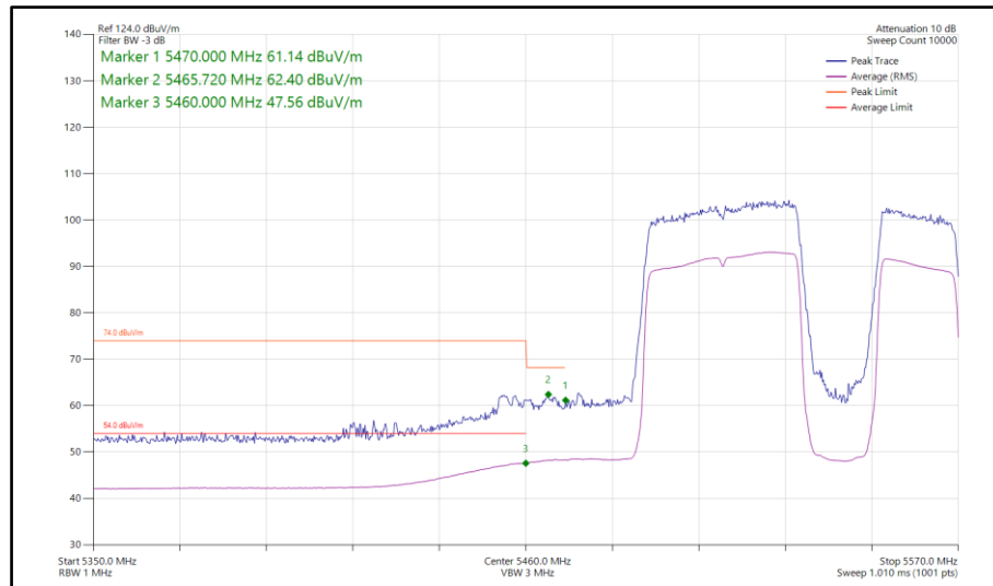
Figure 836 - 802.11be EHT80, RU 484+242-92, SISO, Core 1 - 5530 MHz Band Edge Frequency 5470 MHz
