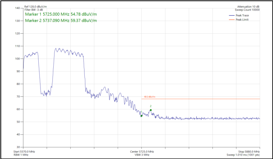
Figure 893 - 802.11be EHT80, RU 484+242-91, SDM, Core 0-1 - 5610 MHz Band Edge Frequency 5725 MHz
