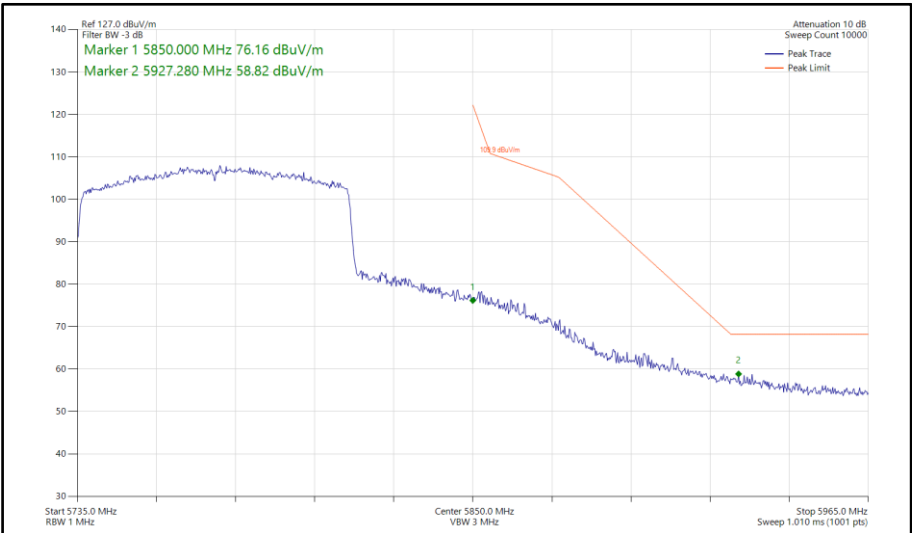
Figure 828 - 802.11ax HE80, SU, SISO, Core 0 - 5775 MHz Band Edge Frequency 5850 MHz
