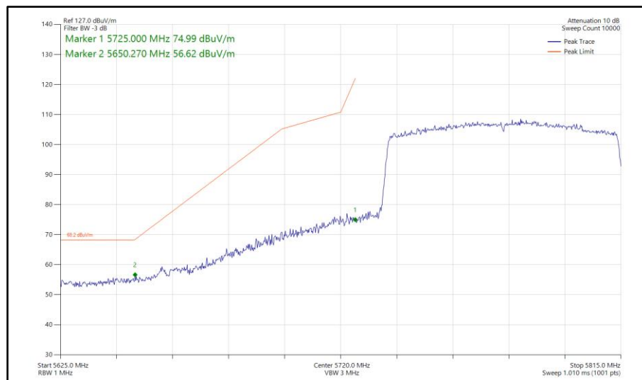
Figure 887 - 802.11ax HE80, SU, SDM, Core 0-1 - 5775 MHz Band Edge Frequency 5725 MHz
