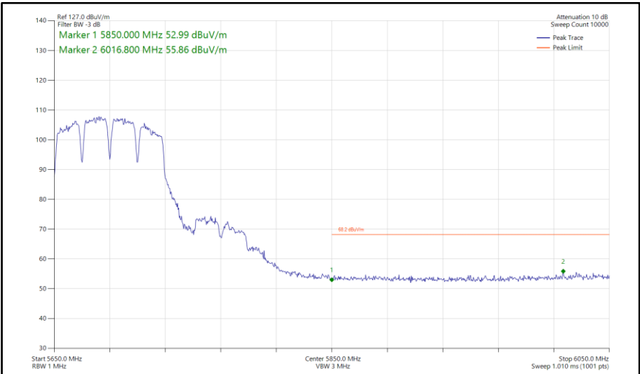
Figure 847 - 802.11a a80, SISO, Core 1 - 5690 MHz Band Edge Frequency 5850 MHz
