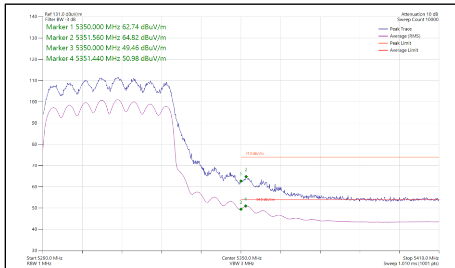
Figure 131 - 802.11ax HE40, SU, CDD, Core 0-1 - 5310 MHz Band Edge Frequency 5350 MHz
