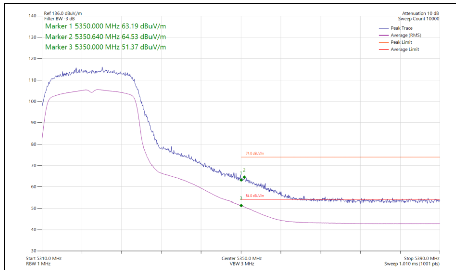
Figure 76 - 802.11ac VHT20, TxBF, Core 0-1 - 5320 MHz Band Edge Frequency 5350 MHz
