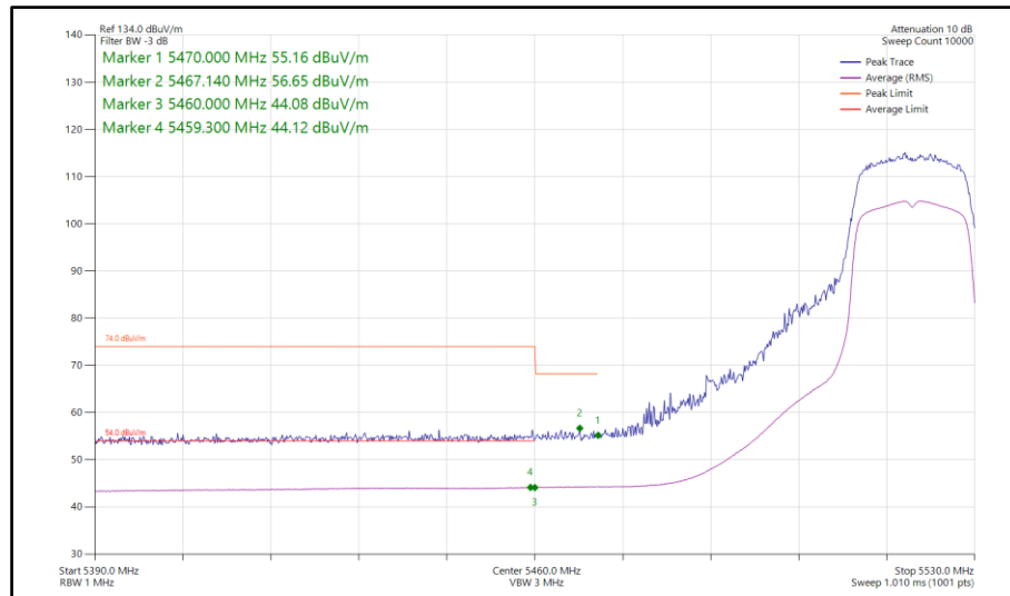
Figure 66 - 802.11n HT20, SDM, Core 0-1 - 5520 MHz Band Edge Frequency 5460 MHz
