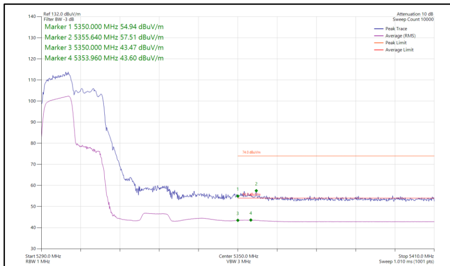
Figure 116 - 802.11ax HE40, RU 106-53, SISO, Core 1 - 5310 MHz Band Edge Frequency 5350 MHz
