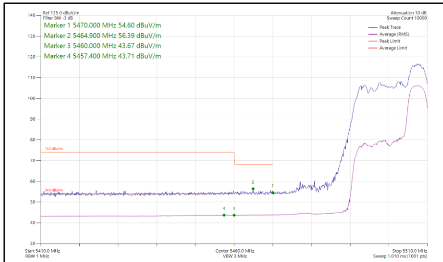
Figure 68 - 802.11ax HE20, RU 52-40, SDM, Core 0-1 - 5500 MHz Band Edge Frequency 5460 MHz
