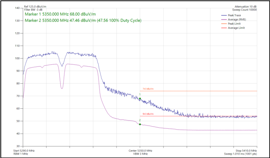
Figure 111 - 802.11a a40, SISO, Core 1 - 5310 MHz Band Edge Frequency 5350 MHz
