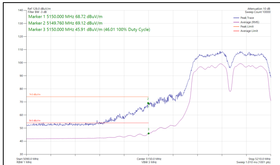
Figure 123 - 802.11a a40, CDD, Core 0-1 - 5190 MHz Band Edge Frequency 5150 MHz
