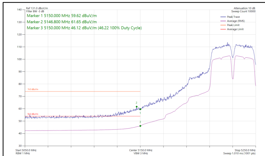
Figure 84 - 802.11a a40, SISO, Core 0 - 5230 MHz Band Edge Frequency 5150 MHz
