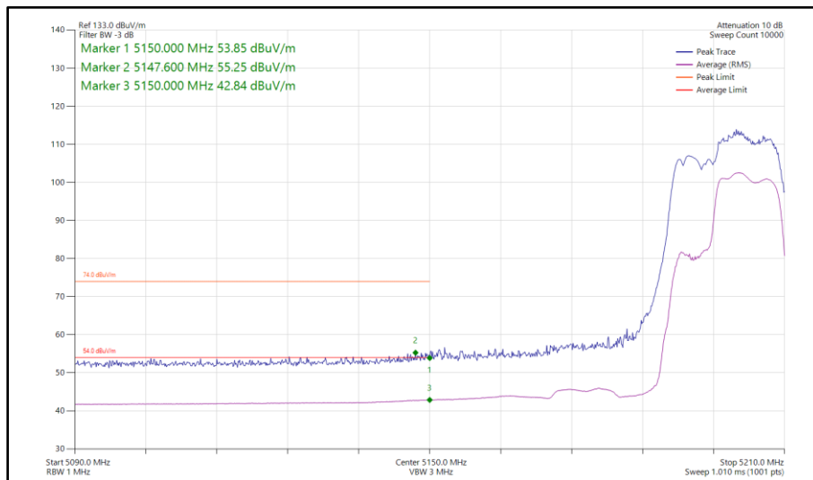
Figure 127 - 802.11be EHT40, RU 106+26-85, CDD, Core 0-1 - 5190 MHz Band Edge Frequency 5150 MHz
