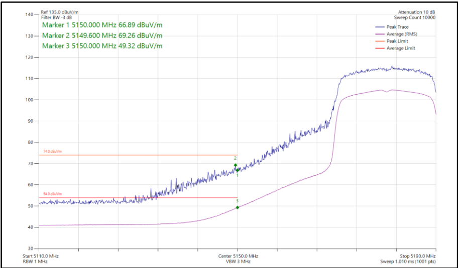
Figure 73 - 802.11ax HE20, SU, TxBF, Core 0-1 - 5180 MHz Band Edge Frequency 5150 MHz
