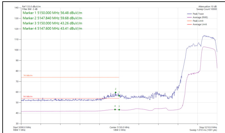
Figure 109 - 802.11ax HE40, RU 106-56, SISO, Core 1 - 5190 MHz Band Edge Frequency 5150 MHz
