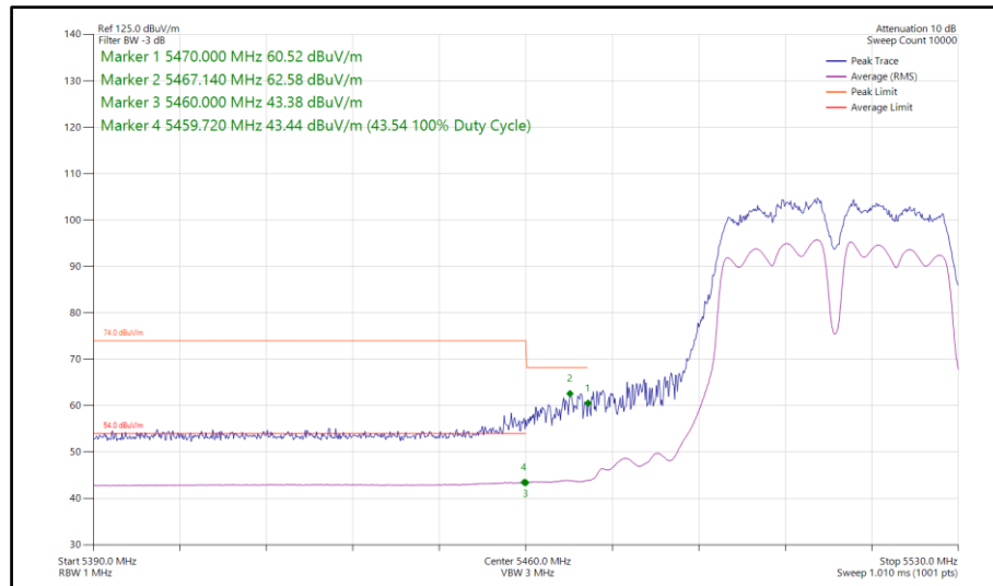
Figure 134 - 802.11a a40, CDD, Core 0-1 - 5510 MHz Band Edge Frequency 5460 MHz
