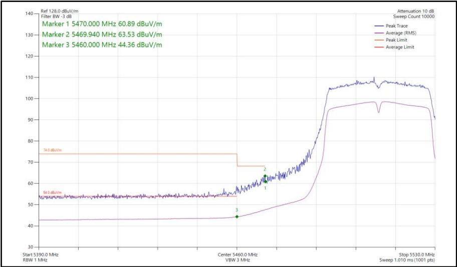
Figure 119 - 802.11n HT40, SISO, Core 1 - 5510 MHz Band Edge Frequency 5460 MHz
