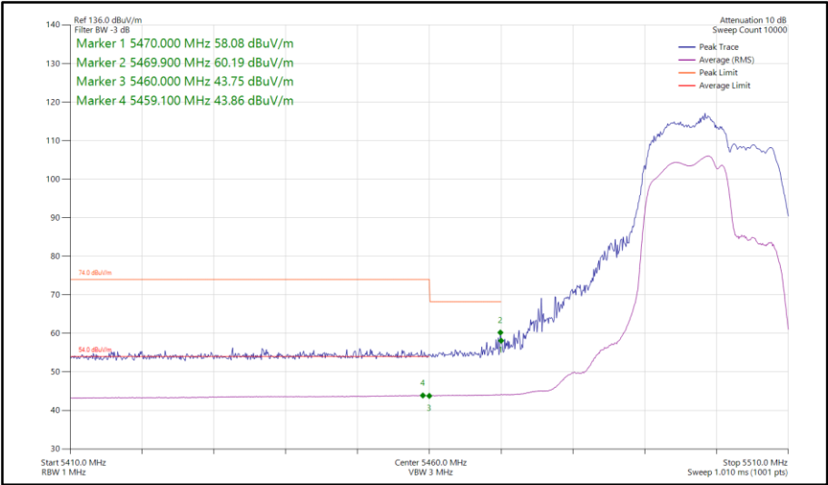
Figure 70 - 802.11be EHT20, RU 106+26-82, SDM, Core 0-1 - 5500 MHz Band Edge Frequency 5460 MHz
