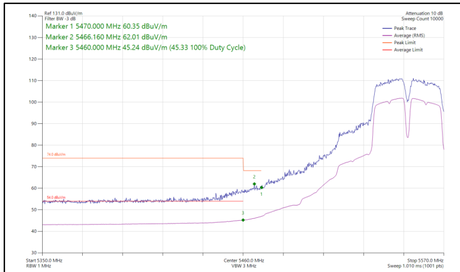
Figure 99 - 802.11a a40, SISO, Core 0 - 5550 MHz Band Edge Frequency 5460 MHz
