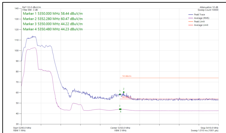
Figure 97 - 802.11be EHT40, RU 52+26-70, SISO, Core 0 - 5310 MHz Band Edge Frequency 5350 MHz
