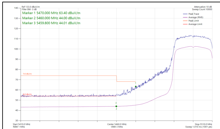
Figure 67 - 802.11ax HE20, SU, SDM, Core 0-1 - 5500 MHz Band Edge Frequency 5460 MHz
