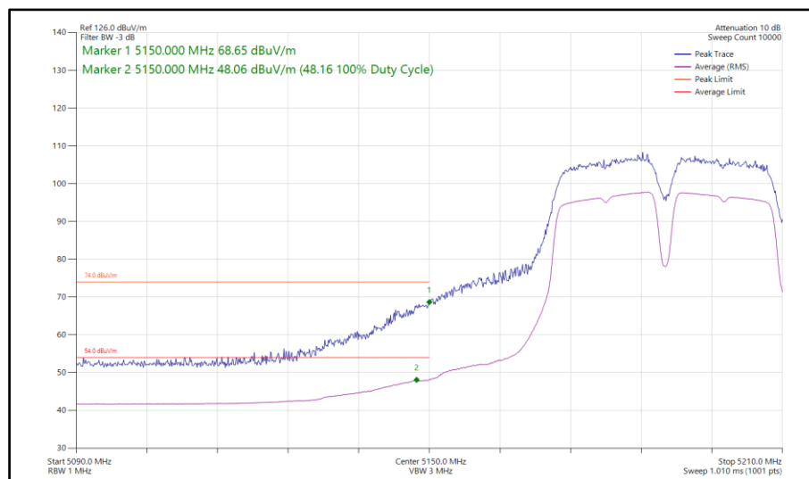
Figure 106 - 802.11a a40, SISO, Core 1 - 5190 MHz Band Edge Frequency 5150 MHz
