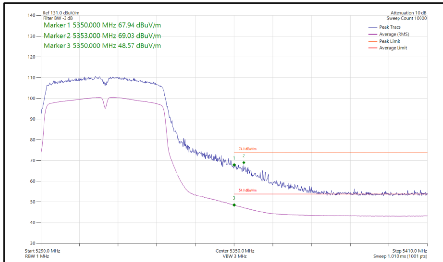
Figure 93 - 802.11n HT40, SISO, Core 0 - 5310 MHz Band Edge Frequency 5350 MHz
