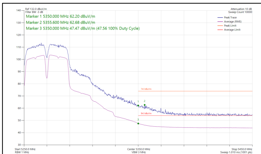
Figure 90 - 802.11a a40, SISO, Core 0 - 5270 MHz Band Edge Frequency 5350 MHz
