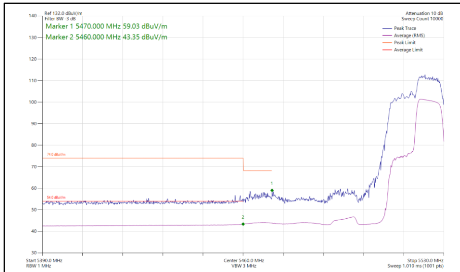
Figure 121 - 802.11ax HE40, RU 106-56, SISO, Core 1 - 5510 MHz Band Edge Frequency 5460 MHz
