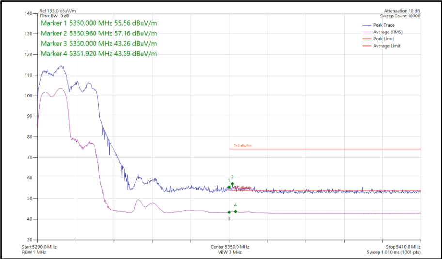
Figure 132 - 802.11ax HE40, RU 106-53, CDD, Core 0-1 - 5310 MHz Band Edge Frequency 5350 MHz
