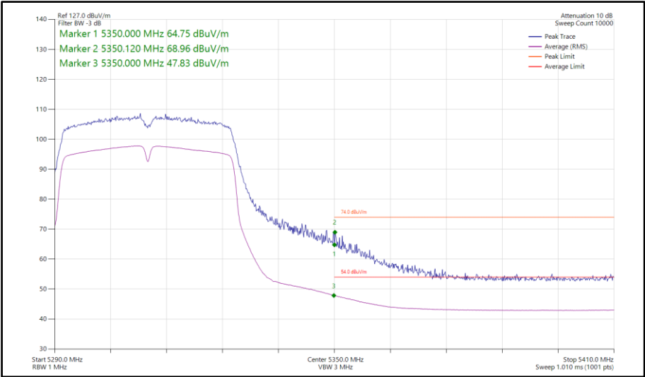
Figure 113 - 802.11n HT40, SISO, Core 1 - 5310 MHz Band Edge Frequency 5350 MHz
