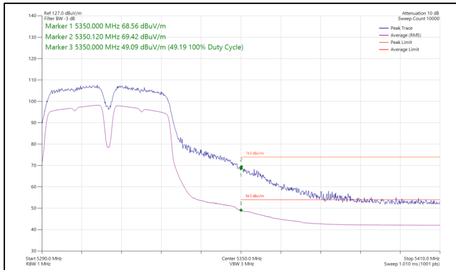
Figure 91 - 802.11a a40, SISO, Core 0 - 5310 MHz Band Edge Frequency 5350 MHz
