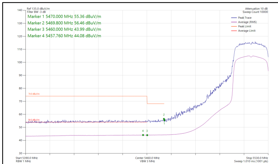
Figure 69 - 802.11ax HE20, SU, SDM, Core 0-1 - 5520 MHz Band Edge Frequency 5460 MHz
