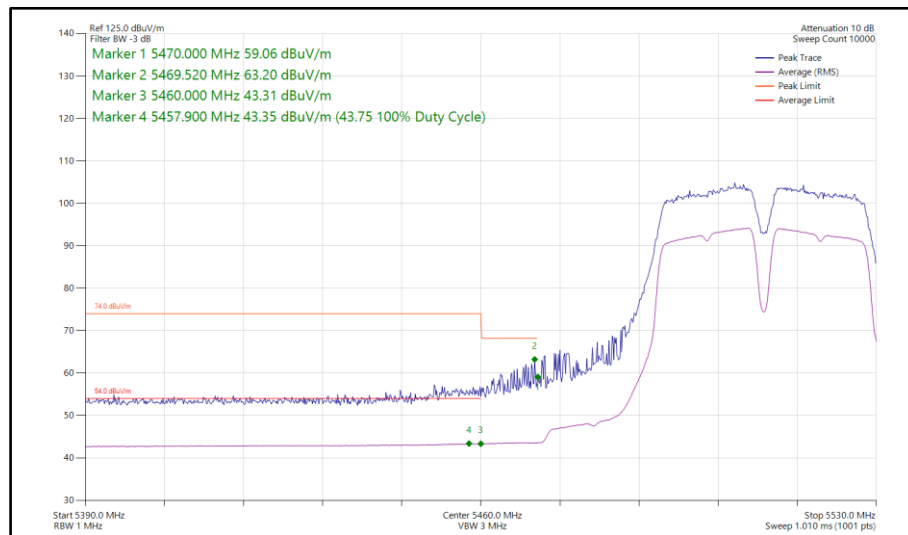
Figure 118 - 802.11a a40, SISO, Core 1 - 5510 MHz Band Edge Frequency 5460 MHz
