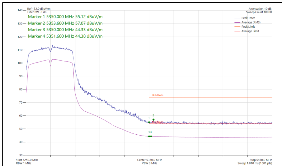
Figure 92 - 802.11n HT40, SISO, Core 0 - 5270 MHz Band Edge Frequency 5350 MHz
