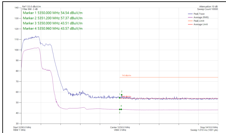
Figure 117 - 802.11be EHT40, RU 106+26-82, SISO, Core 1 - 5310 MHz Band Edge Frequency 5350 MHz
