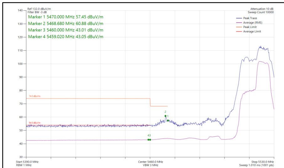
Figure 122 - 802.11be EHT40, RU 52+26-75, SISO, Core 1 - 5510 MHz Band Edge Frequency 5460 MHz
