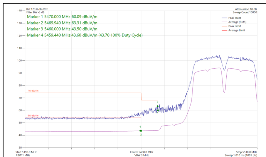
Figure 98 - 802.11a a40, SISO, Core 0 - 5510 MHz Band Edge Frequency 5460 MHz
