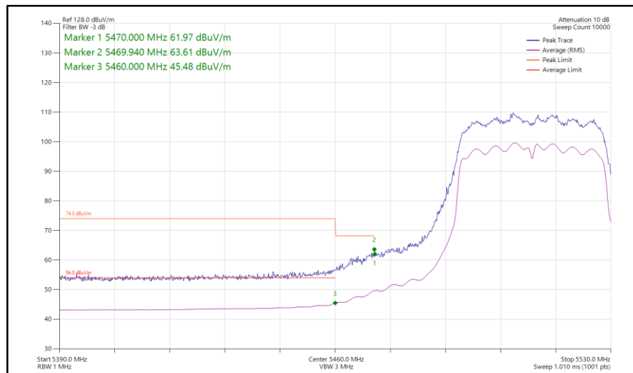
Figure 135 - 802.11n HT40, CDD, Core 0-1 - 5510 MHz Band Edge Frequency 5460 MHz
