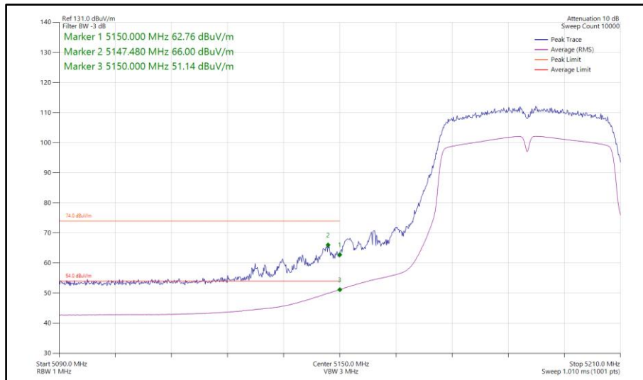
Figure 85 - 802.11n HT40, SISO, Core 0 - 5190 MHz Band Edge Frequency 5150 MHz
