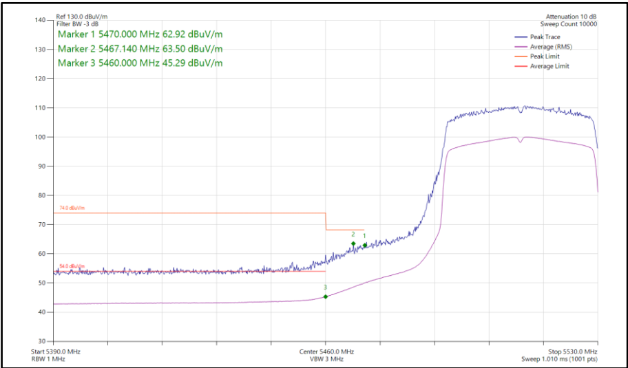
Figure 120 - 802.11ax HE40, SU, SISO, Core 1 - 5510 MHz Band Edge Frequency 5460 MHz
