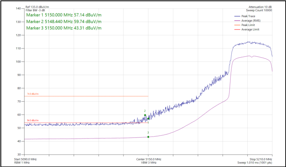
Figure 74 - 802.11ax HE20, SU, TxBF, Core 0-1 - 5200 MHz Band Edge Frequency 5150 MHz
