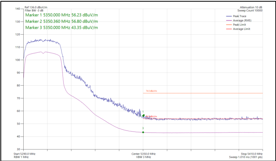
Figure 75 - 802.11ac VHT20, TxBF, Core 0-1 - 5300 MHz Band Edge Frequency 5350 MHz
