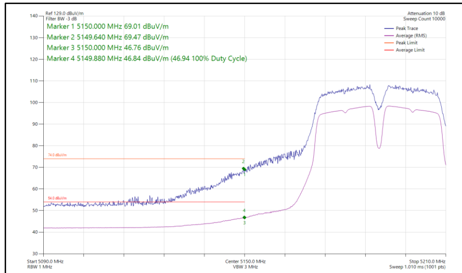
Figure 83 - 802.11a a40, SISO, Core 0 - 5190 MHz Band Edge Frequency 5150 MHz
