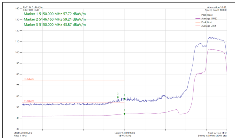
Figure 110 - 802.11be EHT40, RU 106+26-85, SISO, Core 1 - 5190 MHz Band Edge Frequency 5150 MHz
