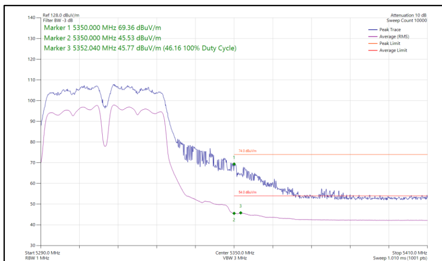
Figure 129 - 802.11a a40, CDD, Core 0-1 - 5310 MHz Band Edge Frequency 5350 MHz
