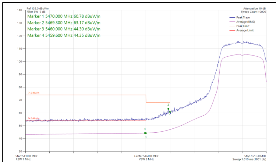
Figure 79 - 802.11ac VHT20, TxBF, Core 0-1 - 5500 MHz Band Edge Frequency 5460 MHz
