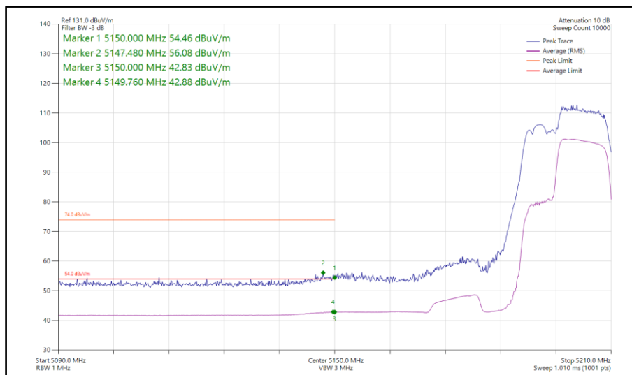
Figure 89 - 802.11be EHT40, RU 106+26-85, SISO, Core 0 - 5190 MHz Band Edge Frequency 5150 MHz
