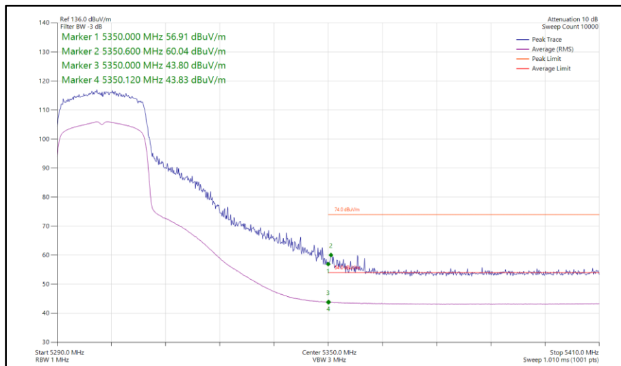
Figure 77 - 802.11ax HE20, SU, TxBF, Core 0-1 - 5300 MHz Band Edge Frequency 5350 MHz
