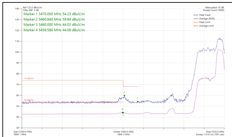
Figure 103 - 802.11ax HE40, RU 52-44, SISO, Core 0 - 5510 MHz Band Edge Frequency 5460 MHz
