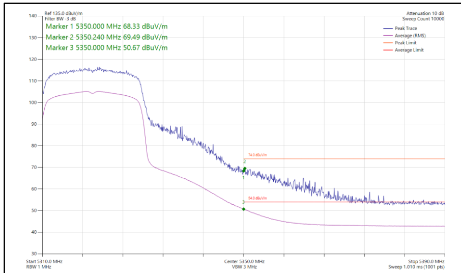
Figure 78 - 802.11ax HE20, SU, TxBF, Core 0-1 - 5320 MHz Band Edge Frequency 5350 MHz
