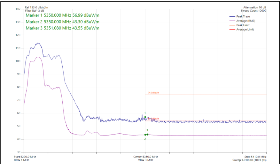
Figure 133 - 802.11be EHT40, RU 52+26-70, CDD, Core 0-1 - 5310 MHz Band Edge Frequency 5350 MHz
