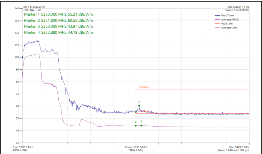
Figure 96 - 802.11ax HE40, RU 106-53, SISO, Core 0 - 5310 MHz Band Edge Frequency 5350 MHz
