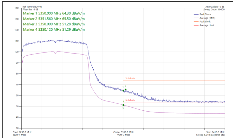
Figure 115 - 802.11ax HE40, SU, SISO, Core 1 - 5310 MHz Band Edge Frequency 5350 MHz
