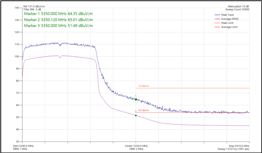
Figure 95 - 802.11ax HE40, SU, SISO, Core 0 - 5310 MHz Band Edge Frequency 5350 MHz
