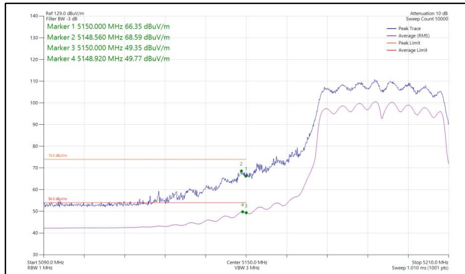
Figure 124 - 802.11n HT40, CDD, Core 0-1 - 5190 MHz Band Edge Frequency 5150 MHz
