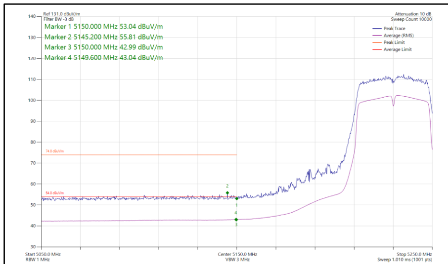
Figure 86 - 802.11n HT40, SISO, Core 0 - 5230 MHz Band Edge Frequency 5150 MHz
