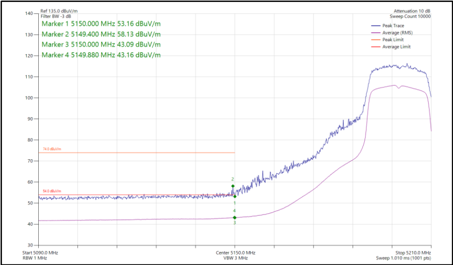
Figure 72 - 802.11ac VHT20, TxBF, Core 0-1 - 5200 MHz Band Edge Frequency 5150 MHz
