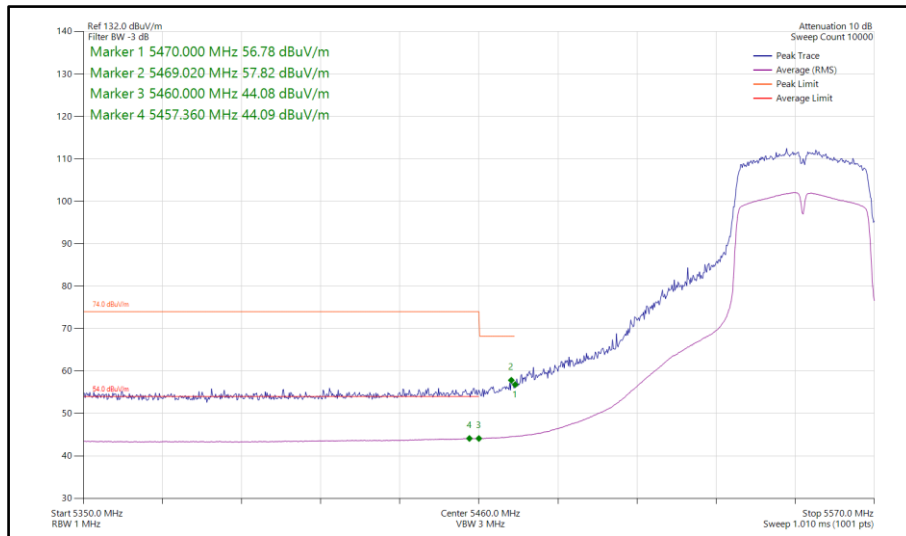
Figure 101 - 802.11n HT40, SISO, Core 0 - 5550 MHz Band Edge Frequency 5460 MHz
