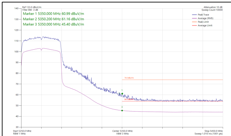
Figure 94 - 802.11ax HE40, SU, SISO, Core 0 - 5270 MHz Band Edge Frequency 5350 MHz
