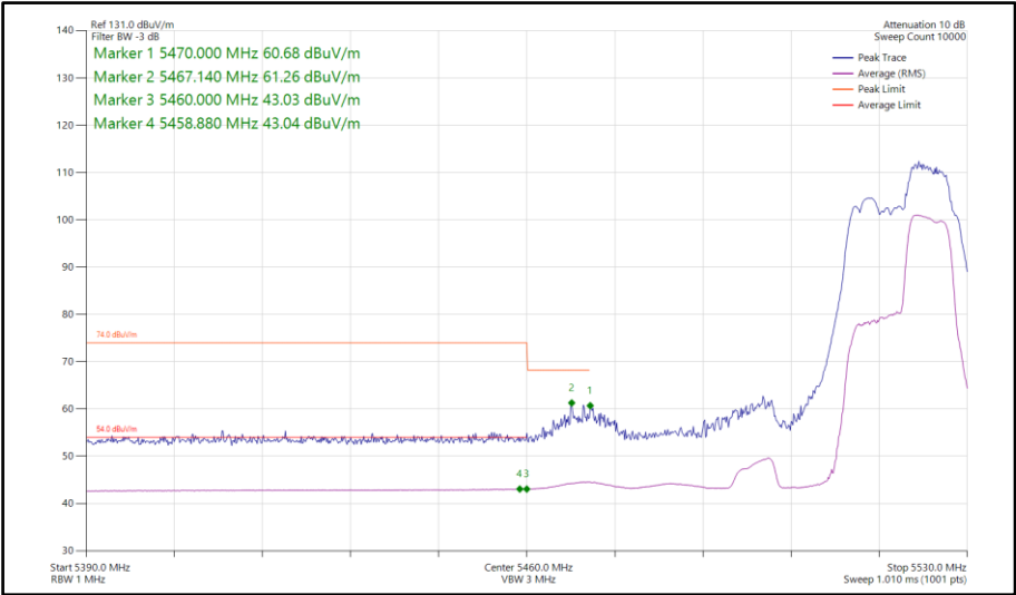
Figure 105 - 802.11be EHT40, RU 52+26-75, SISO, Core 0 - 5510 MHz Band Edge Frequency 5460 MHz
