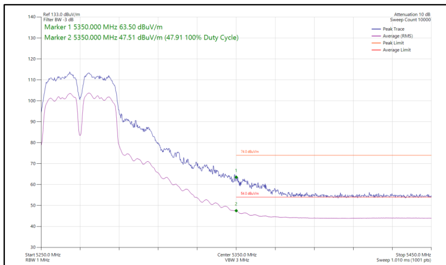
Figure 128 - 802.11a a40, CDD, Core 0-1 - 5270 MHz Band Edge Frequency 5350 MHz
