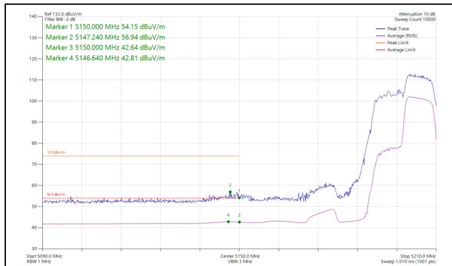
Figure 88 - 802.11ax HE40, RU 106-56, SISO, Core 0 - 5190 MHz Band Edge Frequency 5150 MHz
