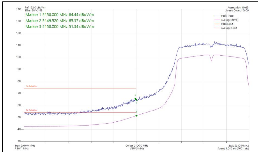
Figure 107 - 802.11n HT40, SISO, Core 1 - 5190 MHz Band Edge Frequency 5150 MHz
