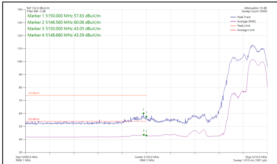
Figure 126 - 802.11ax HE40, RU 106-56, CDD, Core 0-1 - 5190 MHz Band Edge Frequency 5150 MHz
