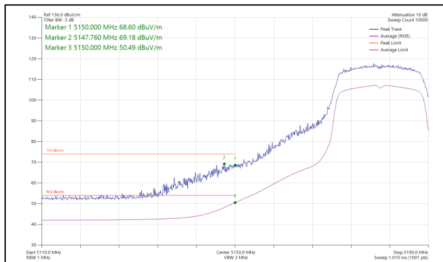
Figure 71 - 802.11ac VHT20, TxBF, Core 0-1 - 5180 MHz Band Edge Frequency 5150 MHz
