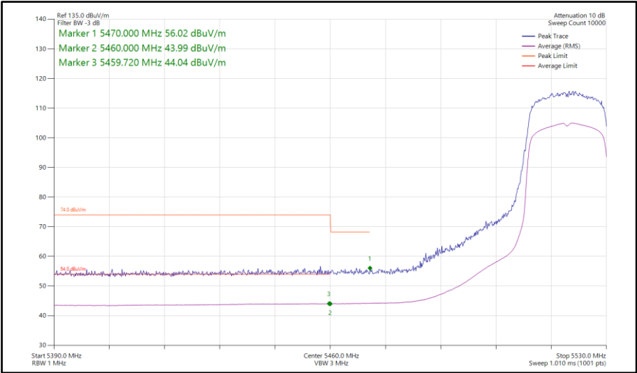
Figure 82 - 802.11ax HE20, SU, TxBF, Core 0-1 - 5520 MHz Band Edge Frequency 5460 MHz
