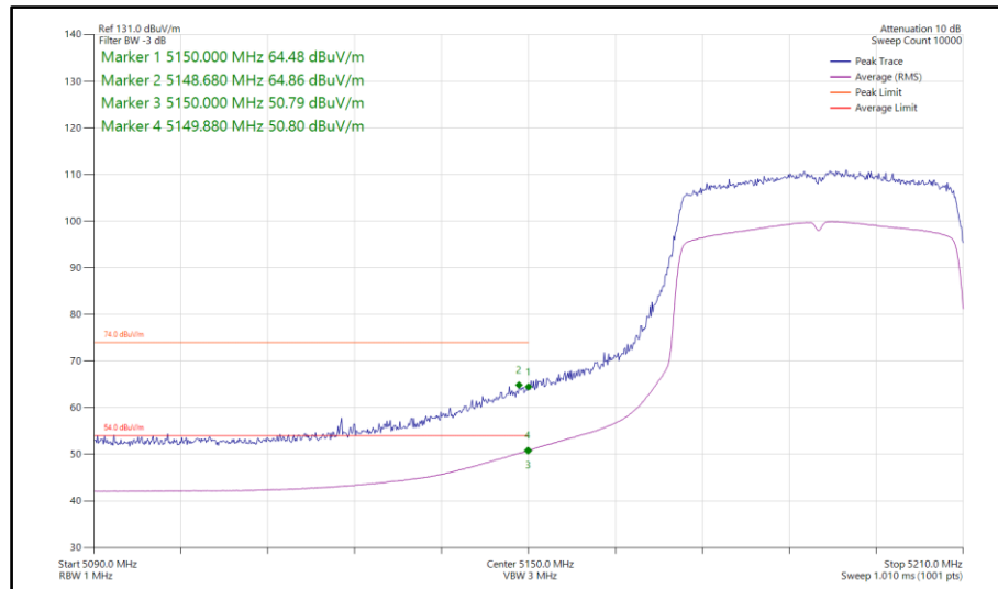
Figure 87 - 802.11ax HE40, SU, SISO, Core 0 - 5190 MHz Band Edge Frequency 5150 MHz
