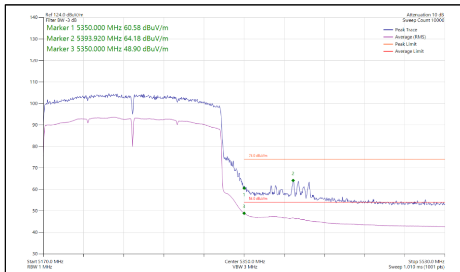
Figure 285 - 802.11ax HE160, SU, TxBF, Core 0-1 - 5250 MHz Band Edge Frequency 5350 MHz
