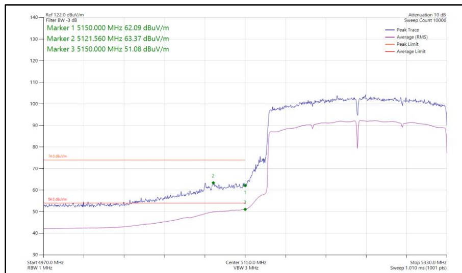
Figure 283 - 802.11ax HE160, SU, TxBF, Core 0-1 - 5250 MHz Band Edge Frequency 5150 MHz
