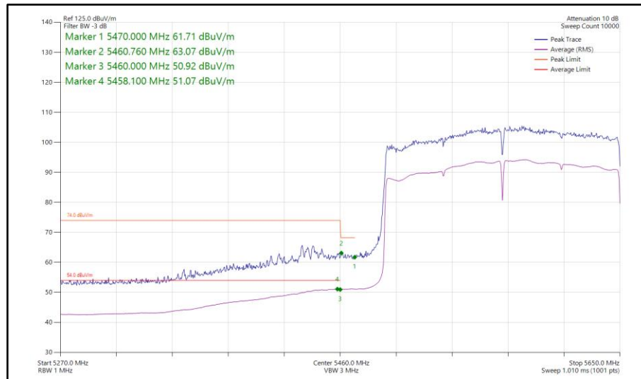
Figure 287 - 802.11ax HE160, SU, TxBF, Core 0-1 - 5570 MHz Band Edge Frequency 5460 MHz
