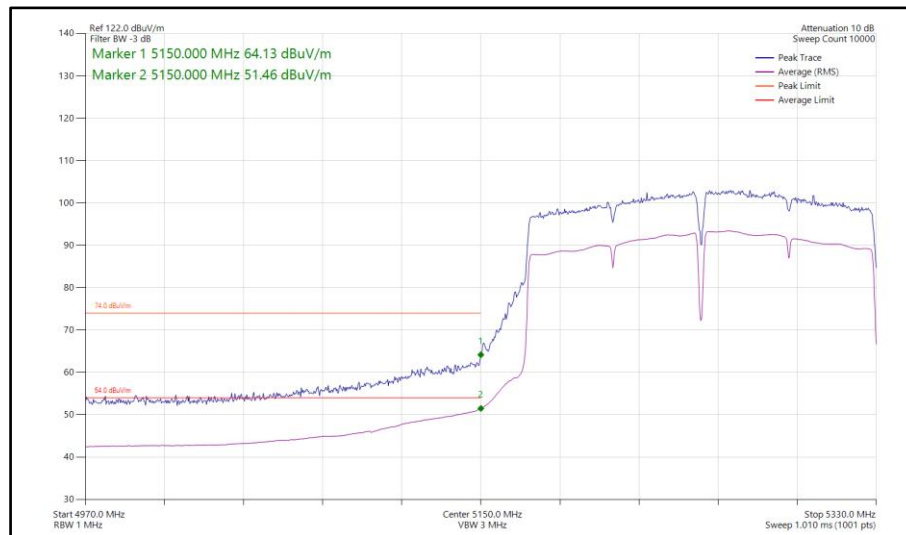
Figure 282 - 802.11ac VHT160, TxBF, Core 0-1 - 5250 MHz Band Edge Frequency 5150 MHz
