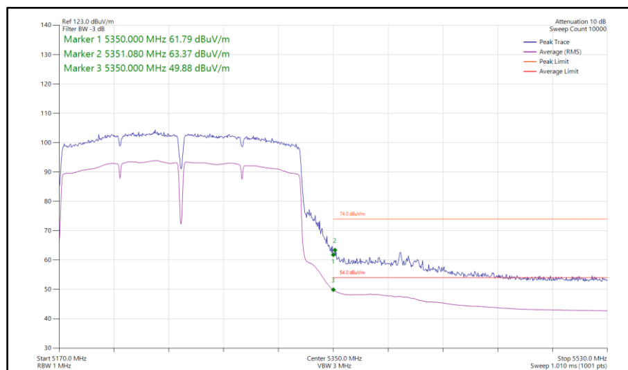
Figure 284 - 802.11ac VHT160, TxBF, Core 0-1 - 5250 MHz Band Edge Frequency 5350 MHz
