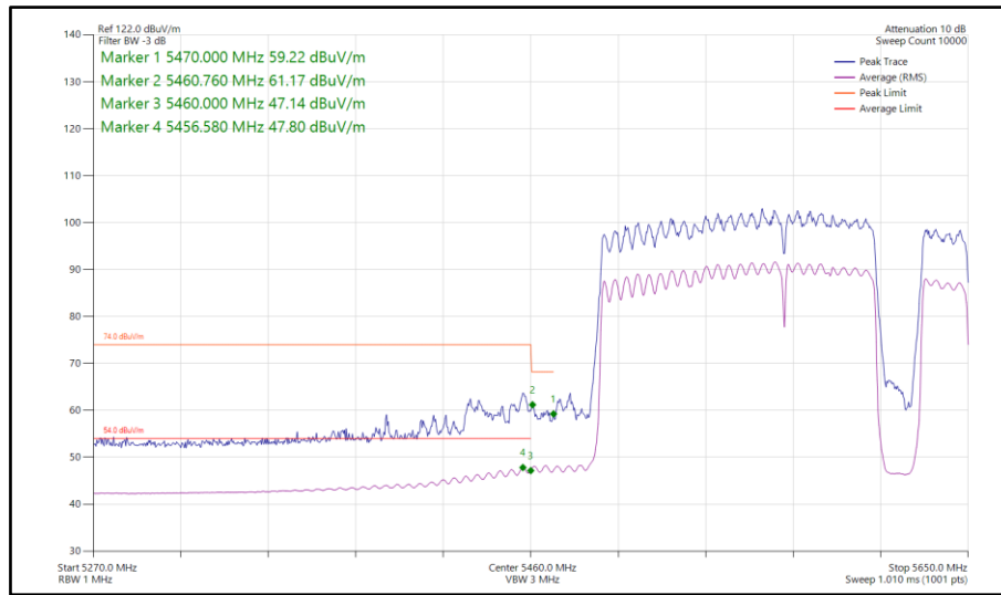
Figure 281 - 802.11be EHT160, RU 996+484+242-98S, SDM, Core 0-1 - 5570 MHz Band Edge Frequency 5460 MHz
