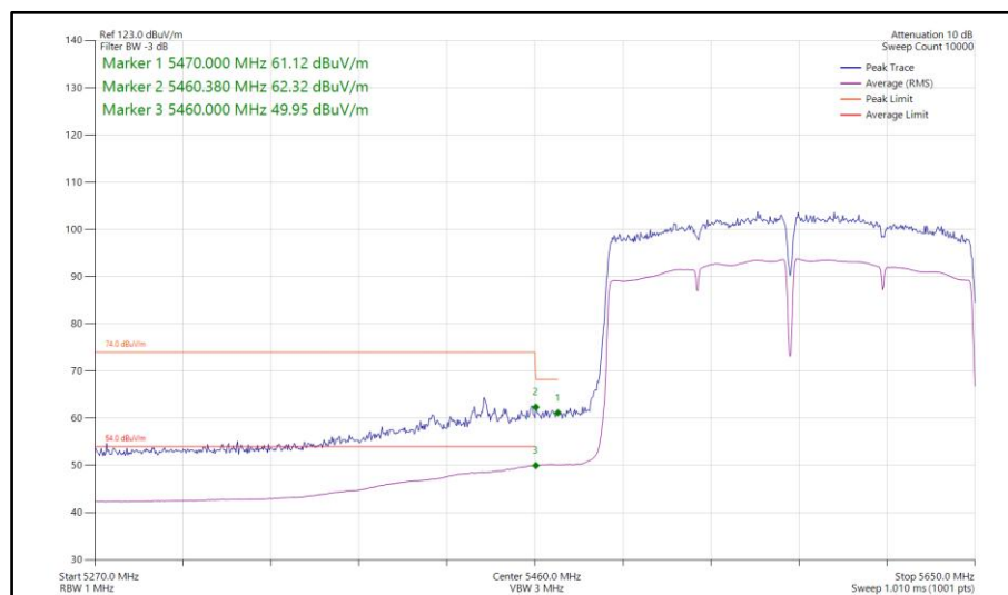
Figure 286 - 802.11ac VHT160, TxBF, Core 0-1 - 5570 MHz Band Edge Frequency 5460 MHz
