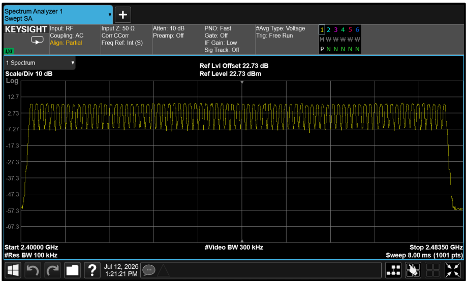
Figure 36 - GFSK (DH5) - Number of Hopping Channels
