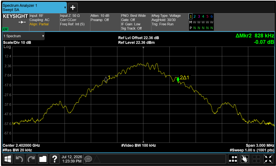
Figure 49 - Core 1 (B) 2402 MHz (CH0) 99% Bandwidth
