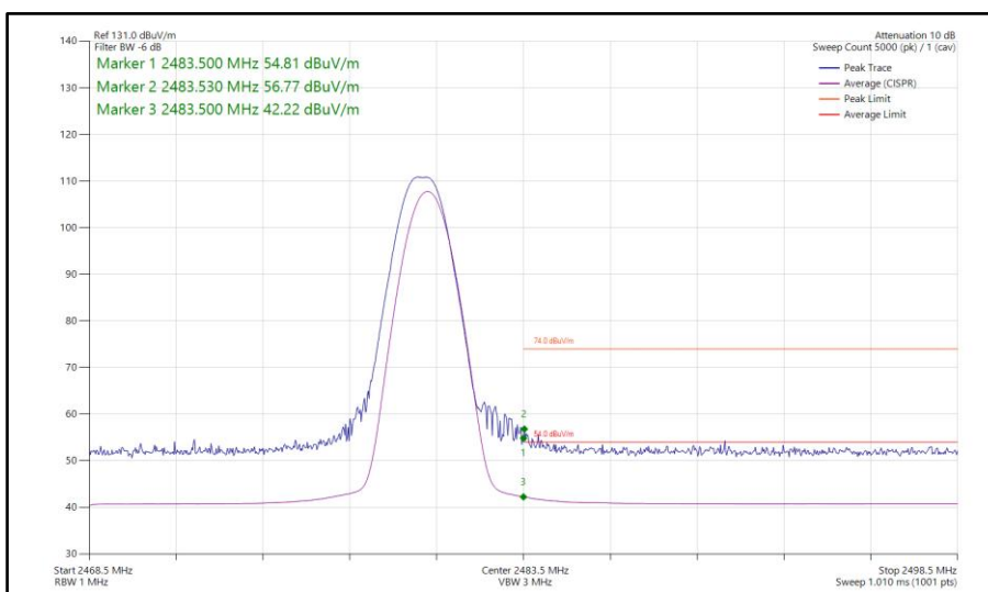
Figure 6 - Bluetooth DH5, SISO, Core 2 - 2480 MHz Band Edge Frequency 2483.5 MHz
