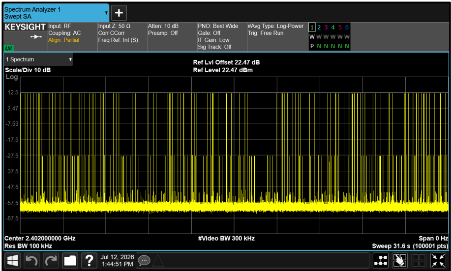
Figure 19 - GFSK - 2402 MHz Accumulated Transmit Time
