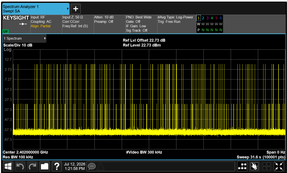
Figure 15 - GFSK - 2402 MHz Accumulated Transmit Time
