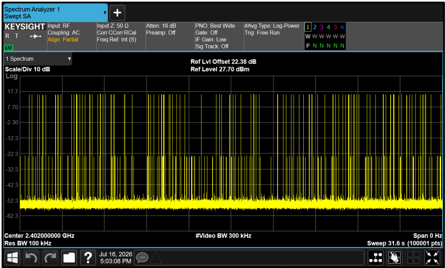
Figure 27 - GFSK - 2402 MHz Accumulated Transmit Time
