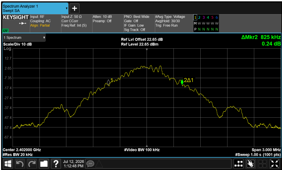
Figure 43 - Core 0 (A) 2402 MHz (CH0) 99% Bandwidth
