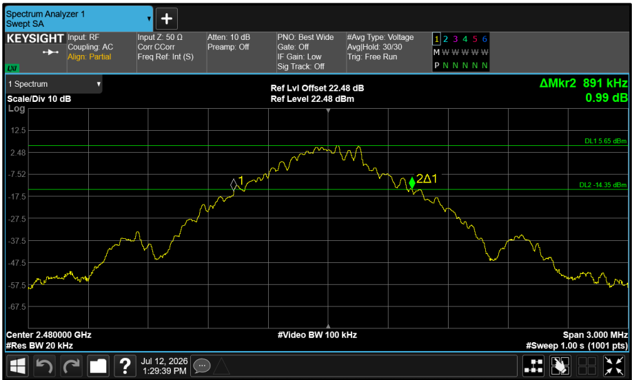
Figure 54 - Core 1 (B) 2480 MHz (CH78) 20 dB Bandwidth
