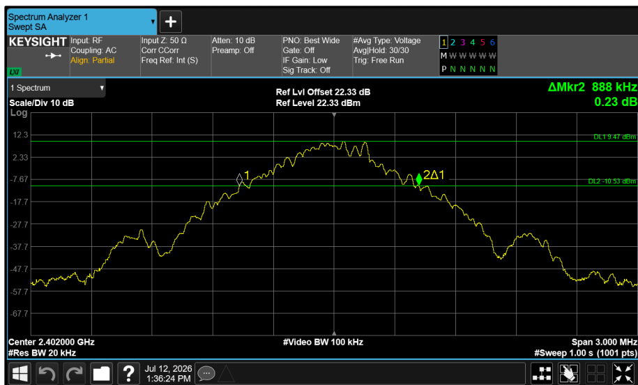
Figure 56 - Core 2 (C) 2402 MHz (CH0) 20 dB Bandwidth
