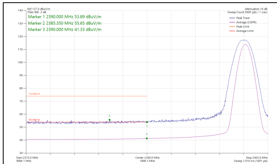
Figure 9 - Bluetooth DH5, SISO, Core 0 - 2402 MHz Band Edge Frequency 2390 MHz
