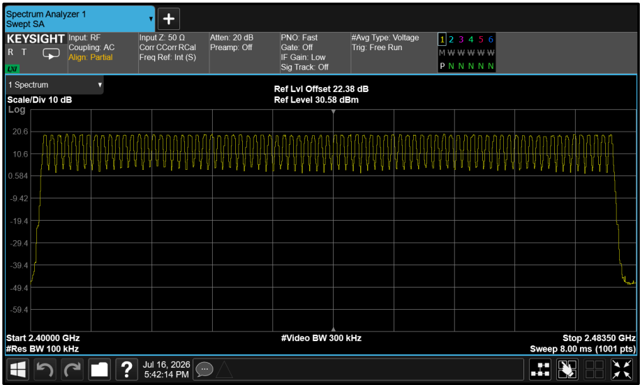
Figure 39 - GFSK (DH5) - Number of Hopping Channels
