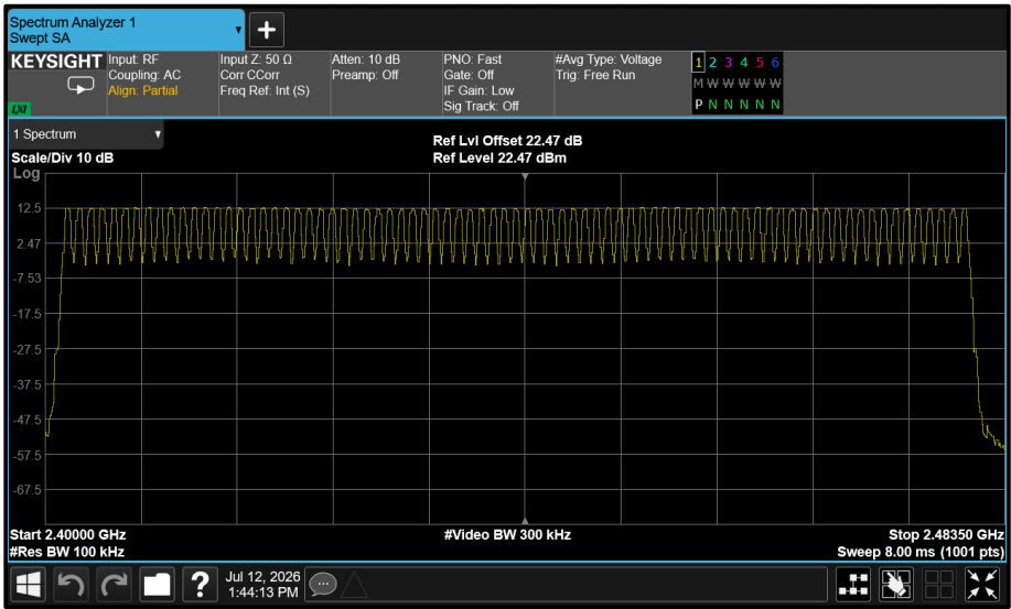
Figure 38 - GFSK (DH5) - Number of Hopping Channels
