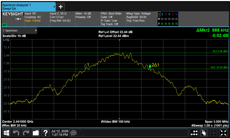
Figure 52 - Core 1 (B) 2441 MHz (CH39) 20 dB Bandwidth
