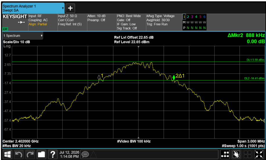
Figure 44 - Core 0 (A) 2402 MHz (CH0) 20 dB Bandwidth
