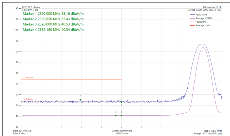
Figure 3 - Bluetooth DH5, SISO, Core 1 - 2402 MHz Band Edge Frequency 2390 MHz
