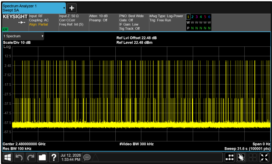
Figure 18 - GFSK - 2480 MHz Accumulated Transmit Time
