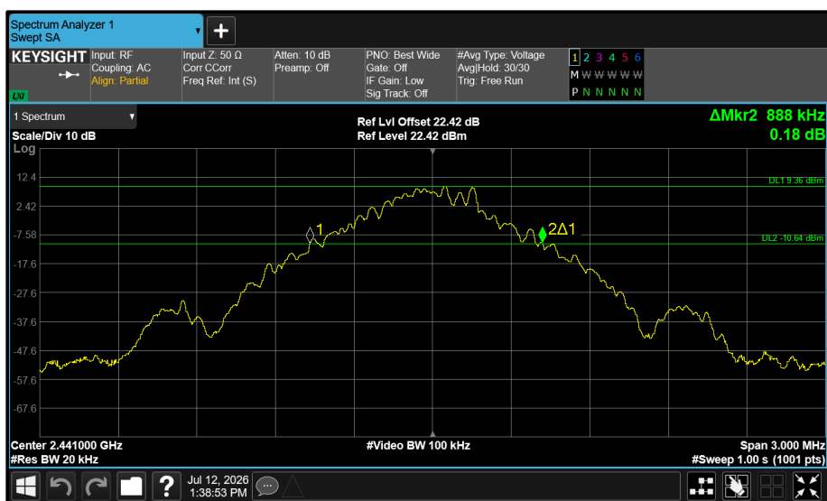
Figure 58 - Core 2 (C) 2441 MHz (CH39) 20 dB Bandwidth
