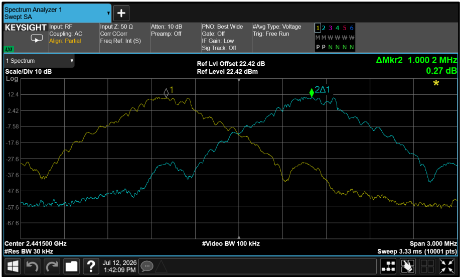
Figure 31 - GFSK - 2441 MHz (CH39)
