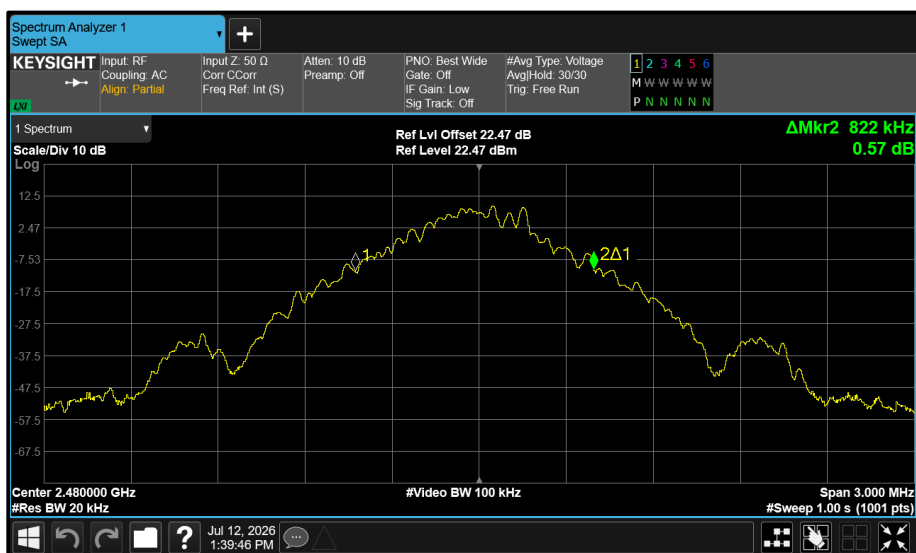
Figure 59 - Core 2 (C) 2480 MHz (CH78) 99% Bandwidth
