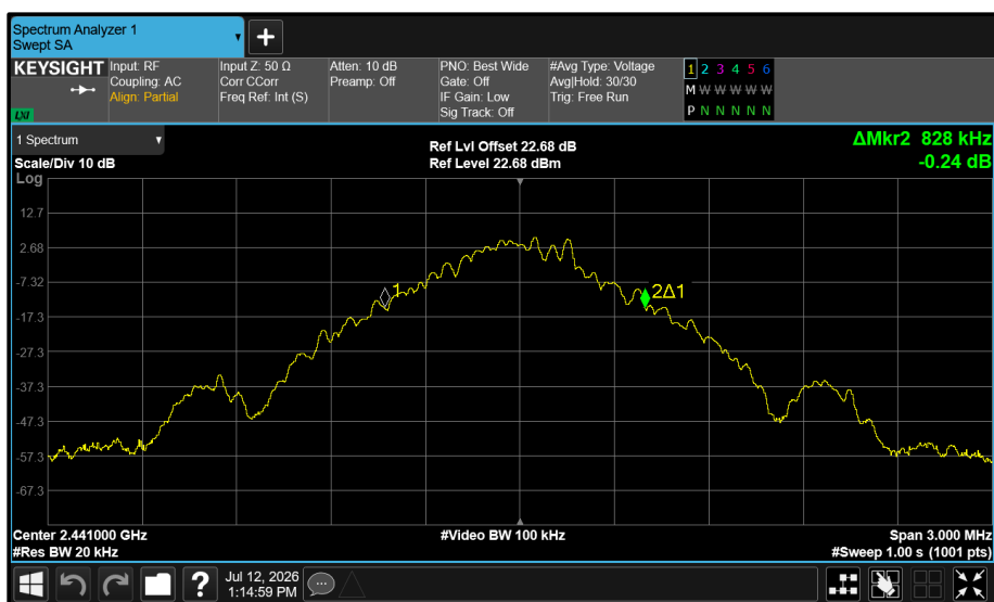
Figure 45 - Core 0 (A) 2441 MHz (CH39) 99% Bandwidth
