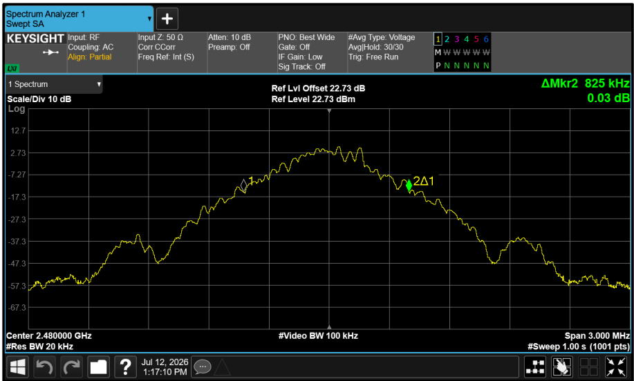
Figure 47 - Core 0 (A) 2480 MHz (CH78) 99% Bandwidth
