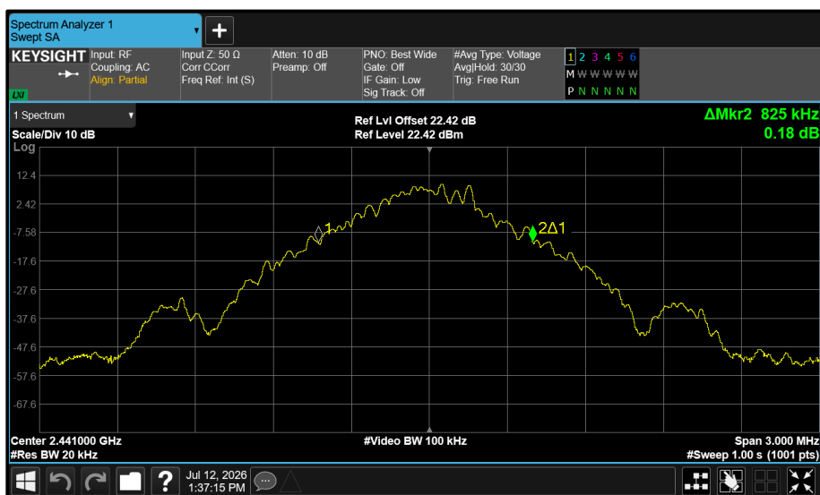
Figure 57 - Core 2 (C) 2441 MHz (CH39) 99% Bandwidth
