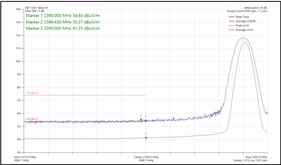
Figure 11 - Bluetooth DH5, SISO, Core 1 - 2402 MHz Band Edge Frequency 2390 MHz
