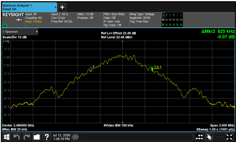
Figure 53 - Core 1 (B) 2480 MHz (CH78) 99% Bandwidth
