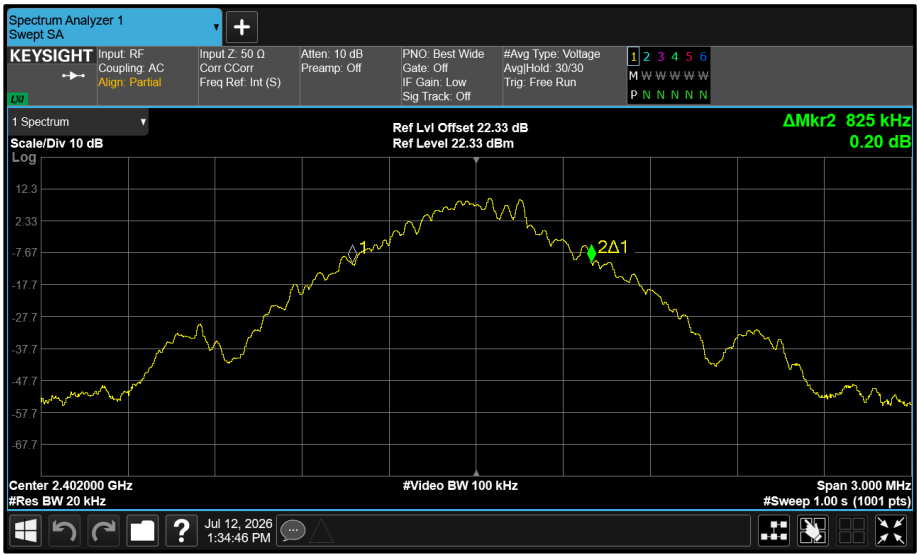
Figure 55 - Core 2 (C) 2402 MHz (CH0) 99% Bandwidth
