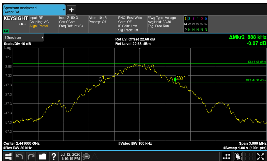
Figure 46 - Core 0 (A) 2441 MHz (CH39) 20 dB Bandwidth
