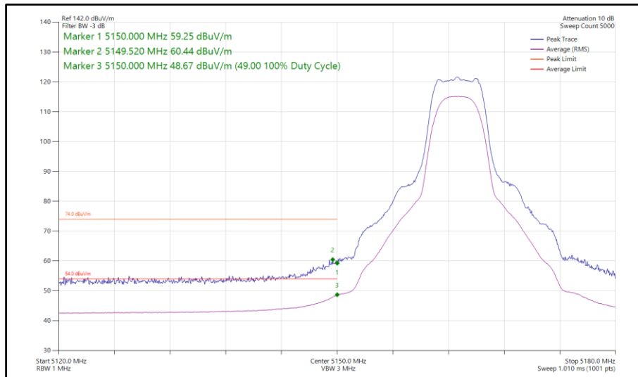
Figure 97 - XHDRPM8, SISO, Core 0 - 5163 MHz Band Edge Frequency 5150 MHz
