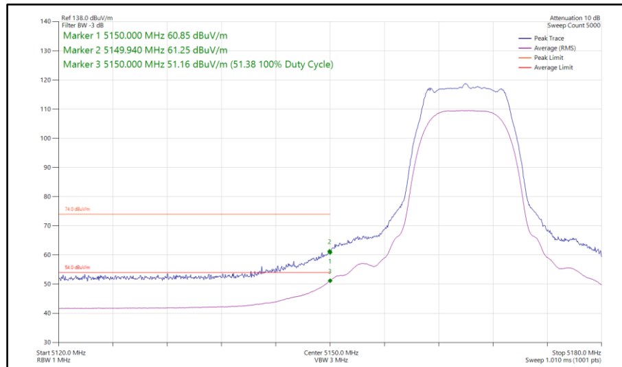
Figure 123 - HDRPL8, SISO, Core 1 - 5165 MHz Band Edge Frequency 5150 MHz
