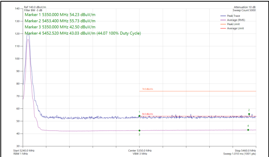
Figure 128 - HDR4, SISO, Core 1 - 5245 MHz Band Edge Frequency 5350 MHz
