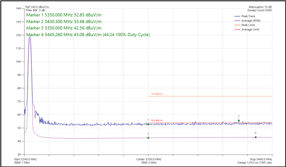
Figure 127 - DH5, SISO, Core 1 - 5245 MHz Band Edge Frequency 5350 MHz
