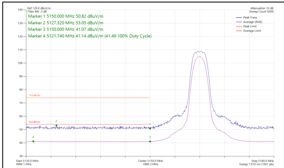
Figure 65 - HDRPS2, MIMO, Core 0-1 - 5162 MHz Band Edge Frequency 5150 MHz
