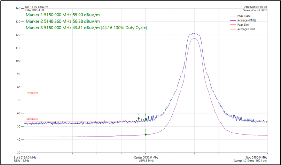
Figure 121 - HDRPS2, SISO, Core 1 - 5162 MHz Band Edge Frequency 5150 MHz
