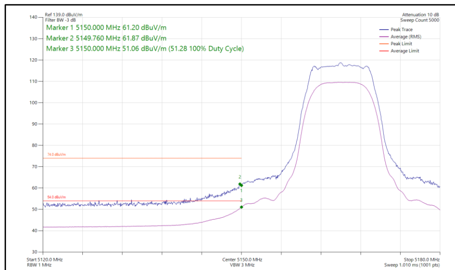
Figure 95 - HDRPL8, SISO, Core 0 - 5165 MHz Band Edge Frequency 5150 MHz
