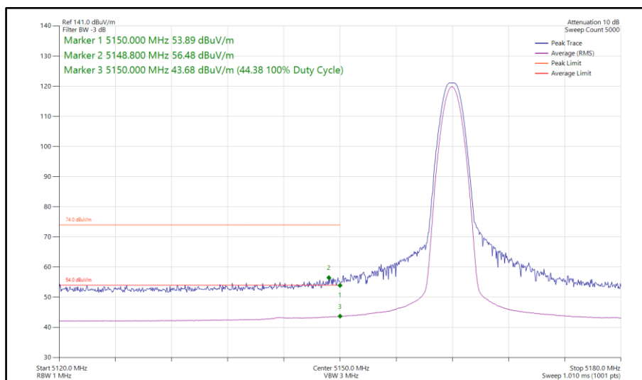
Figure 116 - LE1M, SISO, Core 1 - 5162 MHz Band Edge Frequency 5150 MHz
