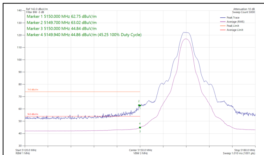
Figure 120 - HDT6, SISO, Core 1 - 5162 MHz Band Edge Frequency 5150 MHz
