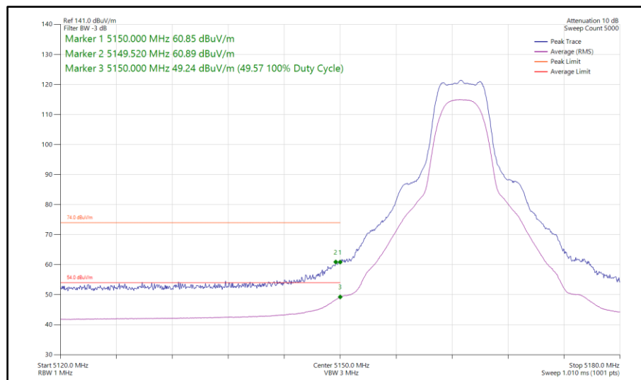
Figure 125 - XHDRPM8, SISO, Core 1 - 5163 MHz Band Edge Frequency 5150 MHz
