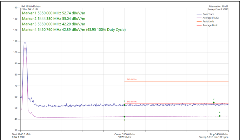
Figure 72 - HDR4, MIMO, Core 0-1 - 5245 MHz Band Edge Frequency 5350 MHz
