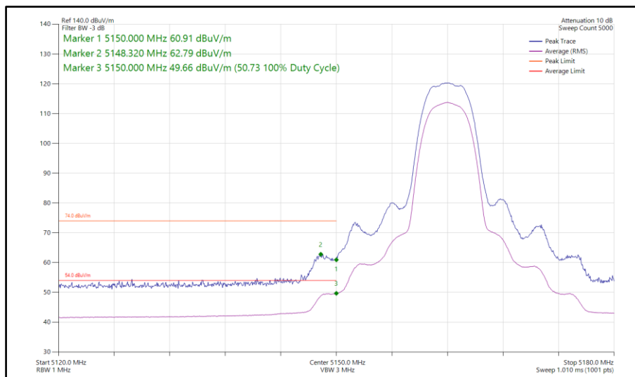
Figure 115 - HDR8, SISO, Core 1 - 5162 MHz Band Edge Frequency 5150 MHz
