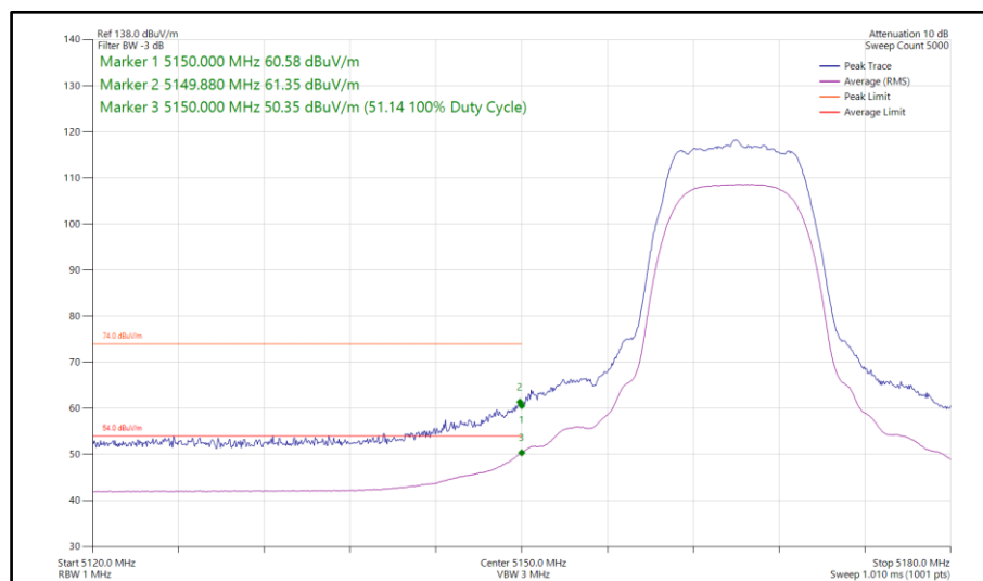
Figure 126 - XHDRPL24, SISO, Core 1 - 5165 MHz Band Edge Frequency 5150 MHz
