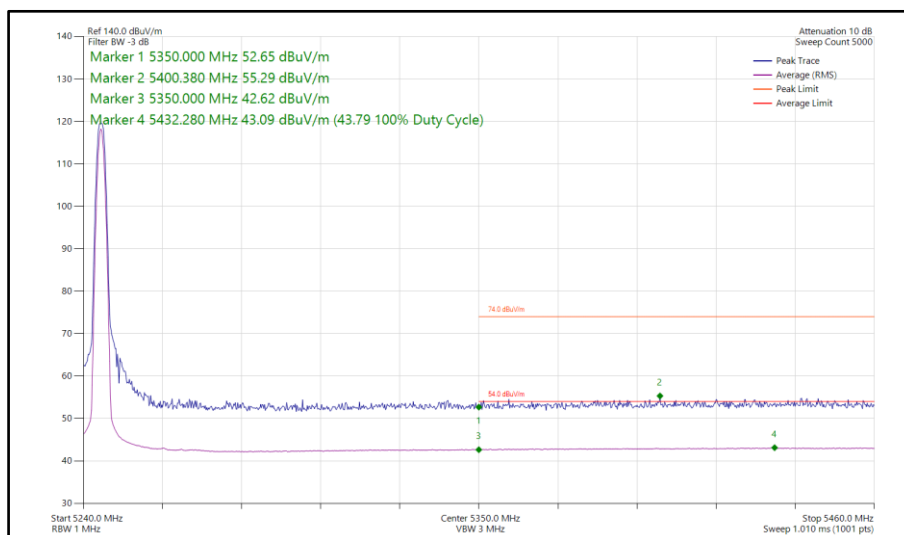
Figure 130 - LE1M, SISO, Core 1 - 5245 MHz Band Edge Frequency 5350 MHz
