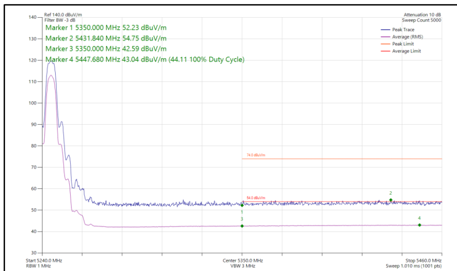
Figure 129 - HDR8, SISO, Core 1 - 5245 MHz Band Edge Frequency 5350 MHz
