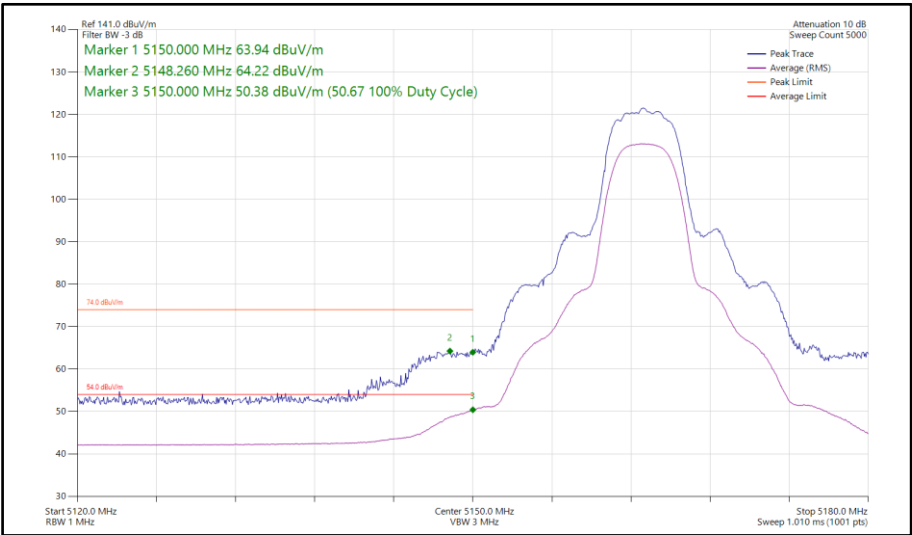
Figure 122 - HDRPM12, SISO, Core 1 - 5163 MHz Band Edge Frequency 5150 MHz
