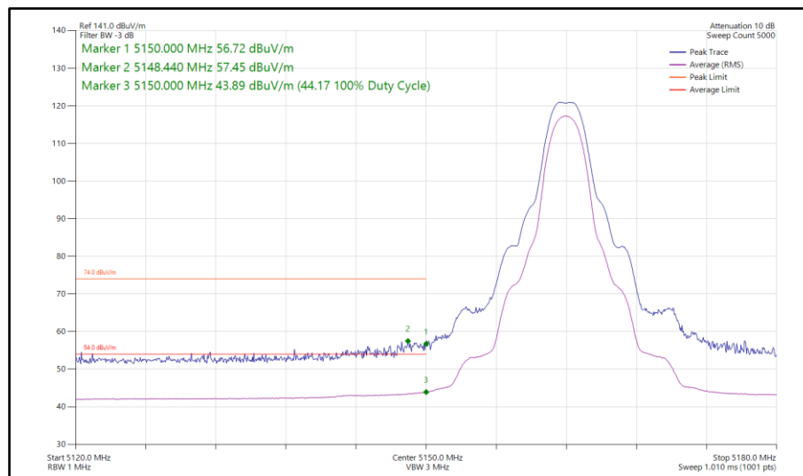
Figure 119 - HDT4, SISO, Core 1 - 5162 MHz Band Edge Frequency 5150 MHz
