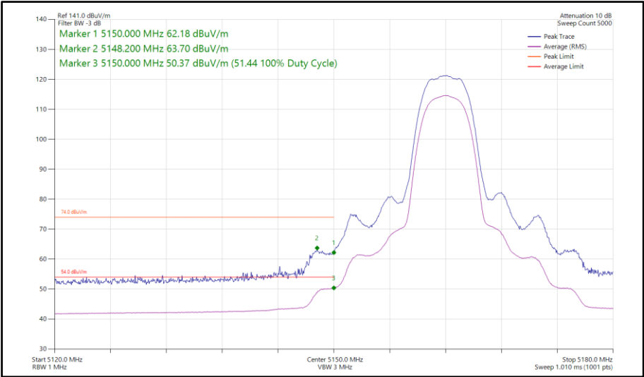
Figure 87 - HDR8, SISO, Core 0 - 5162 MHz Band Edge Frequency 5150 MHz
