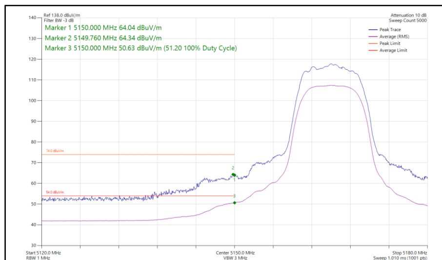
Figure 124 - HDRPL24, SISO, Core 1 - 5165 MHz Band Edge Frequency 5150 MHz
