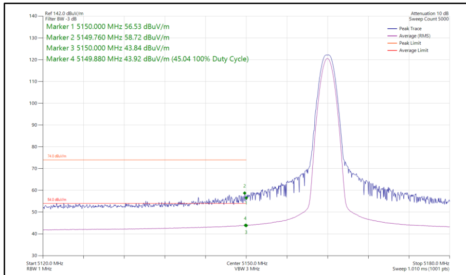
Figure 85 - DH5, SISO, Core 0 - 5162 MHz Band Edge Frequency 5150 MHz
