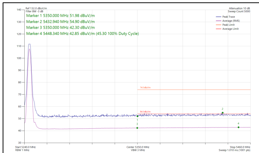
Figure 75 - LE2M, MIMO, Core 0-1 - 5245 MHz Band Edge Frequency 5350 MHz
