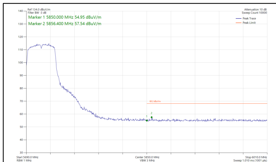
Figure 624 - 802.11ac VHT40, TxBF, Core 0-1 - 5710 MHz Band Edge Frequency 5850 MHz
