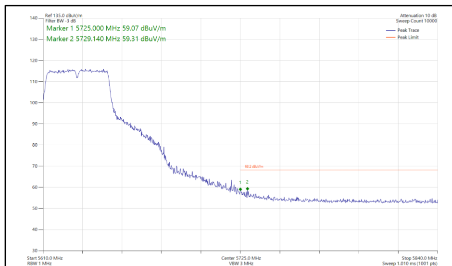
Figure 620 - 802.11ac VHT40, TxBF, Core 0-1 - 5630 MHz Band Edge Frequency 5725 MHz
