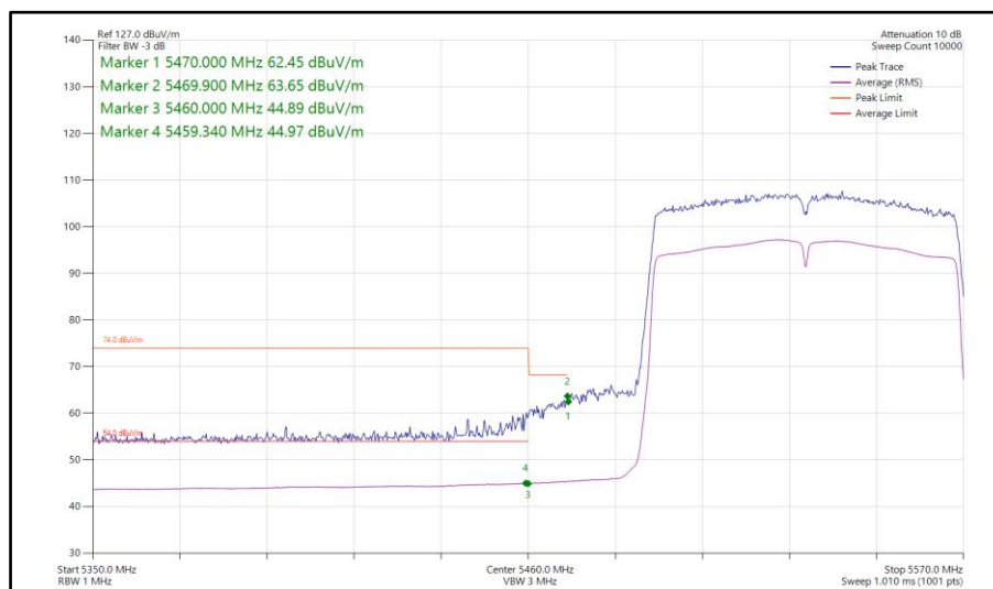
Figure 629 - 802.11ac VHT80, SISO, Core 0 - 5530 MHz Band Edge Frequency 5470 MHz
