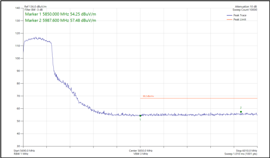
Figure 606 - 802.11ax HE40, SU, SDM, Core 0-1 - 5710 MHz Band Edge Frequency 5850 MHz
