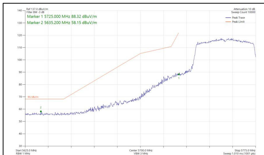
Figure 593 - 802.11ax HE40, SU, SDM, Core 0-1 - 5755 MHz Band Edge Frequency 5725 MHz
