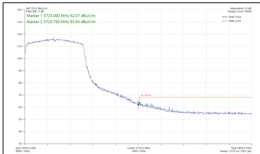
Figure 600 - 802.11ax HE40, SU, SDM, Core 0-1 - 5670 MHz Band Edge Frequency 5725 MHz
