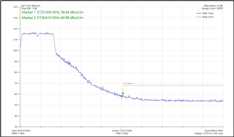
Figure 596 - 802.11n HT40, SDM, Core 0-1 - 5630 MHz Band Edge Frequency 5725 MHz
