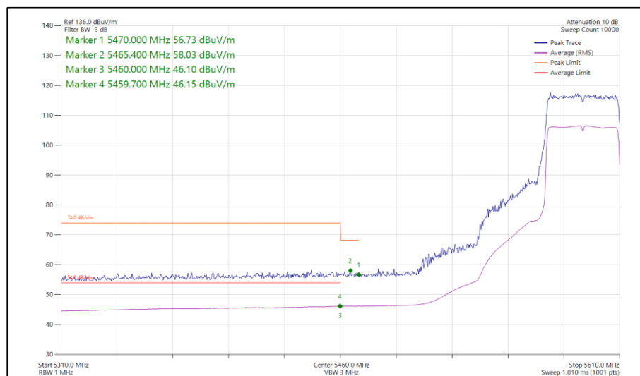
Figure 587 - 802.11ax HE40, SU, SDM, Core 0-1 - 5590 MHz Band Edge Frequency 5470 MHz
