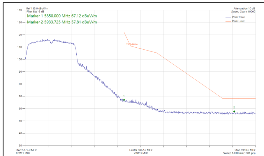
Figure 625 - 802.11ac VHT40, TxBF, Core 0-1 - 5795 MHz Band Edge Frequency 5850 MHz
