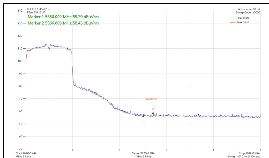
Figure 645 - 802.11ac VHT80, SISO, Core 0 - 5690 MHz Band Edge Frequency 5850 MHz
