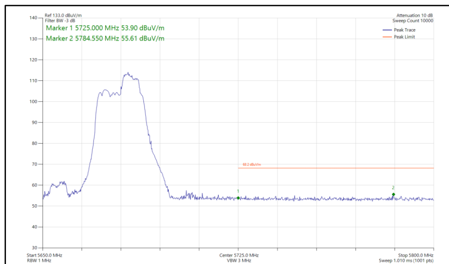
Figure 569 - 802.11be EHT40, RU 52+26-75, CDD, Core 0-1 - 5670 MHz Band Edge Frequency 5725 MHz
