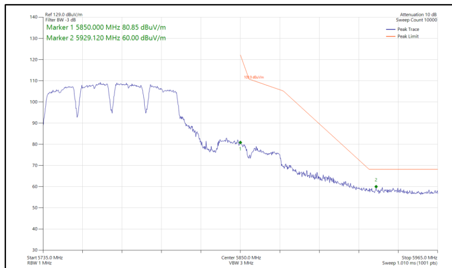
Figure 644 - 802.11a a80, SISO, Core 0 - 5775 MHz Band Edge Frequency 5850 MHz
