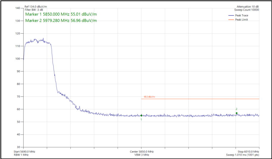
Figure 572 - 802.11n HT40, CDD, Core 0-1 - 5710 MHz Band Edge Frequency 5850 MHz
