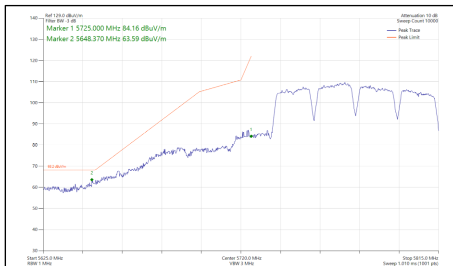
Figure 633 - 802.11a a80, SISO, Core 0 - 5775 MHz Band Edge Frequency 5725 MHz
