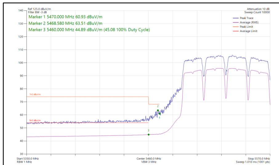
Figure 628 - 802.11a a80, SISO, Core 0 - 5530 MHz Band Edge Frequency 5470 MHz
