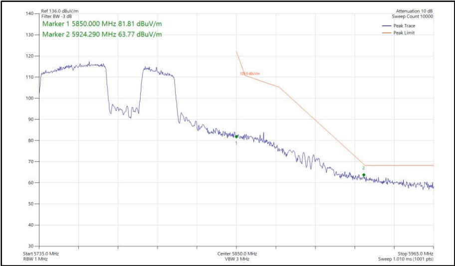
Figure 652 - 802.11be EHT80, RU 484+242-92, SISO, Core 0 - 5775 MHz Band Edge Frequency 5850 MHz
