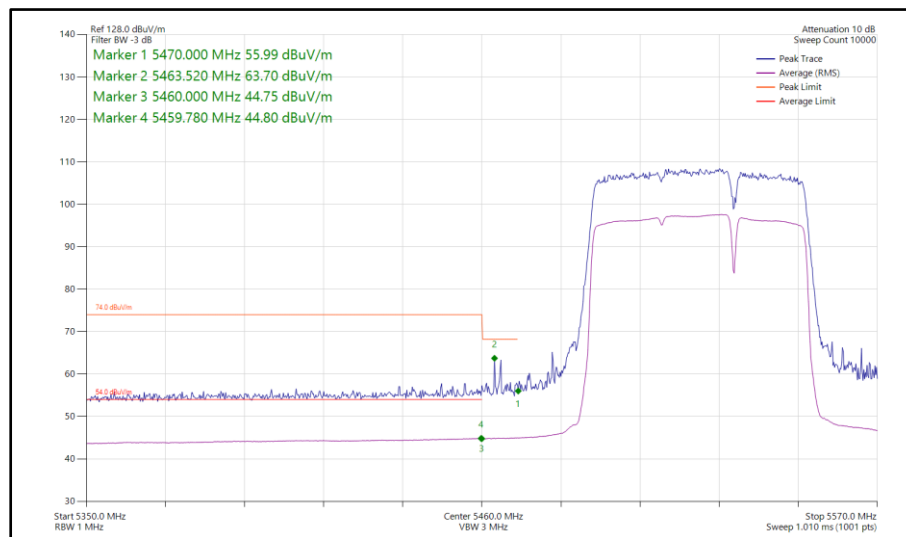
Figure 632 - 802.11be EHT80, RU 484+242-93, SISO, Core 0 - 5530 MHz Band Edge Frequency 5470 MHz
