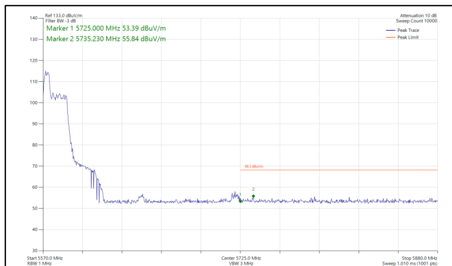
Figure 641 - 802.11ax HE80, RU 52-37, SISO, Core 0 - 5610 MHz Band Edge Frequency 5725 MHz
