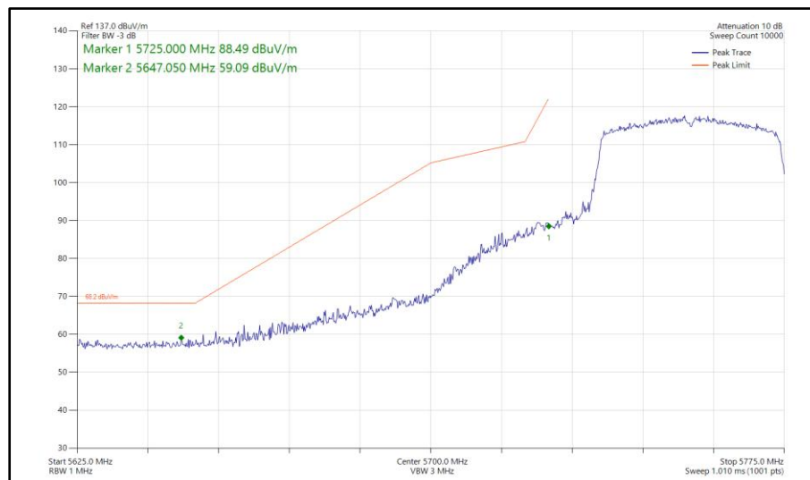
Figure 619 - 802.11ax HE40, SU, TxBF, Core 0-1 - 5755 MHz Band Edge Frequency 5725 MHz
