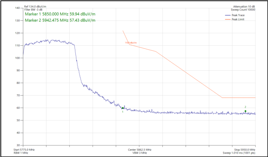
Figure 576 - 802.11ax HE40, SU, CDD, Core 0-1 - 5795 MHz Band Edge Frequency 5850 MHz
