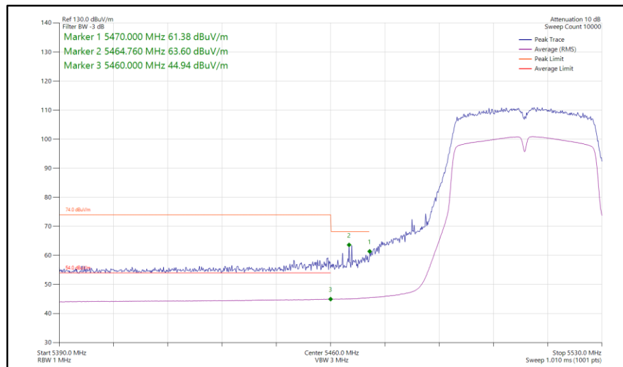
Figure 612 - 802.11ac VHT40, TxBF, Core 0-1 - 5510 MHz Band Edge Frequency 5470 MHz
