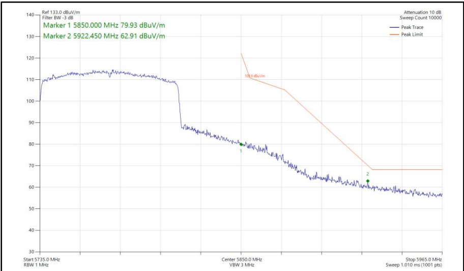
Figure 649 - 802.11ax HE80, SU, SISO, Core 0 - 5775 MHz Band Edge Frequency 5850 MHz
