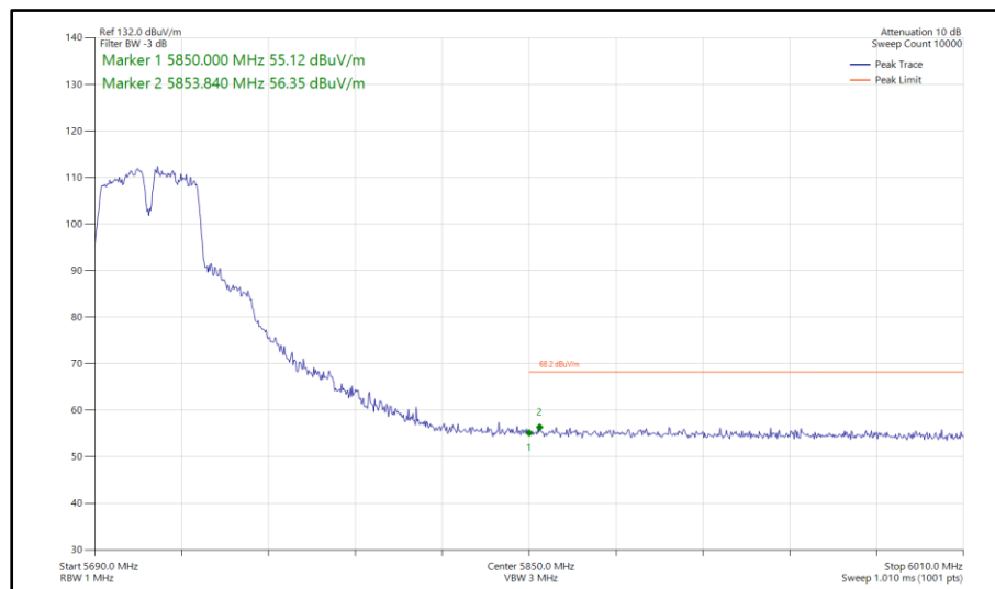
Figure 570 - 802.11a a40, CDD, Core 0-1 - 5710 MHz Band Edge Frequency 5850 MHz
