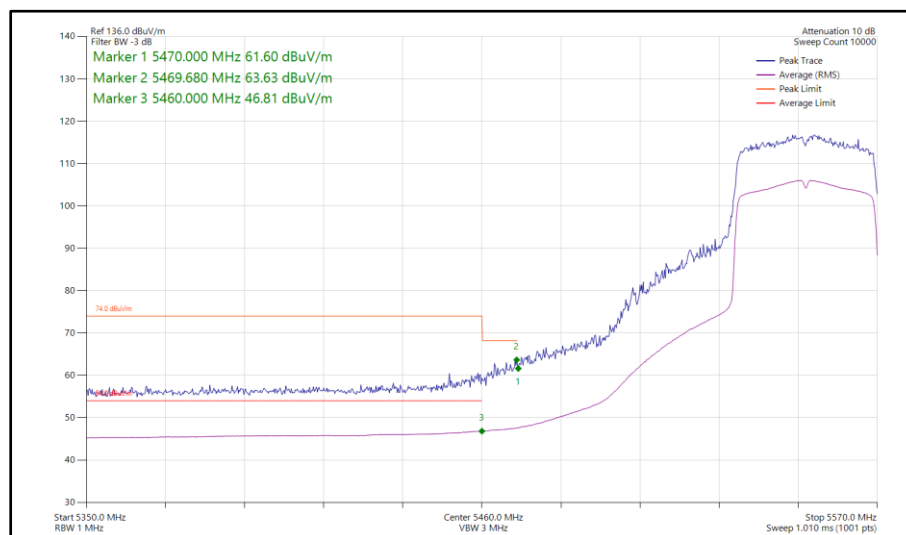
Figure 616 - 802.11ax HE40, SU, TxBF, Core 0-1 - 5550 MHz Band Edge Frequency 5470 MHz
