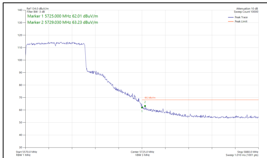
Figure 640 - 802.11ax HE80, SU, SISO, Core 0 - 5610 MHz Band Edge Frequency 5725 MHz
