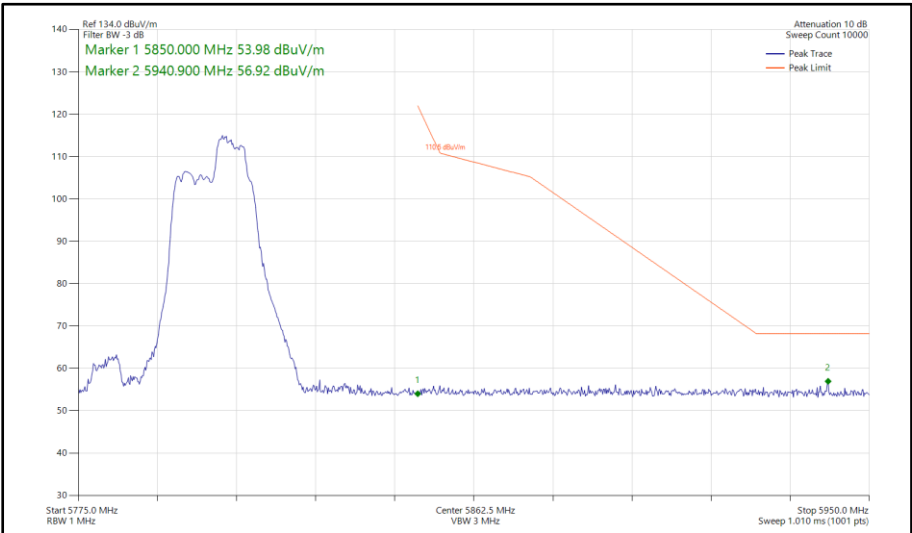
Figure 579 - 802.11be EHT40, RU 52+26-75, CDD, Core 0-1 - 5795 MHz Band Edge Frequency 5850 MHz
