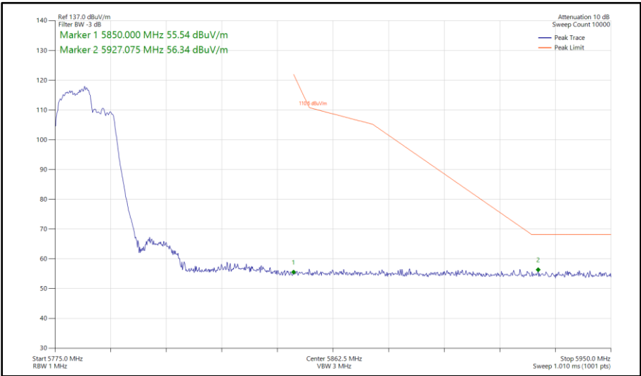
Figure 611 - 802.11be EHT40, RU 106+26-82, SDM, Core 0-1 - 5795 MHz Band Edge Frequency 5850 MHz
