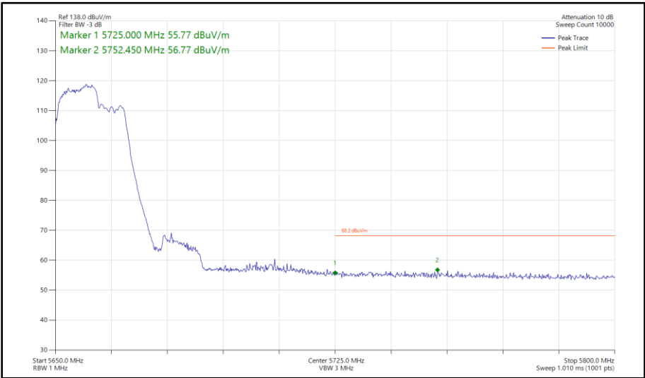
Figure 603 - 802.11be EHT40, RU 106+26-82, SDM, Core 0-1 - 5670 MHz Band Edge Frequency 5725 MHz
