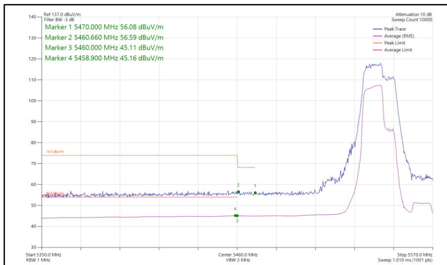
Figure 590 - 802.11be EHT40, RU 106+26-82, SDM, Core 0-1 - 5550 MHz Band Edge Frequency 5470 MHz
