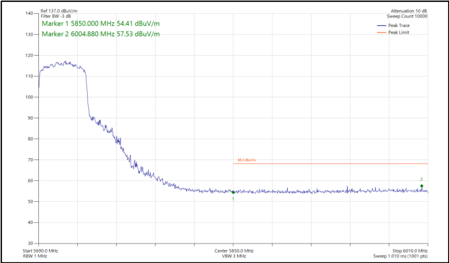
Figure 574 - 802.11ax HE40, SU, CDD, Core 0-1 - 5710 MHz Band Edge Frequency 5850 MHz
