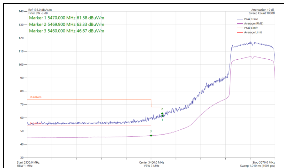
Figure 585 - 802.11ax HE40, SU, SDM, Core 0-1 - 5550 MHz Band Edge Frequency 5470 MHz
