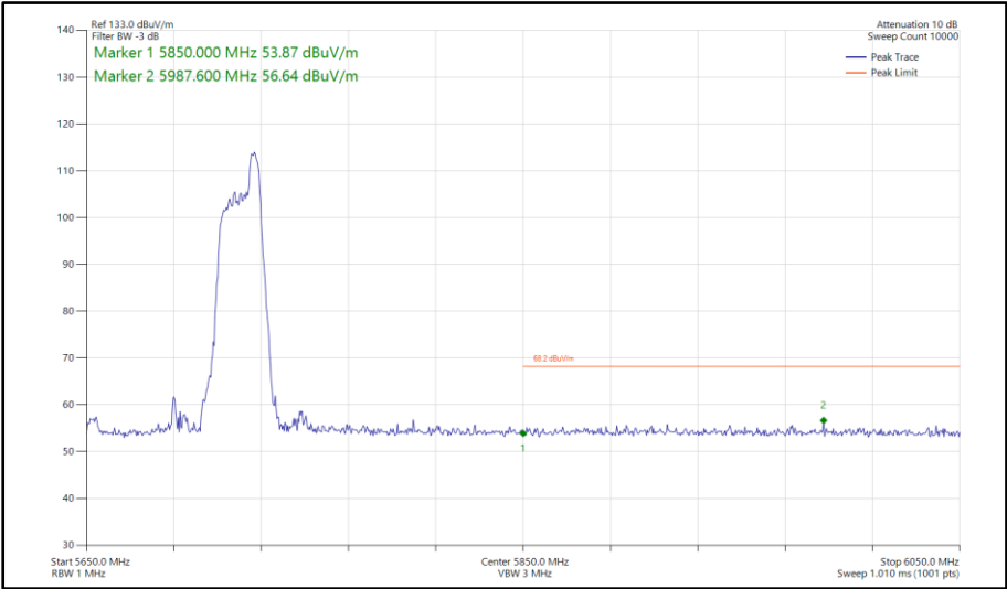
Figure 648 - 802.11ax HE80, RU 52-52, SISO, Core 0 - 5690 MHz Band Edge Frequency 5850 MHz
