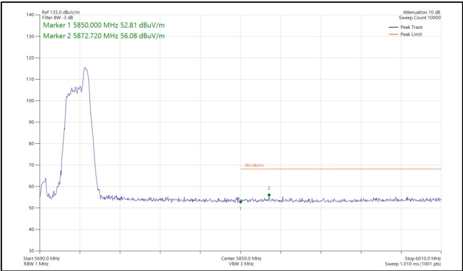
Figure 575 - 802.11ax HE40, RU 52-44, CDD, Core 0-1 - 5710 MHz Band Edge Frequency 5850 MHz
