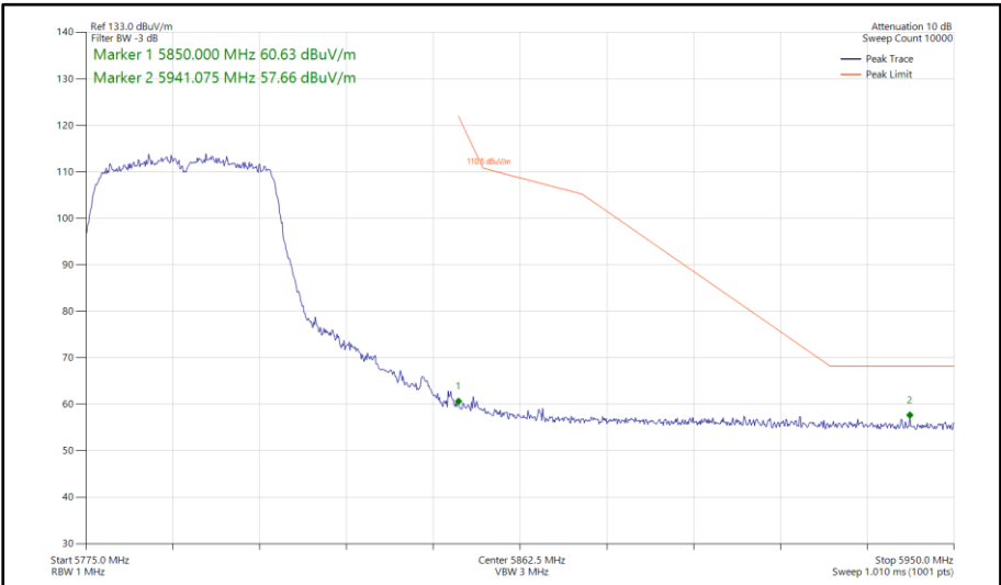
Figure 573 - 802.11n HT40, CDD, Core 0-1 - 5795 MHz Band Edge Frequency 5850 MHz
