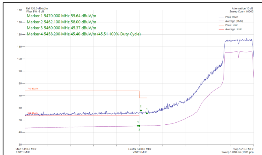
Figure 582 - 802.11n HT40, SDM, Core 0-1 - 5590 MHz Band Edge Frequency 5470 MHz
