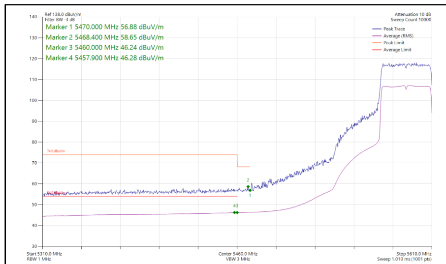
Figure 617 - 802.11ax HE40, SU, TxBF, Core 0-1 - 5590 MHz Band Edge Frequency 5470 MHz
