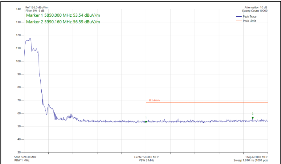
Figure 607 - 802.11ax HE40, RU 106-53, SDM, Core 0-1 - 5710 MHz Band Edge Frequency 5850 MHz
