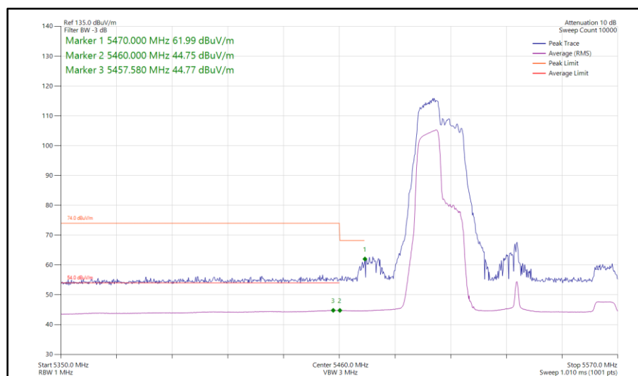
Figure 631 - 802.11ax HE80, RU 106-53, SISO, Core 0 - 5530 MHz Band Edge Frequency 5470 MHz
