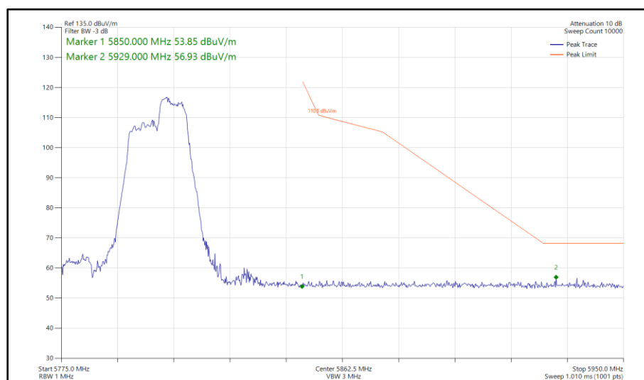
Figure 609 - 802.11ax HE40, RU 106-56, SDM, Core 0-1 - 5795 MHz Band Edge Frequency 5850 MHz
