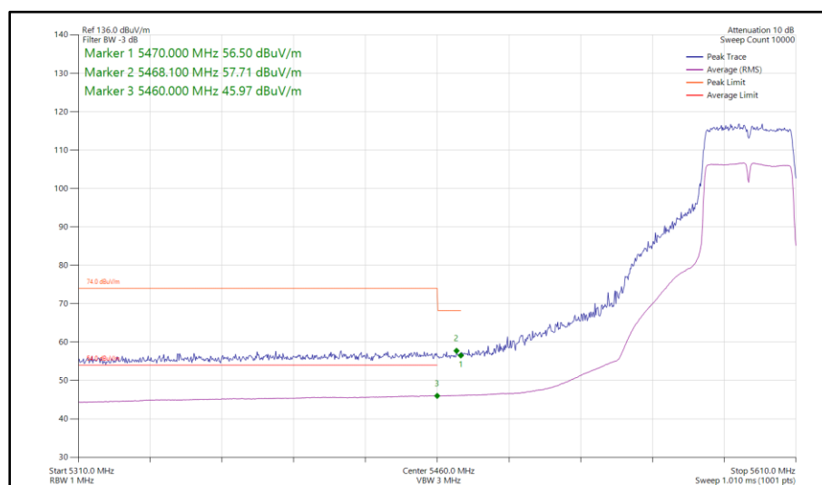
Figure 614 - 802.11ac VHT40, TxBF, Core 0-1 - 5590 MHz Band Edge Frequency 5470 MHz
