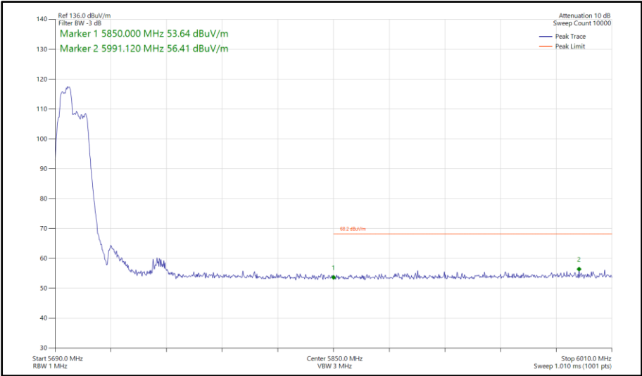
Figure 610 - 802.11be EHT40, RU 52+26-70, SDM, Core 0-1 - 5710 MHz Band Edge Frequency 5850 MHz
