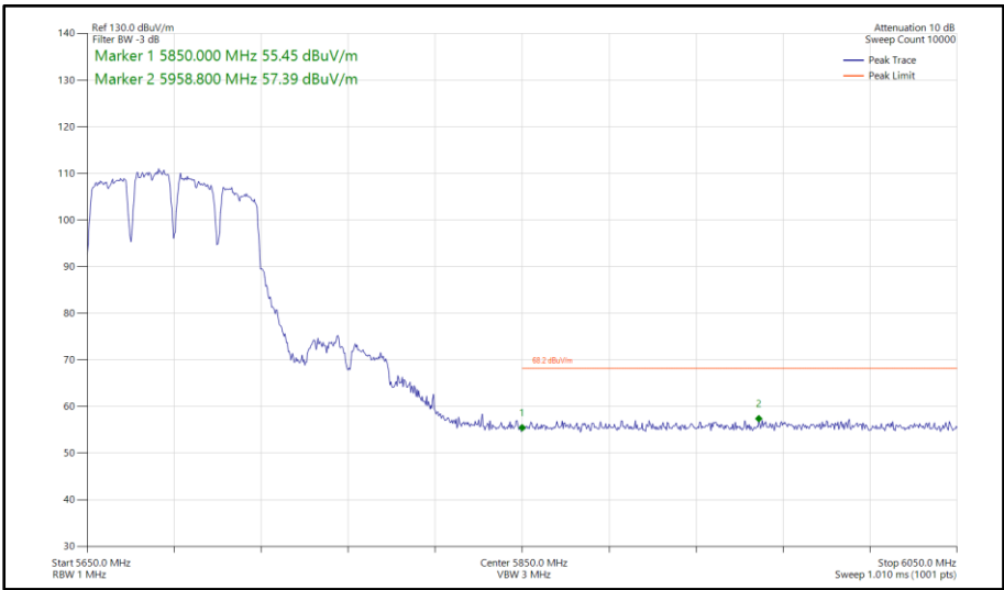
Figure 643 - 802.11a a80, SISO, Core 0 - 5690 MHz Band Edge Frequency 5850 MHz
