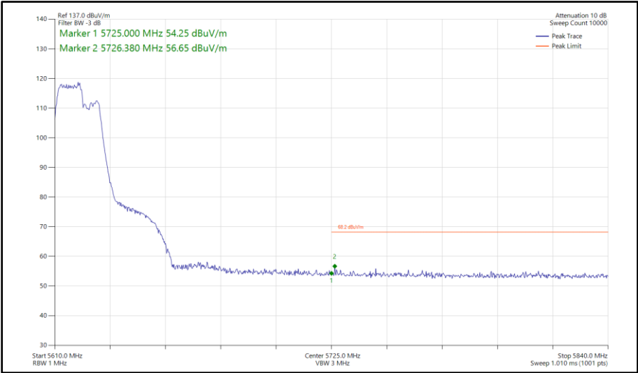
Figure 602 - 802.11be EHT40, RU 106+26-82, SDM, Core 0-1 - 5630 MHz Band Edge Frequency 5725 MHz
