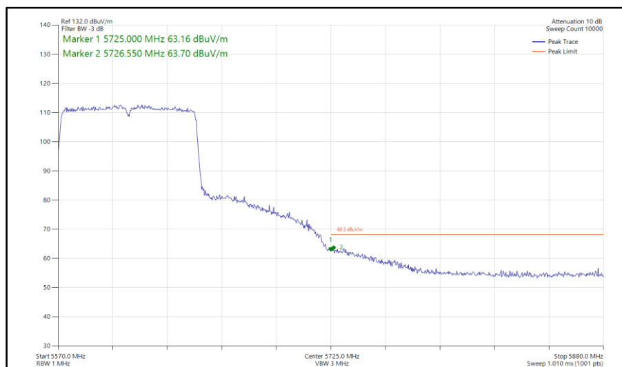
Figure 639 - 802.11ac VHT80, SISO, Core 0 - 5610 MHz Band Edge Frequency 5725 MHz
