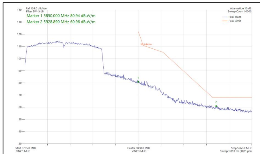
Figure 646 - 802.11ac VHT80, SISO, Core 0 - 5775 MHz Band Edge Frequency 5850 MHz
