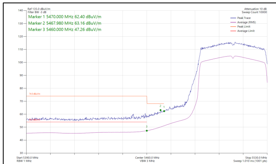
Figure 615 - 802.11ax HE40, SU, TxBF, Core 0-1 - 5510 MHz Band Edge Frequency 5470 MHz
