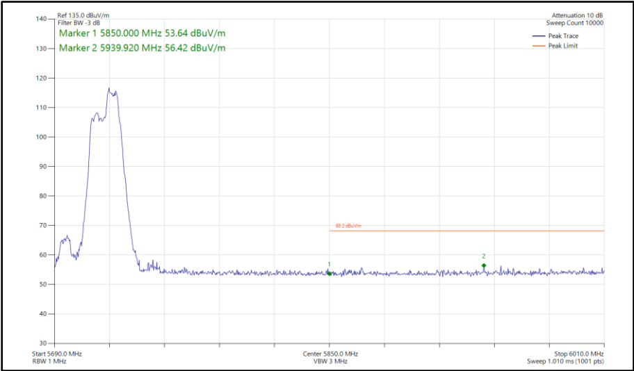
Figure 578 - 802.11be EHT40, RU 52+26-75, CDD, Core 0-1 - 5710 MHz Band Edge Frequency 5850 MHz
