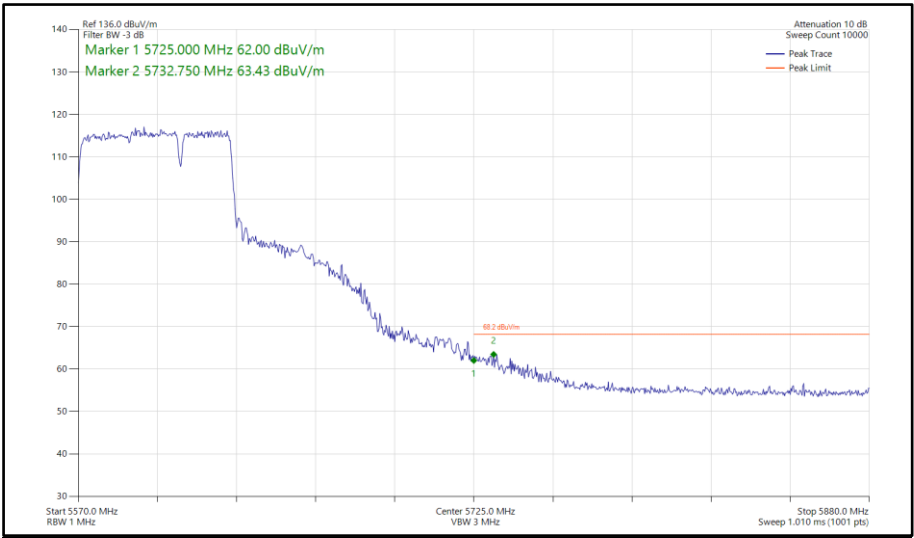
Figure 642 - 802.11be EHT80, RU 484+242-93, SISO, Core 0 - 5610 MHz Band Edge Frequency 5725 MHz
