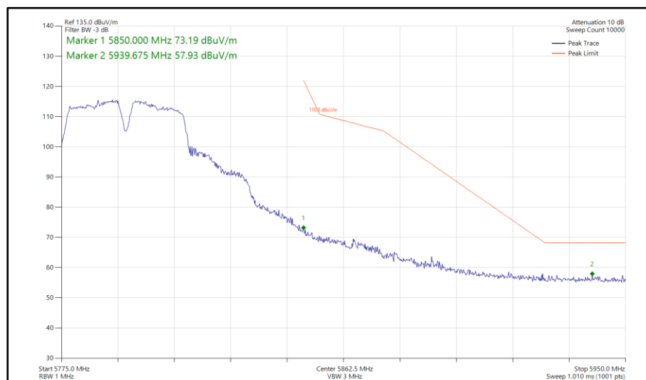
Figure 571 - 802.11a a40, CDD, Core 0-1 - 5795 MHz Band Edge Frequency 5850 MHz
