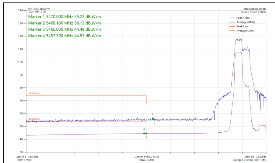
Figure 588 - 802.11ax HE40, RU 106-53, SDM, Core 0-1 - 5590 MHz Band Edge Frequency 5470 MHz
