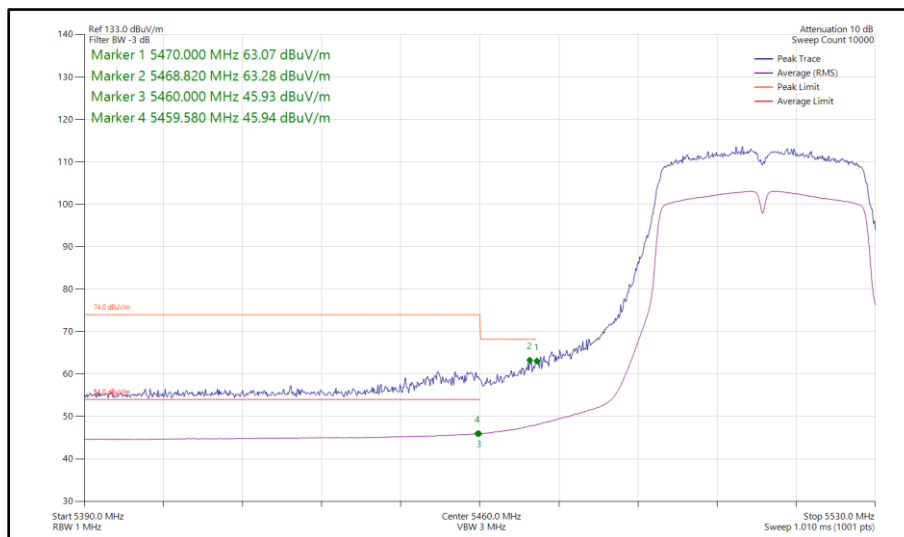
Figure 580 - 802.11n HT40, SDM, Core 0-1 - 5510 MHz Band Edge Frequency 5470 MHz
