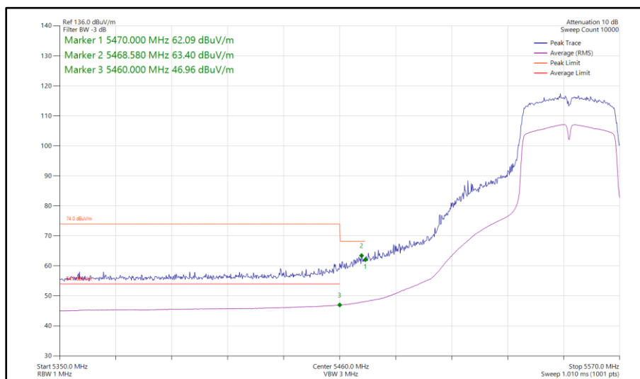
Figure 581 - 802.11n HT40, SDM, Core 0-1 - 5550 MHz Band Edge Frequency 5470 MHz
