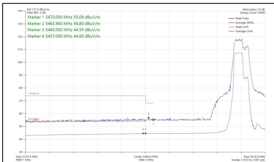
Figure 591 - 802.11be EHT40, RU 106+26-82, SDM, Core 0-1 - 5590 MHz Band Edge Frequency 5470 MHz
