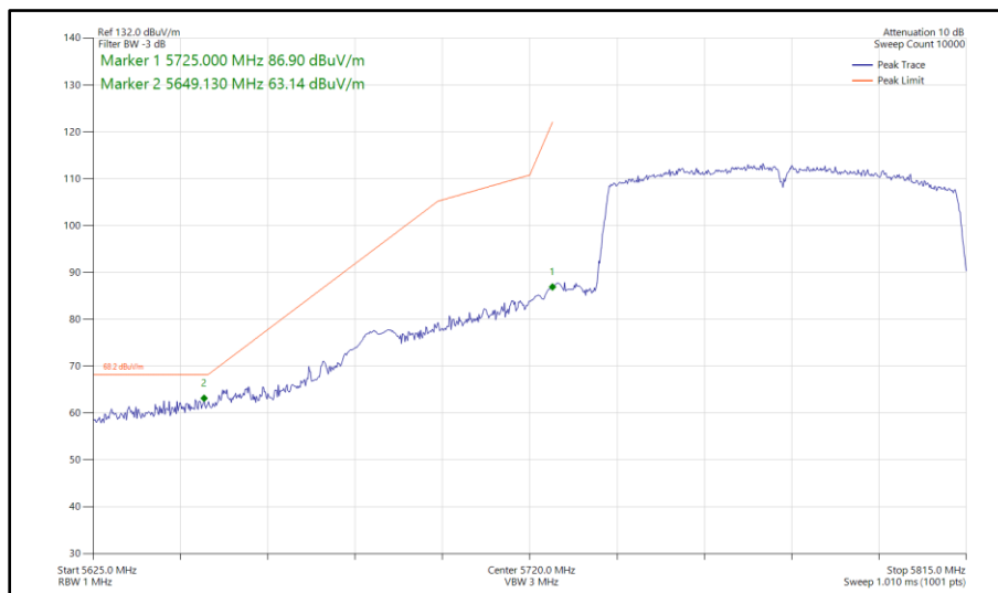
Figure 634 - 802.11ac VHT80, SISO, Core 0 - 5775 MHz Band Edge Frequency 5725 MHz
