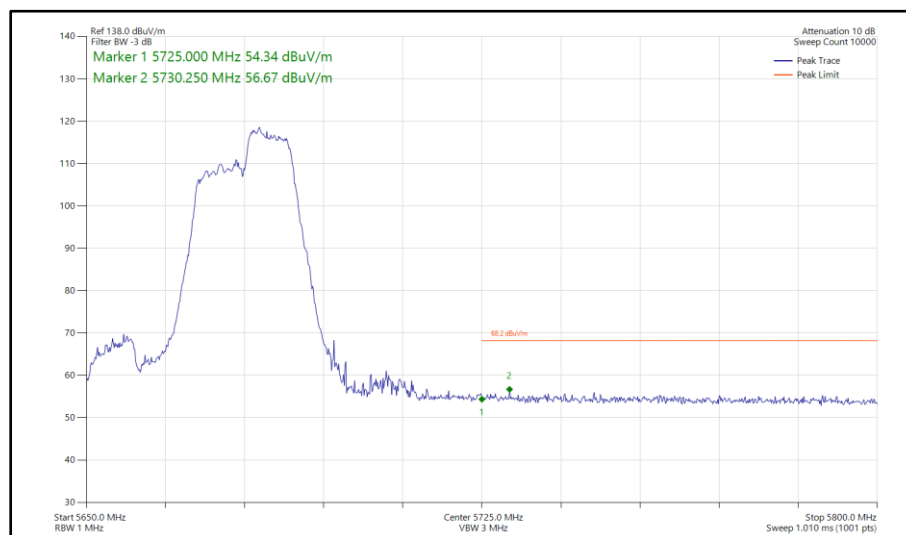
Figure 601 - 802.11ax HE40, RU 106-56, SDM, Core 0-1 - 5670 MHz Band Edge Frequency 5725 MHz
