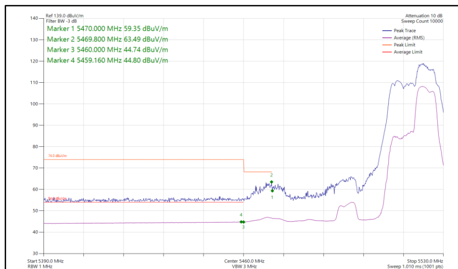
Figure 589 - 802.11be EHT40, RU 52+26-75, SDM, Core 0-1 - 5510 MHz Band Edge Frequency 5470 MHz
