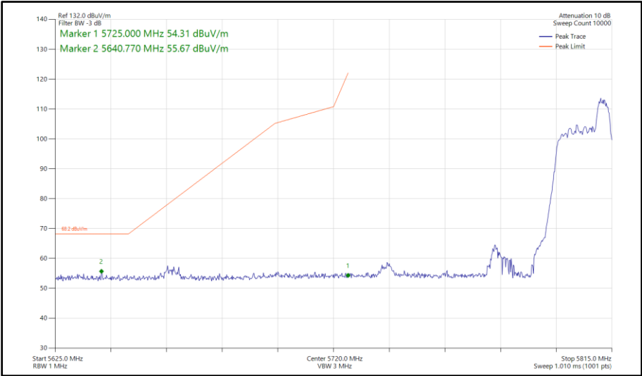
Figure 636 - 802.11ax HE80, RU 52-52, SISO, Core 0 - 5775 MHz Band Edge Frequency 5725 MHz
