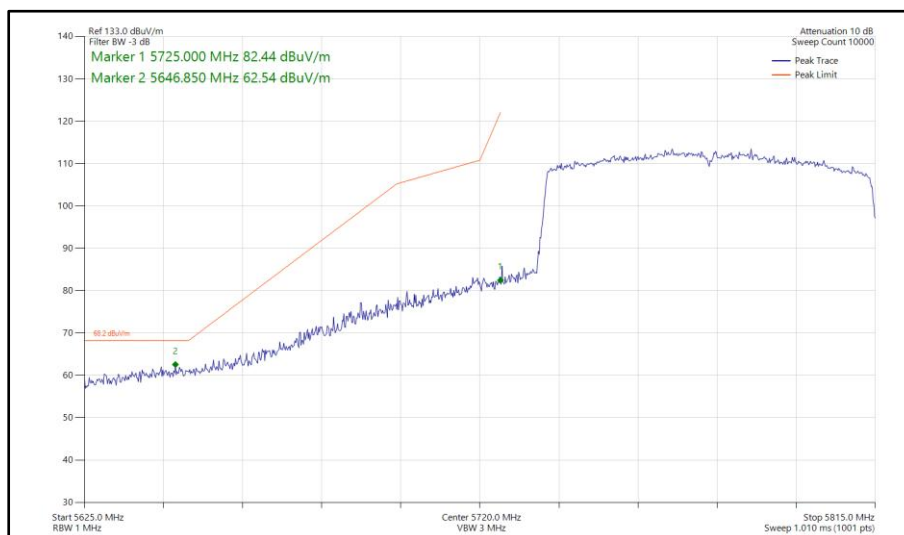
Figure 635 - 802.11ax HE80, SU, SISO, Core 0 - 5775 MHz Band Edge Frequency 5725 MHz
