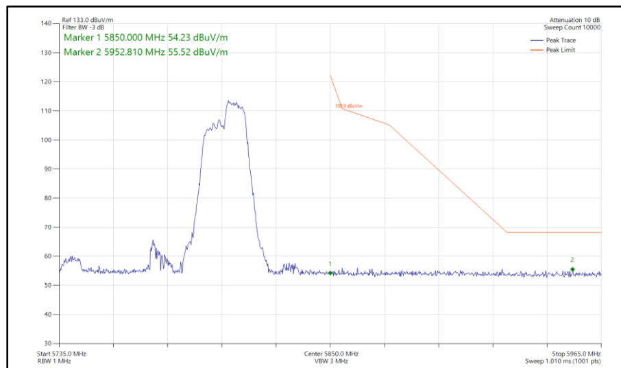
Figure 650 - 802.11ax HE80, RU 106-60, SISO, Core 0 - 5775 MHz Band Edge Frequency 5850 MHz
