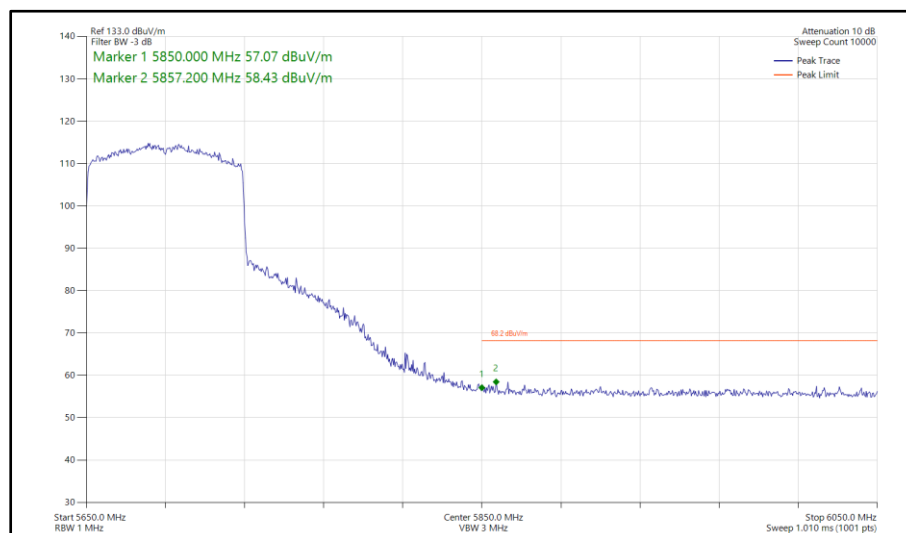
Figure 647 - 802.11ax HE80, SU, SISO, Core 0 - 5690 MHz Band Edge Frequency 5850 MHz
