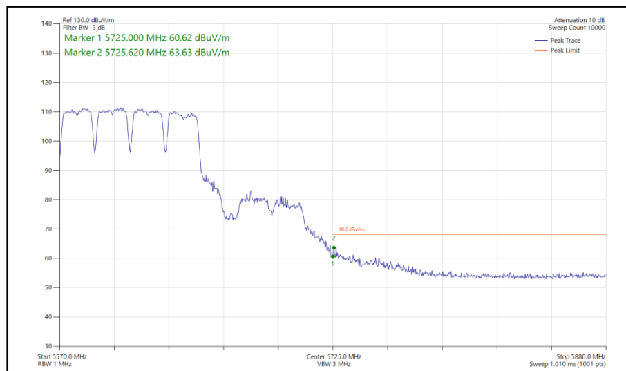
Figure 638 - 802.11a a80, SISO, Core 0 - 5610 MHz Band Edge Frequency 5725 MHz
