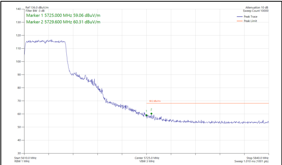
Figure 622 - 802.11ax HE40, SU, TxBF, Core 0-1 - 5630 MHz Band Edge Frequency 5725 MHz
