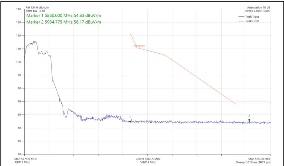
Figure 577 - 802.11ax HE40, RU 106-53, CDD, Core 0-1 - 5795 MHz Band Edge Frequency 5850 MHz
