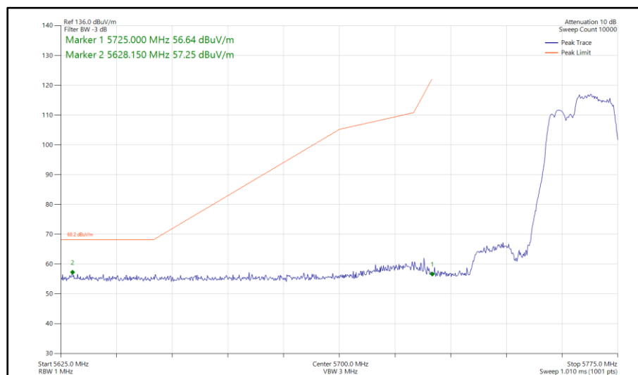
Figure 595 - 802.11be EHT40, RU 106+26-85, SDM, Core 0-1 - 5755 MHz Band Edge Frequency 5725 MHz
