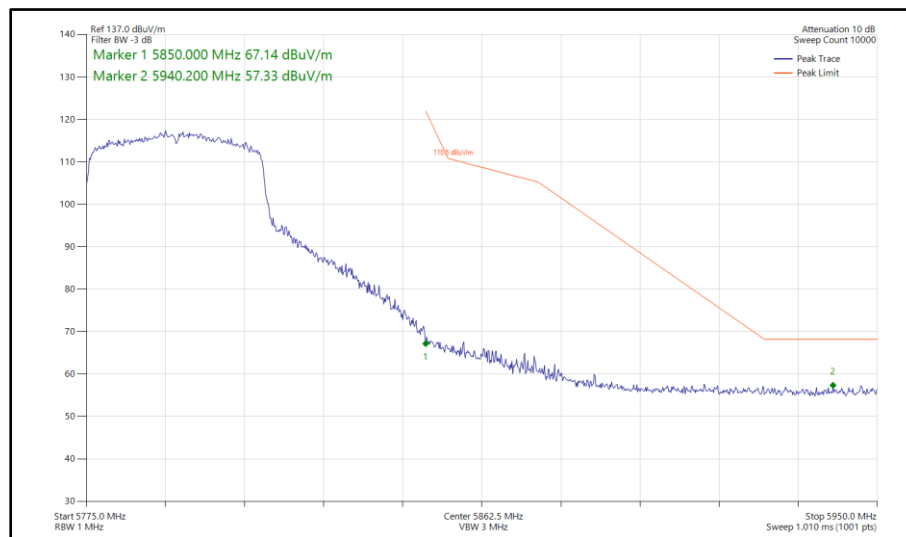
Figure 608 - 802.11ax HE40, SU, SDM, Core 0-1 - 5795 MHz Band Edge Frequency 5850 MHz
