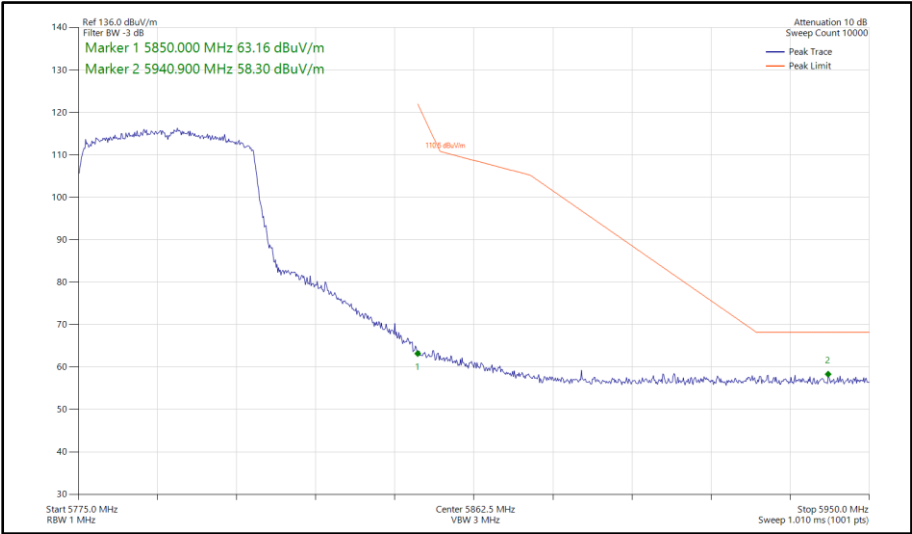
Figure 627 - 802.11ax HE40, SU, TxBF, Core 0-1 - 5795 MHz Band Edge Frequency 5850 MHz
