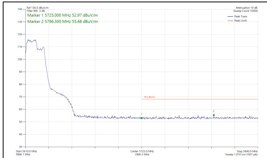
Figure 568 - 802.11be EHT40, RU 106+26-82, CDD, Core 0-1 - 5630 MHz Band Edge Frequency 5725 MHz
