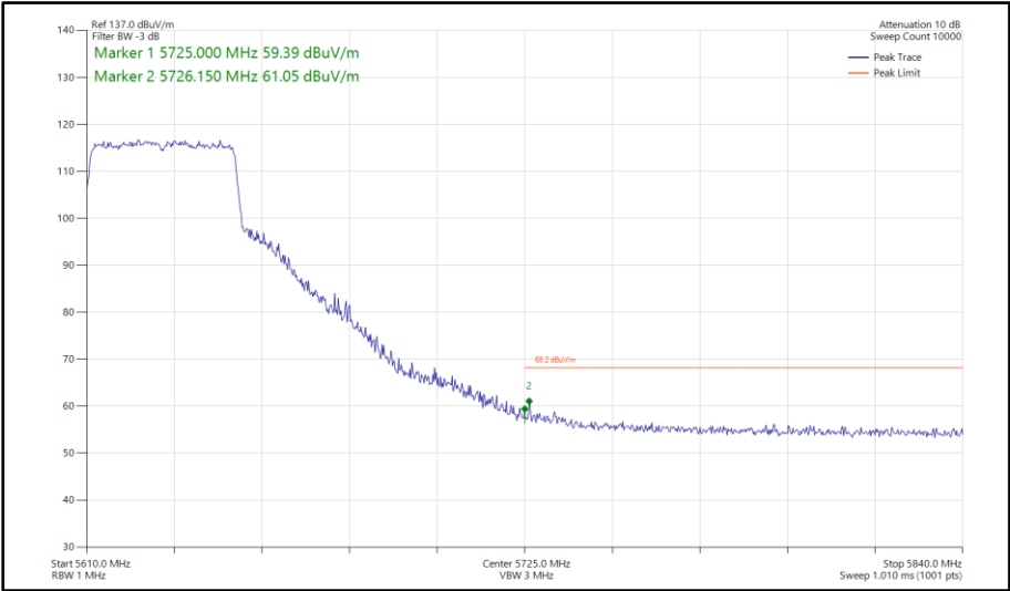
Figure 598 - 802.11ax HE40, SU, SDM, Core 0-1 - 5630 MHz Band Edge Frequency 5725 MHz
