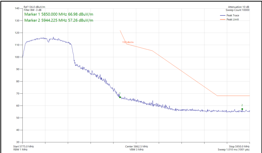
Figure 605 - 802.11n HT40, SDM, Core 0-1 - 5795 MHz Band Edge Frequency 5850 MHz
