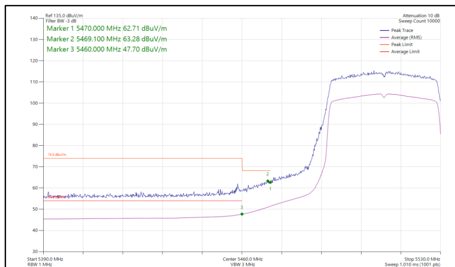
Figure 583 - 802.11ax HE40, SU, SDM, Core 0-1 - 5510 MHz Band Edge Frequency 5470 MHz
