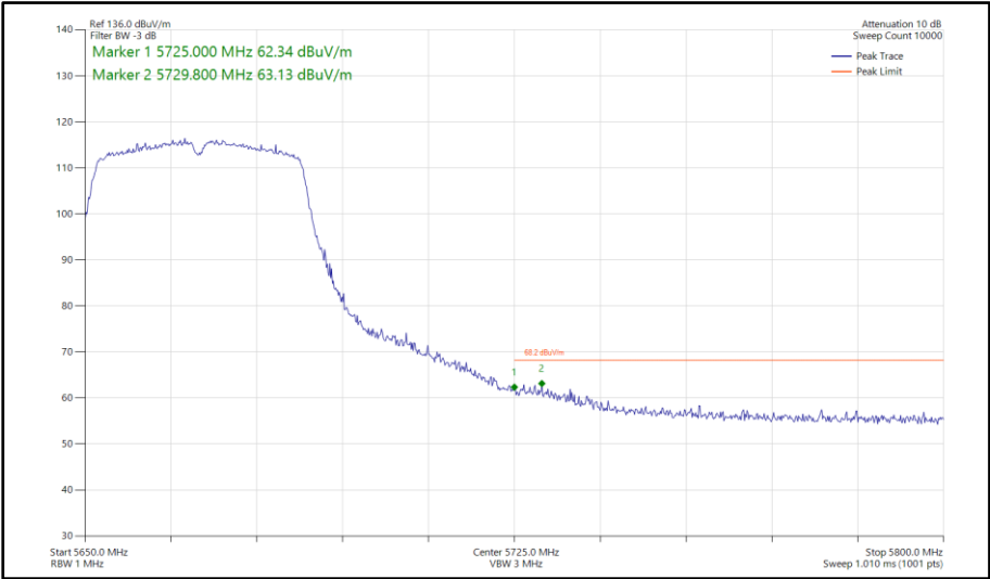
Figure 621 - 802.11ac VHT40, TxBF, Core 0-1 - 5670 MHz Band Edge Frequency 5725 MHz
