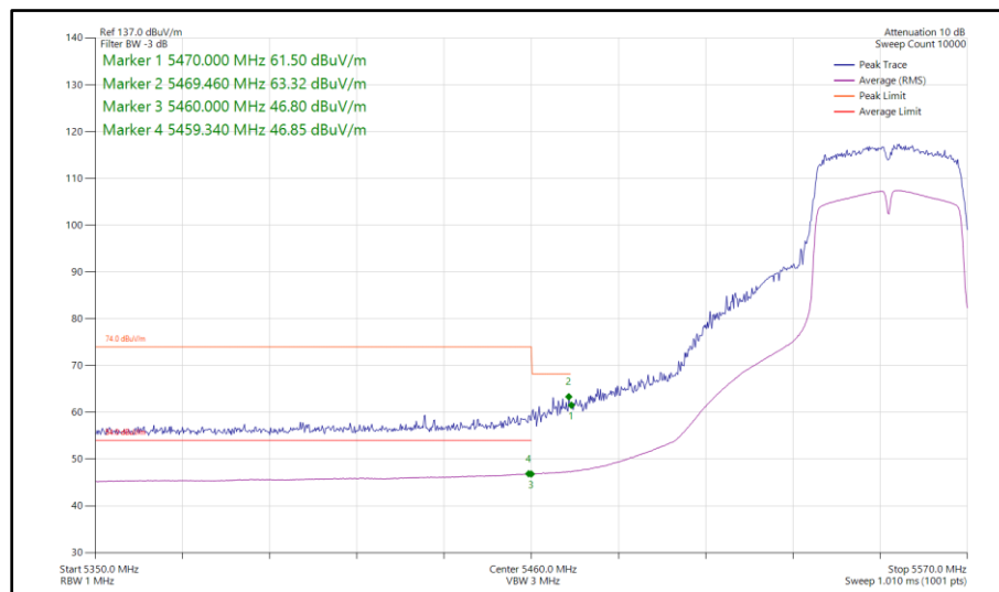
Figure 613 - 802.11ac VHT40, TxBF, Core 0-1 - 5550 MHz Band Edge Frequency 5470 MHz
