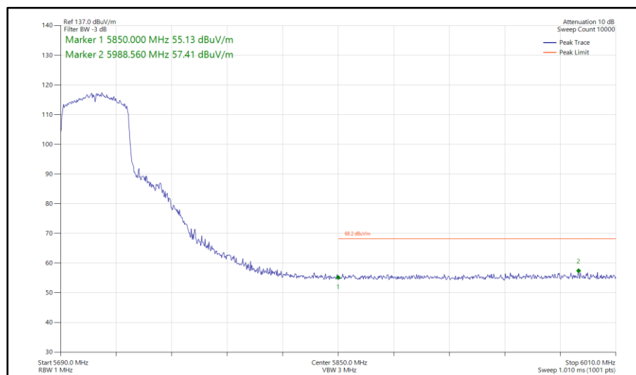
Figure 626 - 802.11ax HE40, SU, TxBF, Core 0-1 - 5710 MHz Band Edge Frequency 5850 MHz
