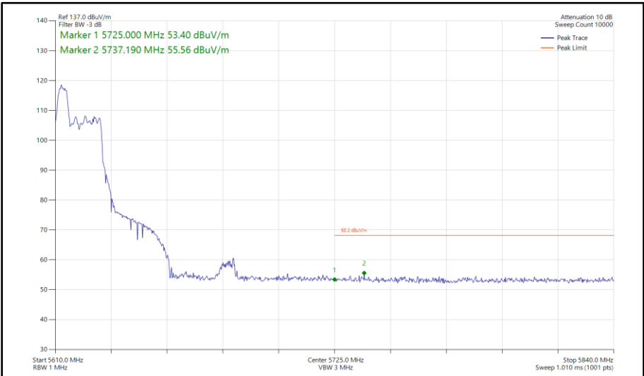
Figure 599 - 802.11ax HE40, RU 52-37, SDM, Core 0-1 - 5630 MHz Band Edge Frequency 5725 MHz
