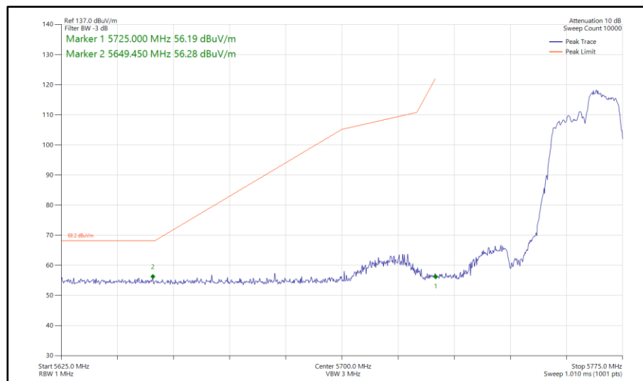
Figure 594 - 802.11ax HE40, RU 106-56, SDM, Core 0-1 - 5755 MHz Band Edge Frequency 5725 MHz
