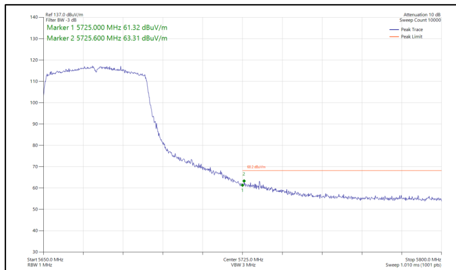
Figure 623 - 802.11ax HE40, SU, TxBF, Core 0-1 - 5670 MHz Band Edge Frequency 5725 MHz
