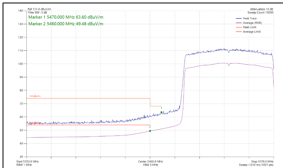
Figure 630 - 802.11ax HE80, SU, SISO, Core 0 - 5530 MHz Band Edge Frequency 5470 MHz
