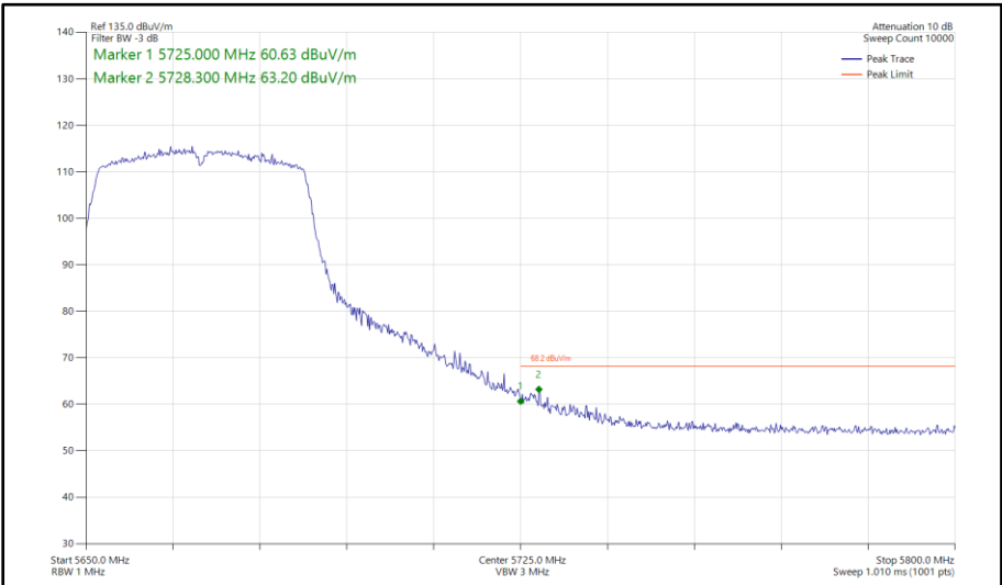
Figure 597 - 802.11n HT40, SDM, Core 0-1 - 5670 MHz Band Edge Frequency 5725 MHz
