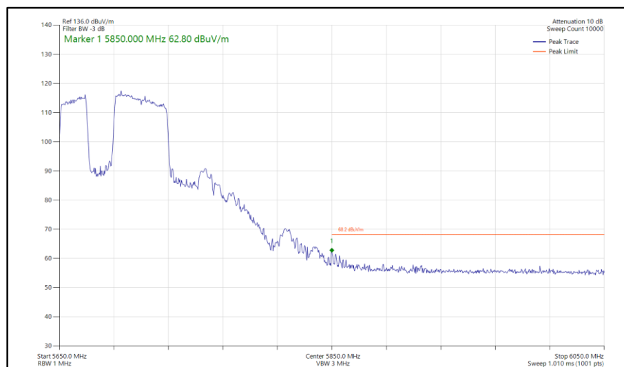
Figure 651 - 802.11be EHT80, RU 484+242-91, SISO, Core 0 - 5690 MHz Band Edge Frequency 5850 MHz
