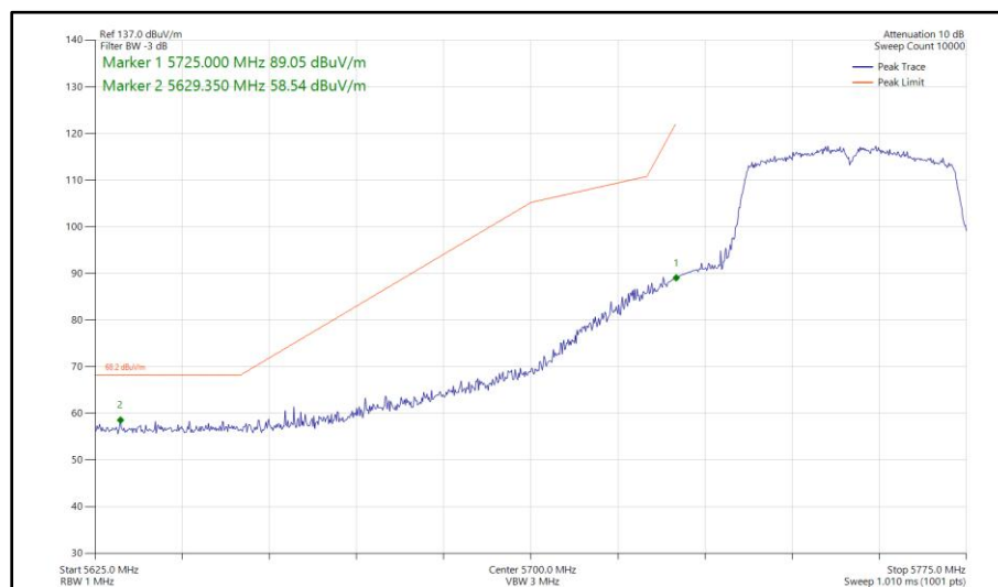
Figure 618 - 802.11ac VHT40, TxBF, Core 0-1 - 5755 MHz Band Edge Frequency 5725 MHz
