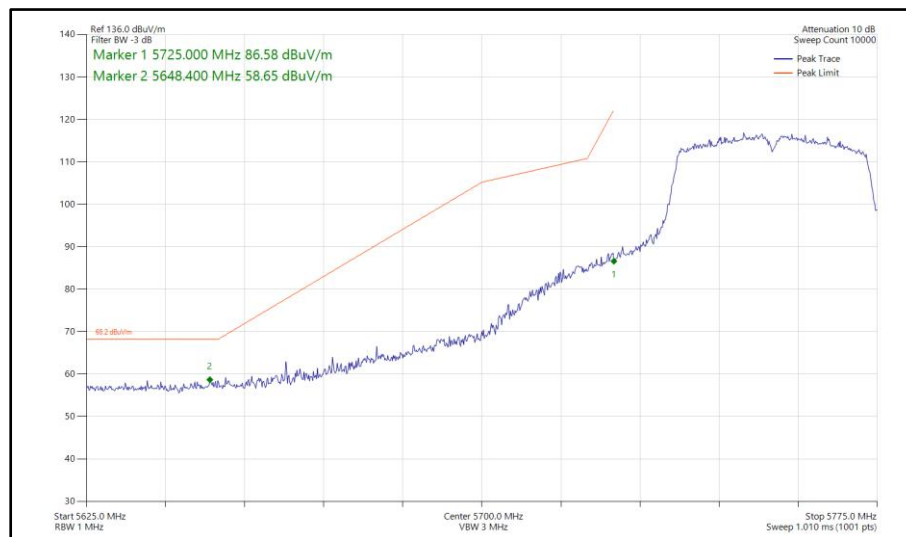
Figure 592 - 802.11n HT40, SDM, Core 0-1 - 5755 MHz Band Edge Frequency 5725 MHz
