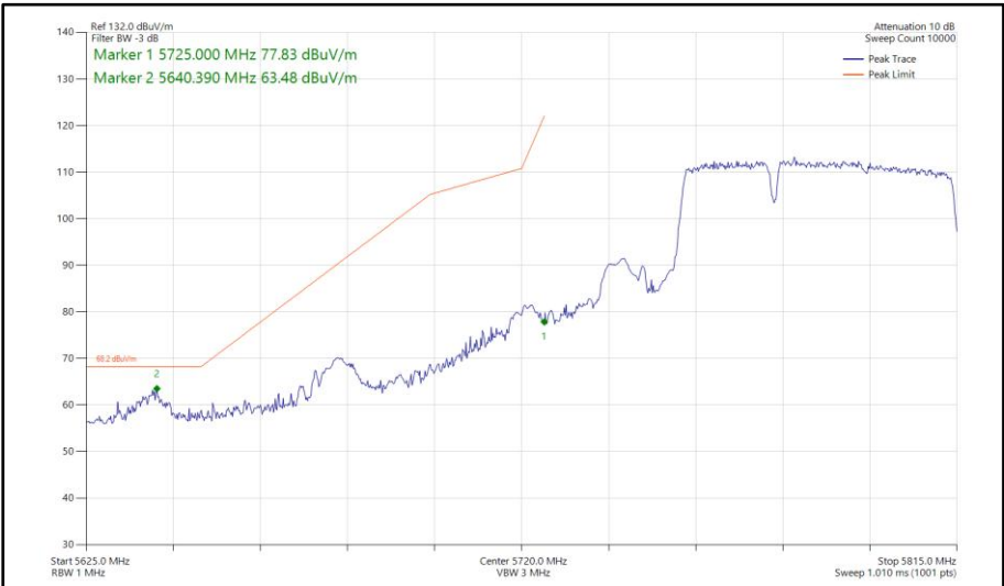
Figure 637 - 802.11be EHT80, RU 484+242-90, SISO, Core 0 - 5775 MHz Band Edge Frequency 5725 MHz
