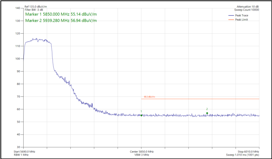
Figure 604 - 802.11n HT40, SDM, Core 0-1 - 5710 MHz Band Edge Frequency 5850 MHz
