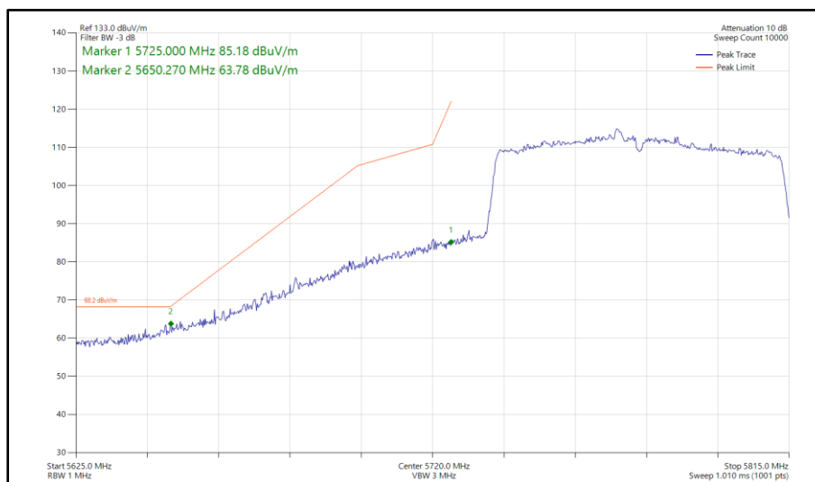
Figure 707 - 802.11ac VHT80, SDM, Core 0-1 - 5775 MHz Band Edge Frequency 5725 MHz
