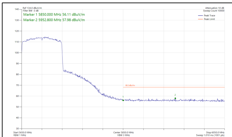
Figure 717 - 802.11ax HE80, SU, SDM, Core 0-1 - 5690 MHz Band Edge Frequency 5850 MHz
