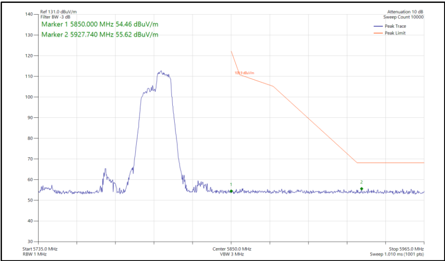
Figure 675 - 802.11ax HE80, RU 106-60, SISO, Core 1 - 5775 MHz Band Edge Frequency 5850 MHz
