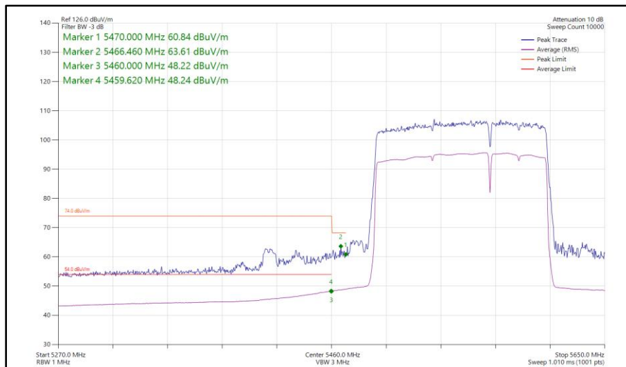
Figure 737 - 802.11be EHT160, RU 996+484-95S, SISO, Core 0 - 5570 MHz Band Edge Frequency 5470 MHz
