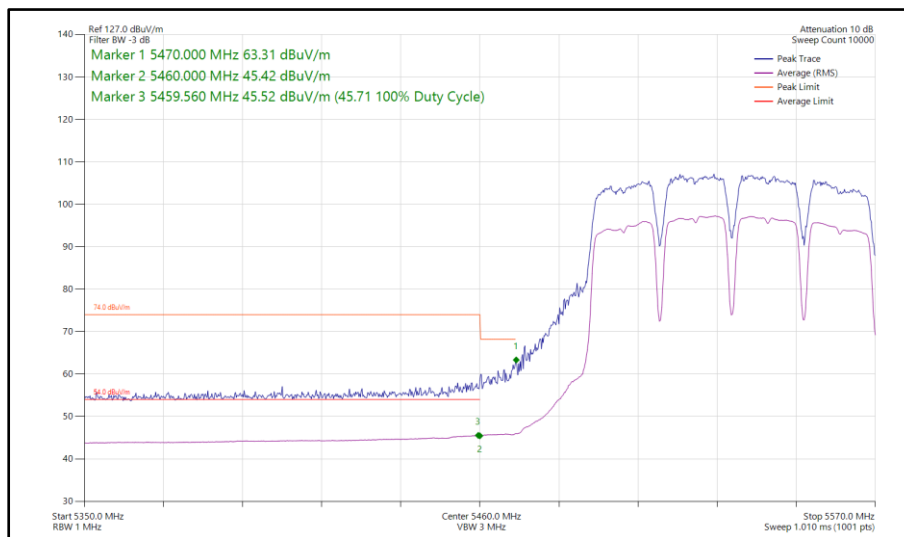
Figure 678 - 802.11a a80, CDD, Core 0-1 - 5530 MHz Band Edge Frequency 5470 MHz
