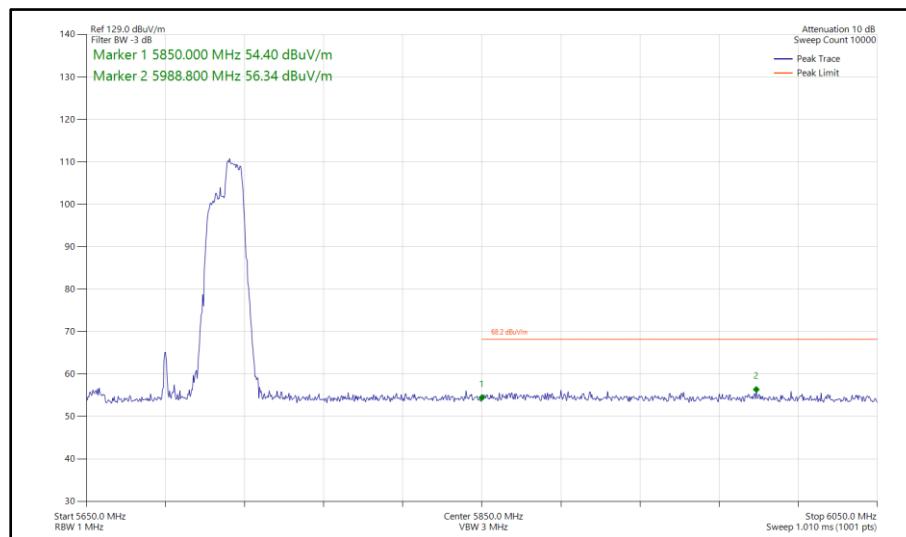
Figure 673 - 802.11ax HE80, RU 106-60, SISO, Core 1 - 5690 MHz Band Edge Frequency 5850 MHz
