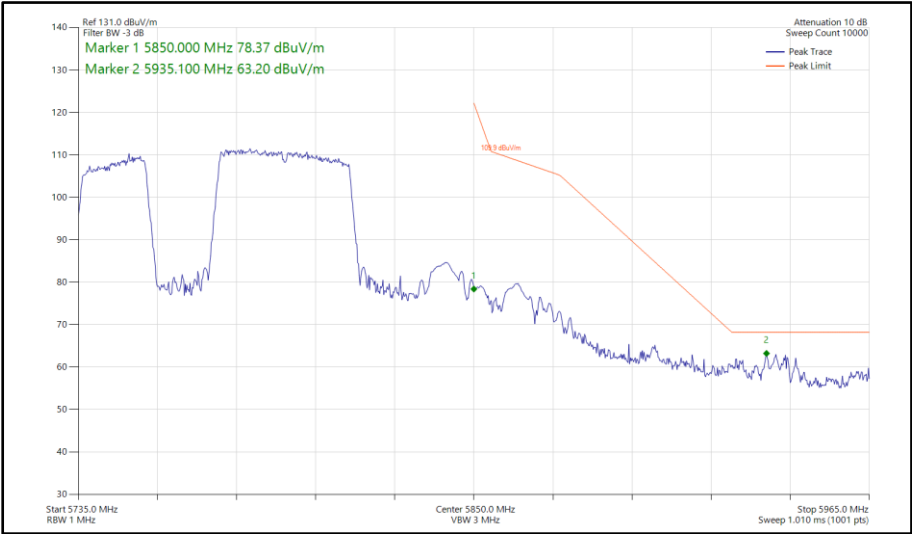
Figure 677 - 802.11be EHT80, RU 484+242-91, SISO, Core 1 - 5775 MHz Band Edge Frequency 5850 MHz
