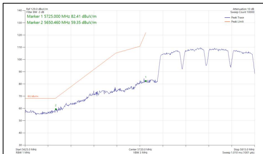
Figure 658 - 802.11a a80, SISO, Core 1 - 5775 MHz Band Edge Frequency 5725 MHz
