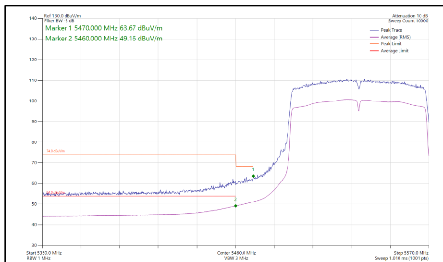
Figure 723 - 802.11ac VHT80, TxBF, Core 0-1 - 5530 MHz Band Edge Frequency 5470 MHz
