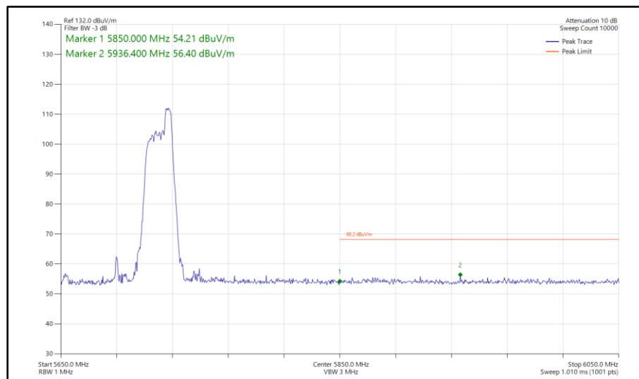
Figure 698 - 802.11ax HE80, RU 52-52, CDD, Core 0-1 - 5690 MHz Band Edge Frequency 5850 MHz
