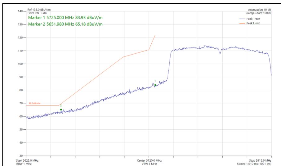
Figure 725 - 802.11ac VHT80, TxBF, Core 0-1 - 5775 MHz Band Edge Frequency 5725 MHz
