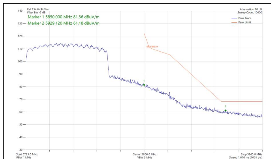
Figure 699 - 802.11ax HE80, SU, CDD, Core 0-1 - 5775 MHz Band Edge Frequency 5850 MHz
