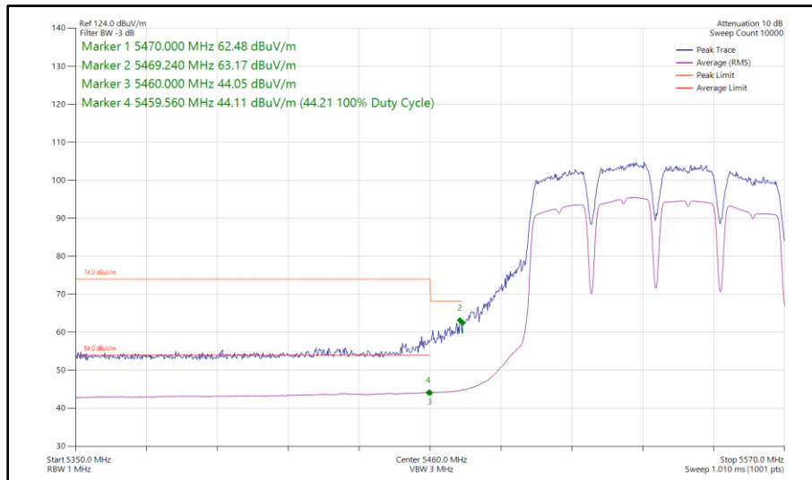
Figure 653 - 802.11a a80, SISO, Core 1 - 5530 MHz Band Edge Frequency 5470 MHz
