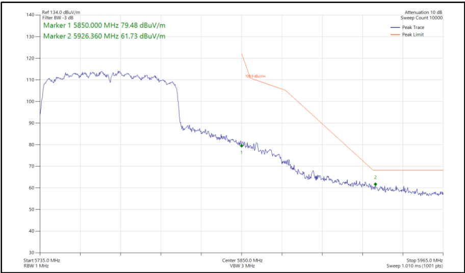
Figure 696 - 802.11ac VHT80, CDD, Core 0-1 - 5775 MHz Band Edge Frequency 5850 MHz
