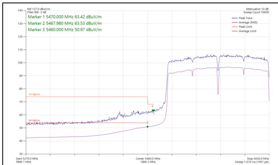
Figure 734 - 802.11ac VHT160, SISO, Core 0 - 5570 MHz Band Edge Frequency 5470 MHz
