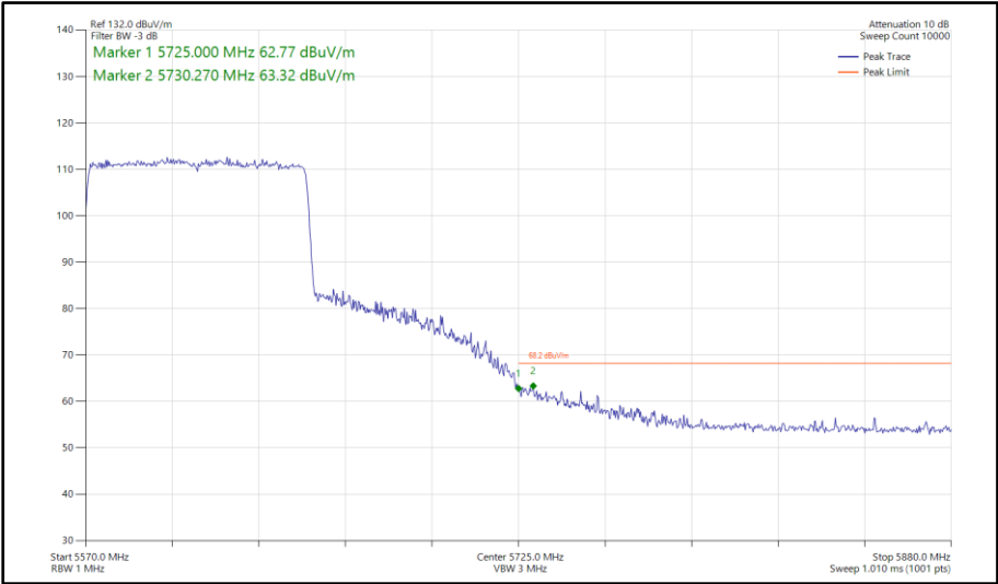
Figure 728 - 802.11ax HE80, SU, TxBF, Core 0-1 - 5610 MHz Band Edge Frequency 5725 MHz
