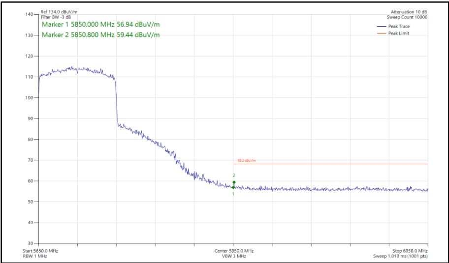
Figure 697 - 802.11ax HE80, SU, CDD, Core 0-1 - 5690 MHz Band Edge Frequency 5850 MHz
