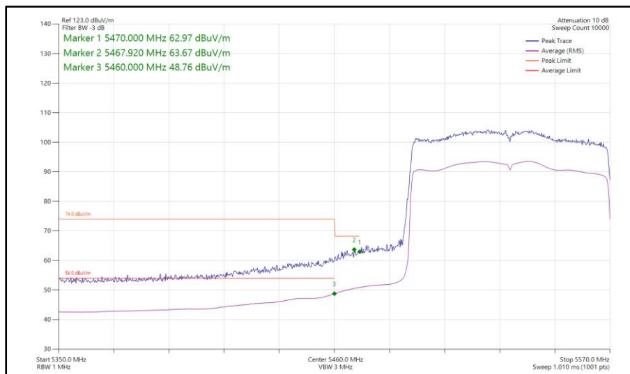
Figure 655 - 802.11ax HE80, SU, SISO, Core 1 - 5530 MHz Band Edge Frequency 5470 MHz
