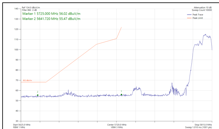
Figure 709 - 802.11ax HE80, RU 106-60, SDM, Core 0-1 - 5775 MHz Band Edge Frequency 5725 MHz
