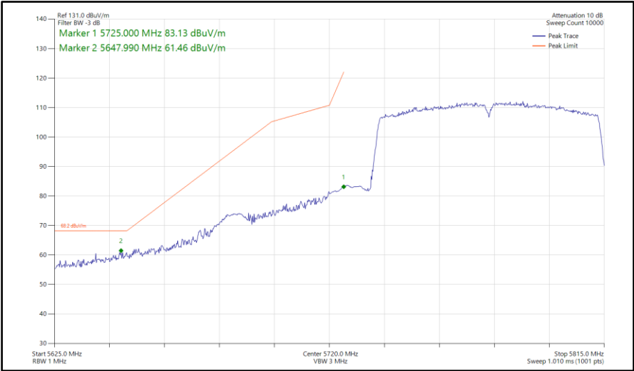
Figure 659 - 802.11ac VHT80, SISO, Core 1 - 5775 MHz Band Edge Frequency 5725 MHz
