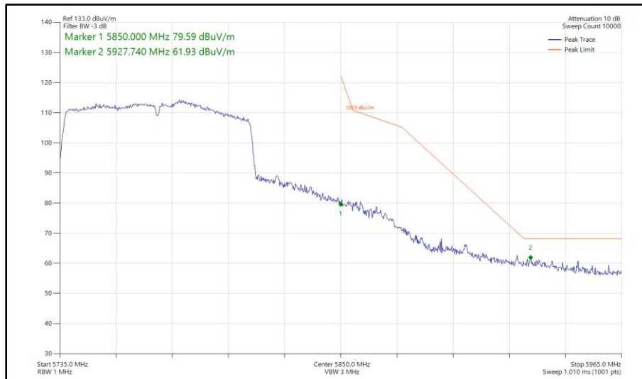
Figure 730 - 802.11ac VHT80, TxBF, Core 0-1 - 5775 MHz Band Edge Frequency 5850 MHz
