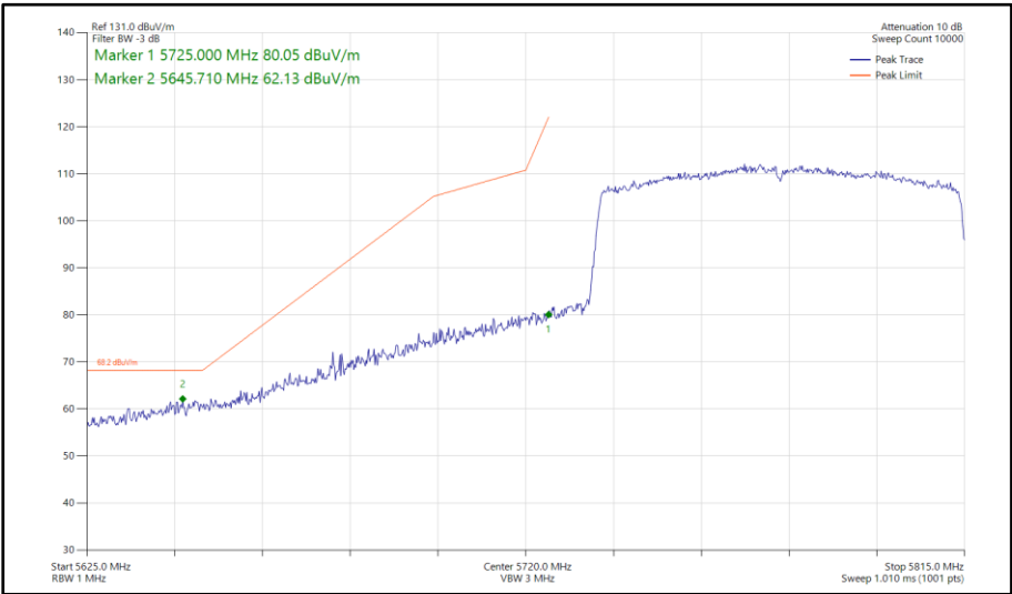
Figure 660 - 802.11ax HE80, SU, SISO, Core 1 - 5775 MHz Band Edge Frequency 5725 MHz
