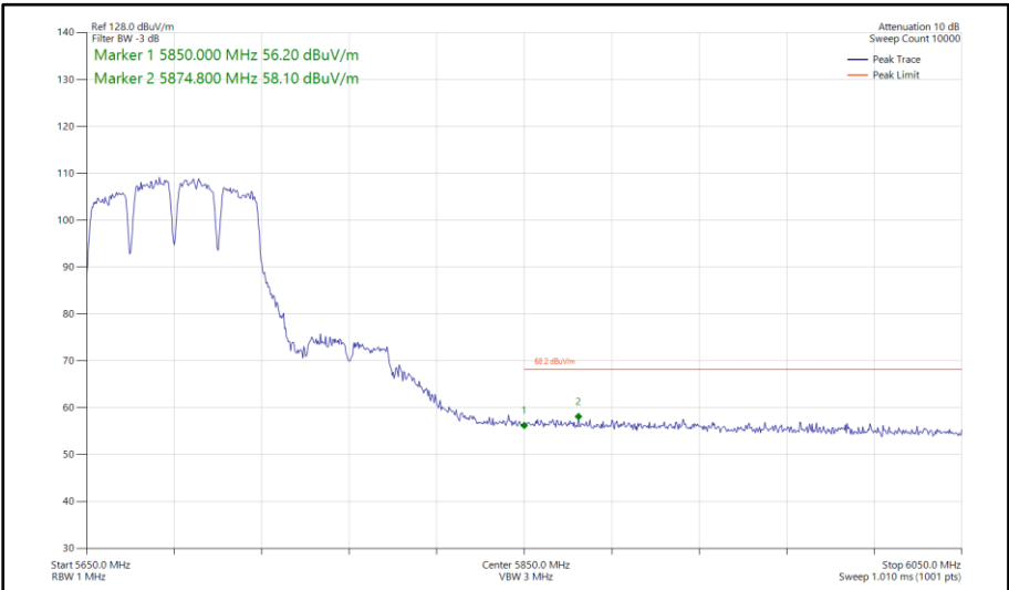
Figure 668 - 802.11a a80, SISO, Core 1 - 5690 MHz Band Edge Frequency 5850 MHz
