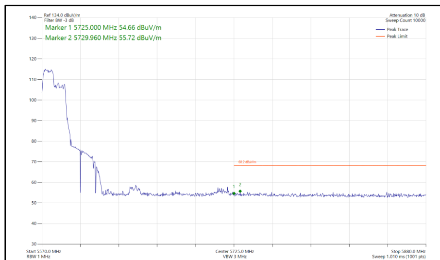
Figure 691 - 802.11ax HE80, RU 106-53, CDD, Core 0-1 - 5610 MHz Band Edge Frequency 5725 MHz
