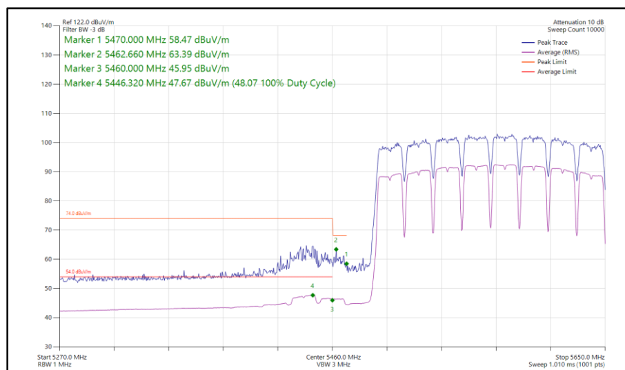
Figure 733 - 802.11a a160, SISO, Core 0 - 5570 MHz Band Edge Frequency 5470 MHz
