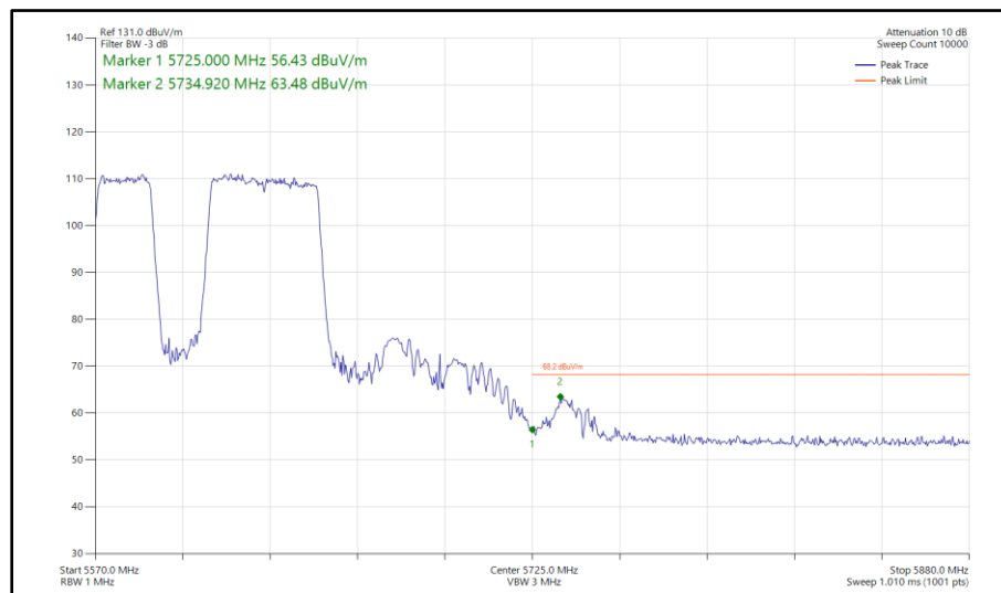
Figure 692 - 802.11be EHT80, RU 484+242-91, CDD, Core 0-1 - 5610 MHz Band Edge Frequency 5725 MHz
