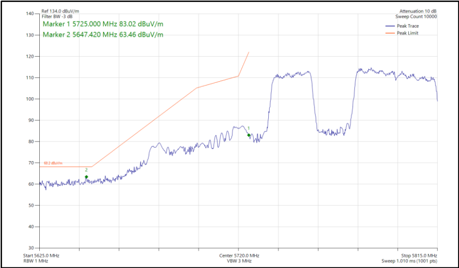
Figure 710 - 802.11be EHT80, RU 484+242-91, SDM, Core 0-1 - 5775 MHz Band Edge Frequency 5725 MHz
