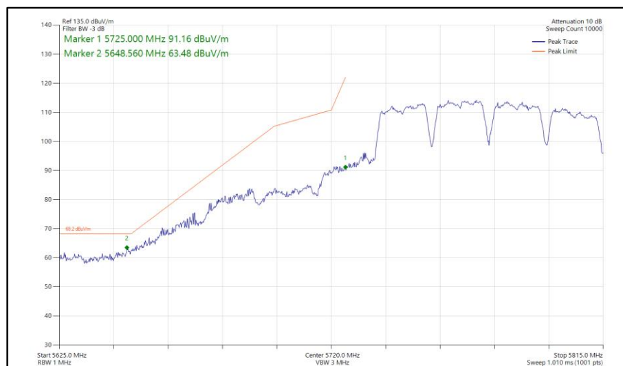
Figure 683 - 802.11a a80, CDD, Core 0-1 - 5775 MHz Band Edge Frequency 5725 MHz
