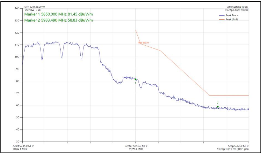
Figure 694 - 802.11a a80, CDD, Core 0-1 - 5775 MHz Band Edge Frequency 5850 MHz
