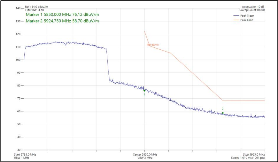
Figure 732 - 802.11ax HE80, SU, TxBF, Core 0-1 - 5775 MHz Band Edge Frequency 5850 MHz
