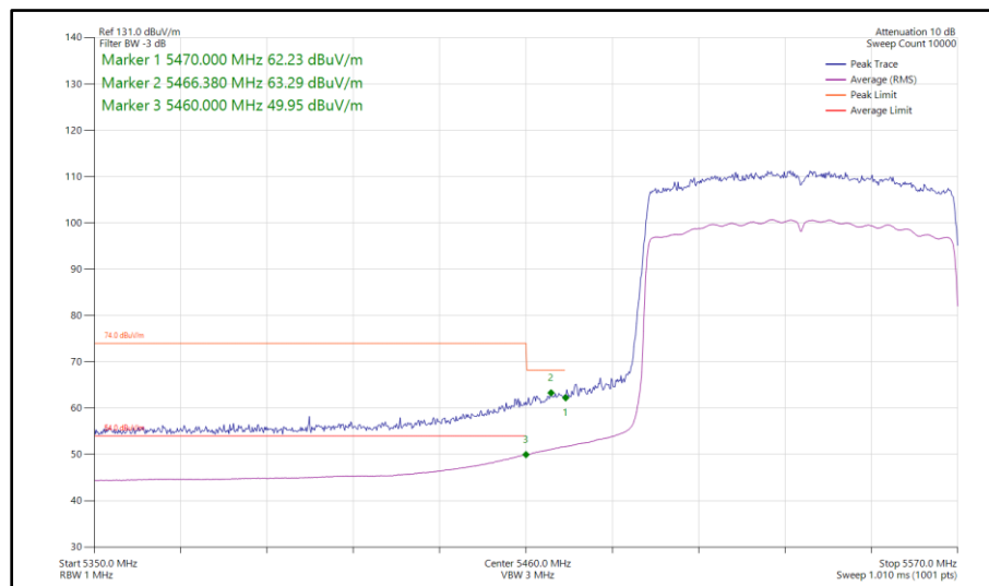
Figure 680 - 802.11ax HE80, SU, CDD, Core 0-1 - 5530 MHz Band Edge Frequency 5470 MHz
