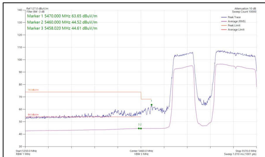
Figure 657 - 802.11be EHT80, RU 484+242-91, SISO, Core 1 - 5530 MHz Band Edge Frequency 5470 MHz
