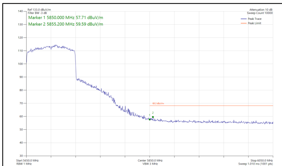
Figure 731 - 802.11ax HE80, SU, TxBF, Core 0-1 - 5690 MHz Band Edge Frequency 5850 MHz
