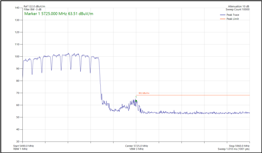
Figure 738 - 802.11a a160, SISO, Core 0 - 5570 MHz Band Edge Frequency 5725 MHz
