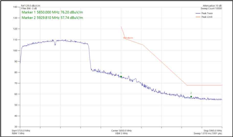
Figure 671 - 802.11ac VHT80, SISO, Core 1 - 5775 MHz Band Edge Frequency 5850 MHz
