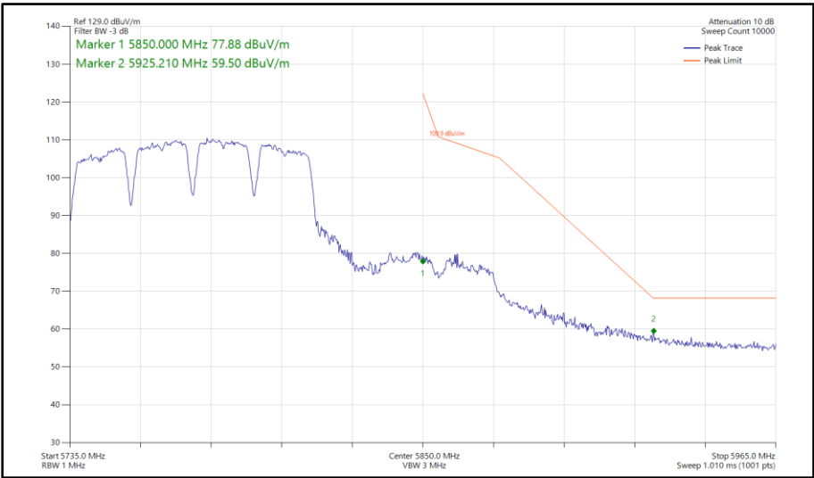
Figure 669 - 802.11a a80, SISO, Core 1 - 5775 MHz Band Edge Frequency 5850 MHz
