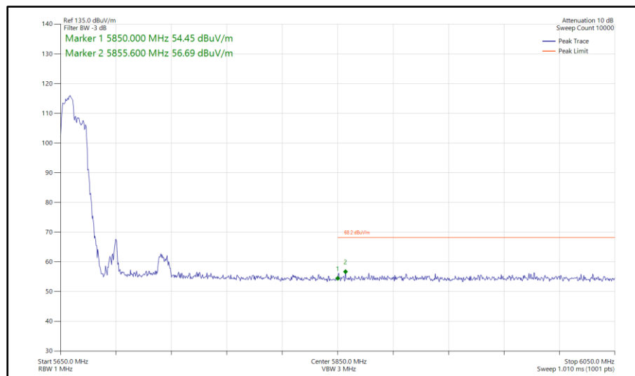
Figure 718 - 802.11ax HE80, RU 106-53, SDM, Core 0-1 - 5690 MHz Band Edge Frequency 5850 MHz
