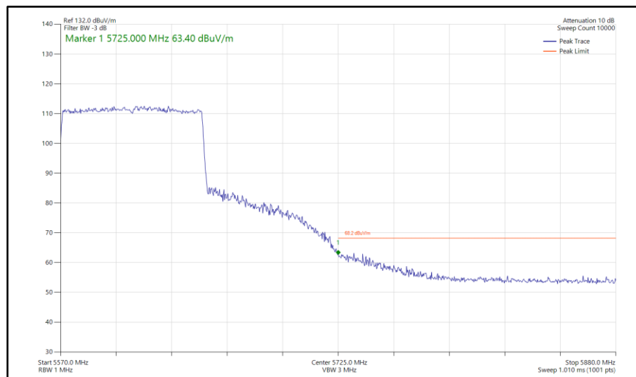
Figure 712 - 802.11ax HE80, SU, SDM, Core 0-1 - 5610 MHz Band Edge Frequency 5725 MHz
