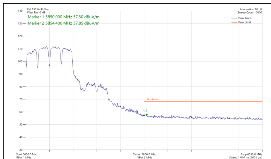
Figure 693 - 802.11a a80, CDD, Core 0-1 - 5690 MHz Band Edge Frequency 5850 MHz
