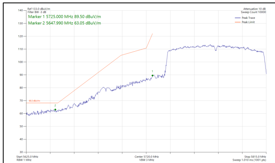
Figure 684 - 802.11ac VHT80, CDD, Core 0-1 - 5775 MHz Band Edge Frequency 5725 MHz
