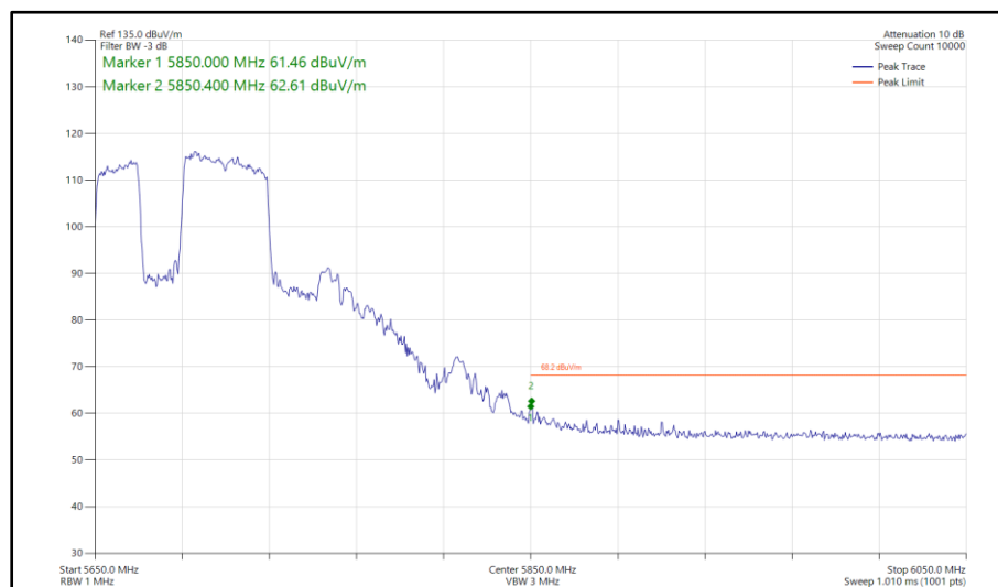
Figure 721 - 802.11be EHT80, RU 484+242-91, SDM, Core 0-1 - 5690 MHz Band Edge Frequency 5850 MHz
