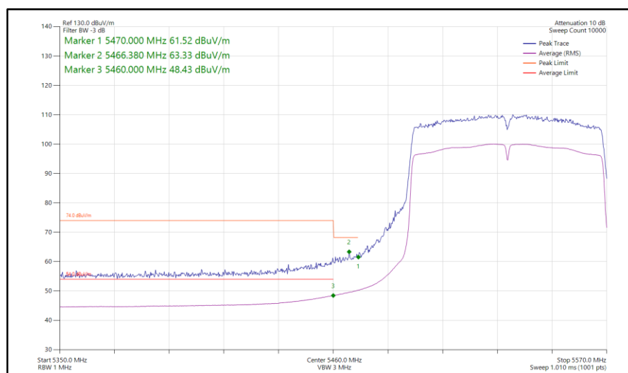
Figure 703 - 802.11ac VHT80, SDM, Core 0-1 - 5530 MHz Band Edge Frequency 5470 MHz
