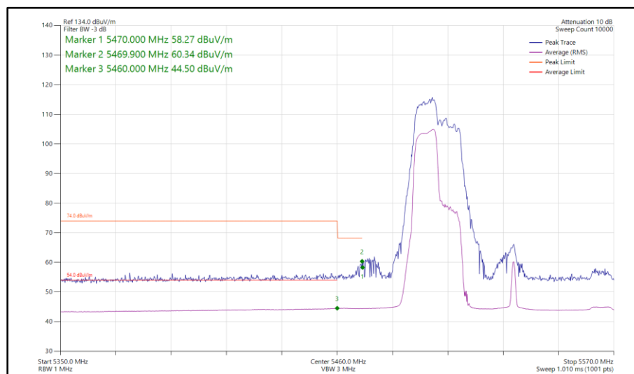
Figure 681 - 802.11ax HE80, RU 106-53, CDD, Core 0-1 - 5530 MHz Band Edge Frequency 5470 MHz
