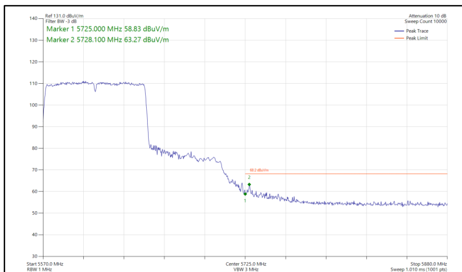
Figure 727 - 802.11ac VHT80, TxBF, Core 0-1 - 5610 MHz Band Edge Frequency 5725 MHz
