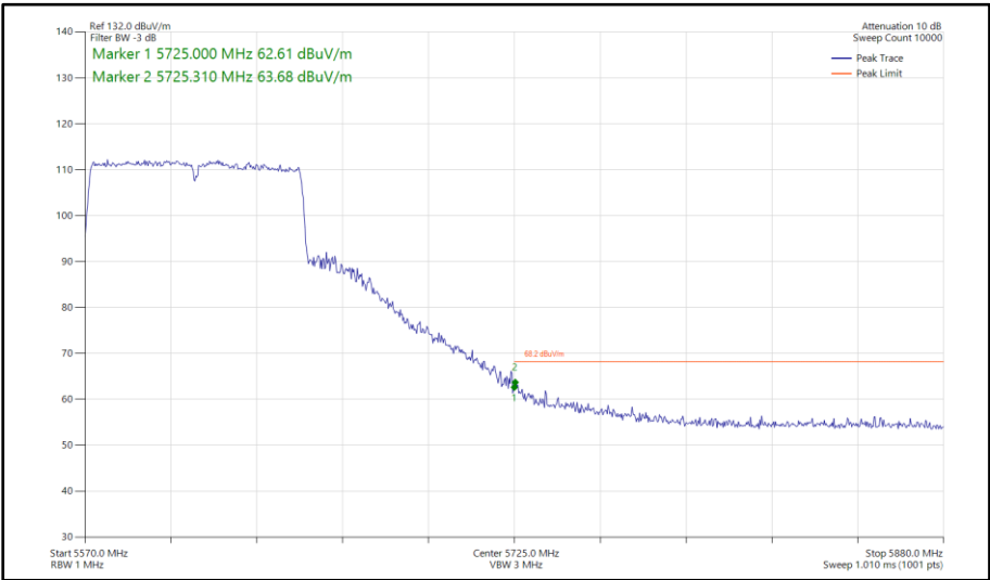
Figure 711 - 802.11ac VHT80, SDM, Core 0-1 - 5610 MHz Band Edge Frequency 5725 MHz
