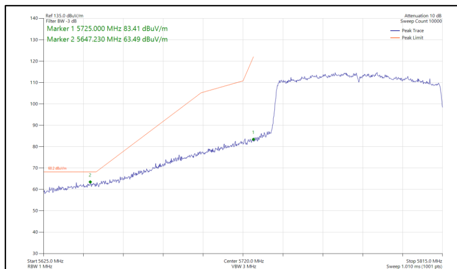
Figure 685 - 802.11ax HE80, SU, CDD, Core 0-1 - 5775 MHz Band Edge Frequency 5725 MHz
