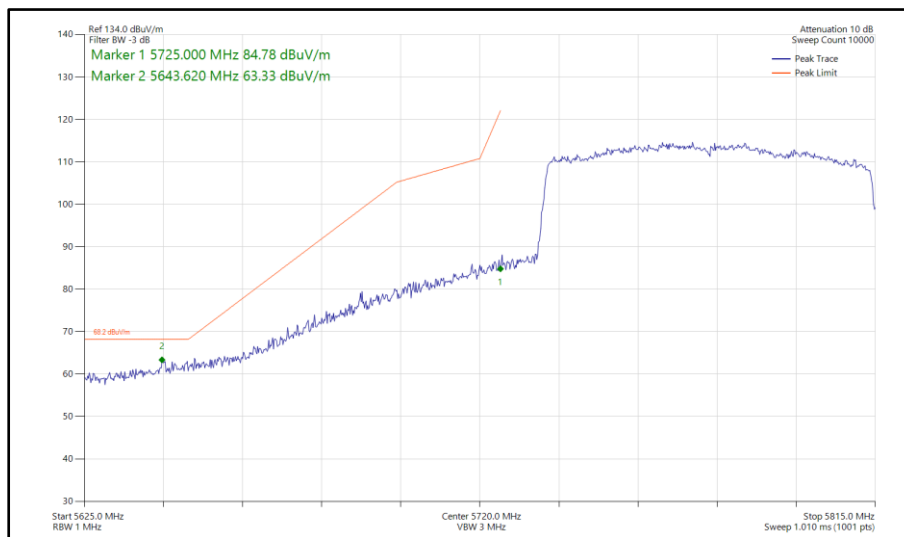
Figure 726 - 802.11ax HE80, SU, TxBF, Core 0-1 - 5775 MHz Band Edge Frequency 5725 MHz
