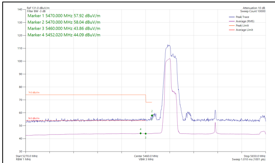
Figure 736 - 802.11ax HE160, RU 106-53P, SISO, Core 0 - 5570 MHz Band Edge Frequency 5470 MHz
