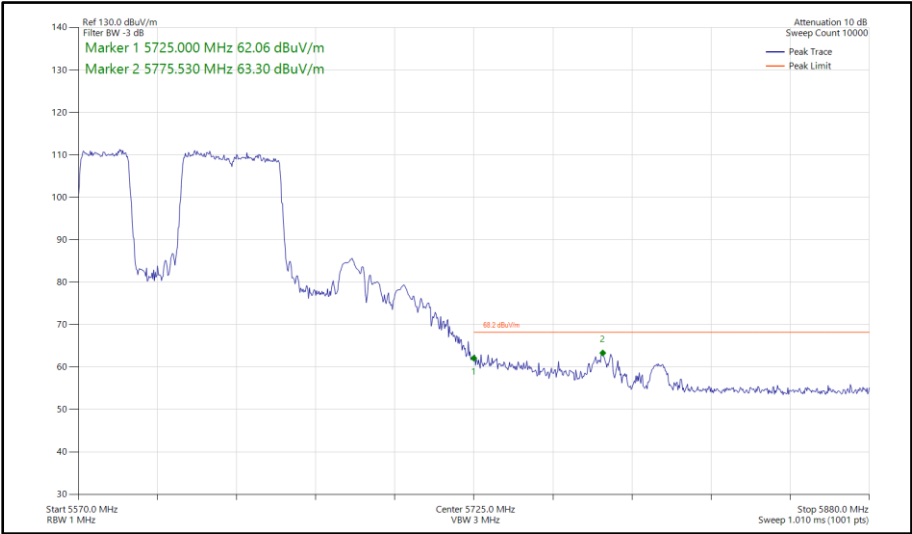
Figure 667 - 802.11be EHT80, RU 484+242-91, SISO, Core 1 - 5610 MHz Band Edge Frequency 5725 MHz
