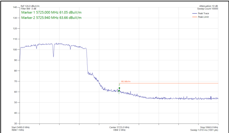
Figure 739 - 802.11ac VHT160, SISO, Core 0 - 5570 MHz Band Edge Frequency 5725 MHz
