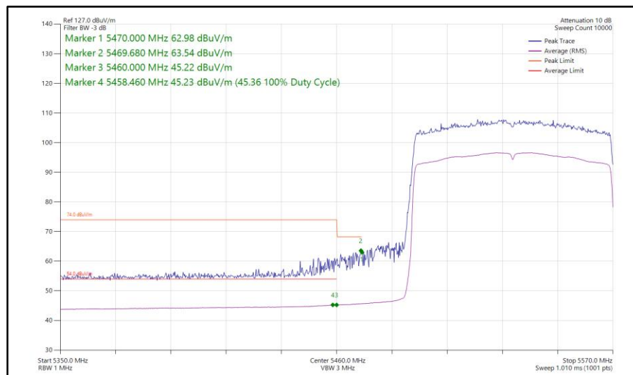
Figure 704 - 802.11ax HE80, SU, SDM, Core 0-1 - 5530 MHz Band Edge Frequency 5470 MHz
