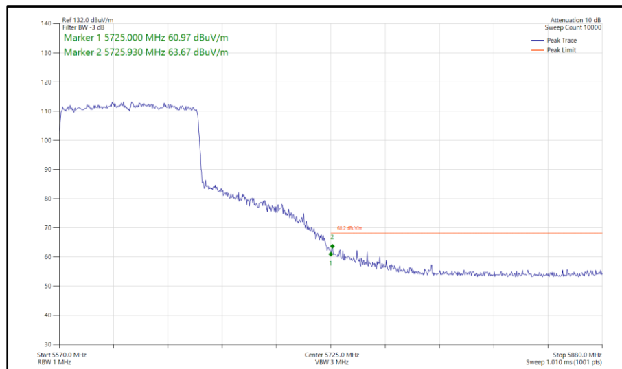
Figure 690 - 802.11ax HE80, SU, CDD, Core 0-1 - 5610 MHz Band Edge Frequency 5725 MHz
