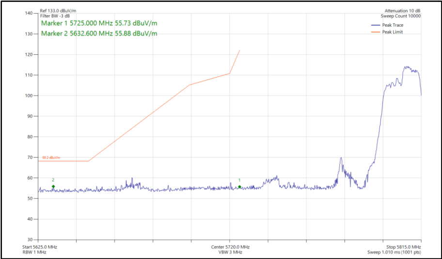
Figure 686 - 802.11ax HE80, RU 106-60, CDD, Core 0-1 - 5775 MHz Band Edge Frequency 5725 MHz
