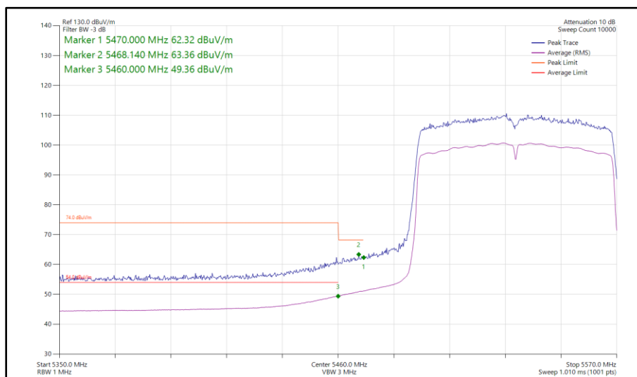
Figure 679 - 802.11ac VHT80, CDD, Core 0-1 - 5530 MHz Band Edge Frequency 5470 MHz
