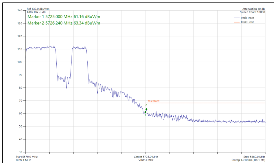
Figure 714 - 802.11be EHT80, RU 484+242-92, SDM, Core 0-1 - 5610 MHz Band Edge Frequency 5725 MHz
