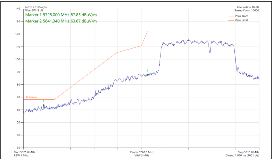
Figure 687 - 802.11be EHT80, RU 484+242-93, CDD, Core 0-1 - 5775 MHz Band Edge Frequency 5725 MHz
