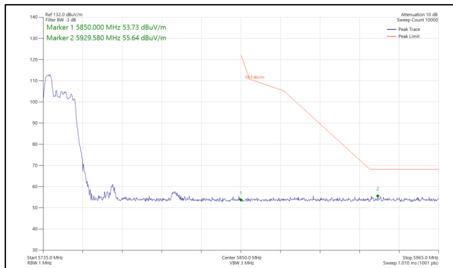
Figure 720 - 802.11ax HE80, RU 52-37, SDM, Core 0-1 - 5775 MHz Band Edge Frequency 5850 MHz
