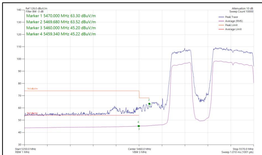
Figure 706 - 802.11be EHT80, RU 484+242-91, SDM, Core 0-1 - 5530 MHz Band Edge Frequency 5470 MHz
