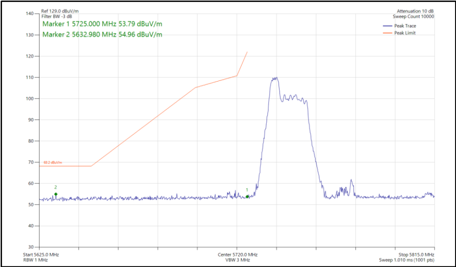
Figure 661 - 802.11ax HE80, RU 52-37, SISO, Core 1 - 5775 MHz Band Edge Frequency 5725 MHz
