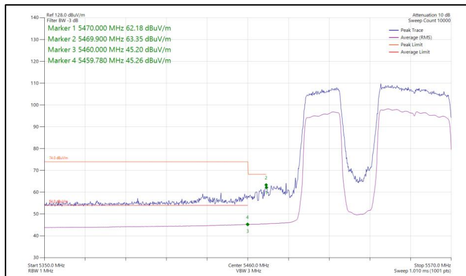
Figure 682 - 802.11be EHT80, RU 484+242-91, CDD, Core 0-1 - 5530 MHz Band Edge Frequency 5470 MHz
