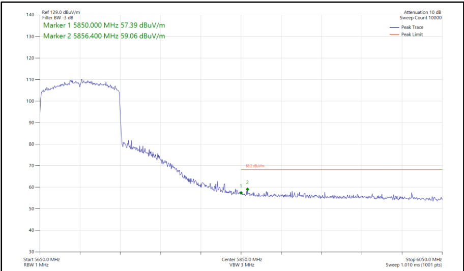
Figure 672 - 802.11ax HE80, SU, SISO, Core 1 - 5690 MHz Band Edge Frequency 5850 MHz
