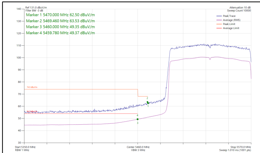
Figure 724 - 802.11ax HE80, SU, TxBF, Core 0-1 - 5530 MHz Band Edge Frequency 5470 MHz
