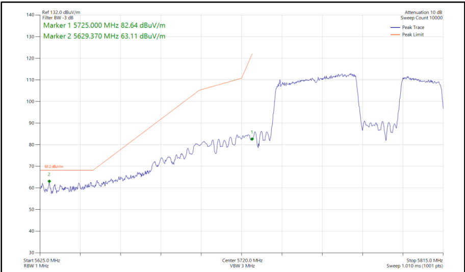
Figure 662 - 802.11be EHT80, RU 484+242-92, SISO, Core 1 - 5775 MHz Band Edge Frequency 5725 MHz
