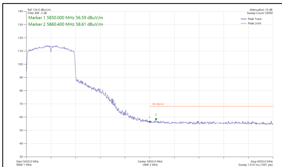
Figure 715 - 802.11ac VHT80, SDM, Core 0-1 - 5690 MHz Band Edge Frequency 5850 MHz
