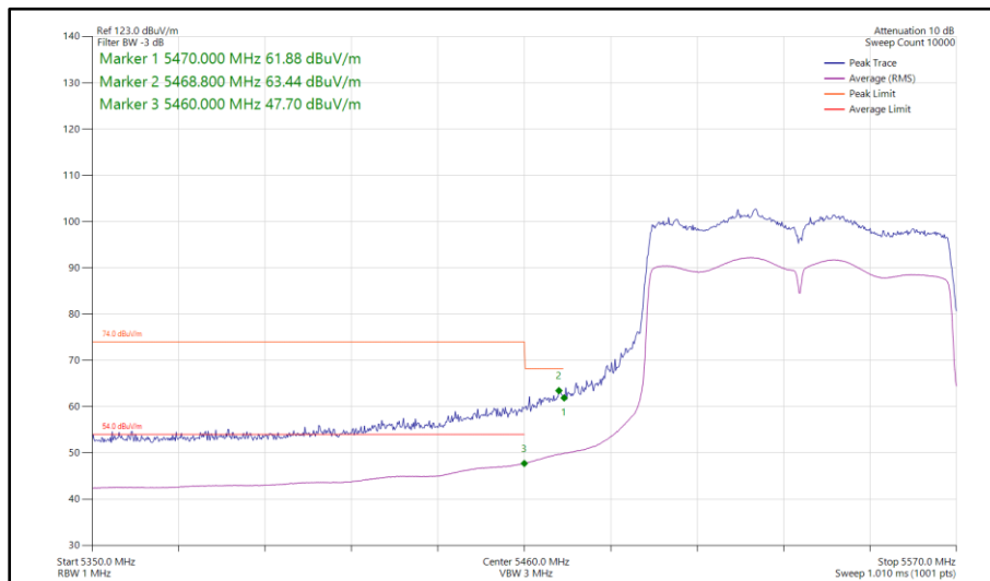
Figure 654 - 802.11ac VHT80, SISO, Core 1 - 5530 MHz Band Edge Frequency 5470 MHz
