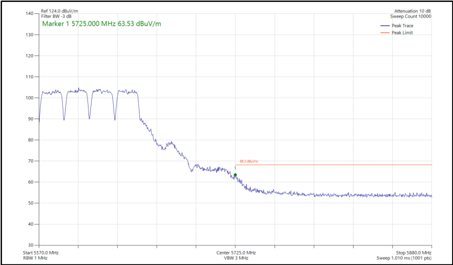
Figure 663 - 802.11a a80, SISO, Core 1 - 5610 MHz Band Edge Frequency 5725 MHz
