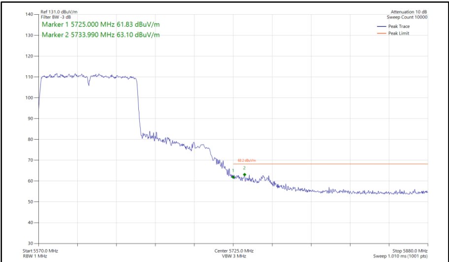
Figure 689 - 802.11ac VHT80, CDD, Core 0-1 - 5610 MHz Band Edge Frequency 5725 MHz
