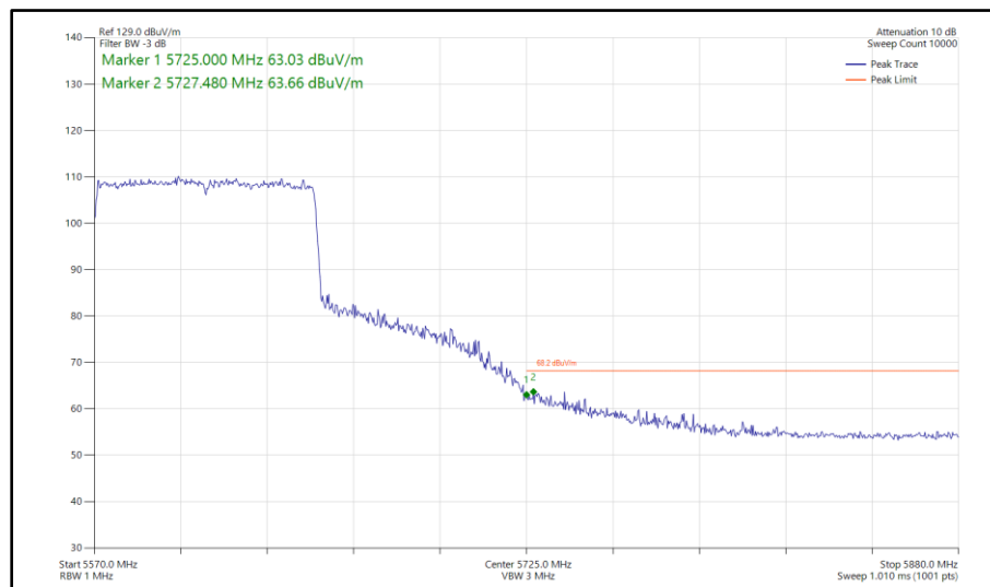
Figure 665 - 802.11ax HE80, SU, SISO, Core 1 - 5610 MHz Band Edge Frequency 5725 MHz
