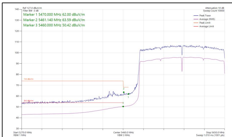
Figure 735 - 802.11ax HE160, SU, SISO, Core 0 - 5570 MHz Band Edge Frequency 5470 MHz
