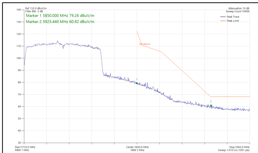
Figure 716 - 802.11ac VHT80, SDM, Core 0-1 - 5775 MHz Band Edge Frequency 5850 MHz
