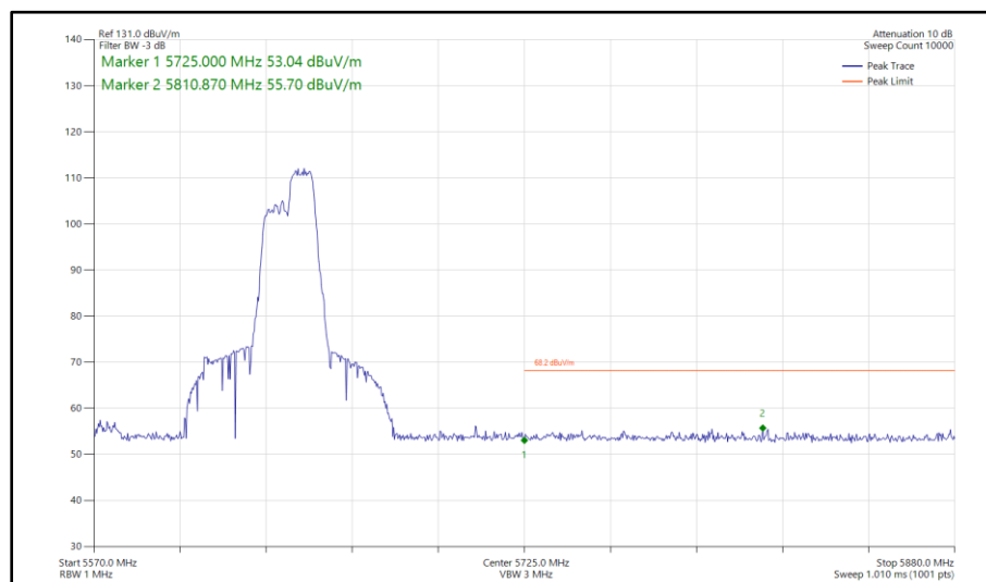
Figure 666 - 802.11ax HE80, RU 106-60, SISO, Core 1 - 5610 MHz Band Edge Frequency 5725 MHz
