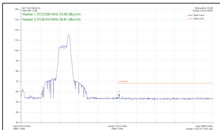
Figure 713 - 802.11ax HE80, RU 52-52, SDM, Core 0-1 - 5610 MHz Band Edge Frequency 5725 MHz
