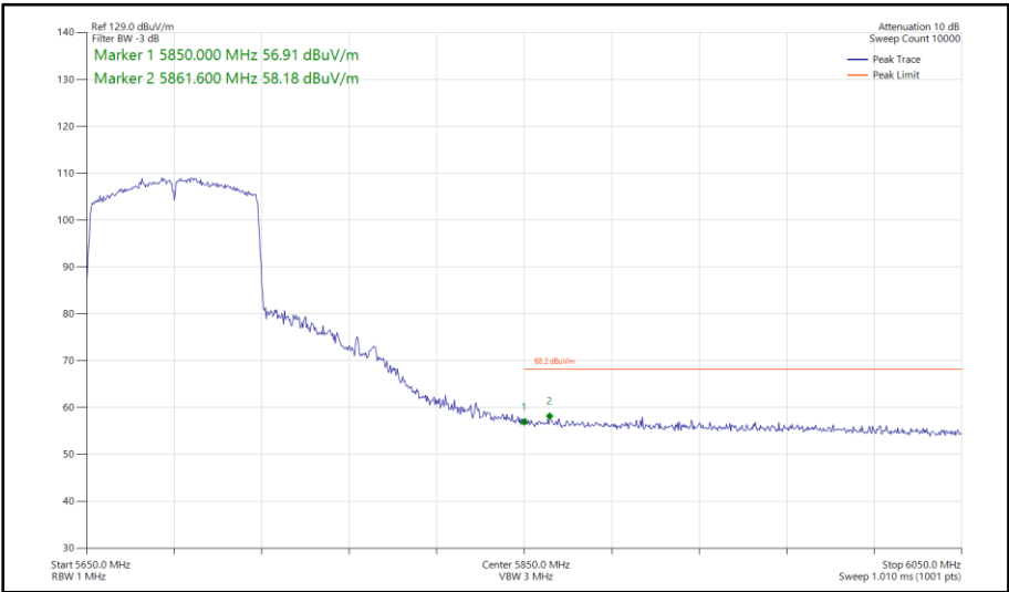
Figure 670 - 802.11ac VHT80, SISO, Core 1 - 5690 MHz Band Edge Frequency 5850 MHz
