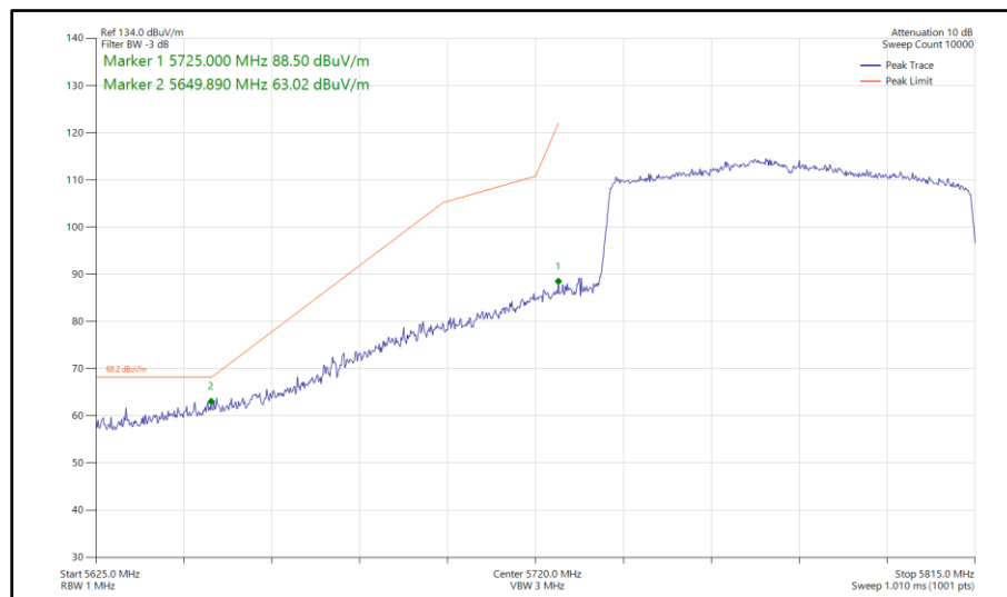
Figure 708 - 802.11ax HE80, SU, SDM, Core 0-1 - 5775 MHz Band Edge Frequency 5725 MHz
