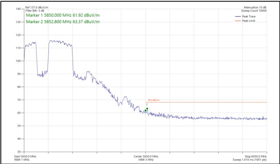
Figure 701 - 802.11be EHT80, RU 484+242-91, CDD, Core 0-1 - 5690 MHz Band Edge Frequency 5850 MHz
