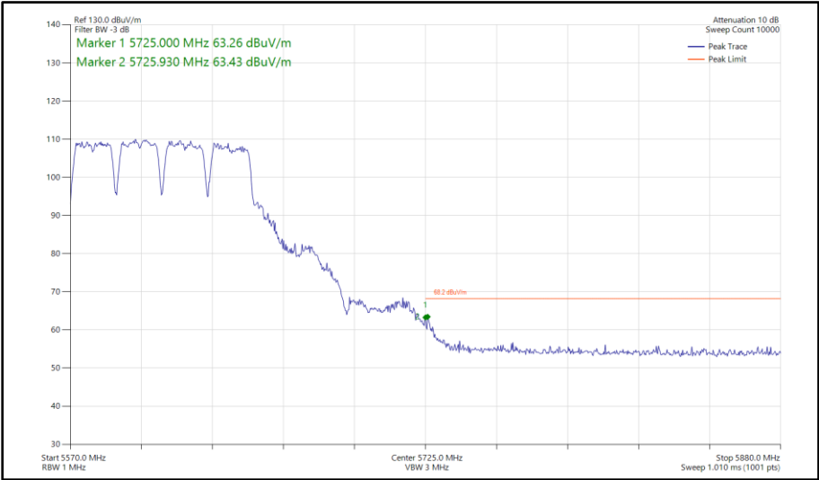
Figure 688 - 802.11a a80, CDD, Core 0-1 - 5610 MHz Band Edge Frequency 5725 MHz
