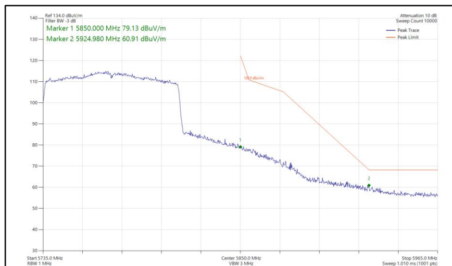
Figure 719 - 802.11ax HE80, SU, SDM, Core 0-1 - 5775 MHz Band Edge Frequency 5850 MHz
