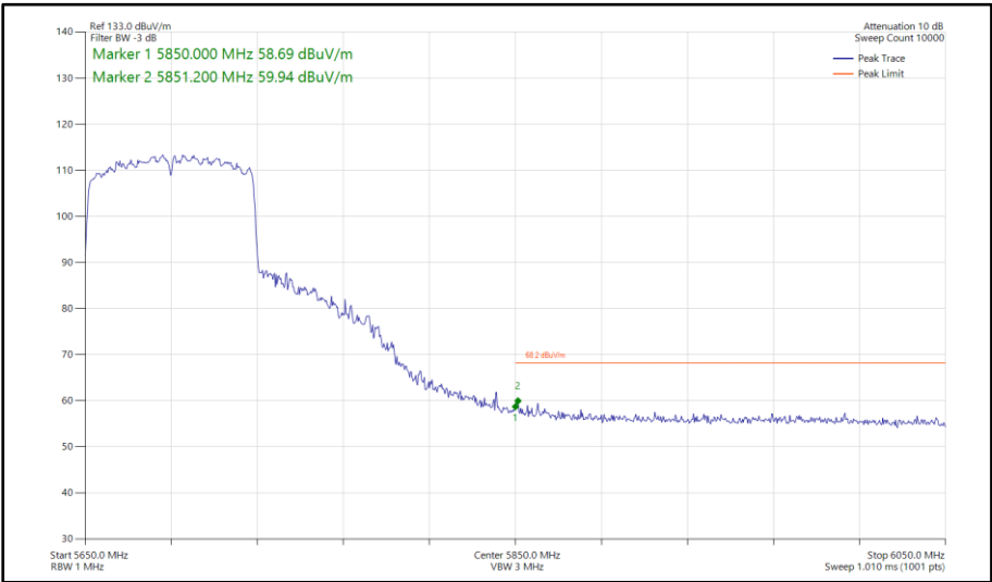
Figure 695 - 802.11ac VHT80, CDD, Core 0-1 - 5690 MHz Band Edge Frequency 5850 MHz
