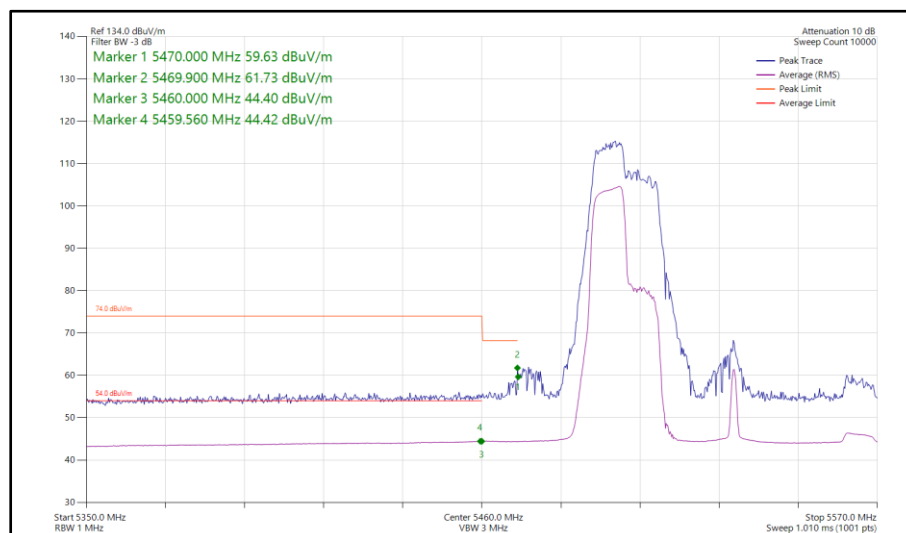
Figure 705 - 802.11ax HE80, RU 106-53, SDM, Core 0-1 - 5530 MHz Band Edge Frequency 5470 MHz
