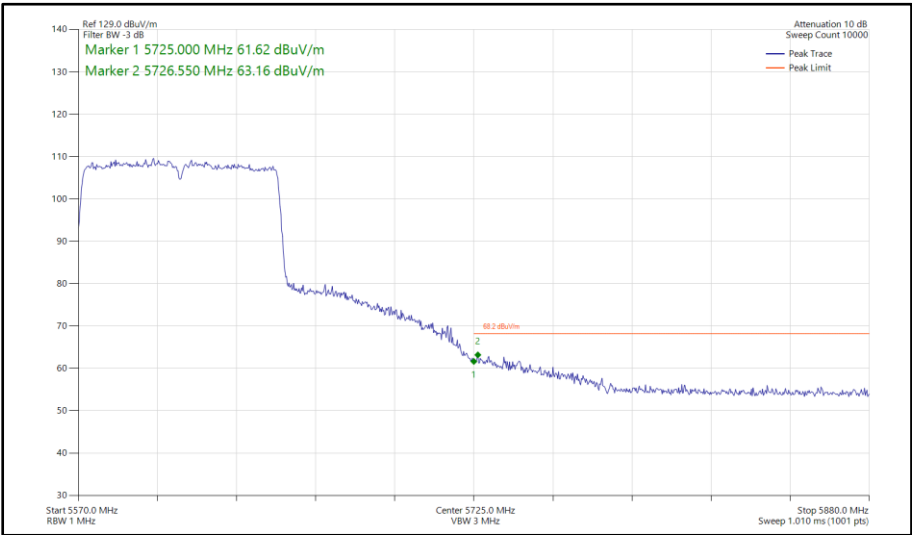
Figure 664 - 802.11ac VHT80, SISO, Core 1 - 5610 MHz Band Edge Frequency 5725 MHz
