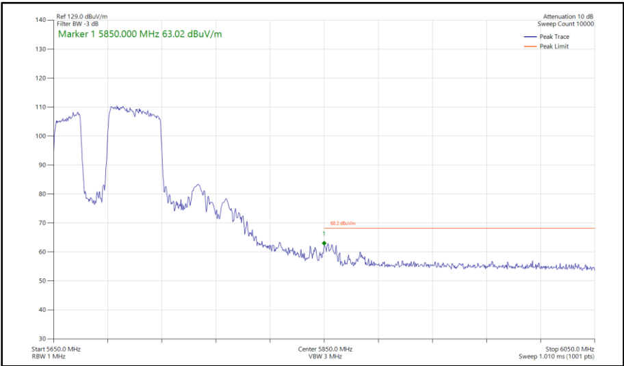
Figure 676 - 802.11be EHT80, RU 484+242-91, SISO, Core 1 - 5690 MHz Band Edge Frequency 5850 MHz
