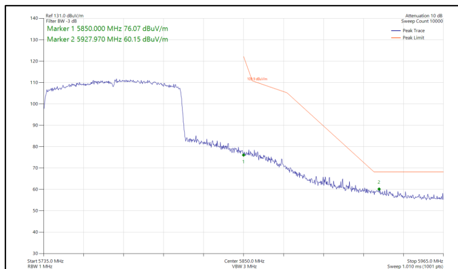
Figure 674 - 802.11ax HE80, SU, SISO, Core 1 - 5775 MHz Band Edge Frequency 5850 MHz
