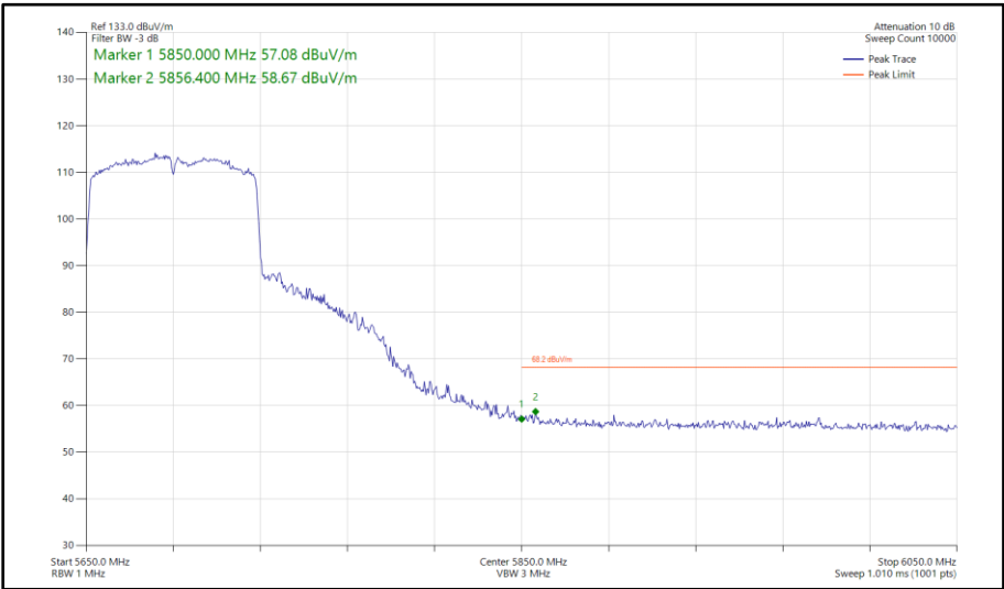
Figure 729 - 802.11ac VHT80, TxBF, Core 0-1 - 5690 MHz Band Edge Frequency 5850 MHz
