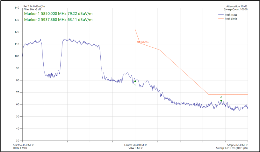
Figure 722 - 802.11be EHT80, RU 484+242-91, SDM, Core 0-1 - 5775 MHz Band Edge Frequency 5850 MHz
