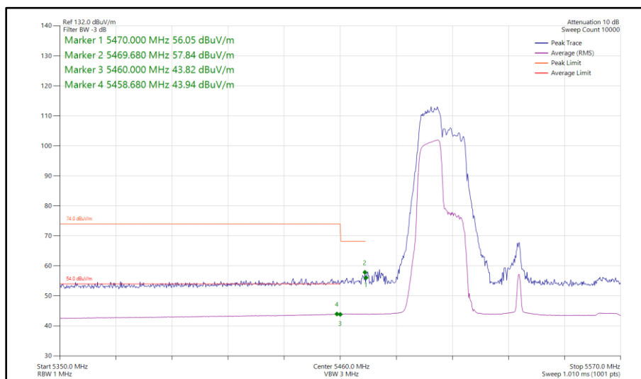
Figure 656 - 802.11ax HE80, RU 106-53, SISO, Core 1 - 5530 MHz Band Edge Frequency 5470 MHz
