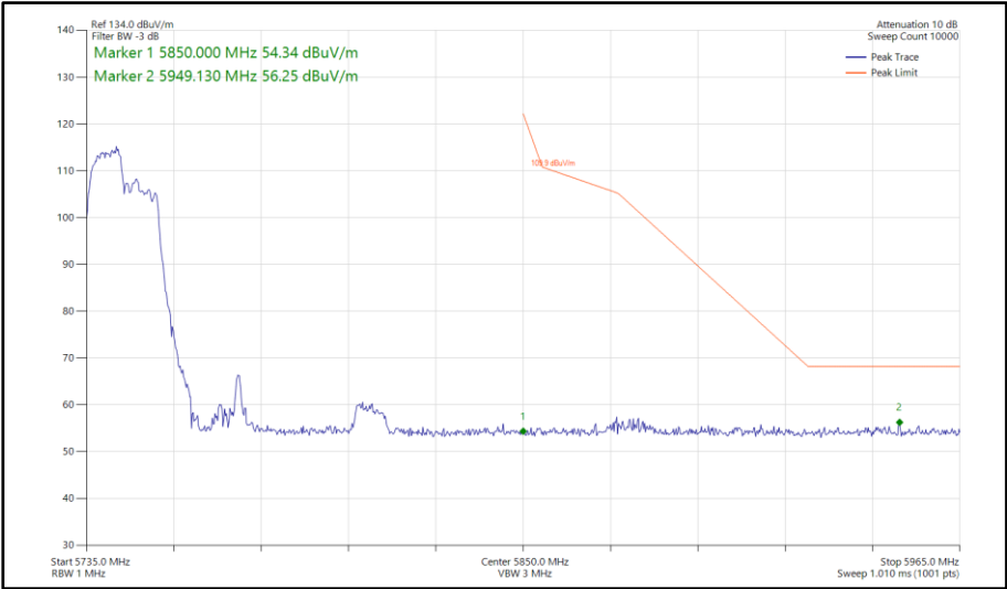
Figure 700 - 802.11ax HE80, RU 106-53, CDD, Core 0-1 - 5775 MHz Band Edge Frequency 5850 MHz
