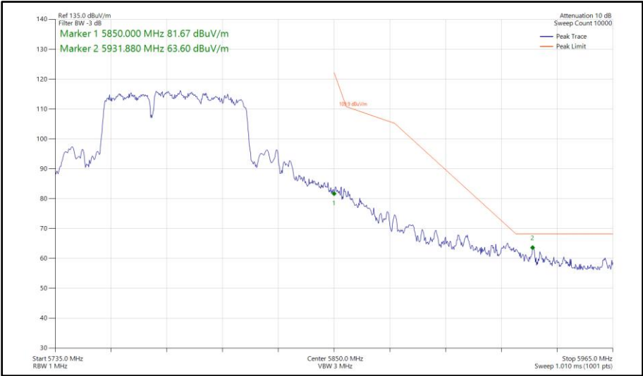
Figure 702 - 802.11be EHT80, RU 484+242-90, CDD, Core 0-1 - 5775 MHz Band Edge Frequency 5850 MHz
