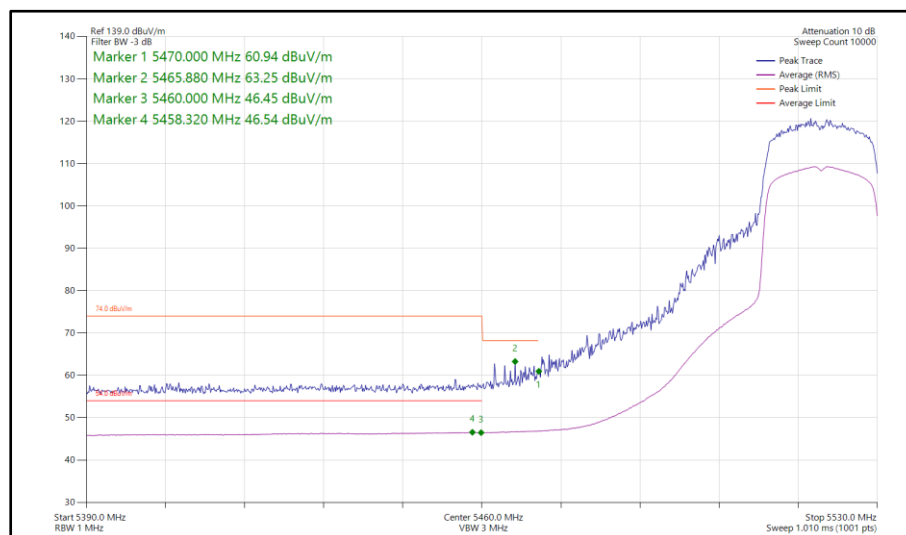
Figure 908 - 802.11ax HE20, SU, TxBF, Core 0-1 - 5520 MHz Band Edge Frequency 5460 MHz
