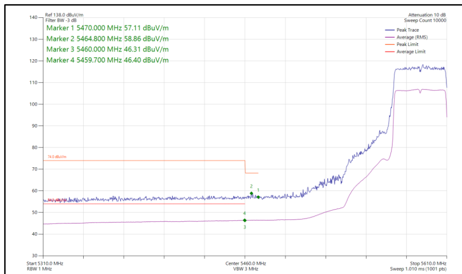
Figure 940 - 802.11ax HE40, SU, SISO, Core 0 - 5590 MHz Band Edge Frequency 5460 MHz
