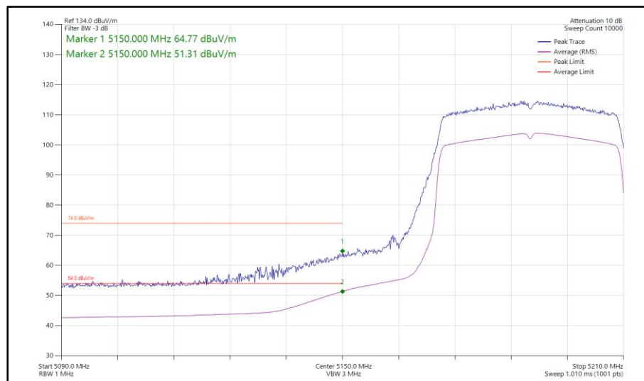
Figure 914 - 802.11ax HE40, SU, SISO, Core 0 - 5190 MHz Band Edge Frequency 5150 MHz
