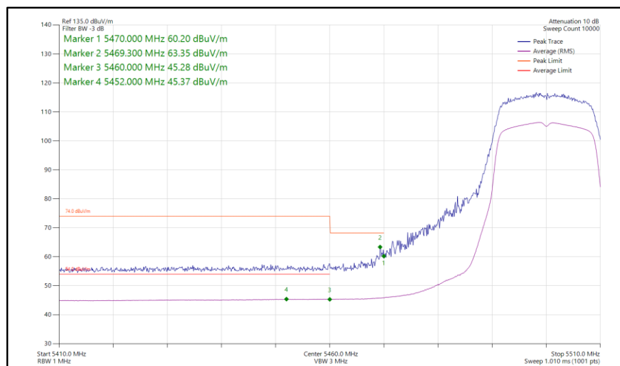
Figure 904 - 802.11ac VHT20, TxBF, Core 0-1 - 5500 MHz Band Edge Frequency 5460 MHz
