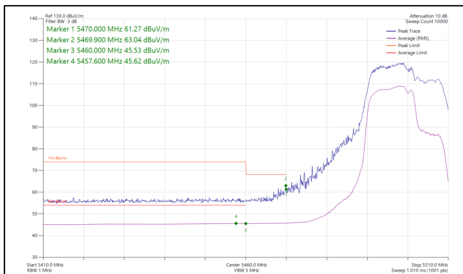
Figure 894 - 802.11be EHT20, RU 106+26-82, SDM, Core 0-1 - 5500 MHz Band Edge Frequency 5460 MHz
