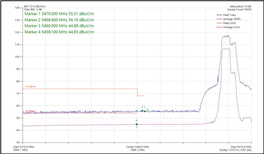
Figure 944 - 802.11be EHT40, RU 106+26-82, SISO, Core 0 - 5590 MHz Band Edge Frequency 5460 MHz
