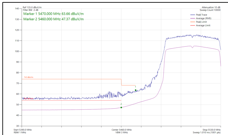
Figure 936 - 802.11ax HE40, SU, SISO, Core 0 - 5510 MHz Band Edge Frequency 5460 MHz
