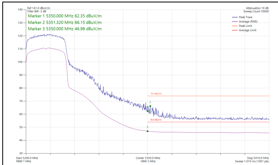
Figure 881 - 802.11ax HE20, SU, SDM, Core 0-1 - 5300 MHz Band Edge Frequency 5350 MHz
