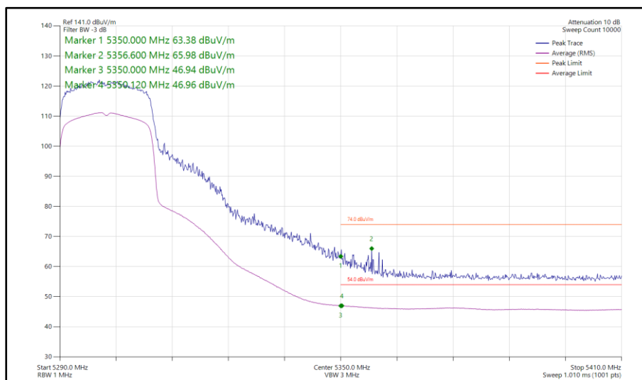
Figure 902 - 802.11ax HE20, SU, TxBF, Core 0-1 - 5300 MHz Band Edge Frequency 5350 MHz
