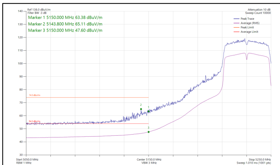
Figure 913 - 802.11n HT40, SISO, Core 0 - 5230 MHz Band Edge Frequency 5150 MHz
