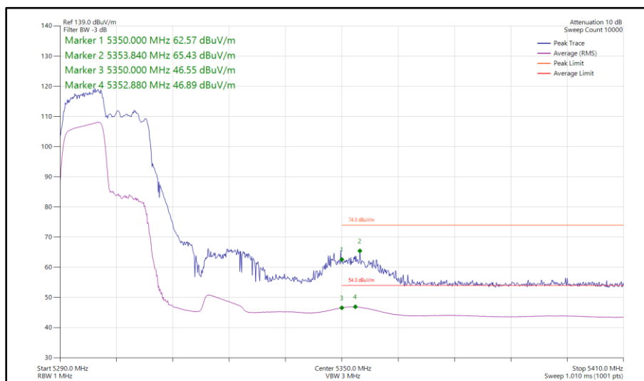
Figure 927 - 802.11ax HE40, RU 106-53, SISO, Core 0 - 5310 MHz Band Edge Frequency 5350 MHz
