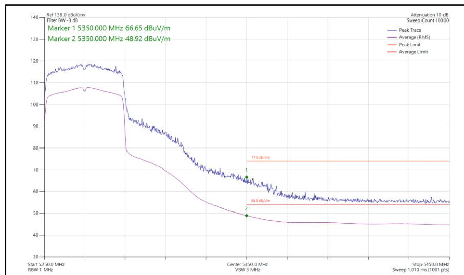
Figure 924 - 802.11ax HE40, SU, SISO, Core 0 - 5270 MHz Band Edge Frequency 5350 MHz
