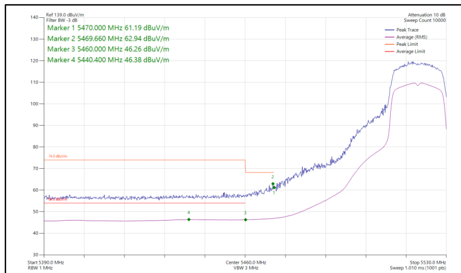
Figure 887 - 802.11n HT20, SDM, Core 0-1 - 5520 MHz Band Edge Frequency 5460 MHz
