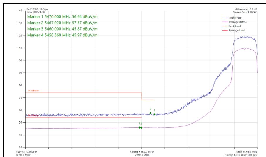
Figure 888 - 802.11n HT20, SDM, Core 0-1 - 5540 MHz Band Edge Frequency 5460 MHz
