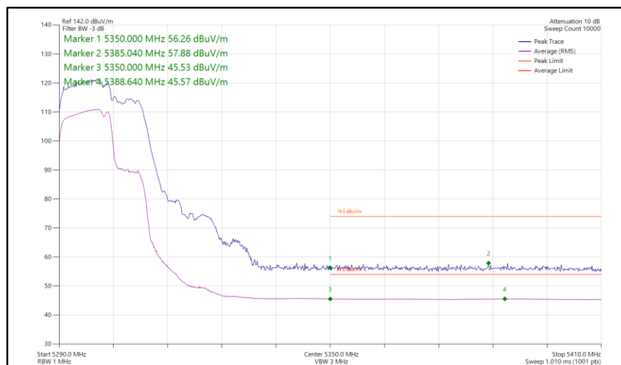
Figure 884 - 802.11be EHT20, RU 106+26-82, SDM, Core 0-1 - 5300 MHz Band Edge Frequency 5350 MHz
