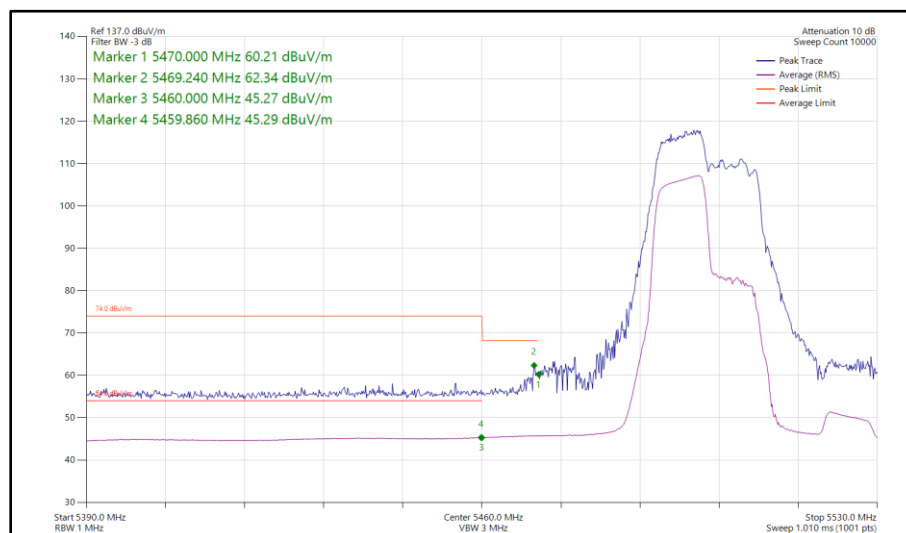
Figure 937 - 802.11ax HE40, RU 106-53, SISO, Core 0 - 5510 MHz Band Edge Frequency 5460 MHz
