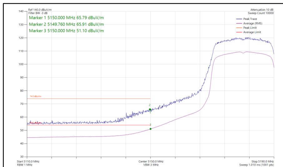
Figure 898 - 802.11ax HE20, SU, TxBF, Core 0-1 - 5180 MHz Band Edge Frequency 5150 MHz
