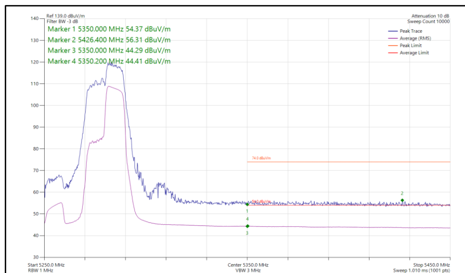
Figure 925 - 802.11ax HE40, RU 106-56, SISO, Core 0 - 5270 MHz Band Edge Frequency 5350 MHz
