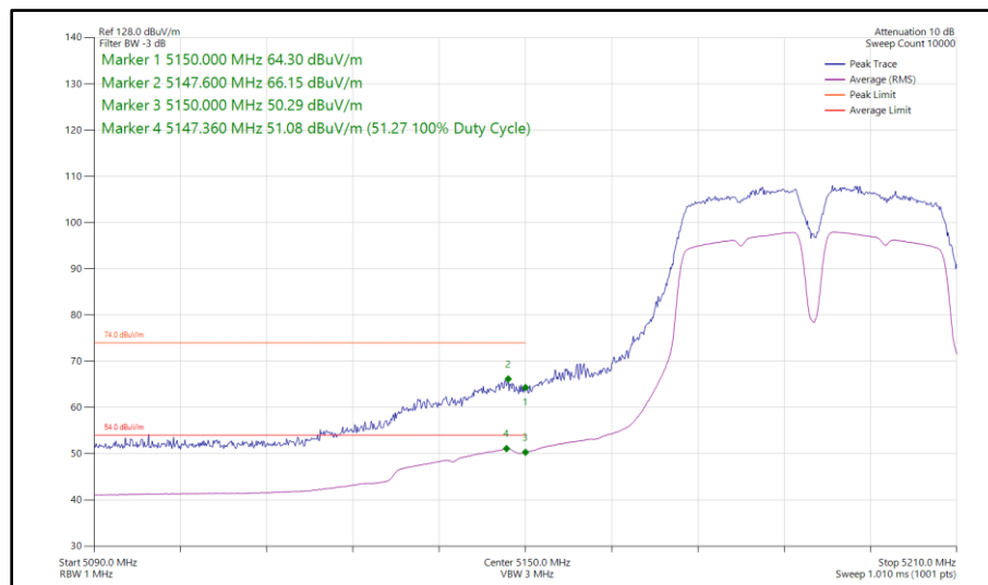
Figure 945 - 802.11a a40, SISO, Core 1 - 5190 MHz Band Edge Frequency 5150 MHz
