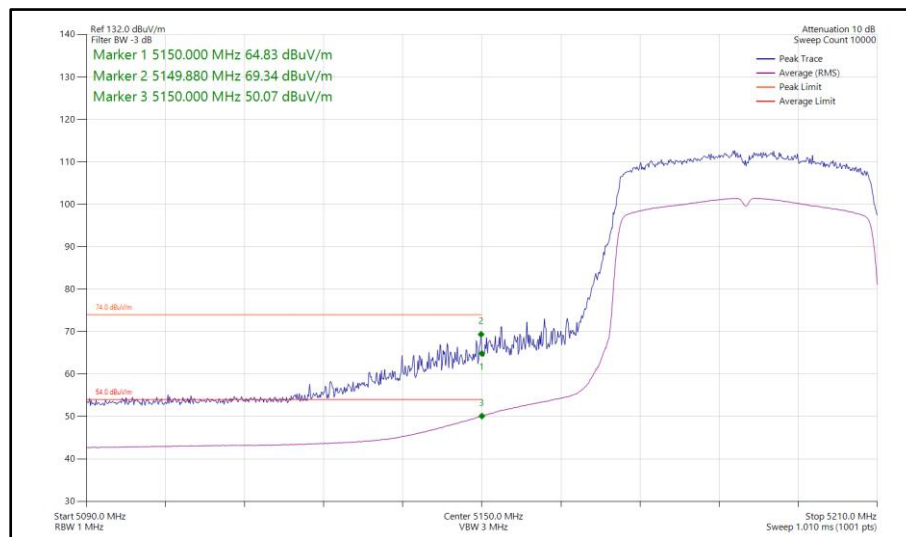
Figure 949 - 802.11ax HE40, SU, SISO, Core 1 - 5190 MHz Band Edge Frequency 5150 MHz
