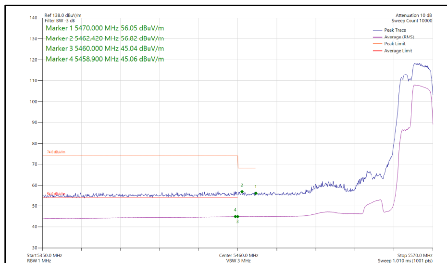
Figure 943 - 802.11be EHT40, RU 106+26-85, SISO, Core 0 - 5550 MHz Band Edge Frequency 5460 MHz
