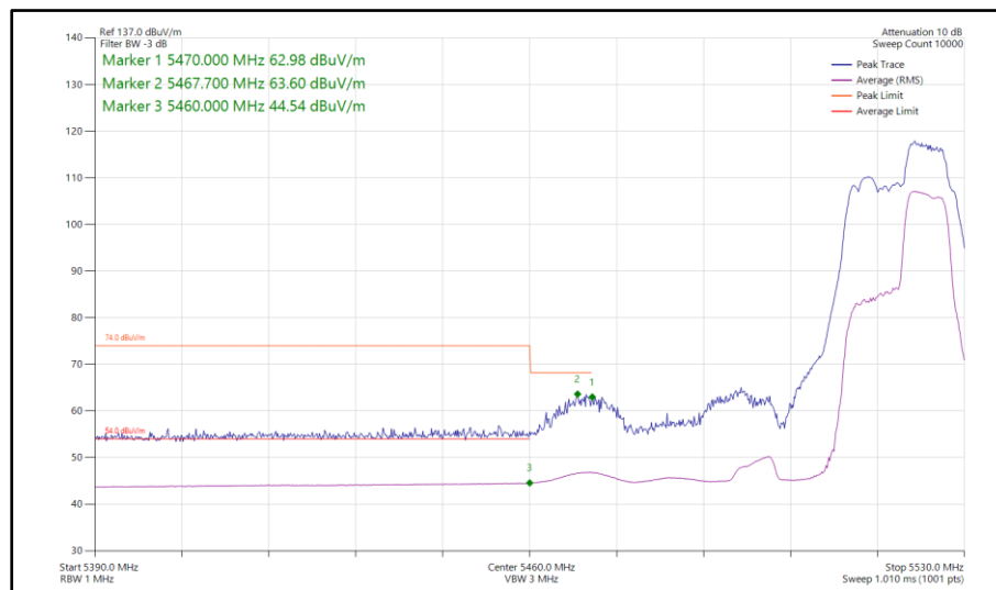
Figure 942 - 802.11be EHT40, RU 52+26-75, SISO, Core 0 - 5510 MHz Band Edge Frequency 5460 MHz
