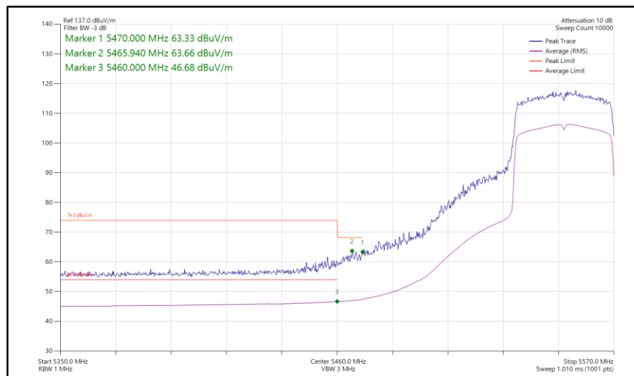
Figure 938 - 802.11ax HE40, SU, SISO, Core 0 - 5550 MHz Band Edge Frequency 5460 MHz
