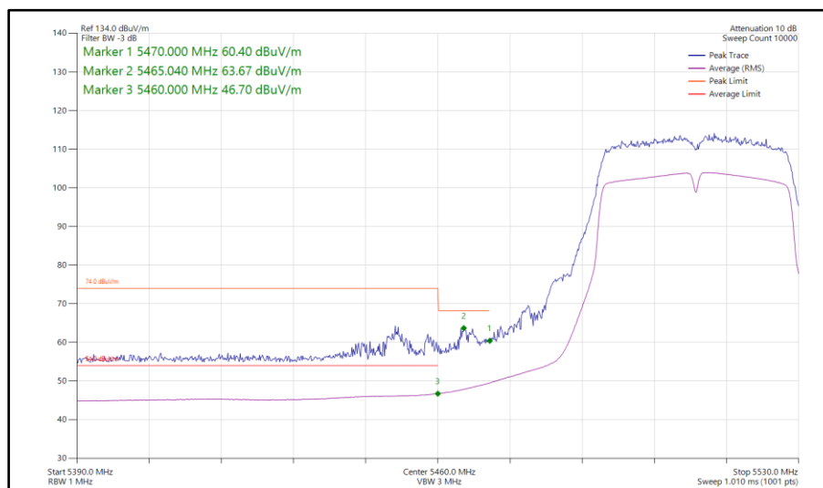
Figure 933 - 802.11n HT40, SISO, Core 0 - 5510 MHz Band Edge Frequency 5460 MHz
