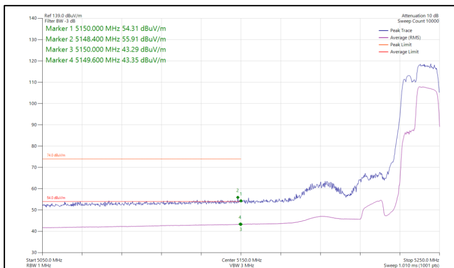
Figure 919 - 802.11be EHT40, RU 106+26-85, SISO, Core 0 - 5230 MHz Band Edge Frequency 5150 MHz
