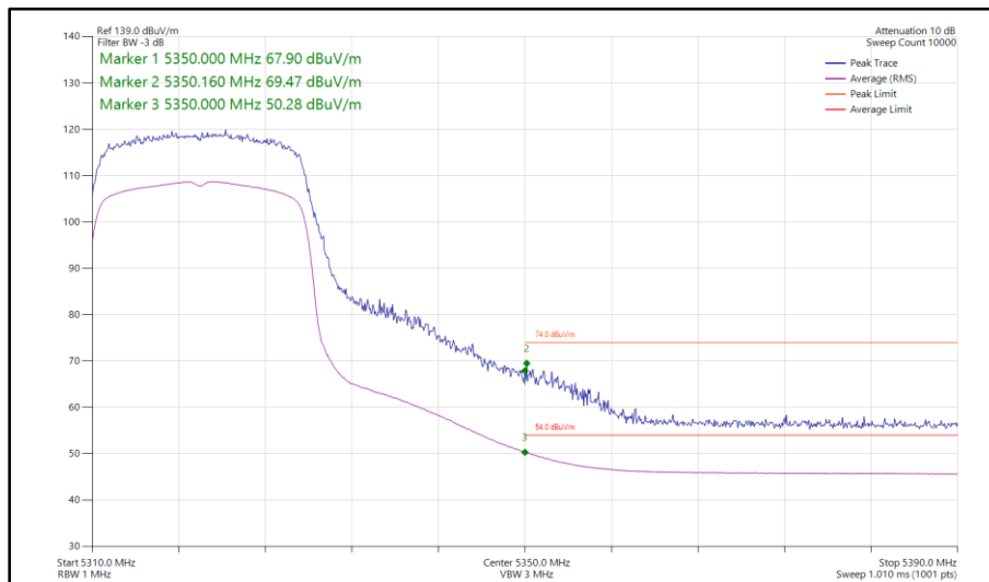
Figure 882 - 802.11ax HE20, SU, SDM, Core 0-1 - 5320 MHz Band Edge Frequency 5350 MHz
