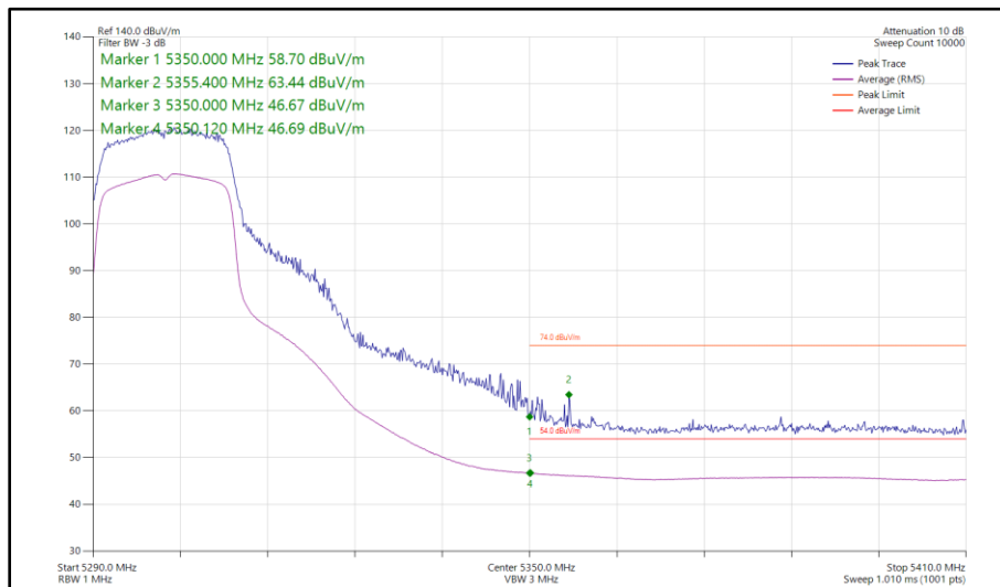
Figure 900 - 802.11ac VHT20, TxBF, Core 0-1 - 5300 MHz Band Edge Frequency 5350 MHz
