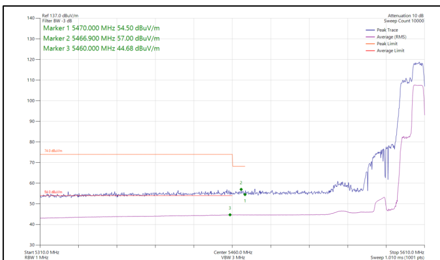
Figure 941 - 802.11ax HE40, RU 106-56, SISO, Core 0 - 5590 MHz Band Edge Frequency 5460 MHz
