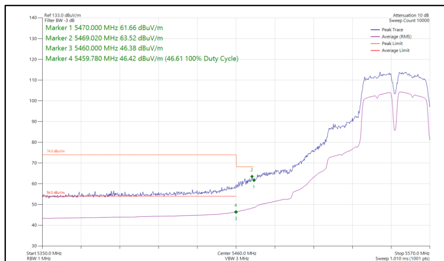
Figure 931 - 802.11a a40, SISO, Core 0 - 5550 MHz Band Edge Frequency 5460 MHz
