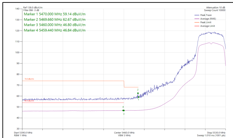
Figure 905 - 802.11ac VHT20, TxBF, Core 0-1 - 5520 MHz Band Edge Frequency 5460 MHz
