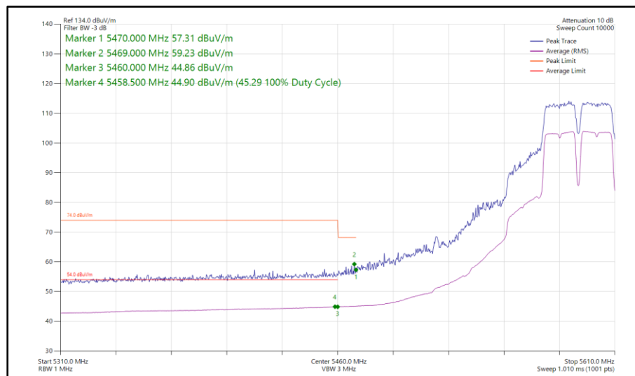
Figure 932 - 802.11a a40, SISO, Core 0 - 5590 MHz Band Edge Frequency 5460 MHz
