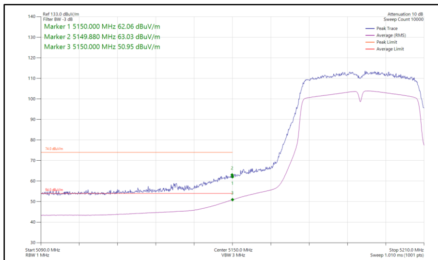
Figure 912 - 802.11n HT40, SISO, Core 0 - 5190 MHz Band Edge Frequency 5150 MHz
