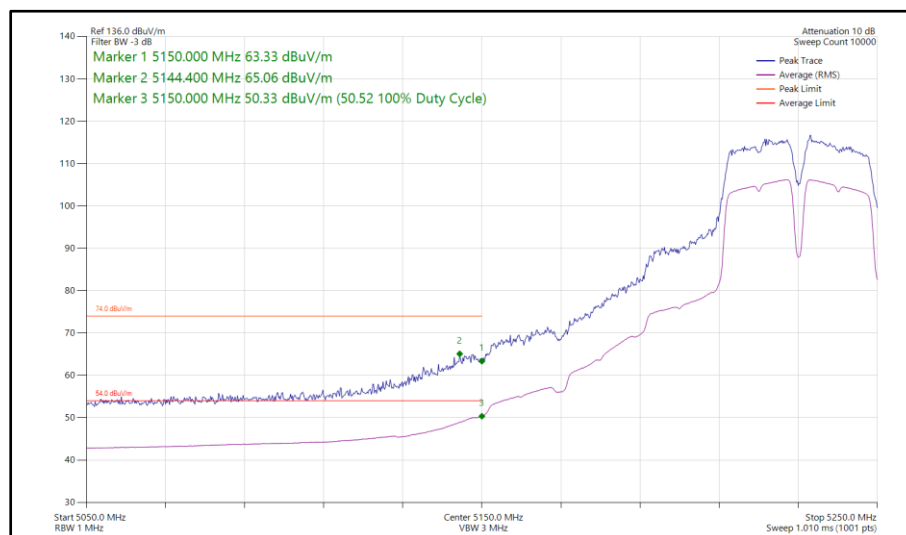
Figure 946 - 802.11a a40, SISO, Core 1 - 5230 MHz Band Edge Frequency 5150 MHz
