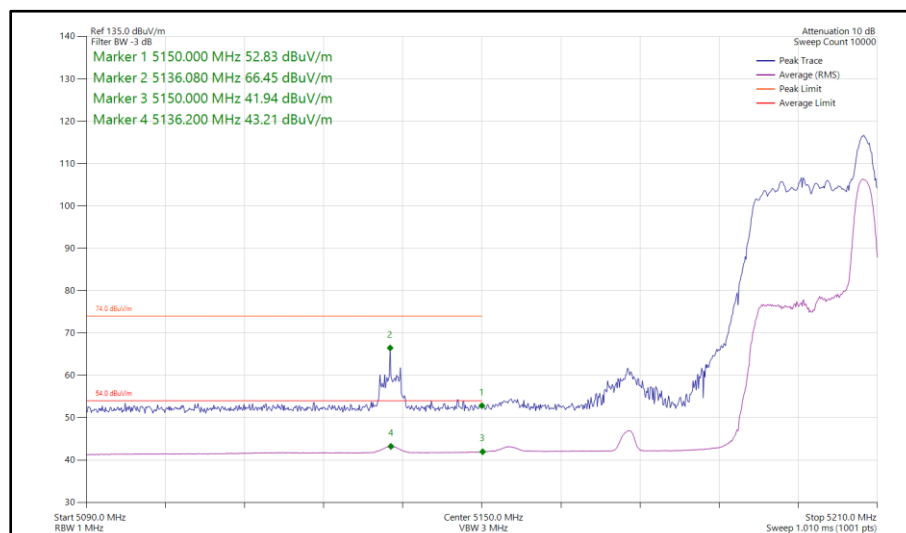
Figure 915 - 802.11ax HE40, RU 26-17, SISO, Core 0 - 5190 MHz Band Edge Frequency 5150 MHz
