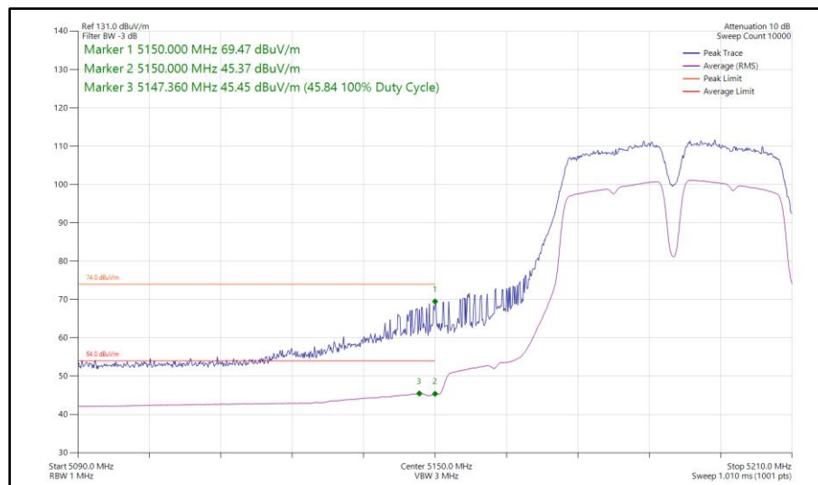
Figure 910 - 802.11a a40, SISO, Core 0 - 5190 MHz Band Edge Frequency 5150 MHz
