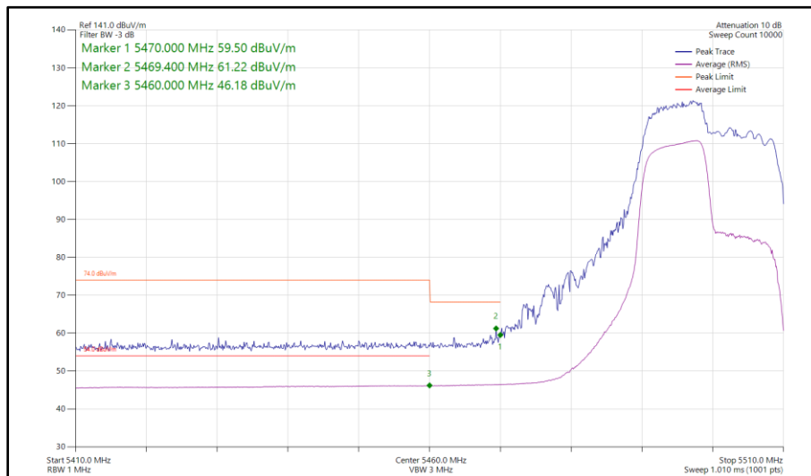
Figure 890 - 802.11ax HE20, RU 106-53, SDM, Core 0-1 - 5500 MHz Band Edge Frequency 5460 MHz
