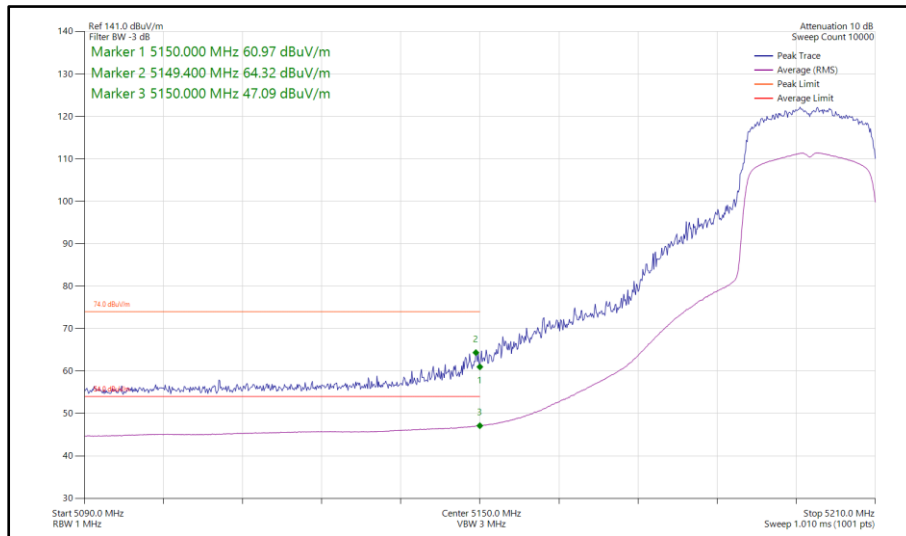
Figure 899 - 802.11ax HE20, SU, TxBF, Core 0-1 - 5200 MHz Band Edge Frequency 5150 MHz
