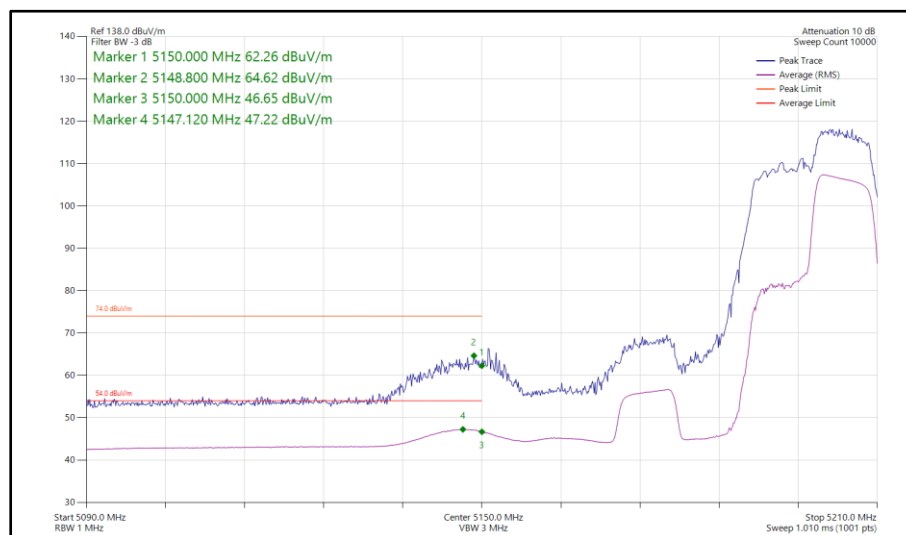
Figure 950 - 802.11ax HE40, RU 106-56, SISO, Core 1 - 5190 MHz Band Edge Frequency 5150 MHz
