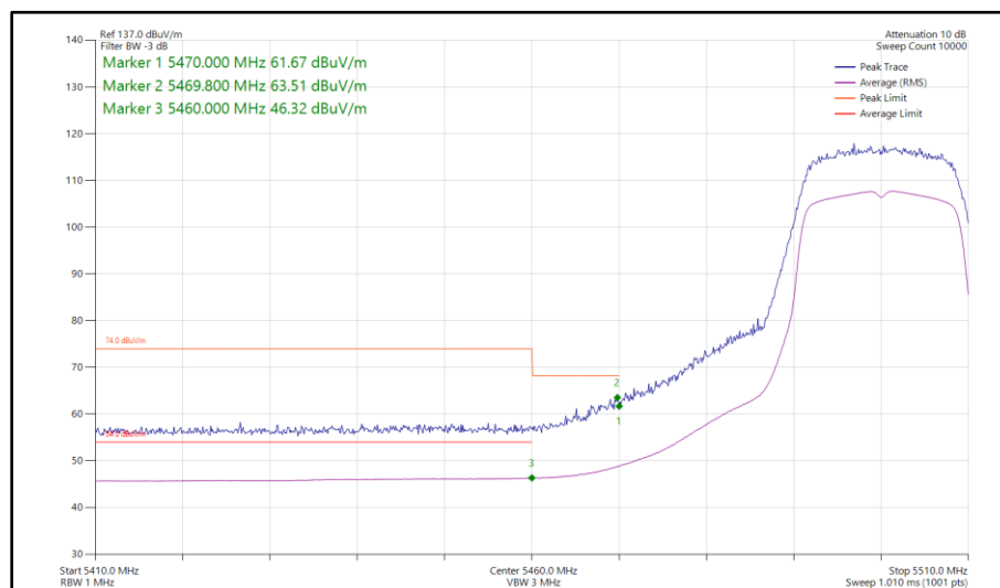
Figure 886 - 802.11n HT20, SDM, Core 0-1 - 5500 MHz Band Edge Frequency 5460 MHz
