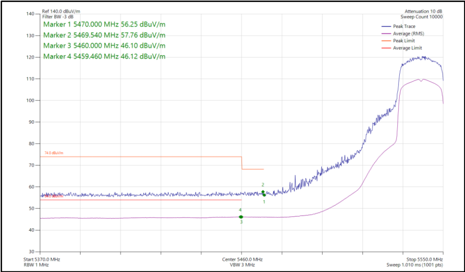
Figure 909 - 802.11ax HE20, SU, TxBF, Core 0-1 - 5540 MHz Band Edge Frequency 5460 MHz
