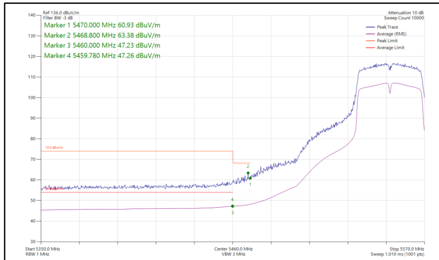
Figure 934 - 802.11n HT40, SISO, Core 0 - 5550 MHz Band Edge Frequency 5460 MHz
