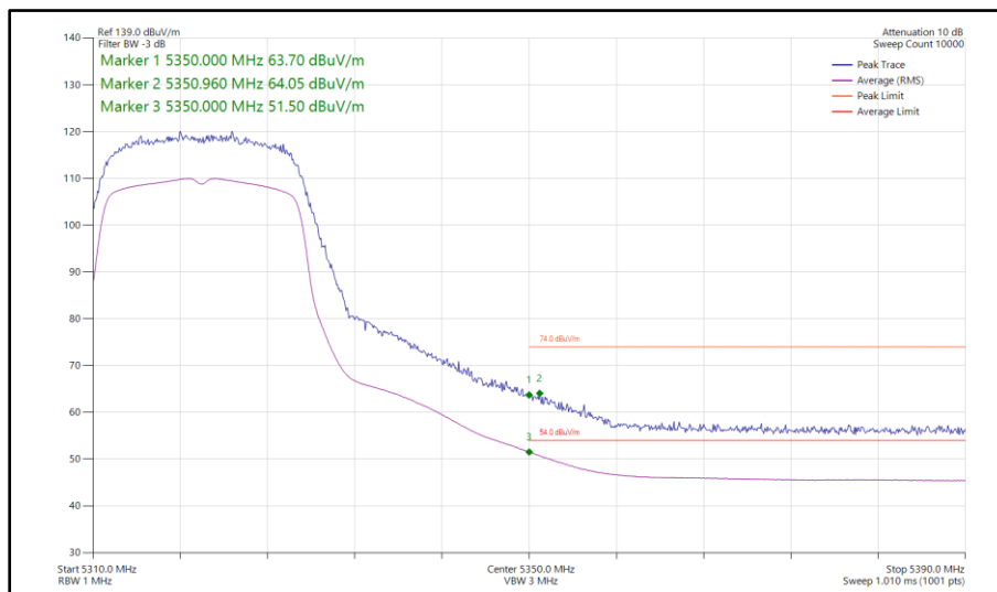
Figure 901 - 802.11ac VHT20, TxBF, Core 0-1 - 5320 MHz Band Edge Frequency 5350 MHz
