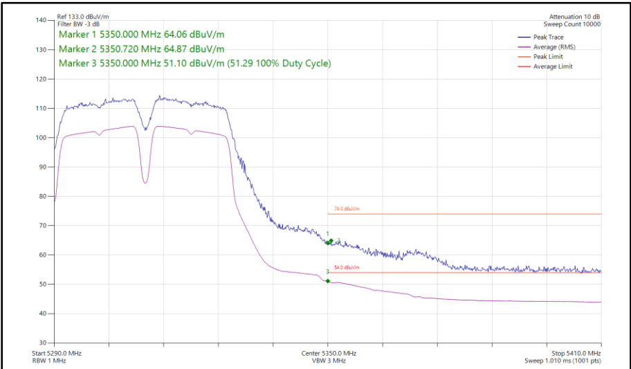
Figure 921 - 802.11a a40, SISO, Core 0 - 5310 MHz Band Edge Frequency 5350 MHz
