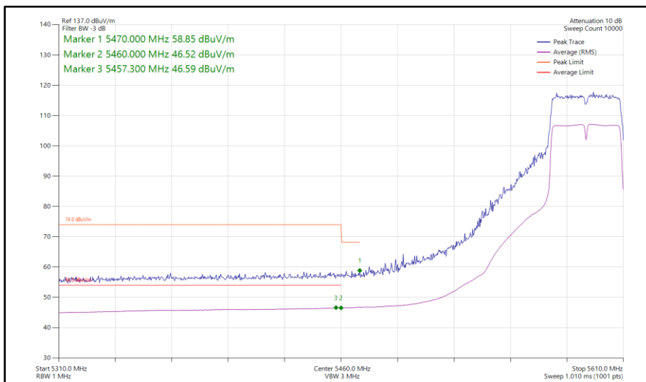
Figure 935 - 802.11n HT40, SISO, Core 0 - 5590 MHz Band Edge Frequency 5460 MHz
