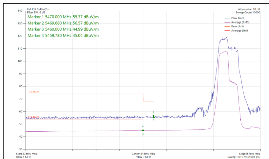
Figure 939 - 802.11ax HE40, RU 106-53, SISO, Core 0 - 5550 MHz Band Edge Frequency 5460 MHz
