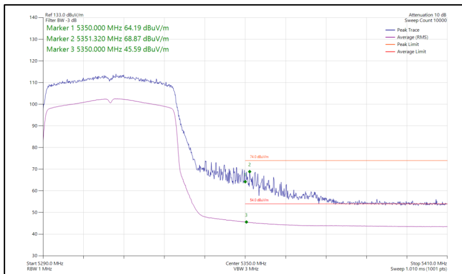
Figure 926 - 802.11ax HE40, SU, SISO, Core 0 - 5310 MHz Band Edge Frequency 5350 MHz
