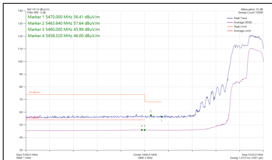
Figure 892 - 802.11ax HE20, RU 106-54, SDM, Core 0-1 - 5520 MHz Band Edge Frequency 5460 MHz
