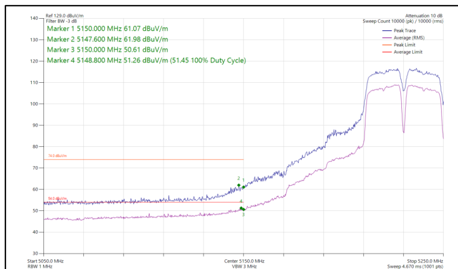
Figure 911 - 802.11a a40, SISO, Core 0 - 5230 MHz Band Edge Frequency 5150 MHz
