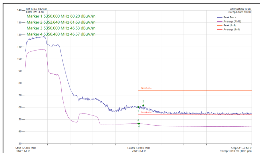
Figure 929 - 802.11be EHT40, RU 106+26-82, SISO, Core 0 - 5310 MHz Band Edge Frequency 5350 MHz
