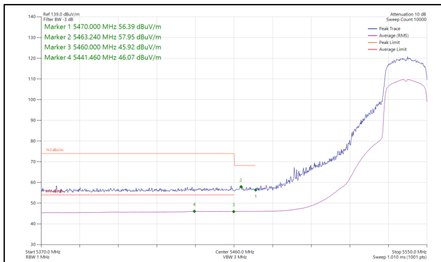
Figure 893 - 802.11ax HE20, SU, SDM, Core 0-1 - 5540 MHz Band Edge Frequency 5460 MHz
