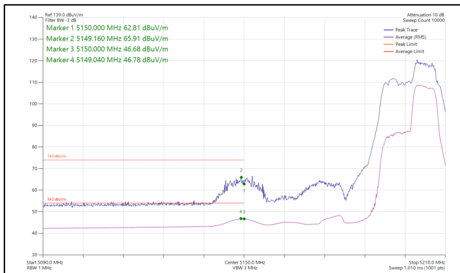
Figure 918 - 802.11be EHT40, RU 52+26-75, SISO, Core 0 - 5190 MHz Band Edge Frequency 5150 MHz
