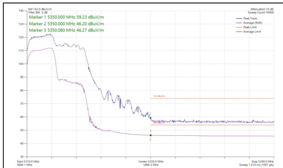
Figure 883 - 802.11ax HE20, RU 106-53, SDM, Core 0-1 - 5320 MHz Band Edge Frequency 5350 MHz
