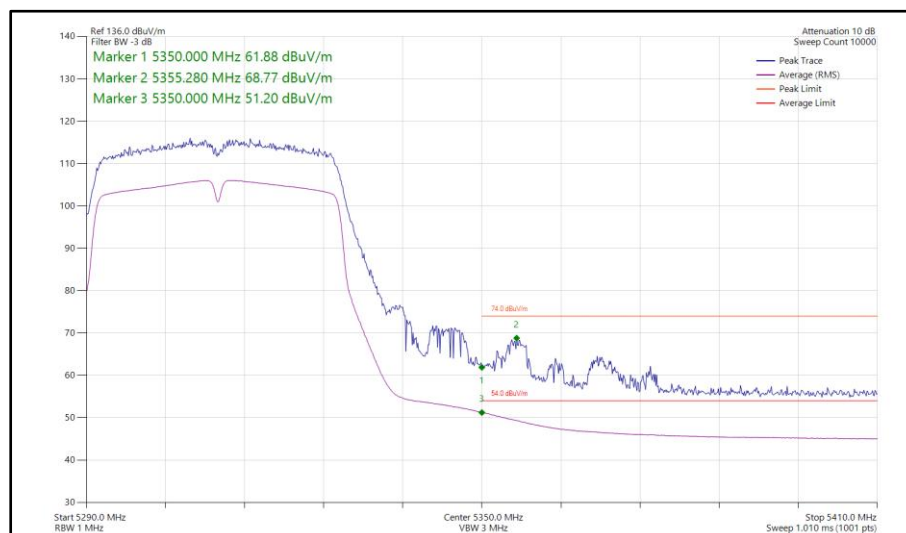
Figure 923 - 802.11n HT40, SISO, Core 0 - 5310 MHz Band Edge Frequency 5350 MHz
