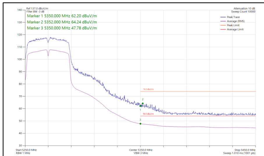
Figure 922 - 802.11n HT40, SISO, Core 0 - 5270 MHz Band Edge Frequency 5350 MHz
