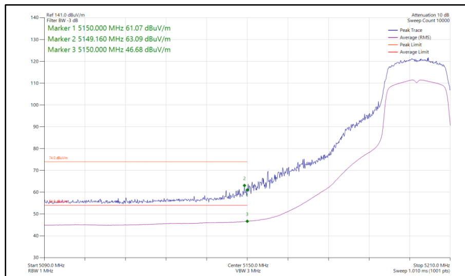
Figure 897 - 802.11ac VHT20, TxBF, Core 0-1 - 5200 MHz Band Edge Frequency 5150 MHz
