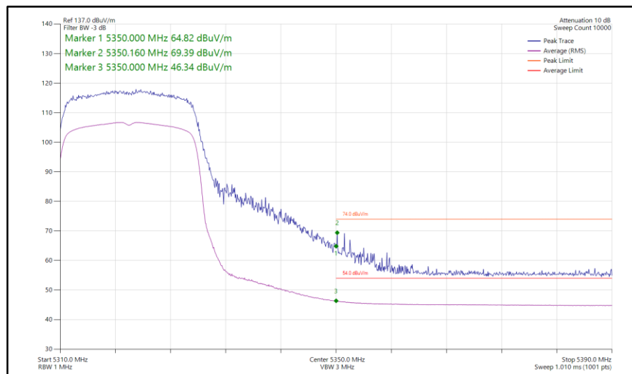
Figure 903 - 802.11ax HE20, SU, TxBF, Core 0-1 - 5320 MHz Band Edge Frequency 5350 MHz
