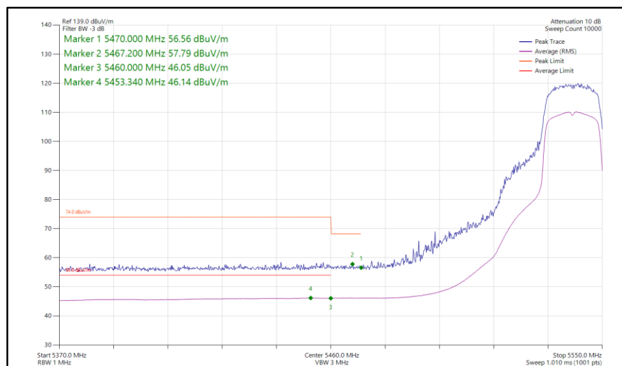
Figure 906 - 802.11ac VHT20, TxBF, Core 0-1 - 5540 MHz Band Edge Frequency 5460 MHz
