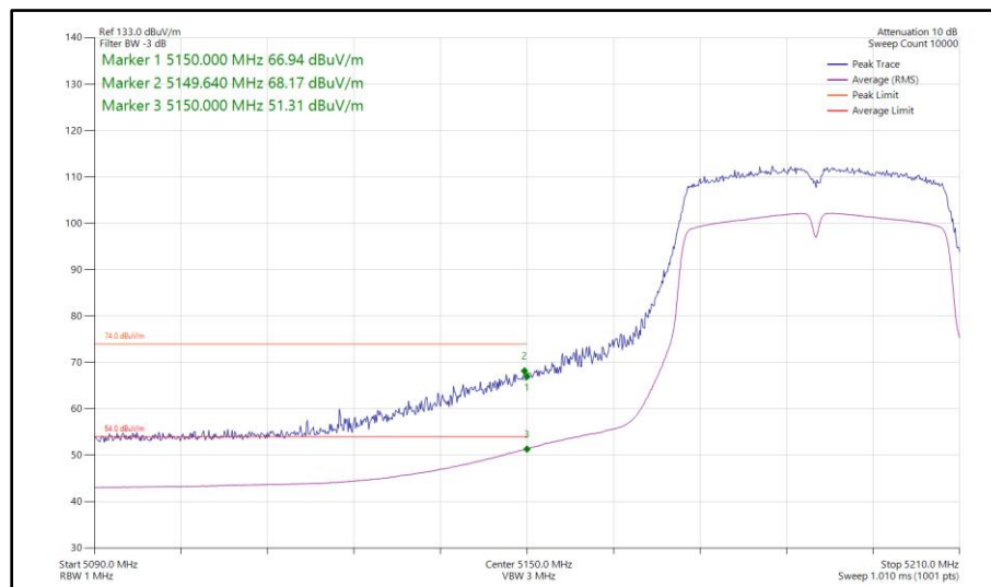
Figure 947 - 802.11n HT40, SISO, Core 1 - 5190 MHz Band Edge Frequency 5150 MHz
