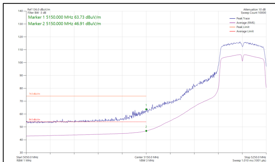
Figure 948 - 802.11n HT40, SISO, Core 1 - 5230 MHz Band Edge Frequency 5150 MHz
