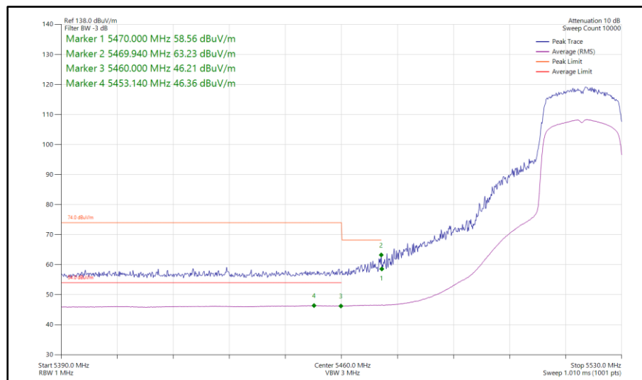
Figure 891 - 802.11ax HE20, SU, SDM, Core 0-1 - 5520 MHz Band Edge Frequency 5460 MHz
