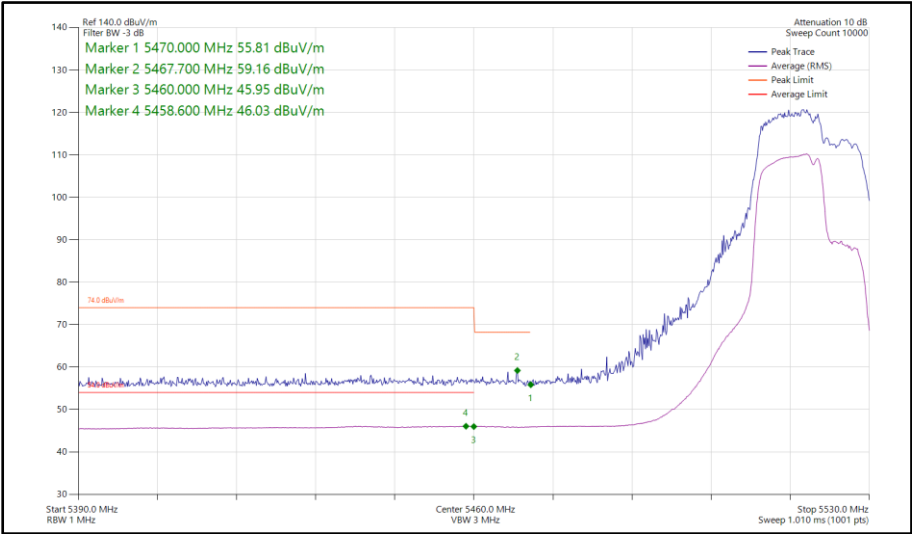
Figure 895 - 802.11be EHT20, RU 106+26-82, SDM, Core 0-1 - 5520 MHz Band Edge Frequency 5460 MHz
