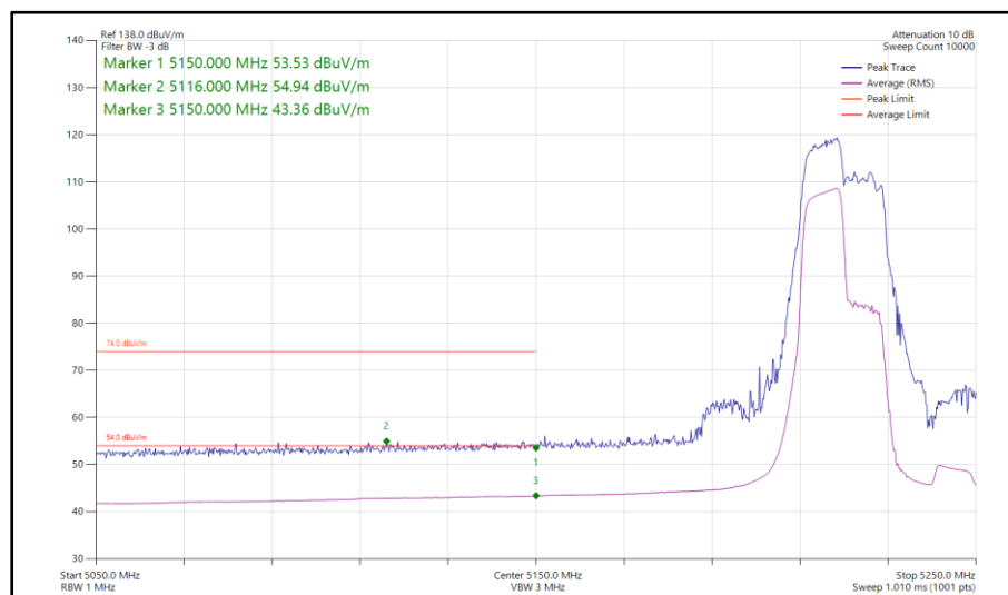
Figure 917 - 802.11ax HE40, RU 106-53, SISO, Core 0 - 5230 MHz Band Edge Frequency 5150 MHz
