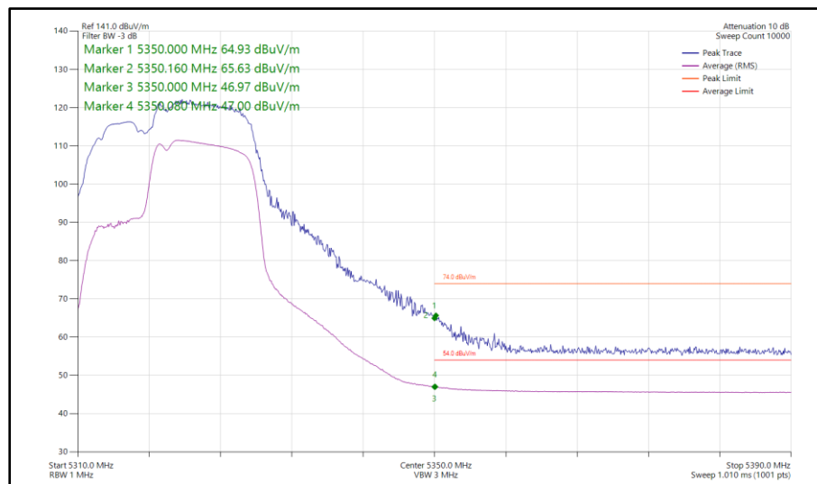
Figure 885 - 802.11be EHT20, RU 106+26-83, SDM, Core 0-1 - 5320 MHz Band Edge Frequency 5350 MHz
