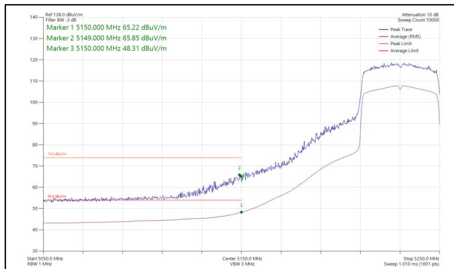
Figure 916 - 802.11ax HE40, SU, SISO, Core 0 - 5230 MHz Band Edge Frequency 5150 MHz
