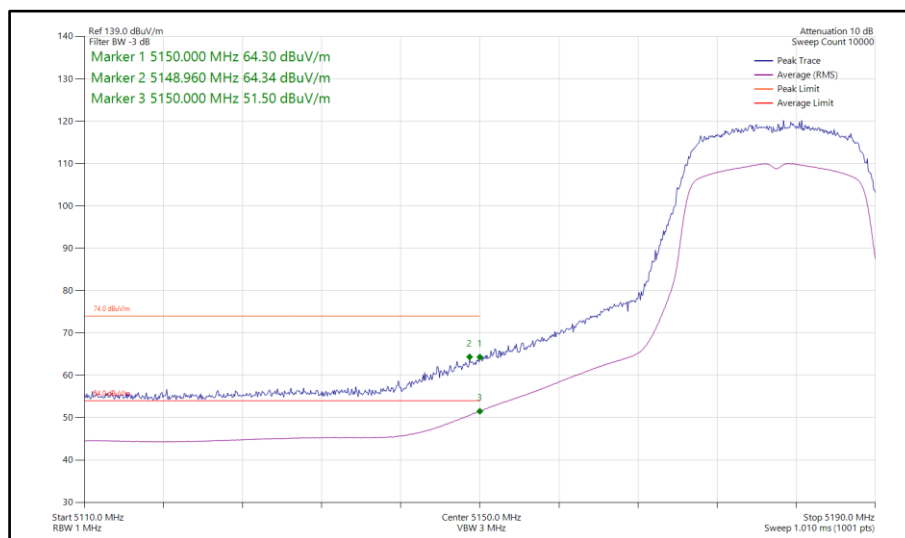
Figure 896 - 802.11ac VHT20, TxBF, Core 0-1 - 5180 MHz Band Edge Frequency 5150 MHz
