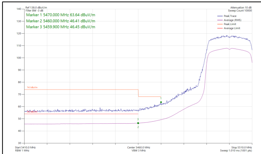
Figure 889 - 802.11ax HE20, SU, SDM, Core 0-1 - 5500 MHz Band Edge Frequency 5460 MHz
