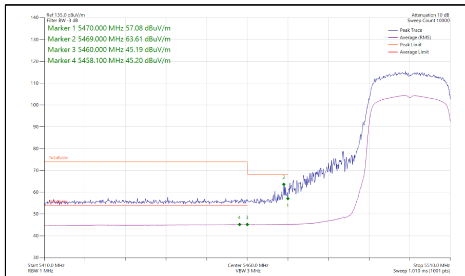
Figure 907 - 802.11ax HE20, SU, TxBF, Core 0-1 - 5500 MHz Band Edge Frequency 5460 MHz
