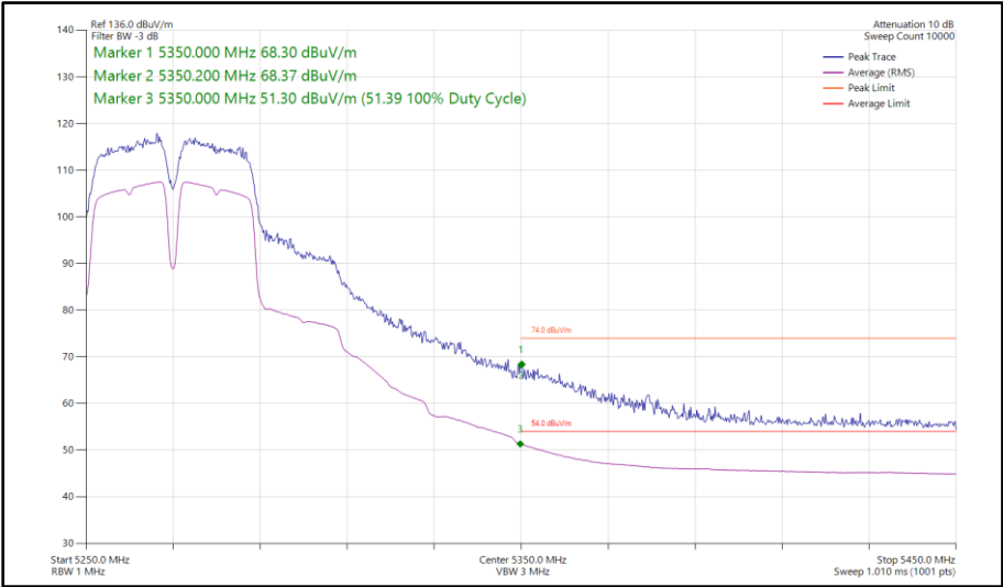
Figure 920 - 802.11a a40, SISO, Core 0 - 5270 MHz Band Edge Frequency 5350 MHz
