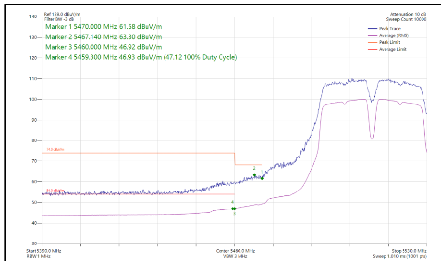
Figure 930 - 802.11a a40, SISO, Core 0 - 5510 MHz Band Edge Frequency 5460 MHz
