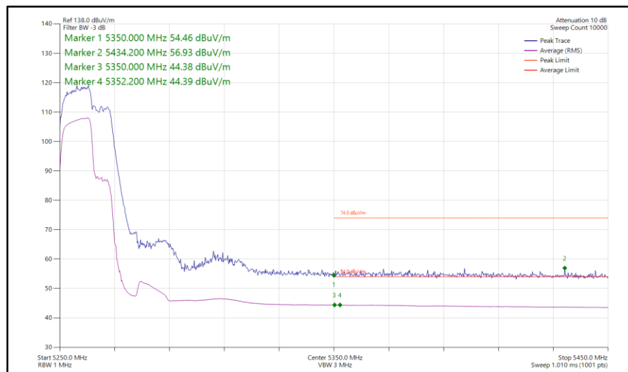
Figure 928 - 802.11be EHT40, RU 106+26-82, SISO, Core 0 - 5270 MHz Band Edge Frequency 5350 MHz
