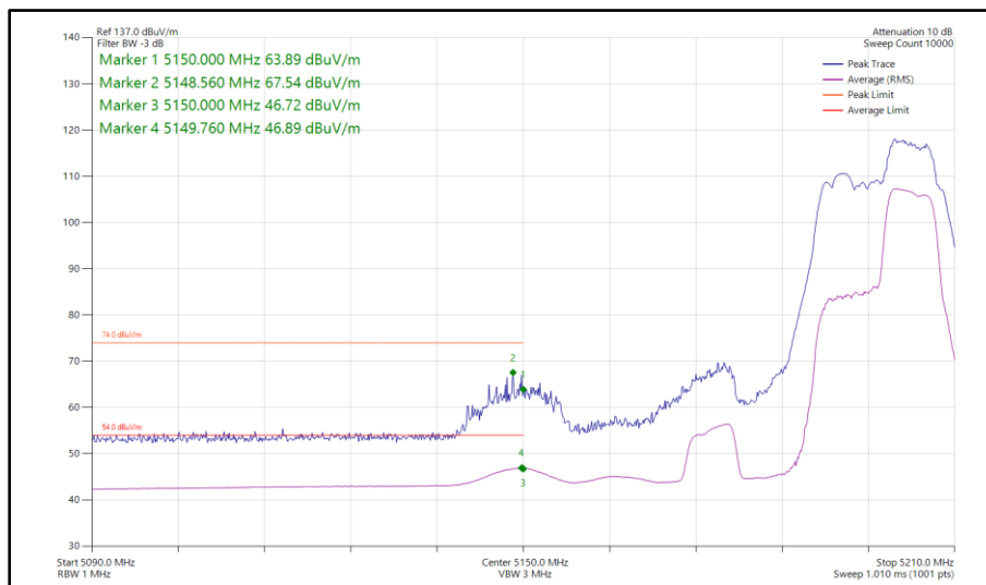
Figure 953 - 802.11be EHT40, RU 52+26-75, SISO, Core 1 - 5190 MHz Band Edge Frequency 5150 MHz
