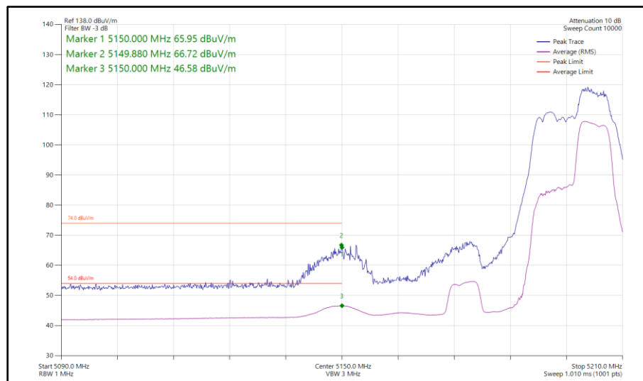
Figure 988 - 802.11be EHT40, RU 52+26-75, CDD, Core 0-1 - 5190 MHz Band Edge Frequency 5150 MHz
