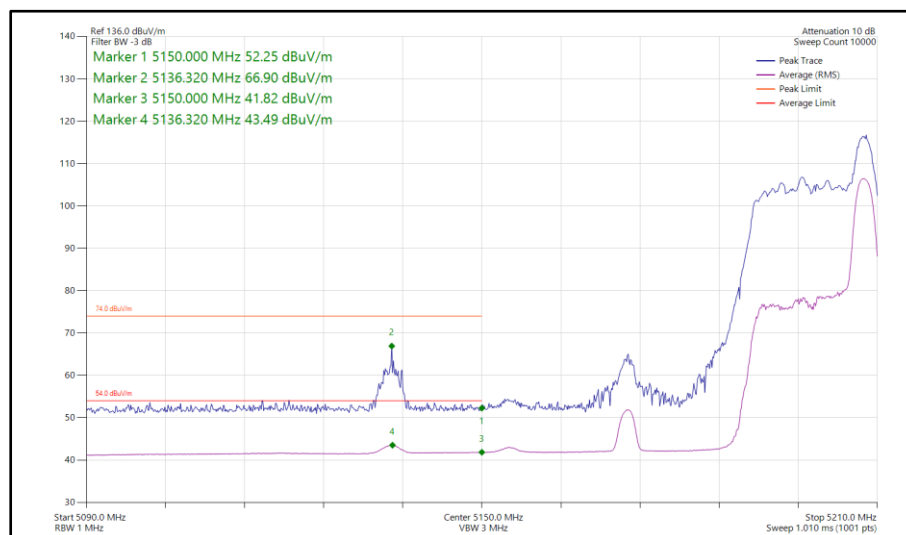
Figure 985 - 802.11ax HE40, RU 26-17, CDD, Core 0-1 - 5190 MHz Band Edge Frequency 5150 MHz
