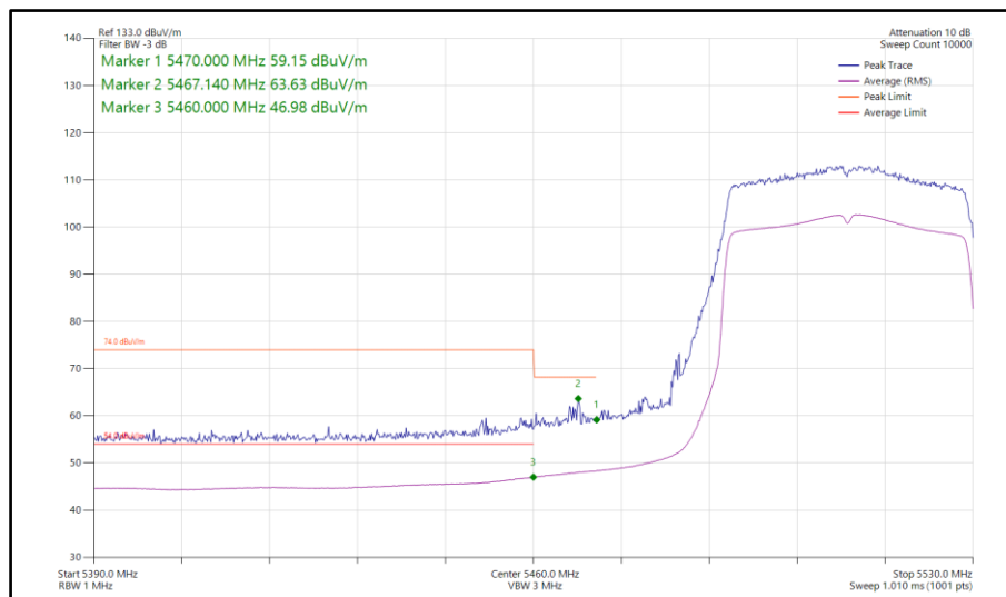
Figure 971 - 802.11ax HE40, SU, SISO, Core 1 - 5510 MHz Band Edge Frequency 5460 MHz
