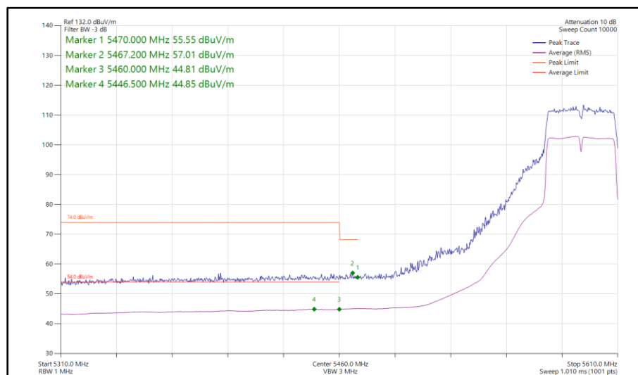
Figure 970 - 802.11n HT40, SISO, Core 1 - 5590 MHz Band Edge Frequency 5460 MHz
