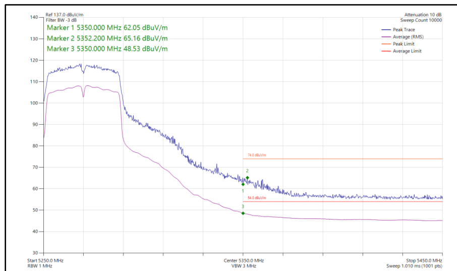
Figure 992 - 802.11n HT40, CDD, Core 0-1 - 5270 MHz Band Edge Frequency 5350 MHz
