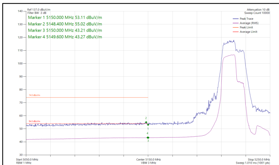
Figure 954 - 802.11be EHT40, RU 106+26-82, SISO, Core 1 - 5230 MHz Band Edge Frequency 5150 MHz
