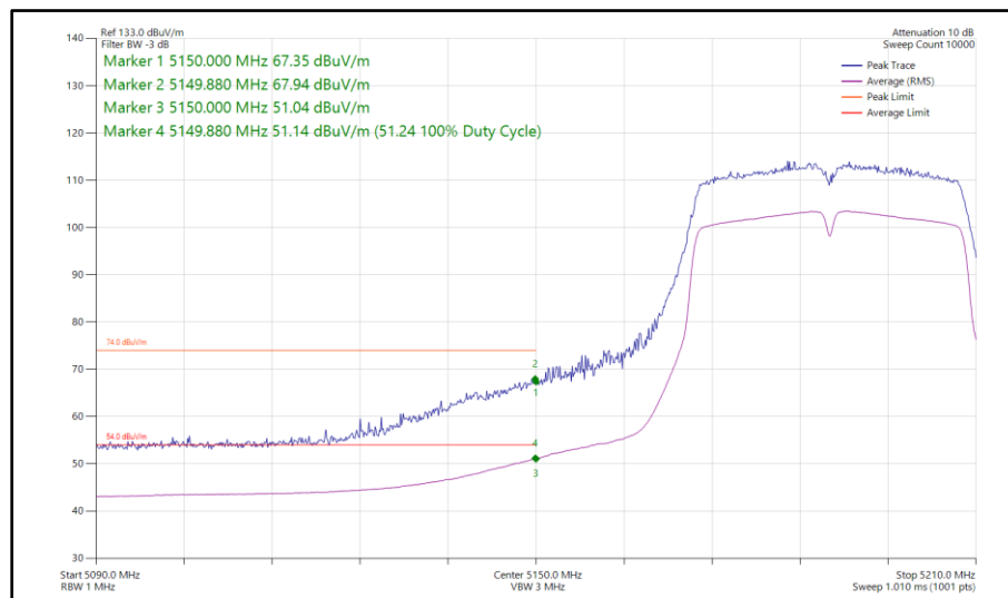
Figure 1015 - 802.11n HT40, SDM, Core 0-1 - 5190 MHz Band Edge Frequency 5150 MHz
