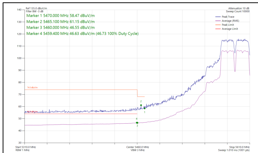
Figure 1002 - 802.11a a40, CDD, Core 0-1 - 5590 MHz Band Edge Frequency 5460 MHz
