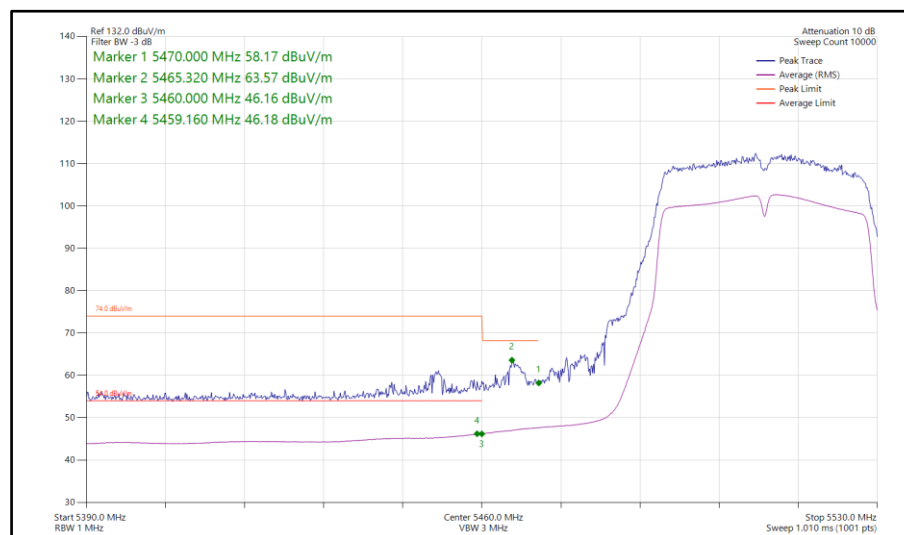
Figure 968 - 802.11n HT40, SISO, Core 1 - 5510 MHz Band Edge Frequency 5460 MHz
