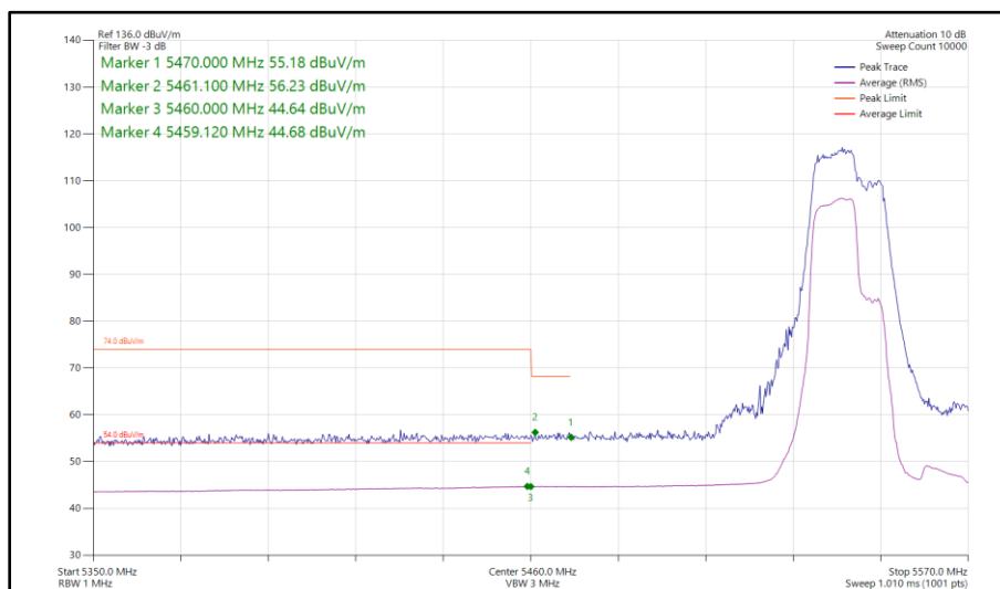
Figure 1013 - 802.11be EHT40, RU 106+26-82, CDD, Core 0-1 - 5550 MHz Band Edge Frequency 5460 MHz
