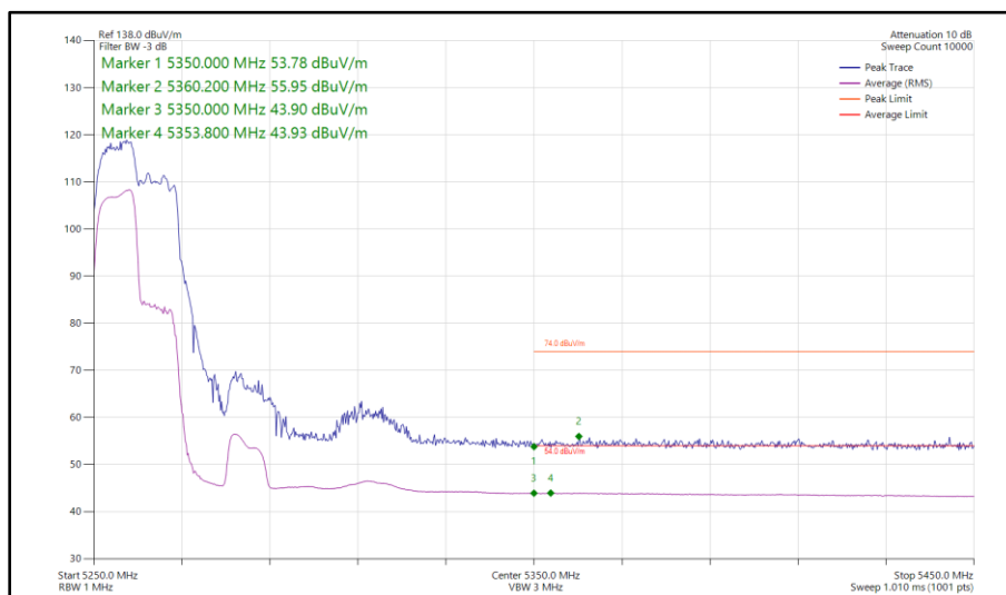
Figure 995 - 802.11ax HE40, RU 106-53, CDD, Core 0-1 - 5270 MHz Band Edge Frequency 5350 MHz
