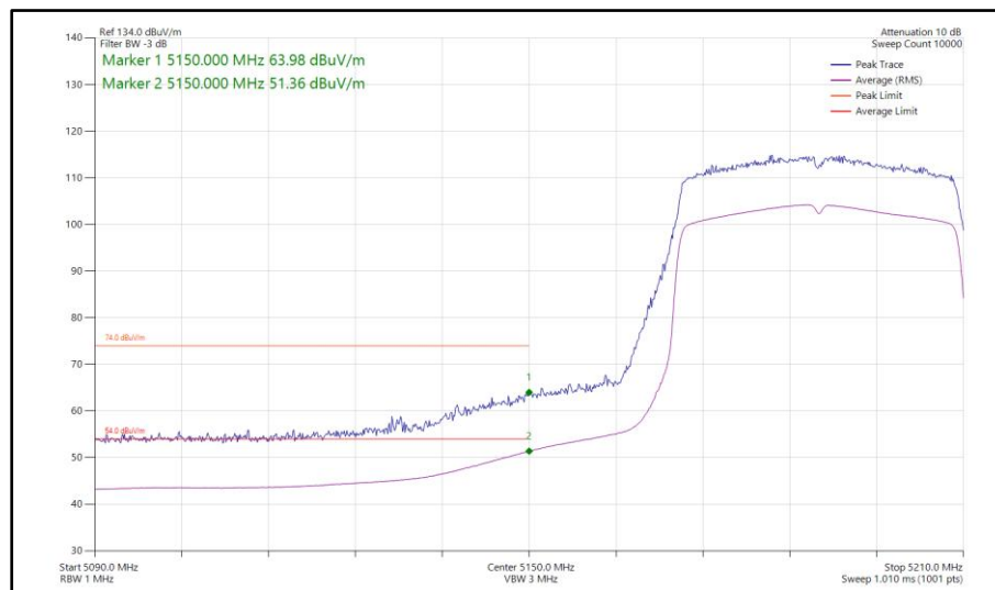
Figure 1017 - 802.11ax HE40, SU, SDM, Core 0-1 - 5190 MHz Band Edge Frequency 5150 MHz
