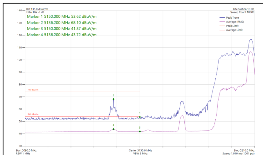
Figure 1018 - 802.11ax HE40, RU 26-17, SDM, Core 0-1 - 5190 MHz Band Edge Frequency 5150 MHz
