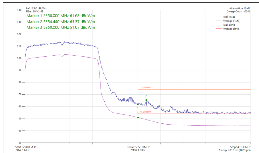
Figure 961 - 802.11ax HE40, SU, SISO, Core 1 - 5310 MHz Band Edge Frequency 5350 MHz
