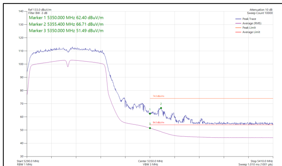
Figure 958 - 802.11n HT40, SISO, Core 1 - 5310 MHz Band Edge Frequency 5350 MHz
