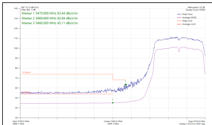
Figure 1003 - 802.11n HT40, CDD, Core 0-1 - 5510 MHz Band Edge Frequency 5460 MHz
