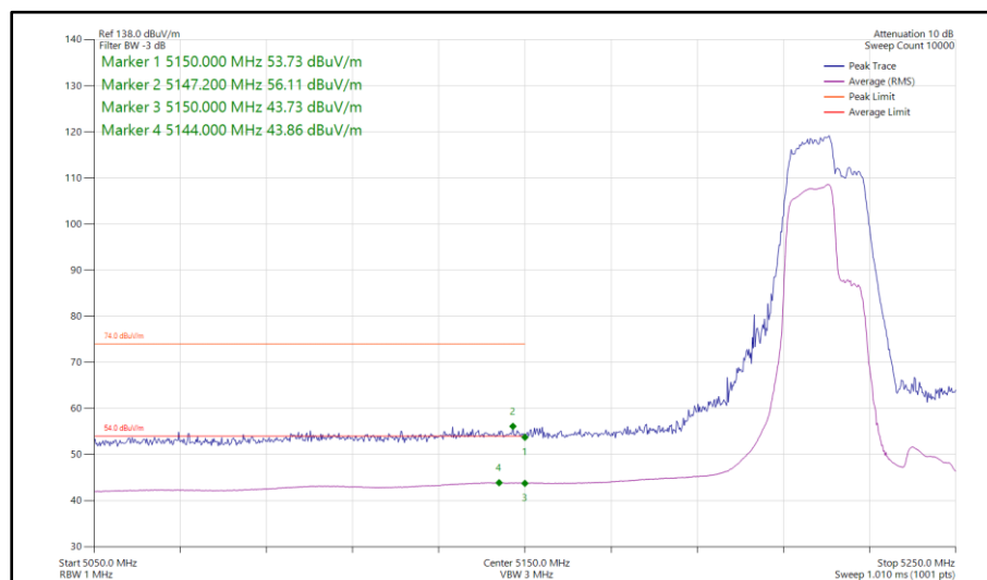
Figure 989 - 802.11be EHT40, RU 106+26-82, CDD, Core 0-1 - 5230 MHz Band Edge Frequency 5150 MHz
