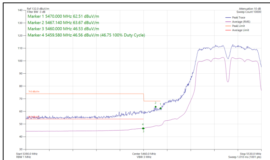
Figure 1000 - 802.11a a40, CDD, Core 0-1 - 5510 MHz Band Edge Frequency 5460 MHz
