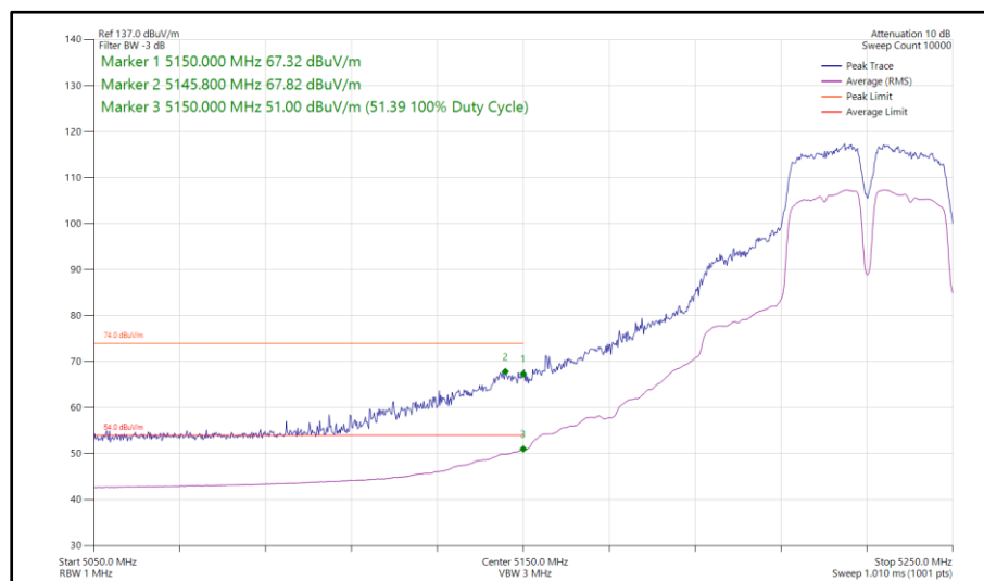
Figure 981 - 802.11a a40, CDD, Core 0-1 - 5230 MHz Band Edge Frequency 5150 MHz
