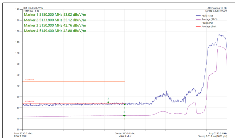
Figure 952 - 802.11ax HE40, RU 106-56, SISO, Core 1 - 5230 MHz Band Edge Frequency 5150 MHz
