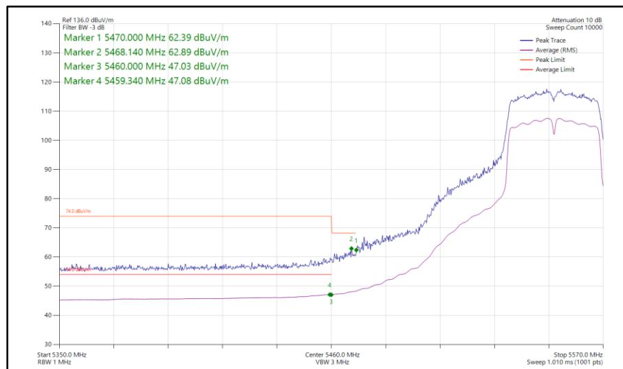
Figure 1004 - 802.11n HT40, CDD, Core 0-1 - 5550 MHz Band Edge Frequency 5460 MHz
