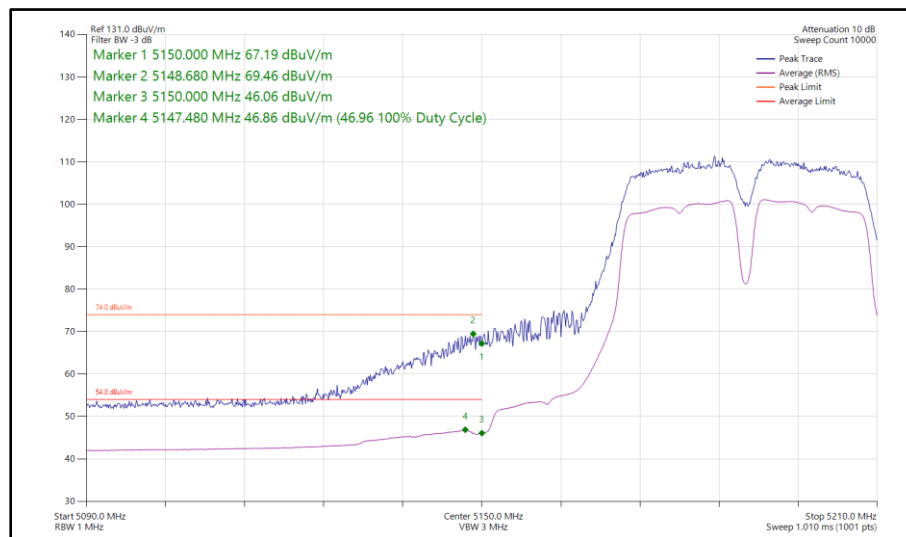
Figure 980 - 802.11a a40, CDD, Core 0-1 - 5190 MHz Band Edge Frequency 5150 MHz
