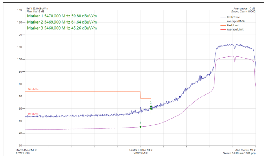
Figure 969 - 802.11n HT40, SISO, Core 1 - 5550 MHz Band Edge Frequency 5460 MHz
