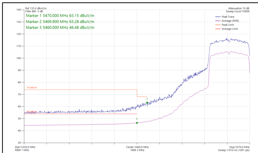
Figure 1008 - 802.11ax HE40, SU, CDD, Core 0-1 - 5550 MHz Band Edge Frequency 5460 MHz
