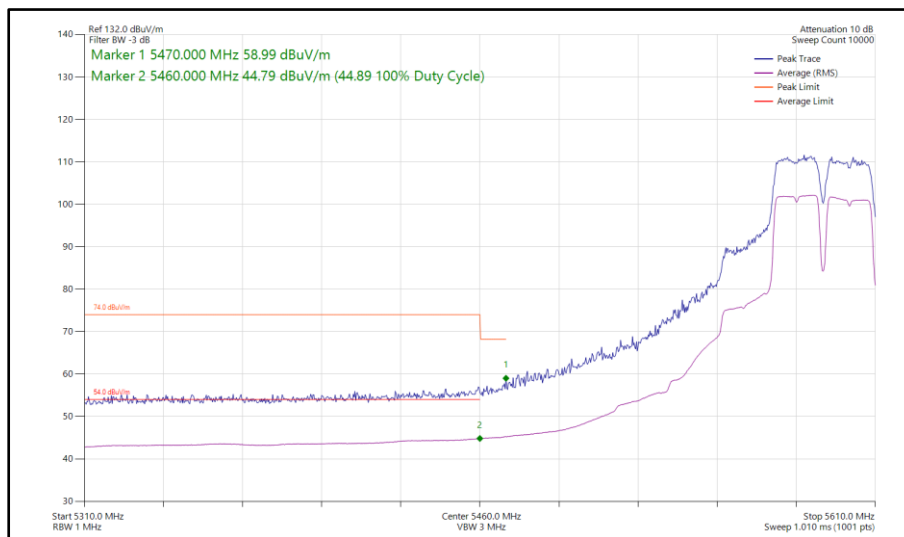
Figure 967 - 802.11a a40, SISO, Core 1 - 5590 MHz Band Edge Frequency 5460 MHz
