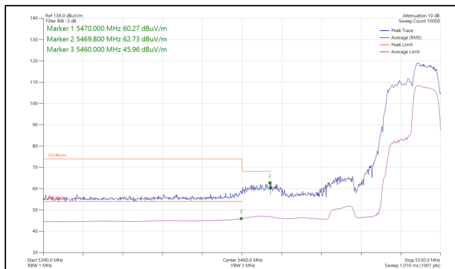
Figure 1007 - 802.11ax HE40, RU 106-56, CDD, Core 0-1 - 5510 MHz Band Edge Frequency 5460 MHz
