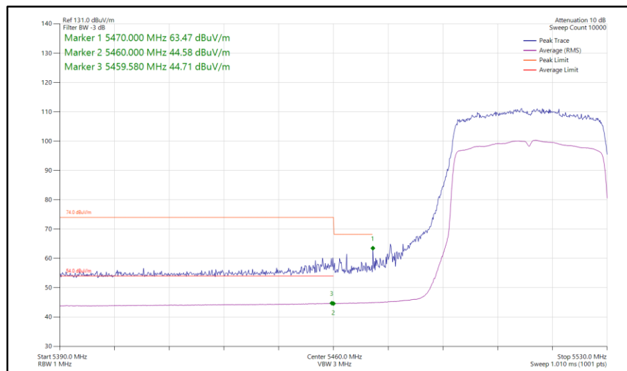
Figure 1006 - 802.11ax HE40, SU, CDD, Core 0-1 - 5510 MHz Band Edge Frequency 5460 MHz
