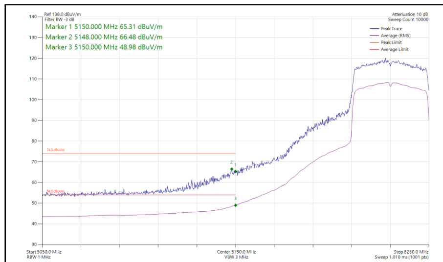
Figure 986 - 802.11ax HE40, SU, CDD, Core 0-1 - 5230 MHz Band Edge Frequency 5150 MHz
