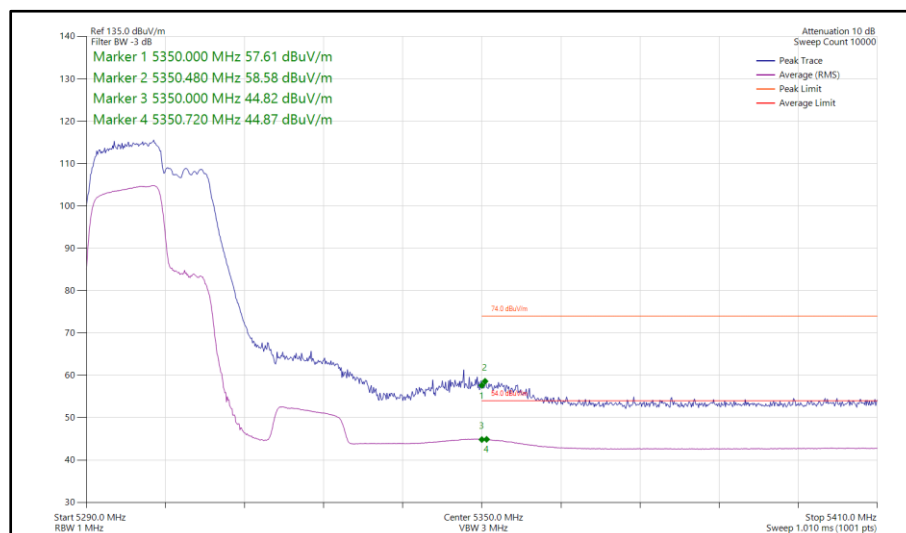
Figure 964 - 802.11be EHT40, RU 106+26-82, SISO, Core 1 - 5310 MHz Band Edge Frequency 5350 MHz
