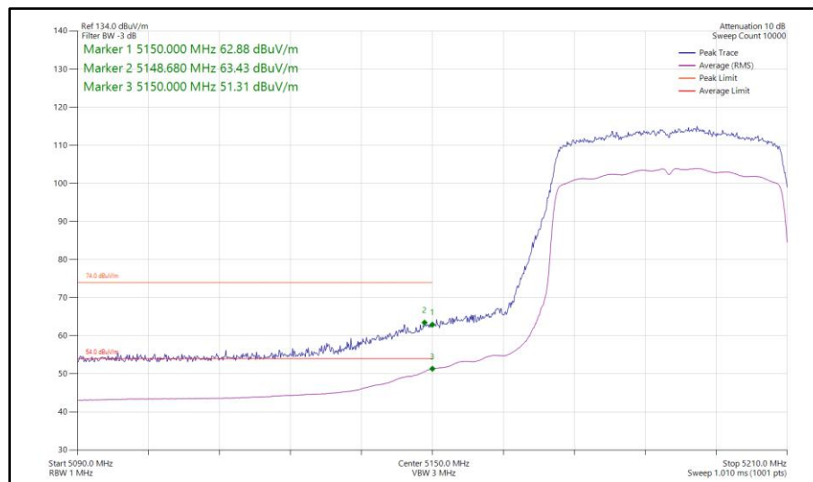
Figure 984 - 802.11ax HE40, SU, CDD, Core 0-1 - 5190 MHz Band Edge Frequency 5150 MHz
