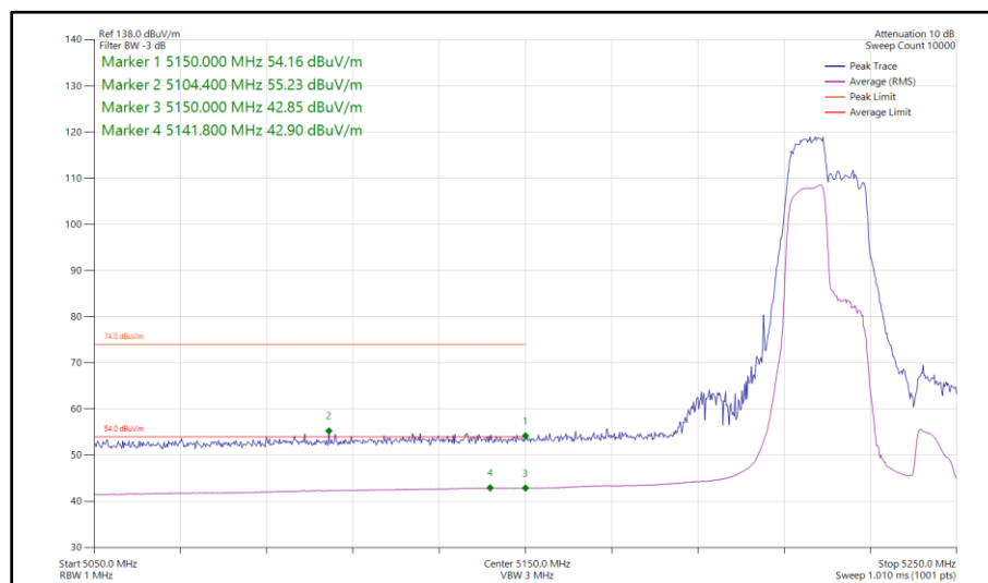
Figure 987 - 802.11ax HE40, RU 106-53, CDD, Core 0-1 - 5230 MHz Band Edge Frequency 5150 MHz
