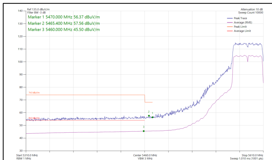
Figure 1005 - 802.11n HT40, CDD, Core 0-1 - 5590 MHz Band Edge Frequency 5460 MHz
