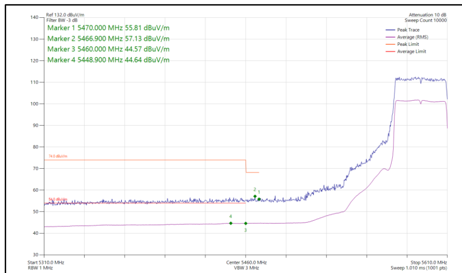
Figure 975 - 802.11ax HE40, SU, SISO, Core 1 - 5590 MHz Band Edge Frequency 5460 MHz
