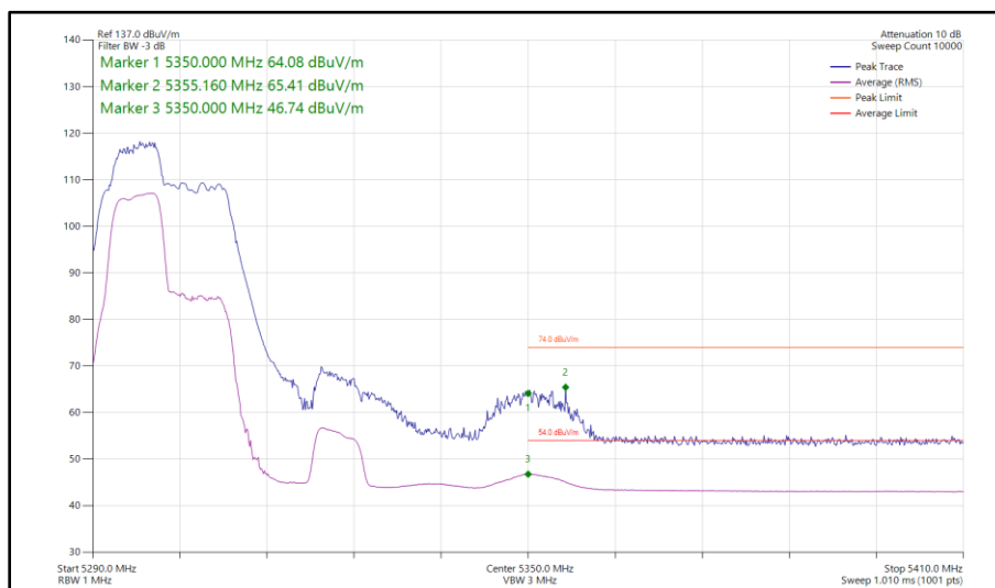
Figure 999 - 802.11be EHT40, RU 52+26-70, CDD, Core 0-1 - 5310 MHz Band Edge Frequency 5350 MHz
