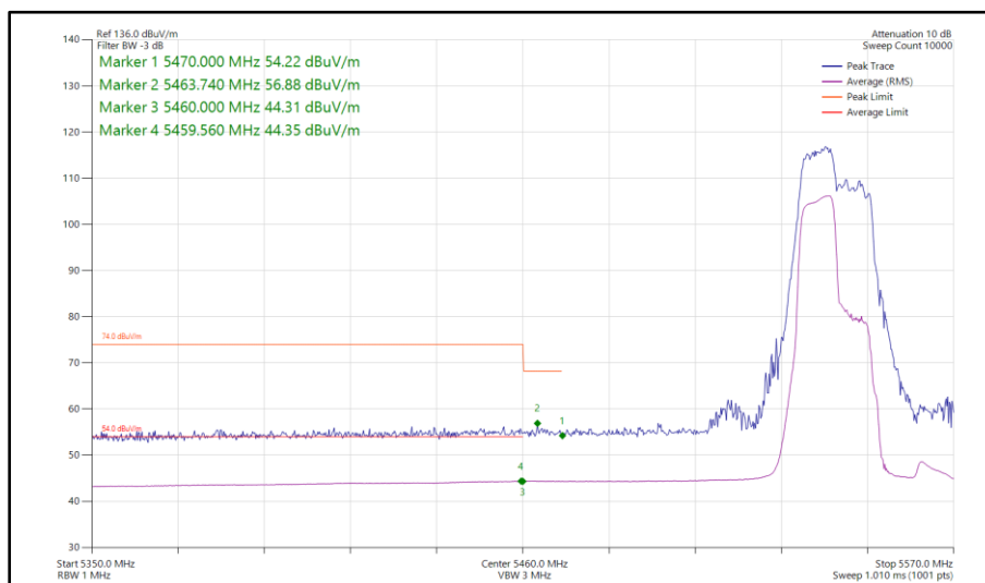
Figure 1009 - 802.11ax HE40, RU 106-53, CDD, Core 0-1 - 5550 MHz Band Edge Frequency 5460 MHz
