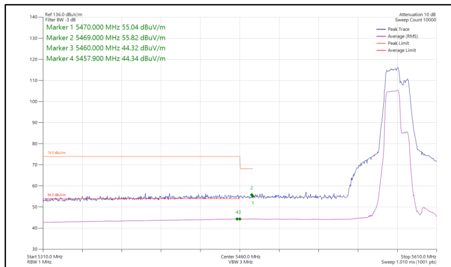
Figure 1014 - 802.11be EHT40, RU 106+26-82, CDD, Core 0-1 - 5590 MHz Band Edge Frequency 5460 MHz
