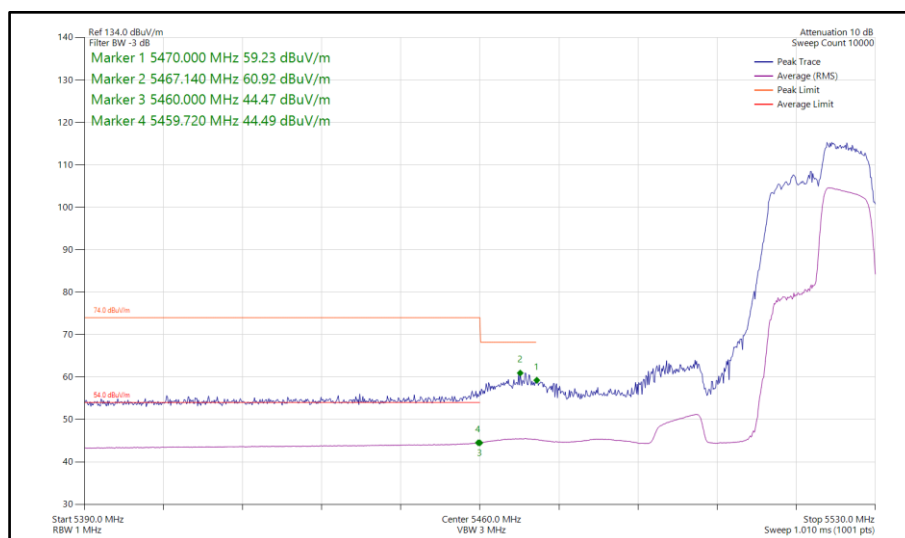
Figure 972 - 802.11ax HE40, RU 106-56, SISO, Core 1 - 5510 MHz Band Edge Frequency 5460 MHz
