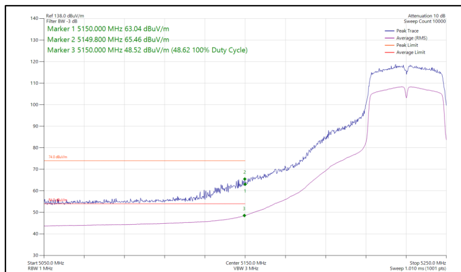
Figure 1016 - 802.11n HT40, SDM, Core 0-1 - 5230 MHz Band Edge Frequency 5150 MHz
