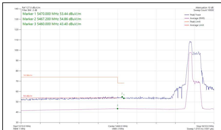
Figure 976 - 802.11ax HE40, RU 52-37, SISO, Core 1 - 5590 MHz Band Edge Frequency 5460 MHz
