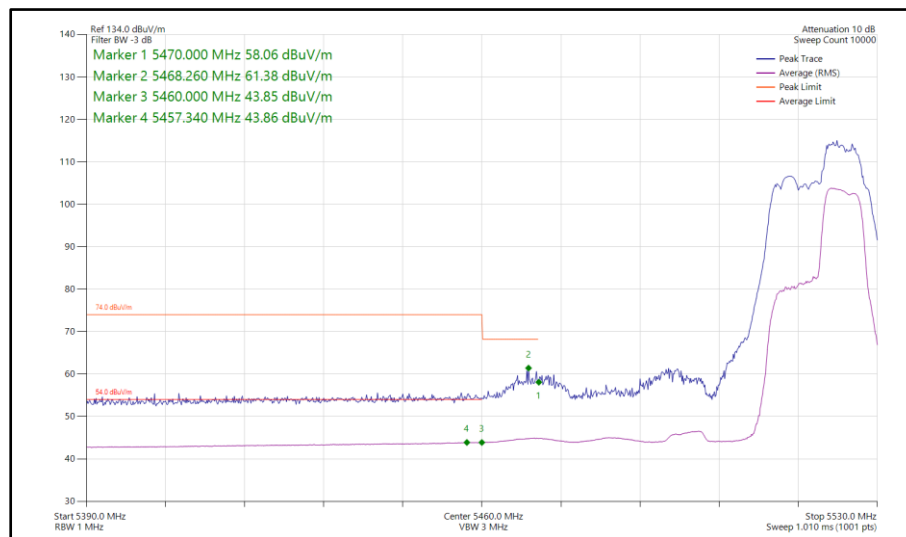
Figure 977 - 802.11be EHT40, RU 52+26-75, SISO, Core 1 - 5510 MHz Band Edge Frequency 5460 MHz
