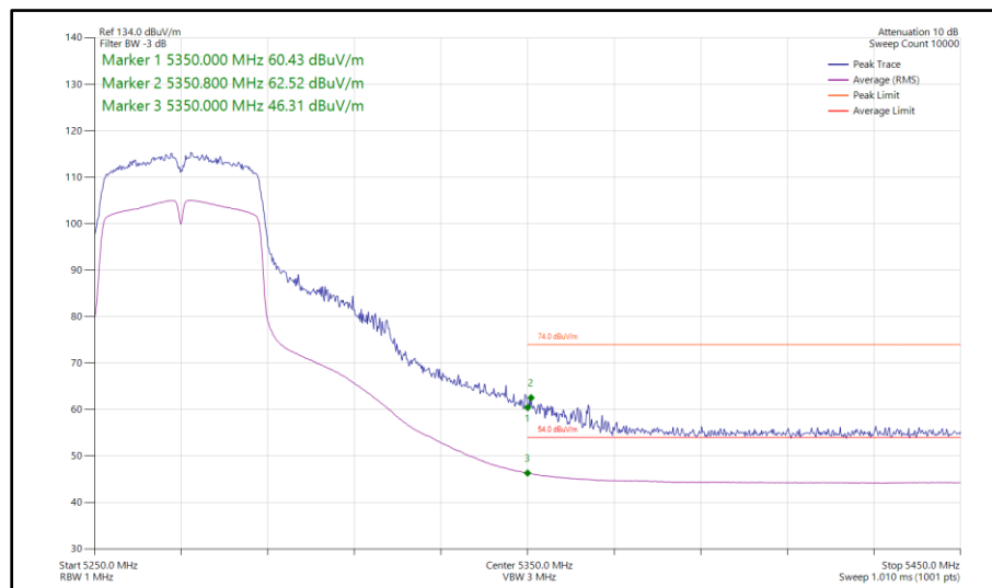
Figure 957 - 802.11n HT40, SISO, Core 1 - 5270 MHz Band Edge Frequency 5350 MHz
