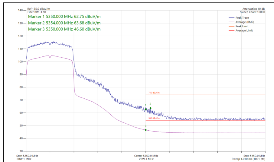
Figure 959 - 802.11ax HE40, SU, SISO, Core 1 - 5270 MHz Band Edge Frequency 5350 MHz
