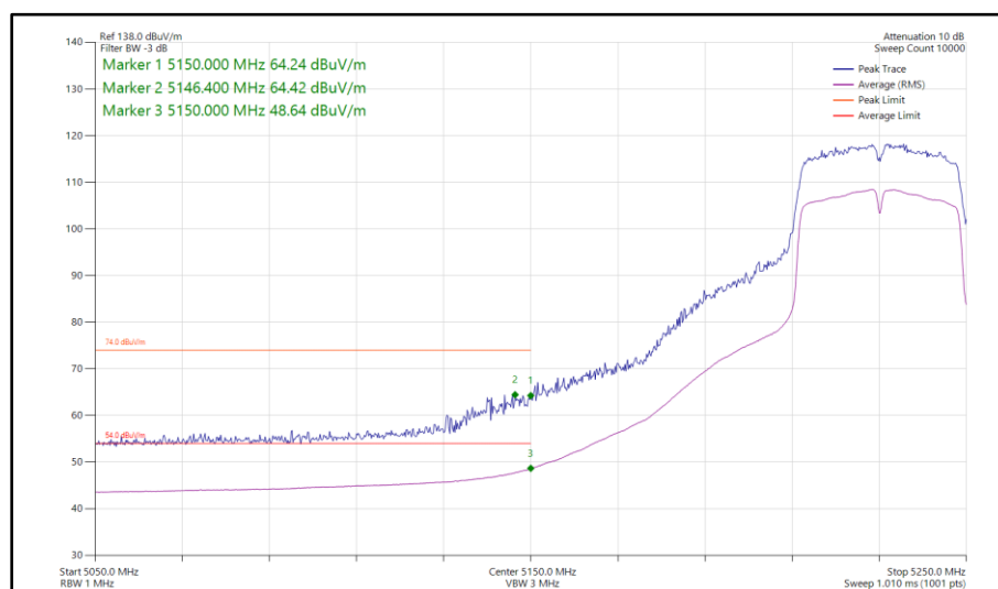
Figure 983 - 802.11n HT40, CDD, Core 0-1 - 5230 MHz Band Edge Frequency 5150 MHz
