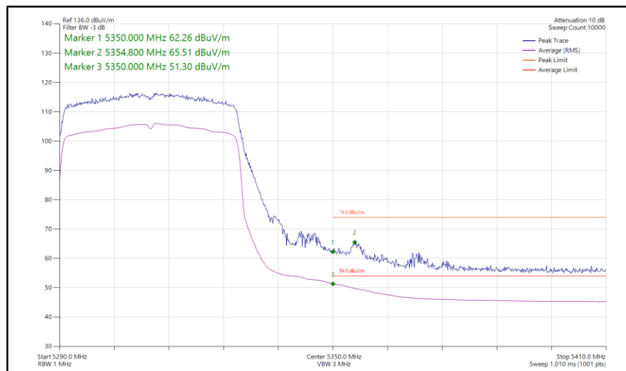
Figure 996 - 802.11ax HE40, SU, CDD, Core 0-1 - 5310 MHz Band Edge Frequency 5350 MHz
