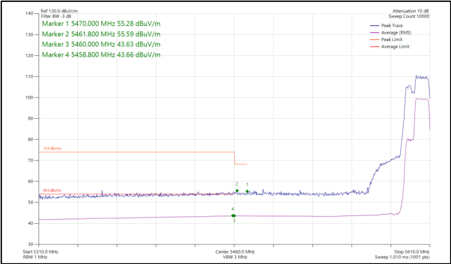
Figure 979 - 802.11be EHT40, RU 106+26-85, SISO, Core 1 - 5590 MHz Band Edge Frequency 5460 MHz
