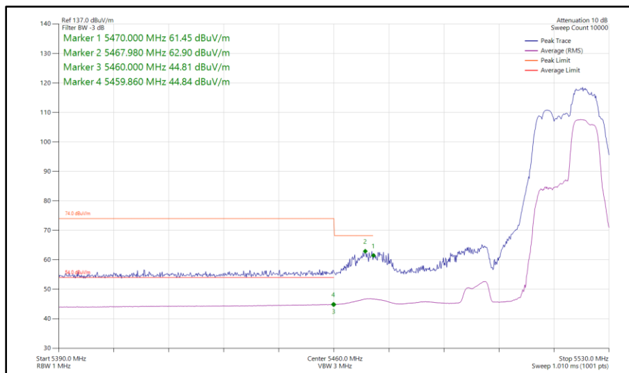
Figure 1012 - 802.11be EHT40, RU 52+26-75, CDD, Core 0-1 - 5510 MHz Band Edge Frequency 5460 MHz
