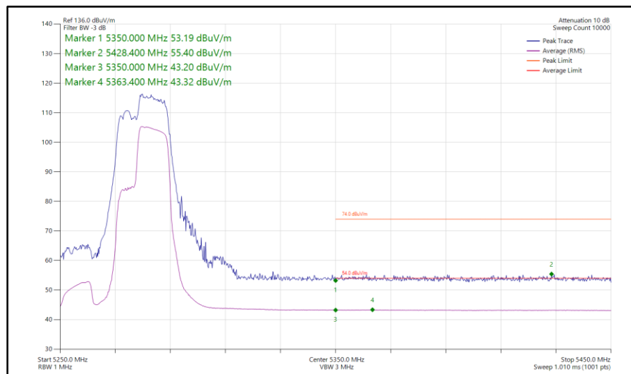
Figure 963 - 802.11be EHT40, RU 106+26-85, SISO, Core 1 - 5270 MHz Band Edge Frequency 5350 MHz
