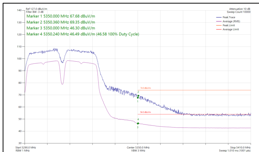
Figure 956 - 802.11a a40, SISO, Core 1 - 5310 MHz Band Edge Frequency 5350 MHz
