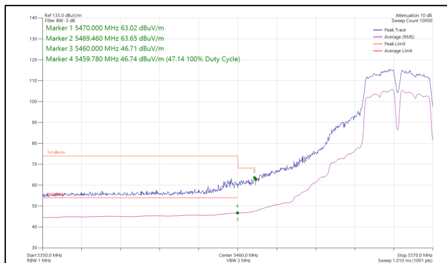
Figure 1001 - 802.11a a40, CDD, Core 0-1 - 5550 MHz Band Edge Frequency 5460 MHz
