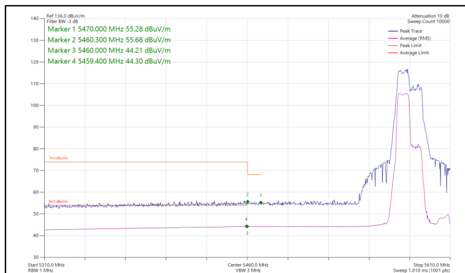
Figure 1011 - 802.11ax HE40, RU 106-53, CDD, Core 0-1 - 5590 MHz Band Edge Frequency 5460 MHz
