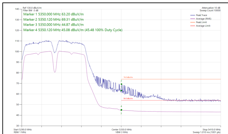
Figure 991 - 802.11a a40, CDD, Core 0-1 - 5310 MHz Band Edge Frequency 5350 MHz
