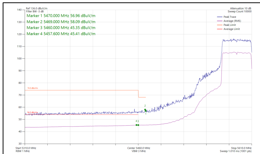
Figure 1010 - 802.11ax HE40, SU, CDD, Core 0-1 - 5590 MHz Band Edge Frequency 5460 MHz
