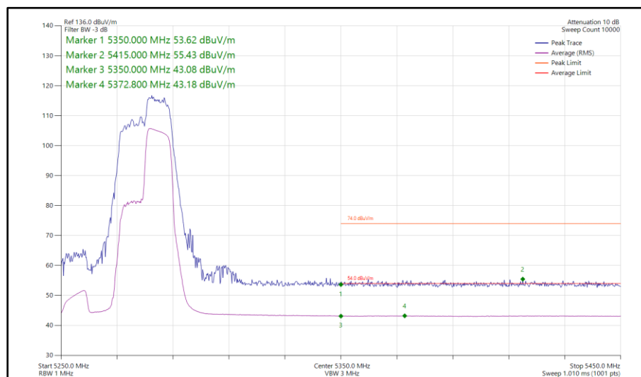
Figure 960 - 802.11ax HE40, RU 106-56, SISO, Core 1 - 5270 MHz Band Edge Frequency 5350 MHz
