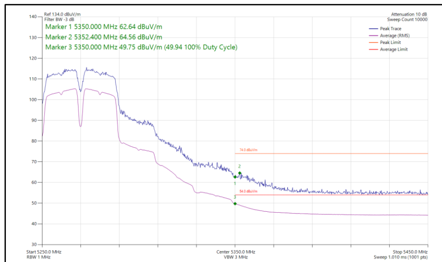
Figure 955 - 802.11a a40, SISO, Core 1 - 5270 MHz Band Edge Frequency 5350 MHz
