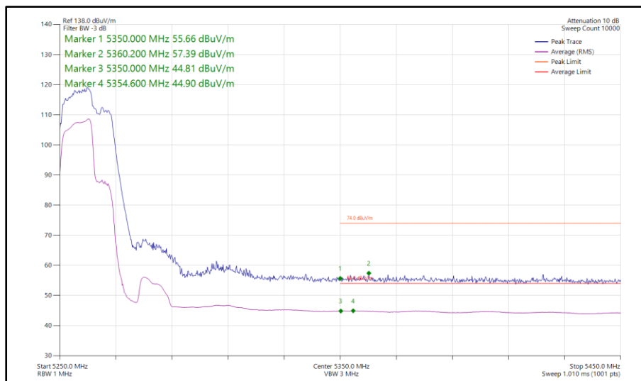
Figure 998 - 802.11be EHT40, RU 106+26-82, CDD, Core 0-1 - 5270 MHz Band Edge Frequency 5350 MHz
