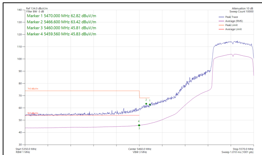
Figure 973 - 802.11ax HE40, SU, SISO, Core 1 - 5550 MHz Band Edge Frequency 5460 MHz
