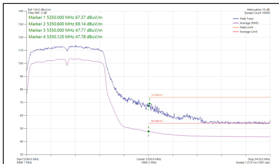
Figure 993 - 802.11n HT40, CDD, Core 0-1 - 5310 MHz Band Edge Frequency 5350 MHz
