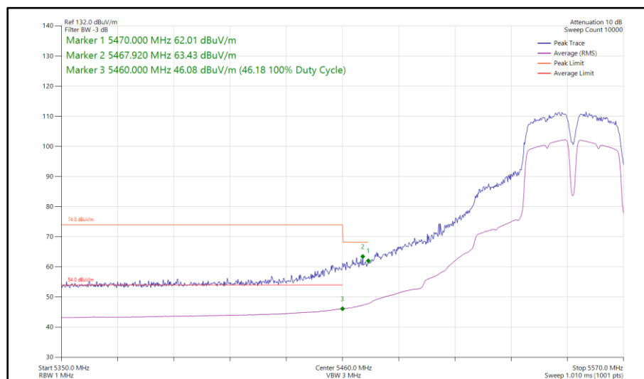
Figure 966 - 802.11a a40, SISO, Core 1 - 5550 MHz Band Edge Frequency 5460 MHz
