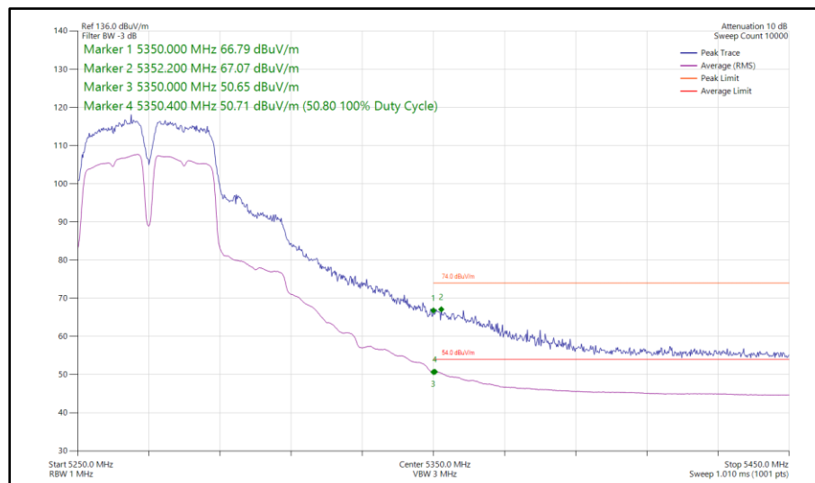
Figure 990 - 802.11a a40, CDD, Core 0-1 - 5270 MHz Band Edge Frequency 5350 MHz
