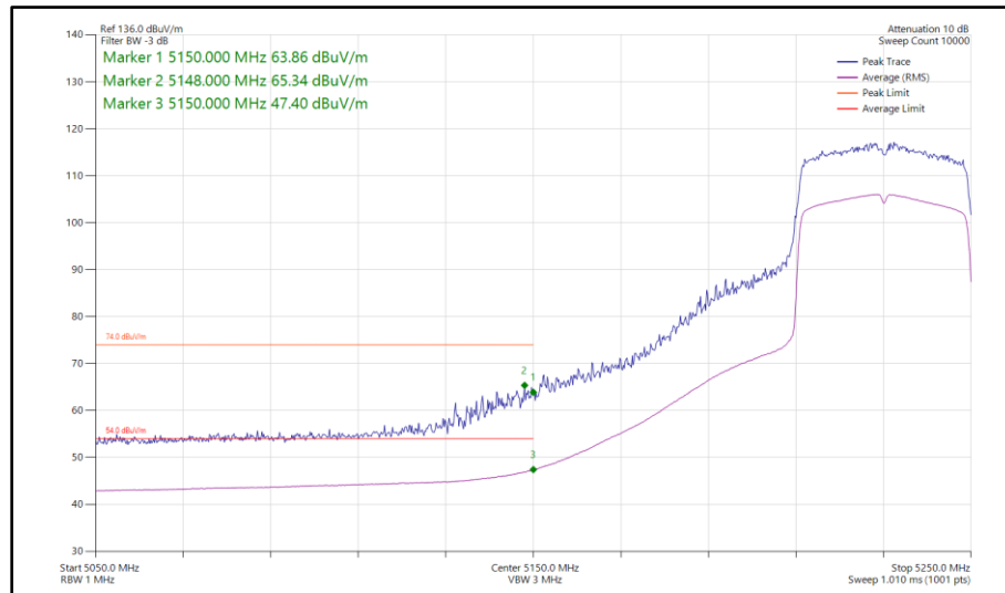
Figure 951 - 802.11ax HE40, SU, SISO, Core 1 - 5230 MHz Band Edge Frequency 5150 MHz
