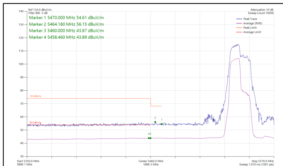
Figure 974 - 802.11ax HE40, RU 106-53, SISO, Core 1 - 5550 MHz Band Edge Frequency 5460 MHz
