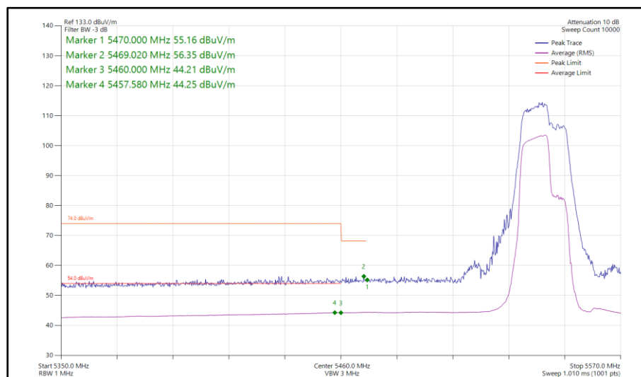
Figure 978 - 802.11be EHT40, RU 106+26-82, SISO, Core 1 - 5550 MHz Band Edge Frequency 5460 MHz
