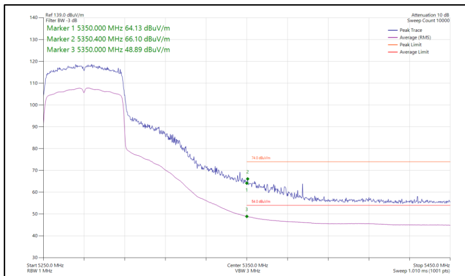
Figure 994 - 802.11ax HE40, SU, CDD, Core 0-1 - 5270 MHz Band Edge Frequency 5350 MHz
