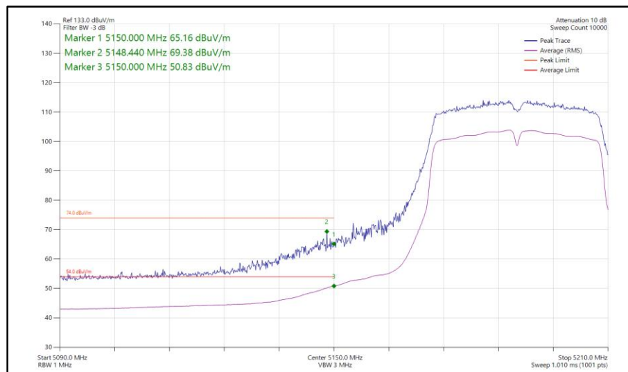
Figure 982 - 802.11n HT40, CDD, Core 0-1 - 5190 MHz Band Edge Frequency 5150 MHz
