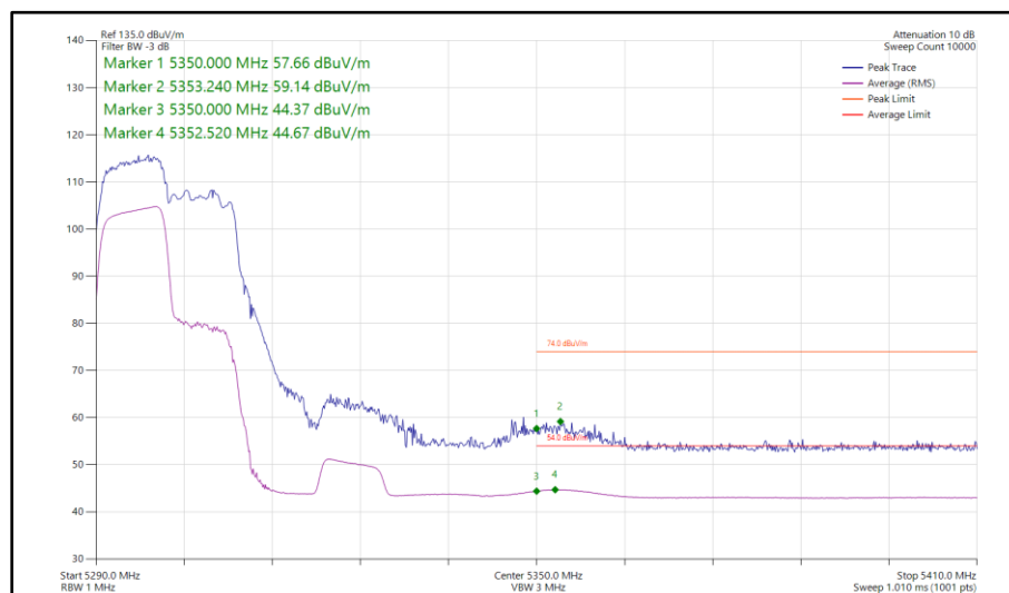
Figure 962 - 802.11ax HE40, RU 106-53, SISO, Core 1 - 5310 MHz Band Edge Frequency 5350 MHz
