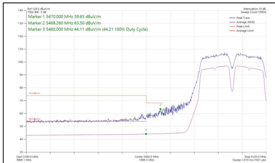
Figure 965 - 802.11a a40, SISO, Core 1 - 5510 MHz Band Edge Frequency 5460 MHz
