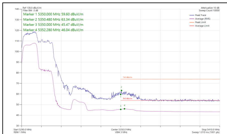
Figure 997 - 802.11ax HE40, RU 106-53, CDD, Core 0-1 - 5310 MHz Band Edge Frequency 5350 MHz
