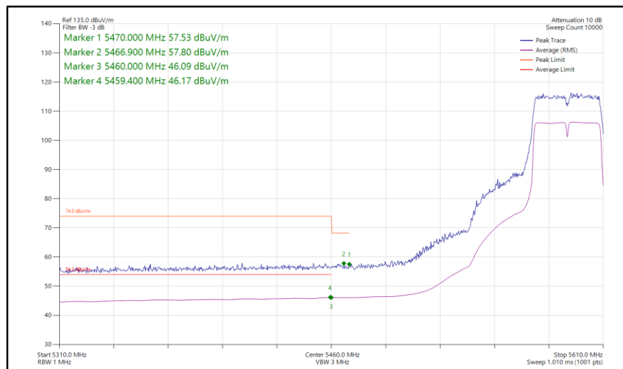
Figure 1033 - 802.11n HT40, SDM, Core 0-1 - 5590 MHz Band Edge Frequency 5460 MHz
