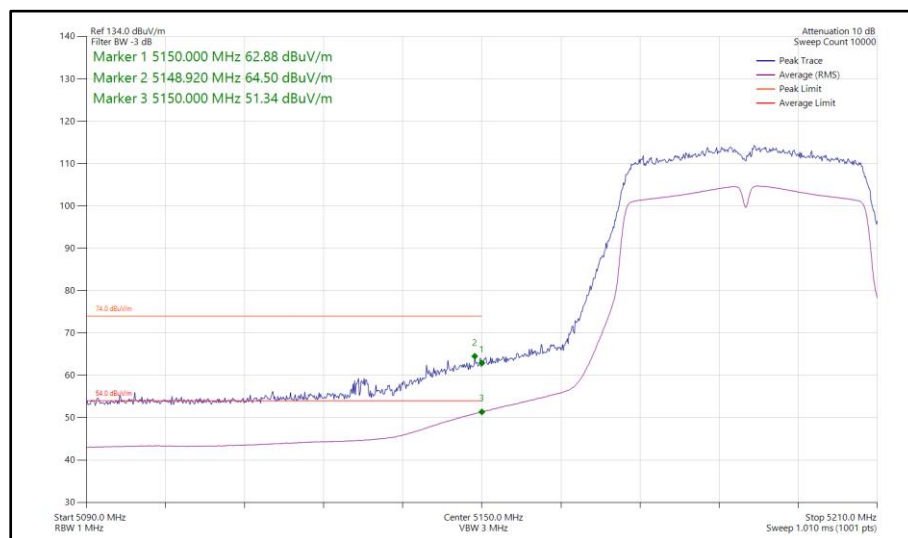
Figure 1043 - 802.11ac VHT40, TxBF, Core 0-1 - 5190 MHz Band Edge Frequency 5150 MHz
