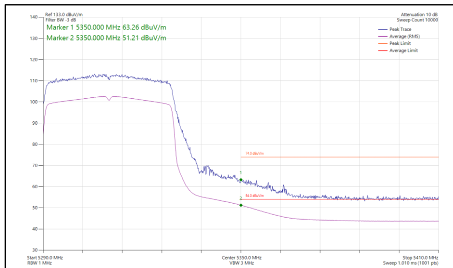
Figure 1050 - 802.11ax HE40, SU, TxBF, Core 0-1 - 5310 MHz Band Edge Frequency 5350 MHz
