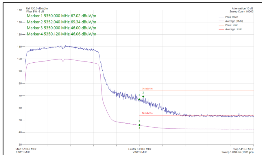
Figure 1027 - 802.11ax HE40, SU, SDM, Core 0-1 - 5310 MHz Band Edge Frequency 5350 MHz
