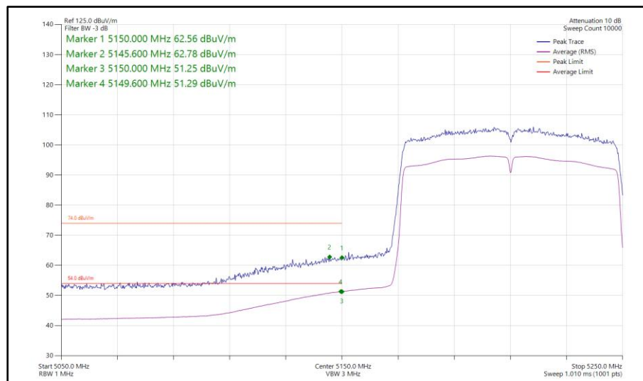
Figure 1073 - 802.11ac VHT80, SISO, Core 1 - 5210 MHz Band Edge Frequency 5150 MHz
