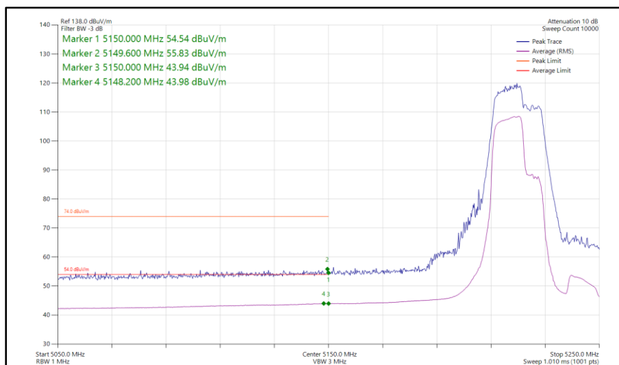
Figure 1022 - 802.11be EHT40, RU 106+26-82, SDM, Core 0-1 - 5230 MHz Band Edge Frequency 5150 MHz
