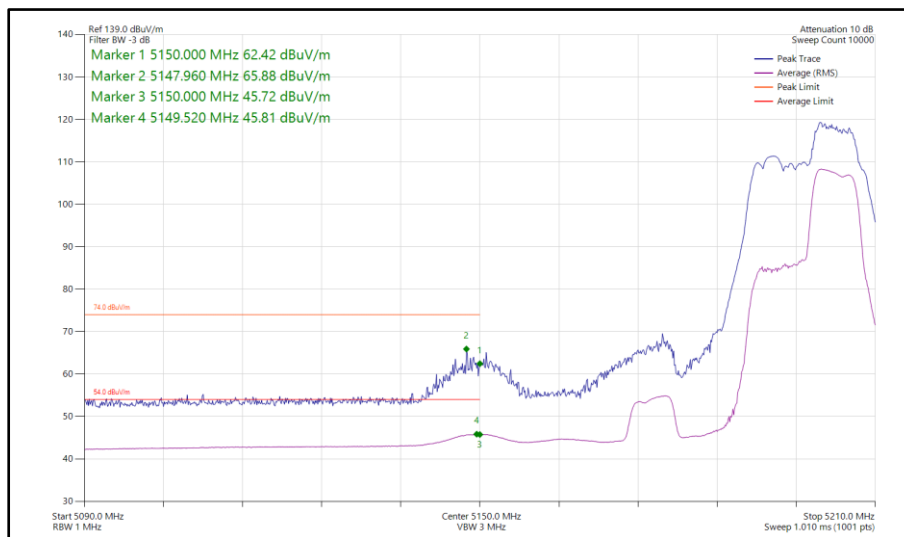
Figure 1021 - 802.11be EHT40, RU 52+26-75, SDM, Core 0-1 - 5190 MHz Band Edge Frequency 5150 MHz
