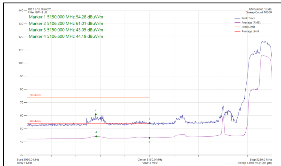
Figure 1060 - 802.11ax HE80, RU 106-60, SISO, Core 0 - 5210 MHz Band Edge Frequency 5150 MHz
