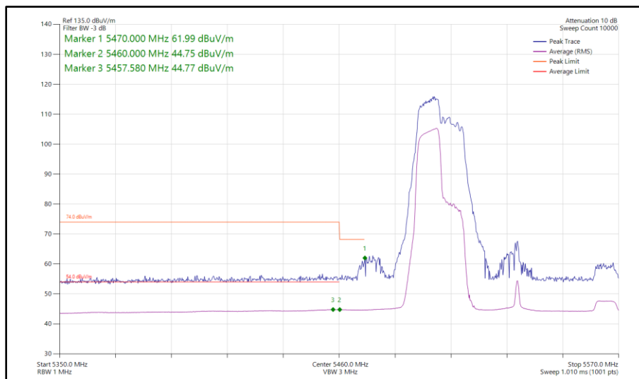
Figure 1070 - 802.11ax HE80, RU 106-53, SISO, Core 0 - 5530 MHz Band Edge Frequency 5460 MHz
