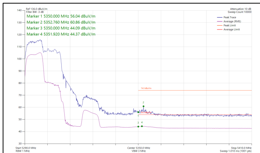
Figure 1028 - 802.11ax HE40, RU 106-53, SDM, Core 0-1 - 5310 MHz Band Edge Frequency 5350 MHz
