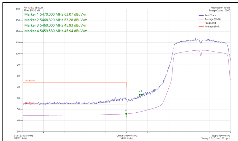
Figure 1031 - 802.11n HT40, SDM, Core 0-1 - 5510 MHz Band Edge Frequency 5460 MHz
