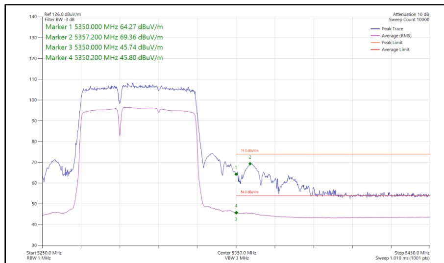
Figure 1081 - 802.11be EHT80, RU 484+242-90, SISO, Core 1 - 5290 MHz Band Edge Frequency 5350 MHz
