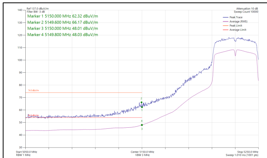
Figure 1044 - 802.11ac VHT40, TxBF, Core 0-1 - 5230 MHz Band Edge Frequency 5150 MHz
