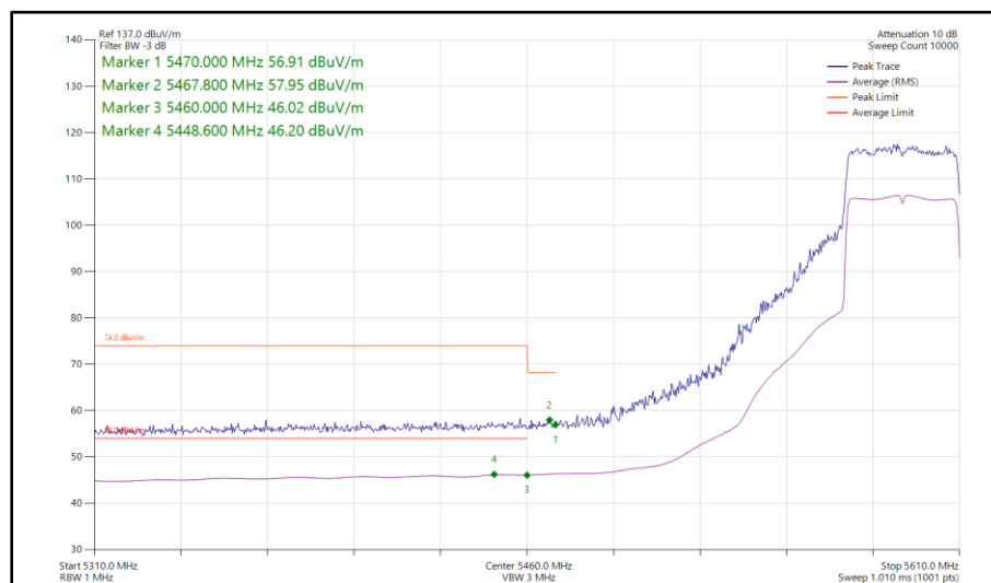
Figure 1038 - 802.11ax HE40, SU, SDM, Core 0-1 - 5590 MHz Band Edge Frequency 5460 MHz
