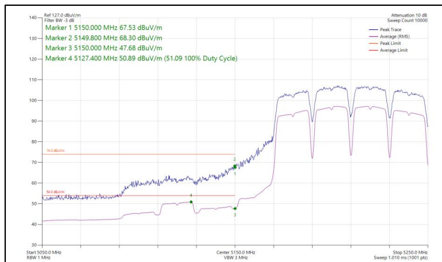
Figure 1072 - 802.11a a80, SISO, Core 1 - 5210 MHz Band Edge Frequency 5150 MHz
