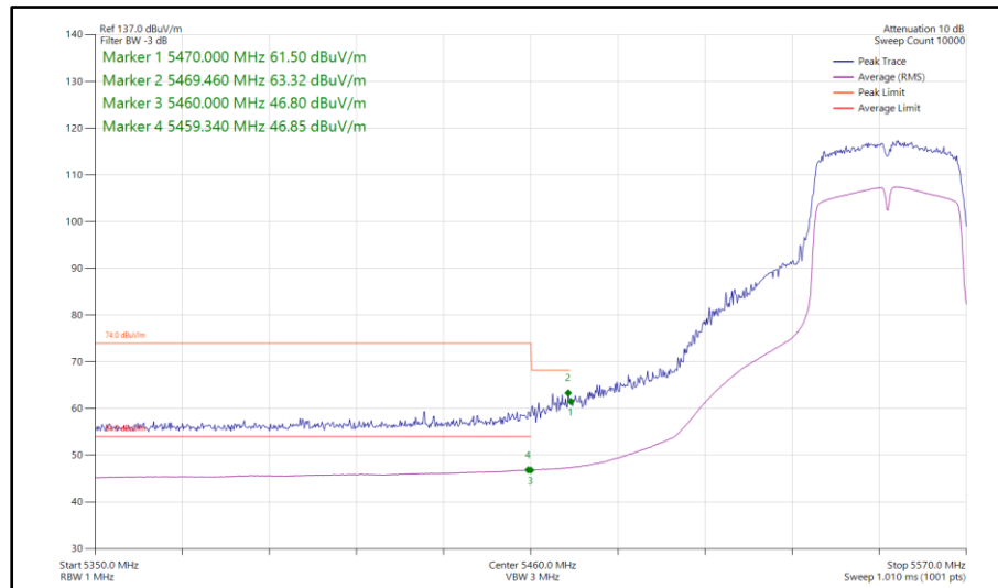
Figure 1052 - 802.11ac VHT40, TxBF, Core 0-1 - 5550 MHz Band Edge Frequency 5460 MHz
