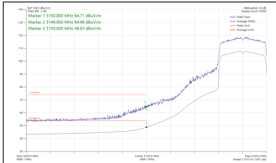
Figure 1019 - 802.11ax HE40, SU, SDM, Core 0-1 - 5230 MHz Band Edge Frequency 5150 MHz
