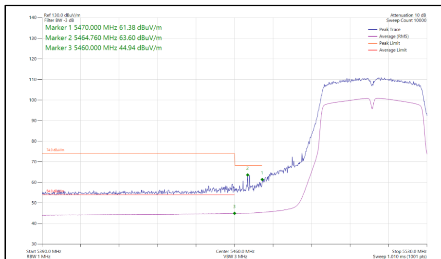
Figure 1051 - 802.11ac VHT40, TxBF, Core 0-1 - 5510 MHz Band Edge Frequency 5460 MHz
