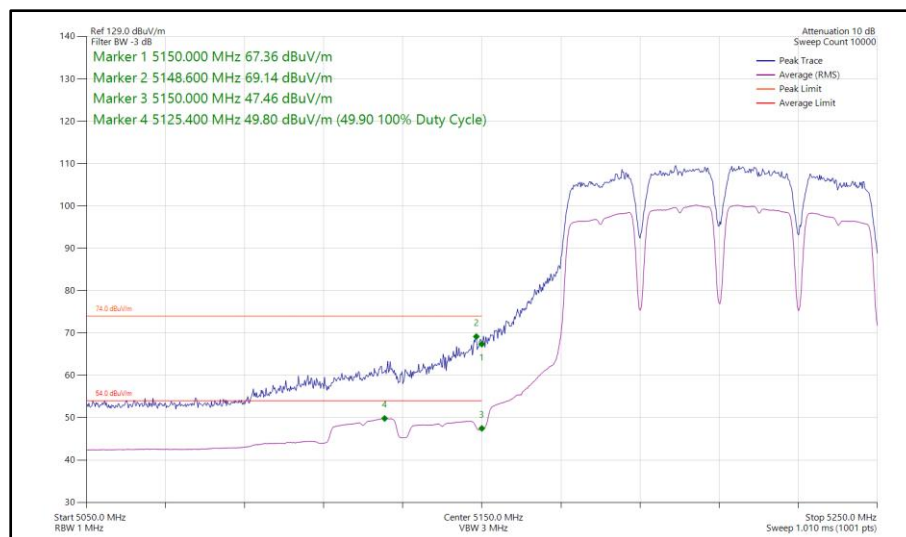
Figure 1087 - 802.11a a80, CDD, Core 0-1 - 5210 MHz Band Edge Frequency 5150 MHz
