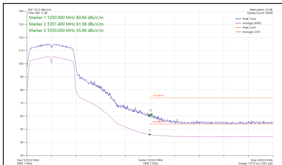
Figure 1047 - 802.11ac VHT40, TxBF, Core 0-1 - 5270 MHz Band Edge Frequency 5350 MHz
