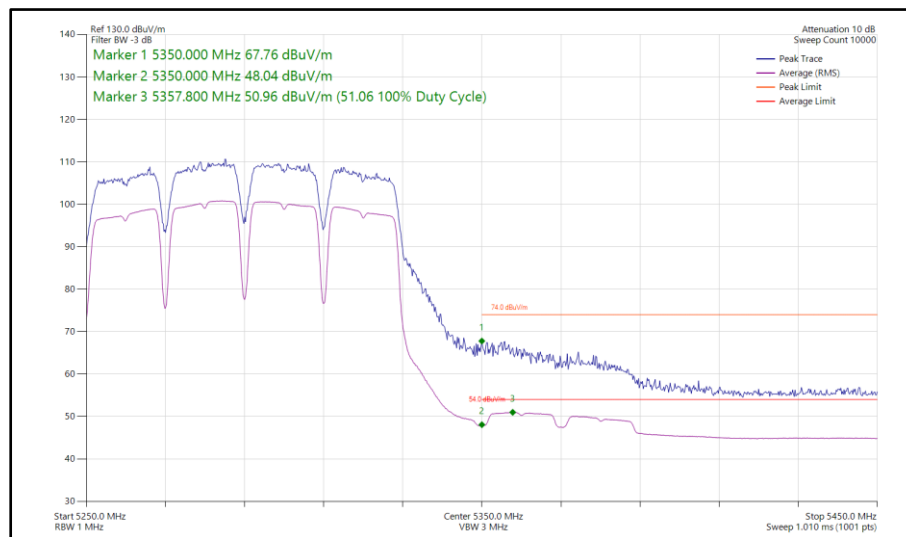
Figure 1062 - 802.11a a80, SISO, Core 0 - 5290 MHz Band Edge Frequency 5350 MHz
