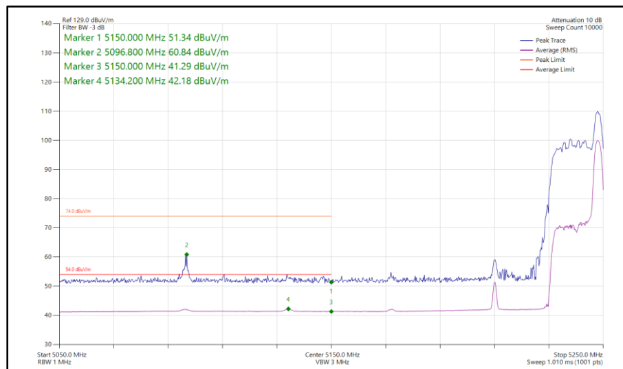
Figure 1075 - 802.11ax HE80, RU 26-36, SISO, Core 1 - 5210 MHz Band Edge Frequency 5150 MHz
