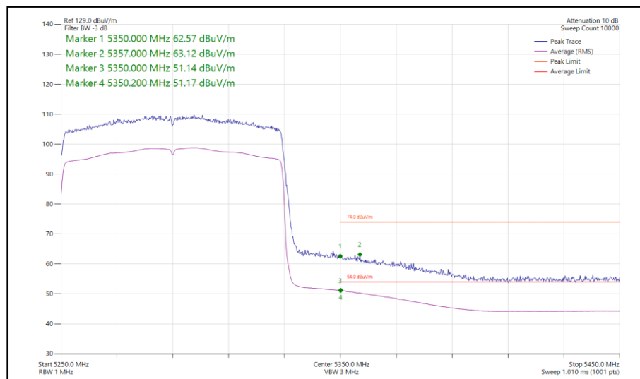
Figure 1079 - 802.11ax HE80, SU, SISO, Core 1 - 5290 MHz Band Edge Frequency 5350 MHz
