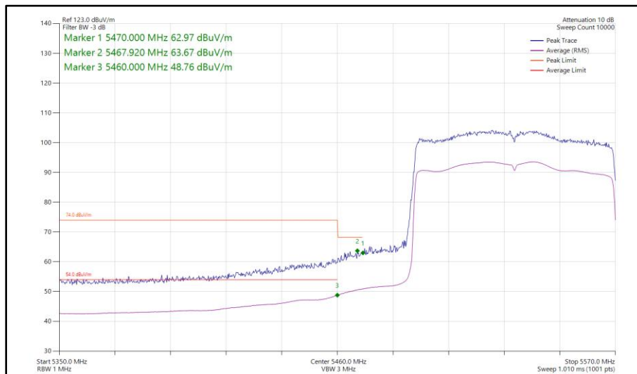
Figure 1084 - 802.11ax HE80, SU, SISO, Core 1 - 5530 MHz Band Edge Frequency 5460 MHz
