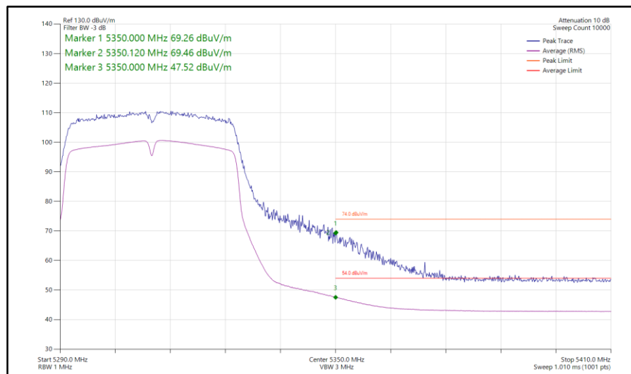
Figure 1048 - 802.11ac VHT40, TxBF, Core 0-1 - 5310 MHz Band Edge Frequency 5350 MHz
