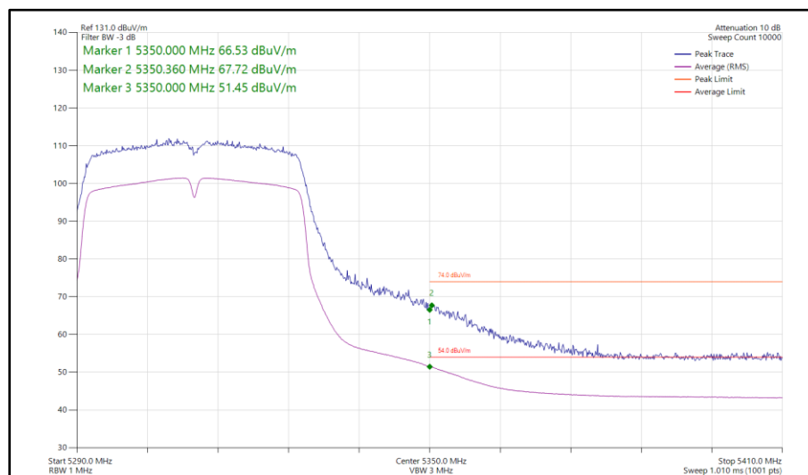
Figure 1024 - 802.11n HT40, SDM, Core 0-1 - 5310 MHz Band Edge Frequency 5350 MHz
