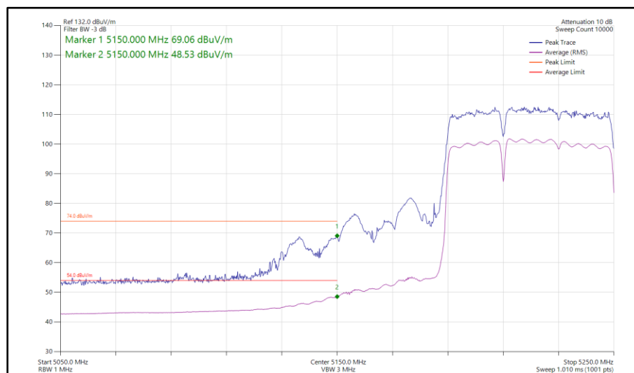
Figure 1091 - 802.11be EHT80, RU 484+242-90, CDD, Core 0-1 - 5210 MHz Band Edge Frequency 5150 MHz
