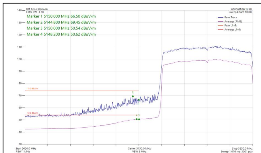
Figure 1089 - 802.11ax HE80, SU, CDD, Core 0-1 - 5210 MHz Band Edge Frequency 5150 MHz
