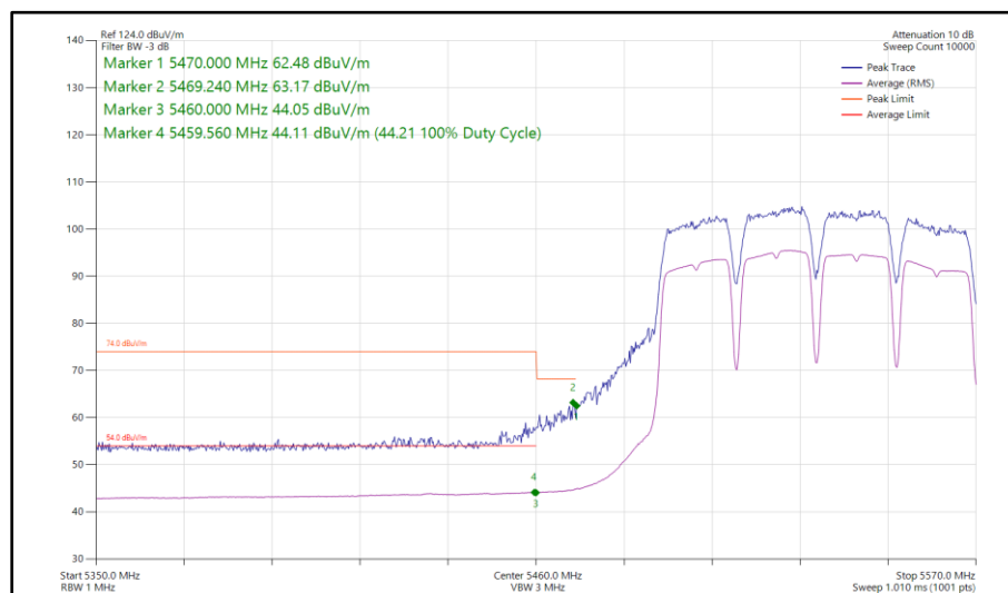
Figure 1082 - 802.11a a80, SISO, Core 1 - 5530 MHz Band Edge Frequency 5460 MHz
