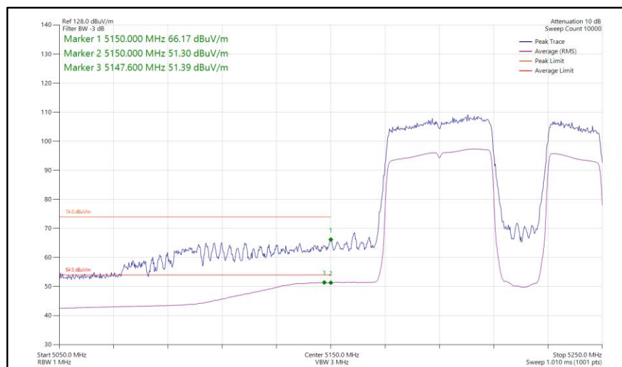
Figure 1076 - 802.11be EHT80, RU 484+242-92, SISO, Core 1 - 5210 MHz Band Edge Frequency 5150 MHz
