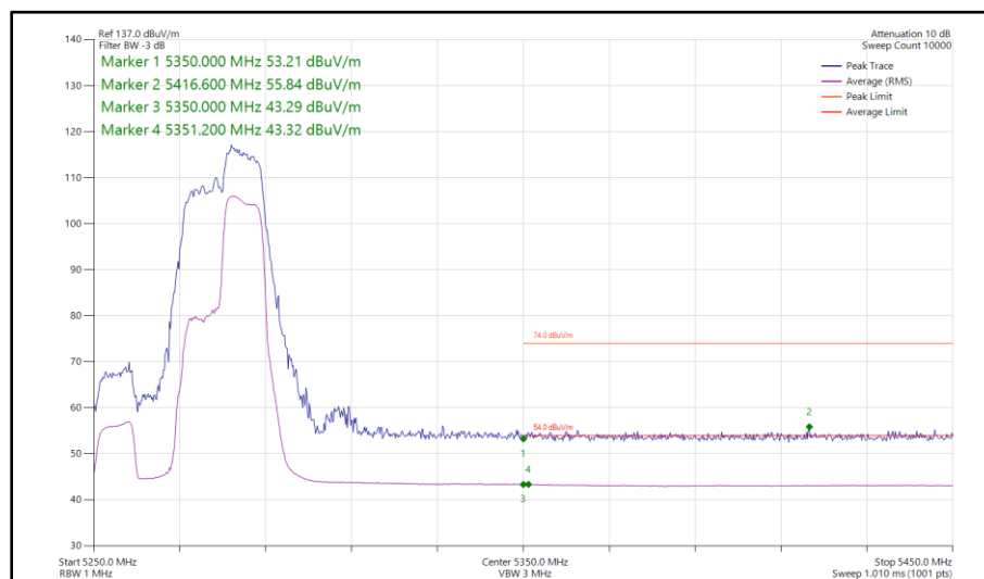
Figure 1026 - 802.11ax HE40, RU 106-56, SDM, Core 0-1 - 5270 MHz Band Edge Frequency 5350 MHz
