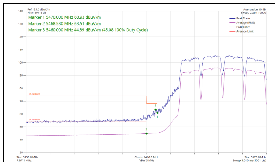
Figure 1067 - 802.11a a80, SISO, Core 0 - 5530 MHz Band Edge Frequency 5460 MHz
