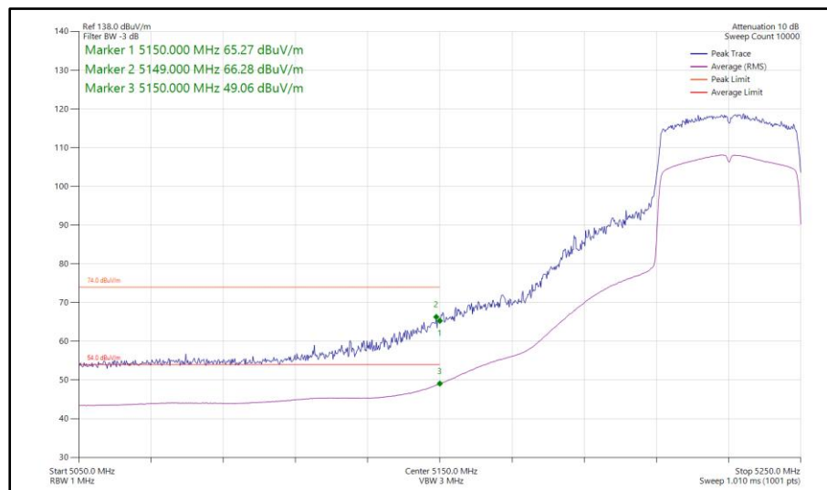
Figure 1046 - 802.11ax HE40, SU, TxBF, Core 0-1 - 5230 MHz Band Edge Frequency 5150 MHz
