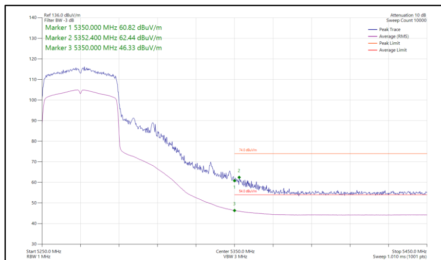
Figure 1049 - 802.11ax HE40, SU, TxBF, Core 0-1 - 5270 MHz Band Edge Frequency 5350 MHz
