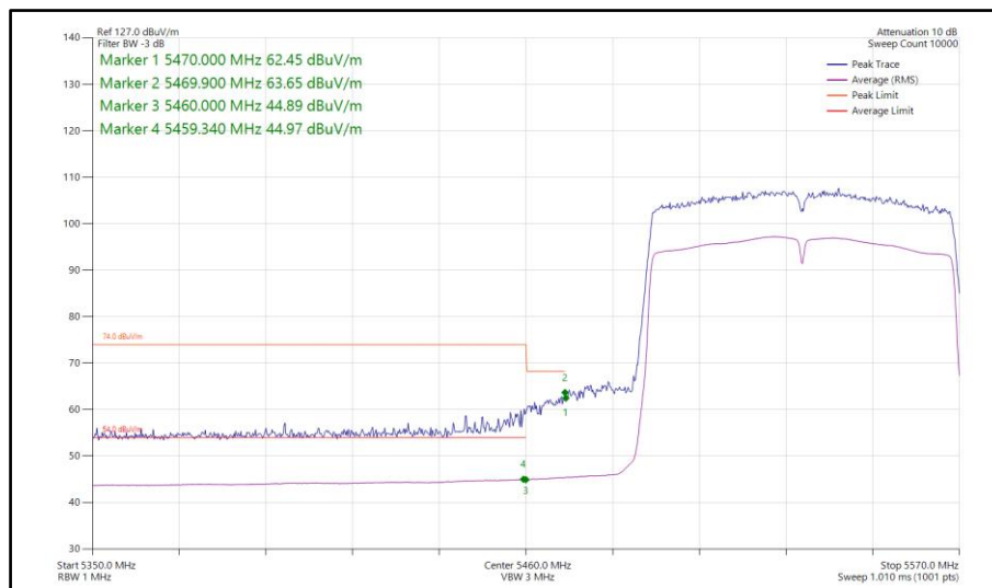
Figure 1068 - 802.11ac VHT80, SISO, Core 0 - 5530 MHz Band Edge Frequency 5460 MHz
