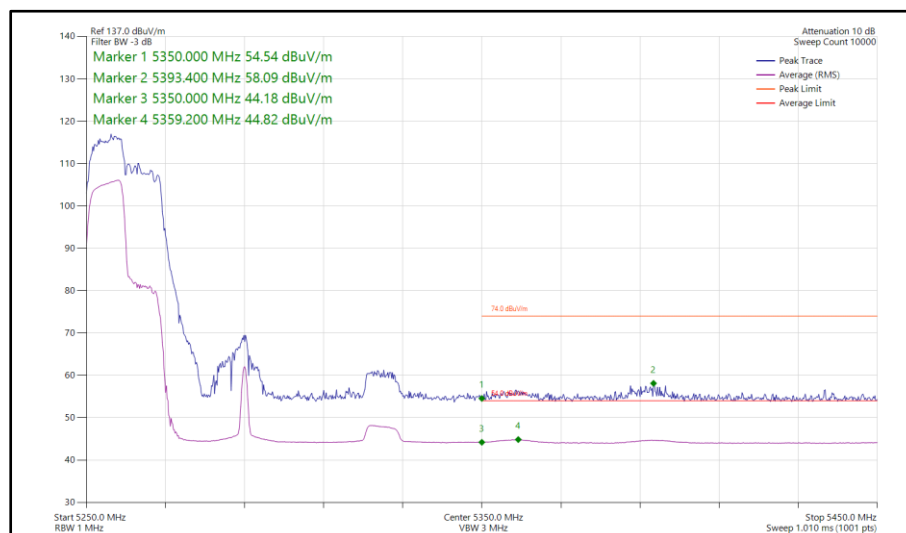
Figure 1065 - 802.11ax HE80, RU 106-53, SISO, Core 0 - 5290 MHz Band Edge Frequency 5350 MHz
