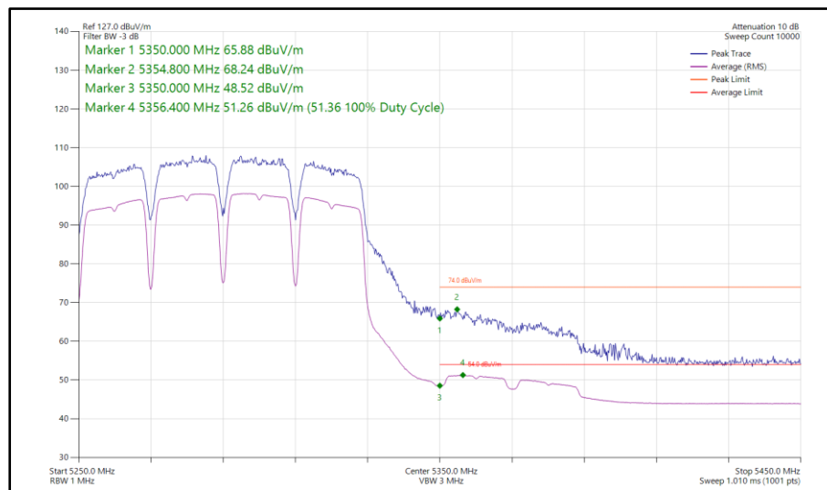
Figure 1077 - 802.11a a80, SISO, Core 1 - 5290 MHz Band Edge Frequency 5350 MHz
