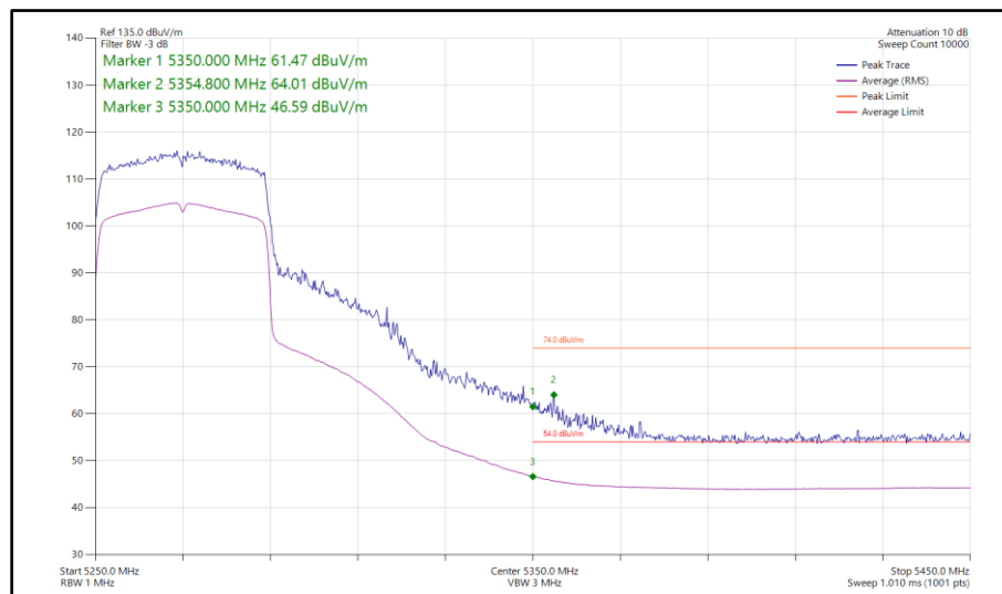
Figure 1025 - 802.11ax HE40, SU, SDM, Core 0-1 - 5270 MHz Band Edge Frequency 5350 MHz
