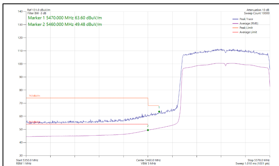
Figure 1069 - 802.11ax HE80, SU, SISO, Core 0 - 5530 MHz Band Edge Frequency 5460 MHz
