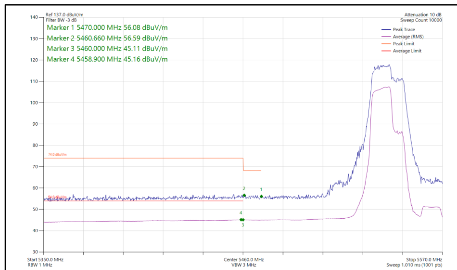
Figure 1041 - 802.11be EHT40, RU 106+26-82, SDM, Core 0-1 - 5550 MHz Band Edge Frequency 5460 MHz
