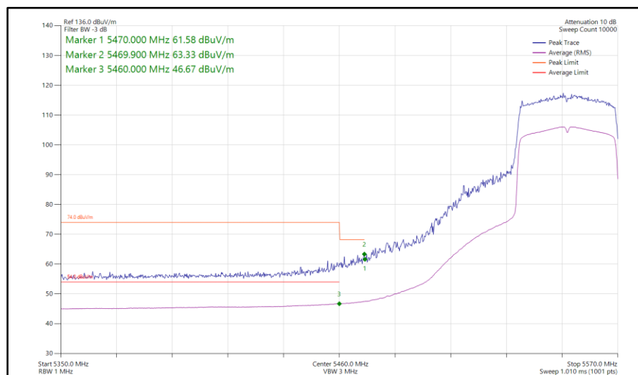
Figure 1036 - 802.11ax HE40, SU, SDM, Core 0-1 - 5550 MHz Band Edge Frequency 5460 MHz
