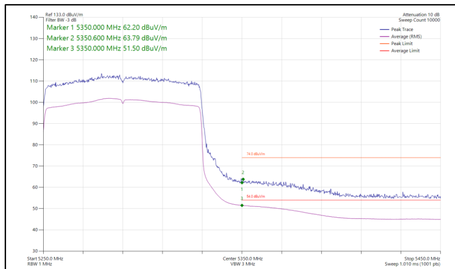
Figure 1064 - 802.11ax HE80, SU, SISO, Core 0 - 5290 MHz Band Edge Frequency 5350 MHz
