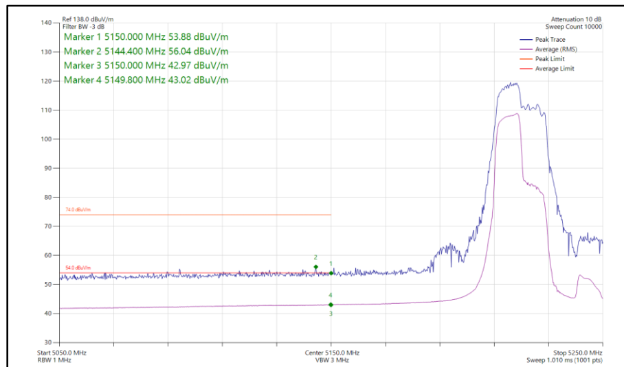
Figure 1020 - 802.11ax HE40, RU 106-53, SDM, Core 0-1 - 5230 MHz Band Edge Frequency 5150 MHz
