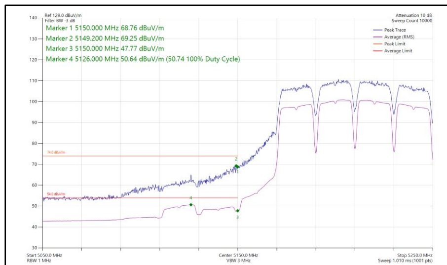
Figure 1057 - 802.11a a80, SISO, Core 0 - 5210 MHz Band Edge Frequency 5150 MHz
