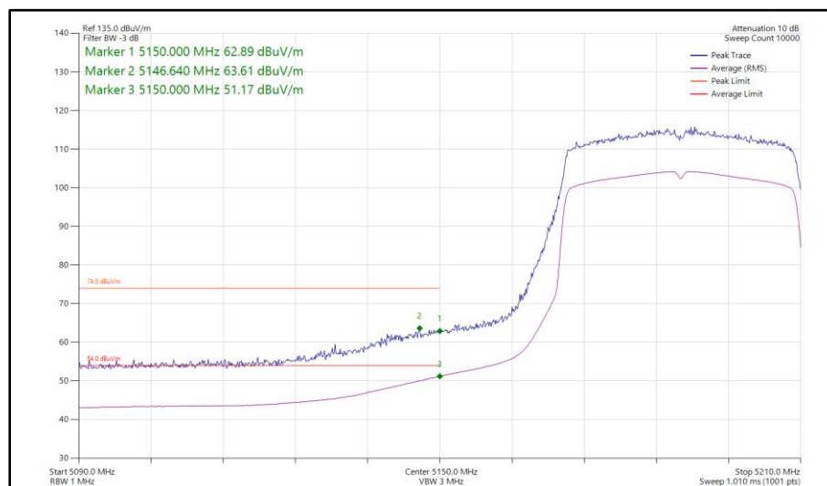
Figure 1045 - 802.11ax HE40, SU, TxBF, Core 0-1 - 5190 MHz Band Edge Frequency 5150 MHz
