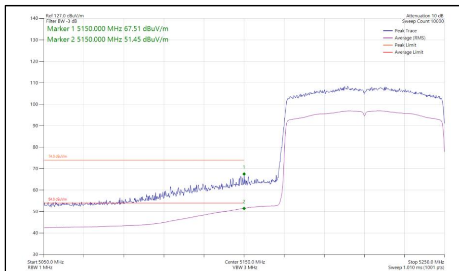
Figure 1074 - 802.11ax HE80, SU, SISO, Core 1 - 5210 MHz Band Edge Frequency 5150 MHz
