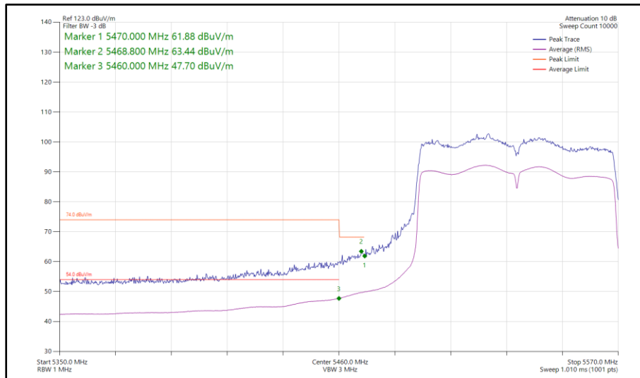
Figure 1083 - 802.11ac VHT80, SISO, Core 1 - 5530 MHz Band Edge Frequency 5460 MHz
