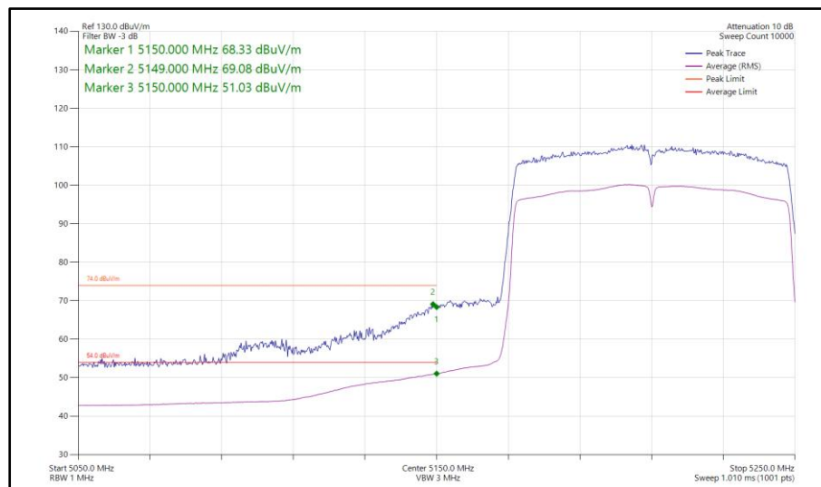
Figure 1058 - 802.11ac VHT80, SISO, Core 0 - 5210 MHz Band Edge Frequency 5150 MHz
