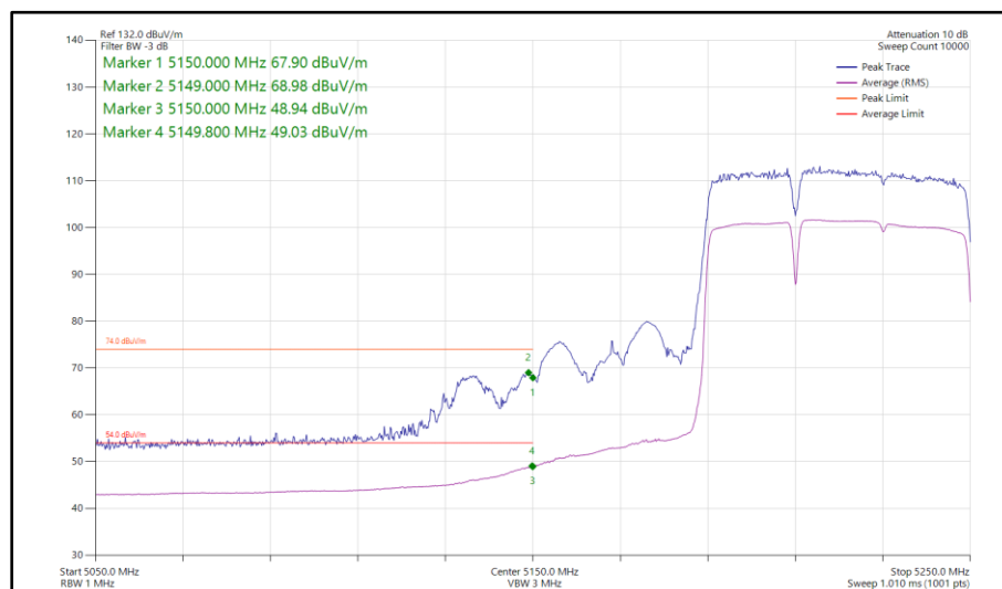
Figure 1061 - 802.11be EHT80, RU 484+242-90, SISO, Core 0 - 5210 MHz Band Edge Frequency 5150 MHz
