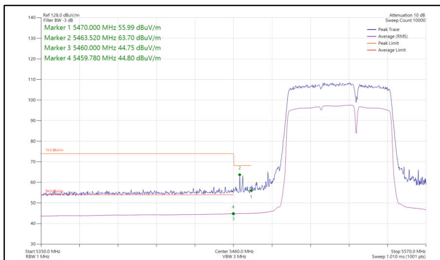
Figure 1071 - 802.11be EHT80, RU 484+242-93, SISO, Core 0 - 5530 MHz Band Edge Frequency 5460 MHz
