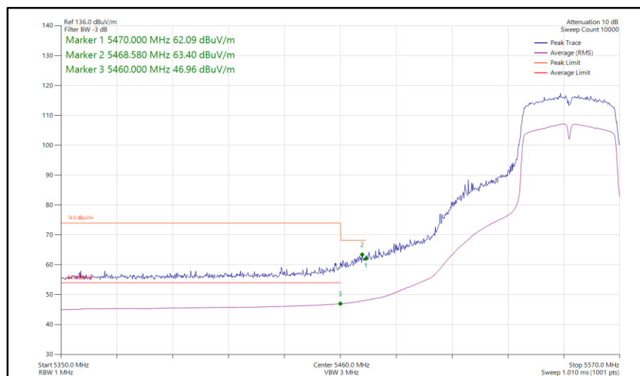
Figure 1032 - 802.11n HT40, SDM, Core 0-1 - 5550 MHz Band Edge Frequency 5460 MHz
