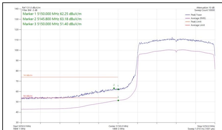
Figure 1059 - 802.11ax HE80, SU, SISO, Core 0 - 5210 MHz Band Edge Frequency 5150 MHz
