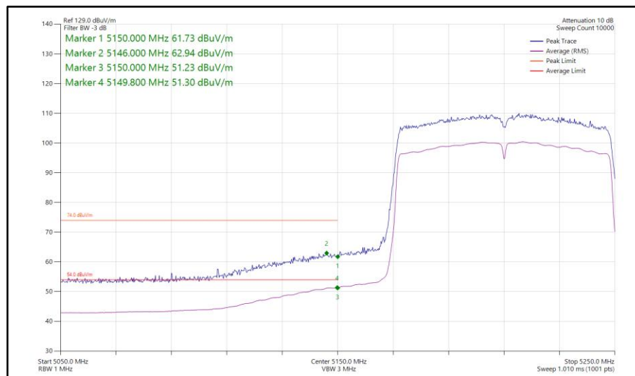
Figure 1088 - 802.11ac VHT80, CDD, Core 0-1 - 5210 MHz Band Edge Frequency 5150 MHz
