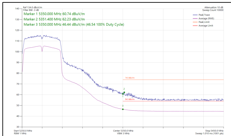
Figure 1023 - 802.11n HT40, SDM, Core 0-1 - 5270 MHz Band Edge Frequency 5350 MHz
