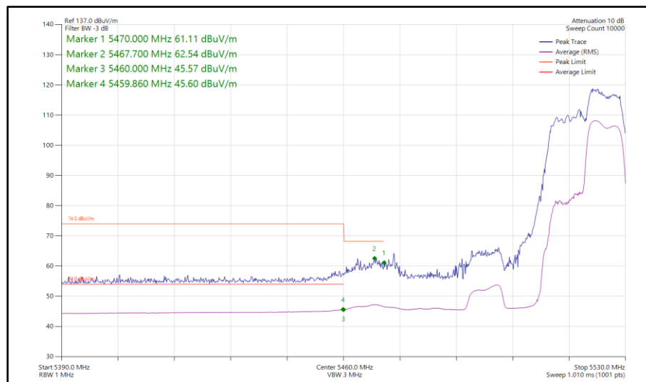
Figure 1035 - 802.11ax HE40, RU 106-56, SDM, Core 0-1 - 5510 MHz Band Edge Frequency 5460 MHz
