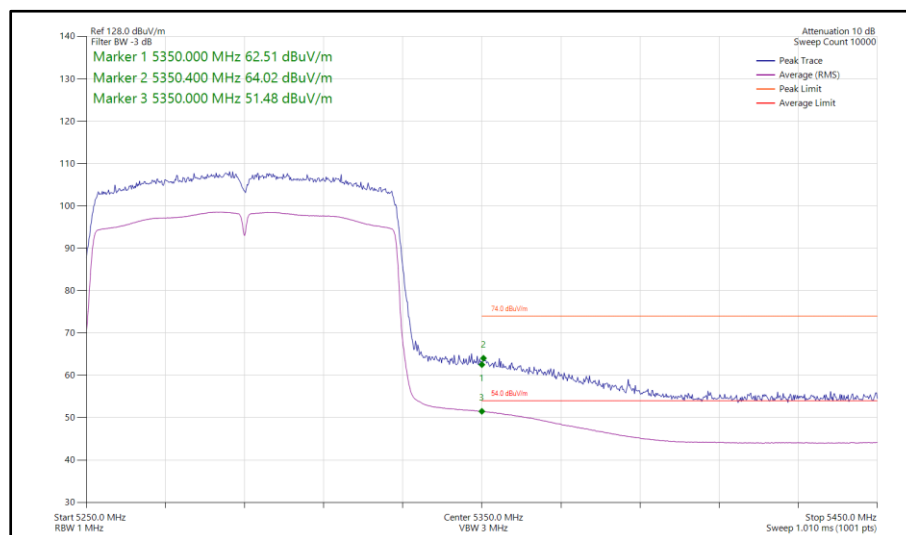
Figure 1078 - 802.11ac VHT80, SISO, Core 1 - 5290 MHz Band Edge Frequency 5350 MHz
