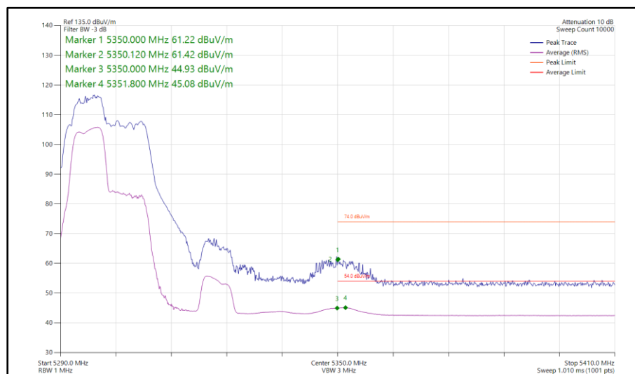
Figure 1030 - 802.11be EHT40, RU 52+26-70, SDM, Core 0-1 - 5310 MHz Band Edge Frequency 5350 MHz
