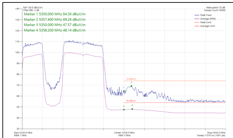
Figure 1066 - 802.11be EHT80, RU 484+242-91, SISO, Core 0 - 5290 MHz Band Edge Frequency 5350 MHz
