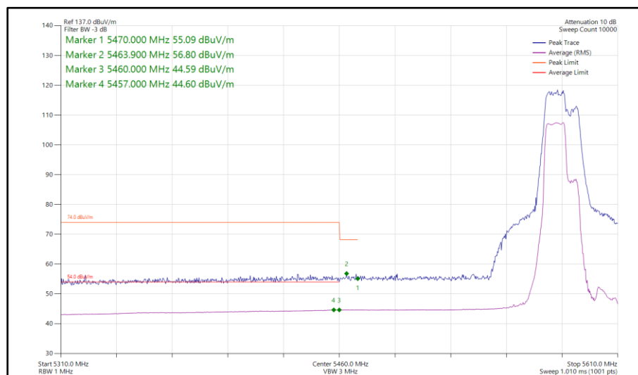
Figure 1042 - 802.11be EHT40, RU 106+26-82, SDM, Core 0-1 - 5590 MHz Band Edge Frequency 5460 MHz
