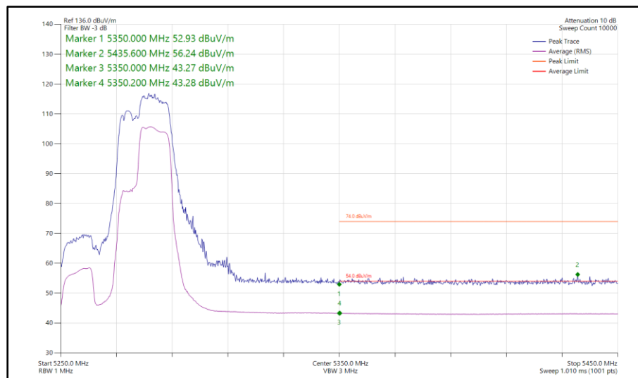
Figure 1029 - 802.11be EHT40, RU 106+26-85, SDM, Core 0-1 - 5270 MHz Band Edge Frequency 5350 MHz
