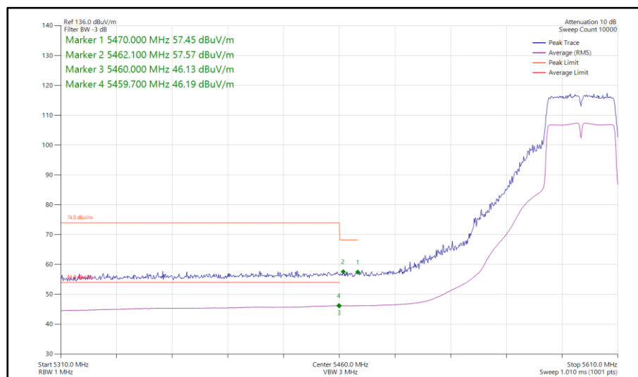
Figure 1053 - 802.11ac VHT40, TxBF, Core 0-1 - 5590 MHz Band Edge Frequency 5460 MHz
