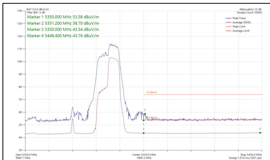
Figure 1080 - 802.11ax HE80, RU 106-60, SISO, Core 1 - 5290 MHz Band Edge Frequency 5350 MHz
