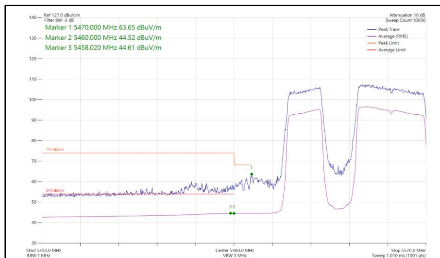
Figure 1086 - 802.11be EHT80, RU 484+242-91, SISO, Core 1 - 5530 MHz Band Edge Frequency 5460 MHz
