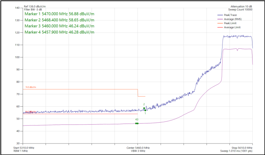
Figure 1056 - 802.11ax HE40, SU, TxBF, Core 0-1 - 5590 MHz Band Edge Frequency 5460 MHz
