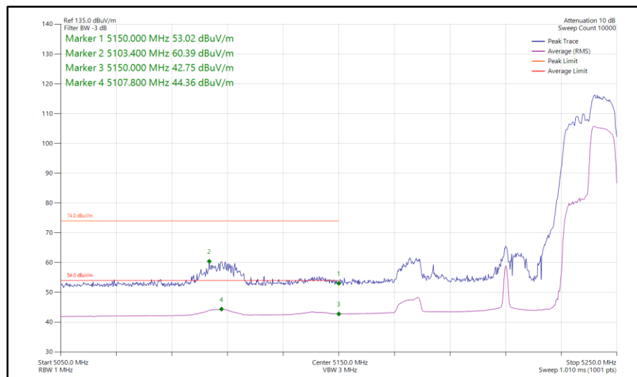
Figure 1090 - 802.11ax HE80, RU 106-60, CDD, Core 0-1 - 5210 MHz Band Edge Frequency 5150 MHz
