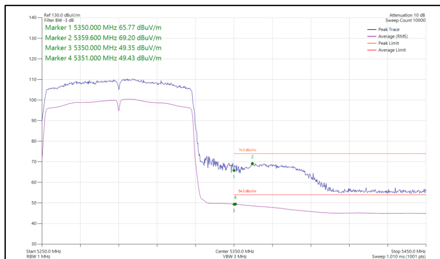
Figure 1063 - 802.11ac VHT80, SISO, Core 0 - 5290 MHz Band Edge Frequency 5350 MHz
