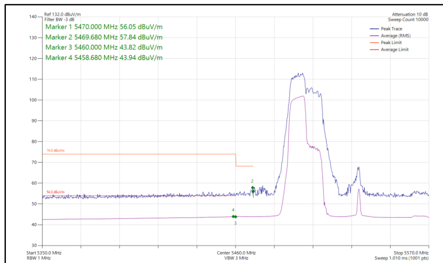
Figure 1085 - 802.11ax HE80, RU 106-53, SISO, Core 1 - 5530 MHz Band Edge Frequency 5460 MHz
