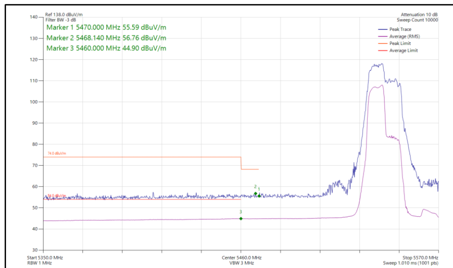
Figure 1037 - 802.11ax HE40, RU 106-53, SDM, Core 0-1 - 5550 MHz Band Edge Frequency 5460 MHz
