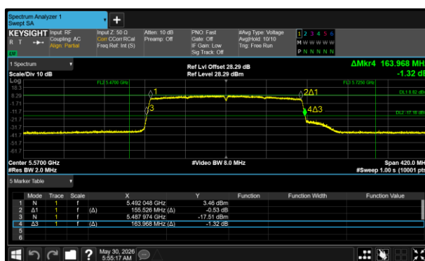
Figure 81 - 802.11ax HE160 SU Minimum 26 dB EBW
