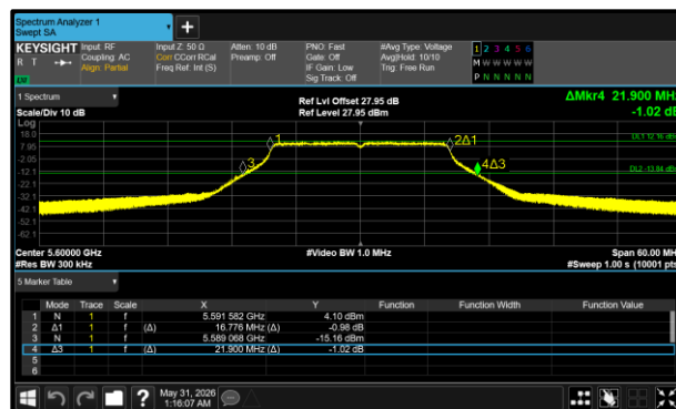
Figure 18 - 802.11a20 Maximum 26 dB EBW
