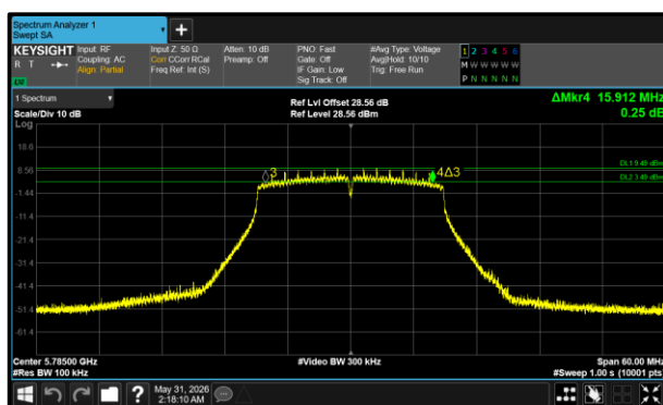
Figure 91 - 802.11n HT20 Minimum 6 dB EBW
