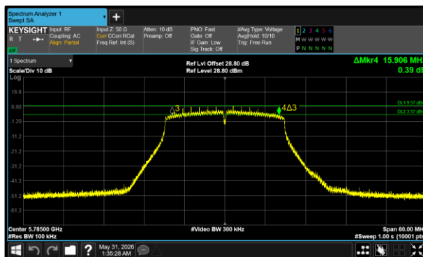
Figure 25 - 802.11n HT20 Minimum 6 dB EBW
