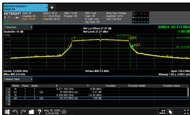
Figure 11 - 802.11ax HE40 SU Minimum 26 dB EBW
