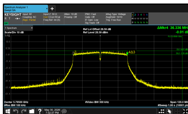
Figure 94 - 802.11n HT40 Maximum 6 dB EBW
