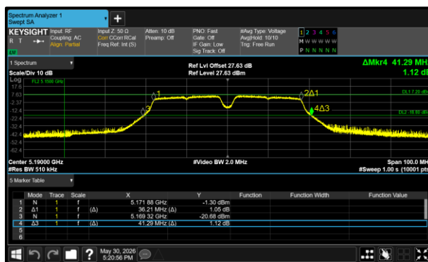
Figure 85 - 802.11a40 Minimum 26 dB EBW
