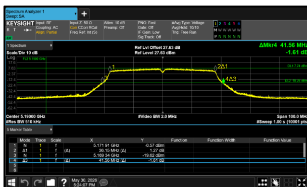
Figure 69 - 802.11n HT40 Minimum 26 dB EBW
