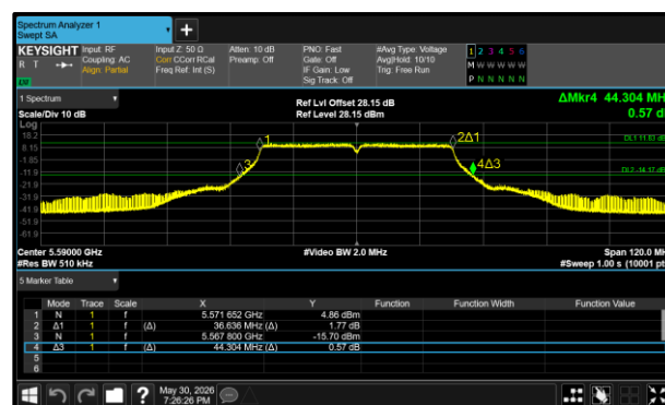
Figure 70 - 802.11n HT40 Maximum 26 dB EBW
