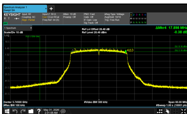
Figure 97 - 802.11ax HE20 SU Minimum 6 dB EBW
