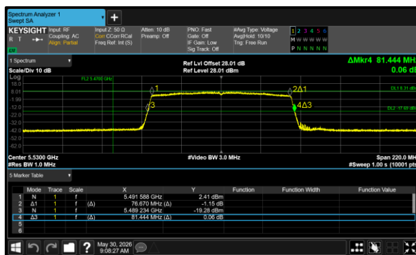
Figure 79 - 802.11ax HE80 SU Minimum 26 dB EBW
