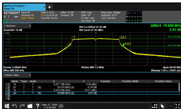
Figure 17 - 802.11a20 Minimum 26 dB EBW
