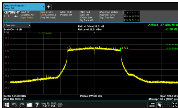
Figure 99 - 802.11ax HE40 SU Minimum 6 dB EBW
