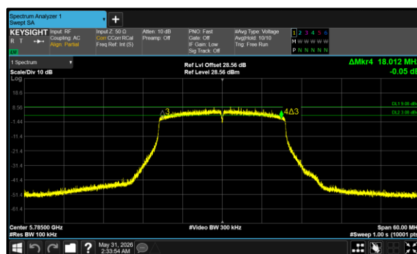
Figure 98 - 802.11ax HE20 SU Maximum 6 dB EBW
