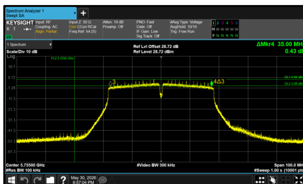
Figure 27 - 802.11n HT40 Minimum 6 dB EBW
