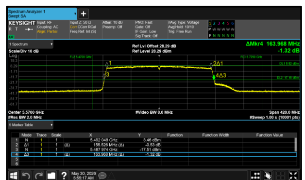
Figure 82 - 802.11ax HE160 SU Maximum 26 dB EBW
