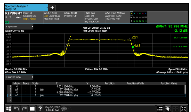
Figure 80 - 802.11ax HE80 SU Maximum 26 dB EBW
