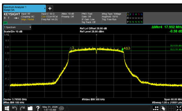
Figure 31 - 802.11ax HE20 SU Minimum 6 dB EBW
