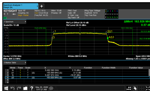
Figure 16 - 802.11ax HE160 SU Maximum 26 dB EBW
