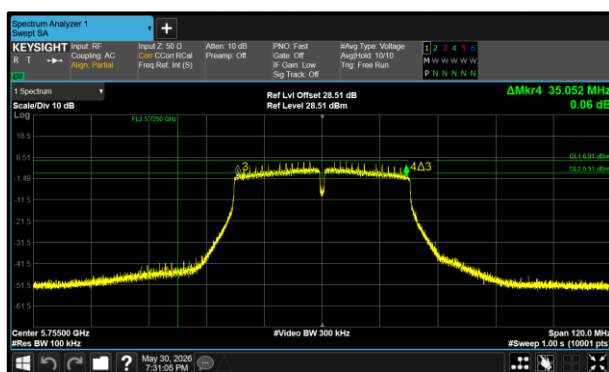
Figure 93 - 802.11n HT40 Minimum 6 dB EBW
