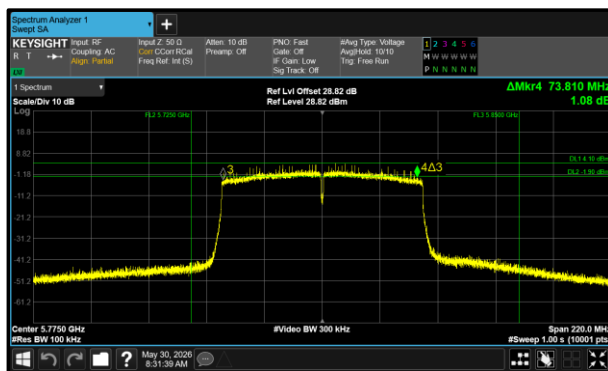
Figure 29 - 802.11ac VHT80 Minimum 6 dB EBW
