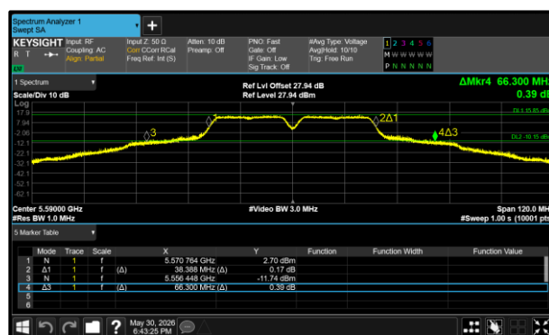
Figure 20 - 802.11a40 Maximum 26 dB EBW
