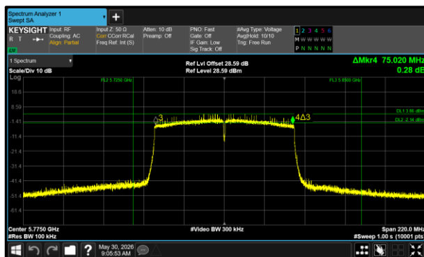
Figure 95 - 802.11ac VHT80 Minimum 6 dB EBW
