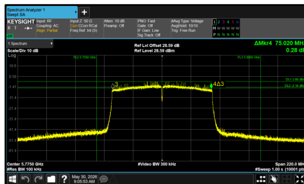
Figure 96 - 802.11ac VHT80 Maximum 6 dB EBW
