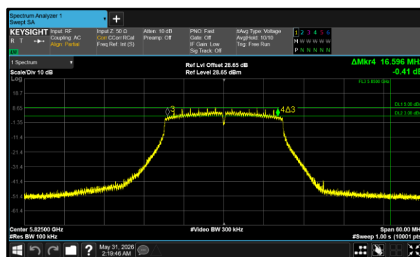
Figure 92 - 802.11n HT20 Maximum 6 dB EBW
