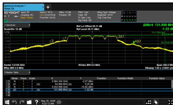
Figure 22 - 802.11a80 Maximum 26 dB EBW
