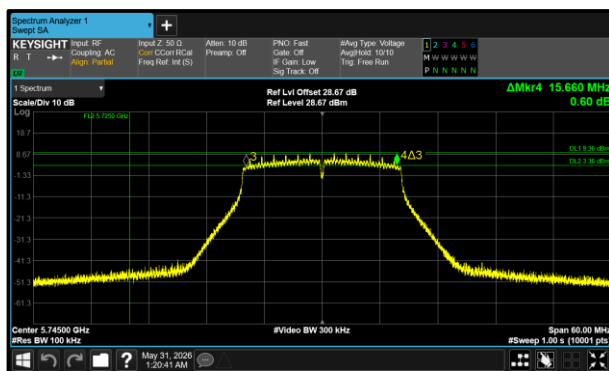
Figure 37 - 802.11a20 Minimum 6 dB EBW
