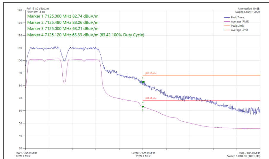
Figure 442 - 802.11a a40, SISO, Core 0 - 7085 MHz Band Edge Frequency 7125 MHz
