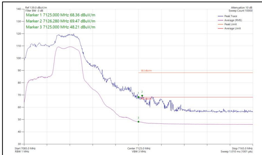
Figure 420 - 802.11ax HE20, RU 106-54, CDD, Core 0-1 - 7095 MHz Band Edge Frequency 7125 MHz
