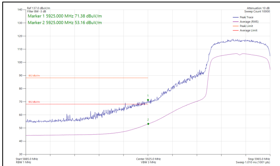
Figure 402 - 802.11ax HE20, SU, SISO, Core 1 - 5955 MHz Band Edge Frequency 5925 MHz
