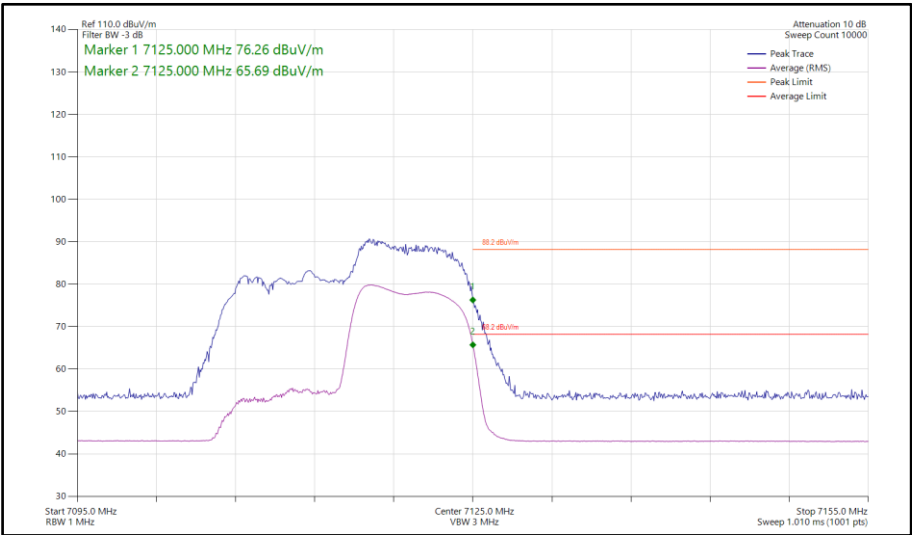
Figure 431 - 802.11ax HE20, RU 106-54, SDM, Core 0-1 - 7115 MHz Band Edge Frequency 7125 MHz
