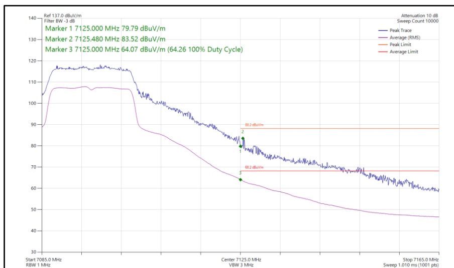
Figure 417 - 802.11a, CDD, Core 0-1 - 7095 MHz Band Edge Frequency 7125 MHz
