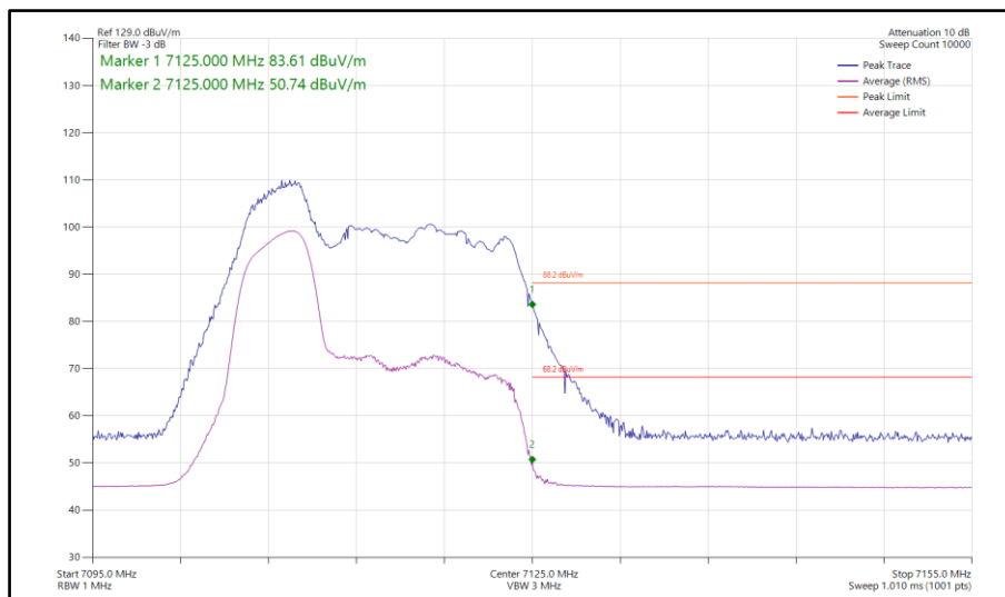
Figure 422 - 802.11ax HE20, RU 52-37, CDD, Core 0-1 - 7115 MHz Band Edge Frequency 7125 MHz
