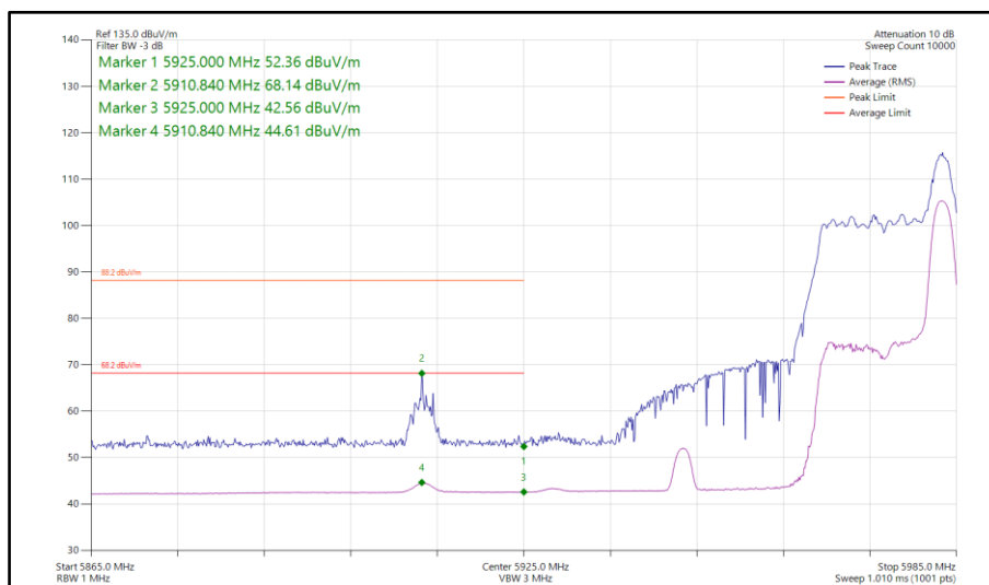
Figure 459 - 802.11ax HE40, RU 26-17, CDD, Core 0-1 - 5965 MHz Band Edge Frequency 5925 MHz
