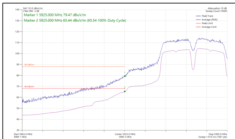
Figure 437 - 802.11a a40, SISO, Core 0 - 5965 MHz Band Edge Frequency 5925 MHz
