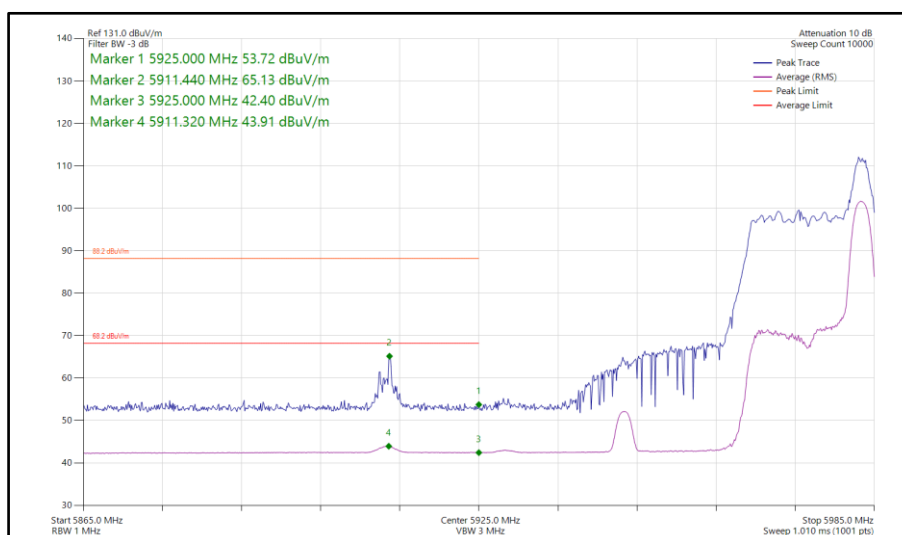
Figure 449 - 802.11ax HE40, RU 26-17, SISO, Core 1 - 5965 MHz Band Edge Frequency 5925 MHz
