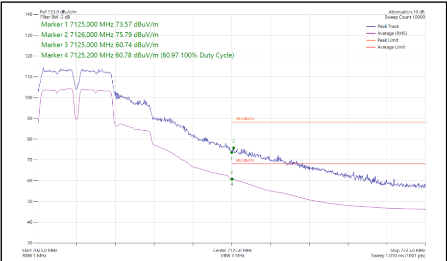
Figure 441 - 802.11a a40, SISO, Core 0 - 7045 MHz Band Edge Frequency 7125 MHz
