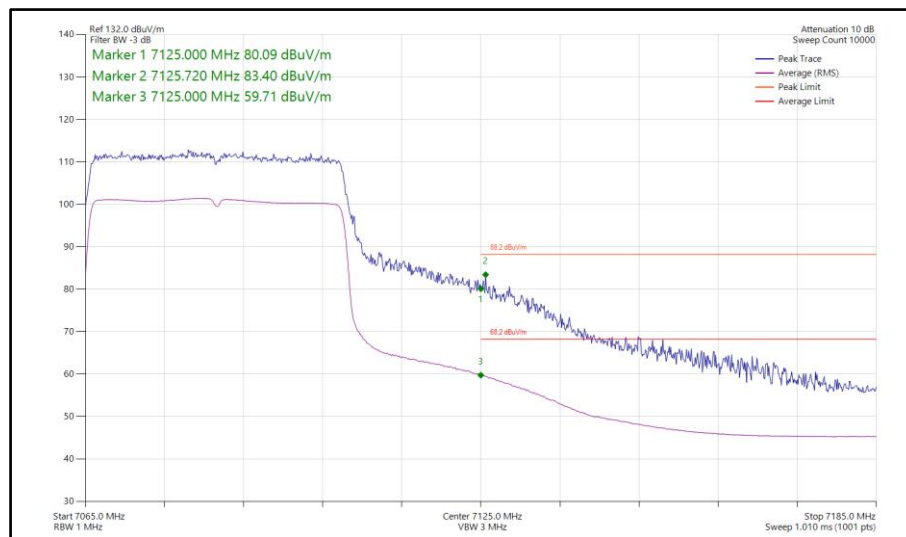
Figure 454 - 802.11ax HE40, SU, SISO, Core 1 - 7085 MHz Band Edge Frequency 7125 MHz
