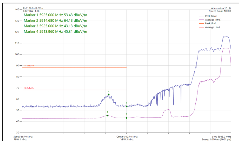
Figure 439 - 802.11ax HE40, RU 52-44, SISO, Core 0 - 5965 MHz Band Edge Frequency 5925 MHz
