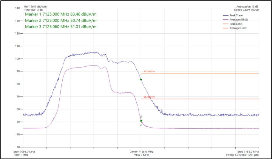
Figure 424 - 802.11be EHT20, CDD, RU 106+26-83, Core 0-1 - 7115 MHz Band Edge Frequency 7125 MHz
