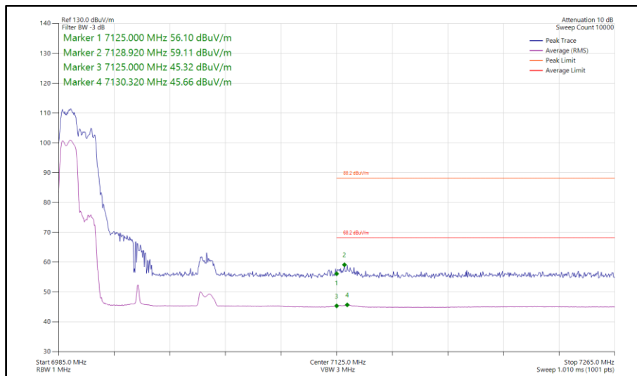
Figure 507 - 802.11ax HE80, RU 106-53, CDD, Core 0-1 - 7025 MHz Band Edge Frequency 7125 MHz
