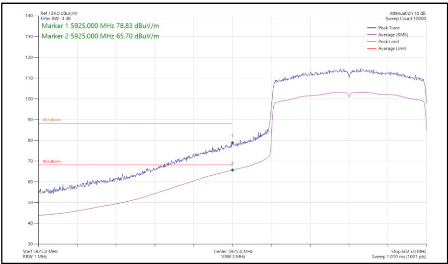
Figure 518 - 802.11ax HE80, SU, TxBF, Core 0-1 - 5985 MHz Band Edge Frequency 5925 MHz
