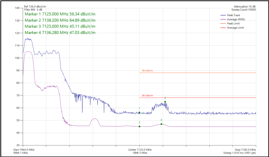
Figure 472 - 802.11ax HE40, RU 52-37, SDM, Core 0-1 - 7085 MHz Band Edge Frequency 7125 MHz
