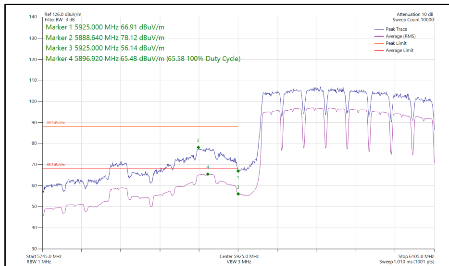
Figure 531 - 802.11a a160, SISO, Core 1 - 6025 MHz Band Edge Frequency 5925 MHz
