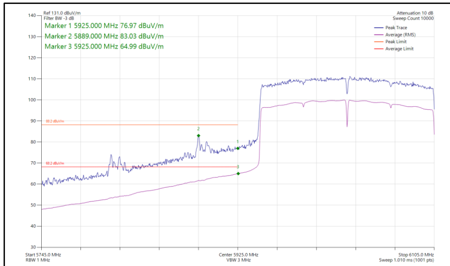
Figure 521 - 802.11ax HE160, SU, SISO, Core 0 - 6025 MHz Band Edge Frequency 5925 MHz
