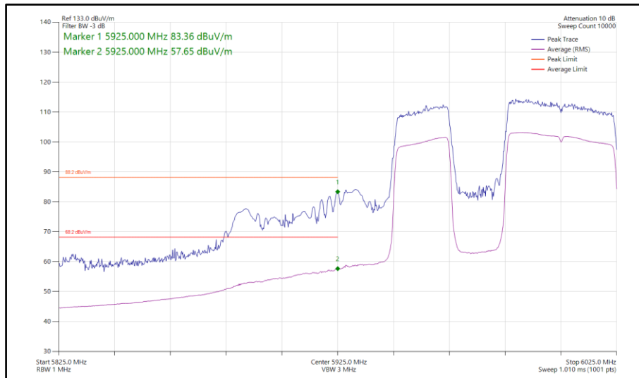
Figure 480 - 802.11be EHT80, RU 484+242-91, SISO, Core 0 - 5985 MHz Band Edge Frequency 5925 MHz
