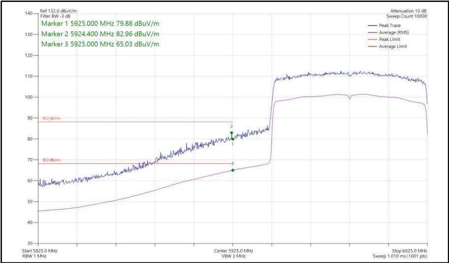
Figure 489 - 802.11ax HE80, SU, SISO, Core 1 - 5985 MHz Band Edge Frequency 5925 MHz
