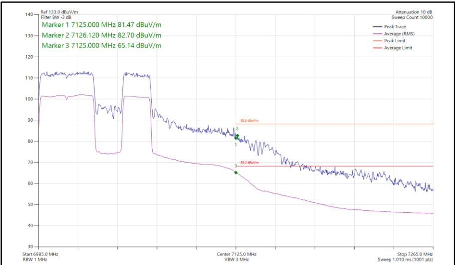
Figure 487 - 802.11be EHT80, RU 484+242-92, SISO, Core 0 - 7025 MHz Band Edge Frequency 7125 MHz
