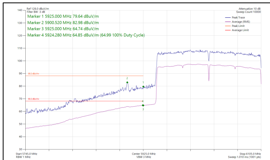
Figure 532 - 802.11ax HE160, SU, SISO, Core 1 - 6025 MHz Band Edge Frequency 5925 MHz
