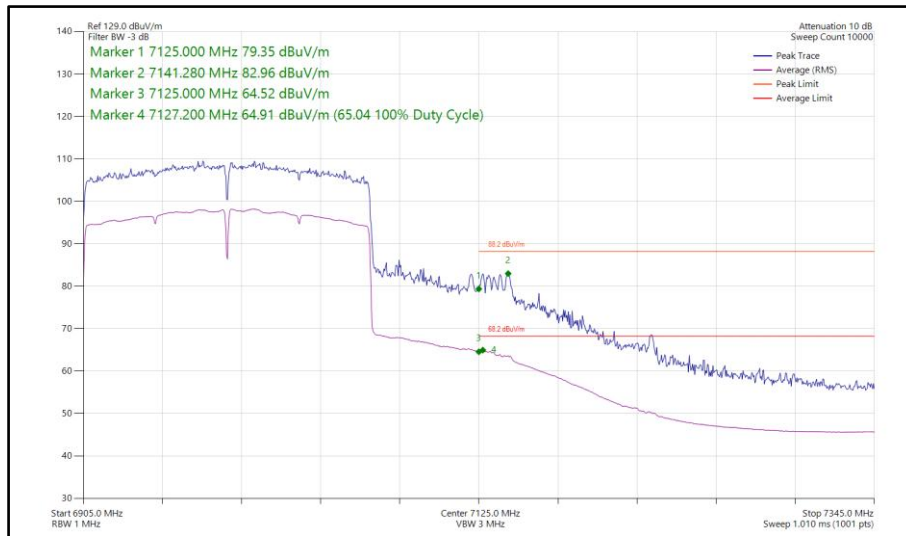
Figure 527 - 802.11ax HE160, SU, SISO, Core 0 - 6985 MHz Band Edge Frequency 7125 MHz
