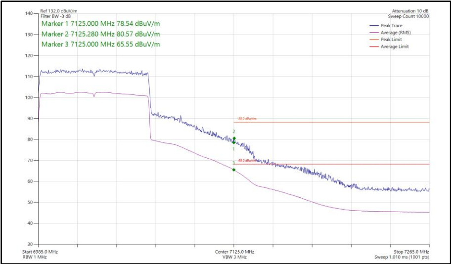
Figure 495 - 802.11ax HE80, SU, SISO, Core 1 - 7025 MHz Band Edge Frequency 7125 MHz
