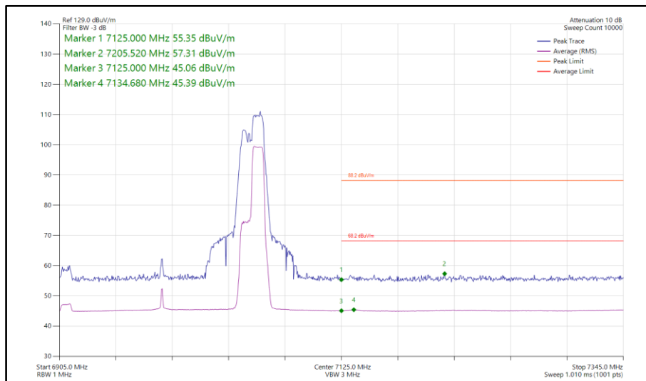
Figure 528 - 802.11ax HE160, RU 106-60S, SISO, Core 0 - 6985 MHz Band Edge Frequency 7125 MHz
