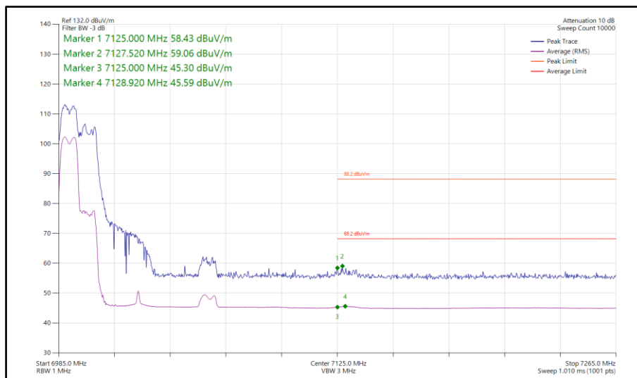
Figure 515 - 802.11ax HE80, RU 106-53, SDM, Core 0-1 - 7025 MHz Band Edge Frequency 7125 MHz
