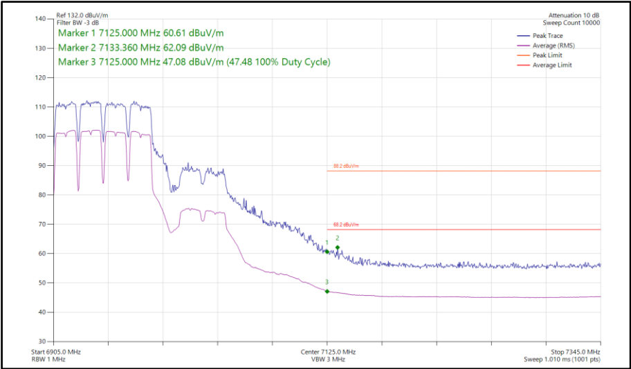
Figure 493 - 802.11a a80, SISO, Core 1 - 6945 MHz Band Edge Frequency 7125 MHz
