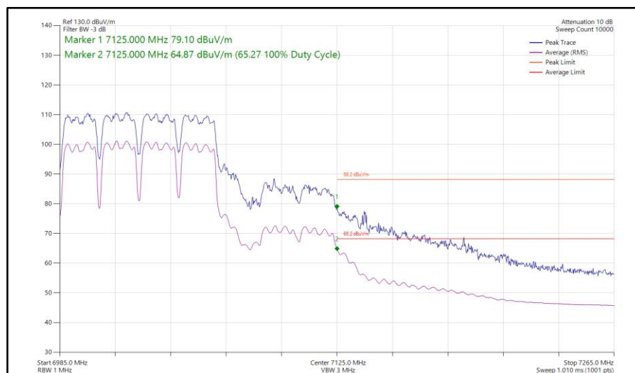
Figure 505 - 802.11a a80, CDD, Core 0-1 - 7025 MHz Band Edge Frequency 7125 MHz
