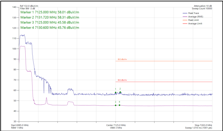
Figure 485 - 802.11ax HE80, RU 106-53, SISO, Core 0 - 7025 MHz Band Edge Frequency 7125 MHz
