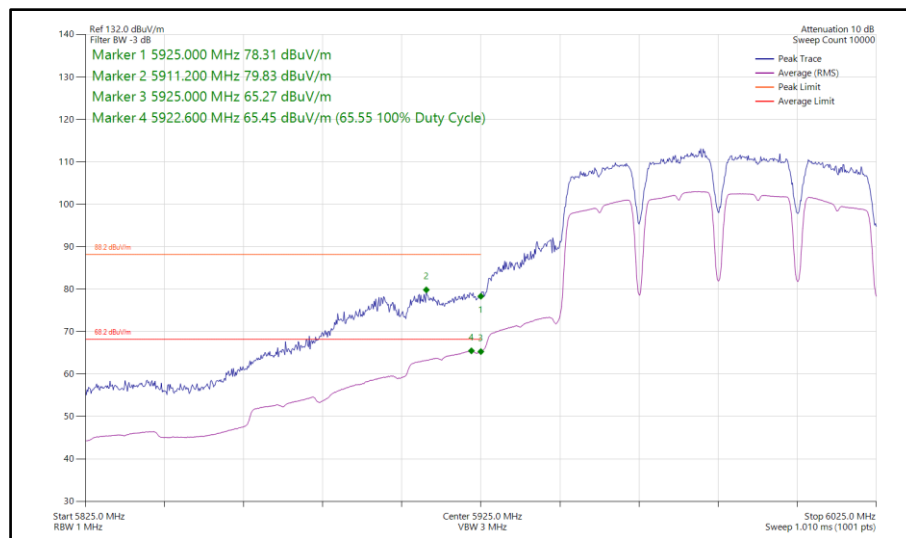
Figure 477 - 802.11a a80, SISO, Core 0 - 5985 MHz Band Edge Frequency 5925 MHz
