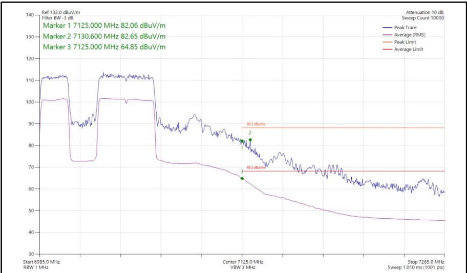
Figure 498 - 802.11be EHT80, RU 484+242-91, SISO, Core 1 - 7025 MHz Band Edge Frequency 7125 MHz
