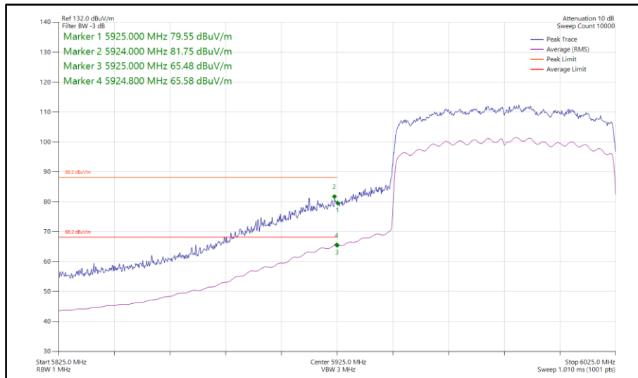
Figure 500 - 802.11ax HE80, SU, CDD, Core 0-1 - 5985 MHz Band Edge Frequency 5925 MHz
