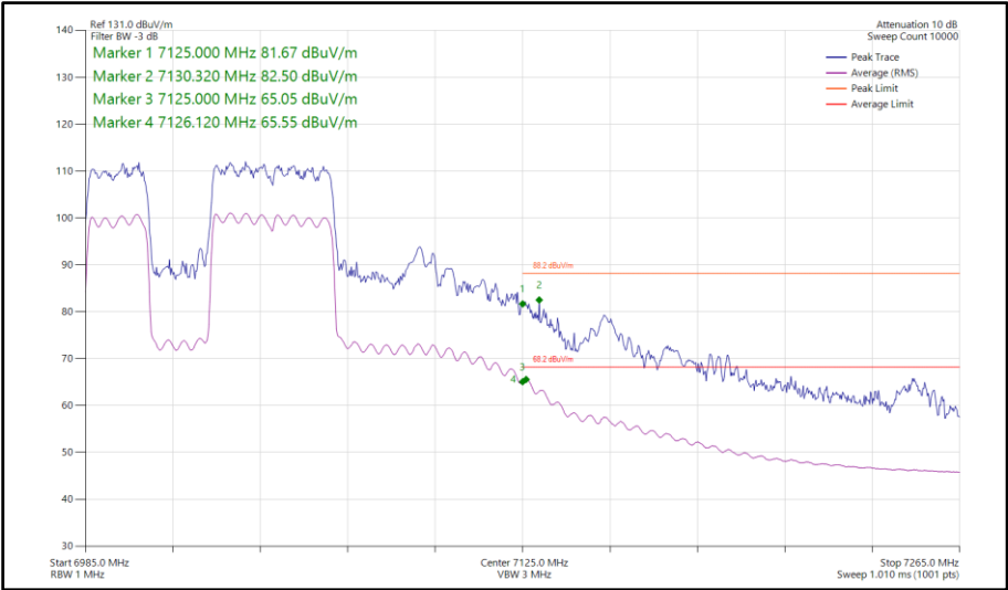
Figure 517 - 802.11be EHT80, RU 484+242-91, SDM, Core 0-1 - 7025 MHz Band Edge Frequency 7125 MHz
