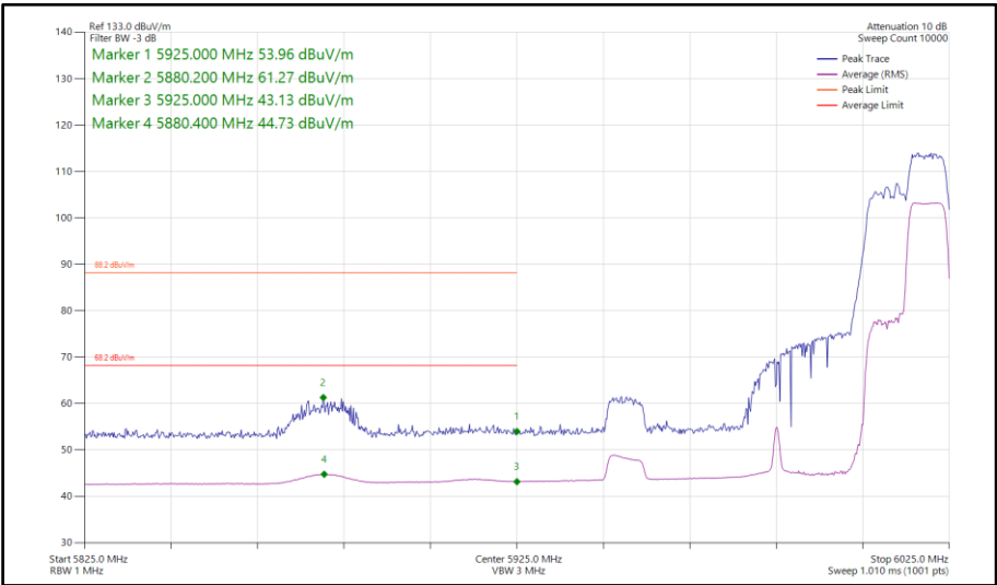
Figure 479 - 802.11ax HE80, RU 106-60, SISO, Core 0 - 5985 MHz Band Edge Frequency 5925 MHz
