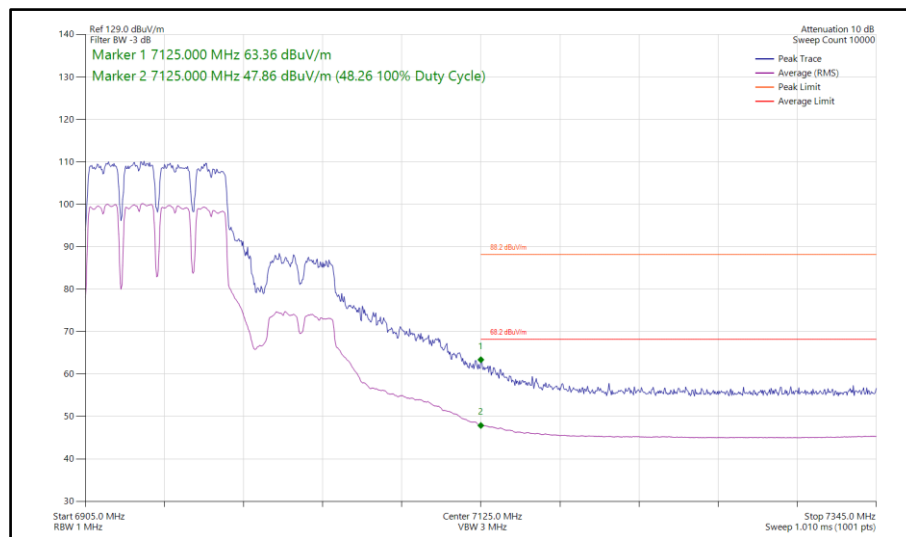
Figure 504 - 802.11a a80, CDD, Core 0-1 - 6945 MHz Band Edge Frequency 7125 MHz
