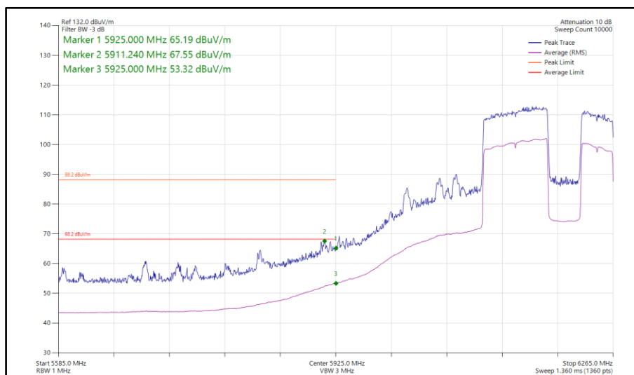
Figure 524 - 802.11be EHT160, RU 996+484-94, SISO, Core 0 - 6185 MHz Band Edge Frequency 5925 MHz
