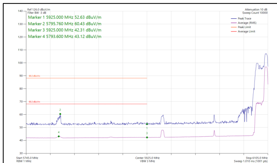
Figure 533 - 802.11ax HE160, RU 52-52S, SISO, Core 1 - 6025 MHz Band Edge Frequency 5925 MHz
