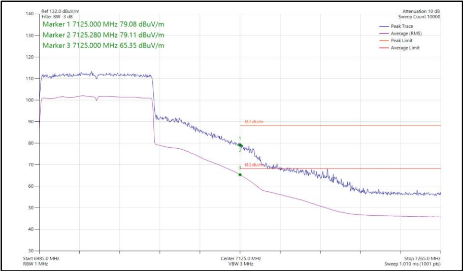
Figure 484 - 802.11ax HE80, SU, SISO, Core 0 - 7025 MHz Band Edge Frequency 7125 MHz
