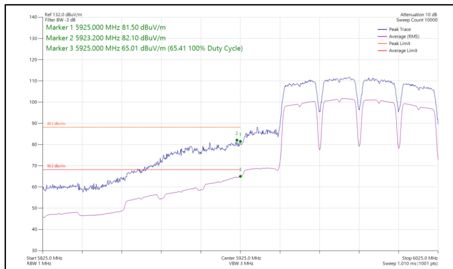
Figure 488 - 802.11a a80, SISO, Core 1 - 5985 MHz Band Edge Frequency 5925 MHz
