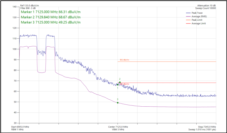
Figure 497 - 802.11be EHT80, RU 484+242-92, SISO, Core 1 - 6945 MHz Band Edge Frequency 7125 MHz
