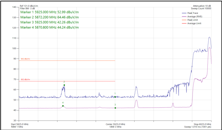
Figure 490 - 802.11ax HE80, RU 26-36, SISO, Core 1 - 5985 MHz Band Edge Frequency 5925 MHz
