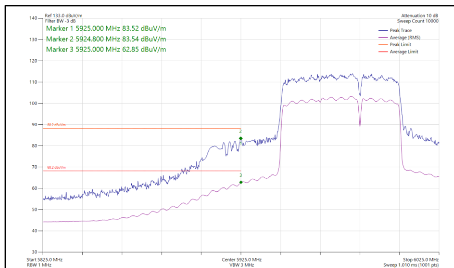
Figure 512 - 802.11be EHT80, RU 484+242-93, SDM, Core 0-1 - 5985 MHz Band Edge Frequency 5925 MHz
