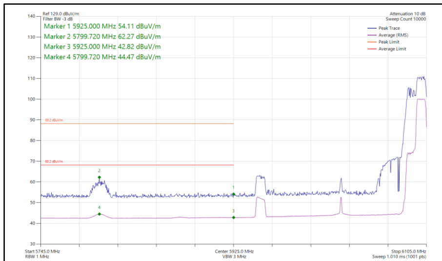
Figure 522 - 802.11ax HE160, RU 106-60S, SISO, Core 0 - 6025 MHz Band Edge Frequency 5925 MHz
