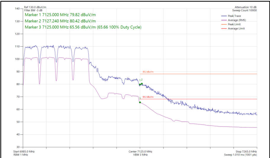
Figure 494 - 802.11a a80, SISO, Core 1 - 7025 MHz Band Edge Frequency 7125 MHz
