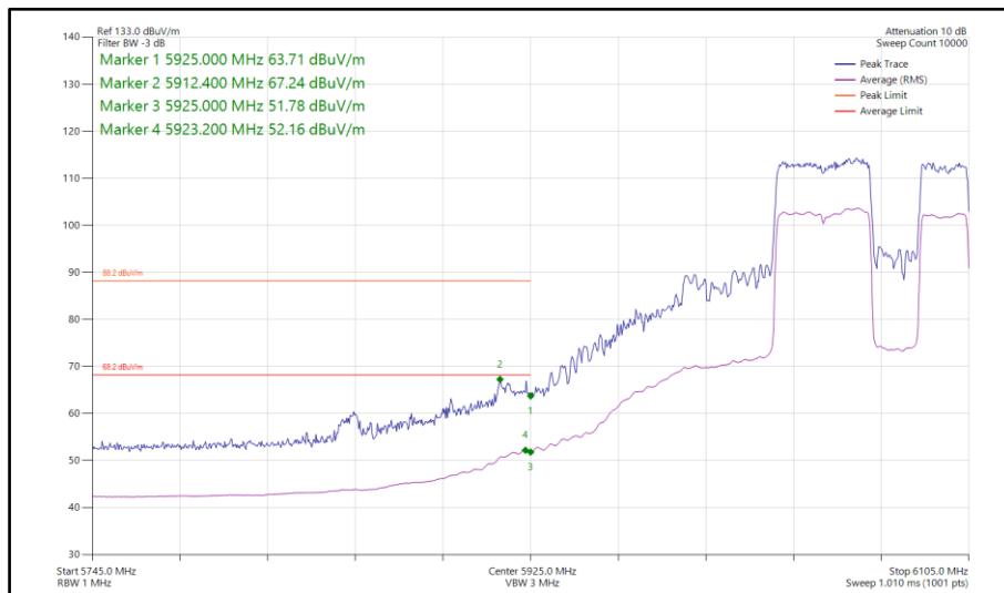
Figure 503 - 802.11be EHT80, RU 484+242-92, CDD, Core 0-1 - 6065 MHz Band Edge Frequency 5925 MHz
