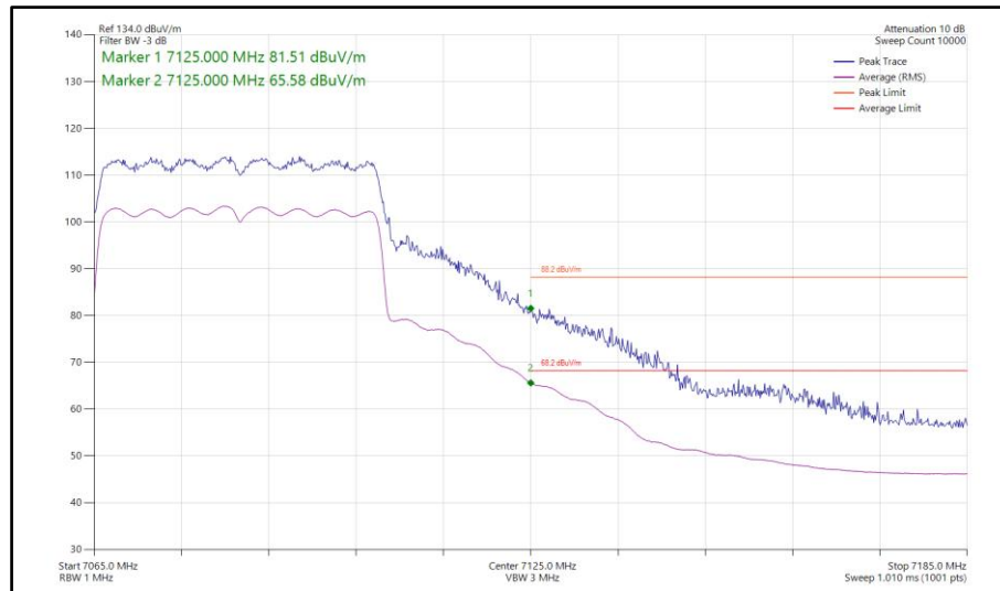
Figure 464 - 802.11ax HE40, SU, CDD, Core 0-1 - 7085 MHz Band Edge Frequency 7125 MHz
