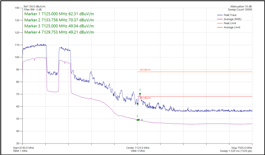
Figure 529 - 802.11be EHT160, RU 996+484-94, SISO, Core 0 - 6825 MHz Band Edge Frequency 7125 MHz
