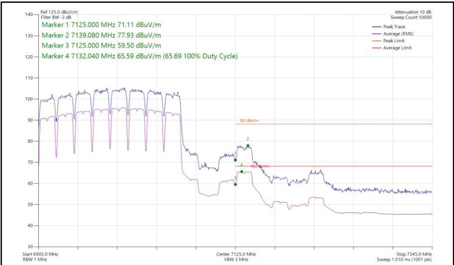
Figure 526 - 802.11a a160, SISO, Core 0 - 6985 MHz Band Edge Frequency 7125 MHz
