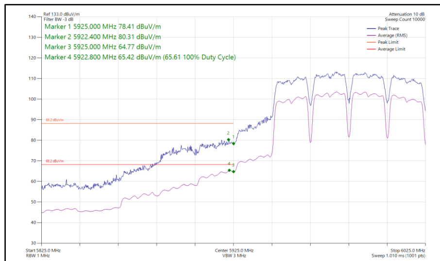
Figure 499 - 802.11a a80, CDD, Core 0-1 - 5985 MHz Band Edge Frequency 5925 MHz
