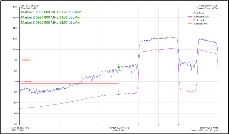
Figure 491 - 802.11be EHT80, RU 484+242-92, SISO, Core 1 - 5985 MHz Band Edge Frequency 5925 MHz
