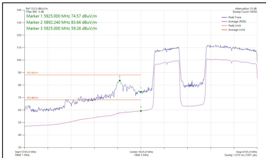
Figure 523 - 802.11be EHT160, RU 996+484-95, SISO, Core 0 - 6025 MHz Band Edge Frequency 5925 MHz
