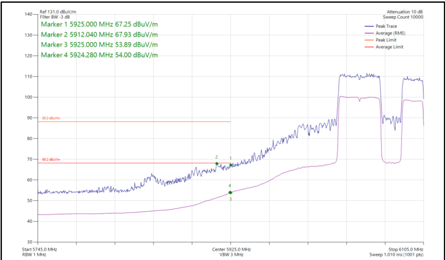
Figure 492 - 802.11be EHT80, RU 484+242,92, SISO, Core 1 - 6065 MHz Band Edge Frequency 5925 MHz
