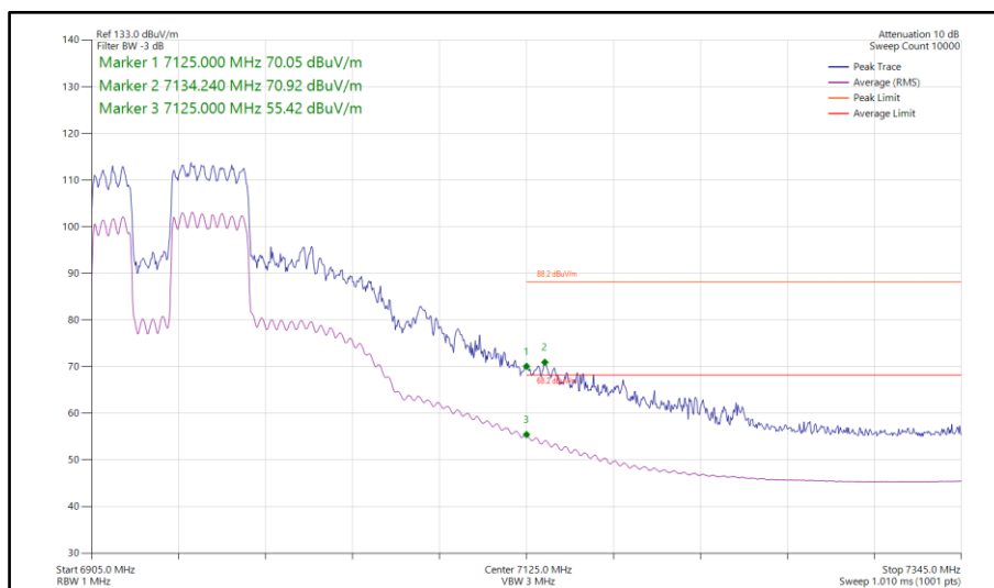
Figure 516 - 802.11be EHT80, RU 484+242-91, SDM, Core 0-1 - 6945 MHz Band Edge Frequency 7125 MHz
