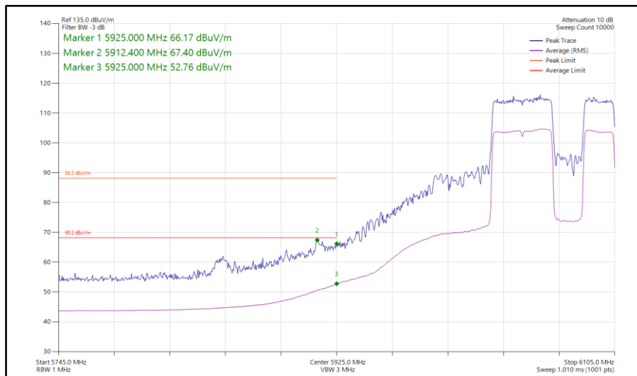
Figure 481 - 802.11be EHT80, RU 484+242-92, SISO, Core 0 - 6065 MHz Band Edge Frequency 5925 MHz
