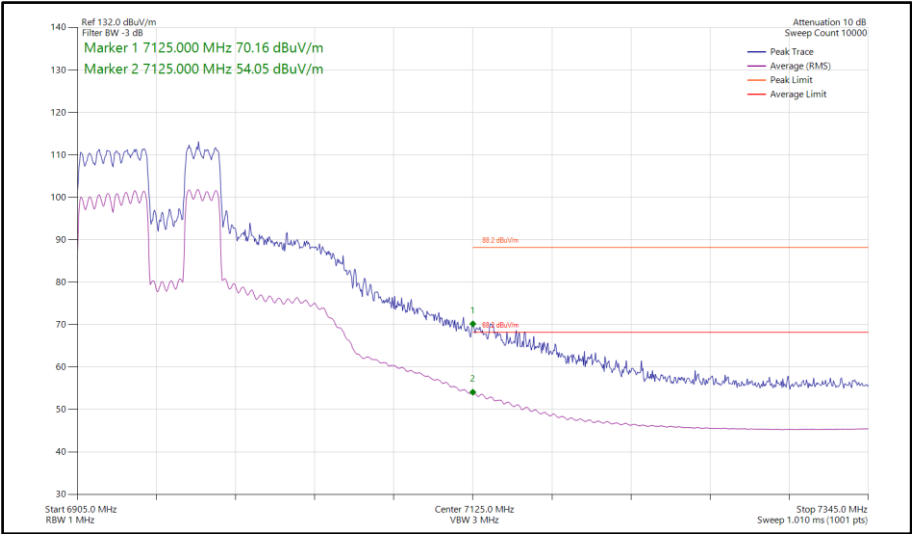
Figure 508 - 802.11be EHT80, RU 484+242-92, CDD, Core 0-1 - 6945 MHz Band Edge Frequency 7125 MHz
