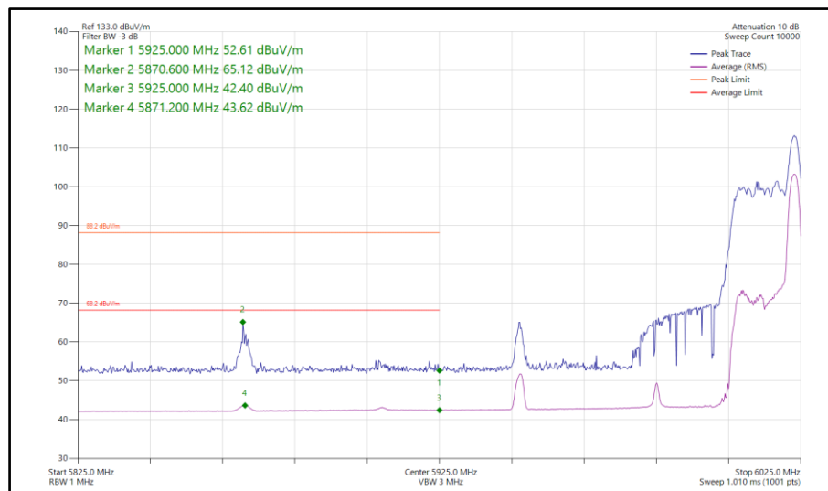
Figure 511 - 802.11ax HE80, RU 26-36, SDM, Core 0-1 - 5985 MHz Band Edge Frequency 5925 MHz
