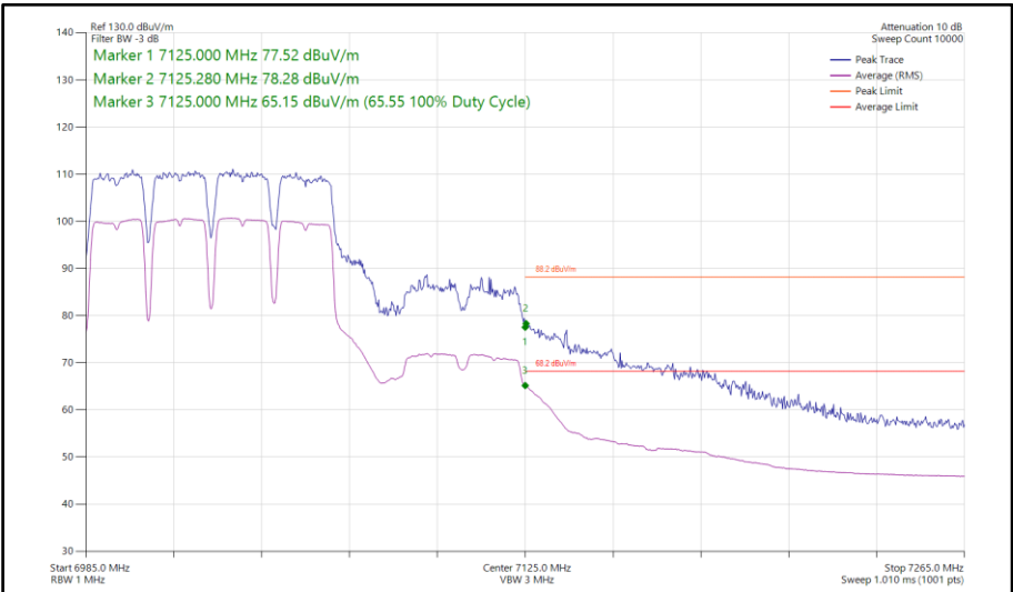
Figure 483 - 802.11a a80, SISO, Core 0 - 7025 MHz Band Edge Frequency 7125 MHz
