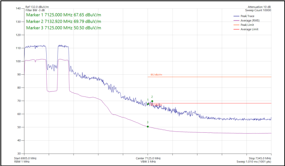
Figure 486 - 802.11be EHT80, RU 484+242-92, SISO, Core 0 - 6945 MHz Band Edge Frequency 7125 MHz
