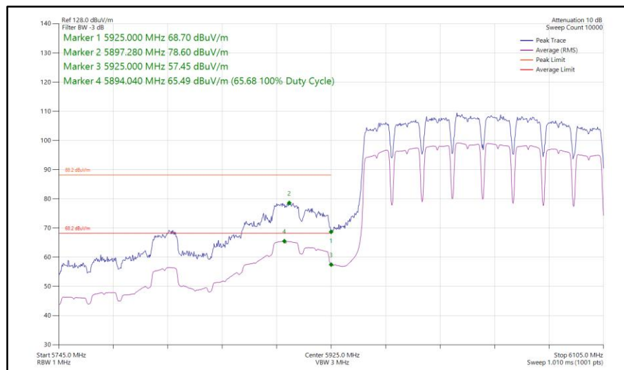
Figure 520 - 802.11a a160, SISO, Core 0 - 6025 MHz Band Edge Frequency 5925 MHz
