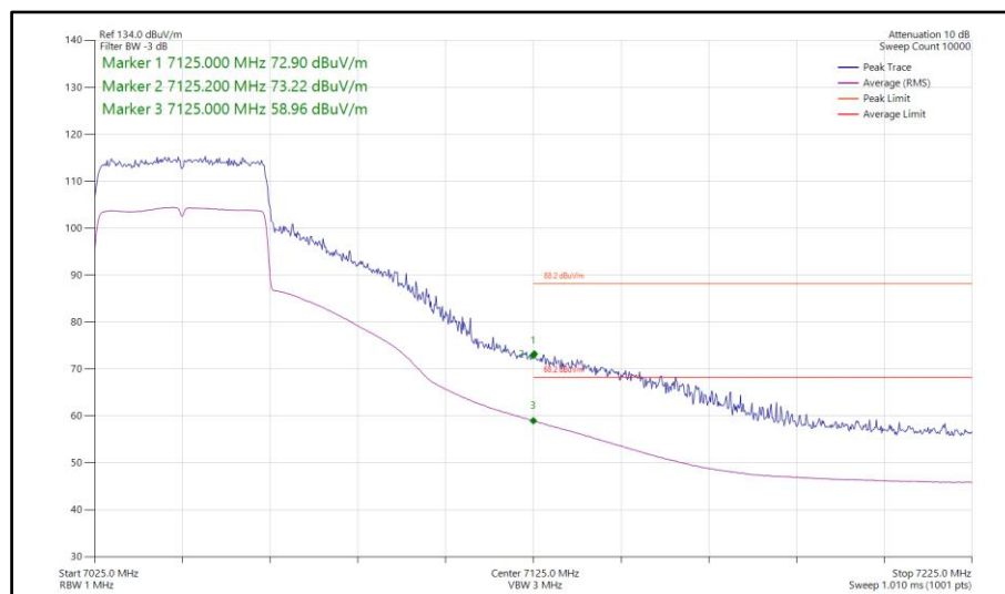
Figure 475 - 802.11ax HE40, SU, TxBF, Core 0-1 - 7045 MHz Band Edge Frequency 7125 MHz
