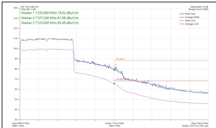
Figure 514 - 802.11ax HE80, SU, SDM, Core 0-1 - 7025 MHz Band Edge Frequency 7125 MHz
