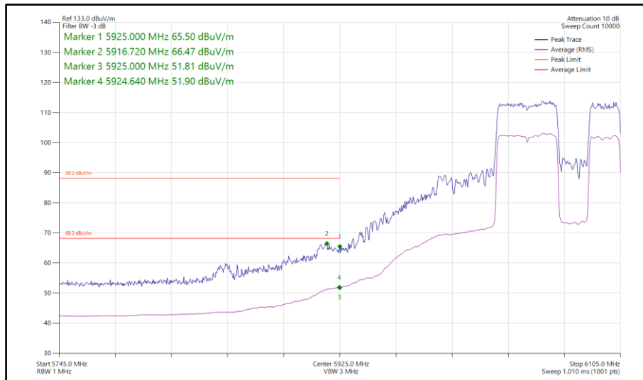
Figure 513 - 802.11be EHT80, RU 484+242-92, SDM, Core 0-1 - 6065 MHz Band Edge Frequency 5925 MHz
