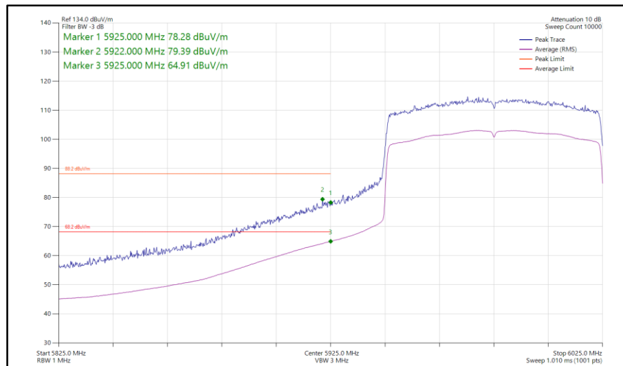
Figure 510 - 802.11ax HE80, SU, SDM, Core 0-1 - 5985 MHz Band Edge Frequency 5925 MHz
