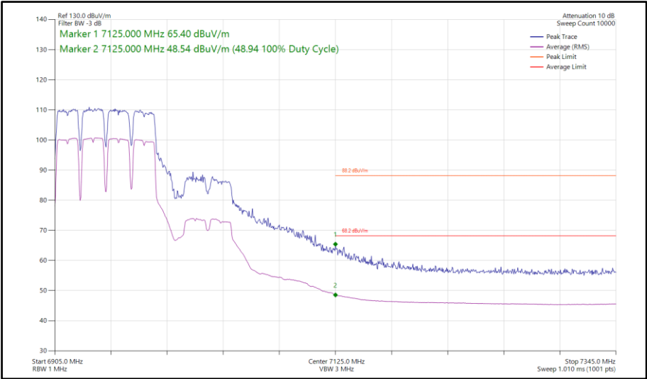
Figure 482 - 802.11a a80, SISO, Core 0 - 6945 MHz Band Edge Frequency 7125 MHz
