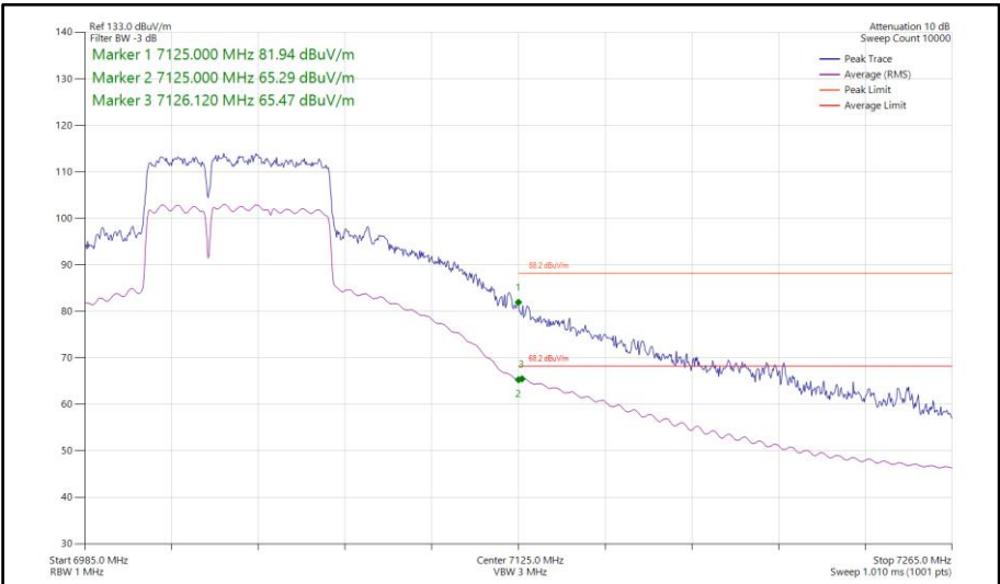
Figure 509 - 802.11be EHT80, RU 484+242-90, CDD, Core 0-1 - 7025 MHz Band Edge Frequency 7125 MHz
