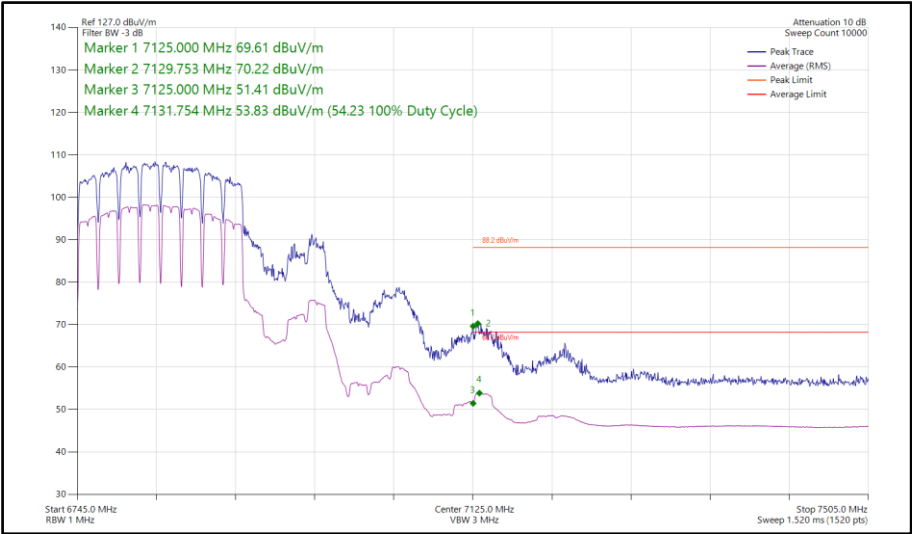
Figure 525 - 802.11a a160, SISO, Core 0 - 6825 MHz Band Edge Frequency 7125 MHz
