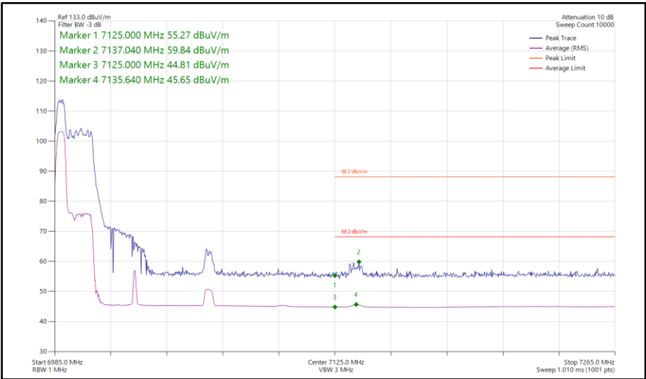
Figure 496 - 802.11ax HE80, RU 52-37, SISO, Core 1 - 7025 MHz Band Edge Frequency 7125 MHz
