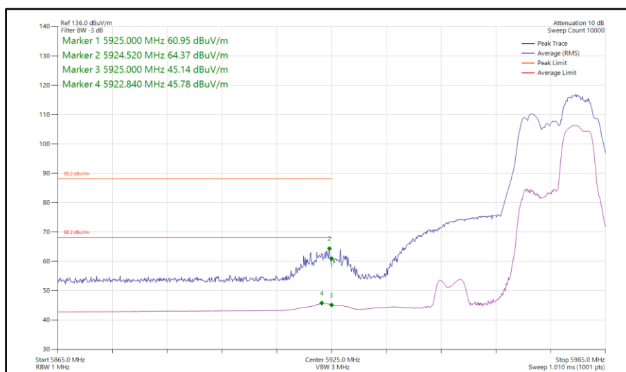
Figure 469 - 802.11be EHT40, RU 52+26-75, SDM, Core 0-1 - 5965 MHz Band Edge Frequency 5925 MHz
