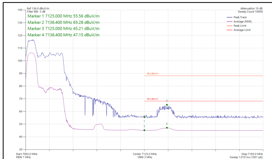
Figure 465 - 802.11ax HE40, RU 52-37, CDD, Core 0-1 - 7085 MHz Band Edge Frequency 7125 MHz
