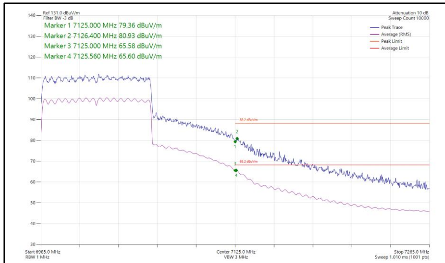
Figure 506 - 802.11ax HE80, SU, CDD, Core 0-1 - 7025 MHz Band Edge Frequency 7125 MHz
