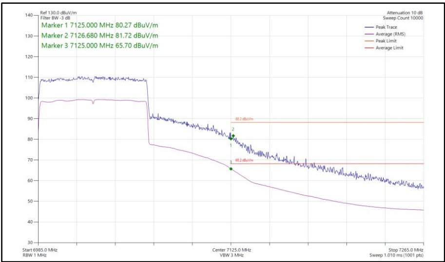
Figure 519 - 802.11ax HE80, SU, TxBF, Core 0-1 - 7025 MHz Band Edge Frequency 7125 MHz
