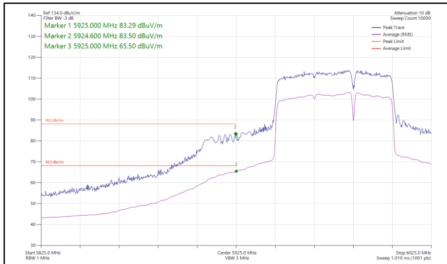
Figure 502 - 802.11be EHT80, RU 484+242-93, CDD, Core 0-1 - 5985 MHz Band Edge Frequency 5925 MHz
