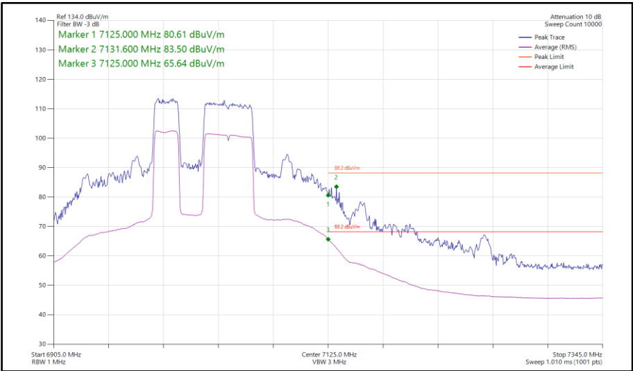
Figure 530 - 802.11be EHT160, RU 484+242-91, SISO, Core 0 - 6985 MHz Band Edge Frequency 7125 MHz
