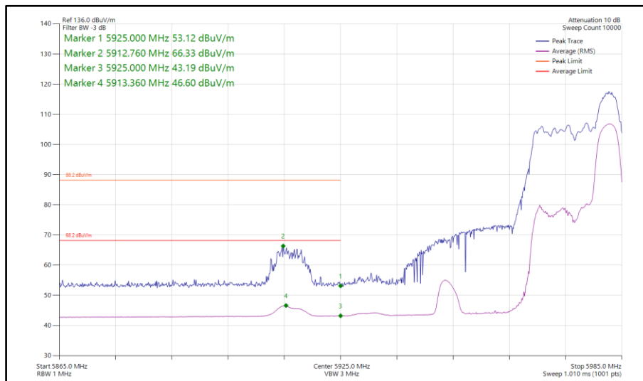
Figure 468 - 802.11ax HE40, RU 52-44, SDM, Core 0-1 - 5965 MHz Band Edge Frequency 5925 MHz
