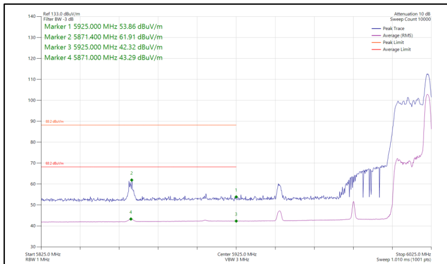
Figure 501 - 802.11ax HE80, RU 26-36, CDD, Core 0-1 - 5985 MHz Band Edge Frequency 5925 MHz
