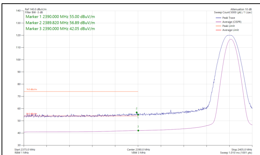
Figure 13 - Bluetooth DH5, MIMO, Core 0-1 - 2402 MHz Band Edge Frequency 2390 MHz
