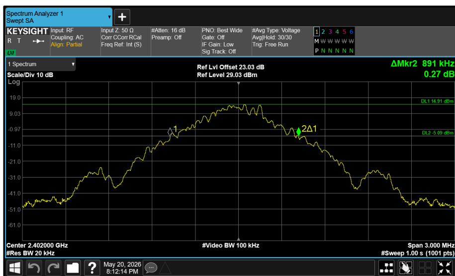
Figure 62 - Core 0 (A) 2402 MHz (CH0) 20 dB Bandwidth
