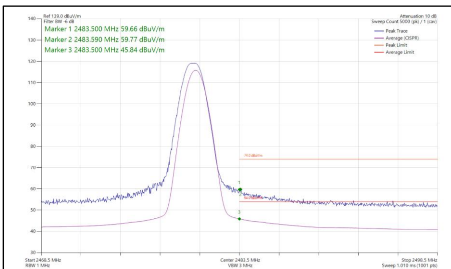
Figure 10 - Bluetooth DH5, SISO, Core 0 - 2480 MHz Band Edge Frequency 2483.5 MHz
