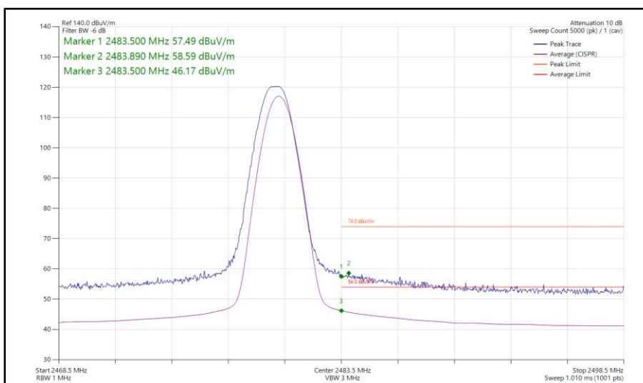
Figure 14 - Bluetooth DH5, MIMO, Core 0-1 - 2480 MHz Band Edge Frequency 2483.5 MHz
