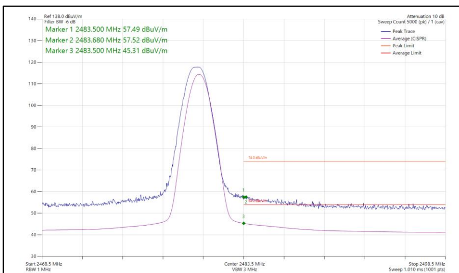
Figure 12 - Bluetooth DH5, SISO, Core 1 - 2480 MHz Band Edge Frequency 2483.5 MHz
