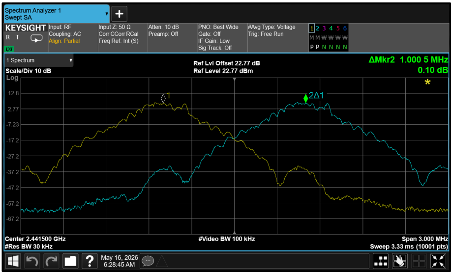
Figure 30 - GFSK - 2441 MHz (CH39)
