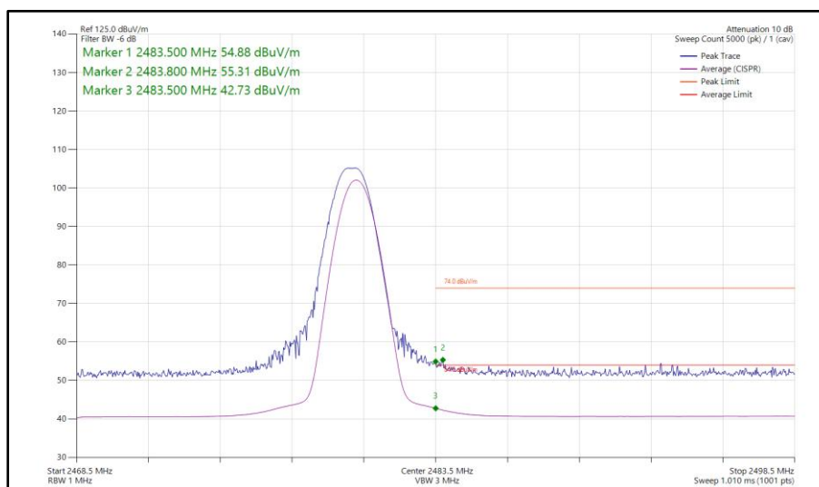
Figure 4 - Bluetooth DH5, SISO, Core 1 - 2480 MHz Band Edge Frequency 2483.5 MHz
