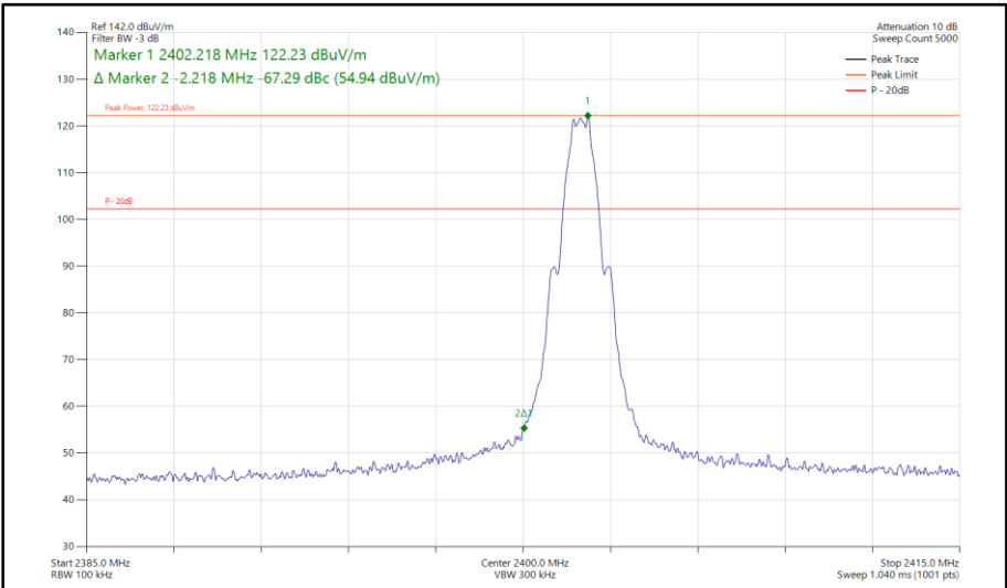
Figure 527 - Bluetooth LE1M, MIMO, Core 0-1 - 2402 MHz Band Edge Frequency 2400 MHz
