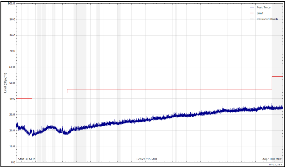
Figure 548 - 2440 MHz, LE1M, iPA, Core 2, 30 MHz to 1 GHz, Vertical (Peak)
