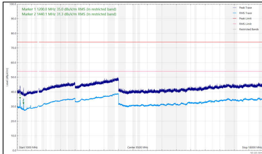
Figure 543 - 2480 MHz, LE1M, iPA, Core 0 + Core 1, 1 GHz to 18 GHz, Vertical
