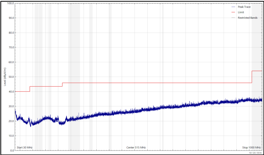
Figure 540 - 2440 MHz, LE1M, iPA, Core 0 + Core 1, 30 MHz to 1 GHz, Vertical (Peak)
