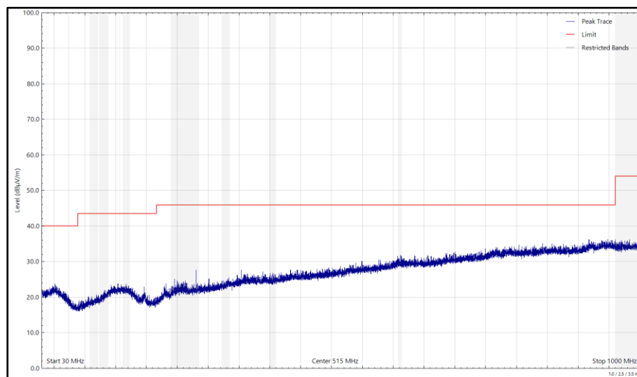
Figure 568 - 2440 MHz, HDR8, ePA, Core 0 + Core 1, 30 MHz to 1 GHz, Horizontal (Peak)
