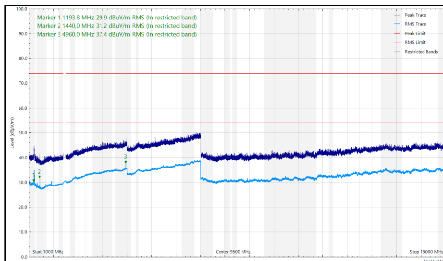
Figure 551 - 2480 MHz, LE1M, iPA, Core 2, 1 GHz to 18 GHz, Vertical
