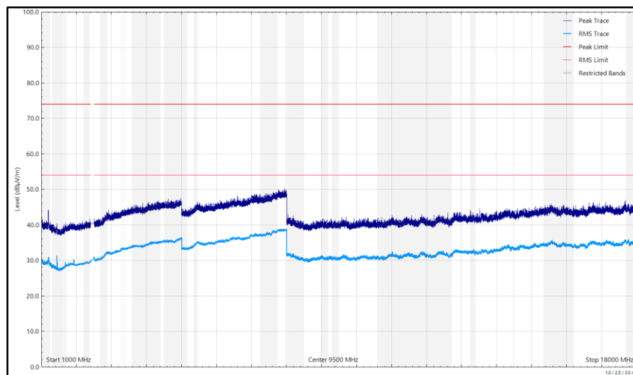
Figure 550 - 2480 MHz, LE1M, iPA, Core 2, 1 GHz to 18 GHz, Horizontal
