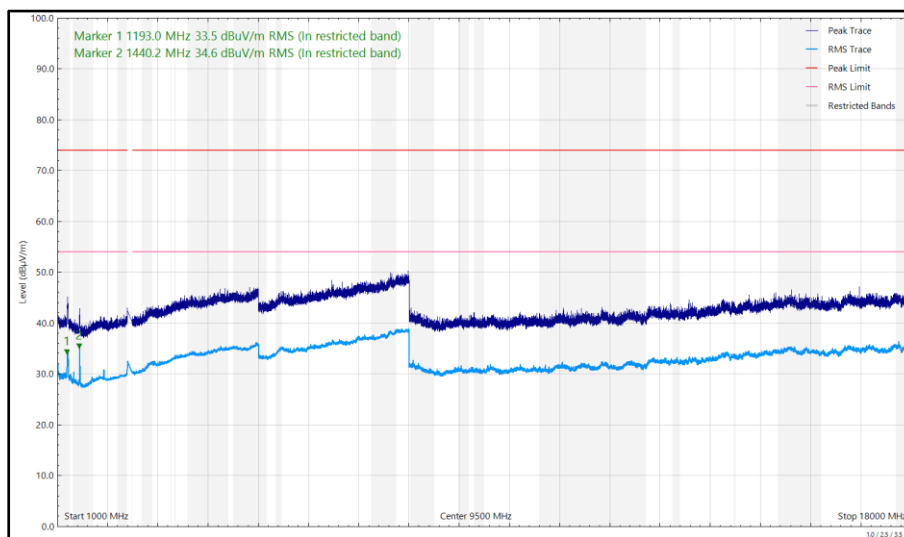
Figure 545 - 2402 MHz, LE1M, iPA, Core 2, 1 GHz to 18 GHz, Vertical
