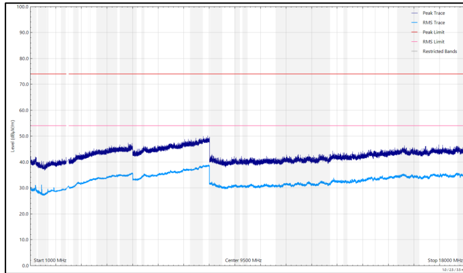
Figure 542 - 2480 MHz, LE1M, iPA, Core 0 + Core 1, 1 GHz to 18 GHz, Horizontal
