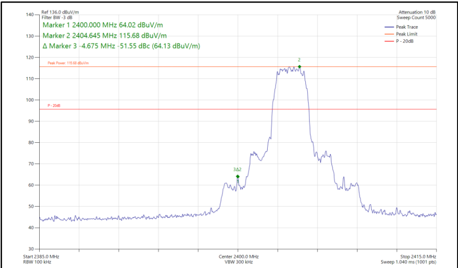
Figure 505 - Bluetooth HDT3, SISO, Core 0 - 2404 MHz Band Edge Frequency 2400 MHz
