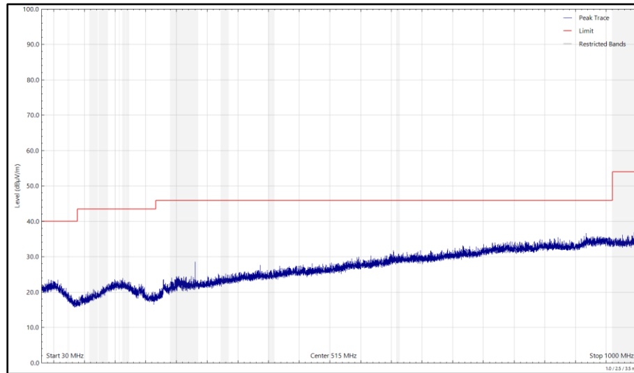
Figure 576 - 2440 MHz, HDT4, iPA, Core 2, 30 MHz to 1 GHz, Horizontal (Peak)
