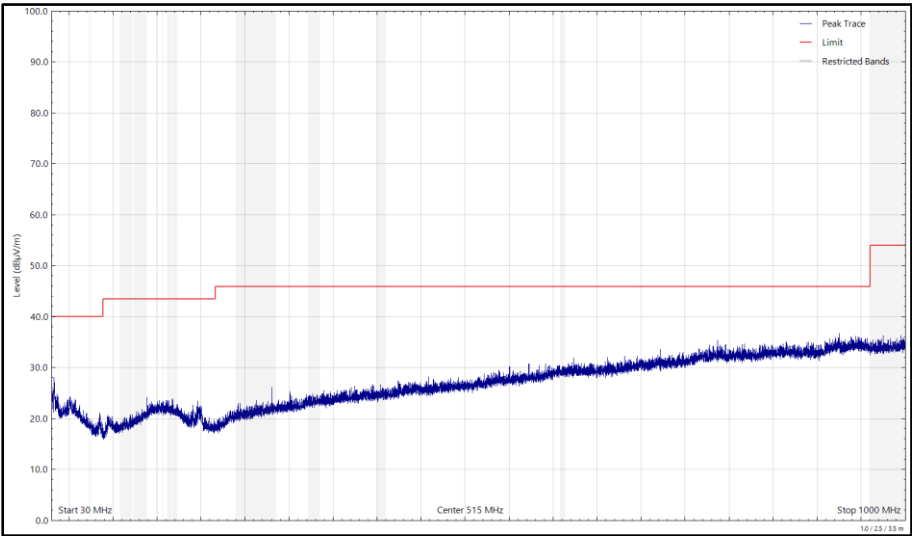
Figure 570 - 2440 MHz, HDR8, ePA, Core 0 + Core 1, 30 MHz to 1 GHz, Vertical (Peak)
