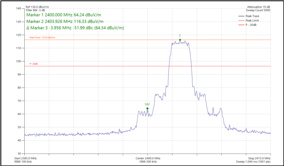
Figure 506 - Bluetooth HDT4, SISO, Core 0 - 2404 MHz Band Edge Frequency 2400 MHz
