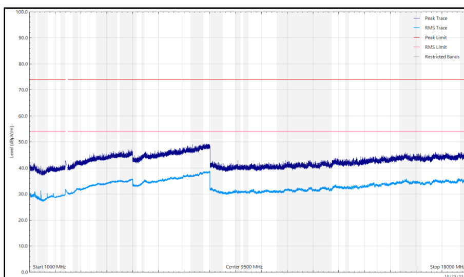
Figure 536 - 2402 MHz, LE1M, iPA, Core 0 + Core 1, 1 GHz to 18 GHz, Horizontal
