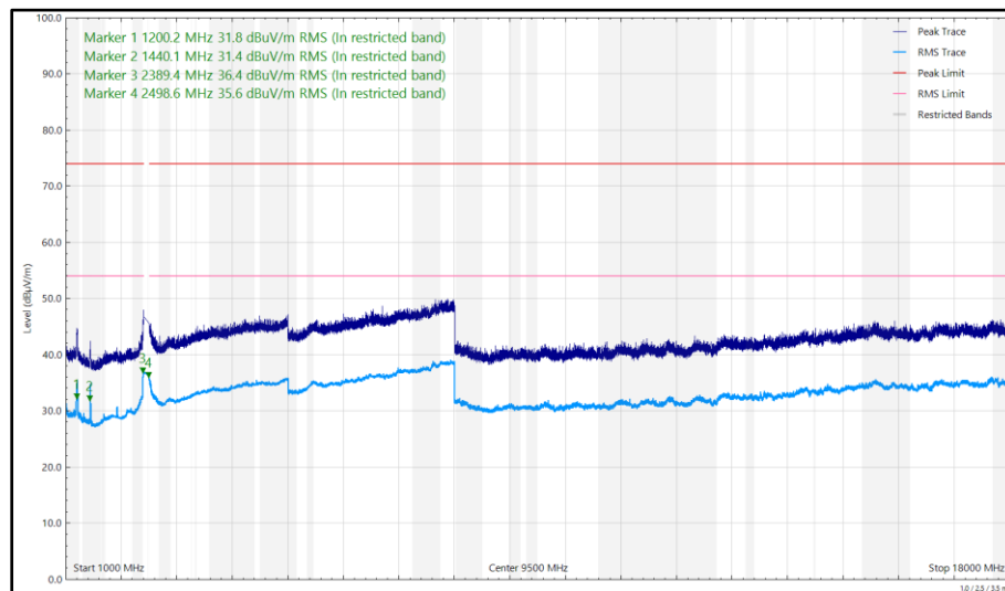
Figure 559 - 2480 MHz, LE1M, ePA, Core 0 + Core 1, 1 GHz to 18 GHz, Vertical
