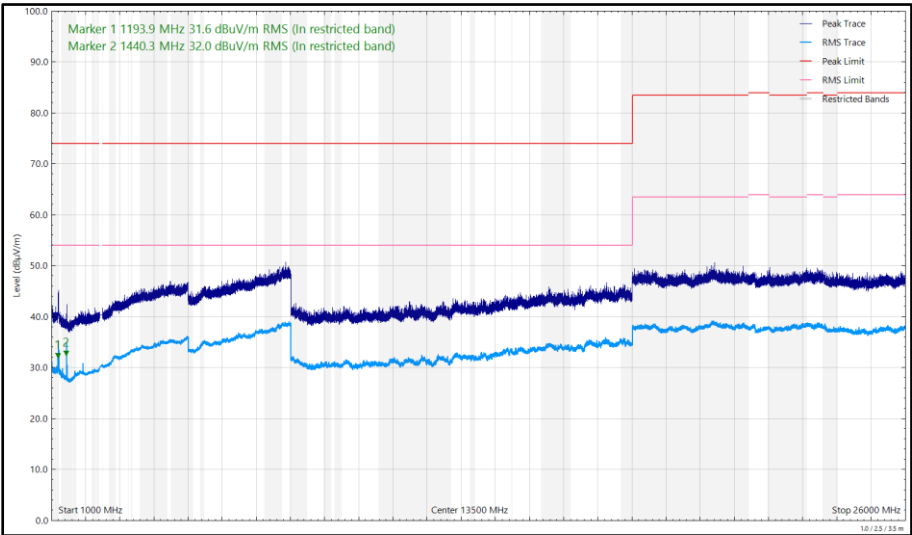
Figure 575 - 2440 MHz, HDT4, iPA, Core 0 + Core 1, 1 GHz to 26 GHz, Vertical
