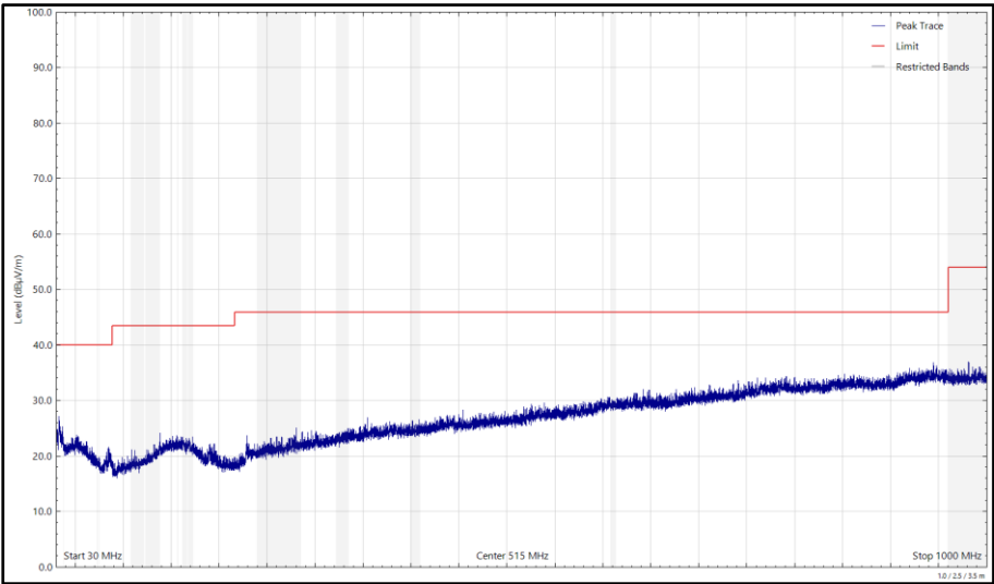
Figure 574 - 2440 MHz, HDT4, iPA, Core 0 + Core 1, 30 MHz to 1 GHz, Vertical (Peak)
