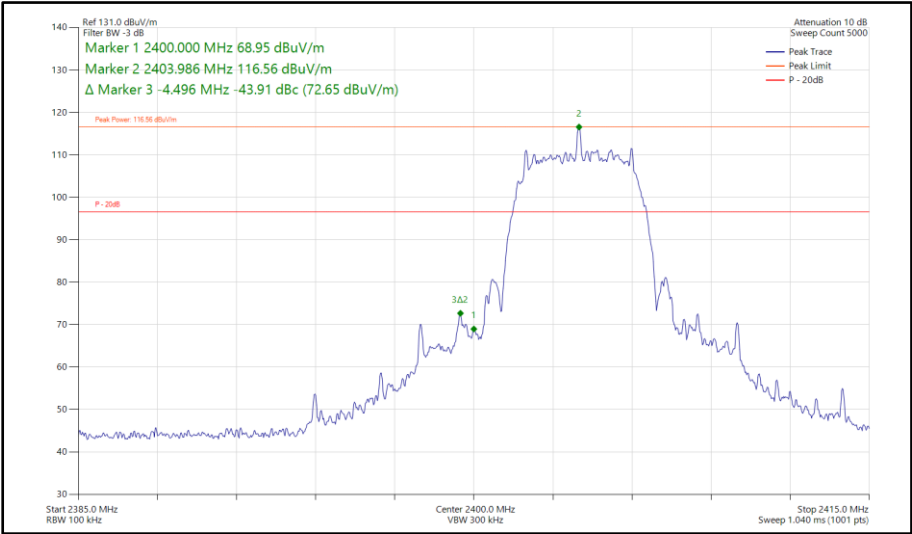
Figure 510 - Bluetooth XHDRPM8, SISO, Core 0 - 2404 MHz Band Edge Frequency 2400 MHz
