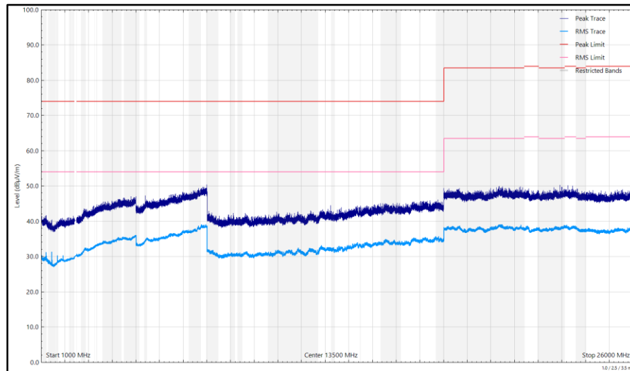
Figure 577 - 2440 MHz, HDT4, iPA, Core 2, 1 GHz to 26 GHz, Horizontal
