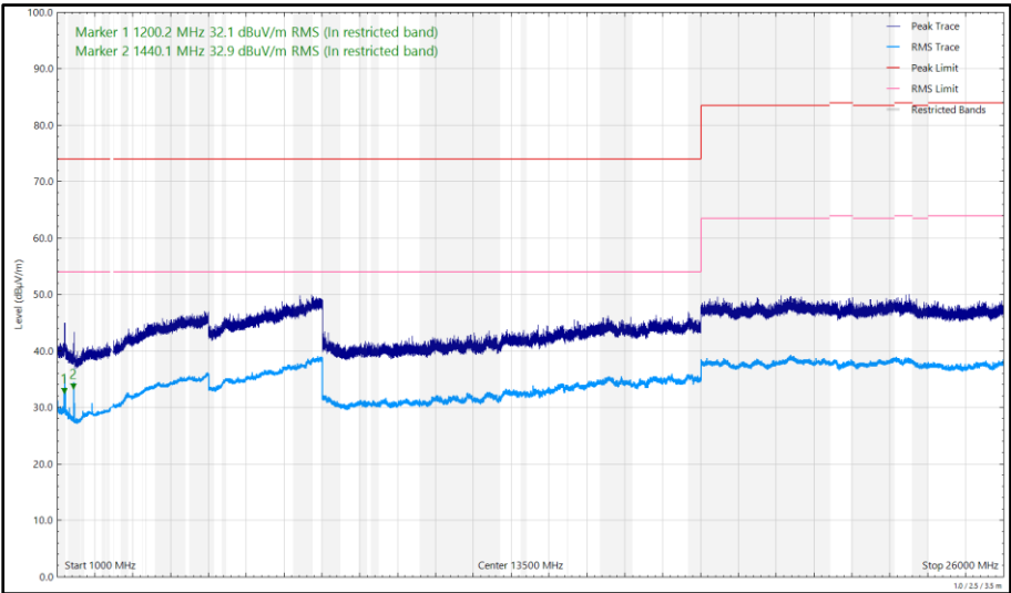
Figure 541 - 2440 MHz, LE1M, iPA, Core 0 + Core 1, 1 GHz to 26 GHz, Vertical
