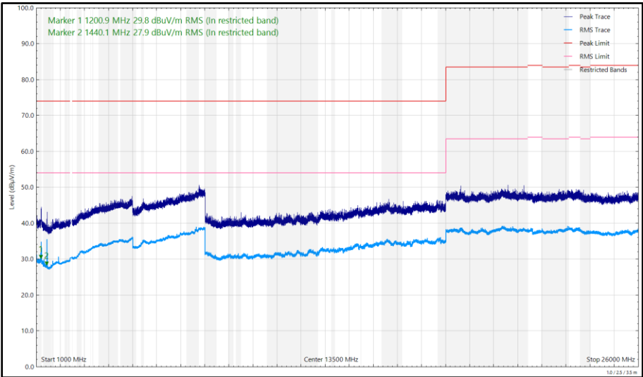
Figure 549 - 2440 MHz, LE1M, iPA, Core 2, 1 GHz to 26 GHz, Vertical
