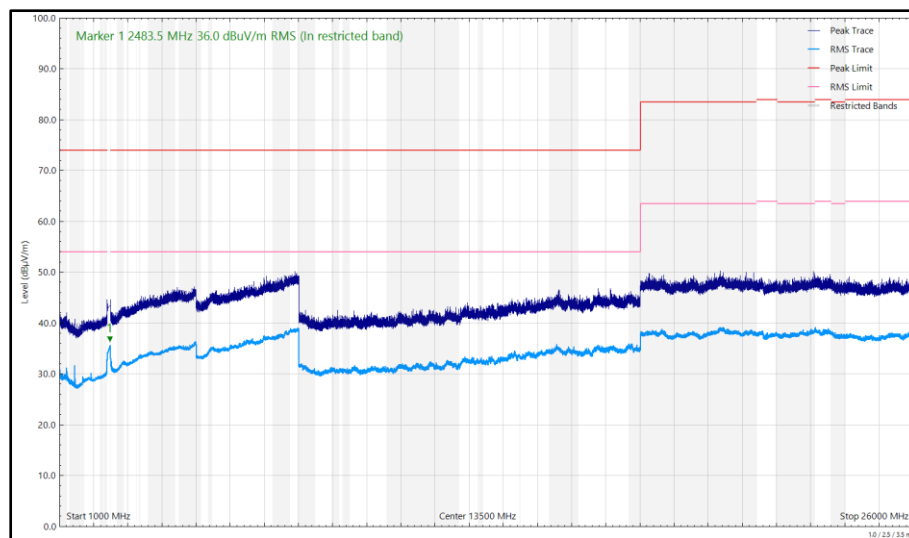
Figure 555 - 2440 MHz, LE1M, ePA, Core 0 + Core 1, 1 GHz to 26 GHz, Horizontal
