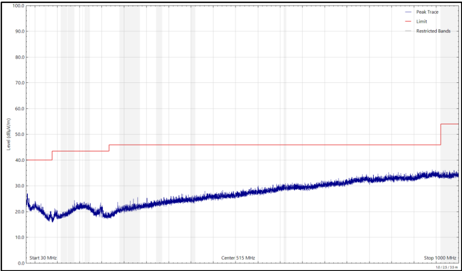
Figure 562 - 2440 MHz, HDR8, iPA, Core 0 + Core 1, 30 MHz to 1 GHz, Vertical (Peak)
