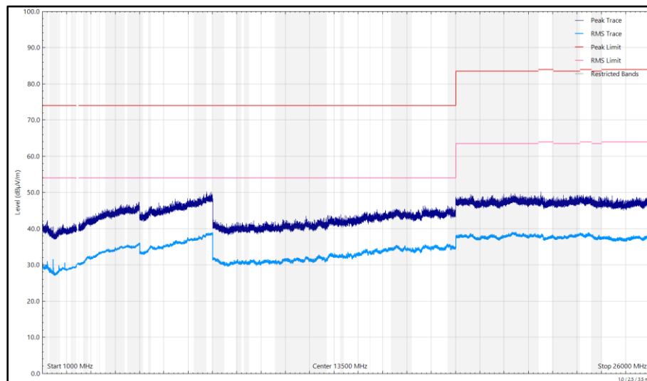
Figure 547 - 2440 MHz, LE1M, iPA, Core 2, 1 GHz to 26 GHz, Horizontal
