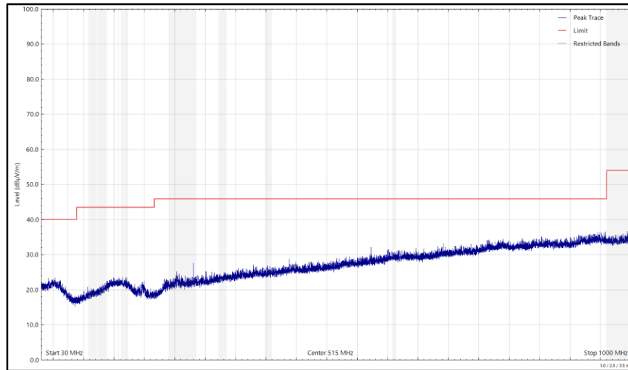
Figure 564 - 2440 MHz, HDR8, iPA, Core 2, 30 MHz to 1 GHz, Horizontal (Peak)
