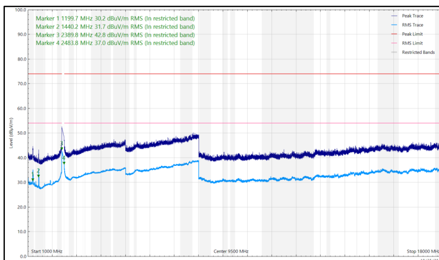
Figure 553 - 2402 MHz, LE1M, ePA, Core 0 + Core 1, 1 GHz to 18 GHz, Vertical
