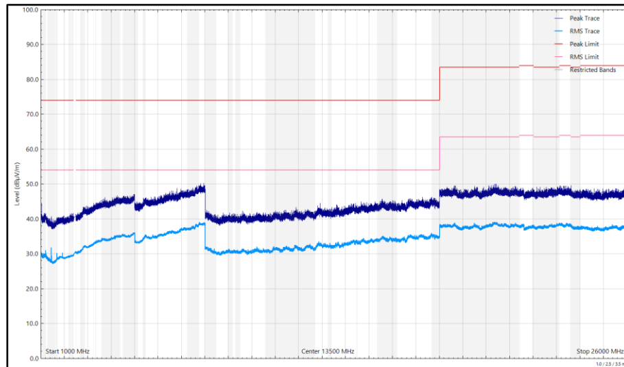
Figure 565 - 2440 MHz, HDR8, iPA, Core 2, 1 GHz to 26 GHz, Horizontal
