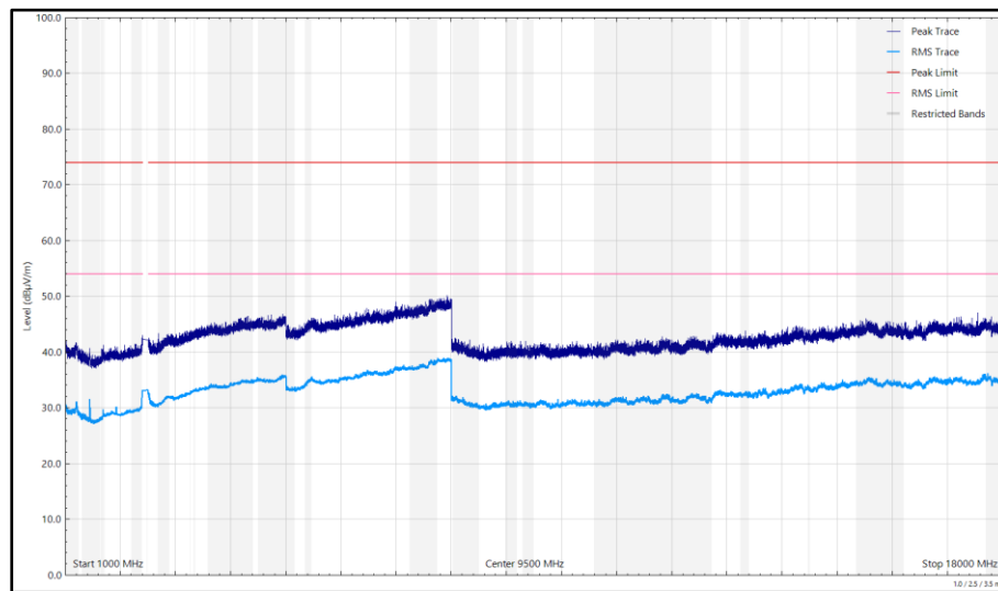
Figure 558 - 2480 MHz, LE1M, ePA, Core 0 + Core 1, 1 GHz to 18 GHz, Horizontal
