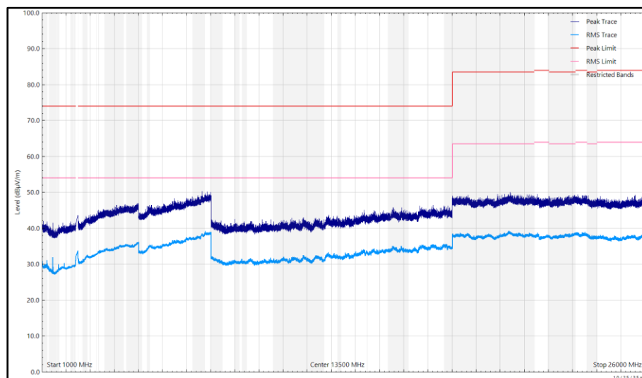
Figure 569 - 2440 MHz, HDR8, ePA, Core 0 + Core 1, 1 GHz to 26 GHz, Horizontal
