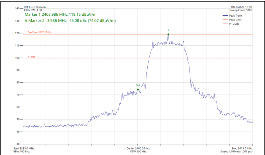
Figure 533 - Bluetooth HDRPM12, MIMO, Core 0-1 - 2404 MHz Band Edge Frequency 2400 MHz
