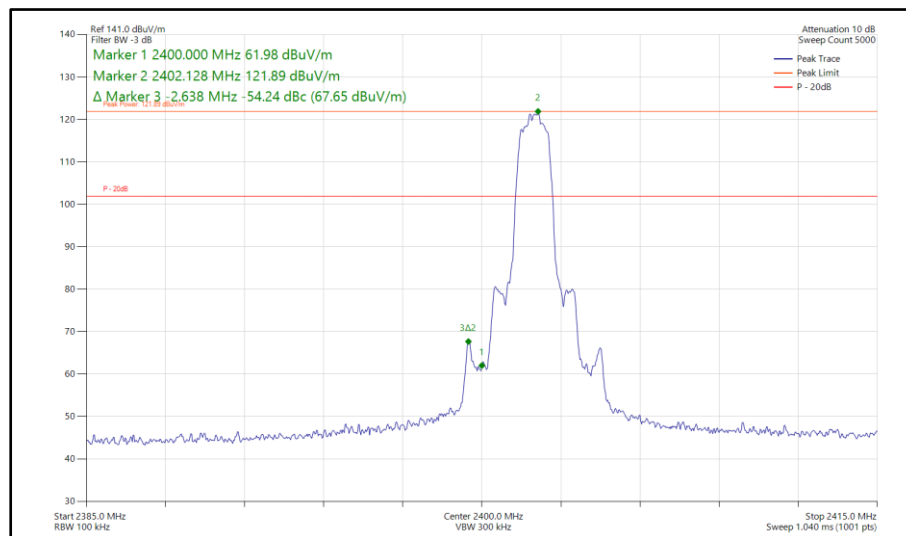
Figure 523 - Bluetooth 2DH5, MIMO, Core 0-1 - 2402 MHz Band Edge Frequency 2400 MHz
