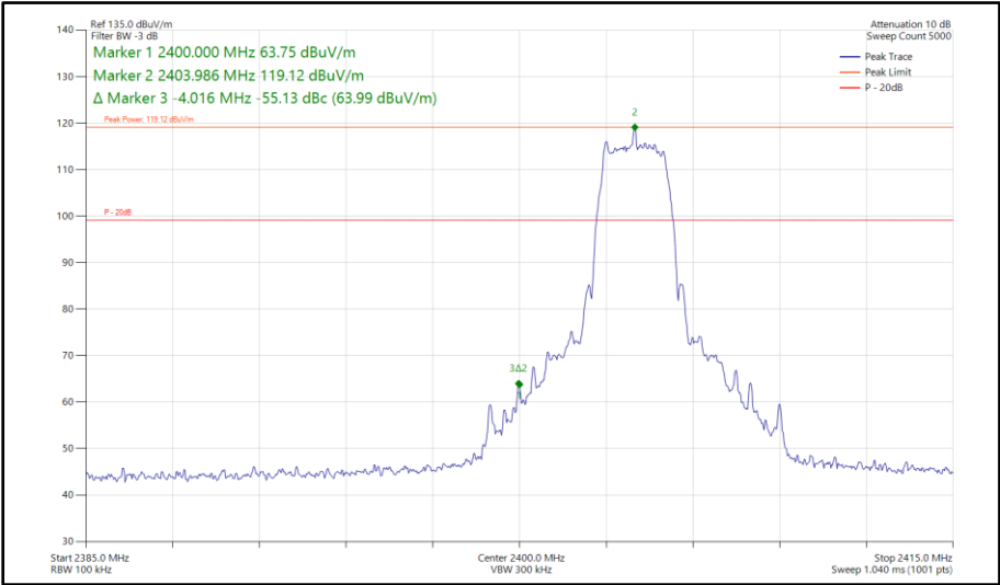
Figure 508 - Bluetooth HDRPS2, SISO, Core 0 - 2404 MHz Band Edge Frequency 2400 MHz
