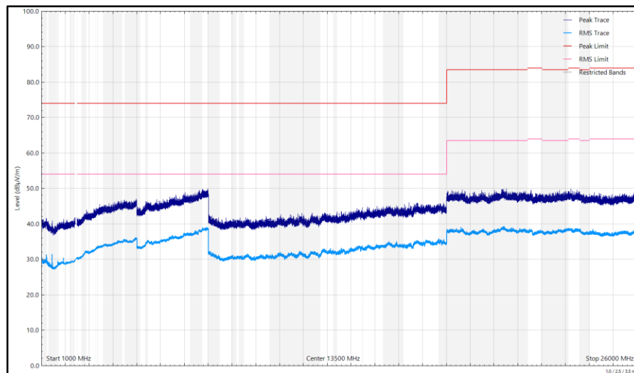
Figure 573 - 2440 MHz, HDT4, iPA, Core 0 + Core 1, 1 GHz to 26 GHz, Horizontal
