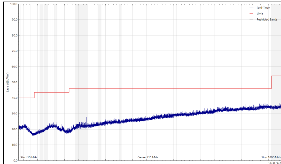
Figure 546 - 2440 MHz, LE1M, iPA, Core 2, 30 MHz to 1 GHz, Horizontal (Peak)
