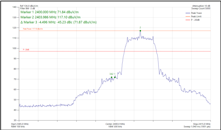
Figure 509 - Bluetooth HDRPM12, SISO, Core 0 - 2404 MHz Band Edge Frequency 2400 MHz
