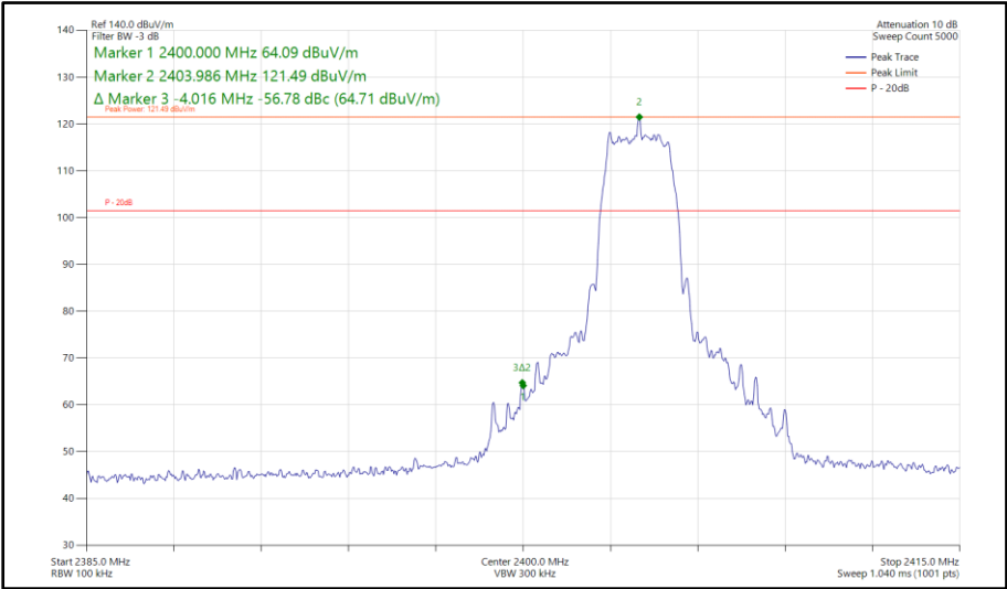
Figure 532 - Bluetooth HDRPS2, MIMO, Core 0-1 - 2404 MHz Band Edge Frequency 2400 MHz
