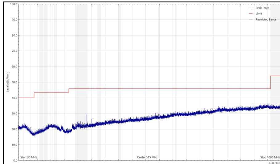
Figure 572 - 2440 MHz, HDT4, iPA, Core 0 + Core 1, 30 MHz to 1 GHz, Horizontal (Peak)
