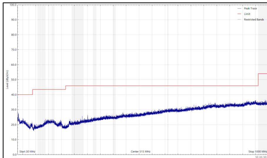
Figure 556 - 2440 MHz, LE1M, ePA, Core 0 + Core 1, 30 MHz to 1 GHz, Vertical (Peak)
