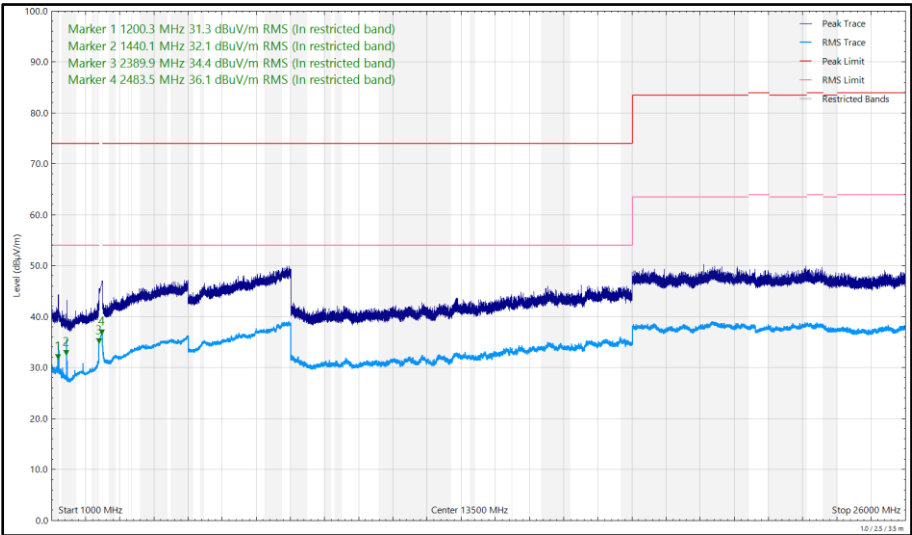
Figure 571 - 2440 MHz, HDR8, ePA, Core 0 + Core 1, 1 GHz to 26 GHz, Vertical
