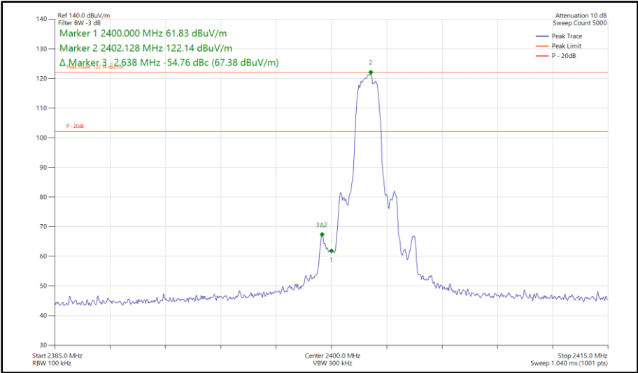
Figure 524 - Bluetooth 3DH5, MIMO, Core 0-1 - 2402 MHz Band Edge Frequency 2400 MHz
