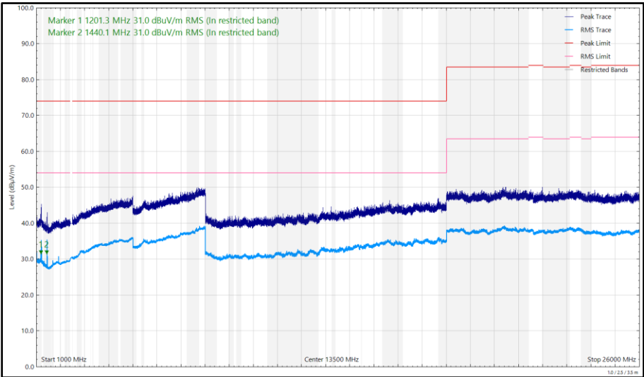
Figure 563 - 2440 MHz, HDR8, iPA, Core 0 + Core 1, 1 GHz to 26 GHz, Vertical
