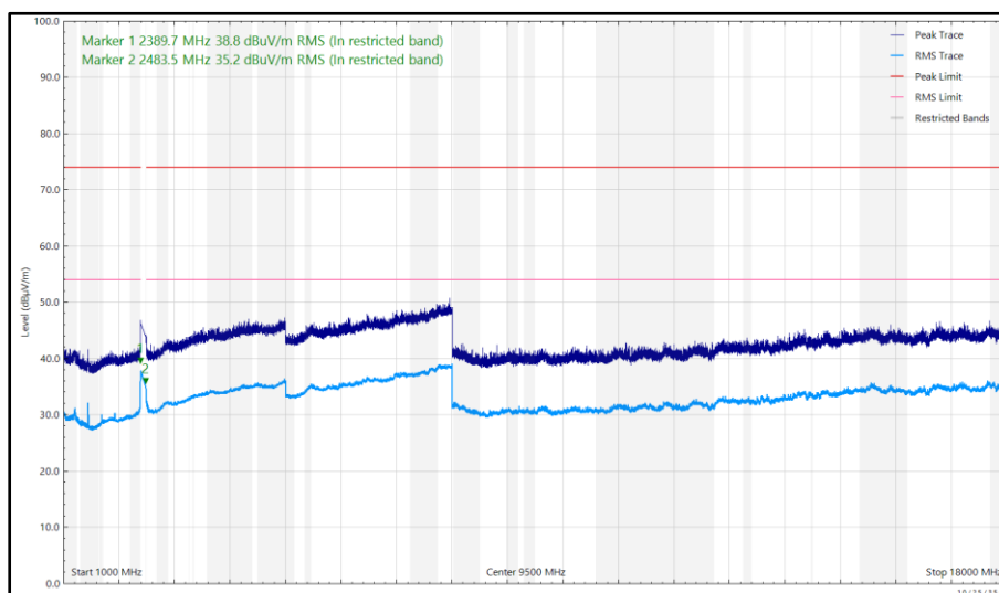
Figure 552 - 2402 MHz, LE1M, ePA, Core 0 + Core 1, 1 GHz to 18 GHz, Horizontal
