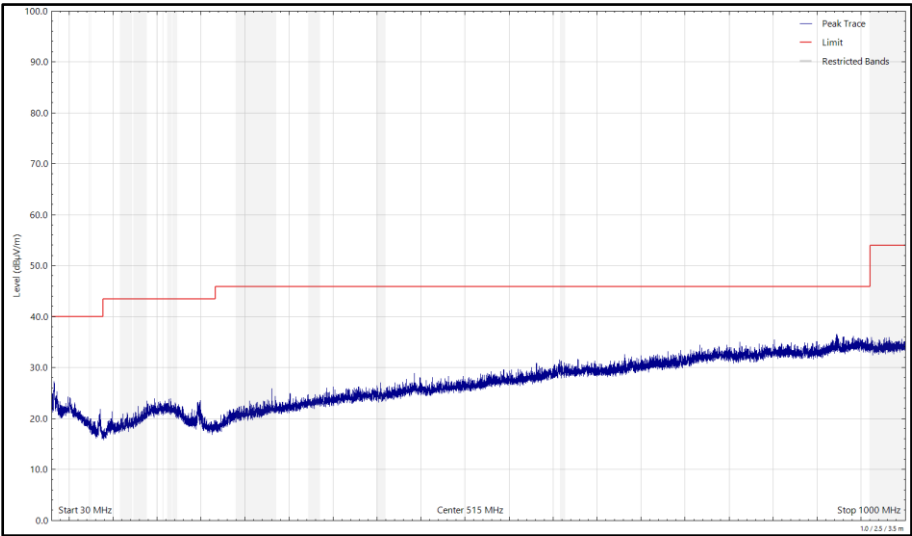
Figure 566 - 2440 MHz, HDR8, iPA, Core 2, 30 MHz to 1 GHz, Vertical (Peak)
