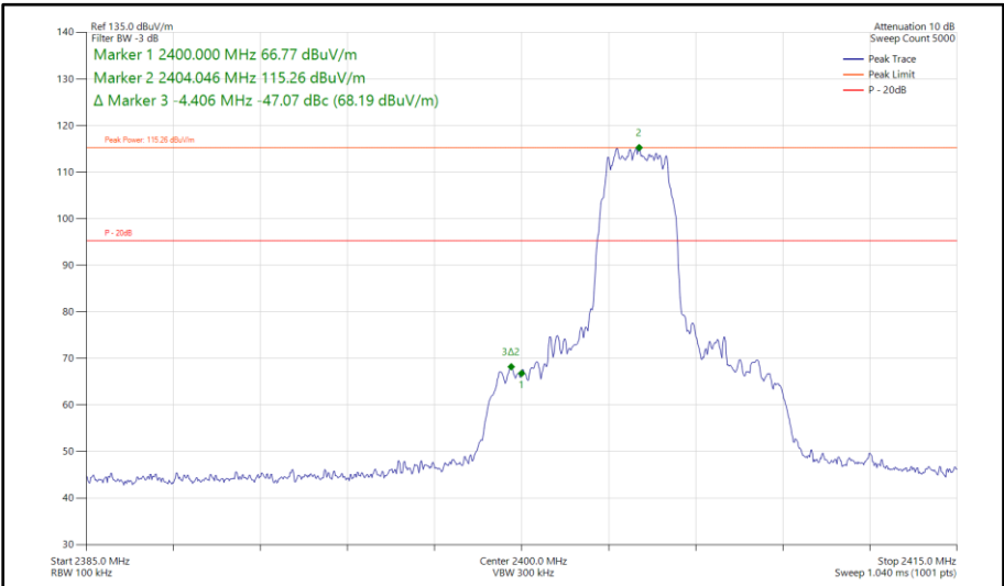
Figure 507 - Bluetooth HDT6, SISO, Core 0 - 2404 MHz Band Edge Frequency 2400 MHz
