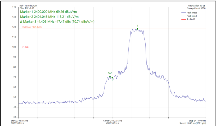
Figure 531 - Bluetooth HDT6, MIMO, Core 0-1 - 2404 MHz Band Edge Frequency 2400 MHz
