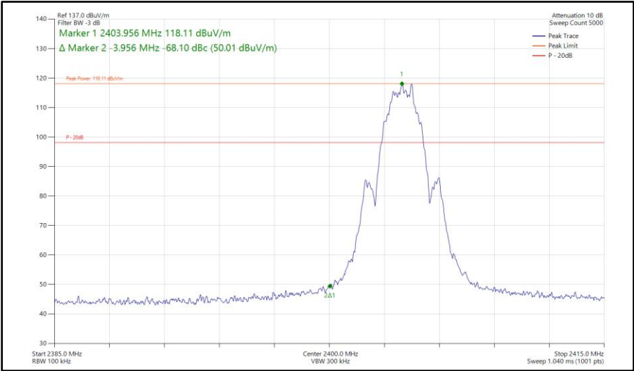
Figure 504 - Bluetooth LE2M, SISO, Core 0 - 2404 MHz Band Edge Frequency 2400 MHz
