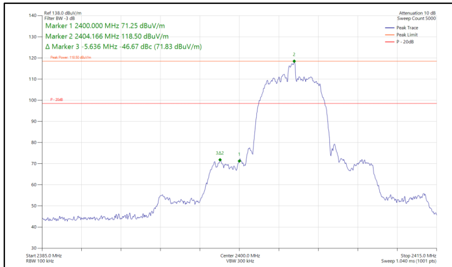
Figure 502 - Bluetooth HDR8, SISO, Core 0 - 2404 MHz Band Edge Frequency 2400 MHz
