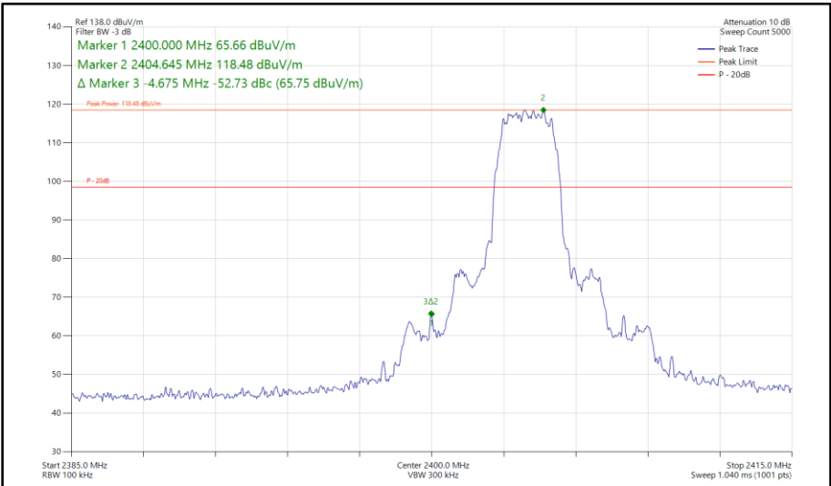
Figure 529 - Bluetooth HDT3, MIMO, Core 0-1 - 2404 MHz Band Edge Frequency 2400 MHz
