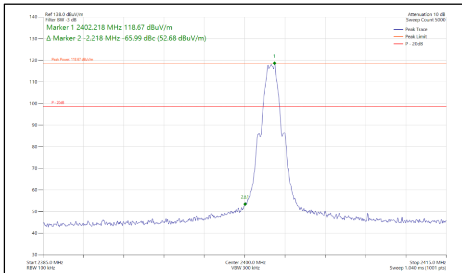
Figure 503 - Bluetooth LE1M, SISO, Core 0 - 2402 MHz Band Edge Frequency 2400 MHz
