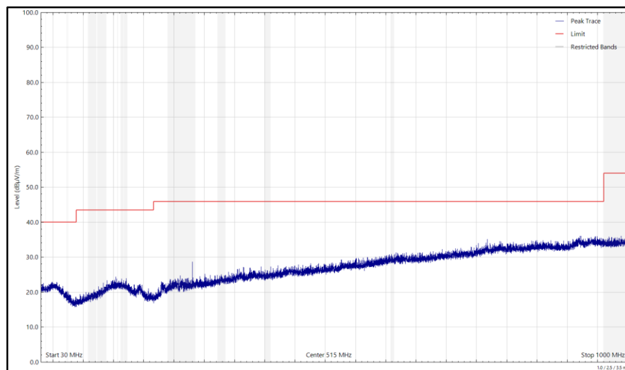
Figure 554 - 2440 MHz, LE1M, ePA, Core 0 + Core 1, 30 MHz to 1 GHz, Horizontal (Peak)
