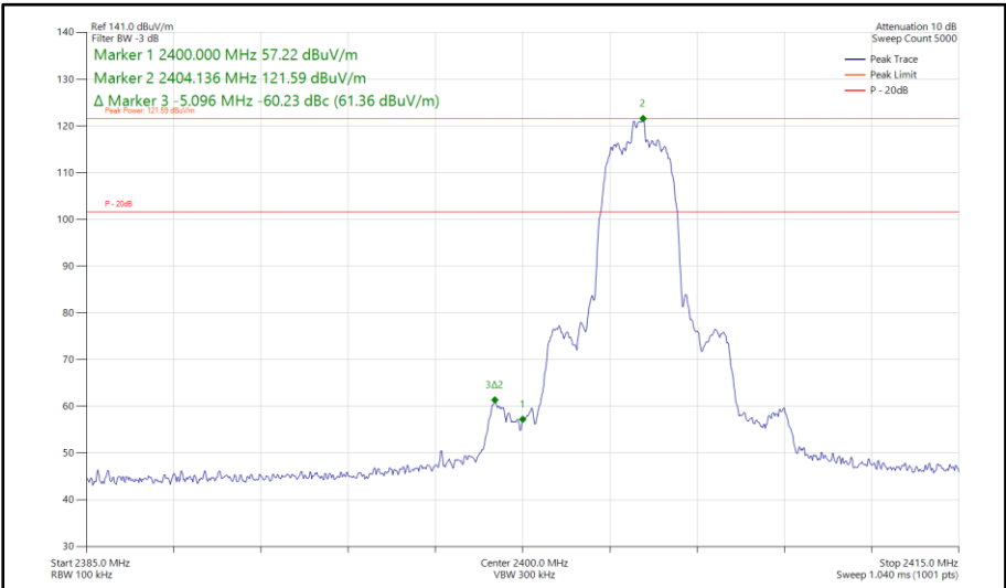
Figure 525 - Bluetooth HDR4, MIMO, Core 0-1 - 2404 MHz Band Edge Frequency 2400 MHz
