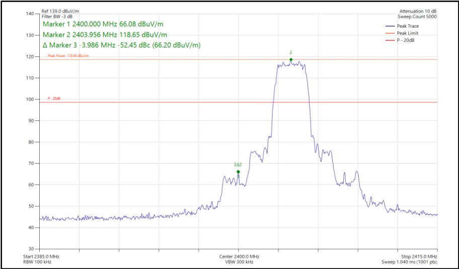
Figure 530 - Bluetooth HDT4, MIMO, Core 0-1 - 2404 MHz Band Edge Frequency 2400 MHz
