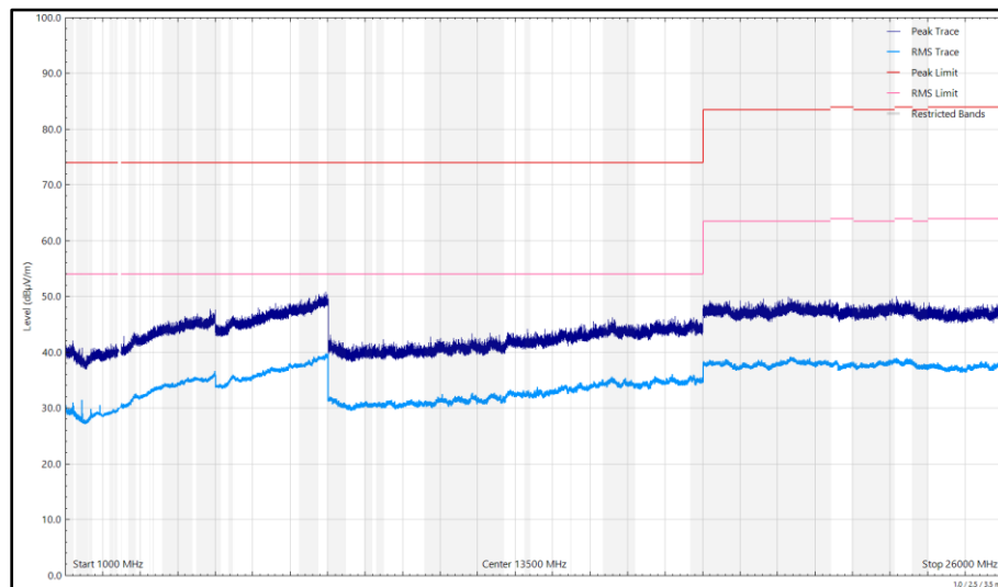
Figure 561 - 2440 MHz, HDR8, iPA, Core 0 + Core 1, 1 GHz to 26 GHz, Horizontal
