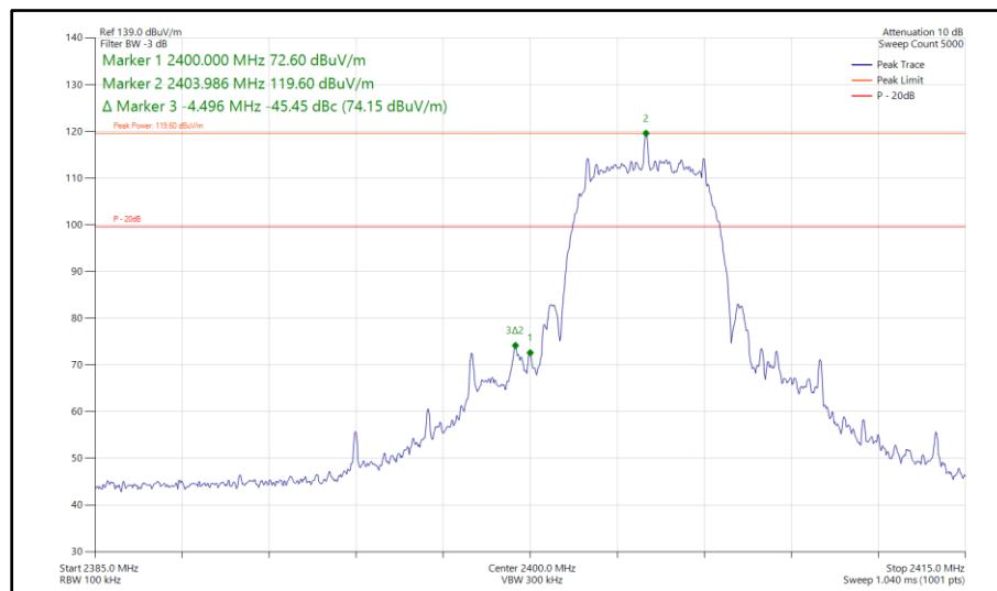
Figure 534 - Bluetooth XHDRPM8, MIMO, Core 0-1 - 2404 MHz Band Edge Frequency 2400 MHz
