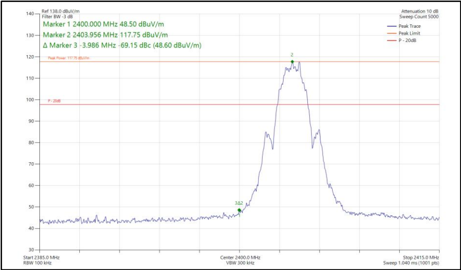
Figure 528 - Bluetooth LE2M, MIMO, Core 0-1 - 2404 MHz Band Edge Frequency 2400 MHz
