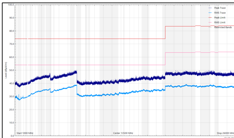
Figure 539 - 2440 MHz, LE1M, iPA, Core 0 + Core 1, 1 GHz to 26 GHz, Horizontal
