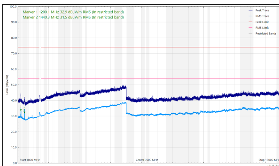
Figure 537 - 2402 MHz, LE1M, iPA, Core 0 + Core 1, 1 GHz to 18 GHz, Vertical
