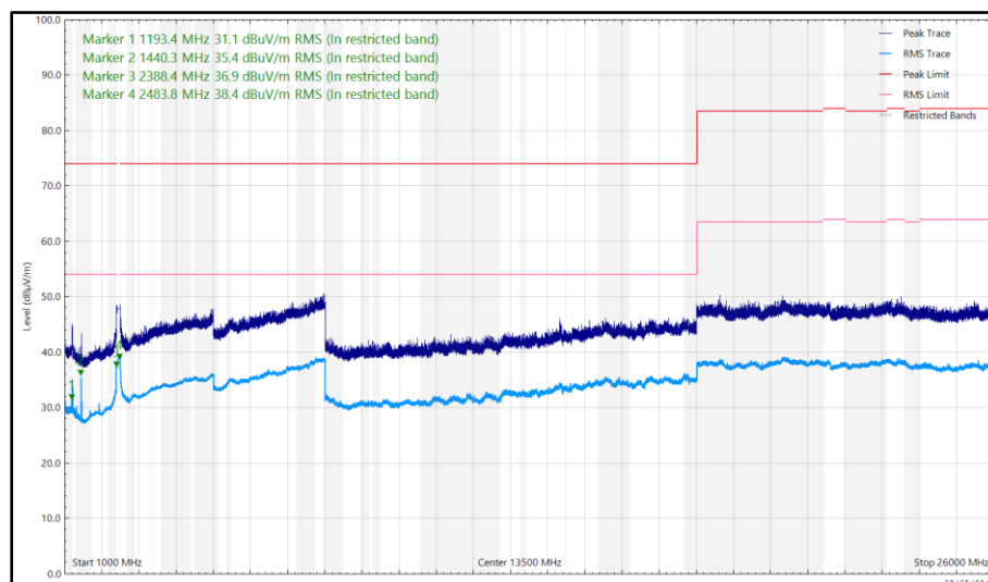
Figure 557 - 2440 MHz, LE1M, ePA, Core 0 + Core 1, 1 GHz to 26 GHz, Vertical
