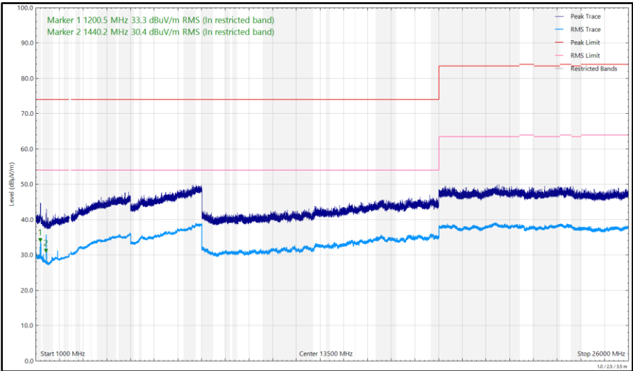
Figure 567 - 2440 MHz, HDR8, iPA, Core 2, 1 GHz to 26 GHz, Vertical
