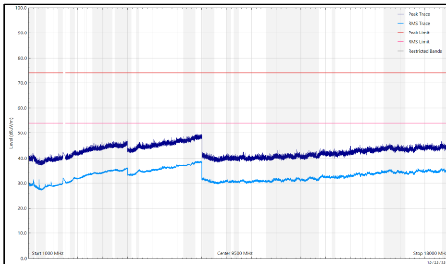
Figure 544 - 2402 MHz, LE1M, iPA, Core 2, 1 GHz to 18 GHz, Horizontal
