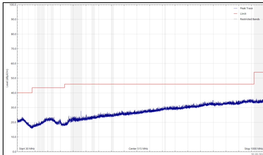
Figure 560 - 2440 MHz, HDR8, iPA, Core 0 + Core 1, 30 MHz to 1 GHz, Horizontal (Peak)
