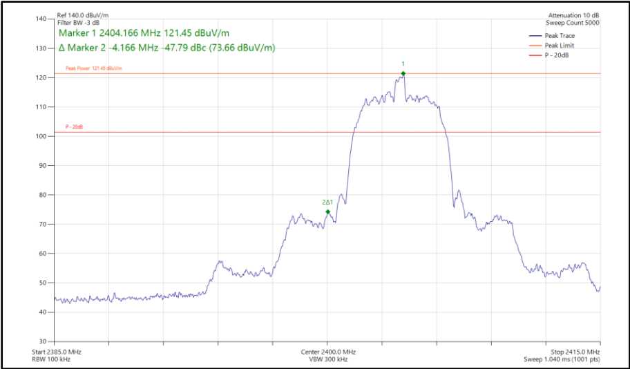
Figure 526 - Bluetooth HDR8, MIMO, Core 0-1 - 2404 MHz Band Edge Frequency 2400 MHz
