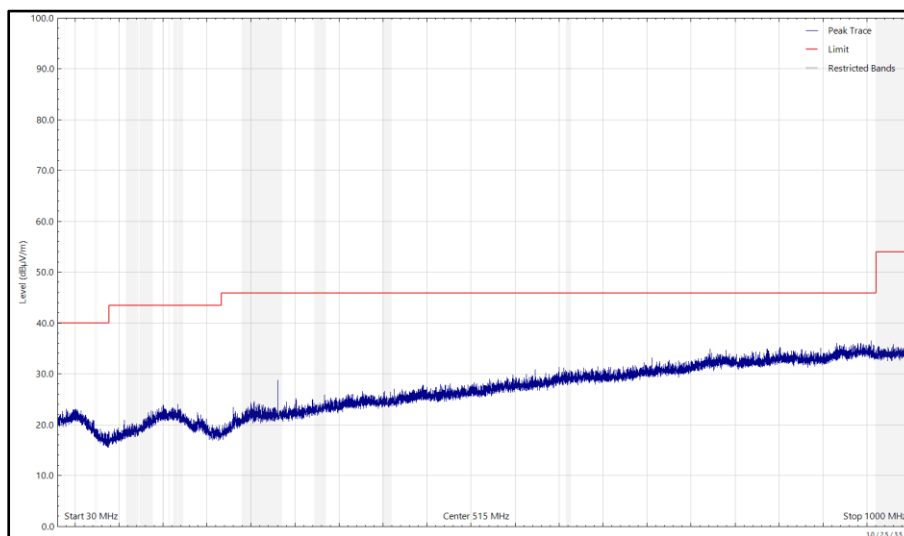
Figure 538 - 2440 MHz, LE1M, iPA, Core 0 + Core 1, 30 MHz to 1 GHz, Horizontal (Peak)
