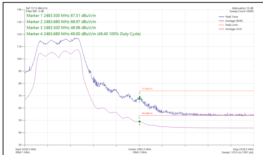
Figure 137 - 802.11g, CDD, Core 0-1 - 2452 MHz Band Edge Frequency 2483.5 MHz
