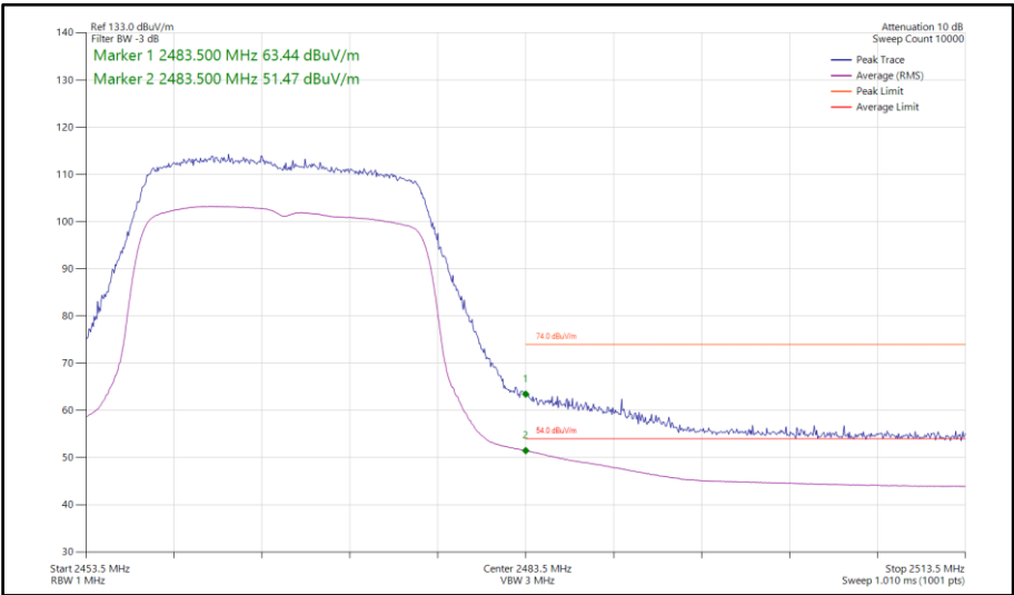
Figure 106 - 802.11ax HE20, SU, SISO, Core 1 - 2467 MHz Band Edge Frequency 2483.5 MHz
