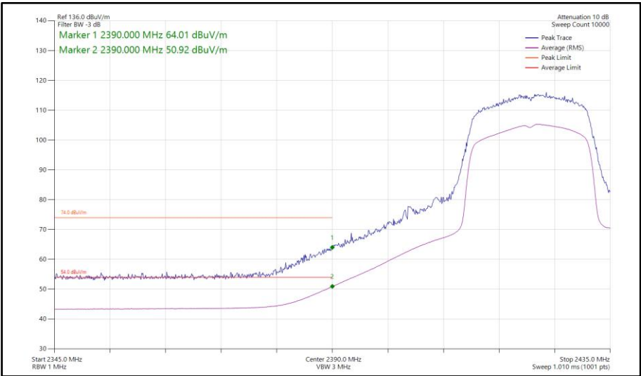
Figure 74 - 802.11ax HE20, SU, SISO, Core 1 - 2422 MHz Band Edge Frequency 2390 MHz
