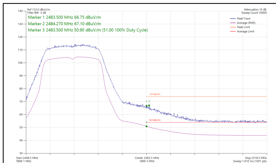
Figure 88 - 802.11g, SISO, Core 1 - 2462 MHz Band Edge Frequency 2483.5 MHz
