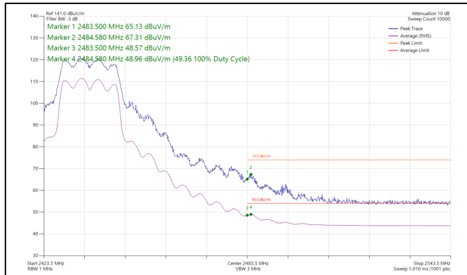
Figure 134 - 802.11g, CDD, Core 0-1 - 2437 MHz Band Edge Frequency 2483.5 MHz
