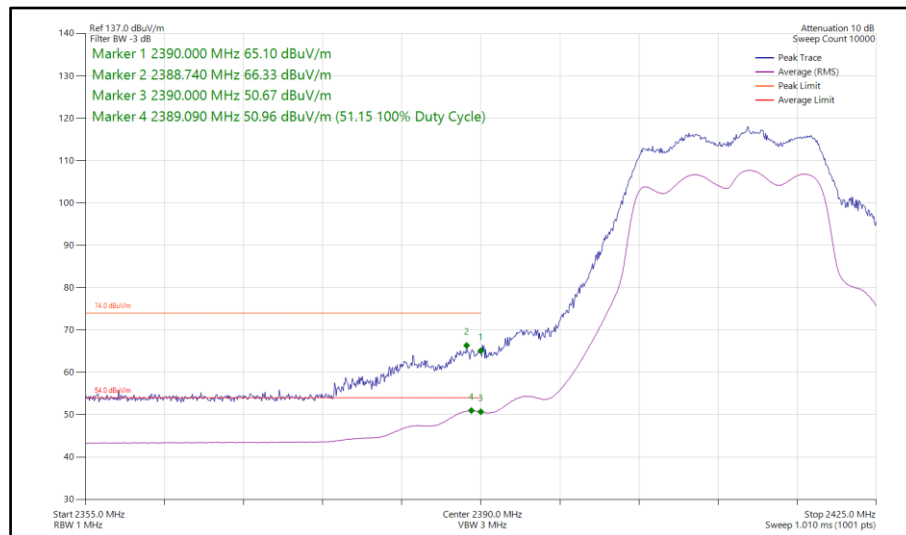
Figure 115 - 802.11g, CDD, Core 0-1 - 2412 MHz Band Edge Frequency 2390 MHz
