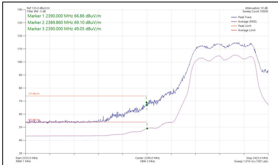
Figure 120 - 802.11n HT20, CDD, Core 0-1 - 2412 MHz Band Edge Frequency 2390 MHz
