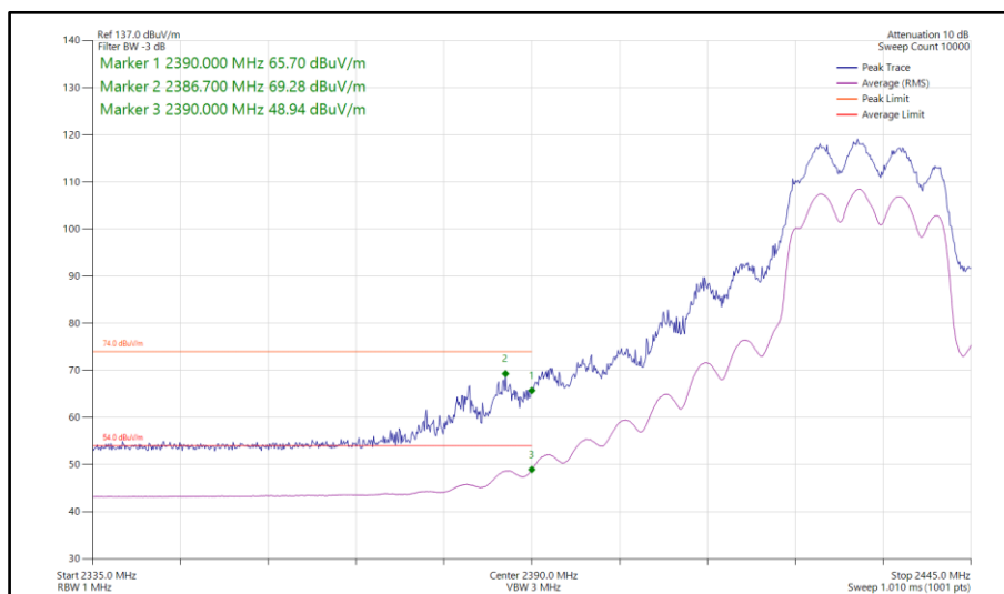
Figure 131 - 802.11ax HE20, SU, CDD, Core 0-1 - 2432 MHz Band Edge Frequency 2390 MHz
