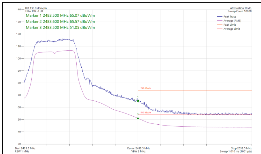
Figure 92 - 802.11n HT20, SISO, Core 1 - 2447 MHz Band Edge Frequency 2483.5 MHz
