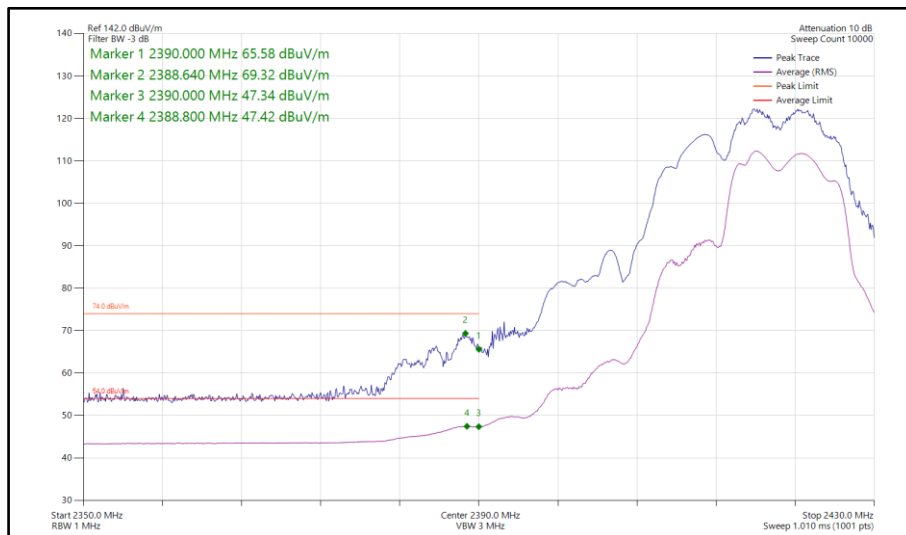
Figure 133 - 802.11be EHT20, RU 106+26-83, CDD, Core 0-1 - 2417 MHz Band Edge Frequency 2390 MHz
