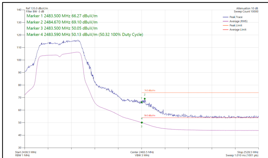
Figure 86 - 802.11g, SISO, Core 1 - 2452 MHz Band Edge Frequency 2483.5 MHz
