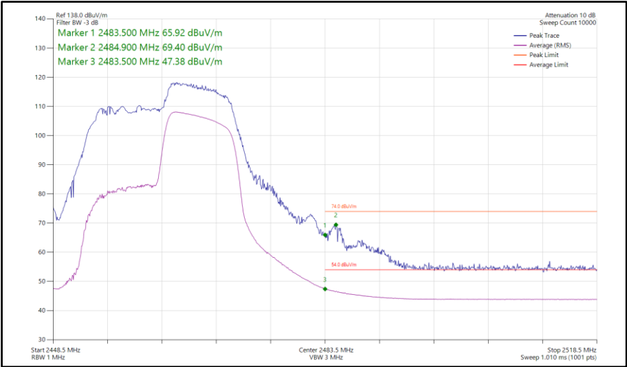
Figure 105 - 802.11ax HE20, RU 106-54, SISO, Core 1 - 2462 MHz Band Edge Frequency 2483.5 MHz
