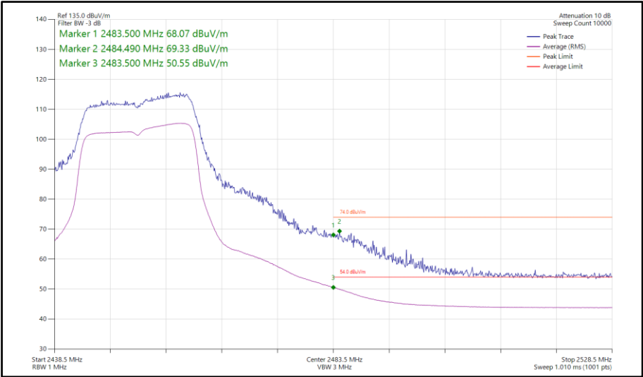
Figure 93 - 802.11n HT20, SISO, Core 1 - 2452 MHz Band Edge Frequency 2483.5 MHz
