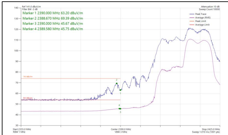
Figure 126 - 802.11ax HE20, RU 106-54, CDD, Core 0-1 - 2412 MHz Band Edge Frequency 2390 MHz
