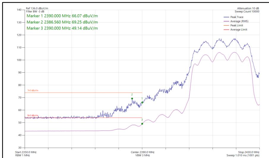
Figure 127 - 802.11ax HE20, SU, CDD, Core 0-1 - 2417 MHz Band Edge Frequency 2390 MHz
