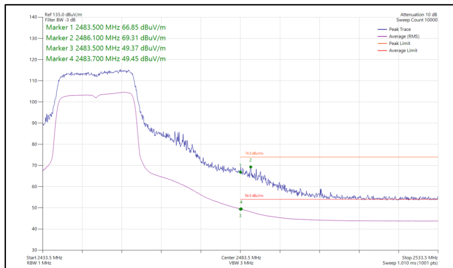
Figure 99 - 802.11ax HE20, SU, SISO, Core 1 - 2447 MHz Band Edge Frequency 2483.5 MHz
