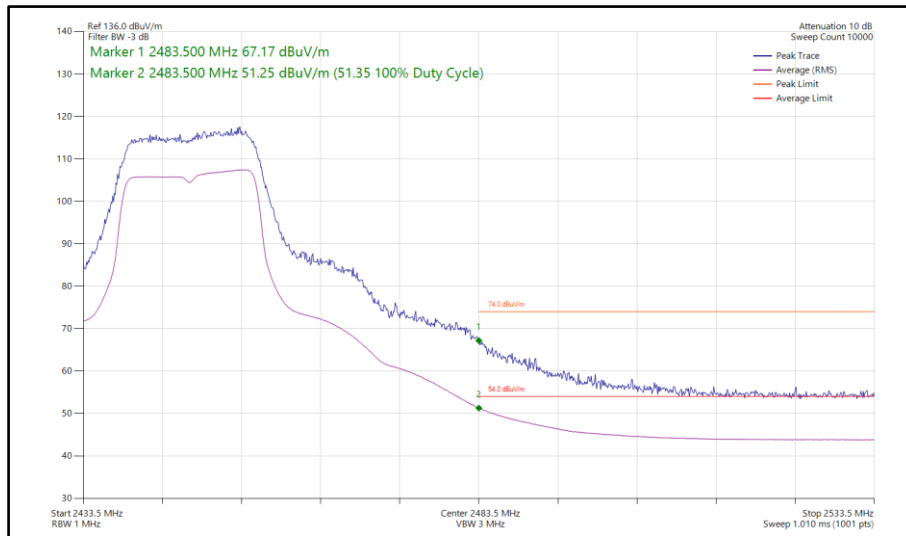
Figure 85 - 802.11g, SISO, Core 1 - 2447 MHz Band Edge Frequency 2483.5 MHz
