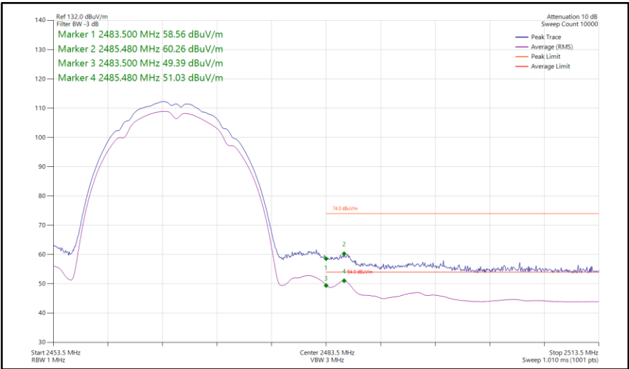
Figure 82 - 802.11b, SISO, Core 1 - 2467 MHz Band Edge Frequency 2483.5 MHz
