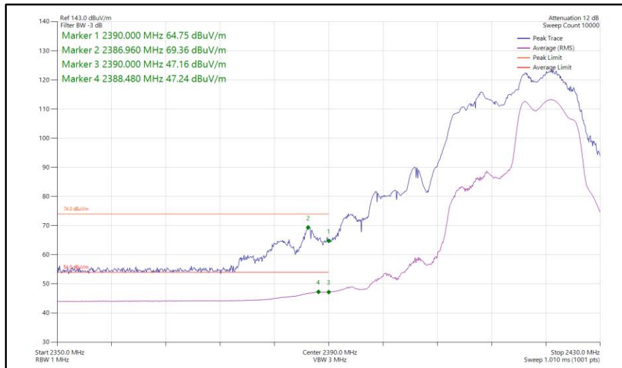
Figure 128 - 802.11ax HE20, RU 106-54, CDD, Core 0-1 - 2417 MHz Band Edge Frequency 2390 MHz
