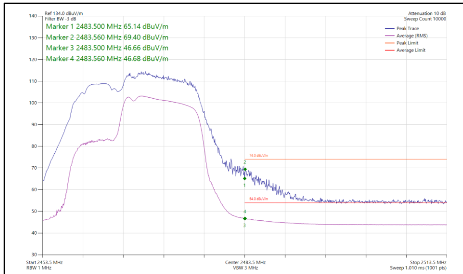
Figure 113 - 802.11be EHT20, RU 106+26-83, SISO, Core 1 - 2467 MHz Band Edge Frequency 2483.5 MHz
