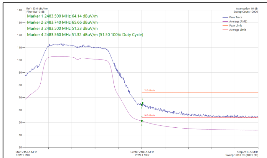
Figure 89 - 802.11g, SISO, Core 1 - 2467 MHz Band Edge Frequency 2483.5 MHz
