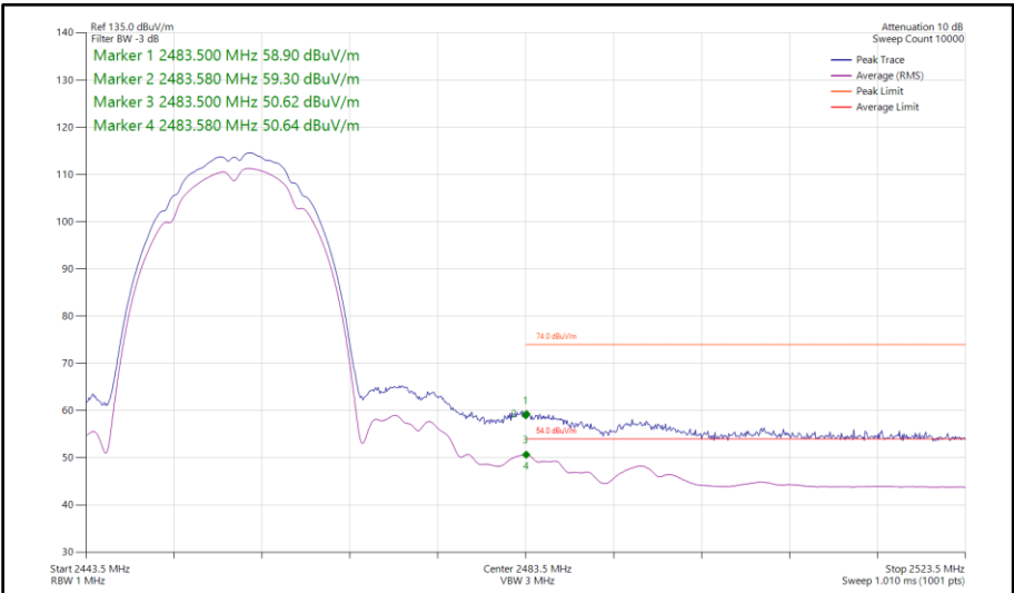
Figure 80 - 802.11b, SISO, Core 1 - 2457 MHz Band Edge Frequency 2483.5 MHz
