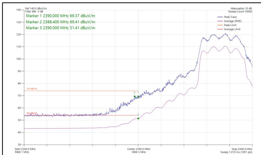
Figure 130 - 802.11ax HE20, SU, CDD, Core 0-1 - 2427 MHz Band Edge Frequency 2390 MHz
