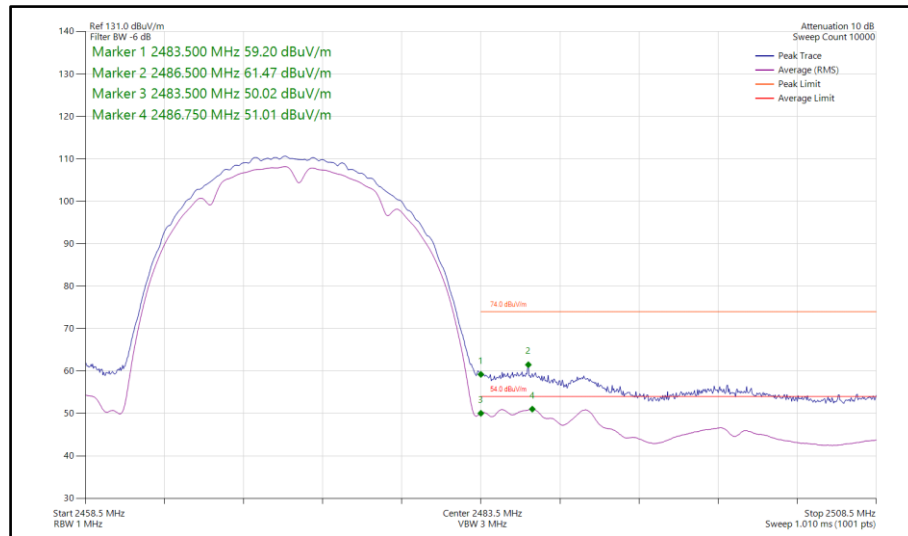
Figure 83 - 802.11b, SISO, Core 1 - 2472 MHz Band Edge Frequency 2483.5 MHz
