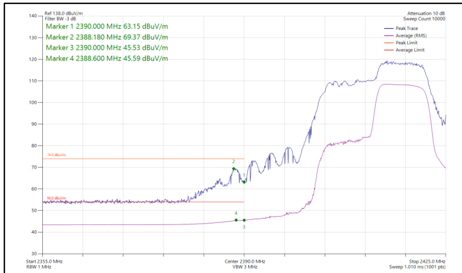
Figure 71 - 802.11ax HE20, RU 106-54, SISO, Core 1 - 2412 MHz Band Edge Frequency 2390 MHz
