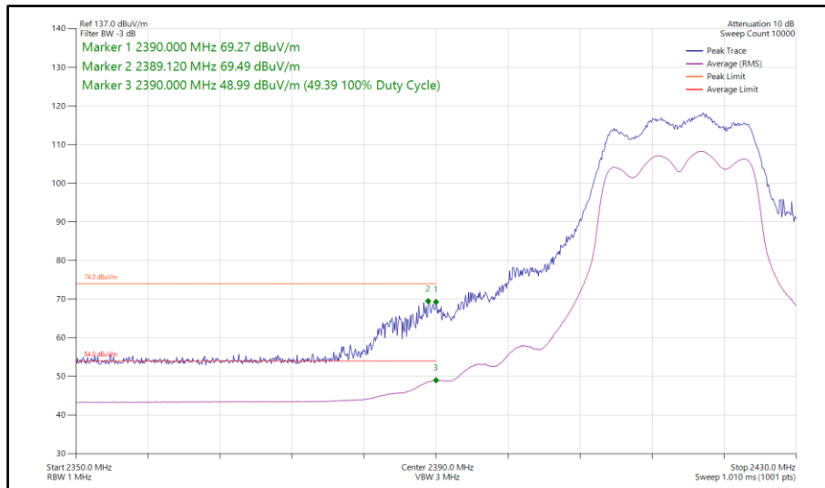
Figure 116 - 802.11g, CDD, Core 0-1 - 2417 MHz Band Edge Frequency 2390 MHz
