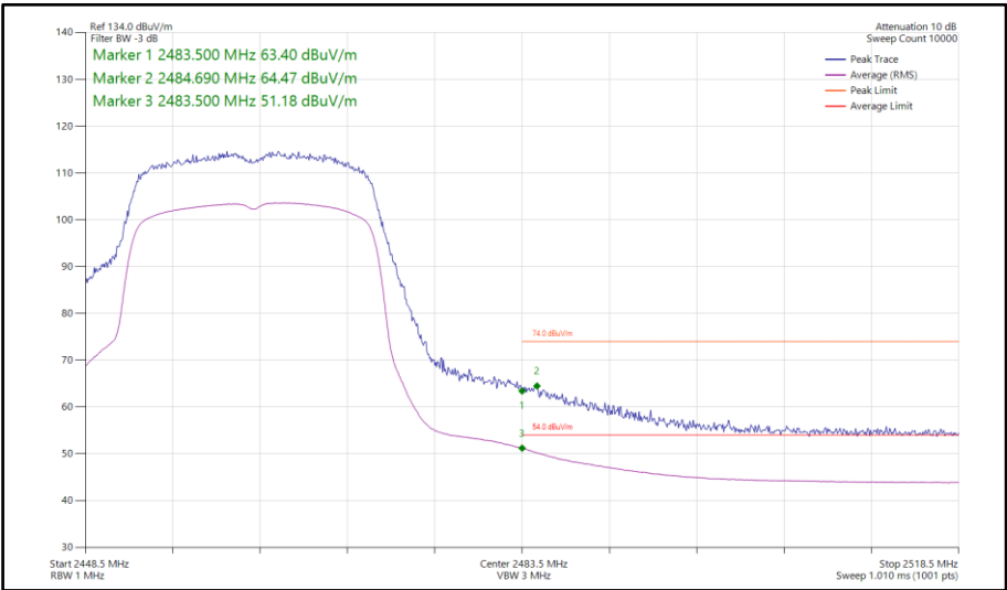
Figure 104 - 802.11ax HE20, SU, SISO, Core 1 - 2462 MHz Band Edge Frequency 2483.5 MHz
