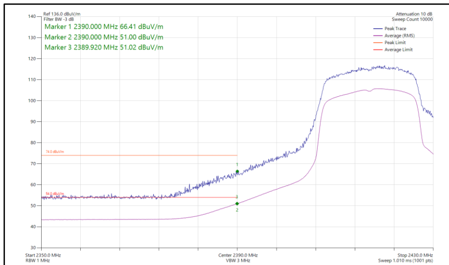
Figure 72 - 802.11ax HE20, SU, SISO, Core 1 - 2417 MHz Band Edge Frequency 2390 MHz
