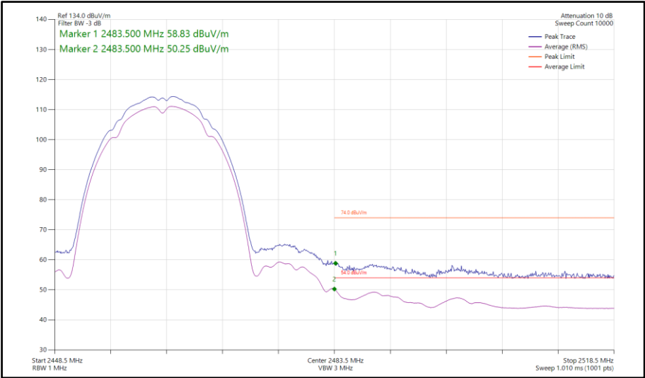
Figure 81 - 802.11b, SISO, Core 1 - 2462 MHz Band Edge Frequency 2483.5 MHz
