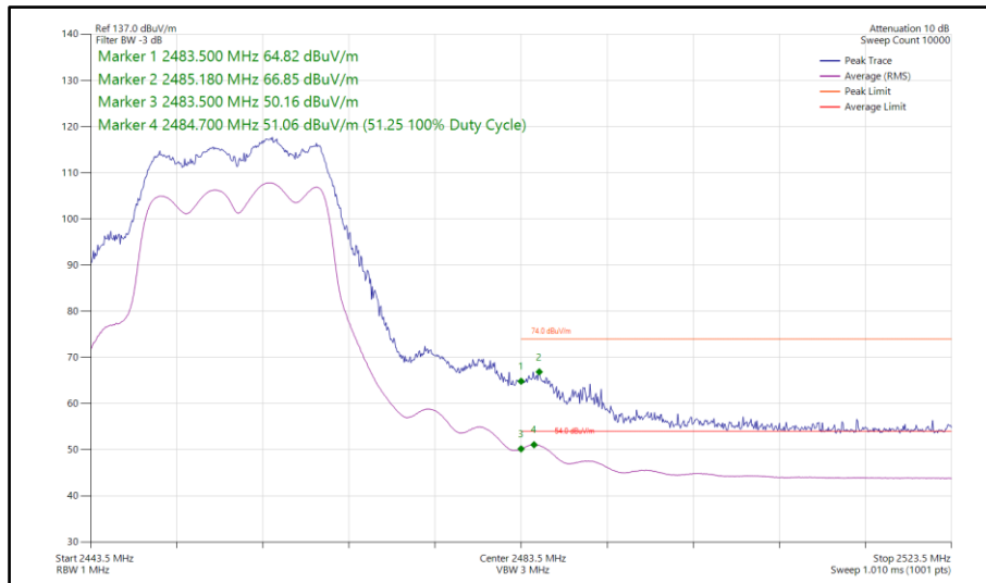
Figure 138 - 802.11g, CDD, Core 0-1 - 2457 MHz Band Edge Frequency 2483.5 MHz
