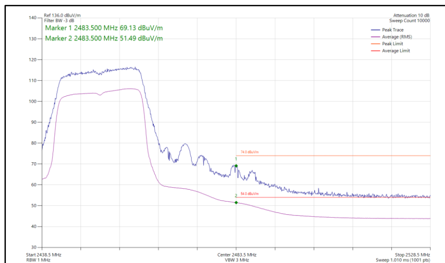
Figure 100 - 802.11ax HE20, SU, SISO, Core 1 - 2452 MHz Band Edge Frequency 2483.5 MHz
