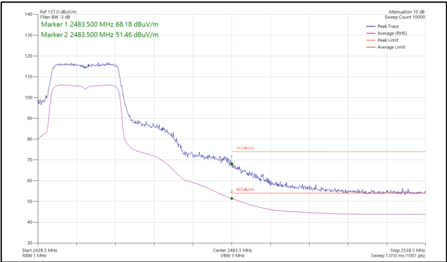
Figure 98 - 802.11ax HE20, SU, SISO, Core 1 - 2442 MHz Band Edge Frequency 2483.5 MHz
