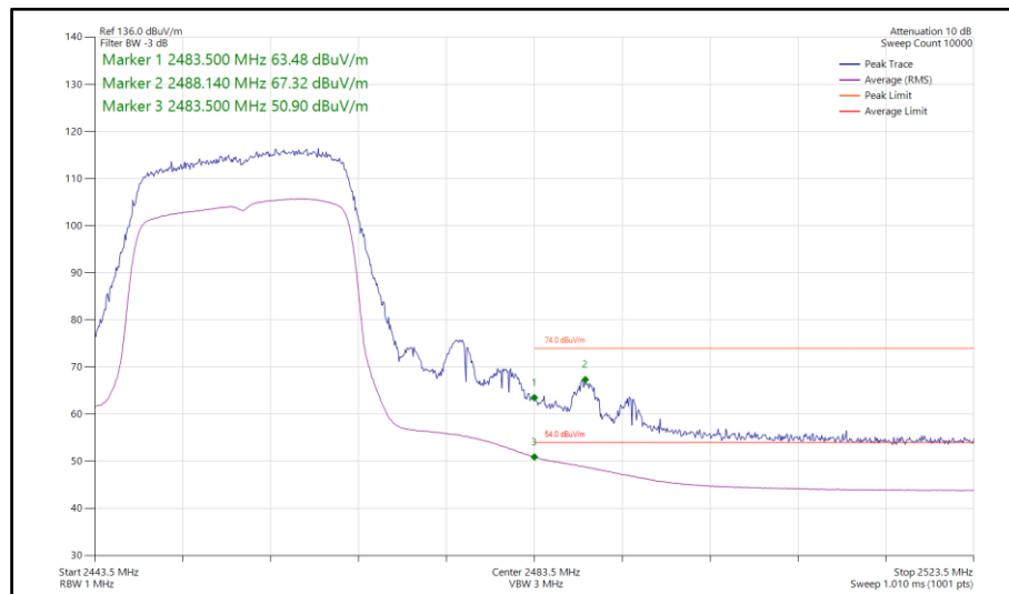
Figure 102 - 802.11ax HE20, SU, SISO, Core 1 - 2457 MHz Band Edge Frequency 2483.5 MHz
