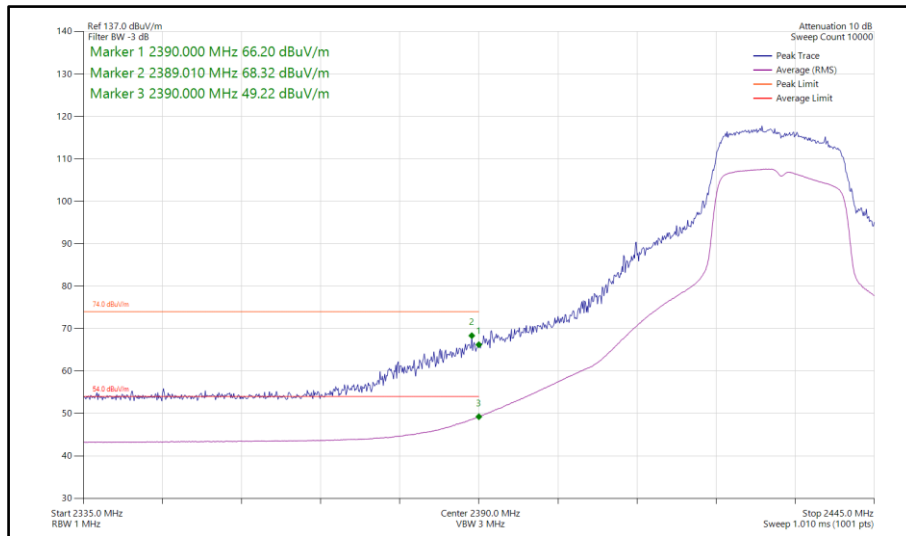
Figure 69 - 802.11n HT20, SISO, Core 1 - 2432 MHz Band Edge Frequency 2390 MHz
