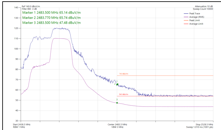
Figure 101 - 802.11ax HE20, RU 106-54, SISO, Core 1 - 2452 MHz Band Edge Frequency 2483.5 MHz
