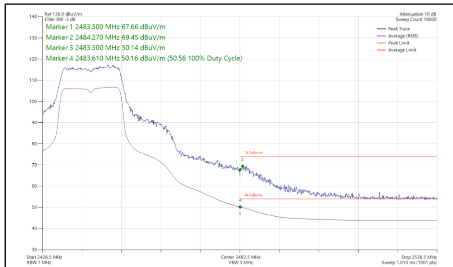
Figure 84 - 802.11g, SISO, Core 1 - 2442 MHz Band Edge Frequency 2483.5 MHz
