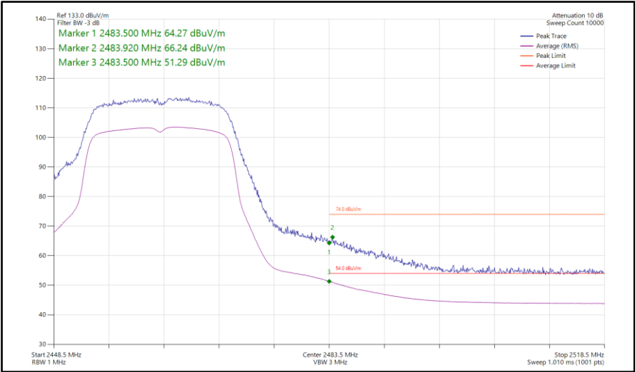
Figure 95 - 802.11n HT20, SISO, Core 1 - 2462 MHz Band Edge Frequency 2483.5 MHz
