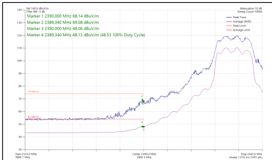
Figure 119 - 802.11g, CDD, Core 0-1 - 2432 MHz Band Edge Frequency 2390 MHz
