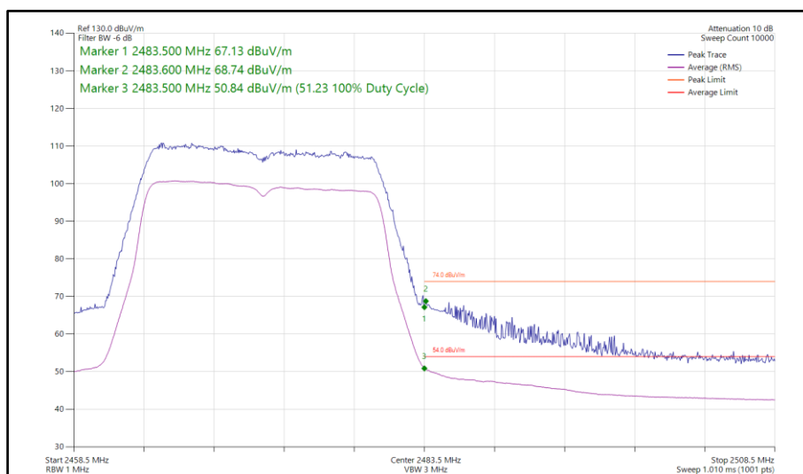
Figure 90 - 802.11g, SISO, Core 1 - 2472 MHz Band Edge Frequency 2483.5 MHz
