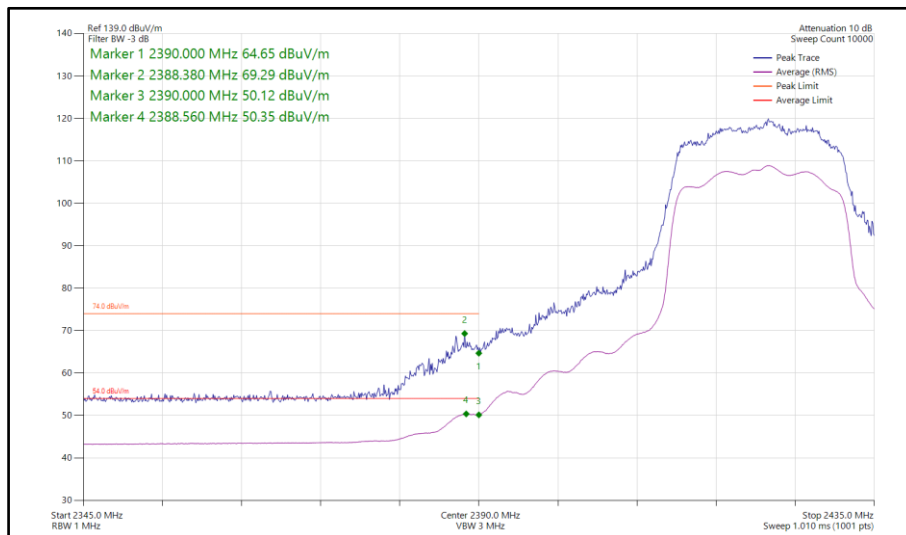
Figure 129 - 802.11ax HE20, SU, CDD, Core 0-1 - 2422 MHz Band Edge Frequency 2390 MHz
