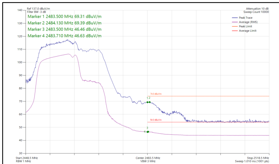
Figure 112 - 802.11be EHT20, RU 106+26-83, SISO, Core 1 - 2462 MHz Band Edge Frequency 2483.5 MHz
