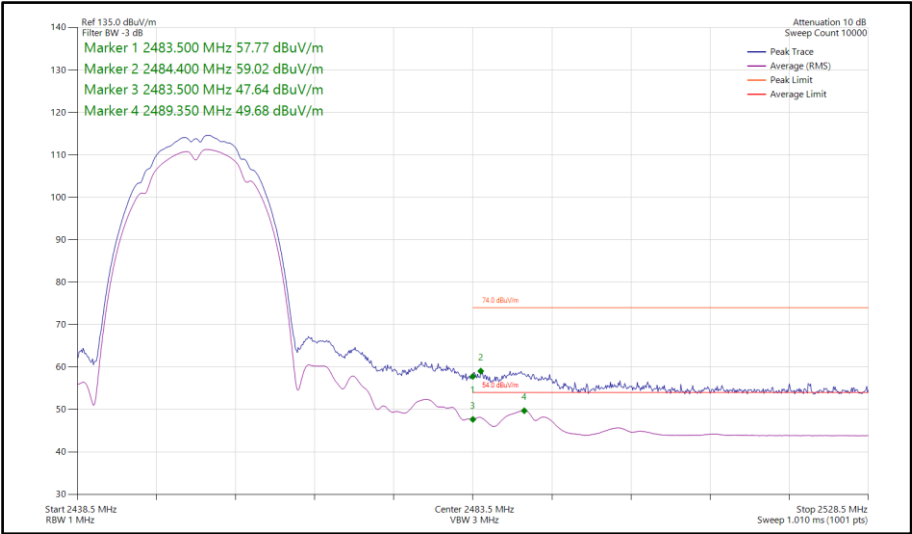
Figure 79 - 802.11b, SISO, Core 1 - 2452 MHz Band Edge Frequency 2483.5 MHz
