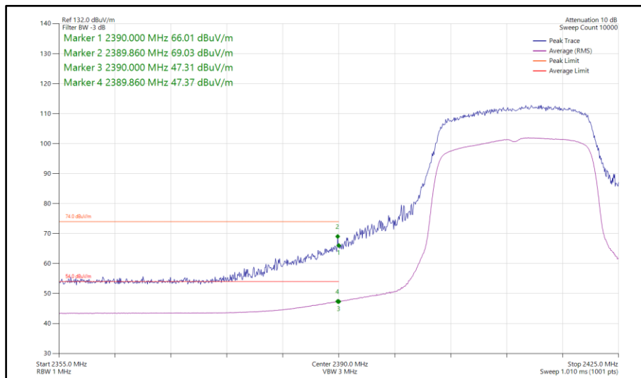
Figure 70 - 802.11ax HE20, SU, SISO, Core 1 - 2412 MHz Band Edge Frequency 2390 MHz
