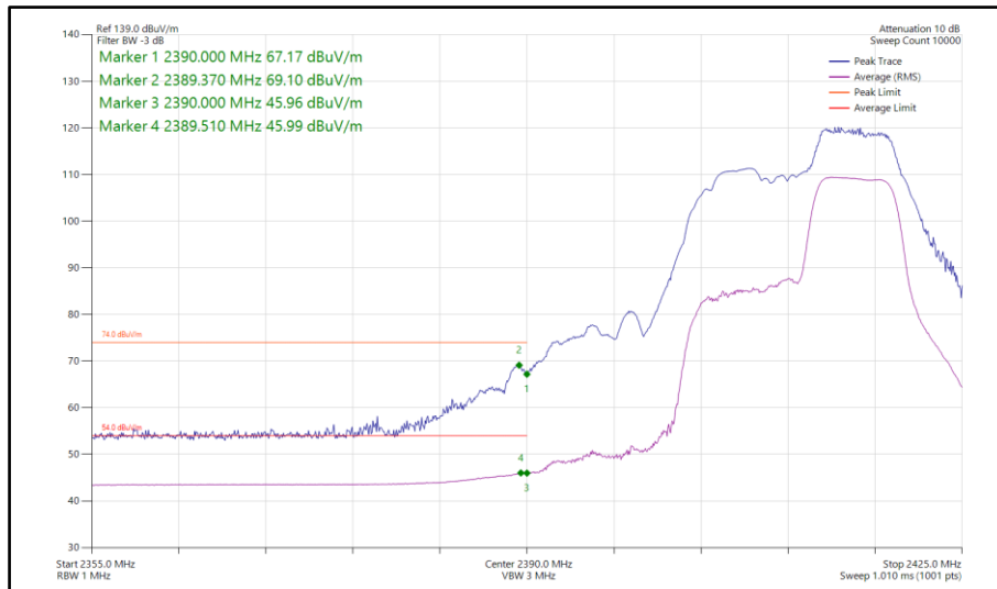
Figure 77 - 802.11be EHT20, RU 52+26-72, SISO, Core 1 - 2412 MHz Band Edge Frequency 2390 MHz
