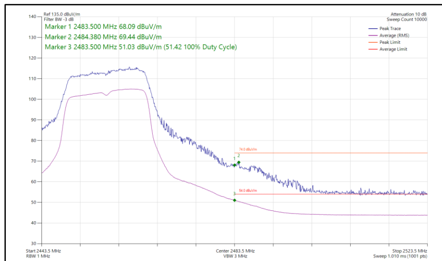
Figure 87 - 802.11g, SISO, Core 1 - 2457 MHz Band Edge Frequency 2483.5 MHz
