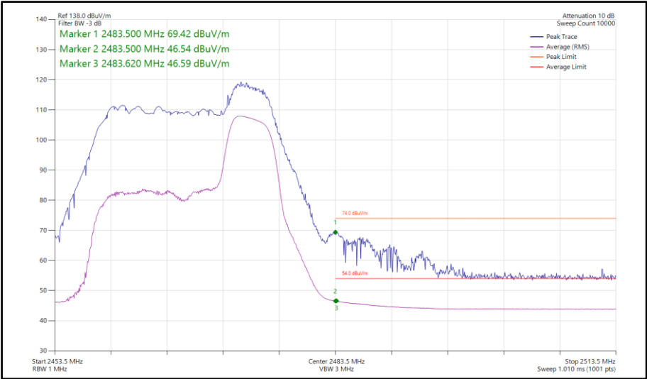
Figure 107 - 802.11ax HE20, RU 52-40, SISO, Core 1 - 2467 MHz Band Edge Frequency 2483.5 MHz
