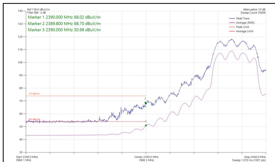
Figure 123 - 802.11n HT20, CDD, Core 0-1 - 2427 MHz Band Edge Frequency 2390 MHz
