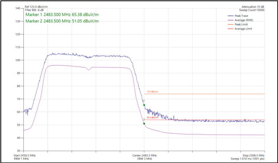
Figure 97 - 802.11n HT20, SISO, Core 1 - 2472 MHz Band Edge Frequency 2483.5 MHz
