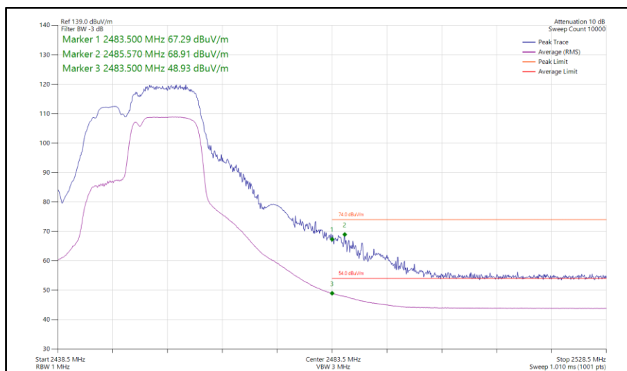
Figure 110 - 802.11be EHT20, RU 106+26-83, SISO, Core 1 - 2452 MHz Band Edge Frequency 2483.5 MHz
