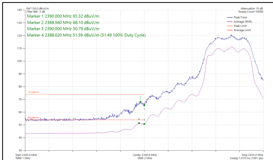
Figure 117 - 802.11g, CDD, Core 0-1 - 2422 MHz Band Edge Frequency 2390 MHz
