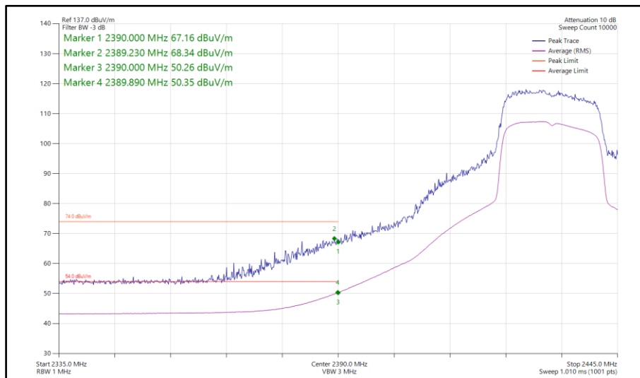
Figure 76 - 802.11ax HE20, SU, SISO, Core 1 - 2432 MHz Band Edge Frequency 2390 MHz
