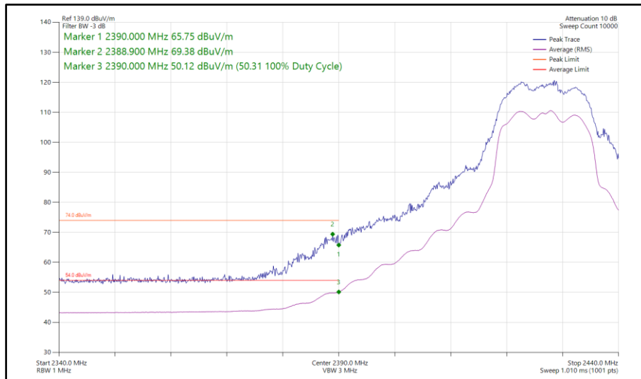
Figure 118 - 802.11g, CDD, Core 0-1 - 2427 MHz Band Edge Frequency 2390 MHz
