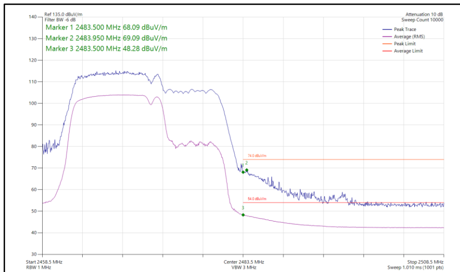
Figure 114 - 802.11be EHT20, RU 106+26-82, SISO, Core 1 - 2472 MHz Band Edge Frequency 2483.5 MHz
