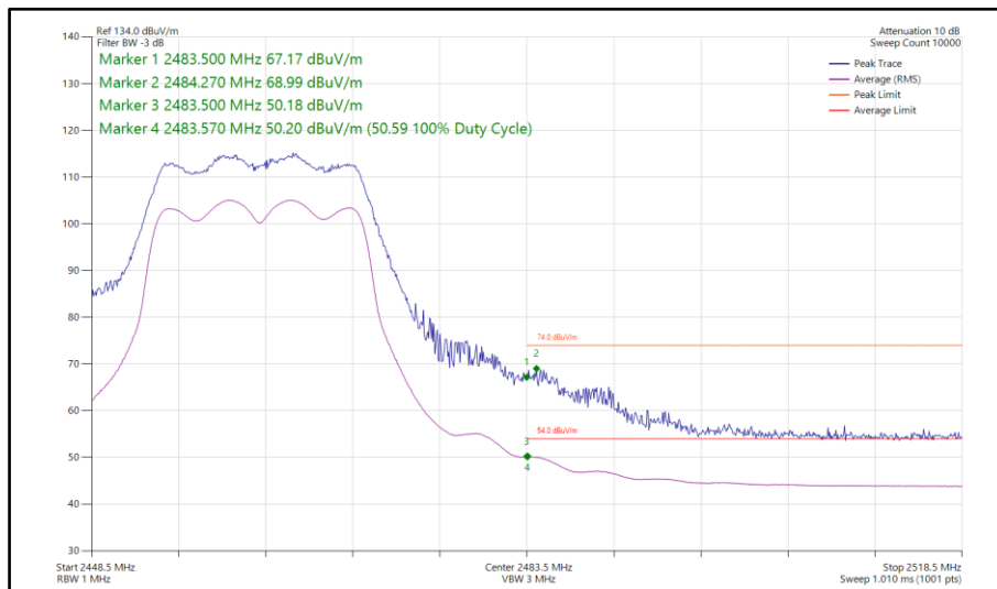
Figure 139 - 802.11g, CDD, Core 0-1 - 2462 MHz Band Edge Frequency 2483.5 MHz
