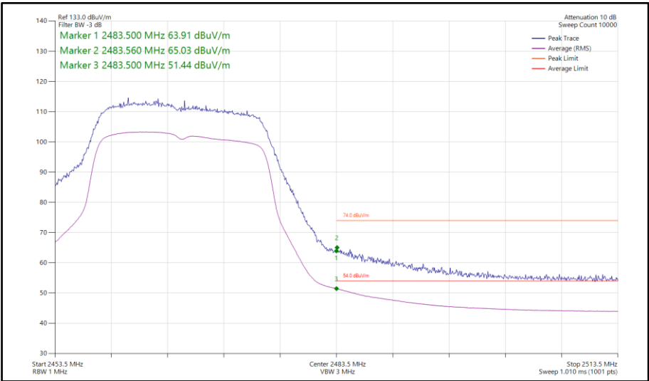
Figure 96 - 802.11n HT20, SISO, Core 1 - 2467 MHz Band Edge Frequency 2483.5 MHz
