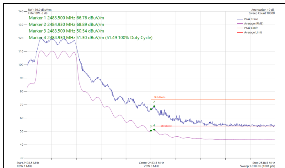
Figure 135 - 802.11g, CDD, Core 0-1 - 2442 MHz Band Edge Frequency 2483.5 MHz
