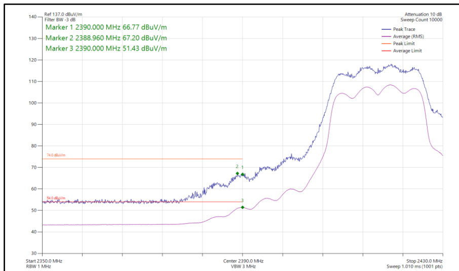
Figure 121 - 802.11n HT20, CDD, Core 0-1 - 2417 MHz Band Edge Frequency 2390 MHz
