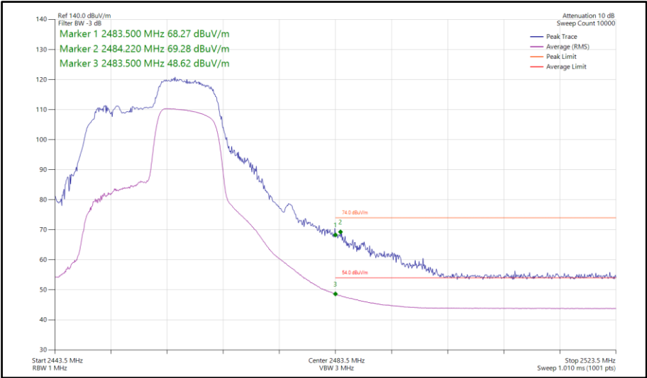
Figure 103 - 802.11ax HE20, RU 106-54, SISO, Core 1 - 2457 MHz Band Edge Frequency 2483.5 MHz
