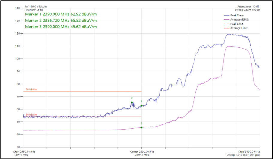
Figure 73 - 802.11ax HE20, RU 106-54, SISO, Core 1 - 2417 MHz Band Edge Frequency 2390 MHz
