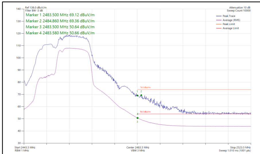
Figure 111 - 802.11be EHT20, RU 106+26-82, SISO, Core 1 - 2457 MHz Band Edge Frequency 2483.5 MHz
