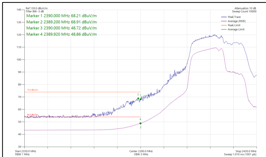
Figure 78 - 802.11be EHT20, RU 106+26-82, SISO, Core 1 - 2417 MHz Band Edge Frequency 2390 MHz
