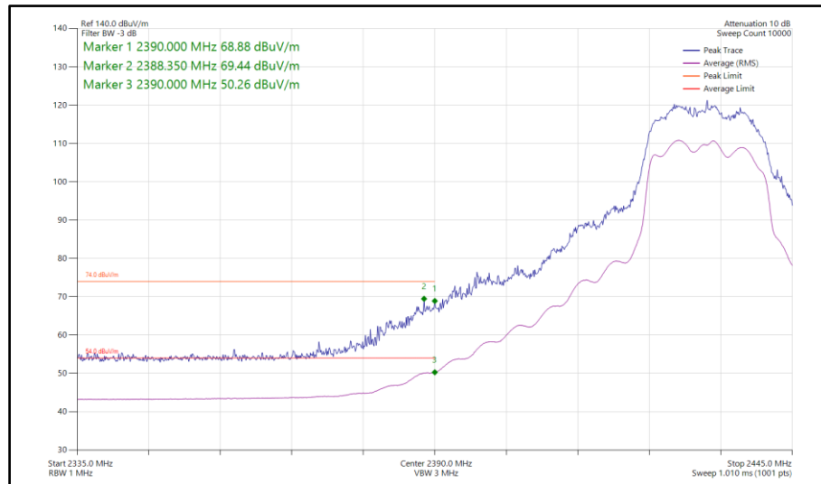
Figure 124 - 802.11n HT20, CDD, Core 0-1 - 2432 MHz Band Edge Frequency 2390 MHz
