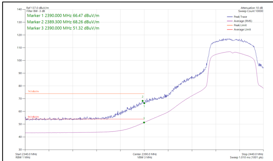
Figure 75 - 802.11ax HE20, SU, SISO, Core 1 - 2427 MHz Band Edge Frequency 2390 MHz
