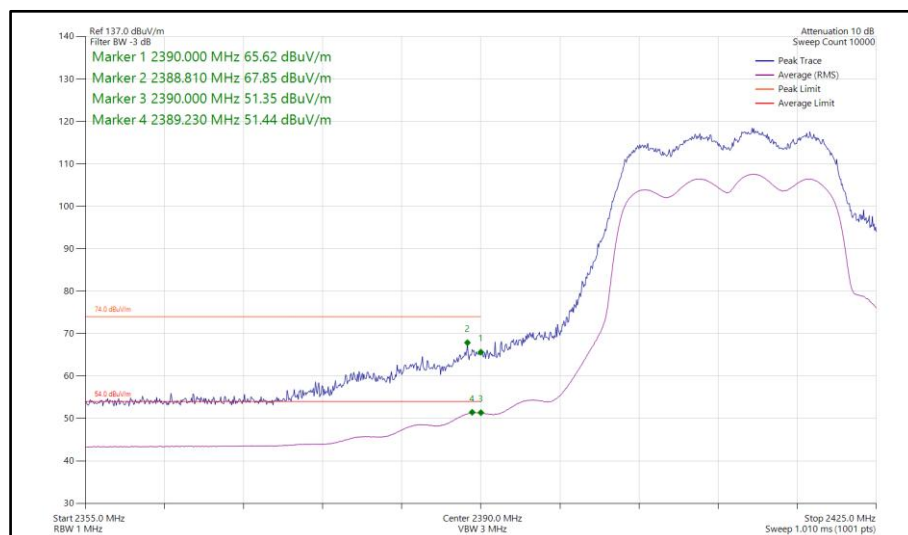
Figure 125 - 802.11ax HE20, SU, CDD, Core 0-1 - 2412 MHz Band Edge Frequency 2390 MHz
