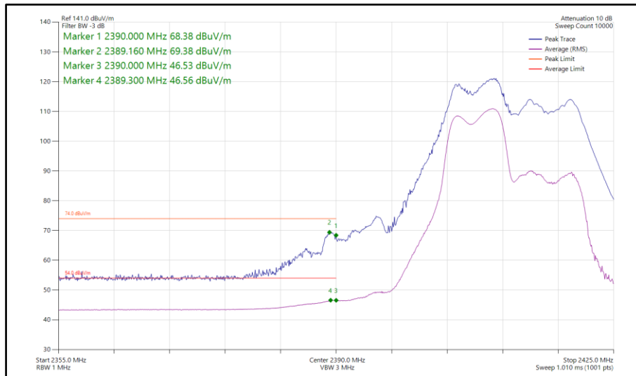
Figure 132 - 802.11be EHT20, RU 52+26-70, CDD, Core 0-1 - 2412 MHz Band Edge Frequency 2390 MHz
