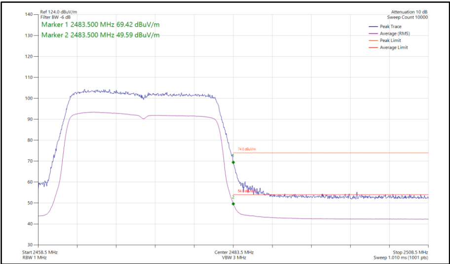
Figure 108 - 802.11ax HE20, SU, SISO, Core 1 - 2472 MHz Band Edge Frequency 2483.5 MHz
