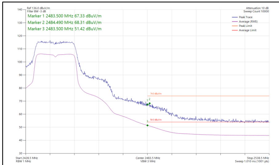
Figure 91 - 802.11n HT20, SISO, Core 1 - 2442 MHz Band Edge Frequency 2483.5 MHz
