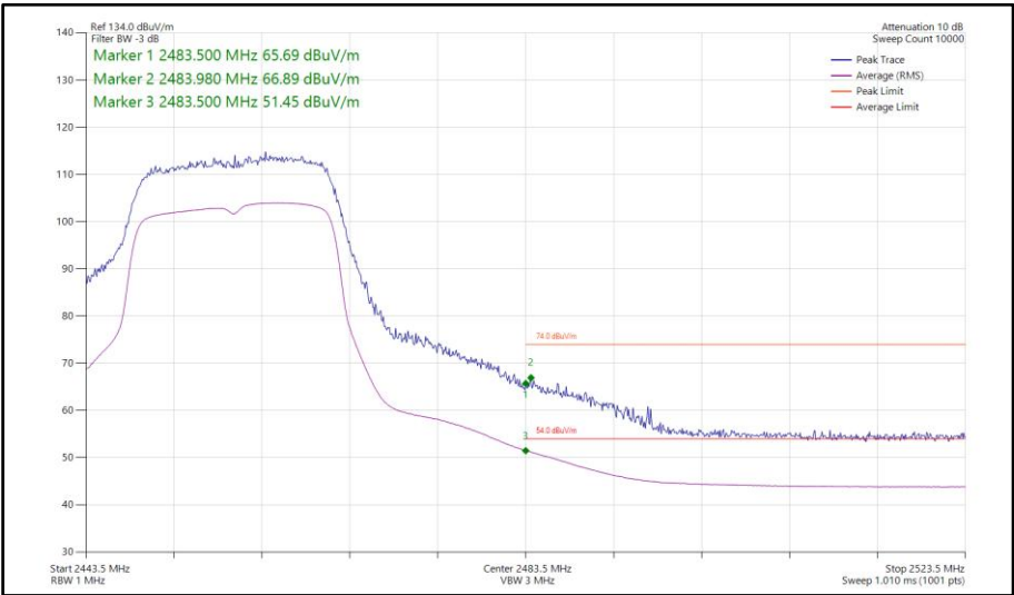
Figure 94 - 802.11n HT20, SISO, Core 1 - 2457 MHz Band Edge Frequency 2483.5 MHz
