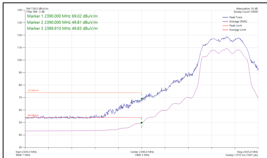
Figure 122 - 802.11n HT20, CDD, Core 0-1 - 2422 MHz Band Edge Frequency 2390 MHz
