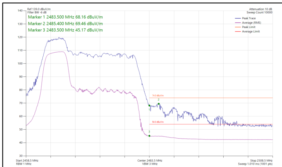
Figure 109 - 802.11ax HE20, RU 52-37, SISO, Core 1 - 2472 MHz Band Edge Frequency 2483.5 MHz
