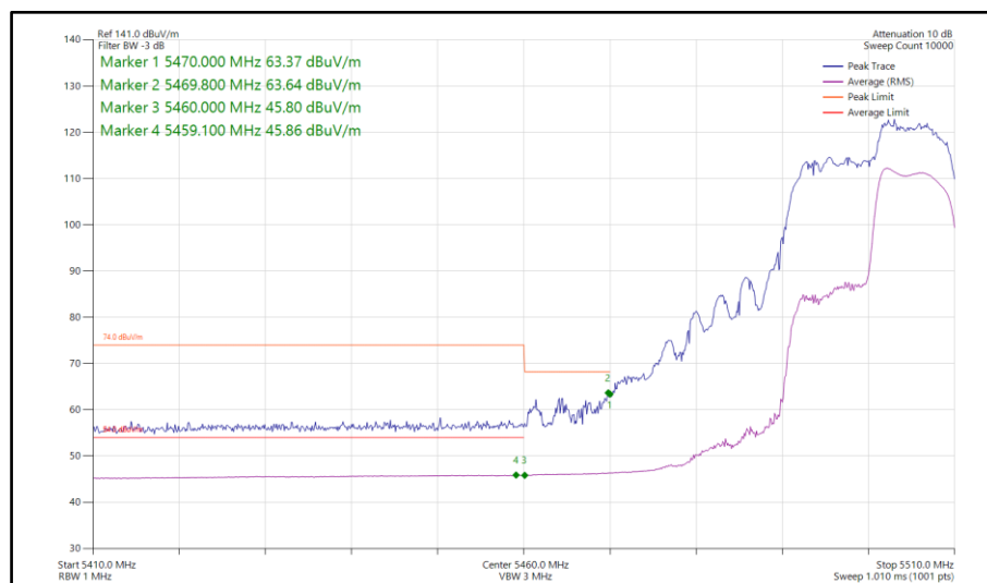
Figure 712 - 802.11ax HE20, RU 106-54, SDM, Core 0-1 - 5500 MHz Band Edge Frequency 5470 MHz
