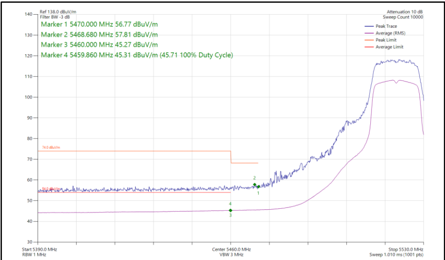
Figure 648 - 802.11a, SISO, Core 1 - 5520 MHz Band Edge Frequency 5470 MHz
