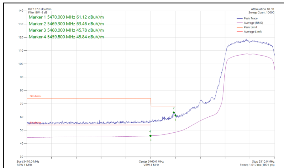
Figure 651 - 802.11ax HE20, SU, SISO, Core 1 - 5500 MHz Band Edge Frequency 5470 MHz
