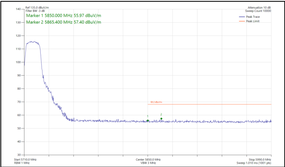
Figure 668 - 802.11a, SISO, Core 1 - 5720 MHz Band Edge Frequency 5850 MHz
