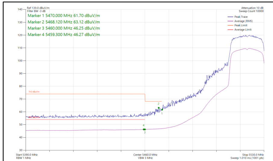
Figure 713 - 802.11ax HE20, SU, SDM, Core 0-1 - 5520 MHz Band Edge Frequency 5470 MHz
