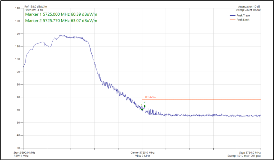
Figure 698 - 802.11be EHT20, RU 106+26-83, CDD, Core 0-1 - 5700 MHz Band Edge Frequency 5725 MHz
