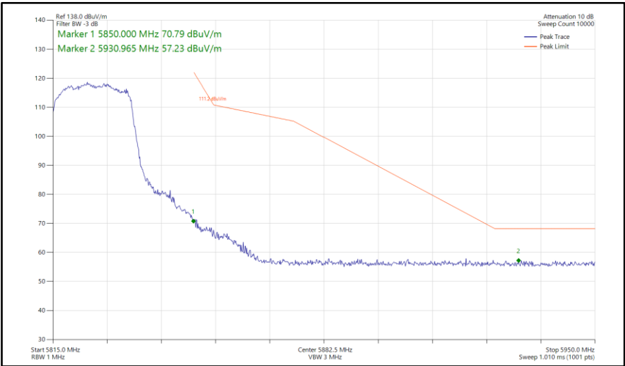
Figure 705 - 802.11ax HE20, SU, CDD, Core 0-1 - 5825 MHz Band Edge Frequency 5850 MHz
