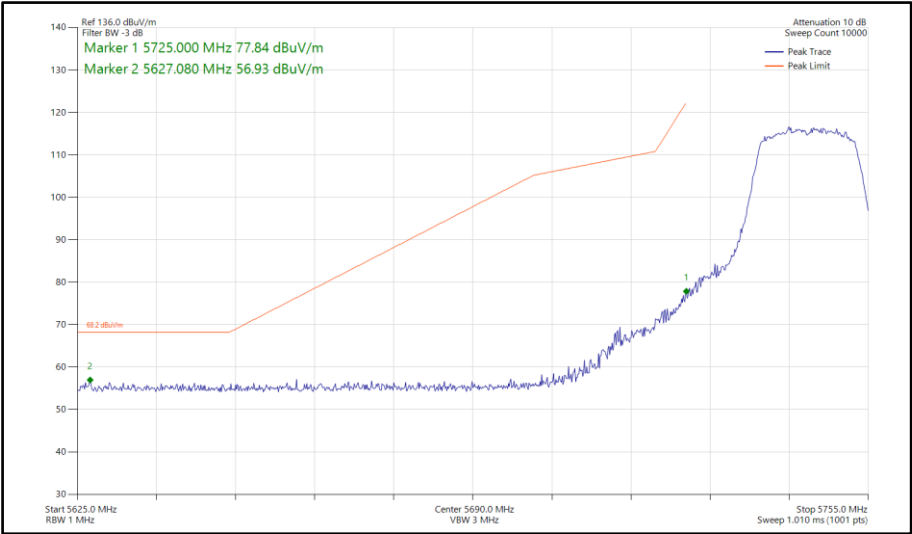
Figure 655 - 802.11a, SISO, Core 1 - 5745 MHz Band Edge Frequency 5725 MHz
