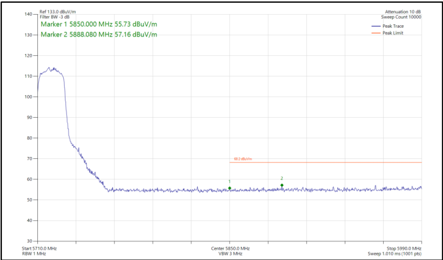
Figure 641 - 802.11ax HE20, SU, SISO, Core 0 - 5720 MHz Band Edge Frequency 5850 MHz
