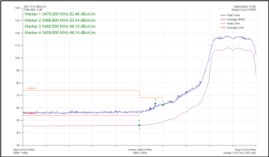
Figure 680 - 802.11n HT20, CDD, Core 0-1 - 5500 MHz Band Edge Frequency 5470 MHz
