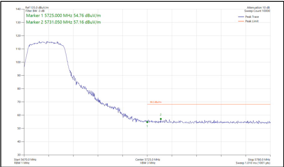
Figure 660 - 802.11a, SISO, Core 1 - 5680 MHz Band Edge Frequency 5725 MHz
