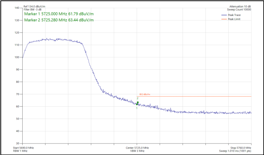
Figure 663 - 802.11n HT20, SISO, Core 1 - 5700 MHz Band Edge Frequency 5725 MHz
