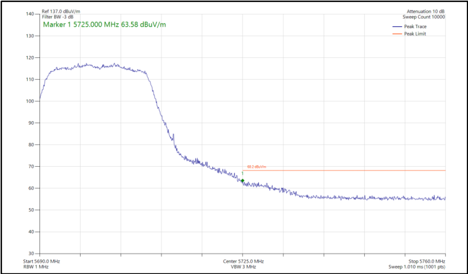
Figure 694 - 802.11n HT20, CDD, Core 0-1 - 5700 MHz Band Edge Frequency 5725 MHz
