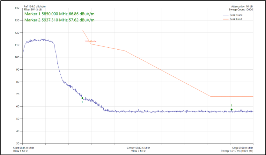
Figure 640 - 802.11n HT20, SISO, Core 0 - 5825 MHz Band Edge Frequency 5850 MHz
