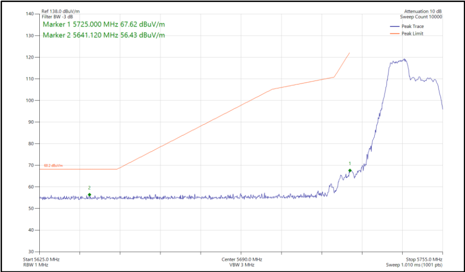
Figure 659 - 802.11be EHT20, RU 52+26-70, SISO, Core 1 - 5745 MHz Band Edge Frequency 5725 MHz
