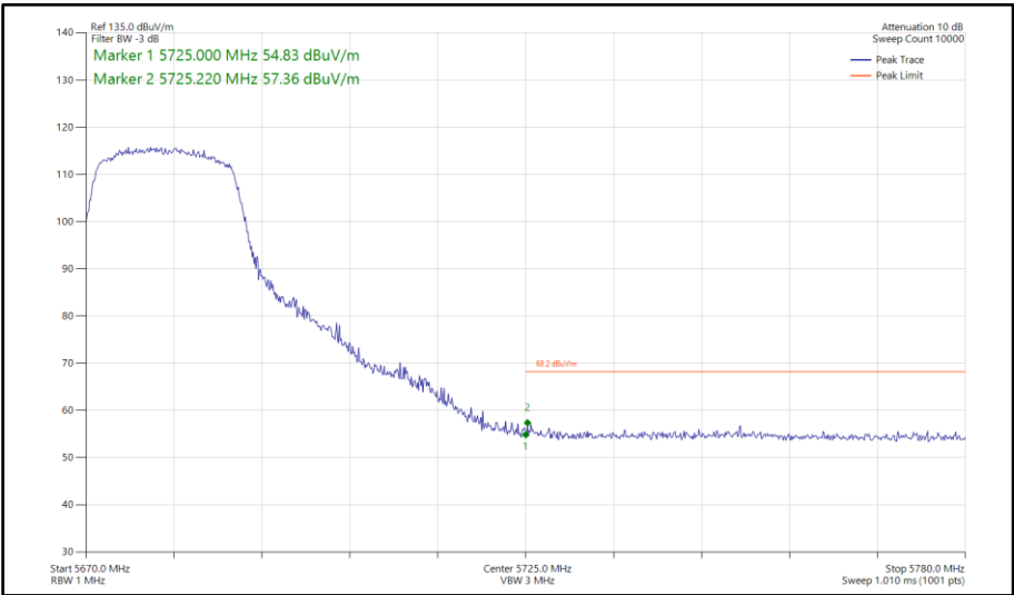
Figure 662 - 802.11n HT20, SISO, Core 1 - 5680 MHz Band Edge Frequency 5725 MHz
