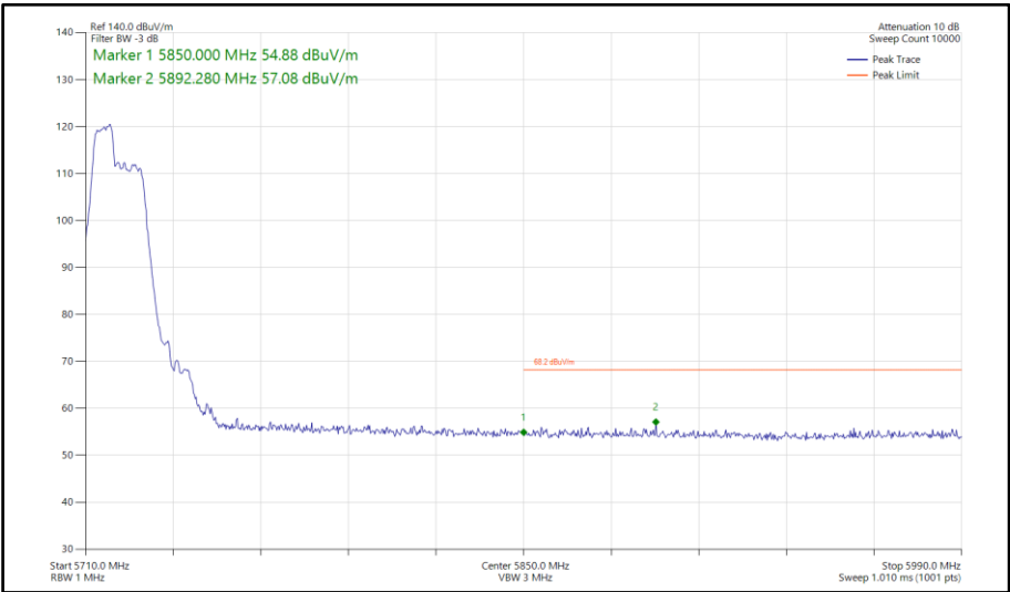
Figure 707 - 802.11be EHT20, RU 52+26-70, CDD, Core 0-1 - 5720 MHz Band Edge Frequency 5850 MHz
