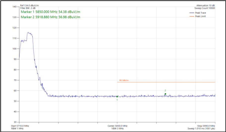
Figure 642 - 802.11ax HE20, RU 106-54, SISO, Core 0 - 5720 MHz Band Edge Frequency 5850 MHz
