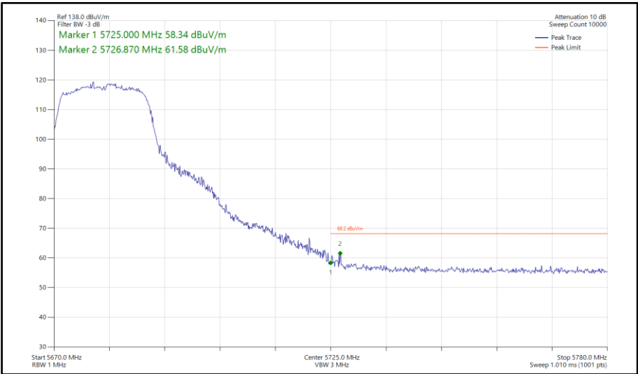
Figure 693 - 802.11n HT20, CDD, Core 0-1 - 5680 MHz Band Edge Frequency 5725 MHz
