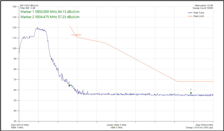
Figure 675 - 802.11ax HE20, RU 106-54, SISO, Core 1 - 5825 MHz Band Edge Frequency 5850 MHz
