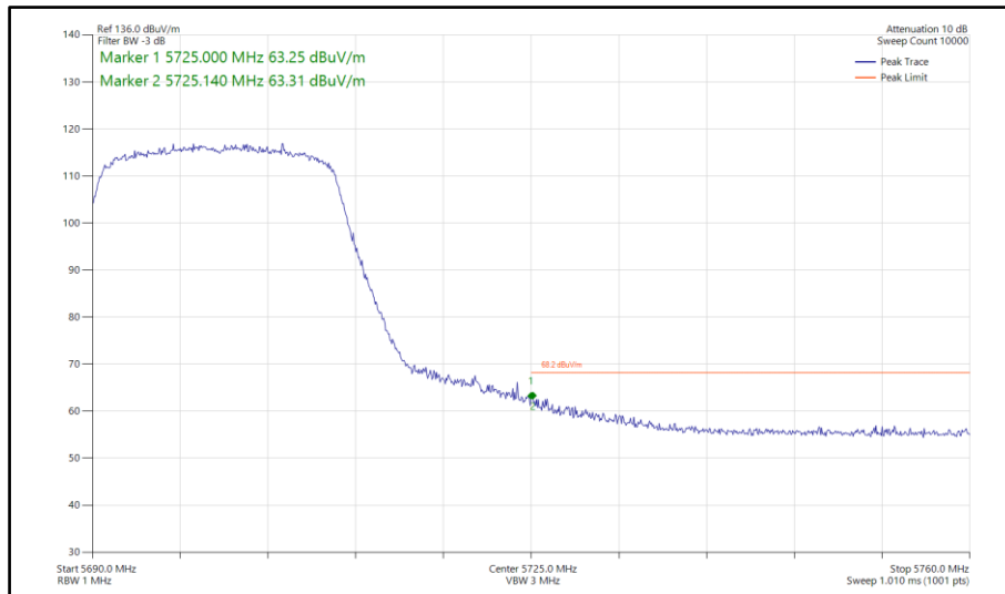
Figure 634 - 802.11ax HE20, SU, SISO, Core 0 - 5700 MHz Band Edge Frequency 5725 MHz
