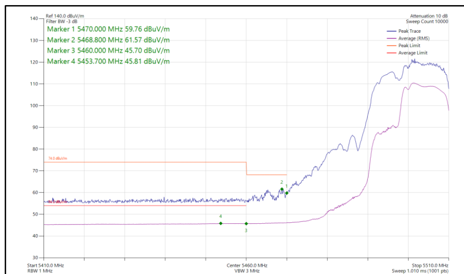
Figure 685 - 802.11be EHT20, RU 106+26-83, CDD, Core 0-1 - 5500 MHz Band Edge Frequency 5470 MHz
