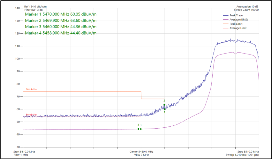
Figure 649 - 802.11n HT20, SISO, Core 1 - 5500 MHz Band Edge Frequency 5470 MHz
