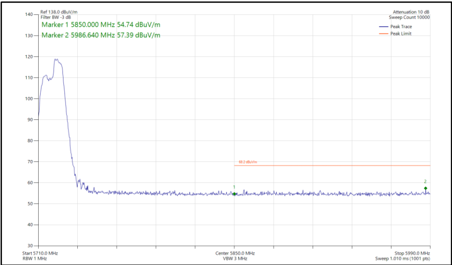
Figure 676 - 802.11be EHT20, RU 52+26-72, SISO, Core 1 - 5720 MHz Band Edge Frequency 5850 MHz
