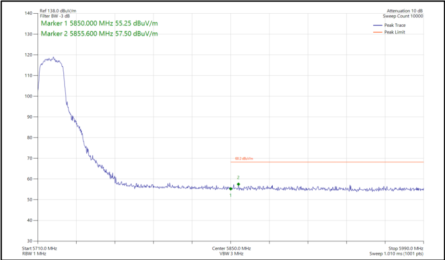
Figure 701 - 802.11n HT20, CDD, Core 0-1 - 5720 MHz Band Edge Frequency 5850 MHz
