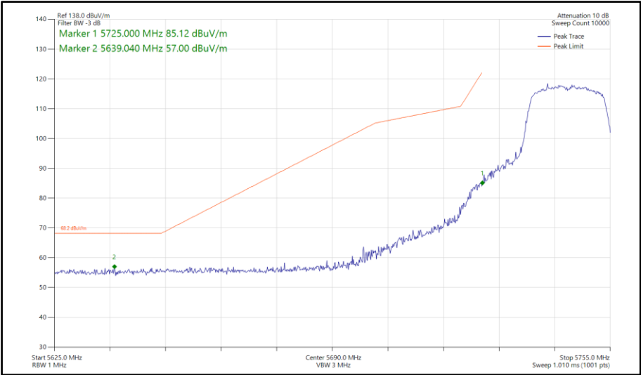
Figure 715 - 802.11n HT20, SDM, Core 0-1 - 5745 MHz Band Edge Frequency 5725 MHz
