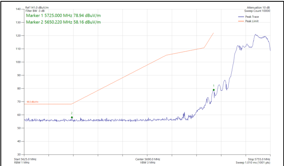
Figure 689 - 802.11ax HE20, RU 106-54, CDD, Core 0-1 - 5745 MHz Band Edge Frequency 5725 MHz
