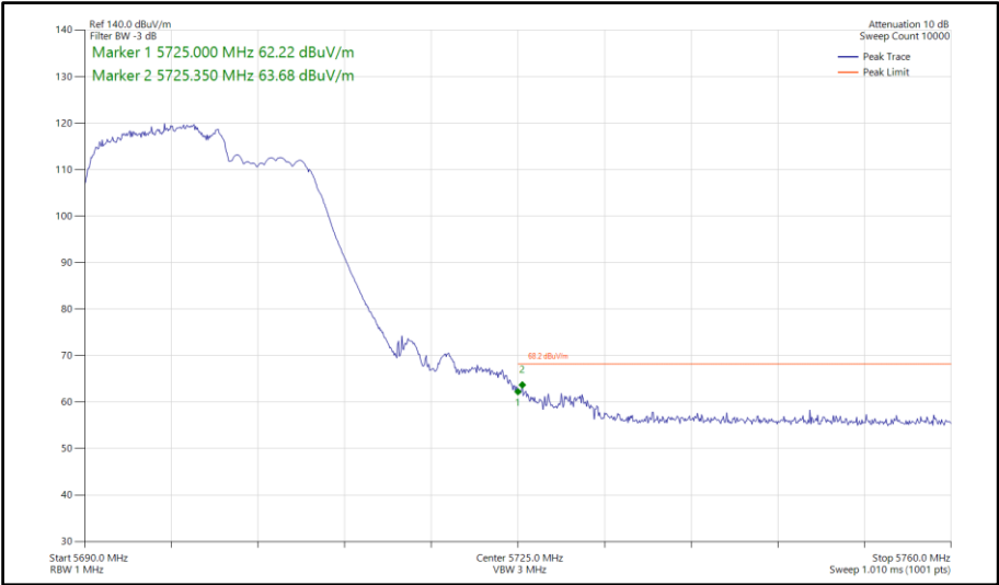
Figure 636 - 802.11be EHT20, RU 106+26-82, SISO, Core 0 - 5700 MHz Band Edge Frequency 5725 MHz
