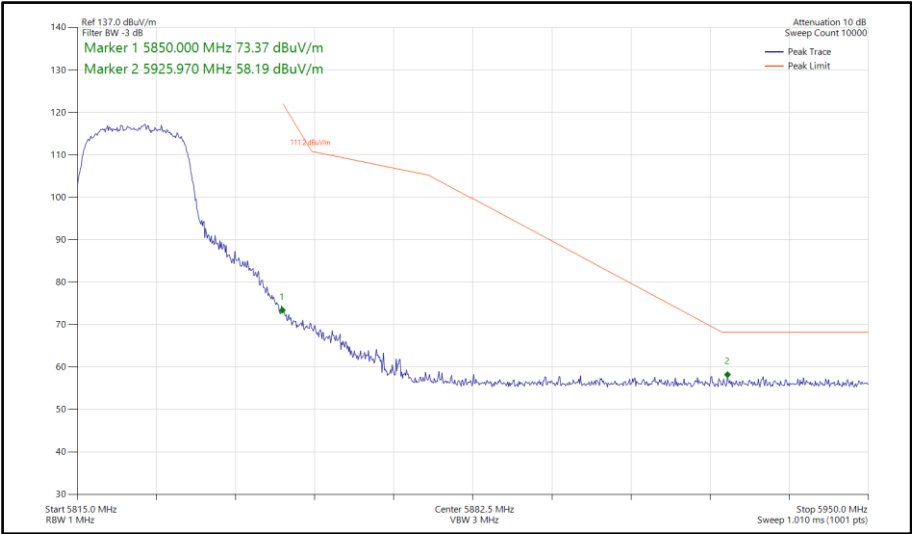
Figure 702 - 802.11n HT20, CDD, Core 0-1 - 5825 MHz Band Edge Frequency 5850 MHz
