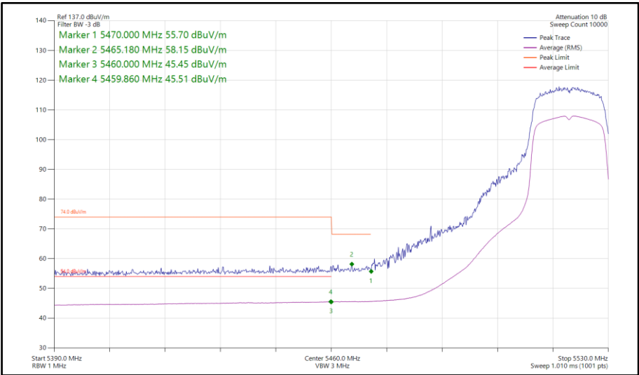
Figure 650 - 802.11n HT20, SISO, Core 1 - 5520 MHz Band Edge Frequency 5470 MHz
