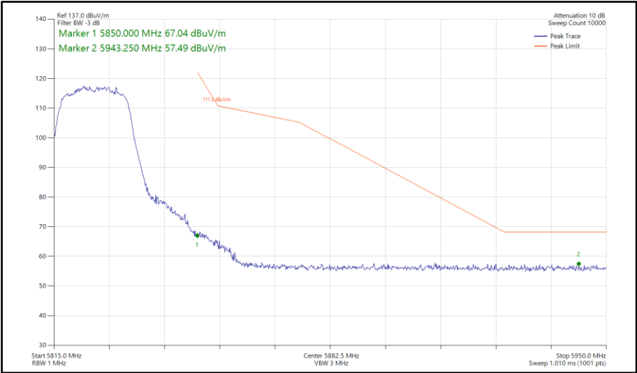
Figure 700 - 802.11a, CDD, Core 0-1 - 5825 MHz Band Edge Frequency 5850 MHz
