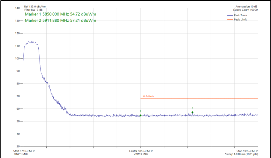
Figure 639 - 802.11n HT20, SISO, Core 0 - 5720 MHz Band Edge Frequency 5850 MHz
