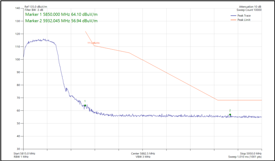
Figure 671 - 802.11n HT20, SISO, Core 1 - 5825 MHz Band Edge Frequency 5850 MHz
