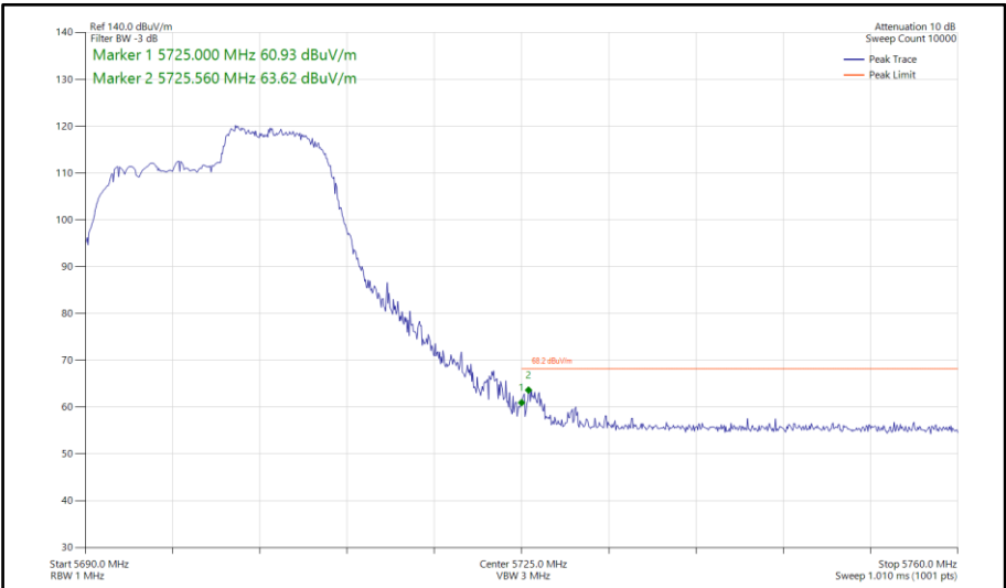
Figure 697 - 802.11ax HE20, RU 106-54, CDD, Core 0-1 - 5700 MHz Band Edge Frequency 5725 MHz
