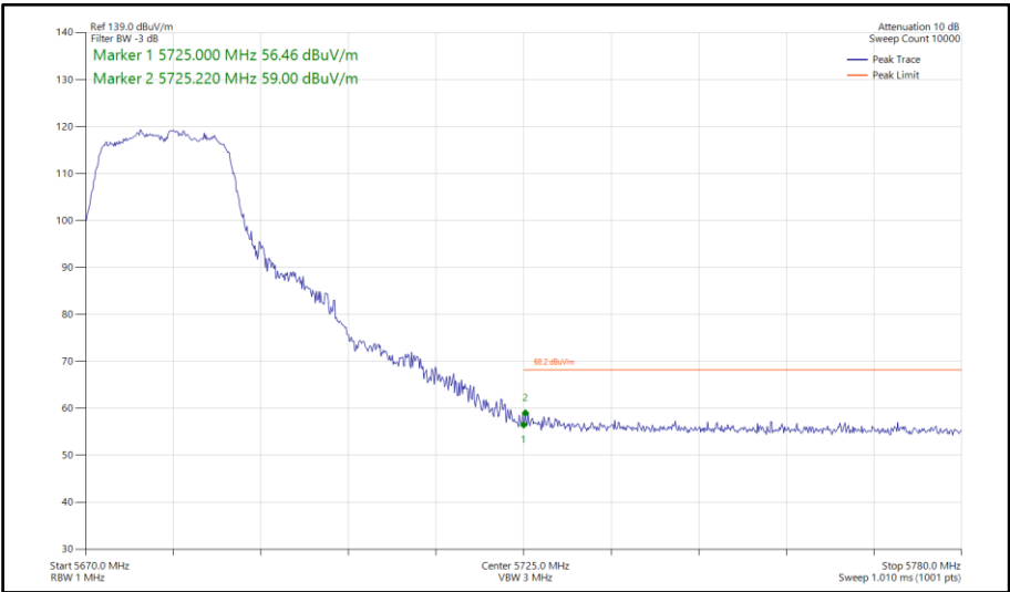
Figure 691 - 802.11a, CDD, Core 0-1 - 5680 MHz Band Edge Frequency 5725 MHz
