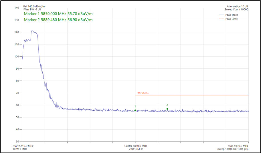
Figure 704 - 802.11ax HE20, RU 106-54, CDD, Core 0-1 - 5720 MHz Band Edge Frequency 5850 MHz
