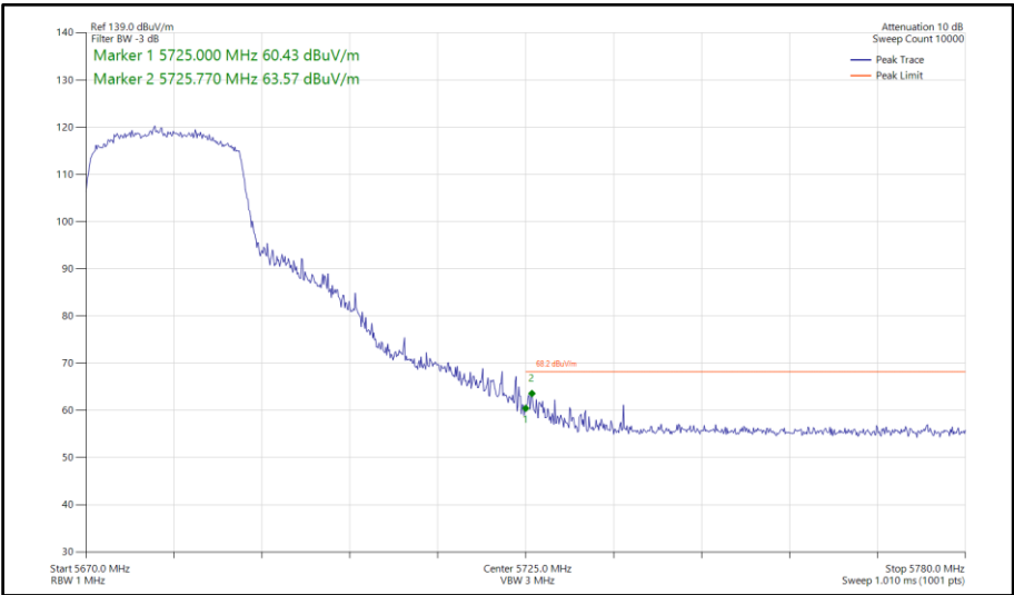
Figure 695 - 802.11ax HE20, SU, CDD, Core 0-1 - 5680 MHz Band Edge Frequency 5725 MHz
