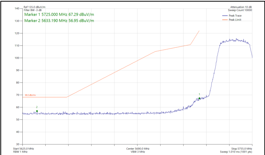
Figure 656 - 802.11n HT20, SISO, Core 1 - 5745 MHz Band Edge Frequency 5725 MHz
