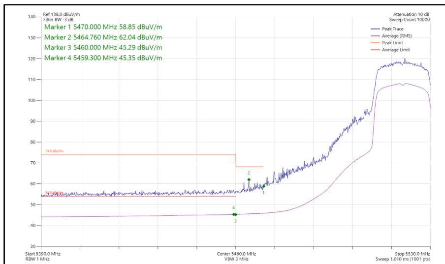
Figure 653 - 802.11ax HE20, SU, SISO, Core 1 - 5520 MHz Band Edge Frequency 5470 MHz
