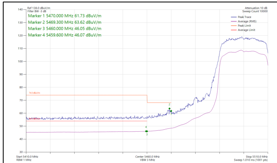
Figure 682 - 802.11ax HE20, SU, CDD, Core 0-1 - 5500 MHz Band Edge Frequency 5470 MHz
