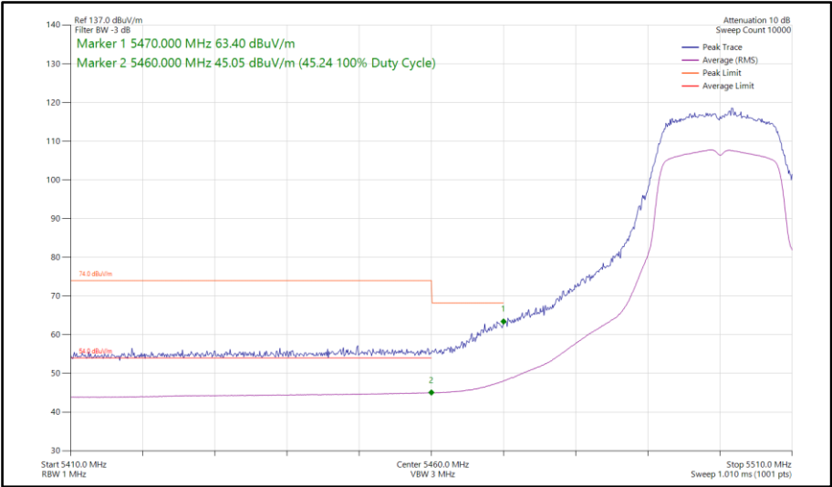
Figure 647 - 802.11a, SISO, Core 1 - 5500 MHz Band Edge Frequency 5470 MHz
