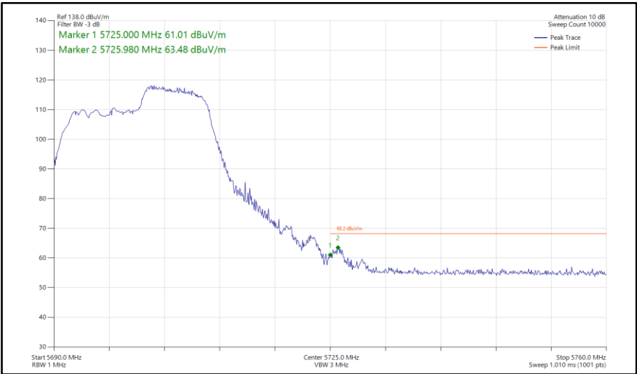
Figure 666 - 802.11ax HE20, RU 106-54, SISO, Core 1 - 5700 MHz Band Edge Frequency 5725 MHz
