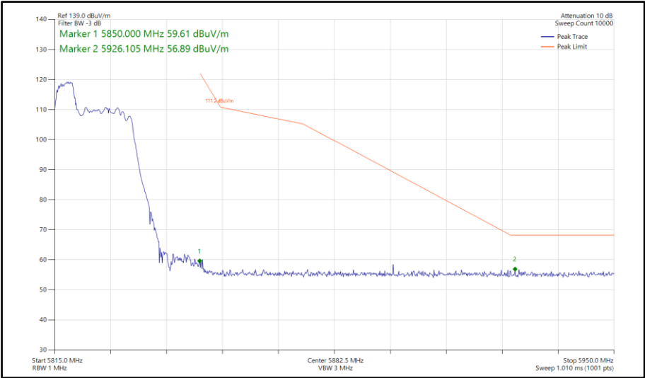
Figure 644 - 802.11ax HE20, RU 52-37, SISO, Core 0 - 5825 MHz Band Edge Frequency 5850 MHz
