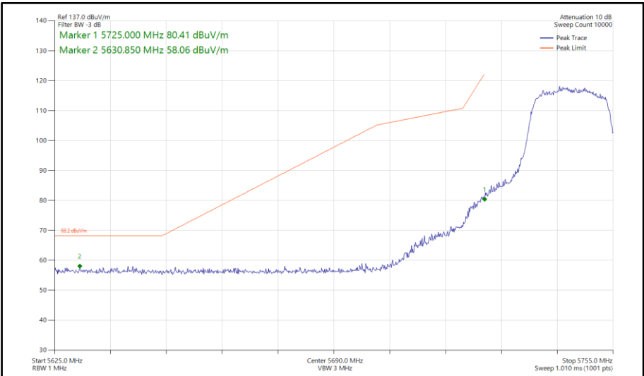
Figure 687 - 802.11n HT20, CDD, Core 0-1 - 5745 MHz Band Edge Frequency 5725 MHz
