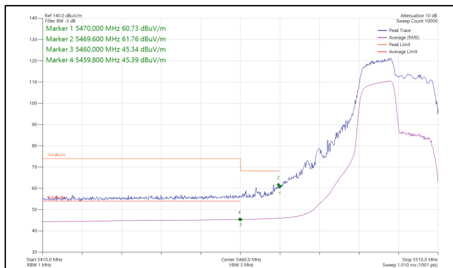
Figure 652 - 802.11ax HE20, RU 106-53, SISO, Core 1 - 5500 MHz Band Edge Frequency 5470 MHz
