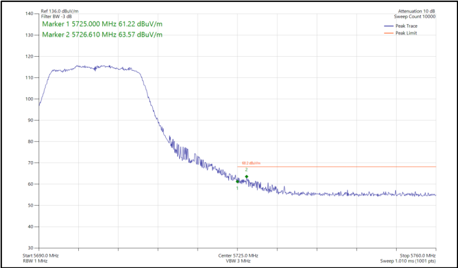
Figure 692 - 802.11a, CDD, Core 0-1 - 5700 MHz Band Edge Frequency 5725 MHz
