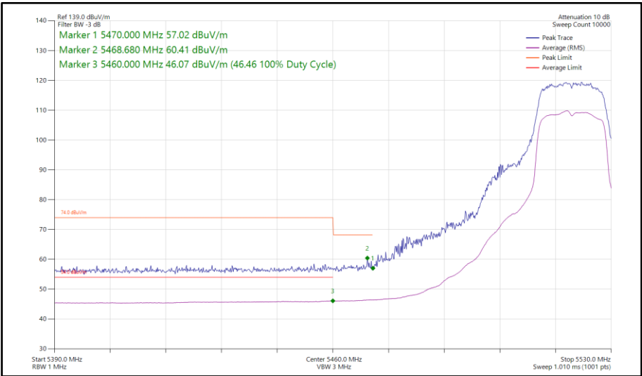
Figure 679 - 802.11a, CDD, Core 0-1 - 5520 MHz Band Edge Frequency 5470 MHz
