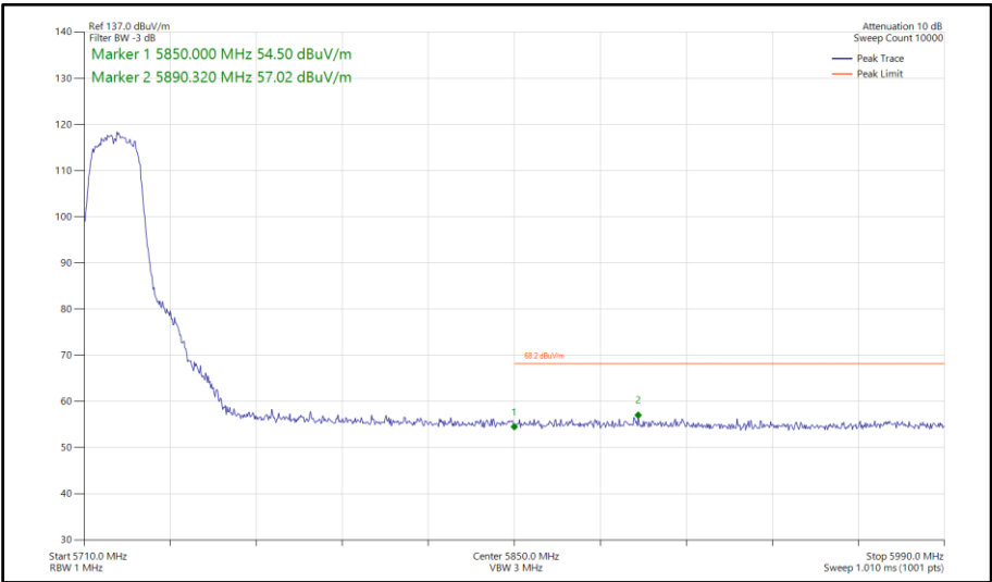
Figure 699 - 802.11a, CDD, Core 0-1 - 5720 MHz Band Edge Frequency 5850 MHz
