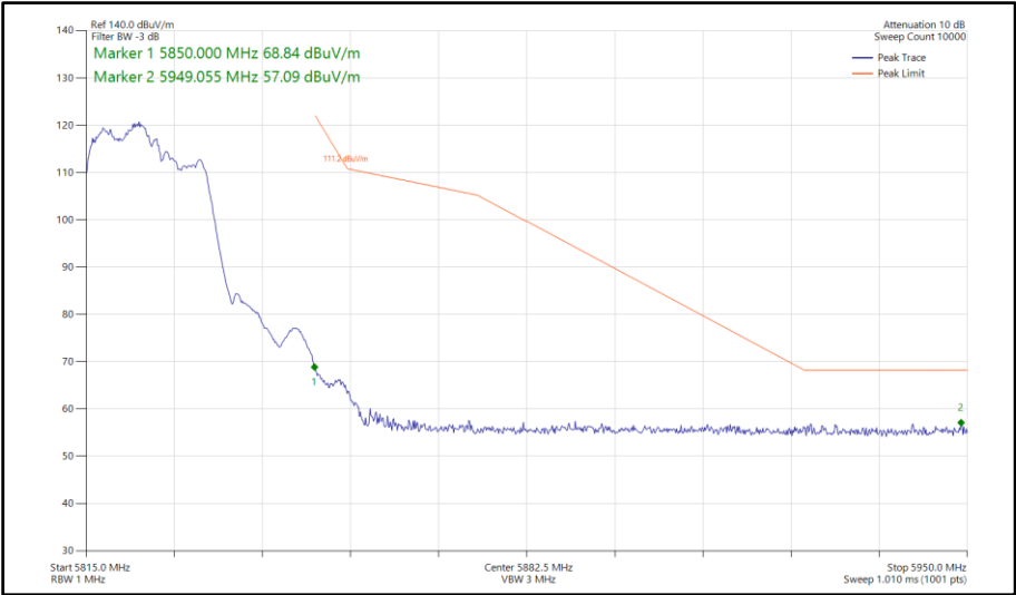
Figure 708 - 802.11be EHT20, RU 106+26-82, CDD, Core 0-1 - 5825 MHz Band Edge Frequency 5850 MHz
