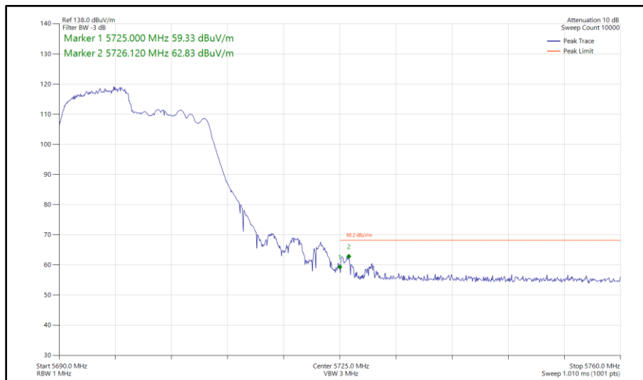
Figure 635 - 802.11ax HE20, RU 106-53, SISO, Core 0 - 5700 MHz Band Edge Frequency 5725 MHz
