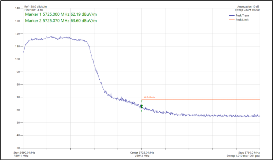
Figure 696 - 802.11ax HE20, SU, CDD, Core 0-1 - 5700 MHz Band Edge Frequency 5725 MHz
