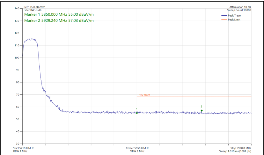
Figure 670 - 802.11n HT20, SISO, Core 1 - 5720 MHz Band Edge Frequency 5850 MHz
