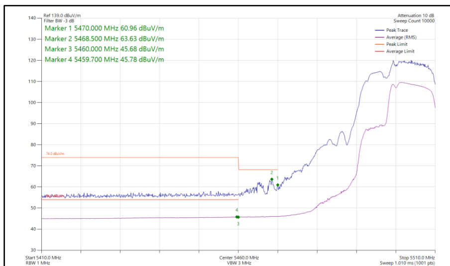
Figure 654 - 802.11be EHT20, RU 106+26-83, SISO, Core 1 - 5500 MHz Band Edge Frequency 5470 MHz
