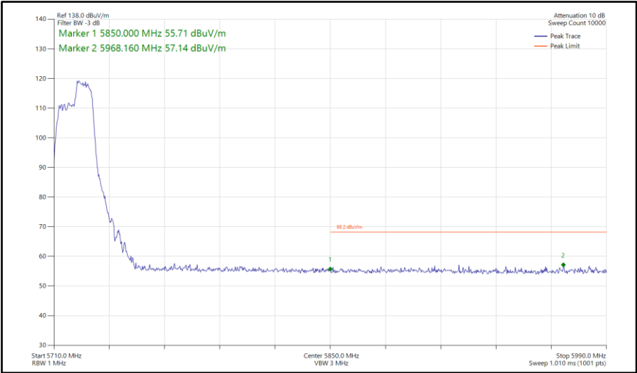
Figure 673 - 802.11ax HE20, RU 106-54, SISO, Core 1 - 5720 MHz Band Edge Frequency 5850 MHz
