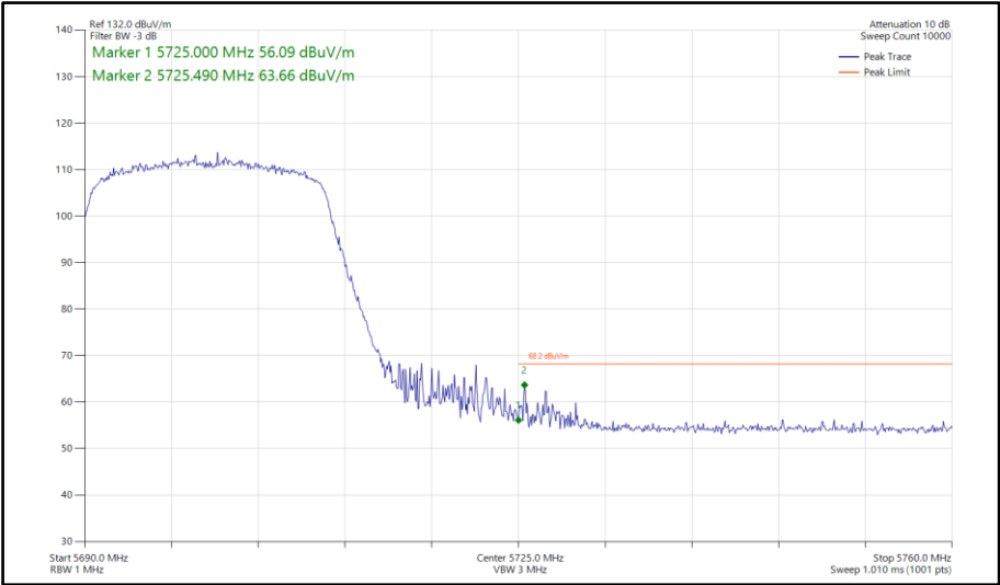
Figure 665 - 802.11ax HE20, SU, SISO, Core 1 - 5700 MHz Band Edge Frequency 5725 MHz
