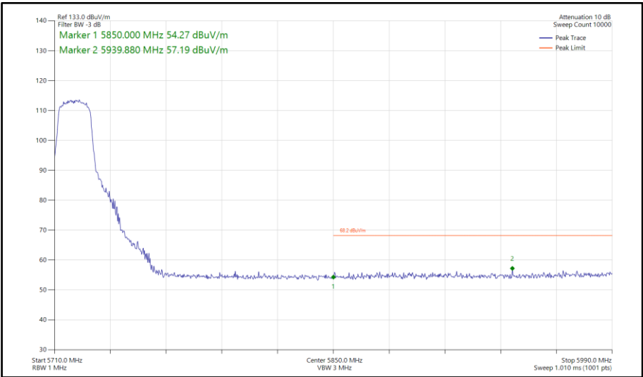
Figure 637 - 802.11a, SISO, Core 0 - 5720 MHz Band Edge Frequency 5850 MHz
