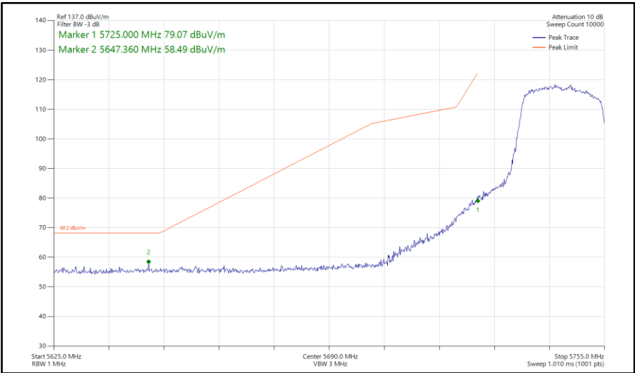
Figure 716 - 802.11ax HE20, SU, SDM, Core 0-1 - 5745 MHz Band Edge Frequency 5725 MHz
