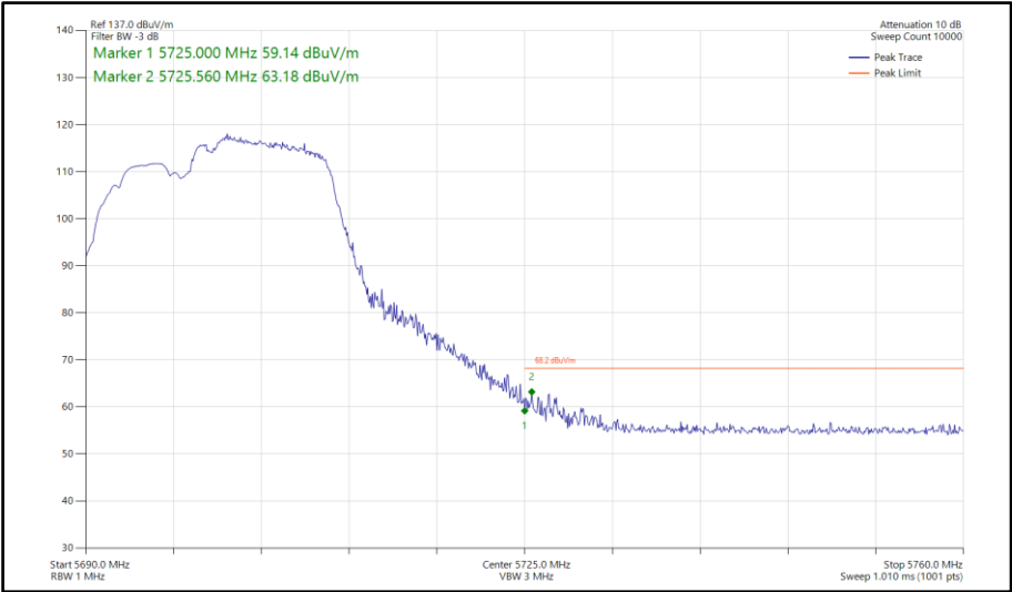
Figure 667 - 802.11be EHT20, RU 106+26-83, SISO, Core 1 - 5700 MHz Band Edge Frequency 5725 MHz
