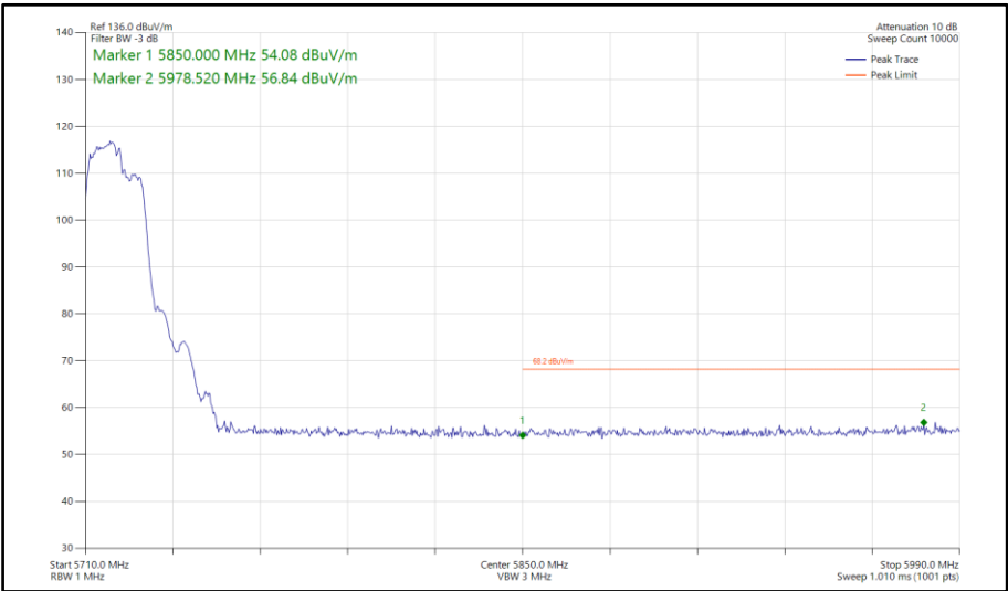
Figure 645 - 802.11be EHT20, RU 106+26-82, SISO, Core 0 - 5720 MHz Band Edge Frequency 5850 MHz
