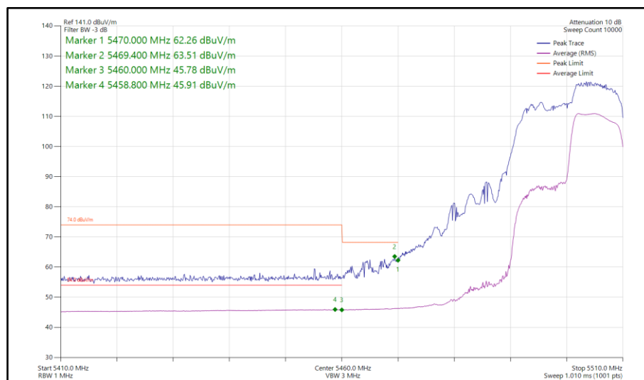
Figure 683 - 802.11ax HE20, RU 106-54, CDD, Core 0-1 - 5500 MHz Band Edge Frequency 5470 MHz
