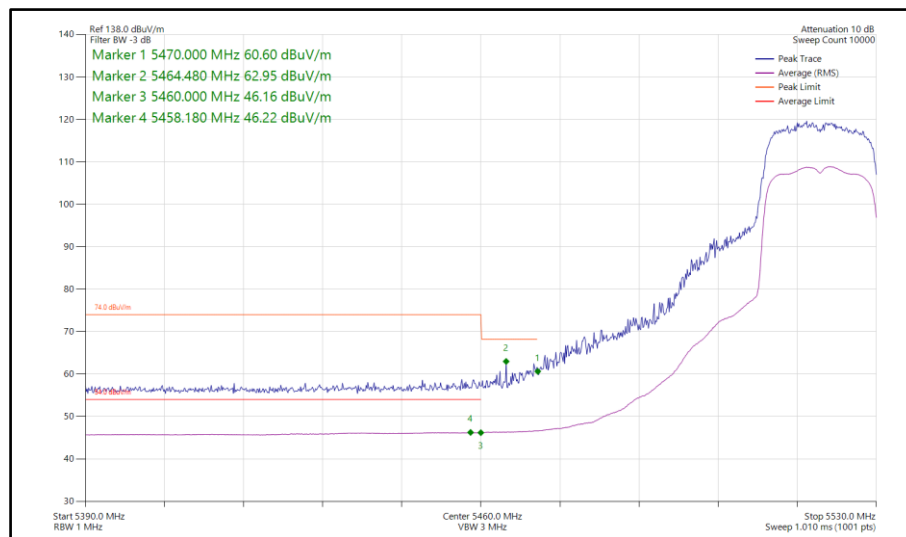
Figure 684 - 802.11ax HE20, SU, CDD, Core 0-1 - 5520 MHz Band Edge Frequency 5470 MHz
