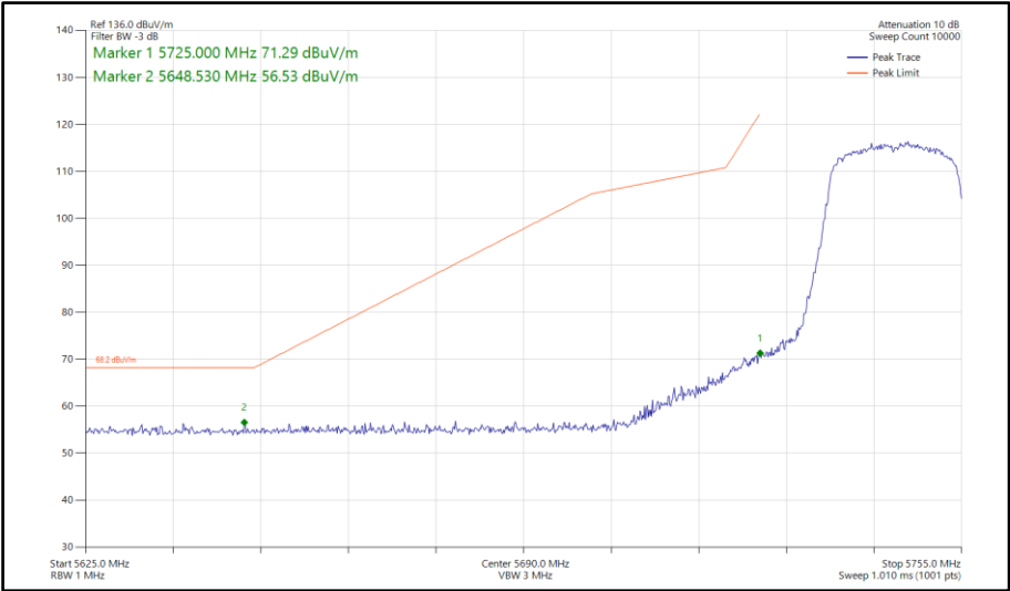
Figure 657 - 802.11ax HE20, SU, SISO, Core 1 - 5745 MHz Band Edge Frequency 5725 MHz
