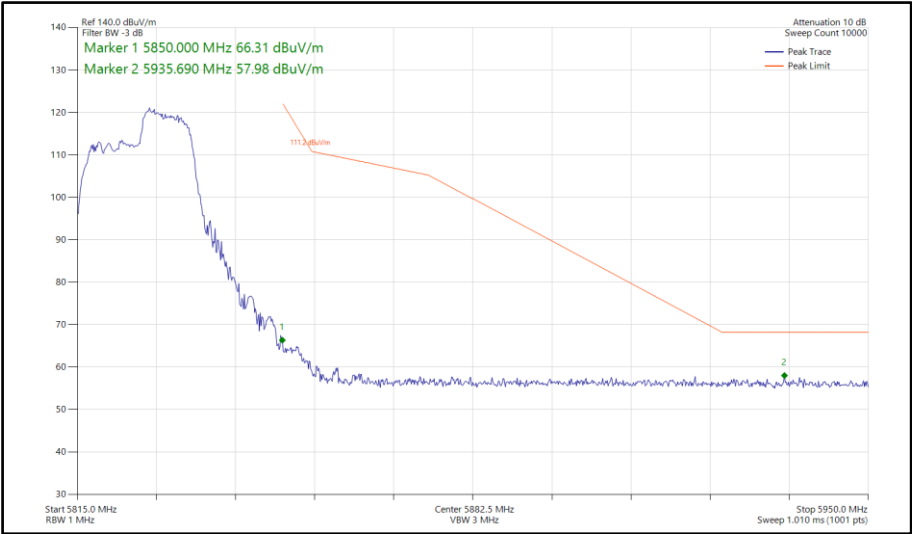
Figure 706 - 802.11ax HE20, RU 106-54, CDD, Core 0-1 - 5825 MHz Band Edge Frequency 5850 MHz
