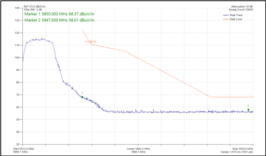
Figure 638 - 802.11a, SISO, Core 0 - 5825 MHz Band Edge Frequency 5850 MHz
