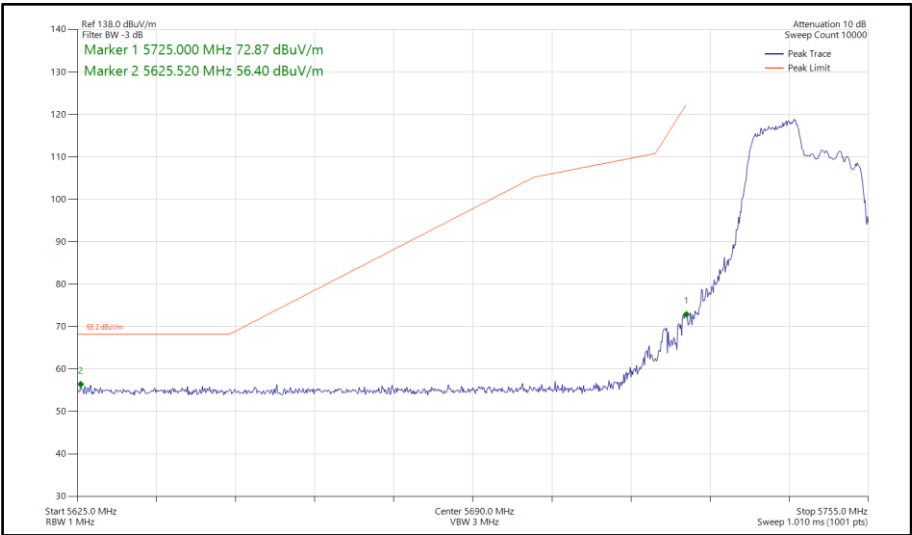
Figure 658 - 802.11ax HE20, RU 106-53, SISO, Core 1 - 5745 MHz Band Edge Frequency 5725 MHz
