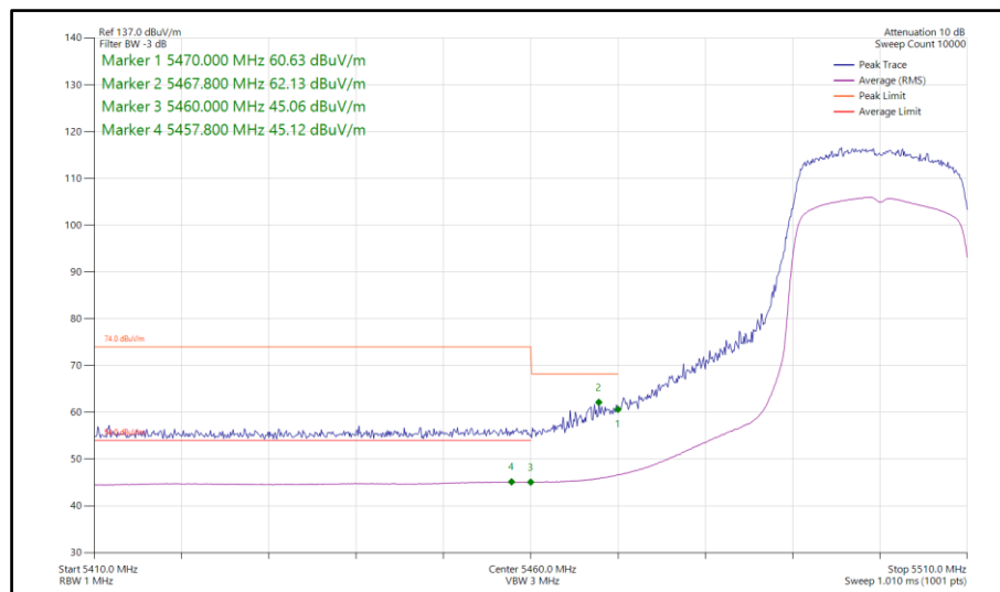
Figure 711 - 802.11ax HE20, SU, SDM, Core 0-1 - 5500 MHz Band Edge Frequency 5470 MHz
