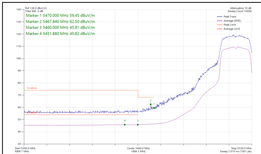
Figure 710 - 802.11n HT20, SDM, Core 0-1 - 5520 MHz Band Edge Frequency 5470 MHz
