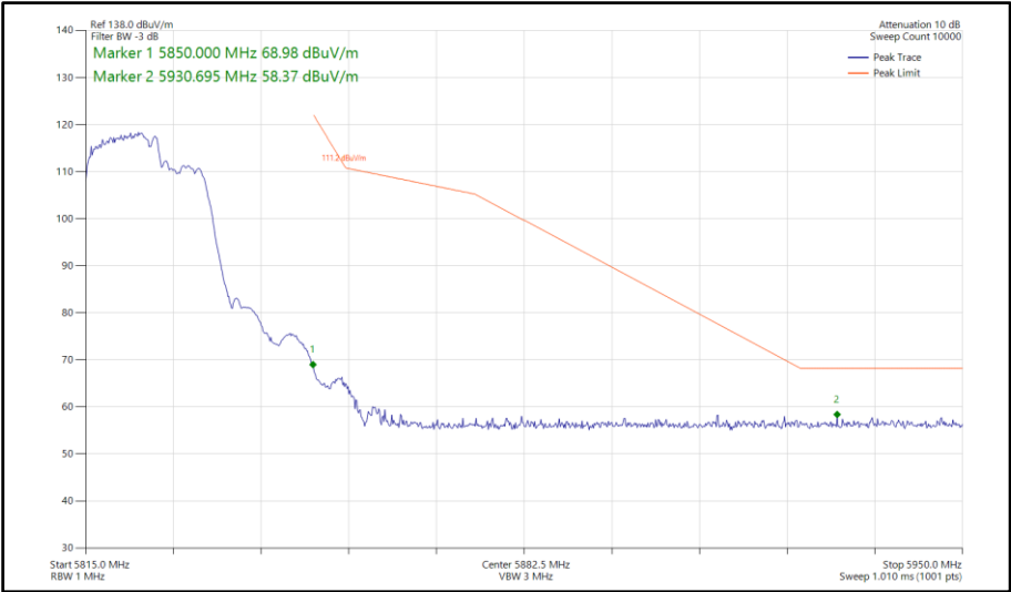
Figure 646 - 802.11be EHT20, RU 106+26-82, SISO, Core 0 - 5825 MHz Band Edge Frequency 5850 MHz
