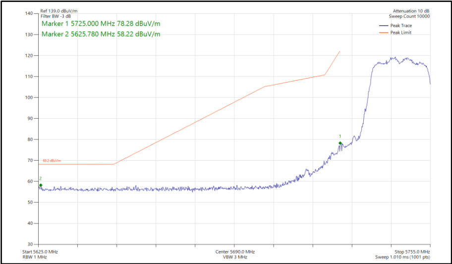
Figure 688 - 802.11ax HE20, SU, CDD, Core 0-1 - 5745 MHz Band Edge Frequency 5725 MHz
