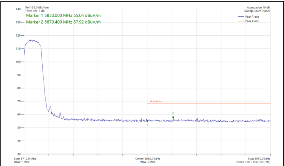
Figure 672 - 802.11ax HE20, SU, SISO, Core 1 - 5720 MHz Band Edge Frequency 5850 MHz
