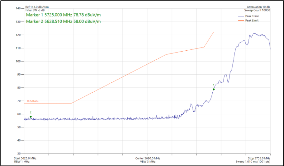
Figure 690 - 802.11be EHT20, RU106+26-83, CDD, Core 0-1 - 5745 MHz Band Edge Frequency 5725 MHz
