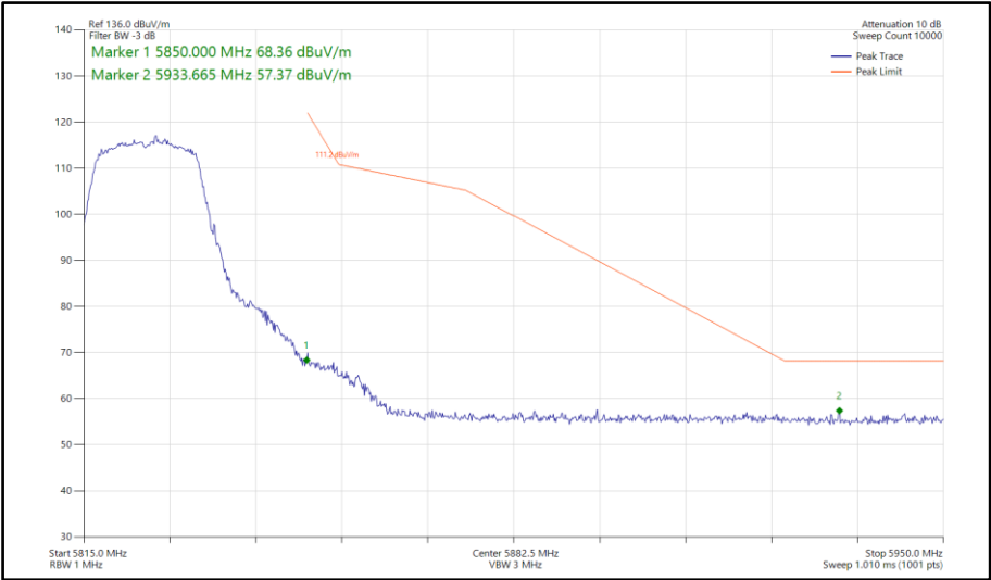
Figure 669 - 802.11a, SISO, Core 1 - 5825 MHz Band Edge Frequency 5850 MHz
