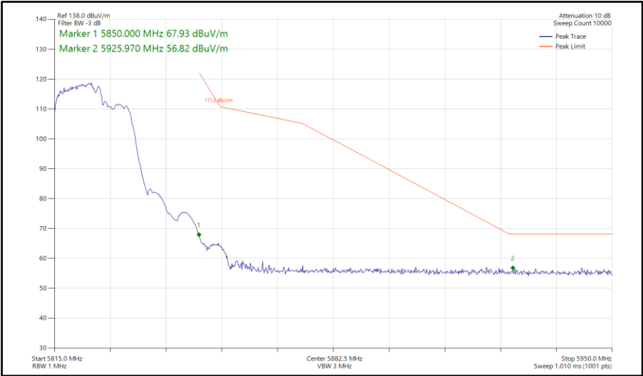
Figure 677 - 802.11be EHT20, RU 106+26-82, SISO, Core 1 - 5825 MHz Band Edge Frequency 5850 MHz
