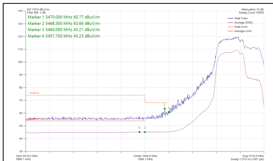
Figure 714 - 802.11be EHT20, RU 106+26-82, SDM, Core 0-1 - 5500 MHz Band Edge Frequency 5470 MHz
