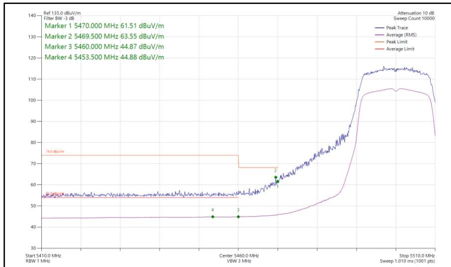
Figure 709 - 802.11n HT20, SDM, Core 0-1 - 5500 MHz Band Edge Frequency 5470 MHz
