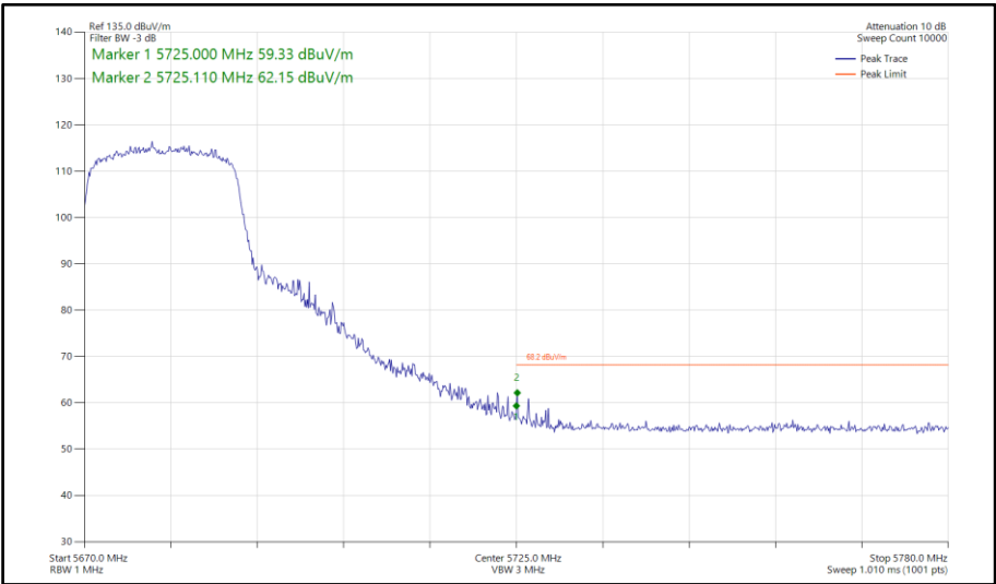
Figure 664 - 802.11ax HE20, SU, SISO, Core 1 - 5680 MHz Band Edge Frequency 5725 MHz
