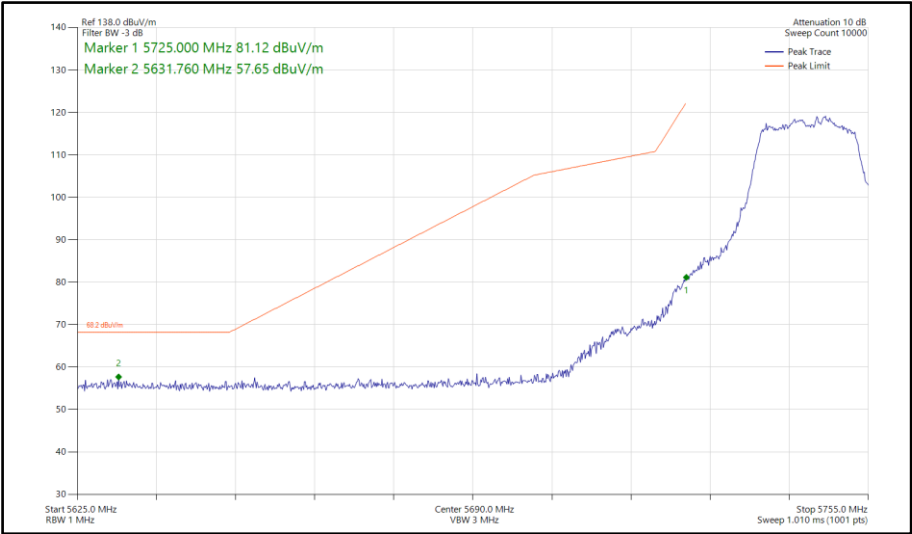
Figure 686 - 802.11a, CDD, Core 0-1 - 5745 MHz Band Edge Frequency 5725 MHz
