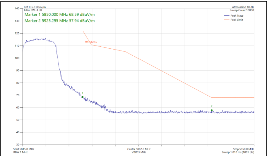
Figure 643 - 802.11ax HE20, SU, SISO, Core 0 - 5825 MHz Band Edge Frequency 5850 MHz
