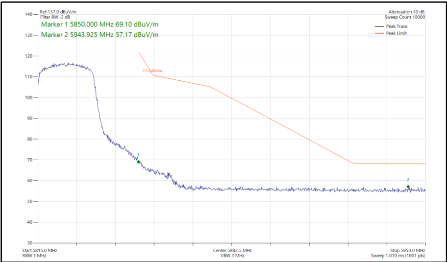
Figure 674 - 802.11ax HE20, SU, SISO, Core 1 - 5825 MHz Band Edge Frequency 5850 MHz
