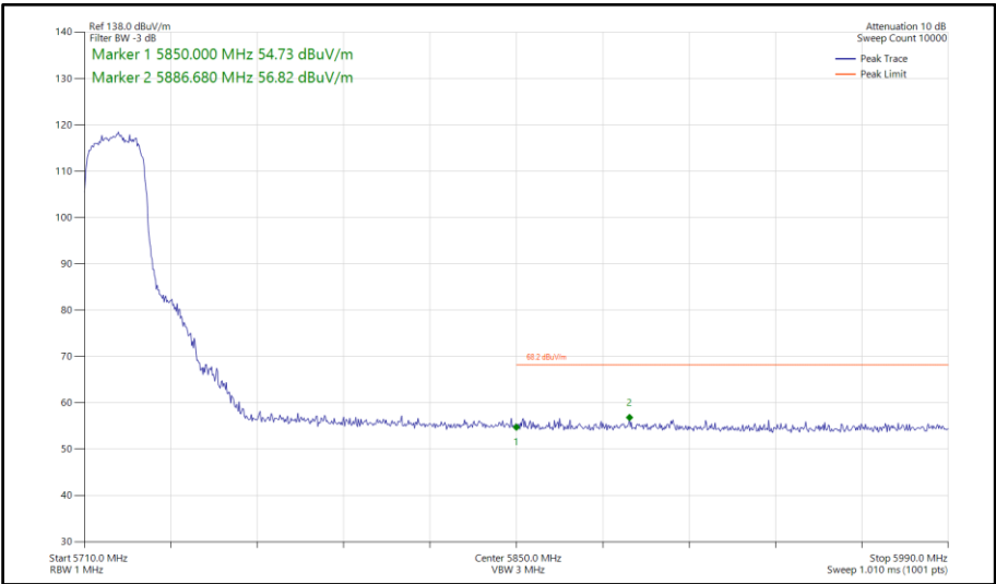
Figure 703 - 802.11ax HE20, SU, CDD, Core 0-1 - 5720 MHz Band Edge Frequency 5850 MHz
