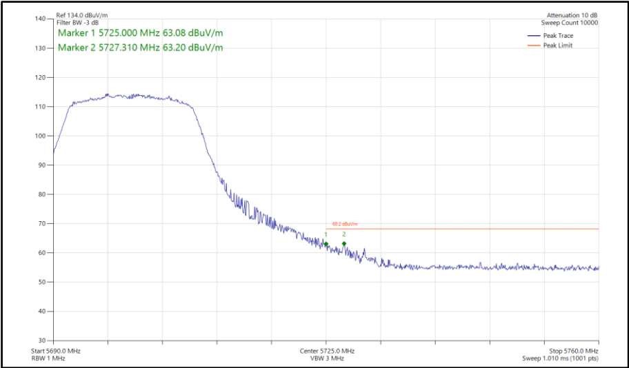
Figure 661 - 802.11a, SISO, Core 1 - 5700 MHz Band Edge Frequency 5725 MHz
