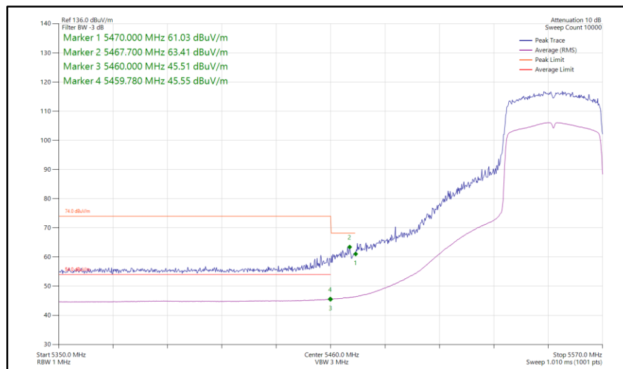
Figure 753 - 802.11ax HE40, SU, SISO, Core 0 - 5550 MHz Band Edge Frequency 5470 MHz
