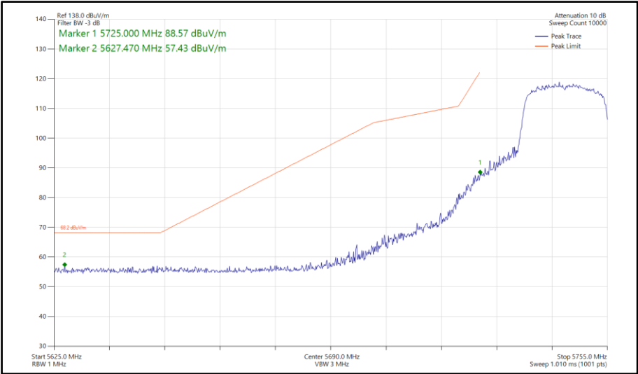
Figure 738 - 802.11ax HE20, SU, TxBF, Core 0-1 - 5745 MHz Band Edge Frequency 5725 MHz
