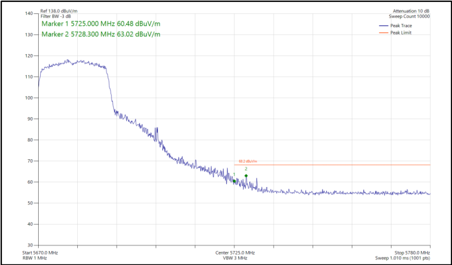
Figure 721 - 802.11ax HE20, SU, SDM, Core 0-1 - 5680 MHz Band Edge Frequency 5725 MHz
