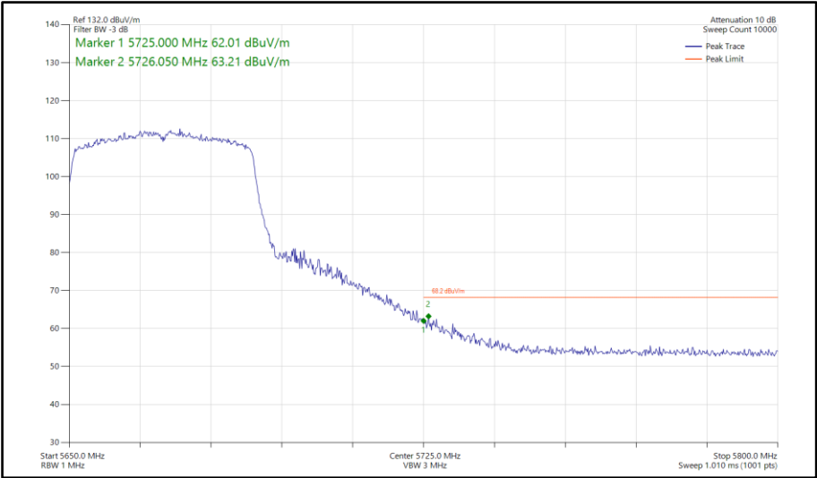
Figure 763 - 802.11ax HE40, SU, SISO, Core 0 - 5670 MHz Band Edge Frequency 5725 MHz
