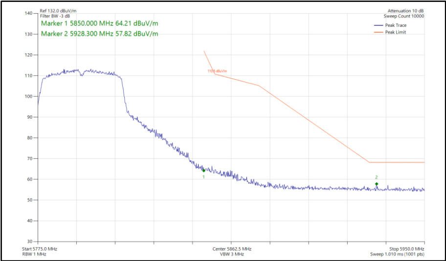
Figure 798 - 802.11n HT40, SISO, Core 1 - 5795 MHz Band Edge Frequency 5850 MHz
