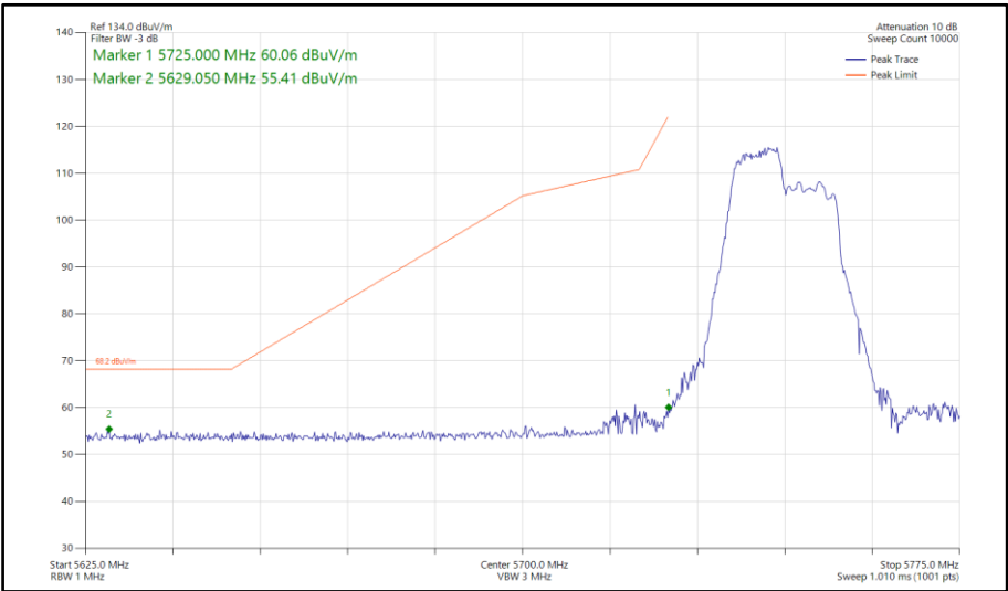
Figure 787 - 802.11ax HE40, RU 106-53, SISO, Core 1 - 5755 MHz Band Edge Frequency 5725 MHz
