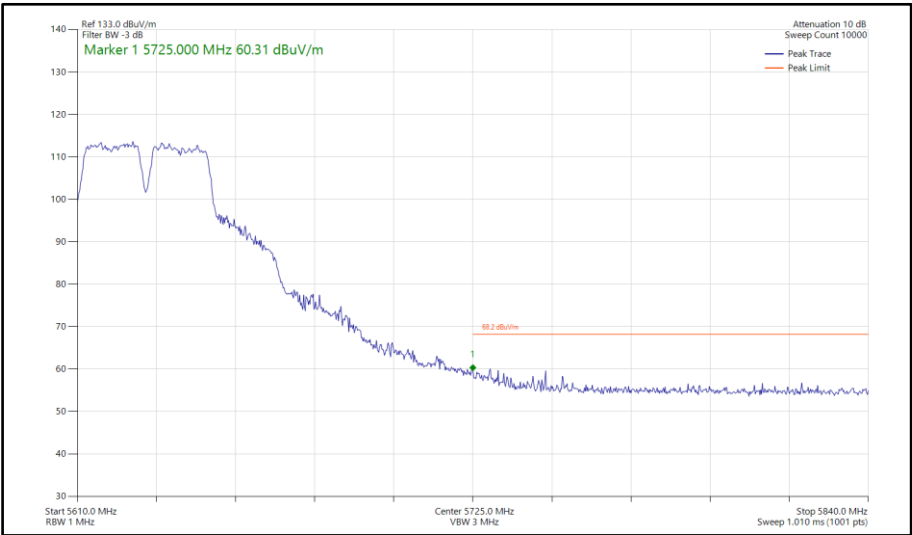
Figure 789 - 802.11a a40, SISO, Core 1 - 5630 MHz Band Edge Frequency 5725 MHz
