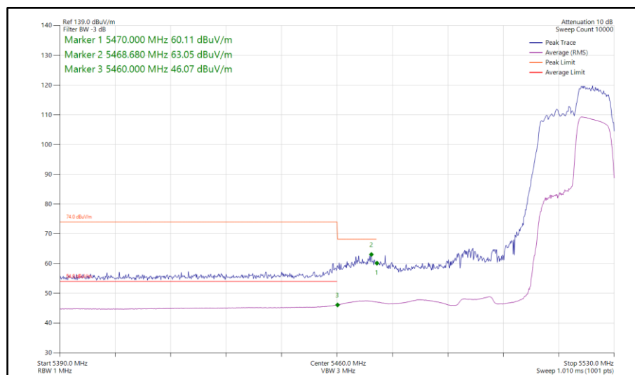
Figure 752 - 802.11ax HE40, RU 106-56, SISO, Core 0 - 5510 MHz Band Edge Frequency 5470 MHz
