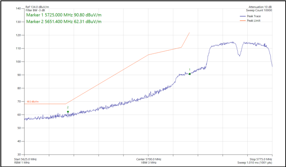
Figure 755 - 802.11a a40, SISO, Core 0 - 5755 MHz Band Edge Frequency 5725 MHz
