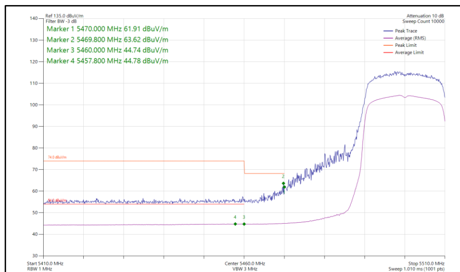
Figure 735 - 802.11ax HE20, SU, TxBF, Core 0-1 - 5500 MHz Band Edge Frequency 5470 MHz
