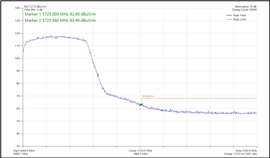
Figure 742 - 802.11ax HE20, SU, TxBF, Core 0-1 - 5700 MHz Band Edge Frequency 5725 MHz
