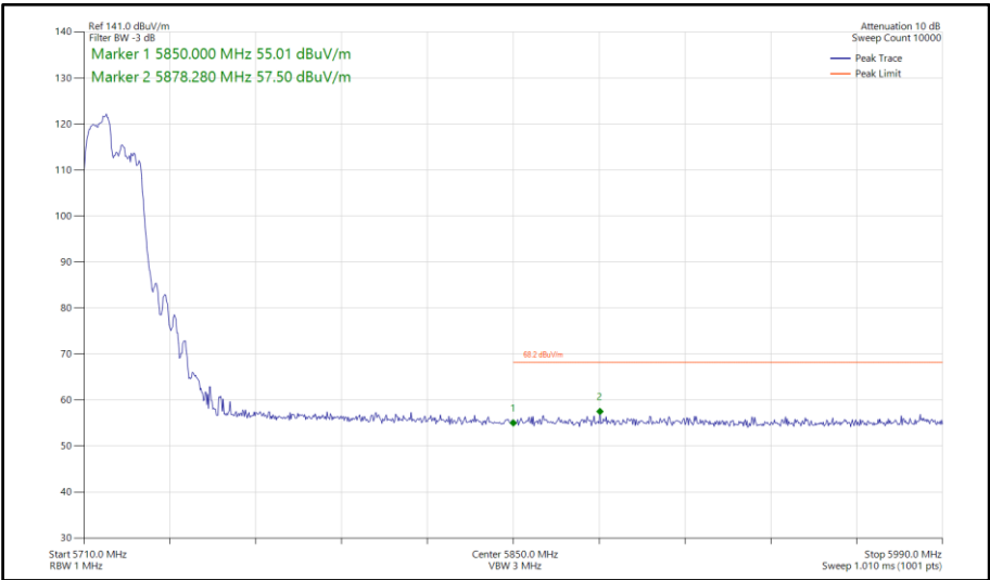
Figure 728 - 802.11ax HE20, RU 106-53, SDM, Core 0-1 - 5720 MHz Band Edge Frequency 5850 MHz
