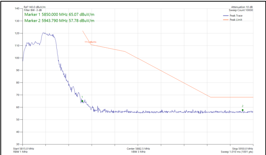
Figure 730 - 802.11ax HE20, RU 106-54, SDM, Core 0-1 - 5825 MHz Band Edge Frequency 5850 MHz
