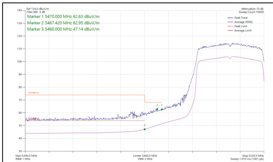
Figure 780 - 802.11ax HE40, SU, SISO, Core 1 - 5510 MHz Band Edge Frequency 5470 MHz
