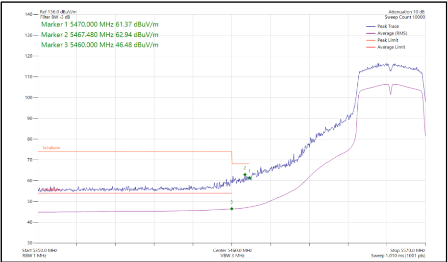
Figure 750 - 802.11n HT40, SISO, Core 0 - 5550 MHz Band Edge Frequency 5470 MHz
