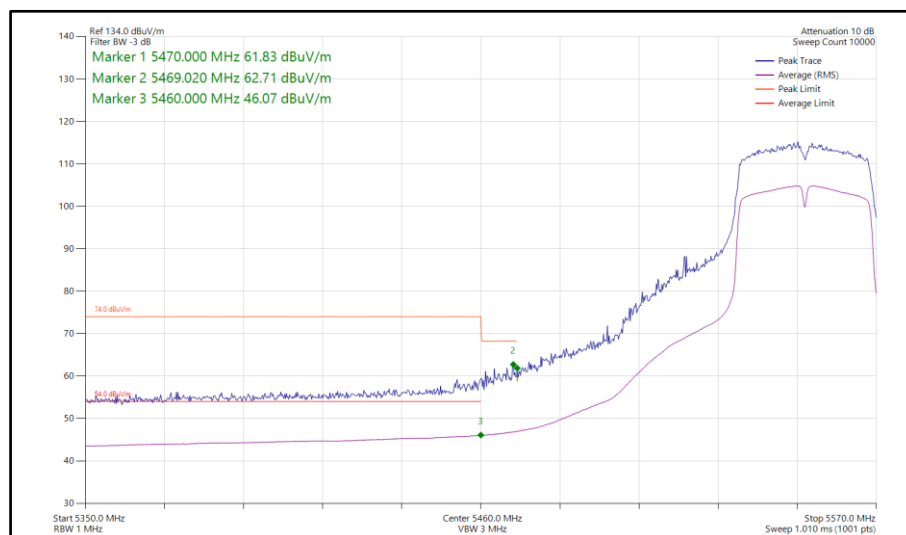
Figure 779 - 802.11n HT40, SISO, Core 1 - 5550 MHz Band Edge Frequency 5470 MHz
