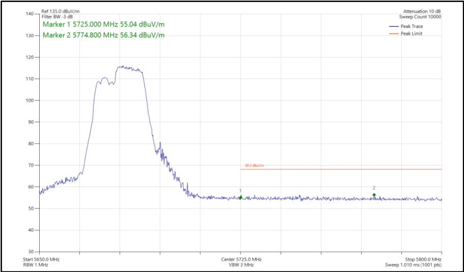
Figure 794 - 802.11be EHT40, RU 106+26-85, SISO, Core 1 - 5670 MHz Band Edge Frequency 5725 MHz
