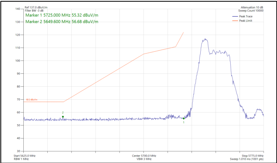
Figure 758 - 802.11ax HE40, RU 52-37, SISO, Core 0 - 5755 MHz Band Edge Frequency 5725 MHz
