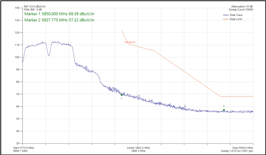
Figure 796 - 802.11a a40, SISO, Core 1 - 5795 MHz Band Edge Frequency 5850 MHz
