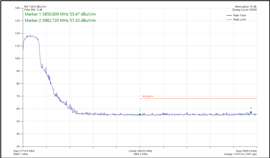
Figure 745 - 802.11ax HE20, SU, TxBF, Core 0-1 - 5720 MHz Band Edge Frequency 5850 MHz
