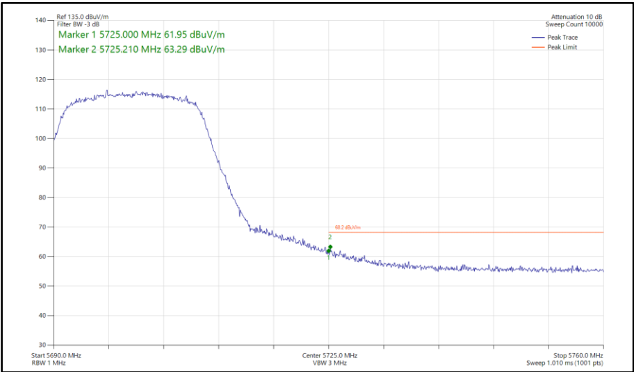
Figure 720 - 802.11n HT20, SDM, Core 0-1 - 5700 MHz Band Edge Frequency 5725 MHz
