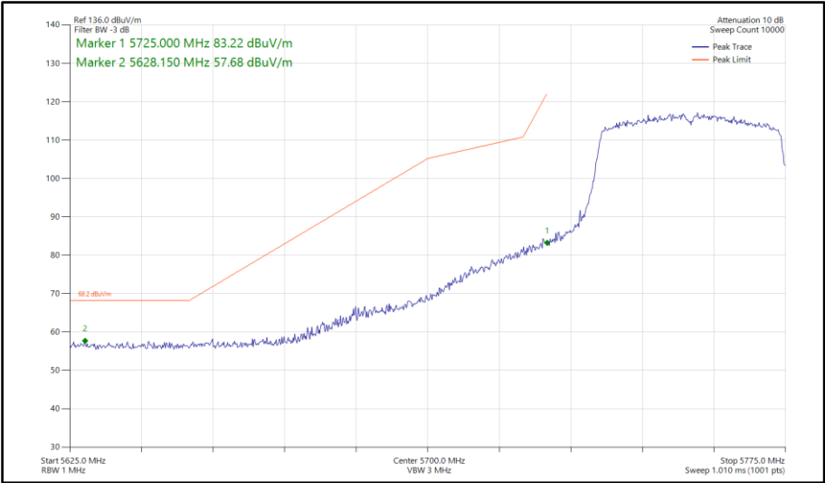
Figure 757 - 802.11ax HE40, SU, SISO, Core 0 - 5755 MHz Band Edge Frequency 5725 MHz
