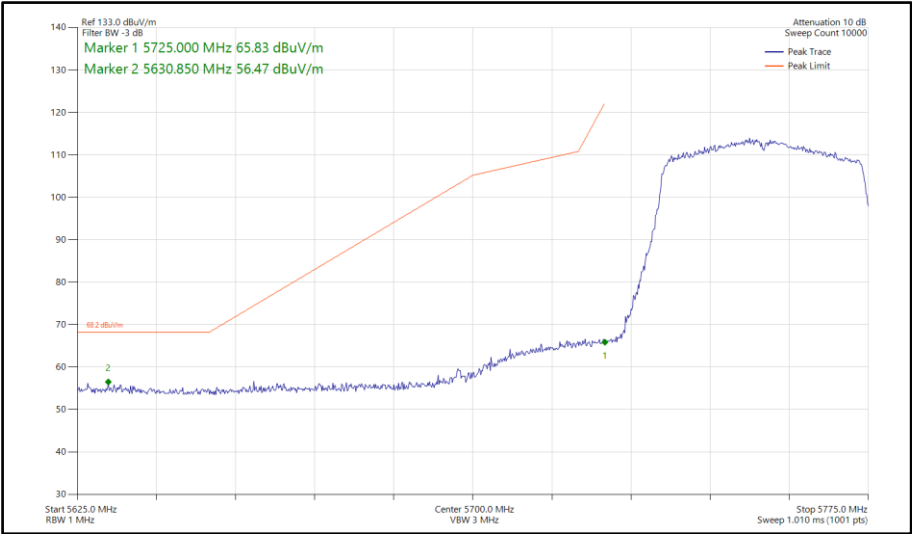
Figure 786 - 802.11ax HE40, SU, SISO, Core 1 - 5755 MHz Band Edge Frequency 5725 MHz
