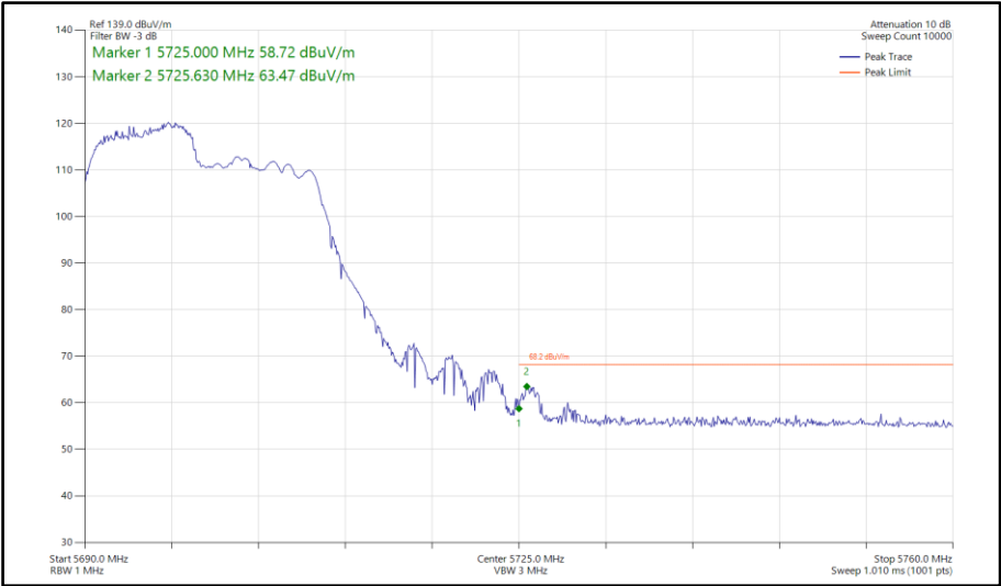
Figure 723 - 802.11ax HE20, RU 106-53, SDM, Core 0-1 - 5700 MHz Band Edge Frequency 5725 MHz
