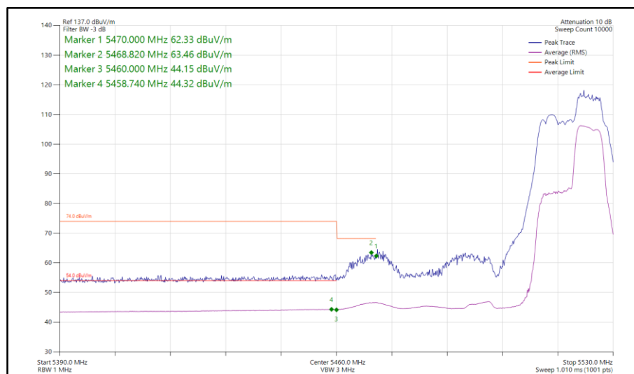
Figure 783 - 802.11be EHT40, RU 52+26-75, SISO, Core 1 - 5510 MHz Band Edge Frequency 5470 MHz
