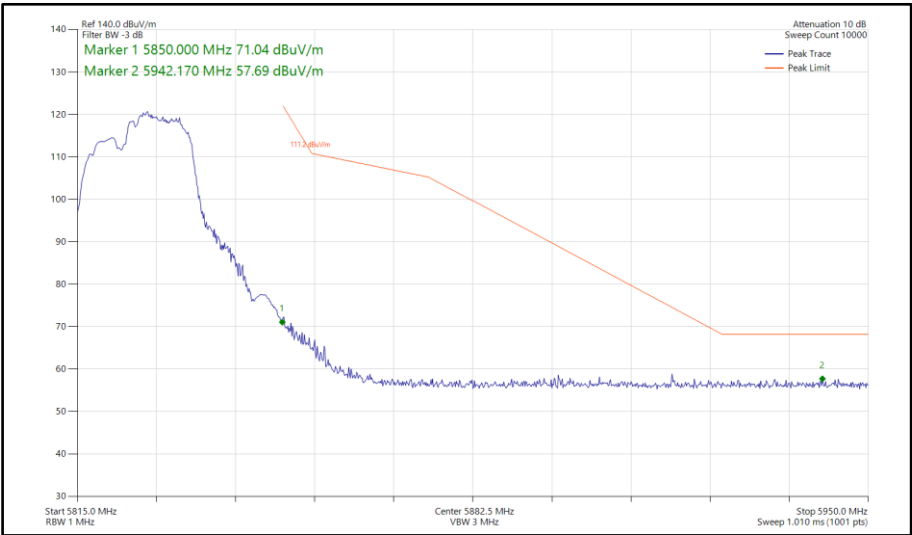
Figure 732 - 802.11be EHT20, RU 106+26-83, SDM, Core 0-1 - 5825 MHz Band Edge Frequency 5850 MHz
