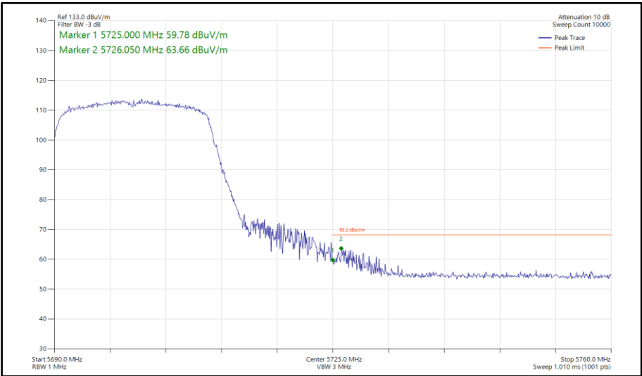
Figure 722 - 802.11ax HE20, SU, SDM, Core 0-1 - 5700 MHz Band Edge Frequency 5725 MHz
