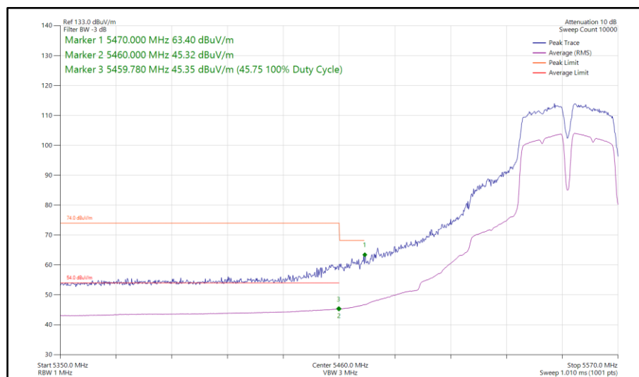
Figure 748 - 802.11a a40, SISO, Core 0 - 5550 MHz Band Edge Frequency 5470 MHz
