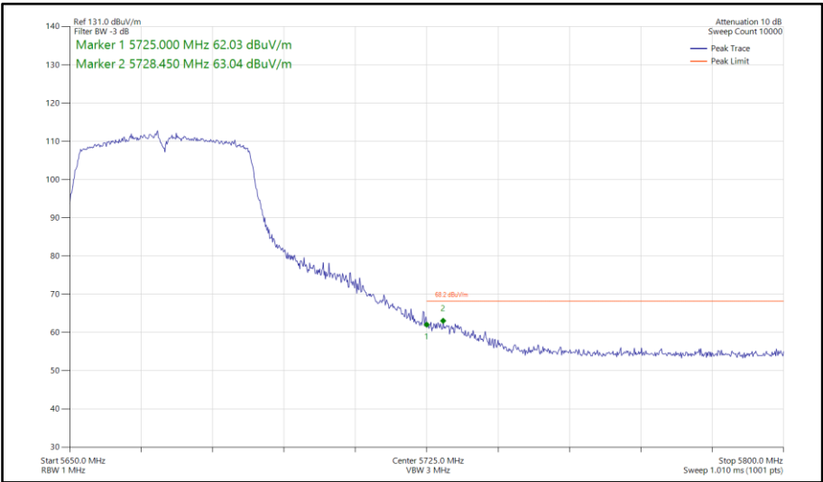
Figure 791 - 802.11n HT40, SISO, Core 1 - 5670 MHz Band Edge Frequency 5725 MHz
