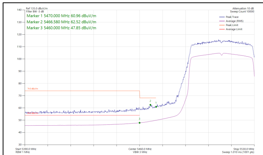
Figure 751 - 802.11ax HE40, SU, SISO, Core 0 - 5510 MHz Band Edge Frequency 5470 MHz
