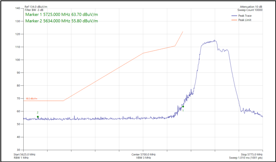
Figure 788 - 802.11be EHT40, RU 106+26-82, SISO, Core 1 - 5755 MHz Band Edge Frequency 5725 MHz
