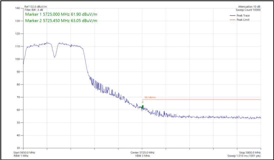
Figure 761 - 802.11a a40, SISO, Core 0 - 5670 MHz Band Edge Frequency 5725 MHz
