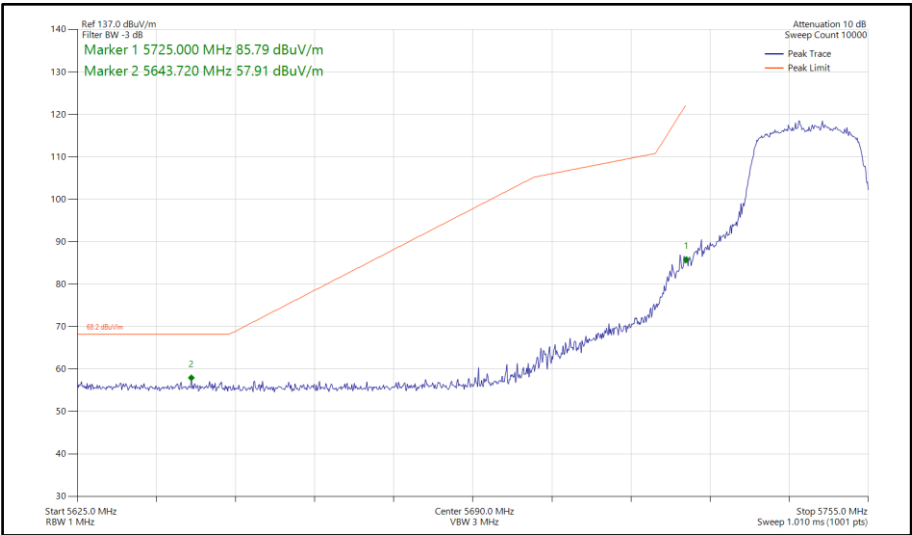
Figure 737 - 802.11ac VHT20, TxBF, Core 0-1 - 5745 MHz Band Edge Frequency 5725 MHz
