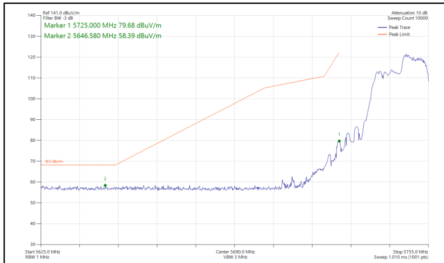
Figure 717 - 802.11ax HE20, RU 106-54, SDM, Core 0-1 - 5745 MHz Band Edge Frequency 5725 MHz
