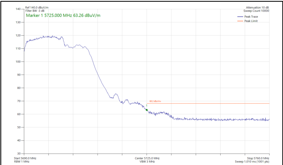
Figure 724 - 802.11be EHT20, RU 106+26-82, SDM, Core 0-1 - 5700 MHz Band Edge Frequency 5725 MHz
