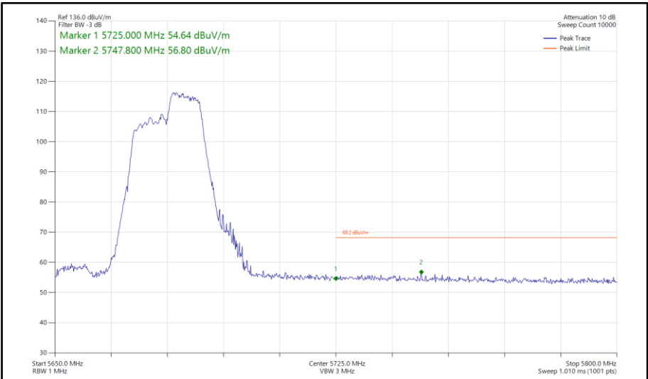
Figure 764 - 802.11ax HE40, RU 106-56, SISO, Core 0 - 5670 MHz Band Edge Frequency 5725 MHz
