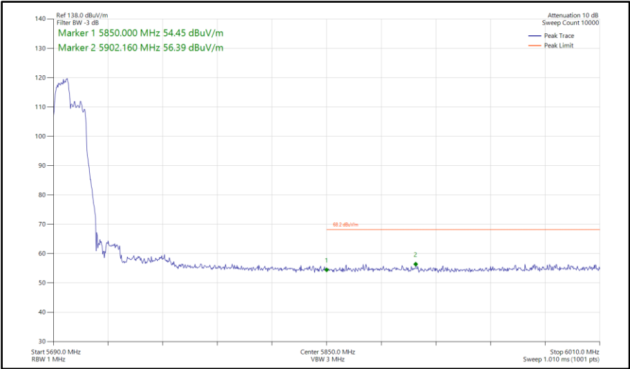
Figure 771 - 802.11ax HE40, RU 106-53, SISO, Core 0 - 5710 MHz Band Edge Frequency 5850 MHz
