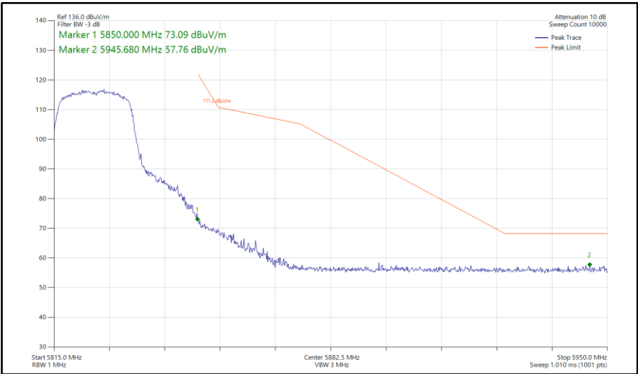
Figure 726 - 802.11n HT20, SDM, Core 0-1 - 5825 MHz Band Edge Frequency 5850 MHz
