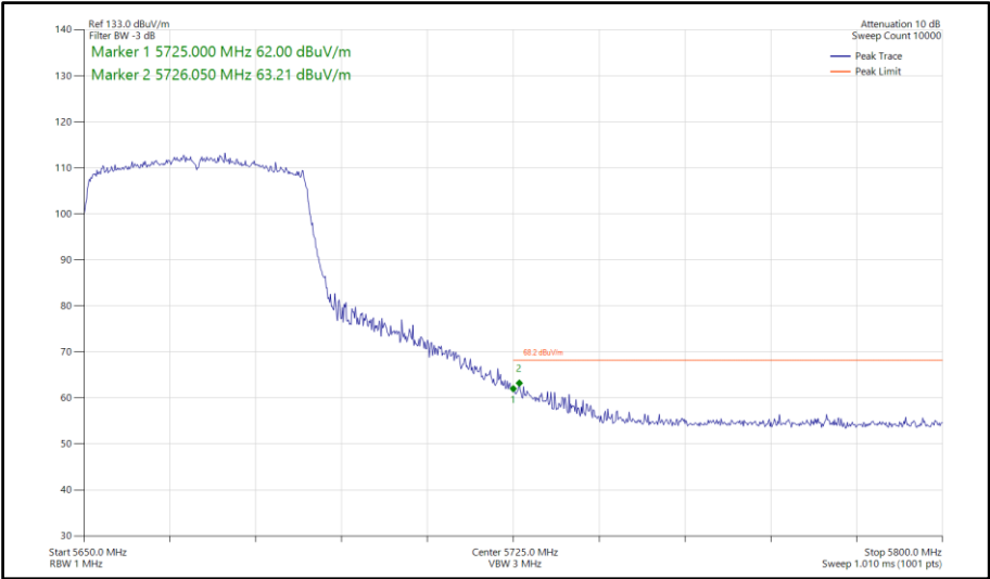
Figure 792 - 802.11ax HE40, SU, SISO, Core 1 - 5670 MHz Band Edge Frequency 5725 MHz
