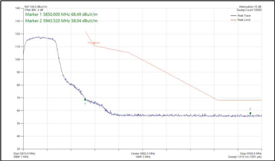
Figure 744 - 802.11ac VHT20, TxBF, Core 0-1 - 5825 MHz Band Edge Frequency 5850 MHz
