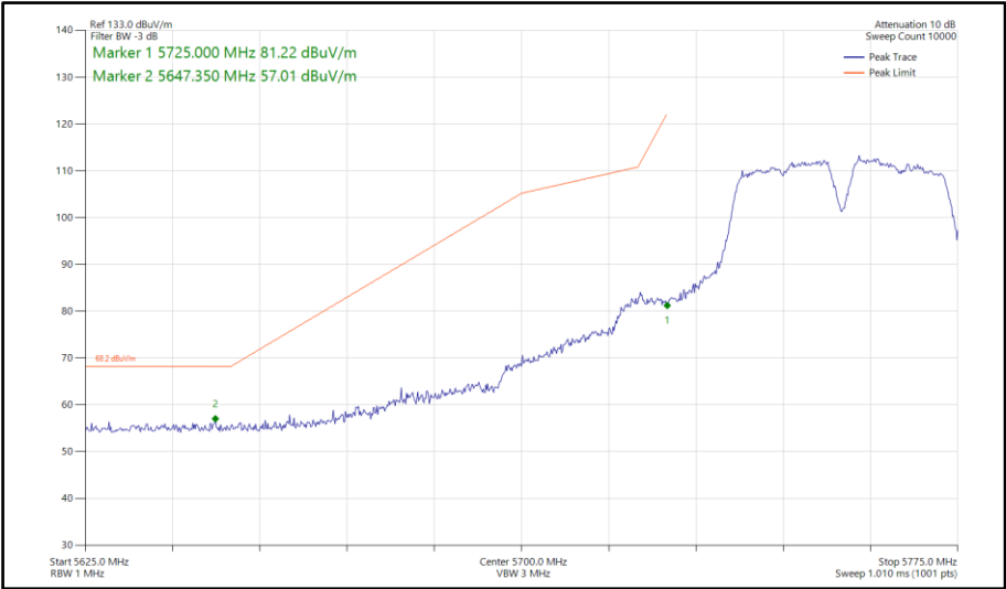
Figure 784 - 802.11a a40, SISO, Core 1 - 5755 MHz Band Edge Frequency 5725 MHz
