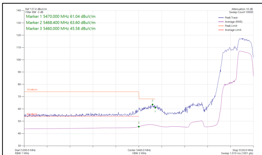
Figure 781 - 802.11ax HE40, RU 106-56, SISO, Core 1 - 5510 MHz Band Edge Frequency 5470 MHz
