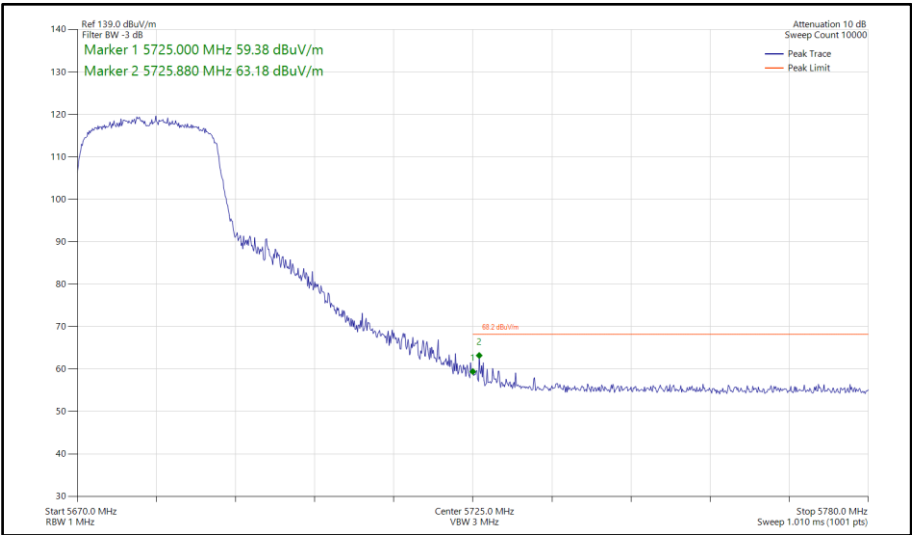
Figure 741 - 802.11ax HE20, SU, TxBF, Core 0-1 - 5680 MHz Band Edge Frequency 5725 MHz
