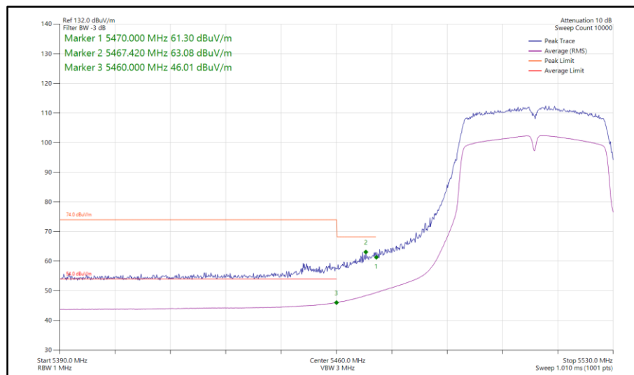
Figure 778 - 802.11n HT40, SISO, Core 1 - 5510 MHz Band Edge Frequency 5470 MHz
