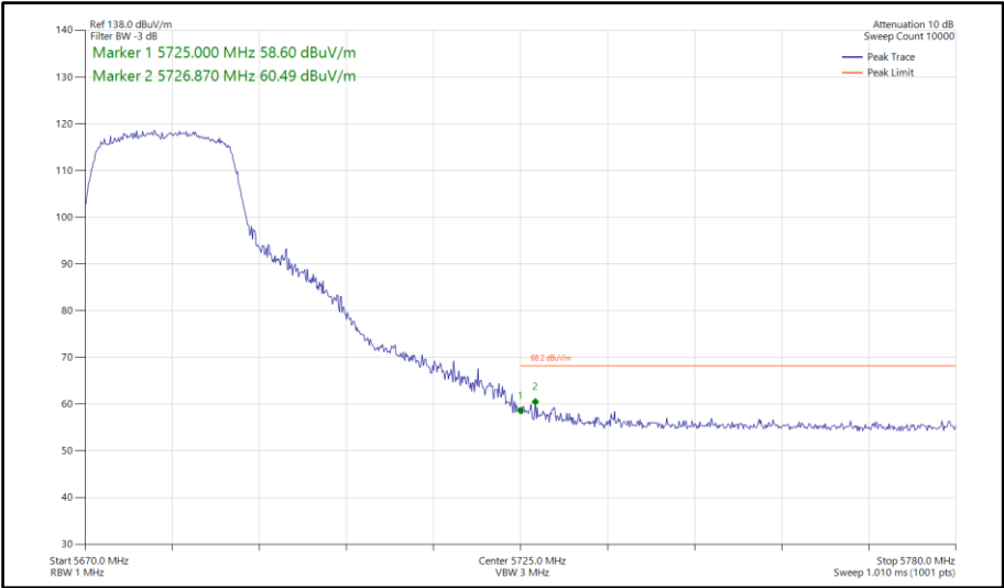
Figure 719 - 802.11n HT20, SDM, Core 0-1 - 5680 MHz Band Edge Frequency 5725 MHz
