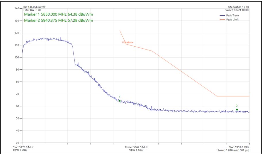
Figure 772 - 802.11ax HE40, SU, SISO, Core 0 - 5795 MHz Band Edge Frequency 5850 MHz
