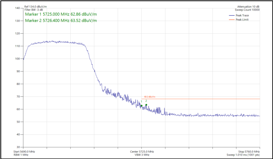
Figure 740 - 802.11ac VHT20, TxBF, Core 0-1 - 5700 MHz Band Edge Frequency 5725 MHz
