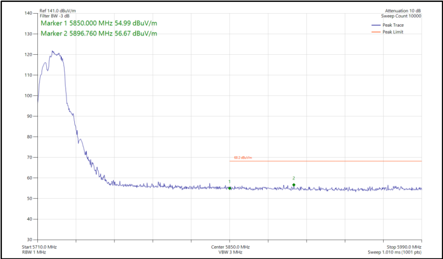
Figure 731 - 802.11be EHT20, RU 106+26-83, SDM, Core 0-1 - 5720 MHz Band Edge Frequency 5850 MHz
