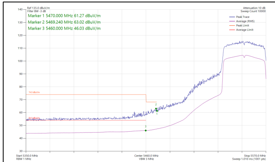
Figure 782 - 802.11ax HE40, SU, SISO, Core 1 - 5550 MHz Band Edge Frequency 5470 MHz
