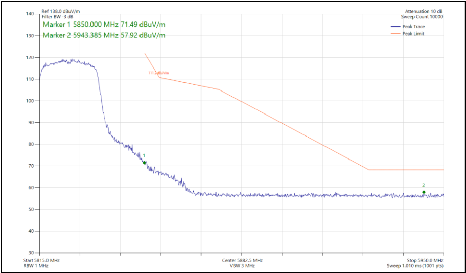
Figure 746 - 802.11ax HE20, SU, TxBF, Core 0-1 - 5825 MHz Band Edge Frequency 5850 MHz
