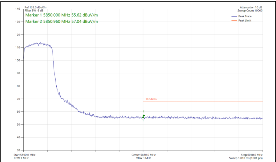
Figure 799 - 802.11ax HE40, SU, SISO, Core 1 - 5710 MHz Band Edge Frequency 5850 MHz
