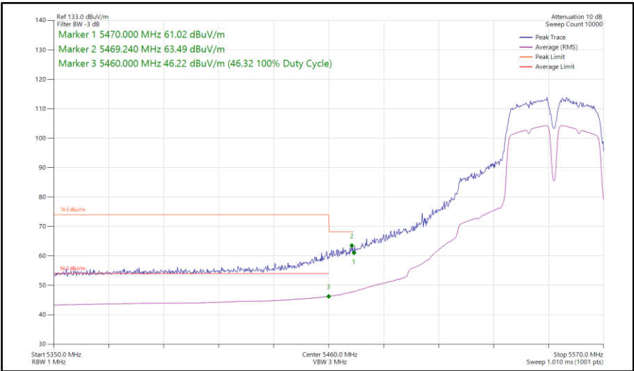
Figure 777 - 802.11a a40, SISO, Core 1 - 5550 MHz Band Edge Frequency 5470 MHz
