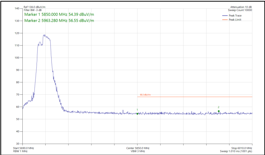
Figure 774 - 802.11be EHT40, RU 106+26-85, SISO, Core 0 - 5710 MHz Band Edge Frequency 5850 MHz
