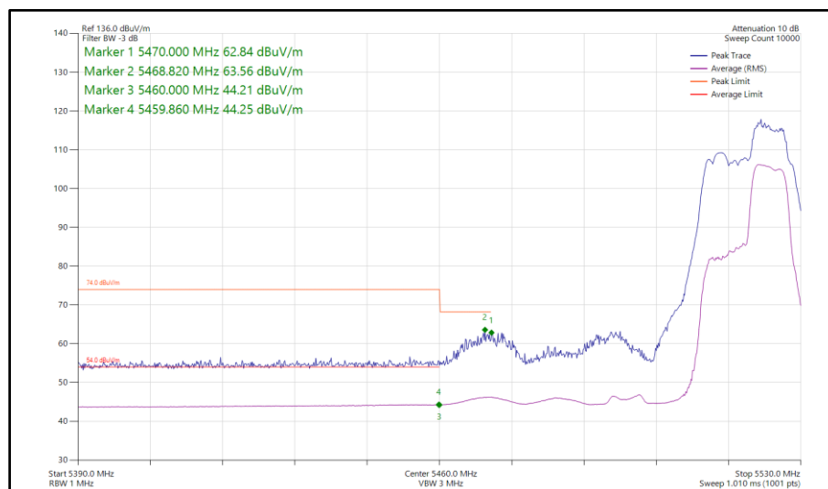
Figure 754 - 802.11be EHT40, RU 52+26-75, SISO, Core 0 - 5510 MHz Band Edge Frequency 5470 MHz
