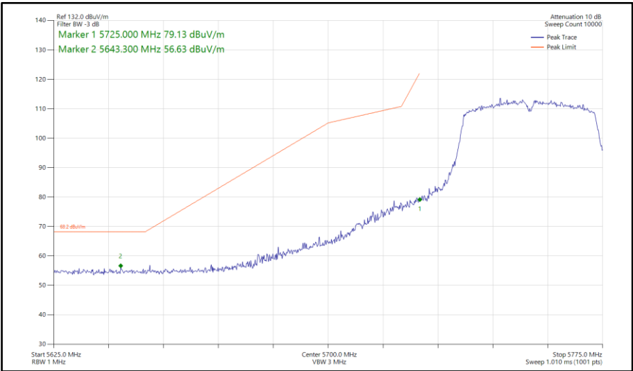
Figure 785 - 802.11n HT40, SISO, Core 1 - 5755 MHz Band Edge Frequency 5725 MHz
