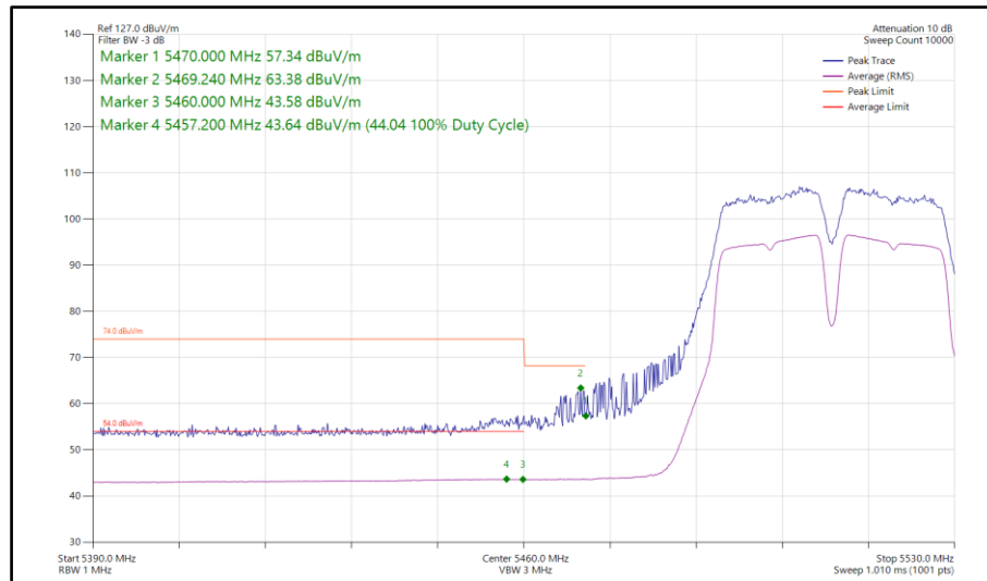
Figure 747 - 802.11a a40, SISO, Core 0 - 5510 MHz Band Edge Frequency 5470 MHz
