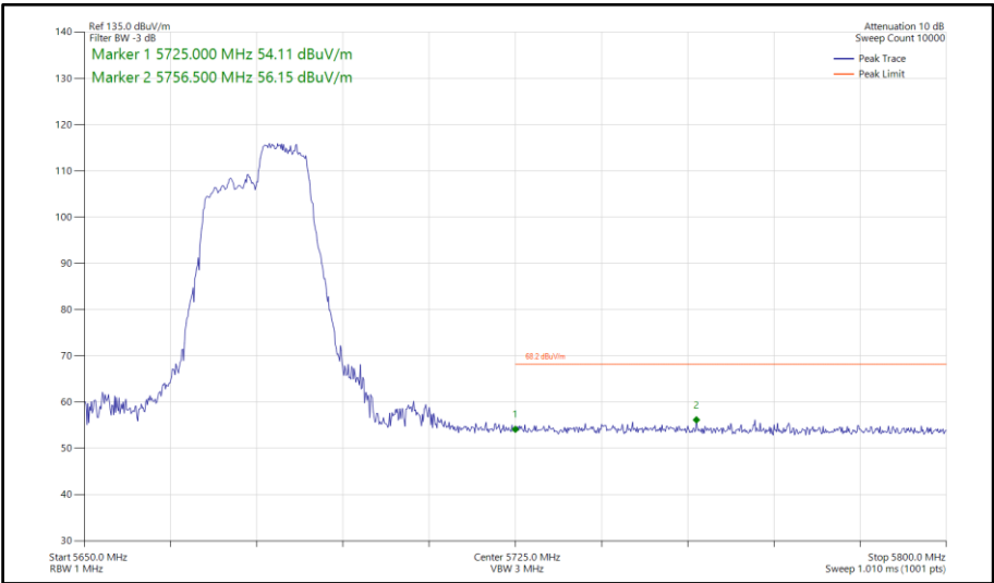
Figure 793 - 802.11ax HE40, RU 106-56, SISO, Core 1 - 5670 MHz Band Edge Frequency 5725 MHz
