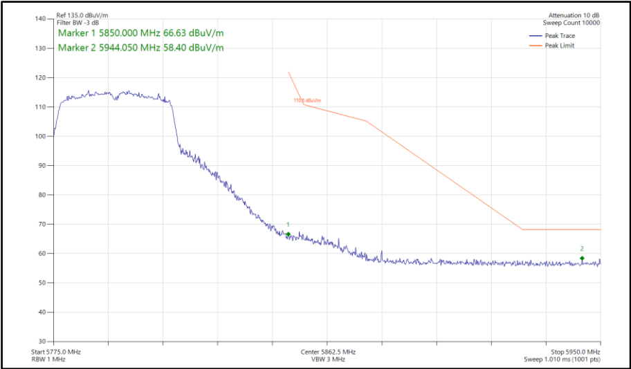
Figure 769 - 802.11n HT40, SISO, Core 0 - 5795 MHz Band Edge Frequency 5850 MHz
