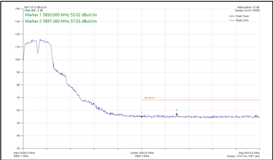
Figure 766 - 802.11a a40, SISO, Core 0 - 5710 MHz Band Edge Frequency 5850 MHz
