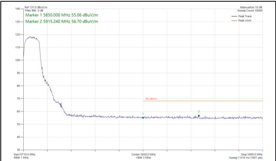
Figure 743 - 802.11ac VHT20, TxBF, Core 0-1 - 5720 MHz Band Edge Frequency 5850 MHz
