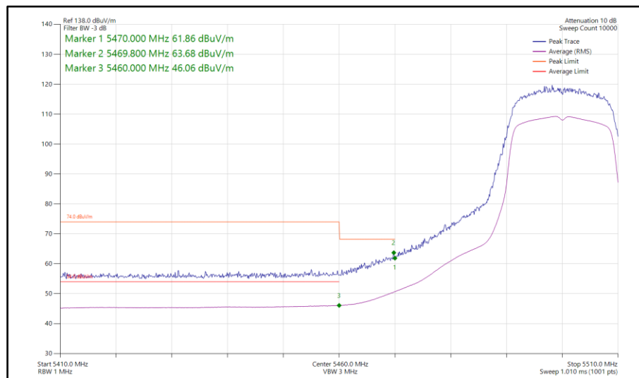
Figure 733 - 802.11ac VHT20, TxBF, Core 0-1 - 5500 MHz Band Edge Frequency 5470 MHz
