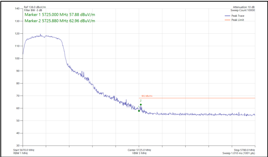
Figure 739 - 802.11ac VHT20, TxBF, Core 0-1 - 5680 MHz Band Edge Frequency 5725 MHz
