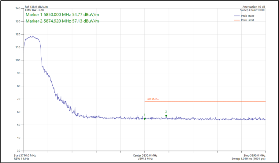
Figure 727 - 802.11ax HE20, SU, SDM, Core 0-1 - 5720 MHz Band Edge Frequency 5850 MHz
