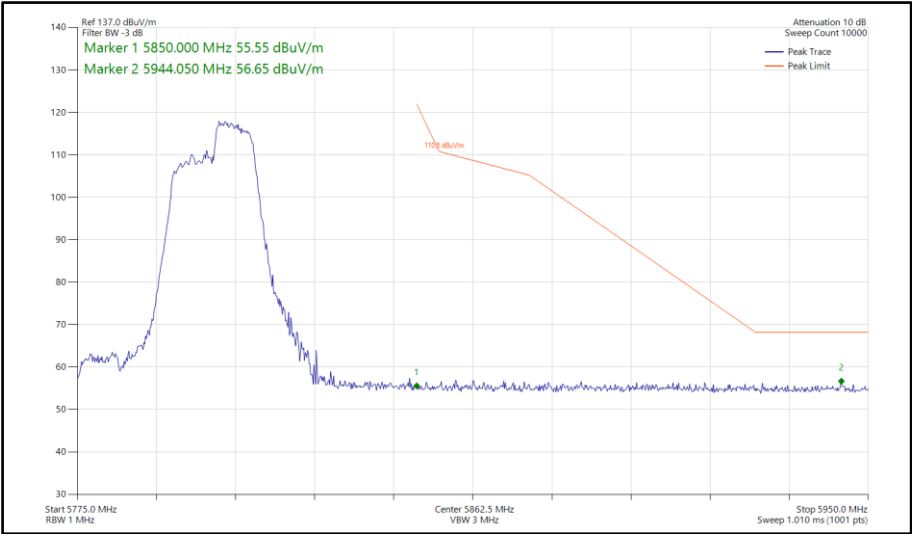
Figure 773 - 802.11ax HE40, RU 106-56, SISO, Core 0 - 5795 MHz Band Edge Frequency 5850 MHz
