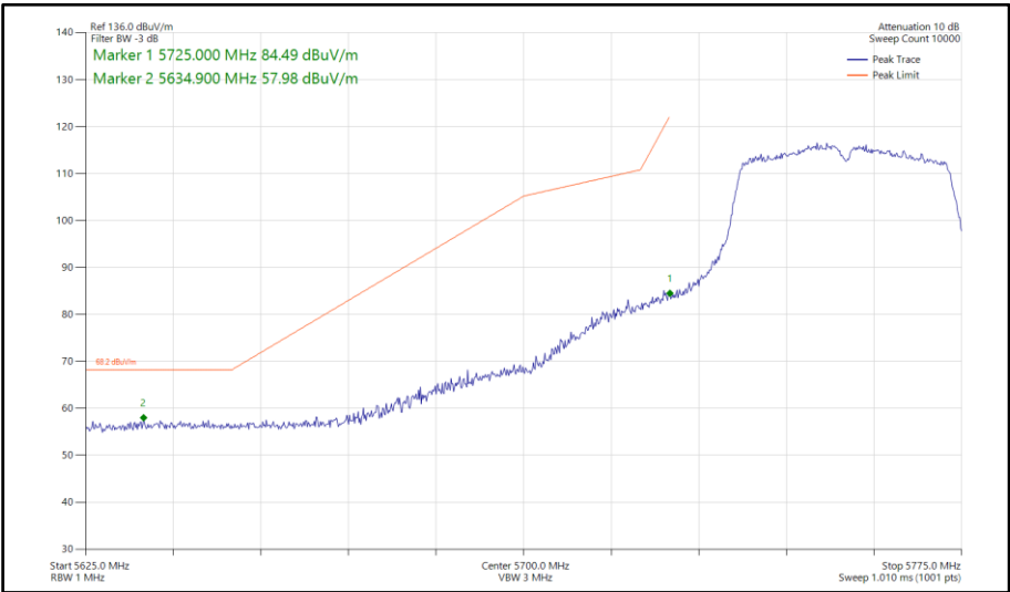
Figure 756 - 802.11n HT40, SISO, Core 0 - 5755 MHz Band Edge Frequency 5725 MHz
