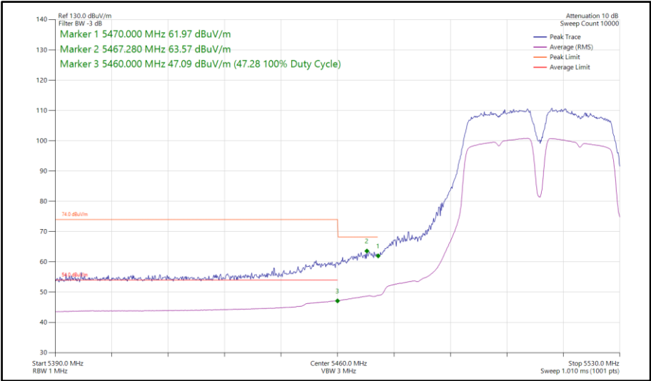
Figure 776 - 802.11a a40, SISO, Core 1 - 5510 MHz Band Edge Frequency 5470 MHz
