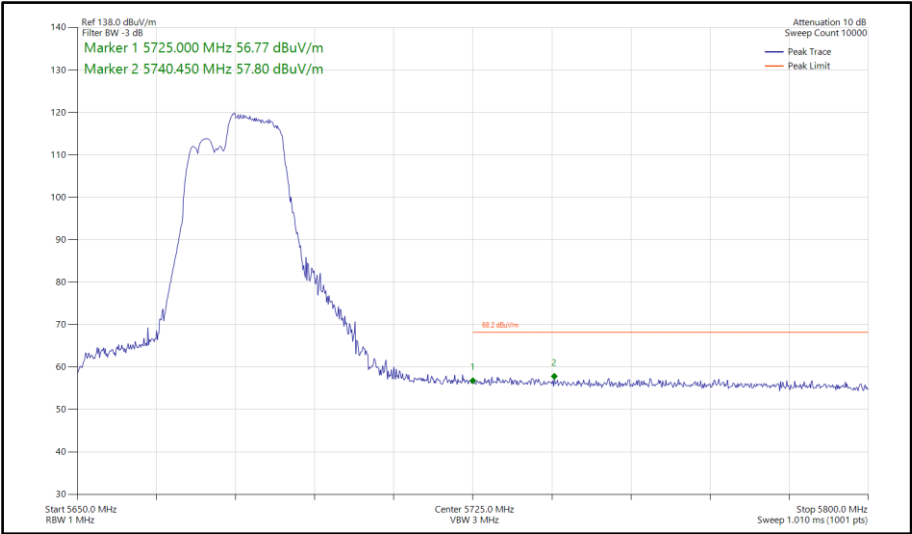
Figure 765 - 802.11be EHT40, RU 106+26-85, SISO, Core 0 - 5670 MHz Band Edge Frequency 5725 MHz
