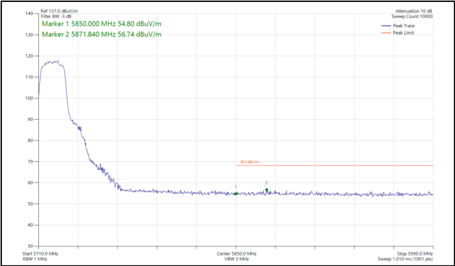
Figure 725 - 802.11n HT20, SDM, Core 0-1 - 5720 MHz Band Edge Frequency 5850 MHz
