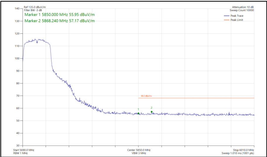
Figure 768 - 802.11n HT40, SISO, Core 0 - 5710 MHz Band Edge Frequency 5850 MHz
