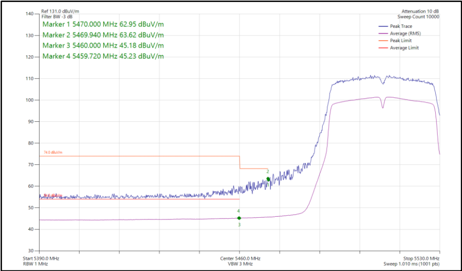
Figure 749 - 802.11n HT40, SISO, Core 0 - 5510 MHz Band Edge Frequency 5470 MHz
