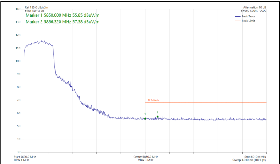
Figure 770 - 802.11ax HE40, SU, SISO, Core 0 - 5710 MHz Band Edge Frequency 5850 MHz
