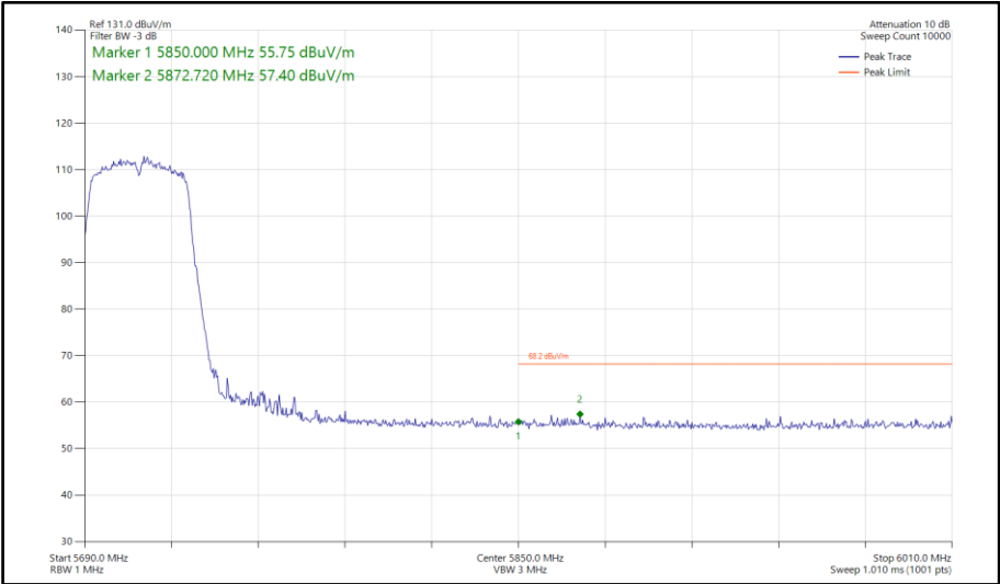
Figure 797 - 802.11n HT40, SISO, Core 1 - 5710 MHz Band Edge Frequency 5850 MHz
