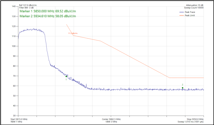
Figure 729 - 802.11ax HE20, SU, SDM, Core 0-1 - 5825 MHz Band Edge Frequency 5850 MHz
