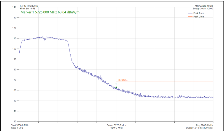
Figure 762 - 802.11n HT40, SISO, Core 0 - 5670 MHz Band Edge Frequency 5725 MHz
