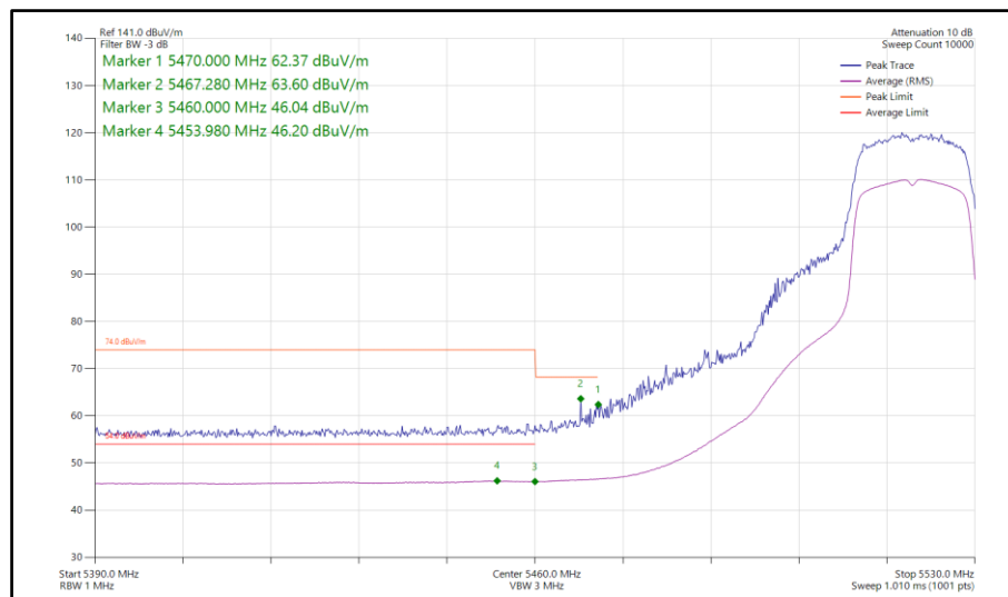
Figure 734 - 802.11ac VHT20, TxBF, Core 0-1 - 5520 MHz Band Edge Frequency 5470 MHz
