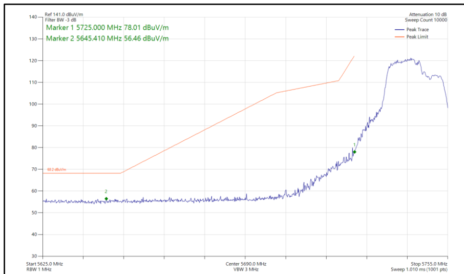
Figure 718 - 802.11be EHT20, RU 106+26-82, SDM, Core 0-1 - 5745 MHz Band Edge Frequency 5725 MHz
