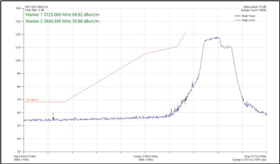
Figure 759 - 802.11be EHT40, RU 106+26-82, SISO, Core 0 - 5755 MHz Band Edge Frequency 5725 MHz
