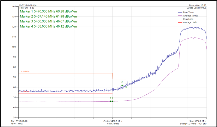
Figure 736 - 802.11ax HE20, SU, TxBF, Core 0-1 - 5520 MHz Band Edge Frequency 5470 MHz
