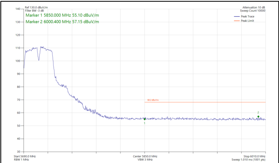
Figure 795 - 802.11a a40, SISO, Core 1 - 5710 MHz Band Edge Frequency 5850 MHz
