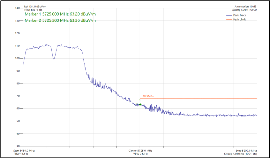
Figure 790 - 802.11a a40, SISO, Core 1 - 5670 MHz Band Edge Frequency 5725 MHz
