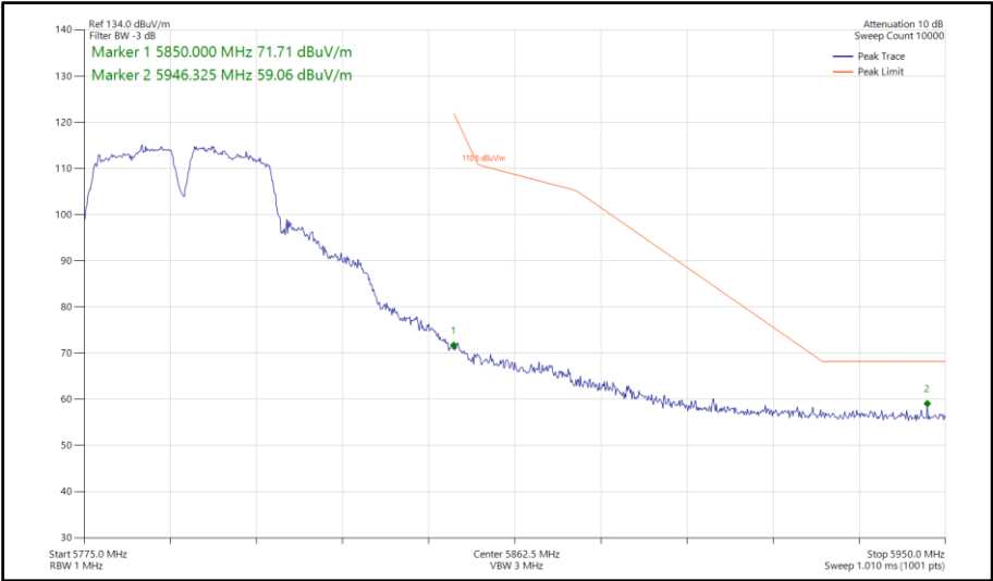
Figure 767 - 802.11a a40, SISO, Core 0 - 5795 MHz Band Edge Frequency 5850 MHz
