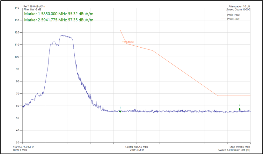
Figure 775 - 802.11be EHT40, RU 106+26-85, SISO, Core 0 - 5795 MHz Band Edge Frequency 5850 MHz
