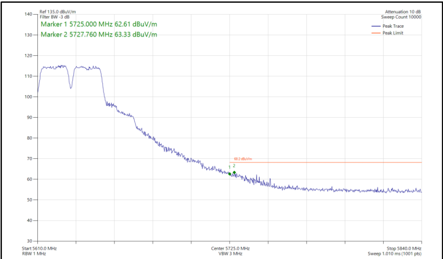
Figure 760 - 802.11a a40, SISO, Core 0 - 5630 MHz Band Edge Frequency 5725 MHz
