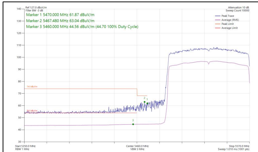
Figure 944 - 802.11ax HE80, SU, SDM, Core 0-1 - 5530 MHz Band Edge Frequency 5470 MHz
