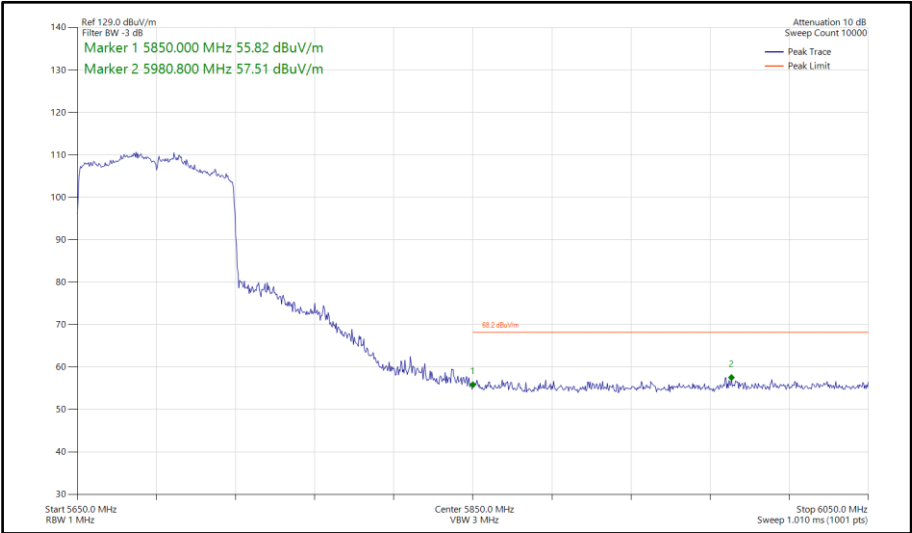
Figure 887 - 802.11ax HE80, SU, SISO, Core 0 - 5690 MHz Band Edge Frequency 5850 MHz
