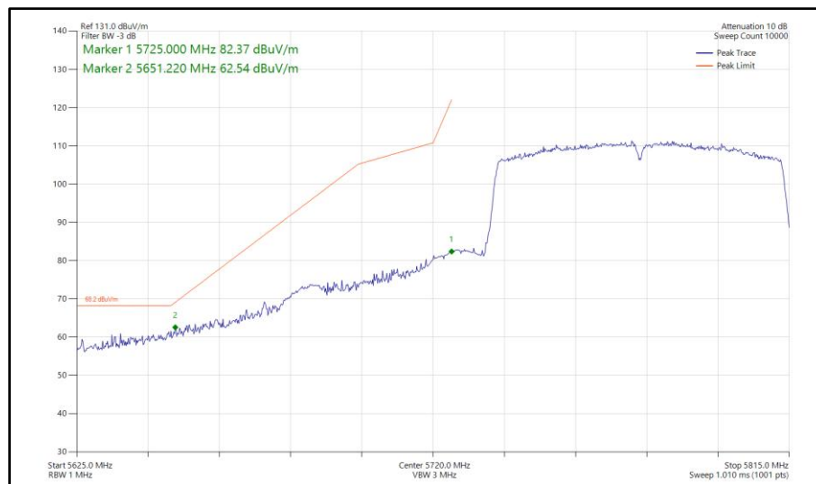
Figure 899 - 802.11ac VHT80, SISO, Core 1 - 5775 MHz Band Edge Frequency 5725 MHz
