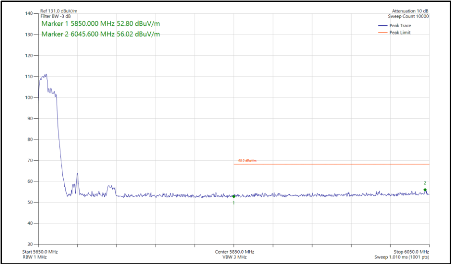
Figure 913 - 802.11ax HE80, RU 106-53, SISO, Core 1 - 5690 MHz Band Edge Frequency 5850 MHz
