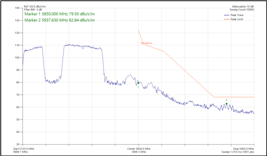
Figure 917 - 802.11be EHT80, RU 484+242-91, SISO, Core 1 - 5775 MHz Band Edge Frequency 5850 MHz
