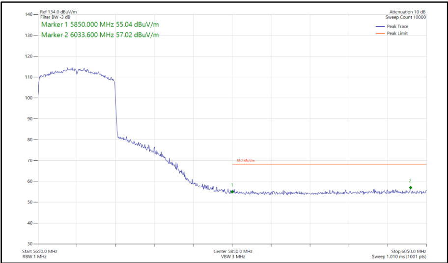
Figure 957 - 802.11ax HE80, SU, SDM, Core 0-1 - 5690 MHz Band Edge Frequency 5850 MHz
