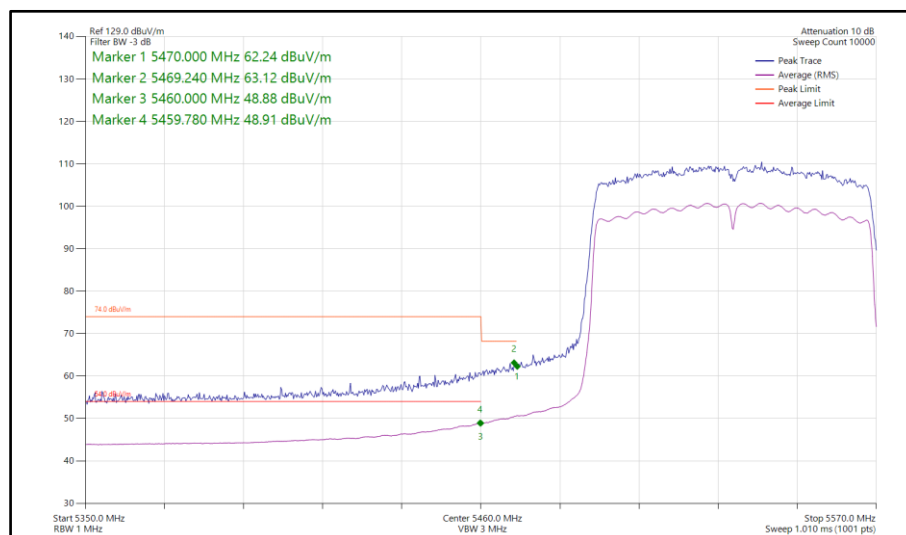
Figure 919 - 802.11ac VHT80, CDD, Core 0-1 - 5530 MHz Band Edge Frequency 5470 MHz
