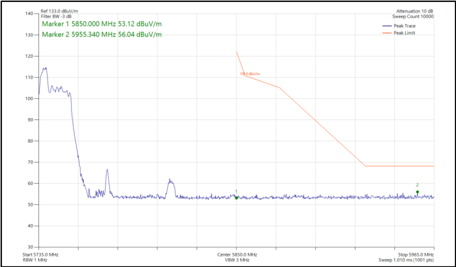
Figure 940 - 802.11ax HE80, RU 52-37, CDD, Core 0-1 - 5775 MHz Band Edge Frequency 5850 MHz
