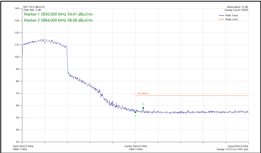
Figure 937 - 802.11ax HE80, SU, CDD, Core 0-1 - 5690 MHz Band Edge Frequency 5850 MHz
