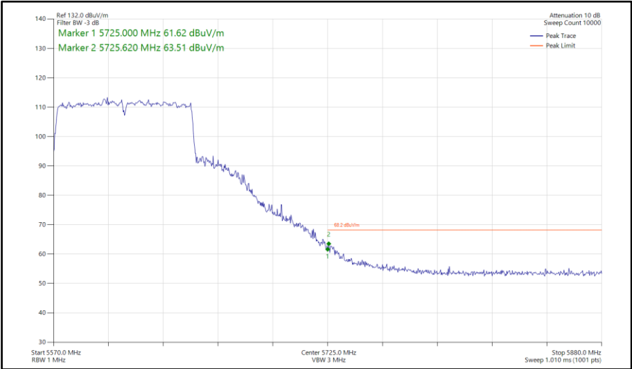
Figure 929 - 802.11ac VHT80, CDD, Core 0-1 - 5610 MHz Band Edge Frequency 5725 MHz
