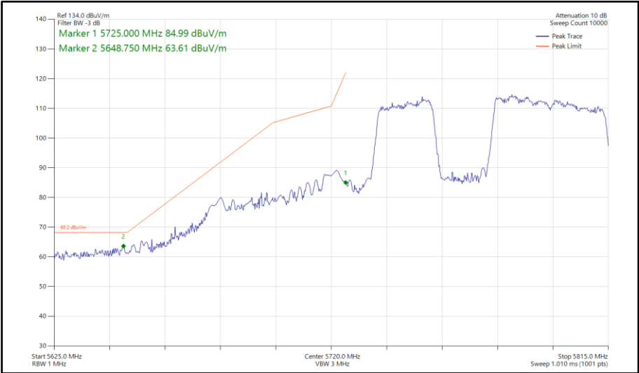
Figure 927 - 802.11be EHT80, RU 484+242-91, CDD, Core 0-1 - 5775 MHz Band Edge Frequency 5725 MHz
