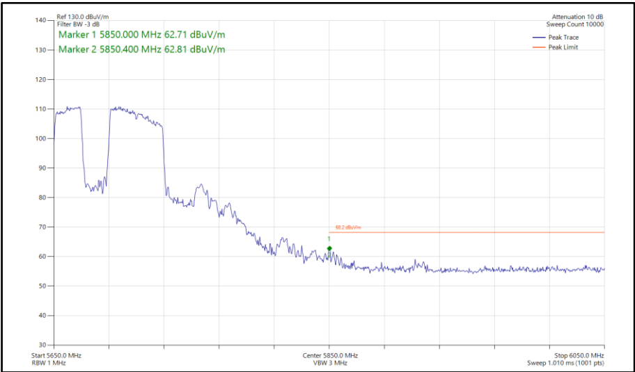
Figure 891 - 802.11be EHT80, RU 484+242-91, SISO, Core 0 - 5690 MHz Band Edge Frequency 5850 MHz
