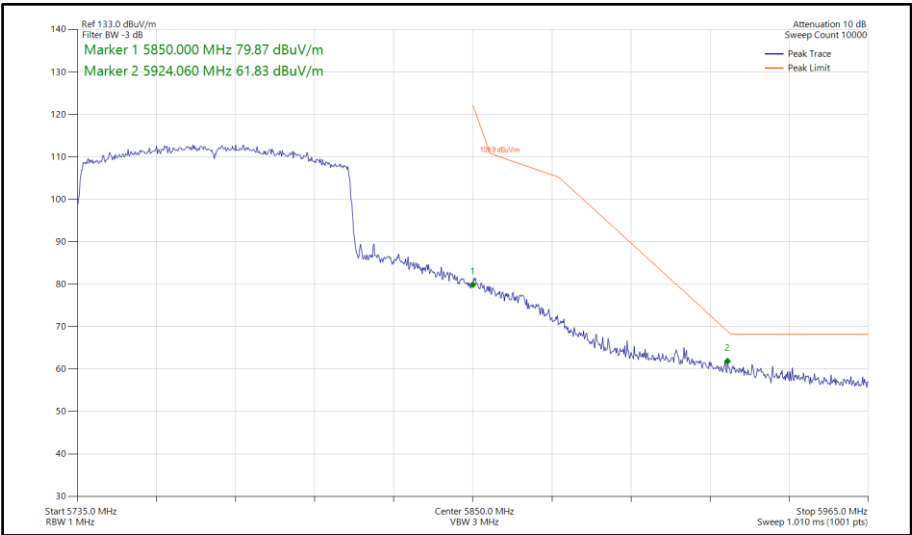
Figure 959 - 802.11ax HE80, SU, SDM, Core 0-1 - 5775 MHz Band Edge Frequency 5850 MHz
