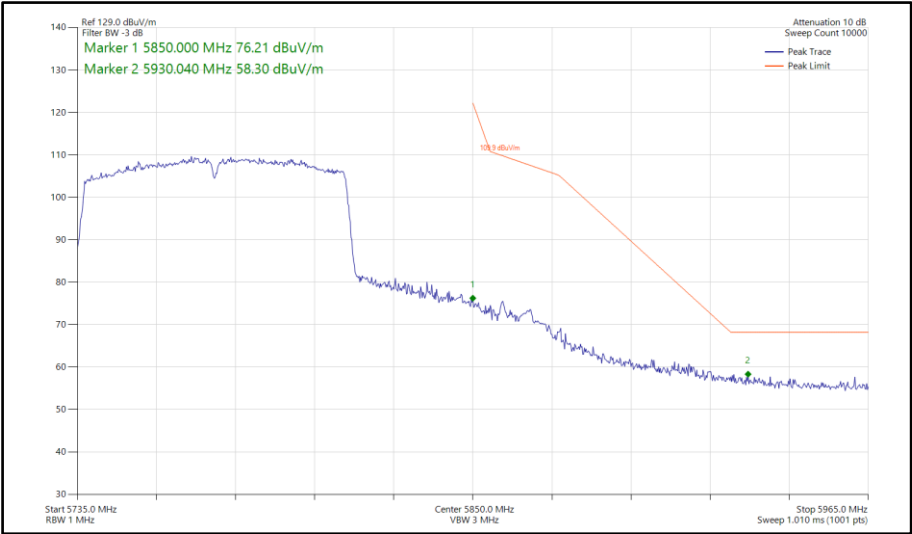
Figure 911 - 802.11ac VHT80, SISO, Core 1 - 5775 MHz Band Edge Frequency 5850 MHz
