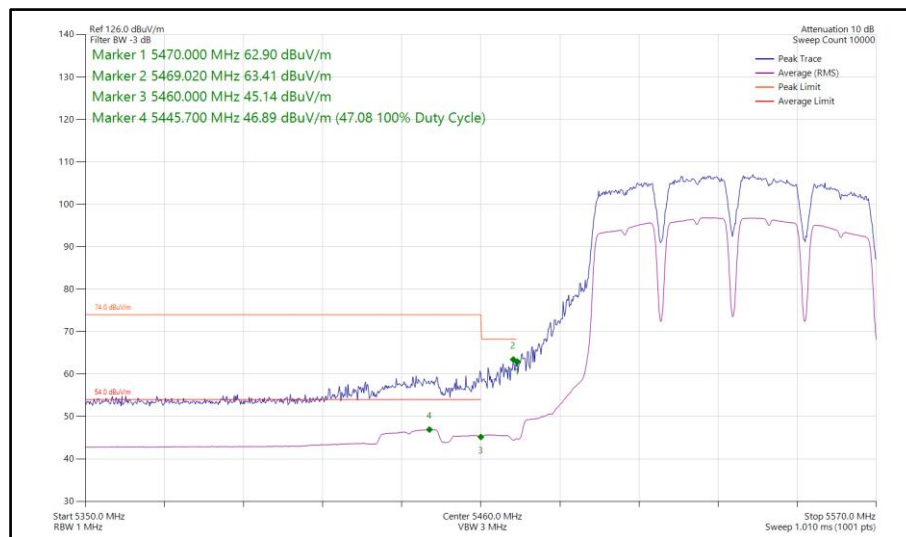
Figure 893 - 802.11a a80, SISO, Core 1 - 5530 MHz Band Edge Frequency 5470 MHz
