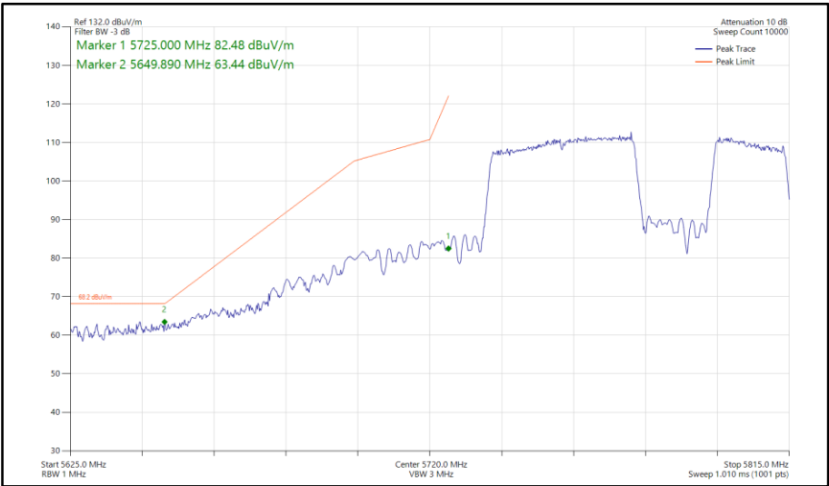
Figure 902 - 802.11be EHT80, RU 484+242-92, SISO, Core 1 - 5775 MHz Band Edge Frequency 5725 MHz
