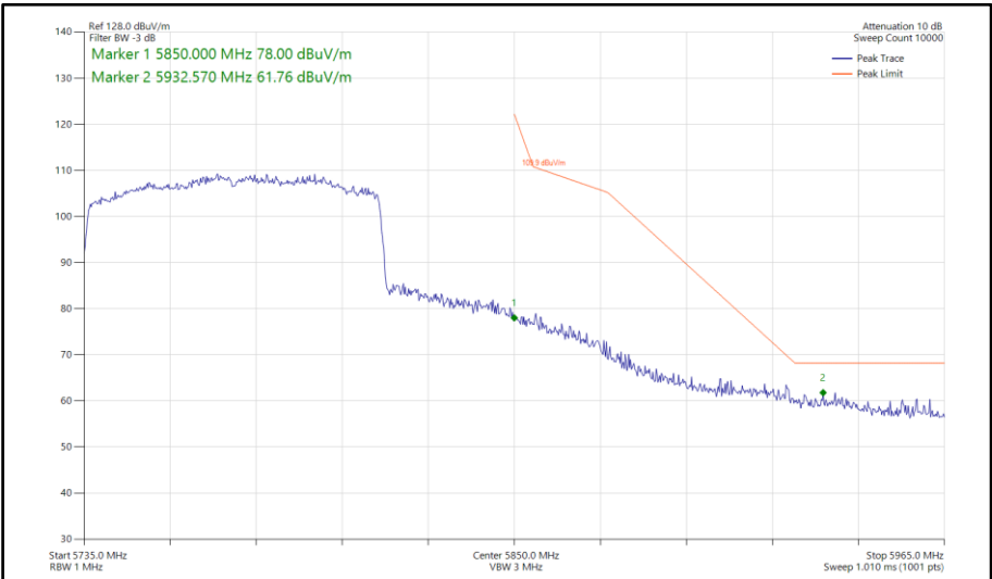
Figure 889 - 802.11ax HE80, SU, SISO, Core 0 - 5775 MHz Band Edge Frequency 5850 MHz
