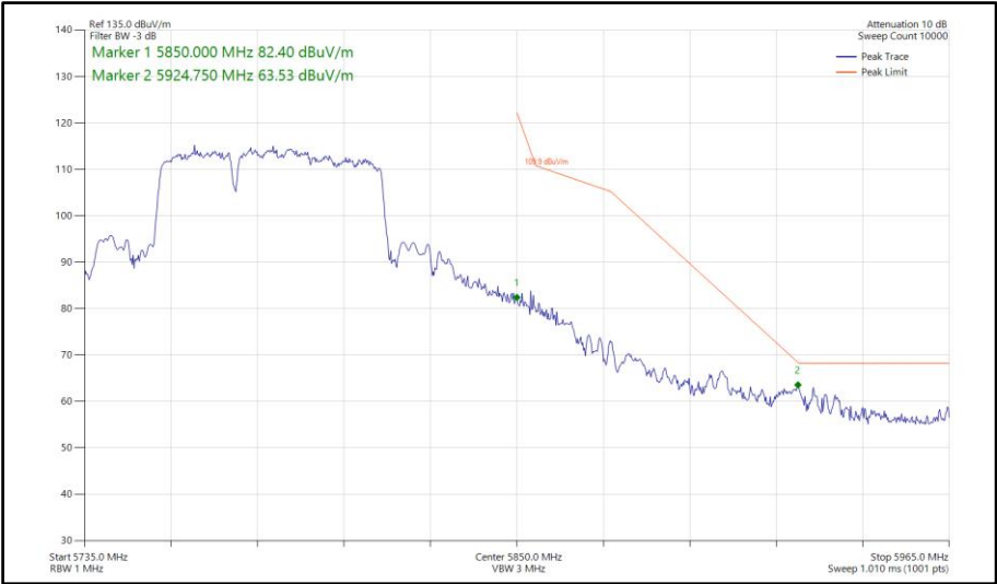
Figure 962 - 802.11be EHT80, RU 484+242-90, SDM, Core 0-1 - 5775 MHz Band Edge Frequency 5850 MHz
