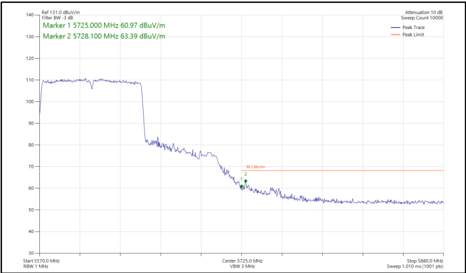
Figure 967 - 802.11ac VHT80, TxBF, Core 0-1 - 5610 MHz Band Edge Frequency 5725 MHz
