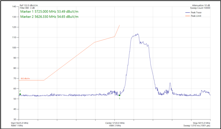
Figure 901 - 802.11ax HE80, RU 106-53, SISO, Core 1 - 5775 MHz Band Edge Frequency 5725 MHz
