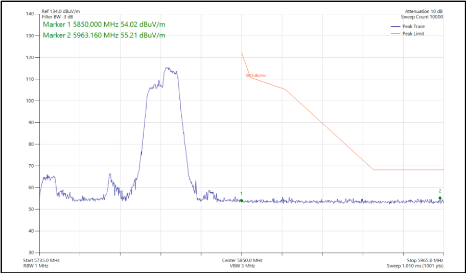
Figure 960 - 802.11ax HE80, RU 106-60, SDM, Core 0-1 - 5775 MHz Band Edge Frequency 5850 MHz
