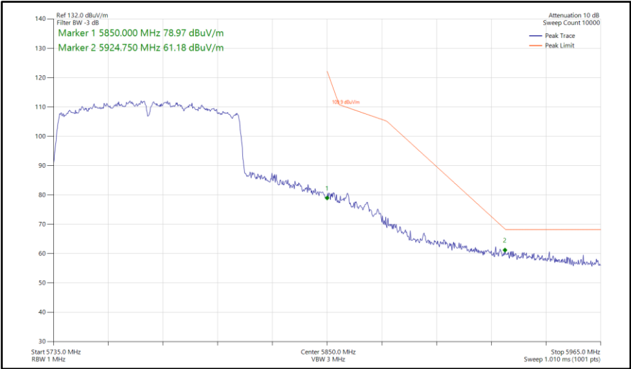
Figure 936 - 802.11ac VHT80, CDD, Core 0-1 - 5775 MHz Band Edge Frequency 5850 MHz
