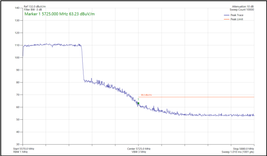
Figure 968 - 802.11ax HE80, SU, TxBF, Core 0-1 - 5610 MHz Band Edge Frequency 5725 MHz
