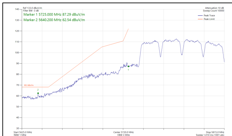
Figure 923 - 802.11a a80, CDD, Core 0-1 - 5775 MHz Band Edge Frequency 5725 MHz
