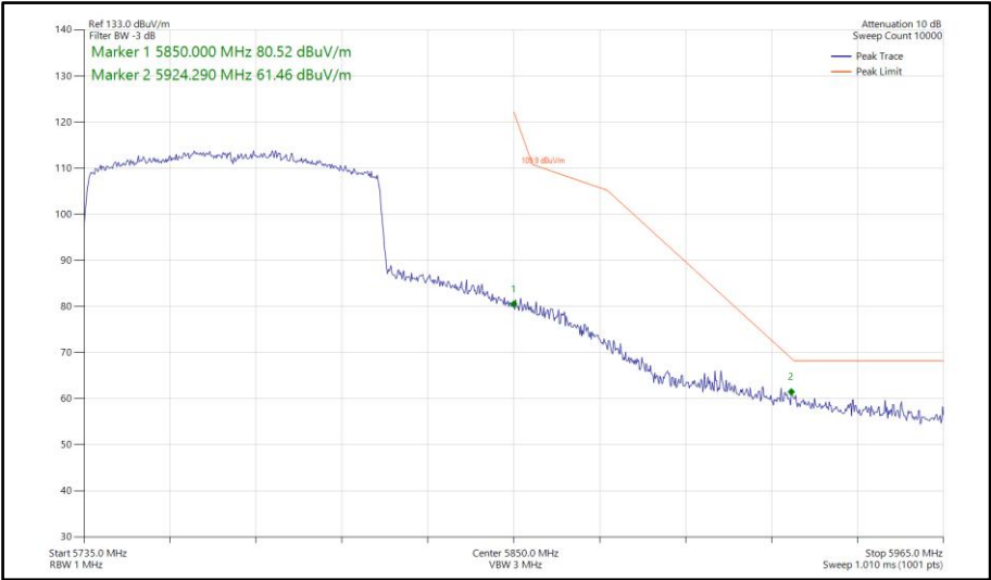
Figure 972 - 802.11ax HE80, SU, TxBF, Core 0-1 - 5775 MHz Band Edge Frequency 5850 MHz
