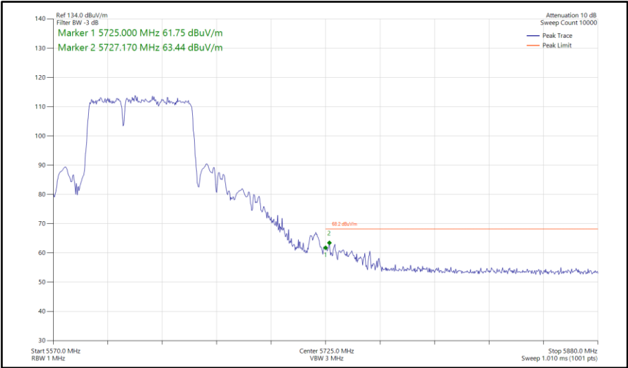
Figure 932 - 802.11be EHT80, RU 484+242-90, CDD, Core 0-1 - 5610 MHz Band Edge Frequency 5725 MHz
