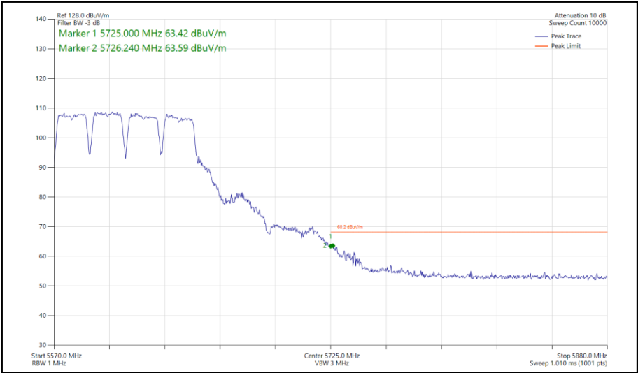
Figure 903 - 802.11a a80, SISO, Core 1 - 5610 MHz Band Edge Frequency 5725 MHz
