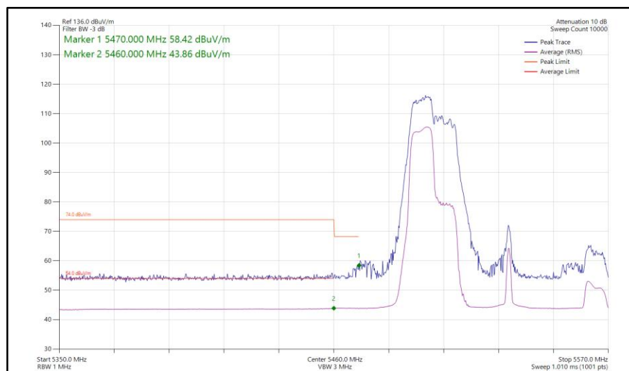
Figure 921 - 802.11ax HE80, RU 106-53, CDD, Core 0-1 - 5530 MHz Band Edge Frequency 5470 MHz
