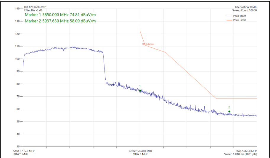
Figure 914 - 802.11ax HE80, SU, SISO, Core 1 - 5775 MHz Band Edge Frequency 5850 MHz
