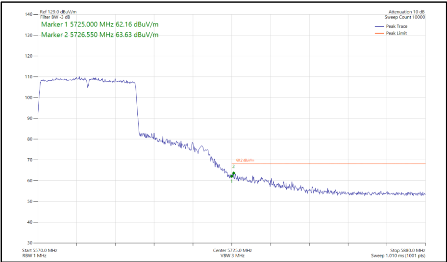
Figure 904 - 802.11ac VHT80, SISO, Core 1 - 5610 MHz Band Edge Frequency 5725 MHz
