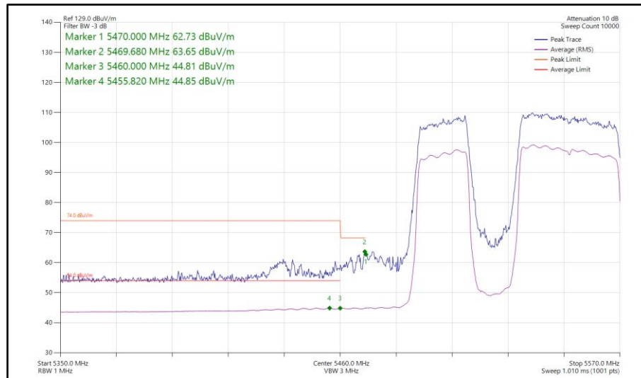
Figure 946 - 802.11be EHT80, RU 484+242-91, SDM, Core 0-1 - 5530 MHz Band Edge Frequency 5470 MHz
