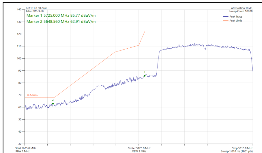
Figure 965 - 802.11ac VHT80, TxBF, Core 0-1 - 5775 MHz Band Edge Frequency 5725 MHz
