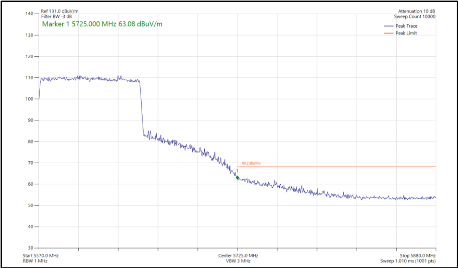
Figure 905 - 802.11ax HE80, SU, SISO, Core 1 - 5610 MHz Band Edge Frequency 5725 MHz
