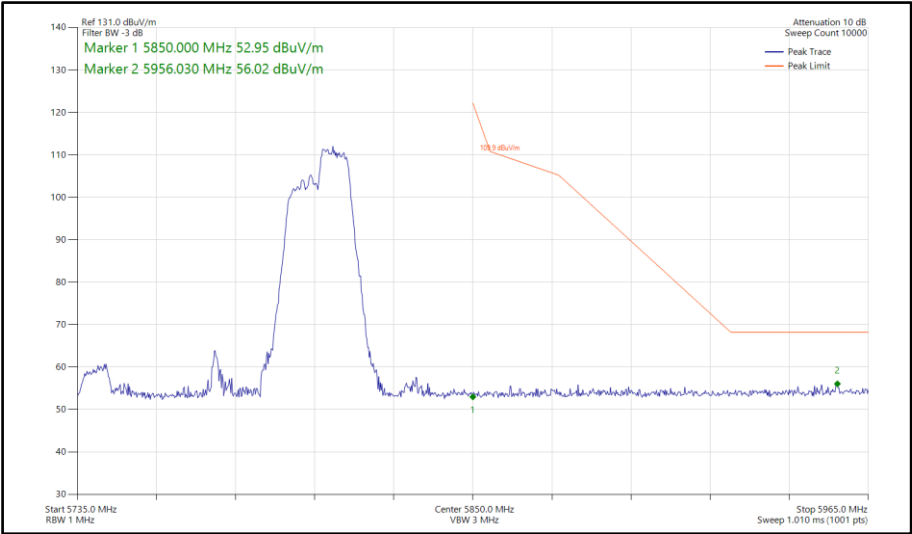
Figure 890 - 802.11ax HE80, RU 106-60, SISO, Core 0 - 5775 MHz Band Edge Frequency 5850 MHz
