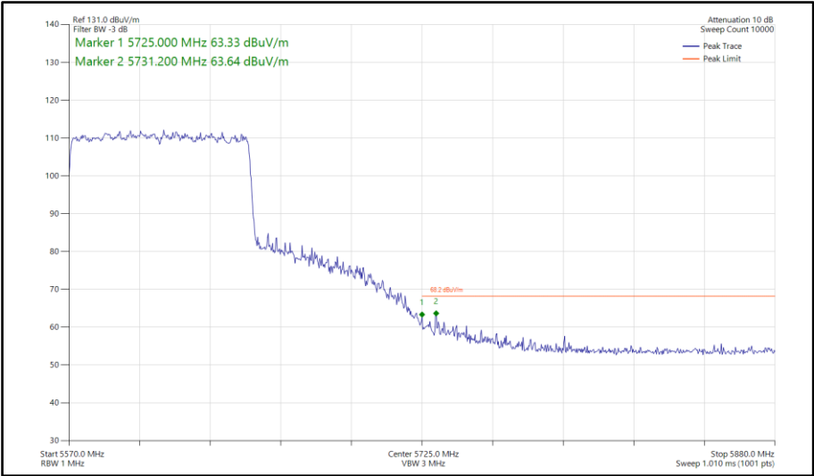
Figure 930 - 802.11ax HE80, SU, CDD, Core 0-1 - 5610 MHz Band Edge Frequency 5725 MHz
