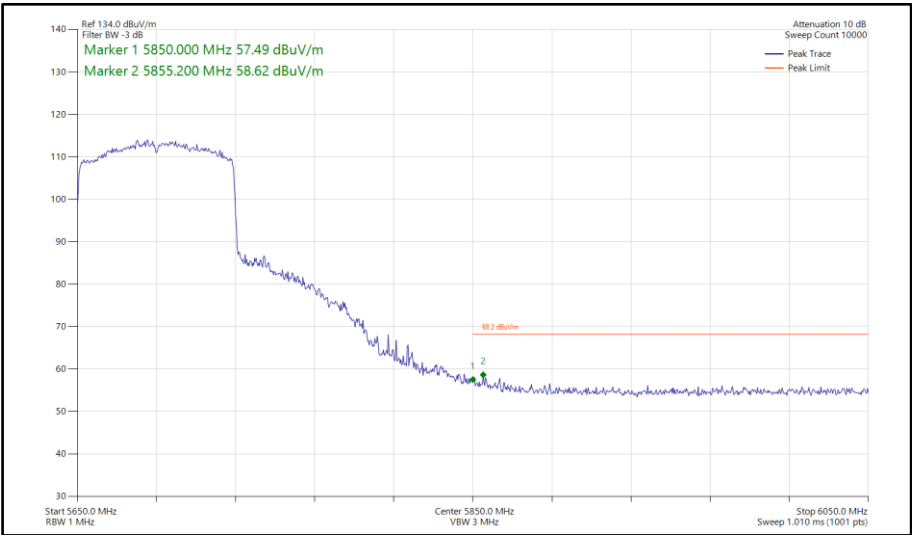
Figure 971 - 802.11ax HE80, SU, TxBF, Core 0-1 - 5690 MHz Band Edge Frequency 5850 MHz
