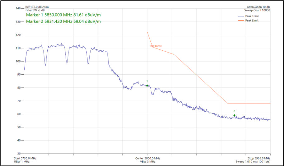
Figure 934 - 802.11a a80, CDD, Core 0-1 - 5775 MHz Band Edge Frequency 5850 MHz
