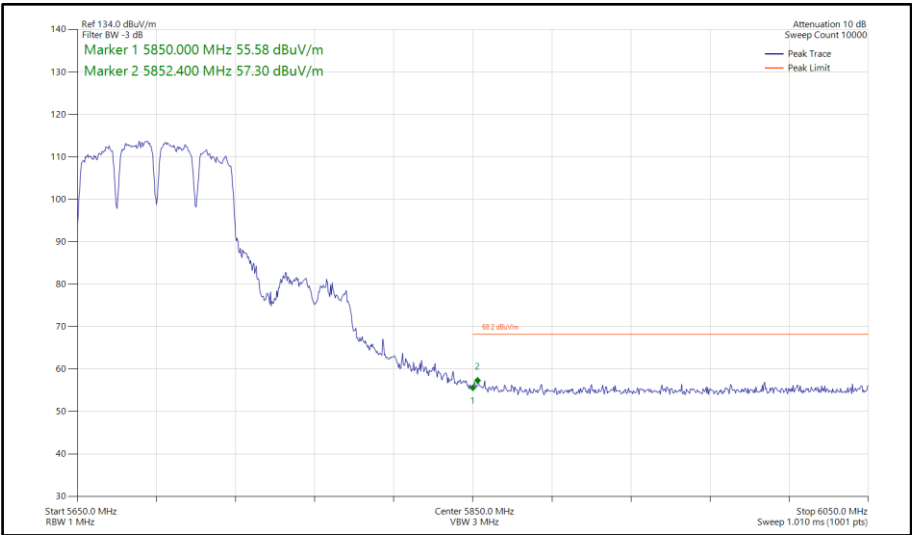
Figure 933 - 802.11a a80, CDD, Core 0-1 - 5690 MHz Band Edge Frequency 5850 MHz
