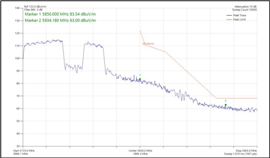
Figure 942 - 802.11be EHT80, RU 484+242-92, CDD, Core 0-1 - 5775 MHz Band Edge Frequency 5850 MHz
