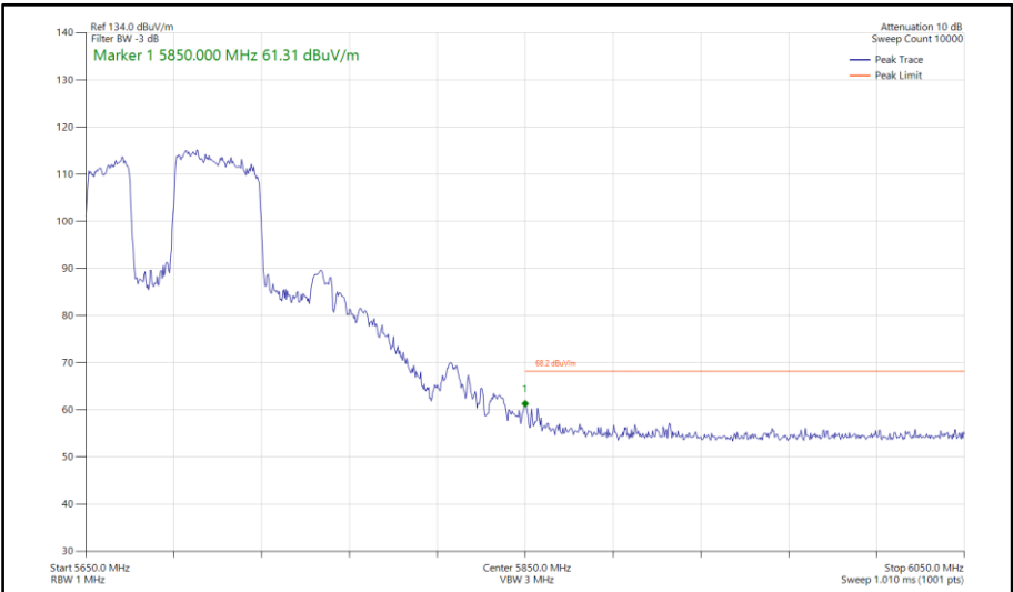
Figure 961 - 802.11be EHT80, RU 484+242-91, SDM, Core 0-1 - 5690 MHz Band Edge Frequency 5850 MHz
