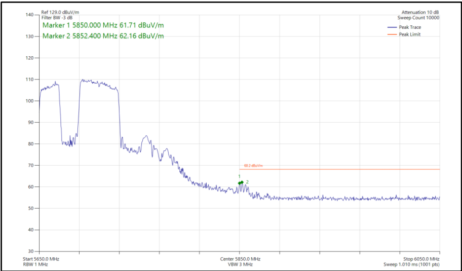
Figure 916 - 802.11be EHT80, RU 484+242-91, SISO, Core 1 - 5690 MHz Band Edge Frequency 5850 MHz
