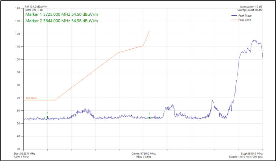
Figure 926 - 802.11ax HE80, RU 106-60, CDD, Core 0-1 - 5775 MHz Band Edge Frequency 5725 MHz
