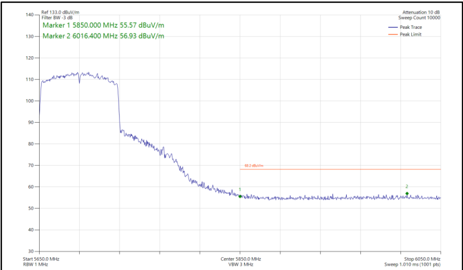
Figure 935 - 802.11ac VHT80, CDD, Core 0-1 - 5690 MHz Band Edge Frequency 5850 MHz
