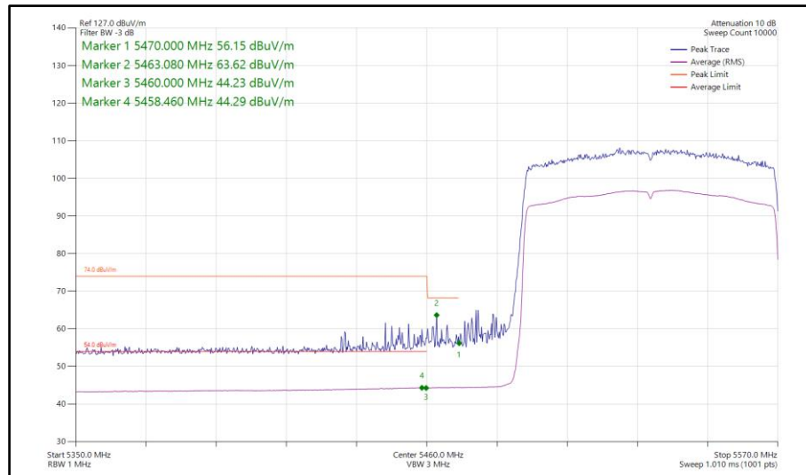
Figure 964 - 802.11ax HE80, SU, TxBF, Core 0-1 - 5530 MHz Band Edge Frequency 5470 MHz
