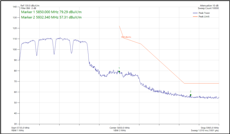
Figure 909 - 802.11a a80, SISO, Core 1 - 5775 MHz Band Edge Frequency 5850 MHz
