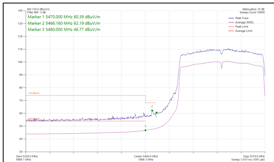
Figure 963 - 802.11ac VHT80, TxBF, Core 0-1 - 5530 MHz Band Edge Frequency 5470 MHz
