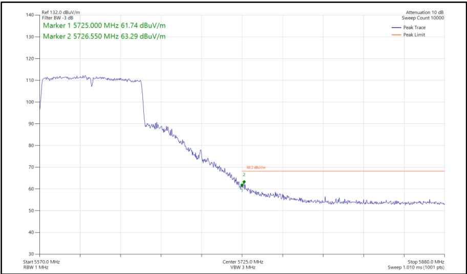
Figure 951 - 802.11ac VHT80, SDM, Core 0-1 - 5610 MHz Band Edge Frequency 5725 MHz
