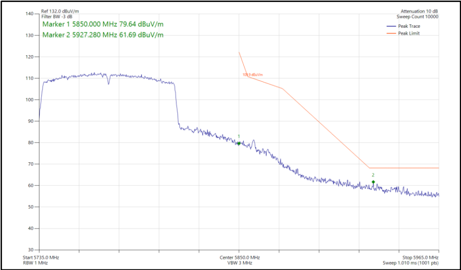
Figure 956 - 802.11ac VHT80, SDM, Core 0-1 - 5775 MHz Band Edge Frequency 5850 MHz
