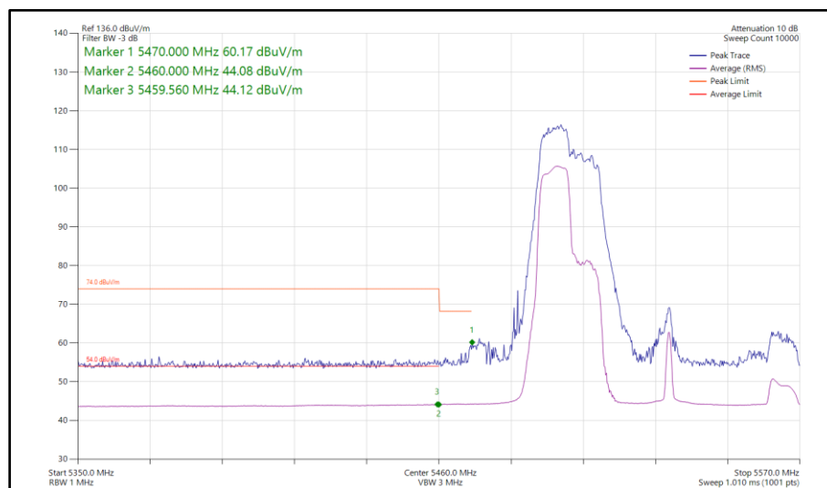
Figure 945 - 802.11ax HE80, RU 106-53, SDM, Core 0-1 - 5530 MHz Band Edge Frequency 5470 MHz
