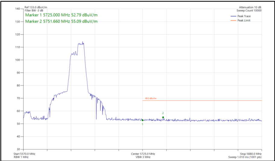
Figure 906 - 802.11ax HE80, RU 106-60, SISO, Core 1 - 5610 MHz Band Edge Frequency 5725 MHz
