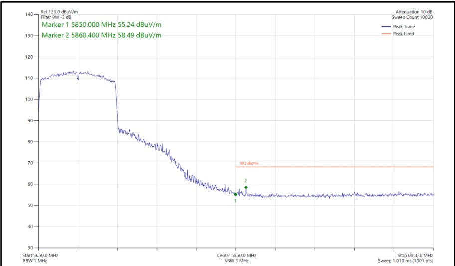
Figure 955 - 802.11ac VHT80, SDM, Core 0-1 - 5690 MHz Band Edge Frequency 5850 MHz
