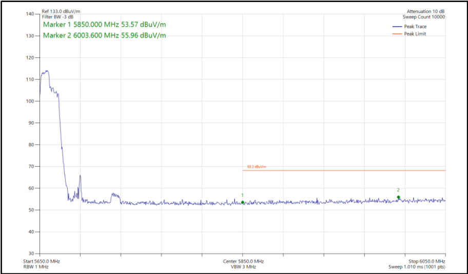
Figure 888 - 802.11ax HE80, RU 106-53, SISO, Core 0 - 5690 MHz Band Edge Frequency 5850 MHz
