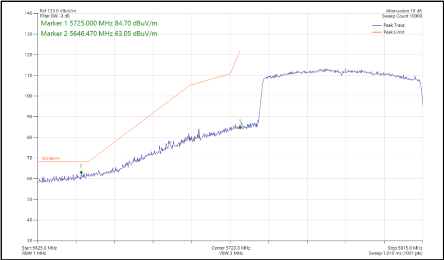
Figure 966 - 802.11ax HE80, SU, TxBF, Core 0-1 - 5775 MHz Band Edge Frequency 5725 MHz
