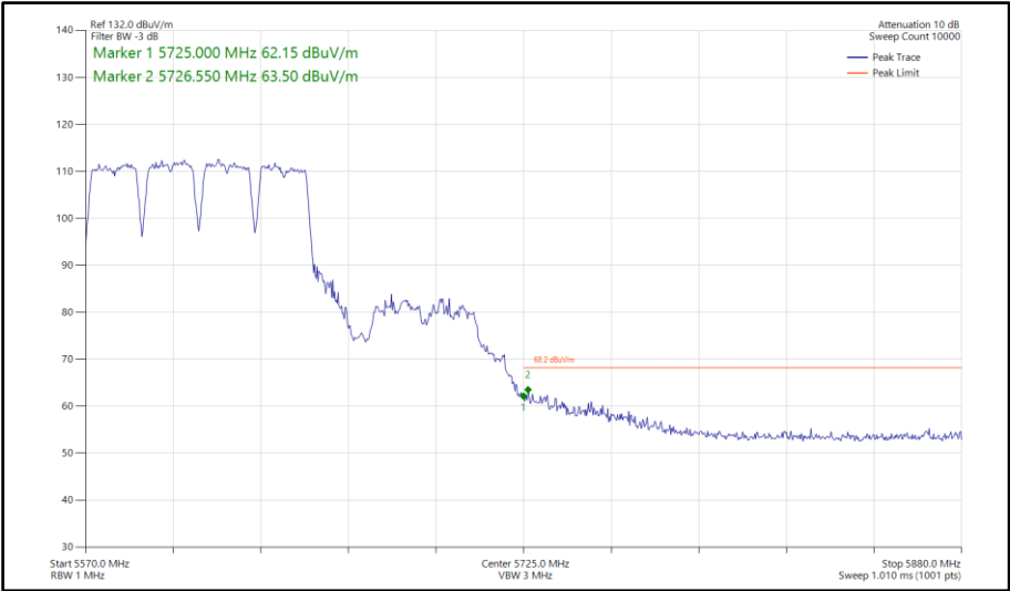
Figure 928 - 802.11a a80, CDD, Core 0-1 - 5610 MHz Band Edge Frequency 5725 MHz
