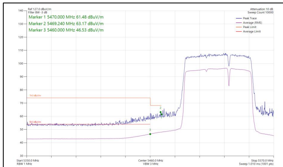
Figure 897 - 802.11be EHT80, RU 484+242-93, SISO, Core 1 - 5530 MHz Band Edge Frequency 5470 MHz
