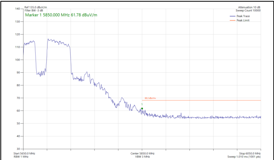
Figure 941 - 802.11be EHT80, RU 484+242-91, CDD, Core 0-1 - 5690 MHz Band Edge Frequency 5850 MHz
