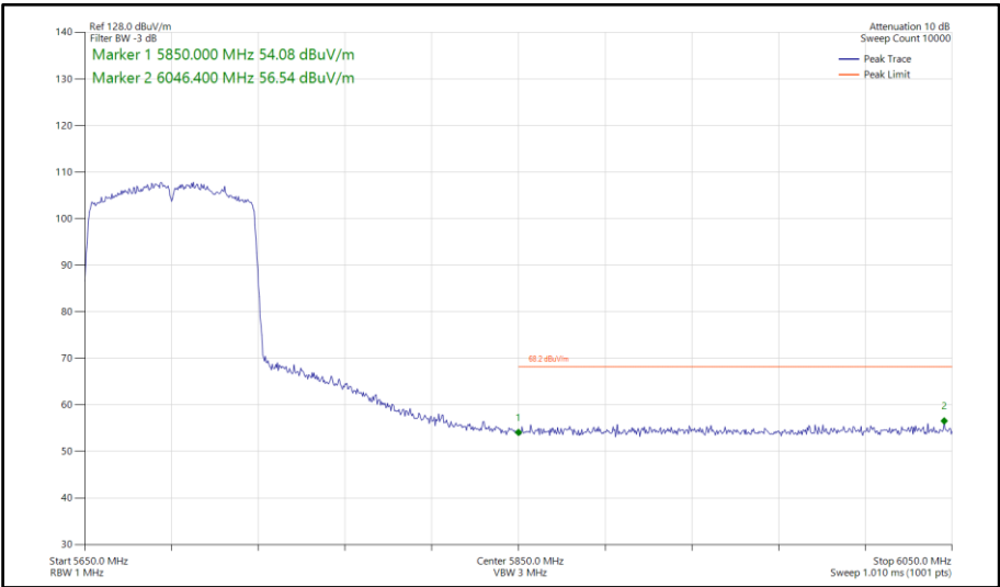
Figure 910 - 802.11ac VHT80, SISO, Core 1 - 5690 MHz Band Edge Frequency 5850 MHz
