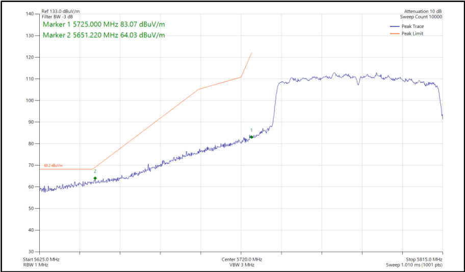
Figure 924 - 802.11ac VHT80, CDD, Core 0-1 - 5775 MHz Band Edge Frequency 5725 MHz
