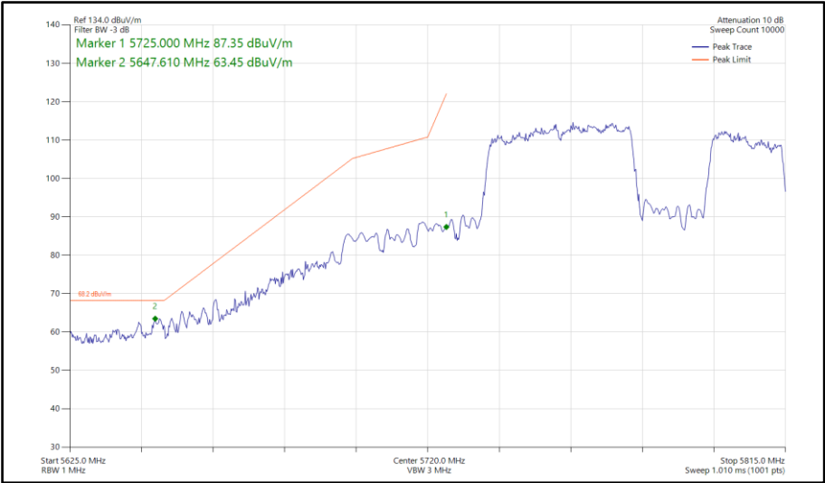
Figure 950 - 802.11be EHT80, RU 484+242-92, SDM, Core 0-1 - 5775 MHz Band Edge Frequency 5725 MHz
