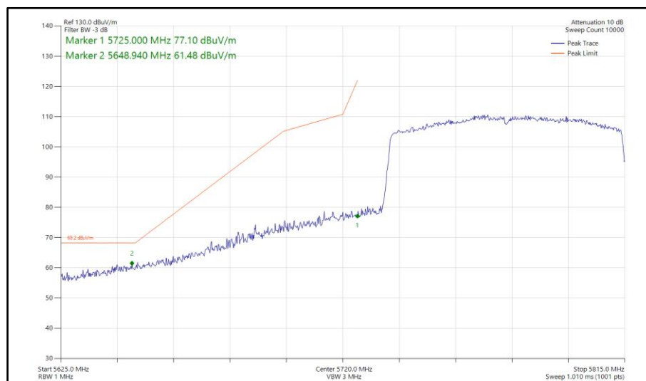
Figure 900 - 802.11ax HE80, SU, SISO, Core 1 - 5775 MHz Band Edge Frequency 5725 MHz
