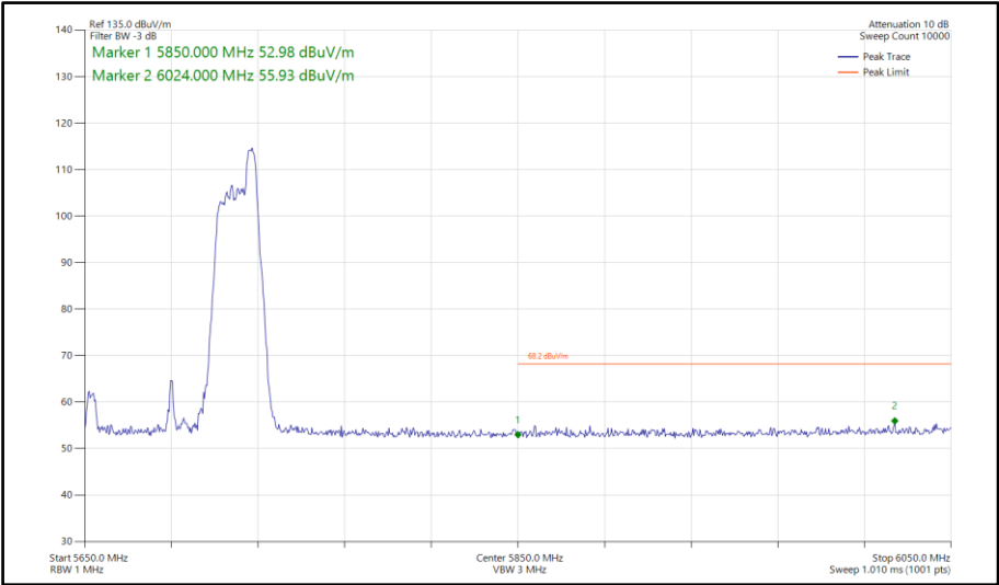
Figure 958 - 802.11ax HE80, RU 52-52, SDM, Core 0-1 - 5690 MHz Band Edge Frequency 5850 MHz
