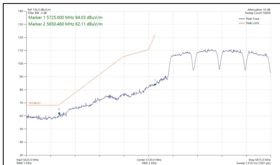
Figure 898 - 802.11a a80, SISO, Core 1 - 5775 MHz Band Edge Frequency 5725 MHz
