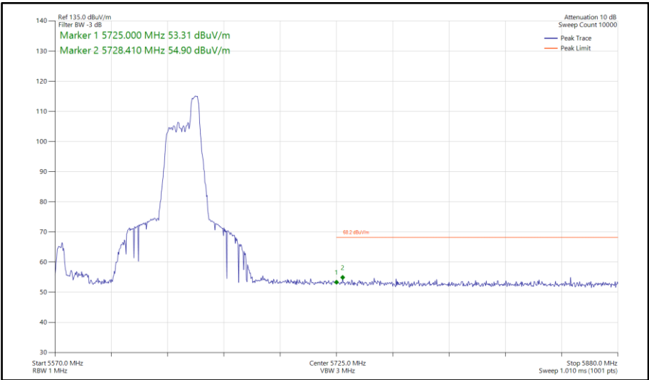
Figure 953 - 802.11ax HE80, RU 52-52, SDM, Core 0-1 - 5610 MHz Band Edge Frequency 5725 MHz
