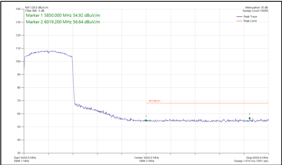
Figure 912 - 802.11ax HE80, SU, SISO, Core 1 - 5690 MHz Band Edge Frequency 5850 MHz
