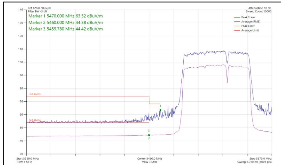
Figure 922 - 802.11be EHT80, RU 484+242-93, CDD, Core 0-1 - 5530 MHz Band Edge Frequency 5470 MHz
