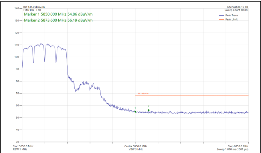
Figure 908 - 802.11a a80, SISO, Core 1 - 5690 MHz Band Edge Frequency 5850 MHz
