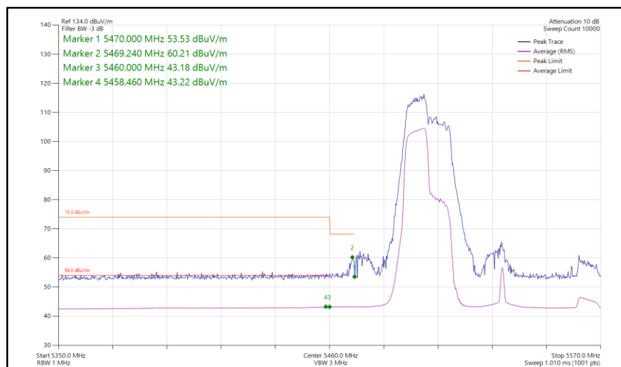
Figure 896 - 802.11ax HE80, RU 106-53, SISO, Core 1 - 5530 MHz Band Edge Frequency 5470 MHz
