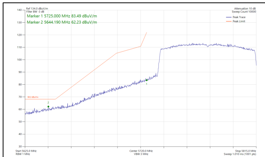
Figure 948 - 802.11ax HE80, SU, SDM, Core 0-1 - 5775 MHz Band Edge Frequency 5725 MHz
