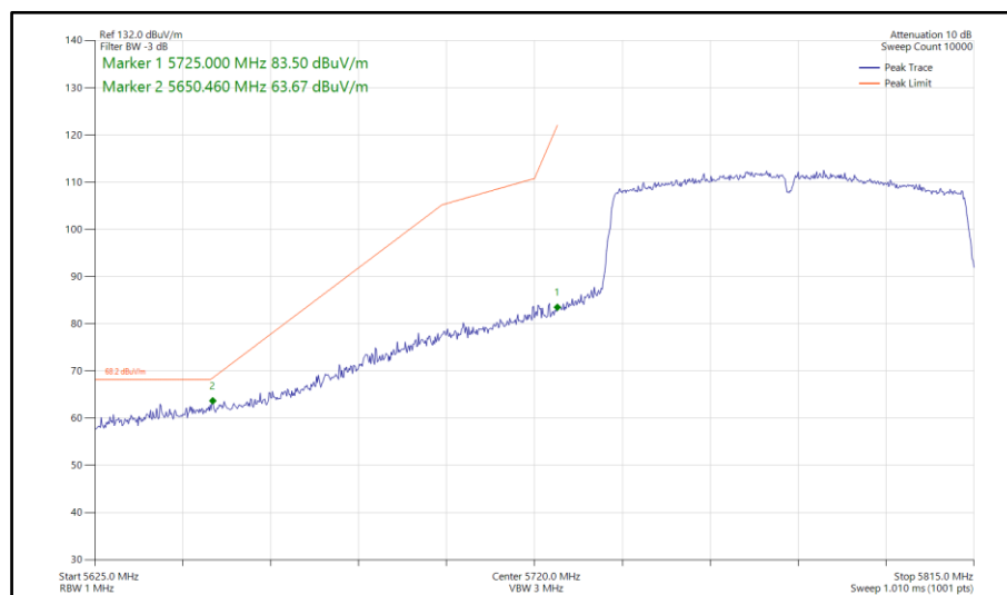
Figure 947 - 802.11ac VHT80, SDM, Core 0-1 - 5775 MHz Band Edge Frequency 5725 MHz
