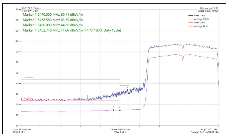
Figure 943 - 802.11ac VHT80, SDM, Core 0-1 - 5530 MHz Band Edge Frequency 5470 MHz
