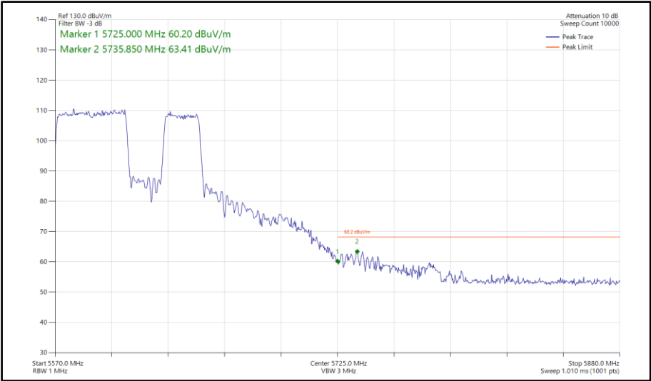
Figure 907 - 802.11be EHT80, RU 484+242-92, SISO, Core 1 - 5610 MHz Band Edge Frequency 5725 MHz
