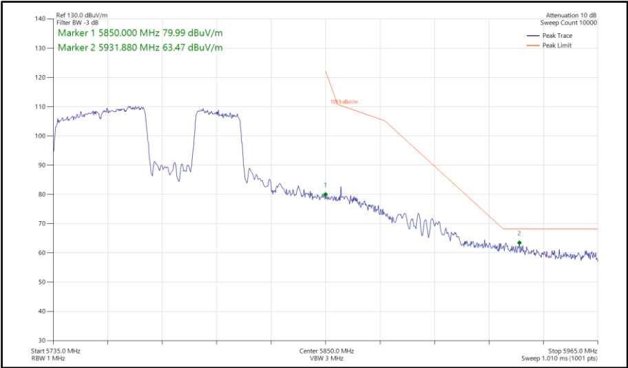
Figure 892 - 802.11be EHT80, RU 484+242-92, SISO, Core 0 - 5775 MHz Band Edge Frequency 5850 MHz
