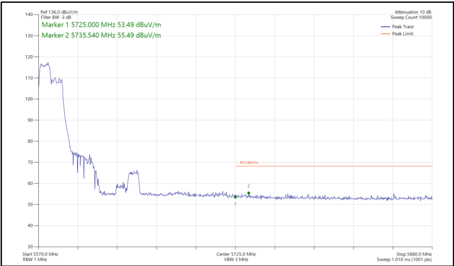
Figure 931 - 802.11ax HE80, RU 106-53, CDD, Core 0-1 - 5610 MHz Band Edge Frequency 5725 MHz
