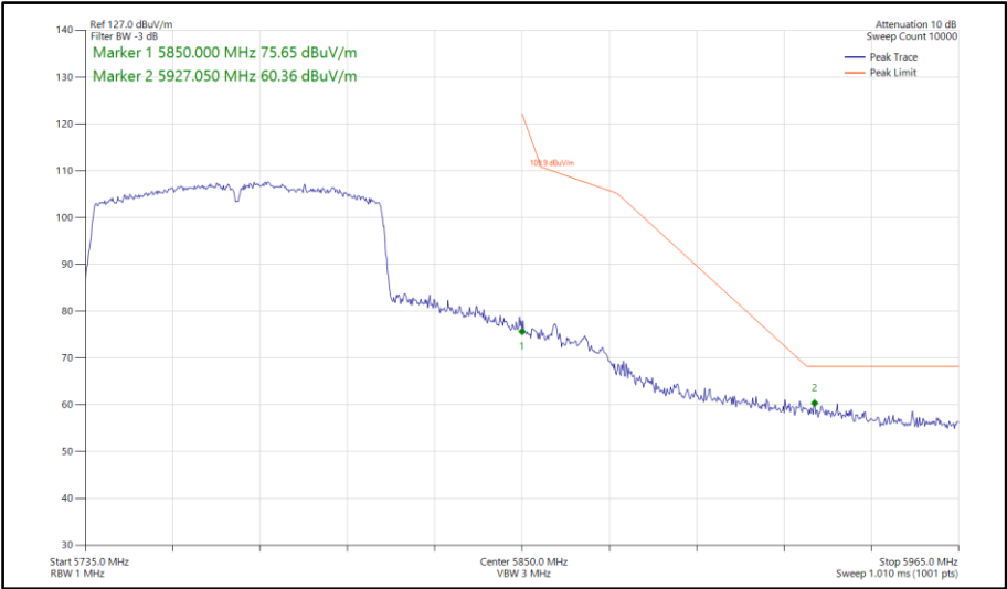
Figure 886 - 802.11ac VHT80, SISO, Core 0 - 5775 MHz Band Edge Frequency 5850 MHz
