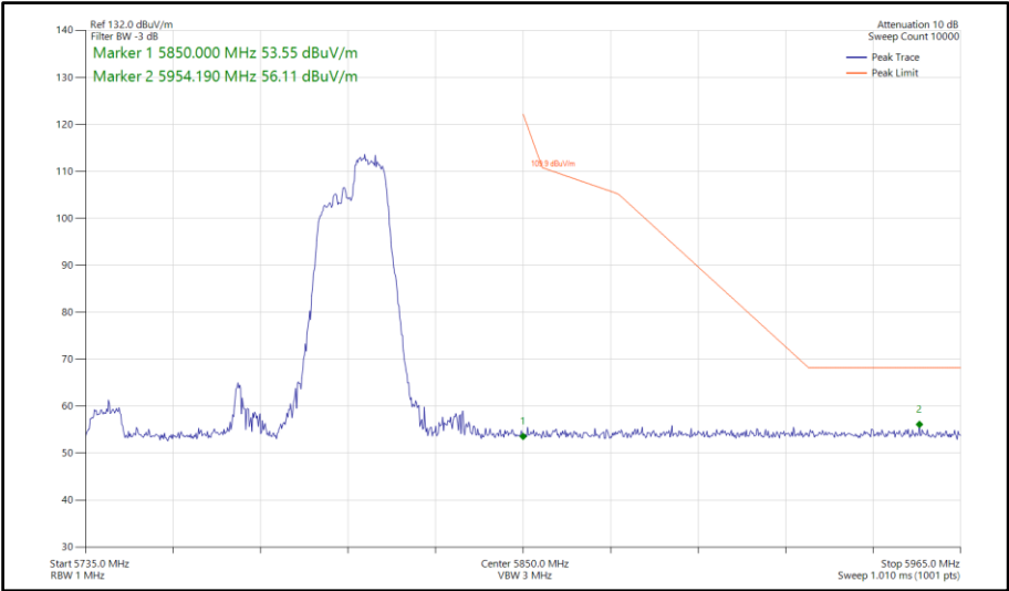
Figure 915 - 802.11ax HE80, RU 106-60, SISO, Core 1 - 5775 MHz Band Edge Frequency 5850 MHz
