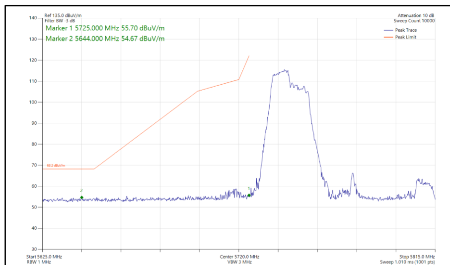
Figure 949 - 802.11ax HE80, RU 106-53, SDM, Core 0-1 - 5775 MHz Band Edge Frequency 5725 MHz
