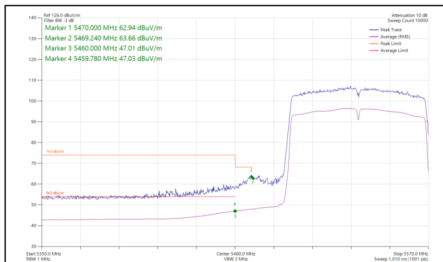
Figure 894 - 802.11ac VHT80, SISO, Core 1 - 5530 MHz Band Edge Frequency 5470 MHz
