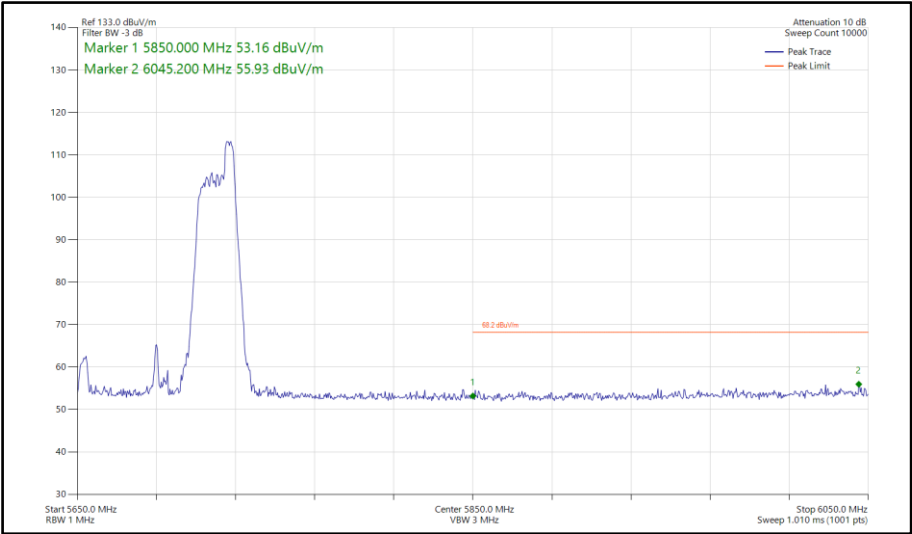
Figure 938 - 802.11ax HE80, RU 52-52, CDD, Core 0-1 - 5690 MHz Band Edge Frequency 5850 MHz
