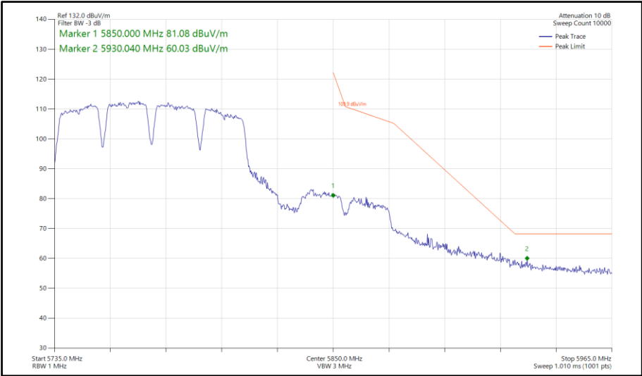
Figure 884 - 802.11a a80, SISO, Core 0 - 5775 MHz Band Edge Frequency 5850 MHz
