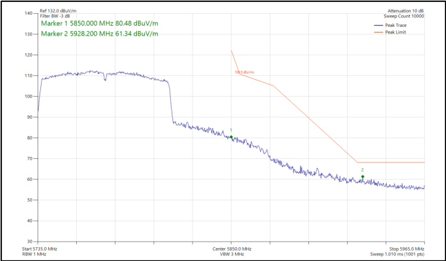
Figure 970 - 802.11ac VHT80, TxBF, Core 0-1 - 5775 MHz Band Edge Frequency 5850 MHz
