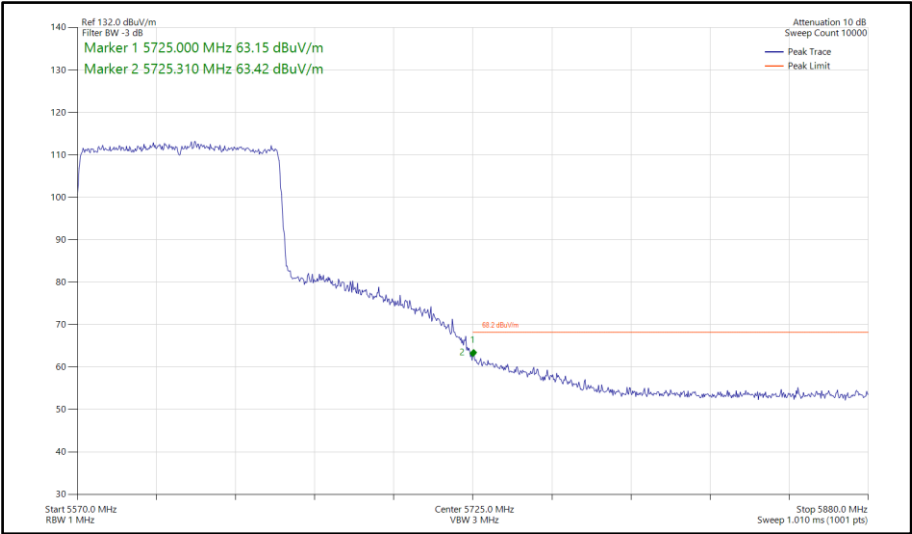
Figure 952 - 802.11ax HE80, SU, SDM, Core 0-1 - 5610 MHz Band Edge Frequency 5725 MHz
