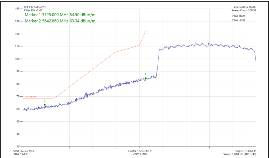
Figure 925 - 802.11ax HE80, SU, CDD, Core 0-1 - 5775 MHz Band Edge Frequency 5725 MHz
