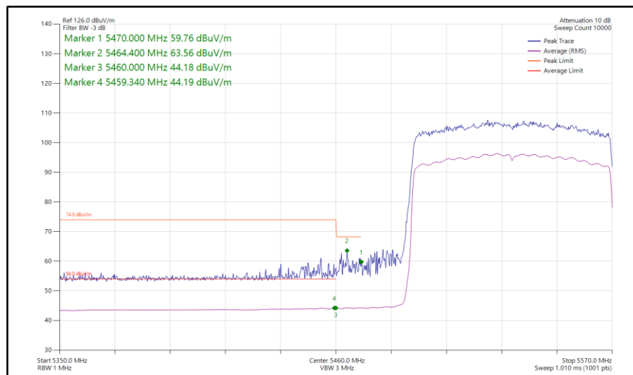
Figure 920 - 802.11ax HE80, SU, CDD, Core 0-1 - 5530 MHz Band Edge Frequency 5470 MHz
