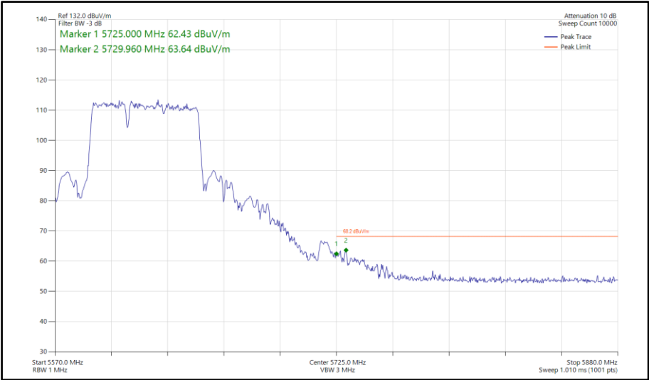
Figure 954 - 802.11be EHT80, RU 484+242-90, SDM, Core 0-1 - 5610 MHz Band Edge Frequency 5725 MHz
