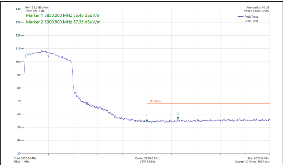
Figure 885 - 802.11ac VHT80, SISO, Core 0 - 5690 MHz Band Edge Frequency 5850 MHz
