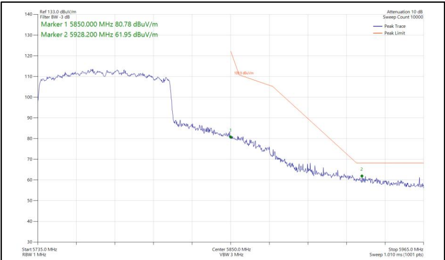
Figure 939 - 802.11ax HE80, SU, CDD, Core 0-1 - 5775 MHz Band Edge Frequency 5850 MHz
