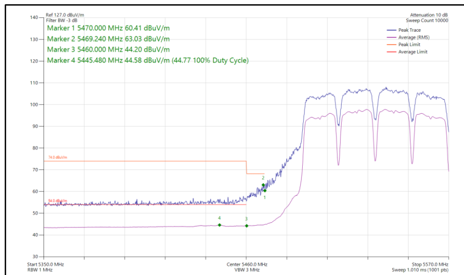
Figure 918 - 802.11a a80, CDD, Core 0-1 - 5530 MHz Band Edge Frequency 5470 MHz
