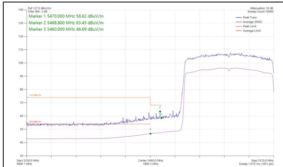
Figure 895 - 802.11ax HE80, SU, SISO, Core 1 - 5530 MHz Band Edge Frequency 5470 MHz
