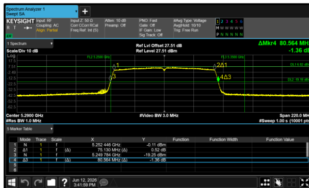
Figure 5 - 802.11ac VHT80 Minimum 26 dB EBW
