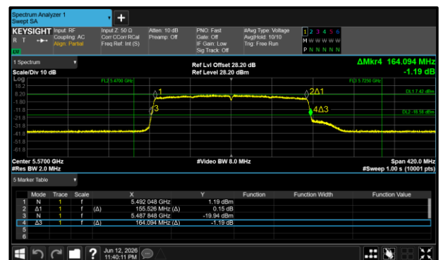
Figure 16 - 802.11ax HE160 SU Maximum 26 dB EBW
