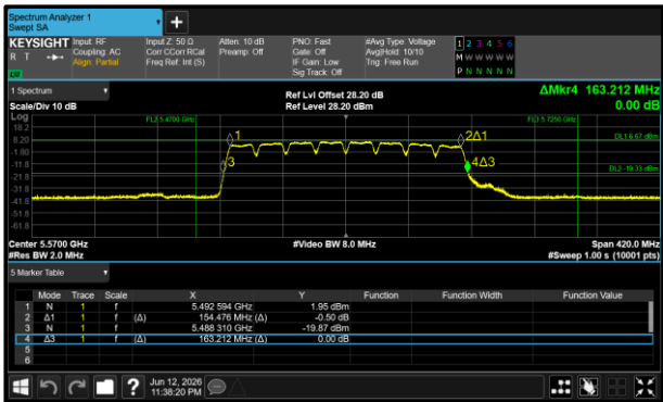
Figure 24 - 802.11a160 Maximum 26 dB EBW
