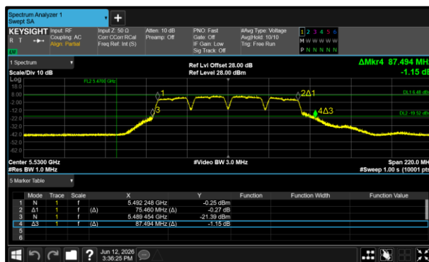
Figure 21 - 802.11a80 Minimum 26 dB EBW
