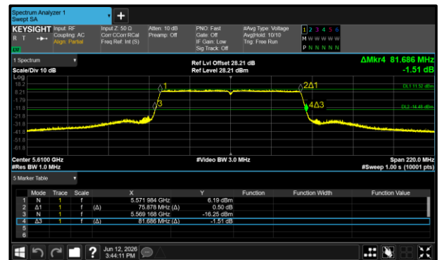
Figure 6 - 802.11ac VHT80 Maximum 26 dB EBW
