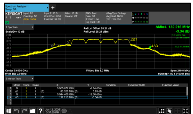
Figure 22 - 802.11a80 Maximum 26 dB EBW
