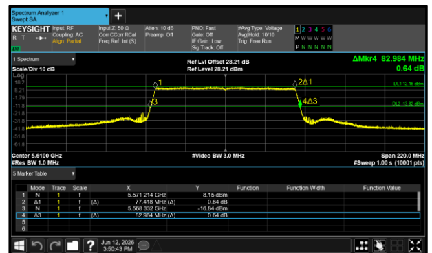
Figure 14 - 802.11ax HE80 SU Maximum 26 dB EBW
