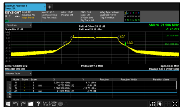
Figure 18 - 802.11a20 Maximum 26 dB EBW
