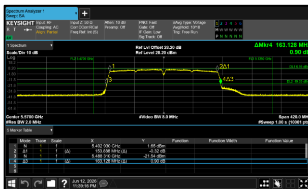
Figure 7 - 802.11ac VHT160 Minimum 26 dB EBW
