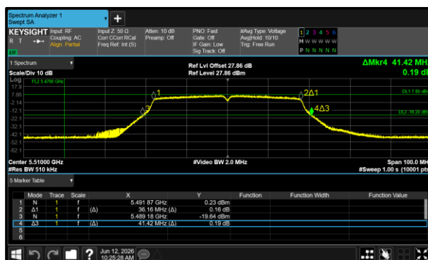
Figure 3 - 802.11n HT40 Minimum 26 dB EBW
