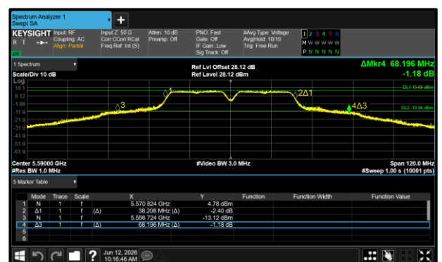
Figure 20 - 802.11a40 Maximum 26 dB EBW
