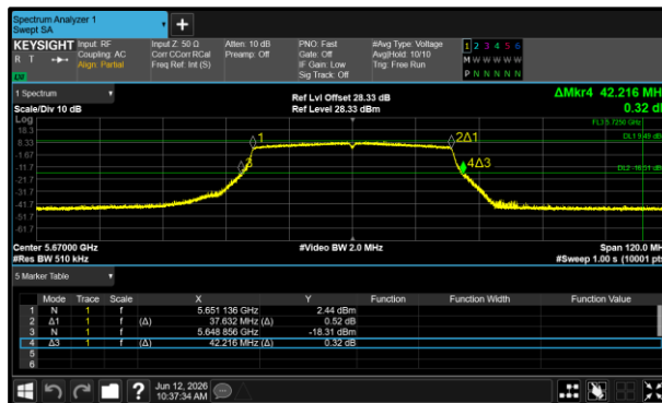
Figure 11 - 802.11ax HE40 SU Minimum 26 dB EBW
