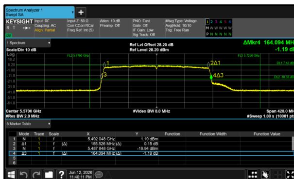
Figure 15 - 802.11ax HE160 SU Minimum 26 dB EBW
