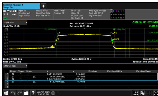
Figure 13 - 802.11ax HE80 SU Minimum 26 dB EBW
