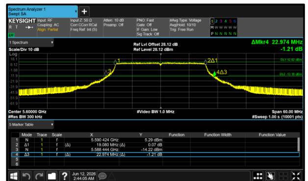
Figure 10 - 802.11ax HE20 SU Maximum 26 dB EBW
