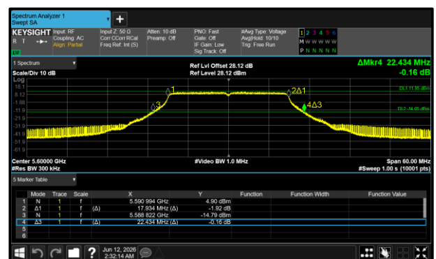
Figure 2 - 802.11n HT20 Maximum 26 dB EBW
