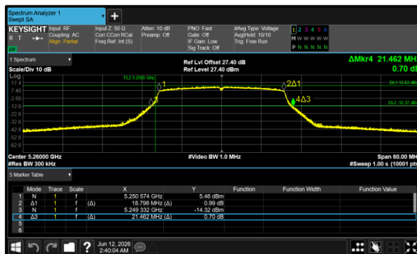
Figure 9 - 802.11ax HE20 SU Minimum 26 dB EBW
