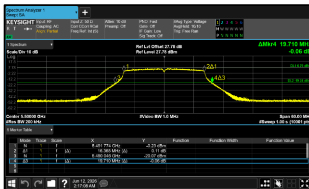
Figure 17 - 802.11a20 Minimum 26 dB EBW
