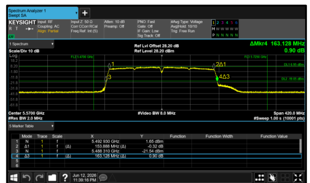
Figure 8 - 802.11ac VHT160 Maximum 26 dB EBW
