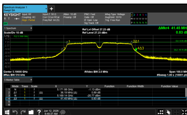
Figure 19 - 802.11a40 Minimum 26 dB EBW
