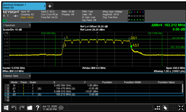
Figure 23 - 802.11a160 Minimum 26 dB EBW
