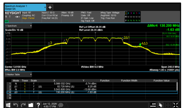
Figure 196 - 802.11a80 Maximum 99% OBW
