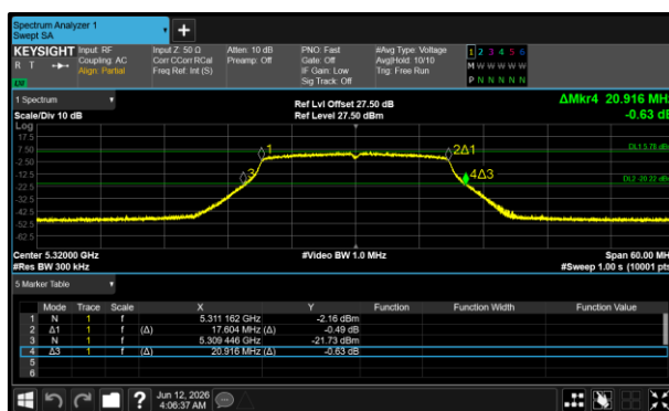
Figure 133 - 802.11n HT20 Minimum 26 dB EBW
