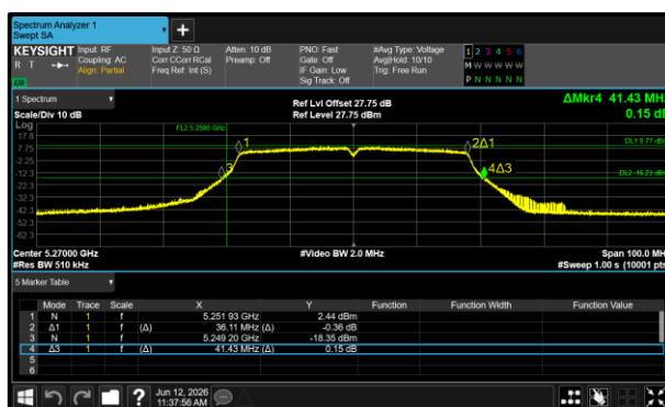
Figure 177 - 802.11n HT40 Minimum 99% OBW
