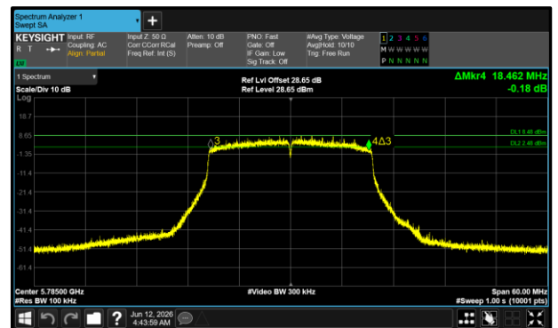
Figure 164 - 802.11ax HE20 SU Maximum 6 dB EBW
