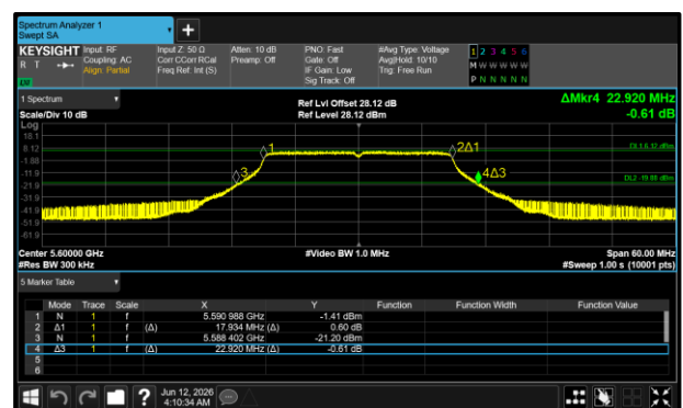
Figure 134 - 802.11n HT20 Maximum 26 dB EBW
