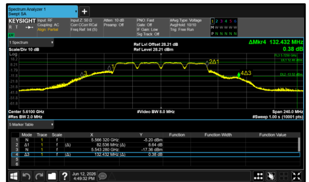
Figure 154 - 802.11a80 Maximum 26 dB EBW
