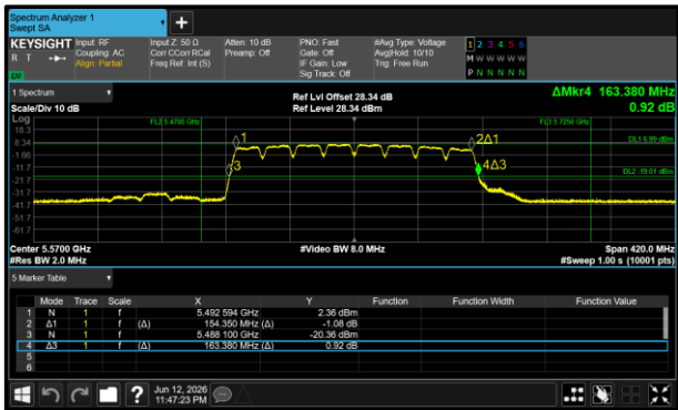
Figure 131 - 802.11a160 Minimum 99% OBW
