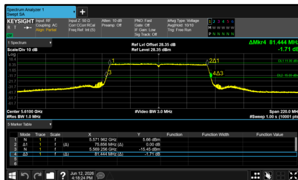
Figure 114 - 802.11ac VHT80 Maximum 99% OBW
