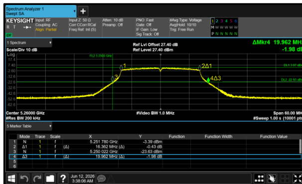
Figure 191 - 802.11a20 Minimum 99% OBW
