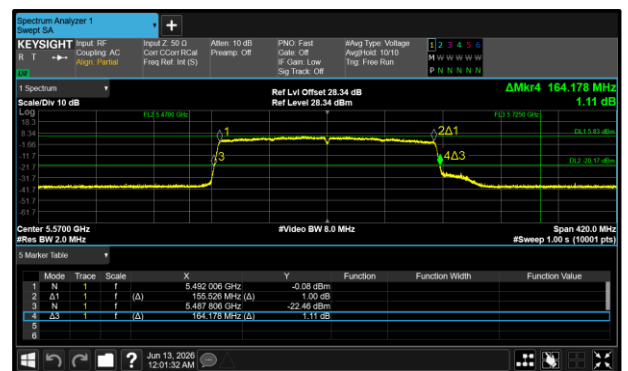
Figure 148 - 802.11ax HE160 SU Maximum 26 dB EBW
