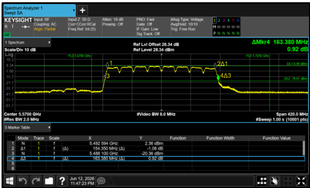
Figure 132 - 802.11a160 Maximum 99% OBW
