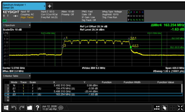
Figure 198 - 802.11a160 Maximum 99% OBW
