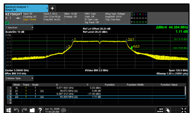
Figure 178 - 802.11n HT40 Maximum 99% OBW
