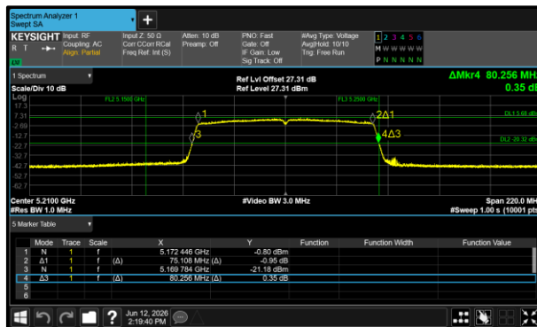
Figure 137 - 802.11ac VHT80 Minimum 26 dB EBW
