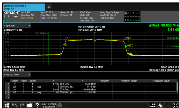
Figure 113 - 802.11ac VHT80 Minimum 99% OBW
