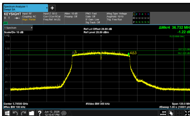
Figure 165 - 802.11ax HE40 SU Minimum 6 dB EBW
