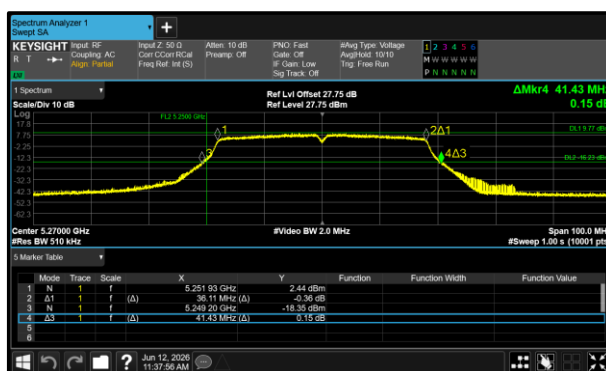
Figure 135 - 802.11n HT40 Minimum 26 dB EBW
