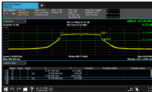
Figure 149 - 802.11a20 Minimum 26 dB EBW
