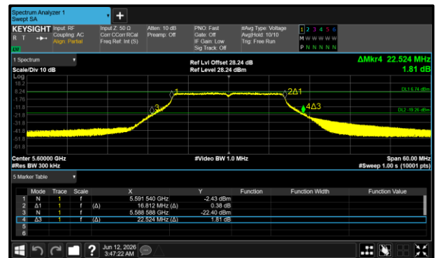
Figure 150 - 802.11a20 Maximum 26 dB EBW
