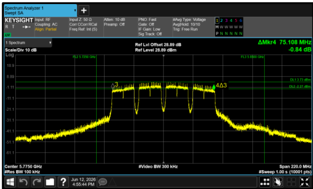
Figure 173 - 802.11a80 Minimum 6 dB EBW
