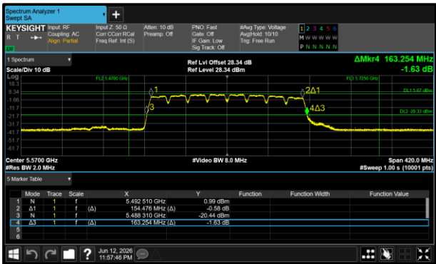
Figure 156 - 802.11a160 Maximum 26 dB EBW
