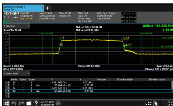
Figure 123 - 802.11ax HE160 SU Minimum 99% OBW
