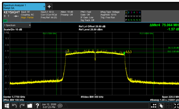
Figure 161 - 802.11ac VHT80 Minimum 6 dB EBW
