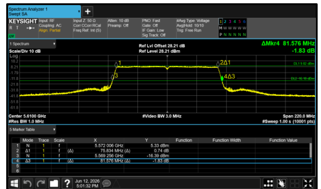
Figure 138 - 802.11ac VHT80 Maximum 26 dB EBW
