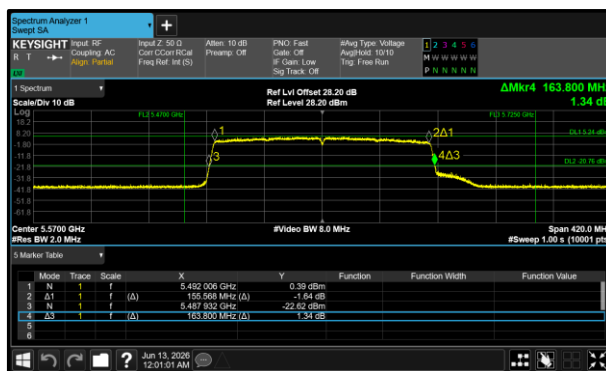
Figure 147 - 802.11ax HE160 SU Minimum 26 dB EBW
