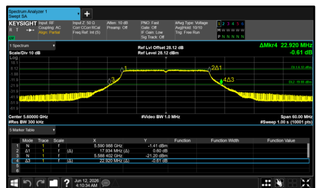
Figure 176 - 802.11n HT20 Maximum 99% OBW
