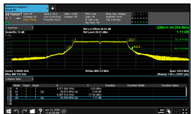
Figure 136 - 802.11n HT40 Maximum 26 dB EBW
