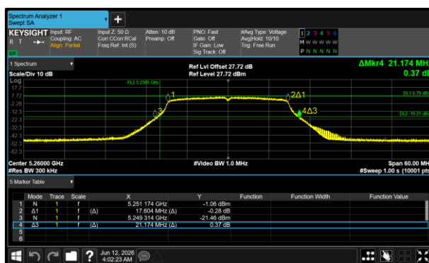
Figure 175 - 802.11n HT20 Minimum 99% OBW
