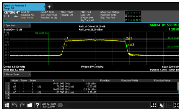
Figure 145 - 802.11ax HE80 SU Minimum 26 dB EBW
