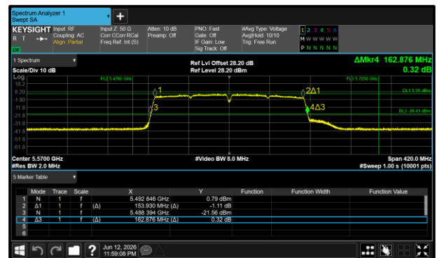
Figure 140 - 802.11ac VHT160 Maximum 26 dB EBW
