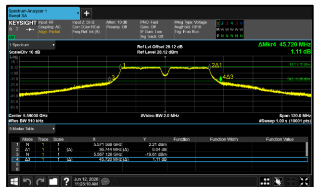
Figure 152 - 802.11a40 Maximum 26 dB EBW
