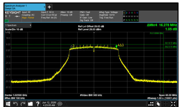
Figure 158 - 802.11n HT20 Maximum 6 dB EBW
