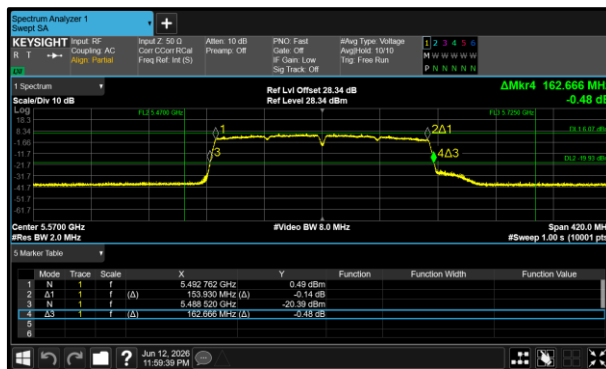
Figure 139 - 802.11ac VHT160 Minimum 26 dB EBW
