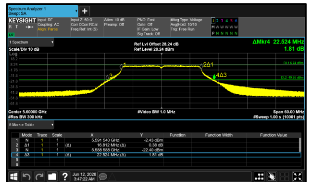
Figure 192 - 802.11a20 Maximum 99% OBW
