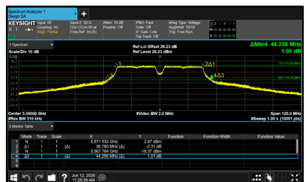
Figure 194 - 802.11a40 Maximum 99% OBW
