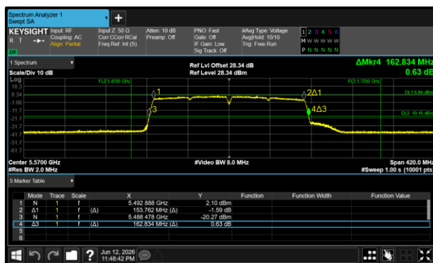
Figure 115 - 802.11ac VHT160 Minimum 99% OBW
