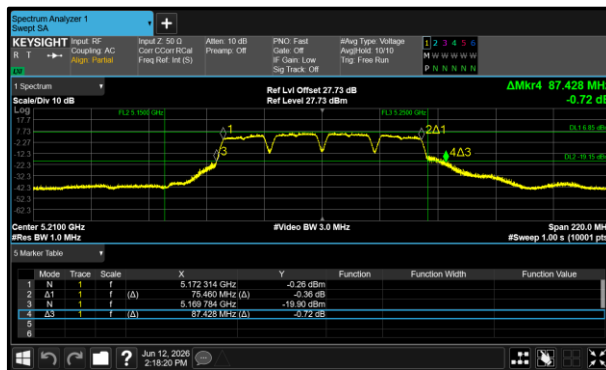
Figure 153 - 802.11a80 Minimum 26 dB EBW
