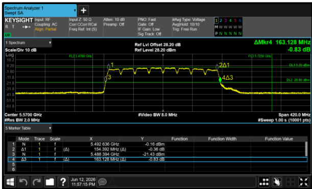
Figure 155 - 802.11a160 Minimum 26 dB EBW
