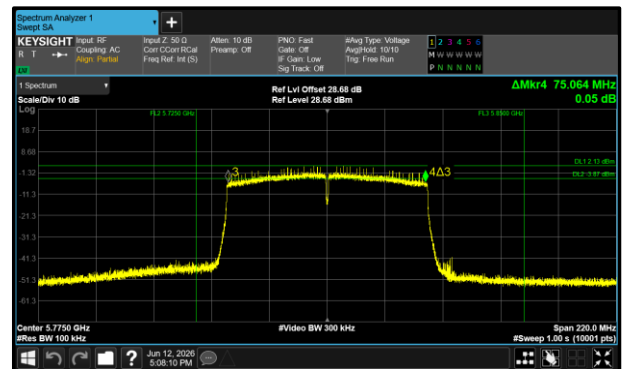
Figure 162 - 802.11ac VHT80 Maximum 6 dB EBW
