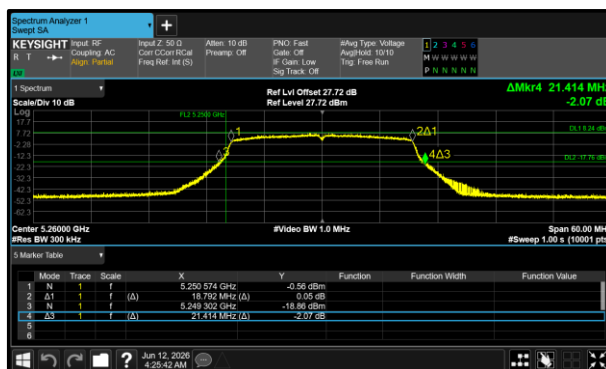
Figure 141 - 802.11ax HE20 SU Minimum 26 dB EBW
