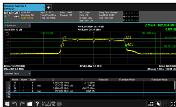
Figure 116 - 802.11ac VHT160 Maximum 99% OBW
