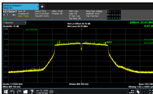
Figure 159 - 802.11n HT40 Minimum 6 dB EBW
