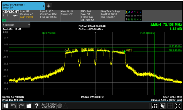
Figure 174 - 802.11a80 Maximum 6 dB EBW
