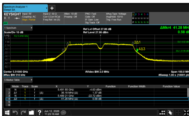
Figure 151 - 802.11a40 Minimum 26 dB EBW
