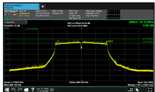
Figure 160 - 802.11n HT40 Maximum 6 dB EBW
