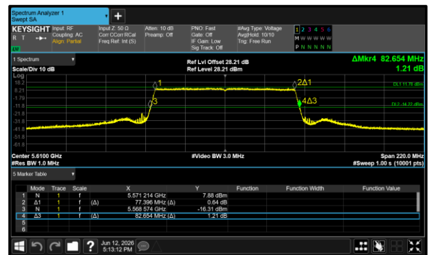
Figure 146 - 802.11ax HE80 SU Maximum 26 dB EBW
