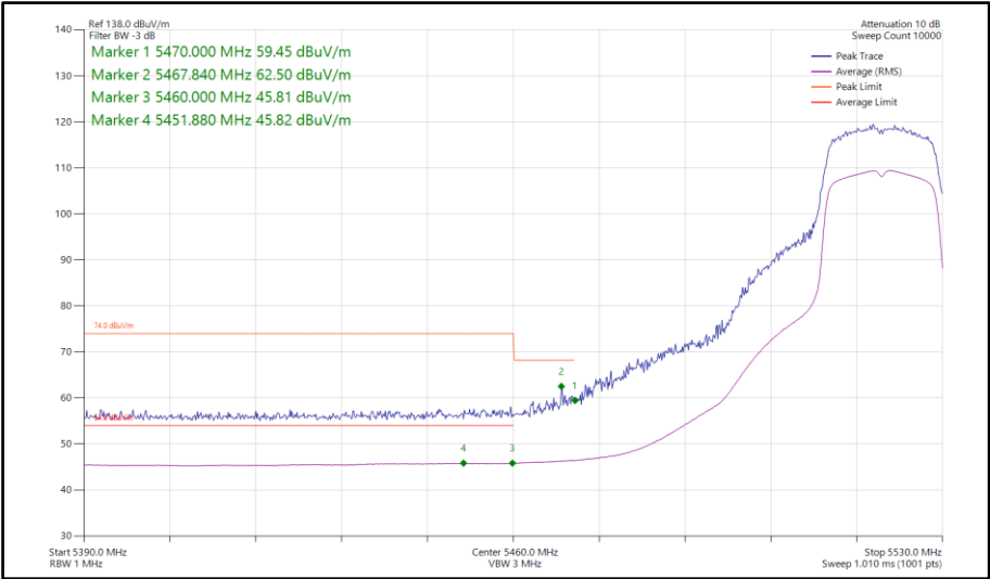
Figure 372 - 802.11n HT20, SDM, Core 0-1 - 5520 MHz Band Edge Frequency 5460 MHz
