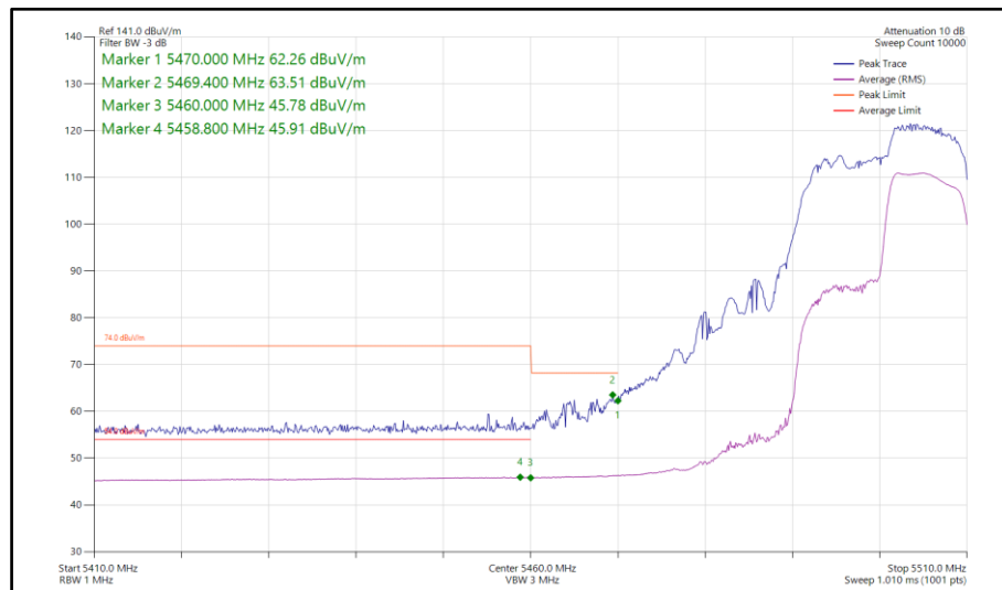
Figure 356 - 802.11ax HE20, RU 106-54, CDD, Core 0-1 - 5500 MHz Band Edge Frequency 5460 MHz
