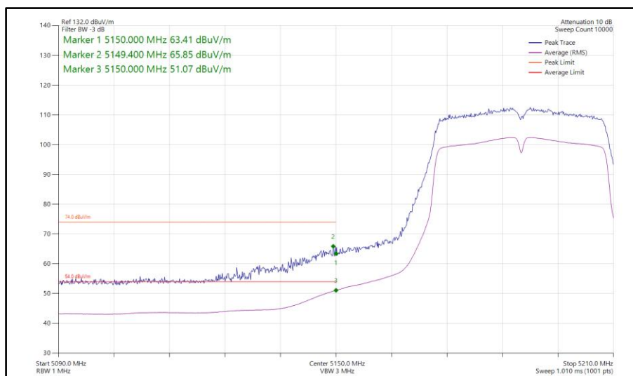
Figure 391 - 802.11n HT40, SISO, Core 0 - 5190 MHz Band Edge Frequency 5150 MHz
