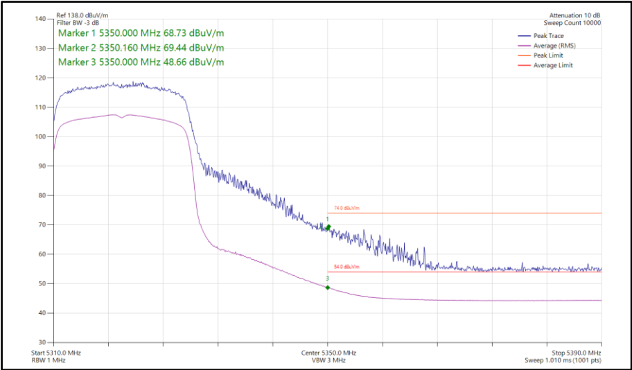
Figure 368 - 802.11ax HE20, SU, SDM, Core 0-1 - 5320 MHz Band Edge Frequency 5350 MHz
