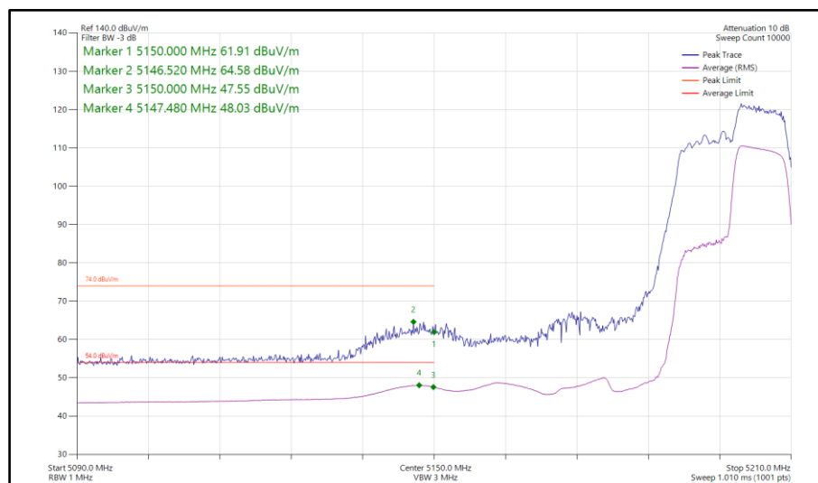
Figure 394 - 802.11ax HE40, RU 106-56, SISO, Core 0 - 5190 MHz Band Edge Frequency 5150 MHz
