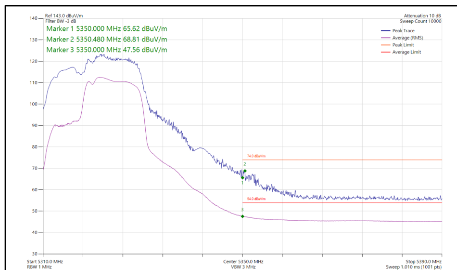
Figure 350 - 802.11be EHT20, RU 106+26-83, CDD, Core 0-1 - 5320 MHz Band Edge Frequency 5350 MHz
