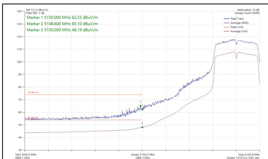
Figure 392 - 802.11n HT40, SISO, Core 0 - 5230 MHz Band Edge Frequency 5150 MHz
