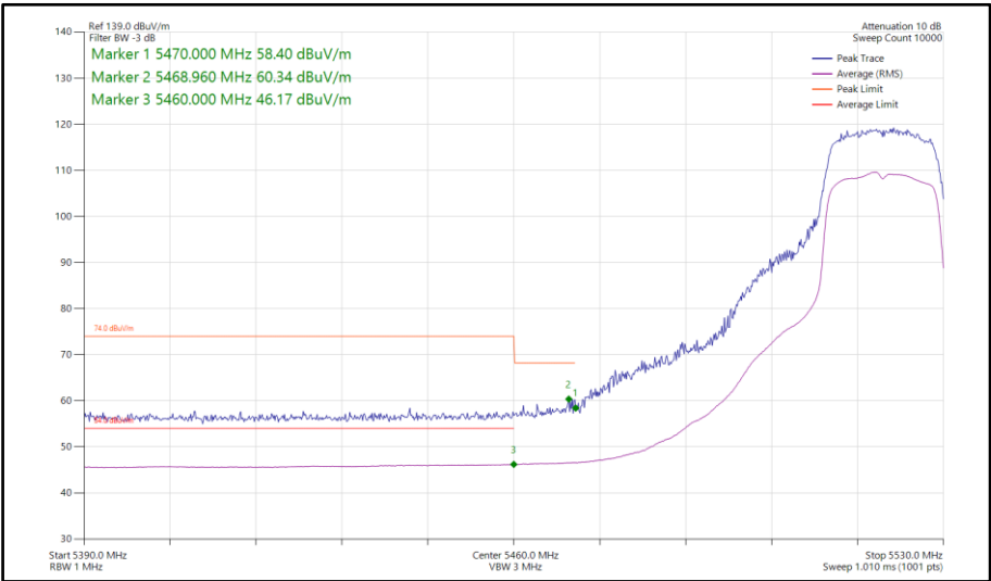
Figure 354 - 802.11n HT20, CDD, Core 0-1 - 5520 MHz Band Edge Frequency 5460 MHz
