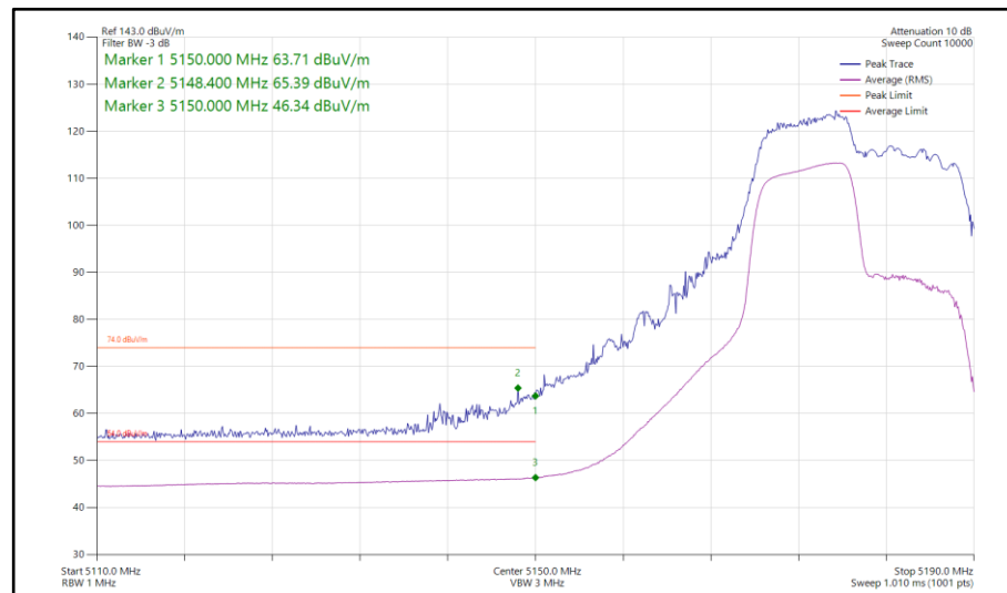
Figure 342 - 802.11be EHT20, RU 106+26-83, CDD, Core 0-1 - 5180 MHz Band Edge Frequency 5150 MHz
