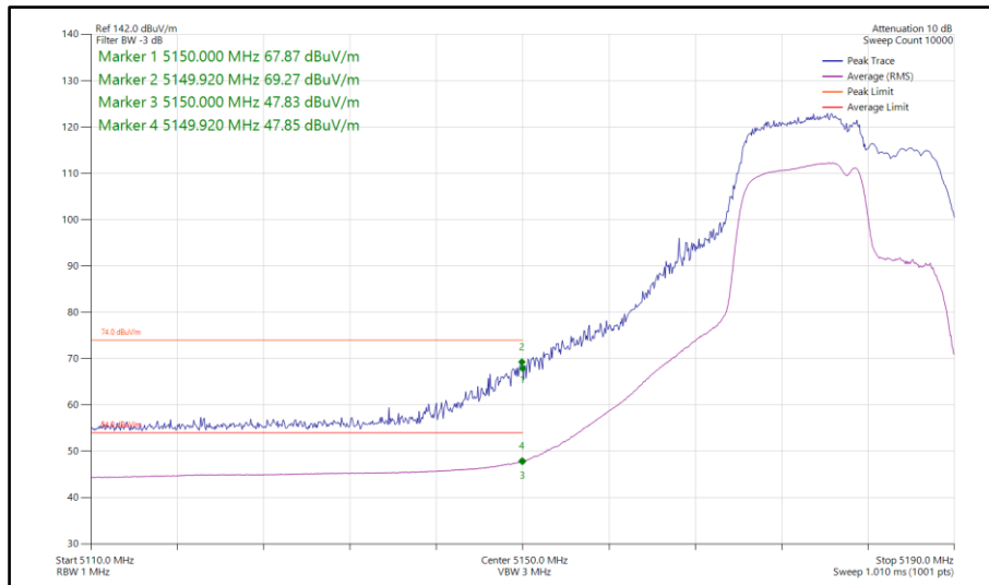
Figure 364 - 802.11be EHT20, RU 106+26-82, SDM, Core 0-1 - 5180 MHz Band Edge Frequency 5150 MHz
