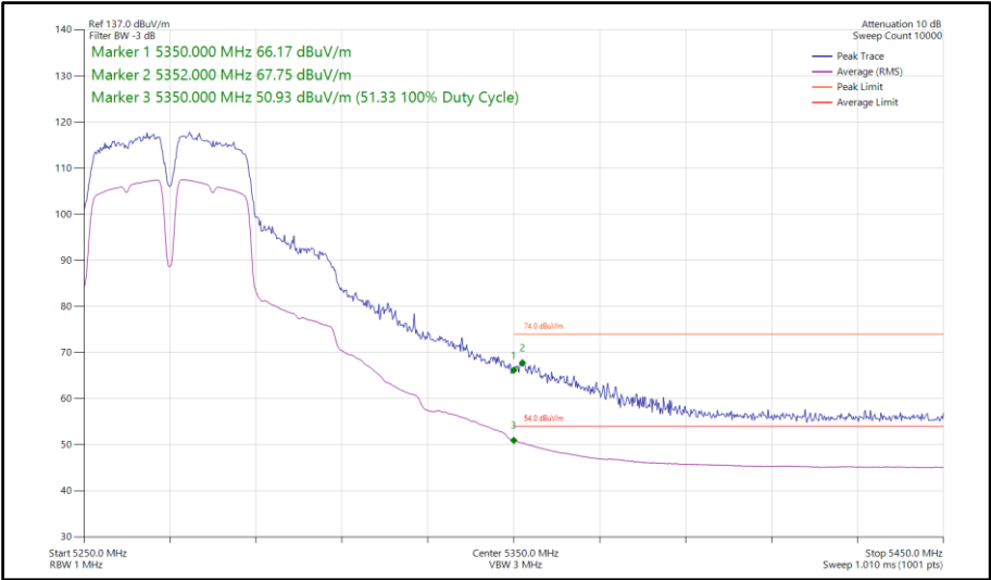
Figure 397 - 802.11a a40, SISO, Core 0 - 5270 MHz Band Edge Frequency 5350 MHz
