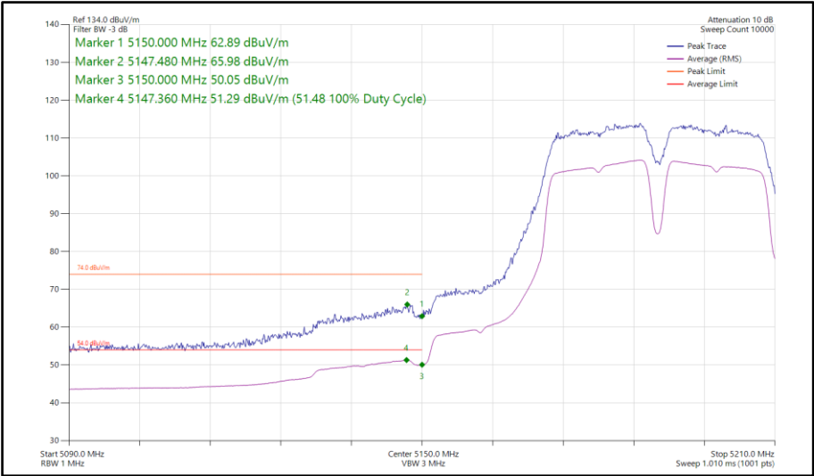
Figure 389 - 802.11a a40, SISO, Core 0 - 5190 MHz Band Edge Frequency 5150 MHz
