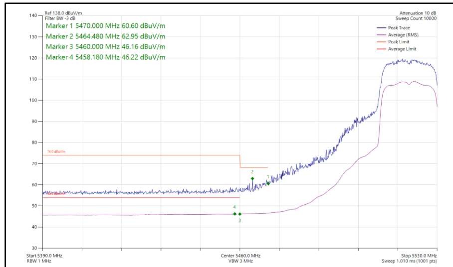
Figure 357 - 802.11ax HE20, SU, CDD, Core 0-1 - 5520 MHz Band Edge Frequency 5460 MHz
