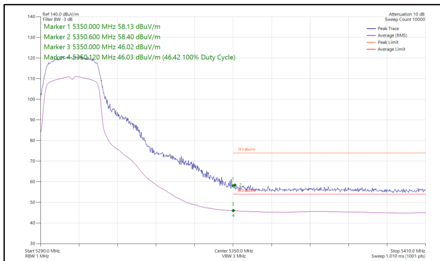
Figure 343 - 802.11a, CDD, Core 0-1 - 5300 MHz Band Edge Frequency 5350 MHz
