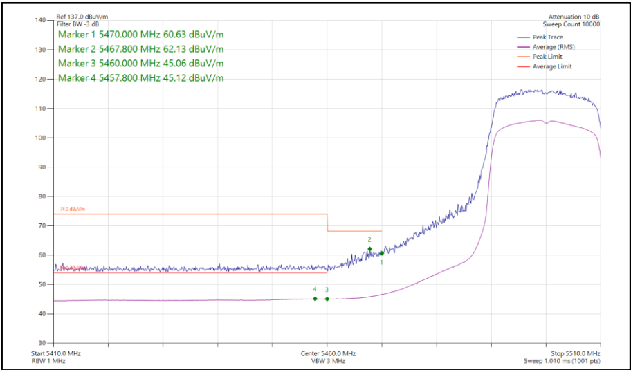
Figure 373 - 802.11ax HE20, SU, SDM, Core 0-1 - 5500 MHz Band Edge Frequency 5460 MHz
