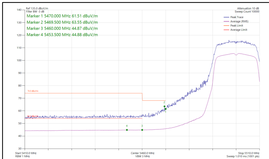
Figure 371 - 802.11n HT20, SDM, Core 0-1 - 5500 MHz Band Edge Frequency 5460 MHz
