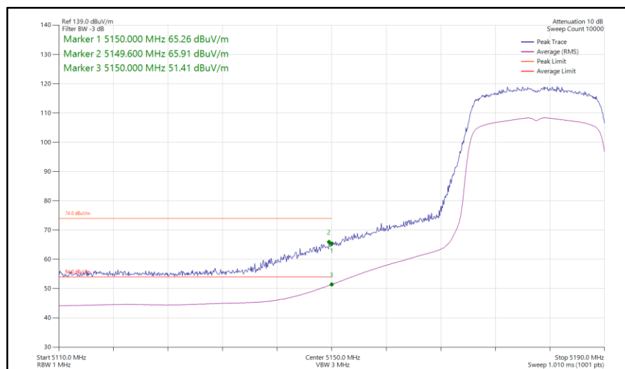
Figure 361 - 802.11ax HE20, SU, SDM, Core 0-1 - 5180 MHz Band Edge Frequency 5150 MHz
