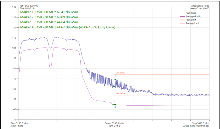
Figure 398 - 802.11a a40, SISO, Core 0 - 5310 MHz Band Edge Frequency 5350 MHz
