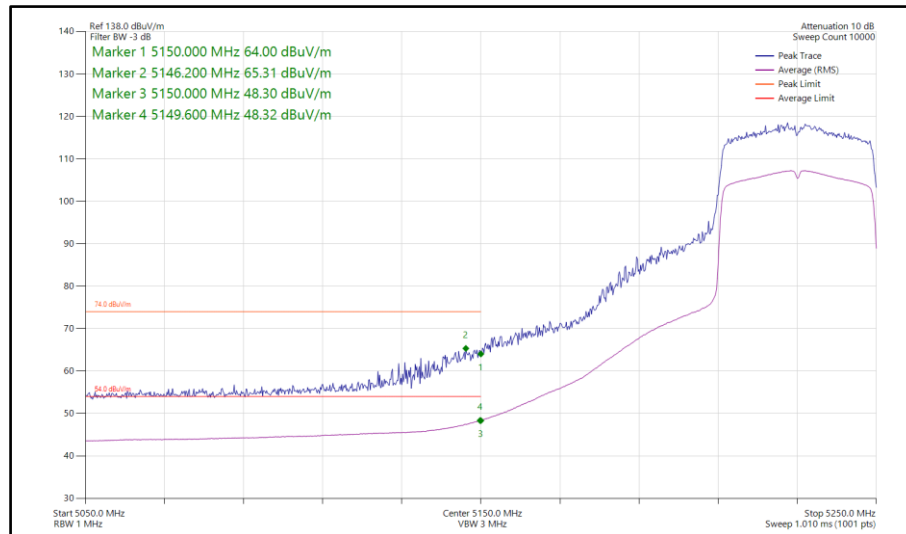
Figure 395 - 802.11ax HE40, SU, SISO, Core 0 - 5230 MHz Band Edge Frequency 5150 MHz
