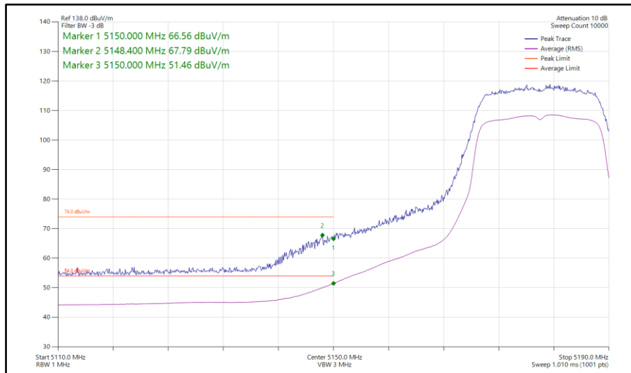
Figure 337 - 802.11n HT20, CDD, Core 0-1 - 5180 MHz Band Edge Frequency 5150 MHz
