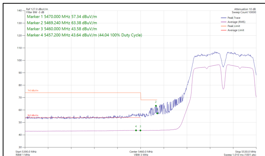
Figure 404 - 802.11a a40, SISO, Core 0 - 5510 MHz Band Edge Frequency 5460 MHz
