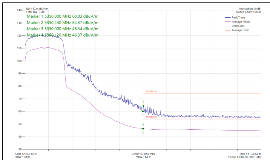
Figure 347 - 802.11ax HE20, SU, CDD, Core 0-1 - 5300 MHz Band Edge Frequency 5350 MHz
