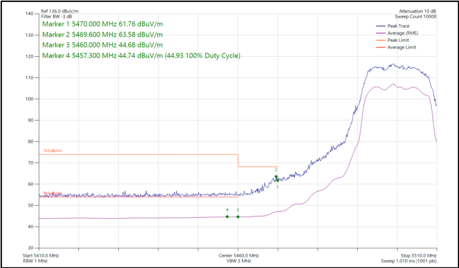
Figure 351 - 802.11a, CDD, Core 0-1 - 5500 MHz Band Edge Frequency 5460 MHz
