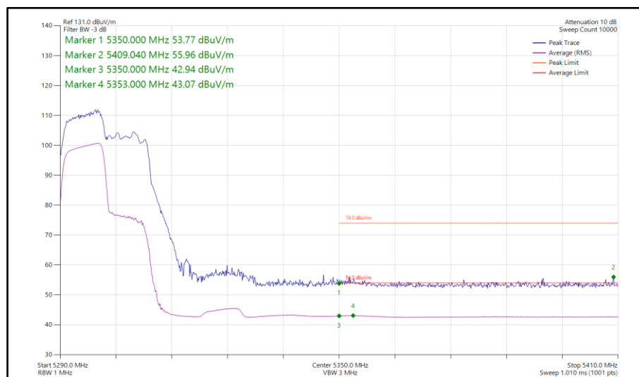
Figure 402 - 802.11ax HE40, RU 106-53, SISO, Core 0 - 5310 MHz Band Edge Frequency 5350 MHz
