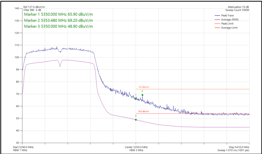
Figure 400 - 802.11n HT40, SISO, Core 0 - 5310 MHz Band Edge Frequency 5350 MHz
