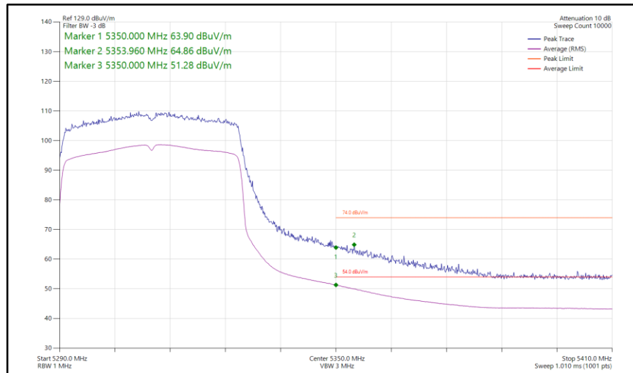
Figure 401 - 802.11ax HE40, SU, SISO, Core 0 - 5310 MHz Band Edge Frequency 5350 MHz
