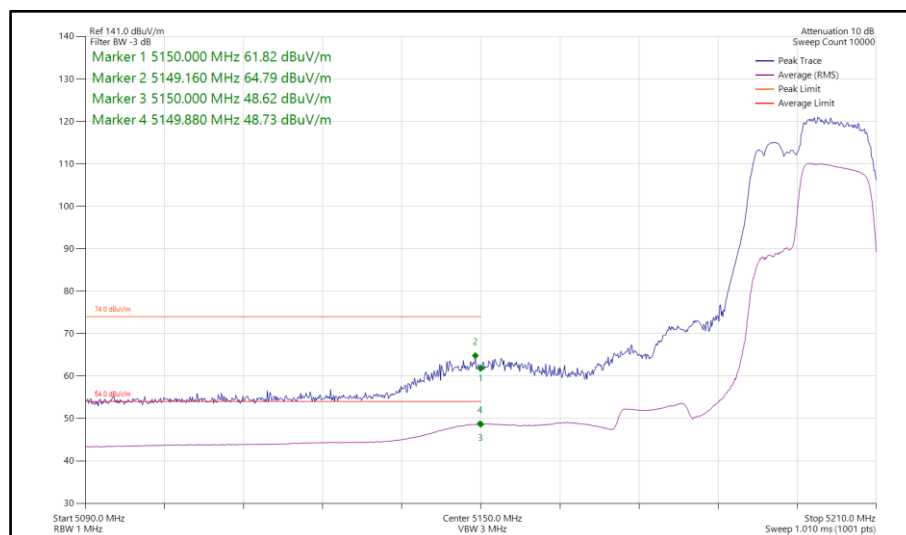
Figure 396 - 802.11be EHT40, RU 106+26-85, SISO, Core 0 - 5190 MHz Band Edge Frequency 5150 MHz
