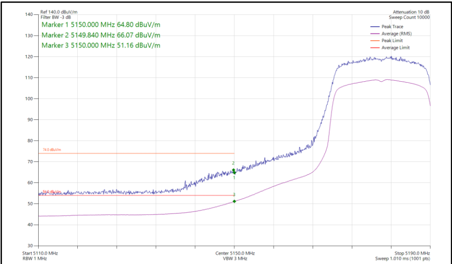
Figure 379 - 802.11ax HE20, SU, TxBF, Core 0-1 - 5180 MHz Band Edge Frequency 5150 MHz
