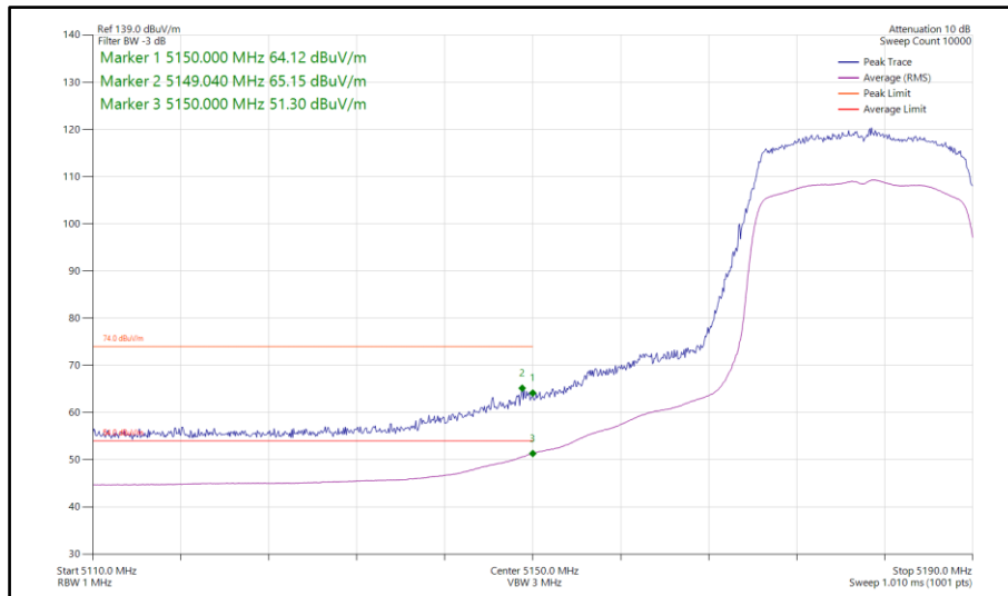
Figure 339 - 802.11ax HE20, SU, CDD, Core 0-1 - 5180 MHz Band Edge Frequency 5150 MHz
