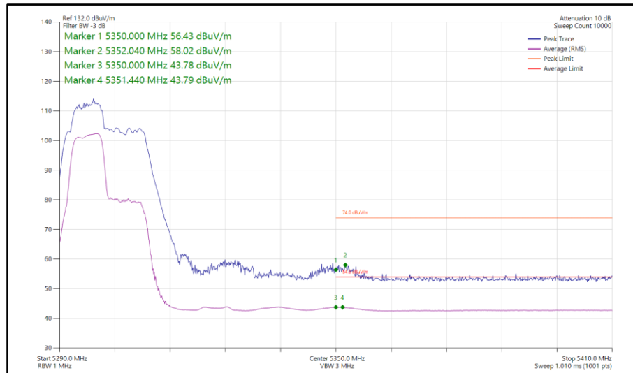
Figure 403 - 802.11be EHT40, RU 52+26-70, SISO, Core 0 - 5310 MHz Band Edge Frequency 5350 MHz
