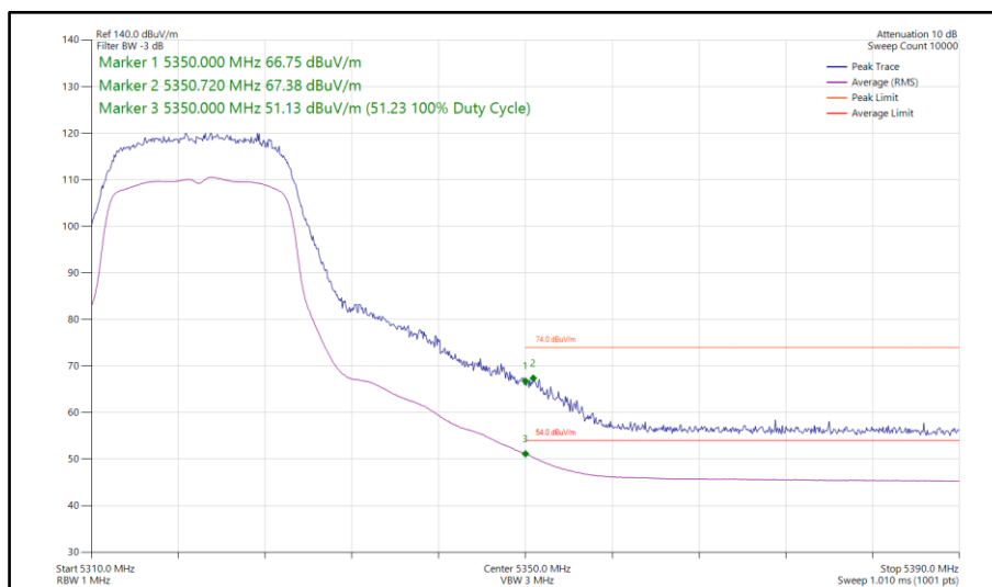
Figure 344 - 802.11a, CDD, Core 0-1 - 5320 MHz Band Edge Frequency 5350 MHz
