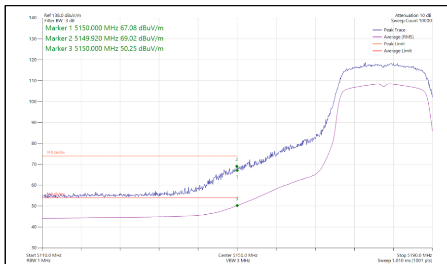
Figure 359 - 802.11n HT20, SDM, Core 0-1 - 5180 MHz Band Edge Frequency 5150 MHz
