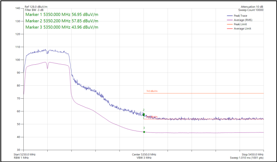
Figure 399 - 802.11n HT40, SISO, Core 0 - 5270 MHz Band Edge Frequency 5350 MHz
