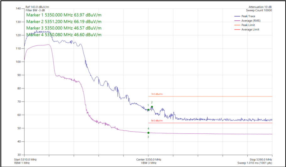
Figure 369 - 802.11ax HE20, RU 106-53, SDM, Core 0-1 - 5320 MHz Band Edge Frequency 5350 MHz
