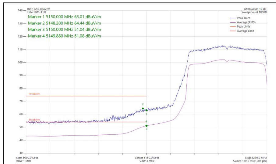
Figure 393 - 802.11ax HE40, SU, SISO, Core 0 - 5190 MHz Band Edge Frequency 5150 MHz
