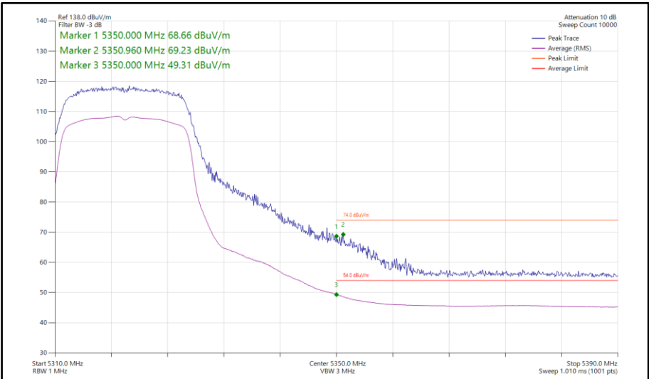
Figure 346 - 802.11n HT20, CDD, Core 0-1 - 5320 MHz Band Edge Frequency 5350 MHz
