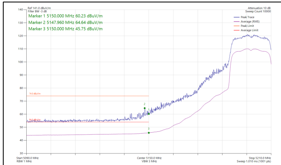
Figure 341 - 802.11ax HE20, SU, CDD, Core 0-1 - 5200 MHz Band Edge Frequency 5150 MHz
