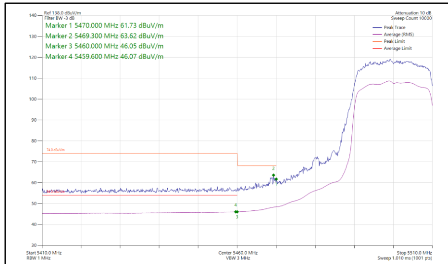
Figure 355 - 802.11ax HE20, SU, CDD, Core 0-1 - 5500 MHz Band Edge Frequency 5460 MHz
