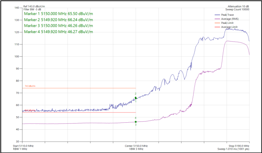
Figure 362 - 802.11ax HE20, RU 106-54, SDM, Core 0-1 - 5180 MHz Band Edge Frequency 5150 MHz
