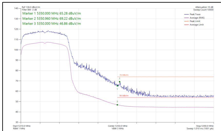
Figure 384 - 802.11ax HE20, SU, TxBF, Core 0-1 - 5320 MHz Band Edge Frequency 5350 MHz
