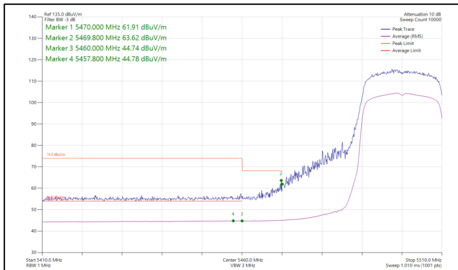
Figure 387 - 802.11ax HE20, SU, TxBF, Core 0-1 - 5500 MHz Band Edge Frequency 5460 MHz
