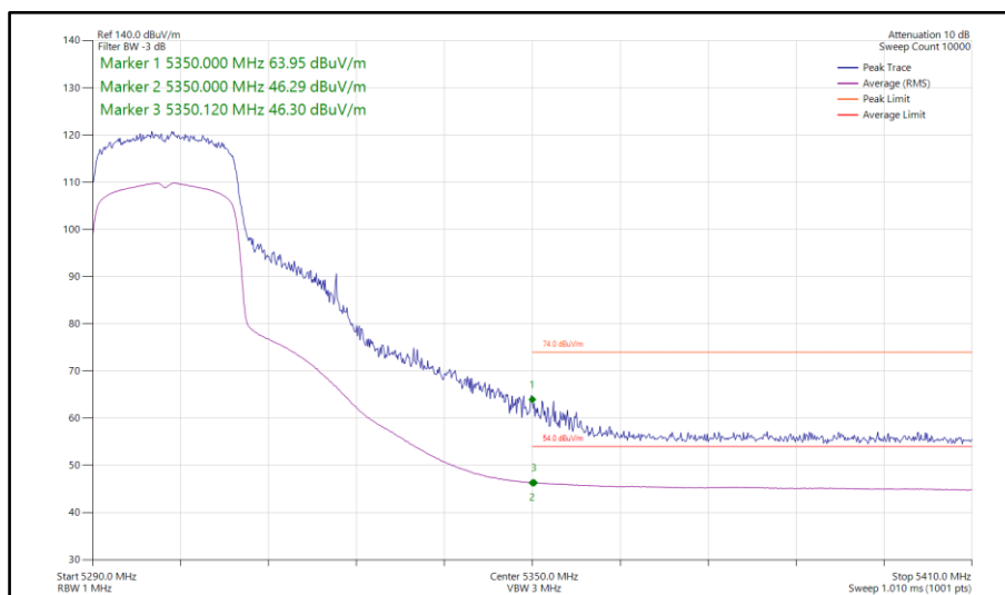
Figure 367 - 802.11ax HE20, SU, SDM, Core 0-1 - 5300 MHz Band Edge Frequency 5350 MHz
