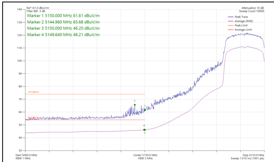
Figure 380 - 802.11ax HE20, SU, TxBF, Core 0-1 - 5200 MHz Band Edge Frequency 5150 MHz
