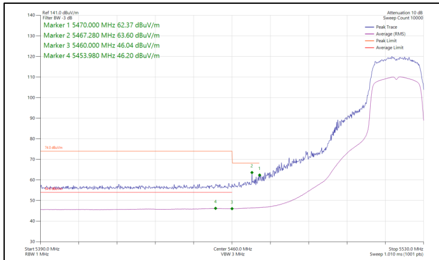
Figure 386 - 802.11ac VHT20, TxBF, Core 0-1 - 5520 MHz Band Edge Frequency 5460 MHz
