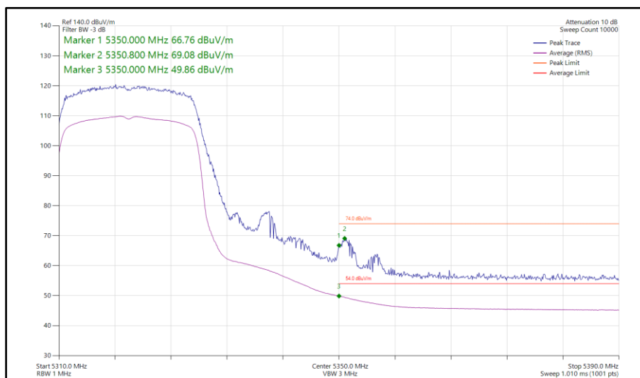
Figure 348 - 802.11ax HE20, SU, CDD, Core 0-1 - 5320 MHz Band Edge Frequency 5350 MHz
