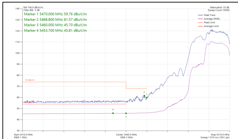
Figure 358 - 802.11be EHT20, RU 106+26-83, CDD, Core 0-1 - 5500 MHz Band Edge Frequency 5460 MHz
