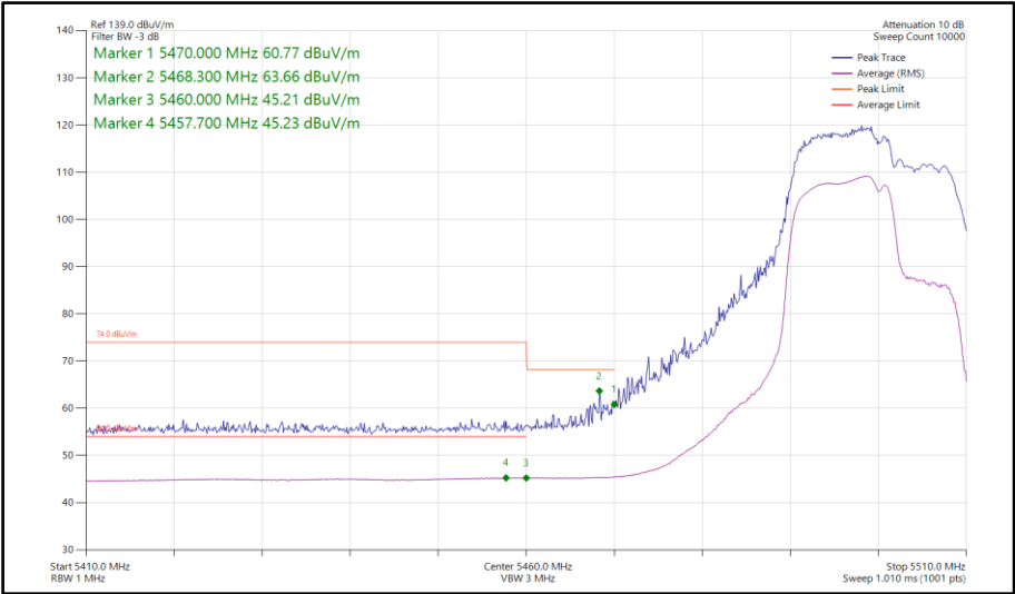
Figure 376 - 802.11be EHT20, RU 106+26-82, SDM, Core 0-1 - 5500 MHz Band Edge Frequency 5460 MHz
