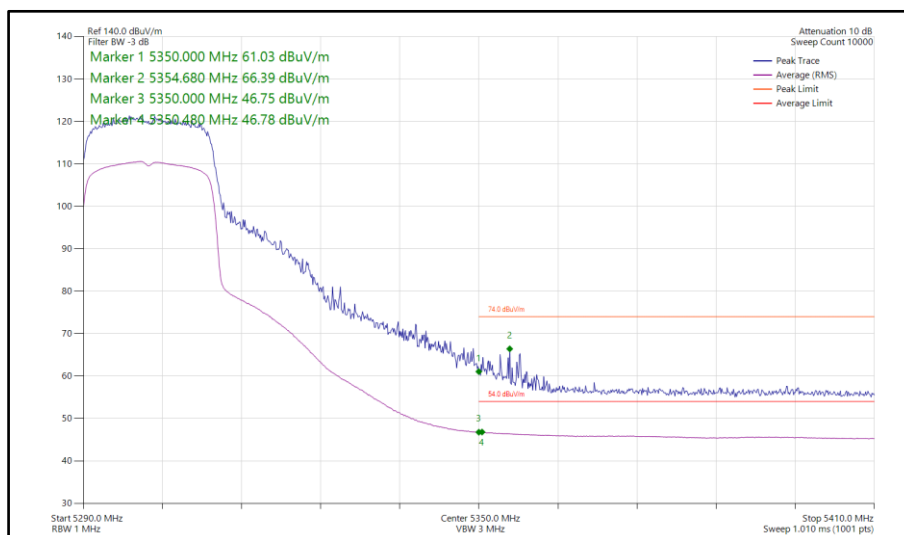
Figure 383 - 802.11ax HE20, SU, TxBF, Core 0-1 - 5300 MHz Band Edge Frequency 5350 MHz
