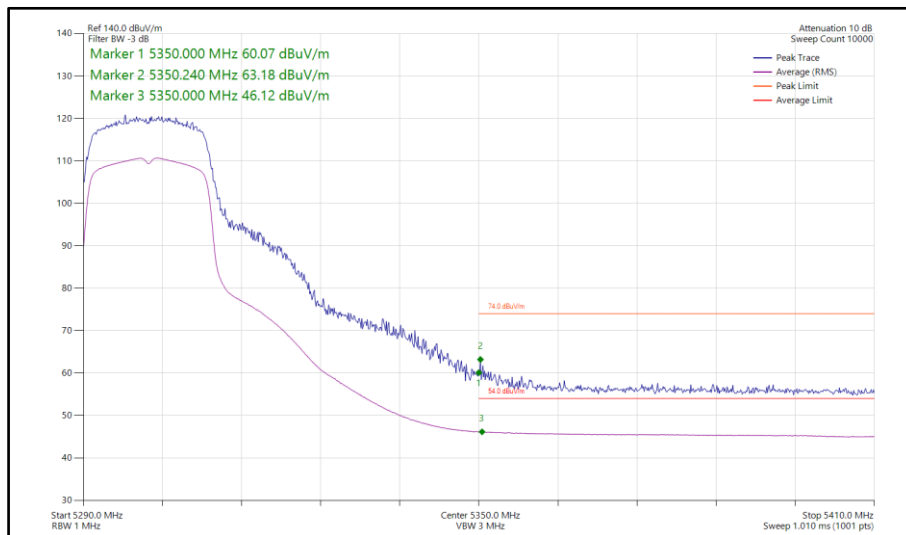
Figure 365 - 802.11n HT20, SDM, Core 0-1 - 5300 MHz Band Edge Frequency 5350 MHz
