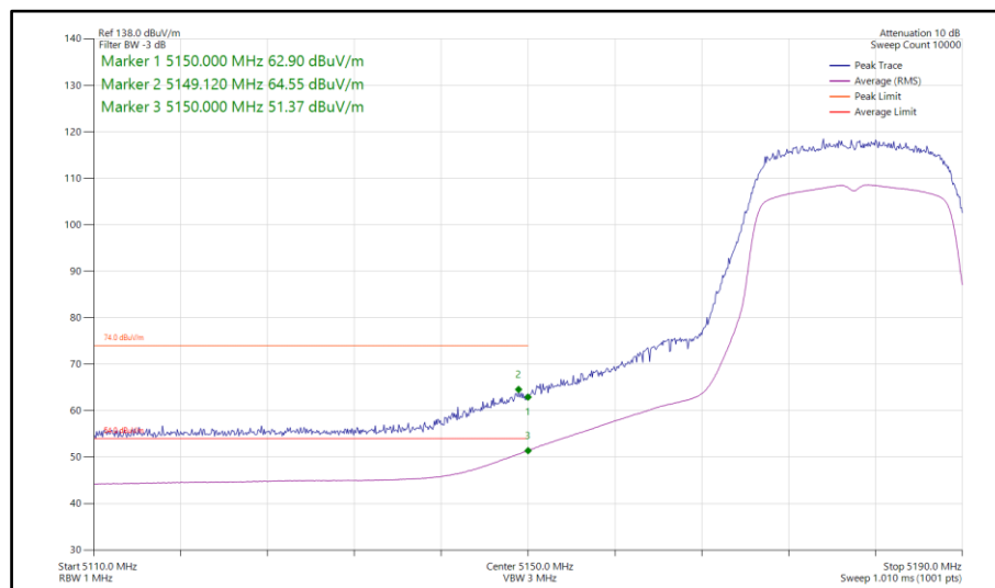
Figure 377 - 802.11ac VHT20, TxBF, Core 0-1 - 5180 MHz Band Edge Frequency 5150 MHz
