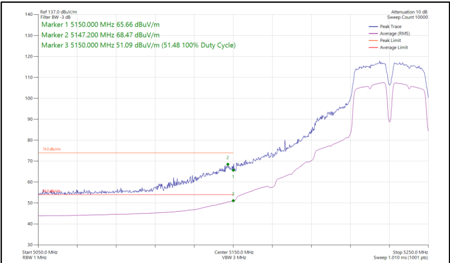
Figure 390 - 802.11a a40, SISO, Core 0 - 5230 MHz Band Edge Frequency 5150 MHz
