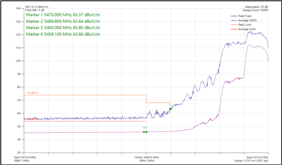
Figure 374 - 802.11ax HE20, RU 106-54, SDM, Core 0-1 - 5500 MHz Band Edge Frequency 5460 MHz
