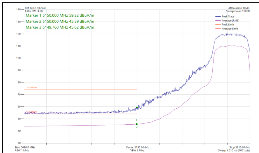
Figure 338 - 802.11n HT20, CDD, Core 0-1 - 5200 MHz Band Edge Frequency 5150 MHz
