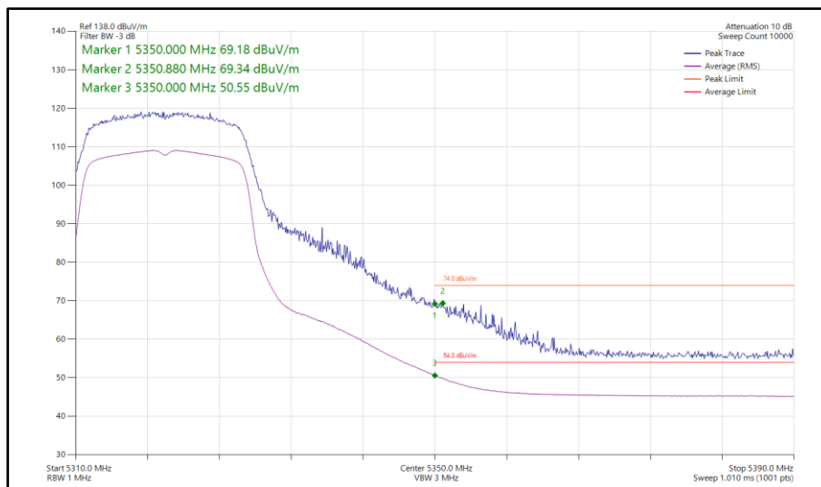
Figure 382 - 802.11ac VHT20, TxBF, Core 0-1 - 5320 MHz Band Edge Frequency 5350 MHz
