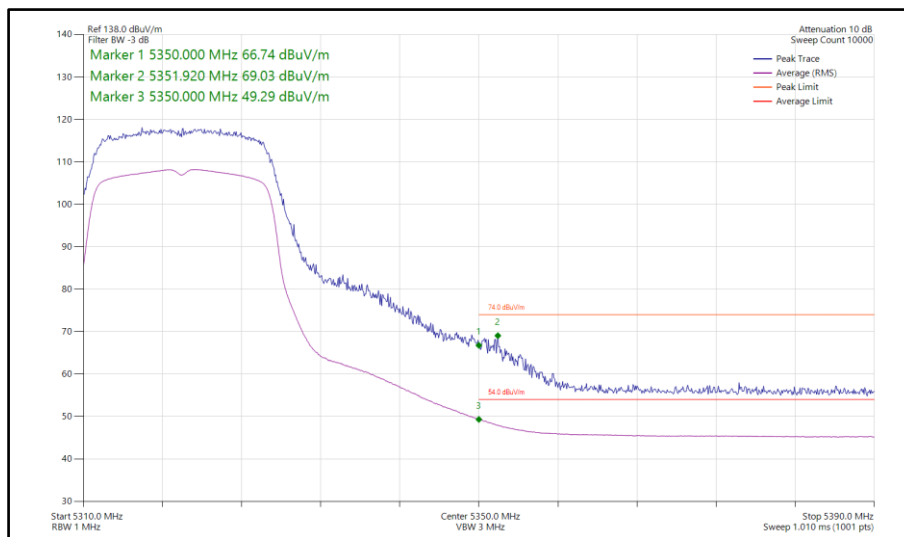
Figure 366 - 802.11n HT20, SDM, Core 0-1 - 5320 MHz Band Edge Frequency 5350 MHz
