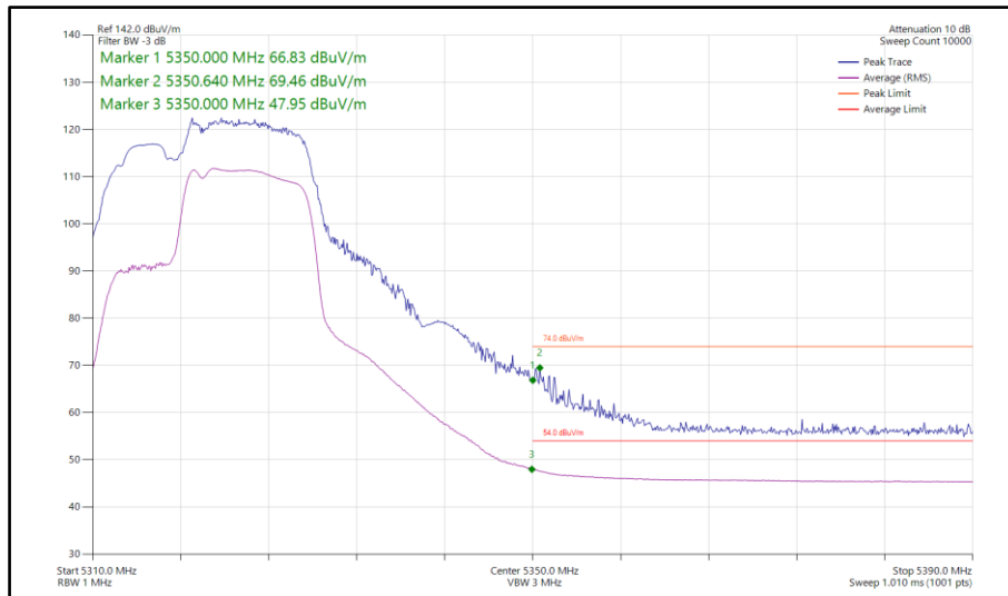
Figure 370 - 802.11be EHT20, RU 106+26-83, SDM, Core 0-1 - 5320 MHz Band Edge Frequency 5350 MHz
