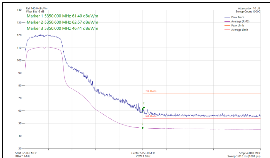
Figure 381 - 802.11ac VHT20, TxBF, Core 0-1 - 5300 MHz Band Edge Frequency 5350 MHz
