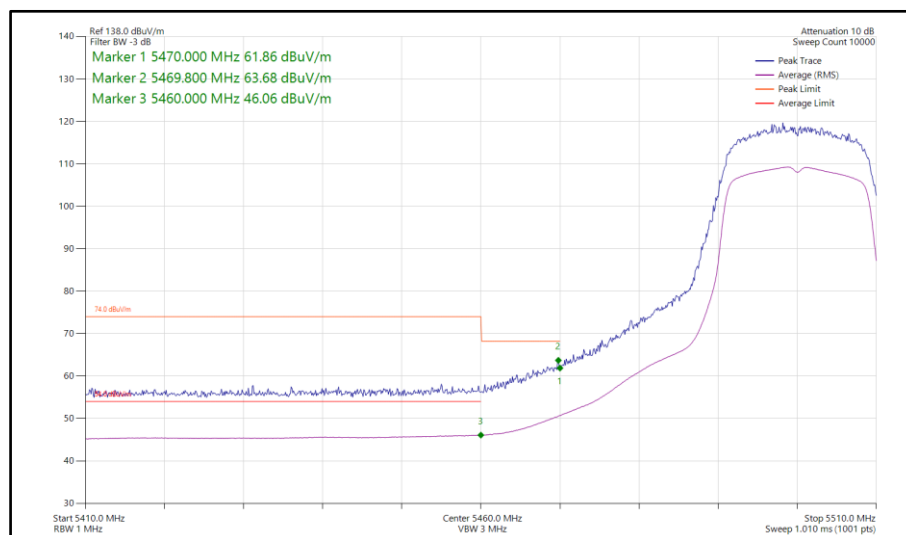
Figure 385 - 802.11ac VHT20, TxBF, Core 0-1 - 5500 MHz Band Edge Frequency 5460 MHz
