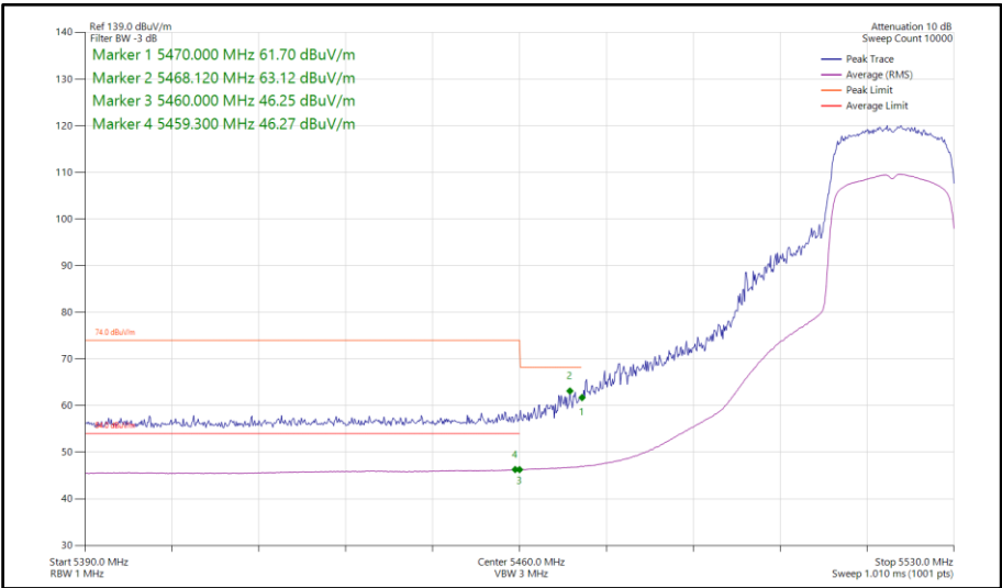
Figure 375 - 802.11ax HE20, SU, SDM, Core 0-1 - 5520 MHz Band Edge Frequency 5460 MHz
