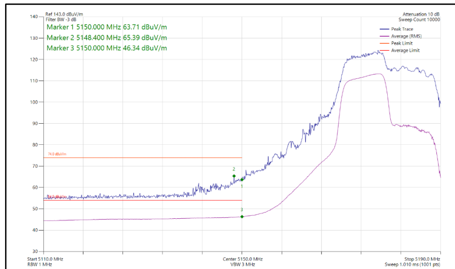
Figure 340 - 802.11ax HE20, RU 106-53, CDD, Core 0-1 - 5180 MHz Band Edge Frequency 5150 MHz
