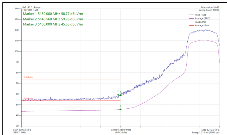
Figure 360 - 802.11n HT20, SDM, Core 0-1 - 5200 MHz Band Edge Frequency 5150 MHz
