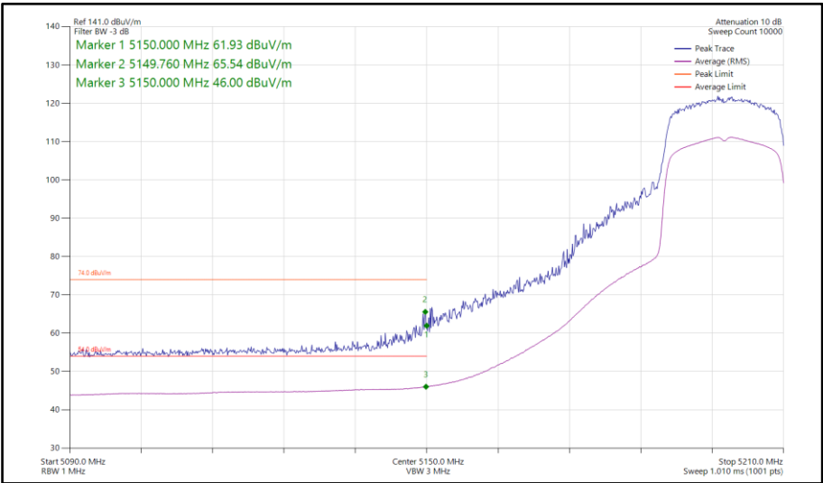
Figure 363 - 802.11ax HE20, SU, SDM, Core 0-1 - 5200 MHz Band Edge Frequency 5150 MHz
