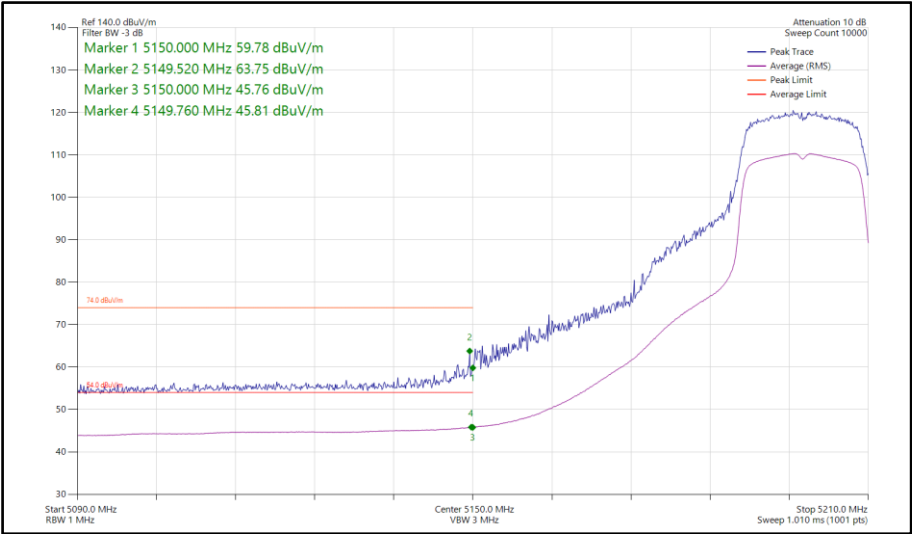
Figure 378 - 802.11ac VHT20, TxBF, Core 0-1 - 5200 MHz Band Edge Frequency 5150 MHz
