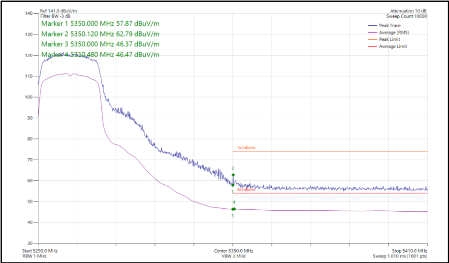
Figure 345 - 802.11n HT20, CDD, Core 0-1 - 5300 MHz Band Edge Frequency 5350 MHz
