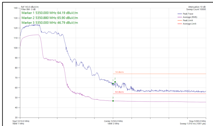
Figure 349 - 802.11ax HE20, RU 106-53, CDD, Core 0-1 - 5320 MHz Band Edge Frequency 5350 MHz
