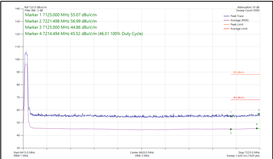
Figure 228 - Bluetooth XHDRPL24, MIMO, Core 0-1 - 6425 MHz Band Edge Frequency 7125 MHz
