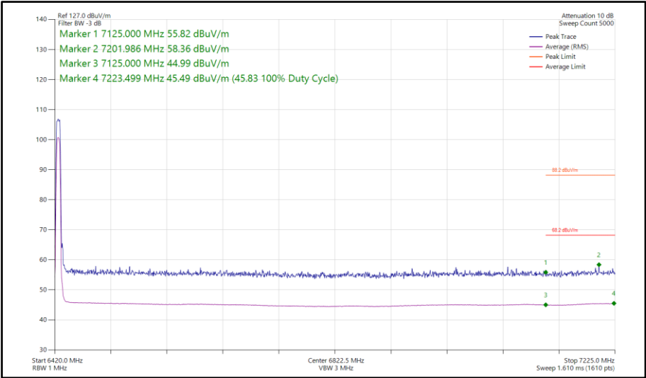
Figure 227 - Bluetooth XHDRPM8, MIMO, Core 0-1 - 6425 MHz Band Edge Frequency 7125 MHz
