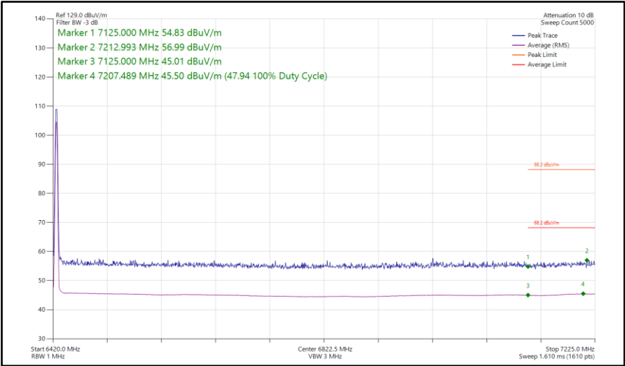
Figure 191 - Bluetooth LE2M, SISO, Core 1 - 6425 MHz Band Edge Frequency 7125 MHz
