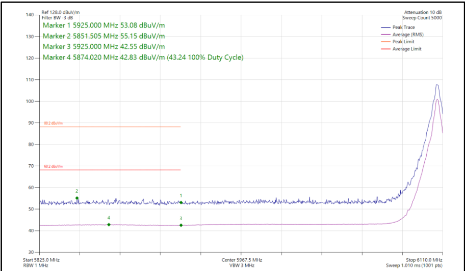
Figure 180 - Bluetooth HDT6, SISO, Core 1 - 6106 MHz Band Edge Frequency 5925 MHz
