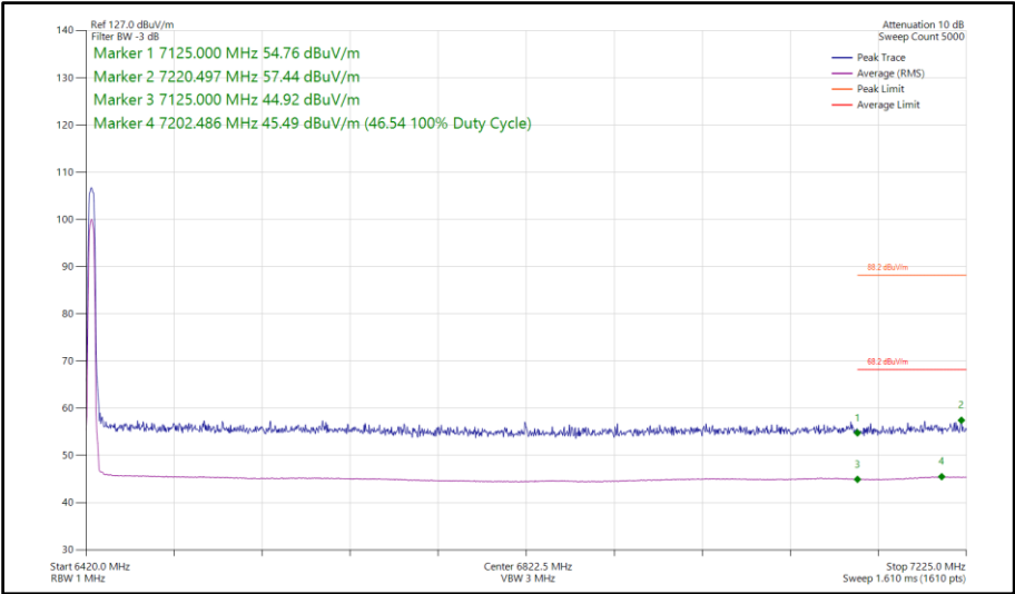
Figure 217 - Bluetooth HDR8, MIMO, Core 0-1 - 6425 MHz Band Edge Frequency 7125 MHz
