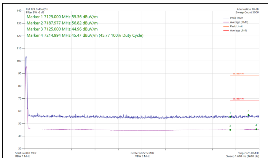
Figure 196 - Bluetooth HDRPM12, SISO, Core 1 - 6425 MHz Band Edge Frequency 7125 MHz
