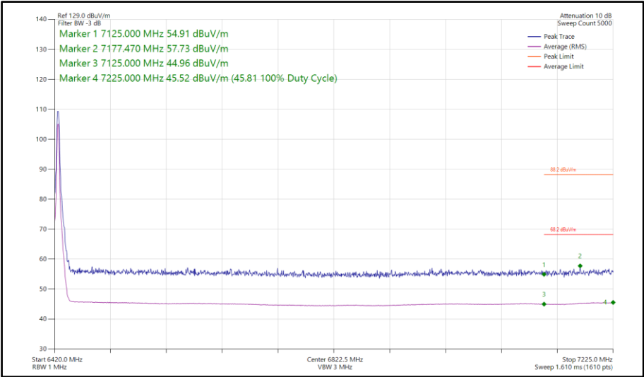
Figure 193 - Bluetooth HDT4, SISO, Core 1 - 6425 MHz Band Edge Frequency 7125 MHz
