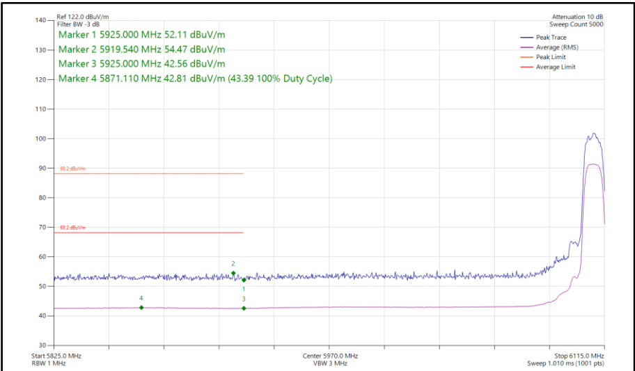
Figure 184 - Bluetooth HDRPL24, SISO, Core 1 - 6109 MHz Band Edge Frequency 5925 MHz
