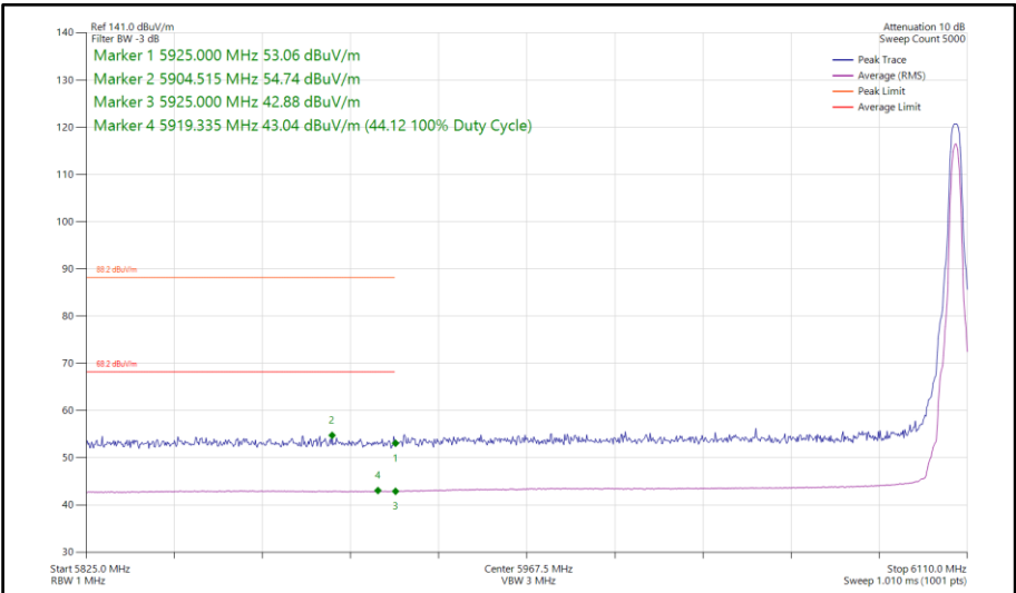
Figure 230 - Bluetooth HDR4, SISO, Core 0 - 6106 MHz Band Edge Frequency 5925 MHz
