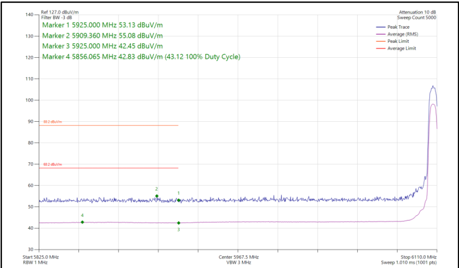
Figure 210 - Bluetooth HDRPM12, MIMO, Core 0-1 - 6107 MHz Band Edge Frequency 5925 MHz
