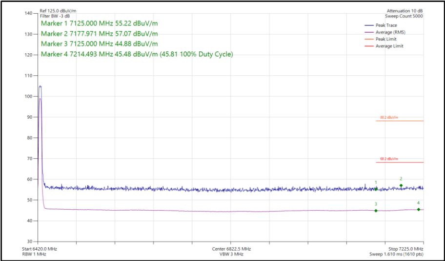
Figure 199 - Bluetooth XHDRPM8, SISO, Core 1 - 6425 MHz Band Edge Frequency 7125 MHz
