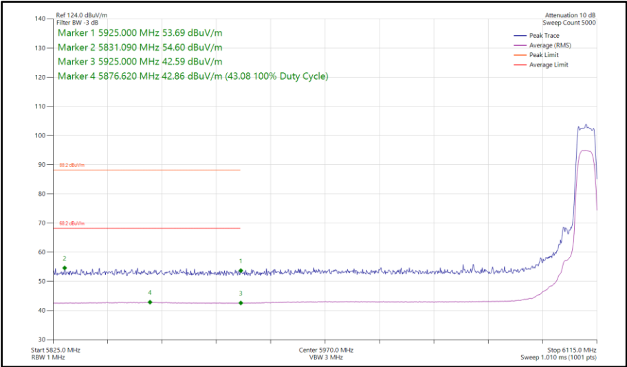
Figure 183 - Bluetooth HDRPL8, SISO, Core 1 - 6109 MHz Band Edge Frequency 5925 MHz
