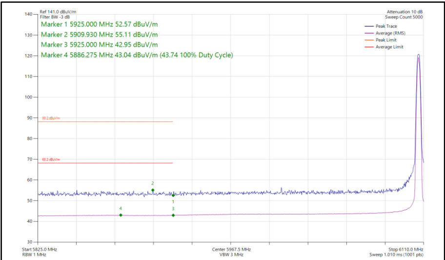
Figure 232 - Bluetooth LE1M, SISO, Core 0 - 6106 MHz Band Edge Frequency 5925 MHz
