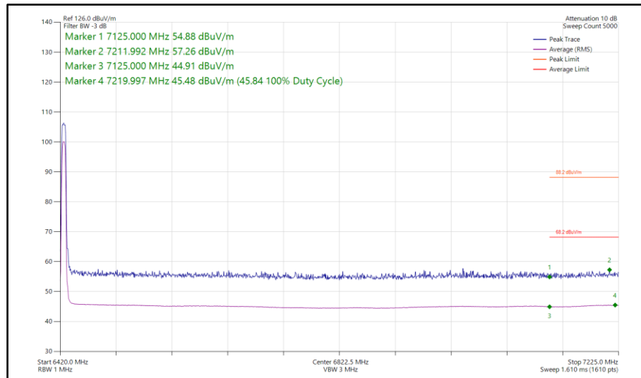
Figure 171 - Bluetooth XHDRPM8, SISO, Core 0 - 6425 MHz Band Edge Frequency 7125 MHz
