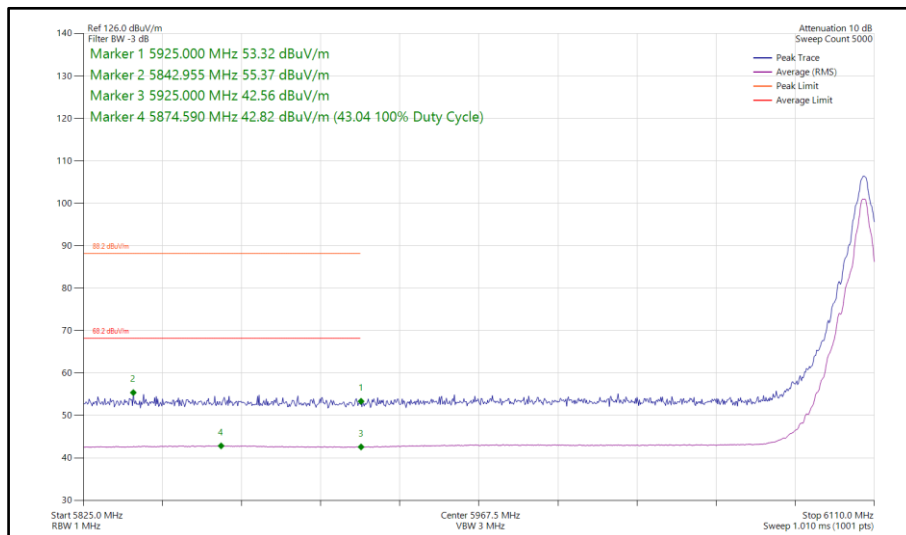
Figure 178 - Bluetooth HDT3, SISO, Core 1 - 6106 MHz Band Edge Frequency 5925 MHz
