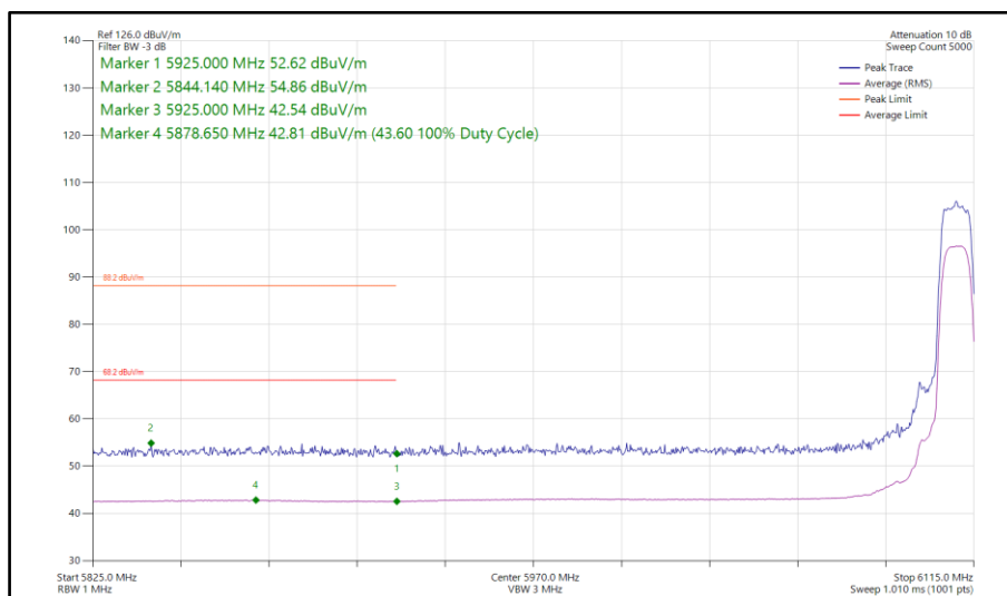
Figure 214 - Bluetooth XHDRPL24, MIMO, Core 0-1 - 6109 MHz Band Edge Frequency 5925 MHz
