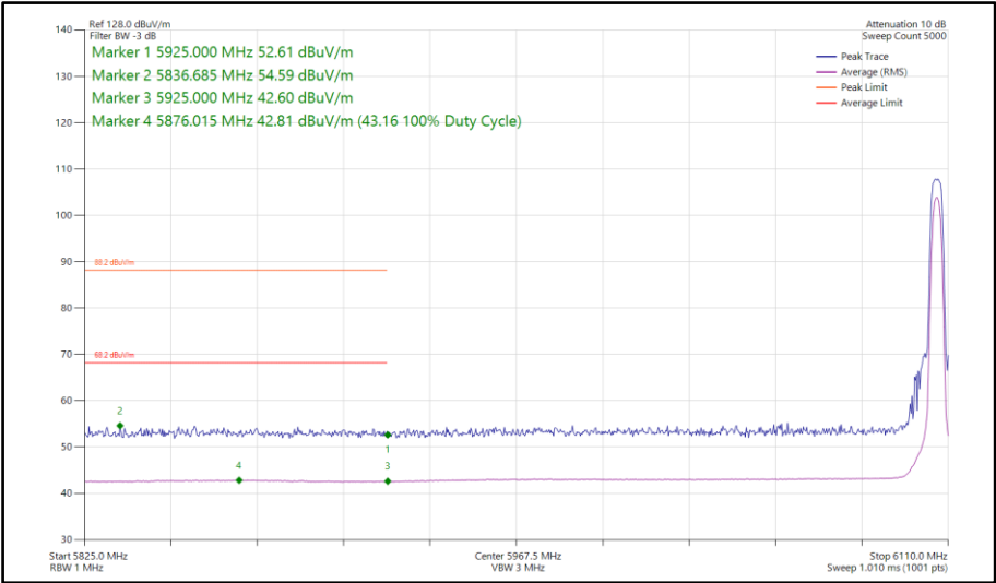
Figure 209 - Bluetooth HDRPS2, MIMO, Core 0-1 - 6106 MHz Band Edge Frequency 5925 MHz
