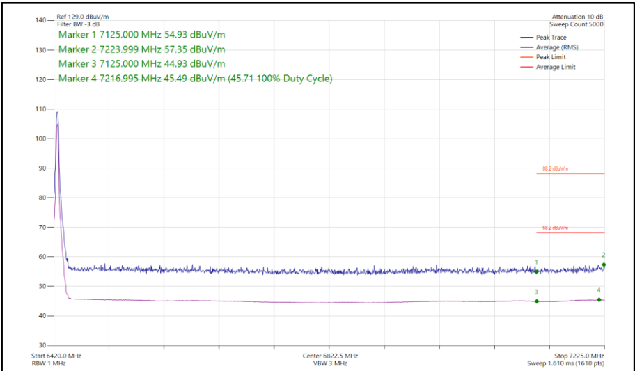
Figure 192 - Bluetooth HDT3, SISO, Core 1 - 6425 MHz Band Edge Frequency 7125 MHz
