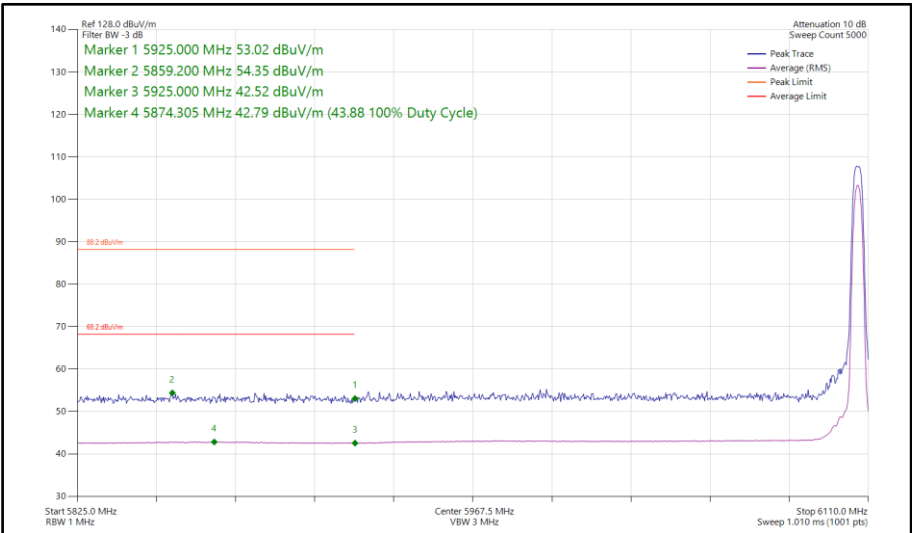
Figure 202 - Bluetooth HDR4, MIMO, Core 0-1 - 6106 MHz Band Edge Frequency 5925 MHz
