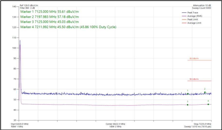
Figure 223 - Bluetooth HDRPS2, MIMO, Core 0-1 - 6425 MHz Band Edge Frequency 7125 MHz
