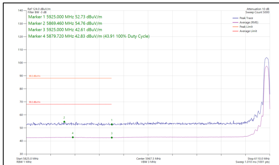
Figure 175 - Bluetooth HDR8, SISO, Core 1 - 6106 MHz Band Edge Frequency 5925 MHz
