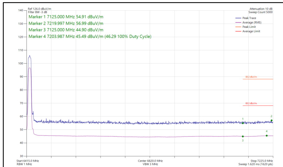
Figure 172 - Bluetooth XHDRPL24, SISO, Core 0 - 6425 MHz Band Edge Frequency 7125 MHz
