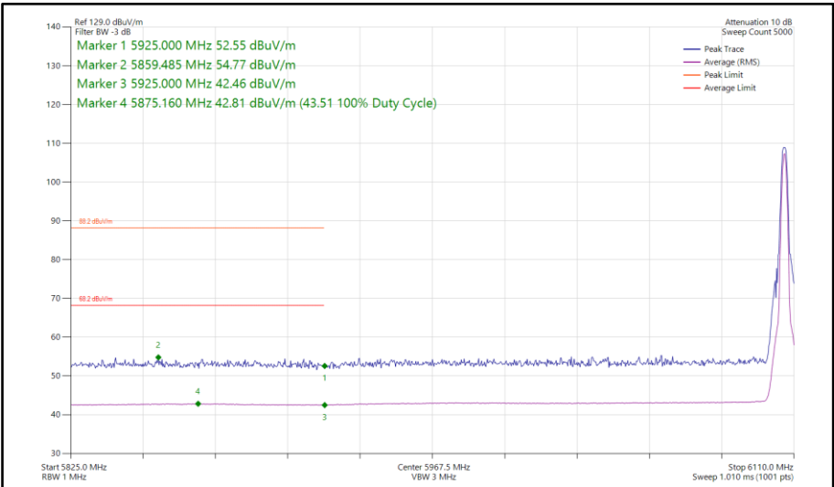
Figure 204 - Bluetooth LE1M, MIMO, Core 0-1 - 6106 MHz Band Edge Frequency 5925 MHz
