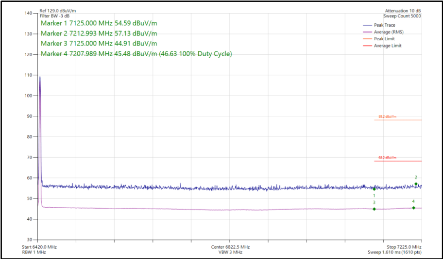
Figure 187 - Bluetooth DH5, SISO, Core 1 - 6425 MHz Band Edge Frequency 7125 MHz
