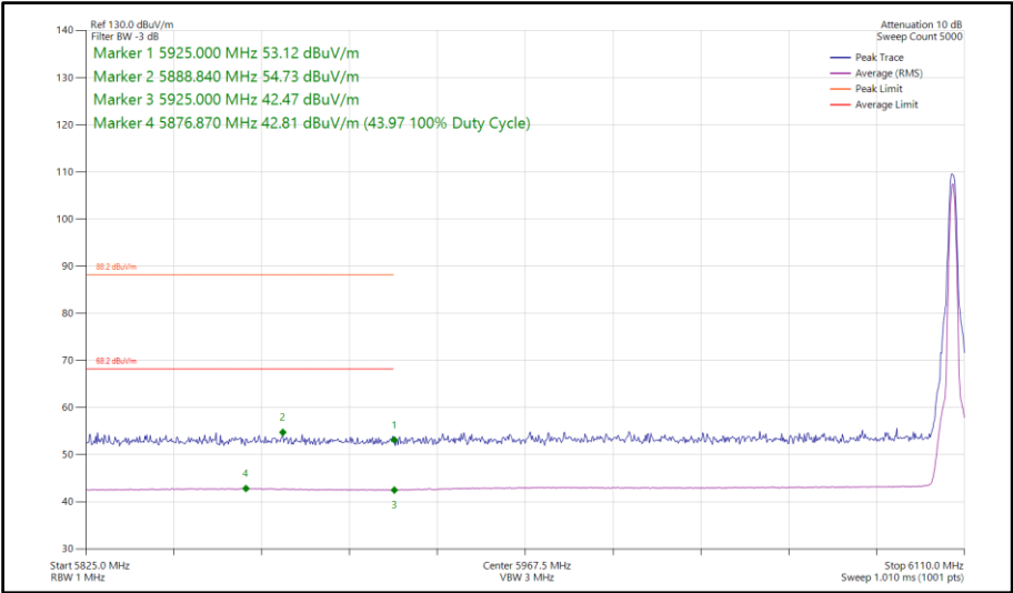
Figure 201 - Bluetooth DH5, MIMO, Core 0-1 - 6106 MHz Band Edge Frequency 5925 MHz
