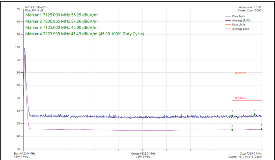
Figure 194 - Bluetooth HDT6, SISO, Core 1 - 6425 MHz Band Edge Frequency 7125 MHz
