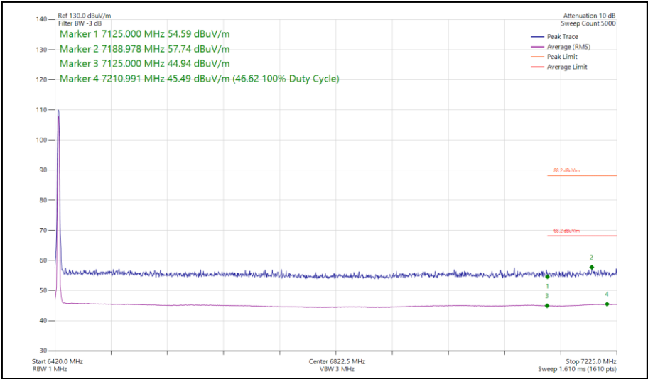
Figure 215 - Bluetooth DH5, MIMO, Core 0-1 - 6425 MHz Band Edge Frequency 7125 MHz
