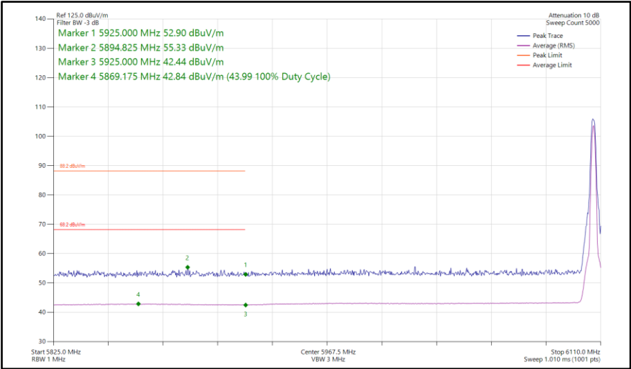
Figure 173 - Bluetooth DH5, SISO, Core 1 - 6106 MHz Band Edge Frequency 5925 MHz
