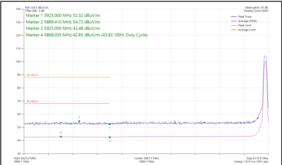
Figure 174 - Bluetooth HDR4, SISO, Core 1 - 6106 MHz Band Edge Frequency 5925 MHz
