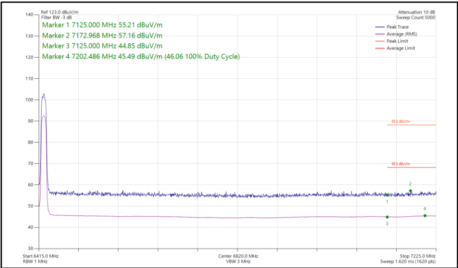
Figure 198 - Bluetooth HDRPL24, SISO, Core 1 - 6425 MHz Band Edge Frequency 7125 MHz
