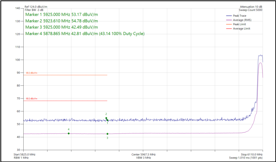
Figure 185 - Bluetooth XHDRPM8, SISO, Core 1 - 6107 MHz Band Edge Frequency 5925 MHz
