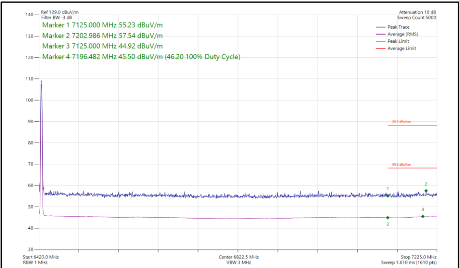
Figure 190 - Bluetooth LE1M, SISO, Core 1 - 6425 MHz Band Edge Frequency 7125 MHz
