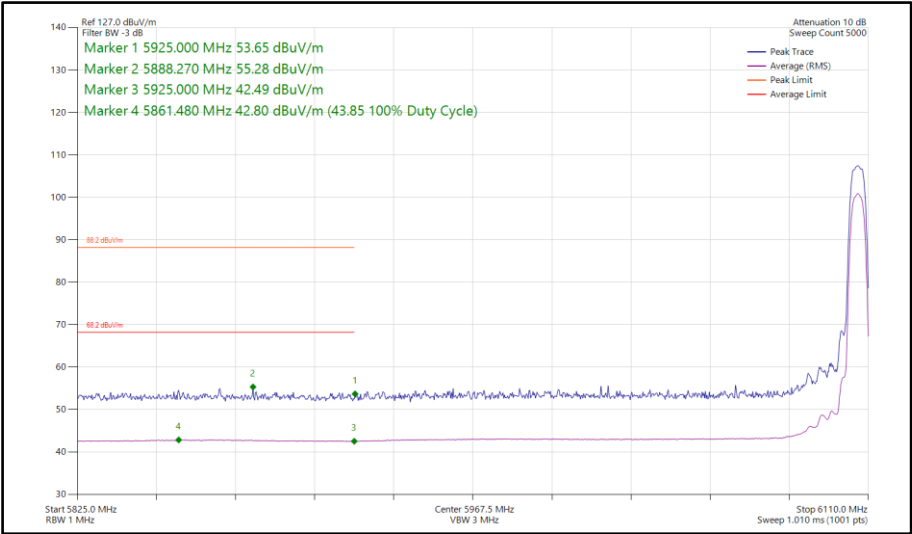
Figure 203 - Bluetooth HDR8, MIMO, Core 0-1 - 6106 MHz Band Edge Frequency 5925 MHz
