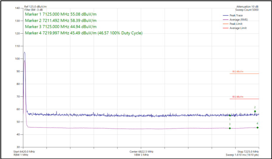
Figure 189 - Bluetooth HDR8, SISO, Core 1 - 6425 MHz Band Edge Frequency 7125 MHz
