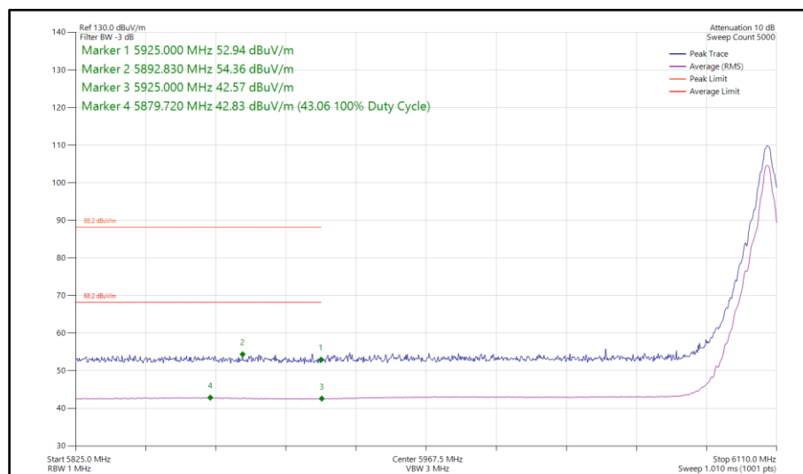
Figure 206 - Bluetooth HDT3, MIMO, Core 0-1 - 6106 MHz Band Edge Frequency 5925 MHz
