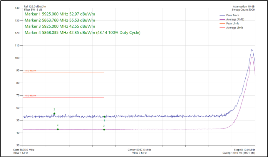
Figure 179 - Bluetooth HDT4, SISO, Core 1 - 6106 MHz Band Edge Frequency 5925 MHz
