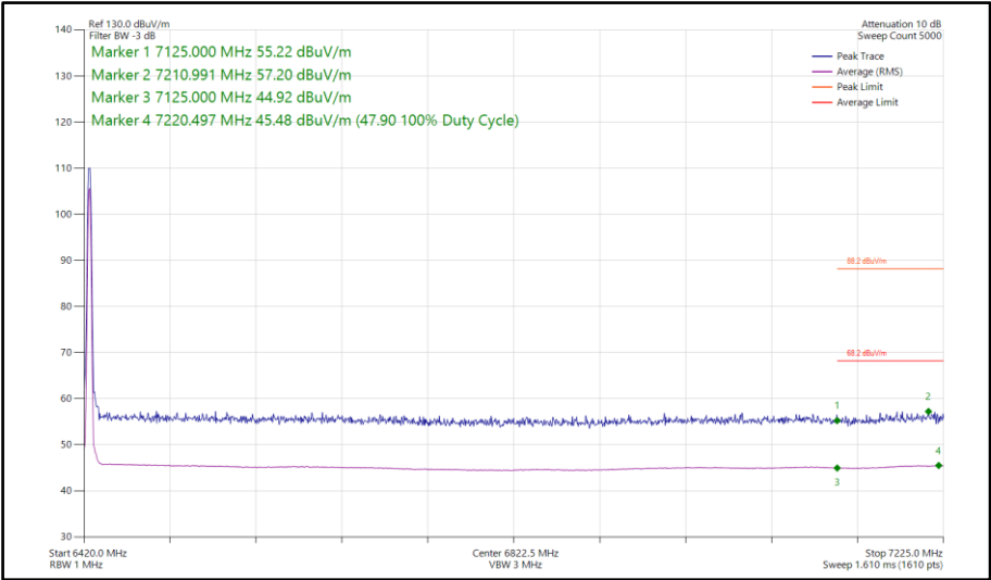
Figure 219 - Bluetooth LE2M, MIMO, Core 0-1 - 6425 MHz Band Edge Frequency 7125 MHz
