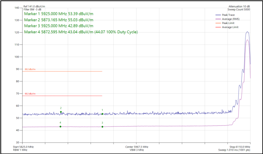
Figure 231 - Bluetooth HDR8, SISO, Core 0 - 6106 MHz Band Edge Frequency 5925 MHz
