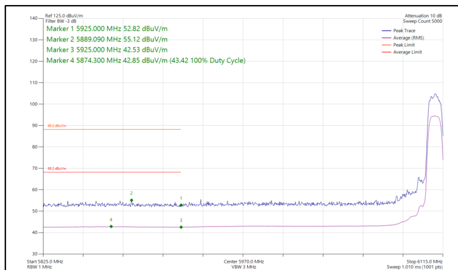
Figure 212 - Bluetooth HDRPL24, MIMO, Core 0-1 - 6109 MHz Band Edge Frequency 5925 MHz
