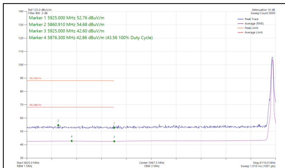
Figure 176 - Bluetooth LE1M, SISO, Core 1 - 6106 MHz Band Edge Frequency 5925 MHz
