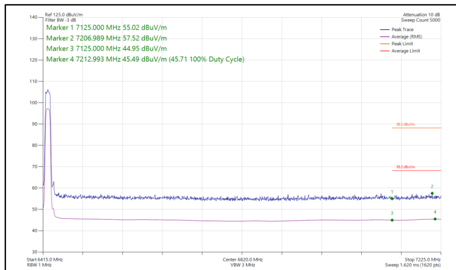
Figure 225 - Bluetooth HDRPL8, MIMO, Core 0-1 - 6425 MHz Band Edge Frequency 7125 MHz
