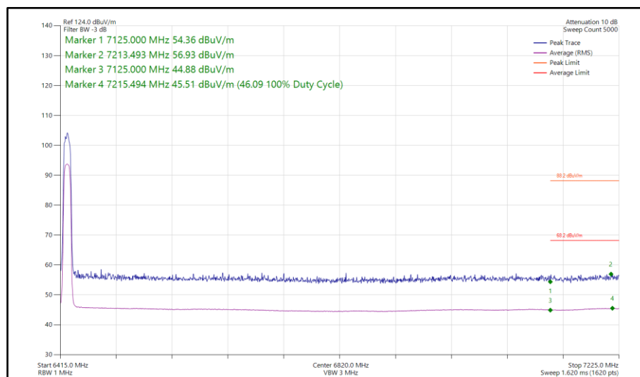
Figure 226 - Bluetooth HDRPL24, MIMO, Core 0-1 - 6425 MHz Band Edge Frequency 7125 MHz
