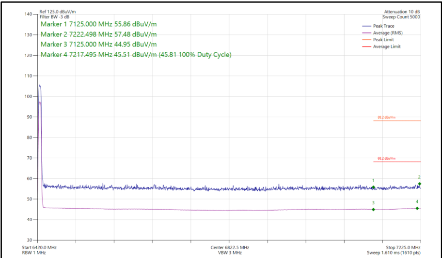
Figure 224 - Bluetooth HDRPM12, MIMO, Core 0-1 - 6425 MHz Band Edge Frequency 7125 MHz
