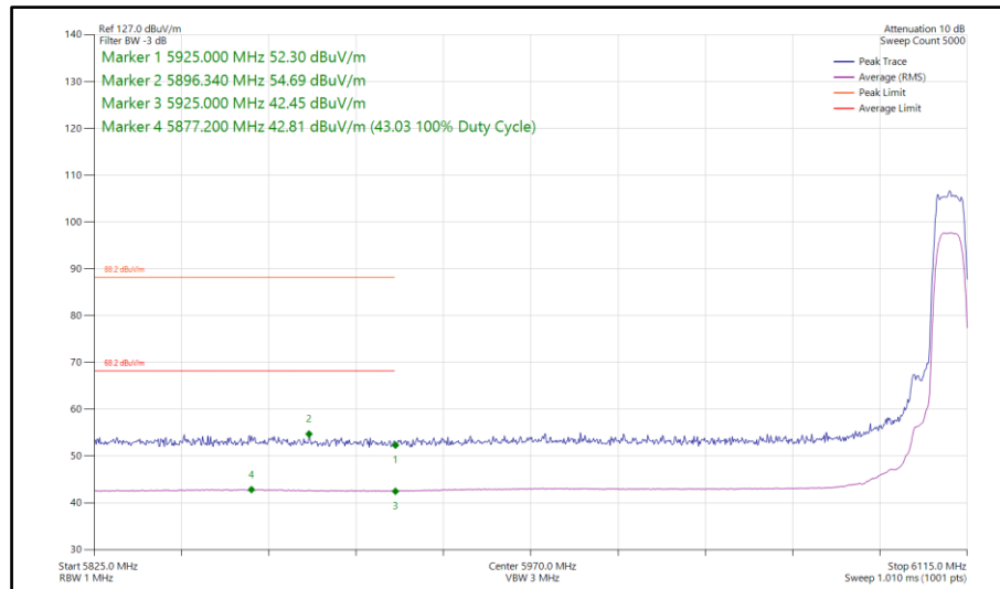
Figure 211 - Bluetooth HDRPL8, MIMO, Core 0-1 - 6109 MHz Band Edge Frequency 5925 MHz
