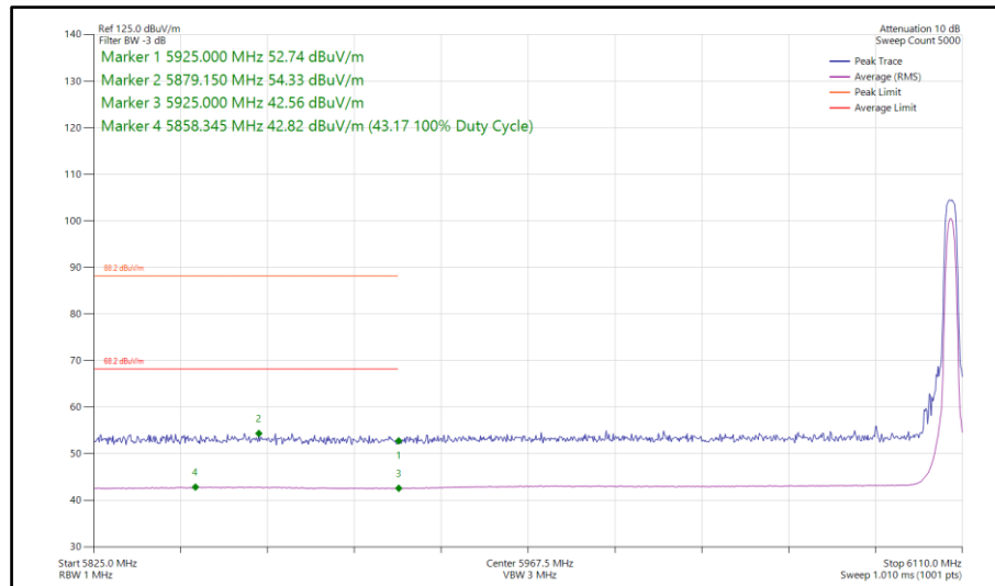
Figure 181 - Bluetooth HDRPS2, SISO, Core 1 - 6106 MHz Band Edge Frequency 5925 MHz
