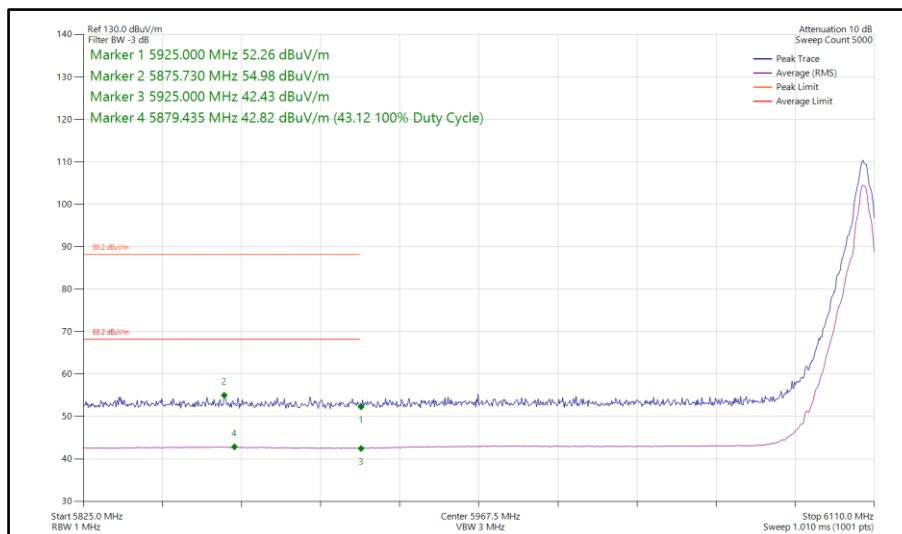
Figure 207 - Bluetooth HDT4, MIMO, Core 0-1 - 6106 MHz Band Edge Frequency 5925 MHz
