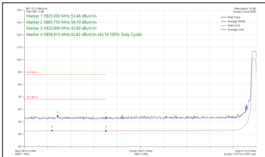
Figure 213 - Bluetooth XHDRPM8, MIMO, Core 0-1 - 6107 MHz Band Edge Frequency 5925 MHz
