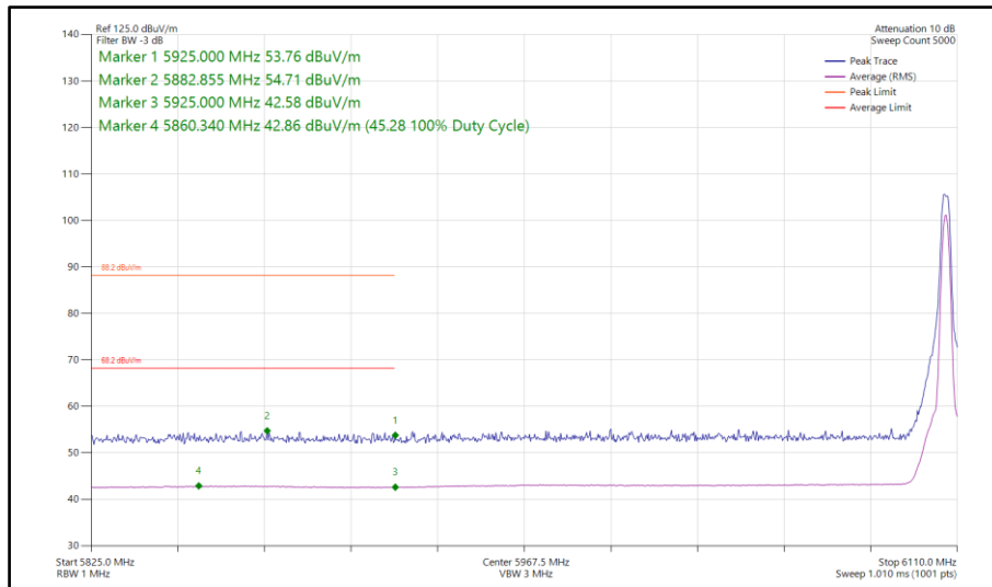
Figure 177 - Bluetooth LE2M, SISO, Core 1 - 6106 MHz Band Edge Frequency 5925 MHz
