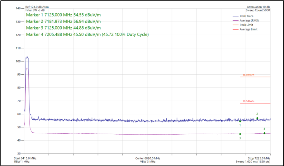
Figure 197 - Bluetooth HDRPL8, SISO, Core 1 - 6425 MHz Band Edge Frequency 7125 MHz
