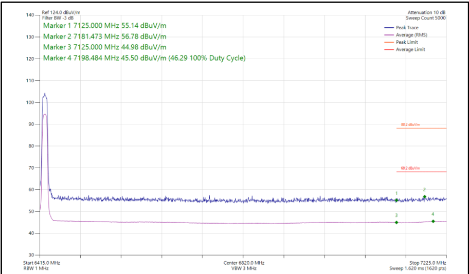
Figure 200 - Bluetooth XHDRPL24, SISO, Core 1 - 6425 MHz Band Edge Frequency 7125 MHz
