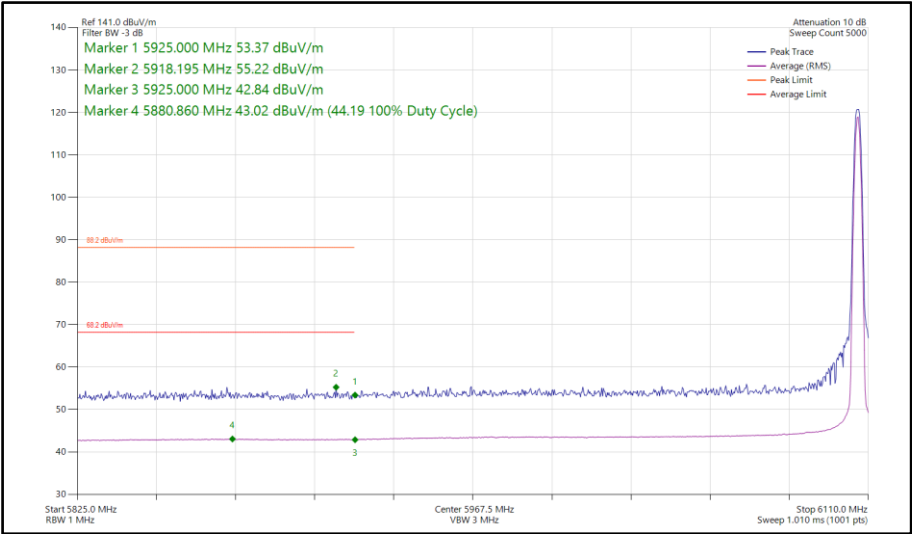
Figure 229 - Bluetooth DH5, SISO, Core 0 - 6106 MHz Band Edge Frequency 5925 MHz
