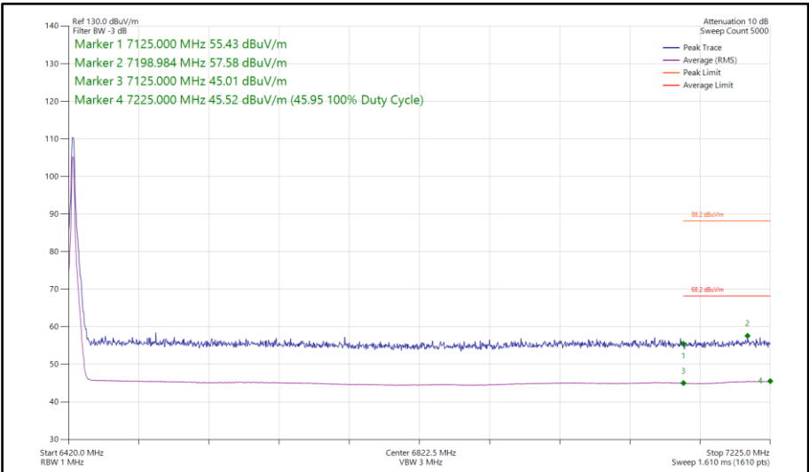
Figure 222 - Bluetooth HDT6, MIMO, Core 0-1 - 6425 MHz Band Edge Frequency 7125 MHz
