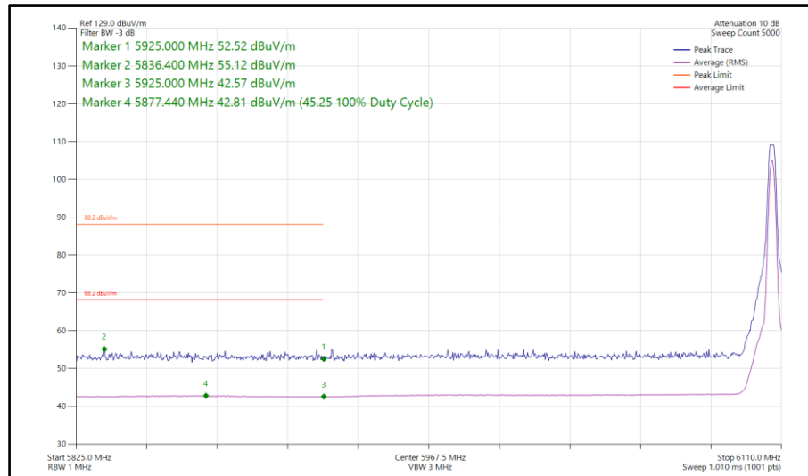
Figure 205 - Bluetooth LE2M, MIMO, Core 0-1 - 6106 MHz Band Edge Frequency 5925 MHz
