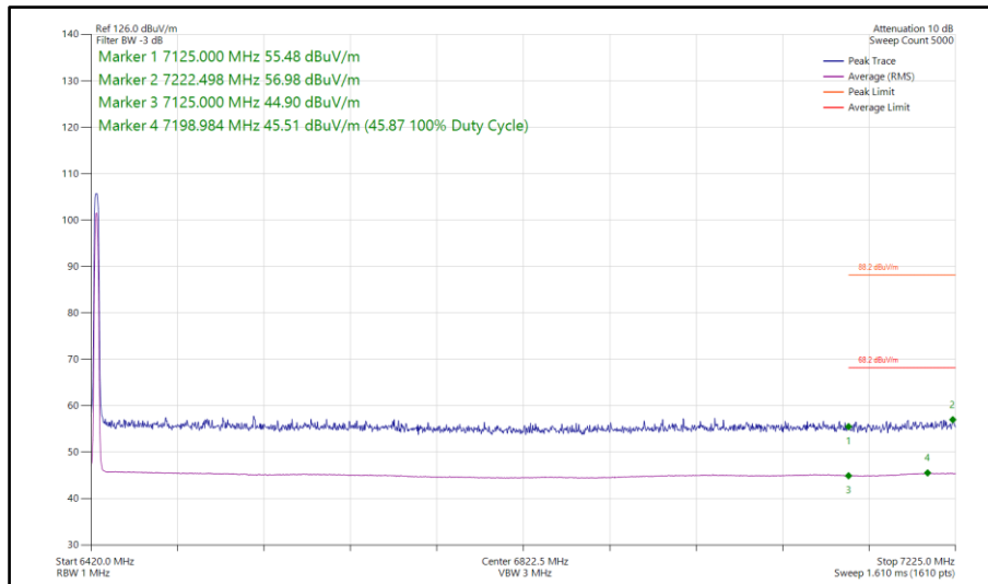
Figure 195 - Bluetooth HDRPS2, SISO, Core 1 - 6425 MHz Band Edge Frequency 7125 MHz
