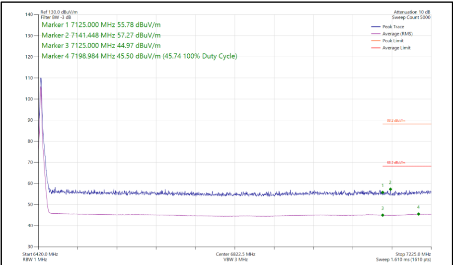
Figure 220 - Bluetooth HDT3, MIMO, Core 0-1 - 6425 MHz Band Edge Frequency 7125 MHz
