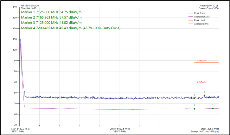
Figure 221 - Bluetooth HDT4, MIMO, Core 0-1 - 6425 MHz Band Edge Frequency 7125 MHz
