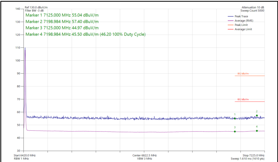
Figure 218 - Bluetooth LE1M, MIMO, Core 0-1 - 6425 MHz Band Edge Frequency 7125 MHz
