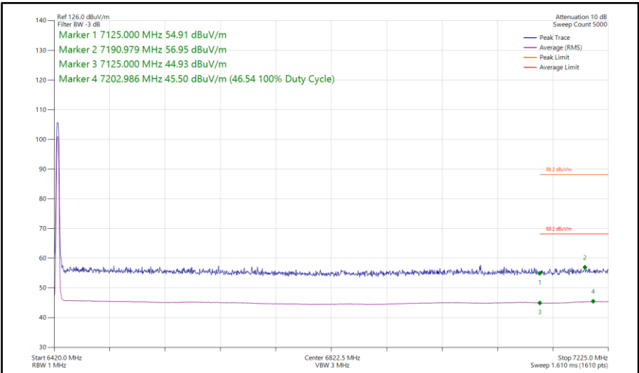
Figure 188 - Bluetooth HDR4, SISO, Core 1 - 6425 MHz Band Edge Frequency 7125 MHz
