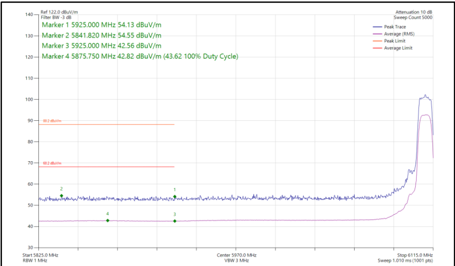
Figure 186 - Bluetooth XHDRPL24, SISO, Core 1 - 6109 MHz Band Edge Frequency 5925 MHz
