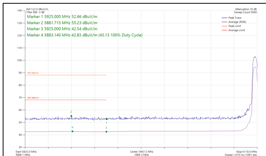
Figure 182 - Bluetooth HDRPM12, SISO, Core 1 - 6107 MHz Band Edge Frequency 5925 MHz
