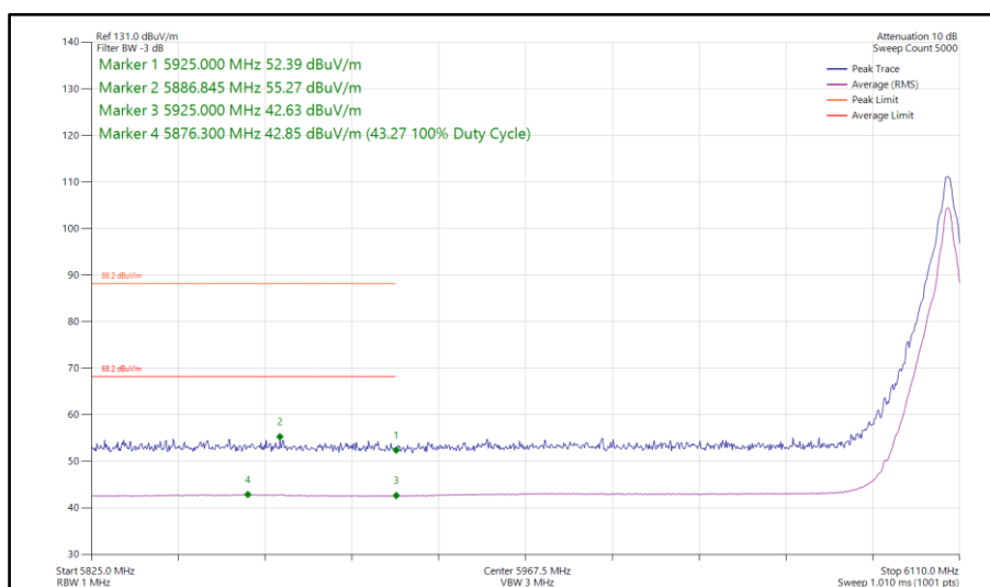
Figure 208 - Bluetooth HDT6, MIMO, Core 0-1 - 6106 MHz Band Edge Frequency 5925 MHz
