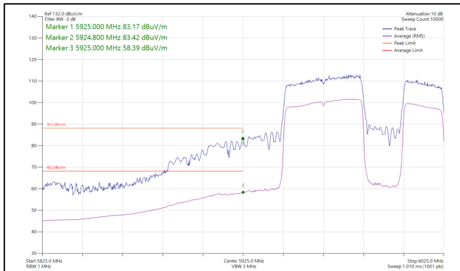
Figure 488 - 802.11be EHT80, RU 484+242-92, SISO, Core 1 - 5985 MHz Band Edge Frequency 5925 MHz
