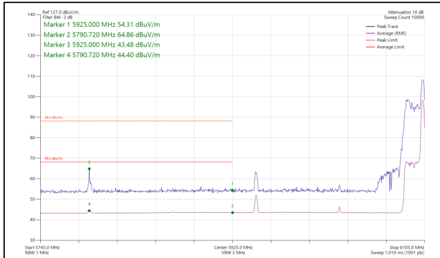
Figure 519 - 802.11ax HE160, RU 26-36S, SISO, Core 1 - 6025 MHz Band Edge Frequency 5925 MHz
