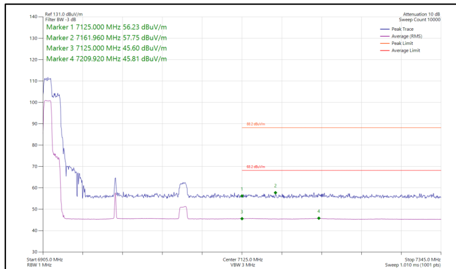
Figure 515 - 802.11ax HE160, RU 106-53P, SISO, Core 0 - 6985 MHz Band Edge Frequency 7125 MHz
