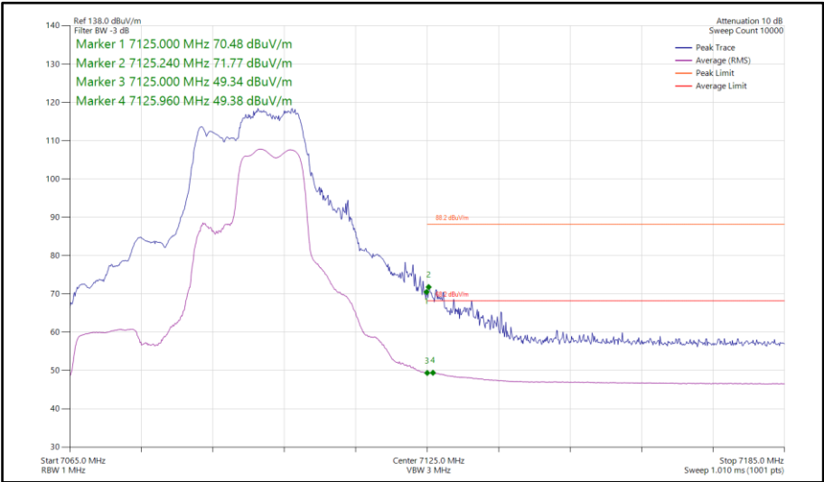
Figure 466 - 802.11be EHT40, RU 106+26-85, CDD, Core 0-1 - 7085 MHz Band Edge Frequency 7125 MHz
