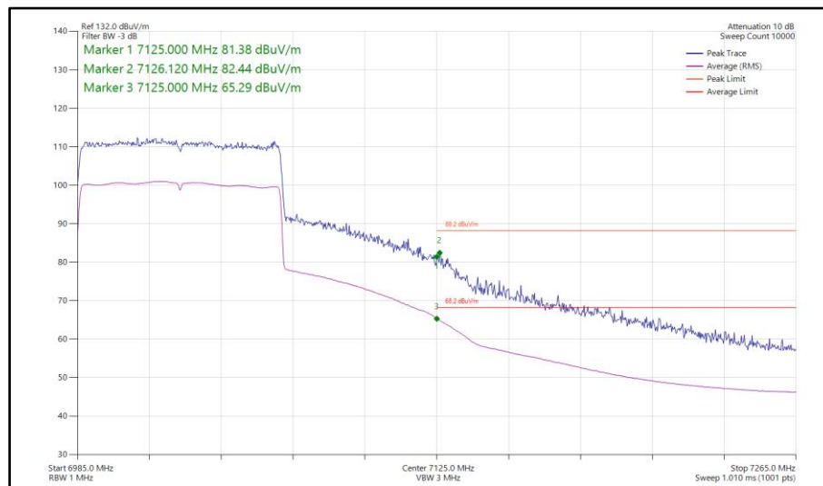
Figure 508 - 802.11ax HE80, SU, TxBF, Core 0-1 - 7025 MHz Band Edge Frequency 7125 MHz
