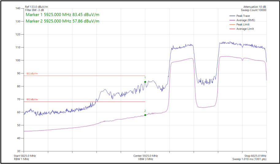
Figure 480 - 802.11be EHT80, RU 484+242-91, SISO, Core 0 - 5985 MHz Band Edge Frequency 5925 MHz
