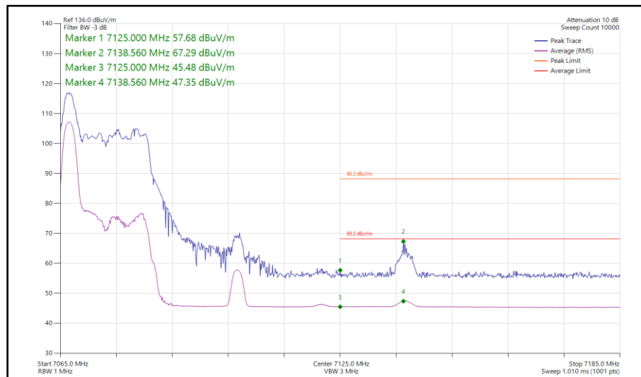
Figure 472 - 802.11ax HE40, RU 26-0, SDM, Core 0-1 - 7085 MHz Band Edge Frequency 7125 MHz
