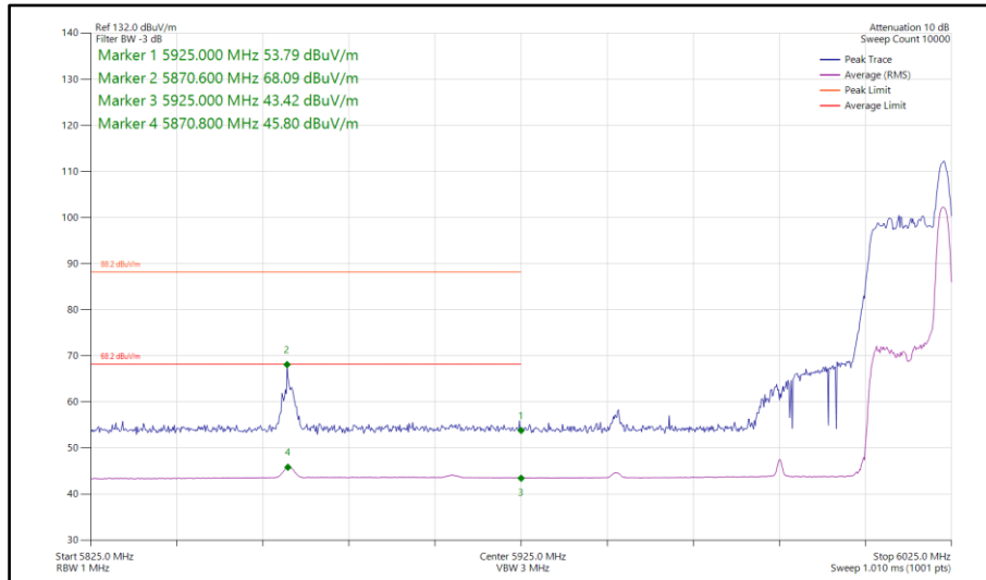
Figure 487 - 802.11ax HE80, RU 26-36, SISO, Core 1 - 5985 MHz Band Edge Frequency 5925 MHz
