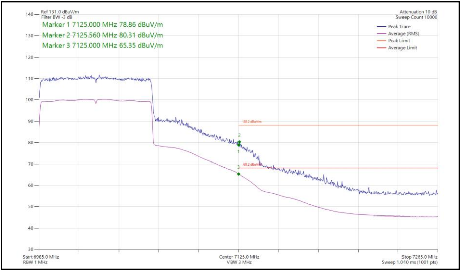
Figure 490 - 802.11ax HE80, SU, SISO, Core 1 - 7025 MHz Band Edge Frequency 7125 MHz
