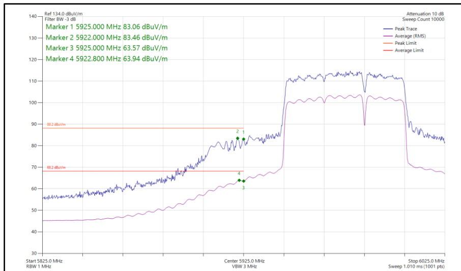
Figure 496 - 802.11be EHT80, RU 484+242-93, CDD, Core 0-1 - 5985 MHz Band Edge Frequency 5925 MHz
