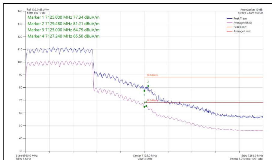
Figure 498 - 802.11ax HE80, SU, CDD, Core 0-1 - 7025 MHz Band Edge Frequency 7125 MHz
