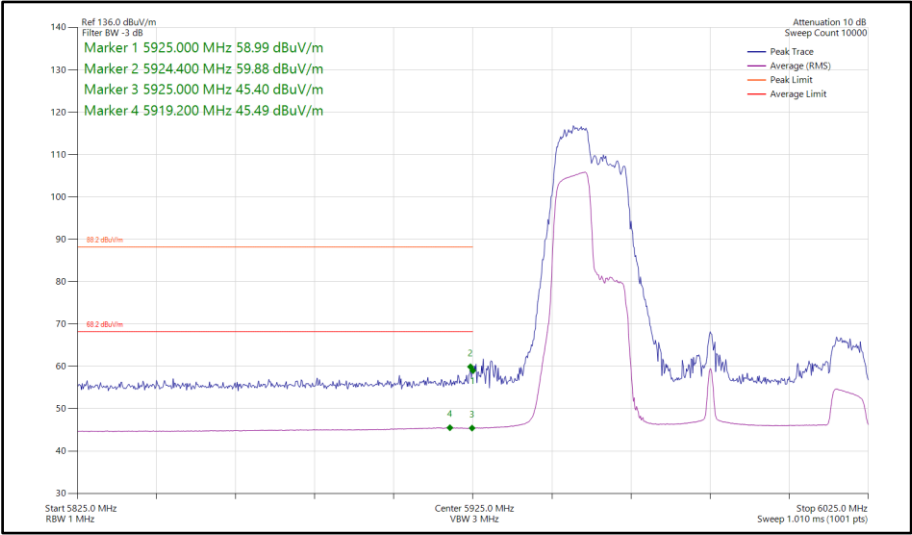
Figure 479 - 802.11ax HE80, RU 106-53, SISO, Core 0 - 5985 MHz Band Edge Frequency 5925 MHz
