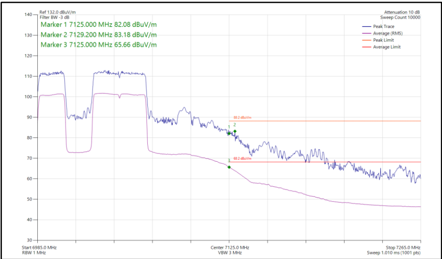
Figure 484 - 802.11be EHT80, RU 484+242-91, SISO, Core 0 - 7025 MHz Band Edge Frequency 7125 MHz
