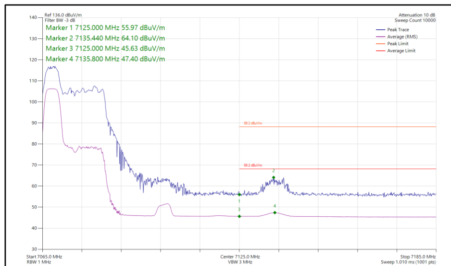
Figure 455 - 802.11ax HE40, RU 52-37, SISO, Core 1 - 7085 MHz Band Edge Frequency 7125 MHz
