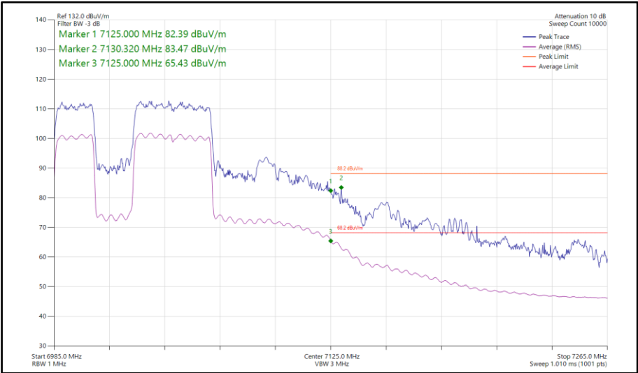
Figure 506 - 802.11be EHT80, RU 484+242-91, SDM, Core 0-1 - 7025 MHz Band Edge Frequency 7125 MHz
