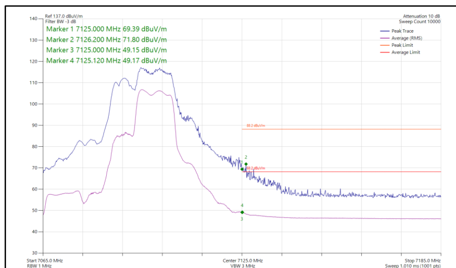
Figure 473 - 802.11be EHT40, RU 106+26-85, SDM, Core 0-1 - 7085 MHz Band Edge Frequency 7125 MHz
