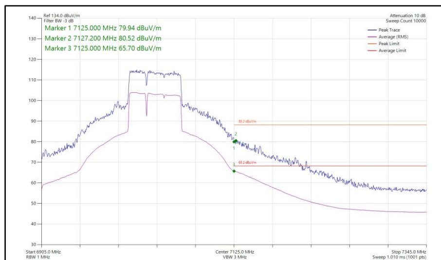
Figure 516 - 802.11be EHT160, RU 484+242-90S, SISO, Core 0 - 6985 MHz Band Edge Frequency 7125 MHz
