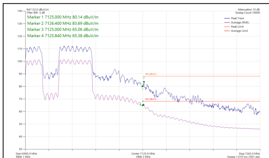
Figure 500 - 802.11be EHT80, RU 484+242-91, CDD, Core 0-1 - 7025 MHz Band Edge Frequency 7125 MHz
