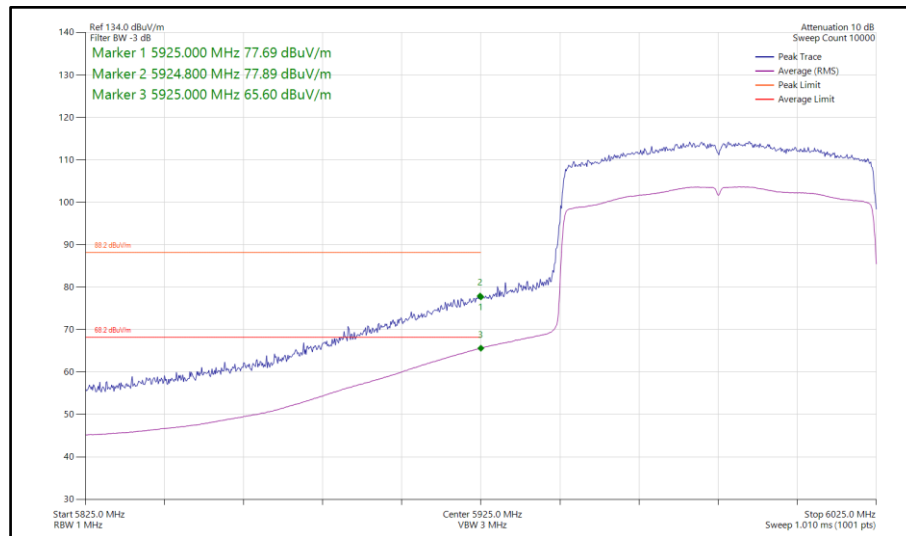
Figure 507 - 802.11ax HE80, SU, TxBF, Core 0-1 - 5985 MHz Band Edge Frequency 5925 MHz
