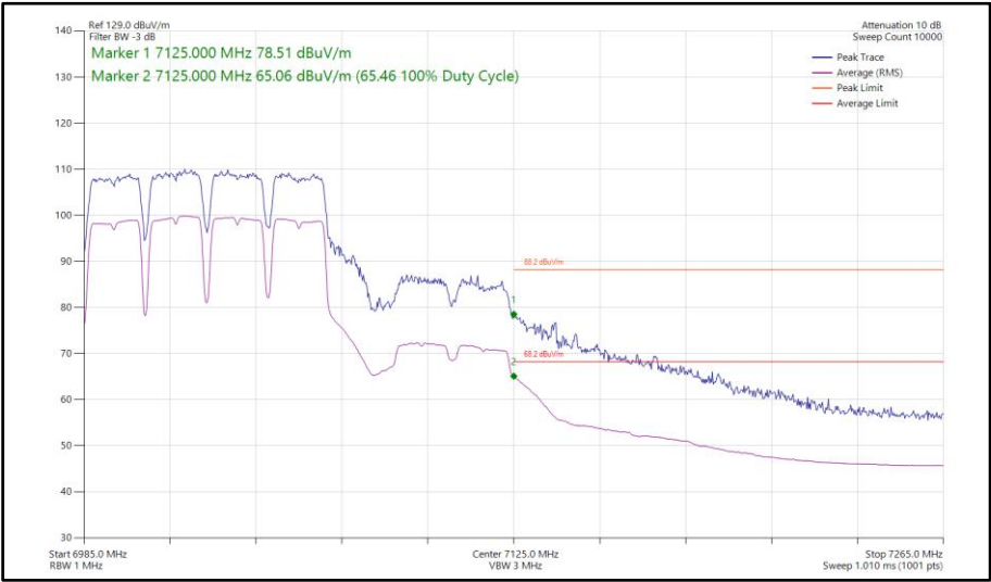
Figure 489 - 802.11a a80, SISO, Core 1 - 7025 MHz Band Edge Frequency 7125 MHz
