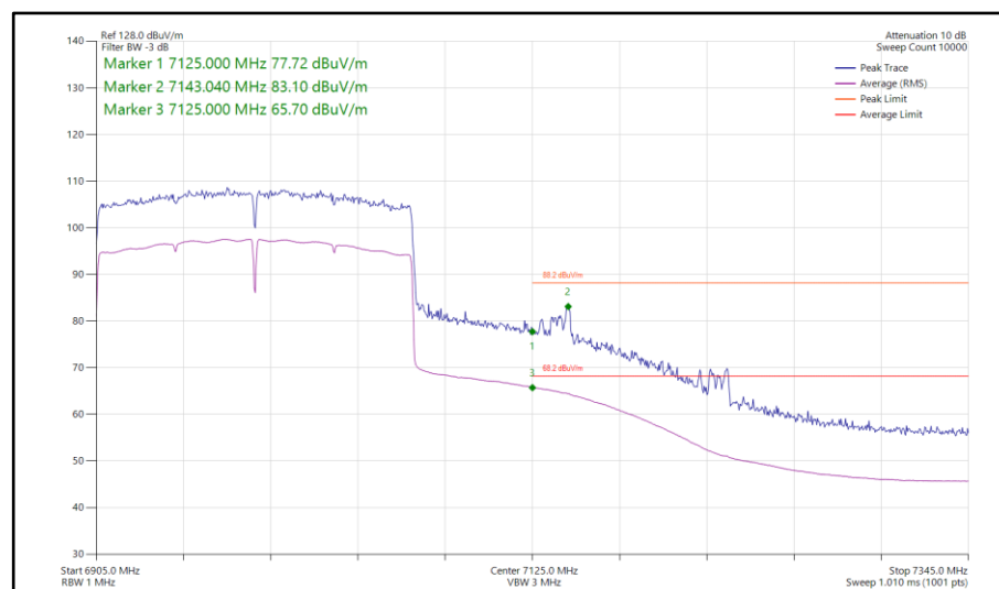
Figure 514 - 802.11ax HE160, SU, SISO, Core 0 - 6985 MHz Band Edge Frequency 7125 MHz
