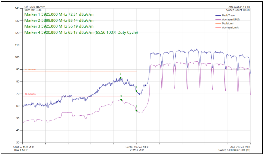
Figure 517 - 802.11a a160, SISO, Core 1 - 6025 MHz Band Edge Frequency 5925 MHz
