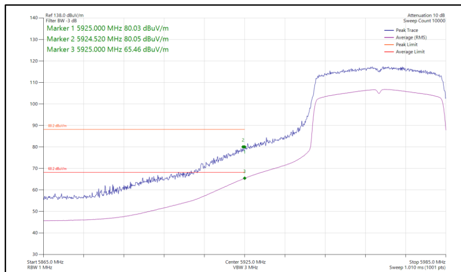
Figure 474 - 802.11ax HE40, SU, TxBF, Core 0-1 - 5965 MHz Band Edge Frequency 5925 MHz
