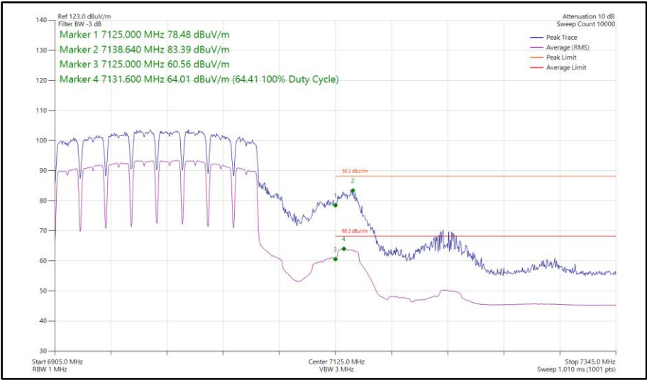
Figure 521 - 802.11a a160, SISO, Core 1 - 6985 MHz Band Edge Frequency 7125 MHz
