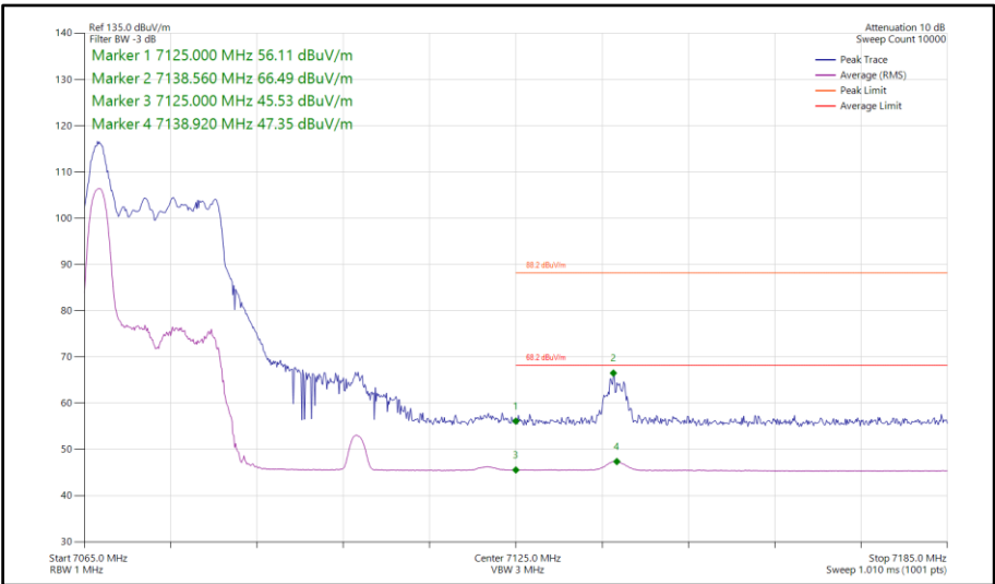
Figure 465 - 802.11ax HE40, RU 26-0, CDD, Core 0-1 - 7085 MHz Band Edge Frequency 7125 MHz
