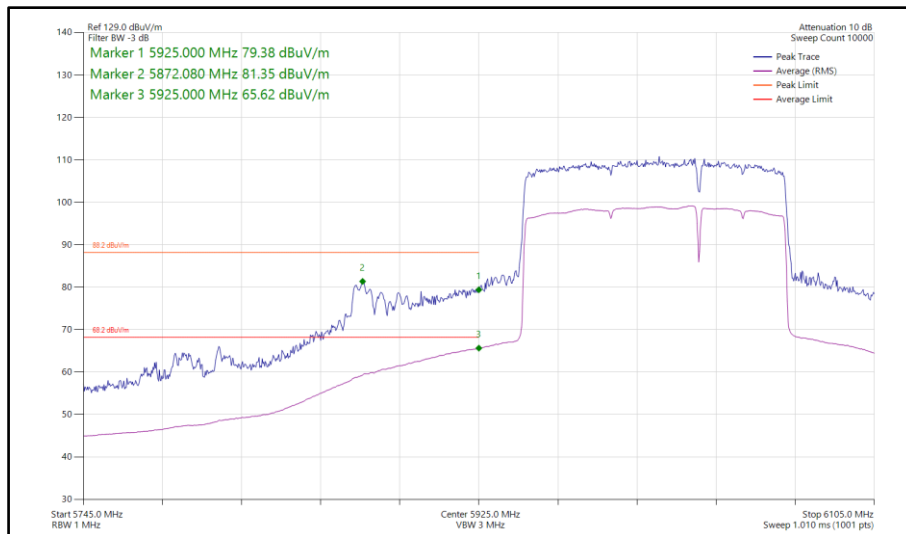
Figure 520 - 802.11be EHT160, RU 996+484-95S, SISO, Core 1 - 6025 MHz Band Edge Frequency 5925 MHz
