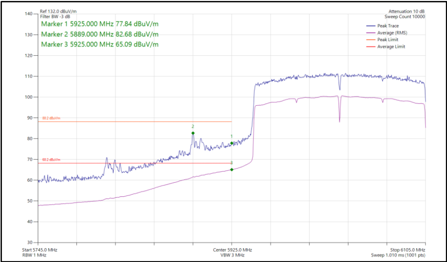
Figure 509 - 802.11a a160, SISO, Core 0 - 6025 MHz Band Edge Frequency 5925 MHz
