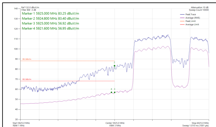
Figure 503 - 802.11be EHT80, RU 484+242-92, SDM, Core 0-1 - 5985 MHz Band Edge Frequency 5925 MHz
