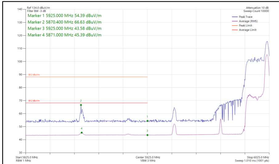
Figure 495 - 802.11ax HE80, RU 26-36, CDD, Core 0-1 - 5985 MHz Band Edge Frequency 5925 MHz
