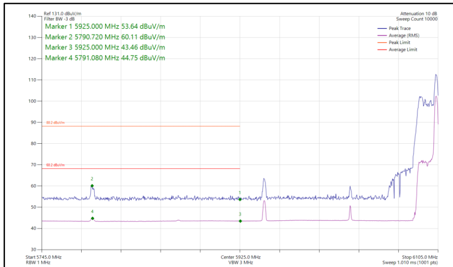
Figure 511 - 802.11ax HE160, RU 26-36S, SISO, Core 0 - 6025 MHz Band Edge Frequency 5925 MHz
