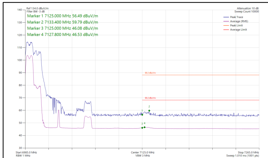
Figure 499 - 802.11ax HE80, RU 106-53, CDD, Core 0-1 - 7025 MHz Band Edge Frequency 7125 MHz
