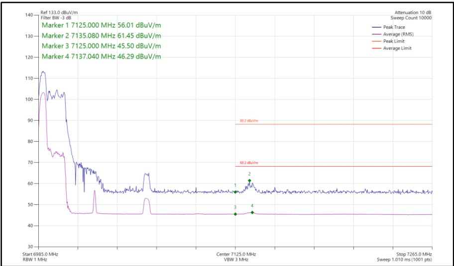
Figure 505 - 802.11ax HE80, RU 52-37, SDM, Core 0-1 - 7025 MHz Band Edge Frequency 7125 MHz
