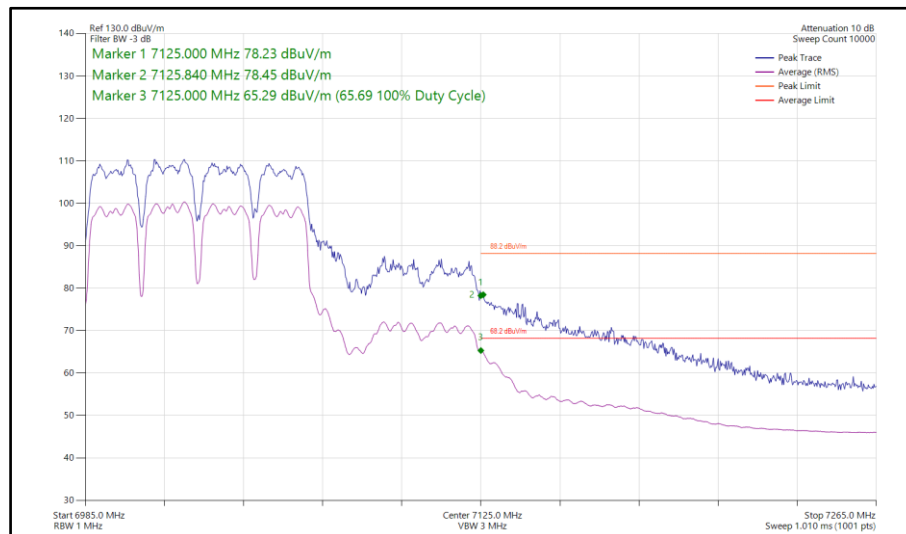
Figure 497 - 802.11a a80, CDD, Core 0-1 - 7025 MHz Band Edge Frequency 7125 MHz
