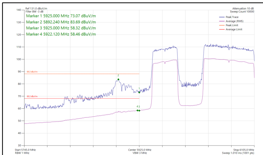
Figure 512 - 802.11be EHT160, RU 996+484-95P, SISO, Core 0 - 6025 MHz Band Edge Frequency 5925 MHz
