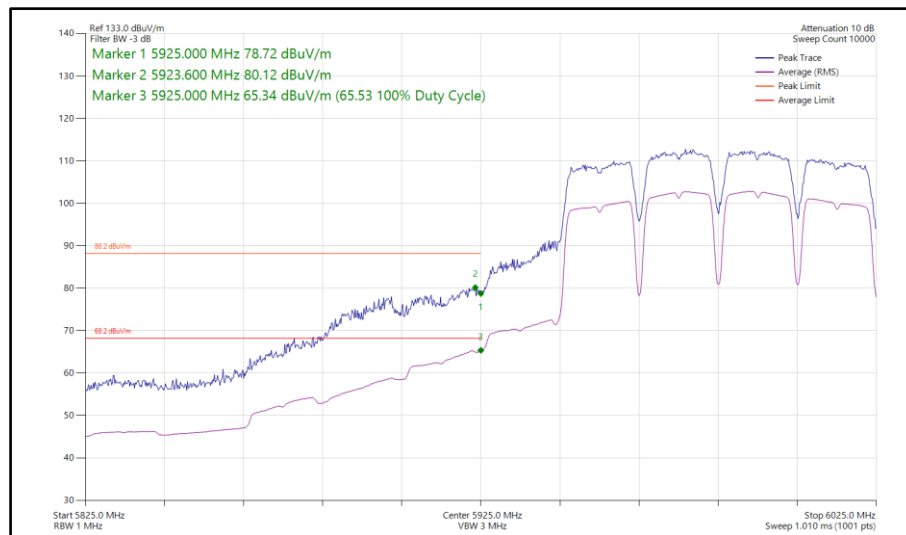
Figure 477 - 802.11a a80, SISO, Core 0 - 5985 MHz Band Edge Frequency 5925 MHz
