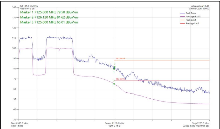
Figure 492 - 802.11be EHT80, RU 484+242-91, SISO, Core 1 - 7025 MHz Band Edge Frequency 7125 MHz
