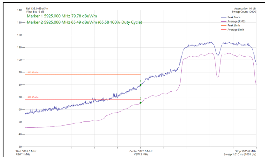
Figure 457 - 802.11a a40, CDD, Core 0-1 - 5965 MHz Band Edge Frequency 5925 MHz
