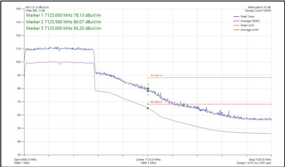
Figure 504 - 802.11ax HE80, SU, SDM, Core 0-1 - 7025 MHz Band Edge Frequency 7125 MHz
