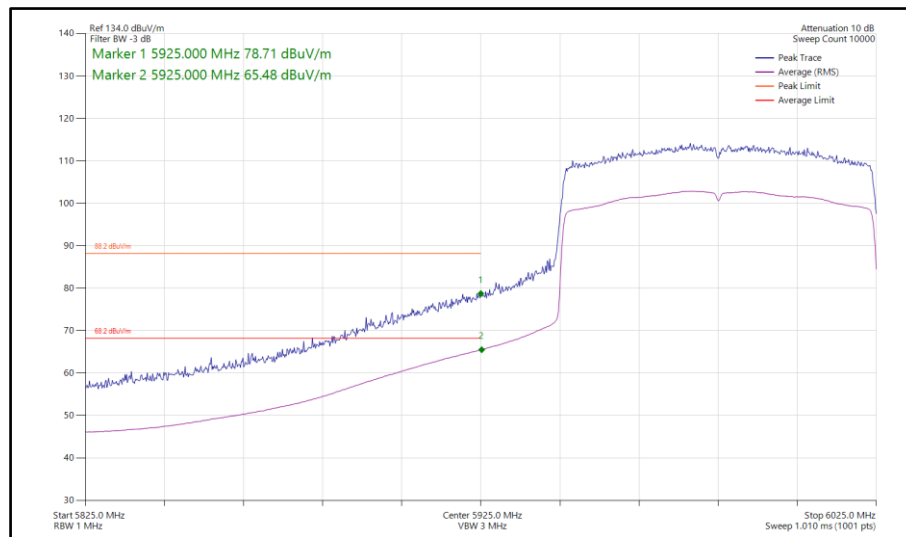
Figure 501 - 802.11ax HE80, SU, SDM, Core 0-1 - 5985 MHz Band Edge Frequency 5925 MHz
