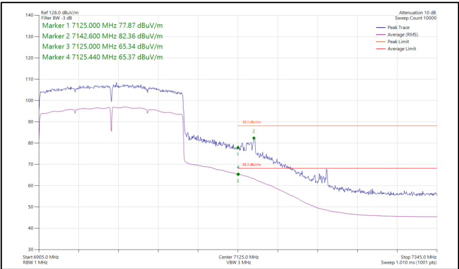
Figure 522 - 802.11ax HE160, SU, SISO, Core 1 - 6985 MHz Band Edge Frequency 7125 MHz
