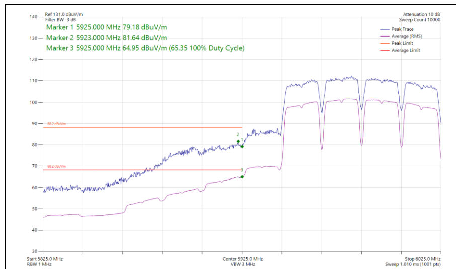
Figure 485 - 802.11a a80, SISO, Core 1 - 5985 MHz Band Edge Frequency 5925 MHz
