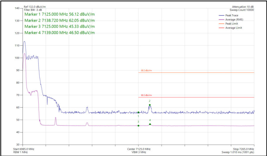
Figure 483 - 802.11ax HE80, RU 26-0, SISO, Core 0 - 7025 MHz Band Edge Frequency 7125 MHz
