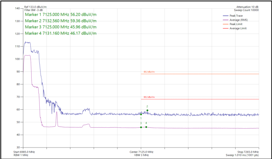
Figure 491 - 802.11ax HE80, RU 106-53, SISO, Core 1 - 7025 MHz Band Edge Frequency 7125 MHz
