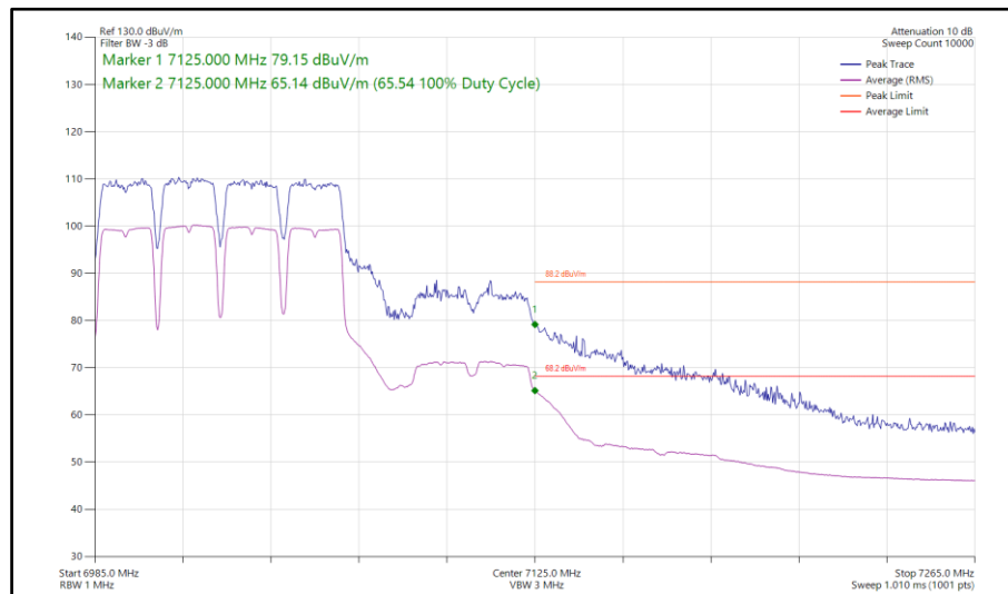
Figure 481 - 802.11a a80, SISO, Core 0 - 7025 MHz Band Edge Frequency 7125 MHz
