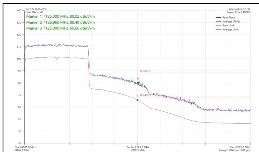
Figure 482 - 802.11ax HE80, SU, SISO, Core 0 - 7025 MHz Band Edge Frequency 7125 MHz
