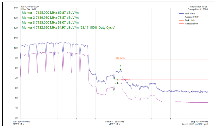
Figure 513 - 802.11a a160, SISO, Core 0 - 6985 MHz Band Edge Frequency 7125 MHz
