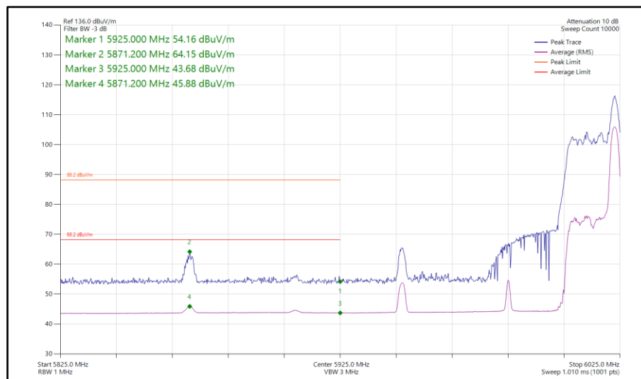
Figure 502 - 802.11ax HE80, RU 26-36, SDM, Core 0-1 - 5985 MHz Band Edge Frequency 5925 MHz
