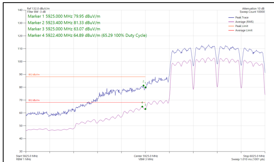
Figure 493 - 802.11a a80, CDD, Core 0-1 - 5985 MHz Band Edge Frequency 5925 MHz
