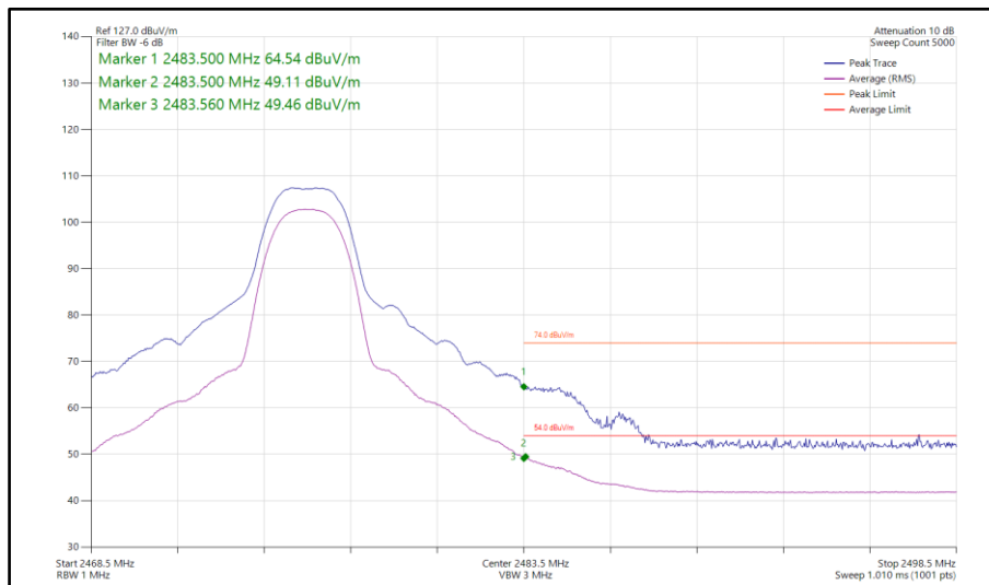
Figure 68 - Bluetooth HDT4, SISO, Core 2 - 2476 MHz Band Edge Frequency 2483.5 MHz
