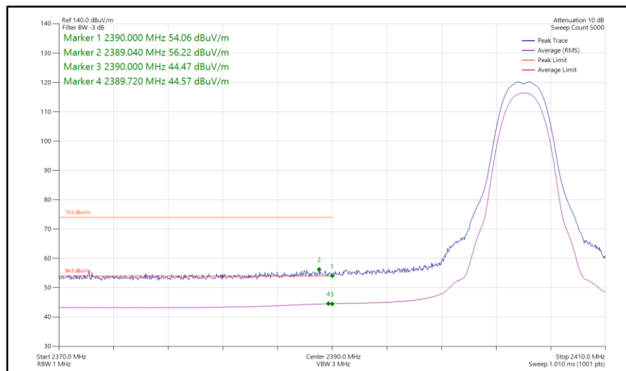
Figure 127 - Bluetooth HDT3, SISO, Core 1 - 2404 MHz Band Edge Frequency 2390 MHz
