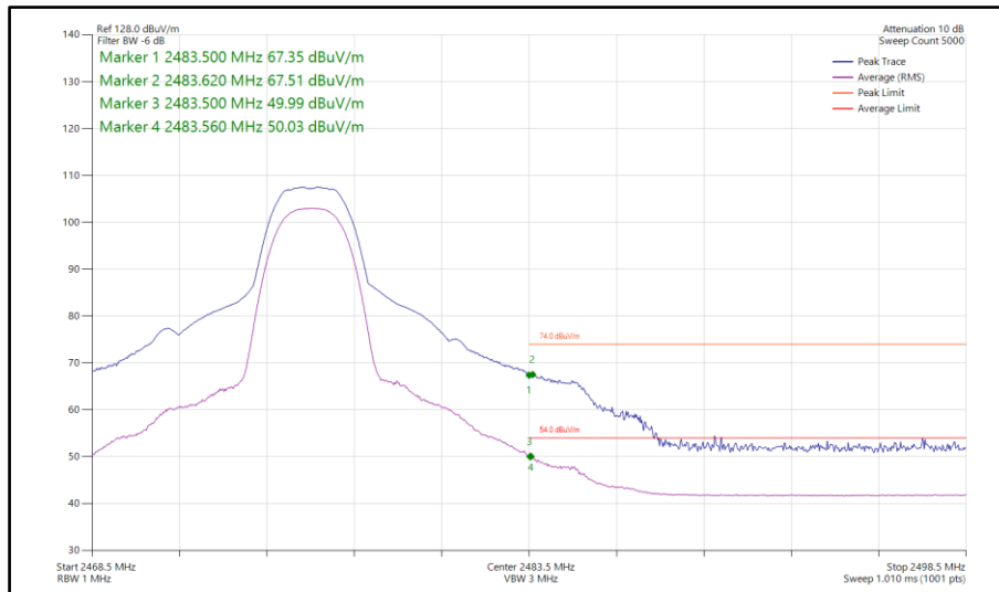
Figure 67 - Bluetooth HDT3, SISO, Core 2 - 2476 MHz Band Edge Frequency 2483.5 MHz
