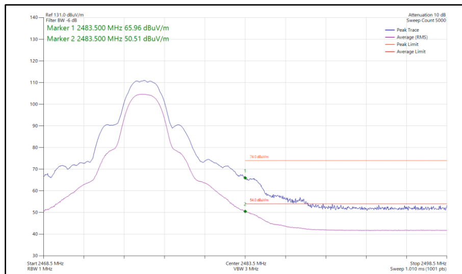
Figure 93 - Bluetooth HDT6, MIMO, Core 0-1 - 2476 MHz Band Edge Frequency 2483.5 MHz
