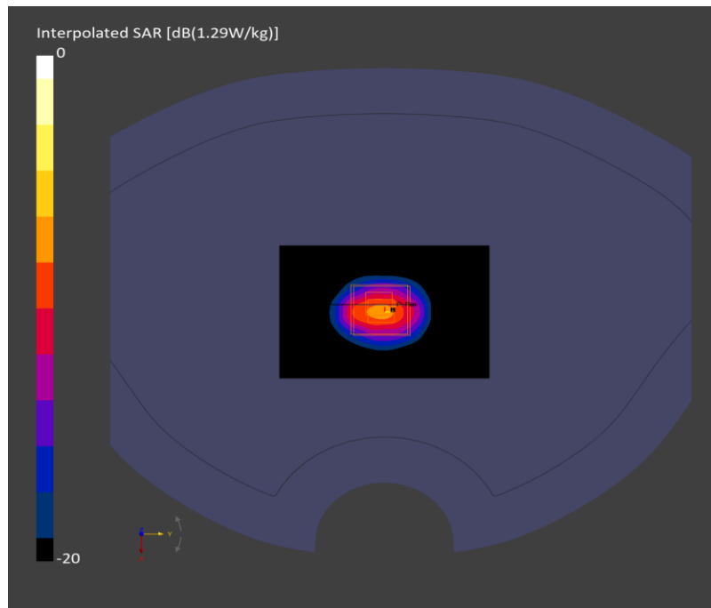
Figure C.1: Testing results for the A3592 at 2402.000 MHz
