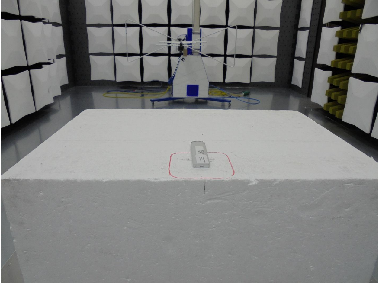
Figure 1– 15C Radiated Disturbance - Below 1 GHz
