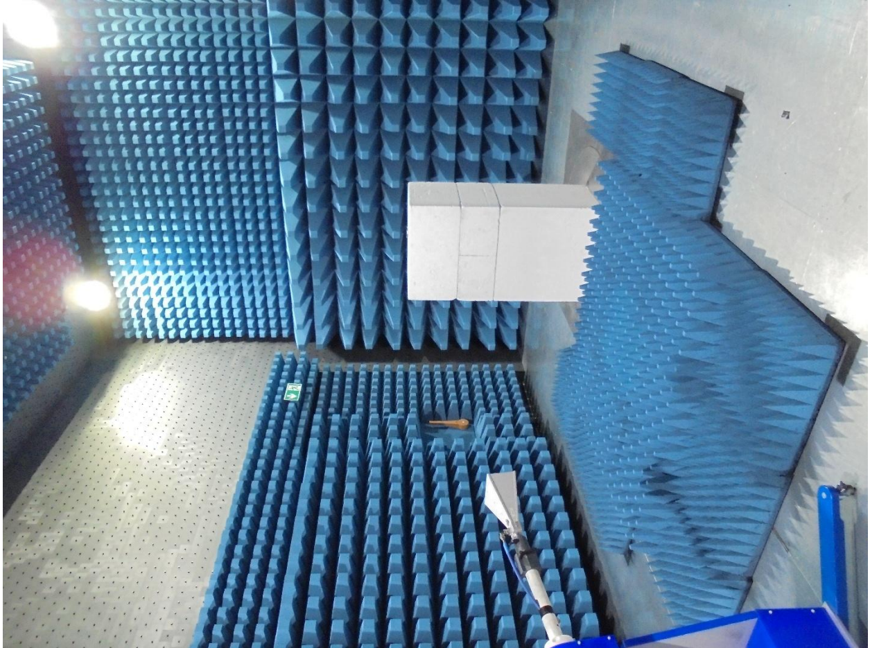
Figure 4– 15C Radiated Disturbance - Above 1 GHz
