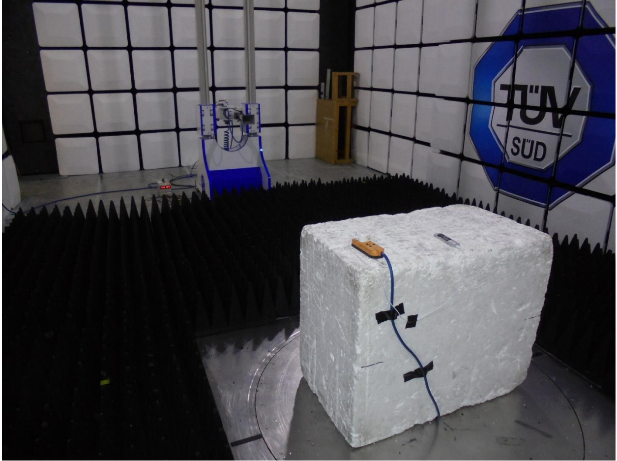
Figure 5– 15B Radiated Disturbance - Above 1 GHz
