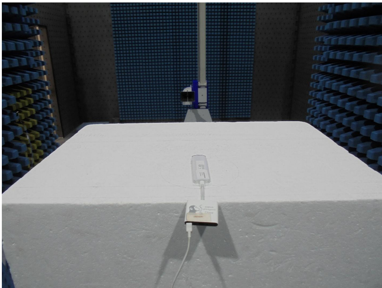
Figure 3– 15C Radiated Disturbance - Above 1 GHz
