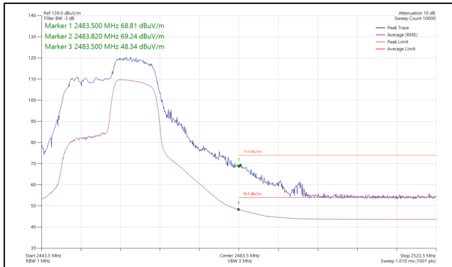
Figure 118 - 802.11ax HE20, RU106-54, SISO, Core 1 - 2457 MHz Band Edge Frequency 2483.5 MHz
