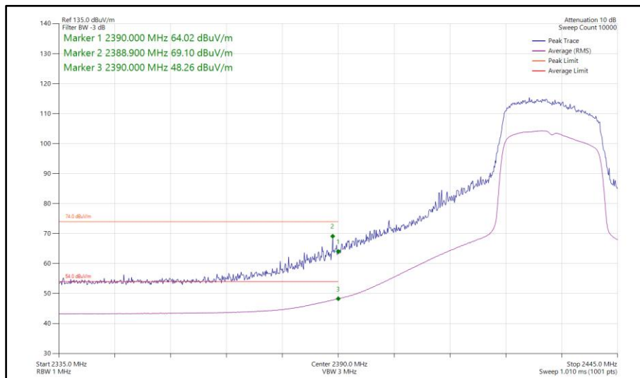
Figure 83 - 802.11ax HE20, SU, SISO, Core 1 - 2432 MHz Band Edge Frequency 2390 MHz
