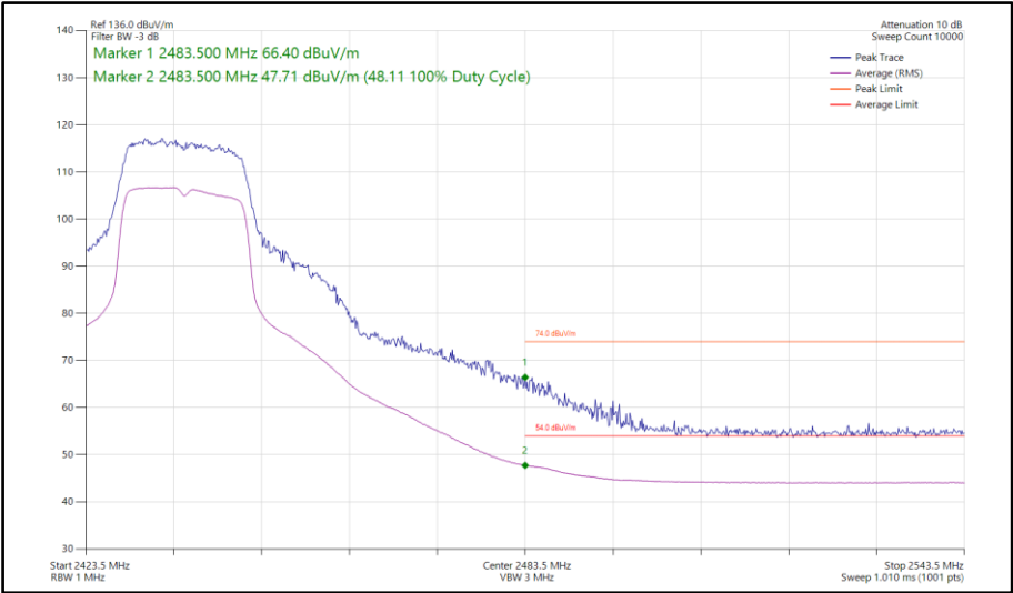
Figure 94 - 802.11g, SISO, Core 1 - 2437 MHz Band Edge Frequency 2483.5 MHz
