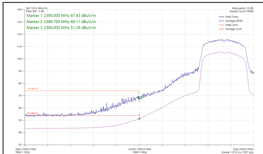
Figure 81 - 802.11ax HE20, SU, SISO, Core 1 - 2427 MHz Band Edge Frequency 2390 MHz
