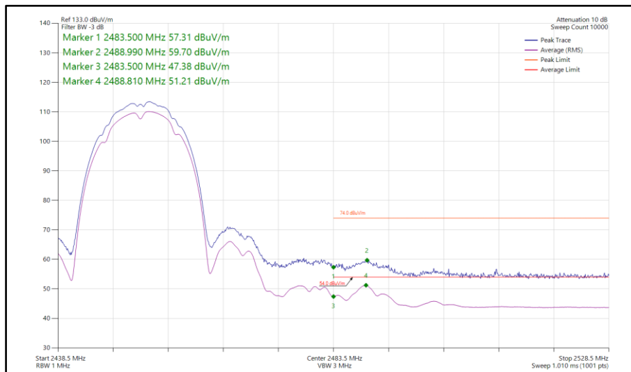
Figure 89 - 802.11b, SISO, Core 1 - 2452 MHz Band Edge Frequency 2483.5 MHz
