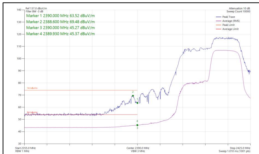
Figure 76 - 802.11ax HE20, RU106-54, SISO, Core 1 - 2412 MHz Band Edge Frequency 2390 MHz
