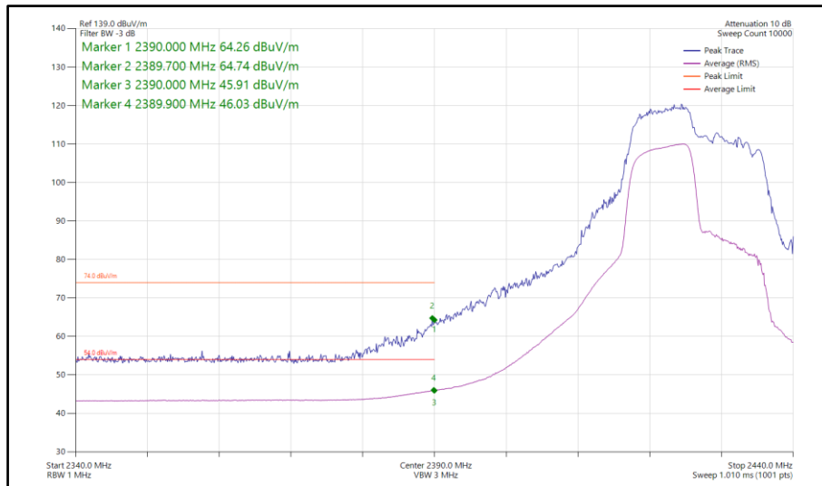
Figure 82 - 802.11ax HE20, RU106-53, SISO, Core 1 - 2427 MHz Band Edge Frequency 2390 MHz
