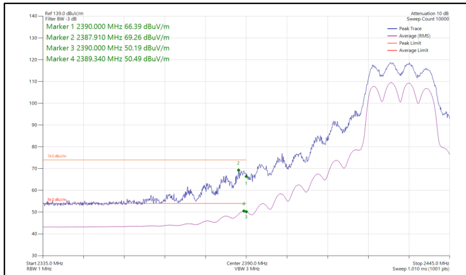
Figure 141 - 802.11n HT20, CDD, Core 0-1 - 2432 MHz Band Edge Frequency 2390 MHz
