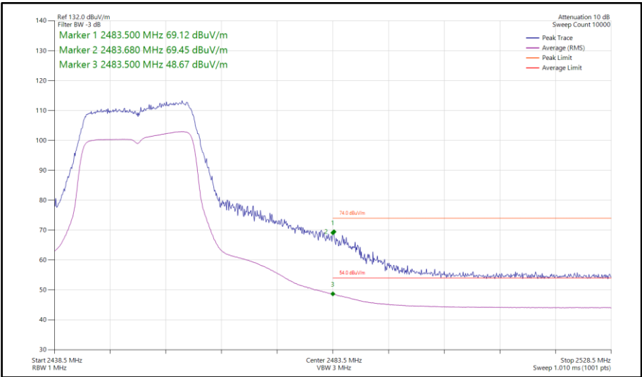
Figure 105 - 802.11n HT20, SISO, Core 1 - 2452 MHz Band Edge Frequency 2483.5 MHz
