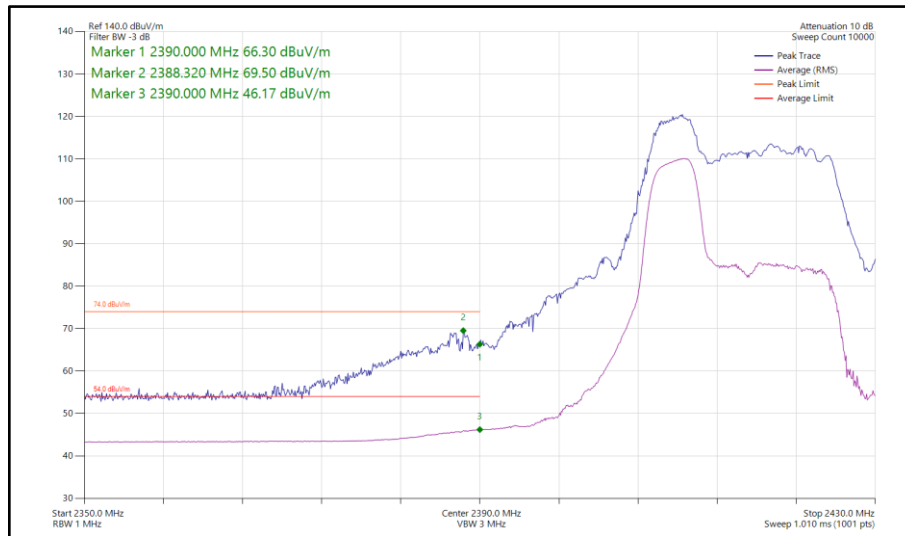
Figure 78 - 802.11ax HE20, RU52-37, SISO, Core 1 - 2417 MHz Band Edge Frequency 2390 MHz
