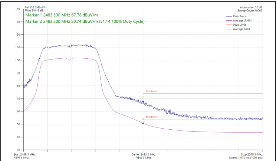
Figure 99 - 802.11g, SISO, Core 1 - 2462 MHz Band Edge Frequency 2483.5 MHz
