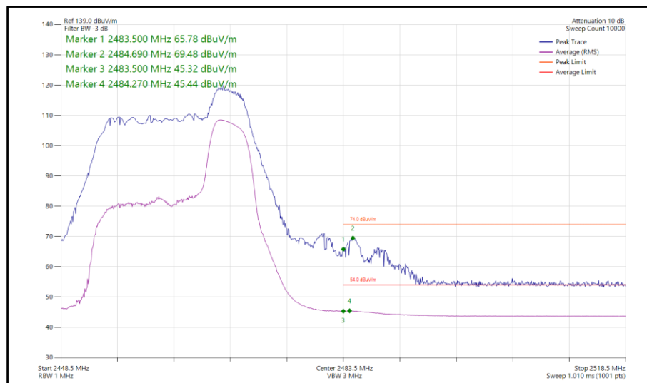
Figure 120 - 802.11ax HE20, RU52-40, SISO, Core 1 - 2462 MHz Band Edge Frequency 2483.5 MHz
