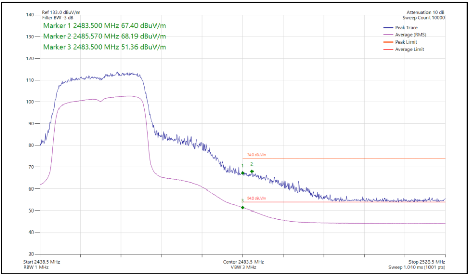
Figure 115 - 802.11ax HE20, SU, SISO, Core 1 - 2452 MHz Band Edge Frequency 2483.5 MHz
