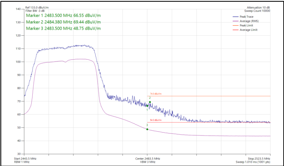
Figure 117 - 802.11ax HE20, SU, SISO, Core 1 - 2457 MHz Band Edge Frequency 2483.5 MHz
