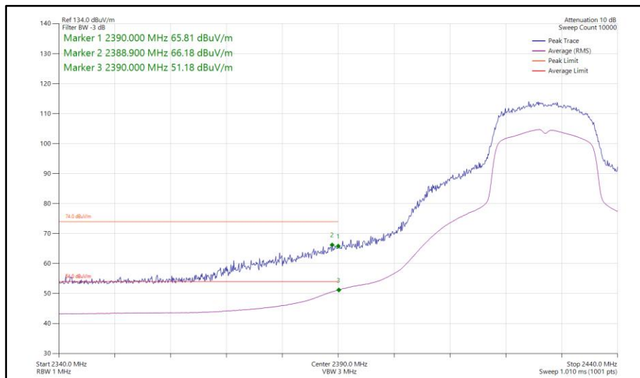
Figure 73 - 802.11n HT20, SISO, Core 1 - 2427 MHz Band Edge Frequency 2390 MHz
