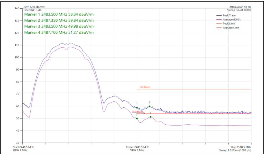
Figure 91 - 802.11b, SISO, Core 1 - 2462 MHz Band Edge Frequency 2483.5 MHz
