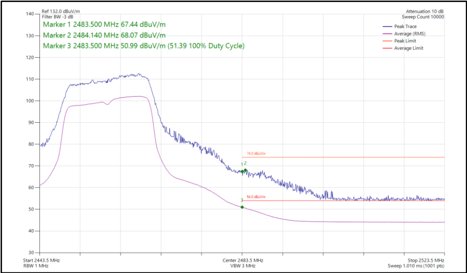
Figure 98 - 802.11g, SISO, Core 1 - 2457 MHz Band Edge Frequency 2483.5 MHz
