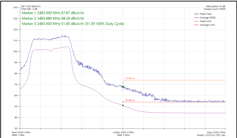
Figure 97 - 802.11g, SISO, Core 1 - 2452 MHz Band Edge Frequency 2483.5 MHz
