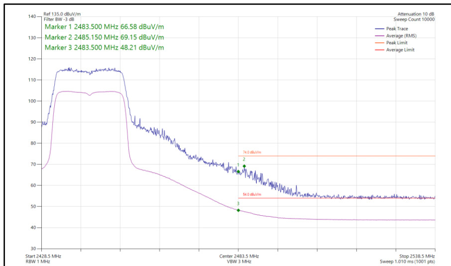
Figure 111 - 802.11ax HE20, SU, SISO, Core 1 - 2442 MHz Band Edge Frequency 2483.5 MHz
