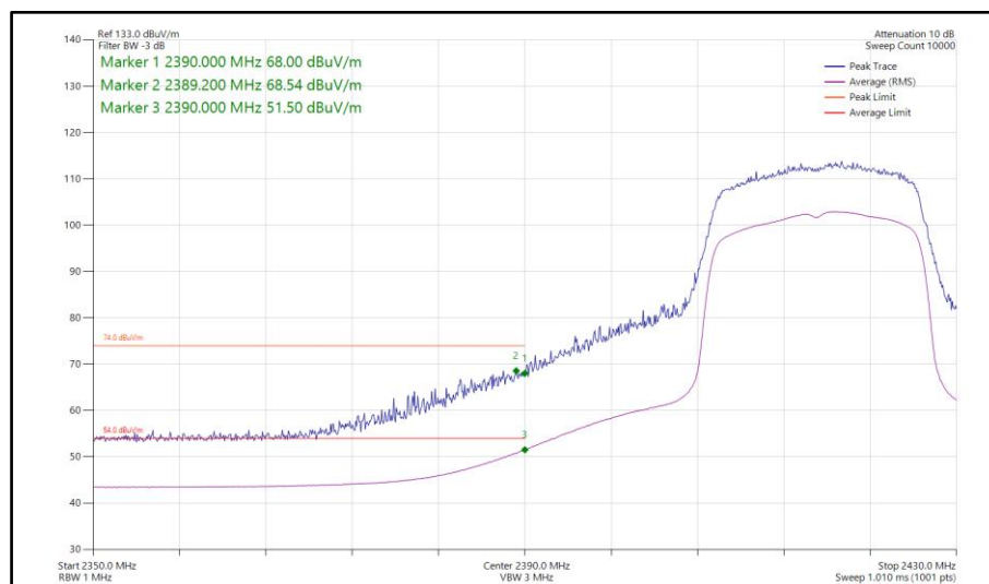
Figure 77 - 802.11ax HE20, SU, SISO, Core 1 - 2417 MHz Band Edge Frequency 2390 MHz
