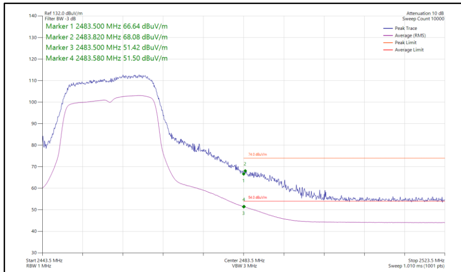
Figure 106 - 802.11n HT20, SISO, Core 1 - 2457 MHz Band Edge Frequency 2483.5 MHz
