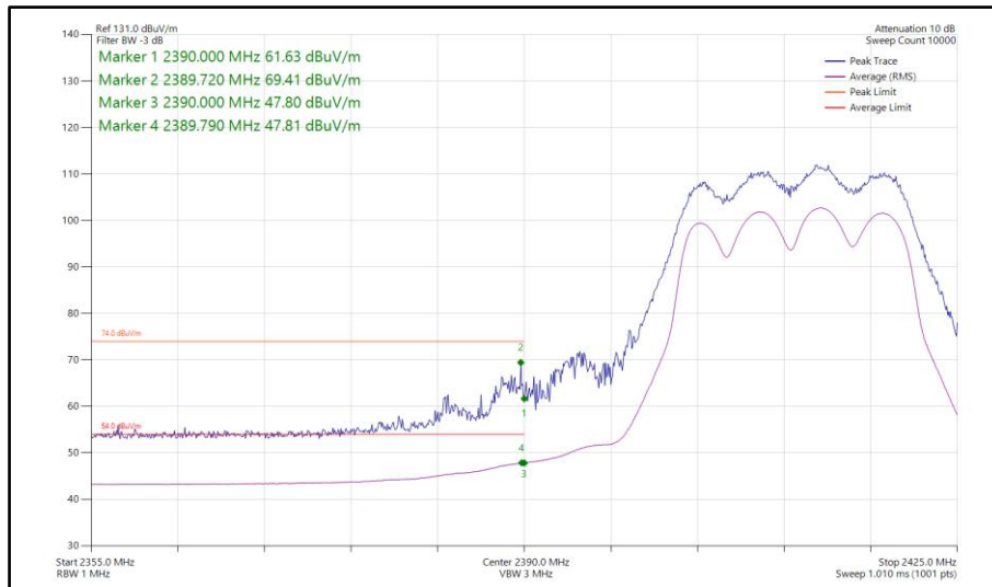
Figure 137 - 802.11n HT20, CDD, Core 0-1 - 2412 MHz Band Edge Frequency 2390 MHz
