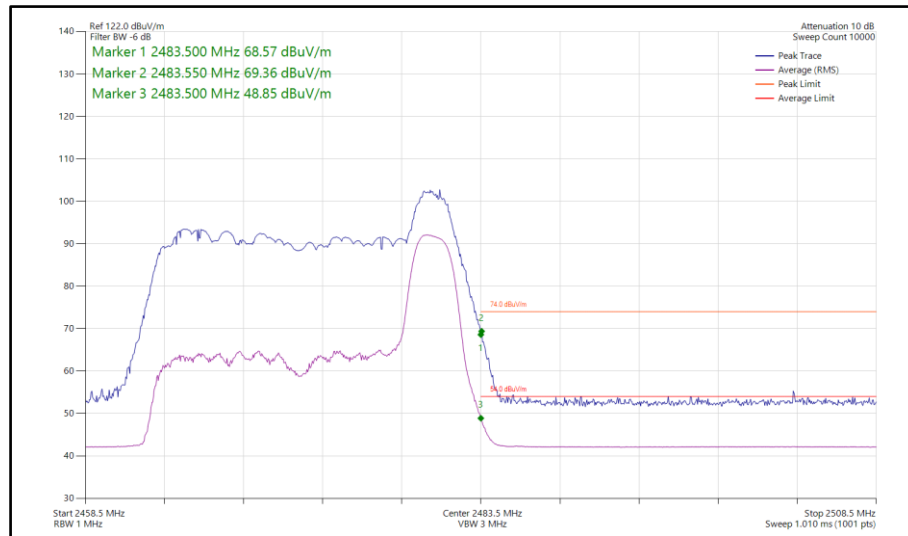
Figure 124 - 802.11ax HE20, RU26-8, SISO, Core 1 - 2472 MHz Band Edge Frequency 2483.5 MHz
