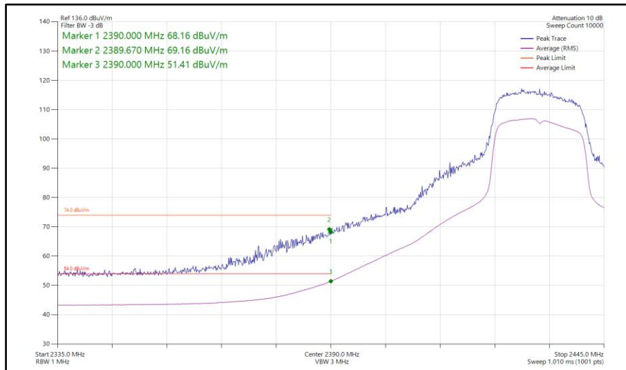
Figure 74 - 802.11n HT20, SISO, Core 1 - 2432 MHz Band Edge Frequency 2390 MHz
