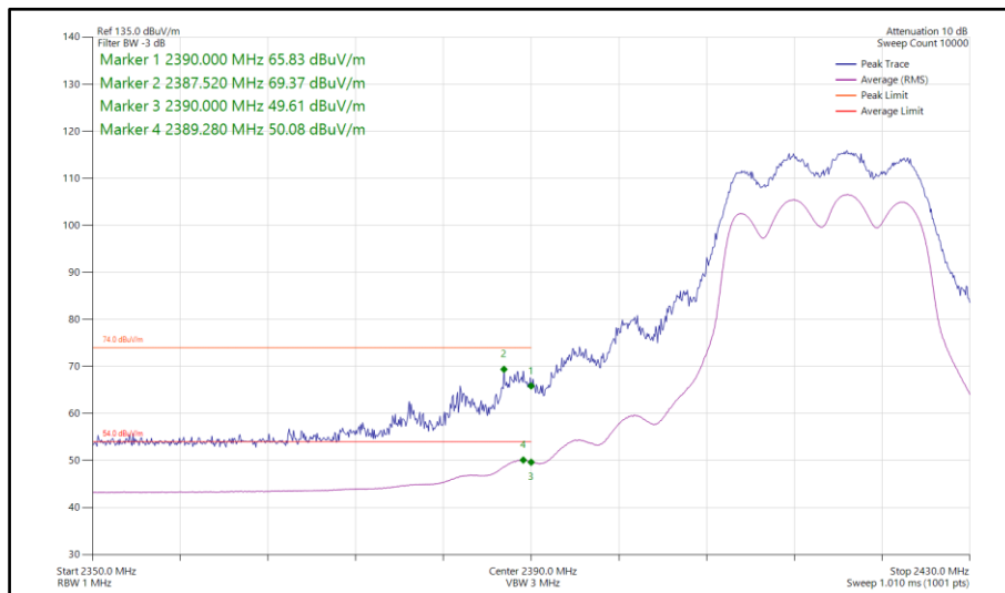
Figure 138 - 802.11n HT20, CDD, Core 0-1 - 2417 MHz Band Edge Frequency 2390 MHz
