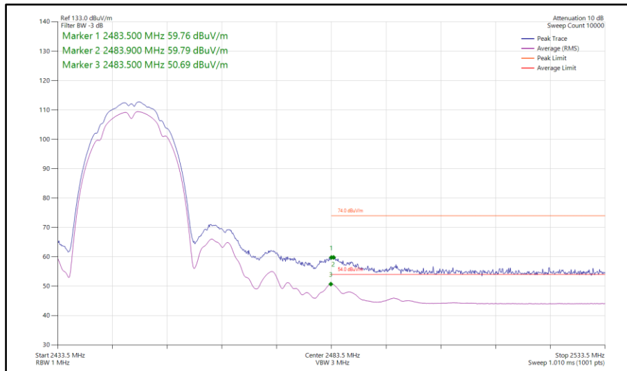
Figure 88 - 802.11b, SISO, Core 1 - 2447 MHz Band Edge Frequency 2483.5 MHz
