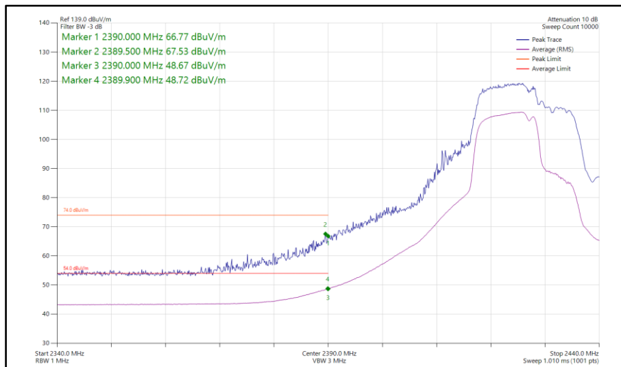
Figure 87 - 802.11be EHT20, RU106+26-82, SISO, Core 1 - 2427 MHz Band Edge Frequency 2390 MHz
