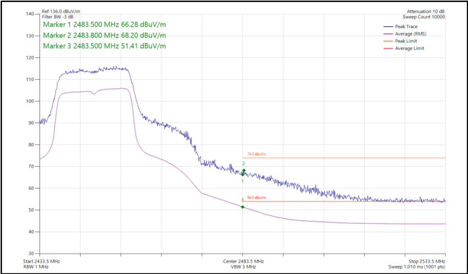
Figure 104 - 802.11n HT20, SISO, Core 1 - 2447 MHz Band Edge Frequency 2483.5 MHz
