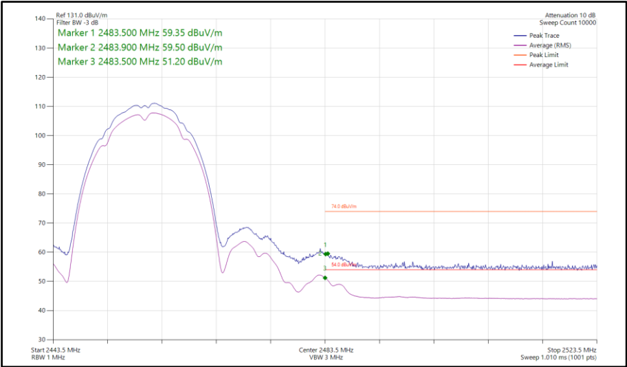
Figure 90 - 802.11b, SISO, Core 1 - 2457 MHz Band Edge Frequency 2483.5 MHz
