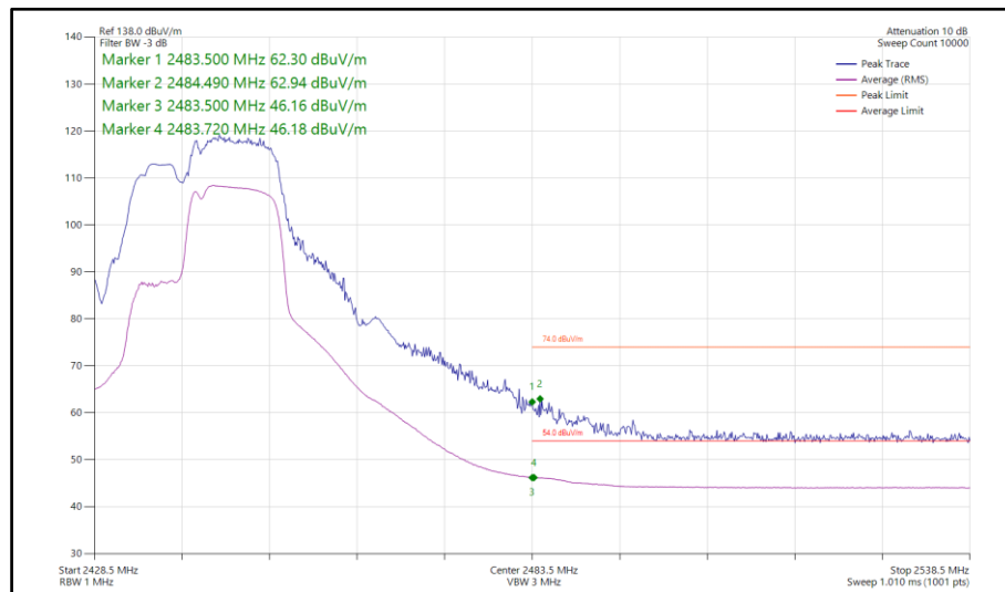
Figure 125 - 802.11be EHT20, RU106+26-83, SISO, Core 1 - 2442 MHz Band Edge Frequency 2483.5 MHz
