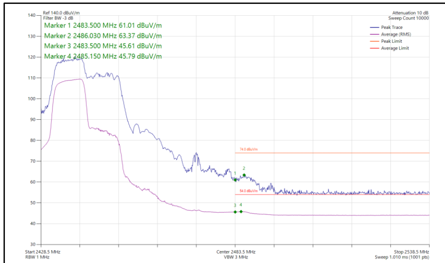
Figure 112 - 802.11ax HE20, RU106-53, SISO, Core 1 - 2442 MHz Band Edge Frequency 2483.5 MHz
