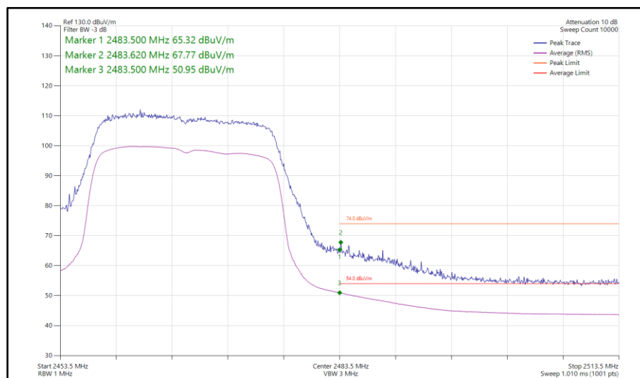
Figure 121 - 802.11ax HE20, SU, SISO, Core 1 - 2467 MHz Band Edge Frequency 2483.5 MHz
