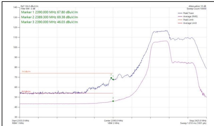
Figure 84 - 802.11be EHT20, RU52+26-70, SISO, Core 1 - 2412 MHz Band Edge Frequency 2390 MHz
