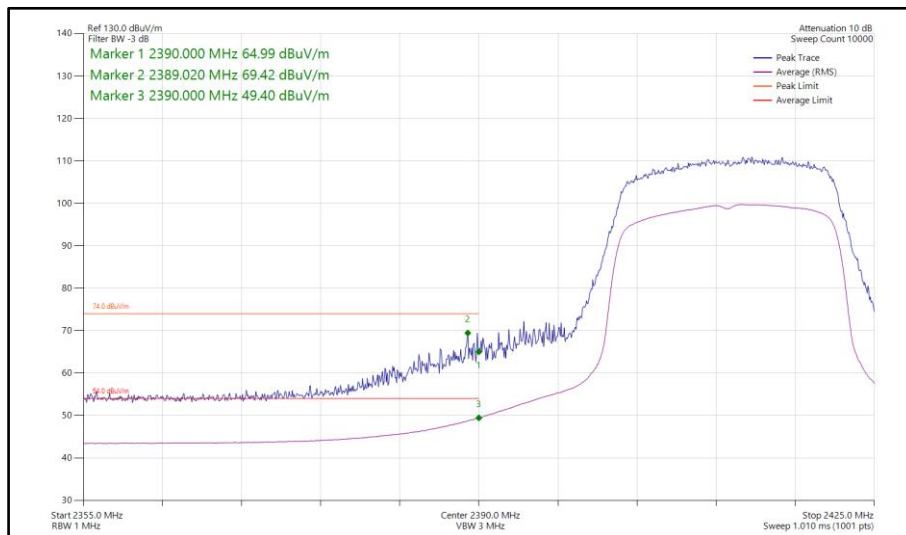
Figure 75 - 802.11ax HE20, SU, SISO, Core 1 - 2412 MHz Band Edge Frequency 2390 MHz
