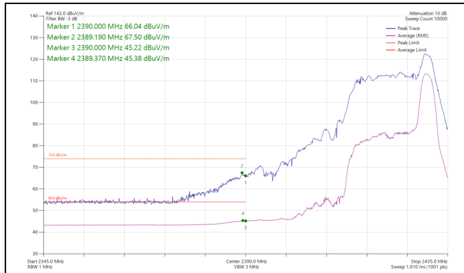
Figure 80 - 802.11ax HE20, RU26-8, SISO, Core 1 - 2422 MHz Band Edge Frequency 2390 MHz
