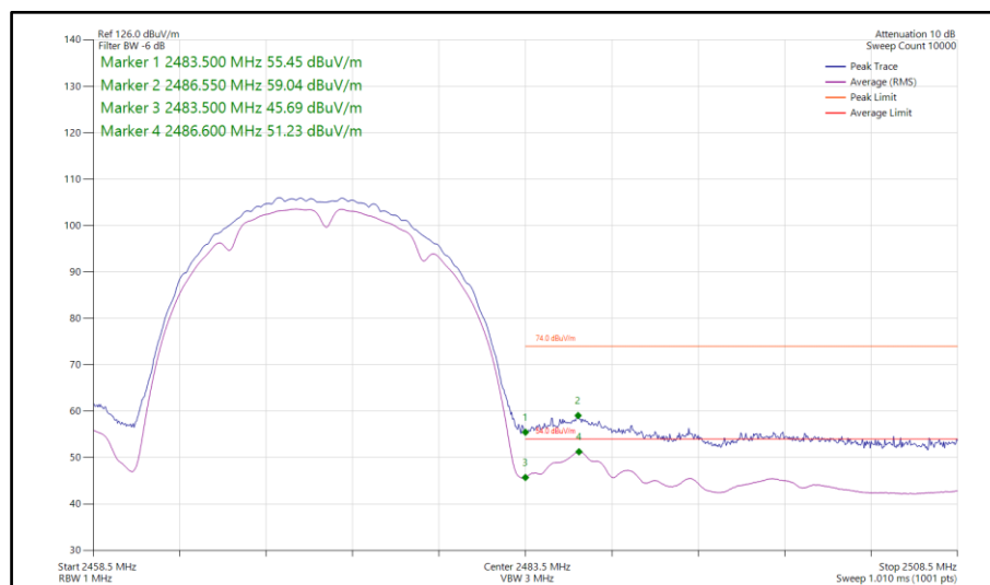
Figure 93 - 802.11b, SISO, Core 1 - 2472 MHz Band Edge Frequency 2483.5 MHz
