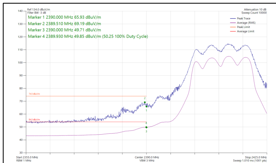
Figure 132 - 802.11g, CDD, Core 0-1 - 2412 MHz Band Edge Frequency 2390 MHz
