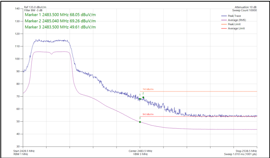
Figure 103 - 802.11n HT20, SISO, Core 1 - 2442 MHz Band Edge Frequency 2483.5 MHz
