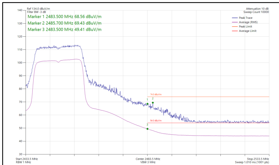
Figure 113 - 802.11ax HE20, SU, SISO, Core 1 - 2447 MHz Band Edge Frequency 2483.5 MHz
