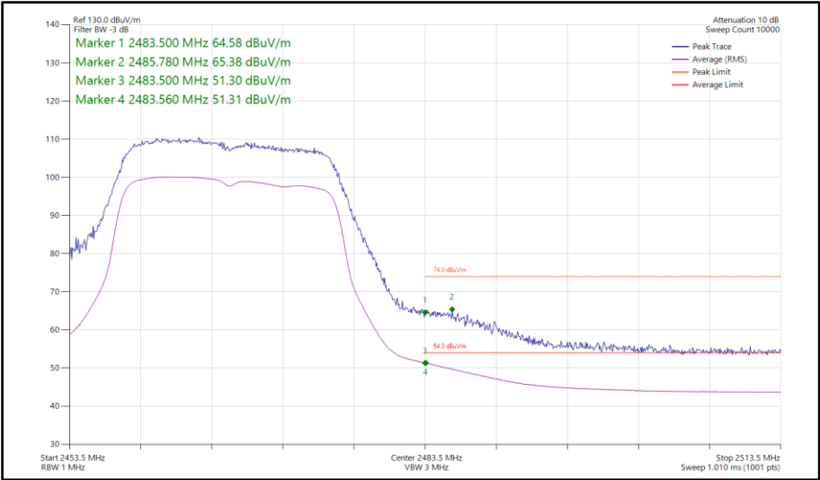
Figure 108 - 802.11n HT20, SISO, Core 1 - 2467 MHz Band Edge Frequency 2483.5 MHz
