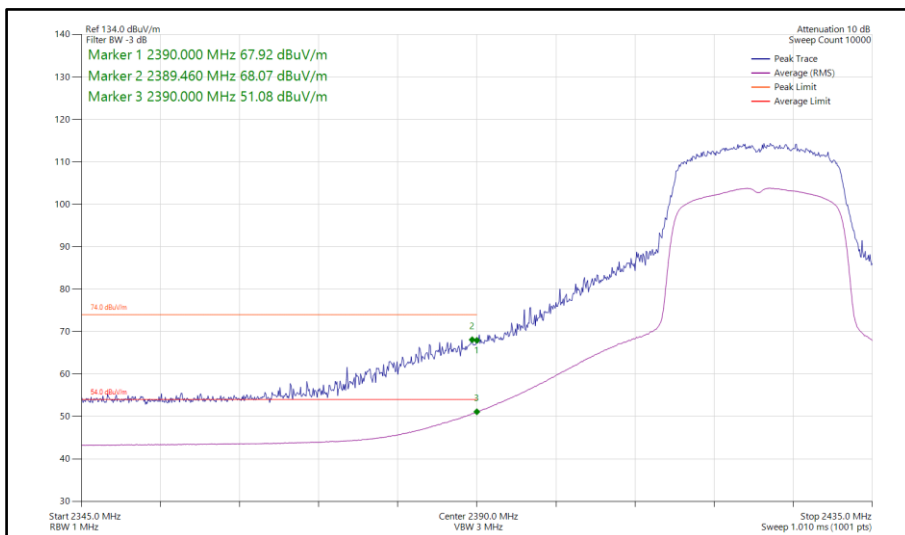
Figure 79 - 802.11ax HE20, SU, SISO, Core 1 - 2422 MHz Band Edge Frequency 2390 MHz
