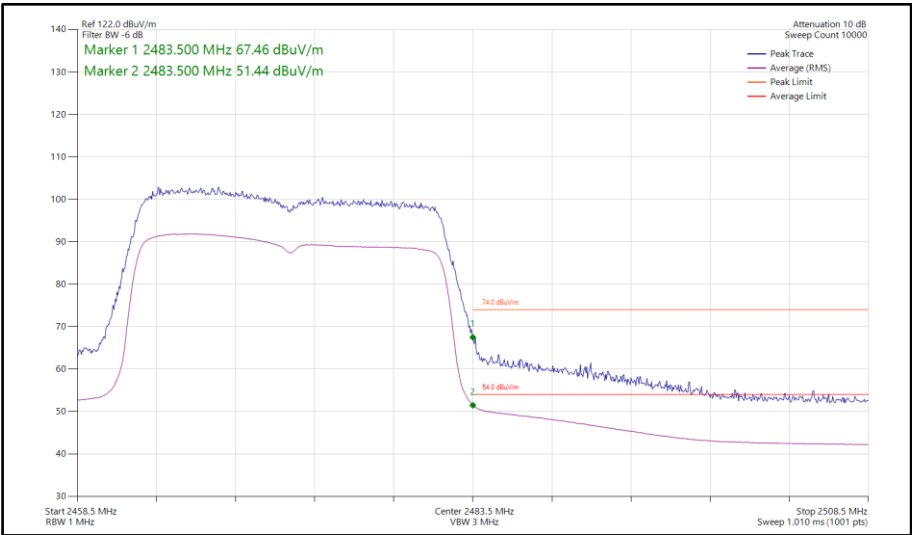
Figure 123 - 802.11ax HE20, SU, SISO, Core 1 - 2472 MHz Band Edge Frequency 2483.5 MHz
