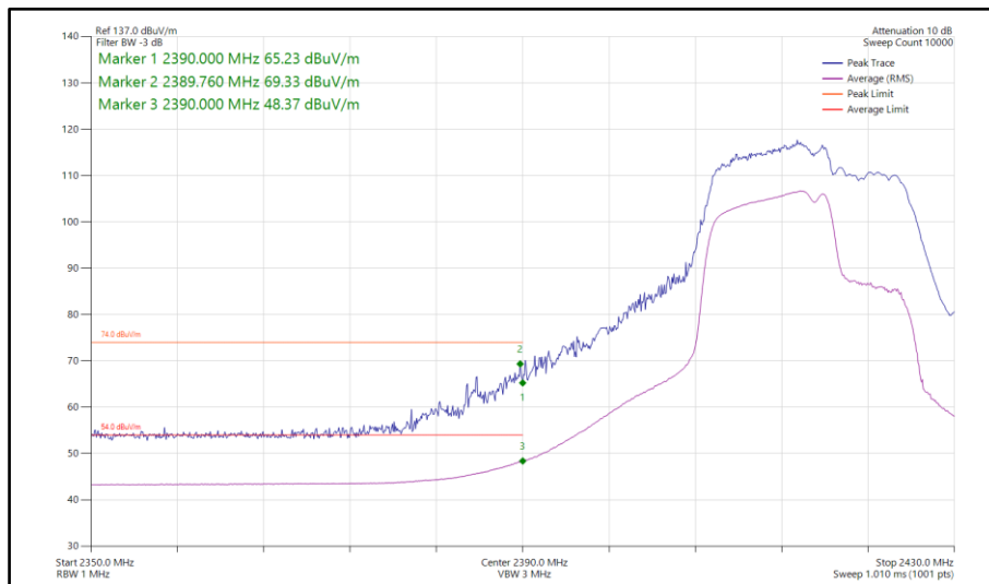
Figure 85 - 802.11be EHT20, RU106+26-82, SISO, Core 1 - 2417 MHz Band Edge Frequency 2390 MHz
