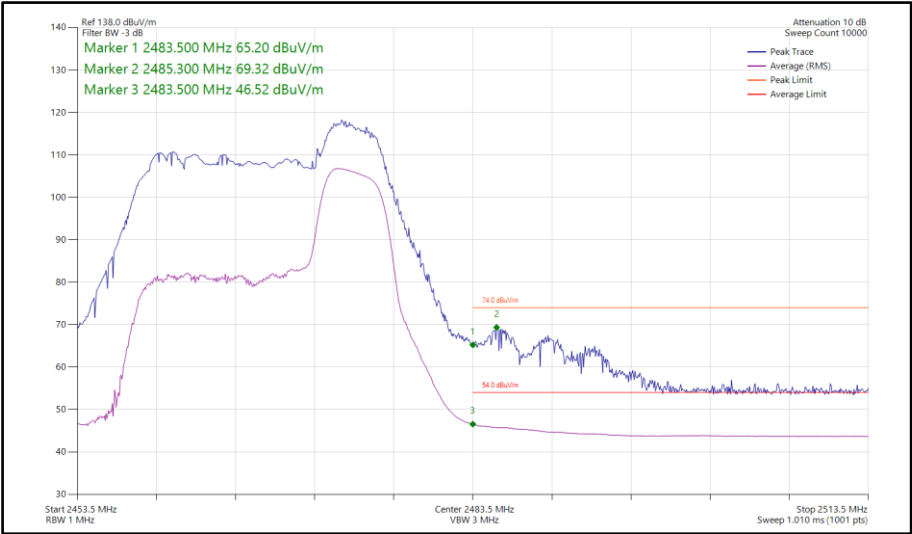
Figure 122 - 802.11ax HE20, RU52-40, SISO, Core 1 - 2467 MHz Band Edge Frequency 2483.5 MHz
