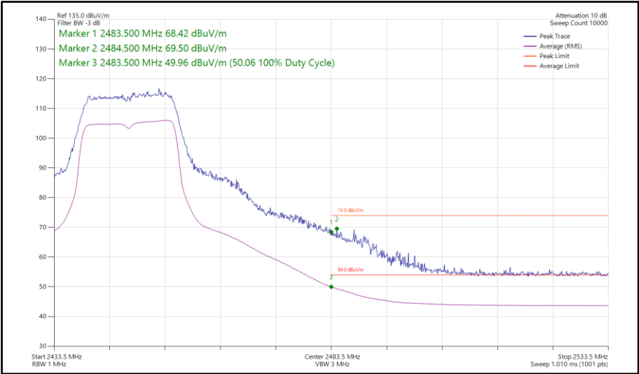
Figure 96 - 802.11g, SISO, Core 1 - 2447 MHz Band Edge Frequency 2483.5 MHz
