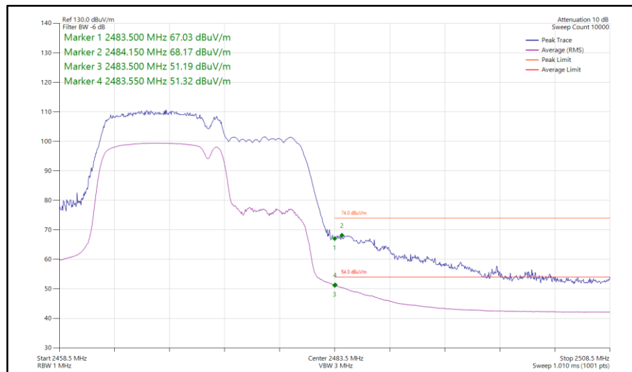
Figure 131 - 802.11be EHT20, RU106+26-82, SISO, Core 1 - 2472 MHz Band Edge Frequency 2483.5 MHz
