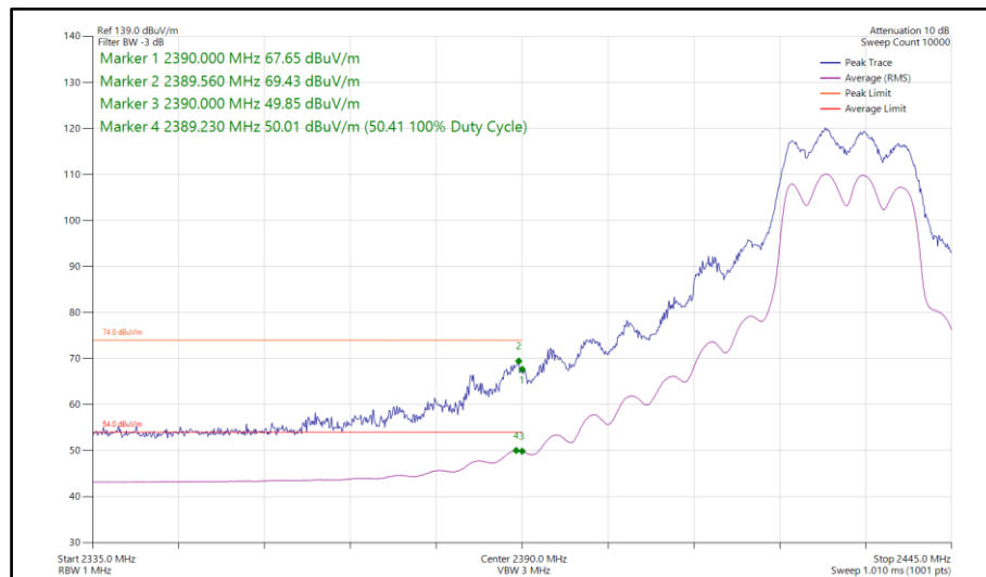
Figure 136 - 802.11g, CDD, Core 0-1 - 2432 MHz Band Edge Frequency 2390 MHz
