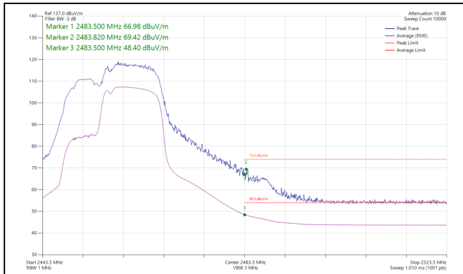
Figure 128 - 802.11be EHT20, RU106+26-83, SISO, Core 1 - 2457 MHz Band Edge Frequency 2483.5 MHz
