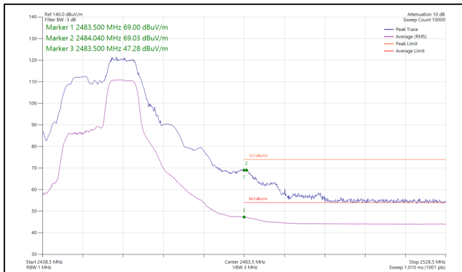
Figure 127 - 802.11be EHT20, RU52+26-72, SISO, Core 1 - 2452 MHz Band Edge Frequency 2483.5 MHz
