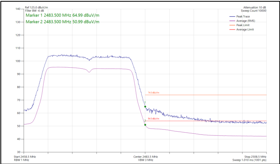
Figure 109 - 802.11n HT20, SISO, Core 1 - 2472 MHz Band Edge Frequency 2483.5 MHz
