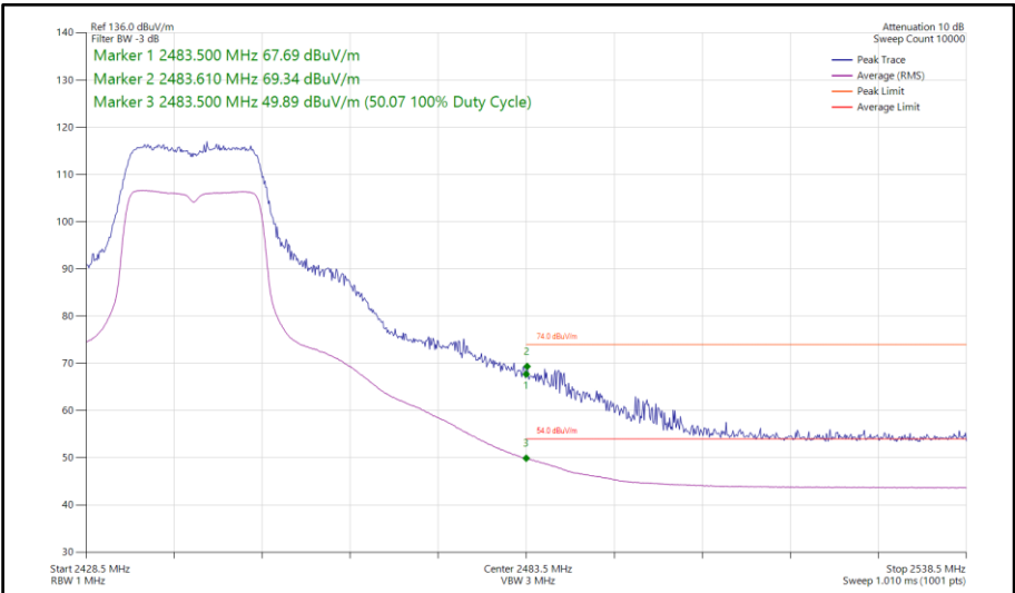
Figure 95 - 802.11g, SISO, Core 1 - 2442 MHz Band Edge Frequency 2483.5 MHz
