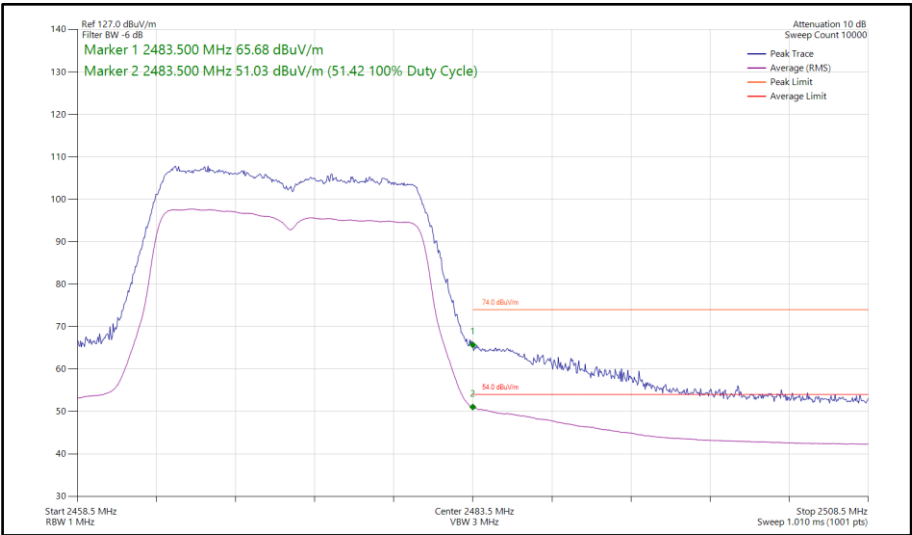
Figure 101 - 802.11g, SISO, Core 1 - 2472 MHz Band Edge Frequency 2483.5 MHz
