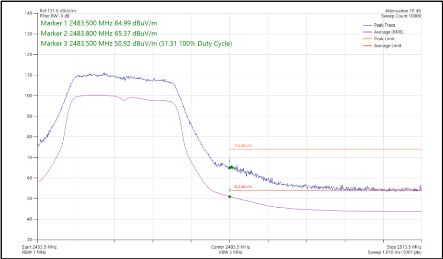
Figure 100 - 802.11g, SISO, Core 1 - 2467 MHz Band Edge Frequency 2483.5 MHz
