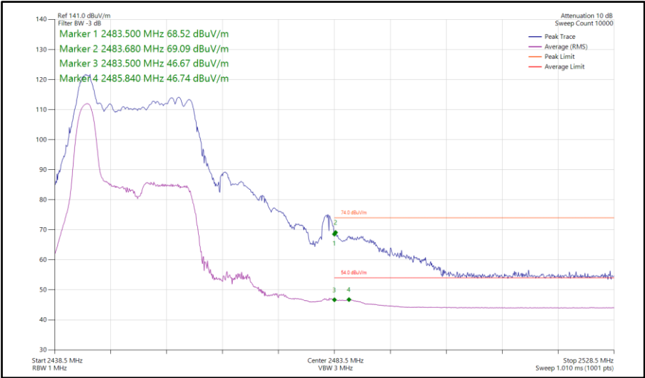
Figure 116 - 802.11ax HE20, RU26-0, SISO, Core 1 - 2452 MHz Band Edge Frequency 2483.5 MHz
