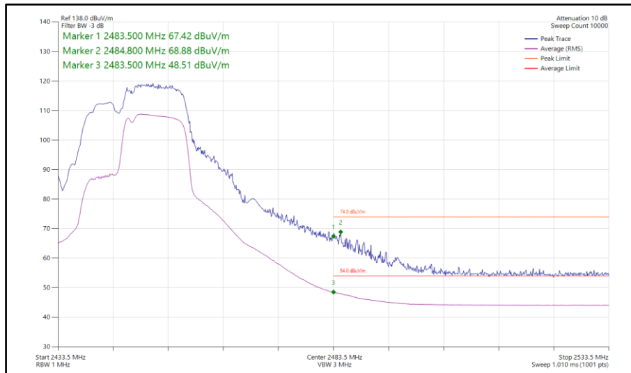
Figure 126 - 802.11be EHT20, RU106+26-83, SISO, Core 1 - 2447 MHz Band Edge Frequency 2483.5 MHz
