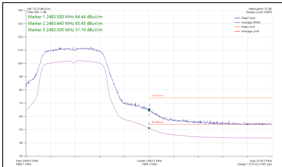
Figure 107 - 802.11n HT20, SISO, Core 1 - 2462 MHz Band Edge Frequency 2483.5 MHz
