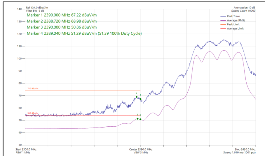
Figure 133 - 802.11g, CDD, Core 0-1 - 2417 MHz Band Edge Frequency 2390 MHz
