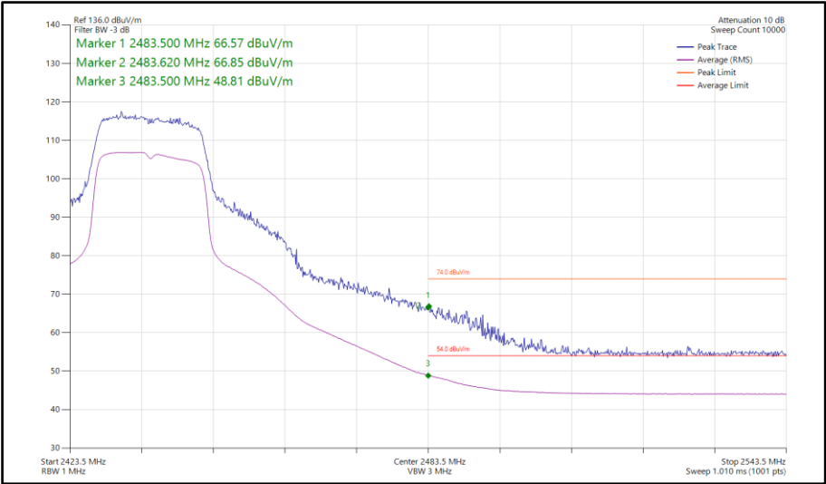
Figure 102 - 802.11n HT20, SISO, Core 1 - 2437 MHz Band Edge Frequency 2483.5 MHz
