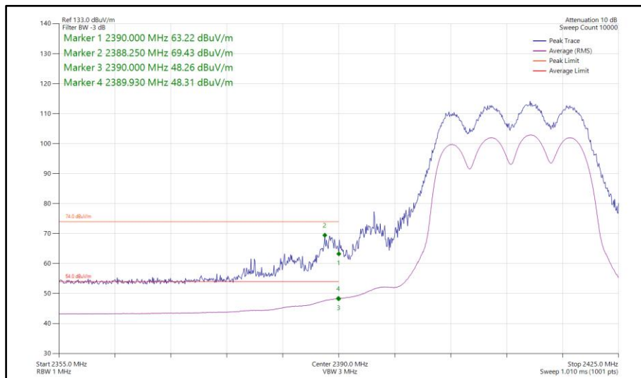
Figure 142 - 802.11ax HE20, SU, CDD, Core 0-1 - 2412 MHz Band Edge Frequency 2390 MHz
