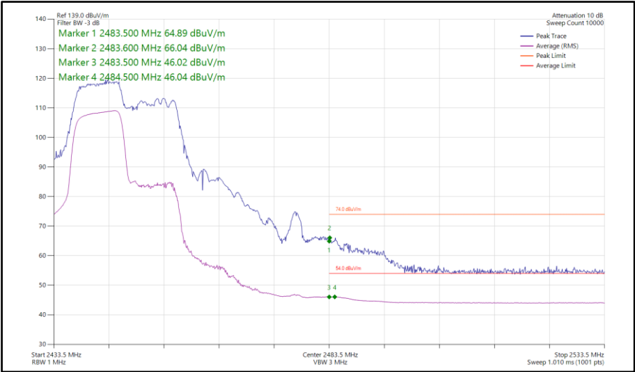
Figure 114 - 802.11ax HE20, RU106-53, SISO, Core 1 - 2447 MHz Band Edge Frequency 2483.5 MHz
