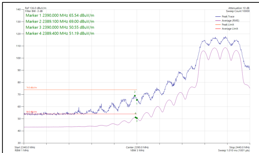
Figure 140 - 802.11n HT20, CDD, Core 0-1 - 2427 MHz Band Edge Frequency 2390 MHz
