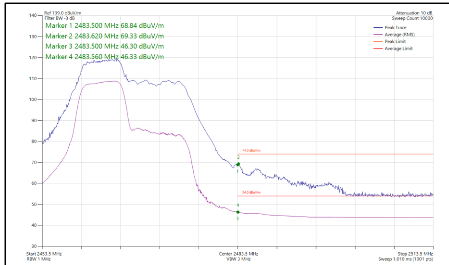
Figure 130 - 802.11be EHT20, RU52+26-70, SISO, Core 1 - 2467 MHz Band Edge Frequency 2483.5 MHz
