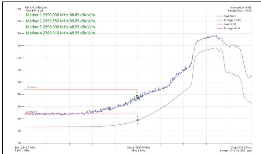
Figure 86 - 802.11be EHT20, RU106+26-82, SISO, Core 1 - 2422 MHz Band Edge Frequency 2390 MHz
