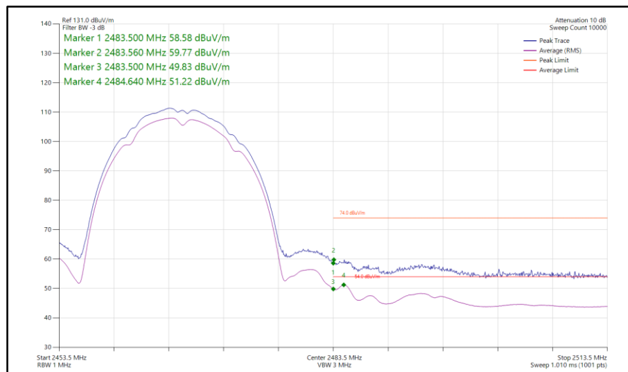
Figure 92 - 802.11b, SISO, Core 1 - 2467 MHz Band Edge Frequency 2483.5 MHz
