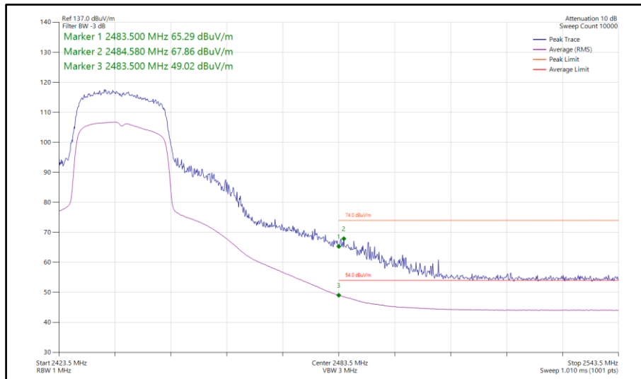
Figure 110 - 802.11ax HE20, SU, SISO, Core 1 - 2437 MHz Band Edge Frequency 2483.5 MHz
