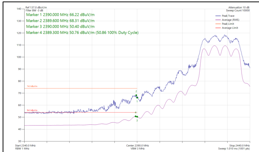
Figure 135 - 802.11g, CDD, Core 0-1 - 2427 MHz Band Edge Frequency 2390 MHz
