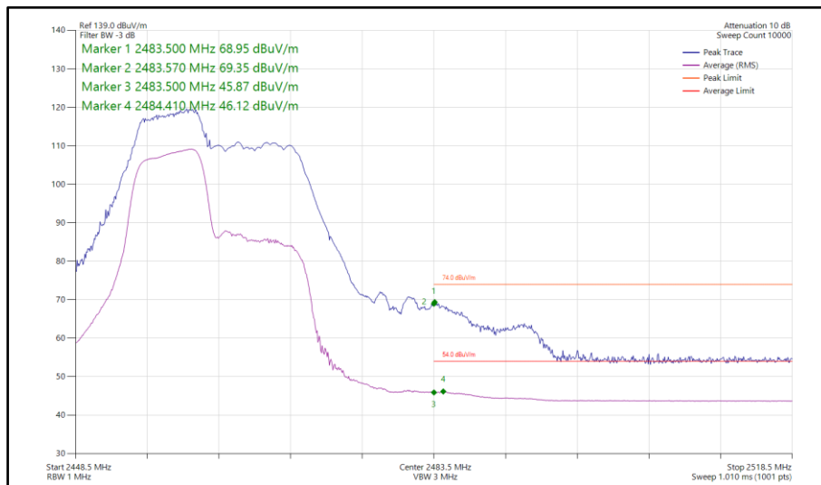
Figure 129 - 802.11be EHT20, RU52+26-70, SISO, Core 1 - 2462 MHz Band Edge Frequency 2483.5 MHz
