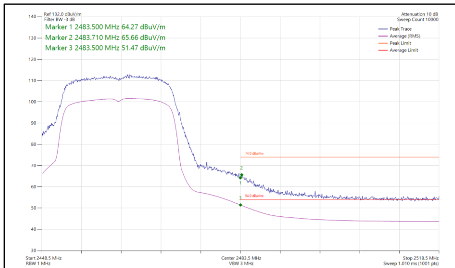
Figure 119 - 802.11ax HE20, SU, SISO, Core 1 - 2462 MHz Band Edge Frequency 2483.5 MHz
