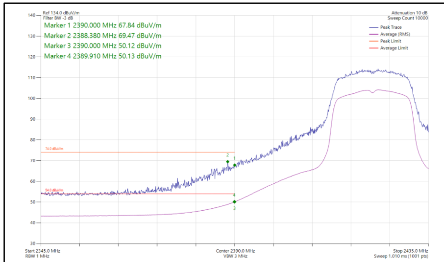
Figure 72 - 802.11n HT20, SISO, Core 1 - 2422 MHz Band Edge Frequency 2390 MHz
