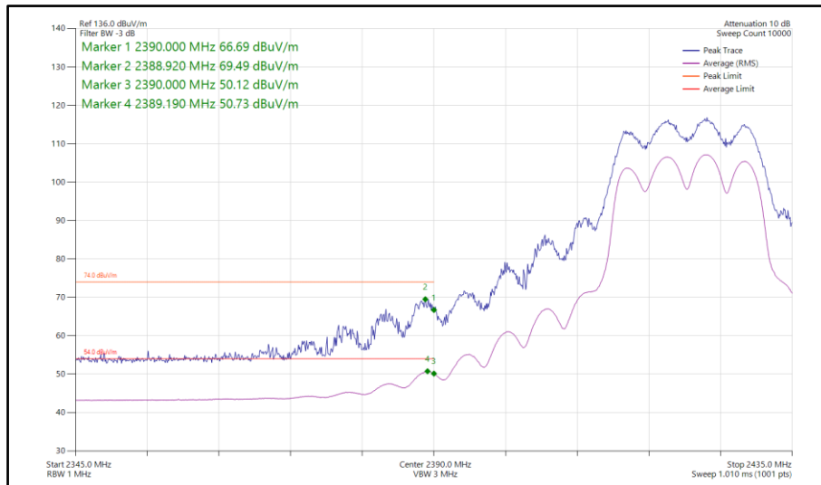
Figure 139 - 802.11n HT20, CDD, Core 0-1 - 2422 MHz Band Edge Frequency 2390 MHz
