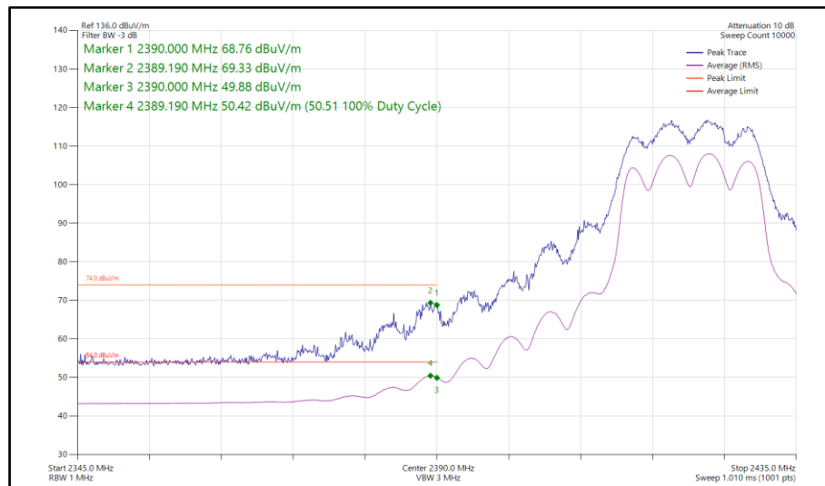
Figure 134 - 802.11g, CDD, Core 0-1 - 2422 MHz Band Edge Frequency 2390 MHz
