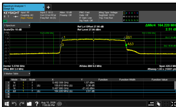
Figure 466 - 802.11ax HE160 SU Minimum 26 dB EBW
