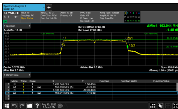
Figure 458 - 802.11ac VHT160 Minimum 26 dB EBW
