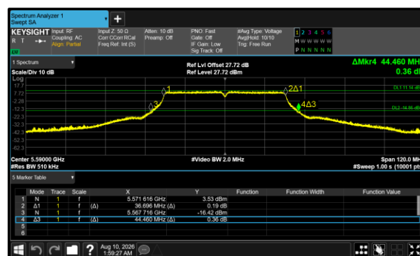
Figure 503 - 802.11n HT40 Maximum 26 dB EBW
