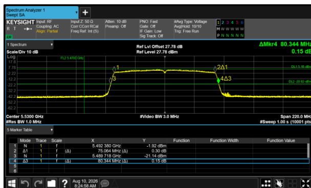
Figure 504 - 802.11ac VHT80 Minimum 26 dB EBW
