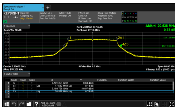
Figure 500 - 802.11n HT20 Minimum 26 dB EBW
