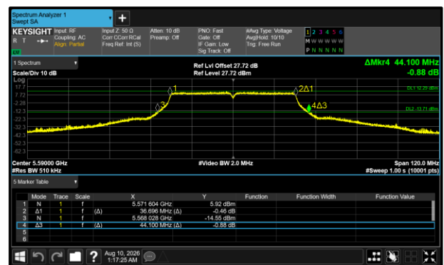
Figure 455 - 802.11n HT40 Maximum 26 dB EBW
