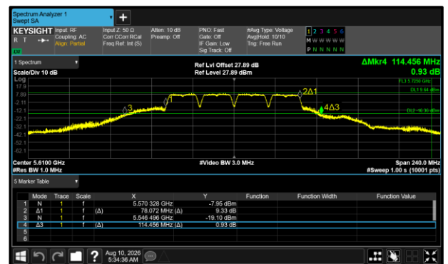
Figure 473 - 802.11a80 Maximum 26 dB EBW
