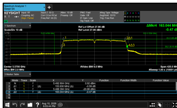
Figure 507 - 802.11ac VHT160 Maximum 26 dB EBW
