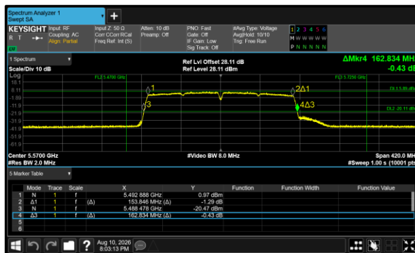
Figure 482 - 802.11ac VHT160 Minimum 99% OBW
