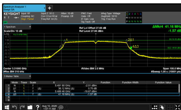
Figure 502 - 802.11n HT40 Minimum 26 dB EBW
