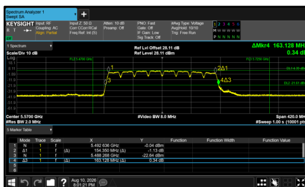
Figure 498 - 802.11a160 Minimum 99% OBW
