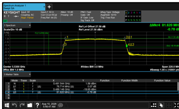
Figure 464 - 802.11ax HE80 SU Minimum 26 dB EBW
