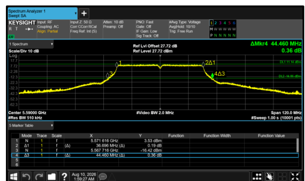
Figure 479 - 802.11n HT40 Maximum 99% OBW
