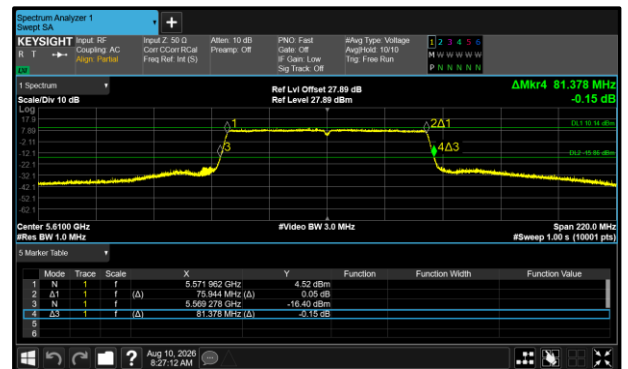
Figure 481 - 802.11ac VHT80 Maximum 99% OBW
