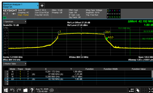
Figure 462 - 802.11ax HE40 SU Minimum 26 dB EBW
