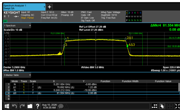
Figure 512 - 802.11ax HE80 SU Minimum 26 dB EBW
