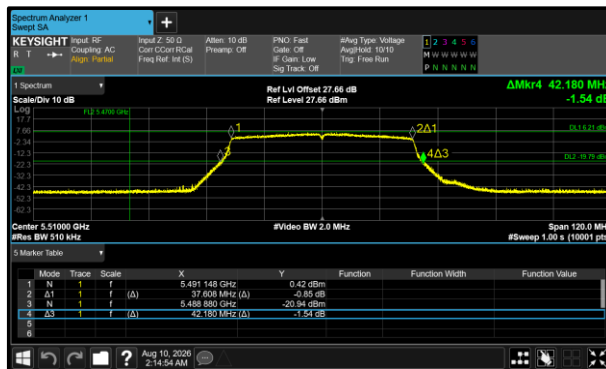
Figure 510 - 802.11ax HE40 SU Minimum 26 dB EBW
