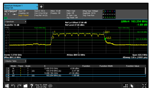
Figure 499 - 802.11a160 Maximum 99% OBW
