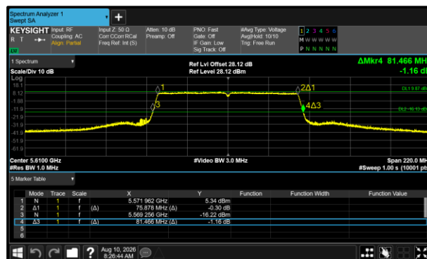
Figure 505 - 802.11ac VHT80 Maximum 26 dB EBW
