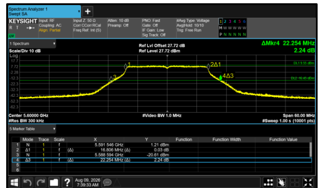
Figure 493 - 802.11a20 Maximum 99% OBW
