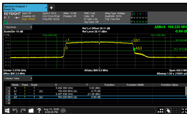
Figure 490 - 802.11ax HE160 SU Minimum 99% OBW
