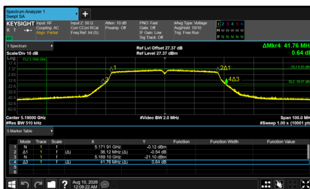
Figure 478 - 802.11n HT40 Minimum 99% OBW
