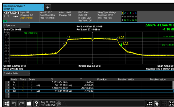
Figure 454 - 802.11n HT40 Minimum 26 dB EBW
