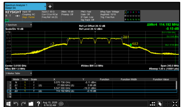
Figure 521 - 802.11a80 Maximum 26 dB EBW
