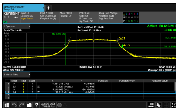
Figure 476 - 802.11n HT20 Minimum 99% OBW
