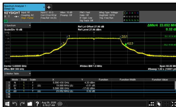
Figure 509 - 802.11ax HE20 SU Maximum 26 dB EBW
