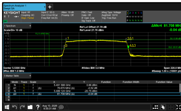
Figure 488 - 802.11ax HE80 SU Minimum 99% OBW
