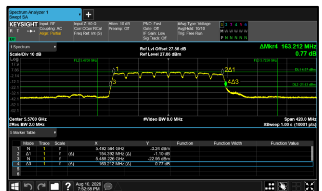
Figure 475 - 802.11a160 Maximum 26 dB EBW
