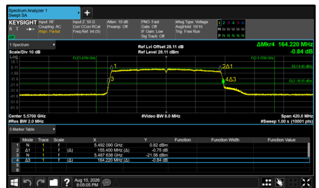
Figure 515 - 802.11ax HE160 SU Maximum 26 dB EBW
