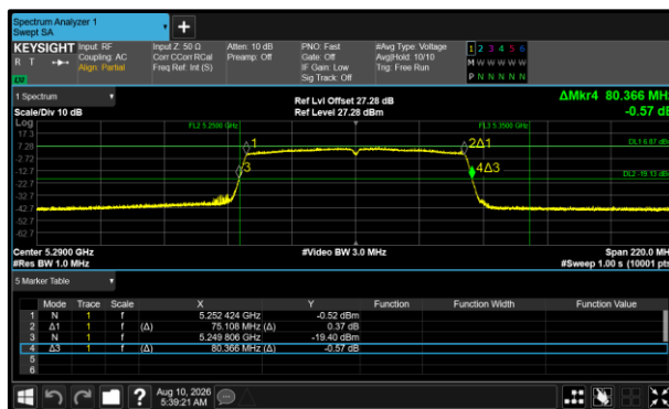
Figure 456 - 802.11ac VHT80 Minimum 26 dB EBW
