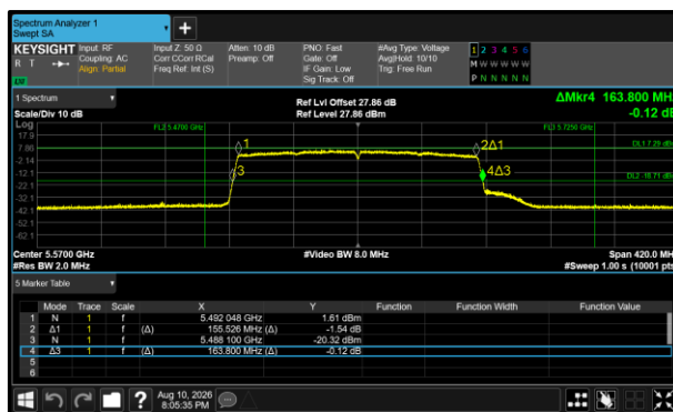
Figure 514 - 802.11ax HE160 SU Minimum 26 dB EBW
