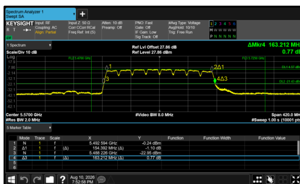
Figure 474 - 802.11a160 Minimum 26 dB EBW
