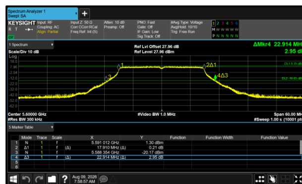
Figure 501 - 802.11n HT20 Maximum 26 dB EBW
