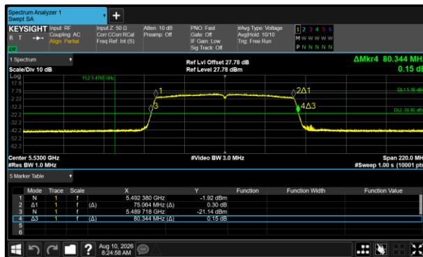
Figure 480 - 802.11ac VHT80 Minimum 99% OBW
