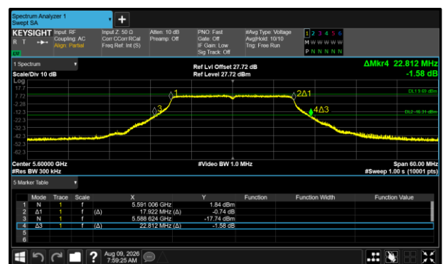
Figure 477 - 802.11n HT20 Maximum 99% OBW
