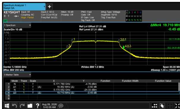
Figure 492 - 802.11a20 Minimum 99% OBW
