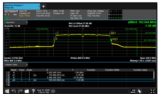
Figure 459 - 802.11ac VHT160 Maximum 26 dB EBW
