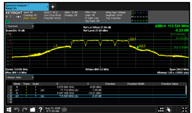
Figure 497 - 802.11a80 Maximum 99% OBW
