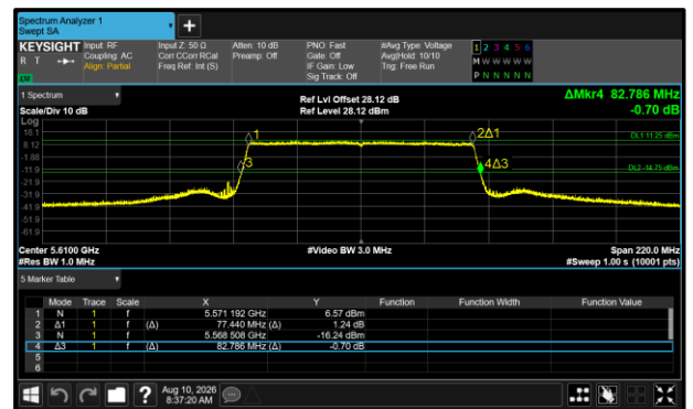
Figure 513 - 802.11ax HE80 SU Maximum 26 dB EBW
