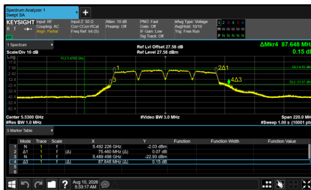
Figure 472 - 802.11a80 Minimum 26 dB EBW
