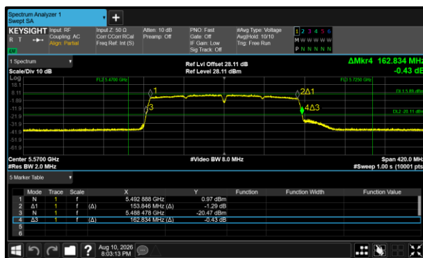
Figure 506 - 802.11ac VHT160 Minimum 26 dB EBW
