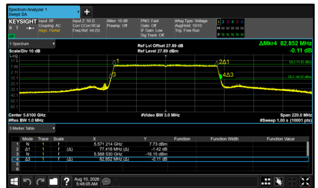
Figure 465 - 802.11ax HE80 SU Maximum 26 dB EBW
