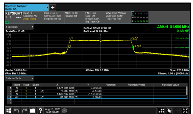
Figure 457 - 802.11ac VHT80 Maximum 26 dB EBW
