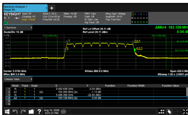
Figure 522 - 802.11a160 Minimum 26 dB EBW
