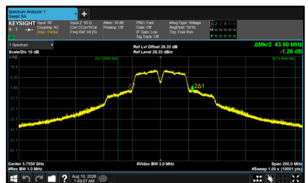
Figure 495 - 802.11a40 Maximum 99% OBW
