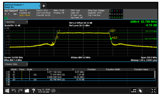
Figure 489 - 802.11ax HE80 SU Maximum 99% OBW
