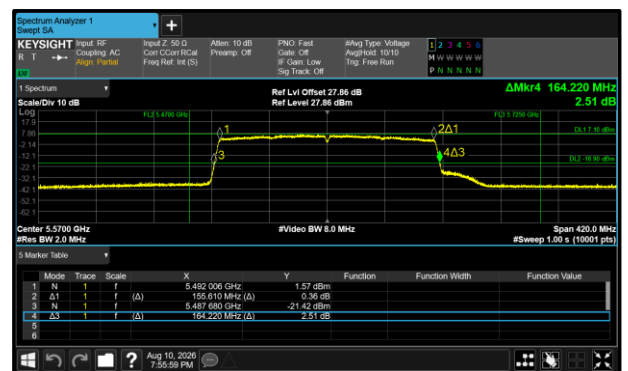
Figure 467 - 802.11ax HE160 SU Maximum 26 dB EBW
