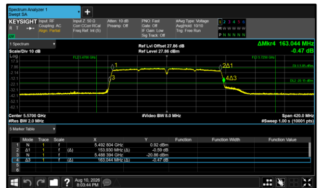
Figure 483 - 802.11ac VHT160 Maximum 99% OBW
