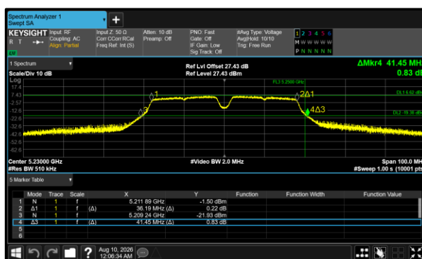
Figure 494 - 802.11a40 Minimum 99% OBW
