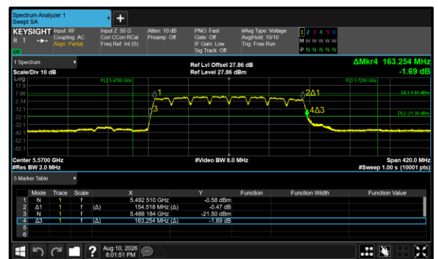
Figure 523 - 802.11a160 Maximum 26 dB EBW
