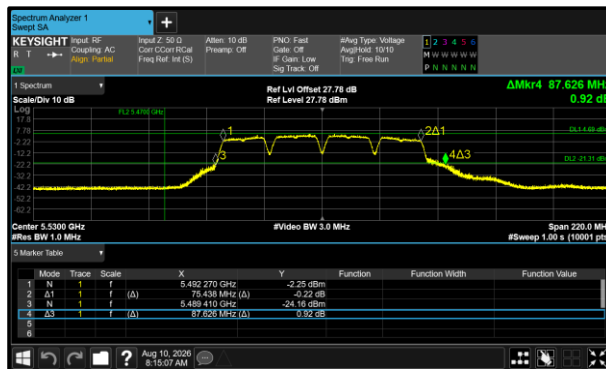
Figure 496 - 802.11a80 Minimum 99% OBW
