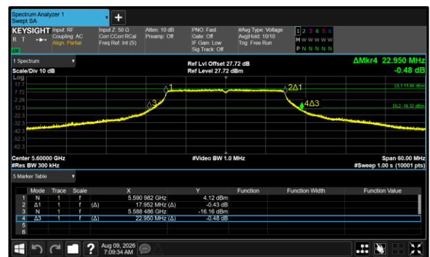
Figure 453 - 802.11n HT20 Maximum 26 dB EBW
