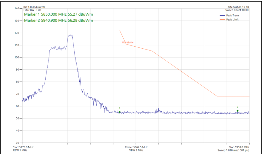
Figure 796 - 802.11ax HE40, RU52-44, SISO, Core 0 - 5795 MHz Band Edge Frequency 5850 MHz
