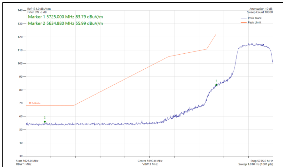
Figure 755 - 802.11ac VHT20, TxBF, Core 0-1 - 5745 MHz Band Edge Frequency 5725 MHz
