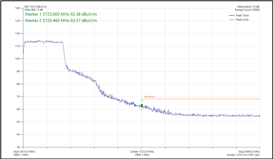
Figure 819 - 802.11ax HE40, SU, SISO, Core 1 - 5630 MHz Band Edge Frequency 5725 MHz
