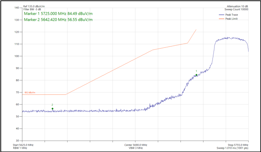
Figure 756 - 802.11ax HE20, SU, TxBF, Core 0-1 - 5745 MHz Band Edge Frequency 5725 MHz
