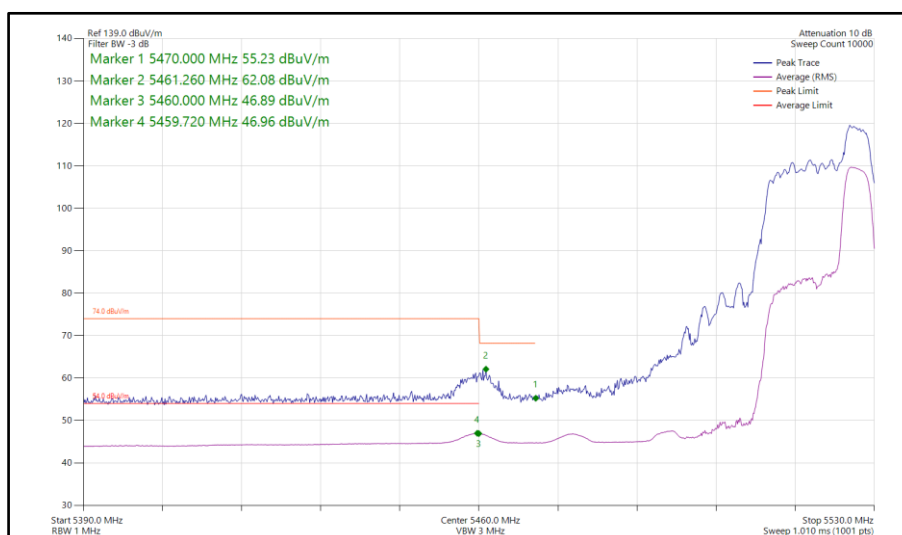
Figure 806 - 802.11ax HE40, RU52-44, SISO, Core 1 - 5510 MHz Band Edge Frequency 5470 MHz
