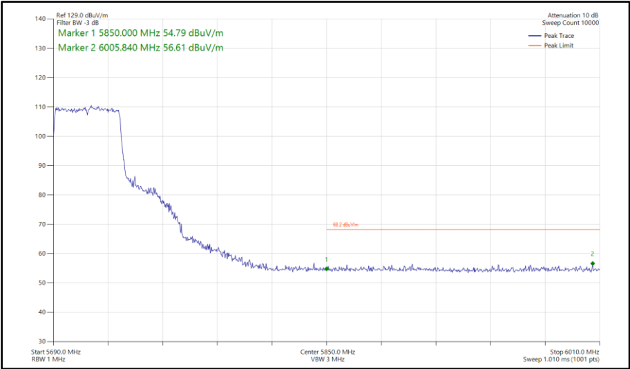
Figure 793 - 802.11ax HE40, SU, SISO, Core 0 - 5710 MHz Band Edge Frequency 5850 MHz
