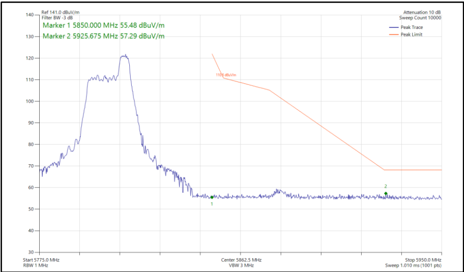
Figure 830 - 802.11ax HE40, RU52-44, SISO, Core 1 - 5795 MHz Band Edge Frequency 5850 MHz
