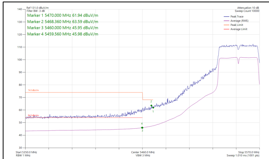
Figure 803 - 802.11n HT40, SISO, Core 1 - 5550 MHz Band Edge Frequency 5470 MHz
