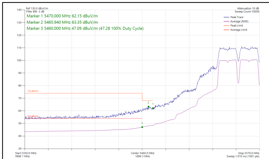
Figure 766 - 802.11a a40, SISO, Core 0 - 5550 MHz Band Edge Frequency 5470 MHz
