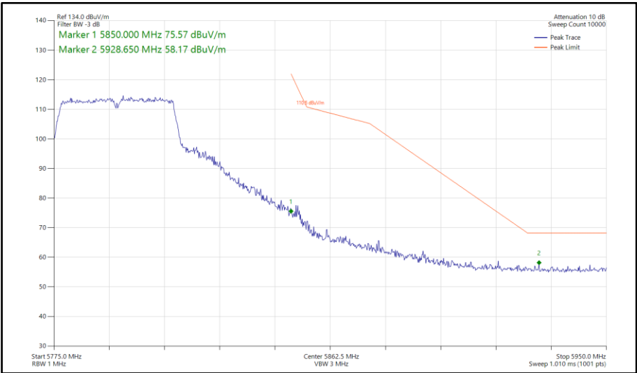
Figure 826 - 802.11n HT40, SISO, Core 1 - 5795 MHz Band Edge Frequency 5850 MHz
