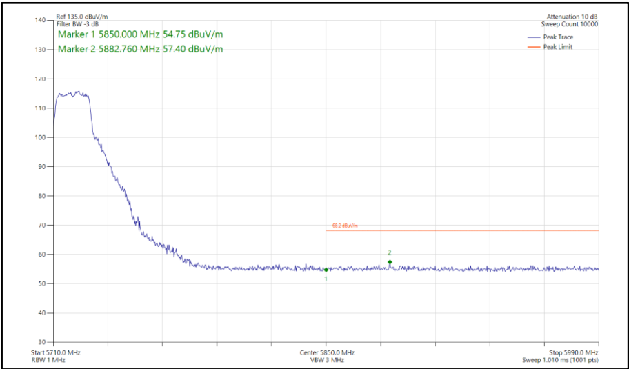
Figure 761 - 802.11ac VHT20, TxBF, Core 0-1 - 5720 MHz Band Edge Frequency 5850 MHz
