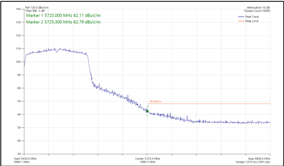
Figure 786 - 802.11ax HE40, SU, SISO, Core 0 - 5670 MHz Band Edge Frequency 5725 MHz
