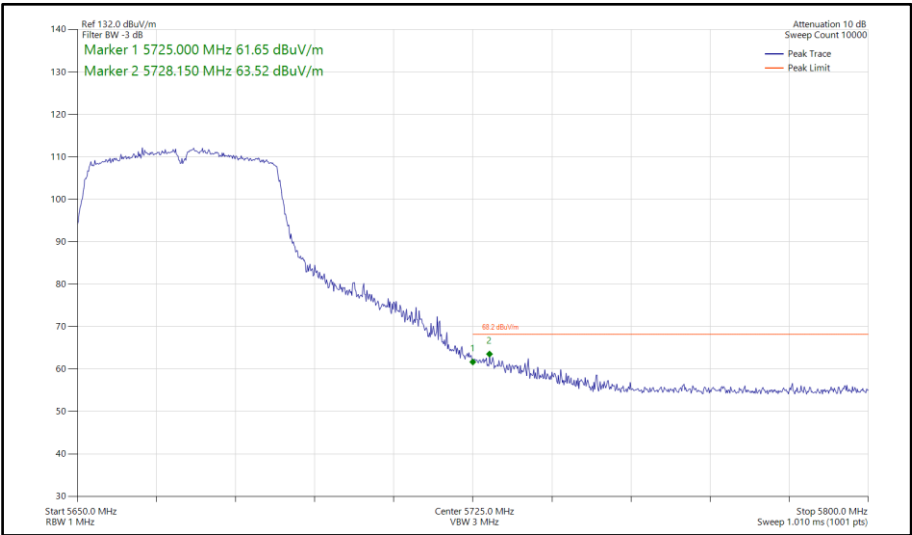
Figure 818 - 802.11n HT40, SISO, Core 1 - 5670 MHz Band Edge Frequency 5725 MHz
