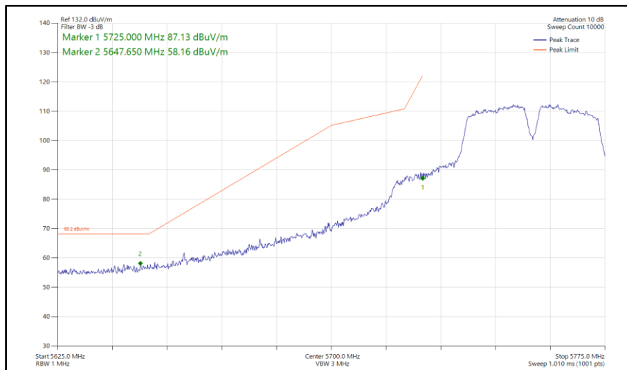
Figure 776 - 802.11a a40, SISO, Core 0 - 5755 MHz Band Edge Frequency 5725 MHz
