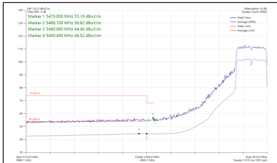
Figure 804 - 802.11n HT40, SISO, Core 1 - 5590 MHz Band Edge Frequency 5470 MHz
