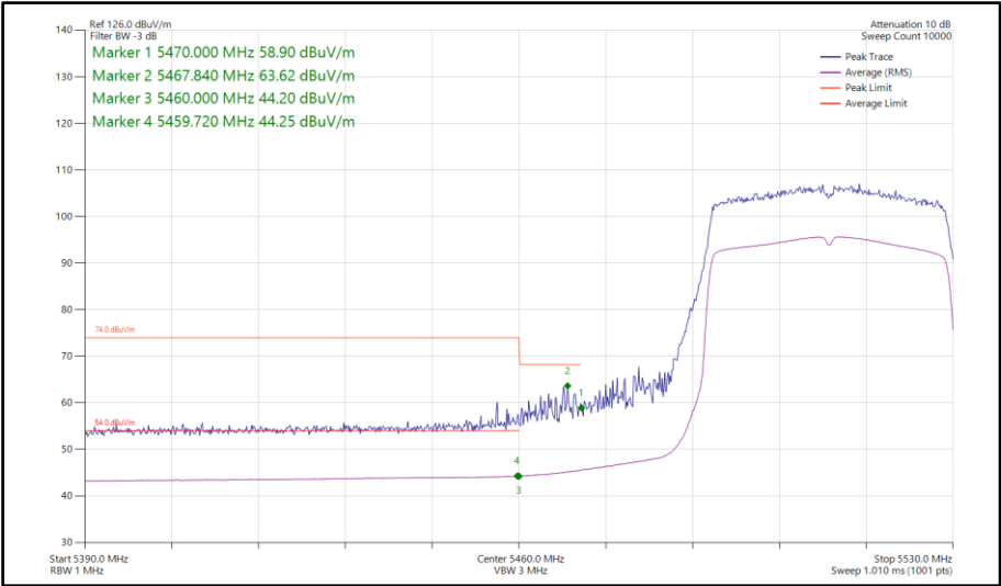
Figure 771 - 802.11ax HE40, SU, SISO, Core 0 - 5510 MHz Band Edge Frequency 5470 MHz
