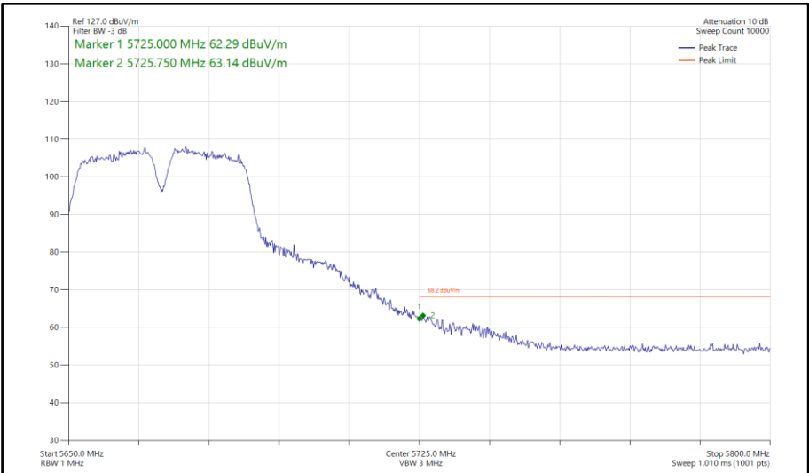
Figure 782 - 802.11a a40, SISO, Core 0 - 5670 MHz Band Edge Frequency 5725 MHz
