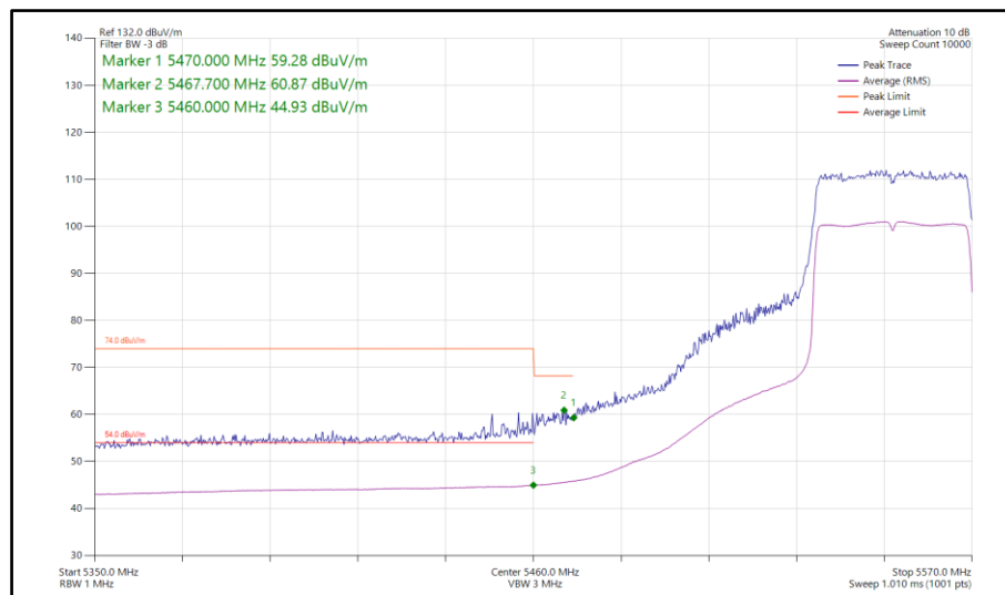
Figure 773 - 802.11ax HE40, SU, SISO, Core 0 - 5550 MHz Band Edge Frequency 5470 MHz
