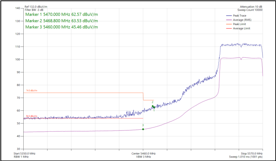
Figure 807 - 802.11ax HE40, SU, SISO, Core 1 - 5550 MHz Band Edge Frequency 5470 MHz
