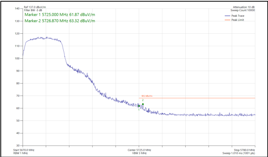
Figure 757 - 802.11ac VHT20, TxBF, Core 0-1 - 5680 MHz Band Edge Frequency 5725 MHz
