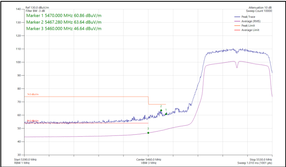
Figure 768 - 802.11n HT40, SISO, Core 0 - 5510 MHz Band Edge Frequency 5470 MHz
