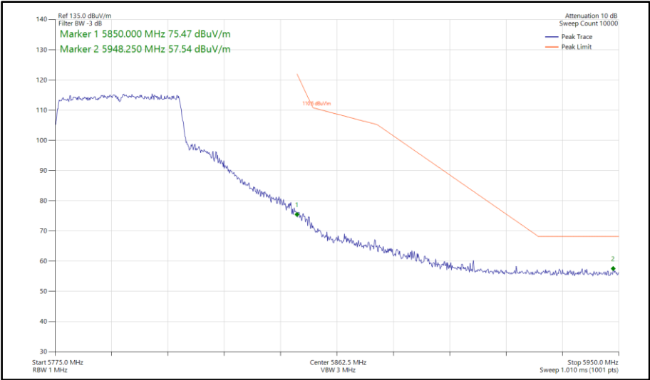
Figure 829 - 802.11ax HE40, SU, SISO, Core 1 - 5795 MHz Band Edge Frequency 5850 MHz
