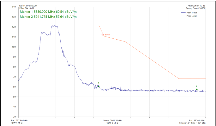
Figure 832 - 802.11be EHT40, RU52+26-75, SISO, Core 1 - 5795 MHz Band Edge Frequency 5850 MHz
