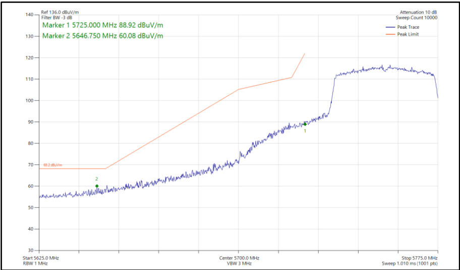
Figure 812 - 802.11ax HE40, SU, SISO, Core 1 - 5755 MHz Band Edge Frequency 5725 MHz
