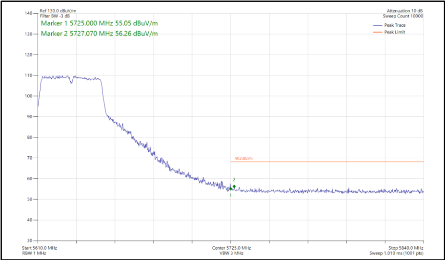
Figure 783 - 802.11n HT40, SISO, Core 0 - 5630 MHz Band Edge Frequency 5725 MHz
