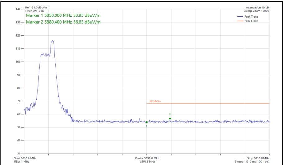
Figure 794 - 802.11ax HE40, RU52-44, SISO, Core 0 - 5710 MHz Band Edge Frequency 5850 MHz
