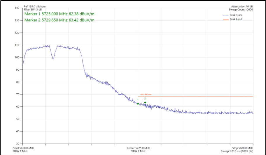
Figure 816 - 802.11a a40, SISO, Core 1 - 5670 MHz Band Edge Frequency 5725 MHz
