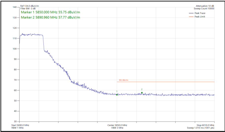
Figure 827 - 802.11ax HE40, SU, SISO, Core 1 - 5710 MHz Band Edge Frequency 5850 MHz
