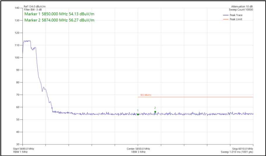
Figure 797 - 802.11be EHT40, RU106+26-82, SISO, Core 0 - 5710 MHz Band Edge Frequency 5850 MHz
