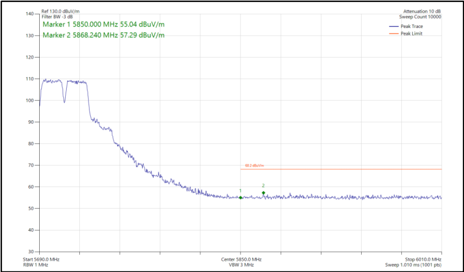
Figure 789 - 802.11a a40, SISO, Core 0 - 5710 MHz Band Edge Frequency 5850 MHz
