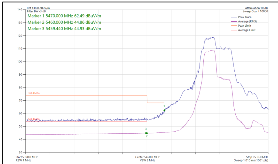
Figure 775 - 802.11be EHT40, RU52+26-70, SISO, Core 0 - 5510 MHz Band Edge Frequency 5470 MHz
