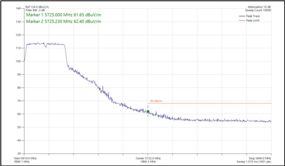
Figure 817 - 802.11n HT40, SISO, Core 1 - 5630 MHz Band Edge Frequency 5725 MHz
