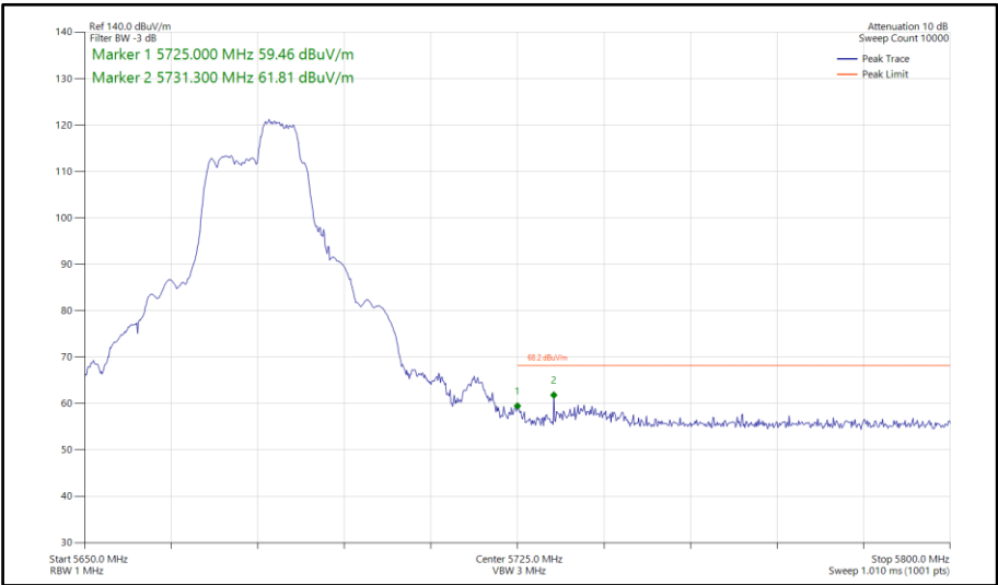
Figure 822 - 802.11be EHT40, RU52+26-75, SISO, Core 1 - 5670 MHz Band Edge Frequency 5725 MHz
