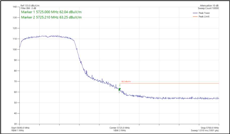
Figure 760 - 802.11ax HE20, SU, TxBF, Core 0-1 - 5700 MHz Band Edge Frequency 5725 MHz
