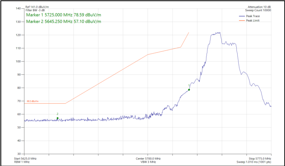
Figure 814 - 802.11be EHT40, RU52+26-70, SISO, Core 1 - 5755 MHz Band Edge Frequency 5725 MHz
