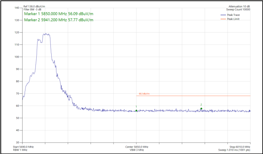
Figure 831 - 802.11be EHT40, RU106+26-85, SISO, Core 1 - 5710 MHz Band Edge Frequency 5850 MHz
