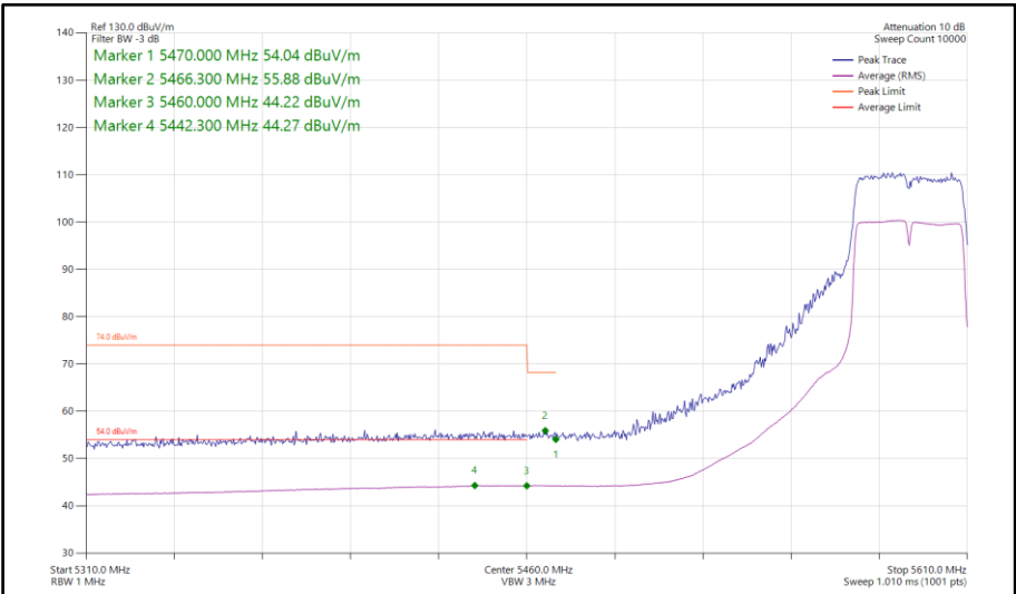
Figure 770 - 802.11n HT40, SISO, Core 0 - 5590 MHz Band Edge Frequency 5470 MHz
