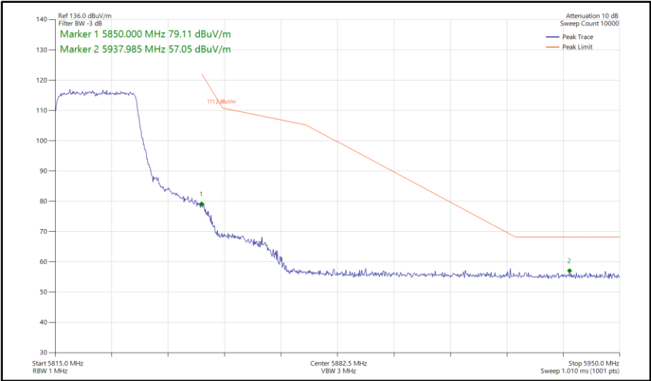
Figure 764 - 802.11ax HE20, SU, TxBF, Core 0-1 - 5825 MHz Band Edge Frequency 5850 MHz
