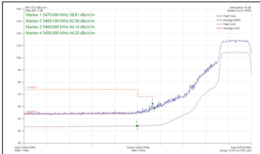
Figure 752 - 802.11ac VHT20, TxBF, Core 0-1 - 5520 MHz Band Edge Frequency 5470 MHz
