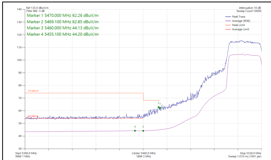
Figure 754 - 802.11ax HE20, SU, TxBF, Core 0-1 - 5520 MHz Band Edge Frequency 5470 MHz
