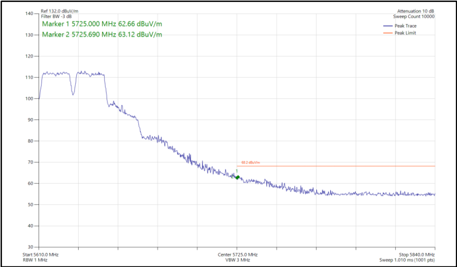
Figure 815 - 802.11a a40, SISO, Core 1 - 5630 MHz Band Edge Frequency 5725 MHz
