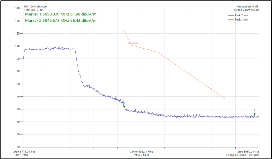
Figure 795 - 802.11ax HE40, SU, SISO, Core 0 - 5795 MHz Band Edge Frequency 5850 MHz
