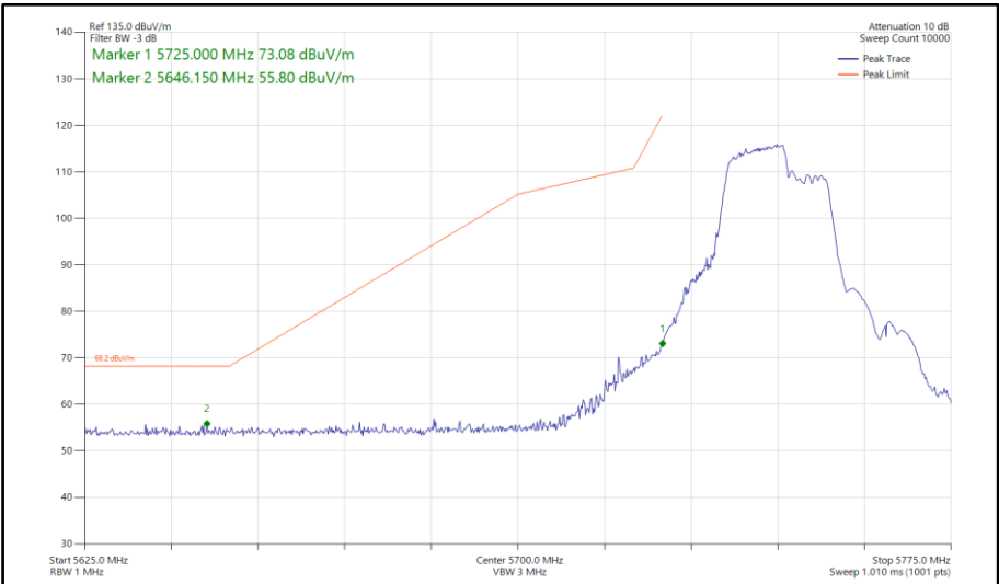
Figure 780 - 802.11be EHT40, RU106+26-82, SISO, Core 0 - 5755 MHz Band Edge Frequency 5725 MHz
