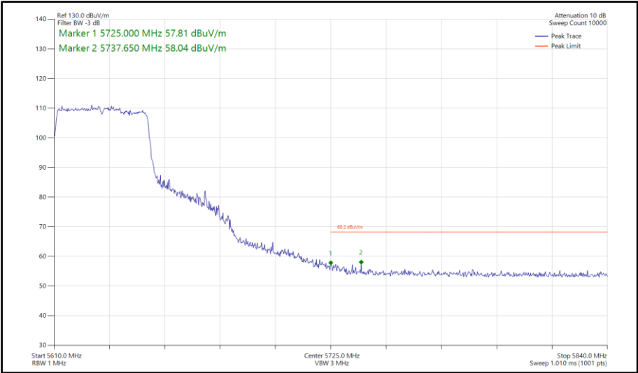
Figure 785 - 802.11ax HE40, SU, SISO, Core 0 - 5630 MHz Band Edge Frequency 5725 MHz
