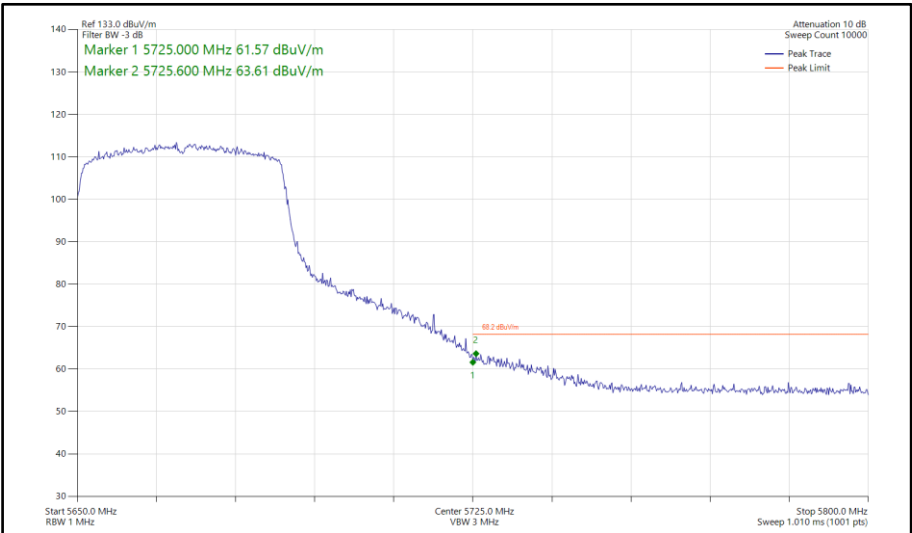
Figure 820 - 802.11ax HE40, SU, SISO, Core 1 - 5670 MHz Band Edge Frequency 5725 MHz
