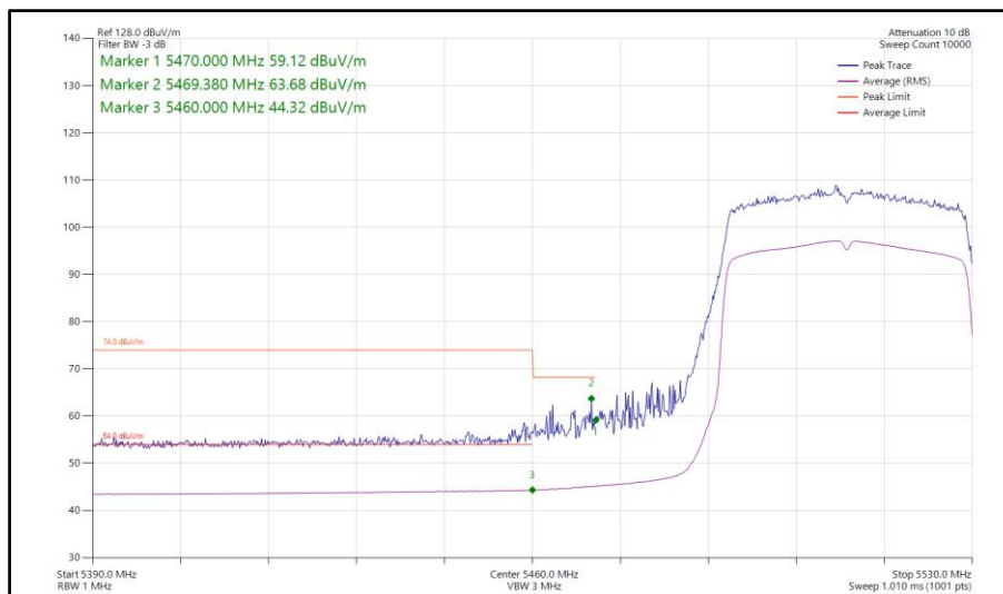
Figure 805 - 802.11ax HE40, SU, SISO, Core 1 - 5510 MHz Band Edge Frequency 5470 MHz
