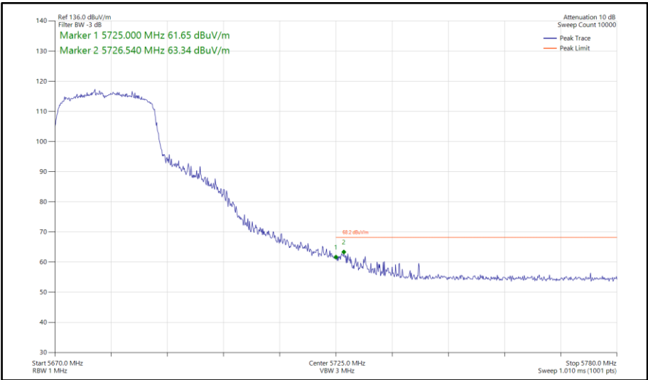
Figure 759 - 802.11ax HE20, SU, TxBF, Core 0-1 - 5680 MHz Band Edge Frequency 5725 MHz
