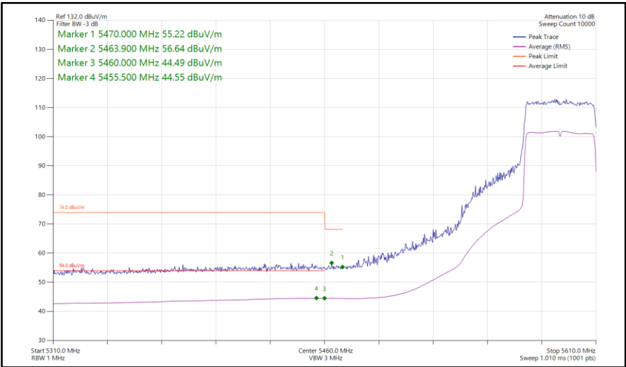
Figure 808 - 802.11ax HE40, SU, SISO, Core 1 - 5590 MHz Band Edge Frequency 5470 MHz
