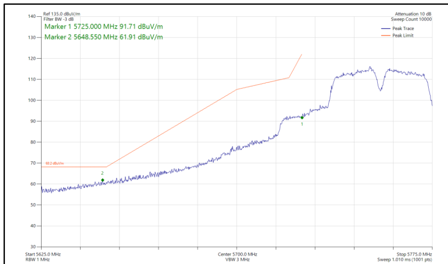
Figure 810 - 802.11a a40, SISO, Core 1 - 5755 MHz Band Edge Frequency 5725 MHz
