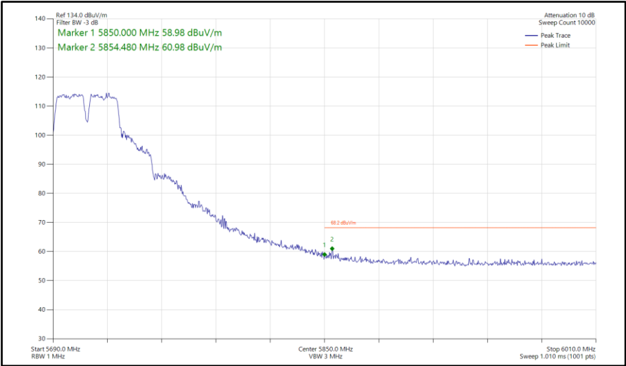
Figure 823 - 802.11a a40, SISO, Core 1 - 5710 MHz Band Edge Frequency 5850 MHz
