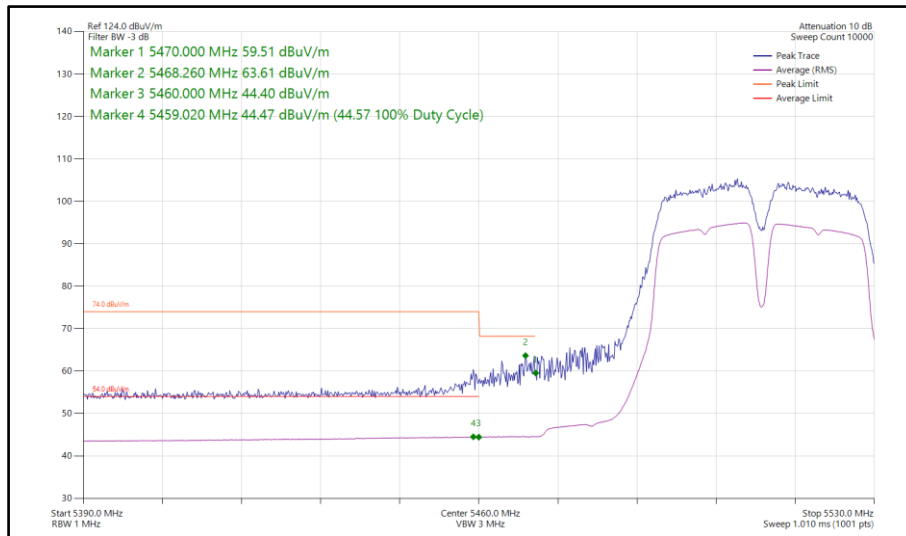
Figure 765 - 802.11a a40, SISO, Core 0 - 5510 MHz Band Edge Frequency 5470 MHz
