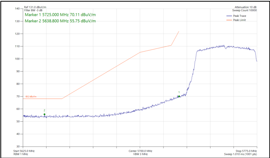
Figure 778 - 802.11ax HE40, SU, SISO, Core 0 - 5755 MHz Band Edge Frequency 5725 MHz
