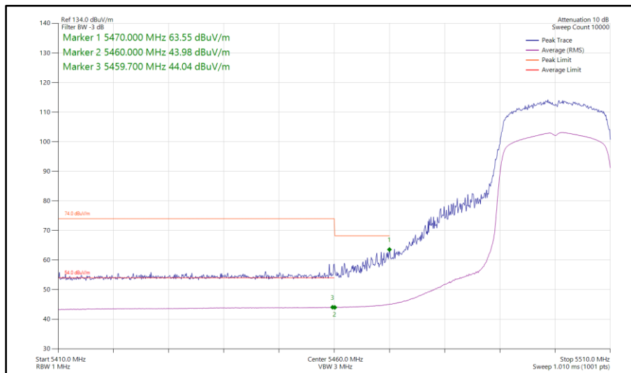
Figure 753 - 802.11ax HE20, SU, TxBF, Core 0-1 - 5500 MHz Band Edge Frequency 5470 MHz
