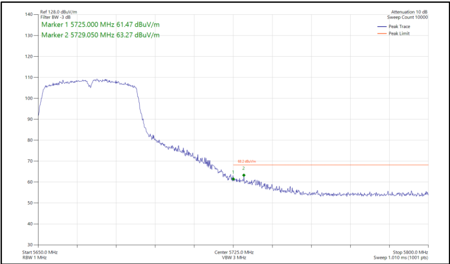
Figure 784 - 802.11n HT40, SISO, Core 0 - 5670 MHz Band Edge Frequency 5725 MHz
