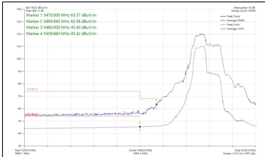
Figure 809 - 802.11be EHT40, RU52+26-70, SISO, Core 1 - 5510 MHz Band Edge Frequency 5470 MHz
