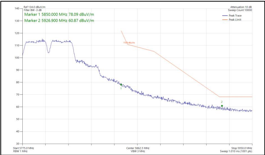
Figure 824 - 802.11a a40, SISO, Core 1 - 5795 MHz Band Edge Frequency 5850 MHz
