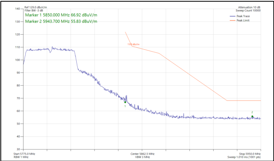
Figure 792 - 802.11n HT40, SISO, Core 0 - 5795 MHz Band Edge Frequency 5850 MHz
