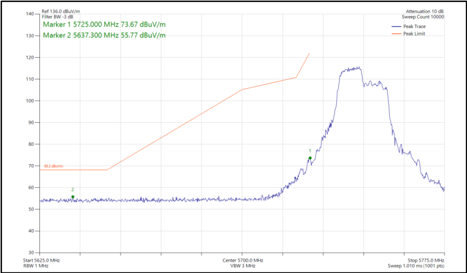
Figure 779 - 802.11ax HE40, RU106-53, SISO, Core 0 - 5755 MHz Band Edge Frequency 5725 MHz
