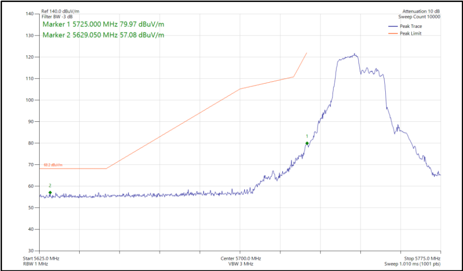
Figure 813 - 802.11ax HE40, RU106-53, SISO, Core 1 - 5755 MHz Band Edge Frequency 5725 MHz
