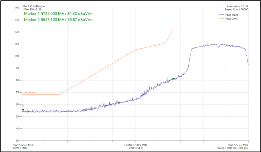
Figure 777 - 802.11n HT40, SISO, Core 0 - 5755 MHz Band Edge Frequency 5725 MHz
