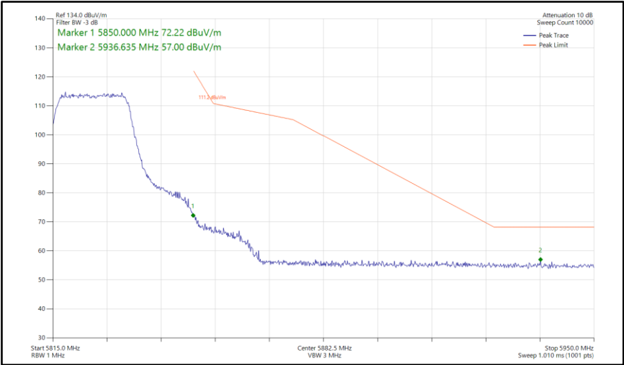
Figure 762 - 802.11ac VHT20, TxBF, Core 0-1 - 5825 MHz Band Edge Frequency 5850 MHz
