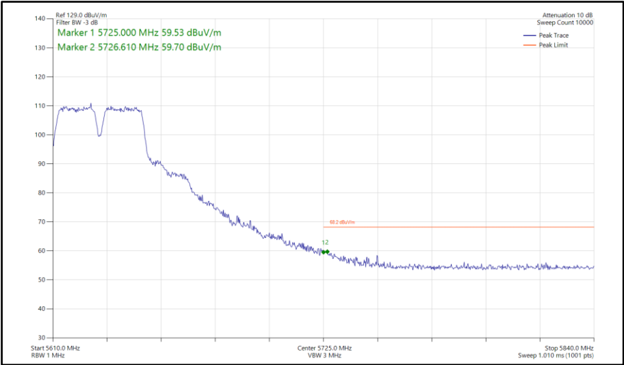
Figure 781 - 802.11a a40, SISO, Core 0 - 5630 MHz Band Edge Frequency 5725 MHz
