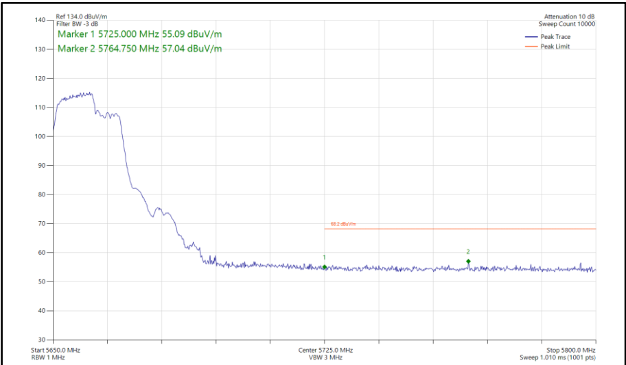
Figure 788 - 802.11be EHT40, RU106+26-82, SISO, Core 0 - 5670 MHz Band Edge Frequency 5725 MHz
