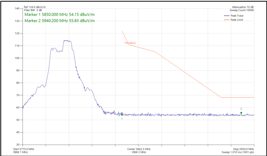
Figure 798 - 802.11be EHT40, RU52+26-75, SISO, Core 0 - 5795 MHz Band Edge Frequency 5850 MHz
