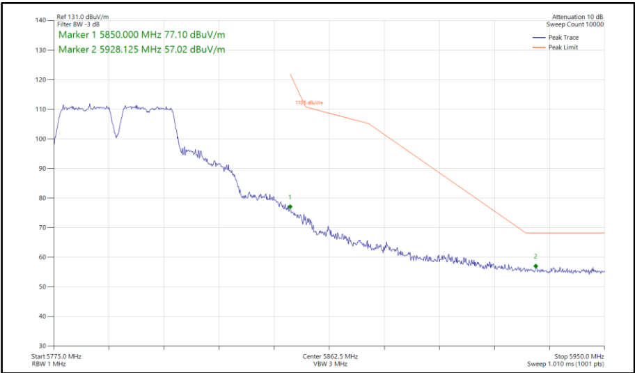
Figure 790 - 802.11a a40, SISO, Core 0 - 5795 MHz Band Edge Frequency 5850 MHz
