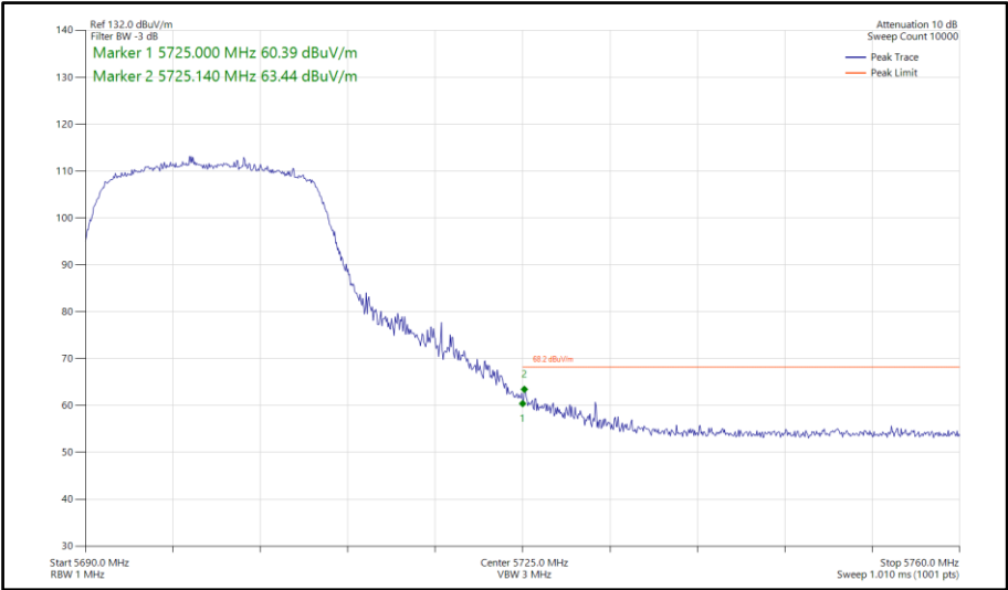
Figure 758 - 802.11ac VHT20, TxBF, Core 0-1 - 5700 MHz Band Edge Frequency 5725 MHz
