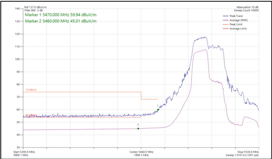
Figure 772 - 802.11ax HE40, RU106-53, SISO, Core 0 - 5510 MHz Band Edge Frequency 5470 MHz
