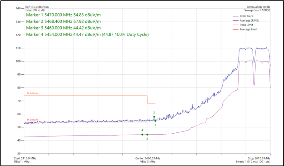
Figure 767 - 802.11a a40, SISO, Core 0 - 5590 MHz Band Edge Frequency 5470 MHz
