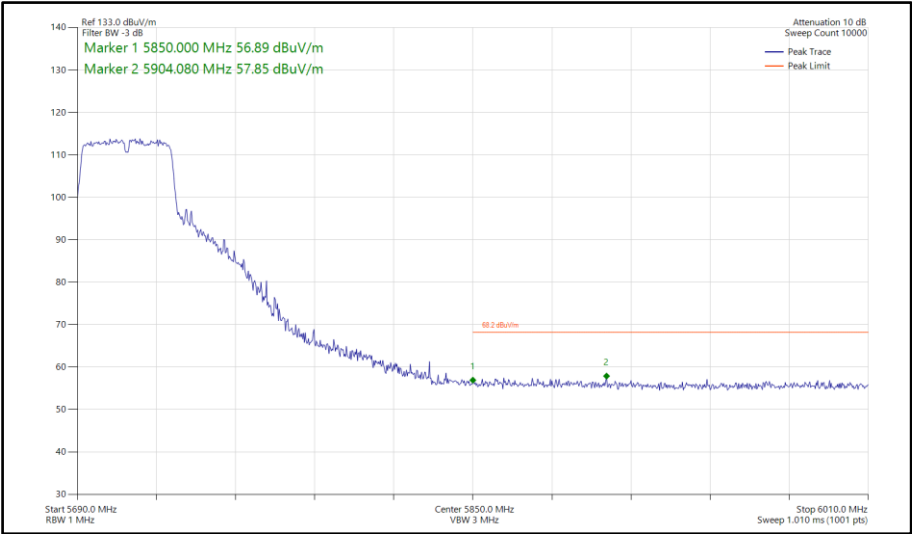
Figure 825 - 802.11n HT40, SISO, Core 1 - 5710 MHz Band Edge Frequency 5850 MHz
