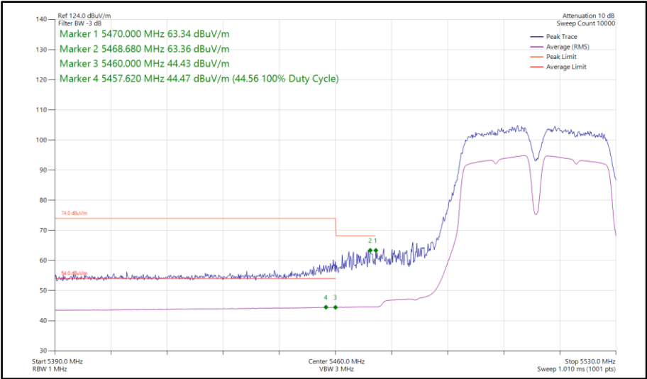
Figure 799 - 802.11a a40, SISO, Core 1 - 5510 MHz Band Edge Frequency 5470 MHz
