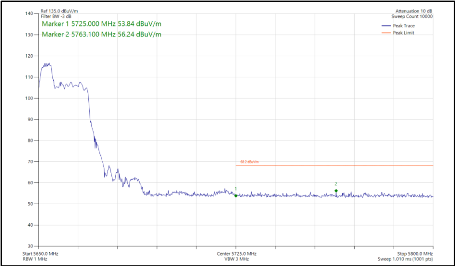
Figure 787 - 802.11ax HE40, RU52-37, SISO, Core 0 - 5670 MHz Band Edge Frequency 5725 MHz
