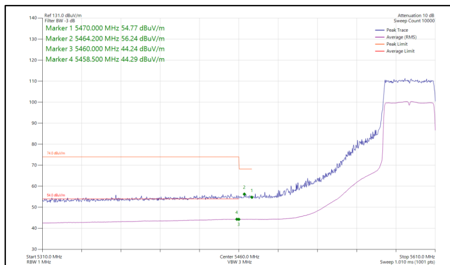
Figure 774 - 802.11ax HE40, SU, SISO, Core 0 - 5590 MHz Band Edge Frequency 5470 MHz
