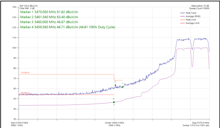
Figure 800 - 802.11a a40, SISO, Core 1 - 5550 MHz Band Edge Frequency 5470 MHz
