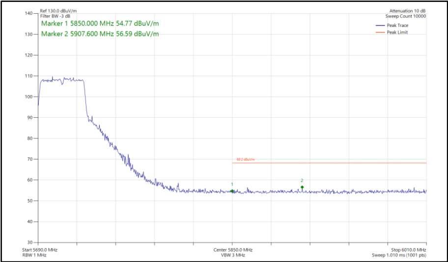
Figure 791 - 802.11n HT40, SISO, Core 0 - 5710 MHz Band Edge Frequency 5850 MHz
