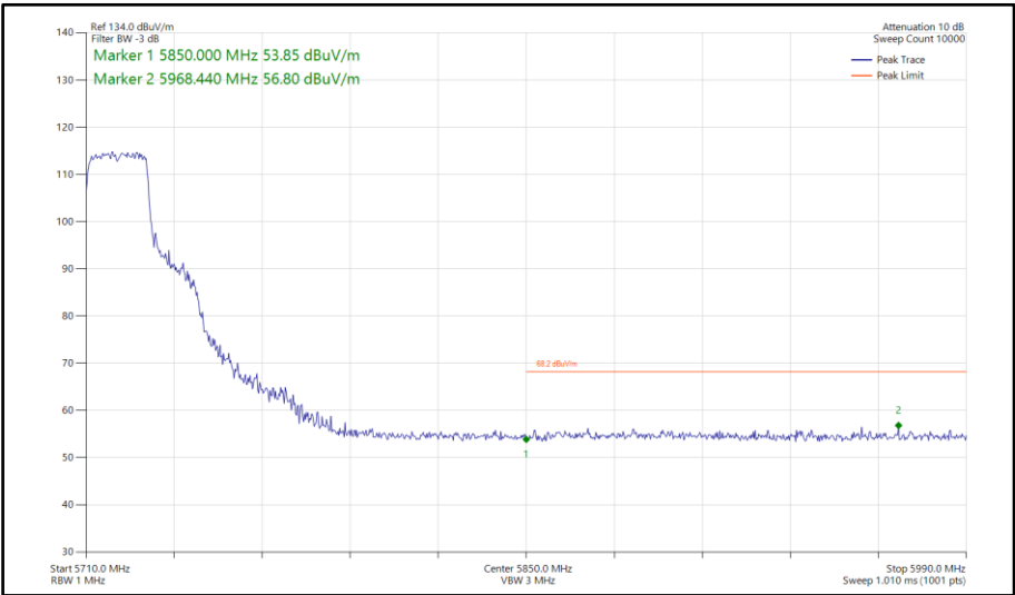
Figure 763 - 802.11ax HE20, SU, TxBF, Core 0-1 - 5720 MHz Band Edge Frequency 5850 MHz
