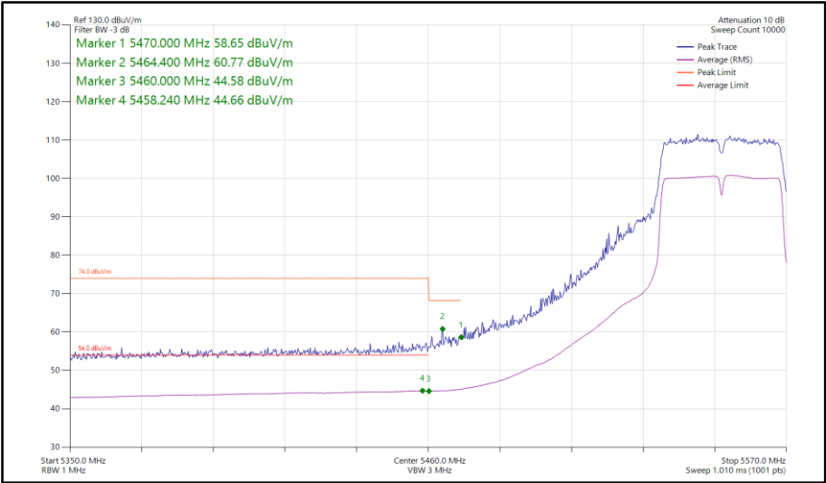
Figure 769 - 802.11n HT40, SISO, Core 0 - 5550 MHz Band Edge Frequency 5470 MHz
