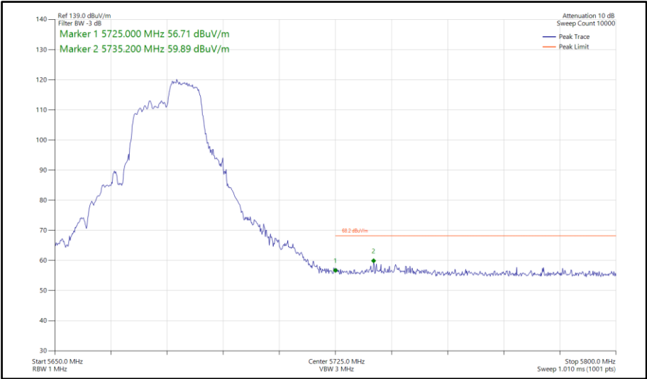
Figure 821 - 802.11ax HE40, RU106-56, SISO, Core 1 - 5670 MHz Band Edge Frequency 5725 MHz
