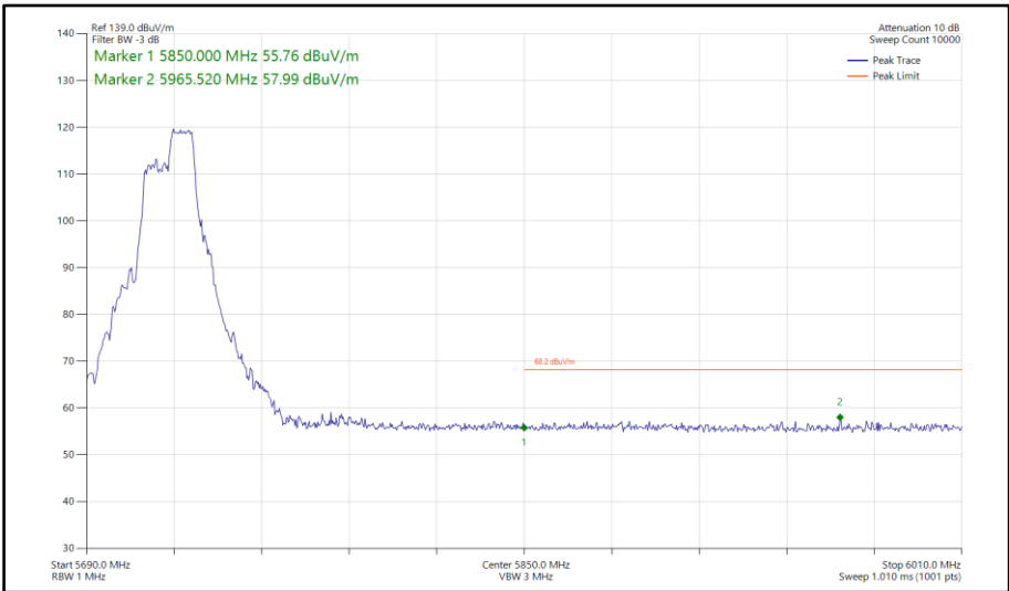
Figure 828 - 802.11ax HE40, RU106-56, SISO, Core 1 - 5710 MHz Band Edge Frequency 5850 MHz
