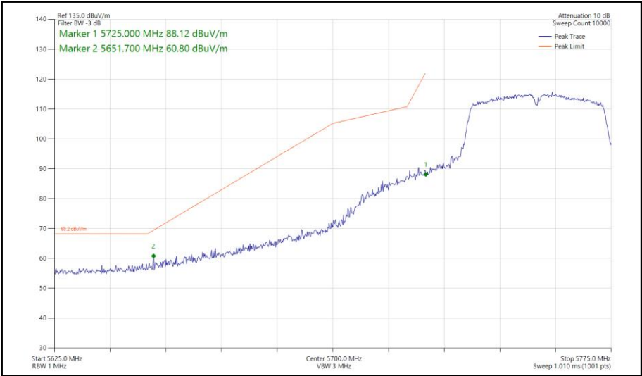
Figure 811 - 802.11n HT40, SISO, Core 1 - 5755 MHz Band Edge Frequency 5725 MHz
