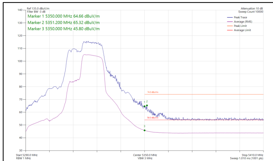
Figure 118 - 802.11be EHT40, RU106+26-85, SISO, Core 0 - 5310 MHz Band Edge Frequency 5350 MHz
