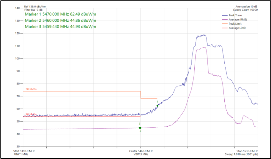
Figure 129 - 802.11be EHT40, RU52+26-70, SISO, Core 0 - 5510 MHz Band Edge Frequency 5460 MHz
