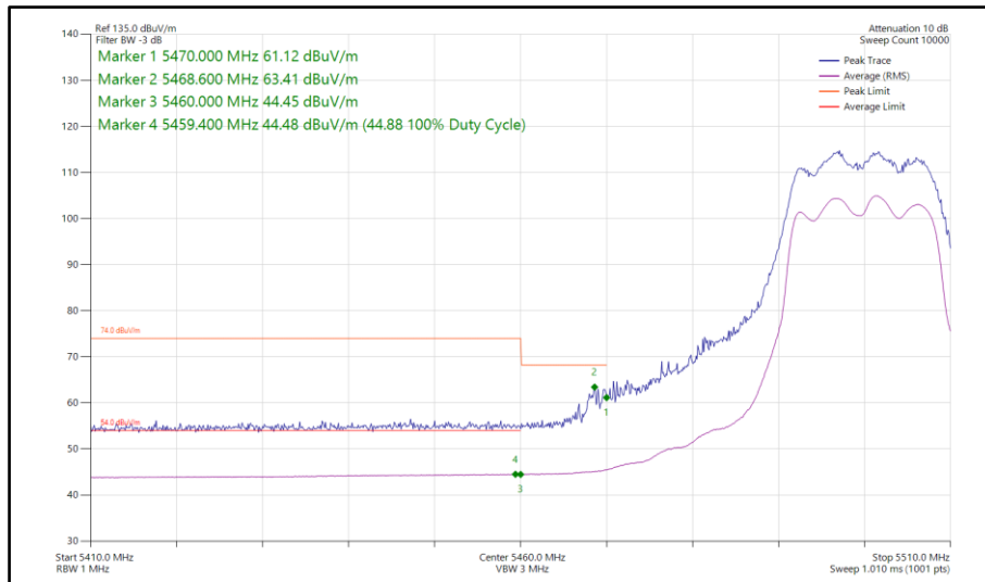
Figure 65 - 802.11a, CDD, Core 0-1 - 5500 MHz Band Edge Frequency 5460 MHz
