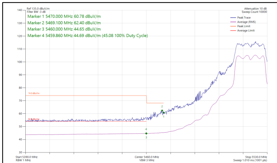
Figure 66 - 802.11a, CDD, Core 0-1 - 5520 MHz Band Edge Frequency 5460 MHz
