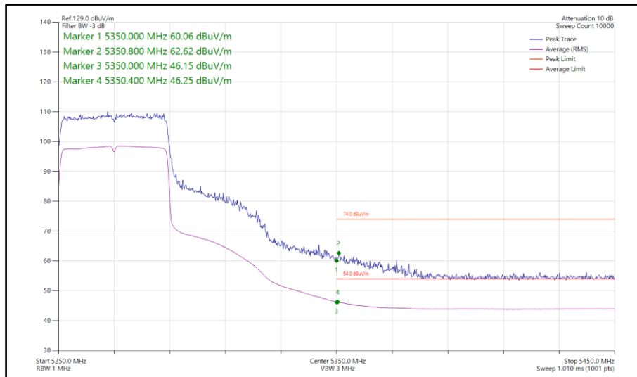
Figure 115 - 802.11ax HE40, SU, SISO, Core 0 - 5270 MHz Band Edge Frequency 5350 MHz
