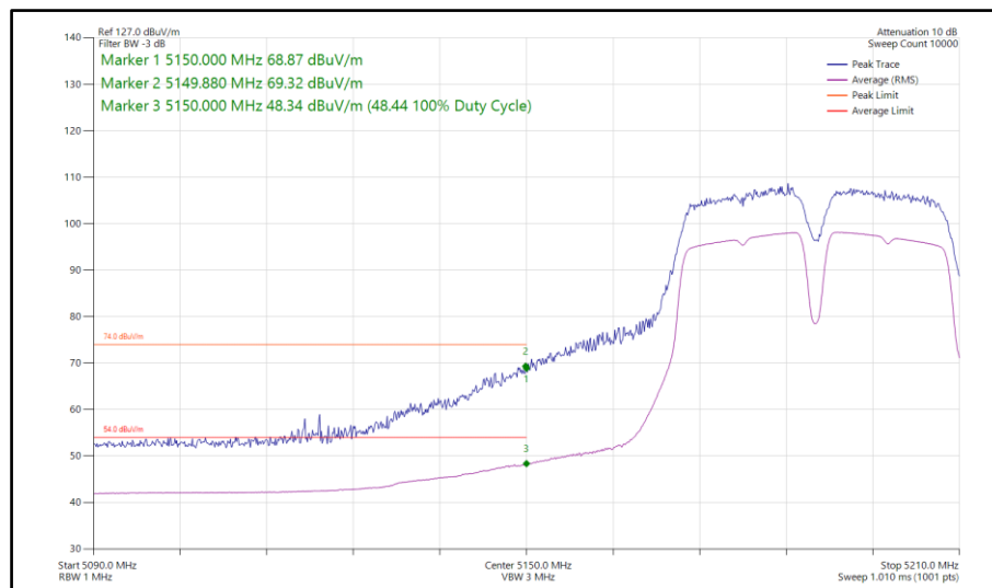
Figure 130 - 802.11a a40, SISO, Core 1 - 5190 MHz Band Edge Frequency 5150 MHz
