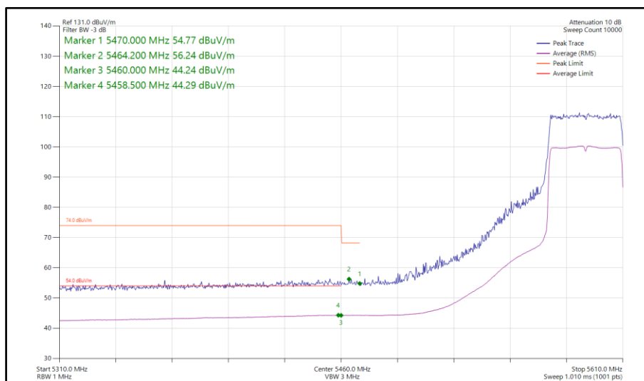
Figure 128 - 802.11ax HE40, SU, SISO, Core 0 - 5590 MHz Band Edge Frequency 5460 MHz
