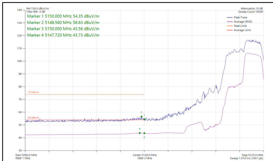
Figure 108 - 802.11ax HE40, RU106-56, SISO, Core 0 - 5190 MHz Band Edge Frequency 5150 MHz
