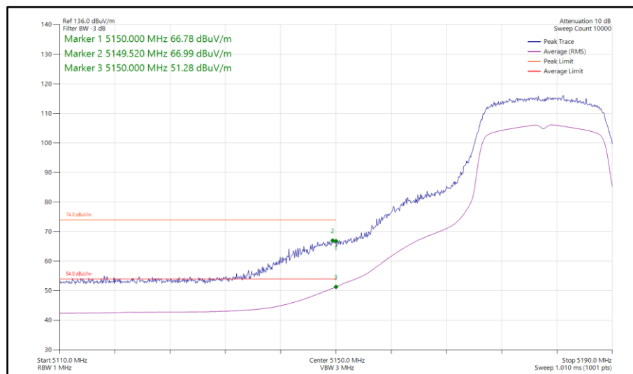
Figure 91 - 802.11ac VHT20, TxBF, Core 0-1 - 5180 MHz Band Edge Frequency 5150 MHz
