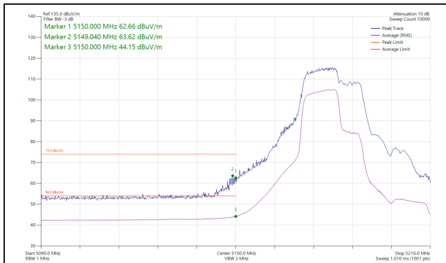
Figure 110 - 802.11be EHT40, RU106+26-82, SISO, Core 0 - 5190 MHz Band Edge Frequency 5150 MHz
