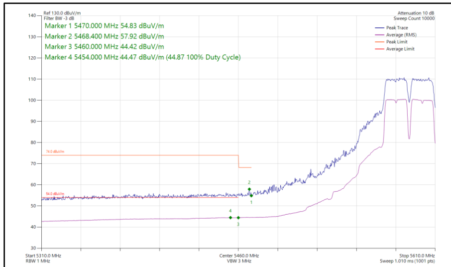
Figure 121 - 802.11a a40, SISO, Core 0 - 5590 MHz Band Edge Frequency 5460 MHz
