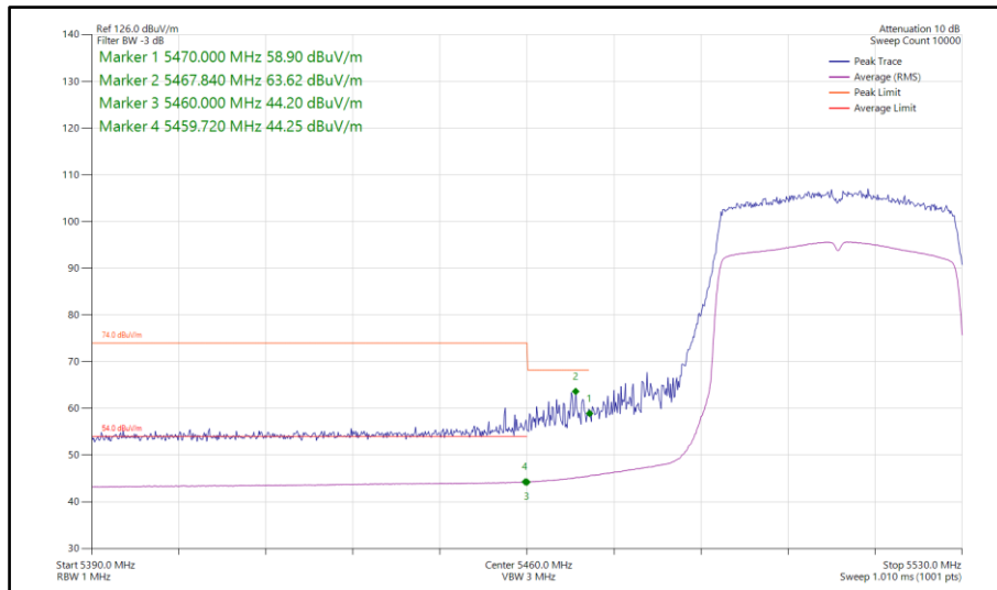
Figure 125 - 802.11ax HE40, SU, SISO, Core 0 - 5510 MHz Band Edge Frequency 5460 MHz
