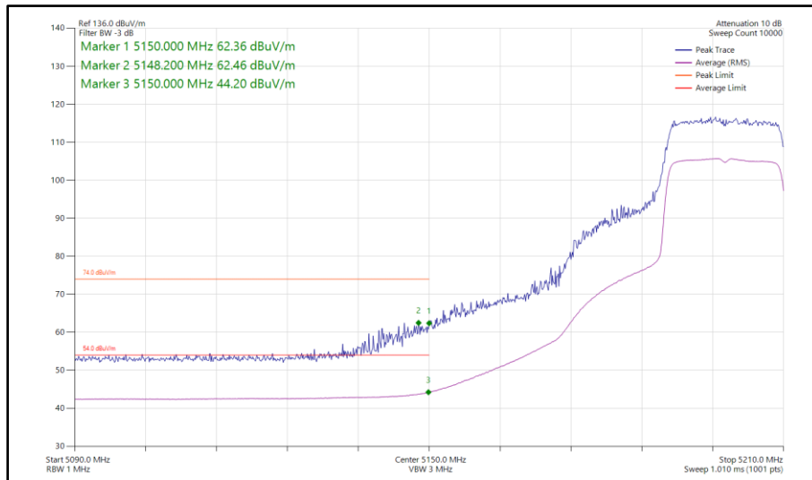
Figure 94 - 802.11ax HE20, SU, TxBF, Core 0-1 - 5200 MHz Band Edge Frequency 5150 MHz
