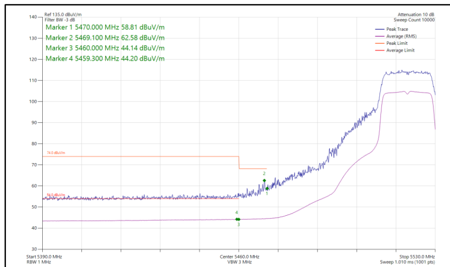
Figure 100 - 802.11ac VHT20, TxBF, Core 0-1 - 5520 MHz Band Edge Frequency 5460 MHz
