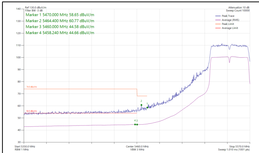
Figure 123 - 802.11n HT40, SISO, Core 0 - 5550 MHz Band Edge Frequency 5460 MHz
