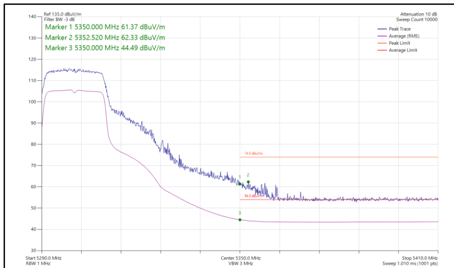
Figure 95 - 802.11ac VHT20, TxBF, Core 0-1 - 5300 MHz Band Edge Frequency 5350 MHz
