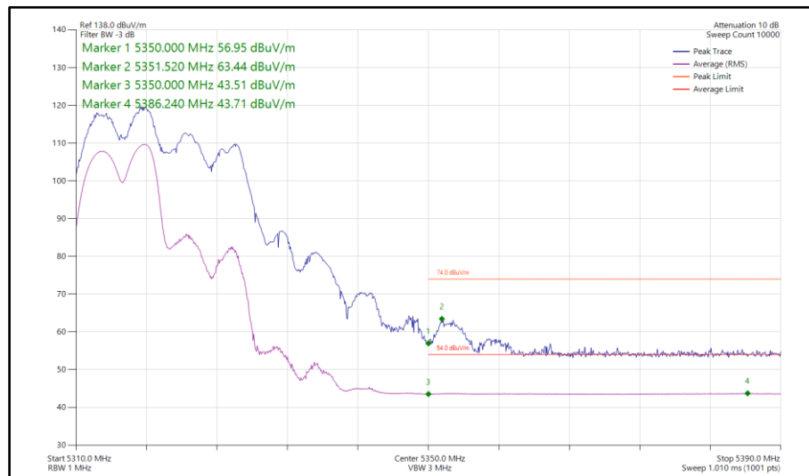
Figure 83 - 802.11ax HE20, RU106-53, SDM, Core 0-1 - 5320 MHz Band Edge Frequency 5350 MHz
