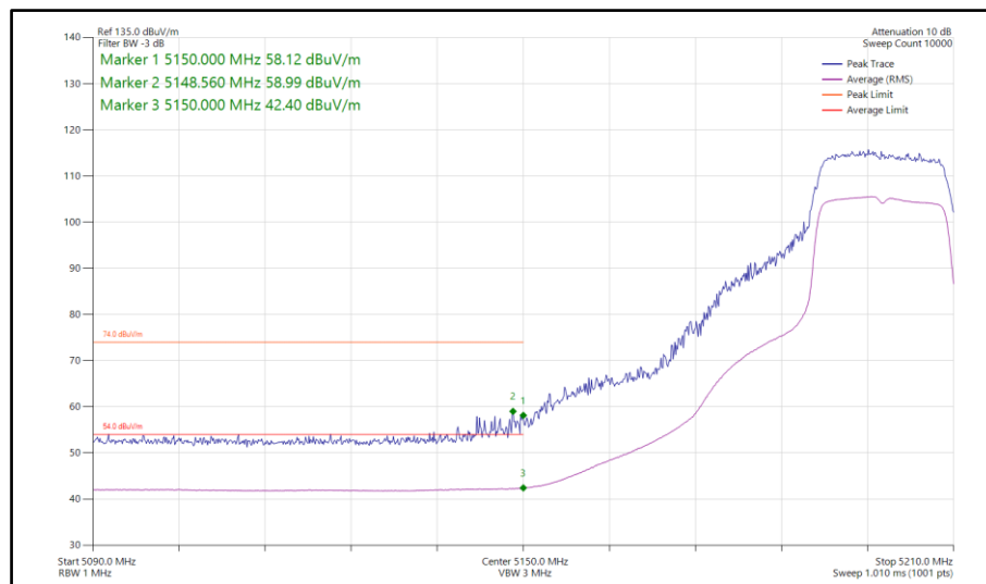
Figure 92 - 802.11ac VHT20, TxBF, Core 0-1 - 5200 MHz Band Edge Frequency 5150 MHz
