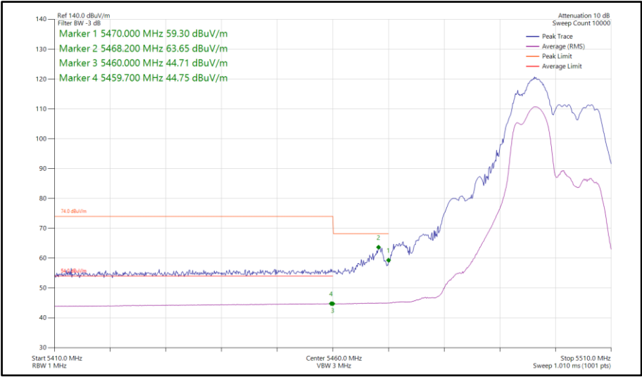
Figure 90 - 802.11be EHT20, RU52+26-70, SDM, Core 0-1 - 5500 MHz Band Edge Frequency 5460 MHz
