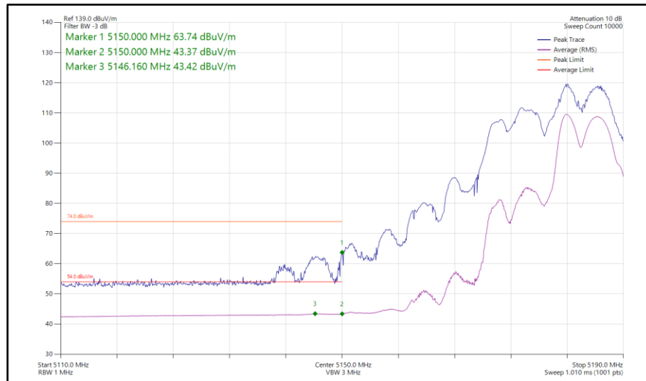
Figure 76 - 802.11ax HE20, RU106-54, SDM, Core 0-1 - 5180 MHz Band Edge Frequency 5150 MHz
