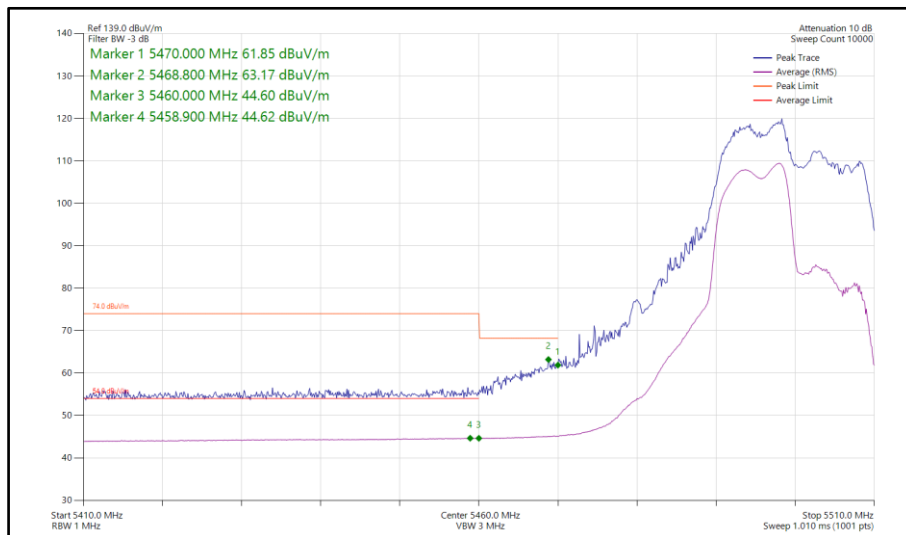
Figure 70 - 802.11ax HE20, RU106-53, CDD, Core 0-1 - 5500 MHz Band Edge Frequency 5460 MHz
