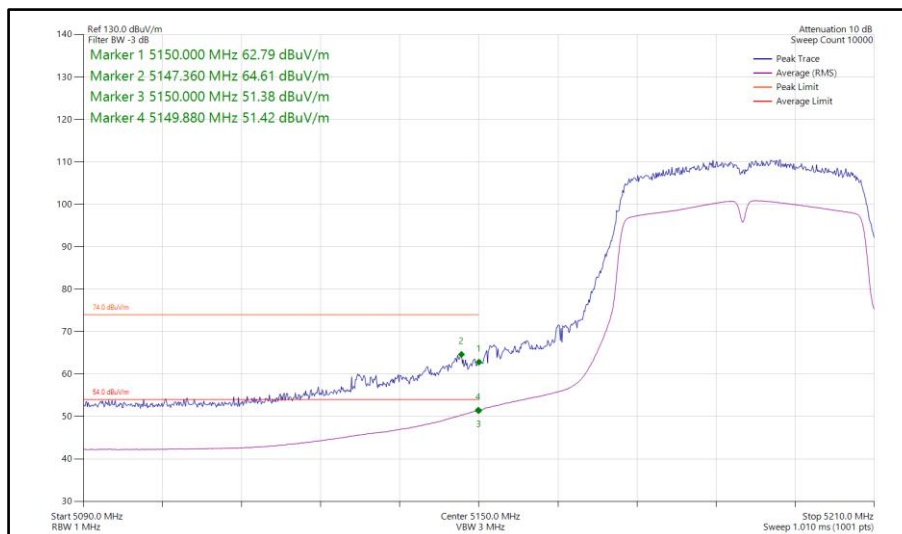
Figure 132 - 802.11n HT40, SISO, Core 1 - 5190 MHz Band Edge Frequency 5150 MHz
