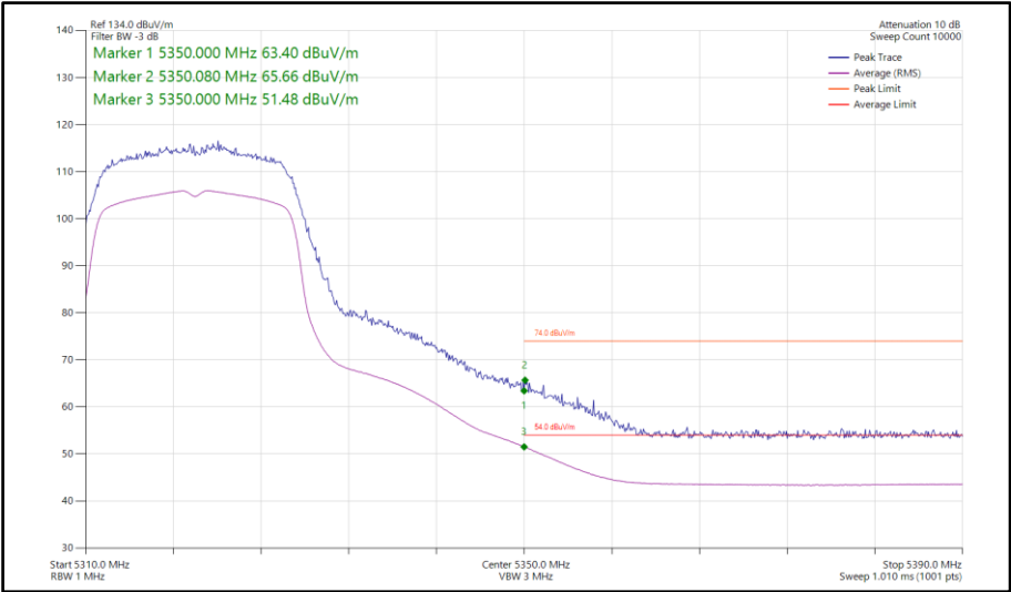
Figure 96 - 802.11ac VHT20, TxBF, Core 0-1 - 5320 MHz Band Edge Frequency 5350 MHz
