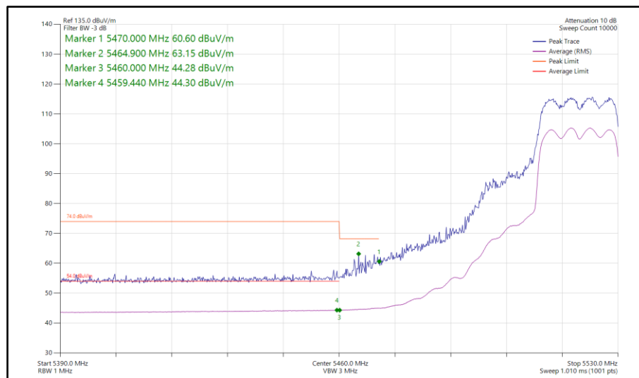
Figure 71 - 802.11ax HE20, SU, CDD, Core 0-1 - 5520 MHz Band Edge Frequency 5460 MHz
