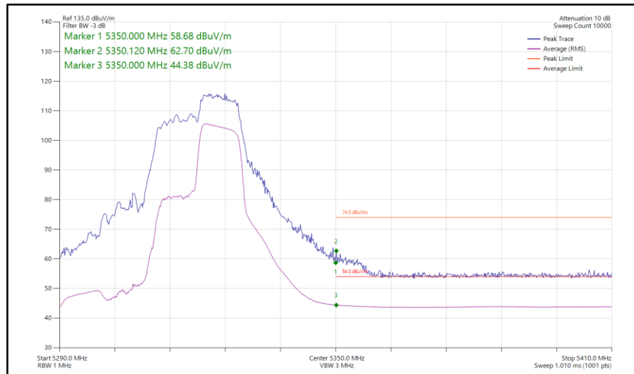
Figure 117 - 802.11ax HE40, RU106-56, SISO, Core 0 - 5310 MHz Band Edge Frequency 5350 MHz
