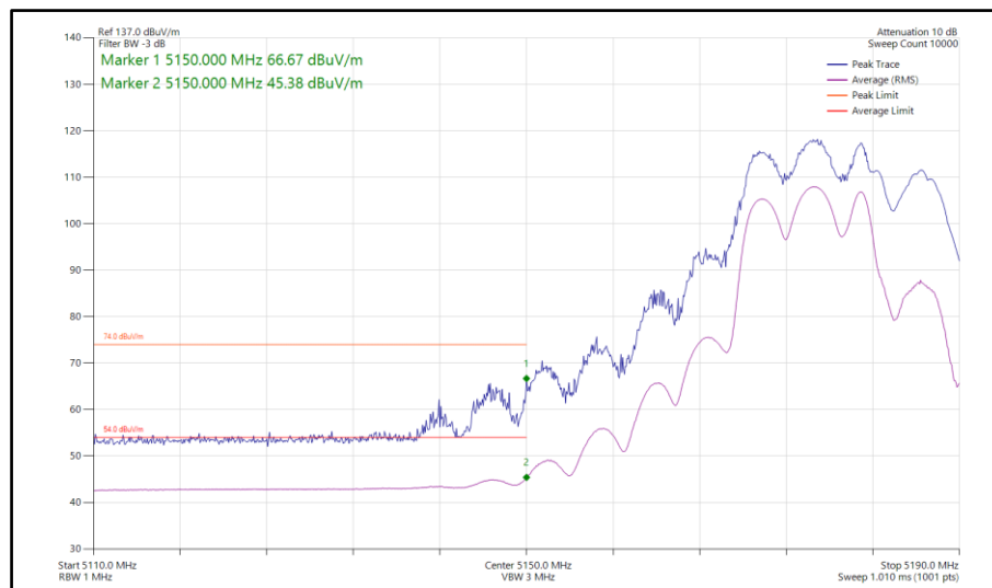
Figure 78 - 802.11be EHT20, RU106+26-82, SDM, Core 0-1 - 5180 MHz Band Edge Frequency 5150 MHz
