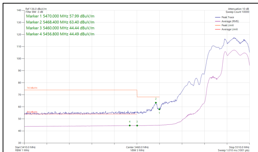
Figure 72 - 802.11be EHT20, RU106+26-83, CDD, Core 0-1 - 5500 MHz Band Edge Frequency 5460 MHz
