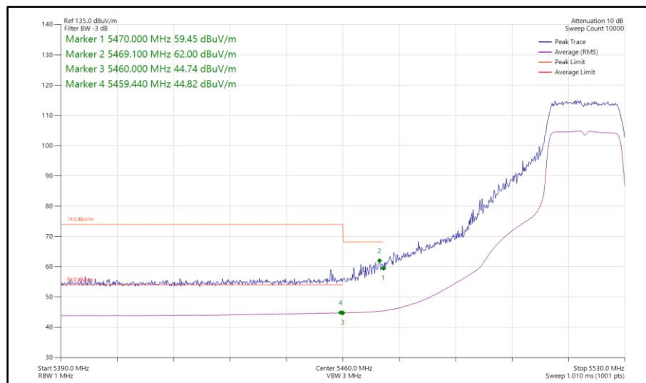
Figure 86 - 802.11n HT20, SDM, Core 0-1 - 5520 MHz Band Edge Frequency 5460 MHz
