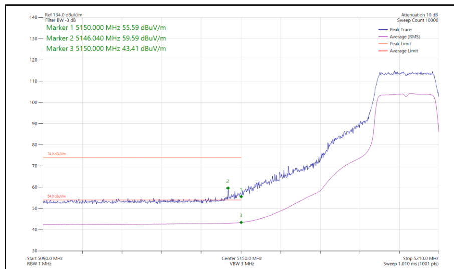
Figure 74 - 802.11n HT20, SDM, Core 0-1 - 5200 MHz Band Edge Frequency 5150 MHz
