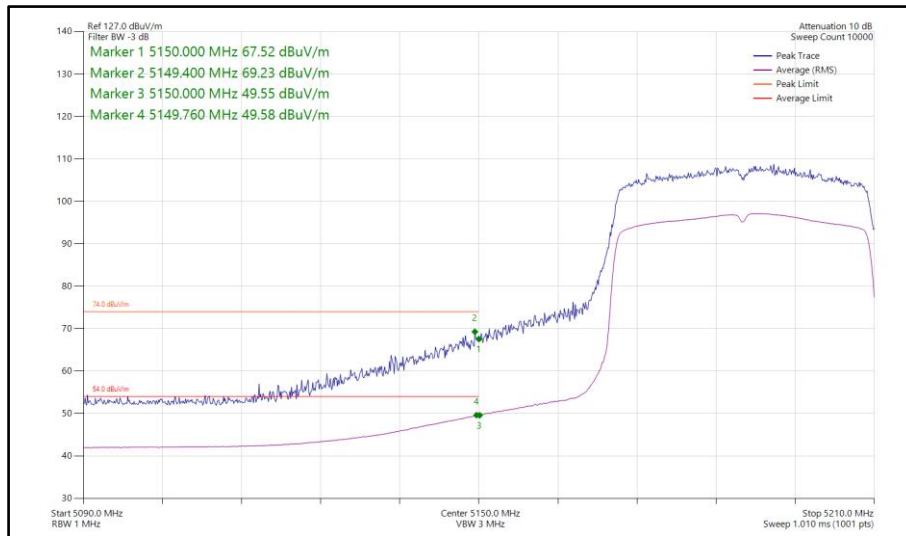
Figure 107 - 802.11ax HE40, SU, SISO, Core 0 - 5190 MHz Band Edge Frequency 5150 MHz
