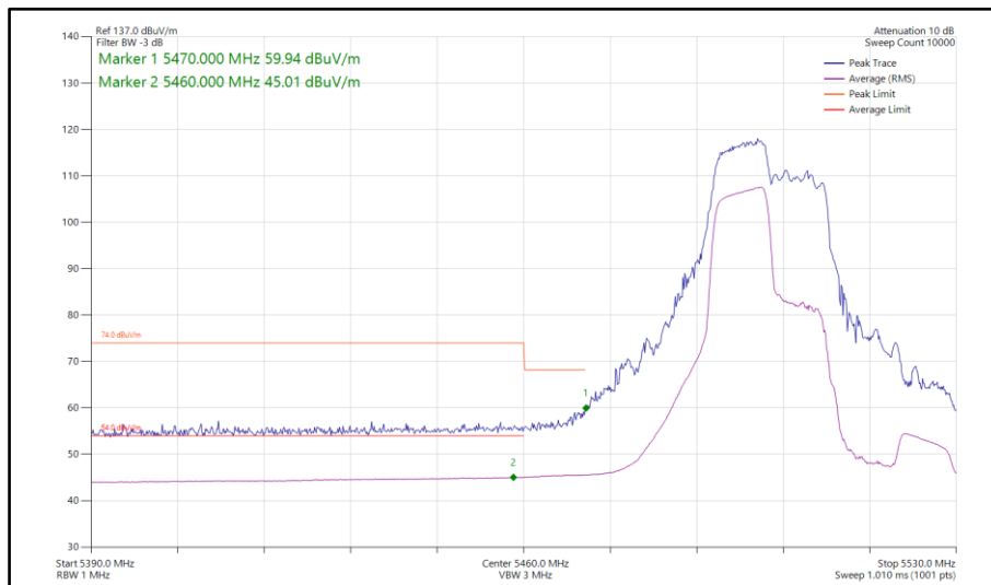
Figure 126 - 802.11ax HE40, RU106-53, SISO, Core 0 - 5510 MHz Band Edge Frequency 5460 MHz
