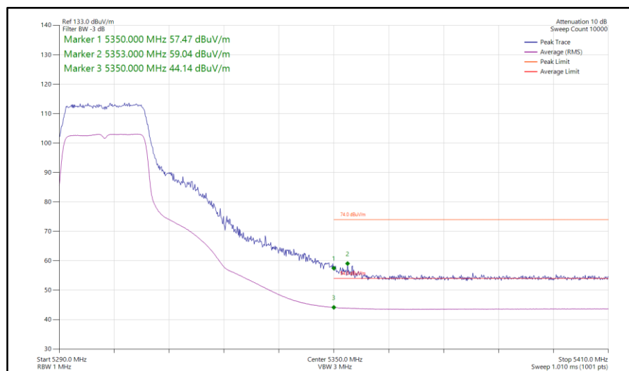
Figure 79 - 802.11n HT20, SDM, Core 0-1 - 5300 MHz Band Edge Frequency 5350 MHz
