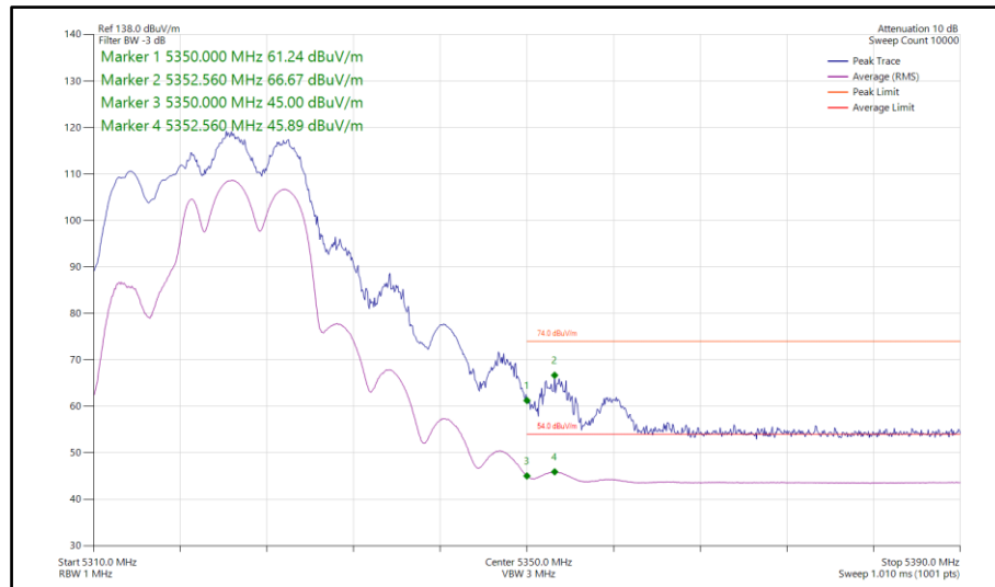
Figure 84 - 802.11be EHT20, RU106+26-83, SDM, Core 0-1 - 5320 MHz Band Edge Frequency 5350 MHz
