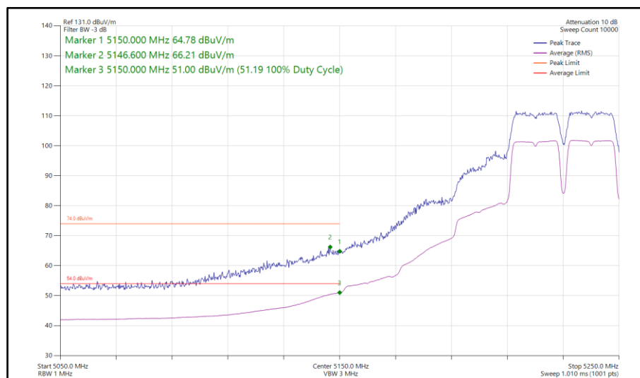
Figure 131 - 802.11a a40, SISO, Core 1 - 5230 MHz Band Edge Frequency 5150 MHz
