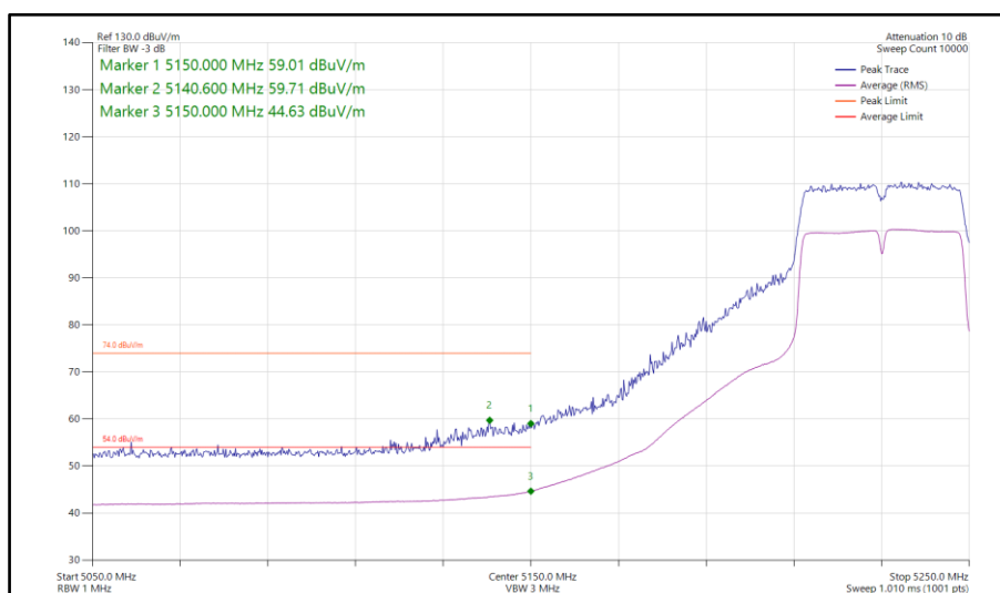
Figure 133 - 802.11n HT40, SISO, Core 1 - 5230 MHz Band Edge Frequency 5150 MHz
