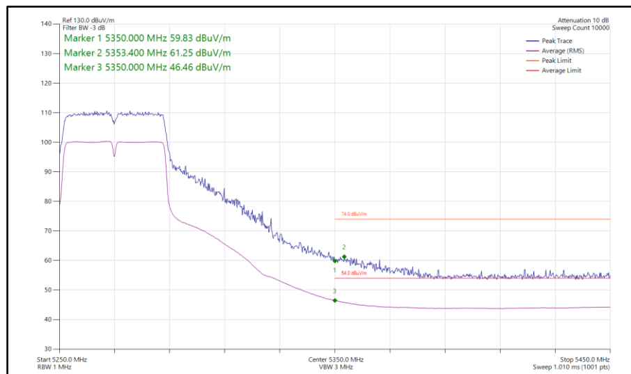
Figure 140 - 802.11n HT40, SISO, Core 1 - 5270 MHz Band Edge Frequency 5350 MHz
