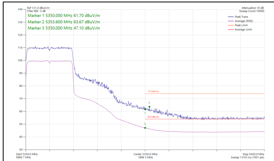
Figure 142 - 802.11ax HE40, SU, SISO, Core 1 - 5270 MHz Band Edge Frequency 5350 MHz
