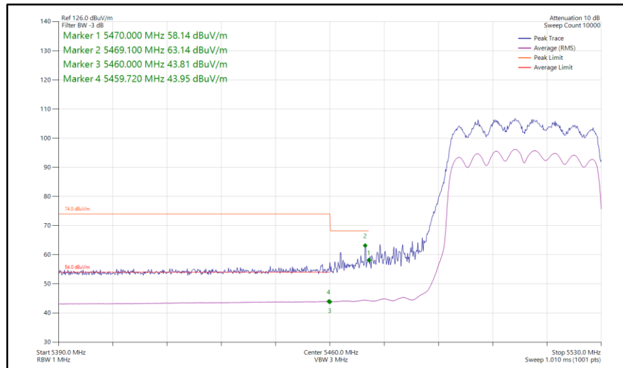
Figure 179 - 802.11ax HE40, SU, CDD, Core 0-1 - 5510 MHz Band Edge Frequency 5460 MHz
