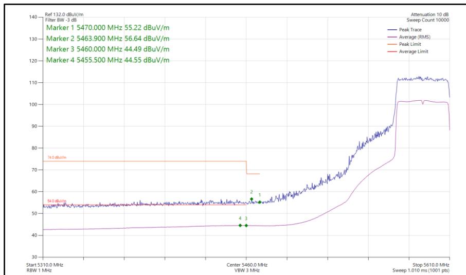
Figure 155 - 802.11ax HE40, SU, SISO, Core 1 - 5590 MHz Band Edge Frequency 5460 MHz
