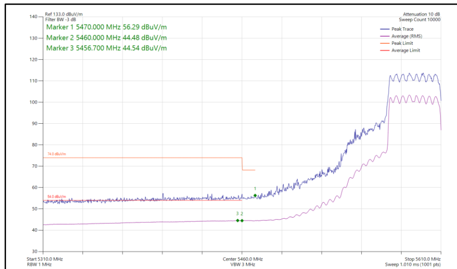
Figure 182 - 802.11ax HE40, SU, CDD, Core 0-1 - 5590 MHz Band Edge Frequency 5460 MHz
