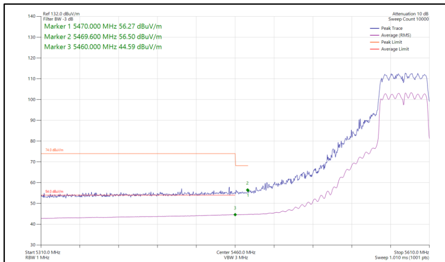
Figure 178 - 802.11n HT40, CDD, Core 0-1 - 5590 MHz Band Edge Frequency 5460 MHz
