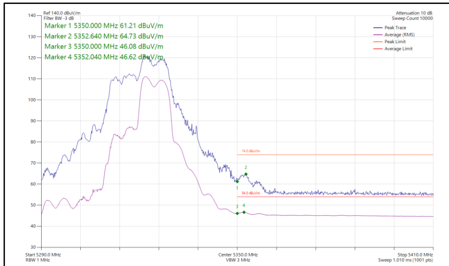
Figure 171 - 802.11ax HE40, RU106-56, CDD, Core 0-1 - 5310 MHz Band Edge Frequency 5350 MHz
