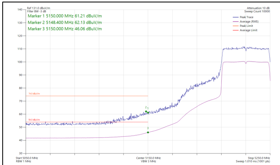
Figure 136 - 802.11ax HE40, SU, SISO, Core 1 - 5230 MHz Band Edge Frequency 5150 MHz
