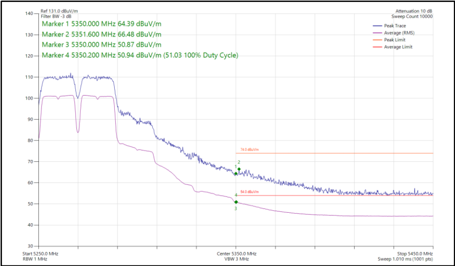
Figure 138 - 802.11a a40, SISO, Core 1 - 5270 MHz Band Edge Frequency 5350 MHz
