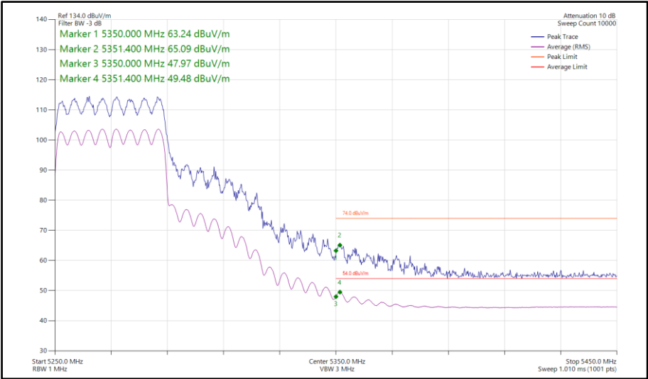
Figure 169 - 802.11ax HE40, SU, CDD, Core 0-1 - 5270 MHz Band Edge Frequency 5350 MHz
