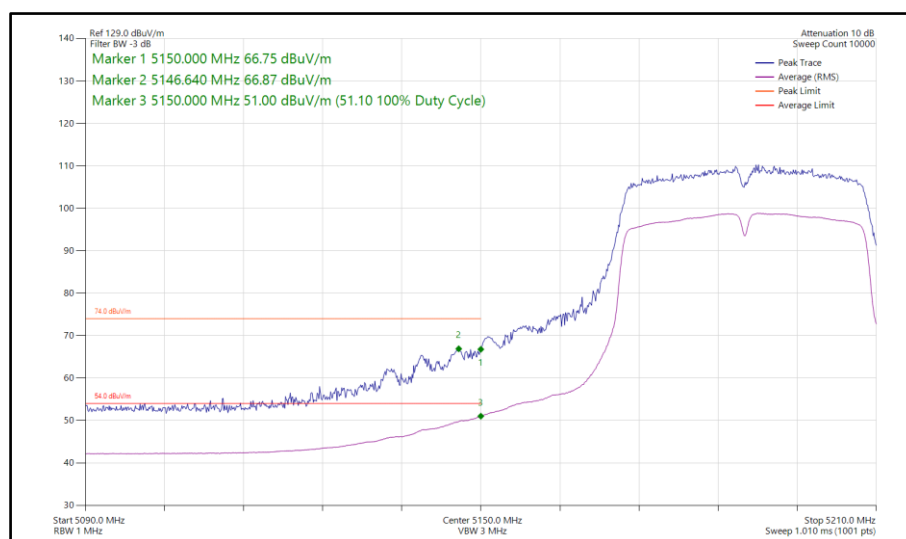
Figure 184 - 802.11n HT40, SDM, Core 0-1 - 5190 MHz Band Edge Frequency 5150 MHz
