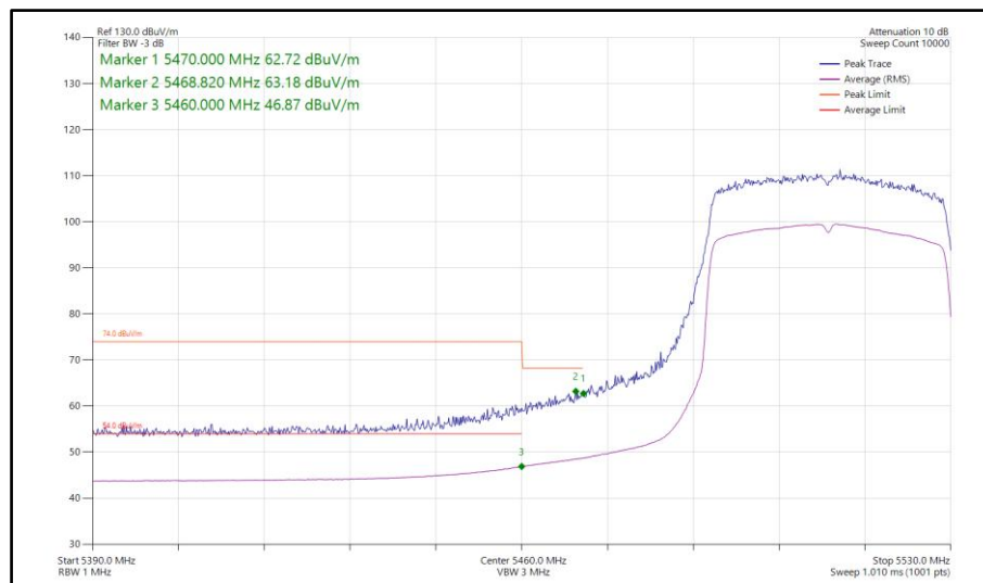
Figure 199 - 802.11ax HE40, SU, SDM, Core 0-1 - 5510 MHz Band Edge Frequency 5460 MHz
