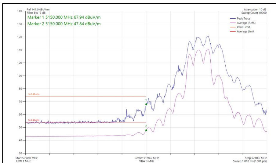
Figure 164 - 802.11be EHT40, RU106+26-82, CDD, Core 0-1 - 5190 MHz Band Edge Frequency 5150 MHz
