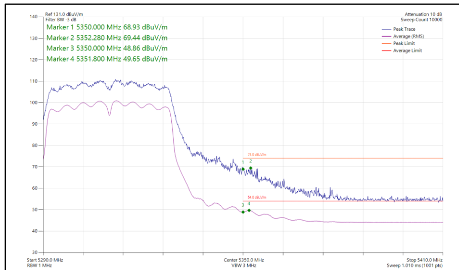
Figure 168 - 802.11n HT40, CDD, Core 0-1 - 5310 MHz Band Edge Frequency 5350 MHz
