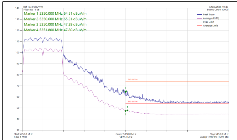
Figure 167 - 802.11n HT40, CDD, Core 0-1 - 5270 MHz Band Edge Frequency 5350 MHz
