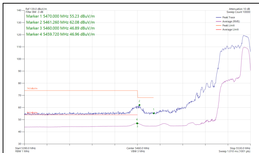
Figure 153 - 802.11ax HE40, RU52-44, SISO, Core 1 - 5510 MHz Band Edge Frequency 5460 MHz
