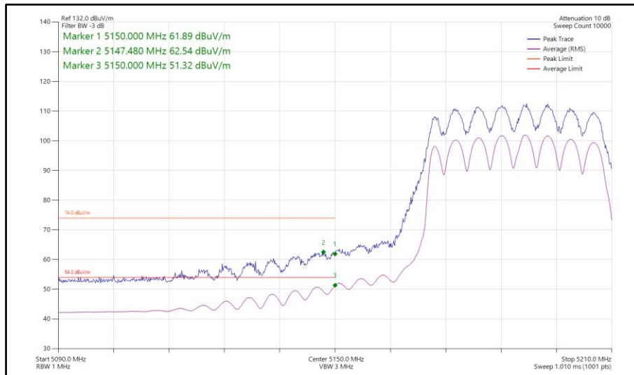
Figure 161 - 802.11ax HE40, SU, CDD, Core 0-1 - 5190 MHz Band Edge Frequency 5150 MHz
