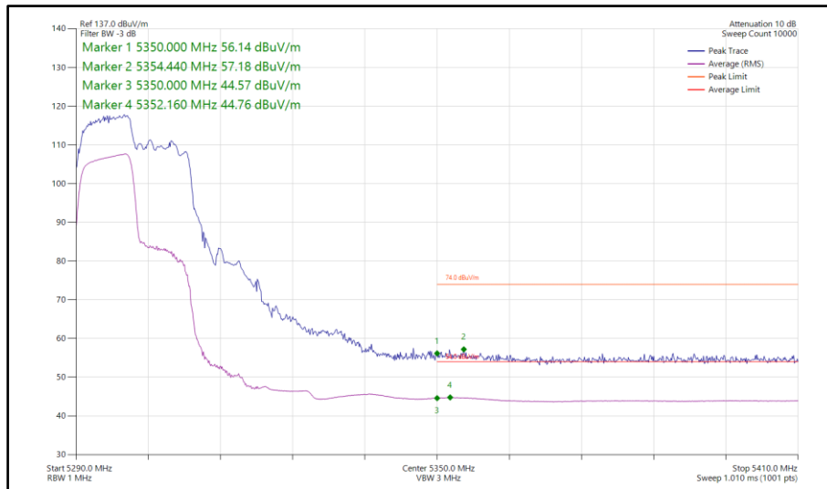
Figure 144 - 802.11ax HE40, RU106-53, SISO, Core 1 - 5310 MHz Band Edge Frequency 5350 MHz
