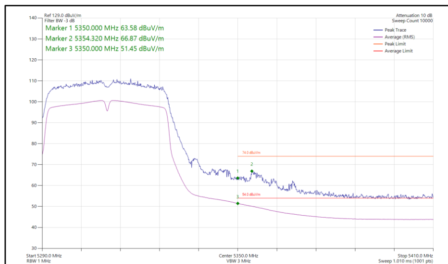
Figure 141 - 802.11n HT40, SISO, Core 1 - 5310 MHz Band Edge Frequency 5350 MHz
