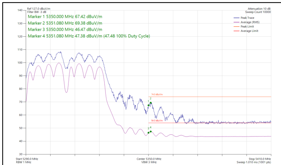
Figure 166 - 802.11a a40, CDD, Core 0-1 - 5310 MHz Band Edge Frequency 5350 MHz
