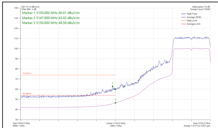
Figure 188 - 802.11ax HE40, SU, SDM, Core 0-1 - 5230 MHz Band Edge Frequency 5150 MHz
