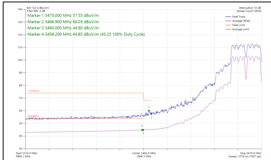
Figure 175 - 802.11a a40, CDD, Core 0-1 - 5590 MHz Band Edge Frequency 5460 MHz
