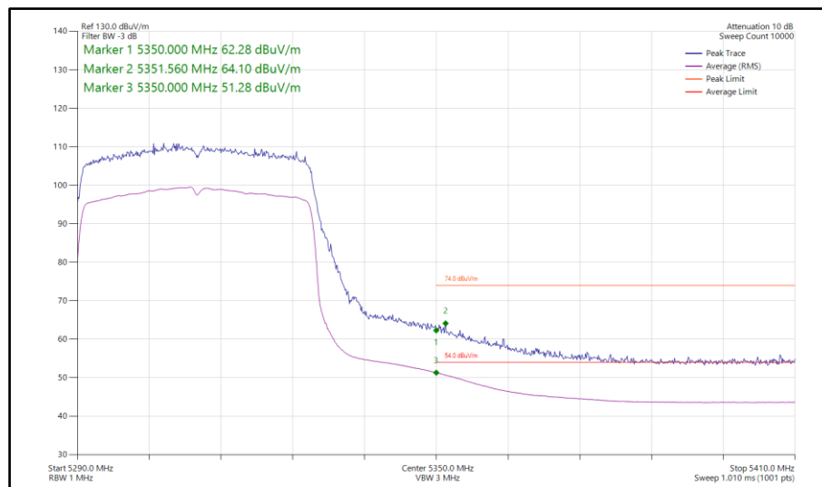
Figure 193 - 802.11ax HE40, SU, SDM, Core 0-1 - 5310 MHz Band Edge Frequency 5350 MHz
