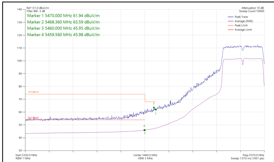
Figure 150 - 802.11n HT40, SISO, Core 1 - 5550 MHz Band Edge Frequency 5460 MHz
