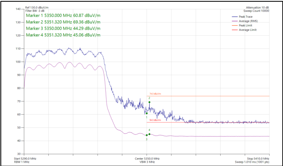
Figure 170 - 802.11ax HE40, SU, CDD, Core 0-1 - 5310 MHz Band Edge Frequency 5350 MHz
