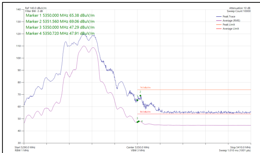
Figure 172 - 802.11be EHT40, RU106+26-85, CDD, Core 0-1 - 5310 MHz Band Edge Frequency 5350 MHz
