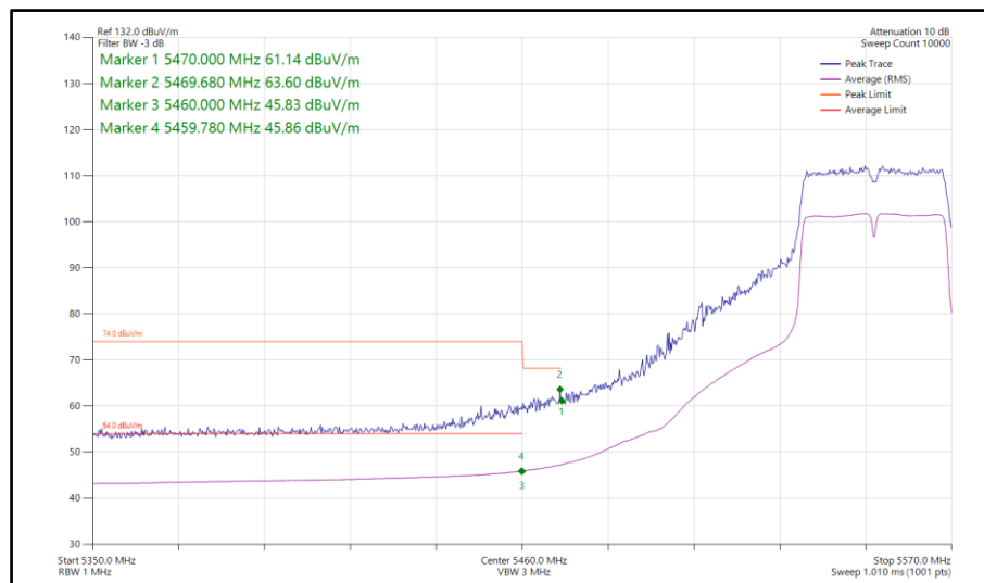
Figure 197 - 802.11n HT40, SDM, Core 0-1 - 5550 MHz Band Edge Frequency 5460 MHz
