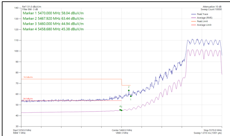
Figure 177 - 802.11n HT40, CDD, Core 0-1 - 5550 MHz Band Edge Frequency 5460 MHz
