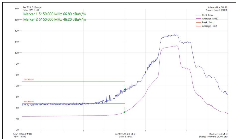
Figure 137 - 802.11be EHT40, RU106+26-82, SISO, Core 1 - 5190 MHz Band Edge Frequency 5150 MHz
