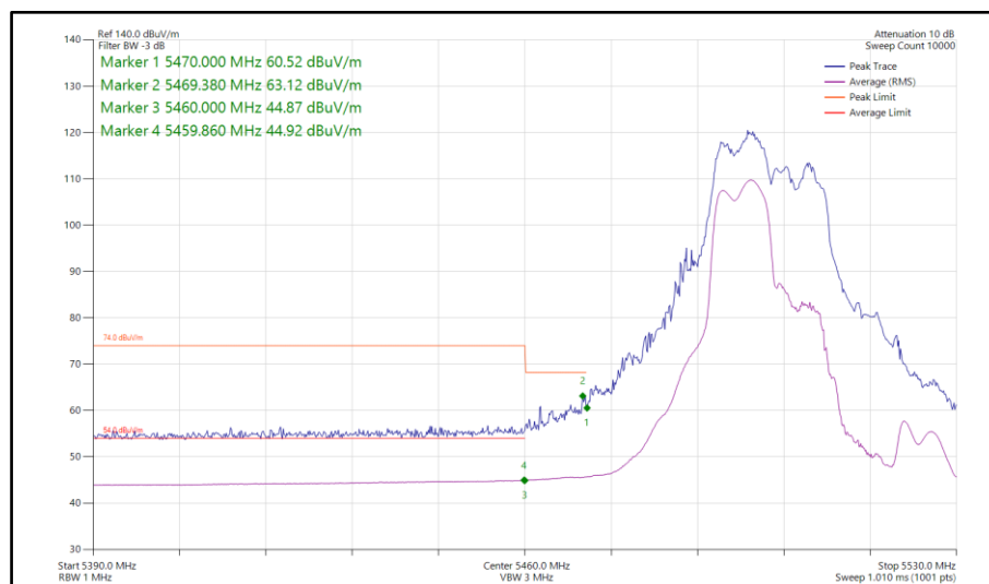
Figure 200 - 802.11ax HE40, RU106-53, SDM, Core 0-1 - 5510 MHz Band Edge Frequency 5460 MHz
