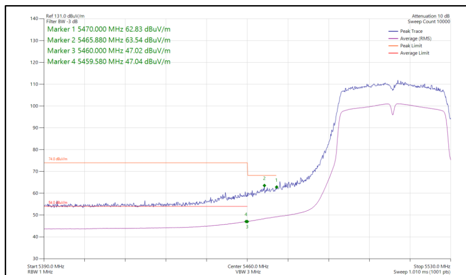
Figure 149 - 802.11n HT40, SISO, Core 1 - 5510 MHz Band Edge Frequency 5460 MHz
