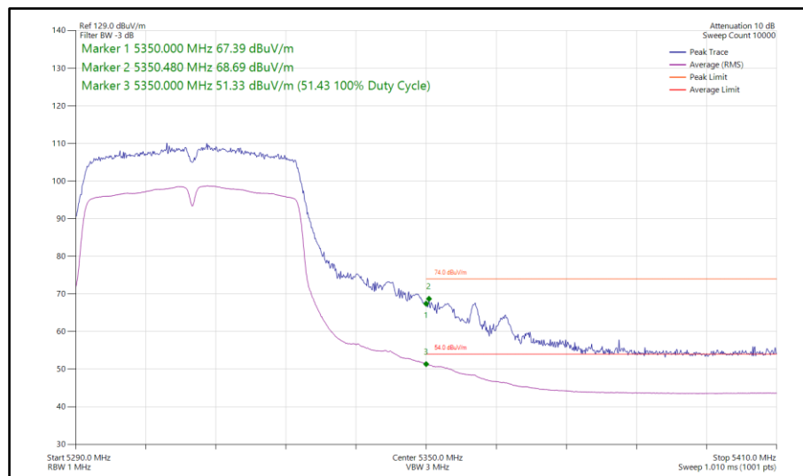
Figure 191 - 802.11n HT40, SDM, Core 0-1 - 5310 MHz Band Edge Frequency 5350 MHz
