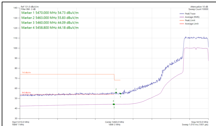
Figure 202 - 802.11ax HE40, SU, SDM, Core 0-1 - 5590 MHz Band Edge Frequency 5460 MHz
