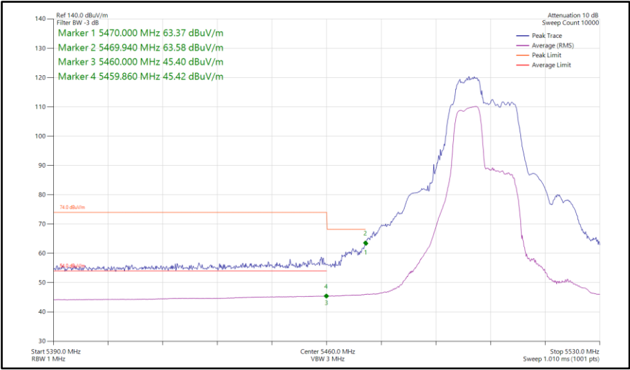
Figure 156 - 802.11be EHT40, RU52+26-70, SISO, Core 1 - 5510 MHz Band Edge Frequency 5460 MHz
