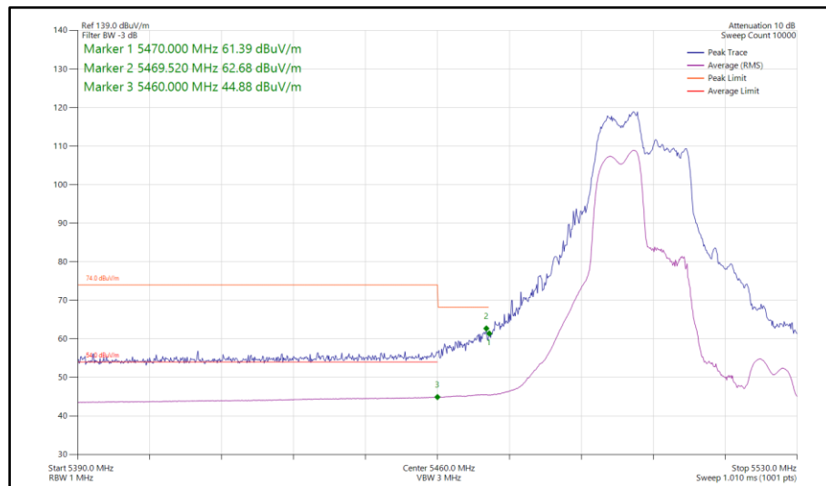
Figure 180 - 802.11ax HE40, RU106-53, CDD, Core 0-1 - 5510 MHz Band Edge Frequency 5460 MHz
