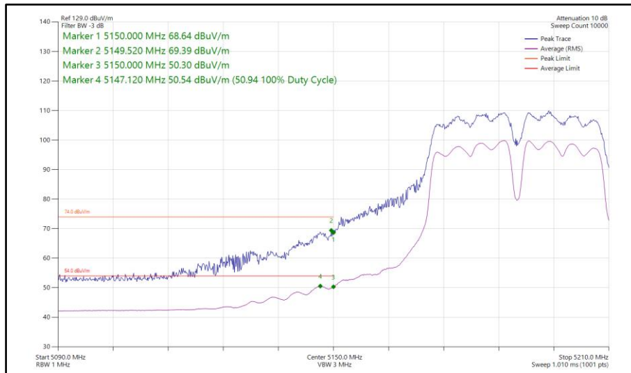
Figure 157 - 802.11a a40, CDD, Core 0-1 - 5190 MHz Band Edge Frequency 5150 MHz
