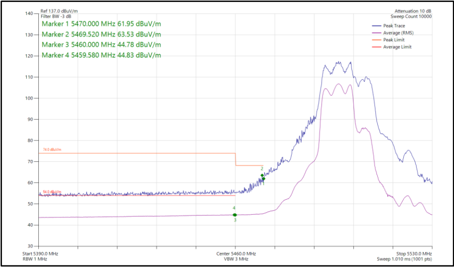
Figure 203 - 802.11be EHT40, RU106+26-82, SDM, Core 0-1 - 5510 MHz Band Edge Frequency 5460 MHz
