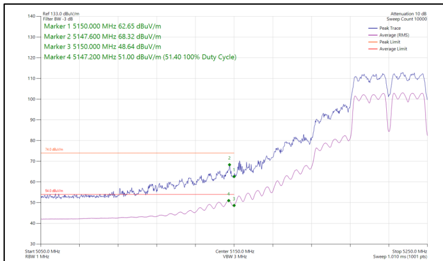
Figure 158 - 802.11a a40, CDD, Core 0-1 - 5230 MHz Band Edge Frequency 5150 MHz
