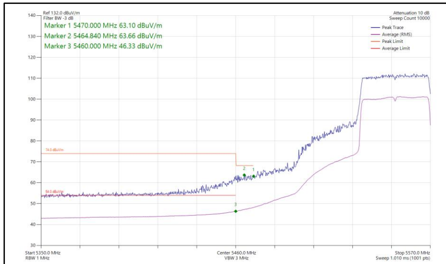
Figure 201 - 802.11ax HE40, SU, SDM, Core 0-1 - 5550 MHz Band Edge Frequency 5460 MHz
