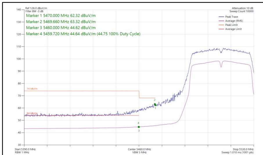
Figure 196 - 802.11n HT40, SDM, Core 0-1 - 5510 MHz Band Edge Frequency 5460 MHz
