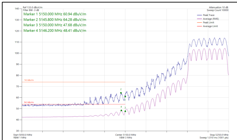
Figure 160 - 802.11n HT40, CDD, Core 0-1 - 5230 MHz Band Edge Frequency 5150 MHz
