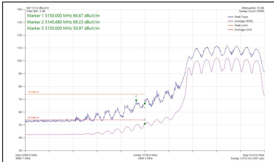
Figure 159 - 802.11n HT40, CDD, Core 0-1 - 5190 MHz Band Edge Frequency 5150 MHz
