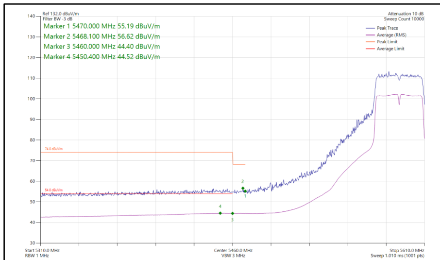
Figure 151 - 802.11n HT40, SISO, Core 1 - 5590 MHz Band Edge Frequency 5460 MHz
