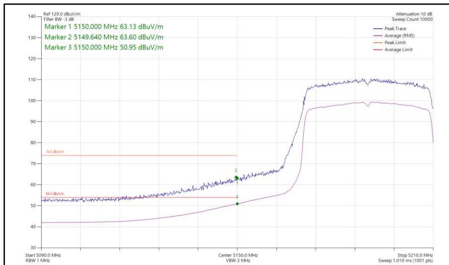
Figure 186 - 802.11ax HE40, SU, SDM, Core 0-1 - 5190 MHz Band Edge Frequency 5150 MHz
