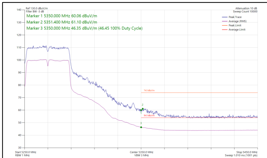
Figure 190 - 802.11n HT40, SDM, Core 0-1 - 5270 MHz Band Edge Frequency 5350 MHz
