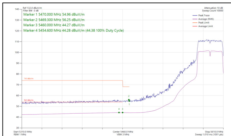
Figure 198 - 802.11n HT40, SDM, Core 0-1 - 5590 MHz Band Edge Frequency 5460 MHz
