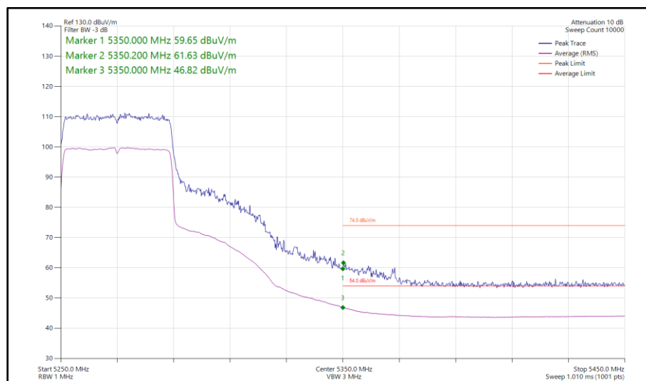
Figure 192 - 802.11ax HE40, SU, SDM, Core 0-1 - 5270 MHz Band Edge Frequency 5350 MHz
