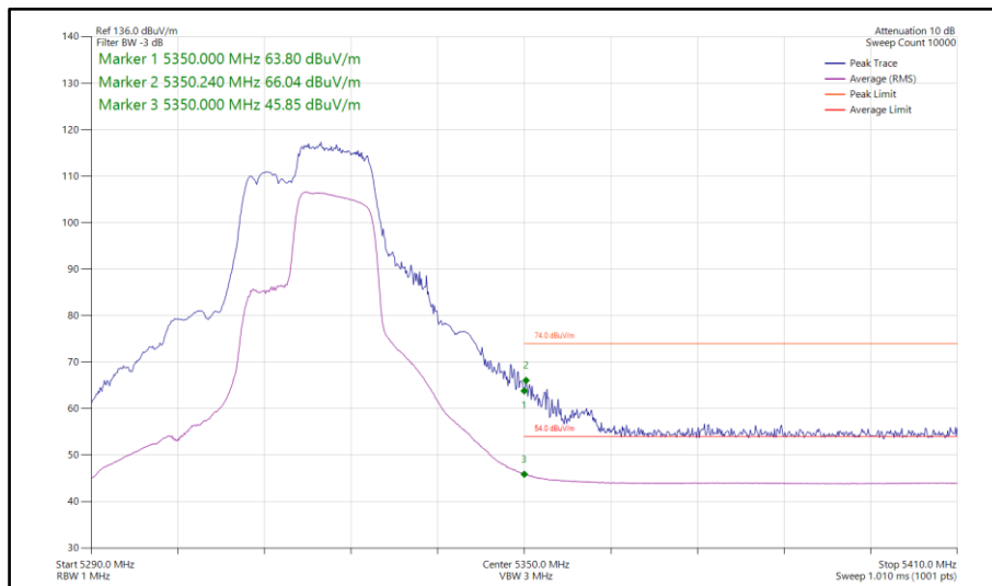
Figure 145 - 802.11be EHT40, RU106+26-85, SISO, Core 1 - 5310 MHz Band Edge Frequency 5350 MHz
