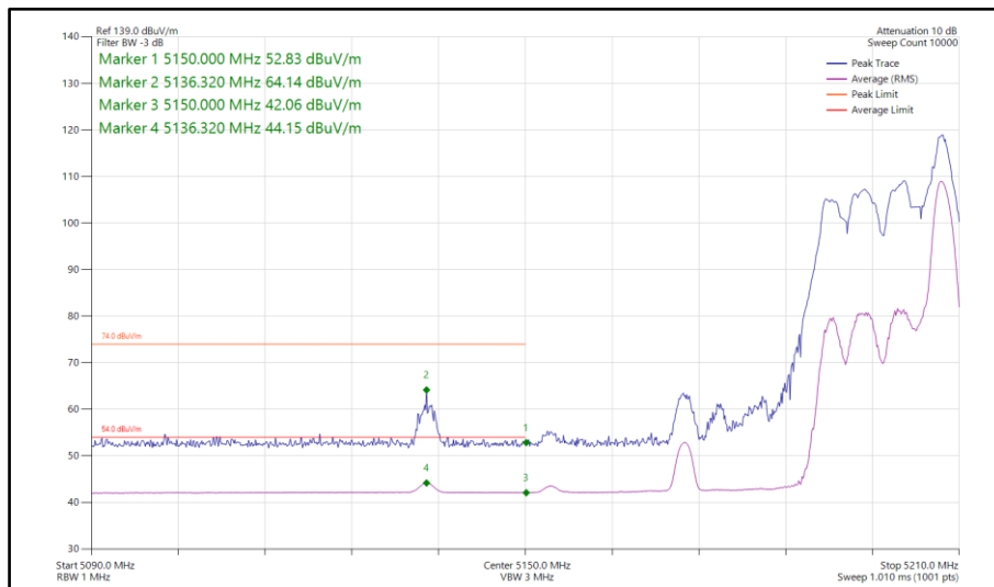
Figure 162 - 802.11ax HE40, RU26-17, CDD, Core 0-1 - 5190 MHz Band Edge Frequency 5150 MHz
