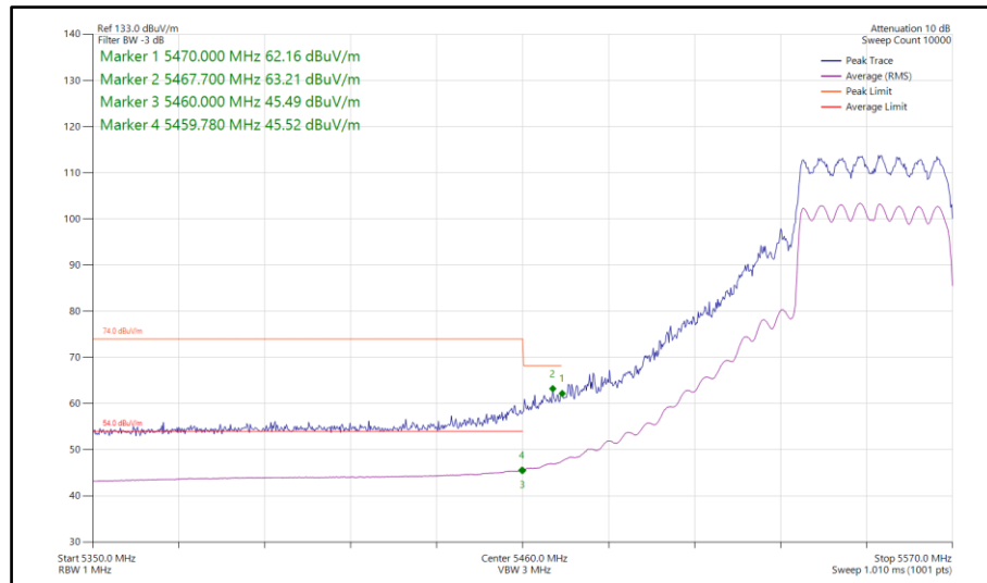
Figure 181 - 802.11ax HE40, SU, CDD, Core 0-1 - 5550 MHz Band Edge Frequency 5460 MHz
