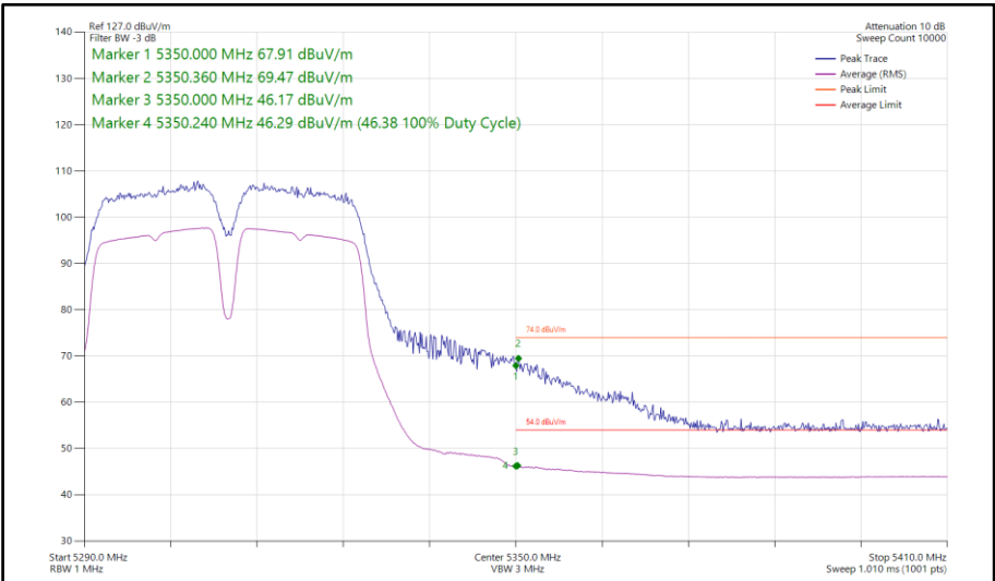
Figure 139 - 802.11a a40, SISO, Core 1 - 5310 MHz Band Edge Frequency 5350 MHz
