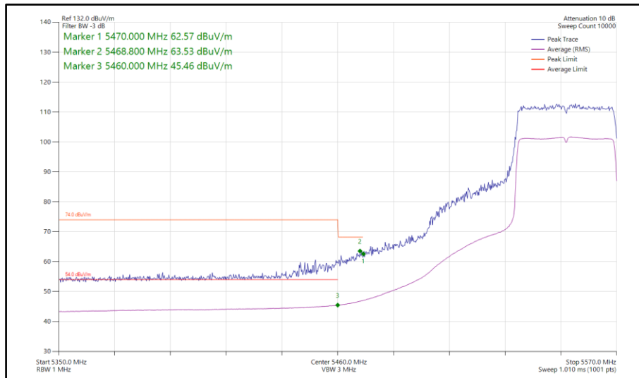
Figure 154 - 802.11ax HE40, SU, SISO, Core 1 - 5550 MHz Band Edge Frequency 5460 MHz
