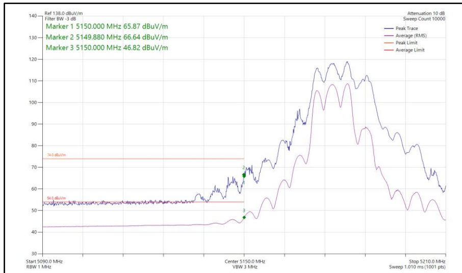
Figure 189 - 802.11be EHT40, RU106+26-82, SDM, Core 0-1 - 5190 MHz Band Edge Frequency 5150 MHz
