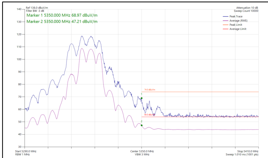
Figure 195 - 802.11be EHT40, RU106+26-85, SDM, Core 0-1 - 5310 MHz Band Edge Frequency 5350 MHz
