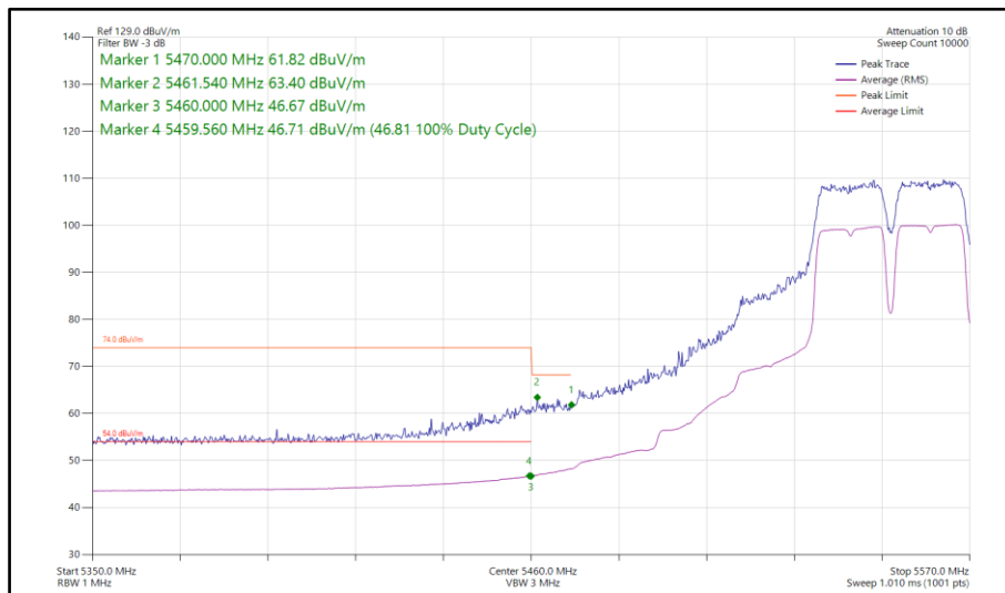
Figure 147 - 802.11a a40, SISO, Core 1 - 5550 MHz Band Edge Frequency 5460 MHz
