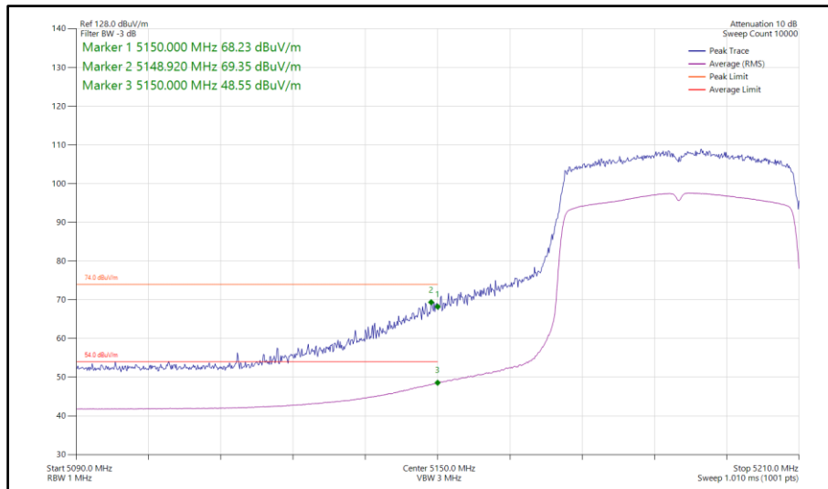
Figure 134 - 802.11ax HE40, SU, SISO, Core 1 - 5190 MHz Band Edge Frequency 5150 MHz
