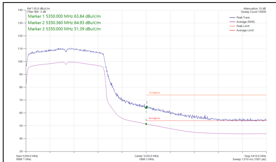
Figure 143 - 802.11ax HE40, SU, SISO, Core 1 - 5310 MHz Band Edge Frequency 5350 MHz
