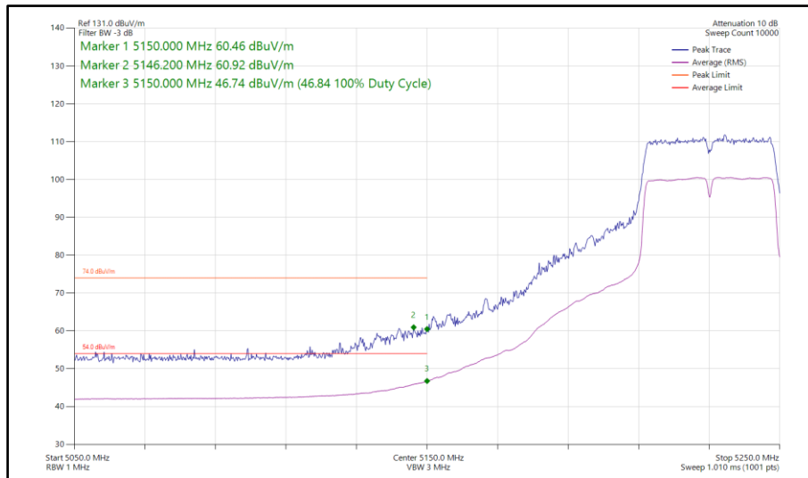
Figure 185 - 802.11n HT40, SDM, Core 0-1 - 5230 MHz Band Edge Frequency 5150 MHz
