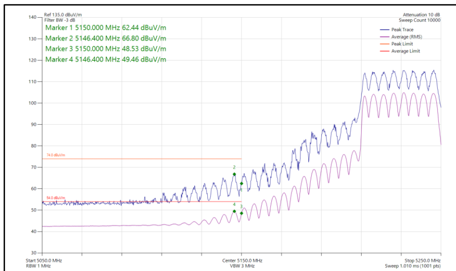
Figure 163 - 802.11ax HE40, SU, CDD, Core 0-1 - 5230 MHz Band Edge Frequency 5150 MHz
