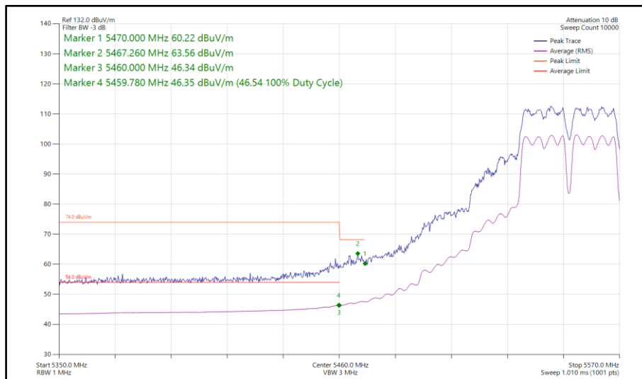
Figure 174 - 802.11a a40, CDD, Core 0-1 - 5550 MHz Band Edge Frequency 5460 MHz
