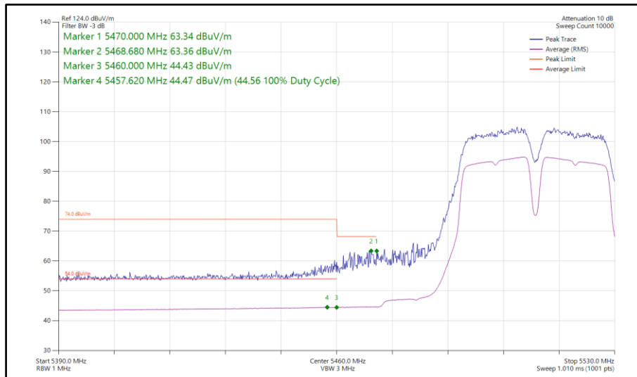
Figure 146 - 802.11a a40, SISO, Core 1 - 5510 MHz Band Edge Frequency 5460 MHz
