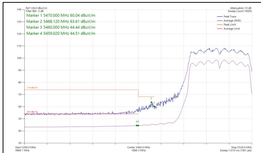
Figure 176 - 802.11n HT40, CDD, Core 0-1 - 5510 MHz Band Edge Frequency 5460 MHz
