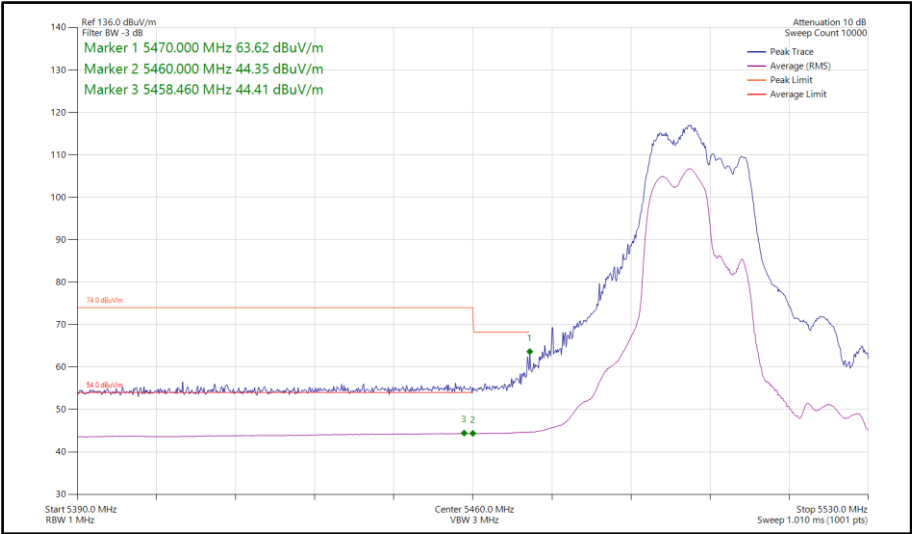
Figure 183 - 802.11be EHT40, RU106+26-82, CDD, Core 0-1 - 5510 MHz Band Edge Frequency 5460 MHz
