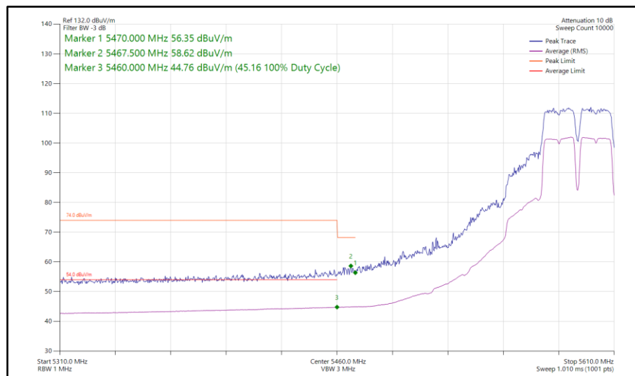
Figure 148 - 802.11a a40, SISO, Core 1 - 5590 MHz Band Edge Frequency 5460 MHz
