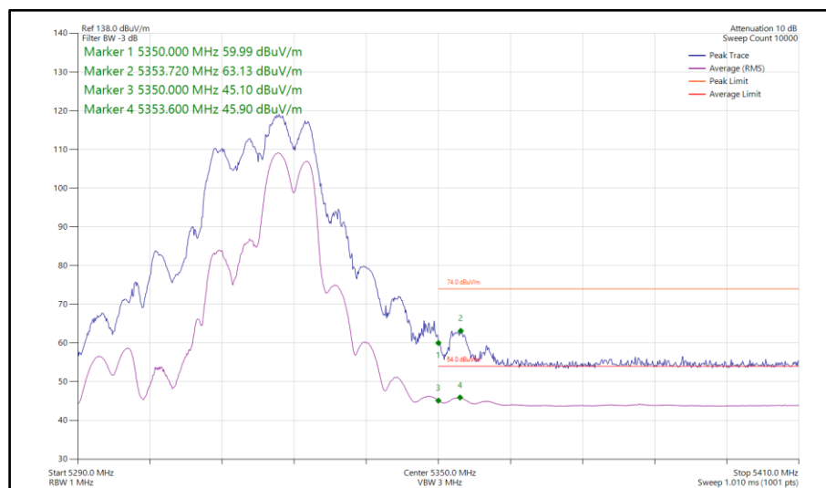
Figure 194 - 802.11ax HE40, RU106-56, SDM, Core 0-1 - 5310 MHz Band Edge Frequency 5350 MHz
