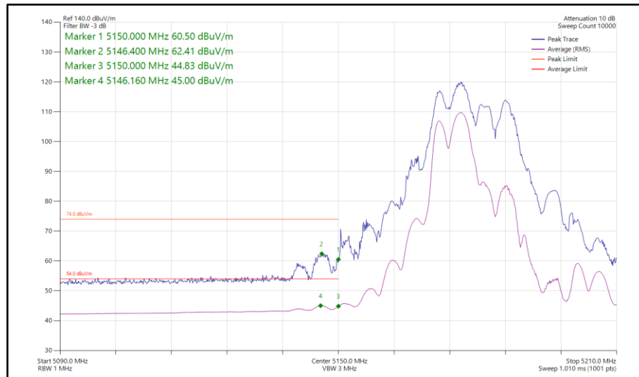
Figure 187 - 802.11ax HE40, RU106-53, SDM, Core 0-1 - 5190 MHz Band Edge Frequency 5150 MHz
