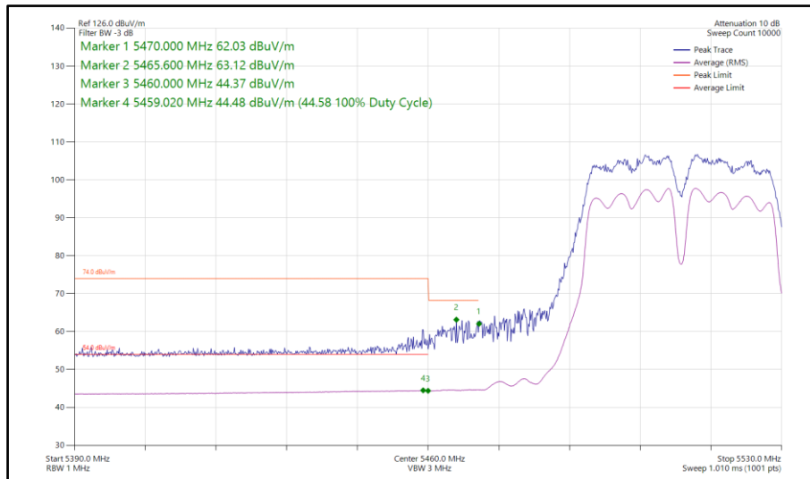
Figure 173 - 802.11a a40, CDD, Core 0-1 - 5510 MHz Band Edge Frequency 5460 MHz
