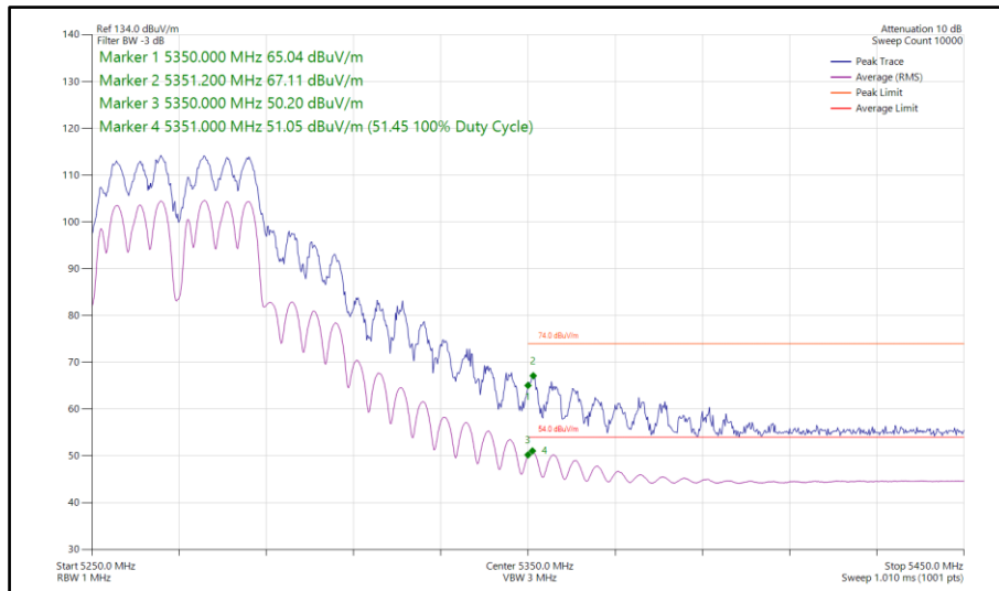
Figure 165 - 802.11a a40, CDD, Core 0-1 - 5270 MHz Band Edge Frequency 5350 MHz
