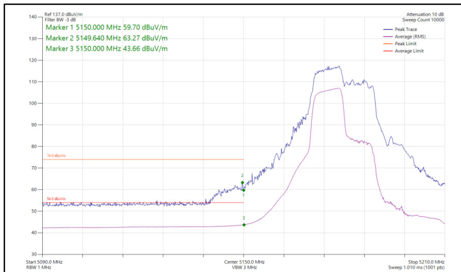
Figure 135 - 802.11ax HE40, RU106-53, SISO, Core 1 - 5190 MHz Band Edge Frequency 5150 MHz
