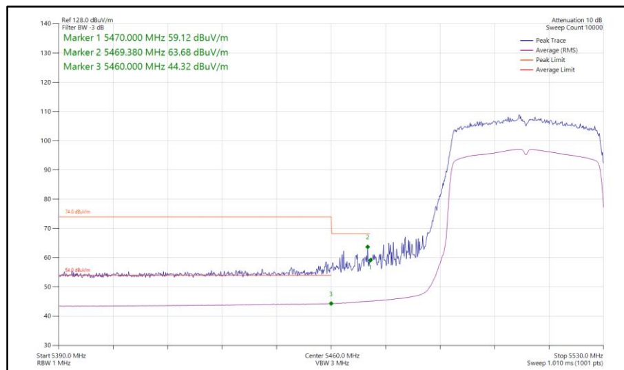
Figure 152 - 802.11ax HE40, SU, SISO, Core 1 - 5510 MHz Band Edge Frequency 5460 MHz
