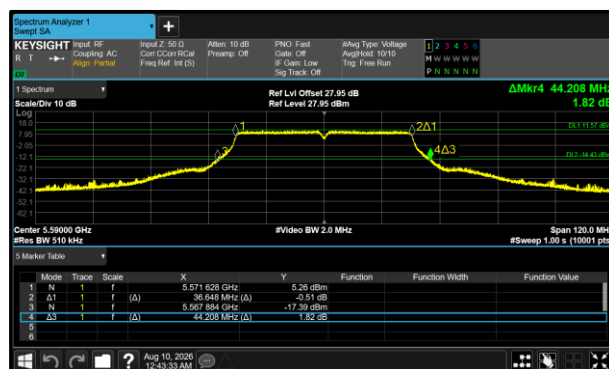
Figure 347 - 802.11n HT40 Maximum 99% OBW
