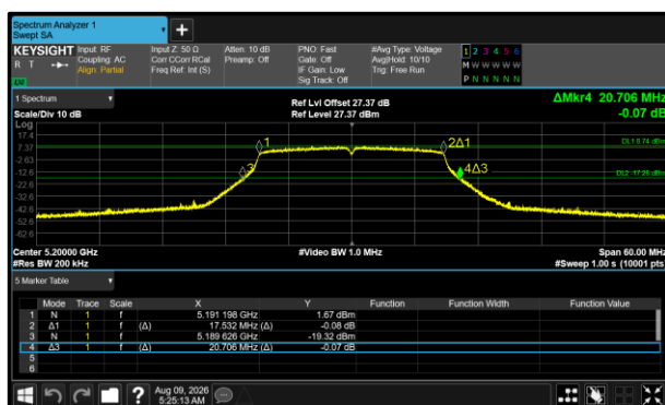
Figure 344 - 802.11n HT20 Minimum 99% OBW
