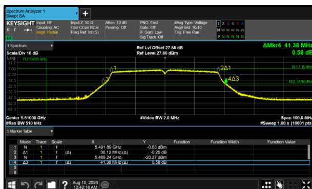
Figure 346 - 802.11n HT40 Minimum 99% OBW
