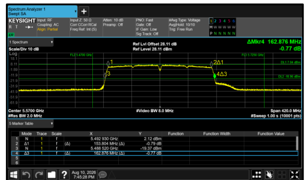
Figure 351 - 802.11ac VHT160 Maximum 99% OBW
