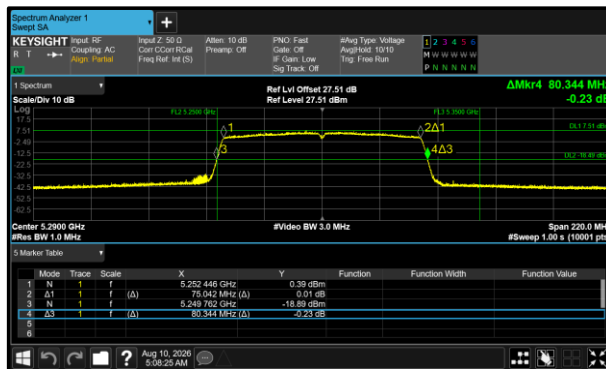
Figure 348 - 802.11ac VHT80 Minimum 99% OBW
