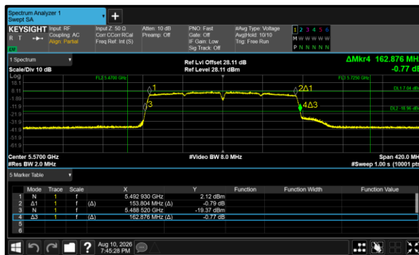
Figure 350 - 802.11ac VHT160 Minimum 99% OBW
