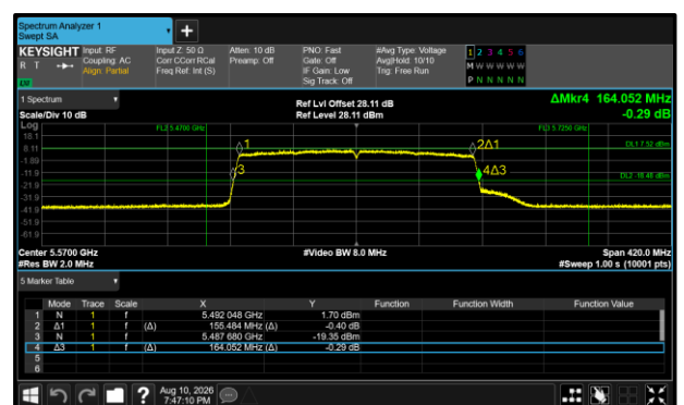
Figure 359 - 802.11ax HE160 SU Maximum 99% OBW
