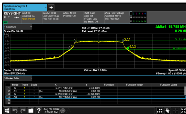
Figure 360 - 802.11a20 Minimum 99% OBW
