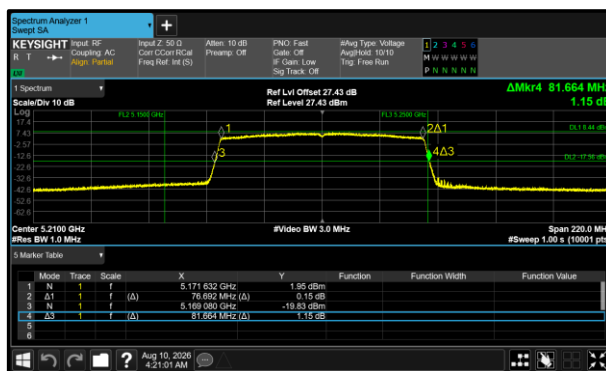
Figure 356 - 802.11ax HE80 SU Minimum 99% OBW
