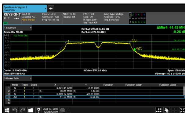
Figure 362 - 802.11a40 Minimum 99% OBW
