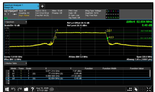
Figure 357 - 802.11ax HE80 SU Maximum 99% OBW
