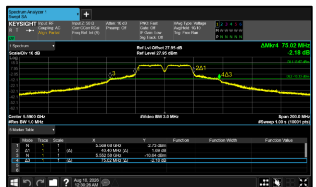
Figure 363 - 802.11a40 Maximum 99% OBW
