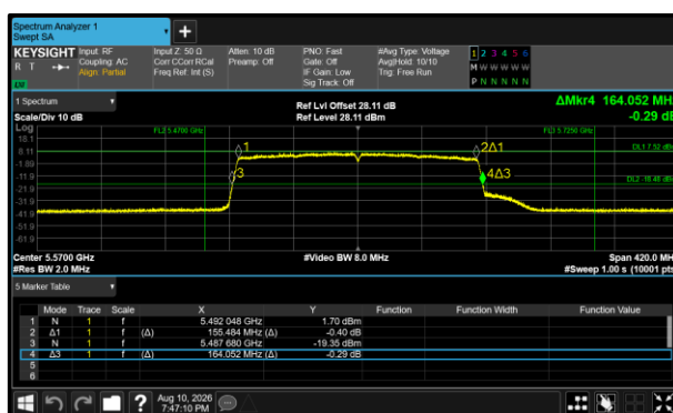
Figure 358 - 802.11ax HE160 SU Minimum 99% OBW
