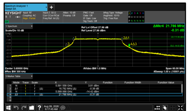
Figure 361 - 802.11a20 Maximum 99% OBW
