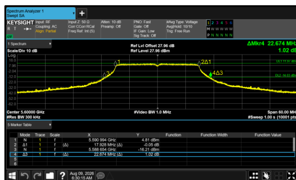
Figure 345 - 802.11n HT20 Maximum 99% OBW
