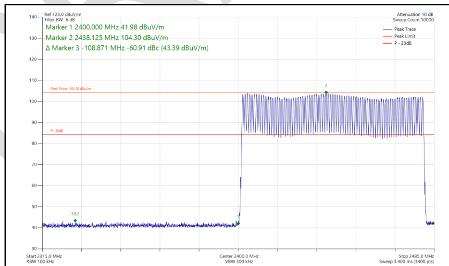
Figure 97 - Bluetooth DH5, SISO, Core 0 - 2402-2480 MHz Band Edge Frequency 2400 MHz
