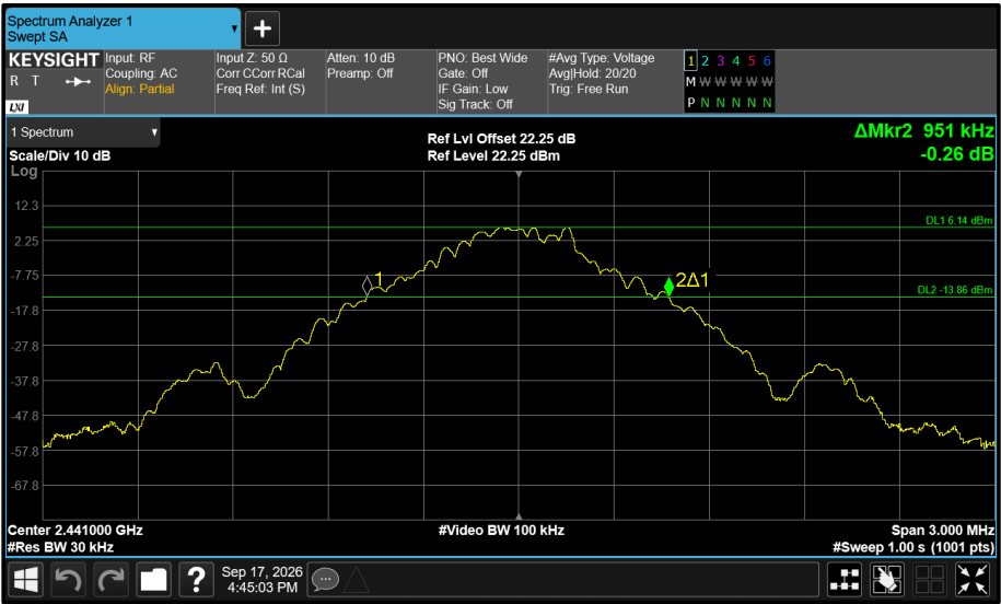
Figure 87 - Core 1 (B) 2441 MHz (CH39) 20 dB Bandwidth
