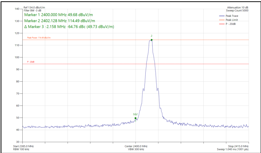
Figure 104 - Bluetooth DH5, SISO, Core 0 - 2402 MHz Band Edge Frequency 2400 MHz
