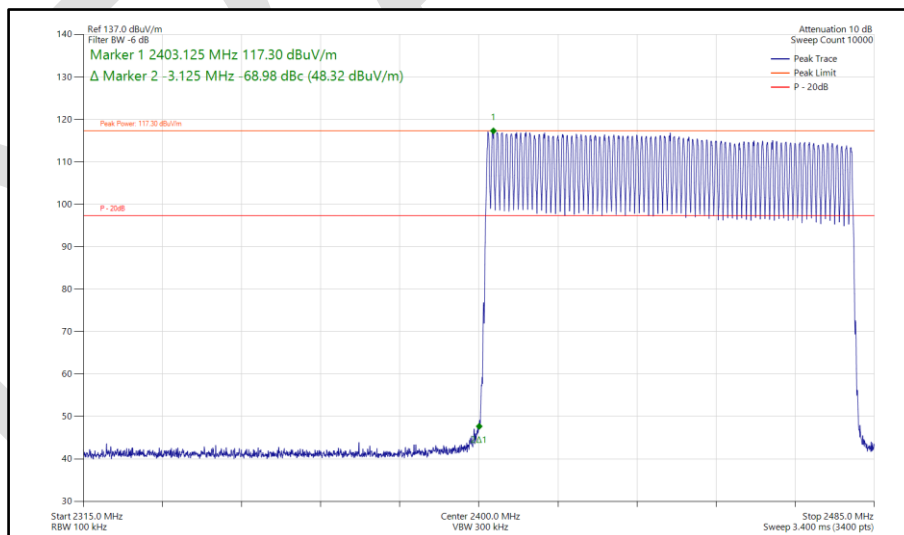
Figure 107 - Bluetooth DH5, SISO, Core 1 - 2402-2480 MHz Band Edge Frequency 2400 MHz
