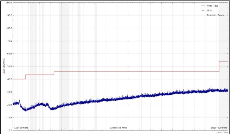
Figure 123 - 2441 MHz (CH2441), DH5, iPA, Core 2, 30 MHz to 1 GHz, Vertical (Peak)
