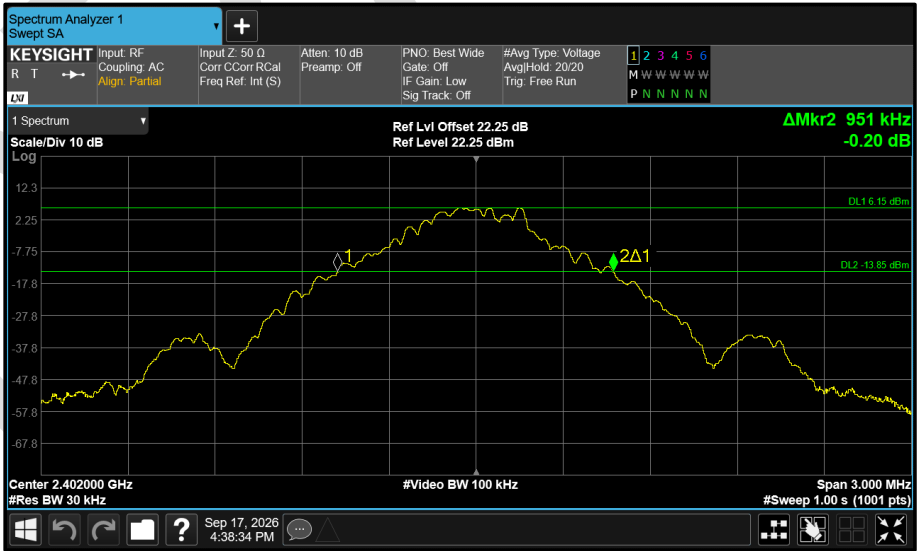
Figure 84 - Core 0 (A) 2402 MHz (CH0) 20 dB Bandwidth
