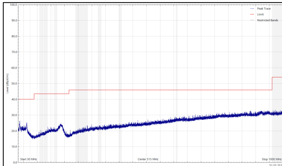
Figure 131 - 2441 MHz (CH2441), DH5, ePA, Core 0 + Core 1, 30 MHz to 1 GHz, Vertical (Peak)
