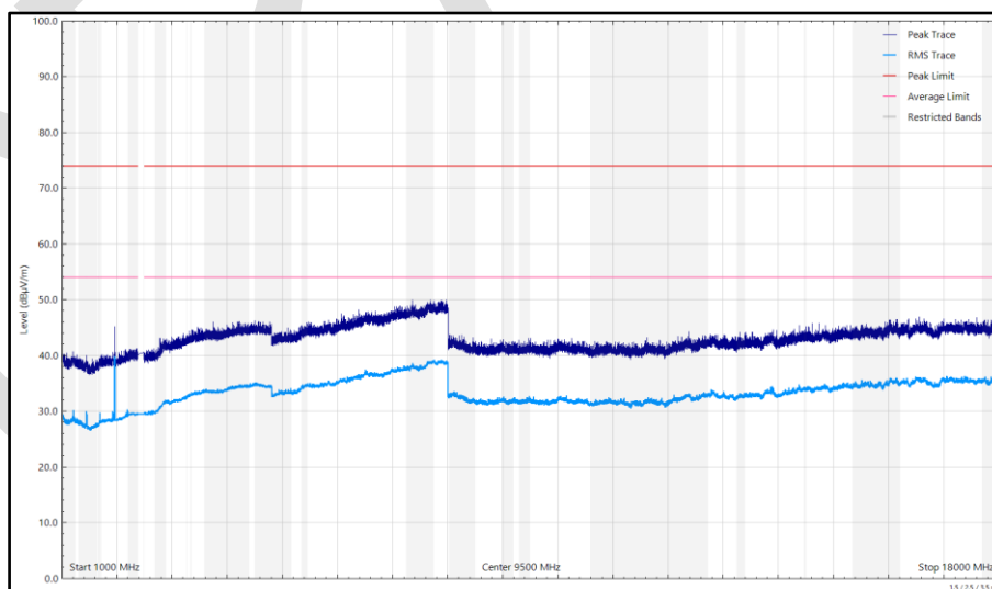
Figure 112 - 2402 MHz (CH2402), DH5, iPA, Core 0 + Core 1, 1 GHz to 18 GHz, Vertical
