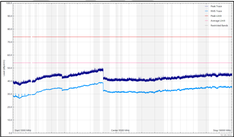
Figure 120 - 2402 MHz (CH2402), DH5, iPA, Core 2, 1 GHz to 18 GHz, Vertical
