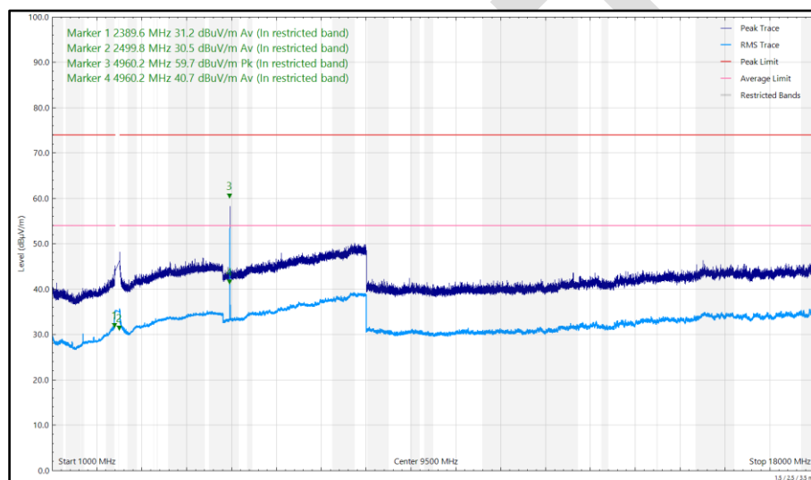
Figure 133 - 2480 MHz (CH2480), DH5, ePA, Core 0 + Core 1, 1 GHz to 18 GHz, Horizontal
