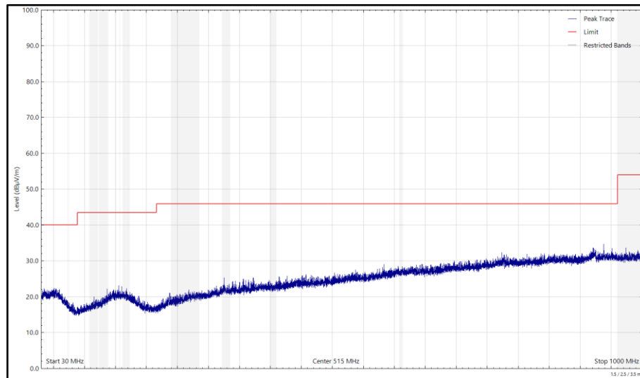
Figure 121 - 2441 MHz (CH2441), DH5, iPA, Core 2, 30 MHz to 1 GHz, Horizontal (Peak)
