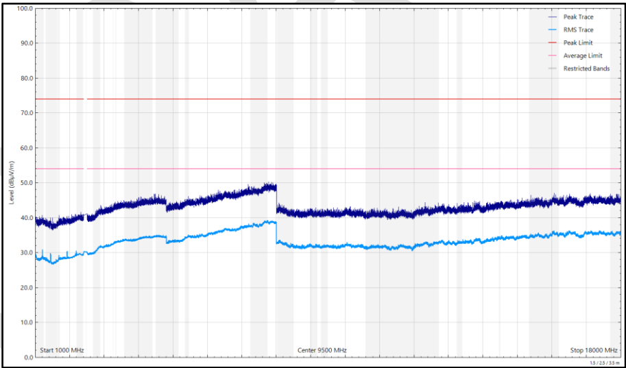
Figure 126 - 2480 MHz (CH2480), DH5, iPA, Core 2, 1 GHz to 18 GHz, Vertical
