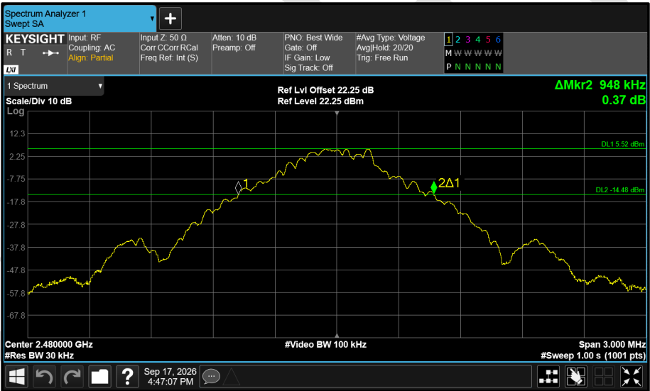
Figure 88 - Core 0 (A) 2480 MHz (CH78) 20 dB Bandwidth
