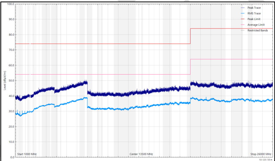
Figure 124 - 2441 MHz (CH2441), DH5, iPA, Core 2, 1 GHz to 26 GHz, Vertical
