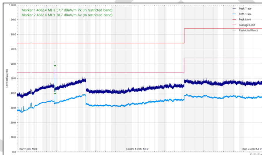
Figure 132 - 2441 MHz (CH2441), DH5, ePA, Core 0 + Core 1, 1 GHz to 26 GHz, Vertical
