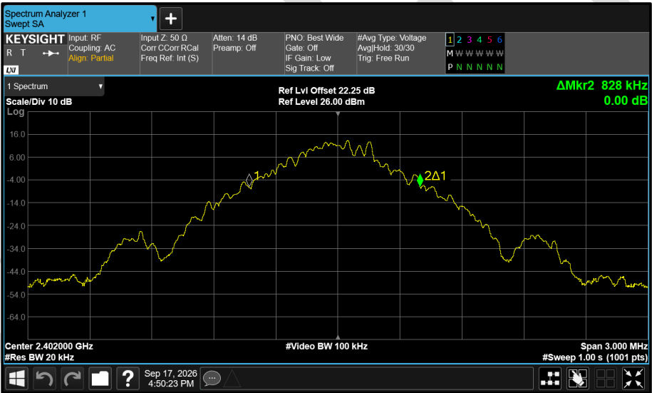
Figure 78 - Core 0 (A) 2402 MHz (CH0) 99% Bandwidth
