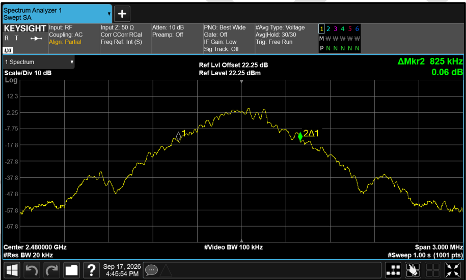
Figure 94 - Core 0 (A) 2480 MHz (CH78) 99% Bandwidth
