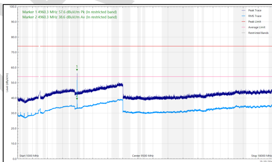
Figure 134 - 2480 MHz (CH2480), DH5, ePA, Core 0 + Core 1, 1 GHz to 18 GHz, Vertical
