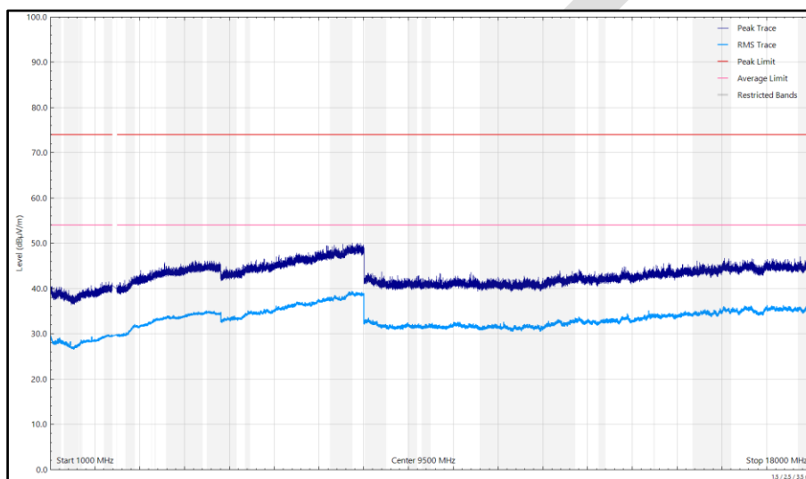
Figure 111 - 2402 MHz (CH2402), DH5, iPA, Core 0 + Core 1, 1 GHz to 18 GHz, Horizontal
