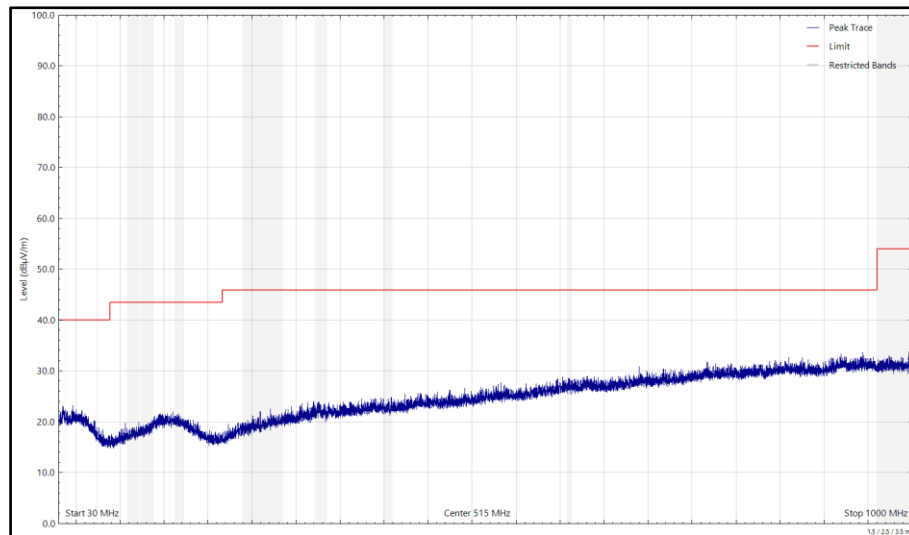
Figure 113 - 2441 MHz (CH2441), DH5, iPA, Core 0 + Core 1, 30 MHz to 1 GHz, Horizontal (Peak)
