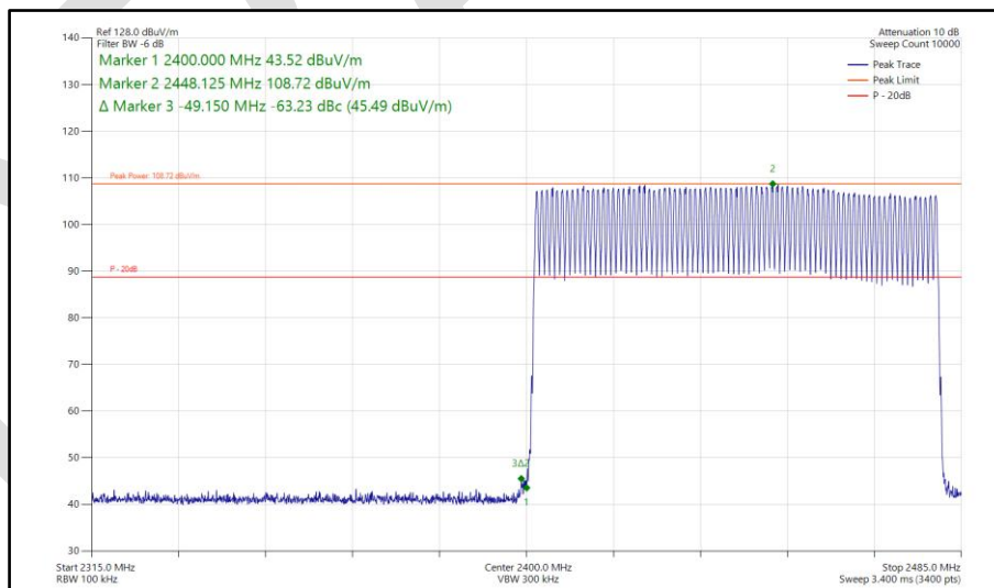
Figure 101 - Bluetooth DH5, SISO, Core 2 - 2402-2480 MHz Band Edge Frequency 2400 MHz
