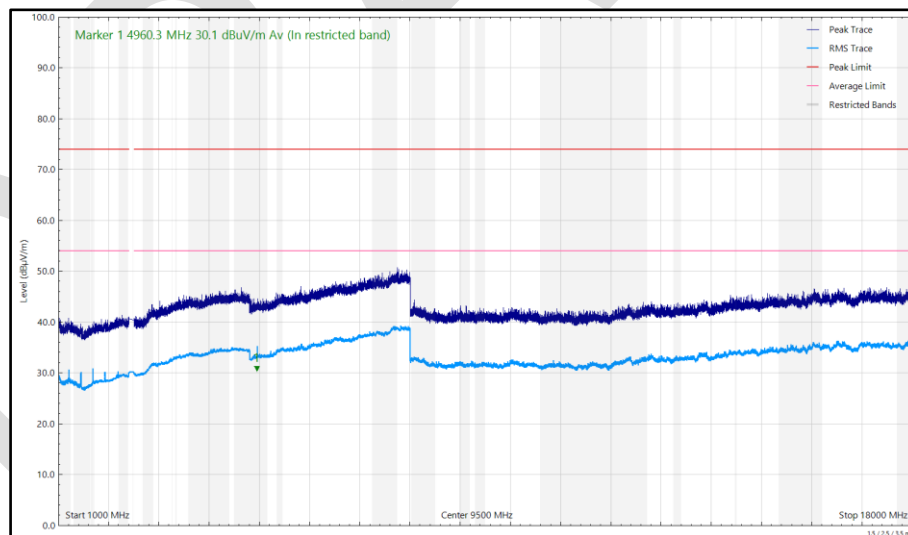
Figure 118 - 2480 MHz (CH2480), DH5, iPA, Core 0 + Core 1, 1 GHz to 18 GHz, Vertical
