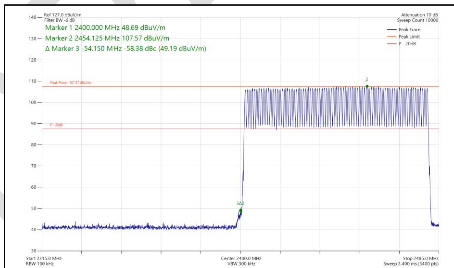
Figure 103 - Bluetooth DH5, MIMO, Core 0-1 - 2402-2480 MHz Band Edge Frequency 2400 MHz
