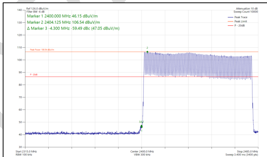
Figure 99 - Bluetooth DH5, SISO, Core 1 - 2402-2480 MHz Band Edge Frequency 2400 MHz
