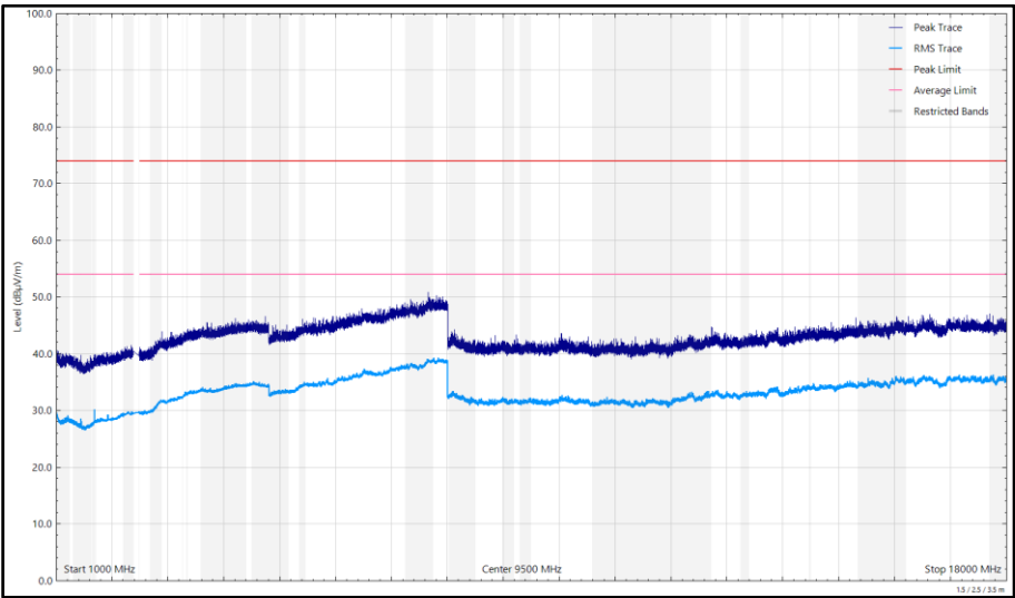
Figure 119 - 2402 MHz (CH2402), DH5, iPA, Core 2, 1 GHz to 18 GHz, Horizontal
