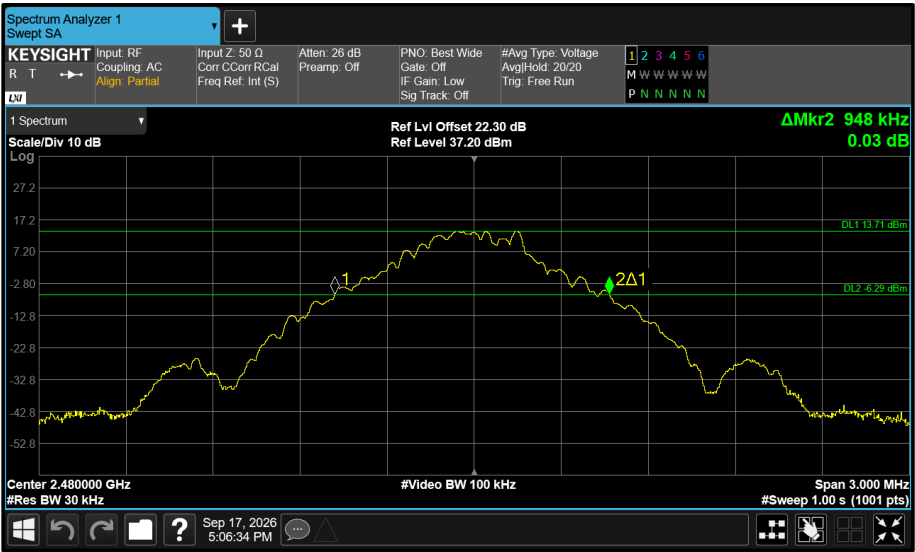
Figure 77 - Core 1 (B) 2480 MHz (CH78) 20 dB Bandwidth
