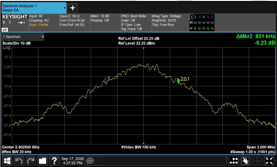
Figure 90 - Core 0 (A) 2402 MHz (CH0) 99% Bandwidth
