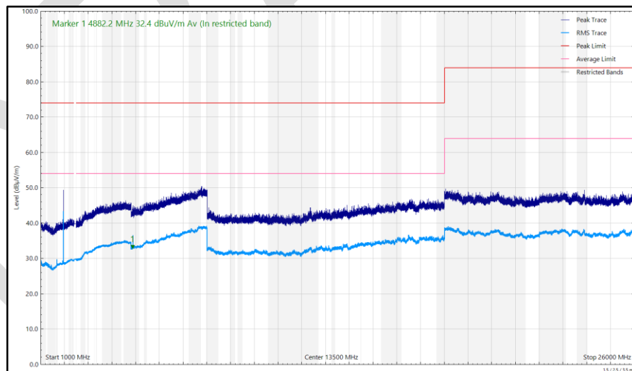
Figure 114 - 2441 MHz (CH2441), DH5, iPA, Core 0 + Core 1, 1 GHz to 26 GHz, Horizontal
