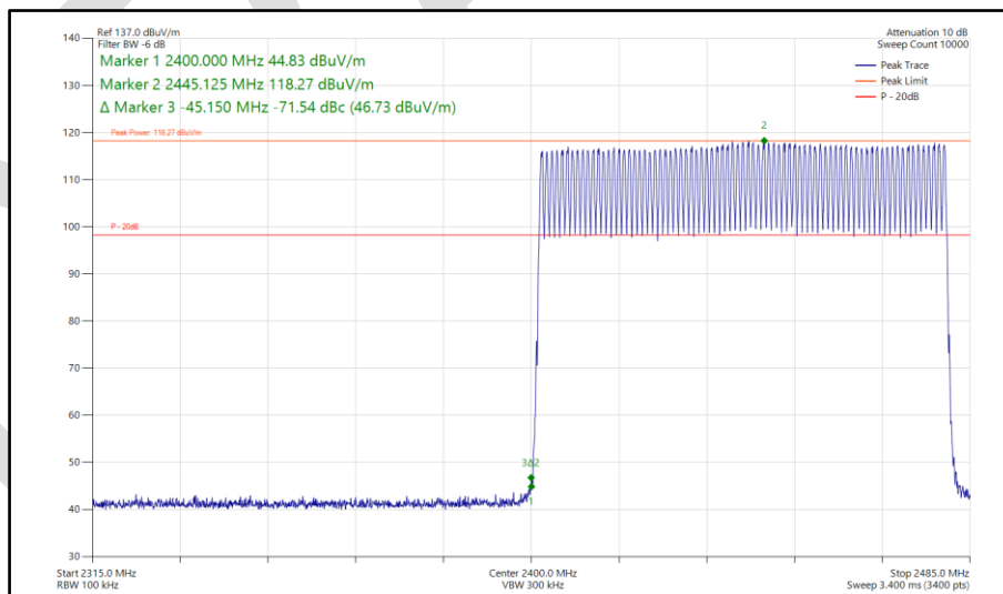
Figure 109 - Bluetooth DH5, MIMO, Core 0-1 - 2402-2480 MHz Band Edge Frequency 2400 MHz
