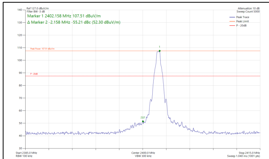
Figure 98 - Bluetooth DH5, SISO, Core 1 - 2402 MHz Band Edge Frequency 2400 MHz
