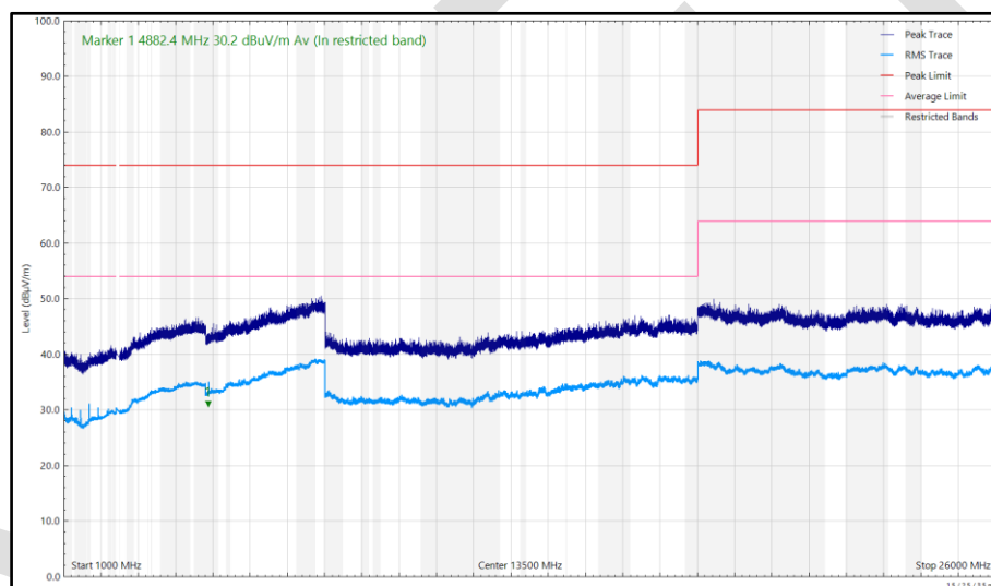
Figure 116 - 2441 MHz (CH2441), DH5, iPA, Core 0 + Core 1, 1 GHz to 26 GHz, Vertical
