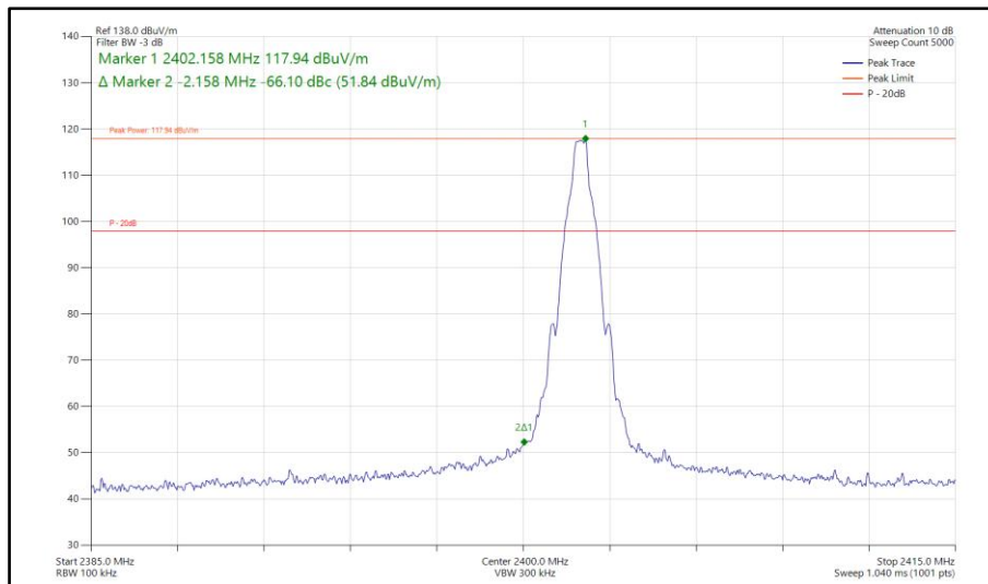
Figure 106 - Bluetooth DH5, SISO, Core 1 - 2402 MHz Band Edge Frequency 2400 MHz
