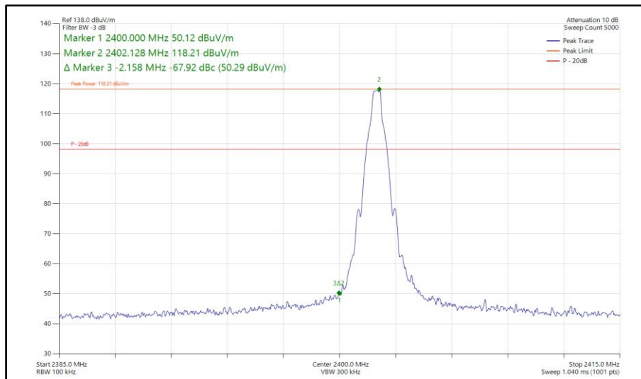
Figure 108 - Bluetooth DH5, MIMO, Core 0-1 - 2402 MHz Band Edge Frequency 2400 MHz
