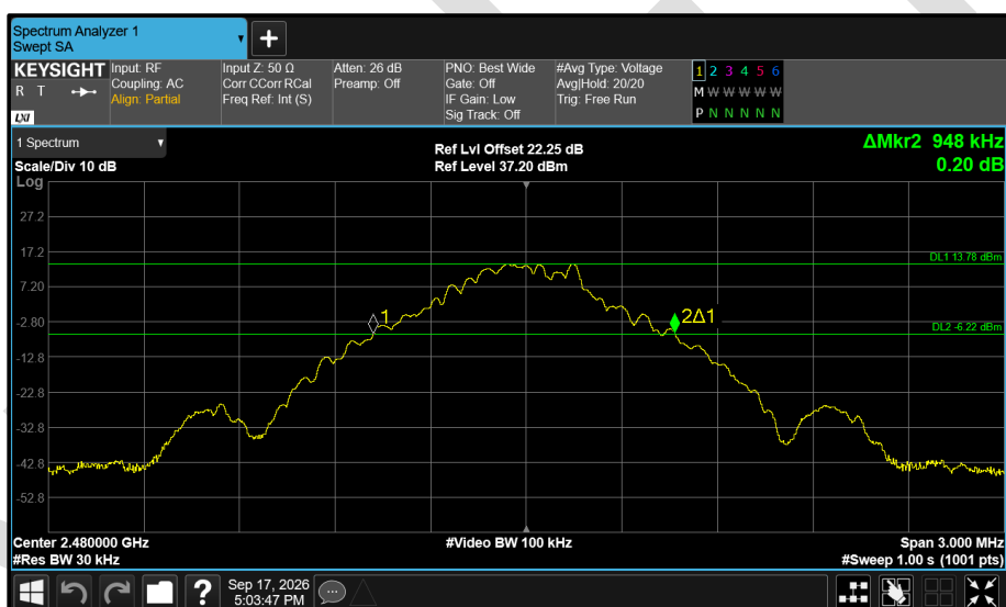
Figure 76 - Core 0 (A) 2480 MHz (CH78) 20 dB Bandwidth
