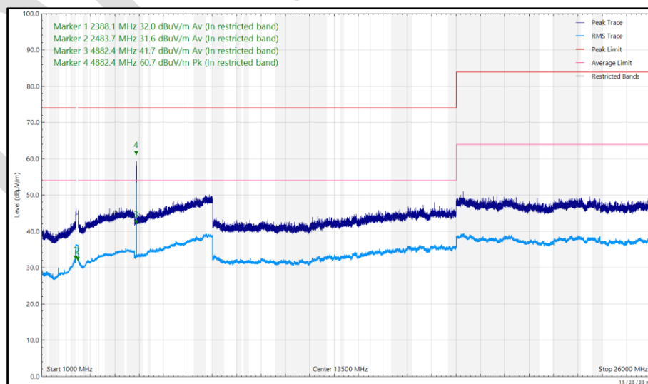
Figure 130 - 2441 MHz (CH2441), DH5, ePA, Core 0 + Core 1, 1 GHz to 26 GHz, Horizontal
