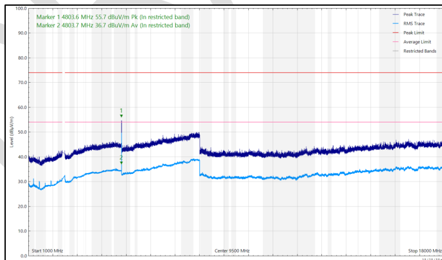
Figure 128 - 2402 MHz (CH2402), DH5, ePA, Core 0 + Core 1, 1 GHz to 18 GHz, Vertical
