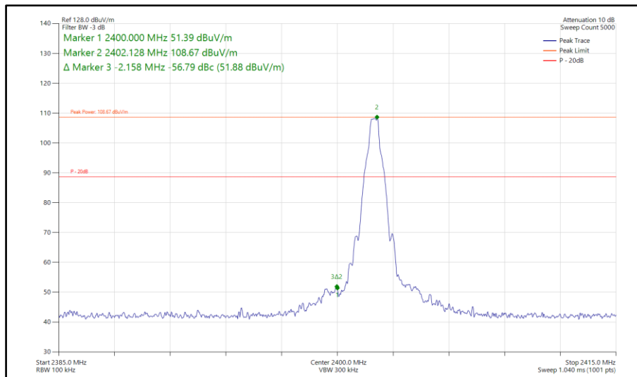
Figure 100 - Bluetooth DH5, SISO, Core 2 - 2402 MHz Band Edge Frequency 2400 MHz
