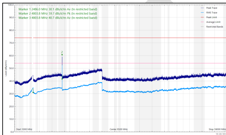
Figure 127 - 2402 MHz (CH2402), DH5, ePA, Core 0 + Core 1, 1 GHz to 18 GHz, Horizontal
