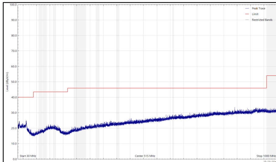
Figure 115 - 2441 MHz (CH2441), DH5, iPA, Core 0 + Core 1, 30 MHz to 1 GHz, Vertical (Peak)
