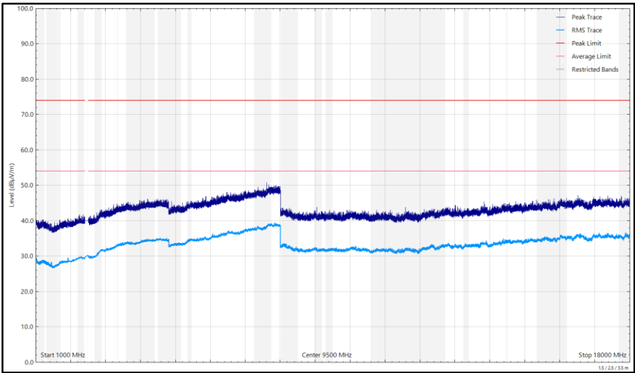
Figure 125 - 2480 MHz (CH2480), DH5, iPA, Core 2, 1 GHz to 18 GHz, Horizontal
