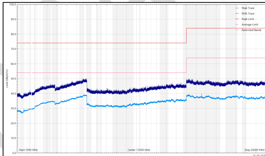
Figure 122 - 2441 MHz (CH2441), DH5, iPA, Core 2, 1 GHz to 26 GHz, Horizontal
