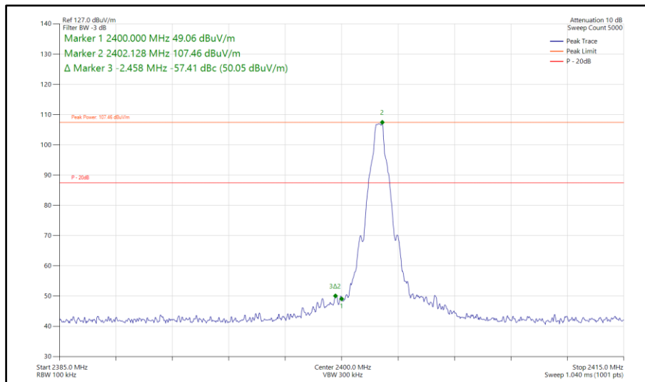
Figure 102 - Bluetooth DH5, MIMO, Core 0-1 - 2402 MHz Band Edge Frequency 2400 MHz
