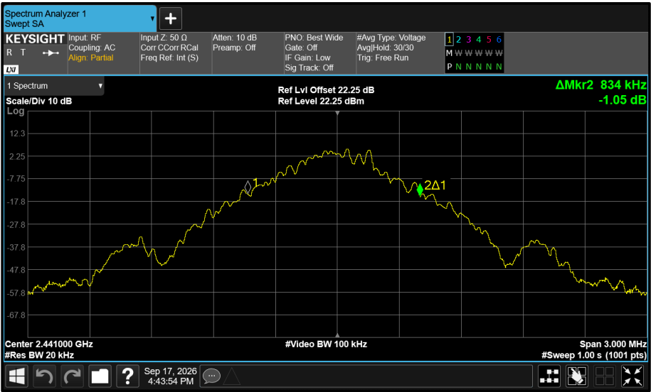
Figure 93 - Core 1 (B) 2441 MHz (CH39) 99% Bandwidth
