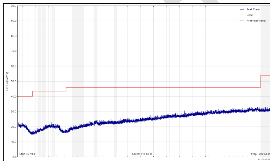
Figure 129 - 2441 MHz (CH2441), DH5, ePA, Core 0 + Core 1, 30 MHz to 1 GHz, Horizontal (Peak)
