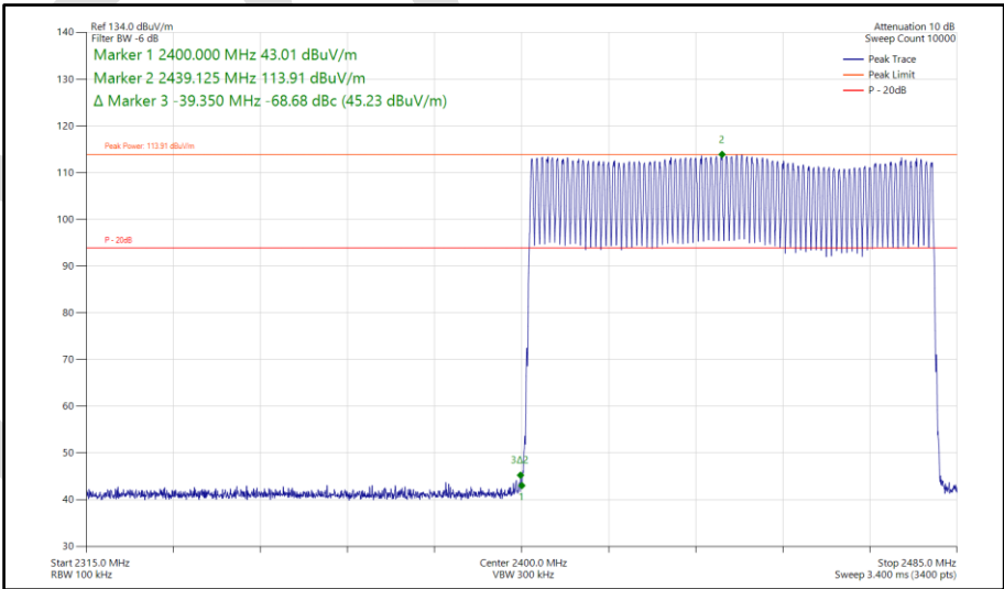
Figure 105 - Bluetooth DH5, SISO, Core 0 - 2402-2480 MHz Band Edge Frequency 2400 MHz
