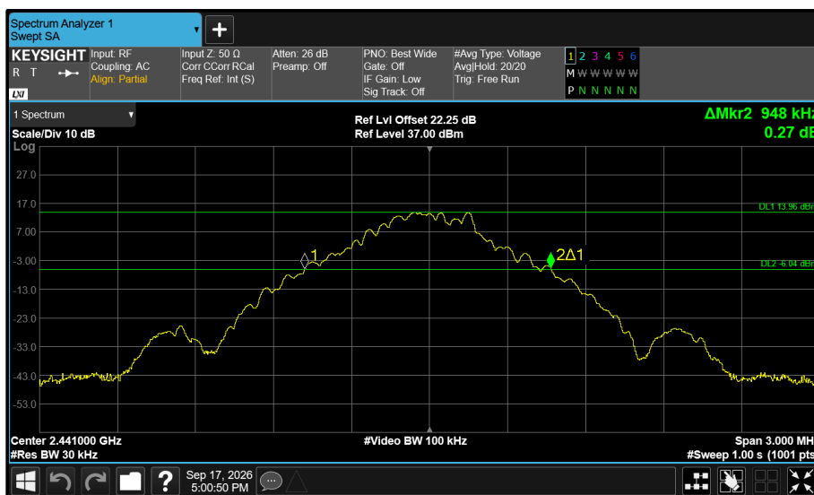
Figure 75 - Core 1 (B) 2441 MHz (CH39) 20 dB Bandwidth
