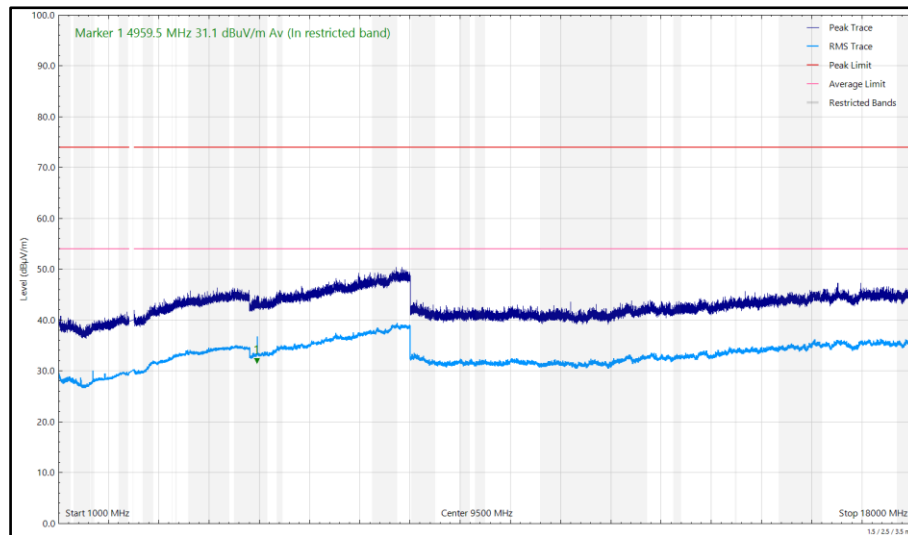
Figure 117 - 2480 MHz (CH2480), DH5, iPA, Core 0 + Core 1, 1 GHz to 18 GHz, Horizontal
