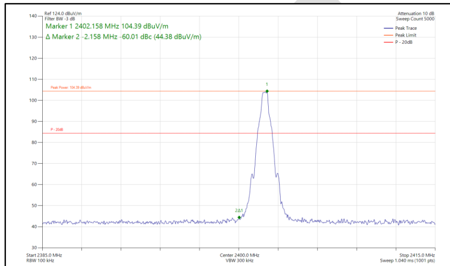
Figure 96 - Bluetooth DH5, SISO, Core 0 - 2402 MHz Band Edge Frequency 2400 MHz
