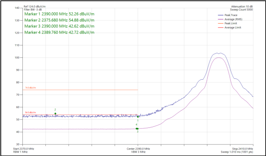
Figure 331 - Bluetooth HDT3, SISO, Core 0 - 2404 MHz Band Edge Frequency 2390 MHz
