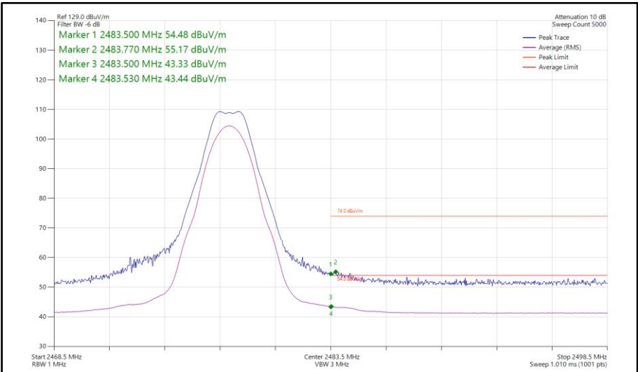
Figure 400 - Bluetooth LE2M, SISO, Core 2 - 2478 MHz Band Edge Frequency 2483.5 MHz
