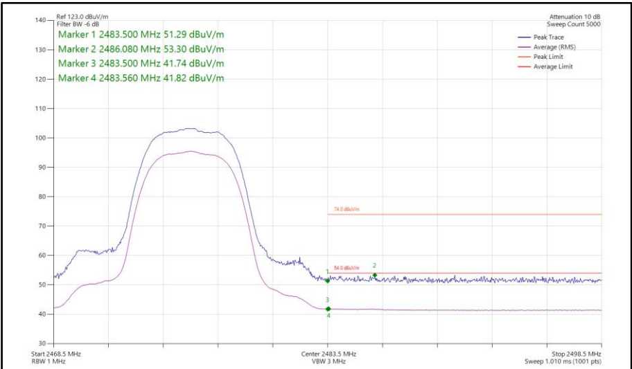
Figure 370 - Bluetooth HDR8, SISO, Core 1 - 2476 MHz Band Edge Frequency 2483.5 MHz
