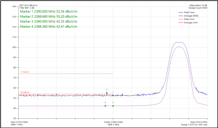
Figure 355 - Bluetooth HDR4, SISO, Core 1 - 2404 MHz Band Edge Frequency 2390 MHz
