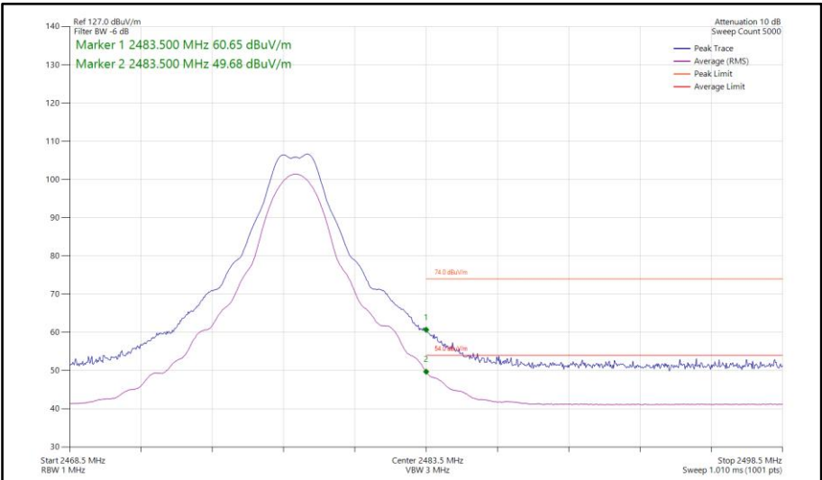
Figure 380 - Bluetooth CS1LE2M, SISO, Core 1 - 2478 MHz Band Edge Frequency 2483.5 MHz
