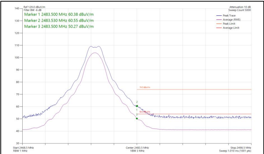
Figure 408 - Bluetooth CS1LE2M, SISO, Core 2 - 2478 MHz Band Edge Frequency 2483.5 MHz
