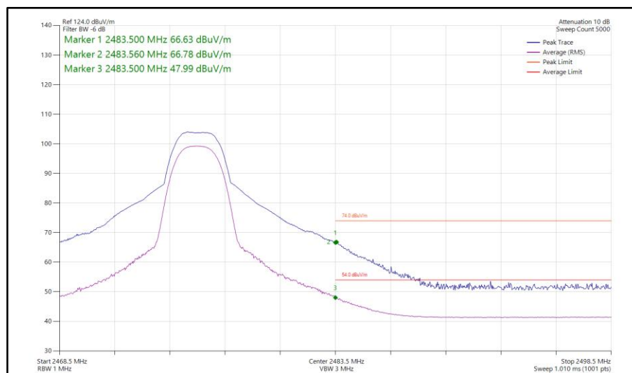
Figure 374 - Bluetooth HDT4, SISO, Core 1 - 2476 MHz Band Edge Frequency 2483.5 MHz
