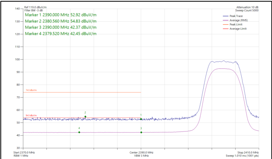
Figure 336 - Bluetooth XHDRPM8, SISO, Core 0 - 2404 MHz Band Edge Frequency 2390 MHz
