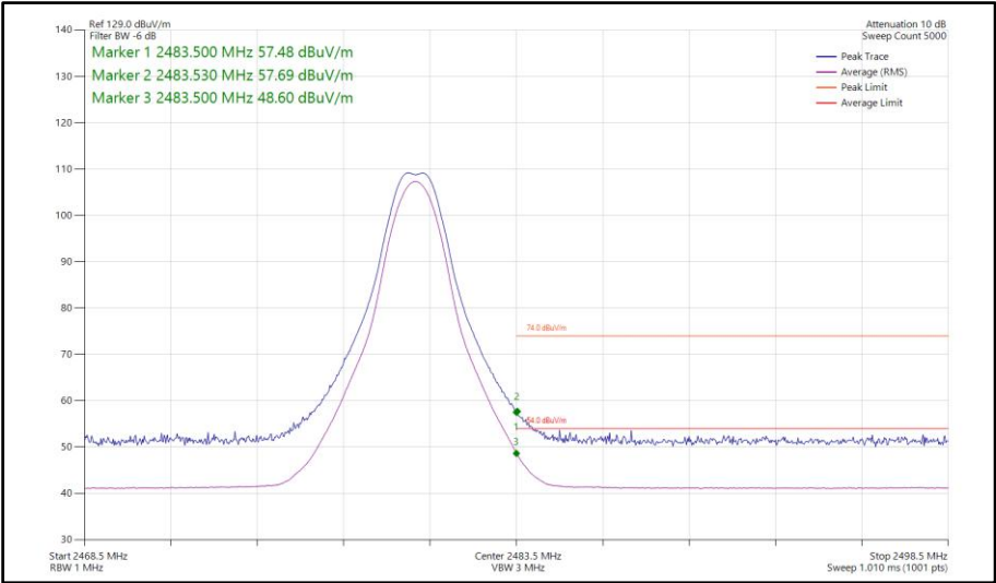
Figure 407 - Bluetooth CS1LE1M, SISO, Core 2 - 2480 MHz Band Edge Frequency 2483.5 MHz
