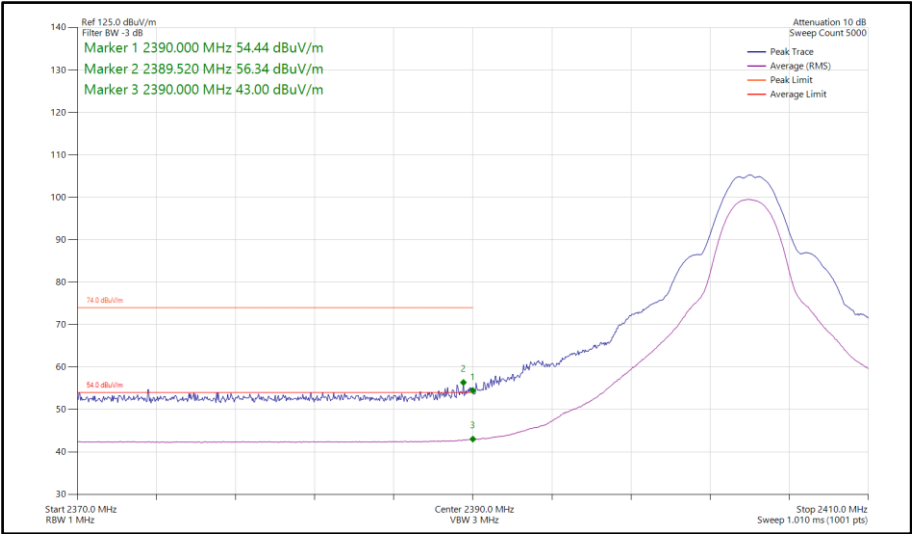
Figure 333 - Bluetooth HDT6, SISO, Core 0 - 2404 MHz Band Edge Frequency 2390 MHz
