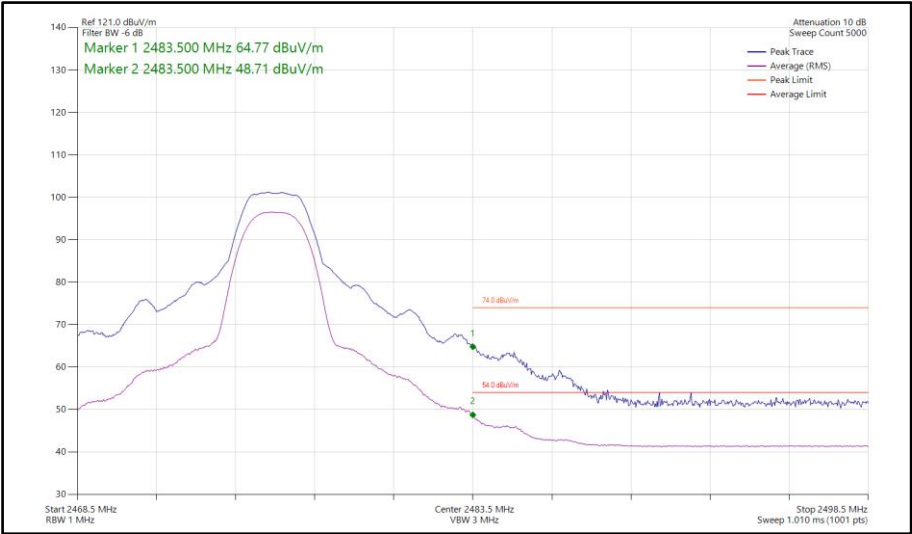
Figure 345 - Bluetooth HDT3, SISO, Core 0 - 2476 MHz Band Edge Frequency 2483.5 MHz
