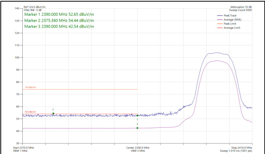
Figure 356 - Bluetooth HDR8, SISO, Core 1 - 2404 MHz Band Edge Frequency 2390 MHz
