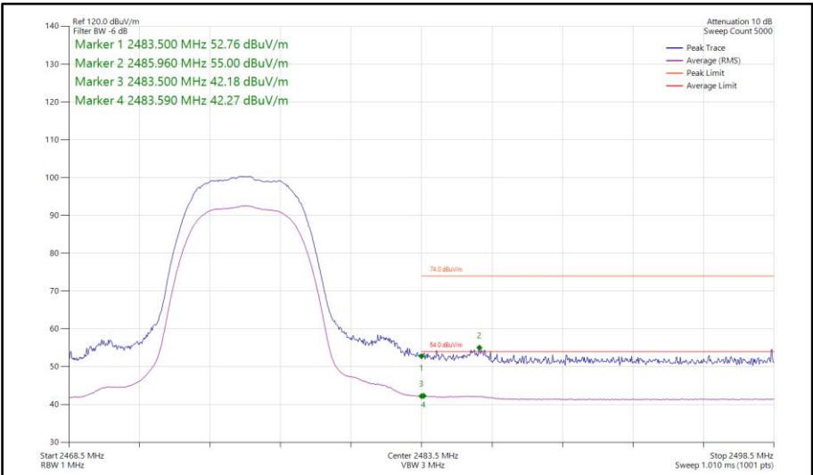
Figure 342 - Bluetooth HDR8, SISO, Core 0 - 2476 MHz Band Edge Frequency 2483.5 MHz
