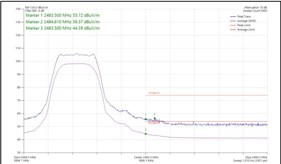
Figure 406 - Bluetooth XHDRPM8, SISO, Core 2 - 2475 MHz Band Edge Frequency 2483.5 MHz
