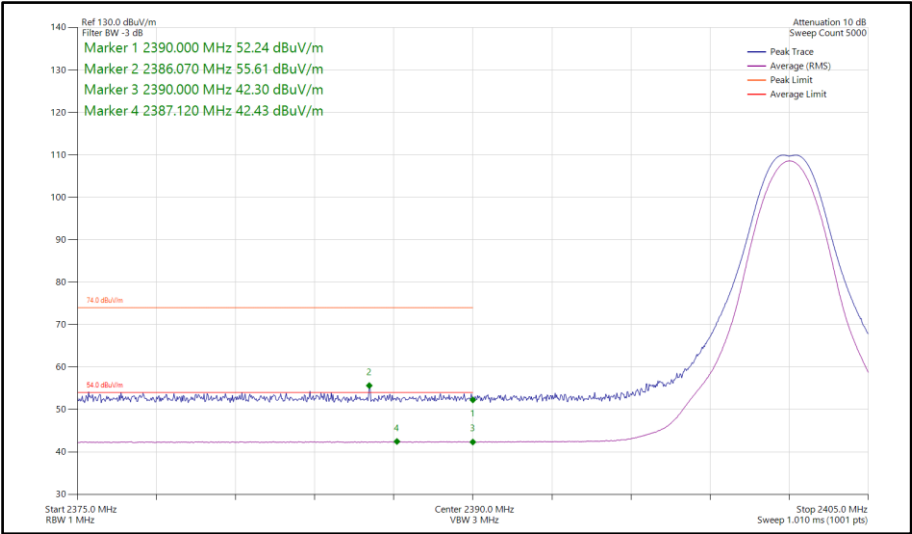
Figure 393 - Bluetooth CS1LE1M, SISO, Core 2 - 2402 MHz Band Edge Frequency 2390 MHz
