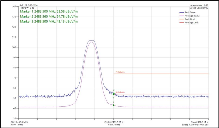
Figure 371 - Bluetooth LE1M, SISO, Core 1 - 2480 MHz Band Edge Frequency 2483.5 MHz
