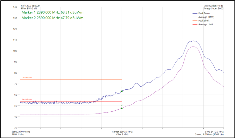
Figure 389 - Bluetooth HDT6, SISO, Core 2 - 2404 MHz Band Edge Frequency 2390 MHz
