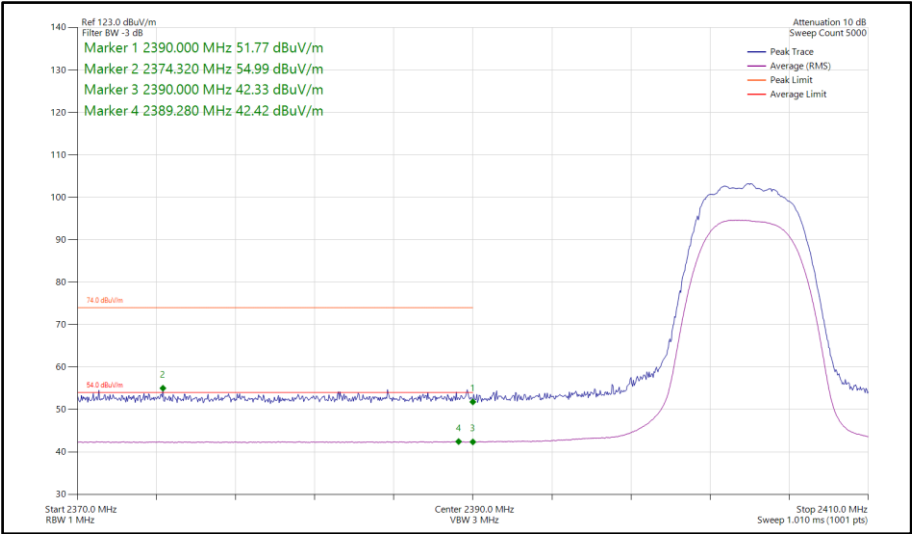
Figure 363 - Bluetooth HDRPM12, SISO, Core 1 - 2404 MHz Band Edge Frequency 2390 MHz
