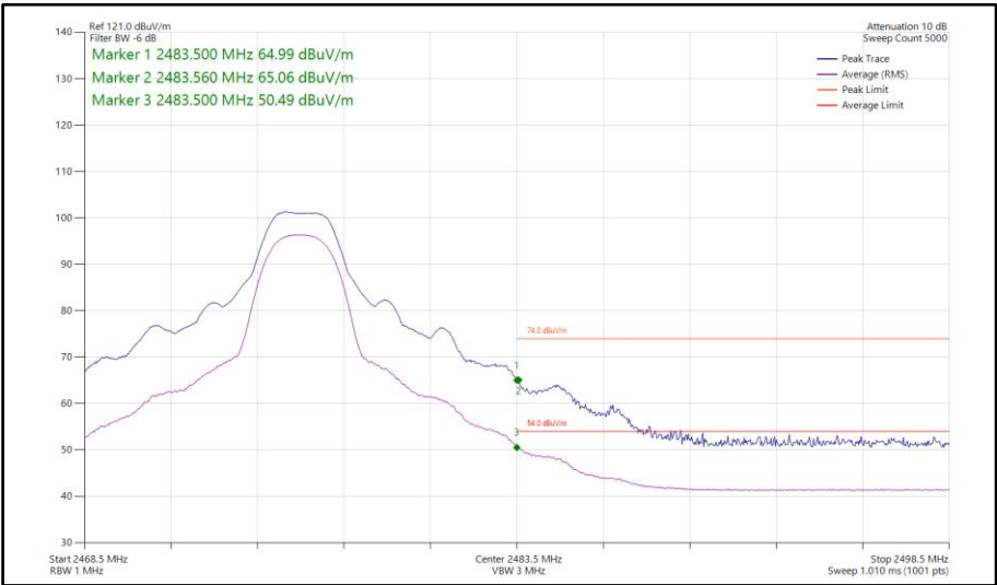
Figure 346 - Bluetooth HDT4, SISO, Core 0 - 2476 MHz Band Edge Frequency 2483.5 MHz
