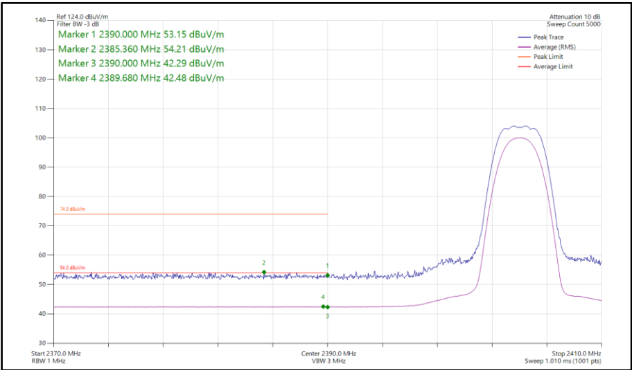
Figure 390 - Bluetooth HDRPS2, SISO, Core 2 - 2404 MHz Band Edge Frequency 2390 MHz
