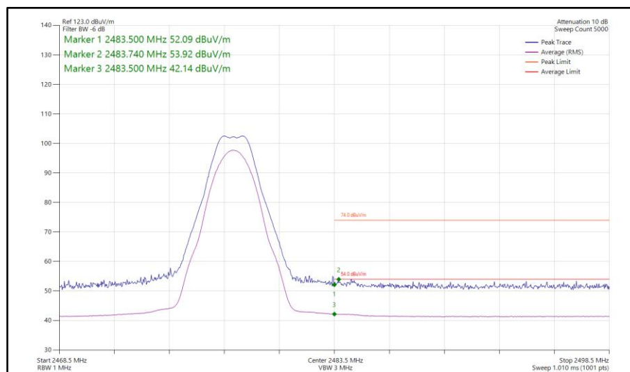
Figure 344 - Bluetooth LE2M, SISO, Core 0 - 2478 MHz Band Edge Frequency 2483.5 MHz
