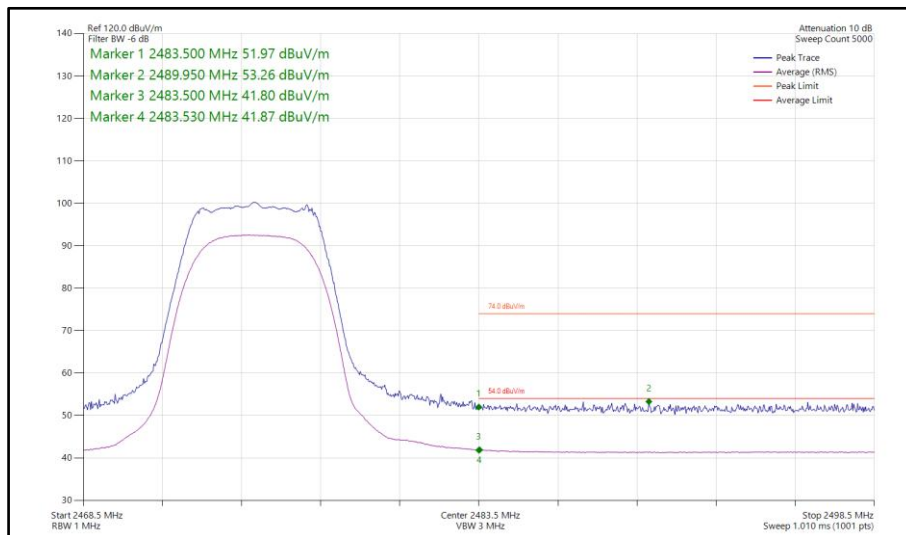
Figure 350 - Bluetooth XHDRPM8, SISO, Core 0 - 2475 MHz Band Edge Frequency 2483.5 MHz
