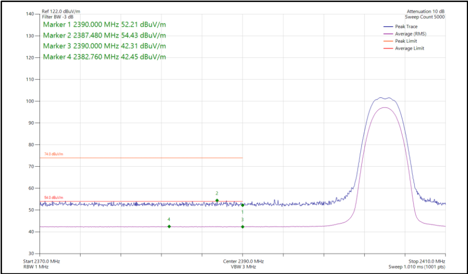
Figure 327 - Bluetooth HDR4, SISO, Core 0 - 2404 MHz Band Edge Frequency 2390 MHz
