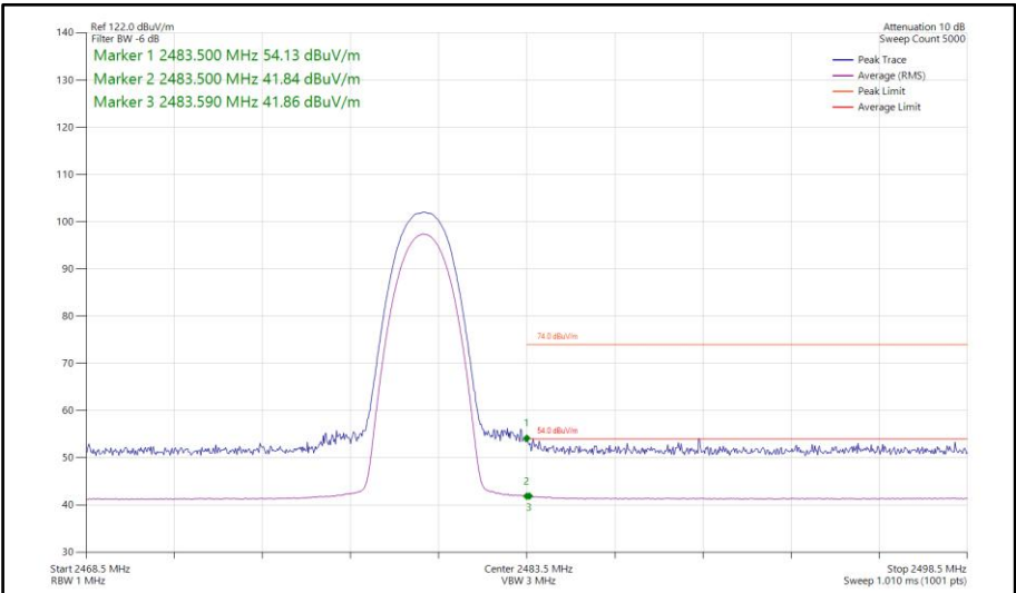
Figure 340 - Bluetooth 3DH5, SISO, Core 0 - 2480 MHz Band Edge Frequency 2483.5 MHz
