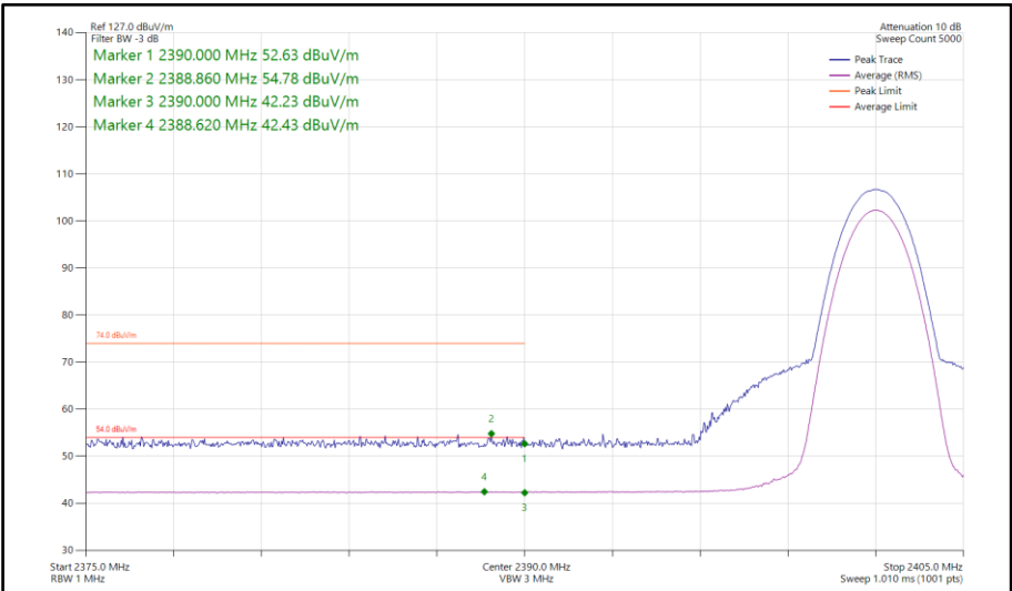
Figure 354 - Bluetooth 3DH5, SISO, Core 1 - 2402 MHz Band Edge Frequency 2390 MHz
