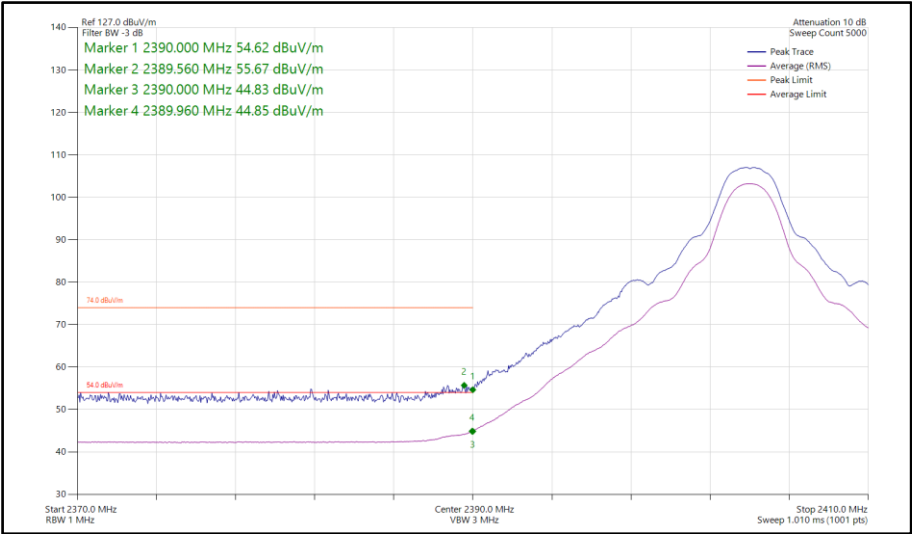
Figure 359 - Bluetooth HDT3, SISO, Core 1 - 2404 MHz Band Edge Frequency 2390 MHz
