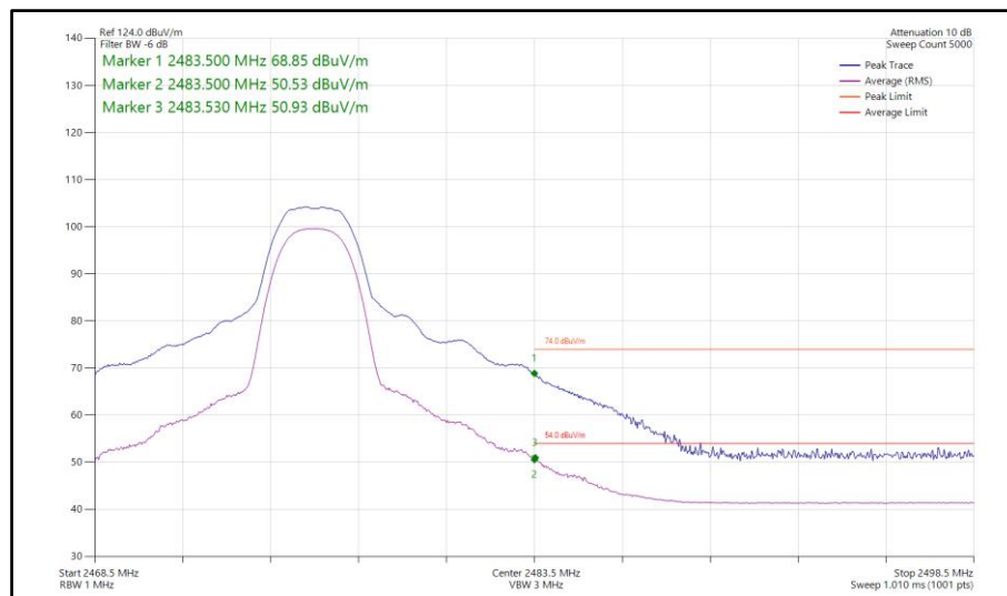
Figure 373 - Bluetooth HDT3, SISO, Core 1 - 2476 MHz Band Edge Frequency 2483.5 MHz
