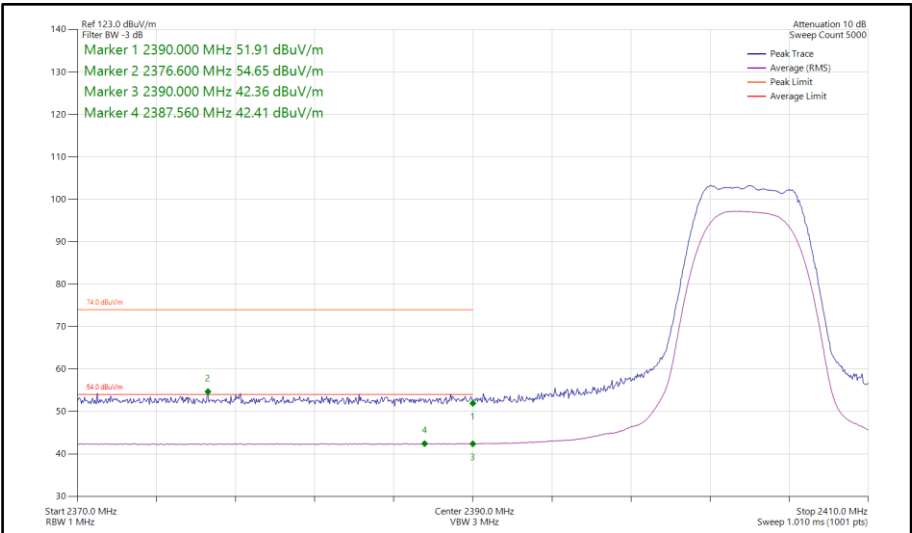
Figure 364 - Bluetooth XHDRPM8, SISO, Core 1 - 2404 MHz Band Edge Frequency 2390 MHz
