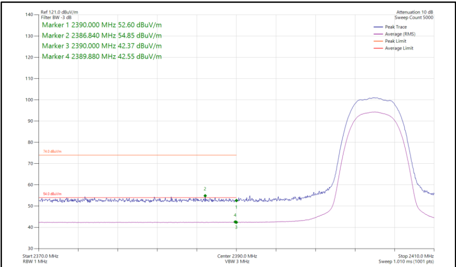
Figure 328 - Bluetooth HDR8, SISO, Core 0 - 2404 MHz Band Edge Frequency 2390 MHz
