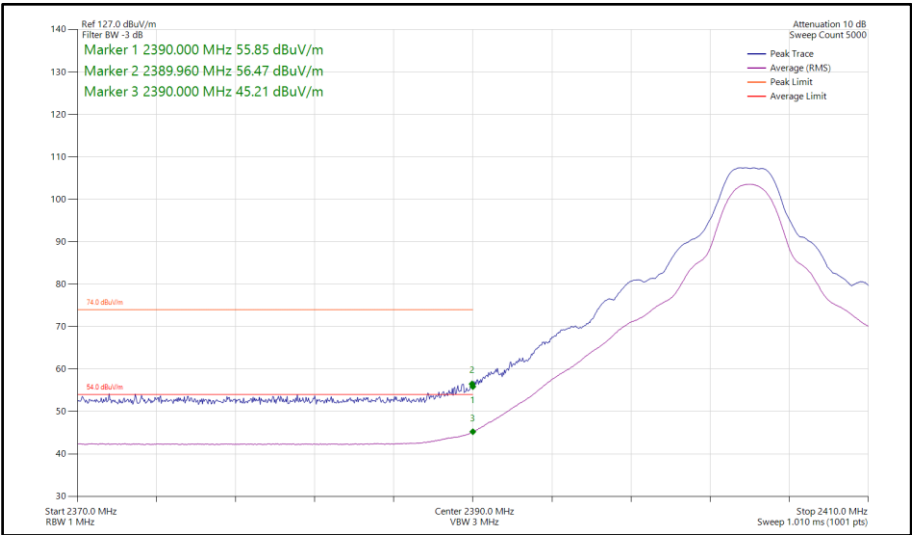
Figure 360 - Bluetooth HDT4, SISO, Core 1 - 2404 MHz Band Edge Frequency 2390 MHz
