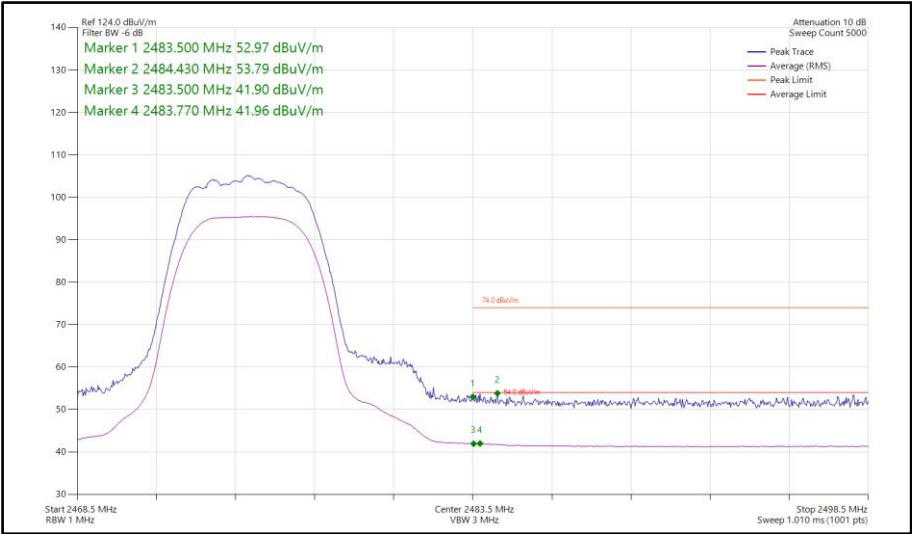
Figure 405 - Bluetooth HDRPM12, SISO, Core 2 - 2475 MHz Band Edge Frequency 2483.5 MHz
