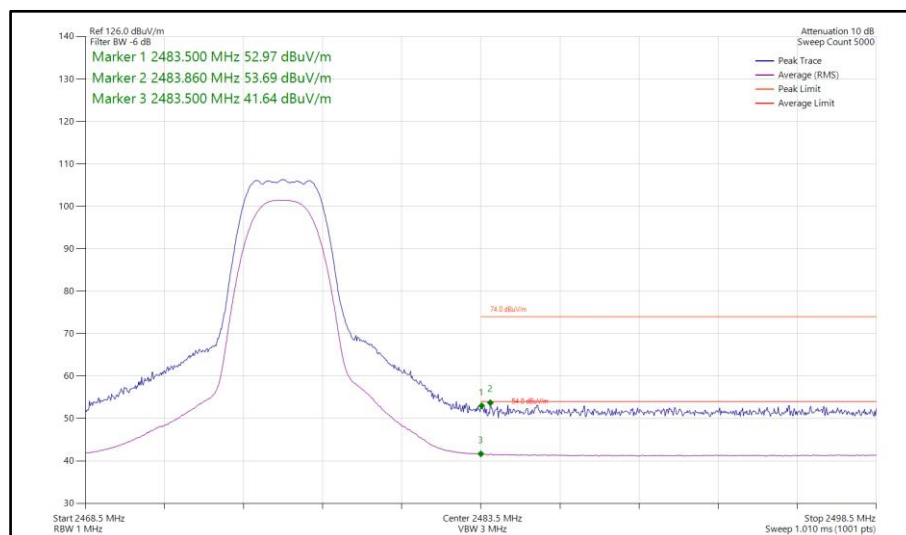
Figure 404 - Bluetooth HDRPS2, SISO, Core 2 - 2476 MHz Band Edge Frequency 2483.5 MHz
