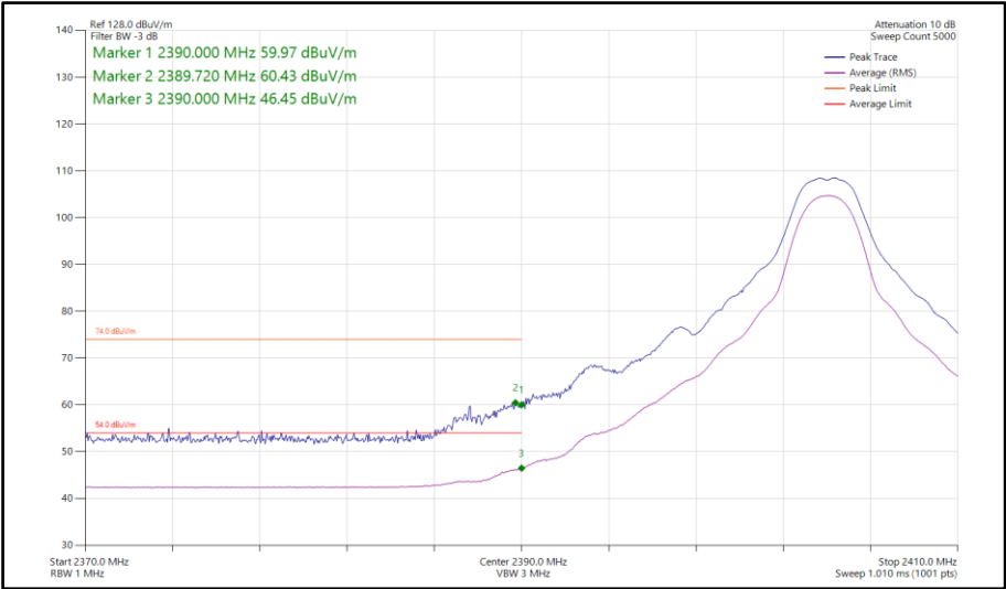
Figure 387 - Bluetooth HDT3, SISO, Core 2 - 2404 MHz Band Edge Frequency 2390 MHz
