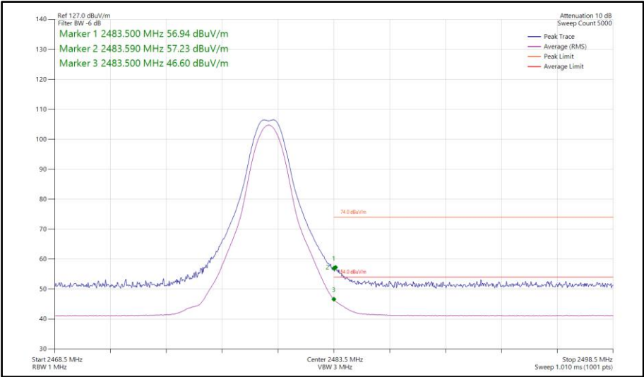
Figure 379 - Bluetooth CS1LE1M, SISO, Core 1 - 2480 MHz Band Edge Frequency 2483.5 MHz
