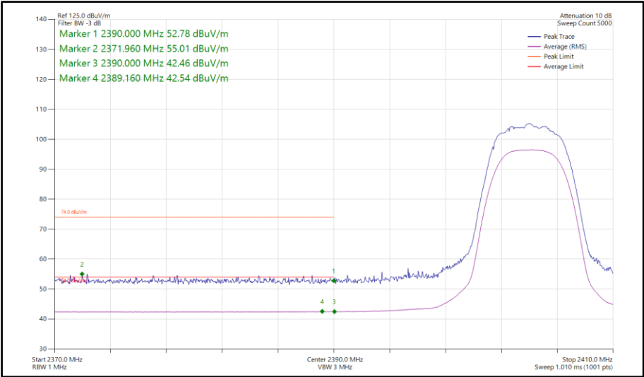
Figure 391 - Bluetooth HDRPM12, SISO, Core 2 - 2404 MHz Band Edge Frequency 2390 MHz
