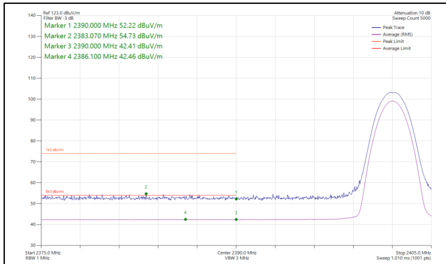
Figure 325 - Bluetooth 2DH5, SISO, Core 0 - 2402 MHz Band Edge Frequency 2390 MHz
