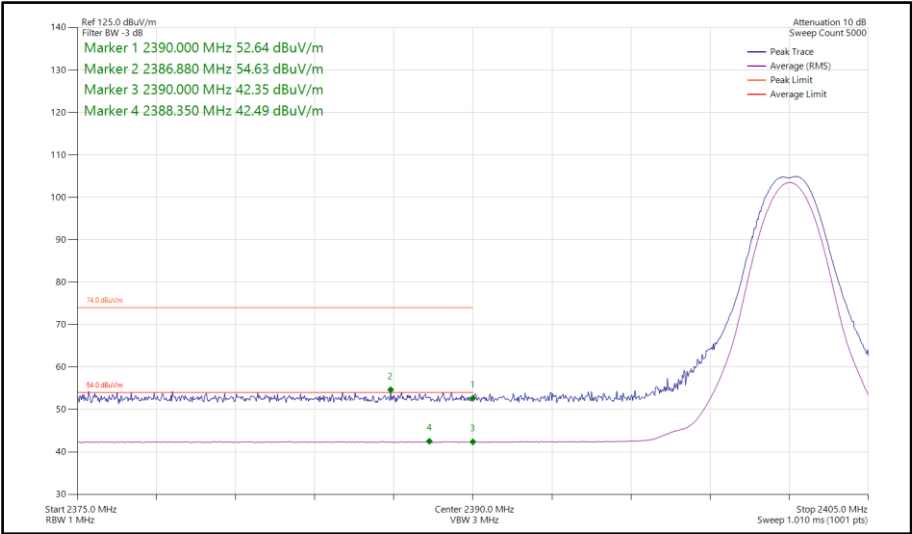
Figure 337 - Bluetooth CS1LE1M, SISO, Core 0 - 2402 MHz Band Edge Frequency 2390 MHz
