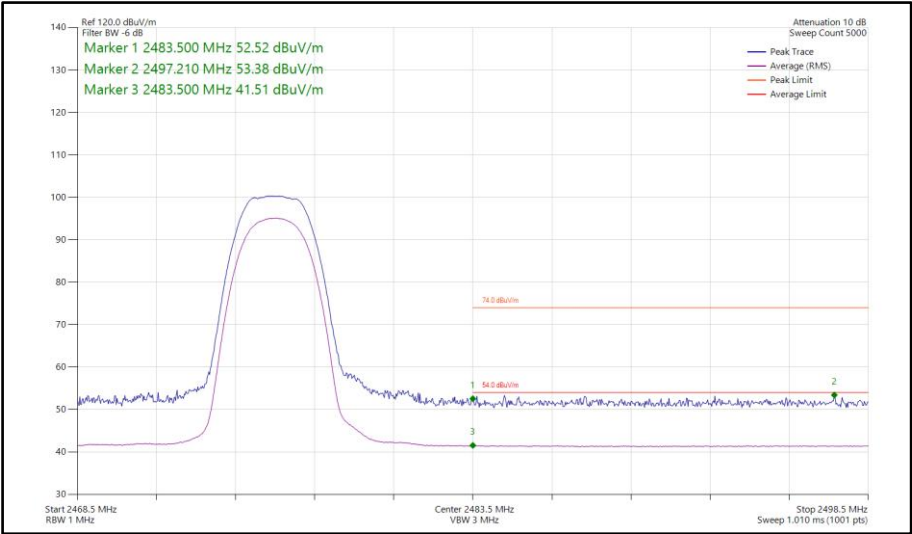
Figure 341 - Bluetooth HDR4, SISO, Core 0 - 2476 MHz Band Edge Frequency 2483.5 MHz
