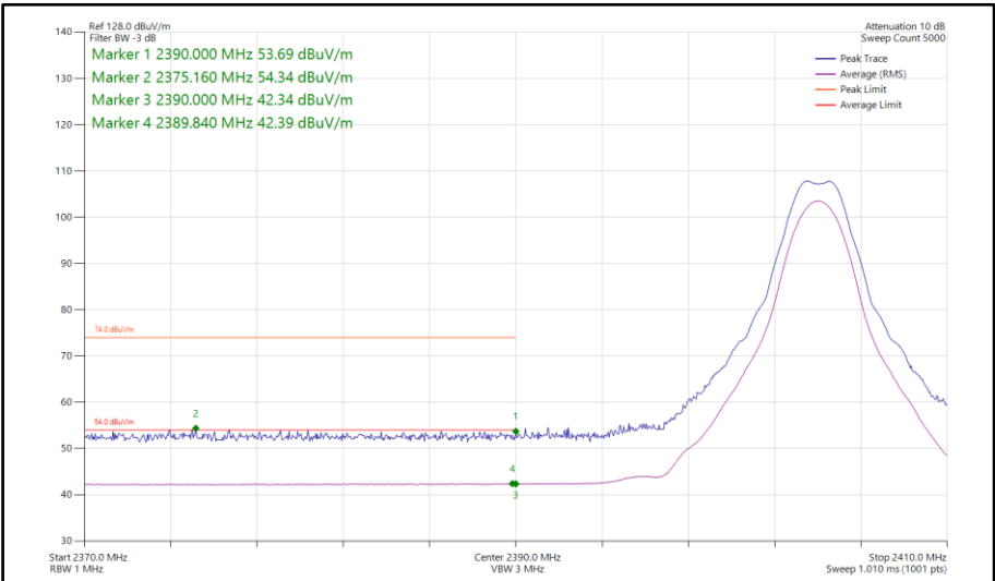
Figure 366 - Bluetooth CS1LE2M, SISO, Core 1 - 2404 MHz Band Edge Frequency 2390 MHz
