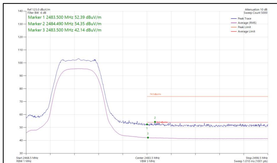
Figure 378 - Bluetooth XHDRPM8, SISO, Core 1 - 2475 MHz Band Edge Frequency 2483.5 MHz
