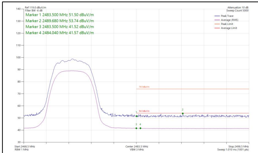
Figure 349 - Bluetooth HDRPM12, SISO, Core 0 - 2475 MHz Band Edge Frequency 2483.5 MHz
