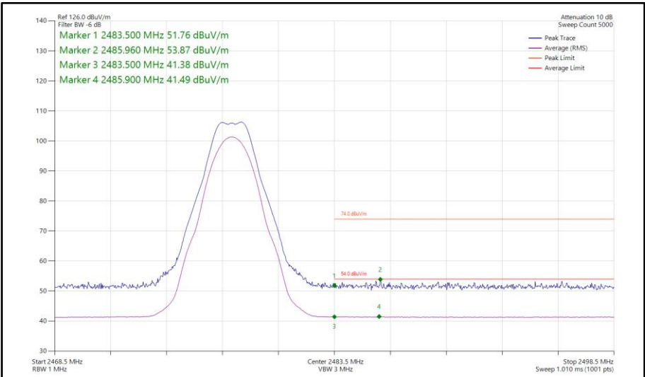
Figure 372 - Bluetooth LE2M, SISO, Core 1 - 2478 MHz Band Edge Frequency 2483.5 MHz
