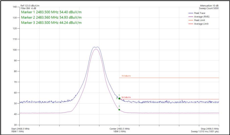
Figure 351 - Bluetooth CS1LE1M, SISO, Core 0 - 2480 MHz Band Edge Frequency 2483.5 MHz
