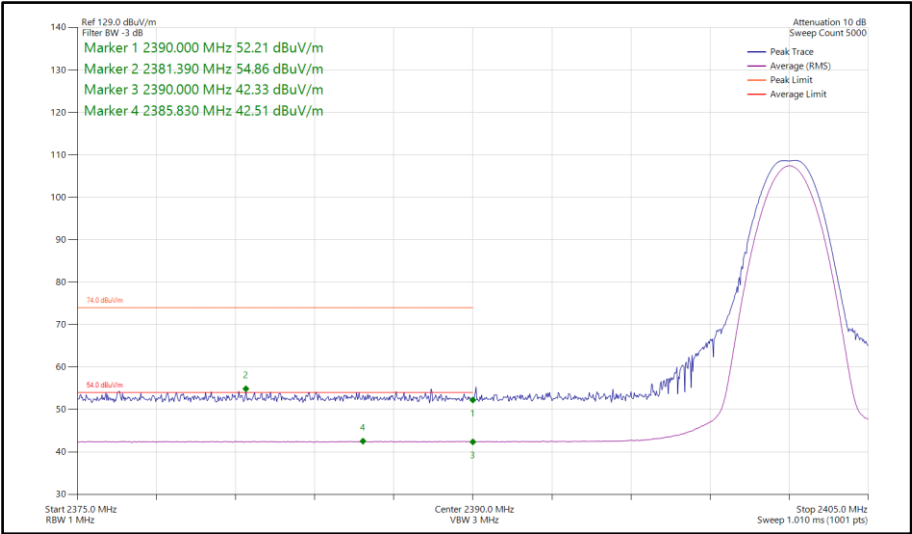
Figure 385 - Bluetooth LE1M, SISO, Core 2 - 2402 MHz Band Edge Frequency 2390 MHz
