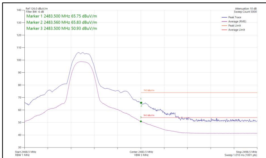
Figure 375 - Bluetooth HDT6, SISO, Core 1 - 2476 MHz Band Edge Frequency 2483.5 MHz
