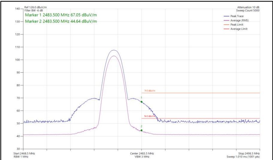
Figure 396 - Bluetooth 3DH5, SISO, Core 2 - 2480 MHz Band Edge Frequency 2483.5 MHz
