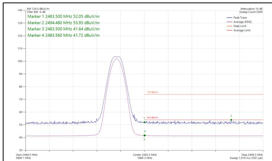
Figure 343 - Bluetooth LE1M, SISO, Core 0 - 2480 MHz Band Edge Frequency 2483.5 MHz
