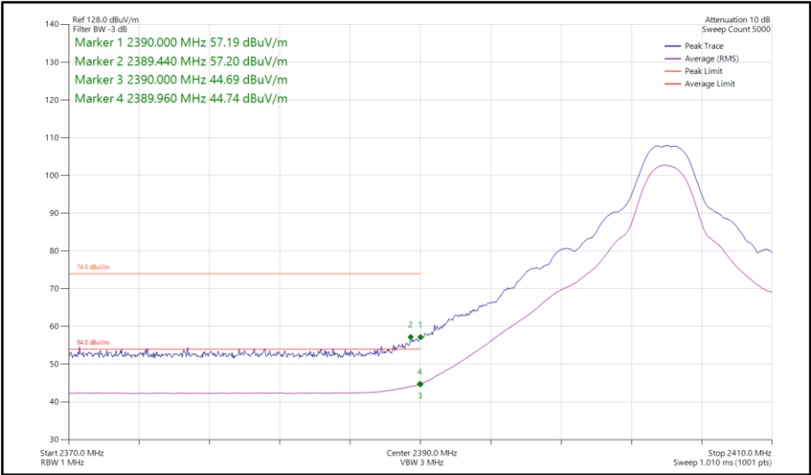
Figure 361 - Bluetooth HDT6, SISO, Core 1 - 2404 MHz Band Edge Frequency 2390 MHz
