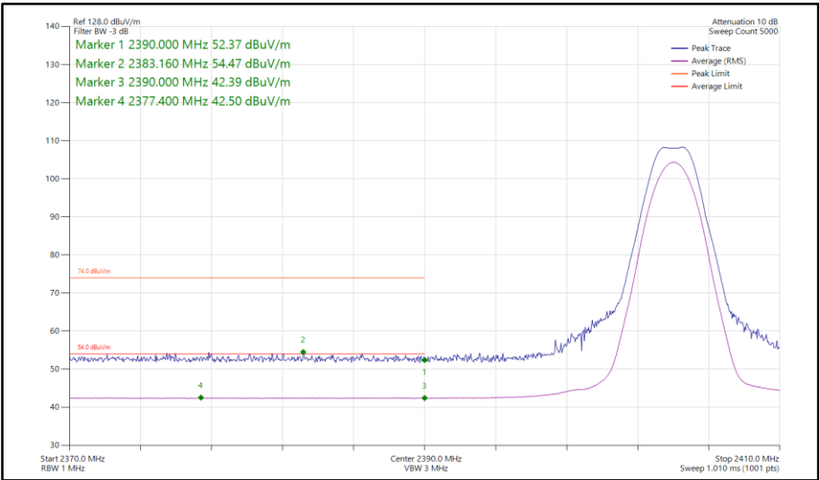
Figure 386 - Bluetooth LE2M, SISO, Core 2 - 2404 MHz Band Edge Frequency 2390 MHz
