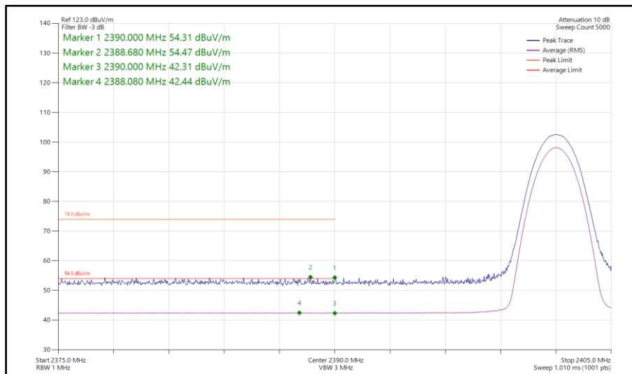
Figure 326 - Bluetooth 3DH5, SISO, Core 0 - 2402 MHz Band Edge Frequency 2390 MHz
