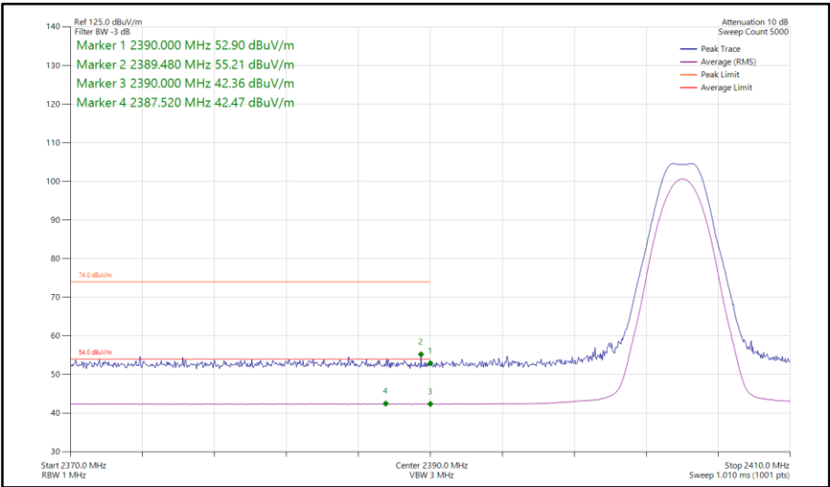
Figure 330 - Bluetooth LE2M, SISO, Core 0 - 2404 MHz Band Edge Frequency 2390 MHz
