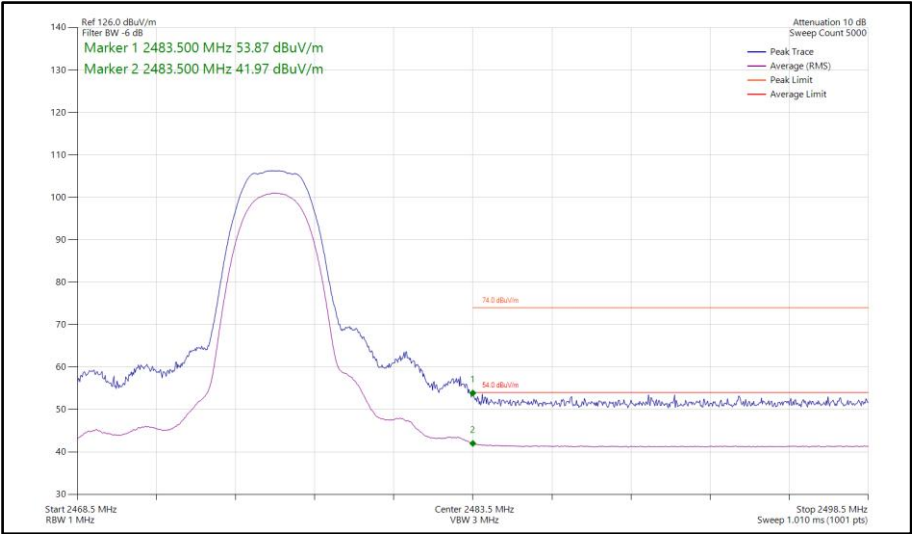
Figure 397 - Bluetooth HDR4, SISO, Core 2 - 2476 MHz Band Edge Frequency 2483.5 MHz
