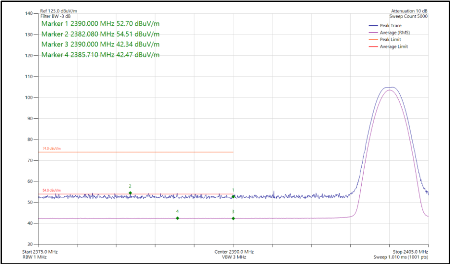
Figure 329 - Bluetooth LE1M, SISO, Core 0 - 2402 MHz Band Edge Frequency 2390 MHz
