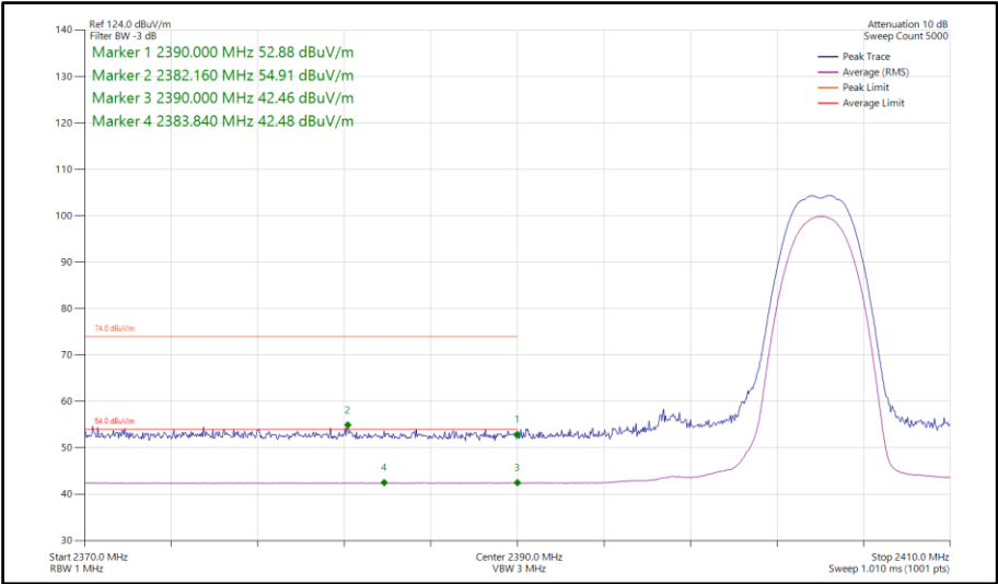
Figure 383 - Bluetooth HDR4, SISO, Core 2 - 2404 MHz Band Edge Frequency 2390 MHz
