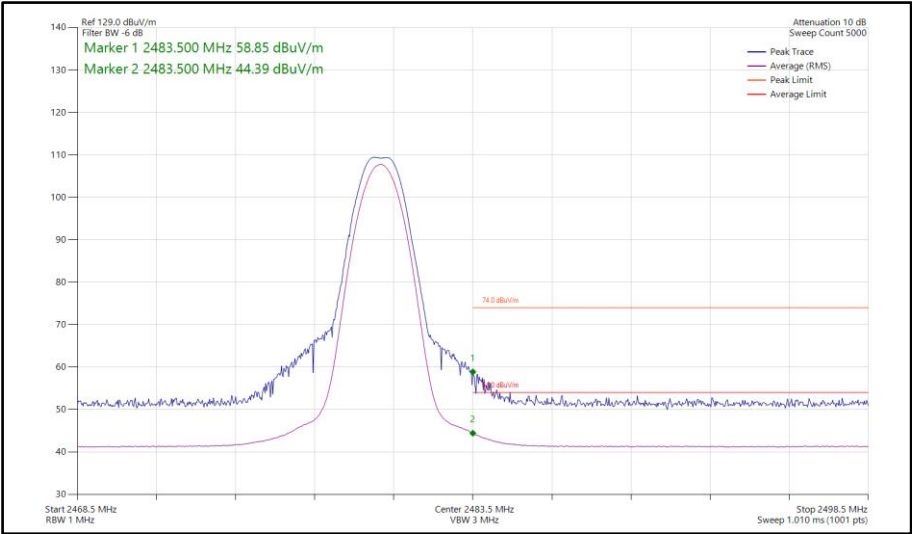
Figure 399 - Bluetooth LE1M, SISO, Core 2 - 2480 MHz Band Edge Frequency 2483.5 MHz
