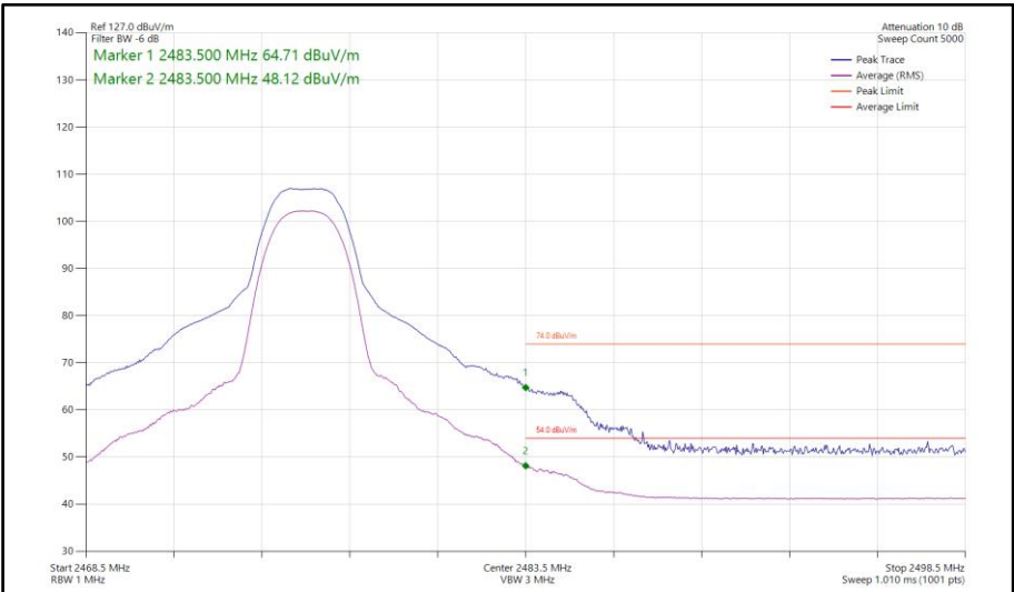
Figure 402 - Bluetooth HDT4, SISO, Core 2 - 2476 MHz Band Edge Frequency 2483.5 MHz
