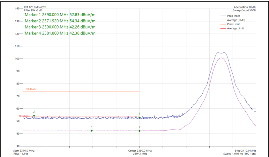
Figure 338 - Bluetooth CS1LE2M, SISO, Core 0 - 2404 MHz Band Edge Frequency 2390 MHz
