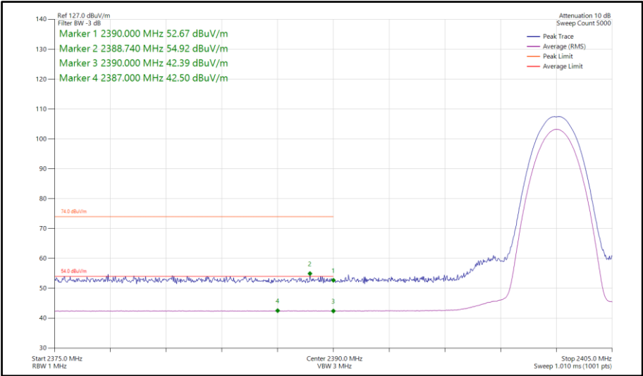
Figure 381 - Bluetooth 2DH5, SISO, Core 2 - 2402 MHz Band Edge Frequency 2390 MHz
