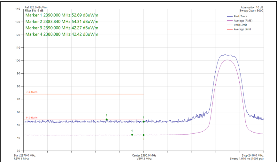
Figure 362 - Bluetooth HDRPS2, SISO, Core 1 - 2404 MHz Band Edge Frequency 2390 MHz
