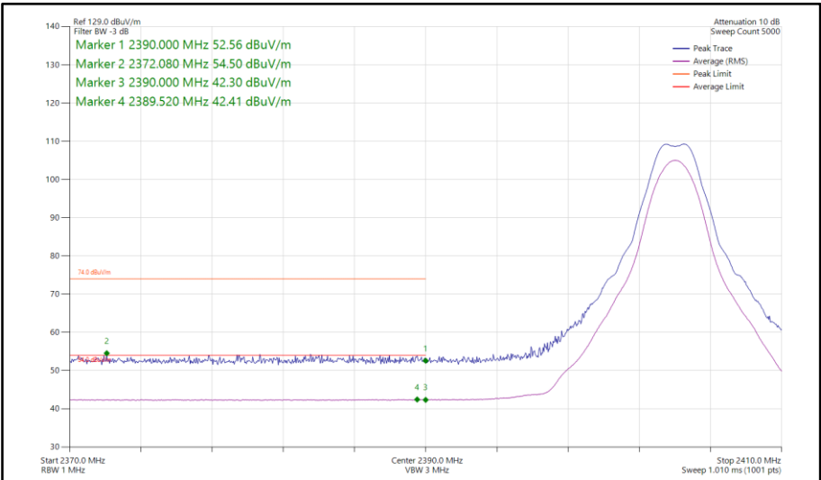
Figure 394 - Bluetooth CS1LE2M, SISO, Core 2 - 2404 MHz Band Edge Frequency 2390 MHz
