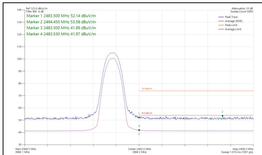
Figure 367 - Bluetooth 2DH5, SISO, Core 1 - 2480 MHz Band Edge Frequency 2483.5 MHz
