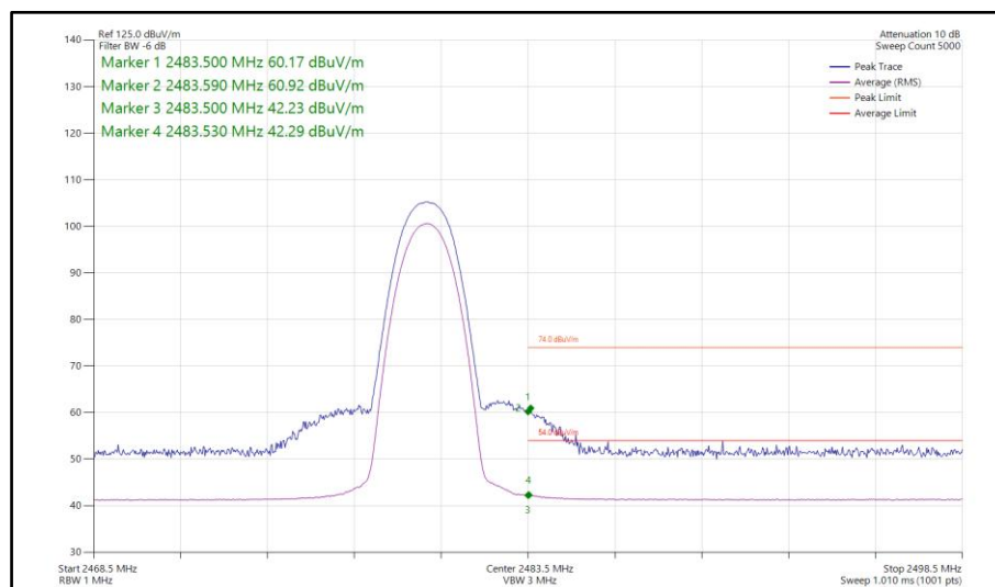
Figure 368 - Bluetooth 3DH5, SISO, Core 1 - 2480 MHz Band Edge Frequency 2483.5 MHz
