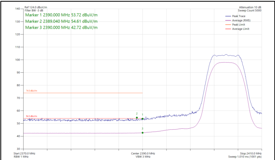
Figure 392 - Bluetooth XHDRPM8, SISO, Core 2 - 2404 MHz Band Edge Frequency 2390 MHz
