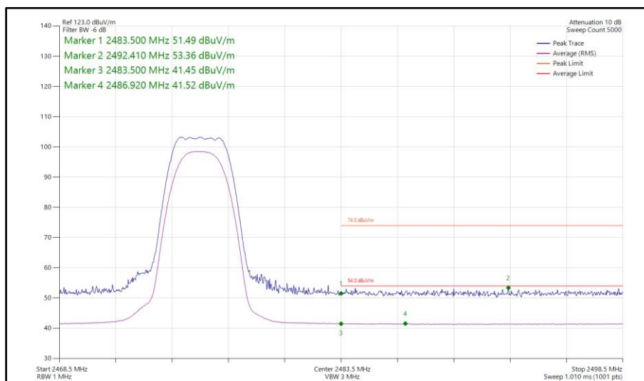
Figure 376 - Bluetooth HDRPS2, SISO, Core 1 - 2476 MHz Band Edge Frequency 2483.5 MHz
