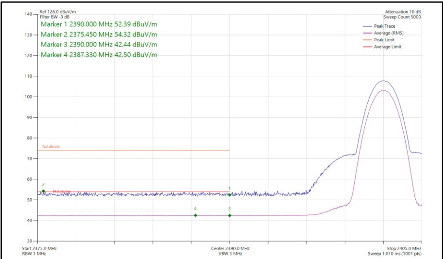
Figure 382 - Bluetooth 3DH5, SISO, Core 2 - 2402 MHz Band Edge Frequency 2390 MHz
