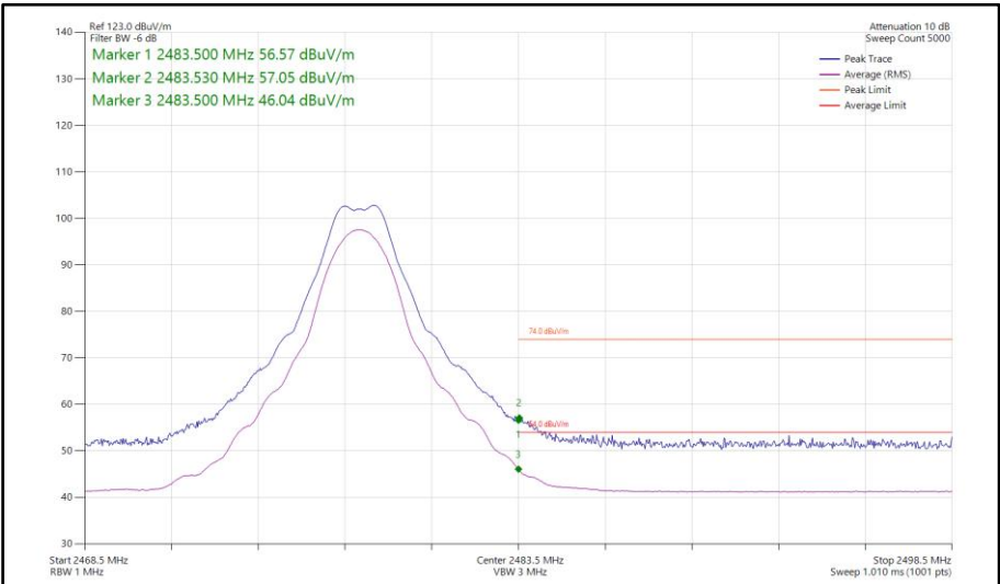
Figure 352 - Bluetooth CS1LE2M, SISO, Core 0 - 2478 MHz Band Edge Frequency 2483.5 MHz
