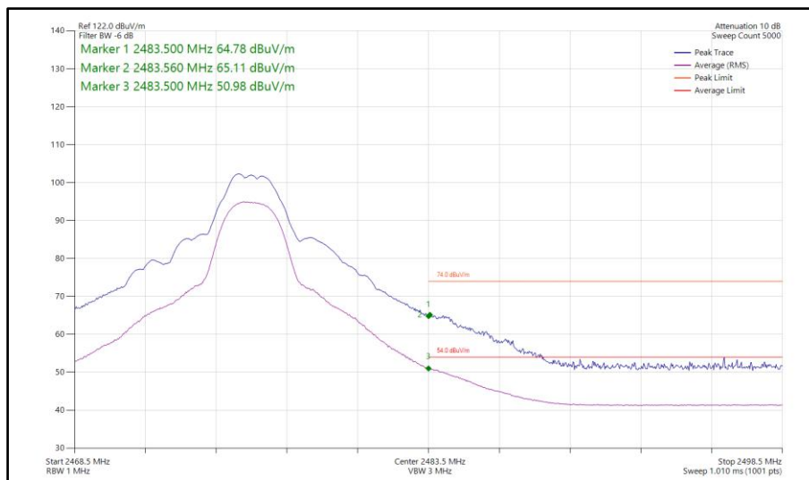
Figure 347 - Bluetooth HDT6, SISO, Core 0 - 2476 MHz Band Edge Frequency 2483.5 MHz
