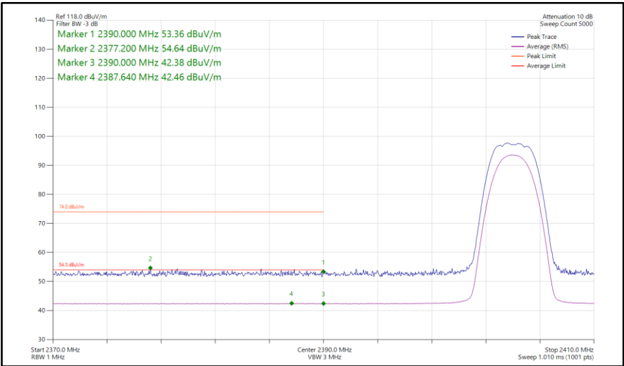
Figure 334 - Bluetooth HDRPS2, SISO, Core 0 - 2404 MHz Band Edge Frequency 2390 MHz
