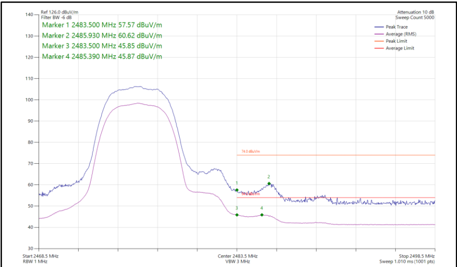
Figure 398 - Bluetooth HDR8, SISO, Core 2 - 2476 MHz Band Edge Frequency 2483.5 MHz
