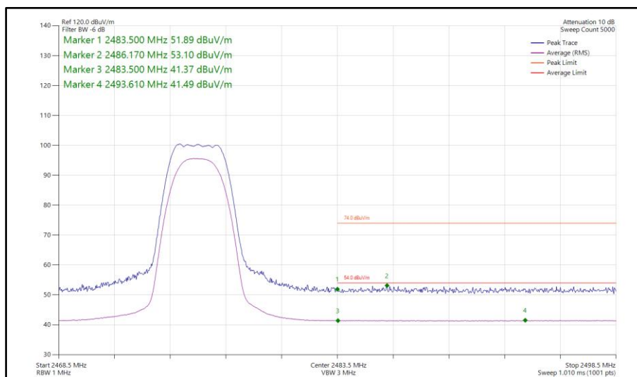
Figure 348 - Bluetooth HDRPS2, SISO, Core 0 - 2476 MHz Band Edge Frequency 2483.5 MHz
