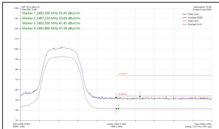
Figure 377 - Bluetooth HDRPM12, SISO, Core 1 - 2475 MHz Band Edge Frequency 2483.5 MHz
