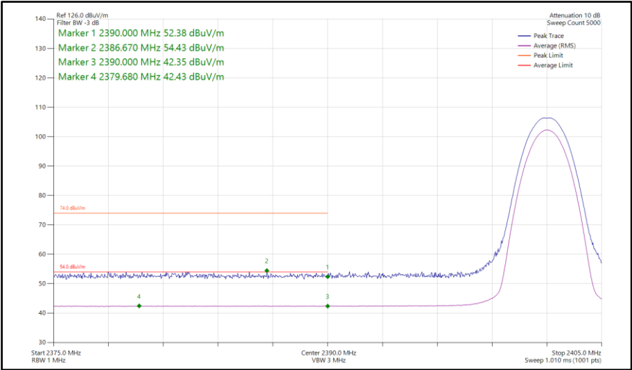
Figure 353 - Bluetooth 2DH5, SISO, Core 1 - 2402 MHz Band Edge Frequency 2390 MHz
