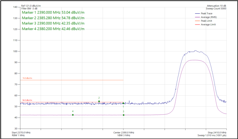
Figure 335 - Bluetooth HDRPM12, SISO, Core 0 - 2404 MHz Band Edge Frequency 2390 MHz
