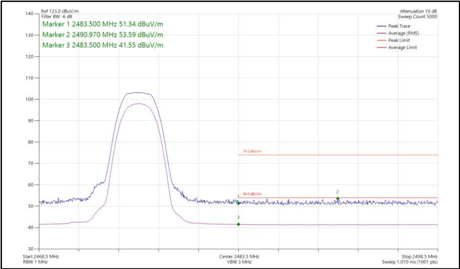
Figure 369 - Bluetooth HDR4, SISO, Core 1 - 2476 MHz Band Edge Frequency 2483.5 MHz
