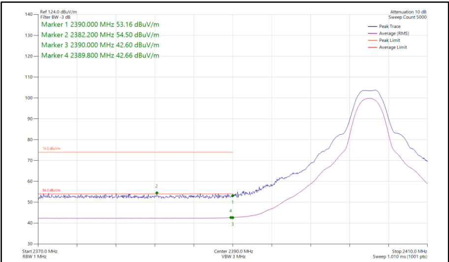
Figure 332 - Bluetooth HDT4, SISO, Core 0 - 2404 MHz Band Edge Frequency 2390 MHz
