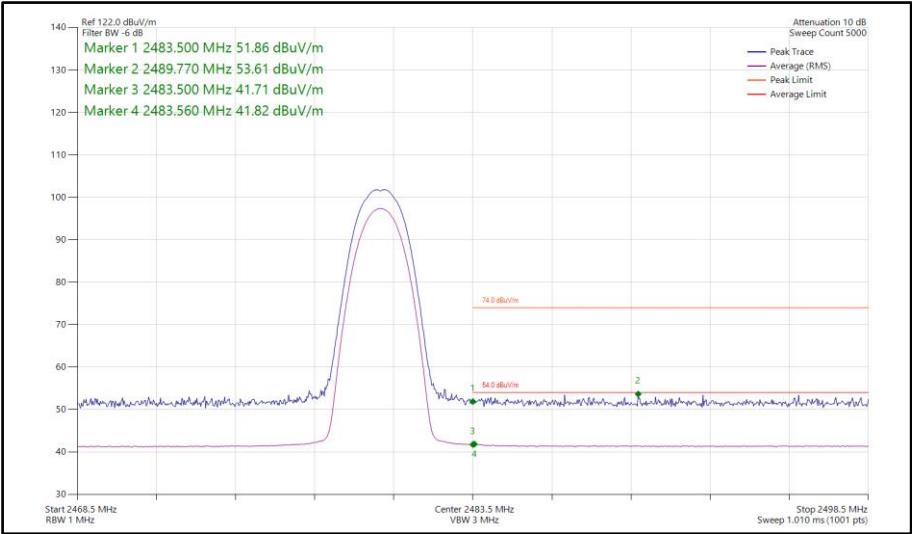
Figure 339 - Bluetooth 2DH5, SISO, Core 0 - 2480 MHz Band Edge Frequency 2483.5 MHz
