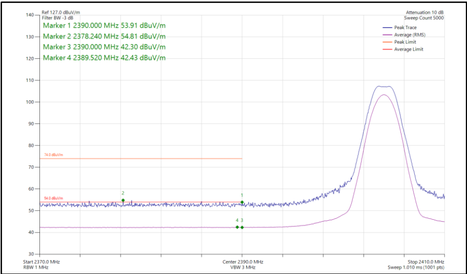
Figure 358 - Bluetooth LE2M, SISO, Core 1 - 2404 MHz Band Edge Frequency 2390 MHz
