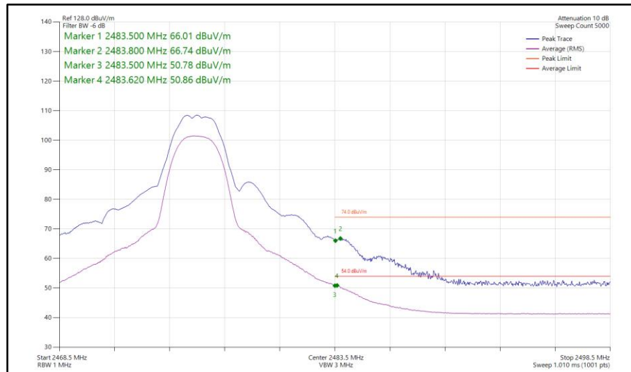
Figure 403 - Bluetooth HDT6, SISO, Core 2 - 2476 MHz Band Edge Frequency 2483.5 MHz
