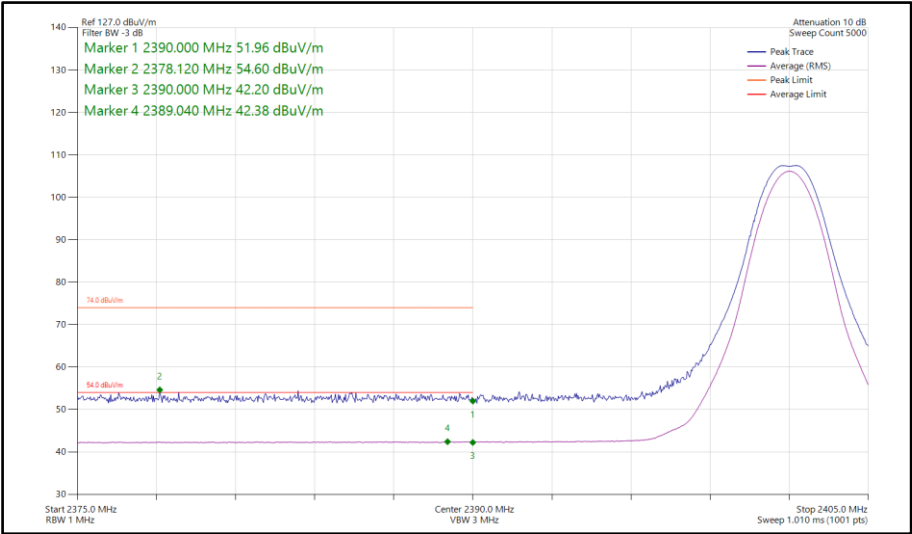
Figure 365 - Bluetooth CS1LE1M, SISO, Core 1 - 2402 MHz Band Edge Frequency 2390 MHz
