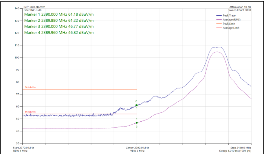
Figure 388 - Bluetooth HDT4, SISO, Core 2 - 2404 MHz Band Edge Frequency 2390 MHz
