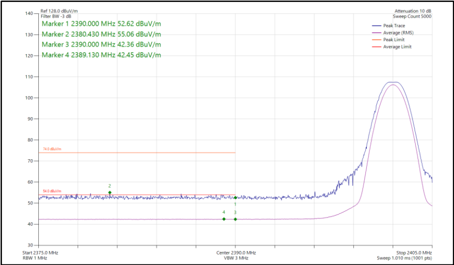
Figure 357 - Bluetooth LE1M, SISO, Core 1 - 2402 MHz Band Edge Frequency 2390 MHz
