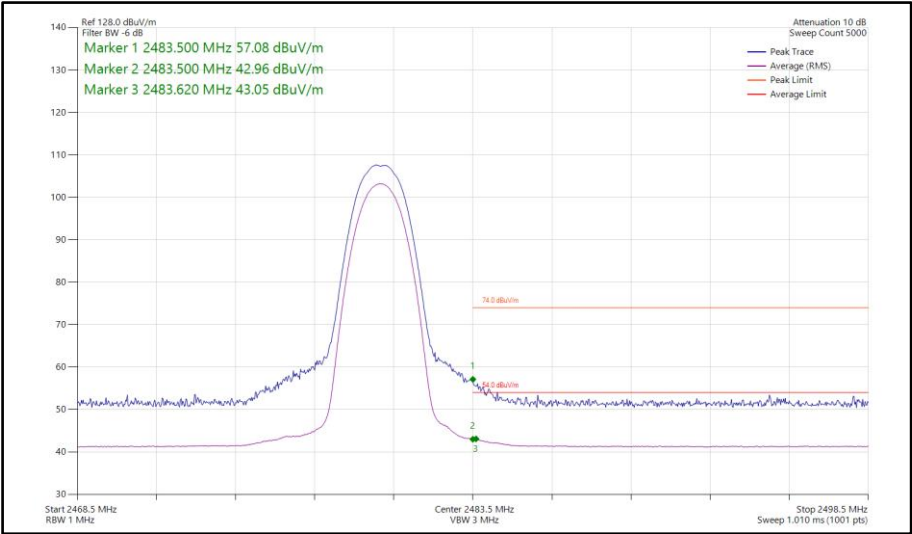
Figure 395 - Bluetooth 2DH5, SISO, Core 2 - 2480 MHz Band Edge Frequency 2483.5 MHz
