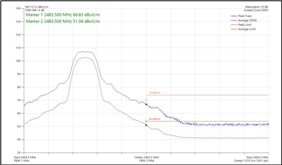
Figure 401 - Bluetooth HDT3, SISO, Core 2 - 2476 MHz Band Edge Frequency 2483.5 MHz
