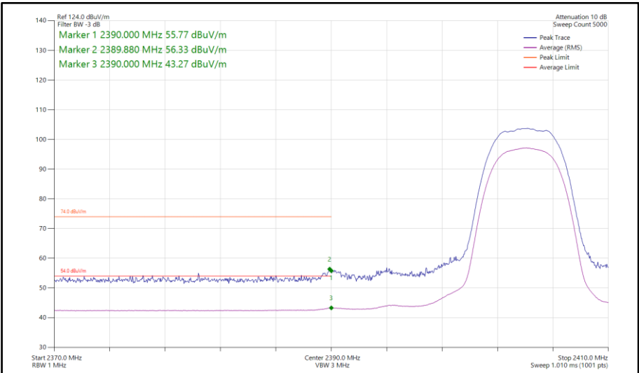
Figure 384 - Bluetooth HDR8, SISO, Core 2 - 2404 MHz Band Edge Frequency 2390 MHz
