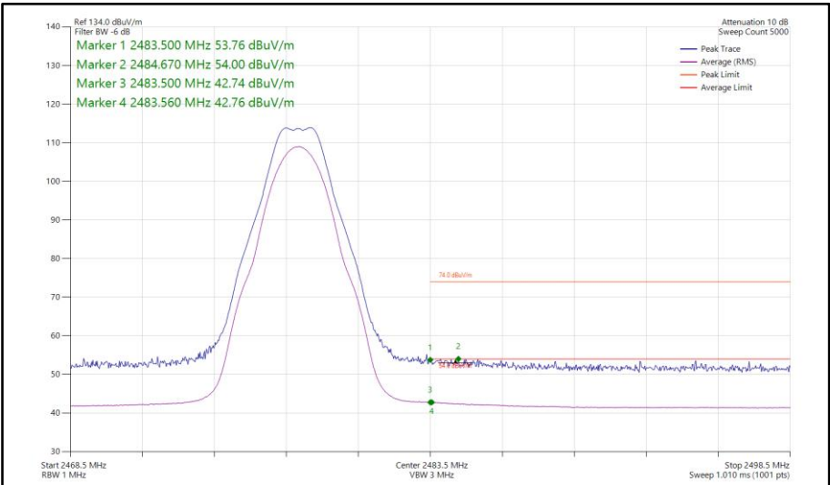
Figure 456 - Bluetooth LE2M, SISO, Core 0 - 2478 MHz Band Edge Frequency 2483.5 MHz
