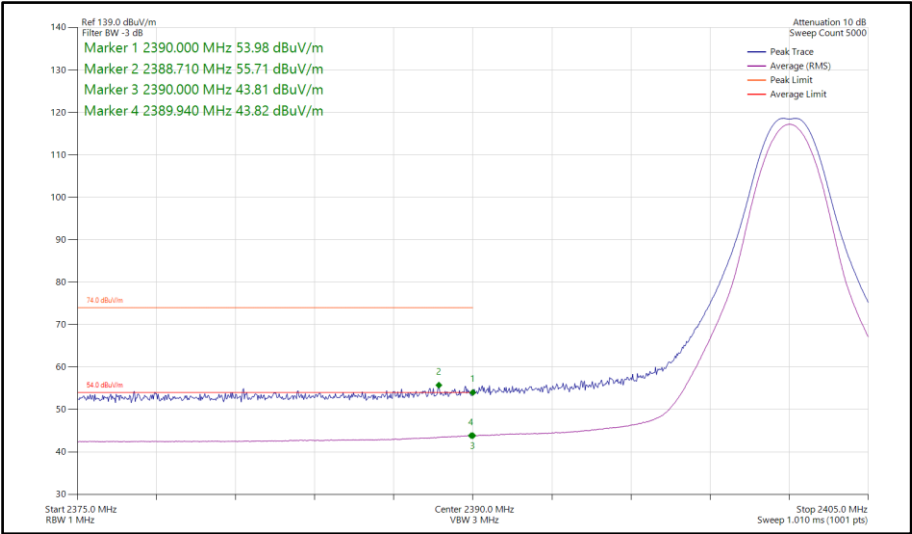
Figure 477 - Bluetooth CS1LE1M, SISO, Core 1 - 2402 MHz Band Edge Frequency 2390 MHz
