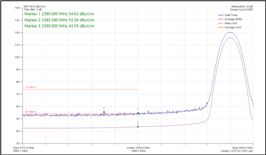
Figure 465 - Bluetooth 2DH5, SISO, Core 1 - 2402 MHz Band Edge Frequency 2390 MHz
