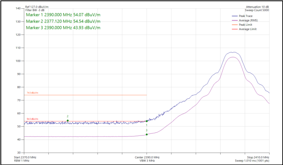
Figure 415 - Bluetooth HDT3, MIMO, Core 0-1 - 2404 MHz Band Edge Frequency 2390 MHz
