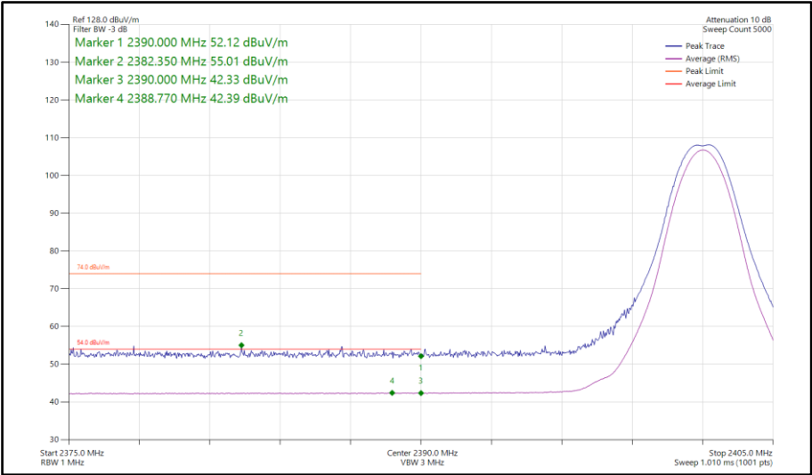
Figure 421 - Bluetooth CS1LE1M, MIMO, Core 0-1 - 2402 MHz Band Edge Frequency 2390 MHz
