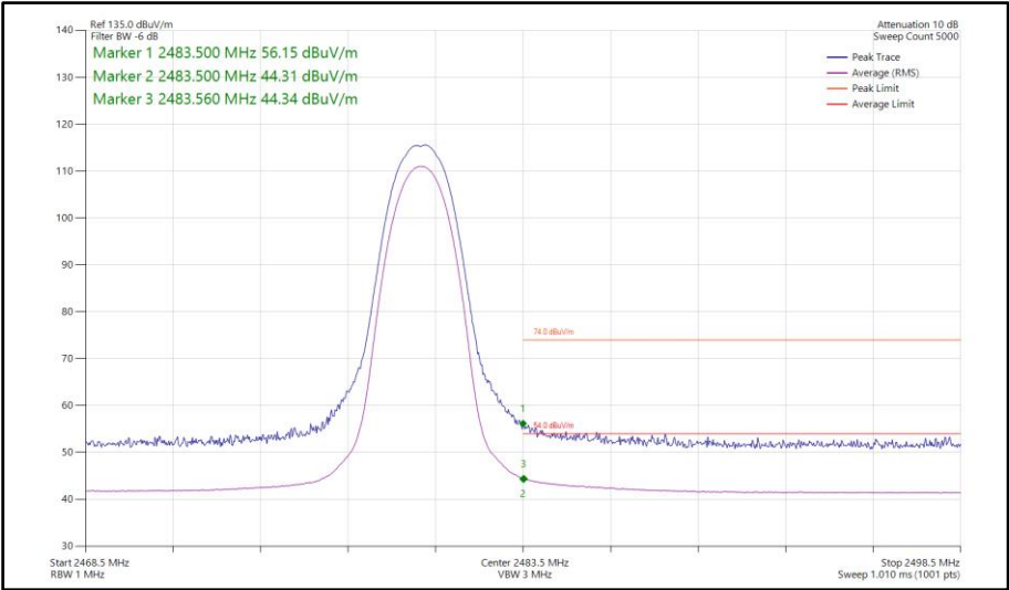
Figure 451 - Bluetooth 2DH5, SISO, Core 0 - 2480 MHz Band Edge Frequency 2483.5 MHz
