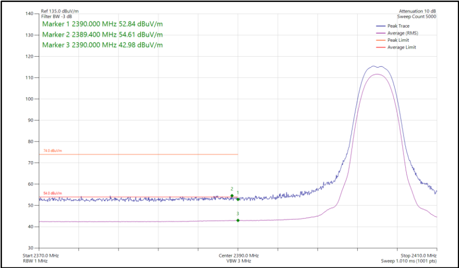
Figure 443 - Bluetooth HDT3, SISO, Core 0 - 2404 MHz Band Edge Frequency 2390 MHz
