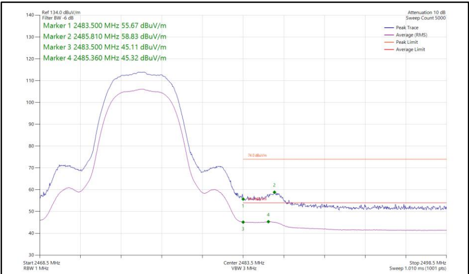
Figure 454 - Bluetooth HDR8, SISO, Core 0 - 2476 MHz Band Edge Frequency 2483.5 MHz
