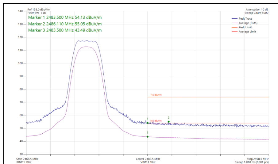
Figure 488 - Bluetooth HDRPS2, SISO, Core 1 - 2476 MHz Band Edge Frequency 2483.5 MHz
