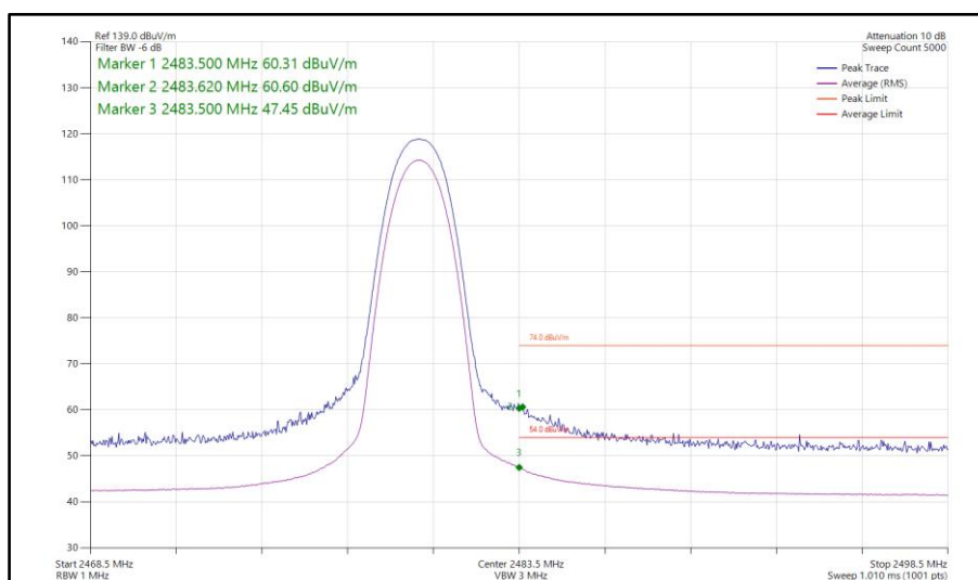
Figure 480 - Bluetooth 3DH5, SISO, Core 1 - 2480 MHz Band Edge Frequency 2483.5 MHz
