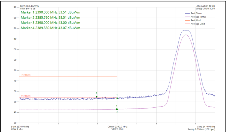
Figure 470 - Bluetooth LE2M, SISO, Core 1 - 2404 MHz Band Edge Frequency 2390 MHz
