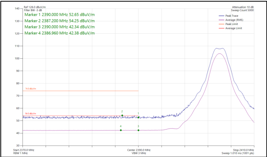
Figure 422 - Bluetooth CS1LE2M, MIMO, Core 0-1 - 2404 MHz Band Edge Frequency 2390 MHz
