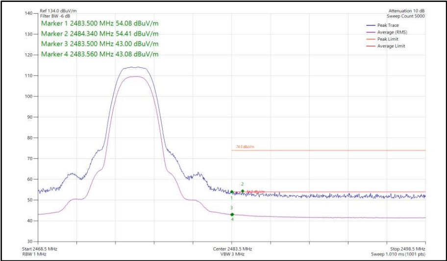
Figure 457 - Bluetooth HDT3, SISO, Core 0 - 2476 MHz Band Edge Frequency 2483.5 MHz
