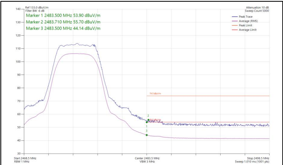
Figure 462 - Bluetooth XHDRPM8, SISO, Core 0 - 2475 MHz Band Edge Frequency 2483.5 MHz
