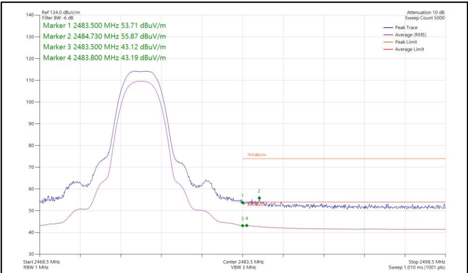
Figure 458 - Bluetooth HDT4, SISO, Core 0 - 2476 MHz Band Edge Frequency 2483.5 MHz
