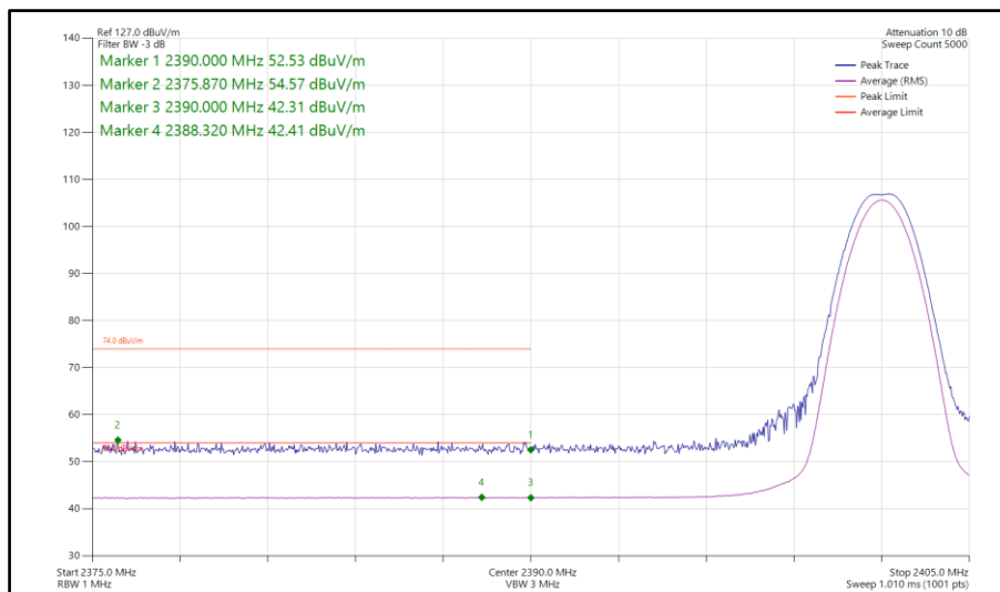
Figure 413 - Bluetooth LE1M, MIMO, Core 0-1 - 2402 MHz Band Edge Frequency 2390 MHz
