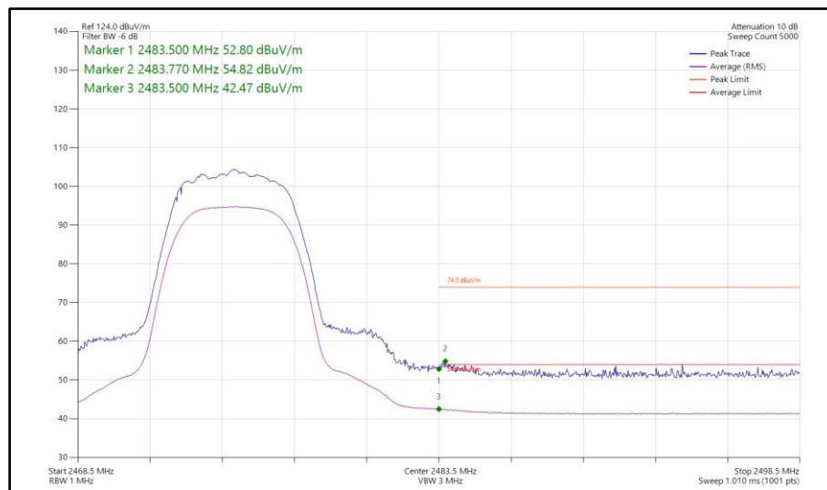
Figure 433 - Bluetooth HDRPM12, MIMO, Core 0-1 - 2475 MHz Band Edge Frequency 2483.5 MHz
