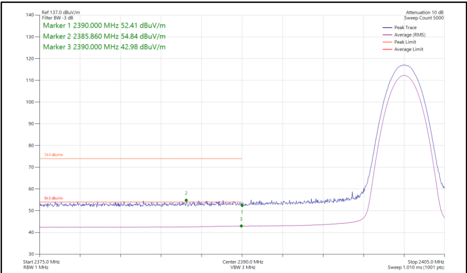
Figure 438 - Bluetooth 3DH5, SISO, Core 0 - 2402 MHz Band Edge Frequency 2390 MHz
