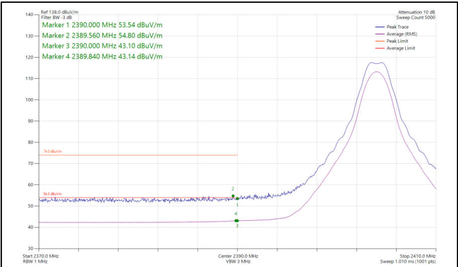
Figure 478 - Bluetooth CS1LE2M, SISO, Core 1 - 2404 MHz Band Edge Frequency 2390 MHz
