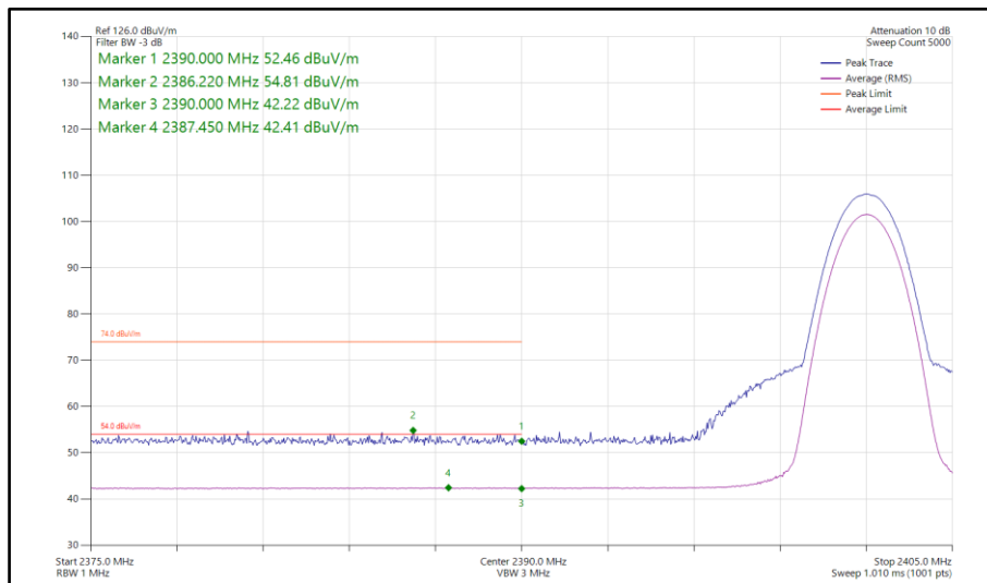
Figure 410 - Bluetooth 3DH5, MIMO, Core 0-1 - 2402 MHz Band Edge Frequency 2390 MHz
