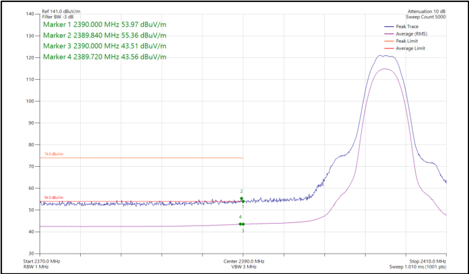
Figure 473 - Bluetooth HDT6, SISO, Core 1 - 2404 MHz Band Edge Frequency 2390 MHz
