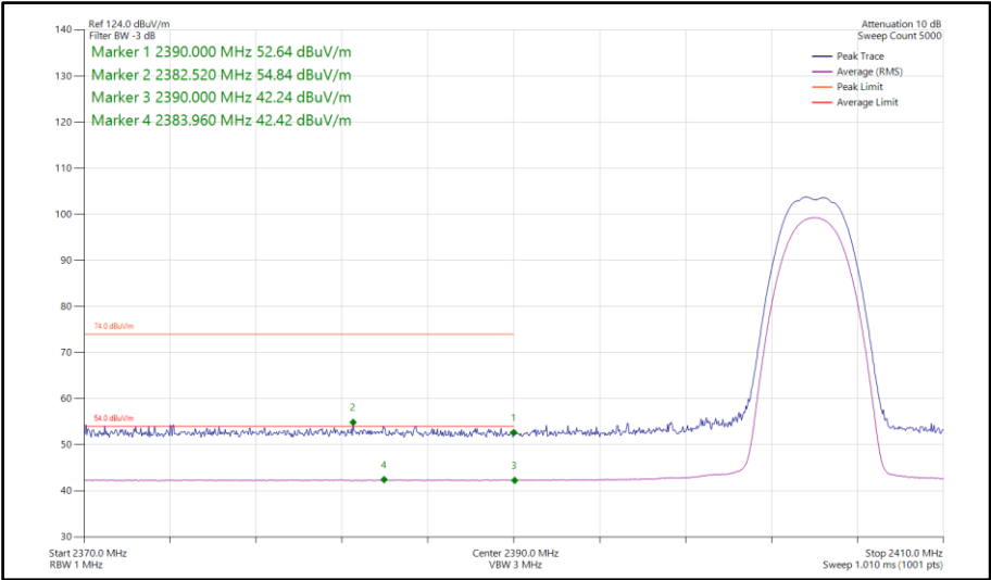
Figure 411 - Bluetooth HDR4, MIMO, Core 0-1 - 2404 MHz Band Edge Frequency 2390 MHz
