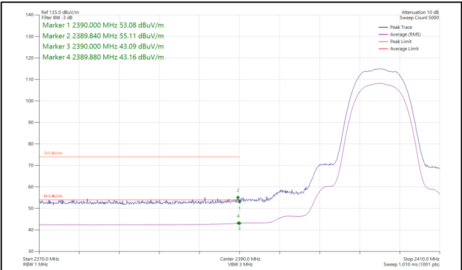
Figure 440 - Bluetooth HDR8, SISO, Core 0 - 2404 MHz Band Edge Frequency 2390 MHz
