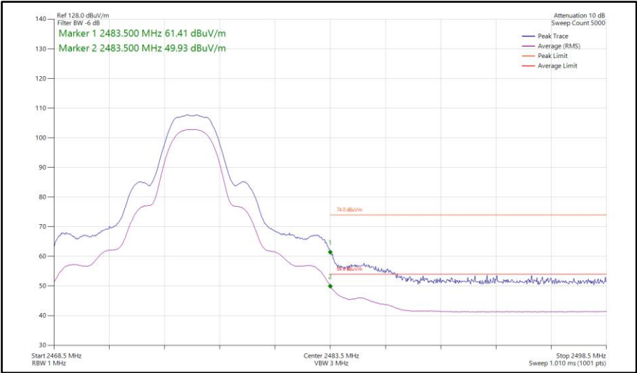
Figure 429 - Bluetooth HDT3, MIMO, Core 0-1 - 2476 MHz Band Edge Frequency 2483.5 MHz
