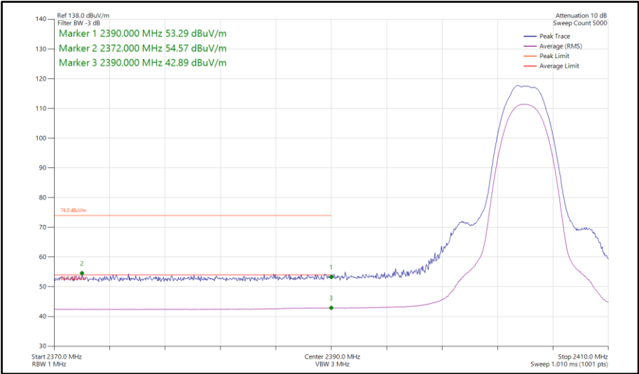
Figure 445 - Bluetooth HDT6, SISO, Core 0 - 2404 MHz Band Edge Frequency 2390 MHz
