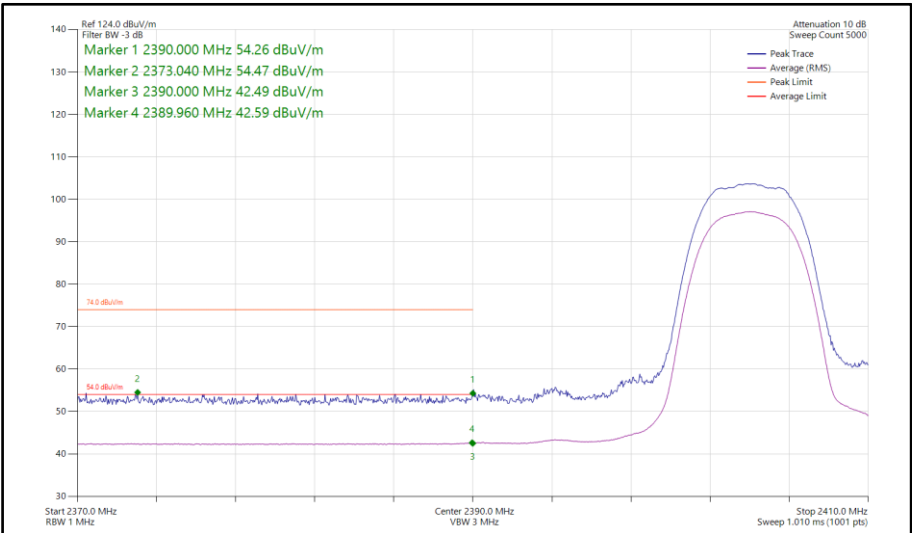
Figure 412 - Bluetooth HDR8, MIMO, Core 0-1 - 2404 MHz Band Edge Frequency 2390 MHz
