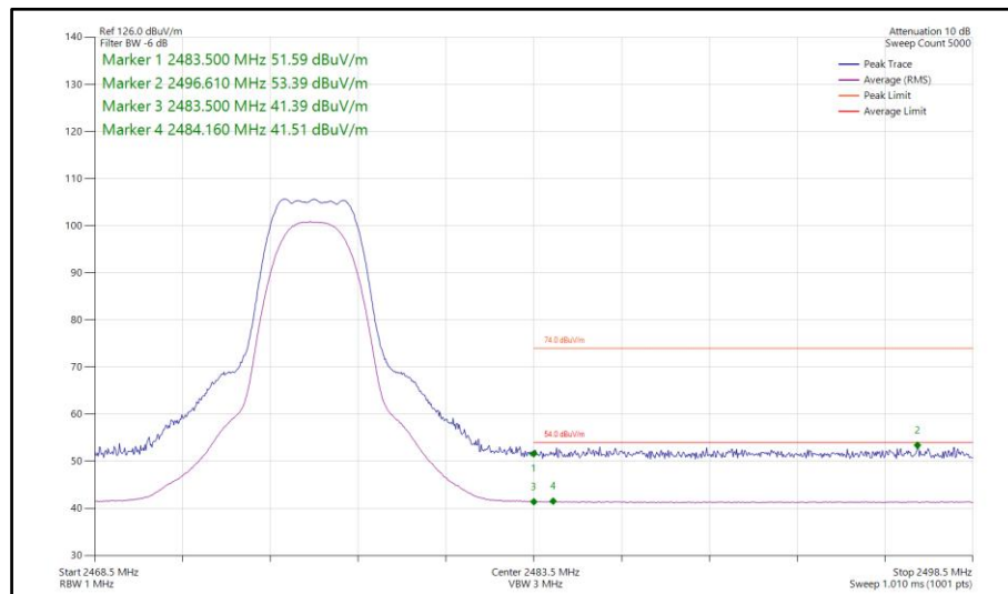
Figure 432 - Bluetooth HDRPS2, MIMO, Core 0-1 - 2476 MHz Band Edge Frequency 2483.5 MHz
