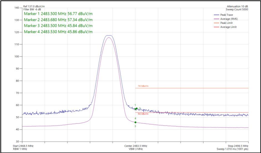
Figure 483 - Bluetooth LE1M, SISO, Core 1 - 2480 MHz Band Edge Frequency 2483.5 MHz
