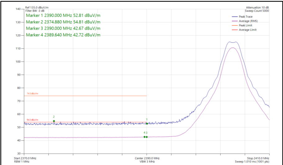
Figure 450 - Bluetooth CS1LE2M, SISO, Core 0 - 2404 MHz Band Edge Frequency 2390 MHz
