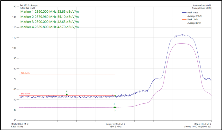
Figure 447 - Bluetooth HDRPM12, SISO, Core 0 - 2404 MHz Band Edge Frequency 2390 MHz
