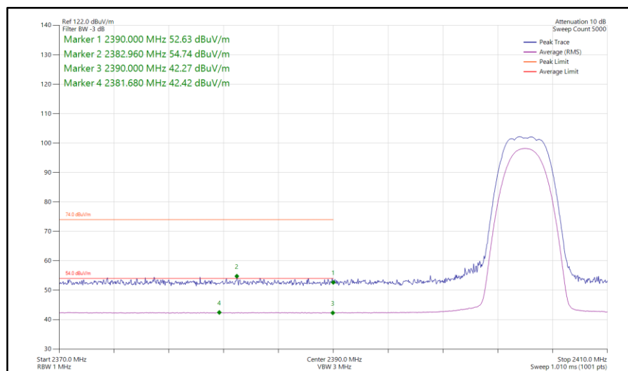
Figure 418 - Bluetooth HDRPS2, MIMO, Core 0-1 - 2404 MHz Band Edge Frequency 2390 MHz
