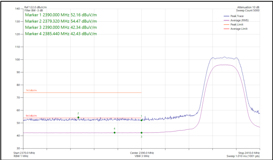
Figure 420 - Bluetooth XHDRPM8, MIMO, Core 0-1 - 2404 MHz Band Edge Frequency 2390 MHz
