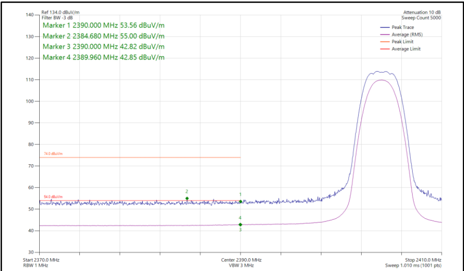
Figure 474 - Bluetooth HDRPS2, SISO, Core 1 - 2404 MHz Band Edge Frequency 2390 MHz
