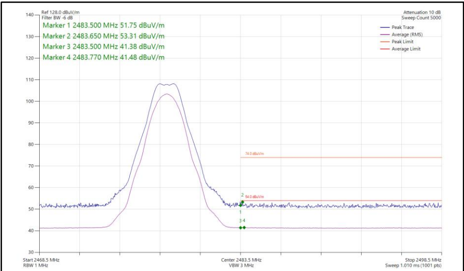
Figure 428 - Bluetooth LE2M, MIMO, Core 0-1 - 2478 MHz Band Edge Frequency 2483.5 MHz
