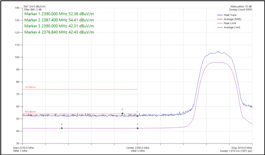
Figure 419 - Bluetooth HDRPM12, MIMO, Core 0-1 - 2404 MHz Band Edge Frequency 2390 MHz
