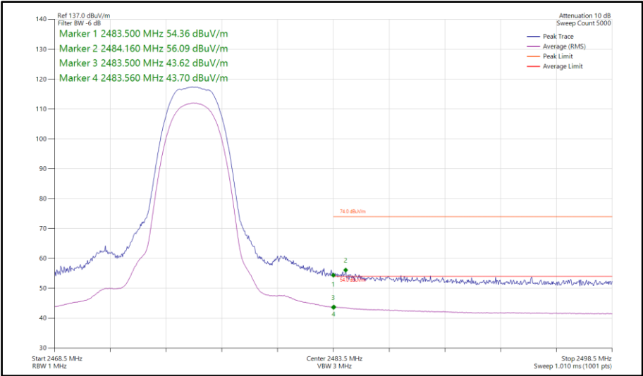
Figure 481 - Bluetooth HDR4, SISO, Core 1 - 2476 MHz Band Edge Frequency 2483.5 MHz
