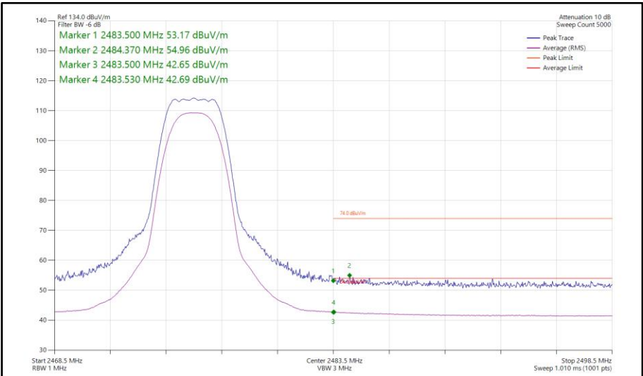
Figure 460 - Bluetooth HDRPS2, SISO, Core 0 - 2476 MHz Band Edge Frequency 2483.5 MHz
