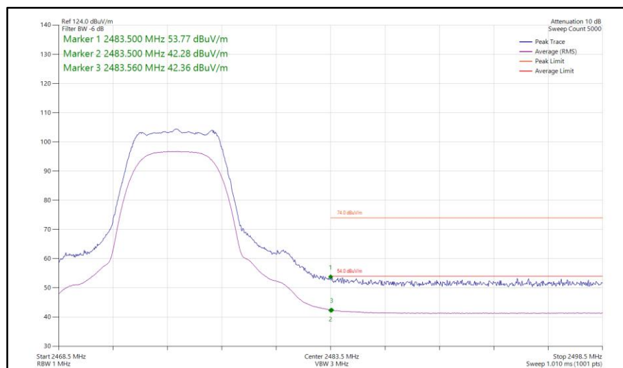
Figure 434 - Bluetooth XHDRPM8, MIMO, Core 0-1 - 2475 MHz Band Edge Frequency 2483.5 MHz
