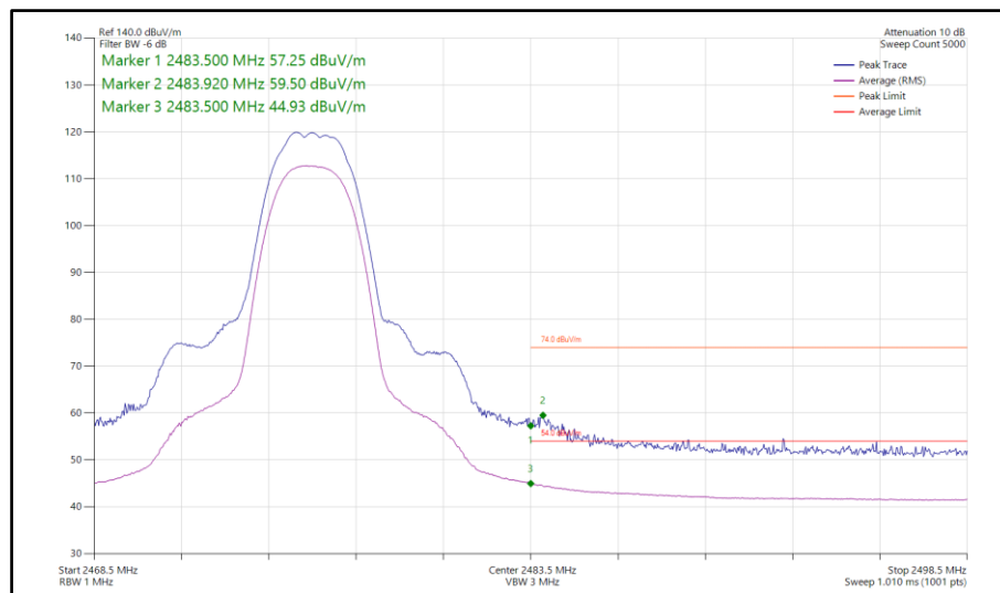
Figure 487 - Bluetooth HDT6, SISO, Core 1 - 2476 MHz Band Edge Frequency 2483.5 MHz
