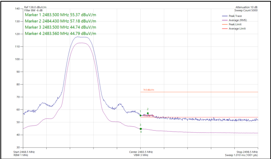
Figure 486 - Bluetooth HDT4, SISO, Core 1 - 2476 MHz Band Edge Frequency 2483.5 MHz
