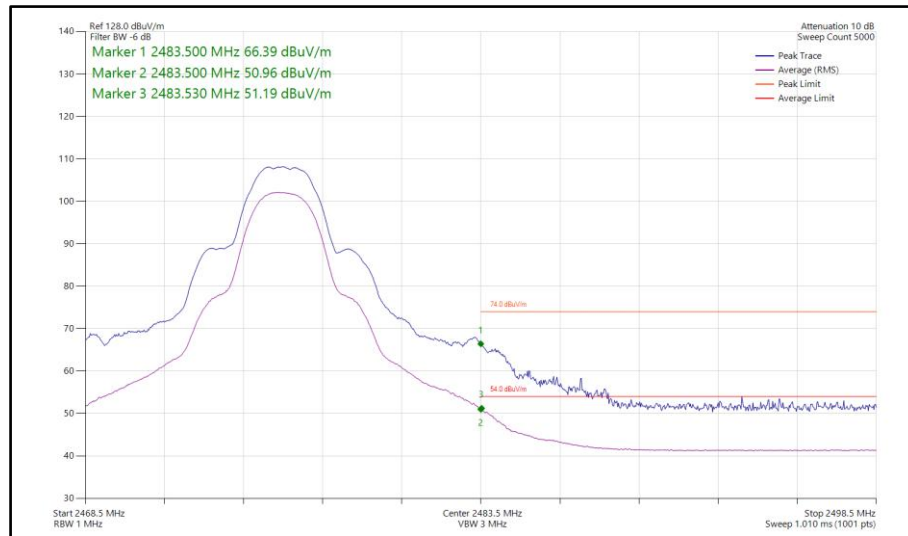
Figure 431 - Bluetooth HDT6, MIMO, Core 0-1 - 2476 MHz Band Edge Frequency 2483.5 MHz
