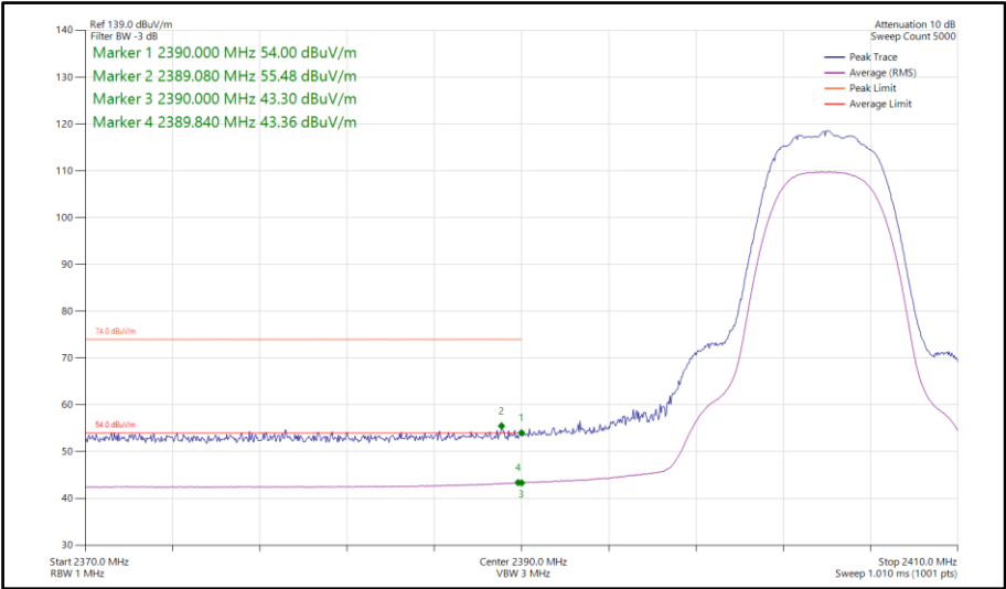
Figure 475 - Bluetooth HDRPM12, SISO, Core 1 - 2404 MHz Band Edge Frequency 2390 MHz
