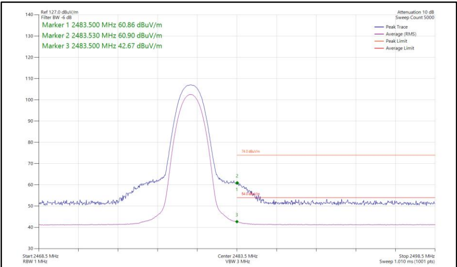
Figure 424 - Bluetooth 3DH5, MIMO, Core 0-1 - 2480 MHz Band Edge Frequency 2483.5 MHz
