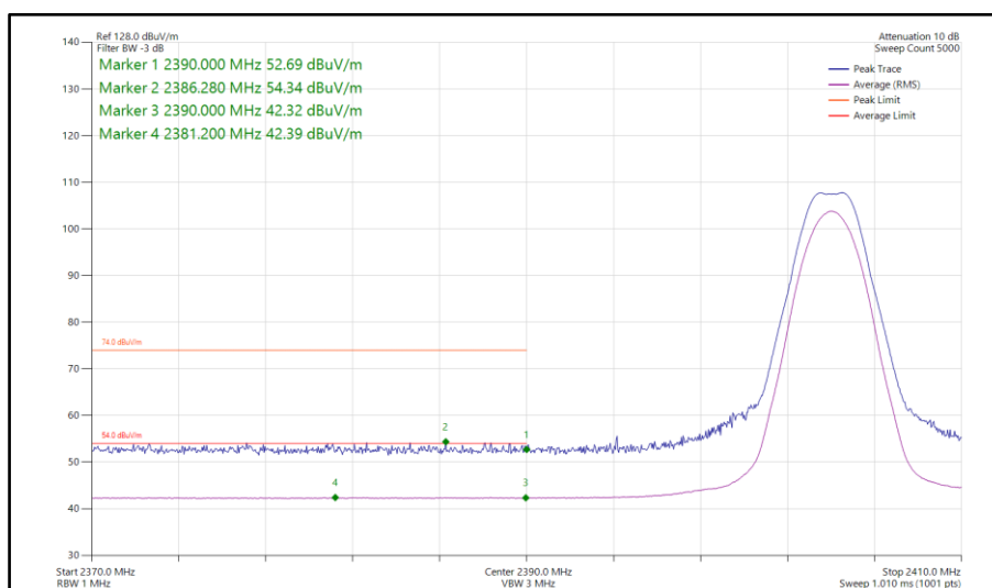
Figure 414 - Bluetooth LE2M, MIMO, Core 0-1 - 2404 MHz Band Edge Frequency 2390 MHz
