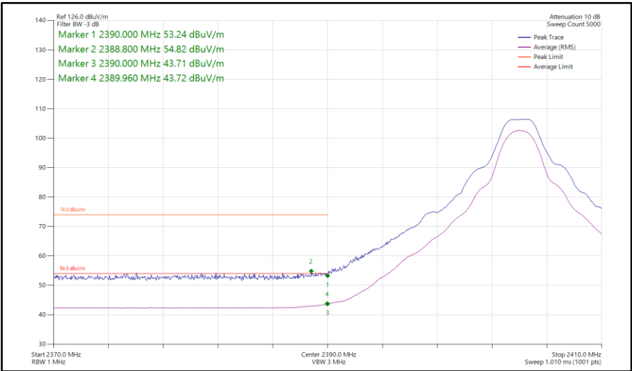
Figure 416 - Bluetooth HDT4, MIMO, Core 0-1 - 2404 MHz Band Edge Frequency 2390 MHz
