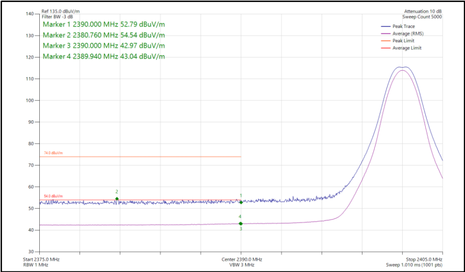
Figure 449 - Bluetooth CS1LE1M, SISO, Core 0 - 2402 MHz Band Edge Frequency 2390 MHz
