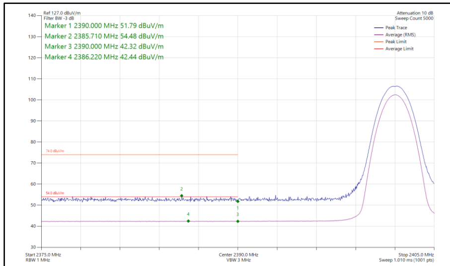
Figure 409 - Bluetooth 2DH5, MIMO, Core 0-1 - 2402 MHz Band Edge Frequency 2390 MHz
