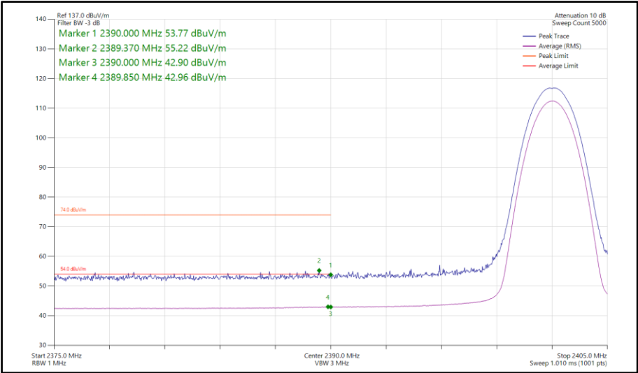
Figure 437 - Bluetooth 2DH5, SISO, Core 0 - 2402 MHz Band Edge Frequency 2390 MHz
