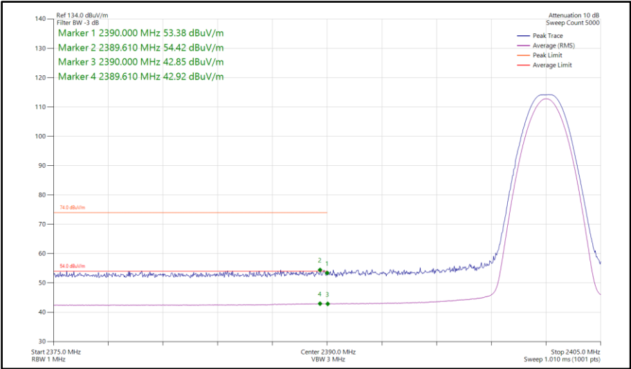
Figure 441 - Bluetooth LE1M, SISO, Core 0 - 2402 MHz Band Edge Frequency 2390 MHz
