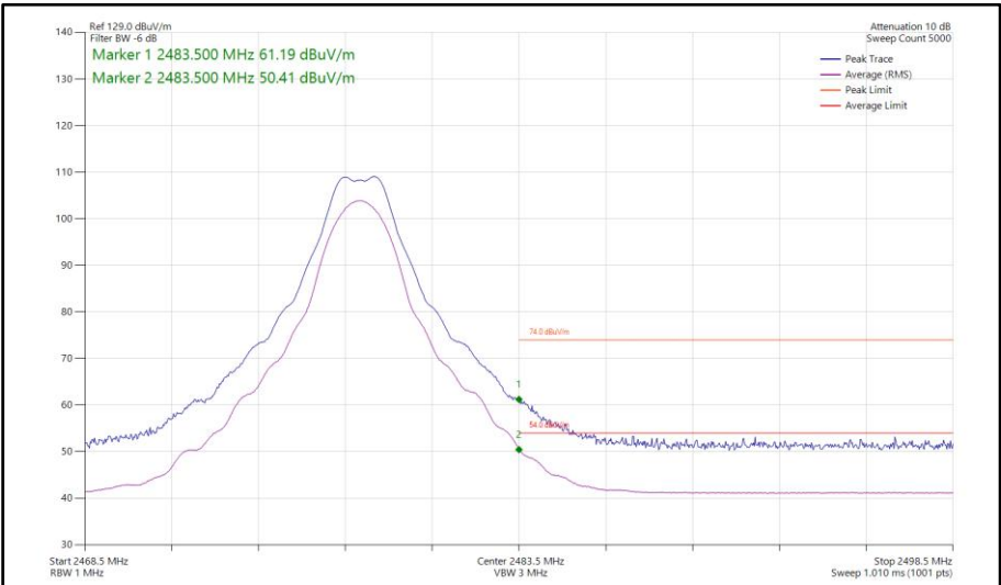
Figure 436 - Bluetooth CS1LE2M, MIMO, Core 0-1 - 2478 MHz Band Edge Frequency 2483.5 MHz
