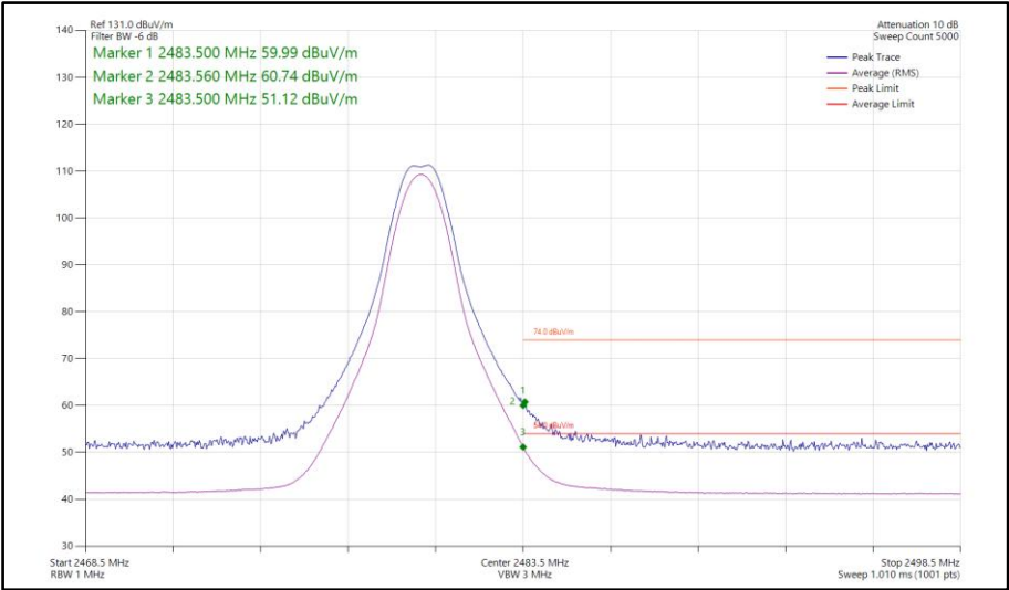
Figure 463 - Bluetooth CS1LE1M, SISO, Core 0 - 2480 MHz Band Edge Frequency 2483.5 MHz
