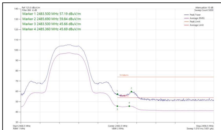
Figure 426 - Bluetooth HDR8, MIMO, Core 0-1 - 2476 MHz Band Edge Frequency 2483.5 MHz
