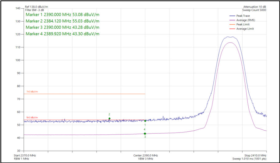
Figure 467 - Bluetooth HDR4, SISO, Core 1 - 2404 MHz Band Edge Frequency 2390 MHz
