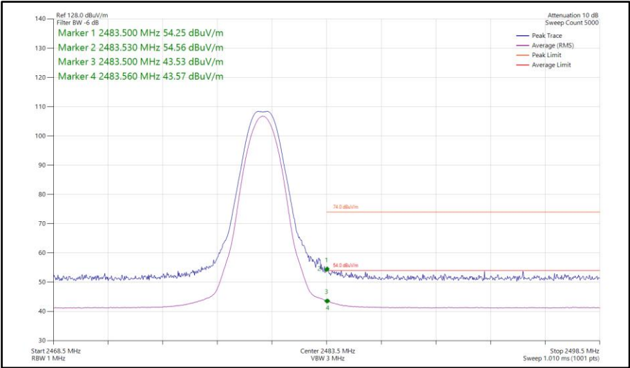
Figure 427 - Bluetooth LE1M, MIMO, Core 0-1 - 2480 MHz Band Edge Frequency 2483.5 MHz
