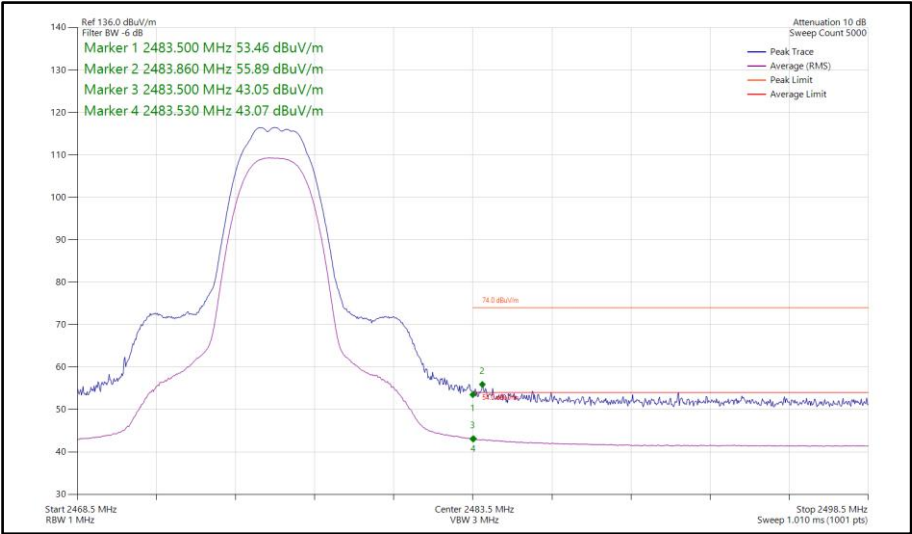
Figure 459 - Bluetooth HDT6, SISO, Core 0 - 2476 MHz Band Edge Frequency 2483.5 MHz
