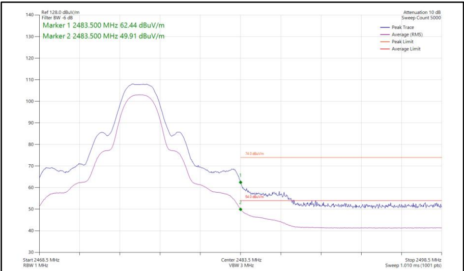
Figure 430 - Bluetooth HDT4, MIMO, Core 0-1 - 2476 MHz Band Edge Frequency 2483.5 MHz
