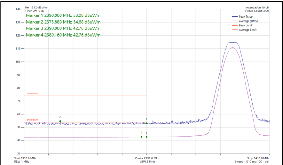
Figure 442 - Bluetooth LE2M, SISO, Core 0 - 2404 MHz Band Edge Frequency 2390 MHz
