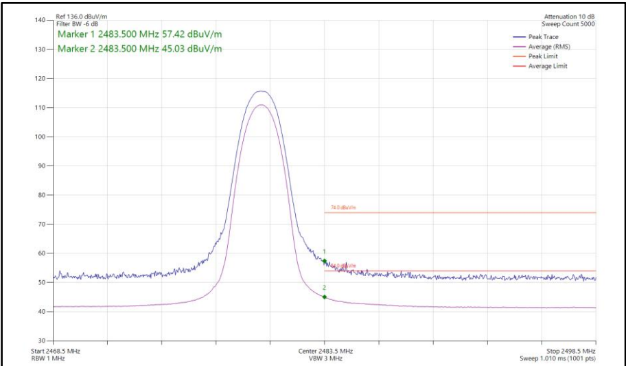
Figure 452 - Bluetooth 3DH5, SISO, Core 0 - 2480 MHz Band Edge Frequency 2483.5 MHz
