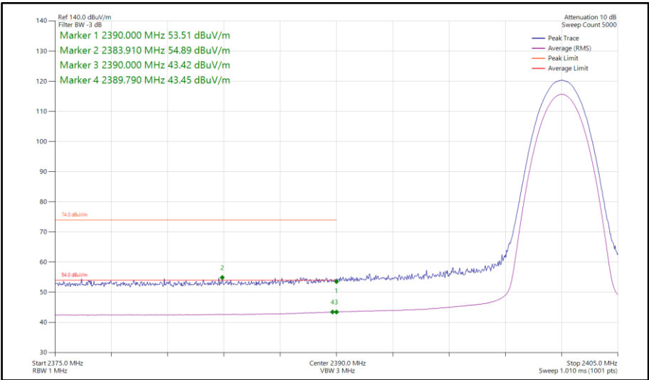
Figure 466 - Bluetooth 3DH5, SISO, Core 1 - 2402 MHz Band Edge Frequency 2390 MHz
