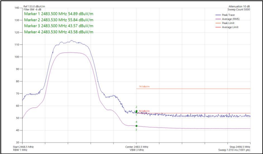
Figure 461 - Bluetooth HDRPM12, SISO, Core 0 - 2475 MHz Band Edge Frequency 2483.5 MHz
