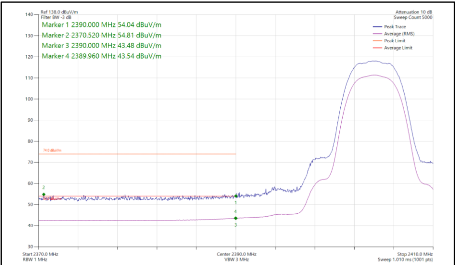
Figure 468 - Bluetooth HDR8, SISO, Core 1 - 2404 MHz Band Edge Frequency 2390 MHz
