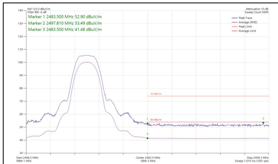
Figure 425 - Bluetooth HDR4, MIMO, Core 0-1 - 2476 MHz Band Edge Frequency 2483.5 MHz
