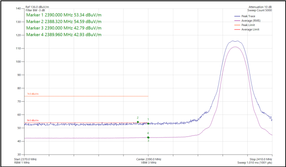
Figure 439 - Bluetooth HDR4, SISO, Core 0 - 2404 MHz Band Edge Frequency 2390 MHz
