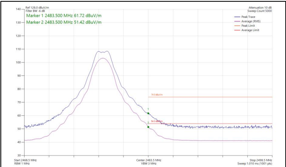
Figure 464 - Bluetooth CS1LE2M, SISO, Core 0 - 2478 MHz Band Edge Frequency 2483.5 MHz
