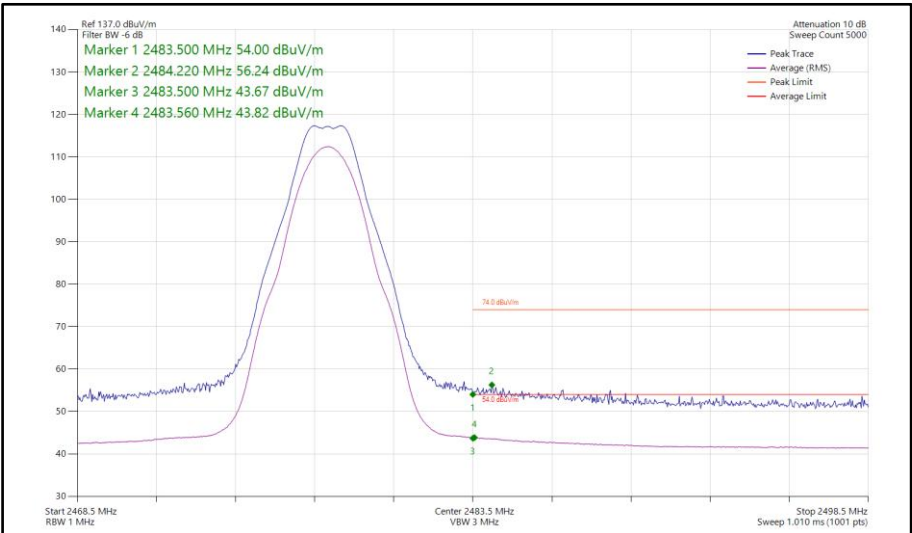
Figure 484 - Bluetooth LE2M, SISO, Core 1 - 2478 MHz Band Edge Frequency 2483.5 MHz
