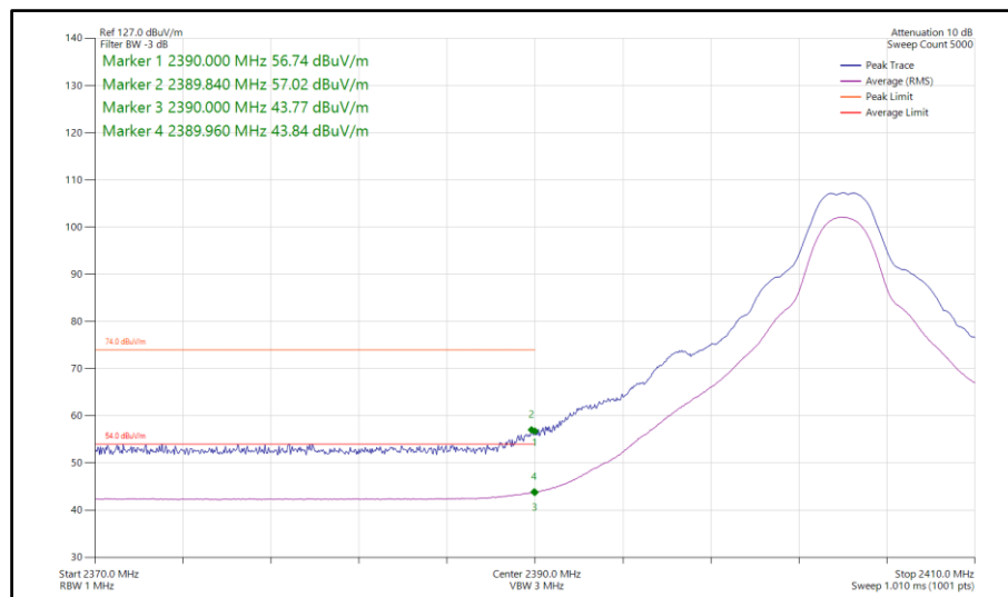
Figure 417 - Bluetooth HDT6, MIMO, Core 0-1 - 2404 MHz Band Edge Frequency 2390 MHz
