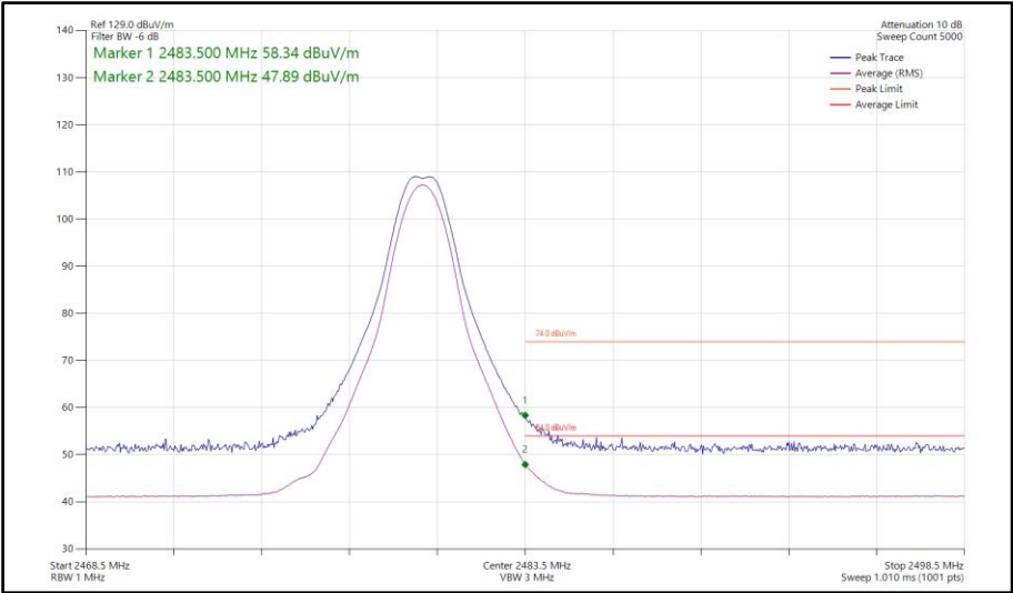
Figure 435 - Bluetooth CS1LE1M, MIMO, Core 0-1 - 2480 MHz Band Edge Frequency 2483.5 MHz
