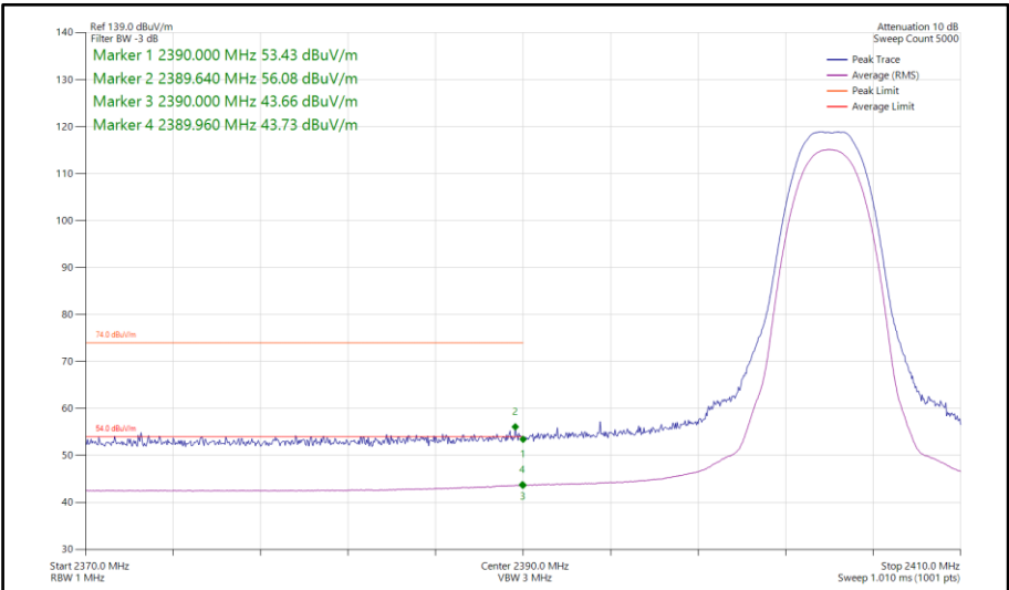
Figure 472 - Bluetooth HDT4, SISO, Core 1 - 2404 MHz Band Edge Frequency 2390 MHz
