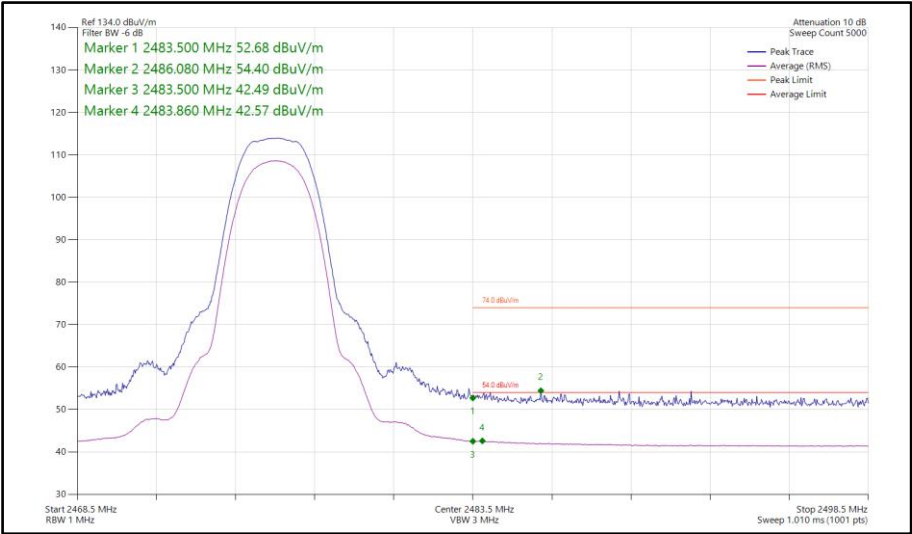
Figure 453 - Bluetooth HDR4, SISO, Core 0 - 2476 MHz Band Edge Frequency 2483.5 MHz
