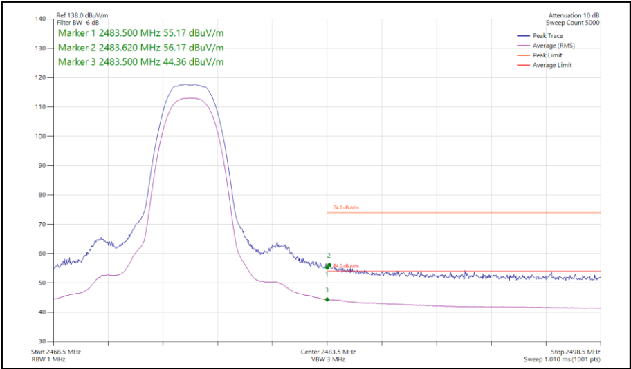
Figure 485 - Bluetooth HDT3, SISO, Core 1 - 2476 MHz Band Edge Frequency 2483.5 MHz
