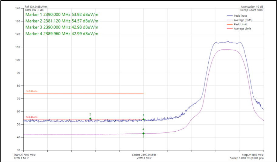
Figure 448 - Bluetooth XHDRPM8, SISO, Core 0 - 2404 MHz Band Edge Frequency 2390 MHz
