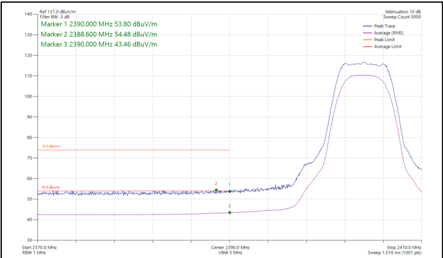
Figure 476 - Bluetooth XHDRPM8, SISO, Core 1 - 2404 MHz Band Edge Frequency 2390 MHz
