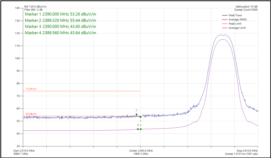
Figure 471 - Bluetooth HDT3, SISO, Core 1 - 2404 MHz Band Edge Frequency 2390 MHz
