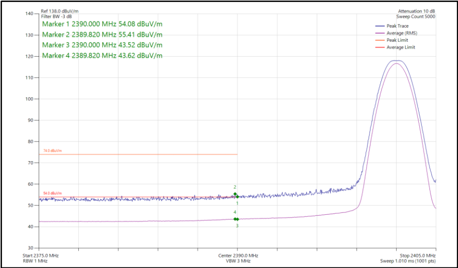
Figure 469 - Bluetooth LE1M, SISO, Core 1 - 2402 MHz Band Edge Frequency 2390 MHz
