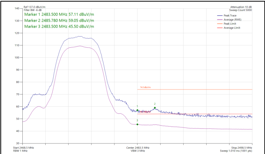
Figure 482 - Bluetooth HDR8, SISO, Core 1 - 2476 MHz Band Edge Frequency 2483.5 MHz
