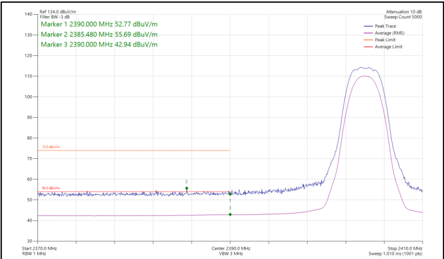
Figure 446 - Bluetooth HDRPS2, SISO, Core 0 - 2404 MHz Band Edge Frequency 2390 MHz
