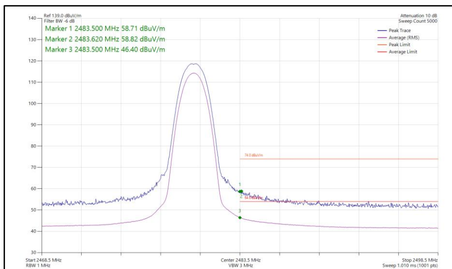
Figure 479 - Bluetooth 2DH5, SISO, Core 1 - 2480 MHz Band Edge Frequency 2483.5 MHz
