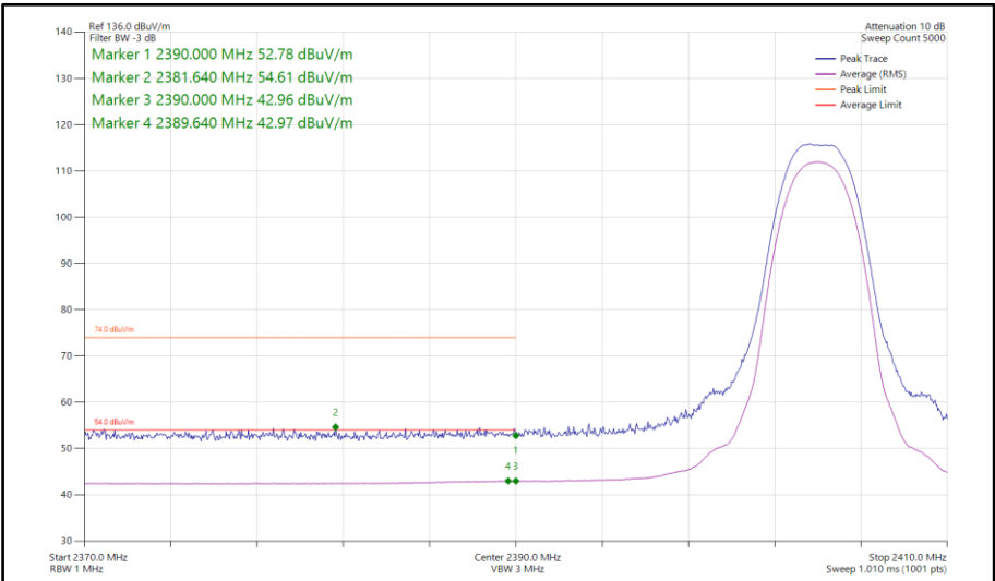
Figure 444 - Bluetooth HDT4, SISO, Core 0 - 2404 MHz Band Edge Frequency 2390 MHz
