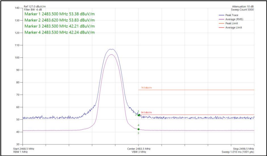
Figure 423 - Bluetooth 2DH5, MIMO, Core 0-1 - 2480 MHz Band Edge Frequency 2483.5 MHz
