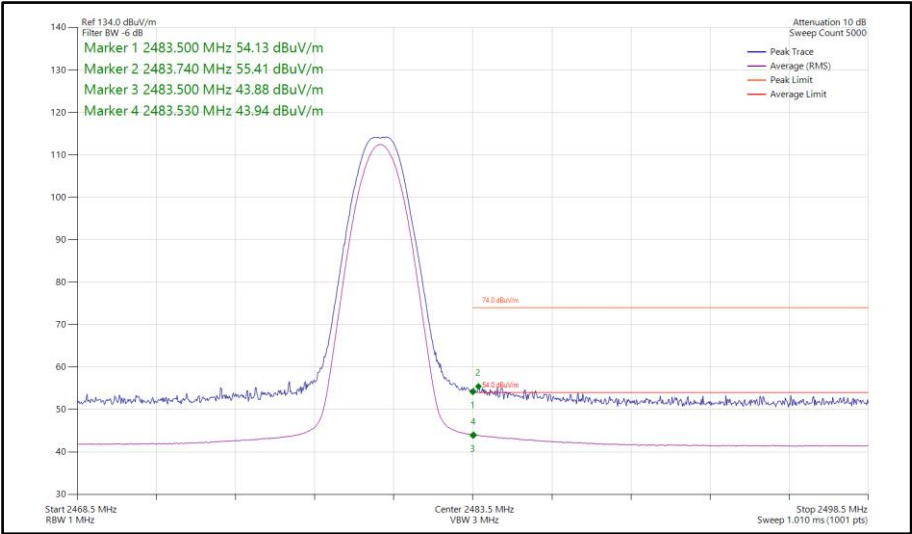
Figure 455 - Bluetooth LE1M, SISO, Core 0 - 2480 MHz Band Edge Frequency 2483.5 MHz
