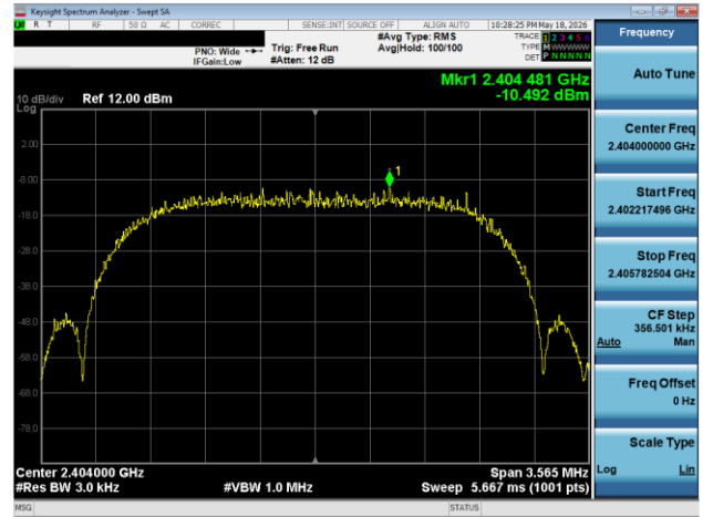
Plot 7-76. Power Spectral Density Plot Antenna WF8 (Bluetooth (HDRPS2), 2Mbps, iPA - Ch. 1)
