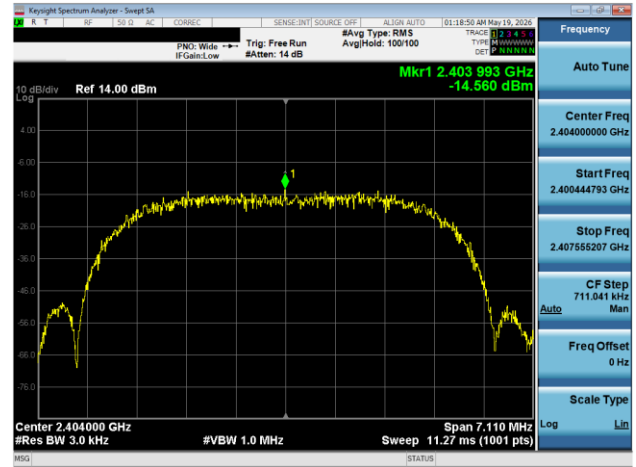
Plot 7-112. Power Spectral Density Plot Antenna WF7 (Bluetooth (XHDRPM6), 6 Mbps, iPA – Ch. 1)
