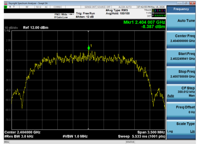
Plot 7-64. Power Spectral Density Plot Antenna WF8 (Bluetooth (HDR4), 4 Mbps, iPA – Ch. 1)
