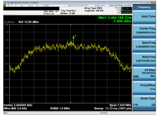
Plot 7-100. Power Spectral Density Plot Antenna WF7 (Bluetooth (HDR8), 8 Mbps, iPA – Ch. 1)
