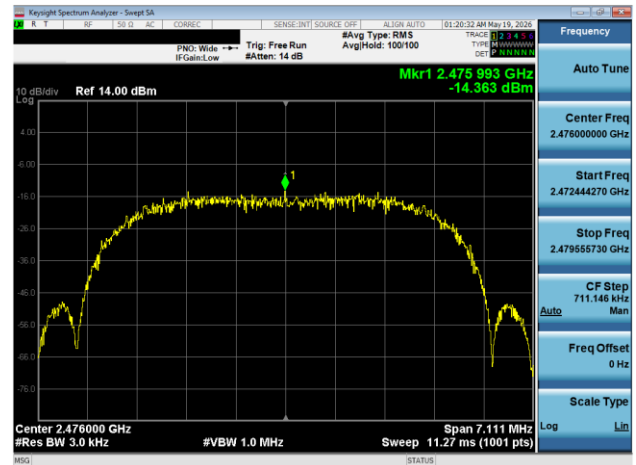
Plot 7-114. Power Spectral Density Plot Antenna WF7 (Bluetooth (XHDRPM6), 6 Mbps, iPA – Ch. 73)
