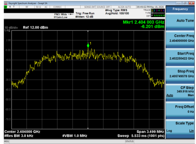
Plot 7-94. Power Spectral Density Plot Antenna WF7 (Bluetooth (HDR4), 4 Mbps, iPA – Ch. 1)
