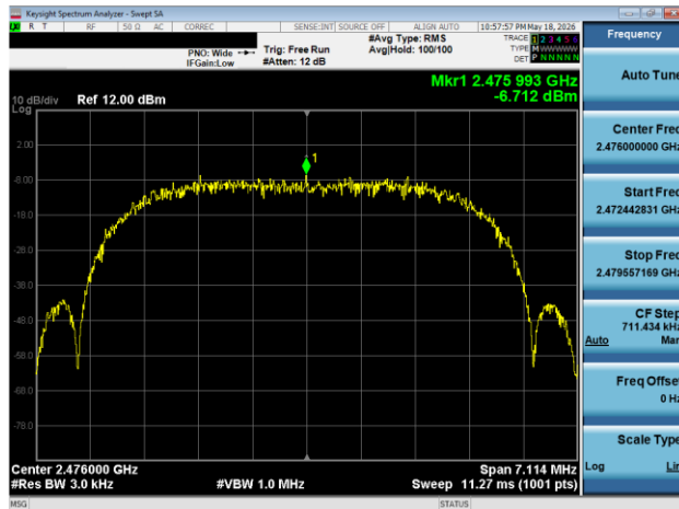
Plot 7-81. Power Spectral Density Plot Antenna WF8 (Bluetooth (XHDRPM6), 6 Mbps, ePA - Ch. 73)
