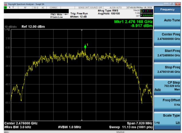
Plot 7-72. Power Spectral Density Plot Antenna WF8 (Bluetooth (HDR), 8 Mbps, iPA – Ch. 73)
