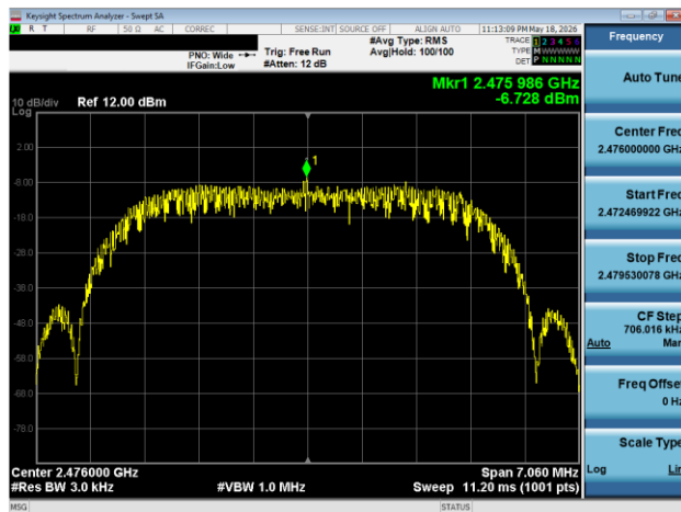
Plot 7-87. Power Spectral Density Plot Antenna WF8 (Bluetooth (HDRPM16), 16 Mbps, ePA – Ch. 73)
