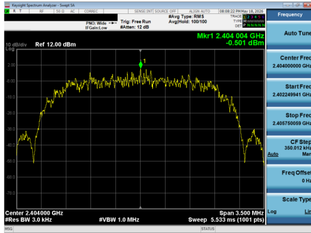
Plot 7-121. Power Spectral Density Plot TxBF Antenna WF8 (Bluetooth (HDR4), 4 Mbps, ePA – Ch. 1)
