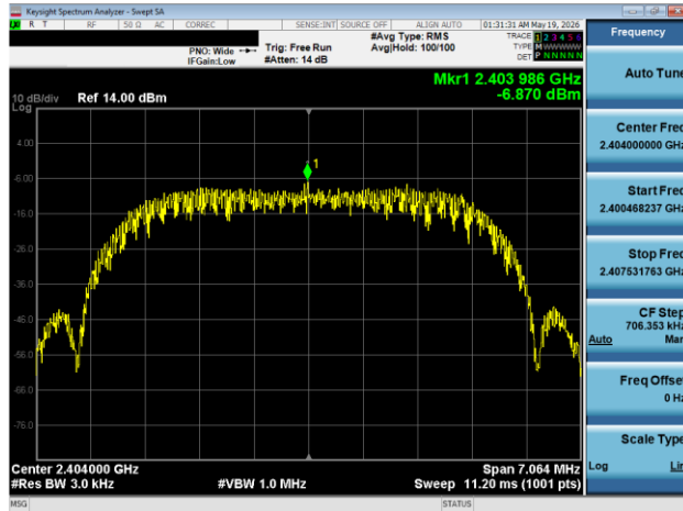
Plot 7-115. Power Spectral Density Plot Antenna WF7 (Bluetooth (HDRPM16), 16 Mbps, ePA – Ch. 1)
