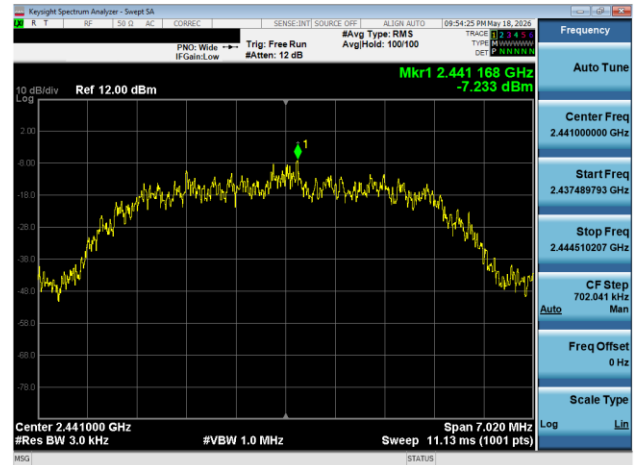
Plot 7-101. Power Spectral Density Plot Antenna WF7 (Bluetooth (HDR8), 8 Mbps, iPA – Ch. 38)
