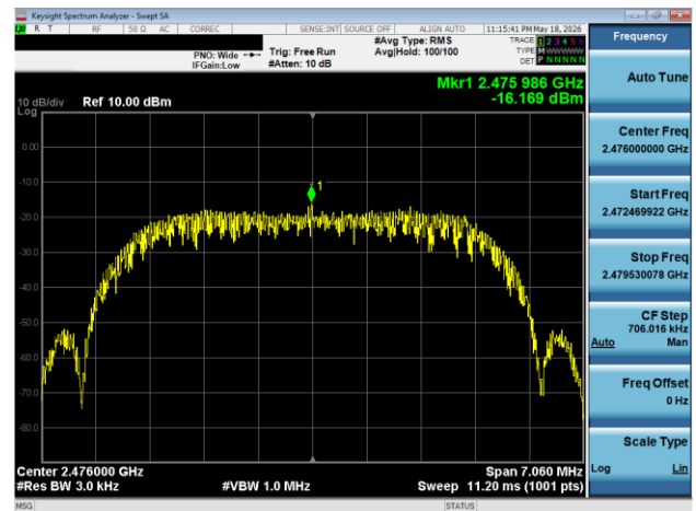
Plot 7-90. Power Spectral Density Plot Antenna WF8 (Bluetooth (HDRPM16), 16 Mbps, iPA – Ch. 73)
