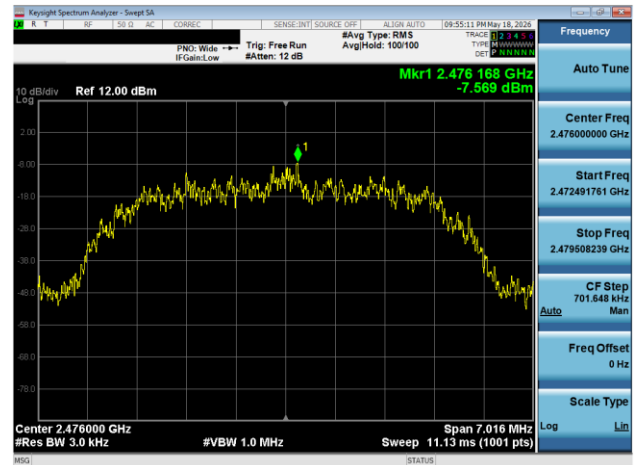
Plot 7-102. Power Spectral Density Plot Antenna WF7 (Bluetooth (HDR8), 8 Mbps, iPA – Ch. 73)
