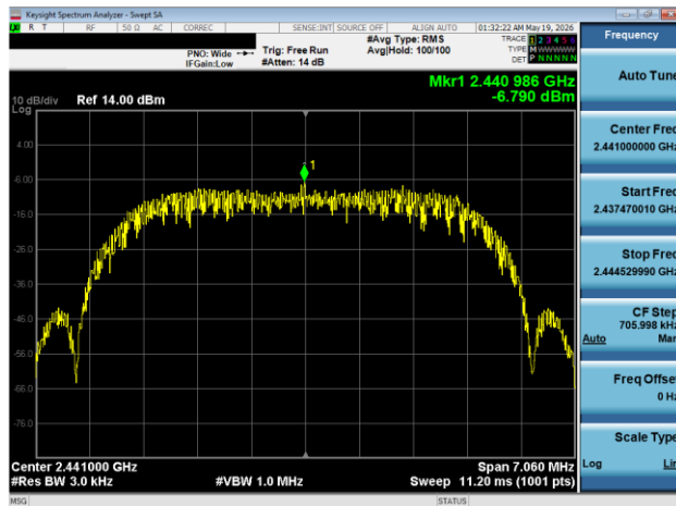
Plot 7-116. Power Spectral Density Plot Antenna WF7 (Bluetooth (HDRPM16), 16 Mbps, ePA – Ch. 38)
