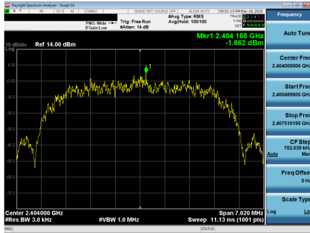
Plot 7-97. Power Spectral Density Plot Antenna WF7 (Bluetooth (HDR8), 8 Mbps, ePA – Ch. 1)
