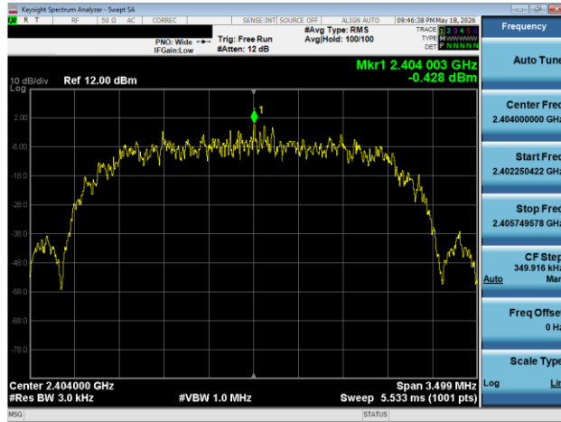
Plot 7-91. Power Spectral Density Plot Antenna WF7 (Bluetooth (HDR4), 4 Mbps, ePA – Ch. 1)
