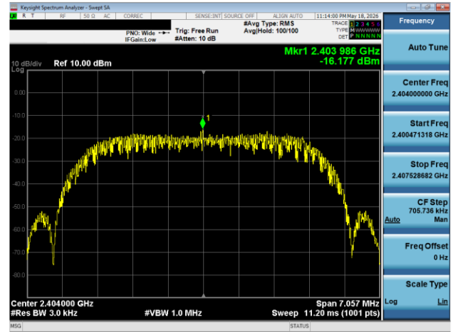
Plot 7-88. Power Spectral Density Plot Antenna WF8 (Bluetooth (HDRPM16), 16 Mbps, iPA – Ch. 1)
