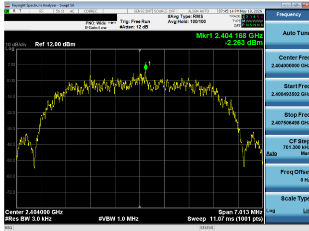
Plot 7-67. Power Spectral Density Plot Antenna WF8 (Bluetooth (HDR), 8 Mbps, ePA – Ch. 1)
