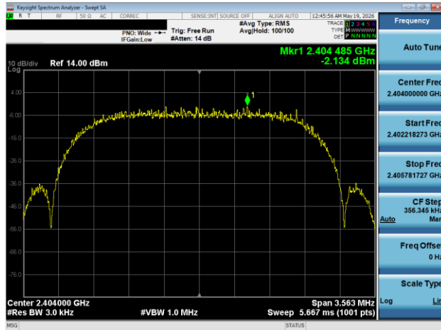
Plot 7-103. Power Spectral Density Plot Antenna WF7 (Bluetooth (HDRPS2), 2Mbps, ePA – Ch. 1)
