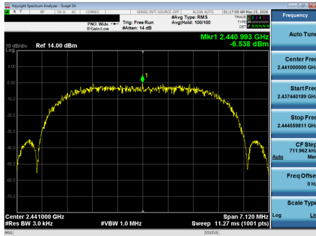
Plot 7-110. Power Spectral Density Plot Antenna WF7 (Bluetooth (XHDRPM6), 6 Mbps, ePA – Ch. 38)
