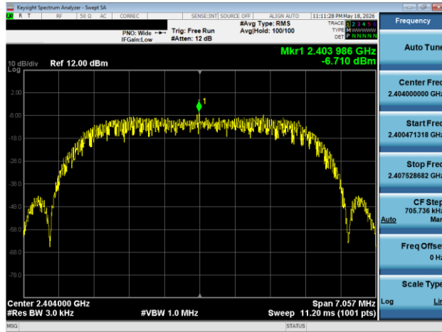
Plot 7-85. Power Spectral Density Plot Antenna WF8 (Bluetooth (HDRPM16), 16 Mbps, ePA – Ch. 1)
