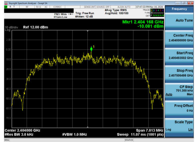
Plot 7-70. Power Spectral Density Plot Antenna WF8 (Bluetooth (HDR), 8 Mbps, iPA – Ch. 1)
