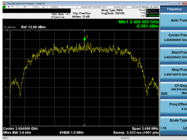
Plot 7-122. Power Spectral Density Plot TxBF Antenna WF7 (Bluetooth (HDR4), 4 Mbps, ePA – Ch. 1)
