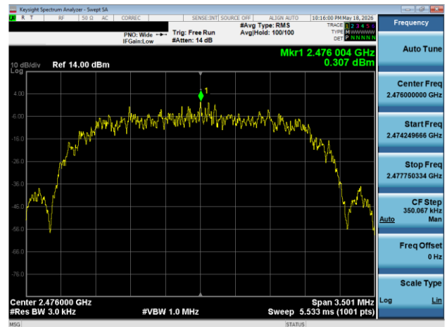
Plot 7-126. Power Spectral Density Plot TxBF Antenna WF7 (Bluetooth (HDR4), 4 Mbps, ePA – Ch. 73)
