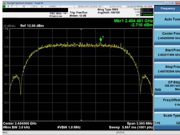
Plot 7-73. Power Spectral Density Plot Antenna WF8 (Bluetooth (HDRPS2), 2Mbps, ePA - Ch. 1)
