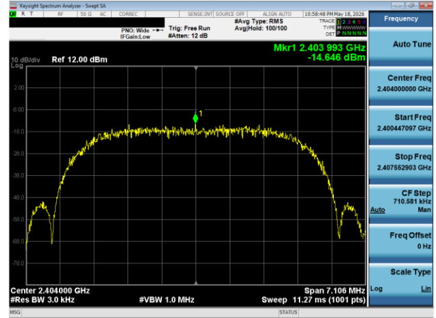
Plot 7-82. Power Spectral Density Plot Antenna WF8 (Bluetooth (XHDRPM6), 6 Mbps, iPA - Ch. 1)
