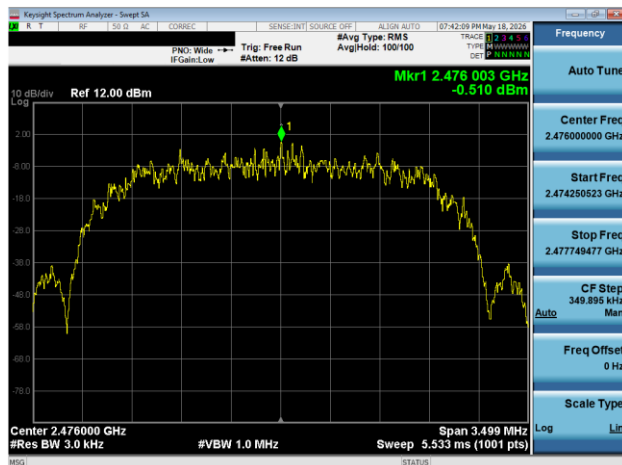
Plot 7-63. Power Spectral Density Plot Antenna WF8 (Bluetooth (HDR4), 4 Mbps, ePA – Ch. 73)
