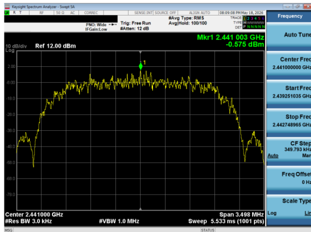
Plot 7-123. Power Spectral Density Plot TxBF Antenna WF8 (Bluetooth (HDR4), 4 Mbps, ePA – Ch. 38)
