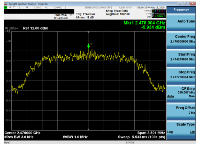
Plot 7-96. Power Spectral Density Plot Antenna WF7 (Bluetooth (HDR4), 4 Mbps, iPA – Ch. 73)
