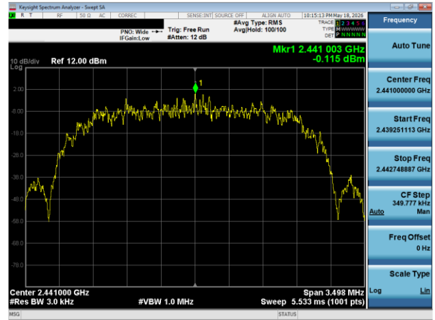
Plot 7-124. Power Spectral Density Plot TxBF Antenna WF7 (Bluetooth (HDR4), 4 Mbps, ePA – Ch. 38)
