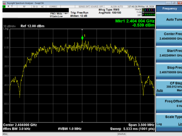
Plot 7-61. Power Spectral Density Plot Antenna WF8 (Bluetooth (HDR4), 4 Mbps, ePA – Ch. 1)
