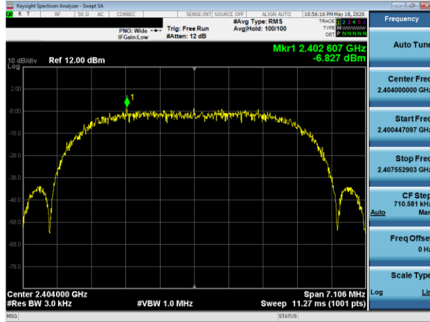
Plot 7-79. Power Spectral Density Plot Antenna WF8 (Bluetooth (XHDRPM6), 6 Mbps, ePA - Ch. 1)
