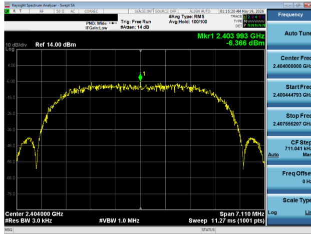
Plot 7-109. Power Spectral Density Plot Antenna WF7 (Bluetooth (XHDRPM6), 6 Mbps, ePA – Ch. 1)
