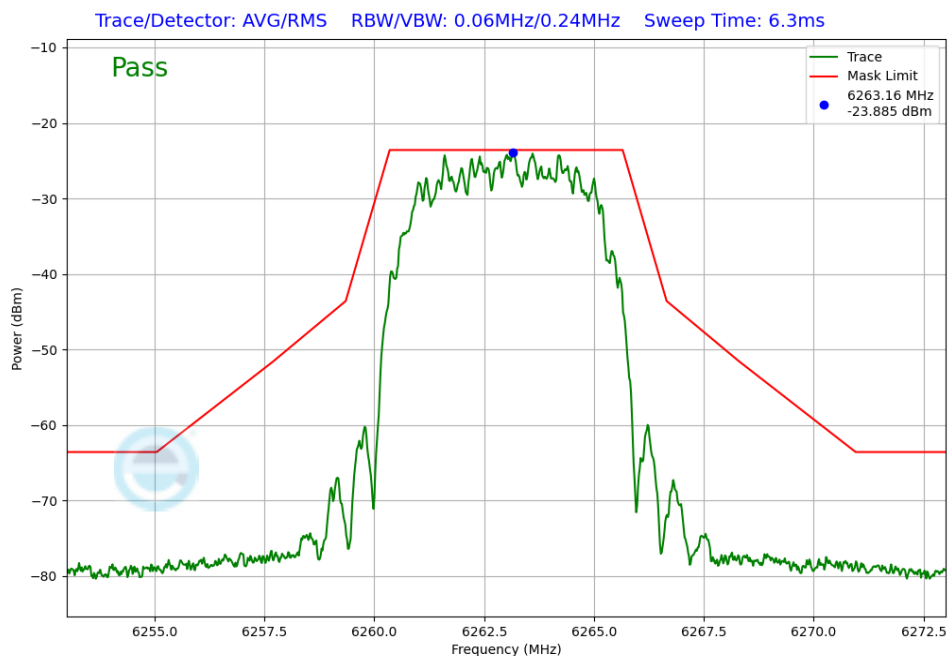
Plot 7-230. In-Band Emission Antenna WF5T (NB UNII HDR8, ePA – 6263 MHz)
