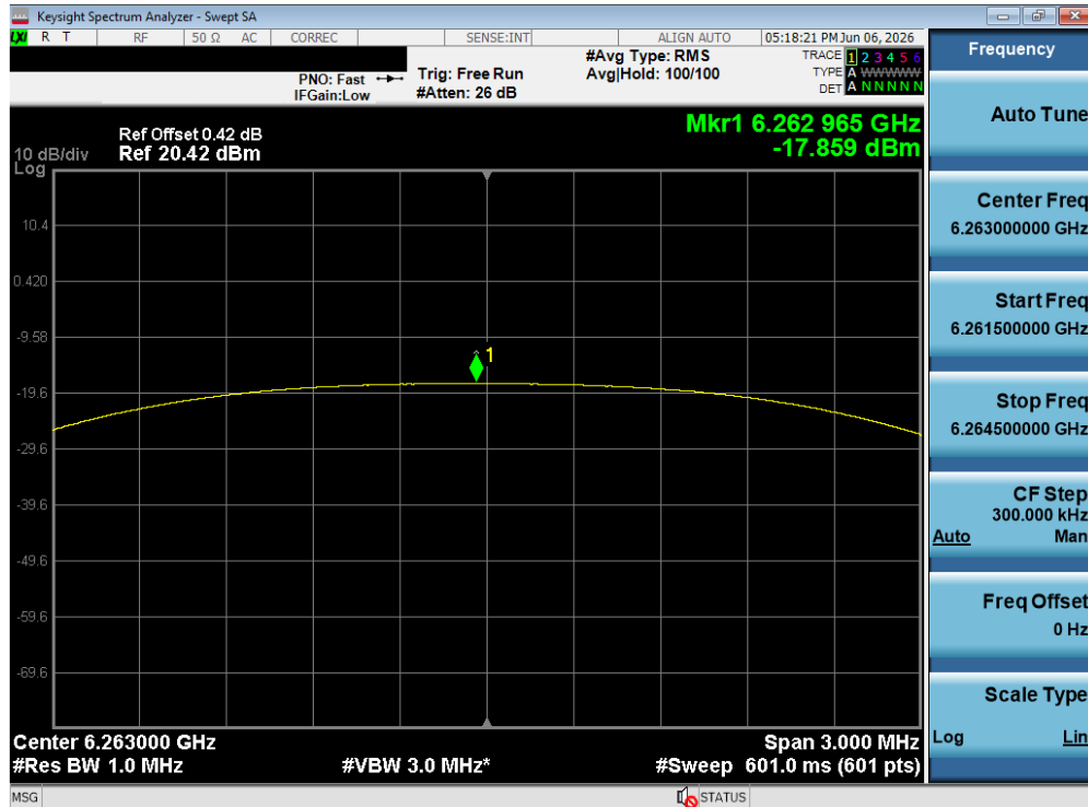
Plot 7-220. PSD Tx BF Diversity Antenna WF5T (NB UNII HDT6, iPA – 6263 MHz)
