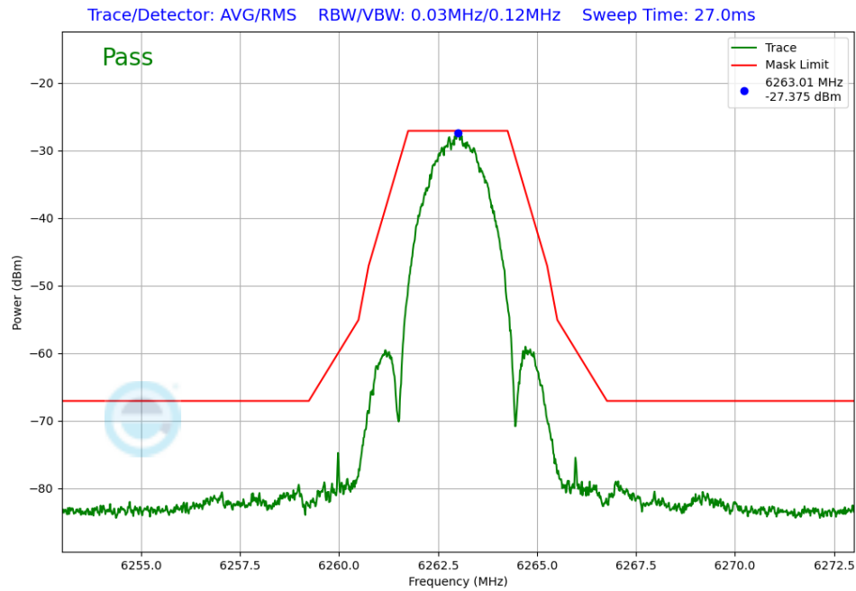
Plot 7-226. In-Band Emission Antenna WF5T (NB UNII LE2M, ePA – 6263 MHz)
