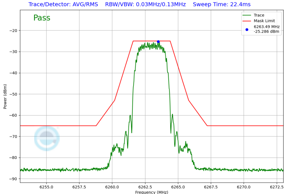
Plot 7-245. In-Band Emission Antenna WF5T (NB UNII HDT4, iPA – 6263 MHz)
