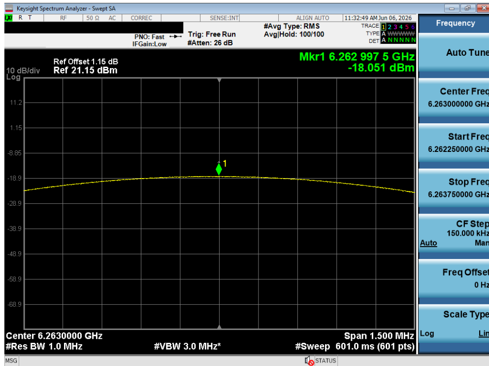
Plot 7-172. PSD Tx BF Diversity Antenna WF5T (NB UNII BDR, iPA – 6263 MHz)
