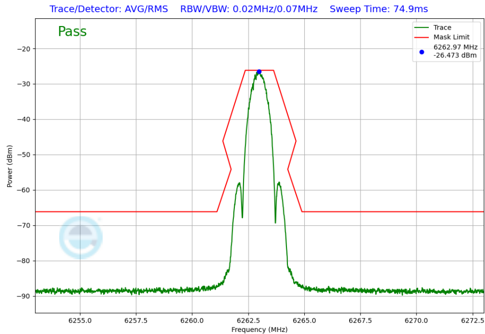
Plot 7-225. In-Band Emission Antenna WF5T (NB UNII LE1M, iPA – 6263 MHz)
