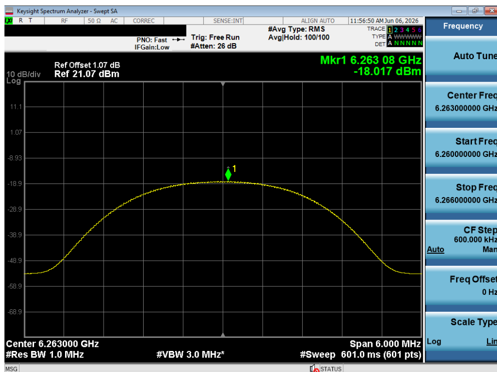
Plot 7-184. PSD TxBF Diversity Antenna WF5T (NB UNII HDR4, iPA – 6263 MHz)
