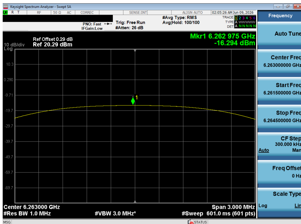
Plot 7-217. PSD TxBF Diversity Antenna WF8 (NB UNII HDT4, iPA – 6263 MHz)
