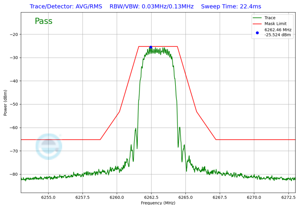
Plot 7-244. In-Band Emission Antenna WF5T (NB UNII HDT4, ePA – 6263 MHz)
