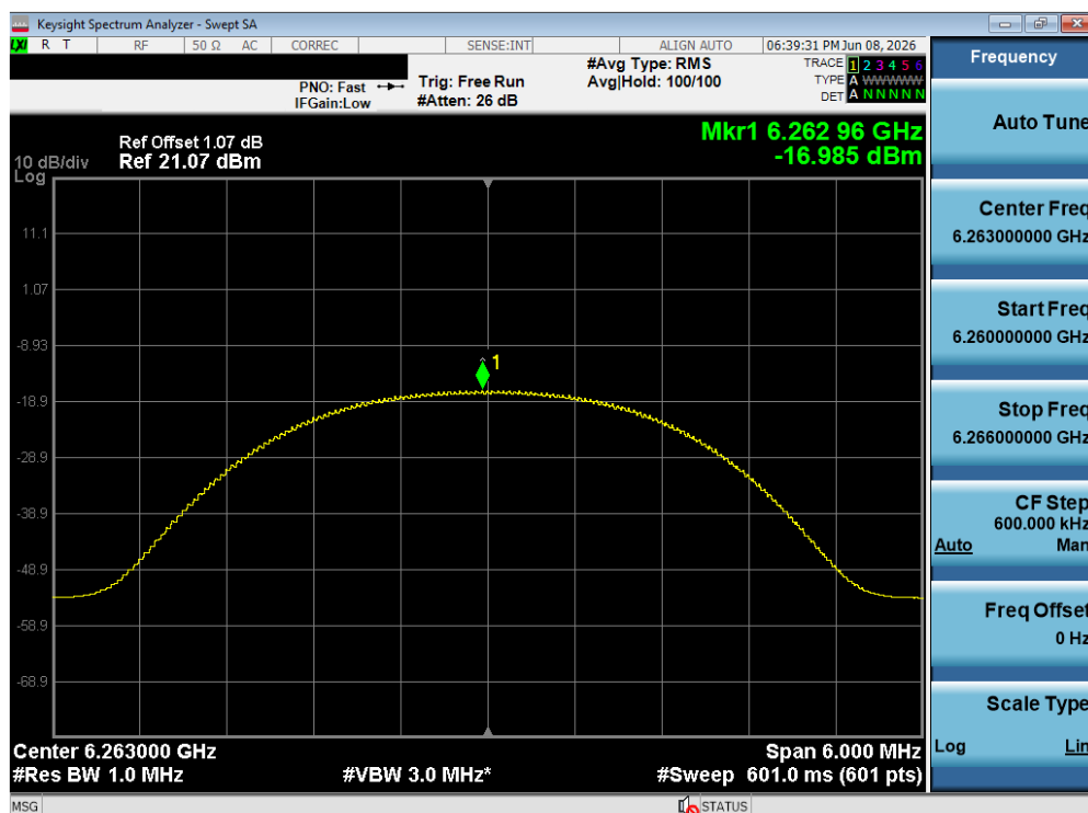
Plot 7-185. PSD TxBF Diversity Antenna WF8 (NB UNII HDR4, iPA – 6263 MHz)
