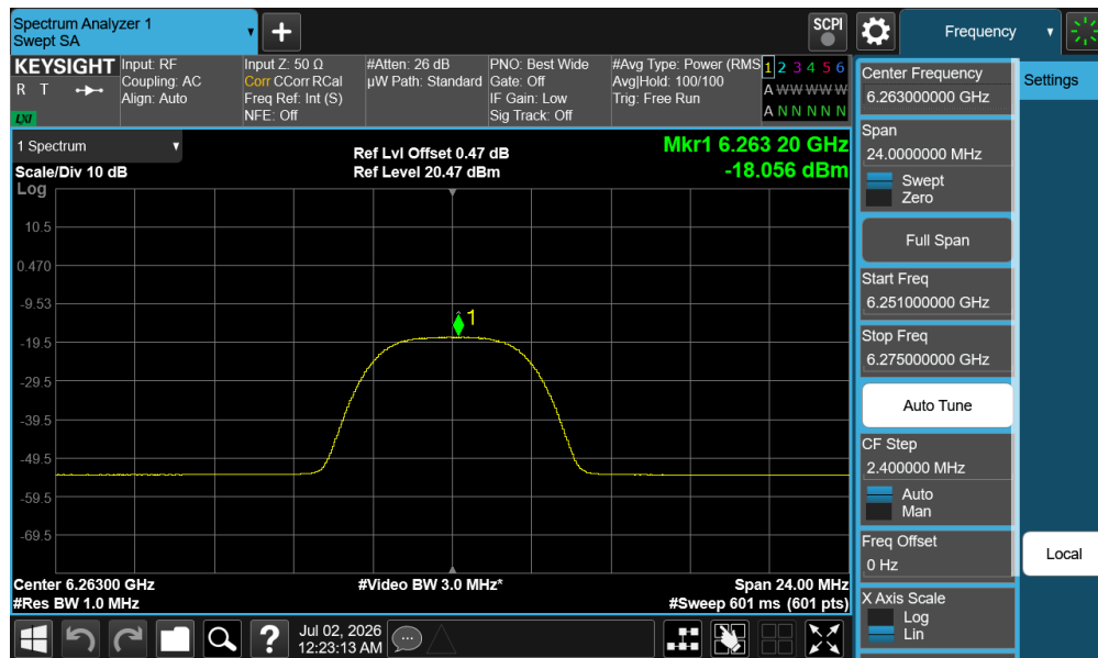
Plot 7-198. PSD Tx BF Diversity Antenna WF5T (NB UNII HDRPM16, ePA – 6263 MHz)
