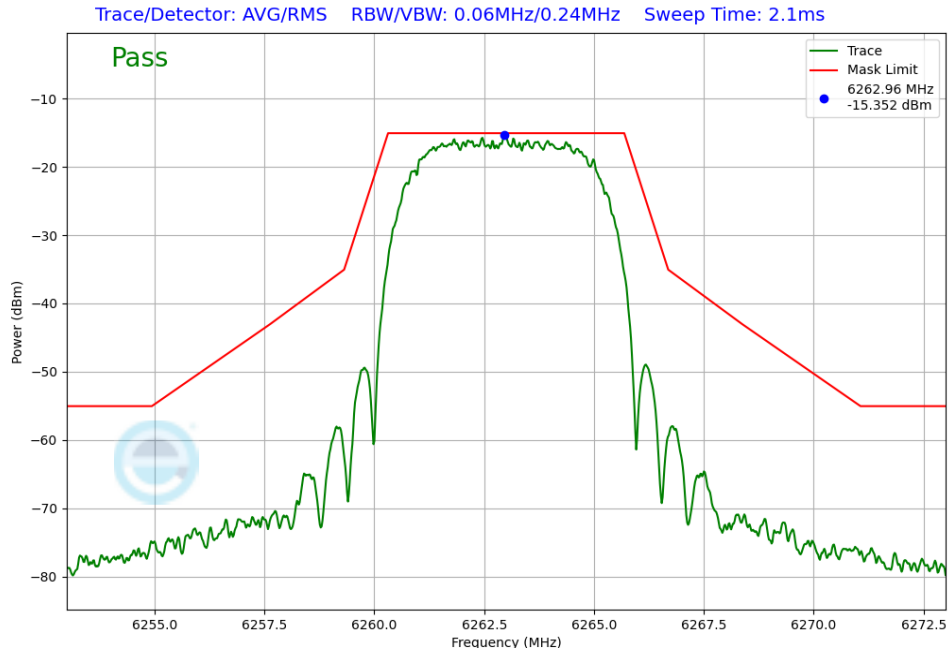
Plot 7-235. In-Band Emission Antenna WF5T (NB UNII XHDRPM6, iPA – 6263 MHz)
