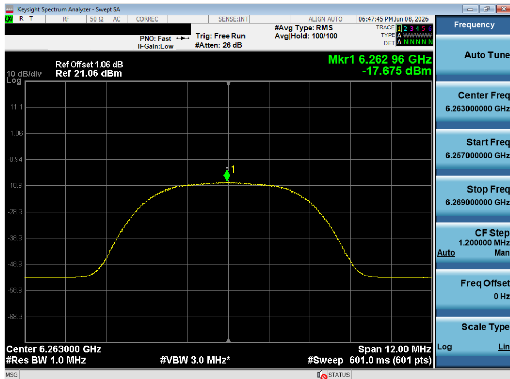
Plot 7-189. PSD TxBF Diversity Antenna WF8 (NB UNII HDR8, iPA – 6263 MHz)
