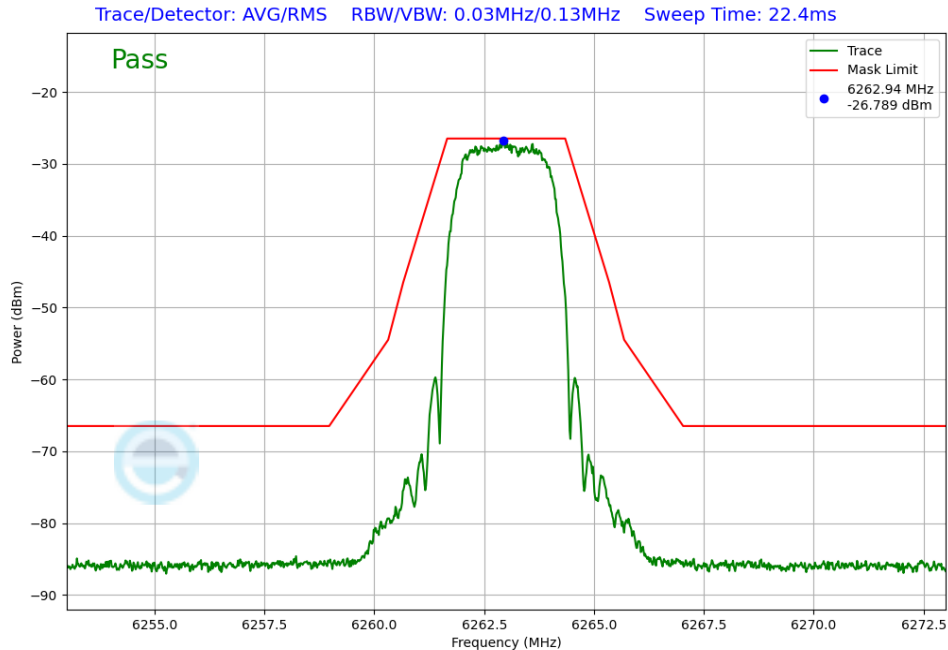
Plot 7-233. In-Band Emission Antenna WF5T (NB UNII HDRPS2, iPA – 6263 MHz)
