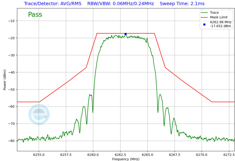
Plot 7-237. In-Band Emission Antenna WF5T (NB UNII HDRPM16, iPA – 6263 MHz)
