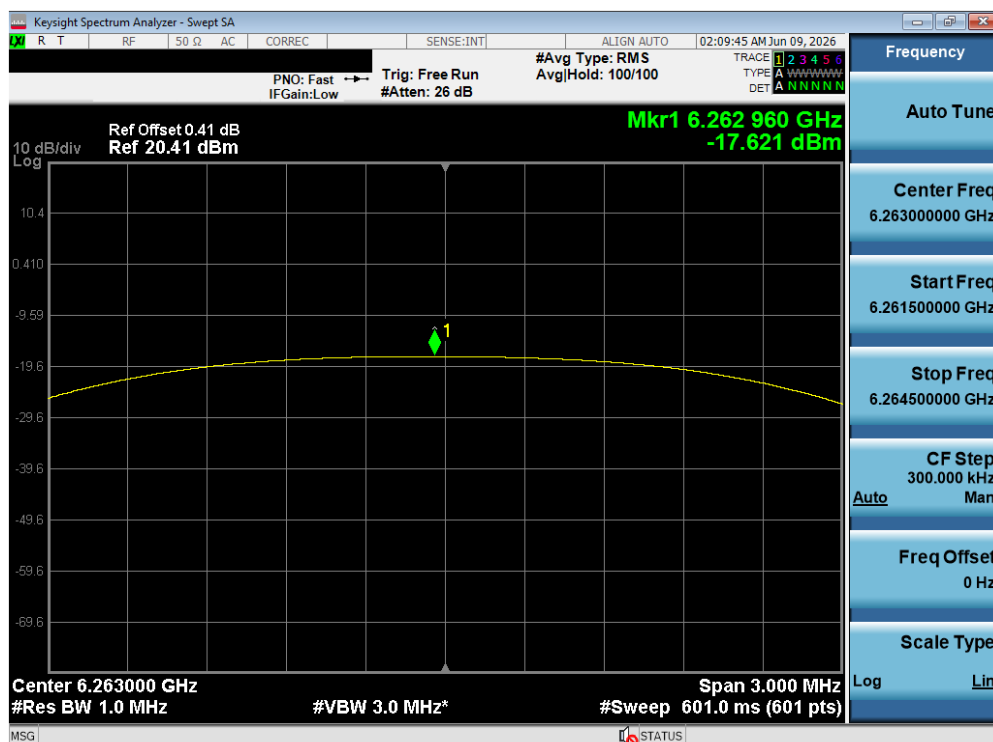
Plot 7-219. PSD TxBF Diversity Antenna WF8 (NB UNII HDT6, ePA – 6263 MHz)
