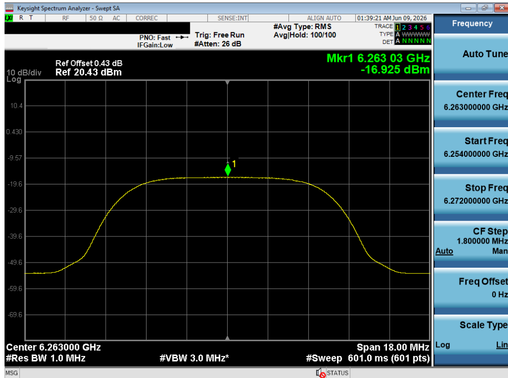
Plot 7-205. PSD Tx BF Diversity Antenna WF8 (NB UNII HDRPL12, iPA – 6263 MHz)
