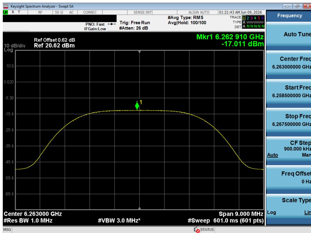
Plot 7-197. PSD TxBF Diversity Antenna WF8 (NB UNII XHDRPM6, iPA – 6263 MHz)
