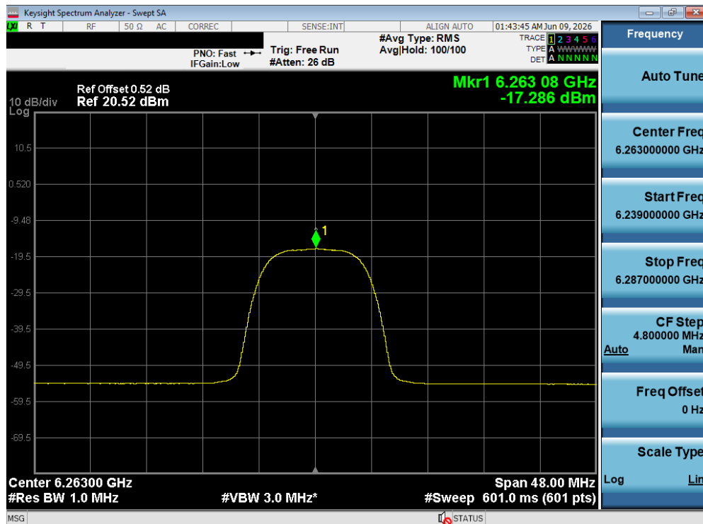
Plot 7-207. PSD TxBF Diversity Antenna WF8 (NB UNII HDRPL32, ePA – 6263 MHz)
