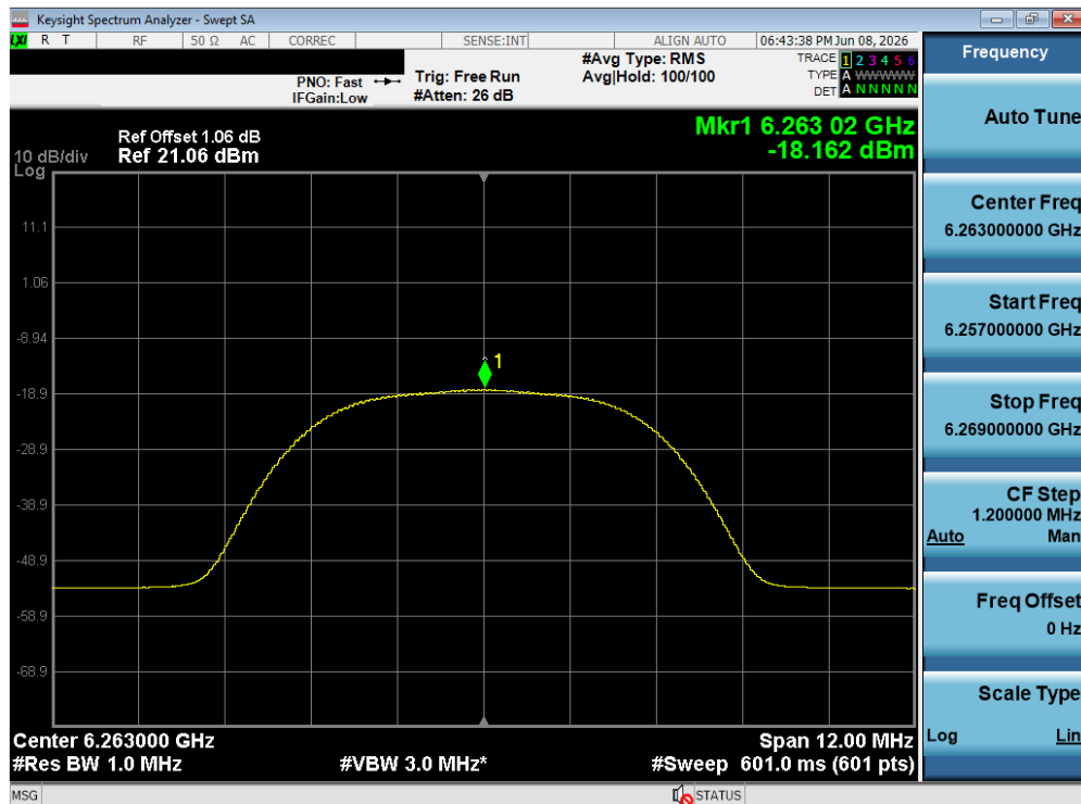
Plot 7-187. PSD TxBF Diversity Antenna WF8 (NB UNII HDR8, ePA – 6263 MHz)
