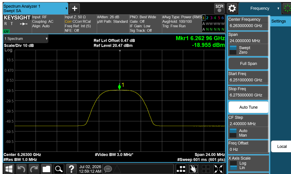
Plot 7-200. PSD Tx BF Diversity Antenna WF5T (NB UNII HDRPM16, iPA – 6263 MHz)
