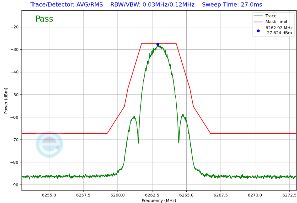
Plot 7-227. In-Band Emission Antenna WF5T (NB UNII LE2M, iPA – 6263 MHz)
