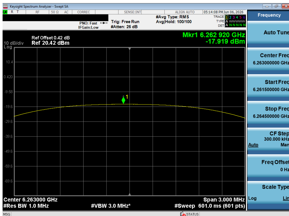
Plot 7-166. PSD TxBF Primary Antenna WF5T (NB UNII HDT6, ePA – 6263 MHz)
