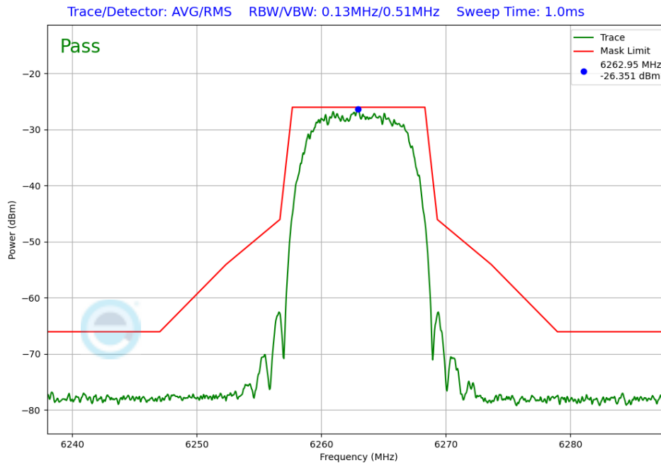
Plot 7-238. In-Band Emission Antenna WF5T (NB UNII HDRPL12, ePA – 6263 MHz)
