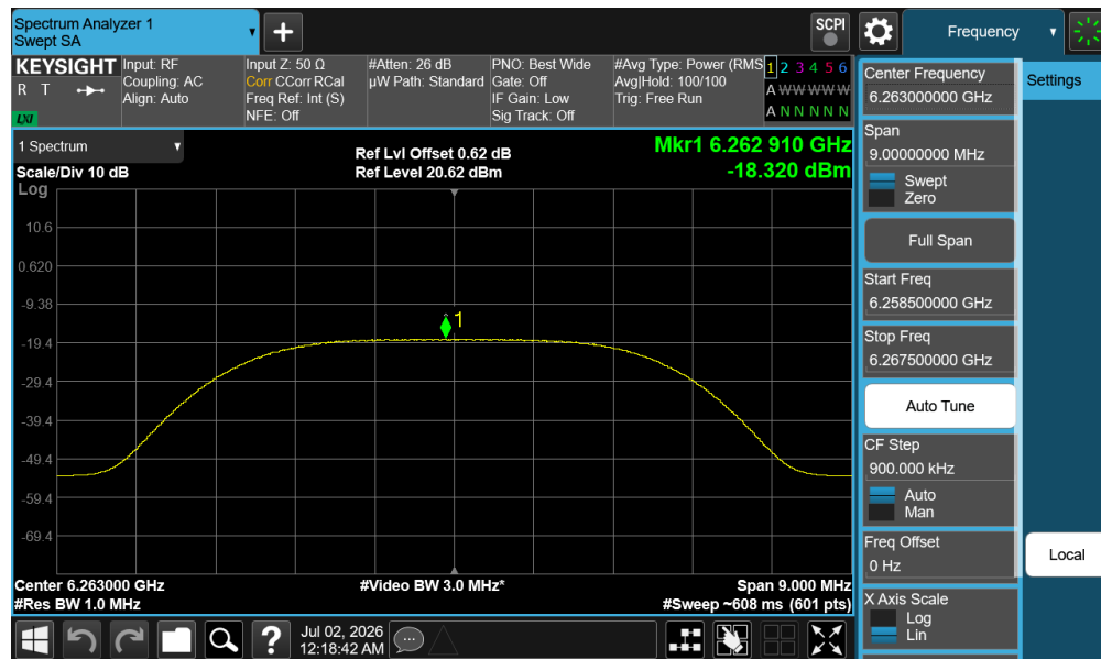
Plot 7-196. PSD TxBF Diversity Antenna WF5T (NB UNII XHDRPM6, iPA – 6263 MHz)
