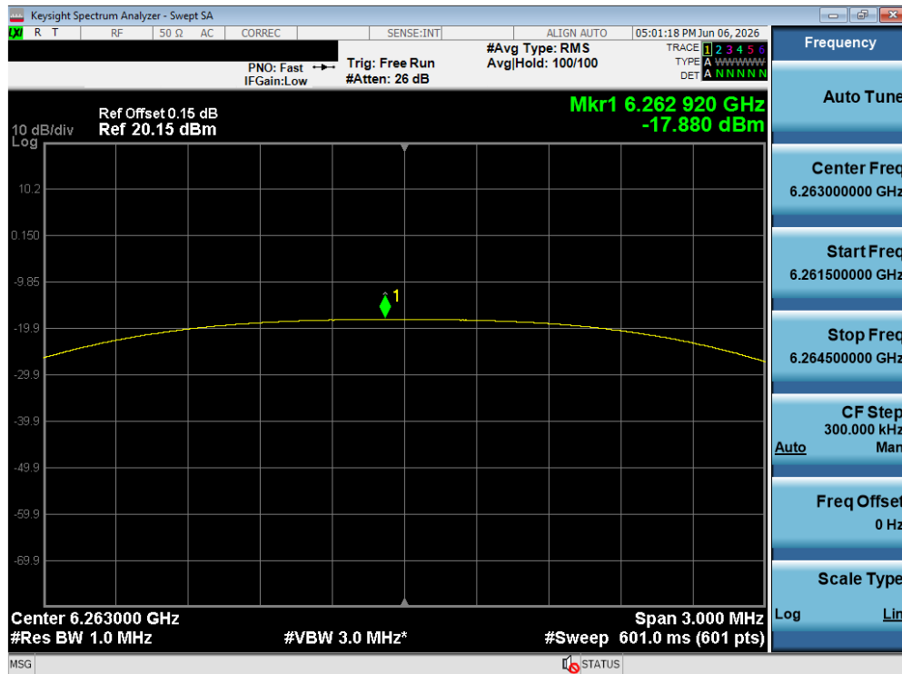
Plot 7-160. PSD TxBF Primary Antenna WF5T (NB UNII HDT2, iPA – 6263 MHz)
