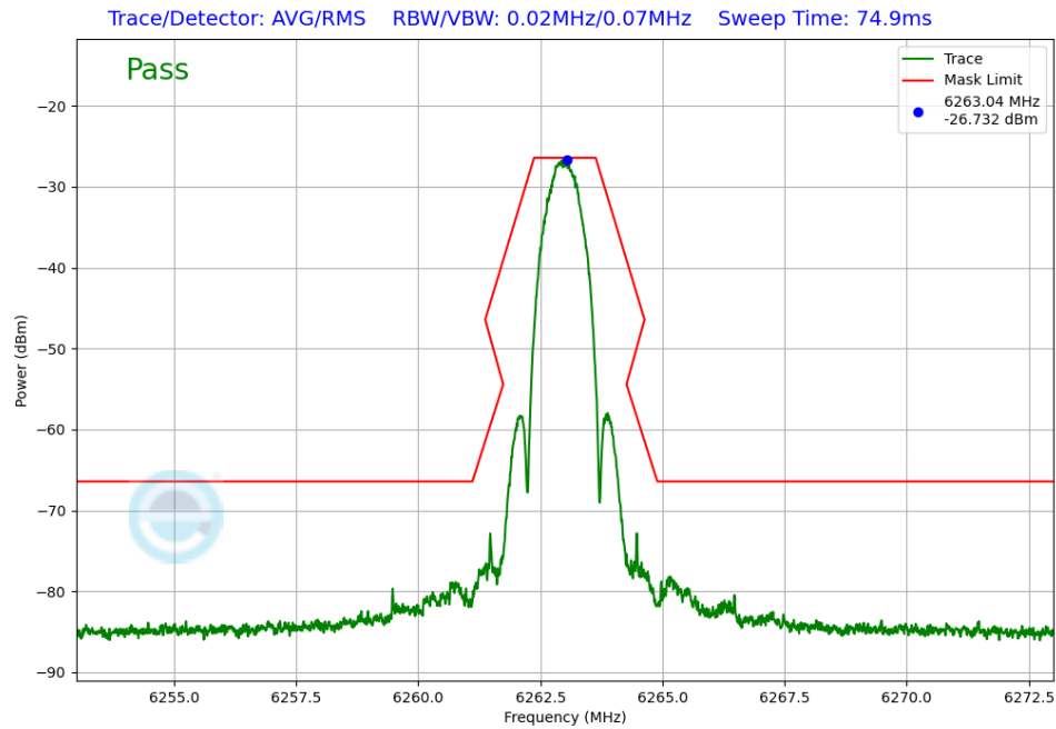
Plot 7-224. In-Band Emission Antenna WF5T (NB UNII LE1M, ePA – 6263 MHz)
