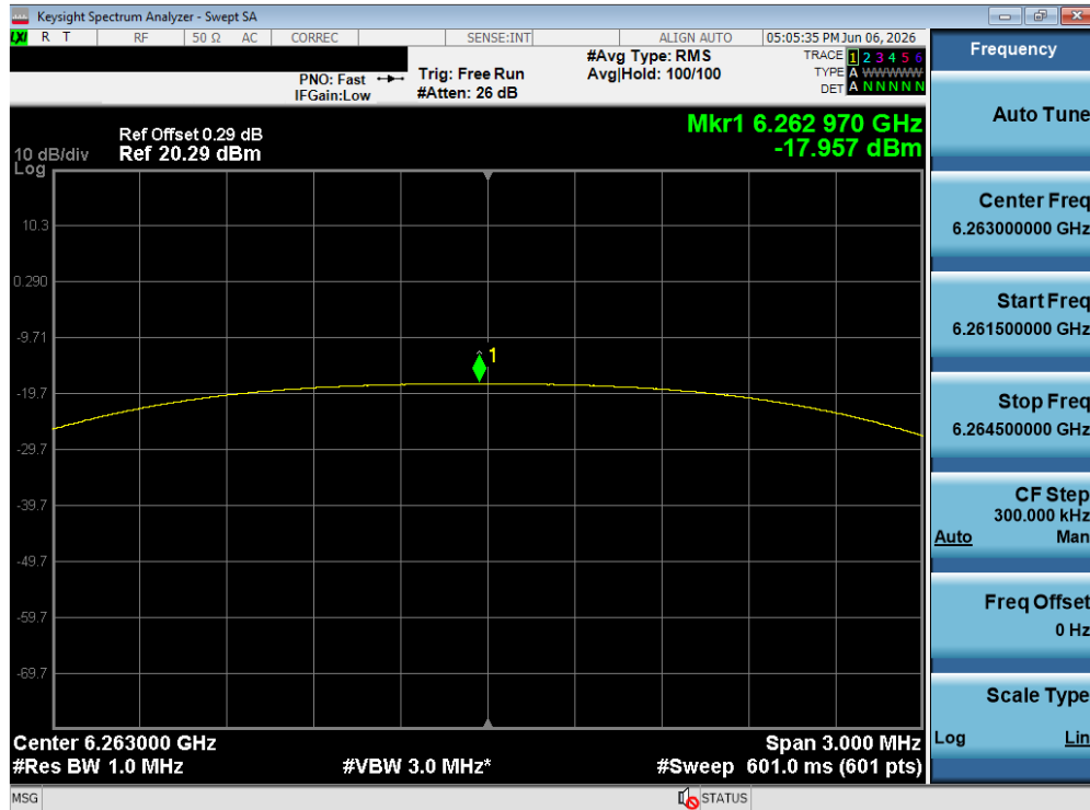
Plot 7-214. PSD TxBF Diversity Antenna WF5T (NB UNII HDT4, ePA – 6263 MHz)
