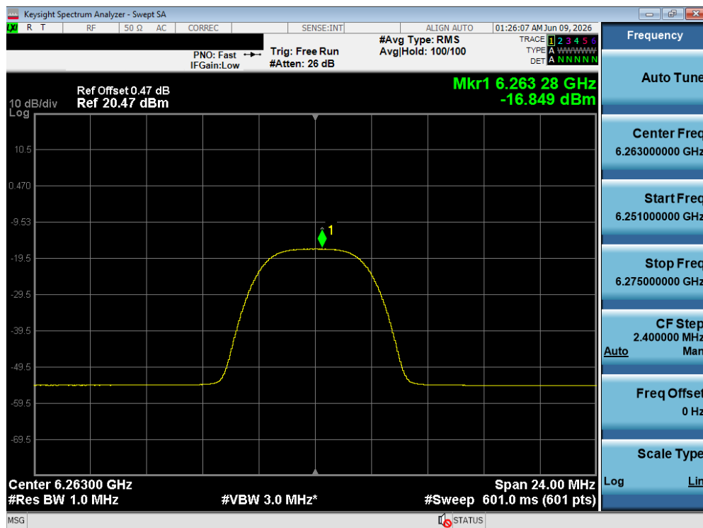
Plot 7-199. PSD Tx BF Diversity Antenna WF8 (NB UNII HDRPM16, ePA – 6263 MHz)
