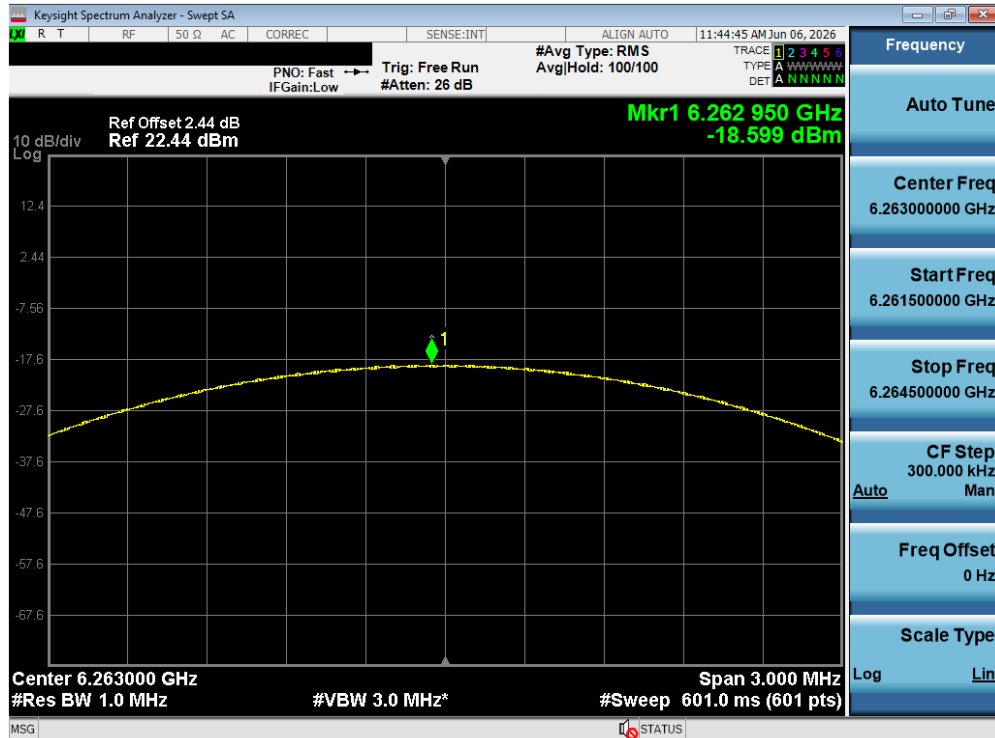
Plot 7-178. PSD TxBF Diversity Antenna WF5T (NB UNII LE2M, ePA – 6263 MHz)
