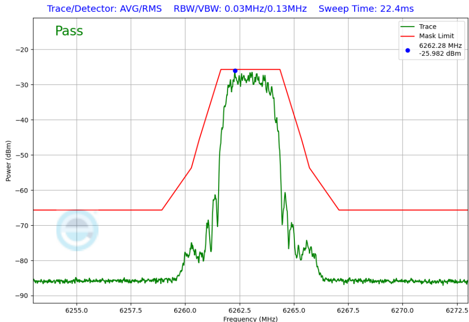
Plot 7-229. In-Band Emission Antenna WF5T (NB UNII HDR4, iPA – 6263 MHz)
