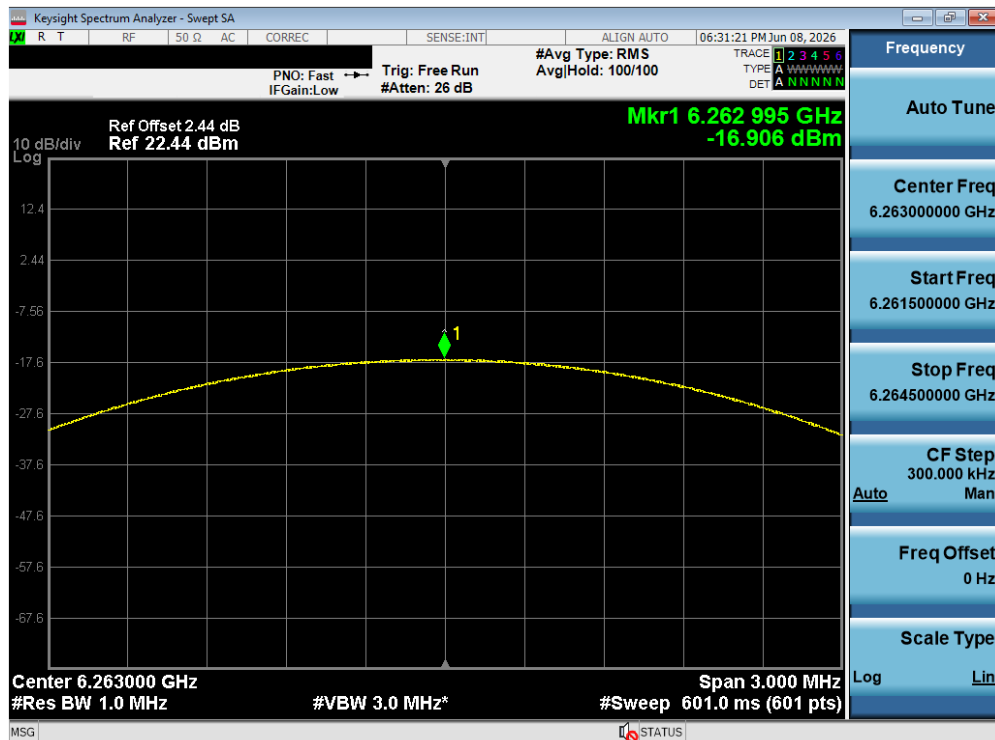
Plot 7-181. PSD TxBF Diversity Antenna WF8 (NB UNII LE2M, iPA – 6263 MHz)
