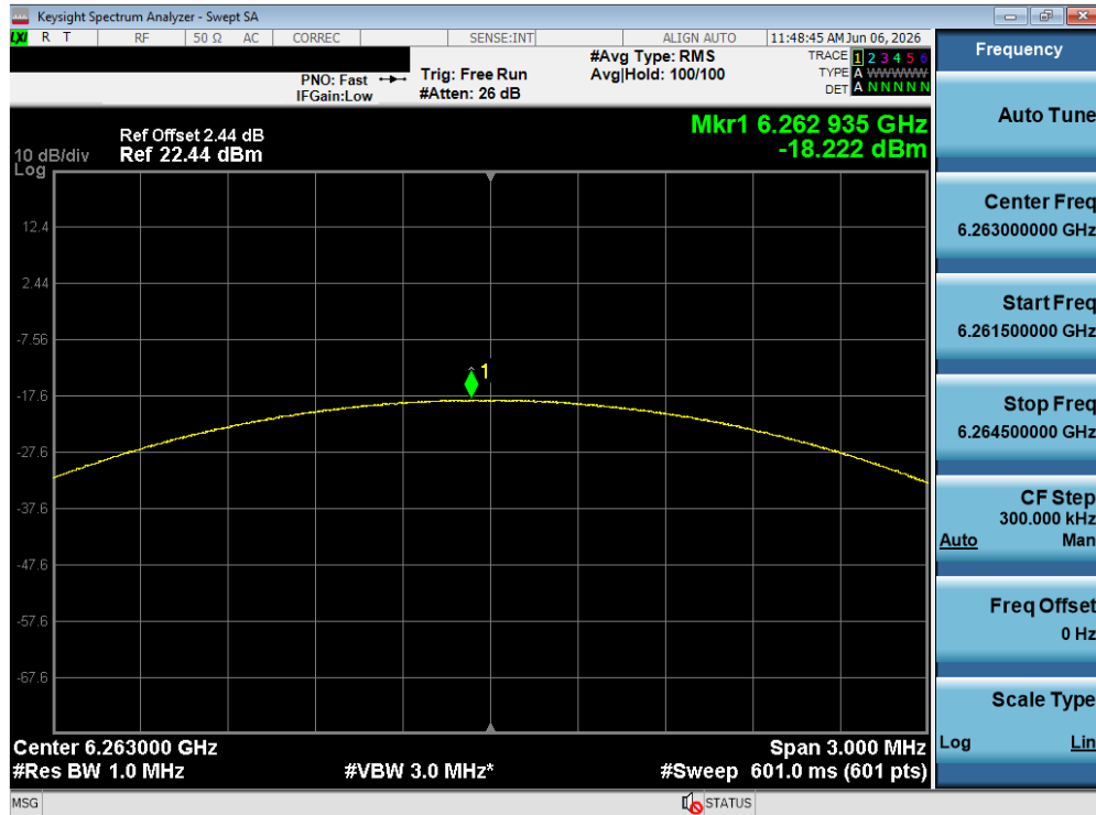
Plot 7-180. PSD TxBF Diversity Antenna WF5T (NB UNII LE2M, iPA – 6263 MHz)
