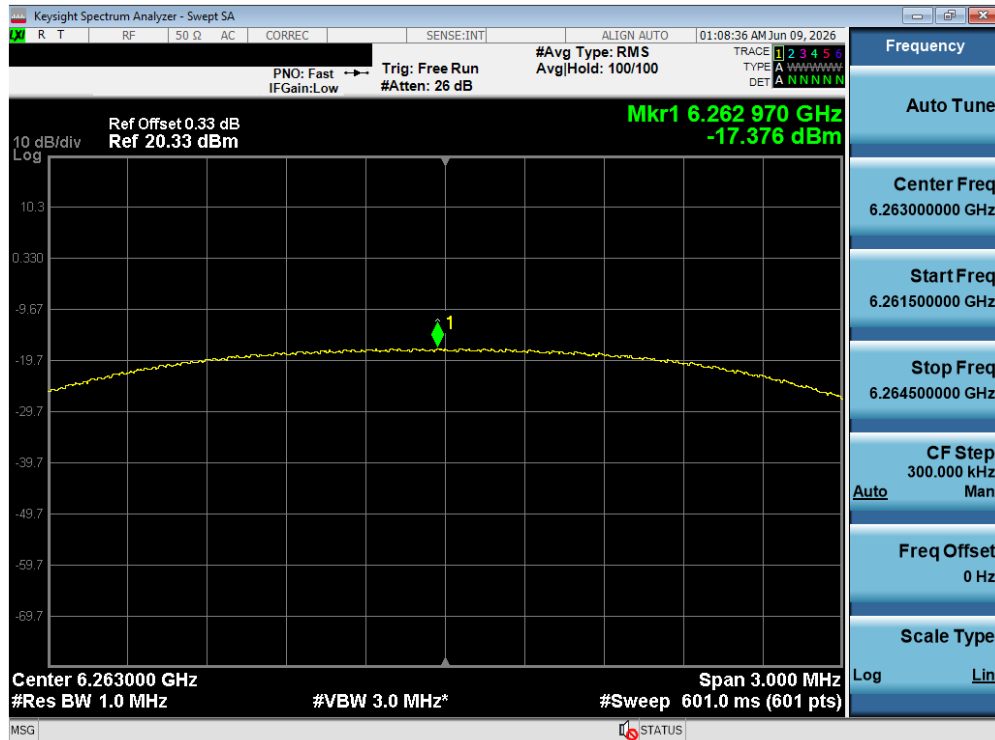
Plot 7-191. PSD TxBF Diversity Antenna WF8 (NB UNII HDRPS2, ePA – 6263 MHz)
