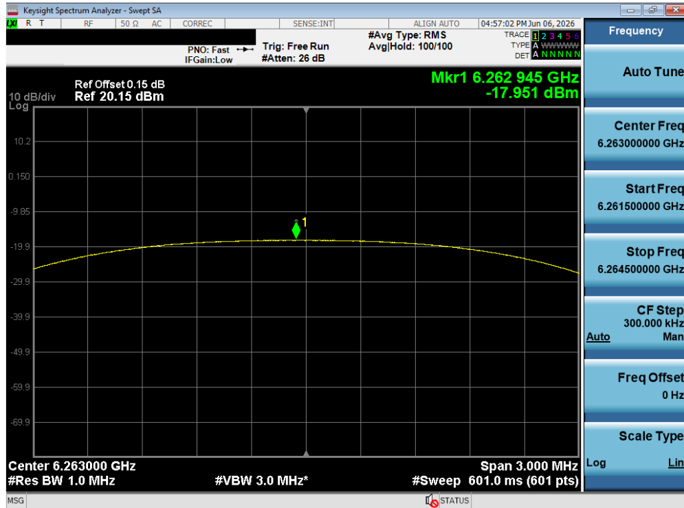
Plot 7-210. PSD TxBF Diversity Antenna WF5T (NB UNII HDT2, ePA – 6263 MHz)
