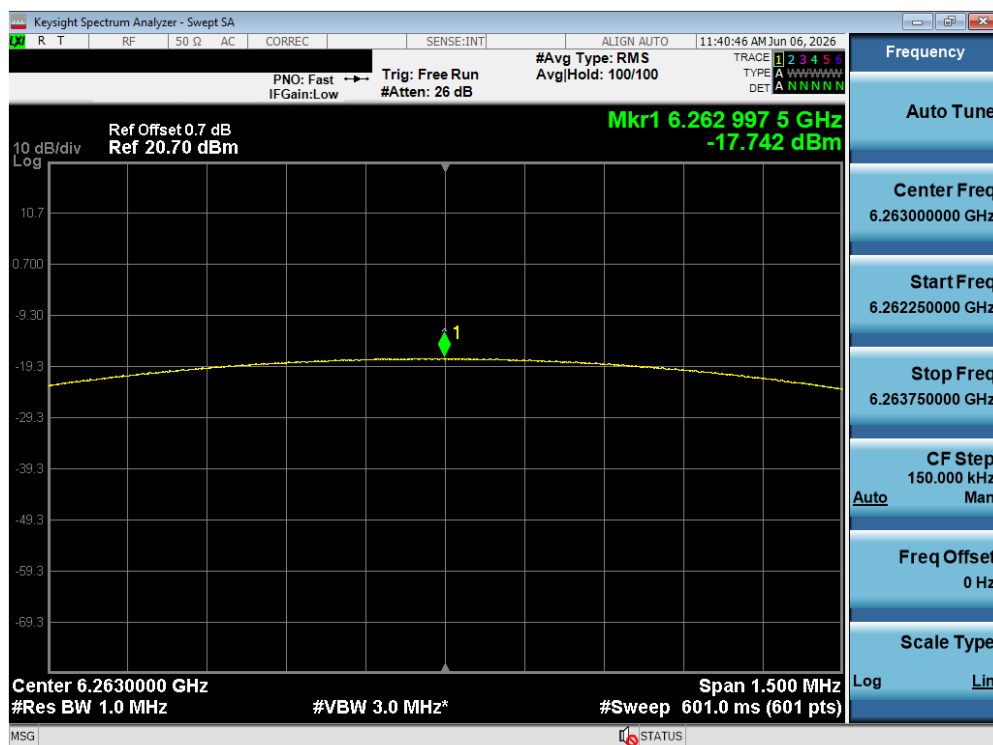
Plot 7-176. PSD TxBF Diversity Antenna WF5T (NB UNII LE1M, iPA – 6263 MHz)
