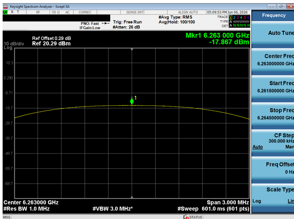
Plot 7-216. PSD TxBF Diversity Antenna WF5T (NB UNII HDT4, iPA – 6263 MHz)
