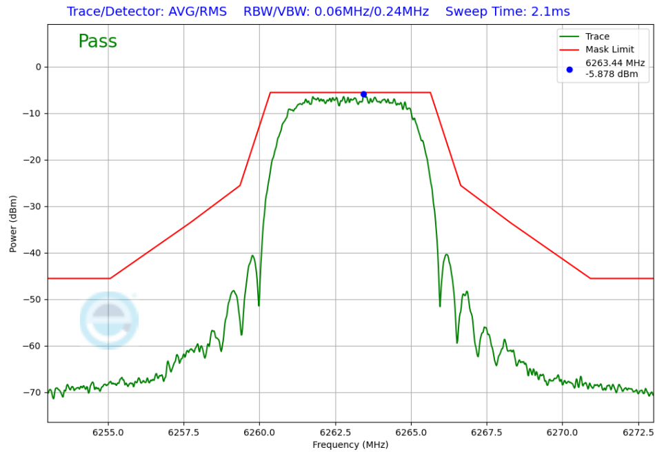
Plot 7-236. In-Band Emission Antenna WF5T (NB UNII HDRPM16, ePA – 6263 MHz)
