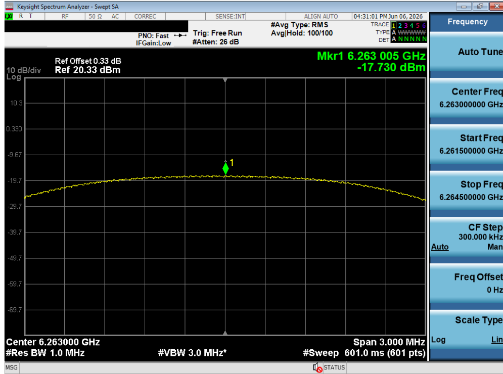
Plot 7-190. PSD TxBF Diversity Antenna WF5T (NB UNII HDRPS2, ePA – 6263 MHz)
