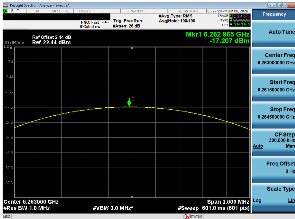
Plot 7-179. PSD TxBF Diversity Antenna WF8 (NB UNII LE2M, ePA – 6263 MHz)
