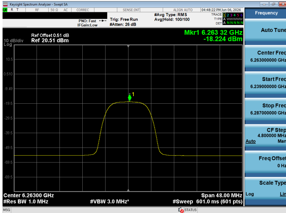
Plot 7-206. PSD TxBF Diversity Antenna WF5T (NB UNII HDRPL32, ePA – 6263 MHz)
