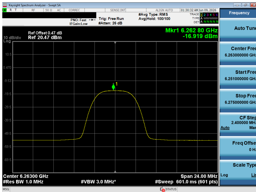
Plot 7-201. PSD Tx BF Diversity Antenna WF8 (NB UNII HDRPM16, iPA – 6263 MHz)
