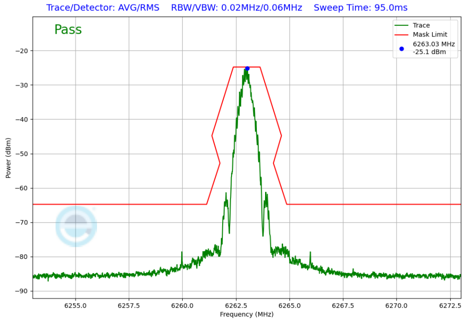
Plot 7-222. In-Band Emission Antenna WF5T (NB UNII BDR, ePA – 6263 MHz)
