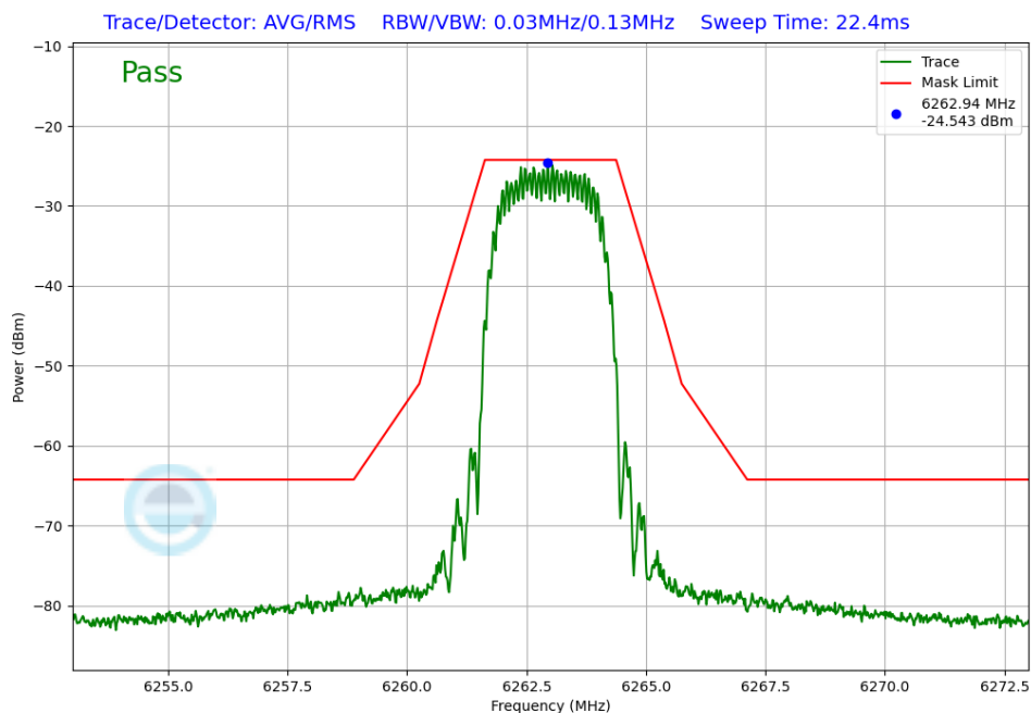
Plot 7-242. In-Band Emission Antenna WF5T (NB UNII HDT2, ePA – 6263 MHz)
