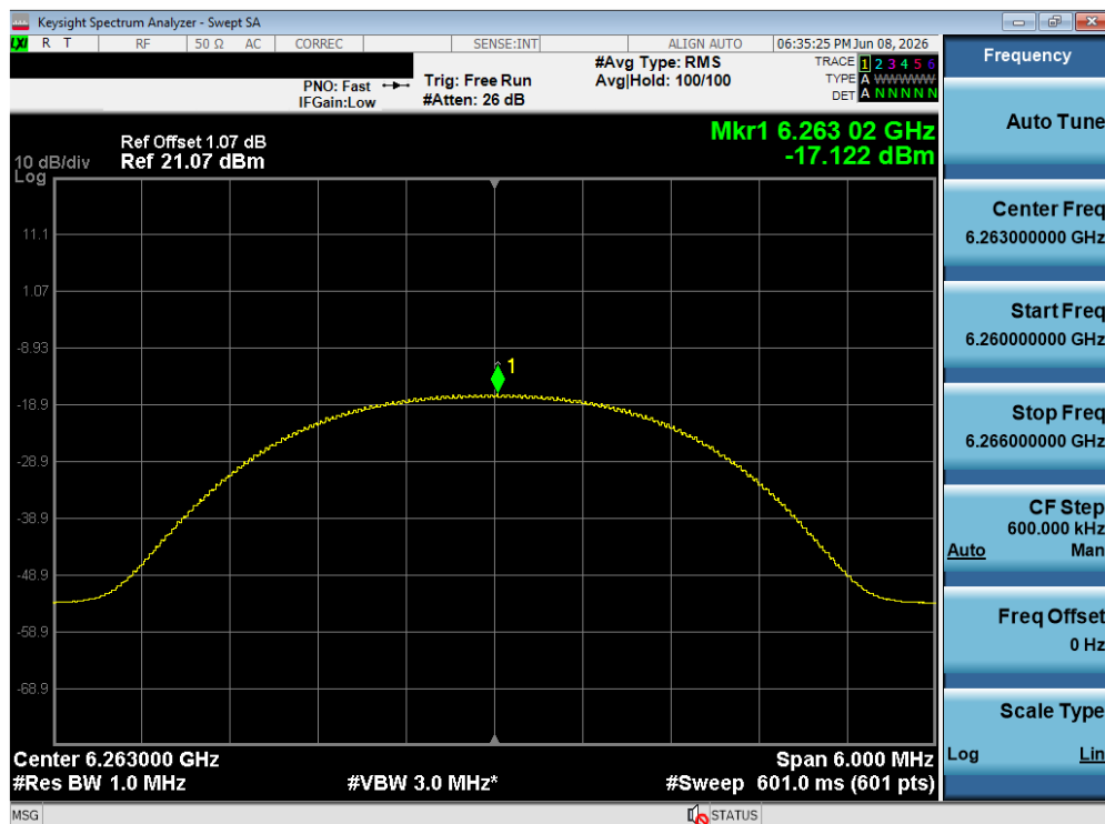
Plot 7-183. PSD TxBF Diversity Antenna WF8 (NB UNII HDR4, ePA – 6263 MHz)
