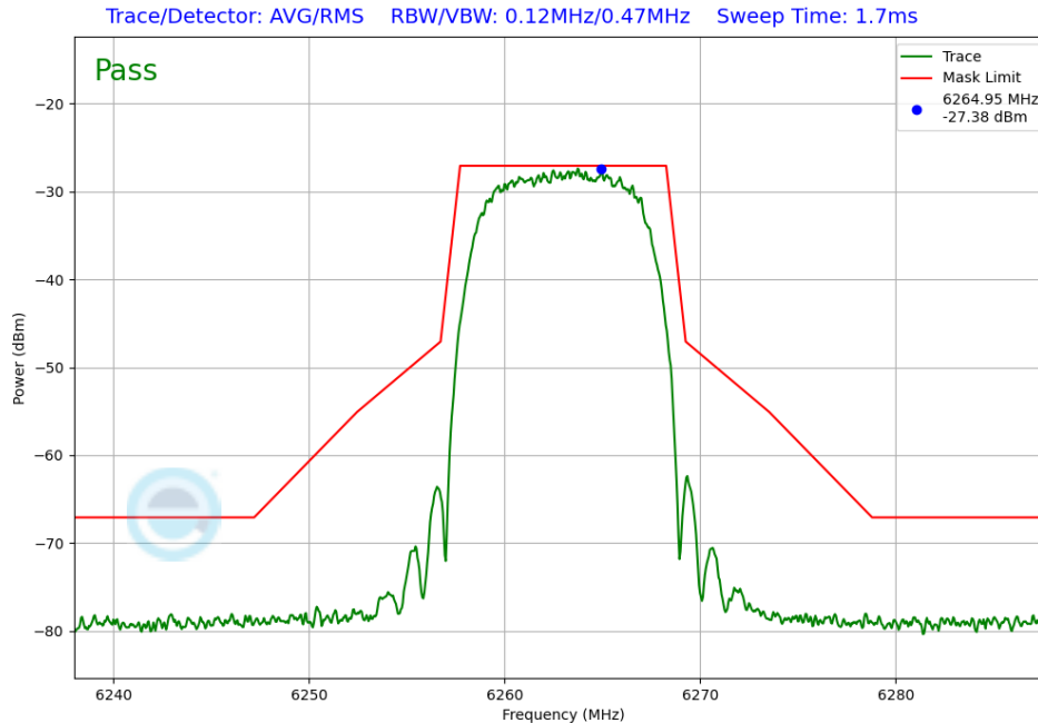
Plot 7-241. In-Band Emission Antenna WF5T (NB UNII HDRPL32, iPA – 6263 MHz)
