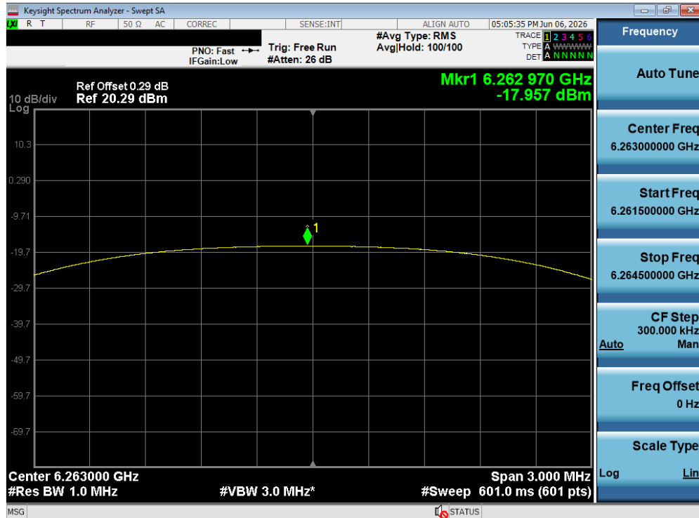
Plot 7-162. PSD TxBF Primary Antenna WF5T (NB UNII HDT4, ePA – 6263 MHz)
