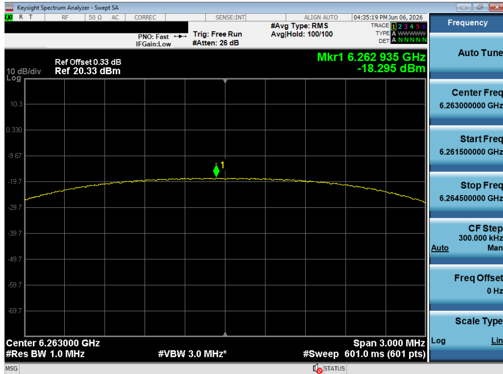
Plot 7-192. PSD TxBF Diversity Antenna WF5T (NB UNII HDRPS2, iPA – 6263 MHz)
