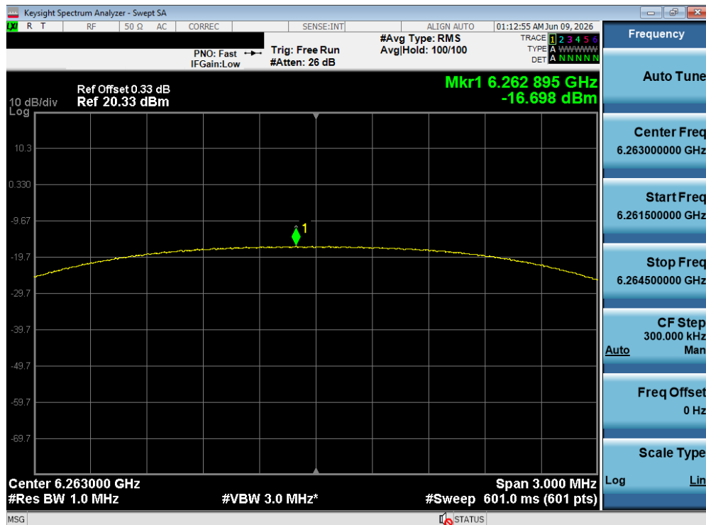
Plot 7-193. PSD TxBF Diversity Antenna WF8 (NB UNII HDRPS2, iPA – 6263 MHz)
