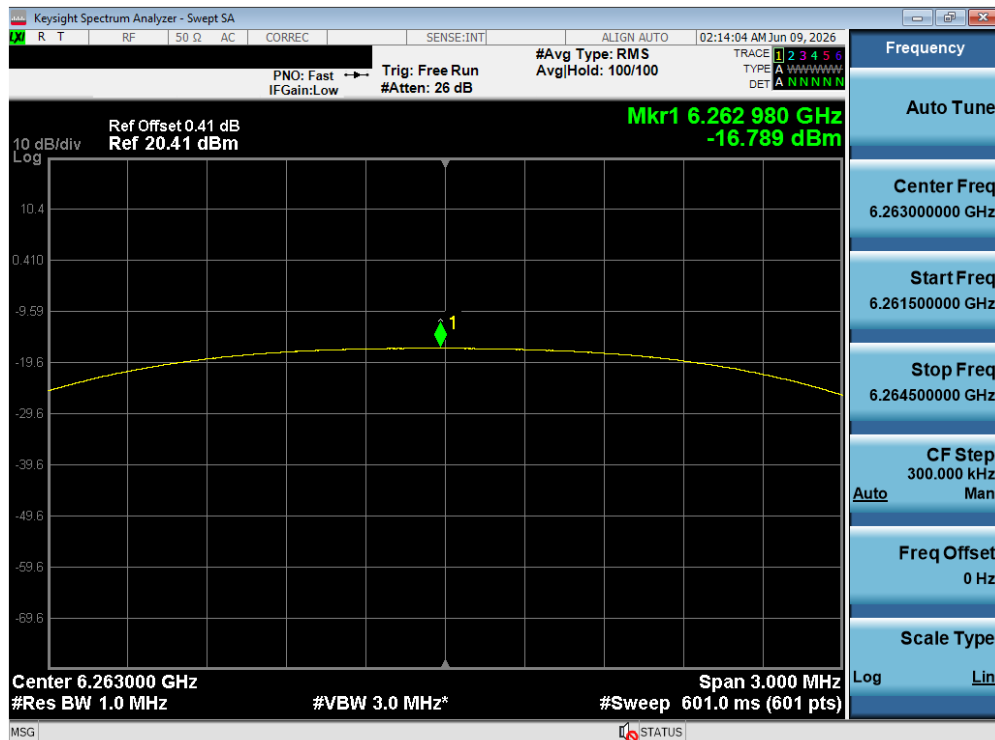
Plot 7-221. PSD Tx BF Diversity Antenna WF8 (NB UNII HDT6, iPA – 6263 MHz)
