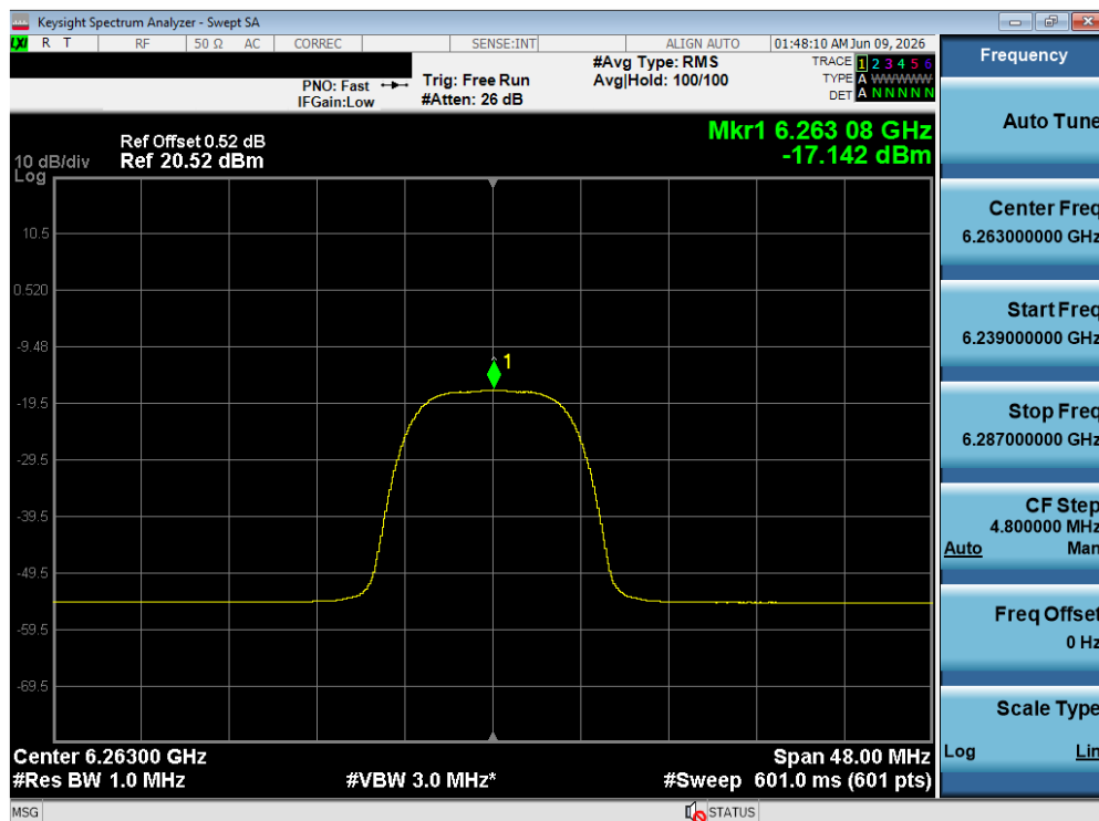
Plot 7-209. PSD TxBF Diversity Antenna WF8 (NB UNII HDRPL32, iPA – 6263 MHz)
