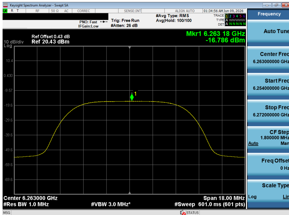
Plot 7-203. PSD TxBF Diversity Antenna WF8 (NB UNII HDRPL12, ePA – 6263 MHz)
