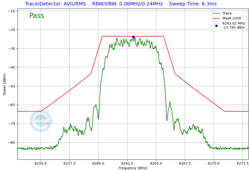
Plot 7-231. In-Band Emission Antenna WF5T (NB UNII HDR8, iPA – 6263 MHz)
