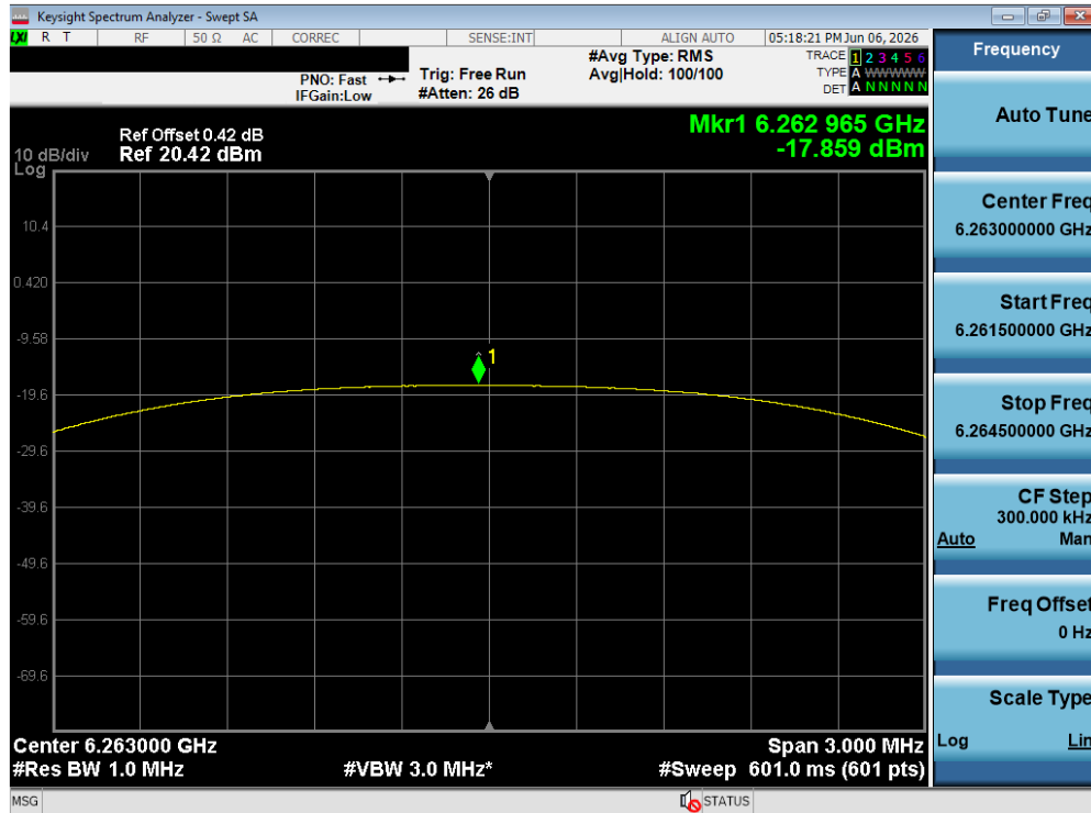
Plot 7-168. PSD TxBF Primary Antenna WF5T (NB UNII HDT6, iPA – 6263 MHz)
