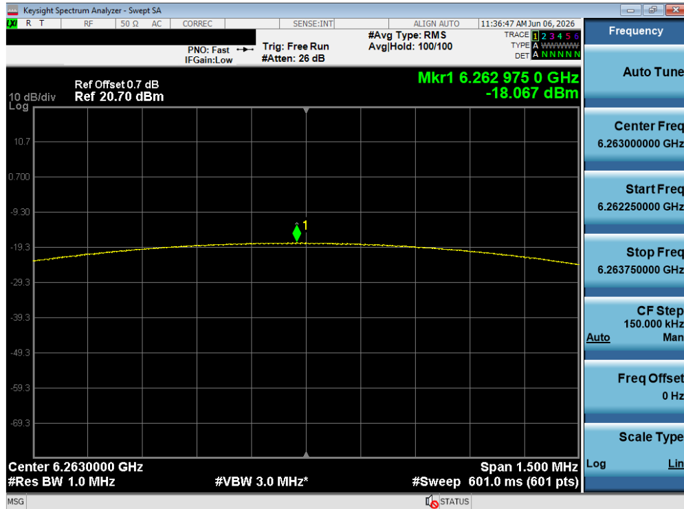
Plot 7-174. PSD TxBF Diversity Antenna WF5T (NB UNII LE1M, ePA – 6263 MHz)
