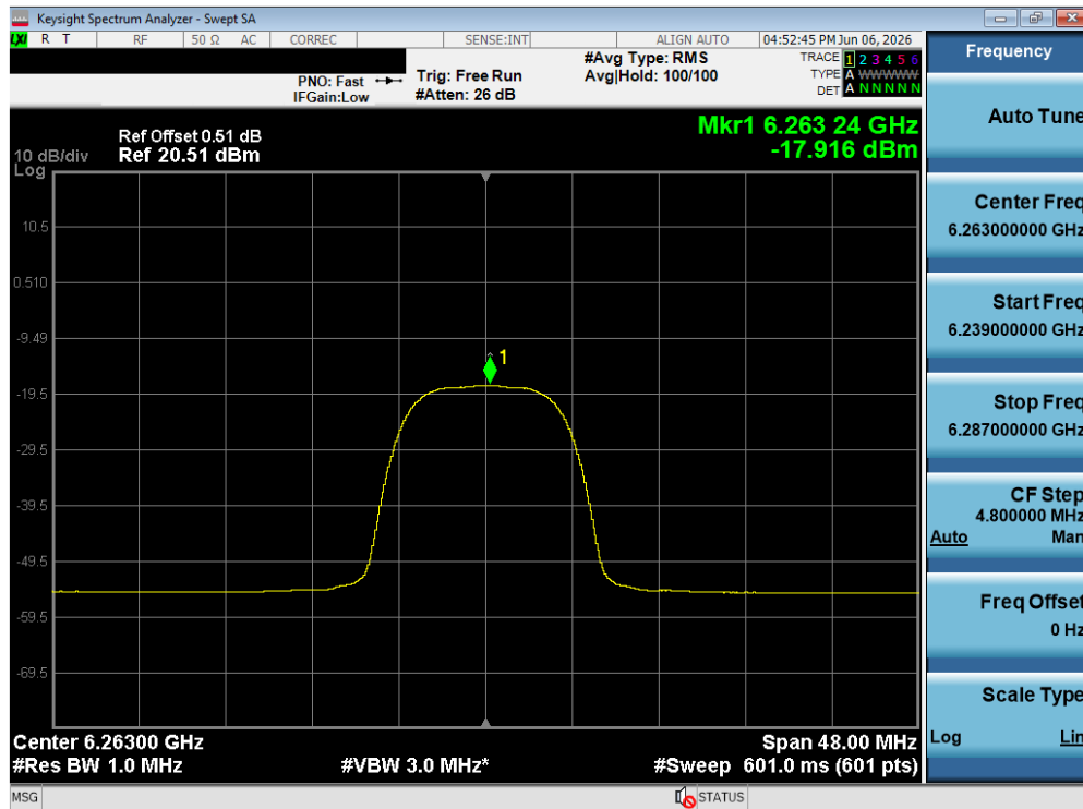
Plot 7-208. PSD TxBF Diversity Antenna WF5T (NB UNII HDRPL32, iPA – 6263 MHz)
