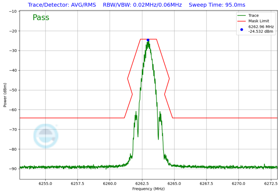
Plot 7-223. In-Band Emission Antenna WF5T (NB UNII BDR, iPA – 6263 MHz)
