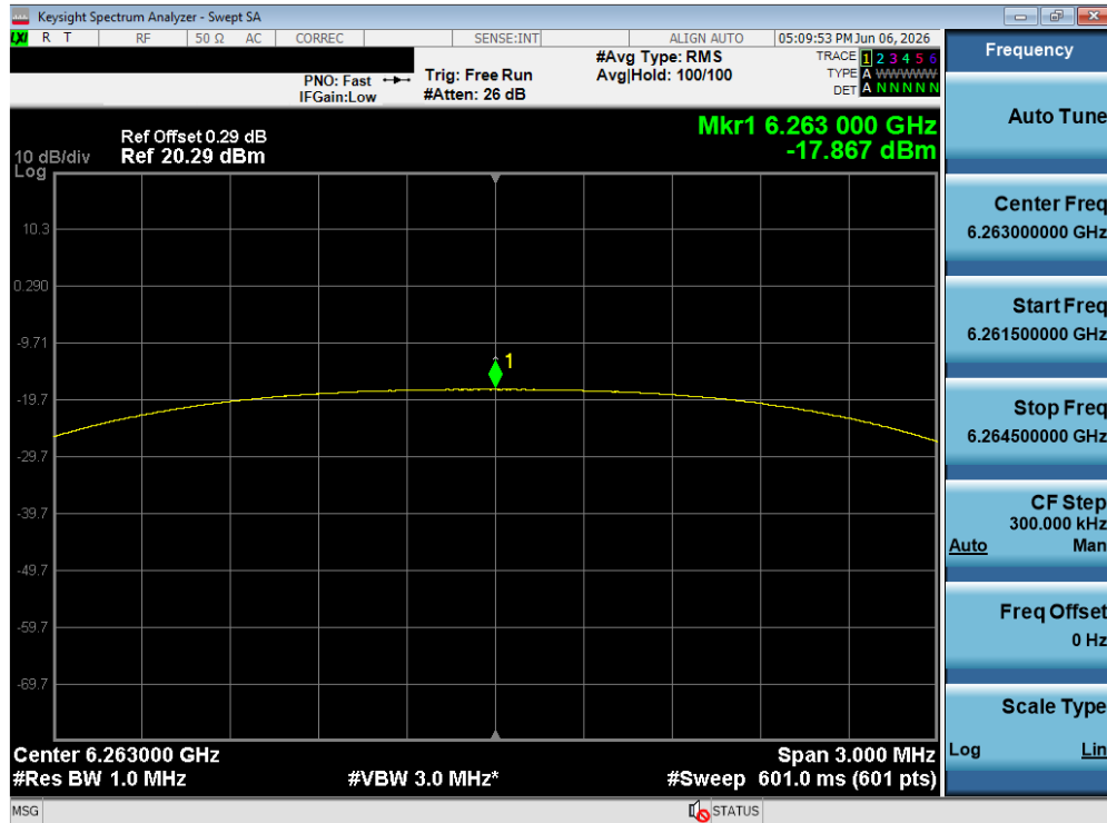
Plot 7-164. PSD TxBF Primary Antenna WF5T (NB UNII HDT4, iPA – 6263 MHz)
