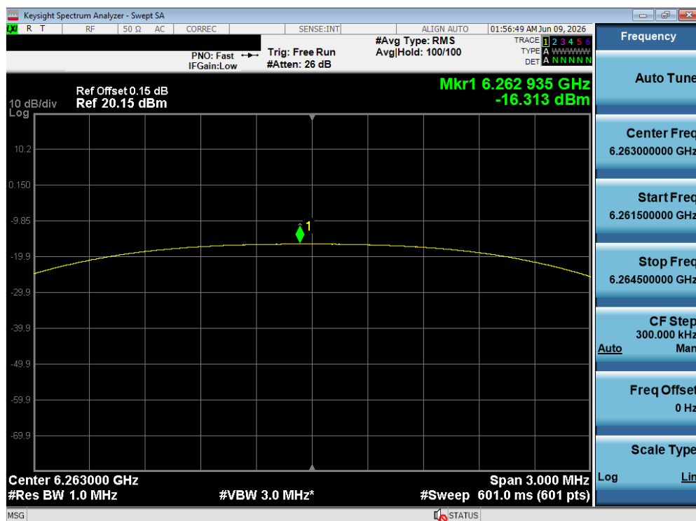
Plot 7-213. PSD Tx BF Diversity Antenna WF8 (NB UNII HDT2, iPA – 6263 MHz)
