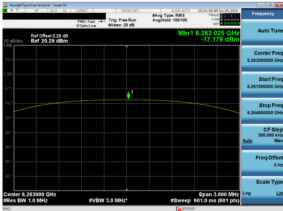
Plot 7-215. PSD TxBF Diversity Antenna WF8 (NB UNII HDT4, ePA – 6263 MHz)
