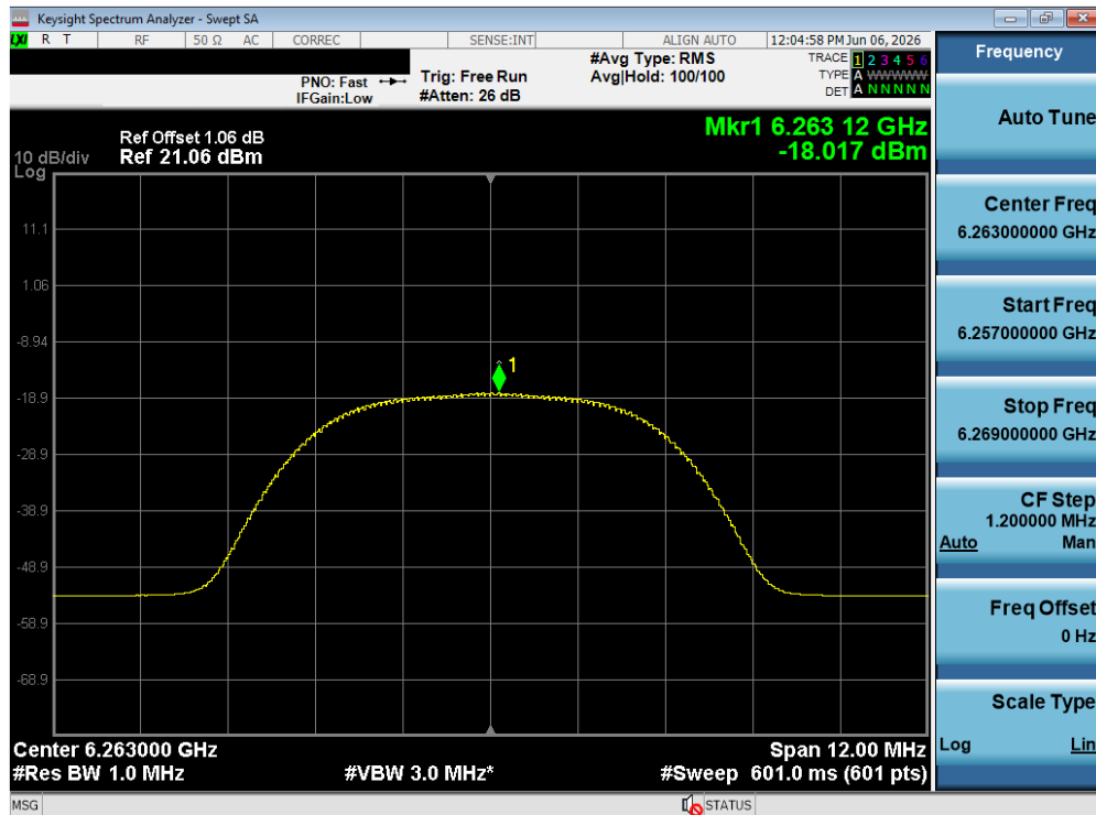
Plot 7-188. PSD TxBF Diversity Antenna WF5T (NB UNII HDR8, iPA – 6263 MHz)
