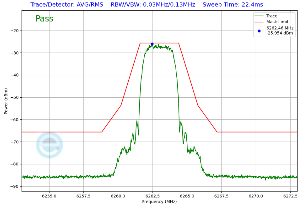
Plot 7-247. In-Band Emission Antenna WF5T (NB UNII HDT6, iPA – 6263 MHz)
