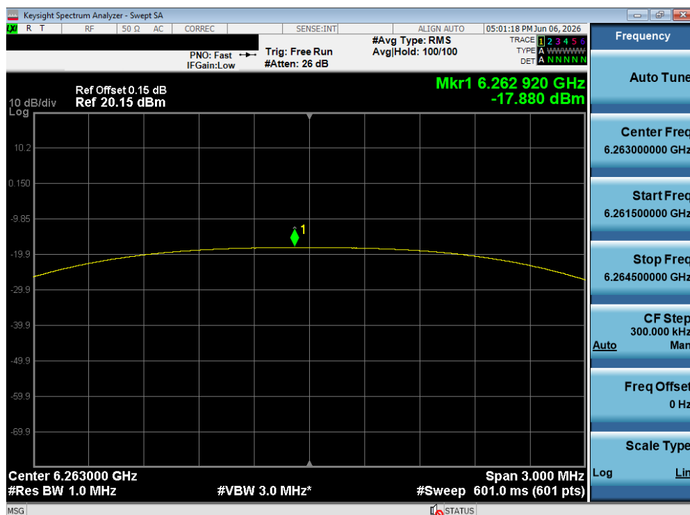
Plot 7-212. PSD Tx BF Diversity Antenna WF5T (NB UNII HDT2, iPA – 6263 MHz)
