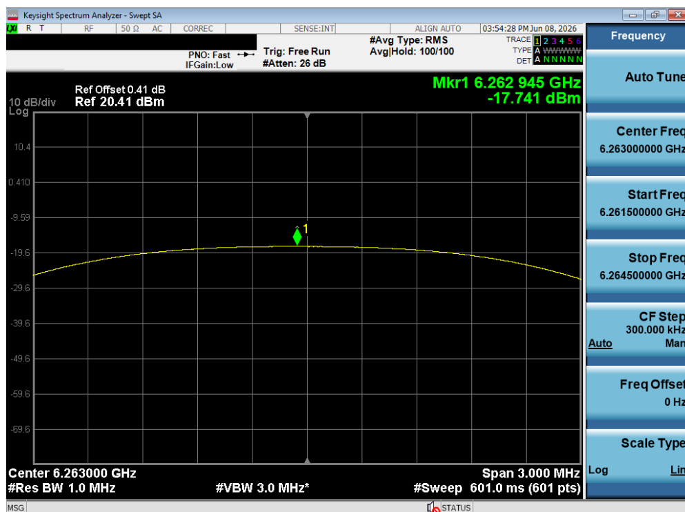
Plot 7-167. PSD TxBF Primary Antenna WF5B (NB UNII HDT6, ePA – 6263 MHz)
