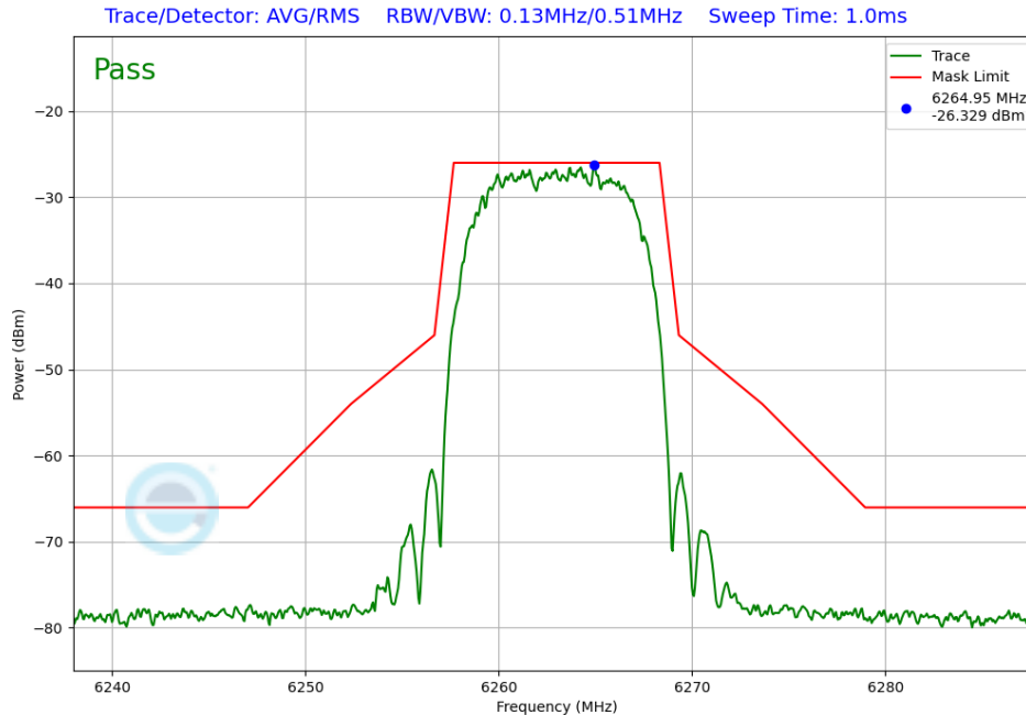
Plot 7-239. In-Band Emission Antenna WF5T (NB UNII HDRPL12, iPA – 6263 MHz)
