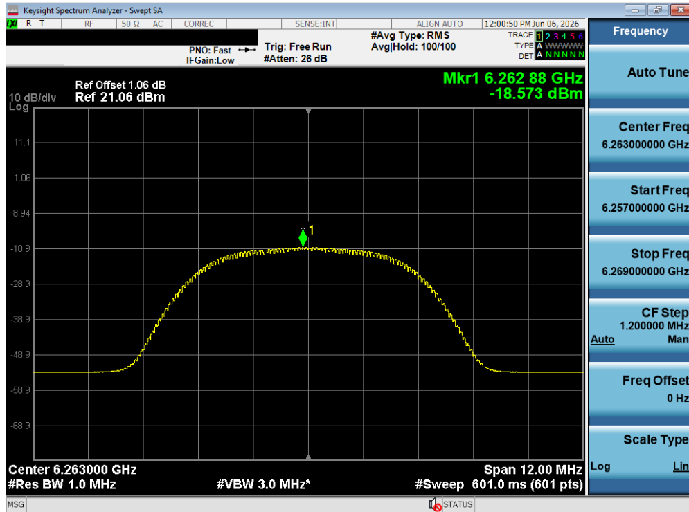
Plot 7-186. PSD TxBF Diversity Antenna WF5T (NB UNII HDR8, ePA – 6263 MHz)
