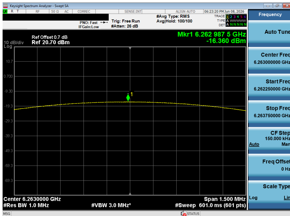
Plot 7-177. PSD TxBF Diversity Antenna WF8 (NB UNII LE1M, iPA – 6263 MHz)
