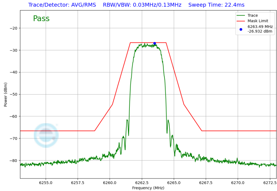
Plot 7-246. In-Band Emission Antenna WF5T (NB UNII HDT6, ePA – 6263 MHz)
