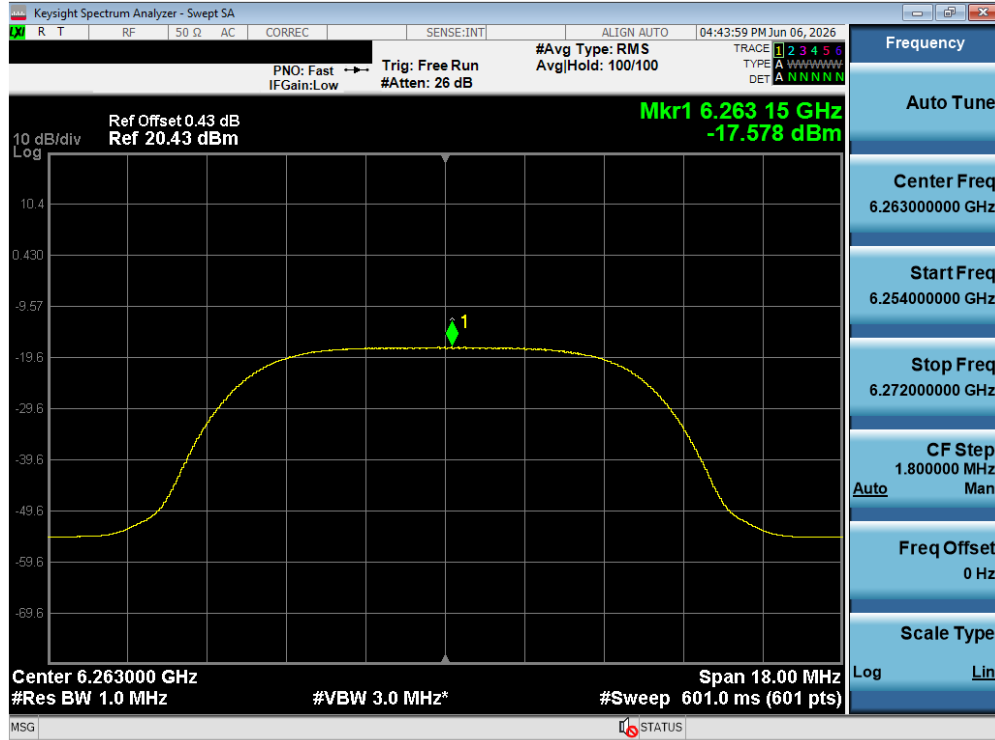
Plot 7-204. PSD Tx BF Diversity Antenna WF5T (NB UNII HDRPL12, iPA – 6263 MHz)
