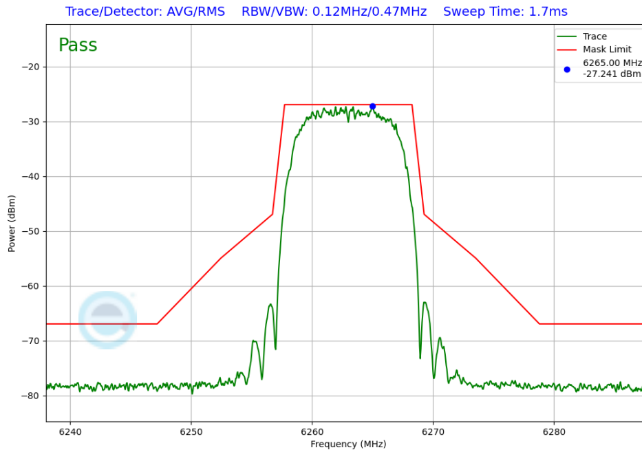
Plot 7-240. In-Band Emission Antenna WF5T (NB UNII HDRPL32, ePA – 6263 MHz)
