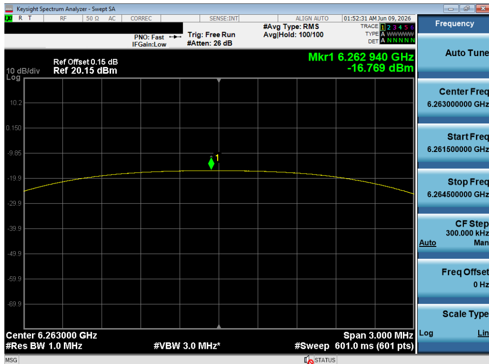
Plot 7-211. PSD TxBF Diversity Antenna WF8 (NB UNII HDT2, ePA – 6263 MHz)
