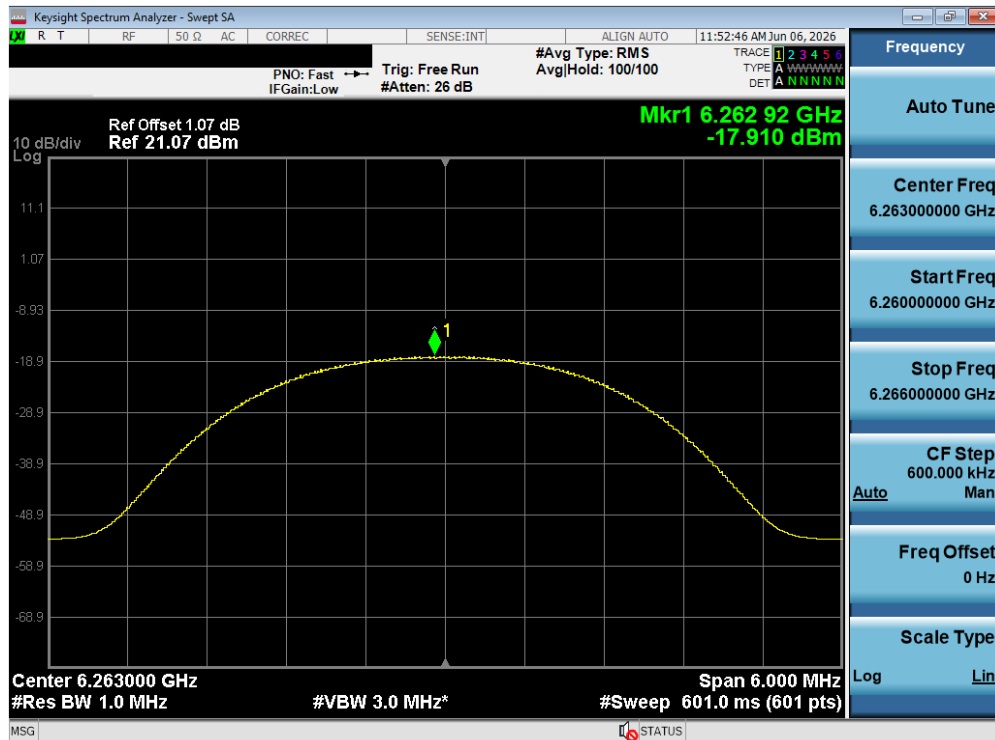
Plot 7-182. PSD TxBF Diversity Antenna WF5T (NB UNII HDR4, ePA – 6263 MHz)
