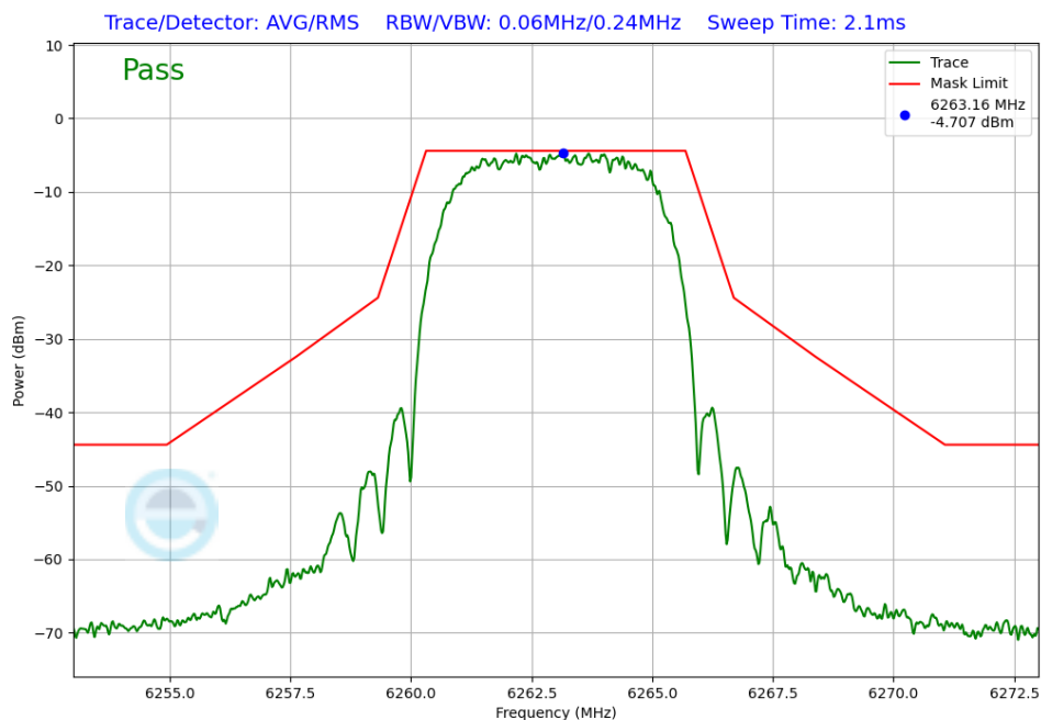
Plot 7-234. In-Band Emission Antenna WF5T (NB UNII XHDRPM6, ePA – 6263 MHz)
