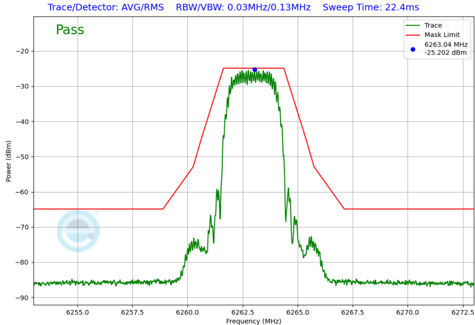
Plot 7-243. In-Band Emission Antenna WF5T (NB UNII HDT2, iPA – 6263 MHz)
