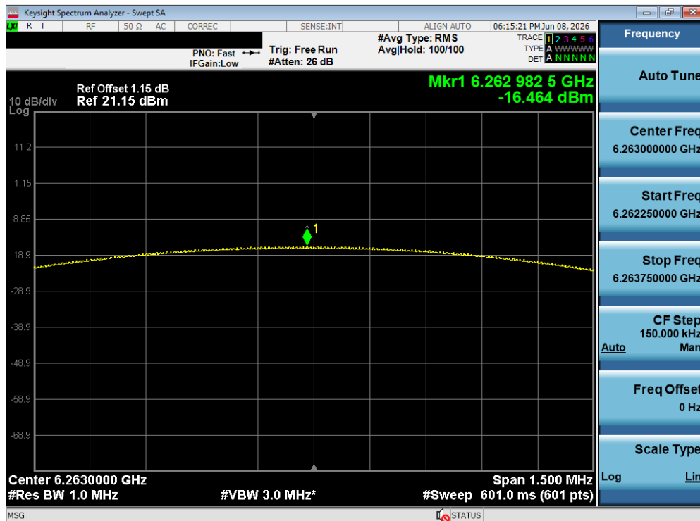
Plot 7-173. PSD Tx BF Diversity Antenna WF8 (NB UNII BDR, iPA – 6263 MHz)
