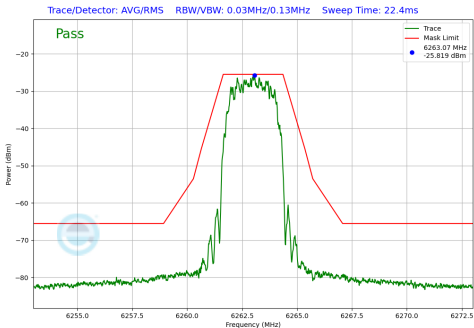
Plot 7-228. In-Band Emission Antenna WF5T (NB UNII HDR4, ePA – 6263 MHz)
