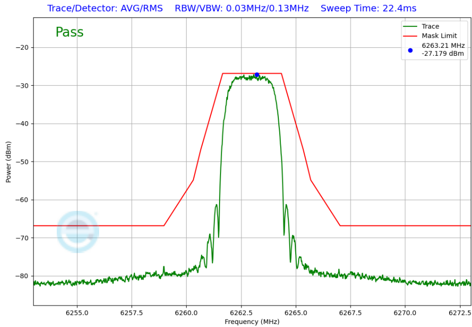
Plot 7-232. In-Band Emission Antenna WF5T (NB UNII HDRPS2, ePA – 6263 MHz)
