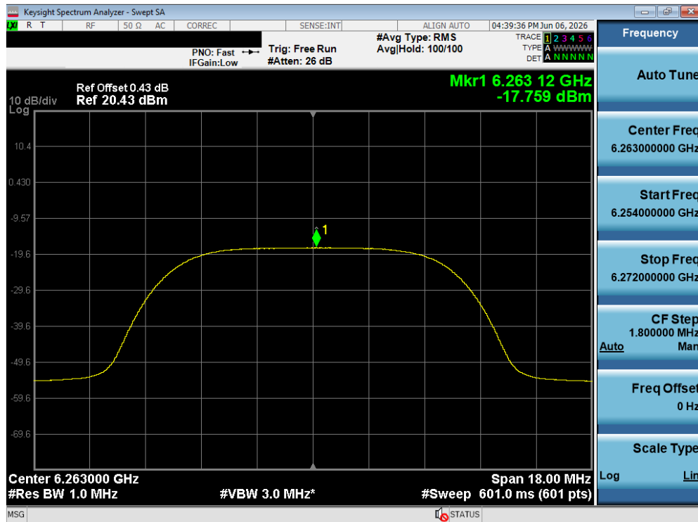
Plot 7-202. PSD TxBF Diversity Antenna WF5T (NB UNII HDRPL12, ePA – 6263 MHz)
