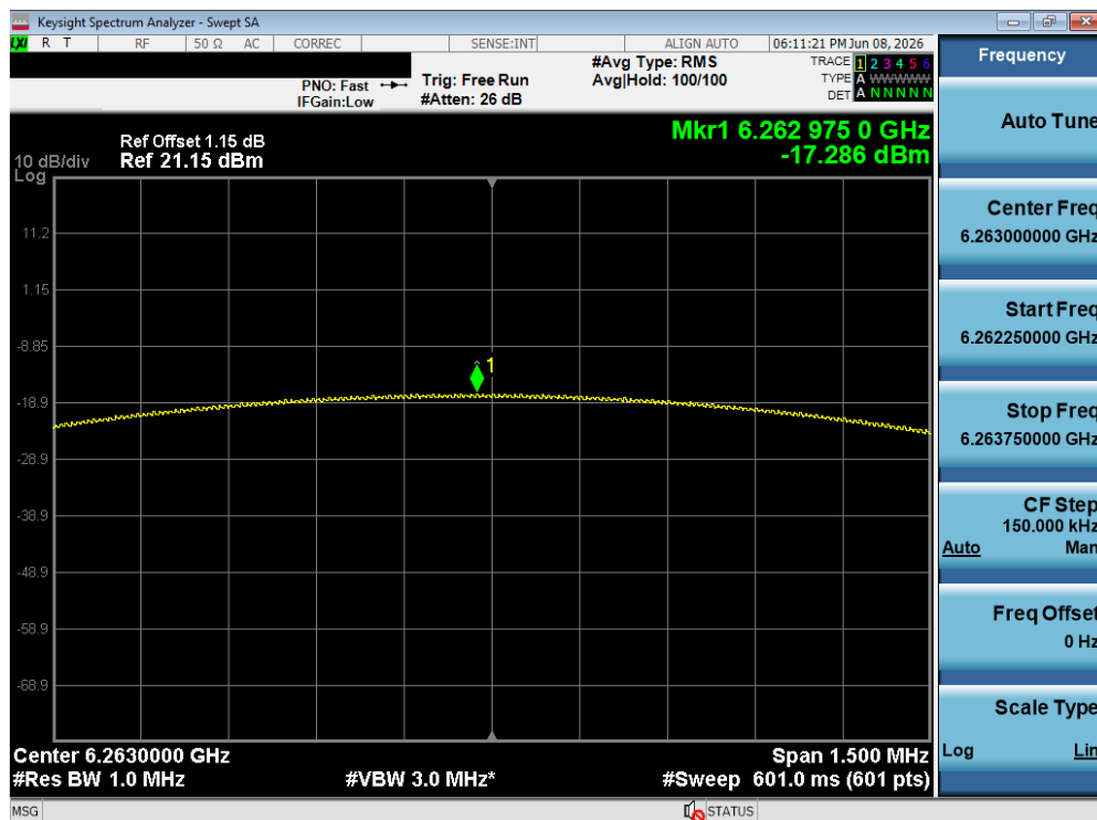
Plot 7-171. PSD TxBF Diversity Antenna WF8 (NB UNII BDR, ePA – 6263 MHz)
