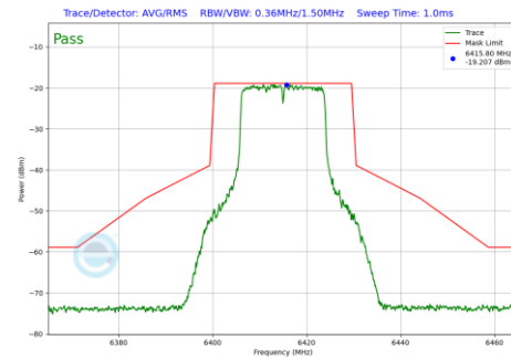
Plot 7-213 In-Band Emission Plot CDD Primary Antenna WF5B (20 MHz BW 802.11a (UNII Band 5) - Ch.93)
