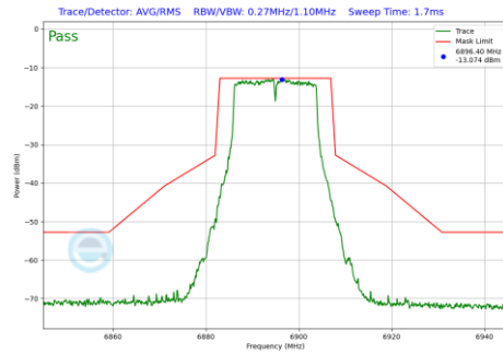
Plot 7-205 In-Band Emission Plot Antenna WF8 (20 MHz BW 802.11a (UNII Band 8) - Ch.189)
