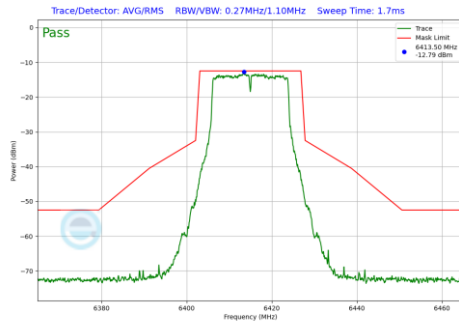
Plot 7-193 In-Band Emission Plot Antenna WF8 (20 MHz BW 802.11a (UNII Band 5) - Ch.93)
