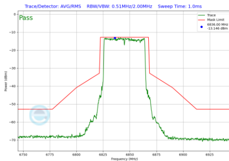
Plot 7-170 In-Band Emission Plot Antenna WF5T (40 MHz BW 802.11be(SU) (UNII Band 7) - Ch.179)
