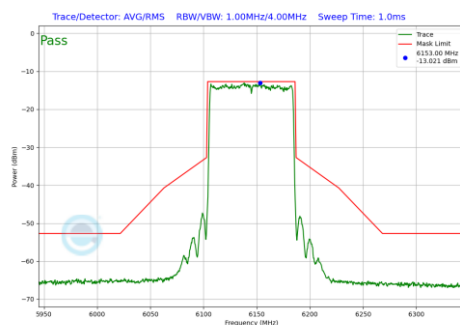
Plot 7-211 In-Band Emission Plot SDM Primary Antenna WF5T (80 MHz BW 802.11be(SU) (UNII Band 5) - Ch.39)
