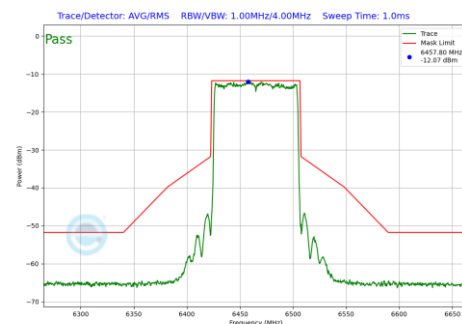
Plot 7-255 In-Band Emission Plot SDM Diversity Antenna WF8 (80 MHz BW 802.11be(SU) (UNII Band 6) - Ch.103)
