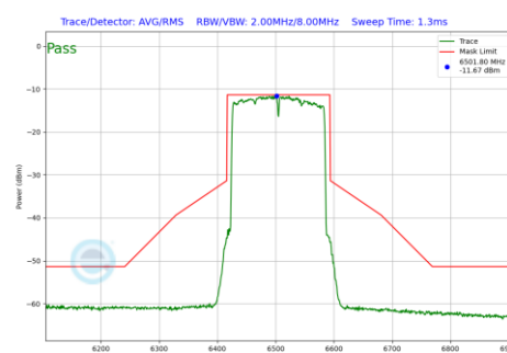
Plot 7-224 In-Band Emission Plot SDM Primary Antenna WF5B (160 MHz BW 802.11be(SU) (UNII Band 6) - Ch.111)
