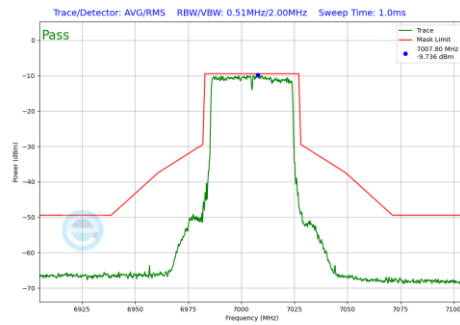
Plot 7-206 In-Band Emission Plot Antenna WF8 (40 MHz BW 802.11be(SU) (UNII Band 8) - Ch.211)
