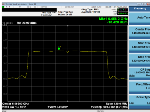
Plot 7-139 PSD SDM Diversity Antenna WF5T (80 MHz BW 802.11be(SU) - Ch.103)
