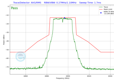
Plot 7-189 In-Band Emission Plot Antenna WF5B (20 MHz BW 802.11a (UNII Band 8) - Ch.189)
