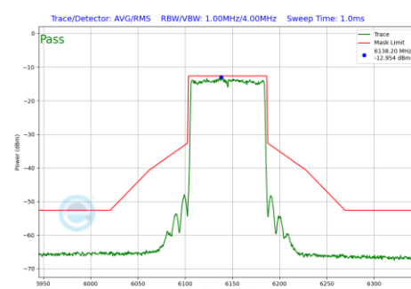
Plot 7-215 In-Band Emission Plot SDM Primary Antenna WF5B (80 MHz BW 802.11be(SU) (UNII Band 5) - Ch.39)
