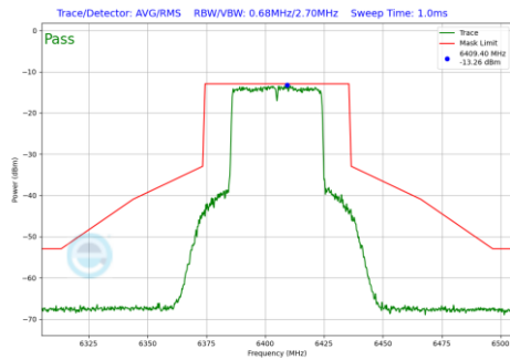
Plot 7-242 In-Band Emission Plot SDM Diversity Antenna WF5T (40 MHz BW 802.11be(SU) (UNII Band 5) - Ch.91)
