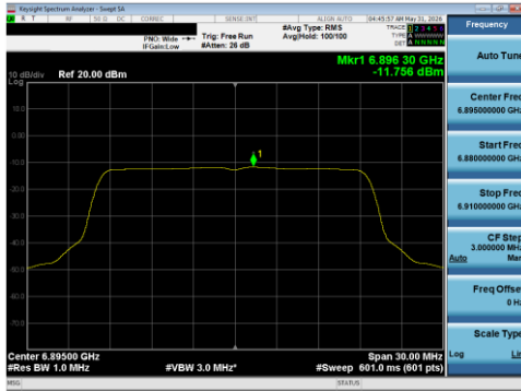
Plot 7-153 PSD SDM Diversity Antenna WF5T (20 MHz BW 802.11be(SU) - Ch.189)
