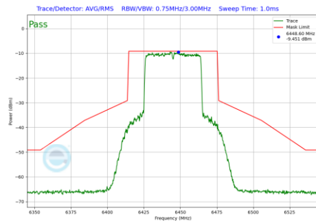
Plot 7-182 In-Band Emission Plot Antenna WF5B (40 MHz BW 802.11be(SU) (UNII Band 6) - Ch.99)
