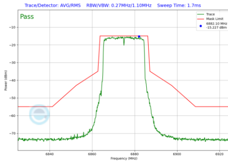
Plot 7-185 In-Band Emission Plot Antenna WF5B (20 MHz BW 802.11be(SU) (UNII Band 7) - Ch.185)
