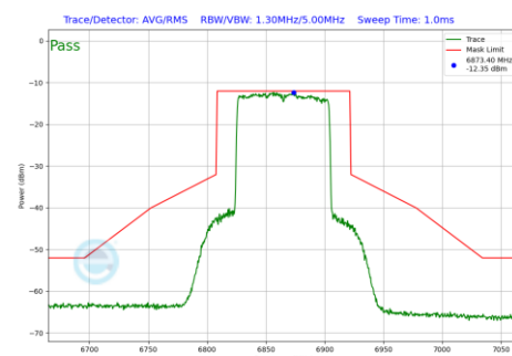
Plot 7-231 In-Band Emission Plot SDM Primary Antenna WF5B (80 MHz BW 802.11be(SU) (UNII Band 7) - Ch.183)
