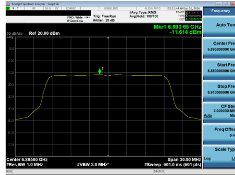
Plot 7-125 PSD SDM Primary Antenna WF5B (20 MHz BW 802.11be(SU) - Ch.189)
