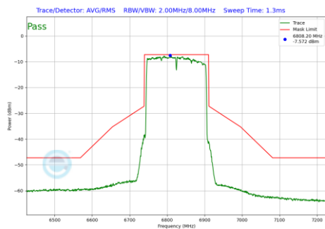
Plot 7-204 In-Band Emission Plot Antenna WF8 (160 MHz BW 802.11be(SU) (UNII Band 7) - Ch.175)
