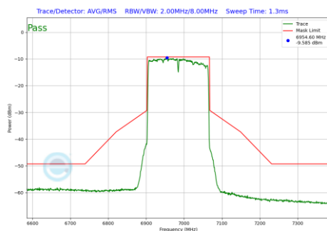
Plot 7-236 In-Band Emission Plot SDM Primary Antenna WF5T (160 MHz BW 802.11be(SU) (UNII Band 8) - Ch.207)
