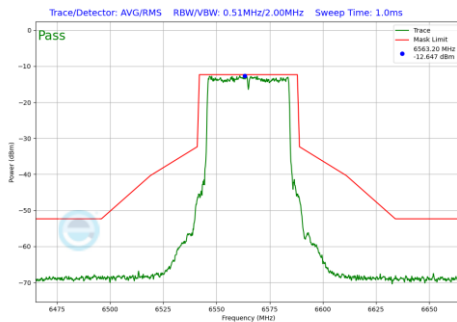
Plot 7-186 In-Band Emission Plot Antenna WF5B (40 MHz BW 802.11be(SU) (UNII Band 7) - Ch.123)
