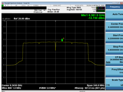
Plot 7-132 PSD SDM Diversity Antenna WF5T (160 MHz BW 802.11be(SU) - Ch.79)
