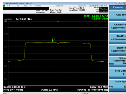
Plot 7-151 PSD SDM Diversity Antenna WF8 (80 MHz BW 802.11be(SU) - Ch.183)
