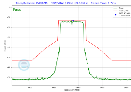
Plot 7-197 In-Band Emission Plot Antenna WF8 (20 MHz BW 802.11be(SU) (UNII Band 6) - Ch.97)
