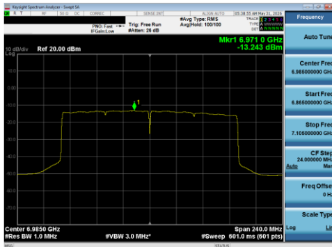
Plot 7-156 PSD SDM Diversity Antenna WF5T (160 MHz BW 802.11be(SU) - Ch.207)
