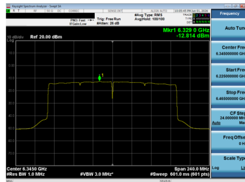
Plot 7-136 PSD SDM Diversity Antenna WF8 (160 MHz BW 802.11be(SU) - Ch.79)
