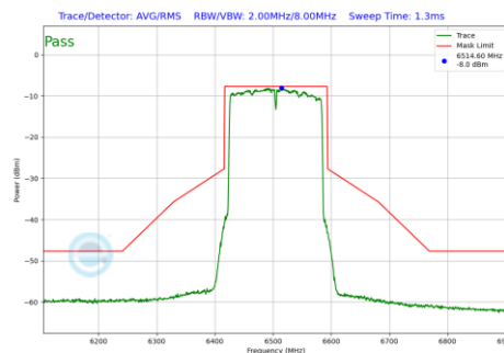
Plot 7-184 In-Band Emission Plot Antenna WF5B (160 MHz BW 802.11be(SU) (UNII Band 6) - Ch.111)
