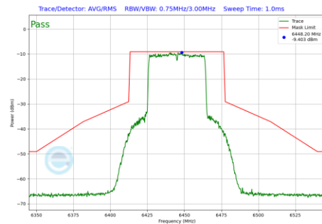
Plot 7-198 In-Band Emission Plot Antenna WF8 (40 MHz BW 802.11be(SU) (UNII Band 6) - Ch.99)
