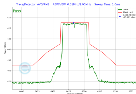
Plot 7-222 In-Band Emission Plot SDM Primary Antenna WF5B (40 MHz BW 802.11be(SU) (UNII Band 6) - Ch.107)
