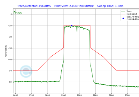
Plot 7-240 In-Band Emission Plot SDM Primary Antenna WF5B (160 MHz BW 802.11be(SU) (UNII Band 8) - Ch.207)
