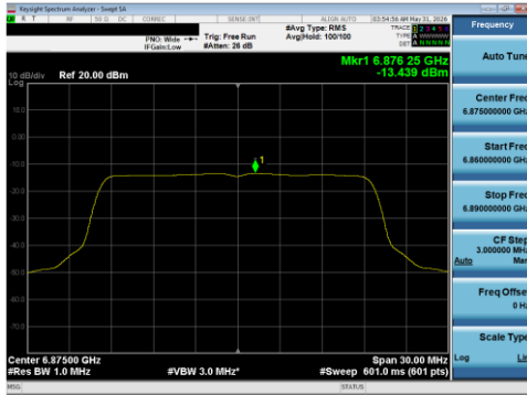
Plot 7-113 PSD SDM Primary Antenna WF5T (20 MHz BW 802.11be(SU) - Ch.185)
