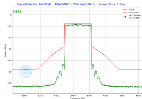
Plot 7-199 In-Band Emission Plot Antenna WF8 (80 MHz BW 802.11be(SU) (UNII Band 6) - Ch.103)
