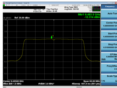
Plot 7-142 PSD SDM Diversity Antenna WF8 (40 MHz BW 802.11be(SU) - Ch.107)
