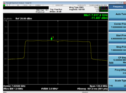
Plot 7-159 PSD SDM Diversity Antenna WF8 (80 MHz BW 802.11be(SU) - Ch.215)
