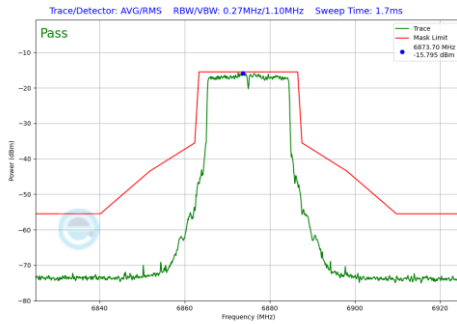
Plot 7-169 In-Band Emission Plot Antenna WF5T (20 MHz BW 802.11be(SU) (UNII Band 7) - Ch.185)
