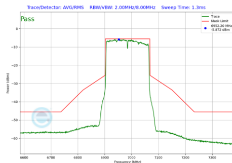
Plot 7-192 In-Band Emission Plot Antenna WF5B (160 MHz BW 802.11be(SU) (UNII Band 8) - Ch.207)
