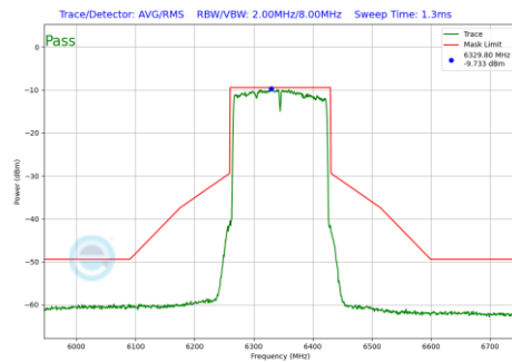
Plot 7-248 In-Band Emission Plot SDM Diversity Antenna WF8 (160 MHz BW 802.11be(SU) (UNII Band 5) - Ch.79)
