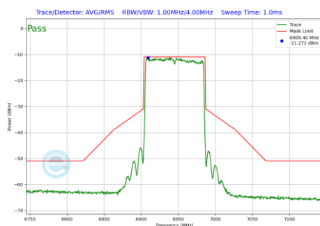
Plot 7-235 In-Band Emission Plot SDM Primary Antenna WF5T (80 MHz BW 802.11be(SU) (UNII Band 8) - Ch.199)
