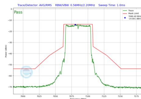
Plot 7-238 In-Band Emission Plot SDM Primary Antenna WF5B (40 MHz BW 802.11be(SU) (UNII Band 8) - Ch.227)
