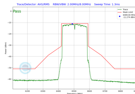
Plot 7-256 In-Band Emission Plot SDM Diversity Antenna WF8 (160 MHz BW 802.11be(SU) (UNII Band 6) - Ch.111)
