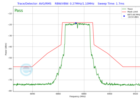
Plot 7-229 In-Band Emission Plot SDM Primary Antenna WF5B (20 MHz BW 802.11be(SU) (UNII Band 7) - Ch.185)
