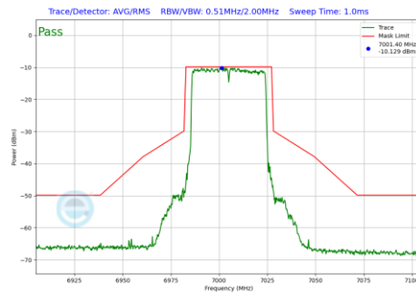
Plot 7-190 In-Band Emission Plot Antenna WF5B (40 MHz BW 802.11be(SU) (UNII Band 8) - Ch.211)
