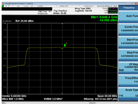
Plot 7-146 PSD SDM Diversity Antenna WF5T (40 MHz BW 802.11be(SU) - Ch.179)
