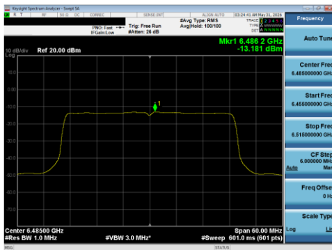
Plot 7-106 PSD SDM Primary Antenna WF5T (40 MHz BW 802.11be(SU) - Ch.107)
