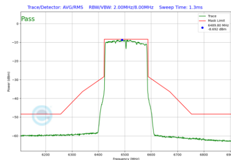
Plot 7-168 In-Band Emission Plot Antenna WF5T (160 MHz BW 802.11be(SU) (UNII Band 6) - Ch.111)
