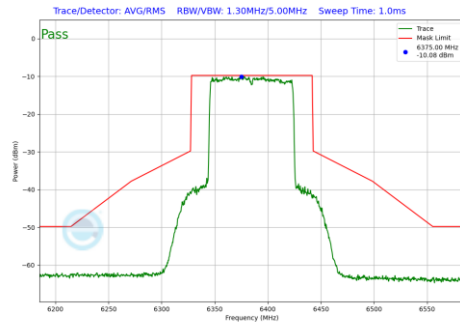
Plot 7-247 In-Band Emission Plot SDM Diversity Antenna WF8 (80 MHz BW 802.11be(SU) (UNII Band 5) - Ch.87)
