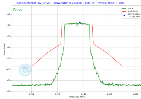
Plot 7-249 In-Band Emission Plot SDM Diversity Antenna WF5T (20 MHz BW 802.11be(SU) (UNII Band 6) - Ch.97)
