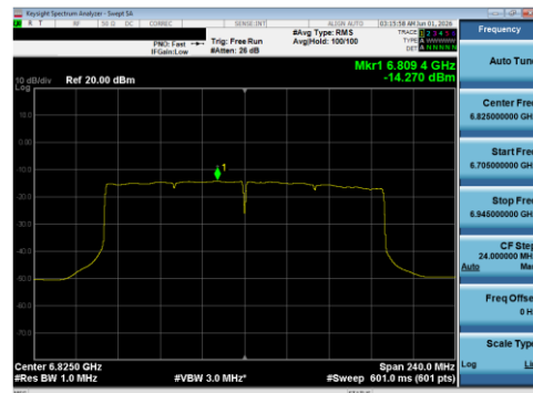
Plot 7-120 PSD SDM Primary Antenna WF5B (160 MHz BW 802.11be(SU) - Ch.175)
