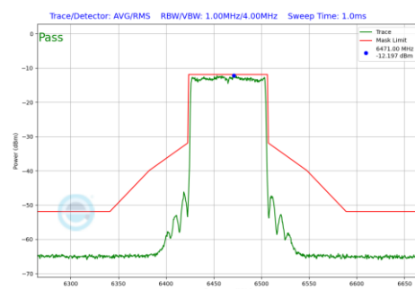
Plot 7-223 In-Band Emission Plot SDM Primary Antenna WF5B (80 MHz BW 802.11be(SU) (UNII Band 6) - Ch.103)
