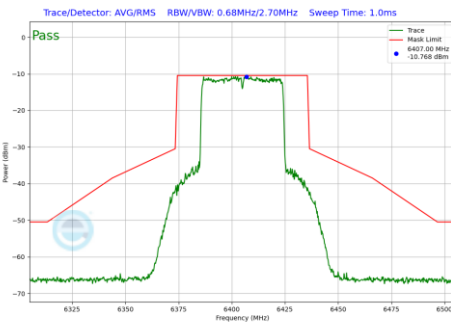
Plot 7-162 In-Band Emission Plot Antenna WF5T (40 MHz BW 802.11be(SU) (UNII Band 5) - Ch.91)
