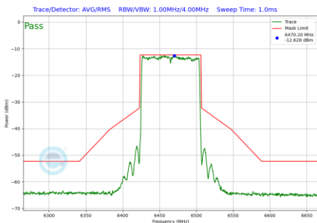
Plot 7-219 In-Band Emission Plot SDM Primary Antenna WF5T (80 MHz BW 802.11be(SU) (UNII Band 6) - Ch.103)
