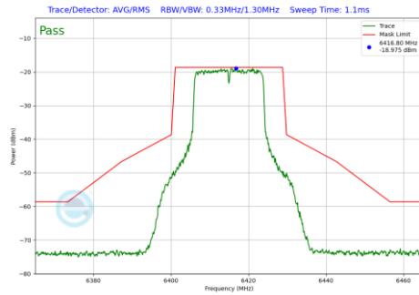
Plot 7-209 In-Band Emission Plot CDD Primary Antenna WF5T (20 MHz BW 802.11a (UNII Band 5) - Ch.93)
