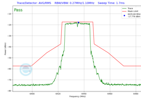
Plot 7-221 In-Band Emission Plot SDM Primary Antenna WF5B (20 MHz BW 802.11be(SU) (UNII Band 6) - Ch.97)
