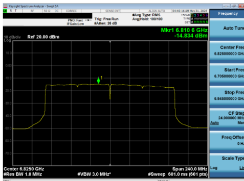
Plot 7-116 PSD SDM Primary Antenna WF5T (160 MHz BW 802.11be(SU) - Ch.175)
