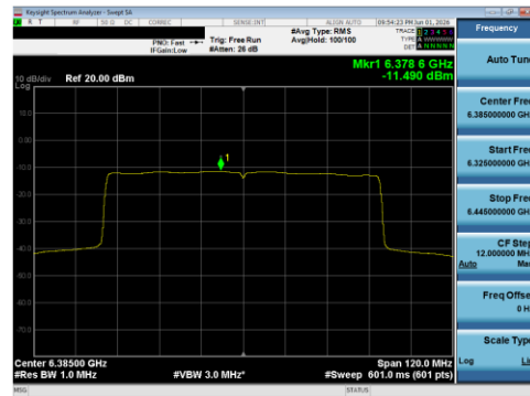
Plot 7-135 PSD SDM Diversity Antenna WF8 (80 MHz BW 802.11be(SU) - Ch.87)
