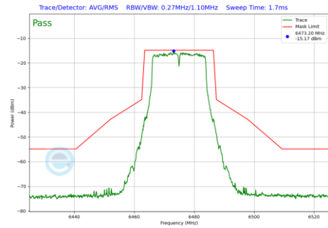
Plot 7-165 In-Band Emission Plot Antenna WF5T (20 MHz BW 802.11a (UNII Band 6) - Ch.105)
