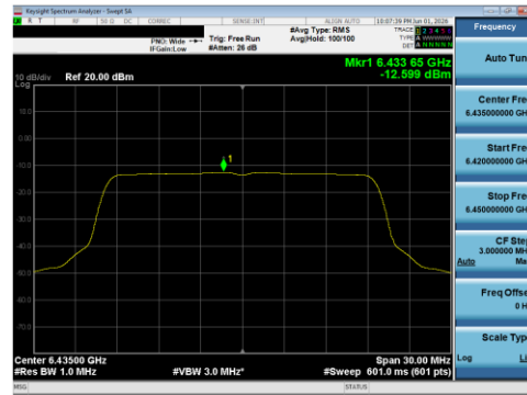
Plot 7-141 PSD SDM Diversity Antenna WF8 (20 MHz BW 802.11be(SU) - Ch.97)
