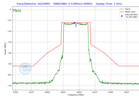
Plot 7-166 In-Band Emission Plot Antenna WF5T (40 MHz BW 802.11be(SU) (UNII Band 6) - Ch.99)
