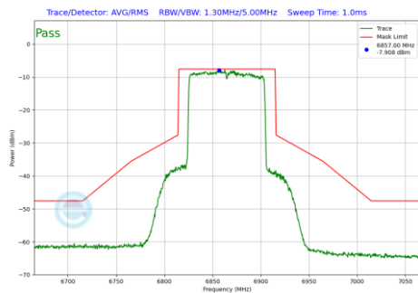
Plot 7-203 In-Band Emission Plot Antenna WF8 (80 MHz BW 802.11be(SU) (UNII Band 7) - Ch.183)
