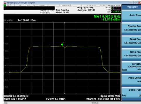
Plot 7-118 PSD SDM Primary Antenna WF5B (40 MHz BW 802.11be(SU) - Ch.123)
