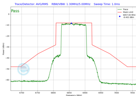
Plot 7-187 In-Band Emission Plot Antenna WF5B (80 MHz BW 802.11be(SU) (UNII Band 7) - Ch.183)
