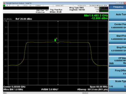
Plot 7-110 PSD SDM Primary Antenna WF5B (40 MHz BW 802.11be(SU) - Ch.107)
