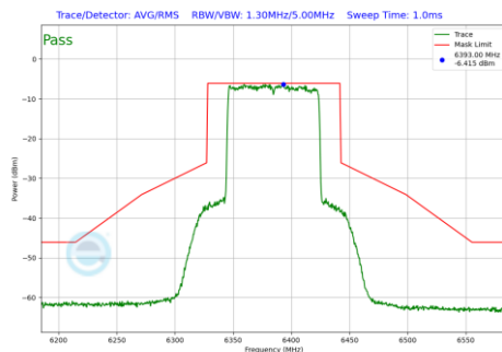
Plot 7-195 In-Band Emission Plot Antenna WF8 (80 MHz BW 802.11be(SU) (UNII Band 5) - Ch.87)
