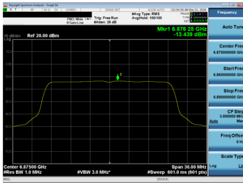
Plot 7-145 PSD SDM Diversity Antenna WF5T (20 MHz BW 802.11be(SU) - Ch.185)
