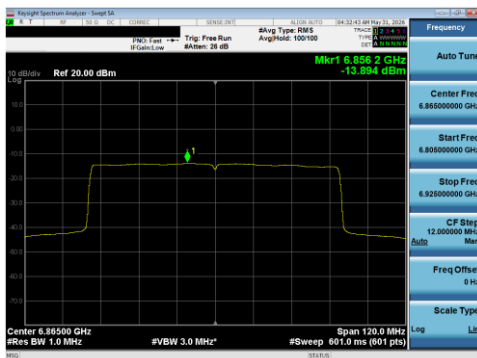
Plot 7-147 PSD SDM Diversity Antenna WF5T (80 MHz BW 802.11be(SU) - Ch.183)
