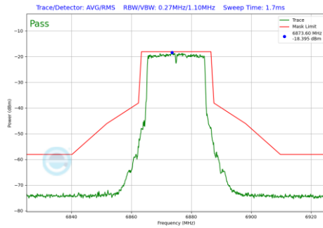
Plot 7-225 In-Band Emission Plot SDM Primary Antenna WF5T (20 MHz BW 802.11be(SU) (UNII Band 7) - Ch.185)
