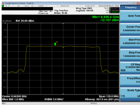
Plot 7-123 PSD SDM Primary Antenna WF5T (80 MHz BW 802.11be(SU) - Ch.199)
