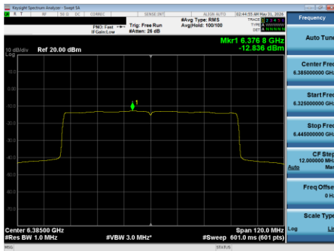
Plot 7-131 PSD SDM Diversity Antenna WF5T (80 MHz BW 802.11be(SU) - Ch.87)
