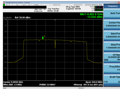
Plot 7-128 PSD SDM Primary Antenna WF5B (160 MHz BW 802.11be(SU) - Ch.207)
