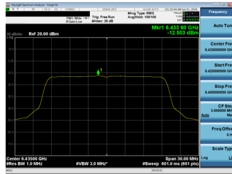
Plot 7-109 PSD SDM Primary Antenna WF5B (20 MHz BW 802.11be(SU) - Ch.97)
