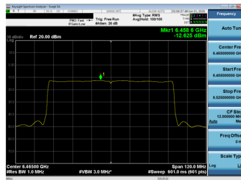
Plot 7-111 PSD SDM Primary Antenna WF5B (80 MHz BW 802.11be(SU) - Ch.103)
