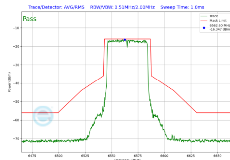
Plot 7-230 In-Band Emission Plot SDM Primary Antenna WF5B (40 MHz BW 802.11be(SU) (UNII Band 7) - Ch.123)
