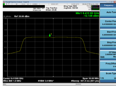
Plot 7-133 PSD SDM Diversity Antenna WF8 (20 MHz BW 802.11be(SU) - Ch.93)
