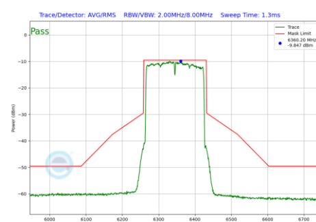
Plot 7-216 In-Band Emission Plot SDM Primary Antenna WF5B (160 MHz BW 802.11be(SU) (UNII Band 5) - Ch.79)
