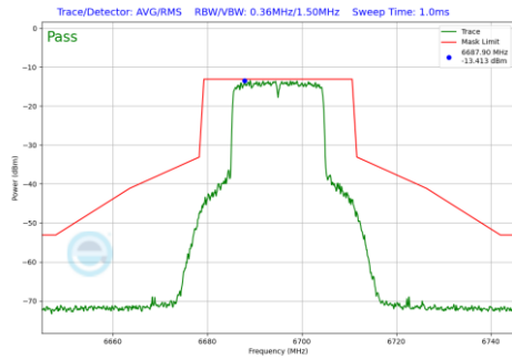
Plot 7-201 In-Band Emission Plot Antenna WF8 (20 MHz BW 802.11be(SU) (UNII Band 7) - Ch.149)
