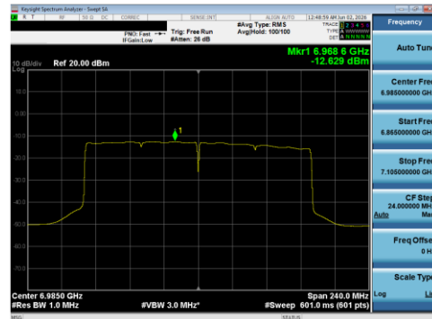
Plot 7-160 PSD SDM Diversity Antenna WF8 (160 MHz BW 802.11be(SU) - Ch.207)
