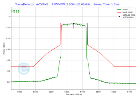
Plot 7-180 In-Band Emission Plot Antenna WF5B (160 MHz BW 802.11be(SU) (UNII Band 5) - Ch.79)
