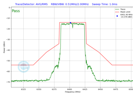
Plot 7-210 In-Band Emission Plot SDM Primary Antenna WF5T (40 MHz BW 802.11be(SU) (UNII Band 5) - Ch.91)
