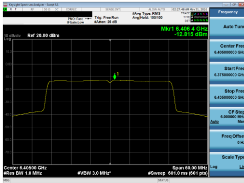
Plot 7-130 PSD SDM Diversity Antenna WF5T (40 MHz BW 802.11be(SU) - Ch.91)
