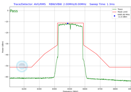
Plot 7-220 In-Band Emission Plot SDM Primary Antenna WF5T (160 MHz BW 802.11be(SU) (UNII Band 6) - Ch.111)
