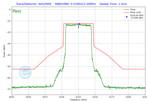
Plot 7-178 In-Band Emission Plot Antenna WF5B (40 MHz BW 802.11be(SU) (UNII Band 5) - Ch.35)
