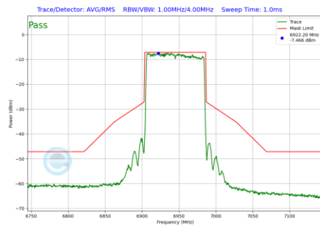
Plot 7-207 In-Band Emission Plot Antenna WF8 (80 MHz BW 802.11be(SU) (UNII Band 8) - Ch.199)
