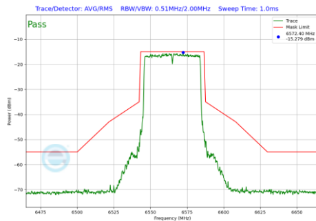
Plot 7-226 In-Band Emission Plot SDM Primary Antenna WF5T (40 MHz BW 802.11be(SU) (UNII Band 7) - Ch.123)
