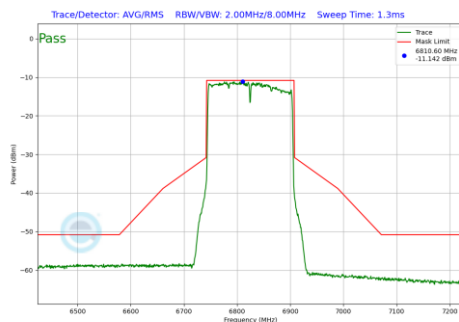
Plot 7-228 In-Band Emission Plot SDM Primary Antenna WF5T (160 MHz BW 802.11be(SU) (UNII Band 7) - Ch.175)
