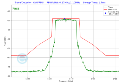
Plot 7-253 In-Band Emission Plot SDM Diversity Antenna WF8 (20 MHz BW 802.11be(SU) (UNII Band 6) - Ch.97)
