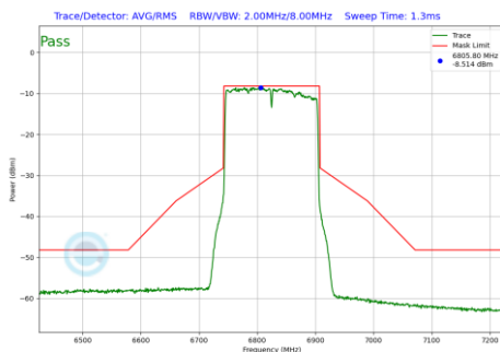
Plot 7-172 In-Band Emission Plot Antenna WF5T (160 MHz BW 802.11be(SU) (UNII Band 7) - Ch.175)
