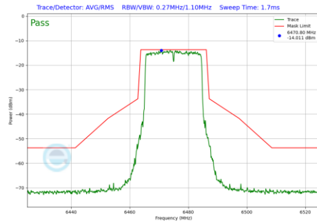
Plot 7-181 In-Band Emission Plot Antenna WF5B (20 MHz BW 802.11be(SU) (UNII Band 6) - Ch.105)
