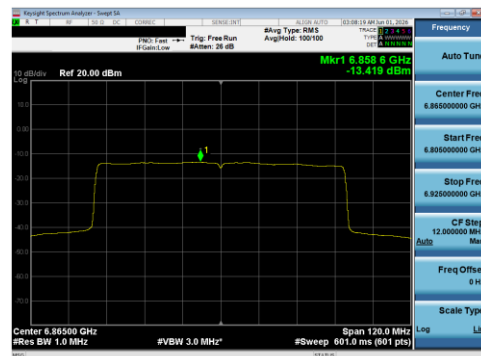
Plot 7-119 PSD SDM Primary Antenna WF5B (80 MHz BW 802.11be(SU) - Ch.183)
