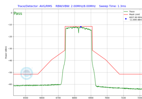
Plot 7-232 In-Band Emission Plot SDM Primary Antenna WF5B (160 MHz BW 802.11be(SU) (UNII Band 7) - Ch.175)
