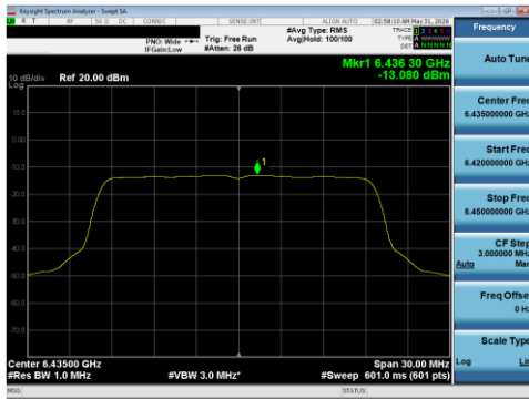
Plot 7-105 PSD SDM Primary Antenna WF5T (20 MHz BW 802.11be(SU) - Ch.97)
