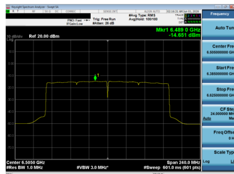
Plot 7-112 PSD SDM Primary Antenna WF5B (160 MHz BW 802.11be(SU) - Ch.111)
