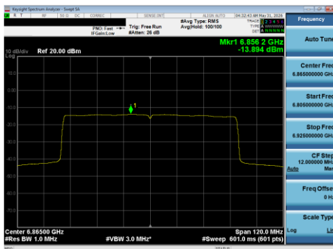
Plot 7-115 PSD SDM Primary Antenna WF5T (80 MHz BW 802.11be(SU) - Ch.183)
