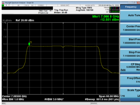
Plot 7-122 PSD SDM Primary Antenna WF5T (40 MHz BW 802.11be(SU) - Ch.227)
