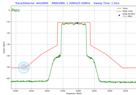
Plot 7-243 In-Band Emission Plot SDM Diversity Antenna WF5T (80 MHz BW 802.11be(SU) (UNII Band 5) - Ch.87)
