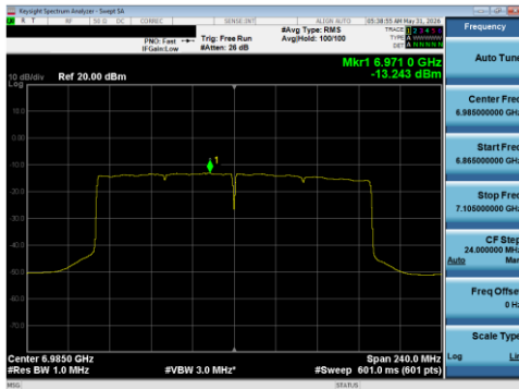
Plot 7-124 PSD SDM Primary Antenna WF5T (160 MHz BW 802.11be(SU) - Ch.207)
