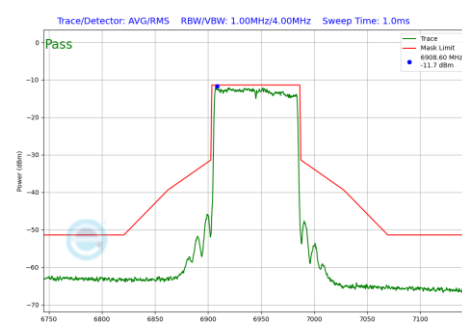
Plot 7-239 In-Band Emission Plot SDM Primary Antenna WF5B (80 MHz BW 802.11be(SU) (UNII Band 8) - Ch.199)
