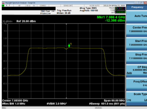
Plot 7-154 PSD SDM Diversity Antenna WF5T (40 MHz BW 802.11be(SU) - Ch.227)
