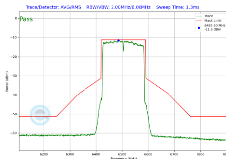
Plot 7-252 In-Band Emission Plot SDM Diversity Antenna WF5T (160 MHz BW 802.11be(SU) (UNII Band 6) - Ch.111)
