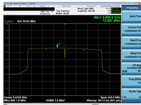
Plot 7-152 PSD SDM Diversity Antenna WF8 (160 MHz BW 802.11be(SU) - Ch.175)
