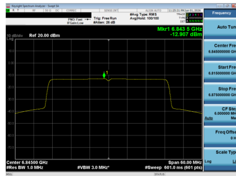
Plot 7-150 PSD SDM Diversity Antenna WF8 (40 MHz BW 802.11be(SU) - Ch.179)
