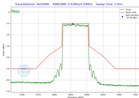
Plot 7-171 In-Band Emission Plot Antenna WF5T (80 MHz BW 802.11be(SU) (UNII Band 7) - Ch.183)
