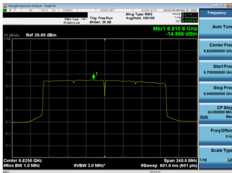
Plot 7-148 PSD SDM Diversity Antenna WF5T (160 MHz BW 802.11be(SU) - Ch.175)
