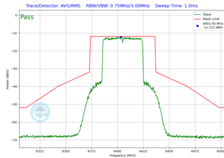
Plot 7-246 In-Band Emission Plot SDM Diversity Antenna WF8 (40 MHz BW 802.11be(SU) (UNII Band 5) - Ch.91)
