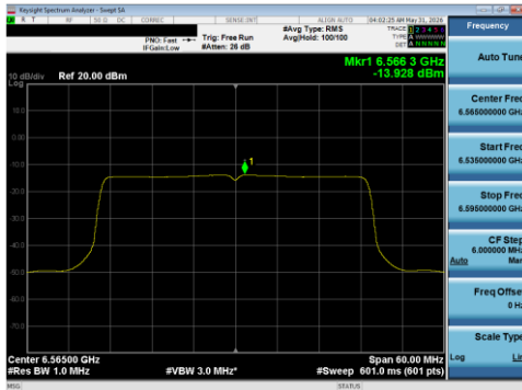
Plot 7-114 PSD SDM Primary Antenna WF5T (40 MHz BW 802.11be(SU) - Ch.123)
