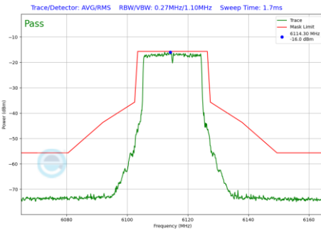
Plot 7-161 In-Band Emission Plot Antenna WF5T (20 MHz BW 802.11be(SU) (UNII Band 5) - Ch.33)
