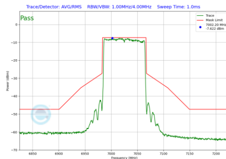
Plot 7-191 In-Band Emission Plot Antenna WF5B (80 MHz BW 802.11be(SU) (UNII Band 8) - Ch.215)
