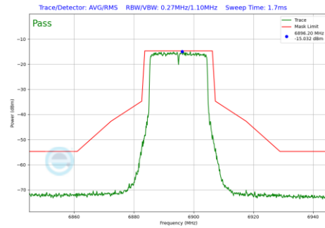
Plot 7-173 In-Band Emission Plot Antenna WF5T (20 MHz BW 802.11be(SU) (UNII Band 8) - Ch.189)
