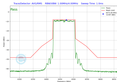
Plot 7-183 In-Band Emission Plot Antenna WF5B (80 MHz BW 802.11be(SU) (UNII Band 6) - Ch.103)
