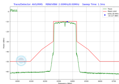
Plot 7-212 In-Band Emission Plot SDM Primary Antenna WF5T (160 MHz BW 802.11be(SU) (UNII Band 5) - Ch.79)
