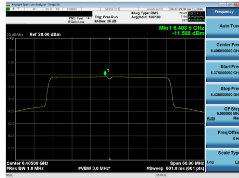
Plot 7-134 PSD SDM Diversity Antenna WF8 (40 MHz BW 802.11be(SU) - Ch.91)
