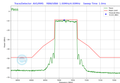
Plot 7-175 In-Band Emission Plot Antenna WF5T (80 MHz BW 802.11be(SU) (UNII Band 8) - Ch.215)
