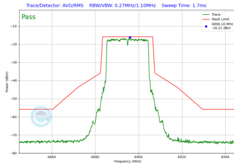
Plot 7-233 In-Band Emission Plot SDM Primary Antenna WF5T (20 MHz BW 802.11be(SU) (UNII Band 8) - Ch.189)
