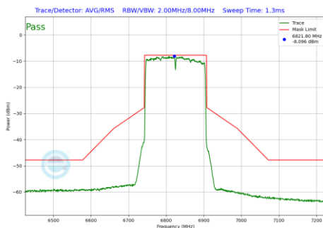
Plot 7-188 In-Band Emission Plot Antenna WF5B (160 MHz BW 802.11be(SU) (UNII Band 7) - Ch.175)
