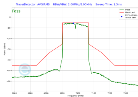
Plot 7-208 In-Band Emission Plot Antenna WF8 (160 MHz BW 802.11be(SU) (UNII Band 8) - Ch.207)
