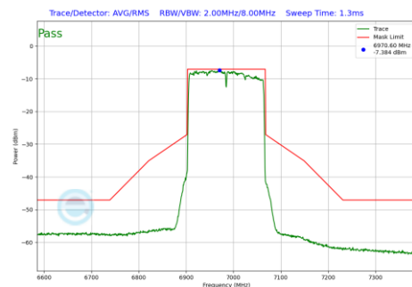
Plot 7-176 In-Band Emission Plot Antenna WF5T (160 MHz BW 802.11be(SU) (UNII Band 8) - Ch.207)
