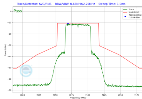
Plot 7-174 In-Band Emission Plot Antenna WF5T (40 MHz BW 802.11be(SU) (UNII Band 8) - Ch.227)
