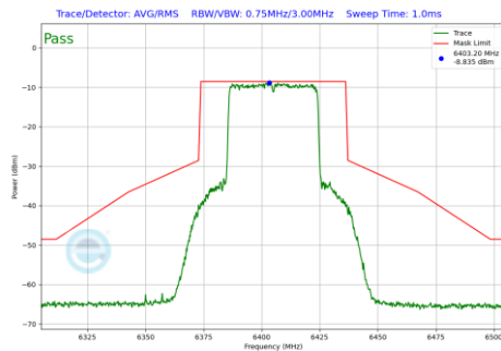
Plot 7-194 In-Band Emission Plot Antenna WF8 (40 MHz BW 802.11be(SU) (UNII Band 5) - Ch.91)
