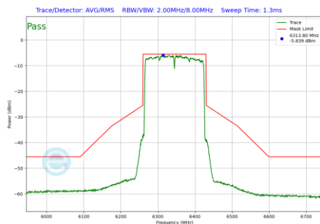
Plot 7-196 In-Band Emission Plot Antenna WF8 (160 MHz BW 802.11be(SU) (UNII Band 5) - Ch.79)
