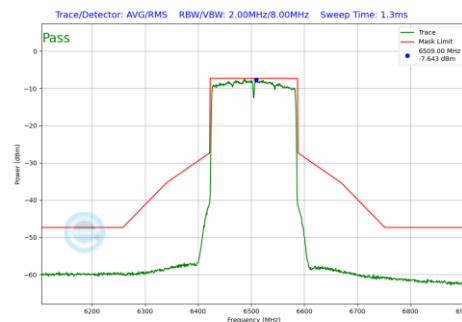
Plot 7-200 In-Band Emission Plot Antenna WF8 (160 MHz BW 802.11be(SU) (UNII Band 6) - Ch.111)
