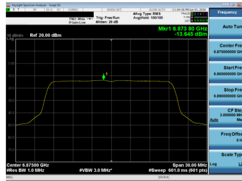
Plot 7-149 PSD SDM Diversity Antenna WF8 (20 MHz BW 802.11be(SU) - Ch.185)
