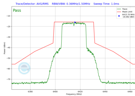
Plot 7-245 In-Band Emission Plot SDM Diversity Antenna WF8 (20 MHz BW 802.11be(SU) (UNII Band 5) - Ch.93)
