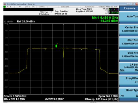
Plot 7-144 PSD SDM Diversity Antenna WF8 (160 MHz BW 802.11be(SU) - Ch.111)
