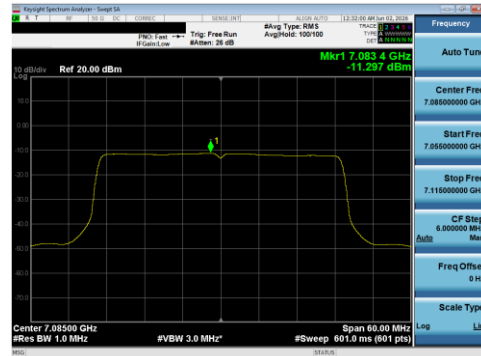
Plot 7-158 PSD SDM Diversity Antenna WF8 (40 MHz BW 802.11be(SU) - Ch.227)
