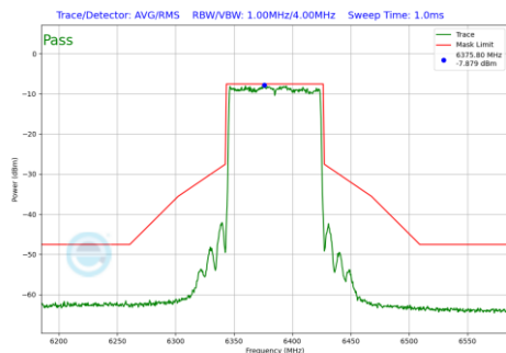
Plot 7-179 In-Band Emission Plot Antenna WF5B (80 MHz BW 802.11be(SU) (UNII Band 5) - Ch.87)
