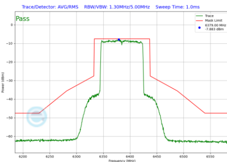
Plot 7-163 In-Band Emission Plot Antenna WF5T (80 MHz BW 802.11be(SU) (UNII Band 5) - Ch.87)
