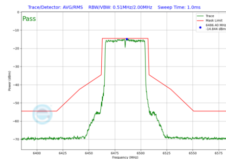
Plot 7-254 In-Band Emission Plot SDM Diversity Antenna WF8 (40 MHz BW 802.11be(SU) (UNII Band 6) - Ch.107)
