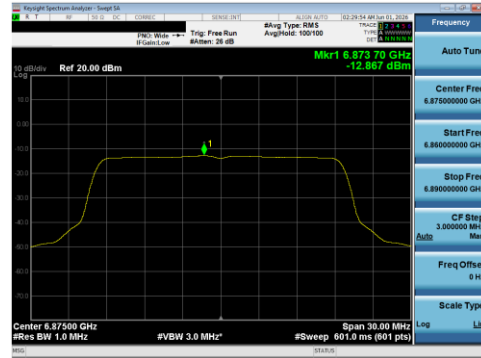
Plot 7-117 PSD SDM Primary Antenna WF5B (20 MHz BW 802.11be(SU) - Ch.185)
