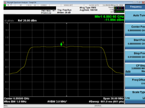
Plot 7-157 PSD SDM Diversity Antenna WF8 (20 MHz BW 802.11be(SU) - Ch.189)
