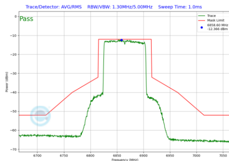
Plot 7-227 In-Band Emission Plot SDM Primary Antenna WF5T (80 MHz BW 802.11be(SU) (UNII Band 7) - Ch.183)
