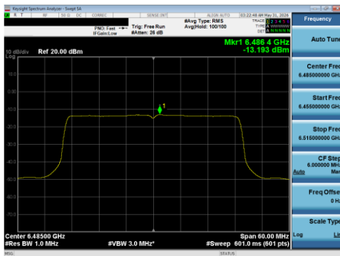
Plot 7-138 PSD SDM Diversity Antenna WF5T (40 MHz BW 802.11be(SU) - Ch.107)
