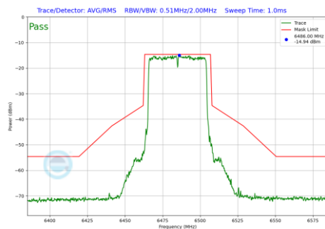
Plot 7-250 In-Band Emission Plot SDM Diversity Antenna WF5T (40 MHz BW 802.11be(SU) (UNII Band 6) - Ch.107)
