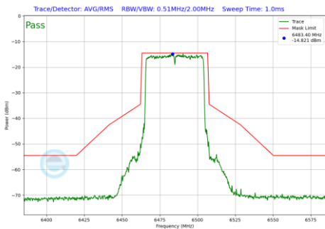
Plot 7-218 In-Band Emission Plot SDM Primary Antenna WF5T (40 MHz BW 802.11be(SU) (UNII Band 6) - Ch.107)
