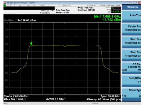
Plot 7-126 PSD SDM Primary Antenna WF5B (40 MHz BW 802.11be(SU) - Ch.227)
