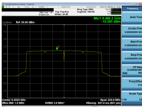
Plot 7-108 PSD SDM Primary Antenna WF5T (160 MHz BW 802.11be(SU) - Ch.111)
