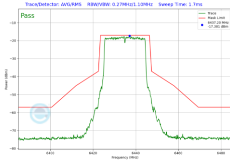
Plot 7-217 In-Band Emission Plot SDM Primary Antenna WF5T (20 MHz BW 802.11be(SU) (UNII Band 6) - Ch.97)
