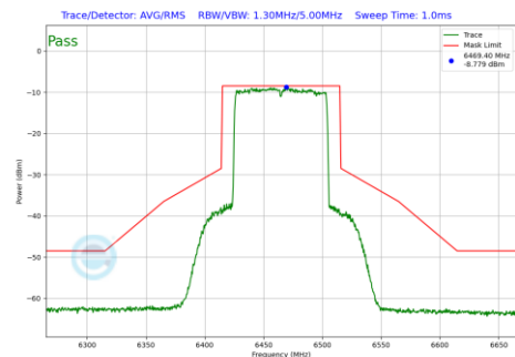
Plot 7-167 In-Band Emission Plot Antenna WF5T (80 MHz BW 802.11be(SU) (UNII Band 6) - Ch.103)
