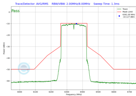
Plot 7-244 In-Band Emission Plot SDM Diversity Antenna WF5T (160 MHz BW 802.11be(SU) (UNII Band 5) - Ch.79)
