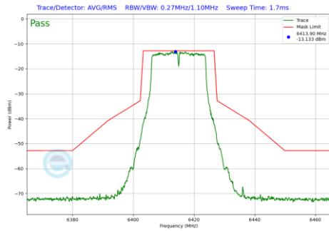
Plot 7-177 In-Band Emission Plot Antenna WF5B (20 MHz BW 802.11a (UNII Band 5) - Ch.93)
