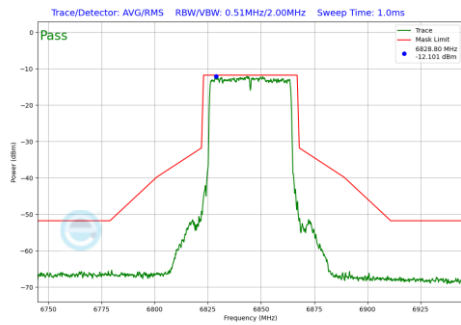
Plot 7-202 In-Band Emission Plot Antenna WF8 (40 MHz BW 802.11be(SU) (UNII Band 7) - Ch.179)
