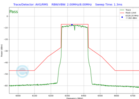
Plot 7-164 In-Band Emission Plot Antenna WF5T (160 MHz BW 802.11be(SU) (UNII Band 5) - Ch.79)
