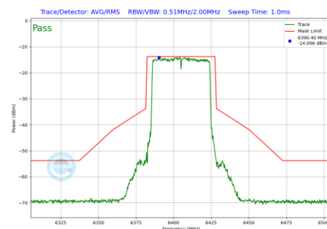
Plot 7-214 In-Band Emission Plot SDM Primary Antenna WF5B (40 MHz BW 802.11be(SU) (UNII Band 5) - Ch.91)
