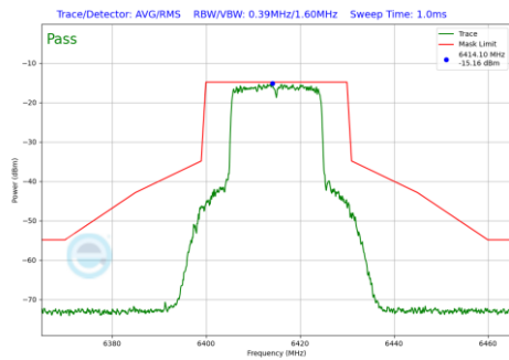
Plot 7-241 In-Band Emission Plot SDM Diversity Antenna WF5T (20 MHz BW 802.11be(SU) (UNII Band 5) - Ch.93)
