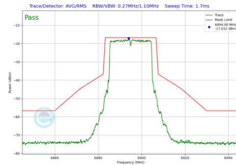
Plot 7-237 In-Band Emission Plot SDM Primary Antenna WF5B (20 MHz BW 802.11be(SU) (UNII Band 8) - Ch.189)
