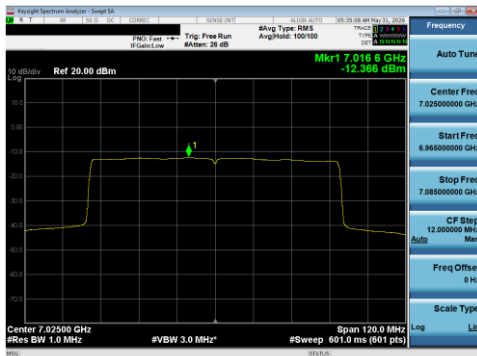
Plot 7-155 PSD SDM Diversity Antenna WF5T (80 MHz BW 802.11be(SU) - Ch.215)
