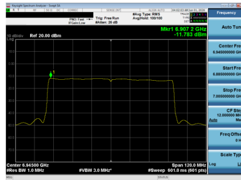
Plot 7-127 PSD SDM Primary Antenna WF5B (80 MHz BW 802.11be(SU) - Ch.199)
