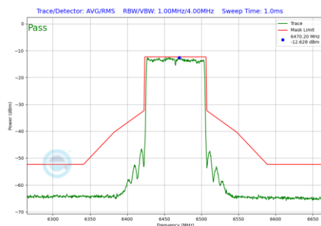
Plot 7-251 In-Band Emission Plot SDM Diversity Antenna WF5T (80 MHz BW 802.11be(SU) (UNII Band 6) - Ch.103)
