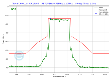
Plot 7-234 In-Band Emission Plot SDM Primary Antenna WF5T (40 MHz BW 802.11be(SU) (UNII Band 8) - Ch.227)
