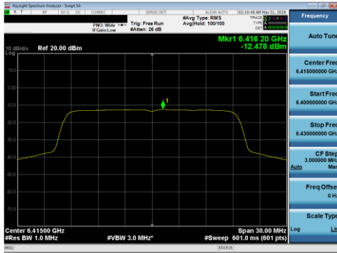
Plot 7-129 PSD SDM Diversity Antenna WF5T (20 MHz BW 802.11be(SU) - Ch.93)
